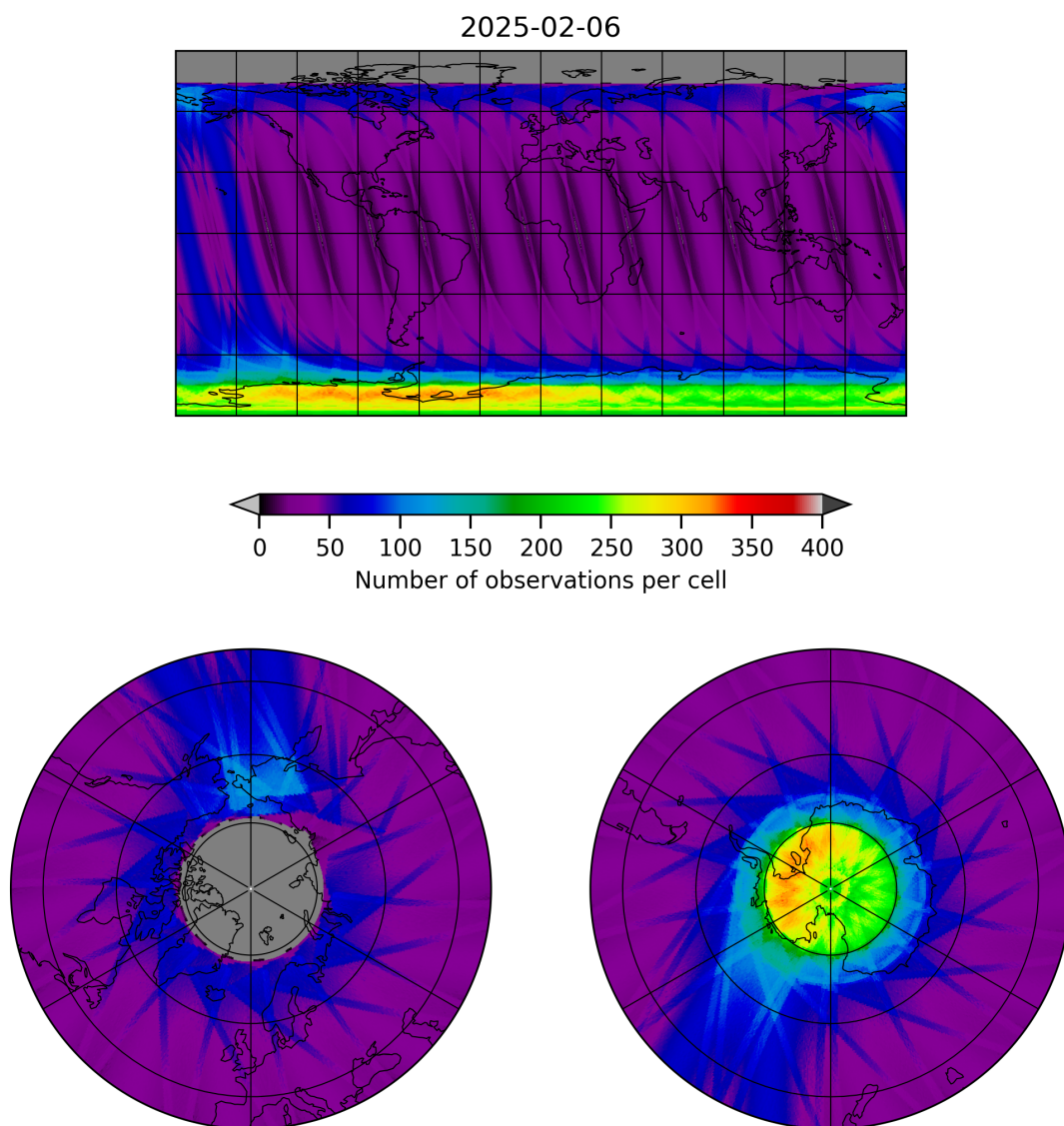
Figure 12: Map of the number of observations for 2025-02-05 to 2025-02-07
