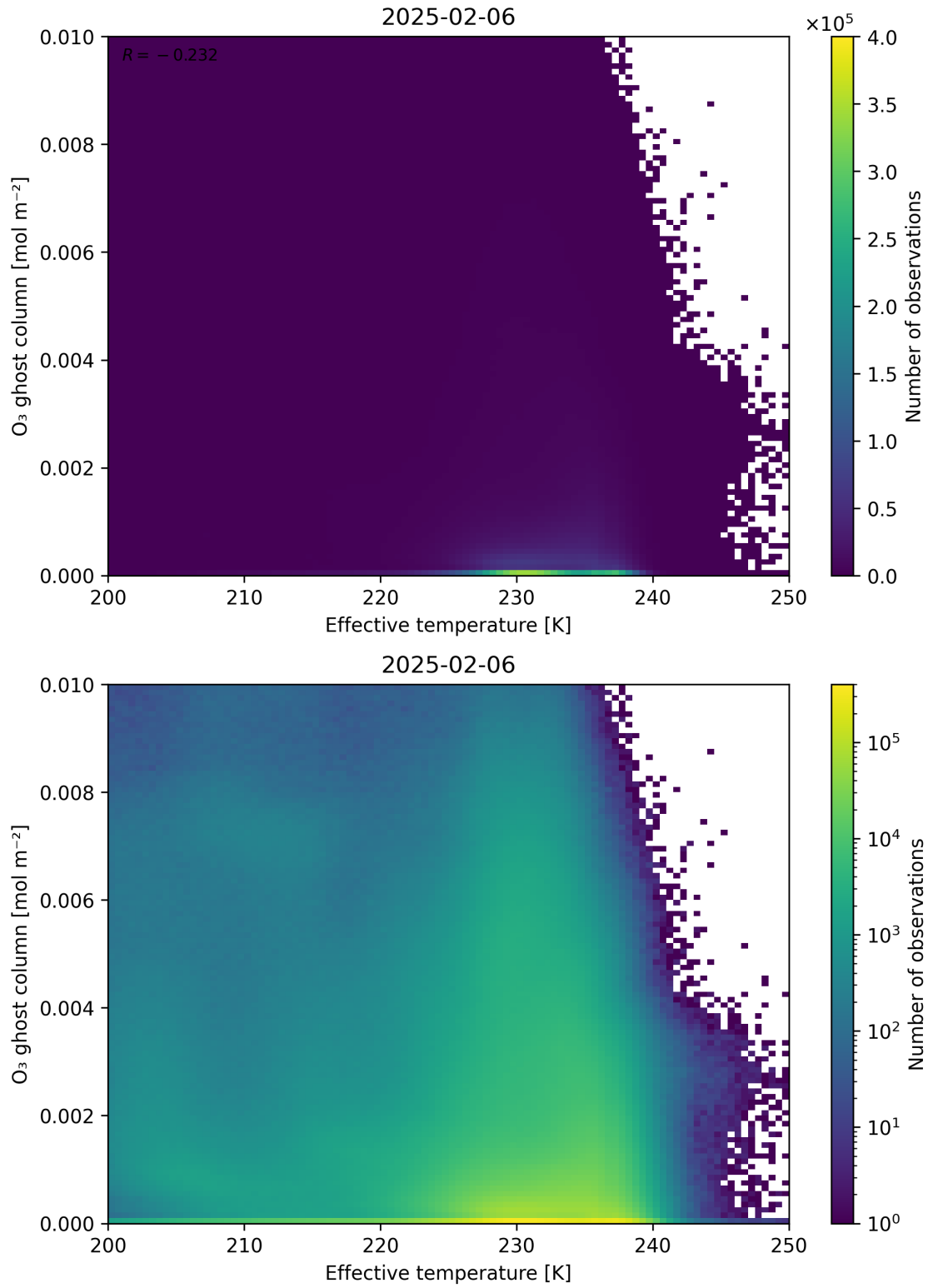
Figure 38: Scatter density plot of “Effective temperature” against “O 3 ghost column” for 2025-02-05 to 2025-02-07.
