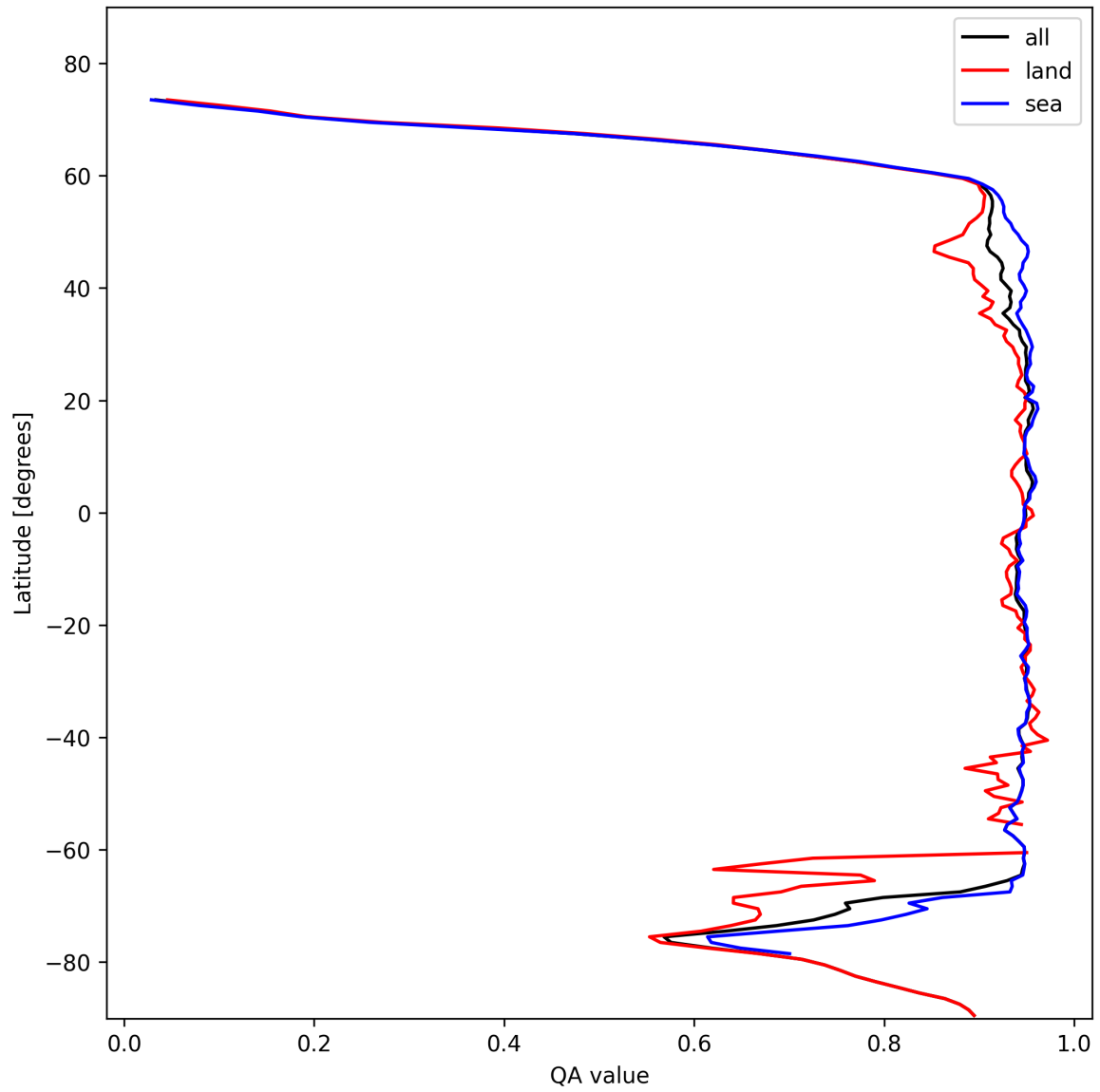
Figure 13: Zonal average of “QA value” for 2025-02-05 to 2025-02-07.
