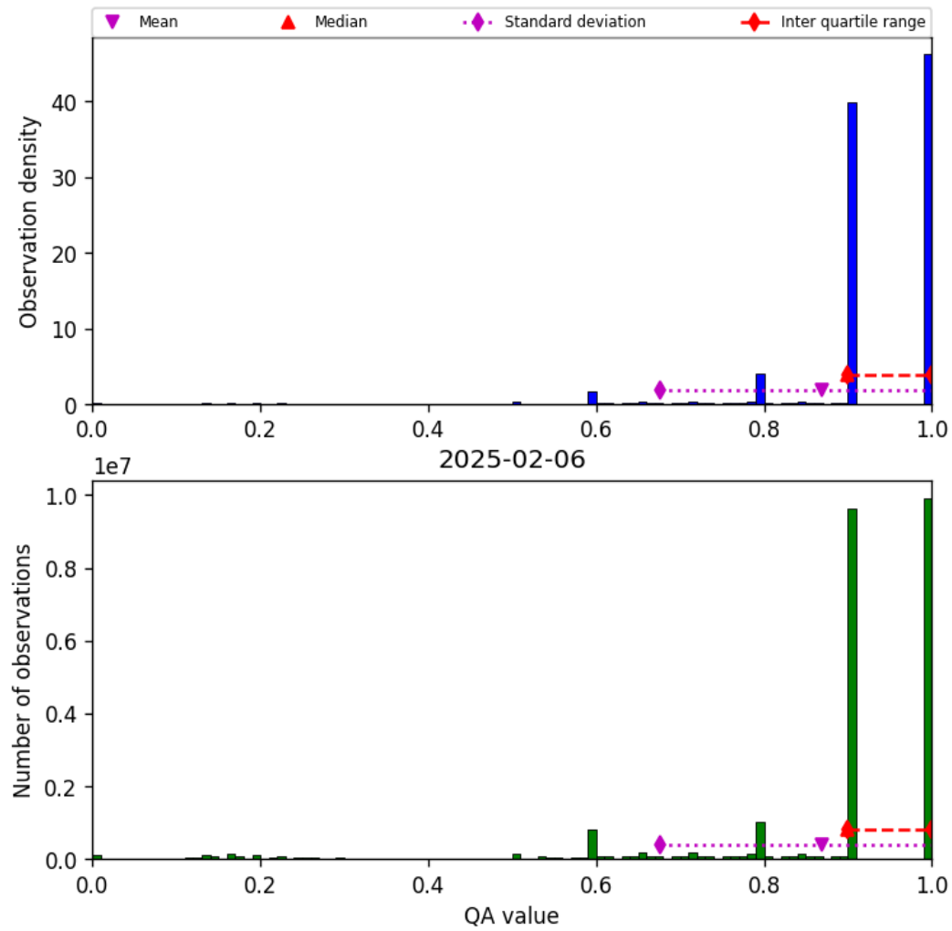
Figure 20: Histogram of “QA value” for 2025-02-05 to 2025-02-07
