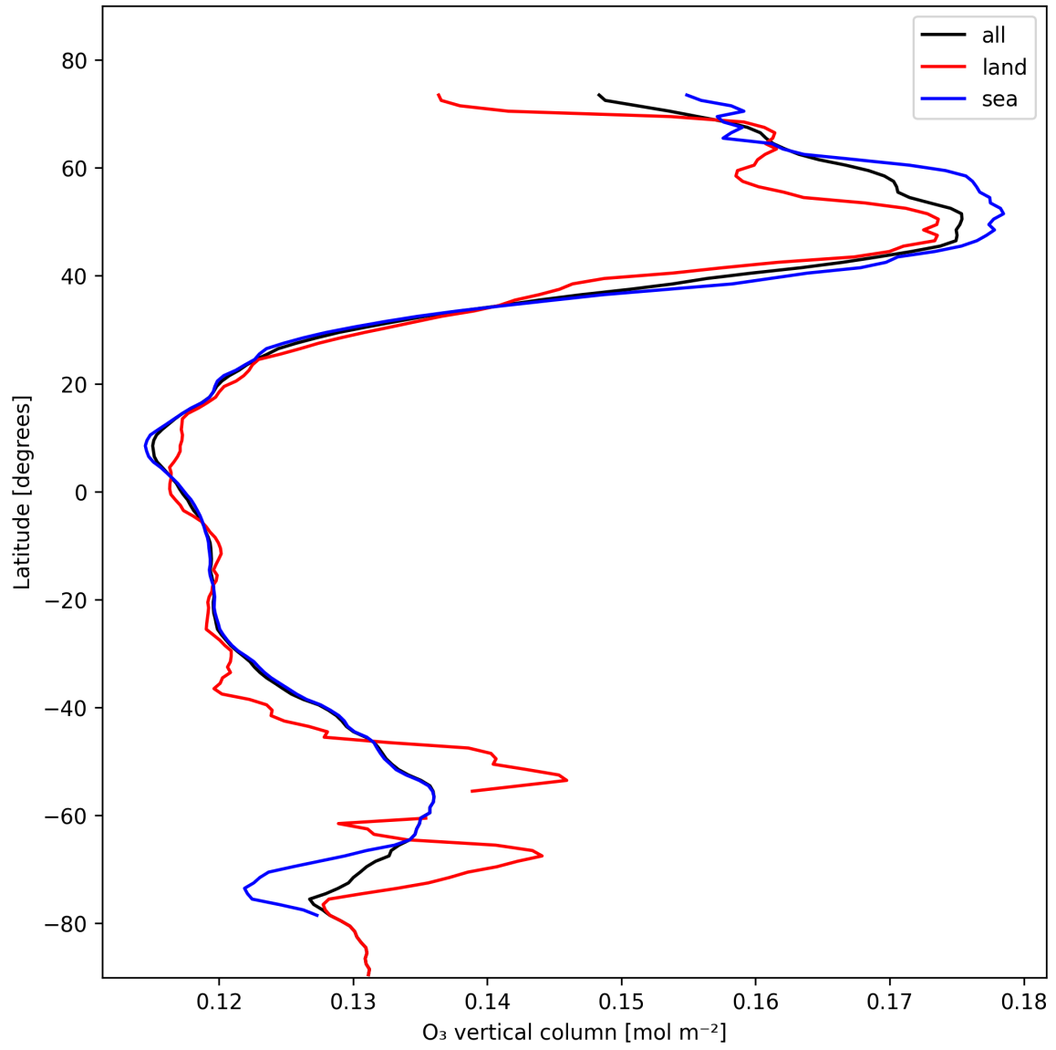
Figure 14: Zonal average of “O 3 vertical column” for 2025-02-05 to 2025-02-07.
