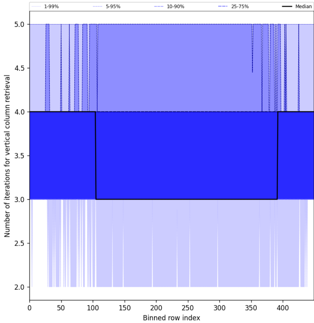
Figure 33: Along track statistics of “Number of iterations for vertical column retrieval” for 2025-02-05 to 2025-02-07
