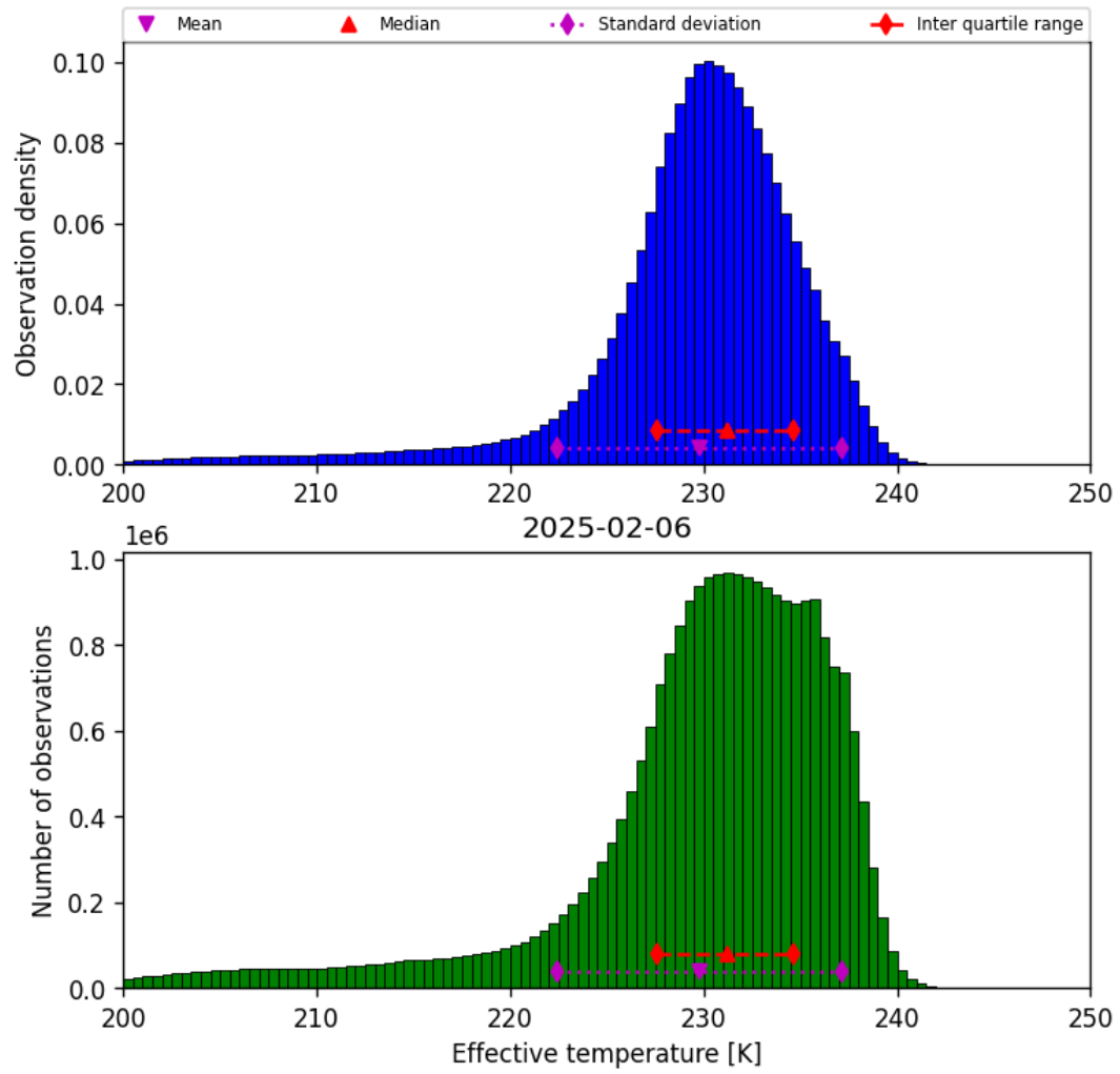
Figure 24: Histogram of “Effective temperature” for 2025-02-05 to 2025-02-07
