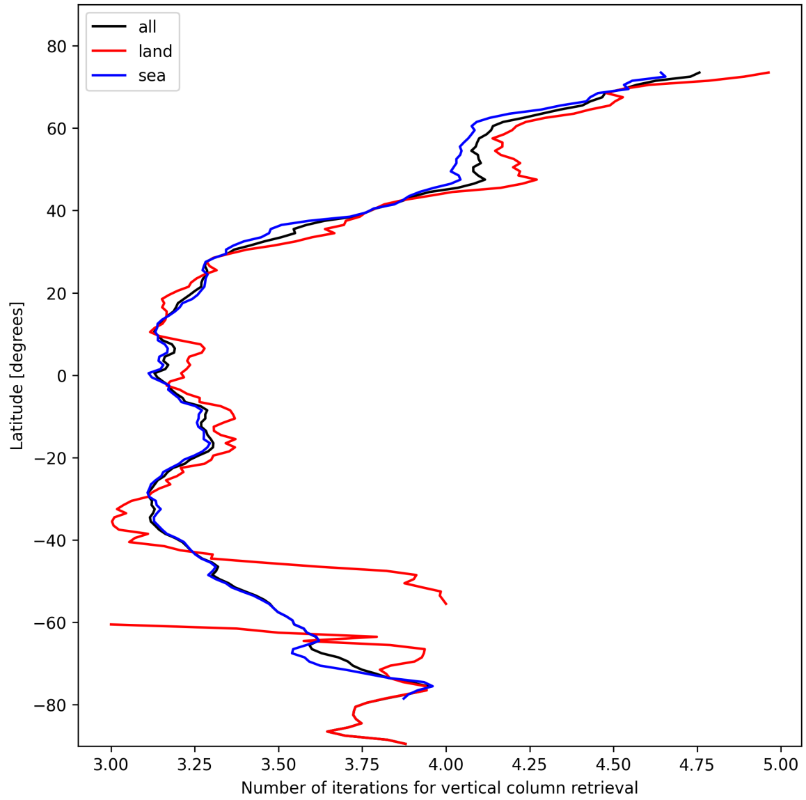
Figure 19: Zonal average of “Number of iterations for vertical column retrieval” for 2025-02-05 to 2025-02-07.
