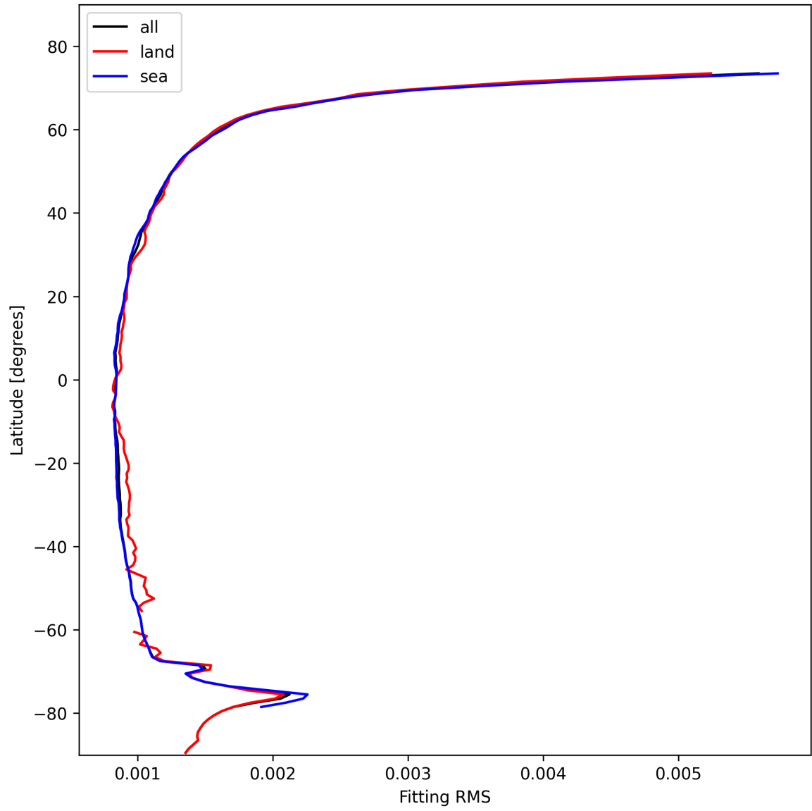
Figure 16: Zonal average of “Fitting RMS” for 2025-02-05 to 2025-02-07.
