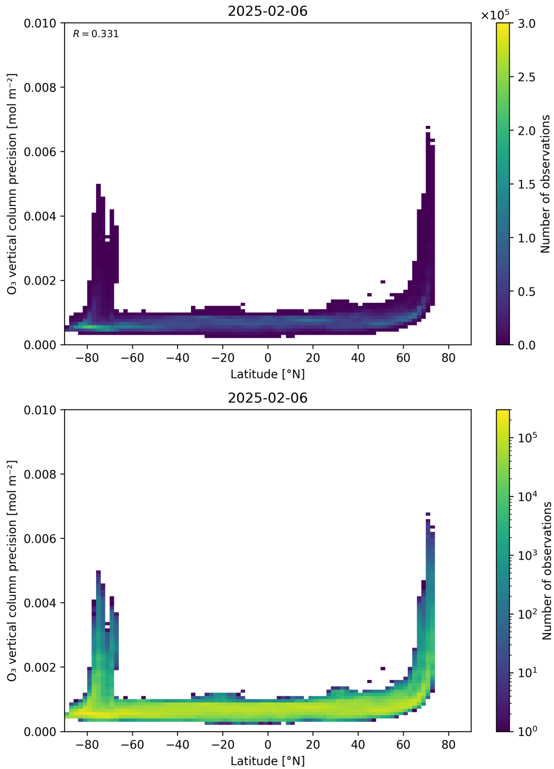
Figure 37: Scatter density plot of “Latitude” against “O 3 vertical column precision” for 2025-02-05 to 2025-02-07.
