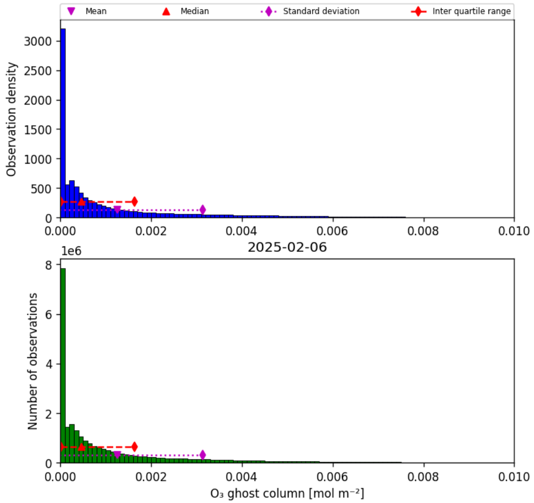
Figure 25: Histogram of “O 3 ghost column” for 2025-02-05 to 2025-02-07
