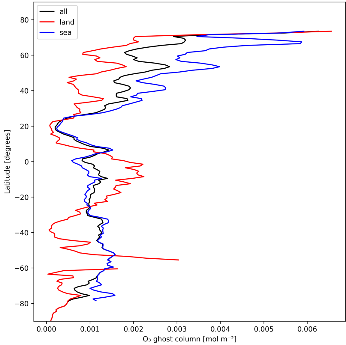
Figure 18: Zonal average of “O 3 ghost column” for 2025-02-05 to 2025-02-07.
