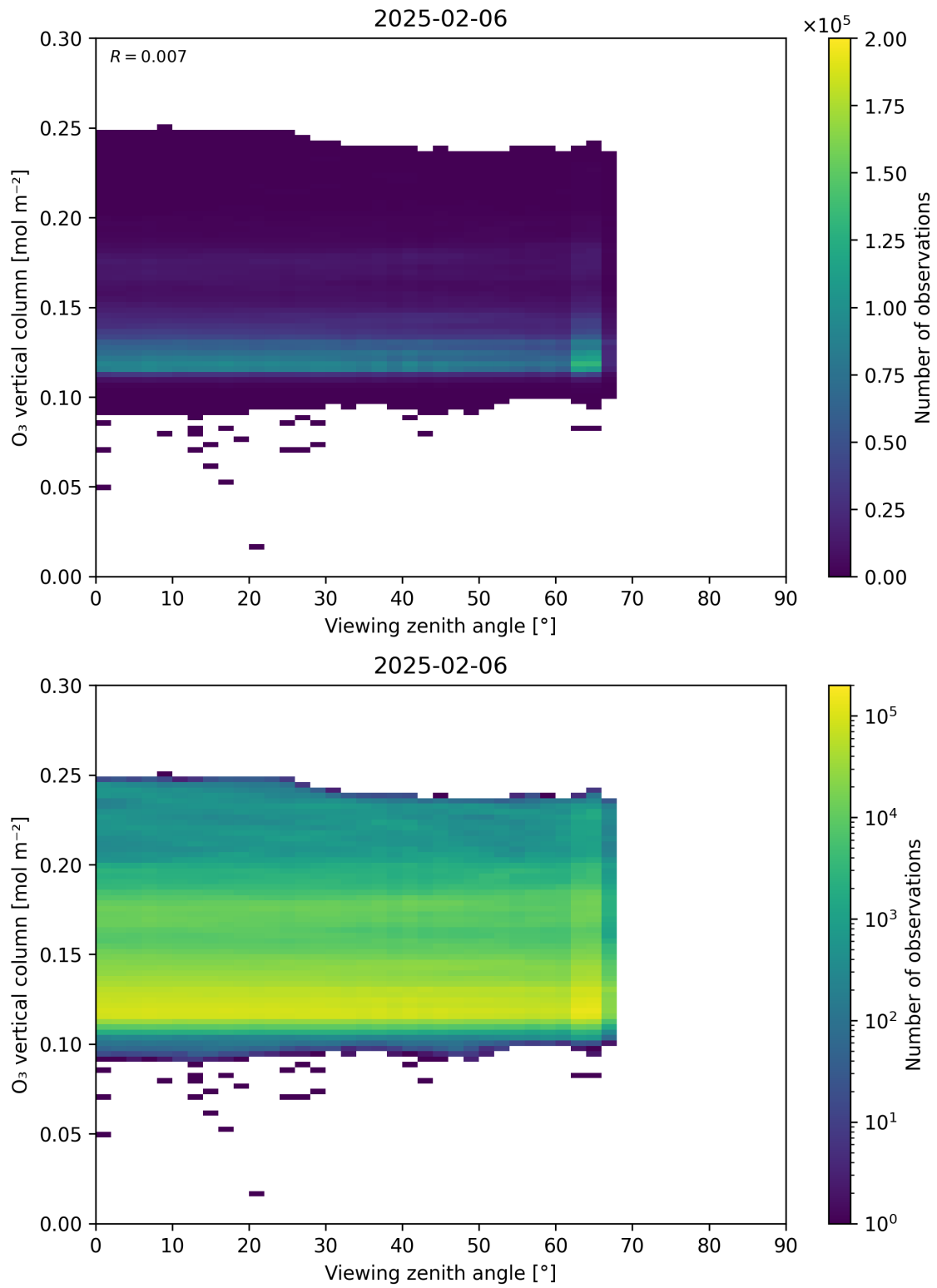
Figure 52: Scatter density plot of “Viewing zenith angle” against “O 3 vertical column” for 2025-02-05 to 2025-02-07.
