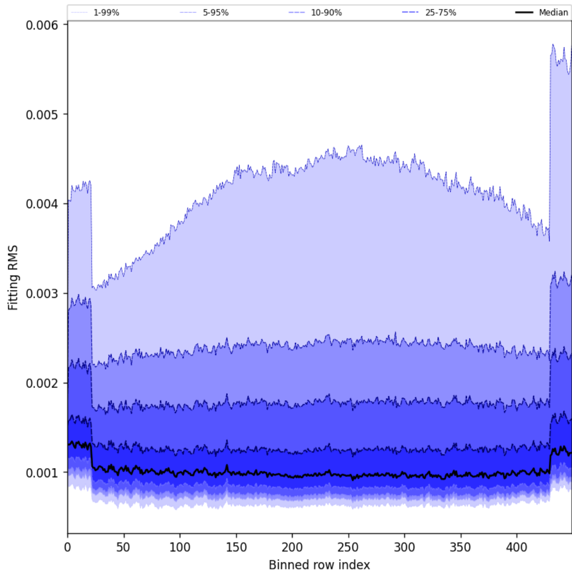
Figure 30: Along track statistics of “Fitting RMS” for 2025-02-05 to 2025-02-07
