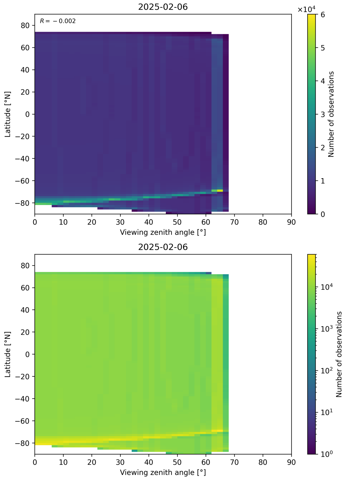
Figure 49: Scatter density plot of “Viewing zenith angle” against “Latitude” for 2025-02-05 to 2025-02-07.
