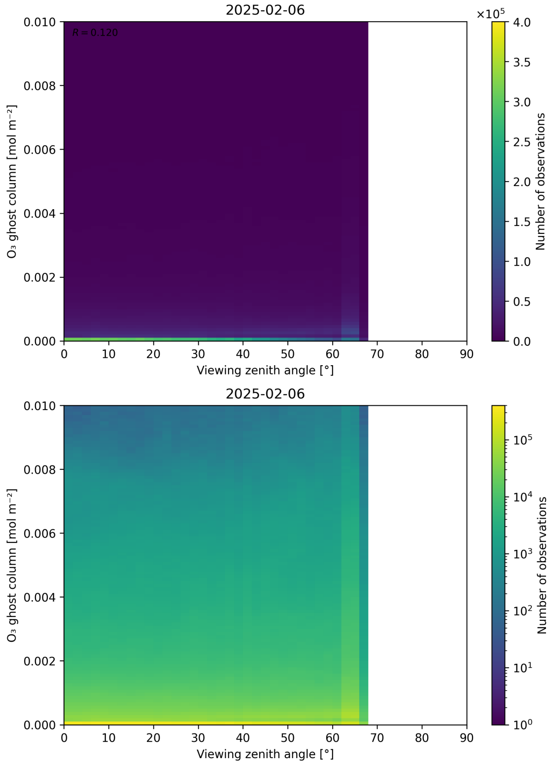
Figure 51: Scatter density plot of “Viewing zenith angle” against “O 3 ghost column” for 2025-02-05 to 2025-02-07.
