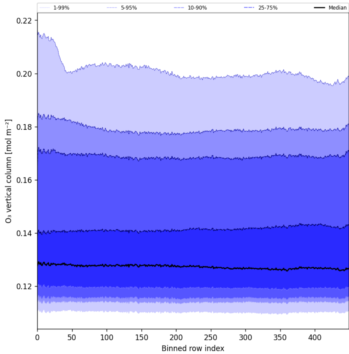
Figure 28: Along track statistics of “O 3 vertical column” for 2025-02-05 to 2025-02-07
