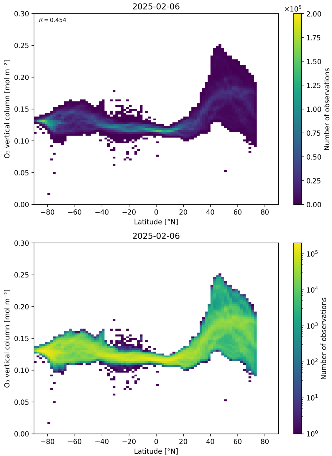
Figure 36: Scatter density plot of “Latitude” against “O 3 vertical column” for 2025-02-05 to 2025-02-07.
