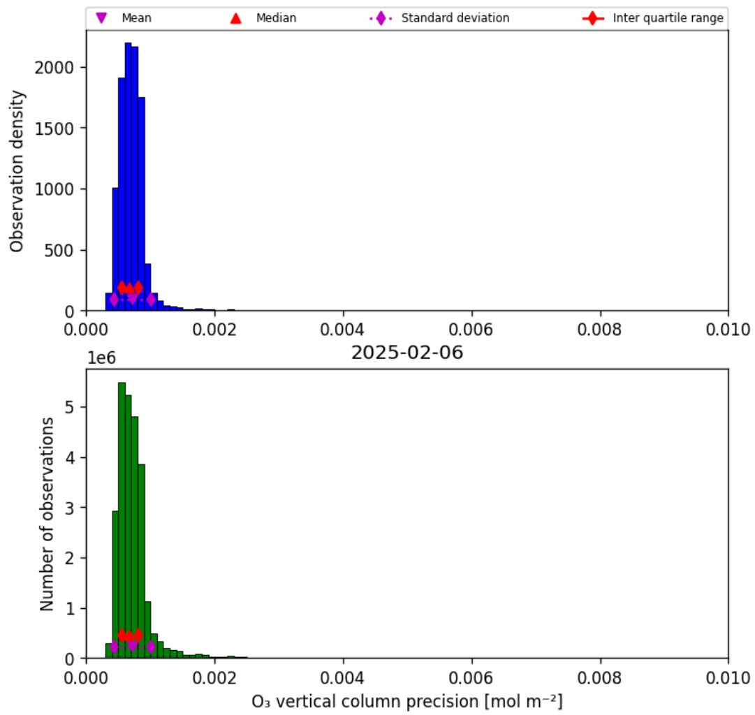
Figure 22: Histogram of “O 3 vertical column precision” for 2025-02-05 to 2025-02-07
