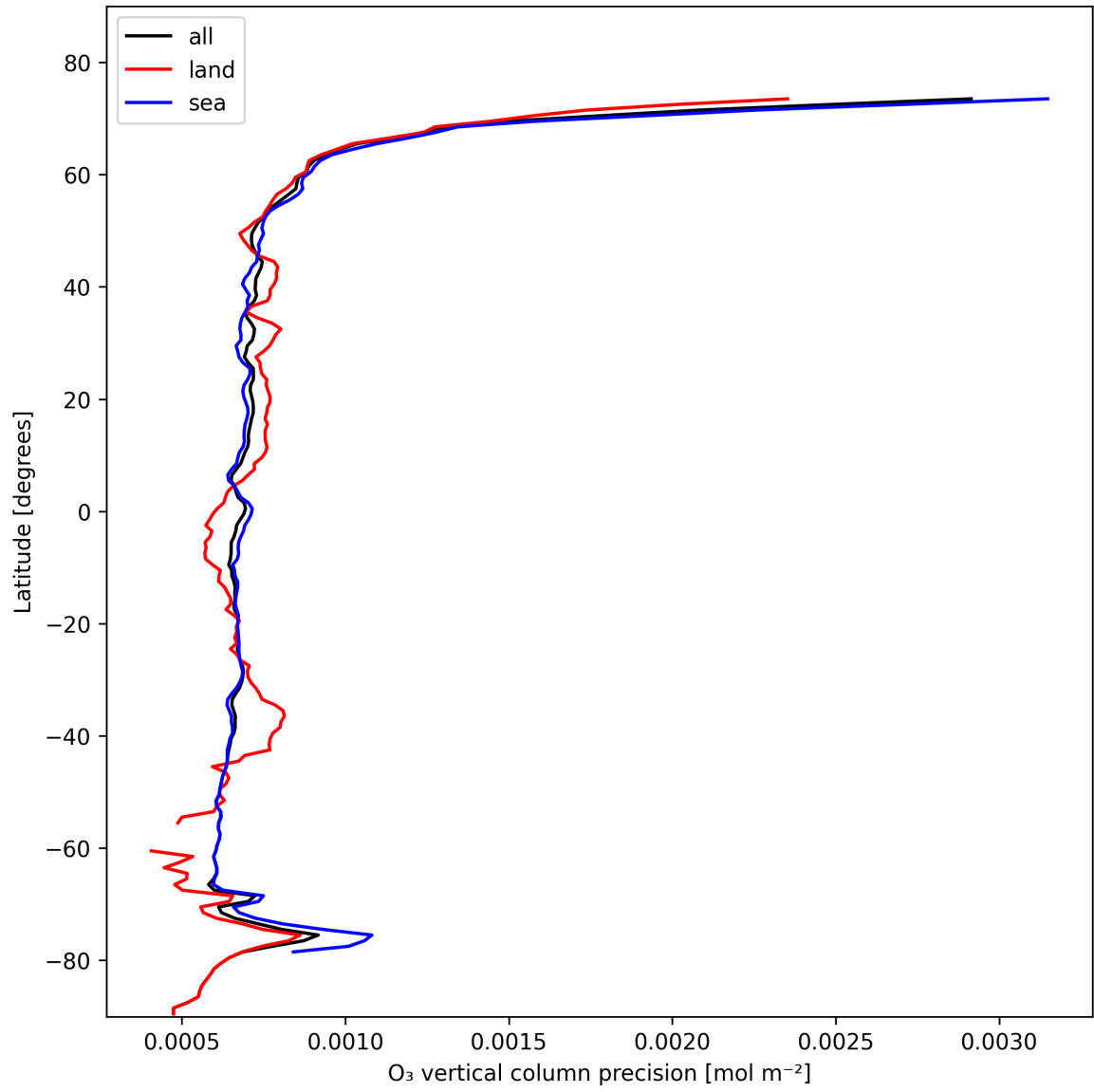
Figure 15: Zonal average of “O 3 vertical column precision” for 2025-02-05 to 2025-02-07.
