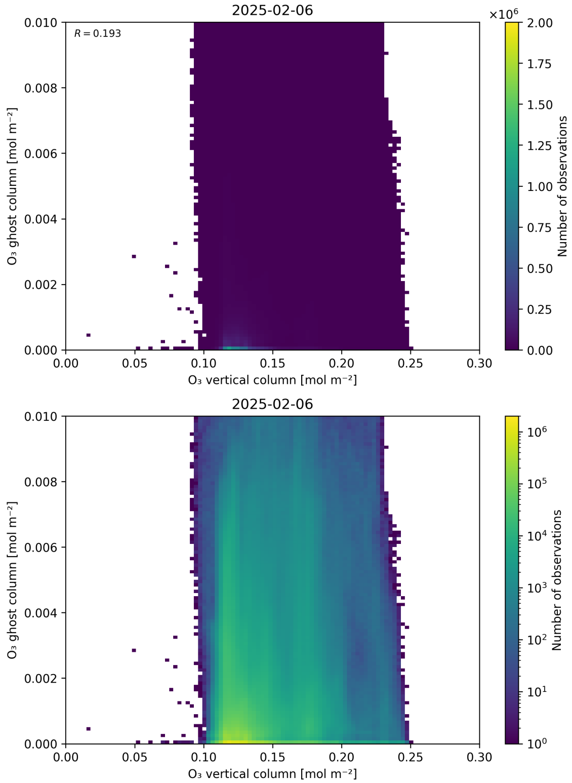
Figure 40: Scatter density plot of “O 3 vertical column” against “O 3 ghost column” for 2025-02-05 to 2025-02-07.
