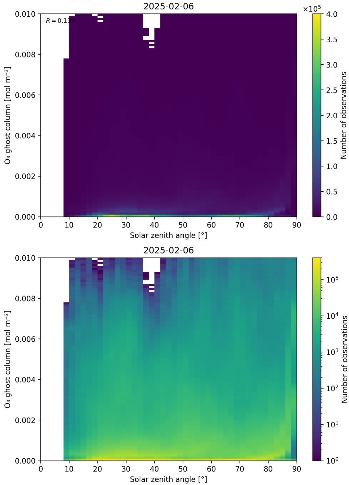
Figure 46: Scatter density plot of “Solar zenith angle” against “O 3 ghost column” for 2025-02-05 to 2025-02-07.
