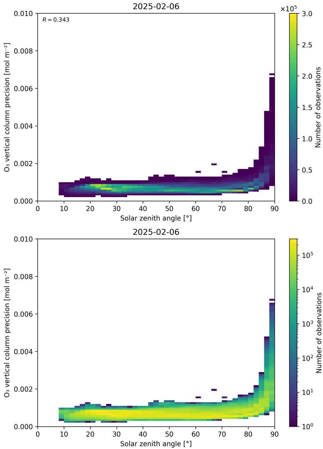
Figure 48: Scatter density plot of “Solar zenith angle” against “O 3 vertical column precision” for 2025-02-05 to 2025-02-07.
