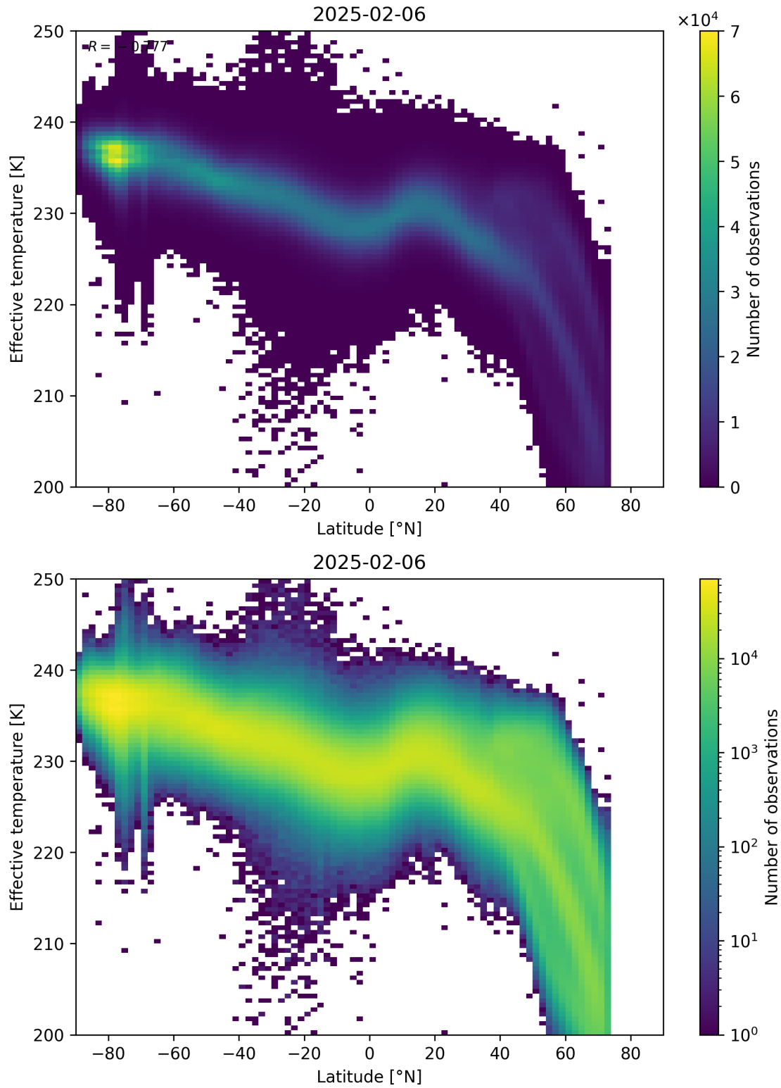
Figure 34: Scatter density plot of “Latitude” against “Effective temperature” for 2025-02-05 to 2025-02-07.
