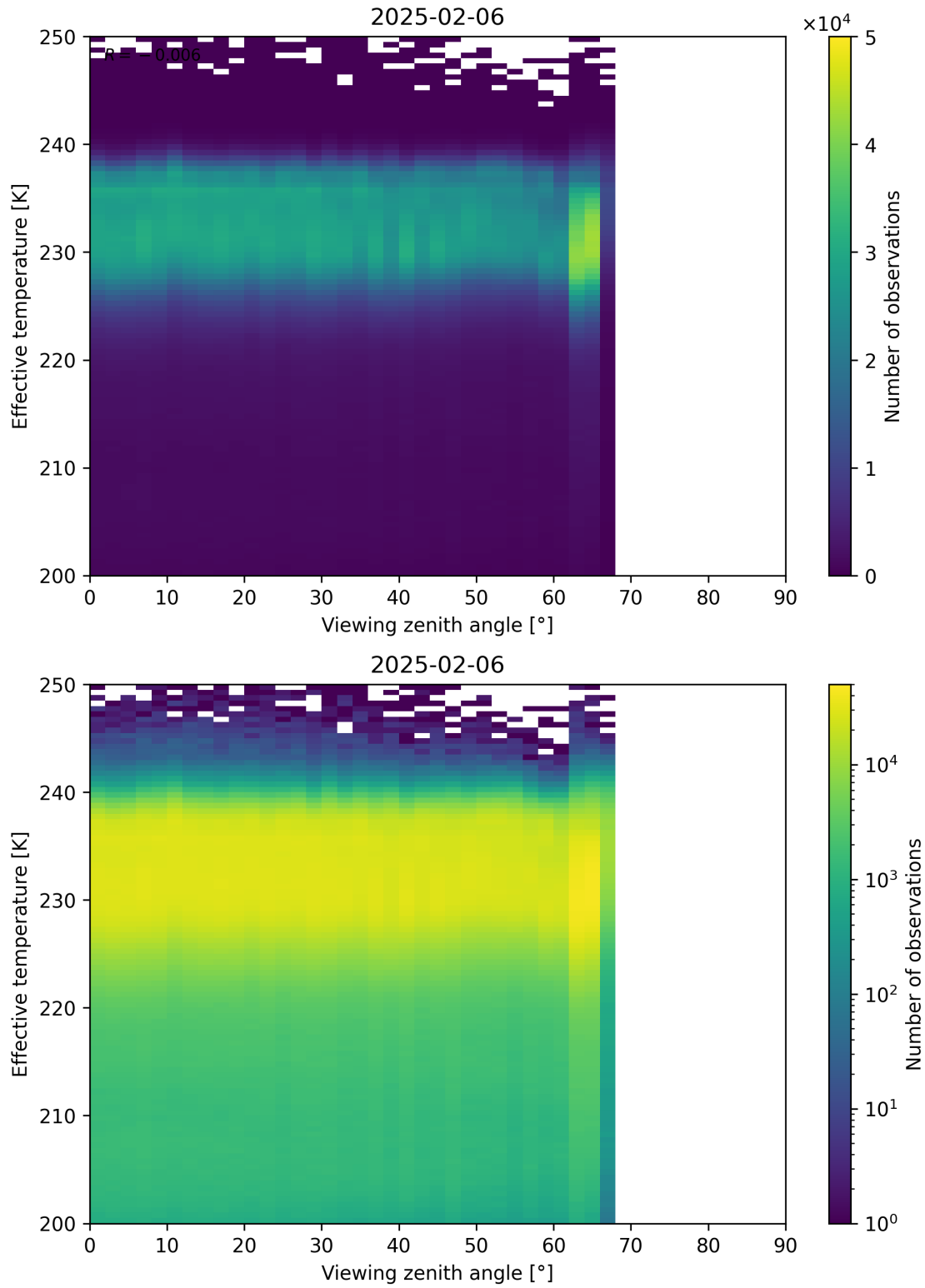
Figure 50: Scatter density plot of “Viewing zenith angle” against “Effective temperature” for 2025-02-05 to 2025-02-07.
