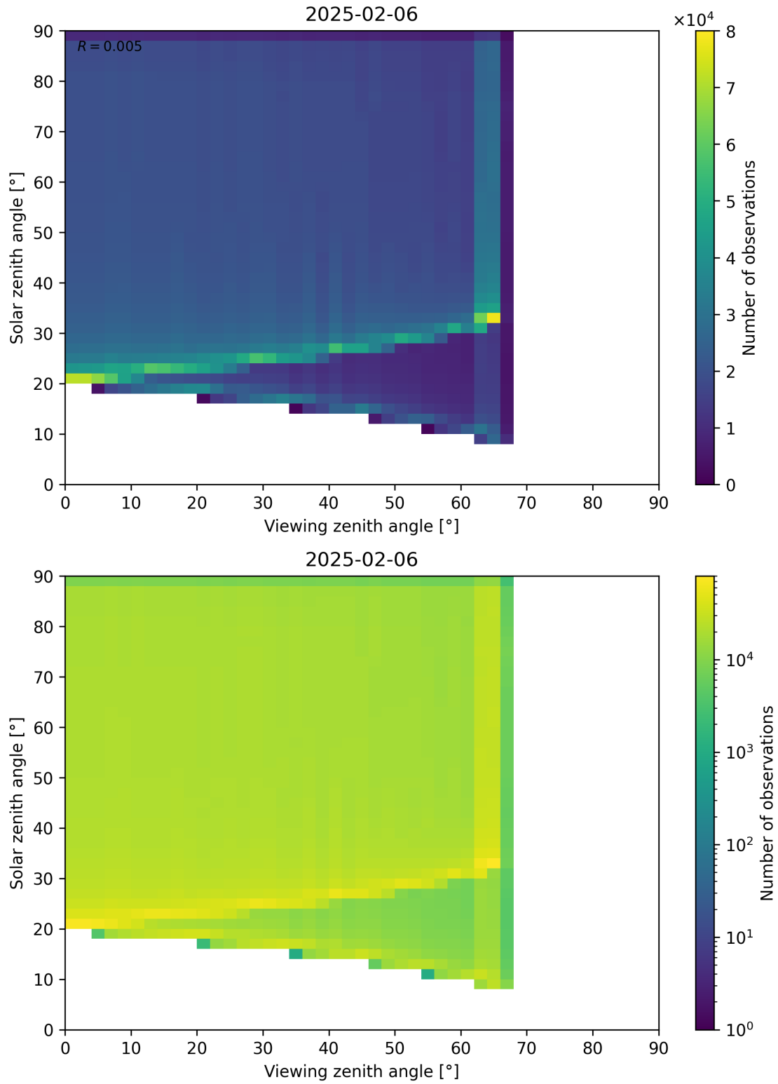
Figure 54: Scatter density plot of “Viewing zenith angle” against “Solar zenith angle” for 2025-02-05 to 2025-02-07.
