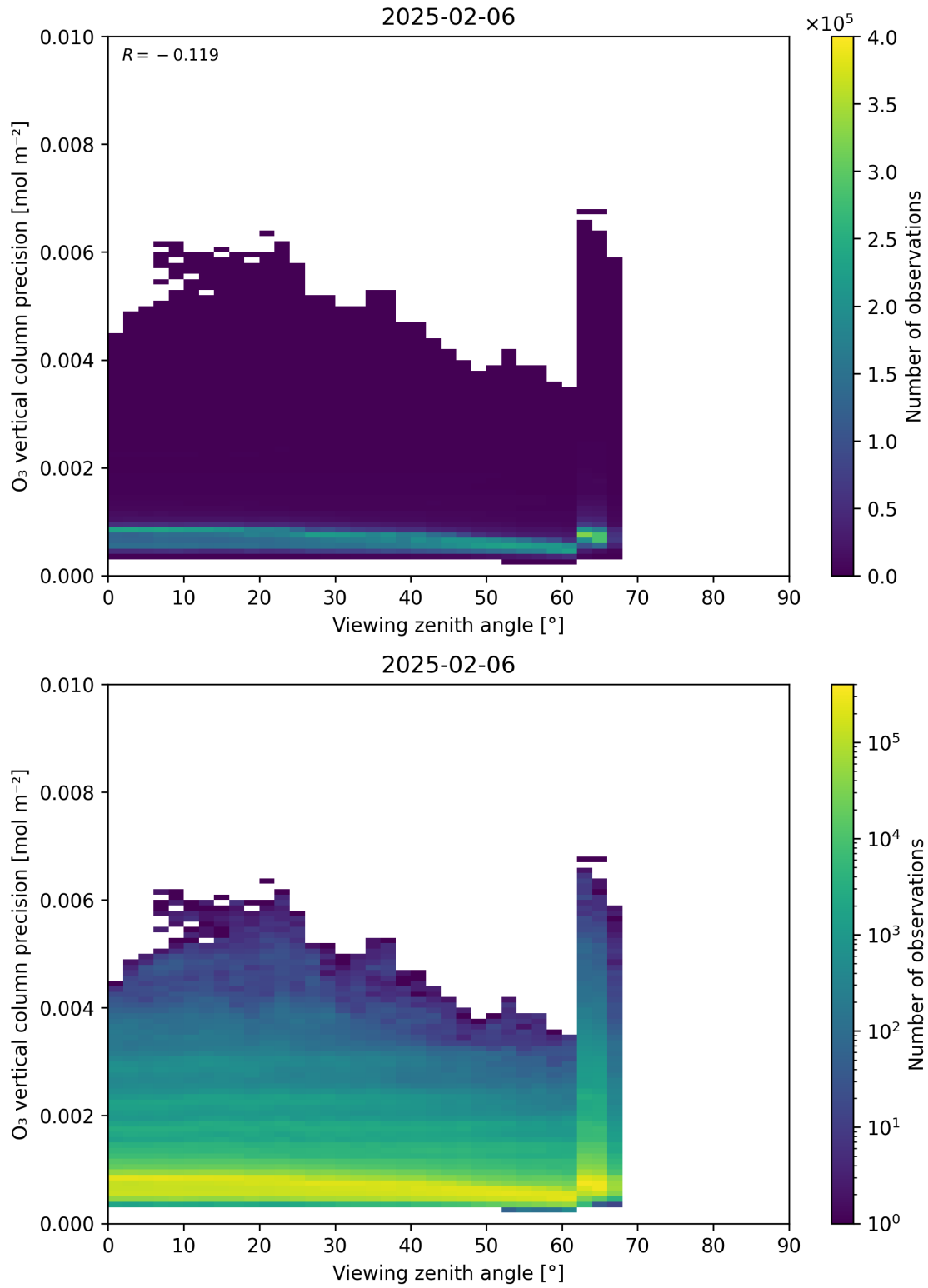
Figure 53: Scatter density plot of “Viewing zenith angle” against “O 3 vertical column precision” for 2025-02-05 to 2025-02-07.
