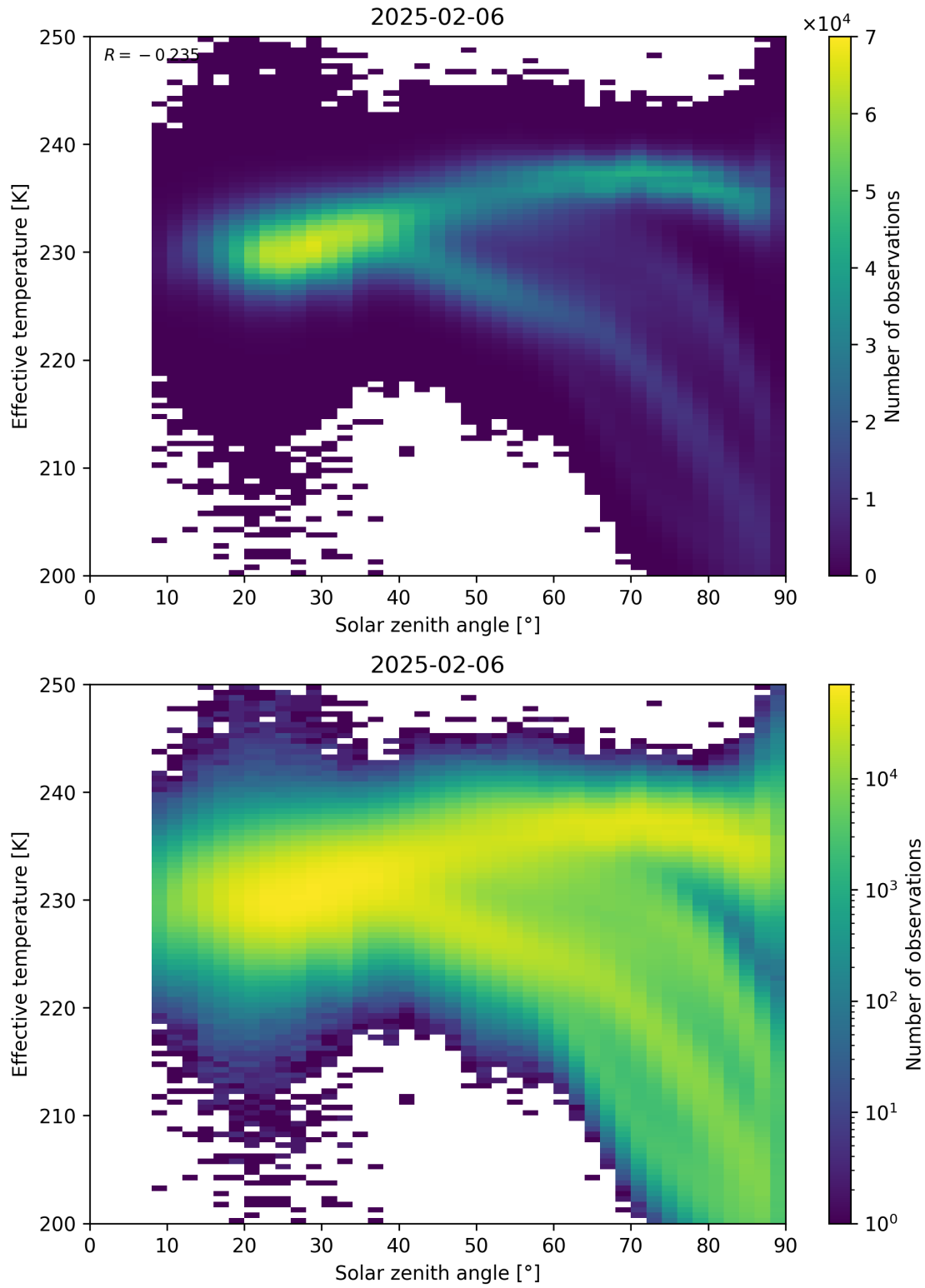
Figure 45: Scatter density plot of “Solar zenith angle” against “Effective temperature” for 2025-02-05 to 2025-02-07.
