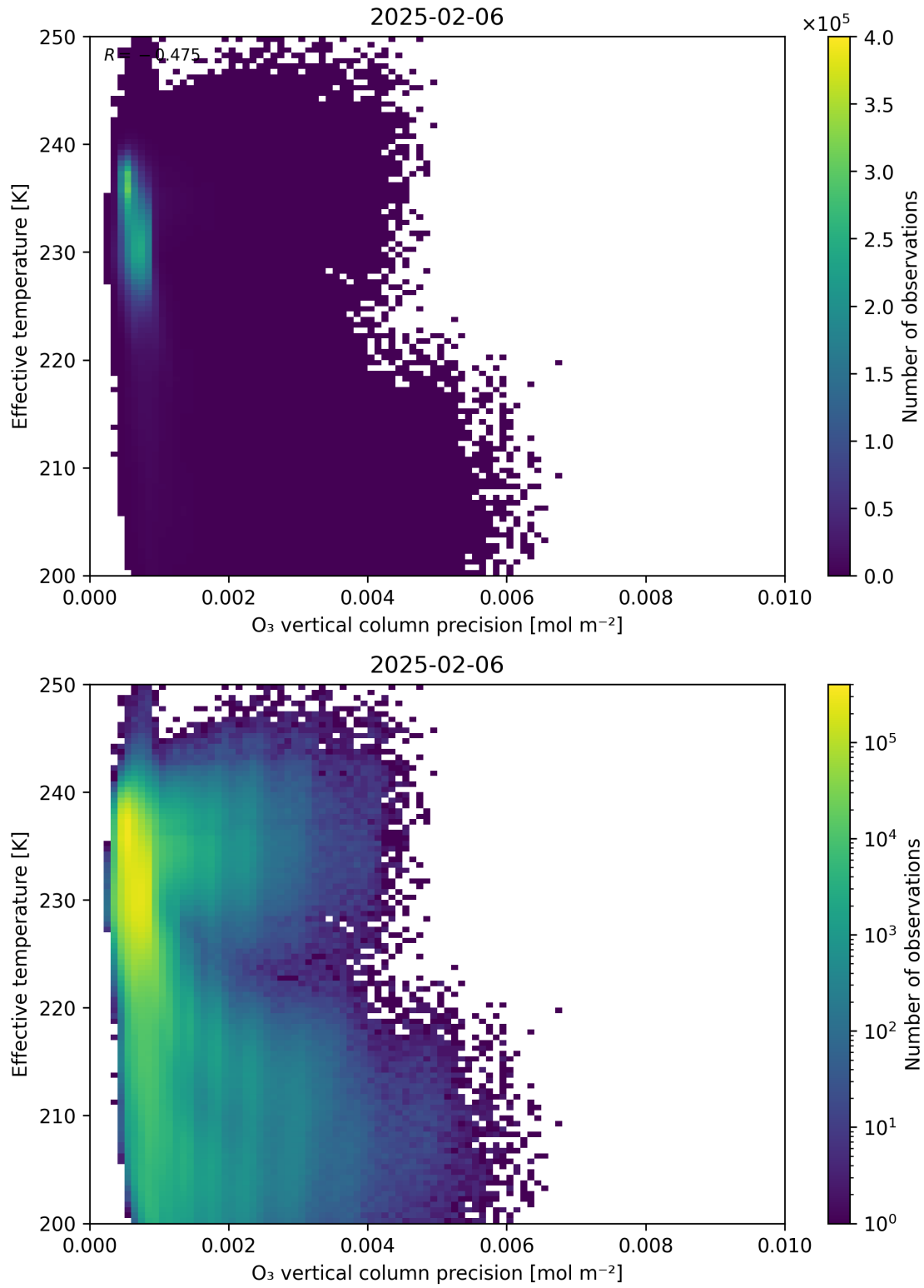
Figure 42: Scatter density plot of “O 3 vertical column precision” against “Effective temperature” for 2025-02-05 to 2025-02-07.
