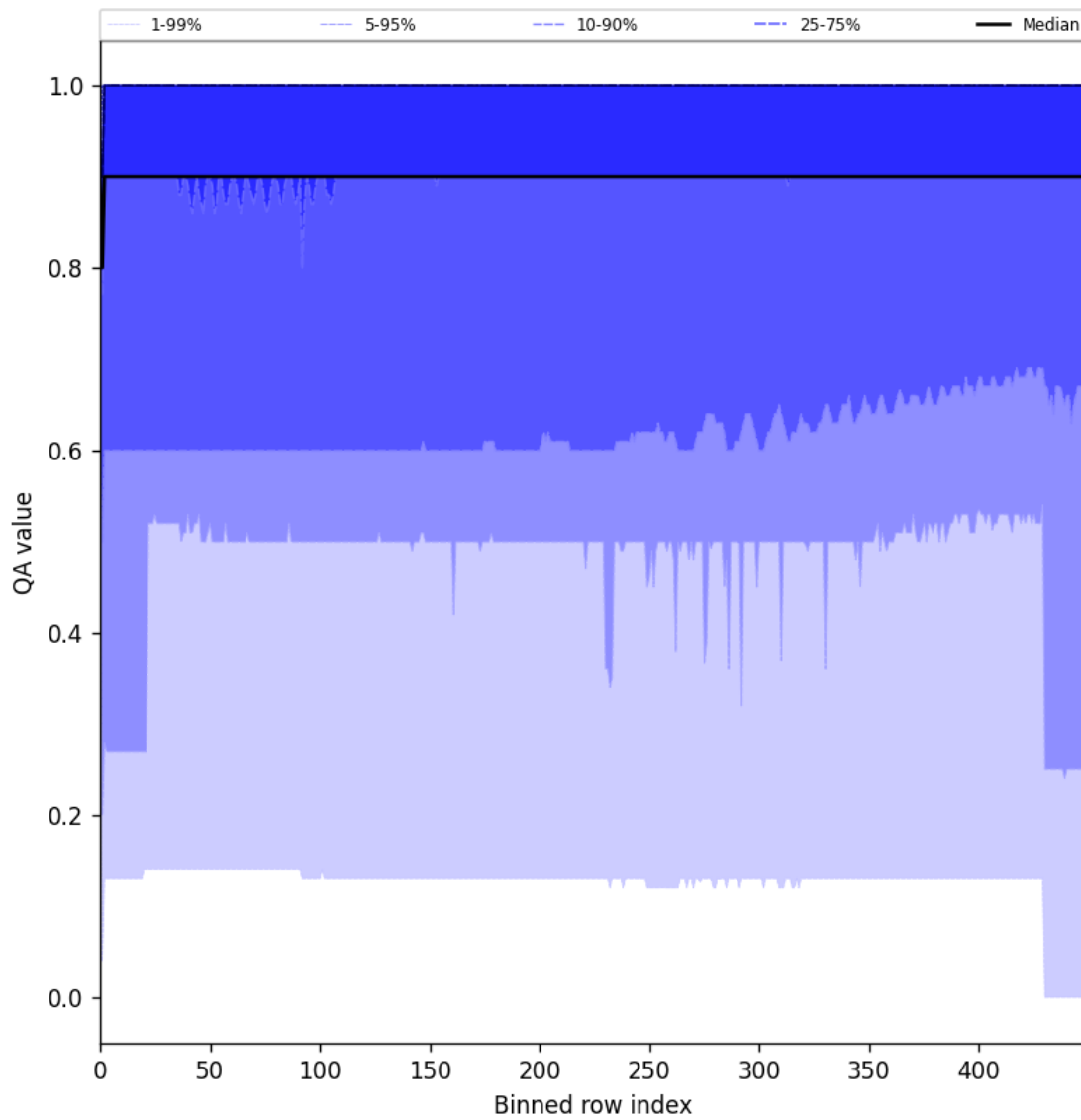
Figure 27: Along track statistics of “QA value” for 2025-02-05 to 2025-02-07
