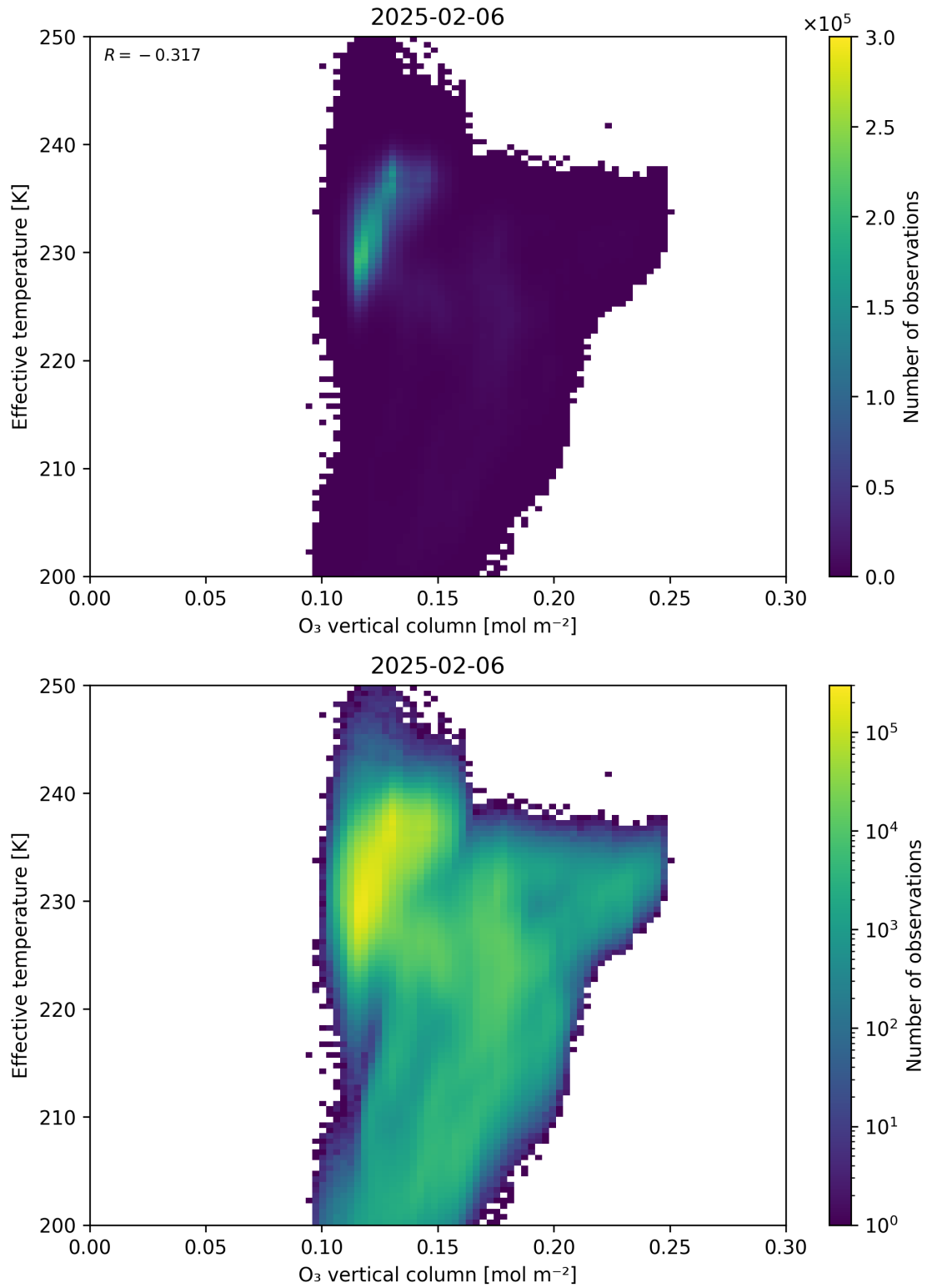
Figure 39: Scatter density plot of “O 3 vertical column” against “Effective temperature” for 2025-02-05 to 2025-02-07.
