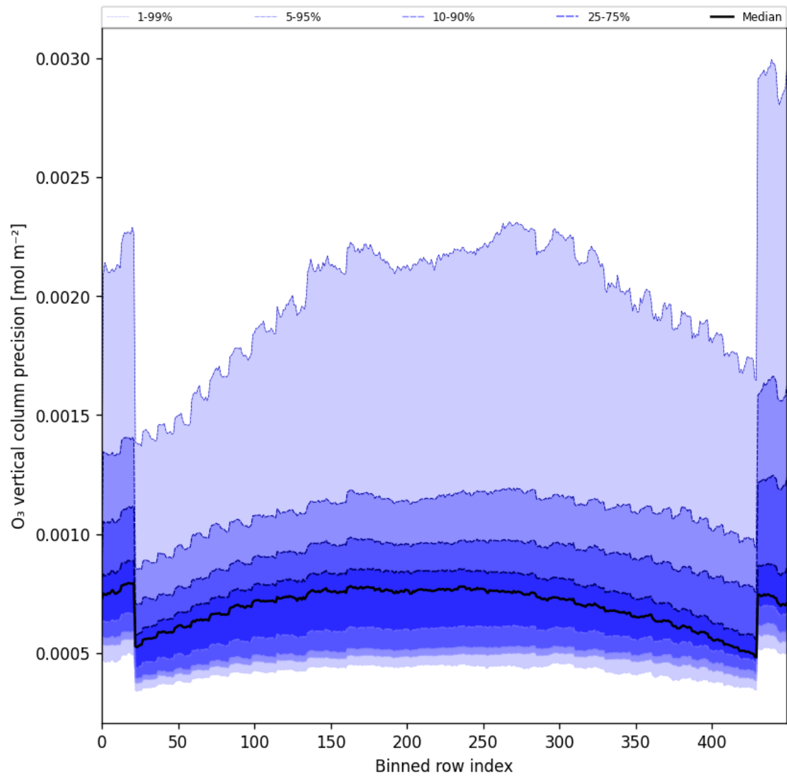
Figure 29: Along track statistics of “O 3 vertical column precision” for 2025-02-05 to 2025-02-07
