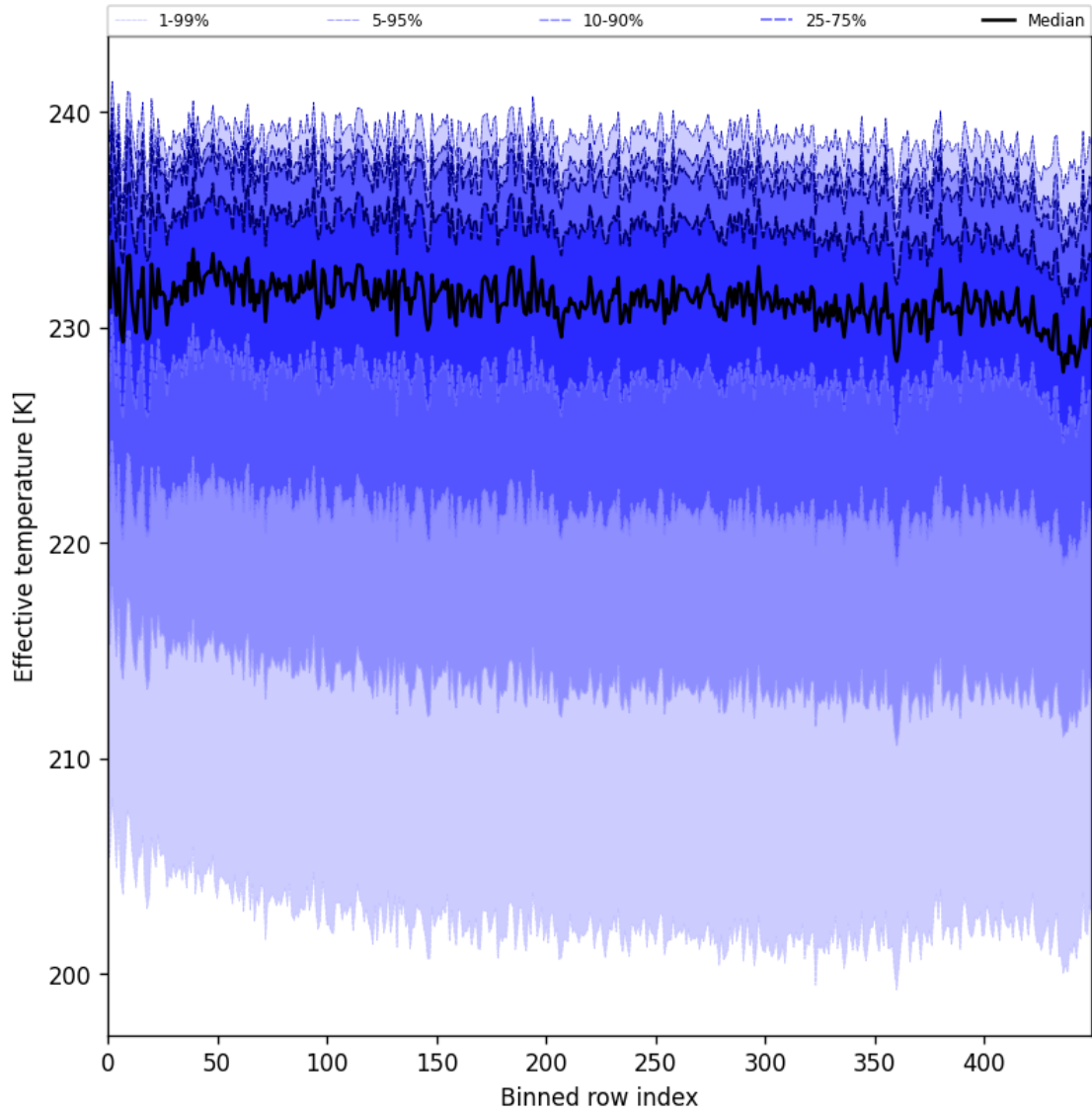
Figure 31: Along track statistics of “Effective temperature” for 2025-02-05 to 2025-02-07
