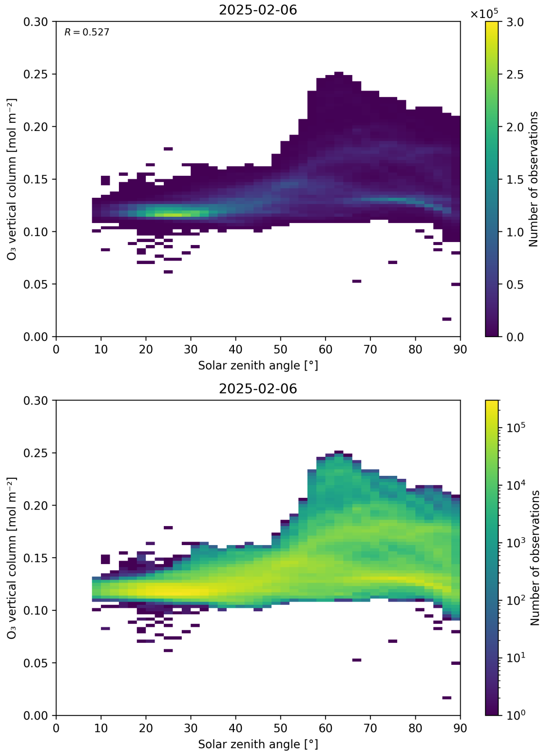
Figure 47: Scatter density plot of “Solar zenith angle” against “O 3 vertical column” for 2025-02-05 to 2025-02-07.
