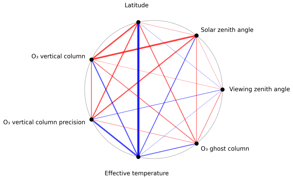
Figure 1: Map of correlation graph for 2025-02-05 to 2025-02-07.
