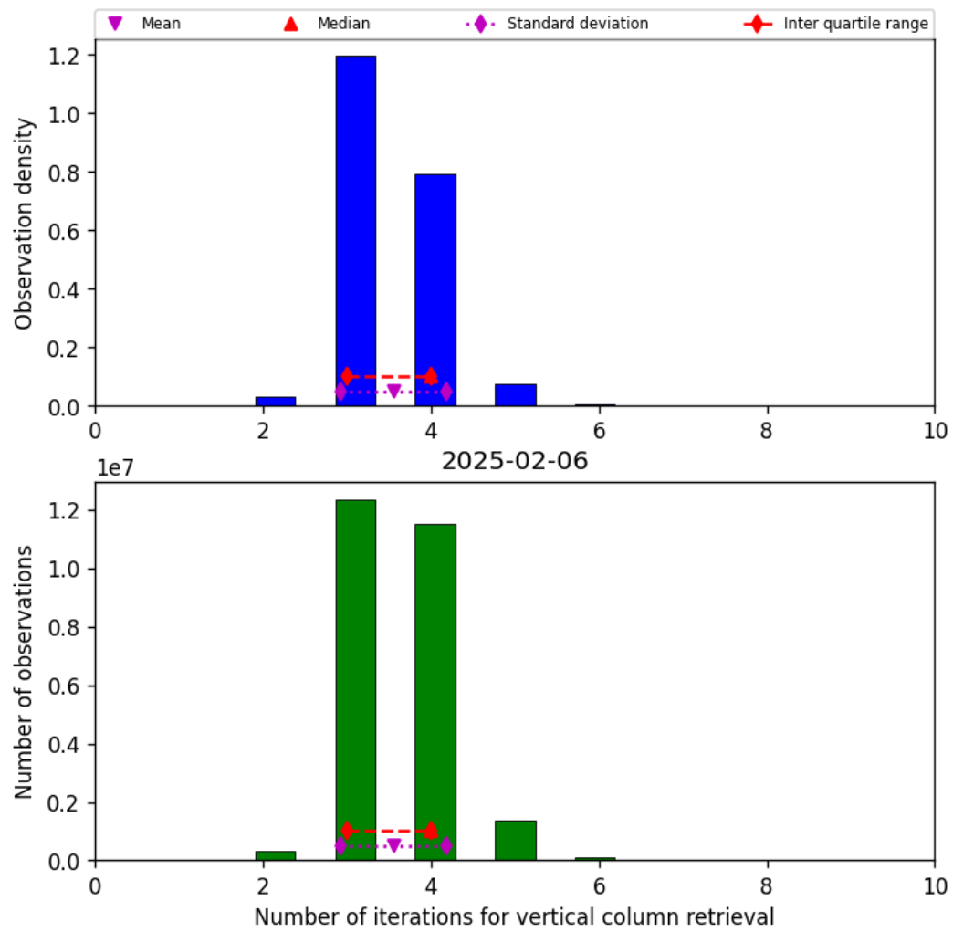
Figure 26: Histogram of “Number of iterations for vertical column retrieval” for 2025-02-05 to 2025-02-07
