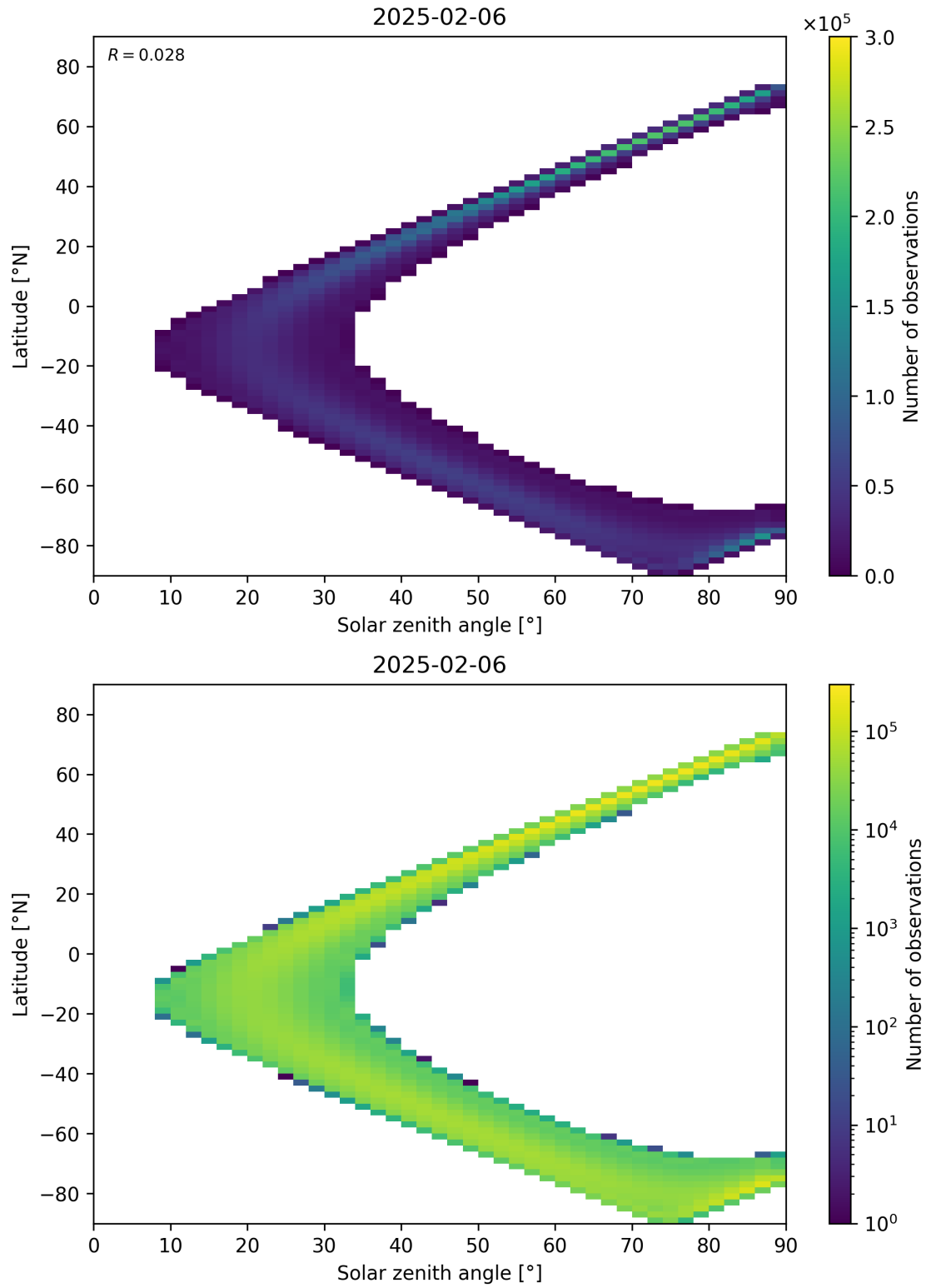
Figure 44: Scatter density plot of “Solar zenith angle” against “Latitude” for 2025-02-05 to 2025-02-07.
