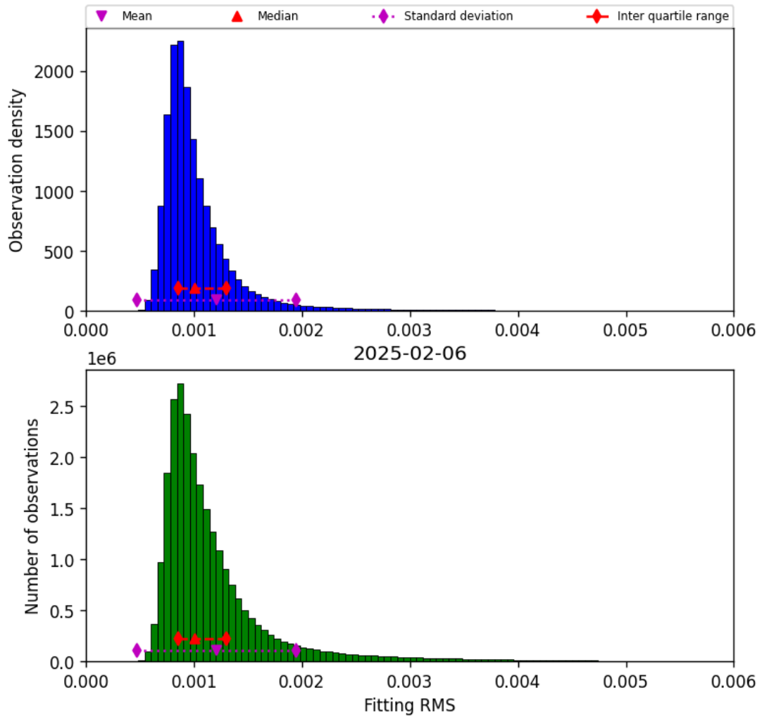
Figure 23: Histogram of “Fitting RMS” for 2025-02-05 to 2025-02-07
