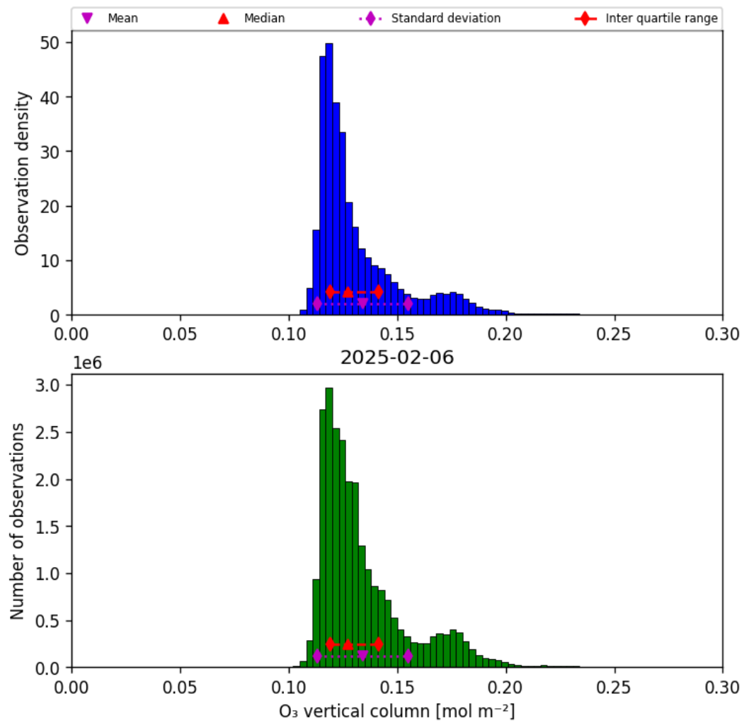
Figure 21: Histogram of “O 3 vertical column” for 2025-02-05 to 2025-02-07
