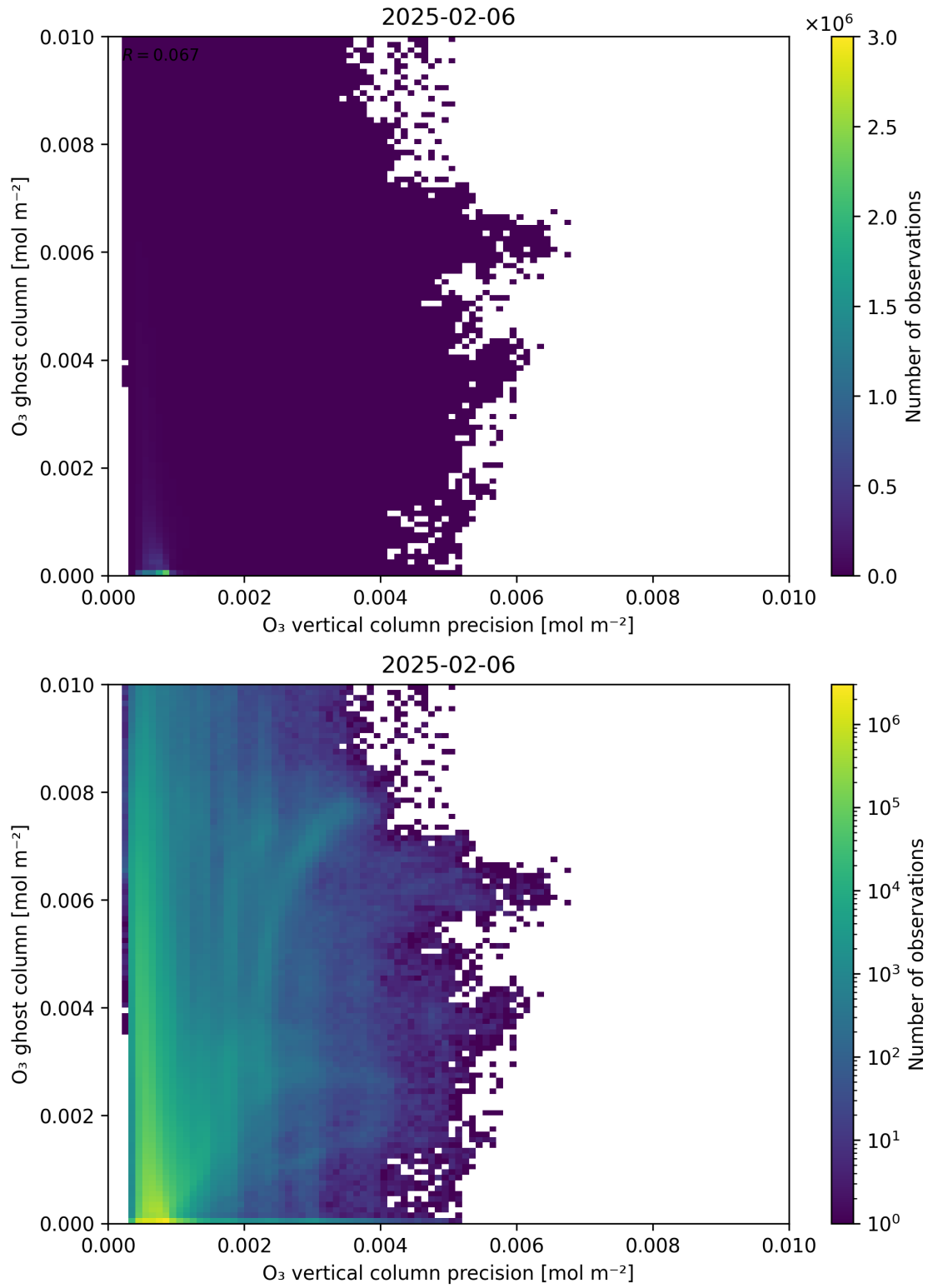
Figure 43: Scatter density plot of “ \text{O}_3 vertical column precision” against “ \text{O}_3 ghost column” for 2025-02-05 to 2025-02-07.
