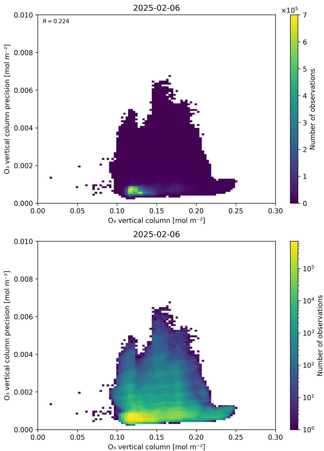
Figure 41: Scatter density plot of “O 3 vertical column” against “O 3 vertical column precision” for 2025-02-05 to 2025-02-07.
