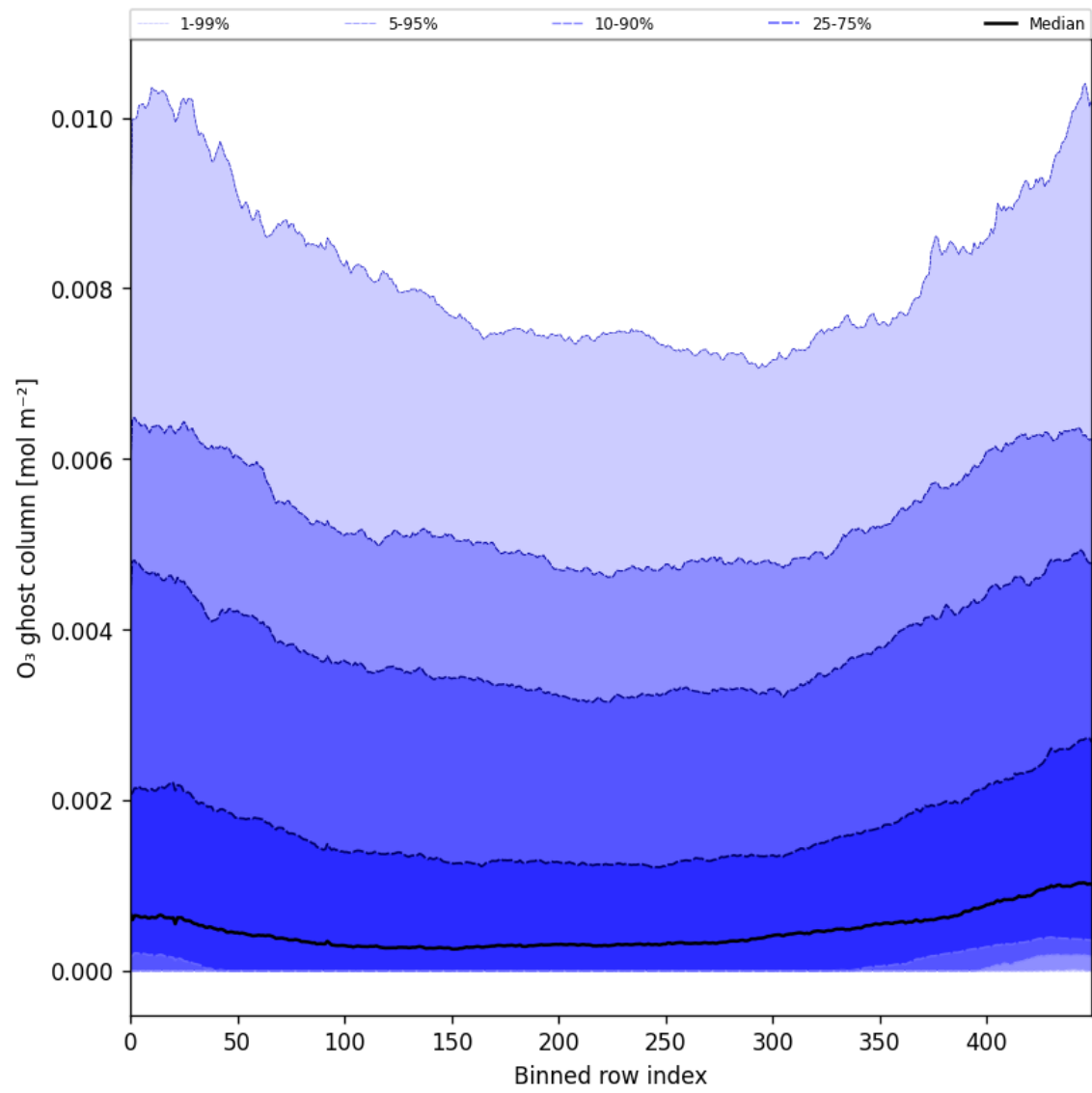
Figure 32: Along track statistics of “O 3 ghost column” for 2025-02-05 to 2025-02-07
