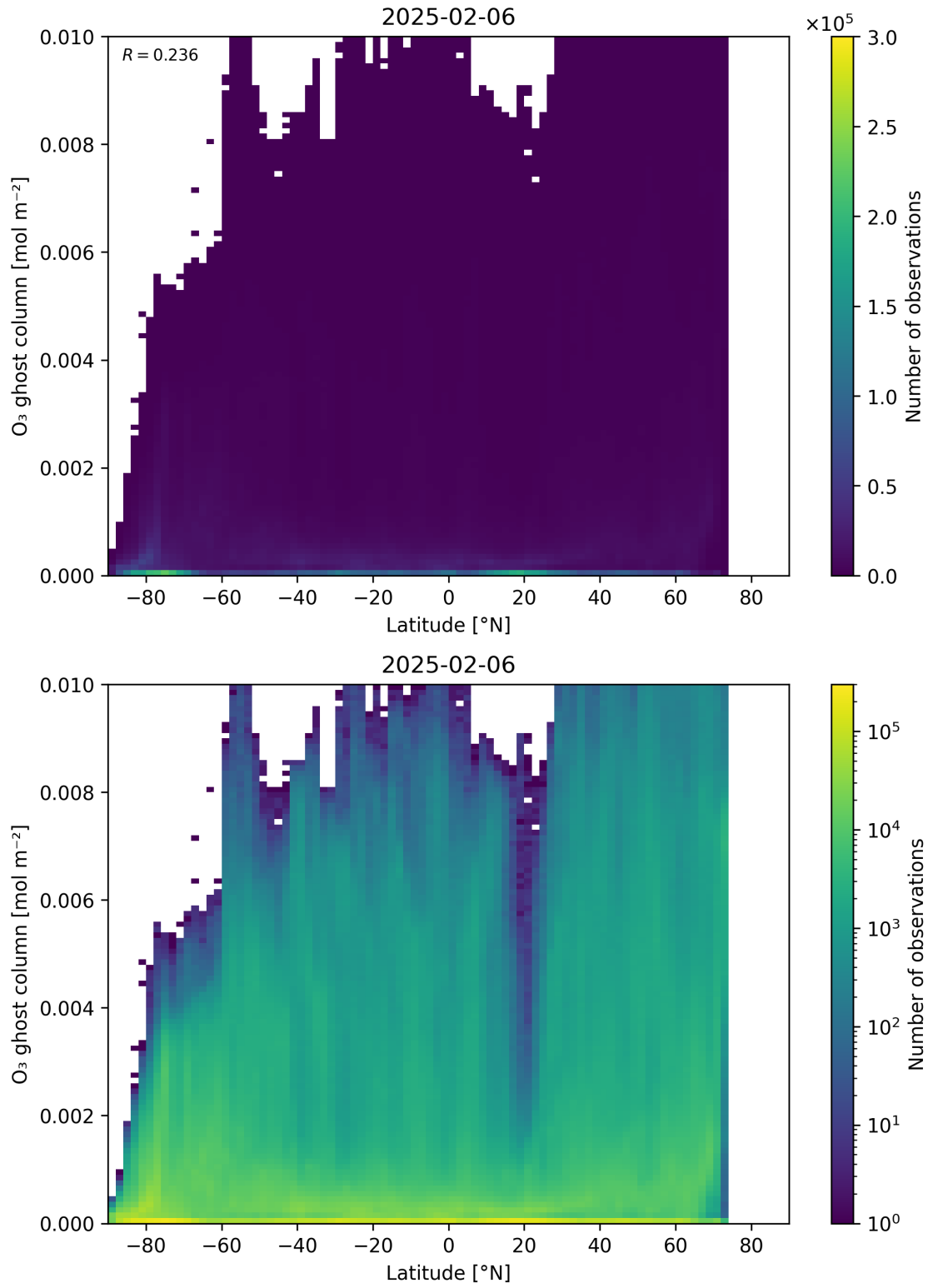
Figure 35: Scatter density plot of “Latitude” against “O 3 ghost column” for 2025-02-05 to 2025-02-07.
