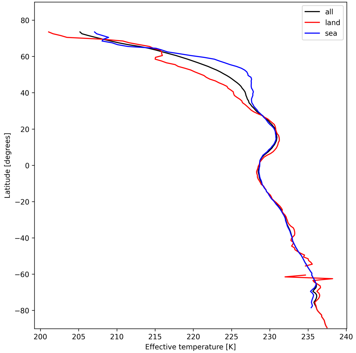
Figure 17: Zonal average of "Effective temperature" for 2025-02-05 to 2025-02-07.
