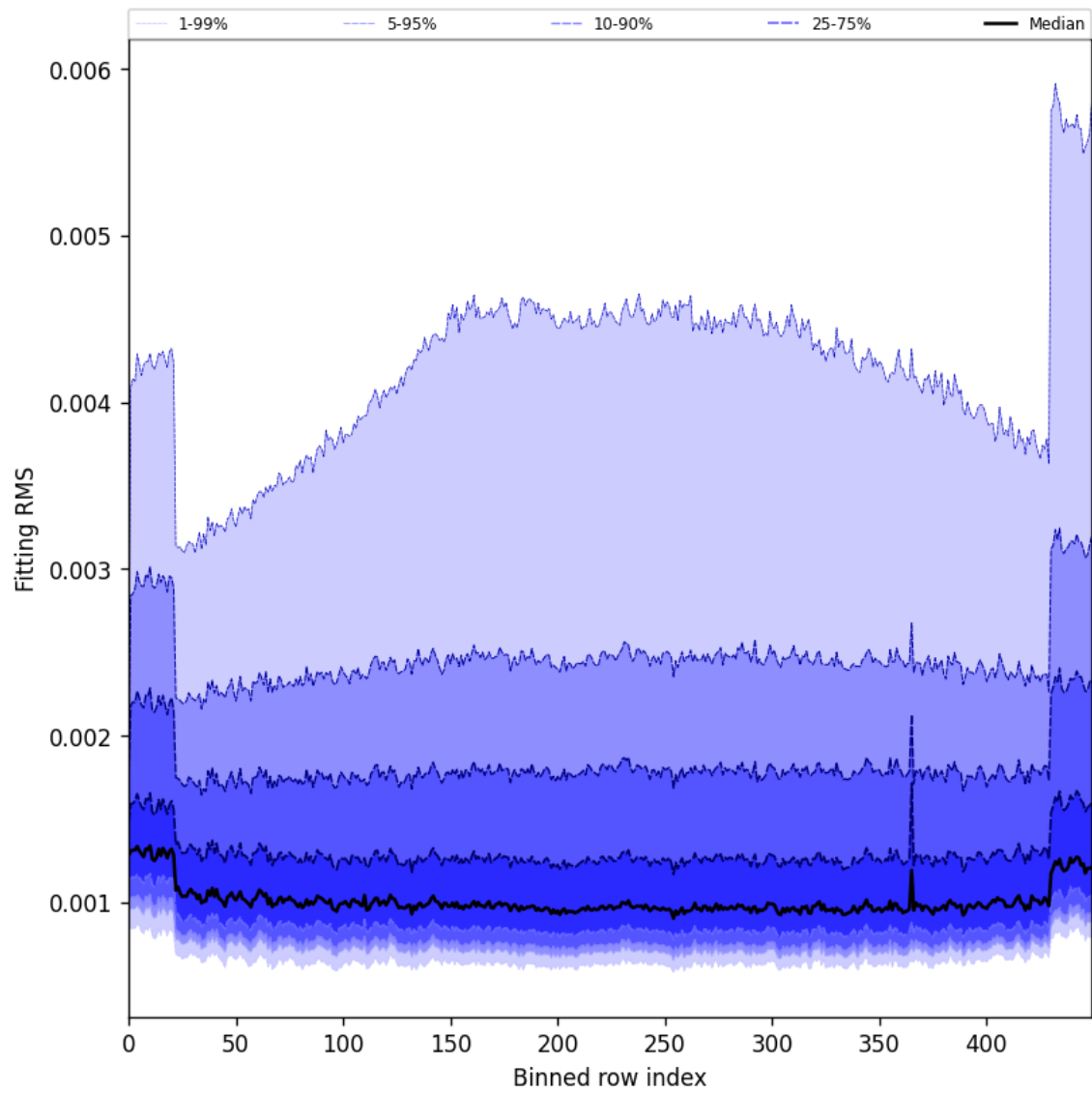
Figure 30: Along track statistics of “Fitting RMS” for 2025-02-06 to 2025-02-08
