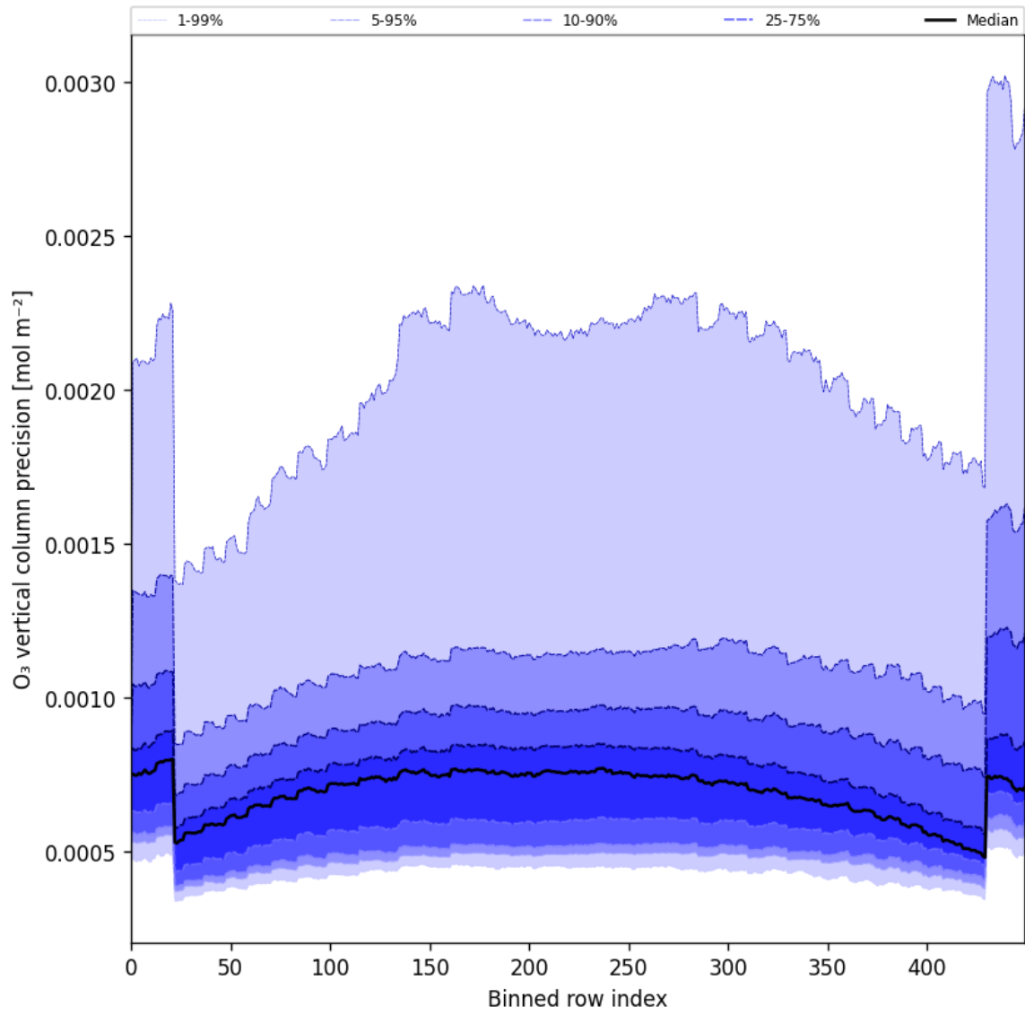
Figure 29: Along track statistics of “O 3 vertical column precision” for 2025-02-06 to 2025-02-08
