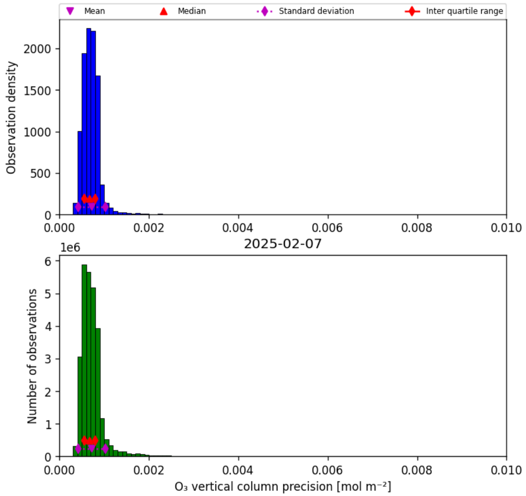
Figure 22: Histogram of “O 3 vertical column precision” for 2025-02-06 to 2025-02-08
