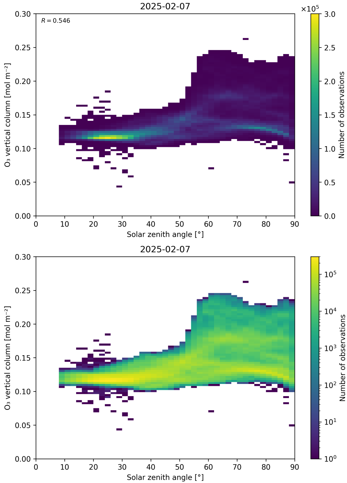
Figure 47: Scatter density plot of “Solar zenith angle” against “O 3 vertical column” for 2025-02-06 to 2025-02-08.
