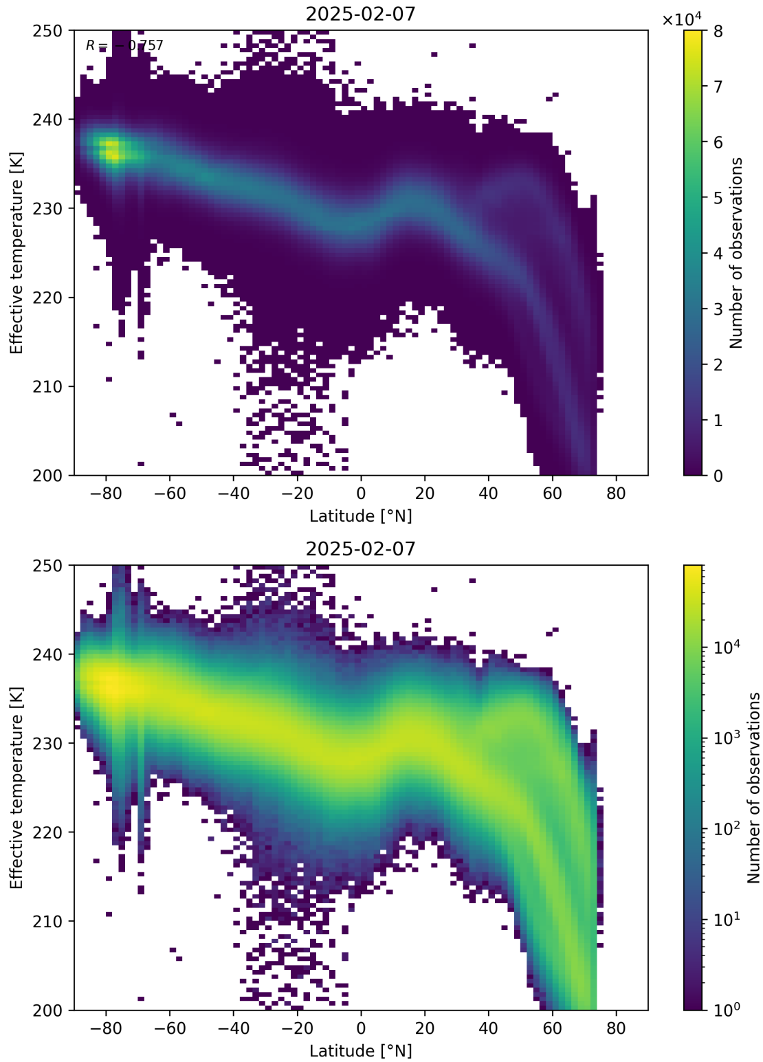
Figure 34: Scatter density plot of “Latitude” against “Effective temperature” for 2025-02-06 to 2025-02-08.
