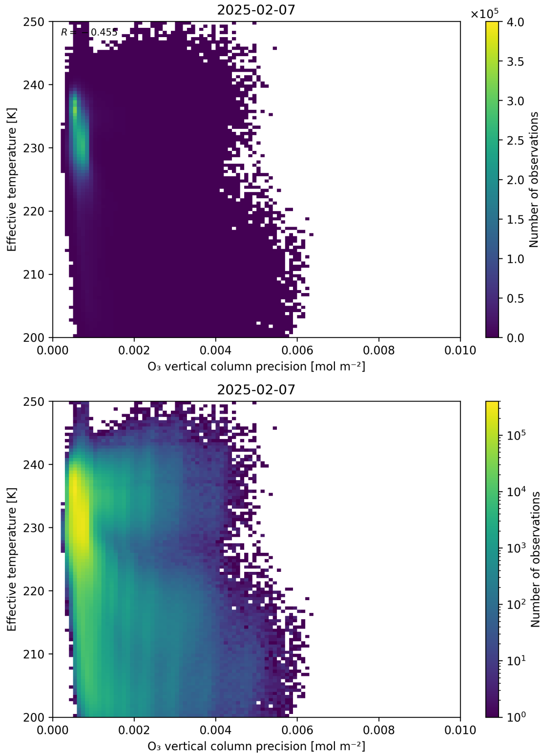
Figure 42: Scatter density plot of “O 3 vertical column precision” against “Effective temperature” for 2025-02-06 to 2025-02-08.
