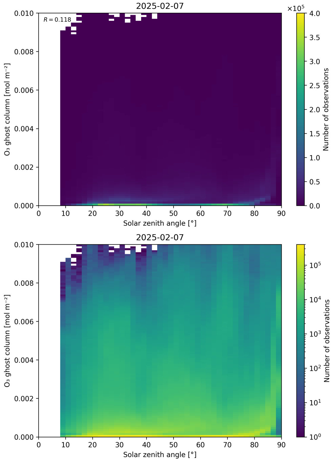
Figure 46: Scatter density plot of “Solar zenith angle” against “O 3 ghost column” for 2025-02-06 to 2025-02-08.
