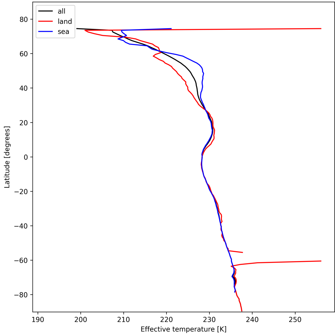
Figure 17: Zonal average of “Effective temperature” for 2025-02-06 to 2025-02-08.
