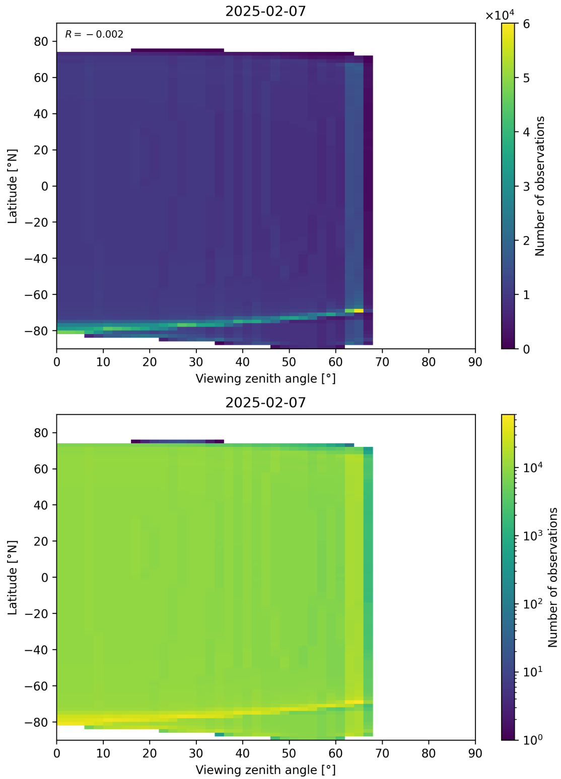
Figure 49: Scatter density plot of “Viewing zenith angle” against “Latitude” for 2025-02-06 to 2025-02-08.
