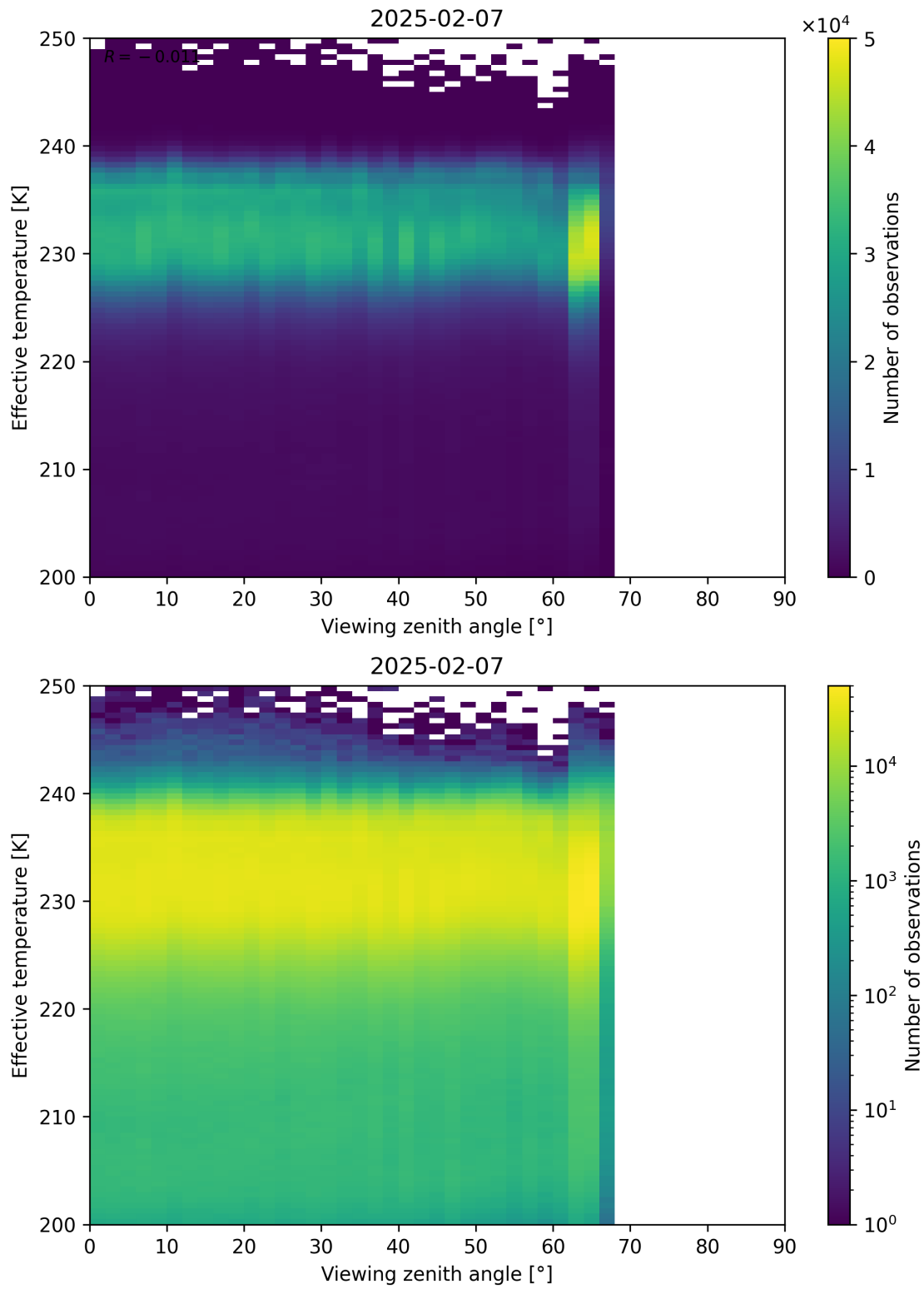
Figure 50: Scatter density plot of “Viewing zenith angle” against “Effective temperature” for 2025-02-06 to 2025-02-08.
