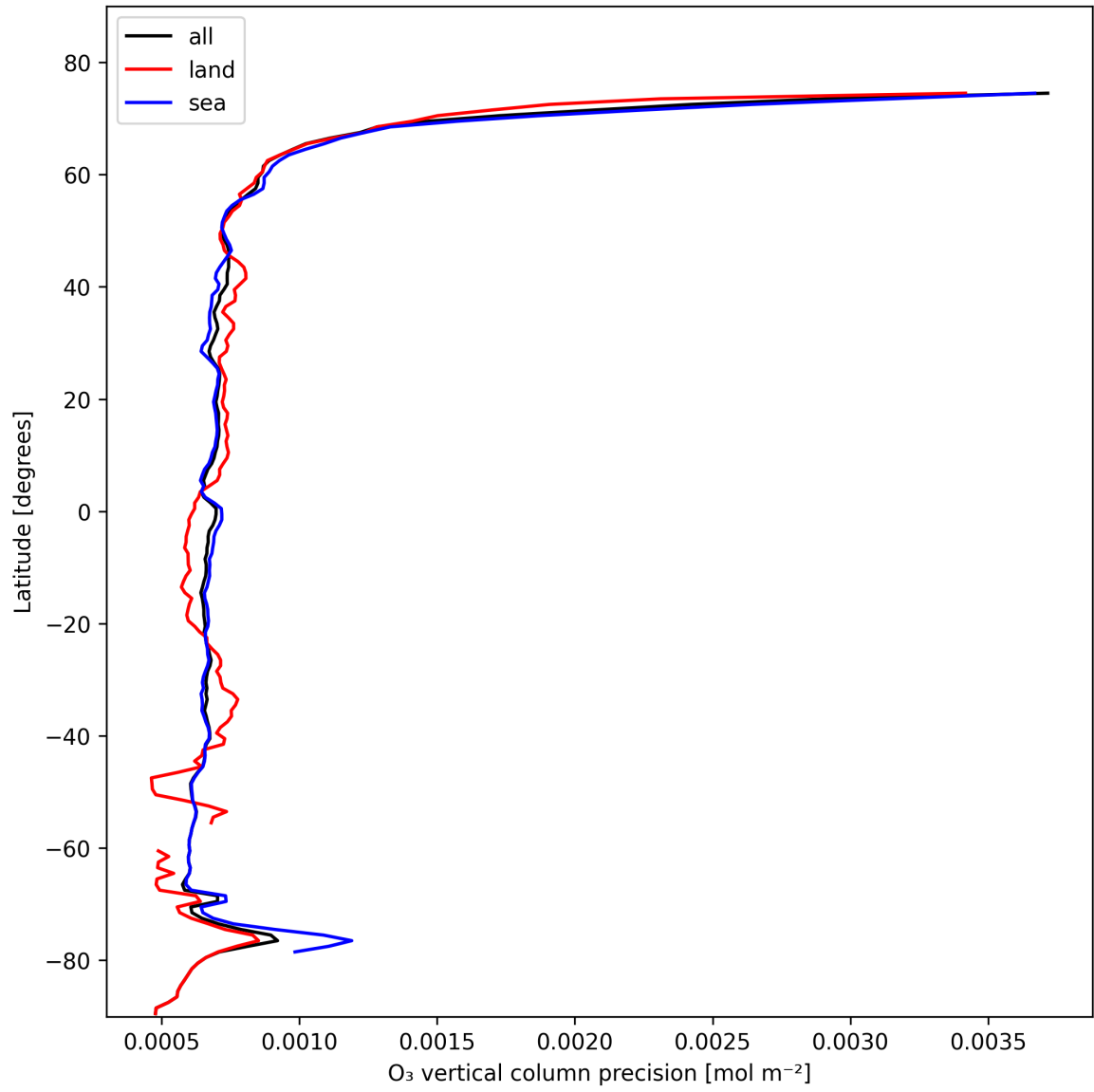
Figure 15: Zonal average of “O 3 vertical column precision” for 2025-02-06 to 2025-02-08.
