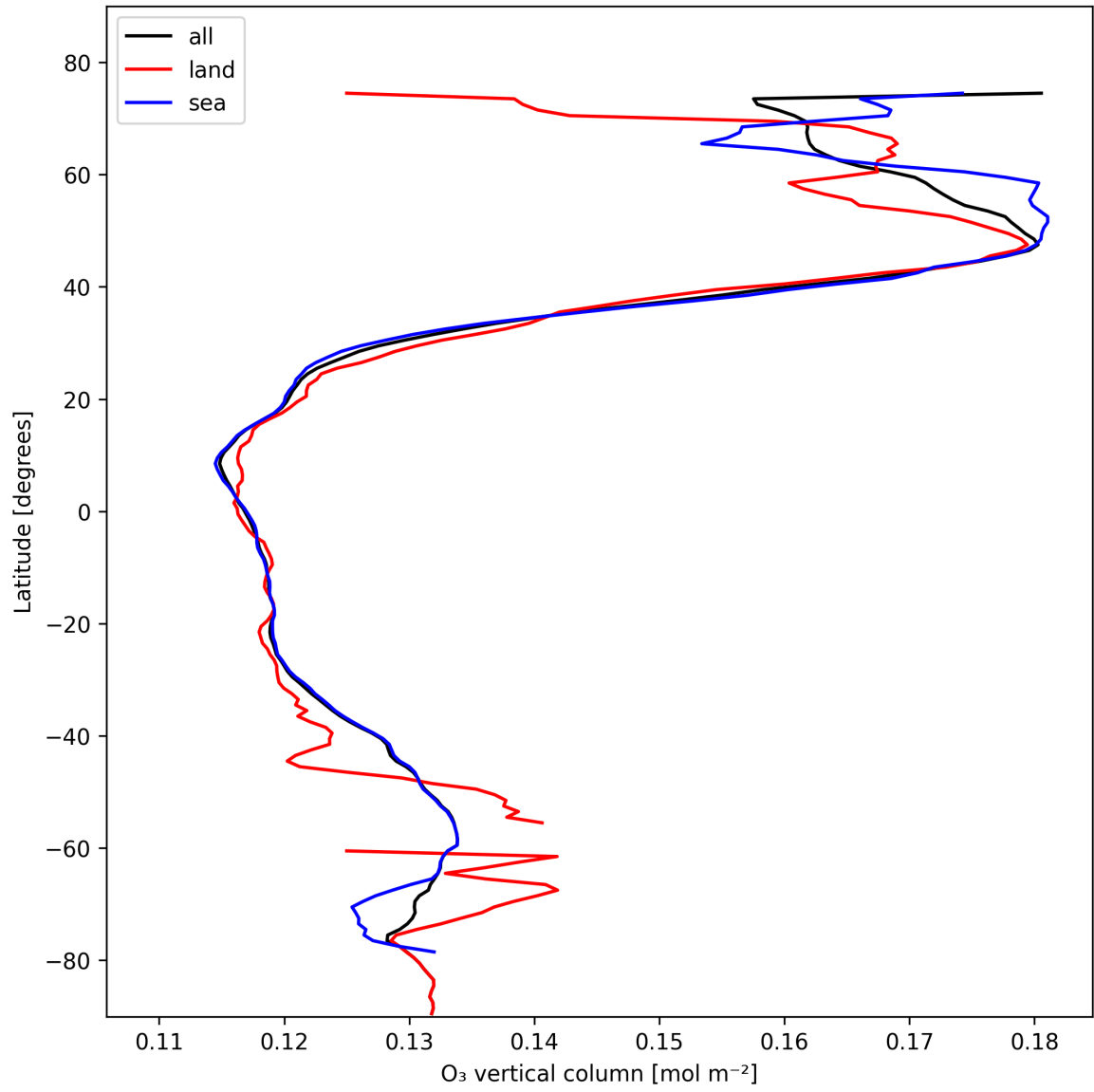
Figure 14: Zonal average of “O 3 vertical column” for 2025-02-06 to 2025-02-08.
