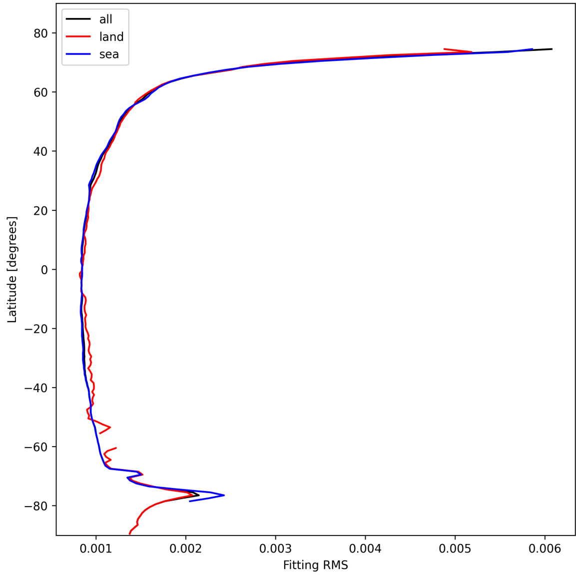
Figure 16: Zonal average of “Fitting RMS” for 2025-02-06 to 2025-02-08.
