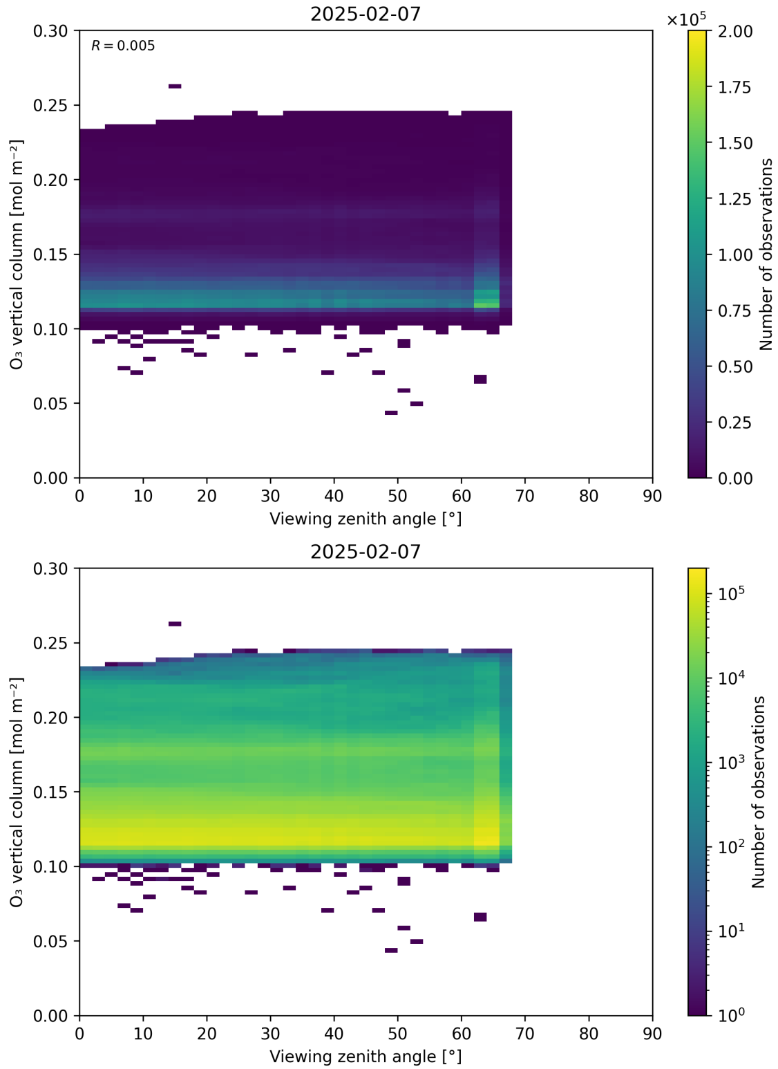
Figure 52: Scatter density plot of “Viewing zenith angle” against “O 3 vertical column” for 2025-02-06 to 2025-02-08.
