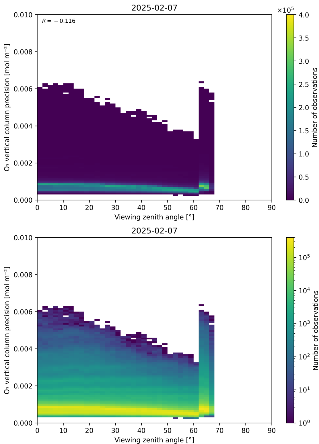
Figure 53: Scatter density plot of “Viewing zenith angle” against “O 3 vertical column precision” for 2025-02-06 to 2025-02-08.
