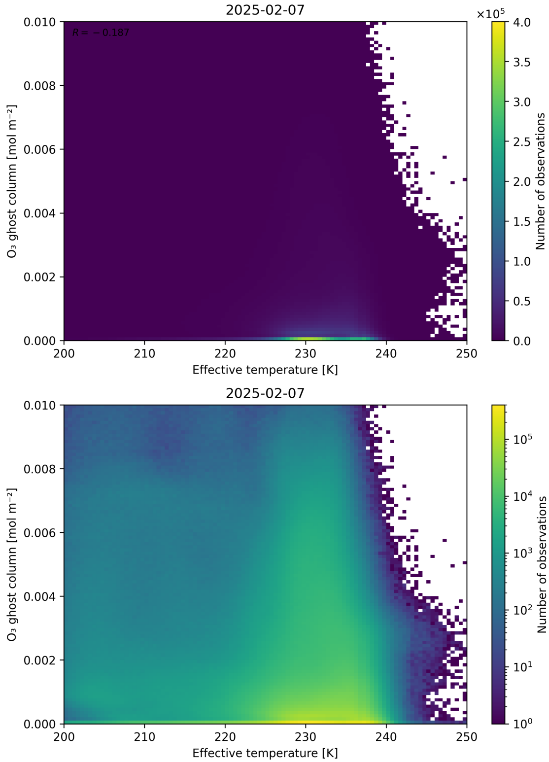
Figure 38: Scatter density plot of “Effective temperature” against “O 3 ghost column” for 2025-02-06 to 2025-02-08.
