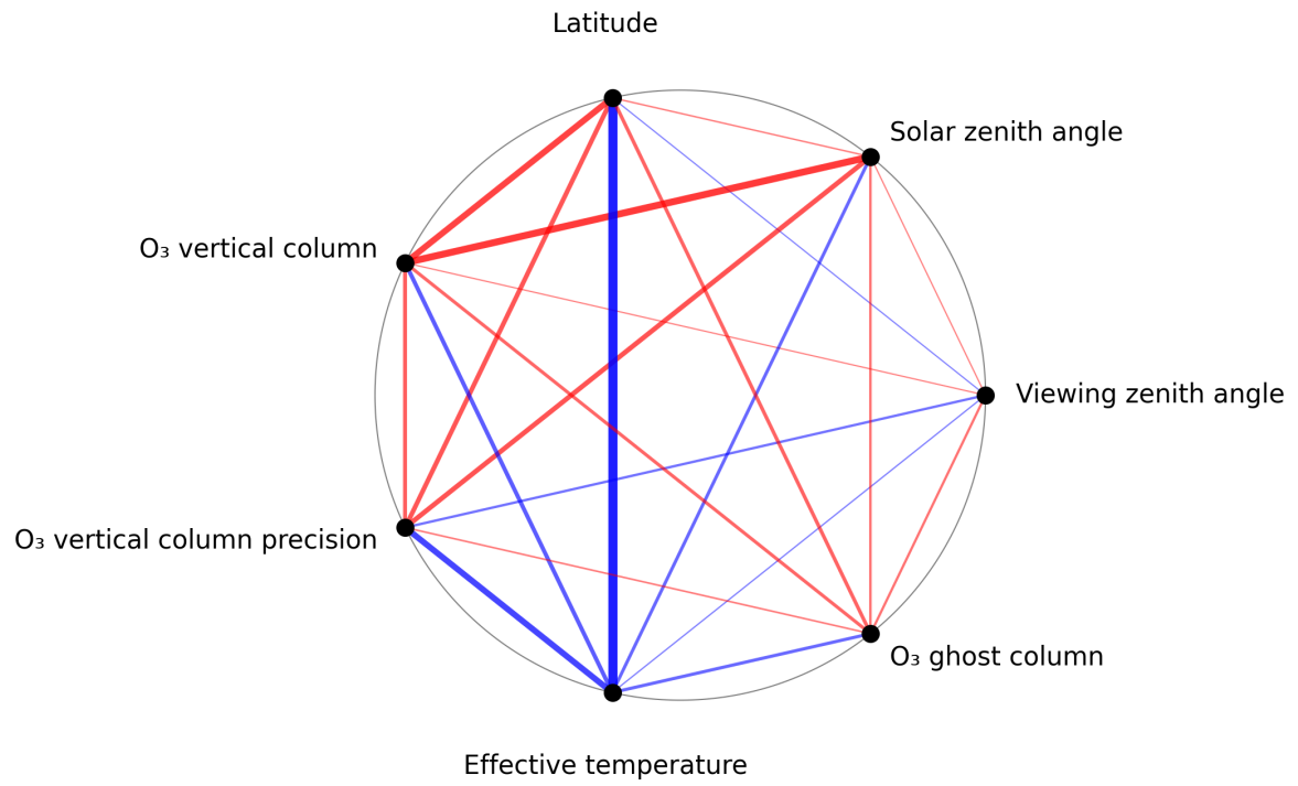
Figure 1: Map of correlation graph for 2025-02-06 to 2025-02-08.
