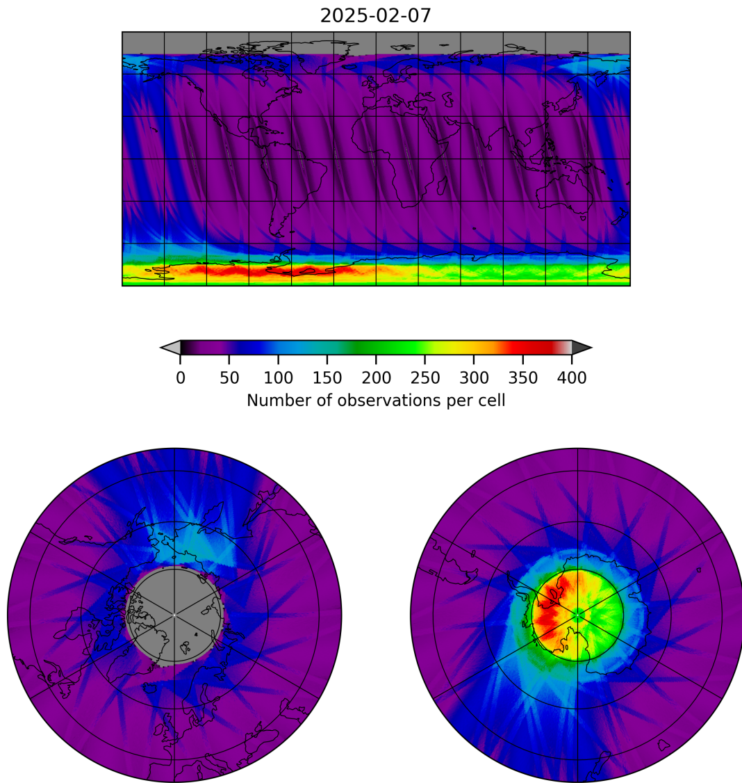
Figure 12: Map of the number of observations for 2025-02-06 to 2025-02-08
