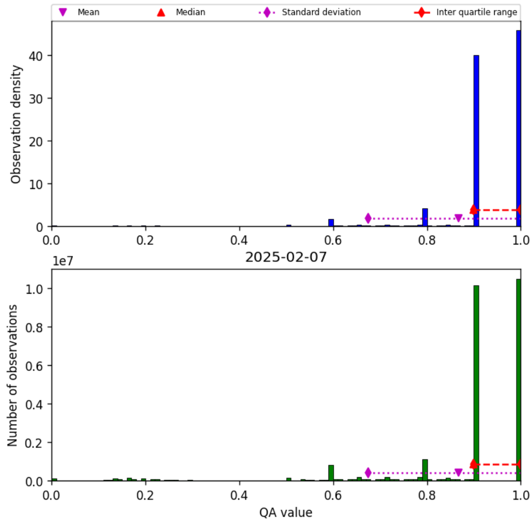
Figure 20: Histogram of “QA value” for 2025-02-06 to 2025-02-08
