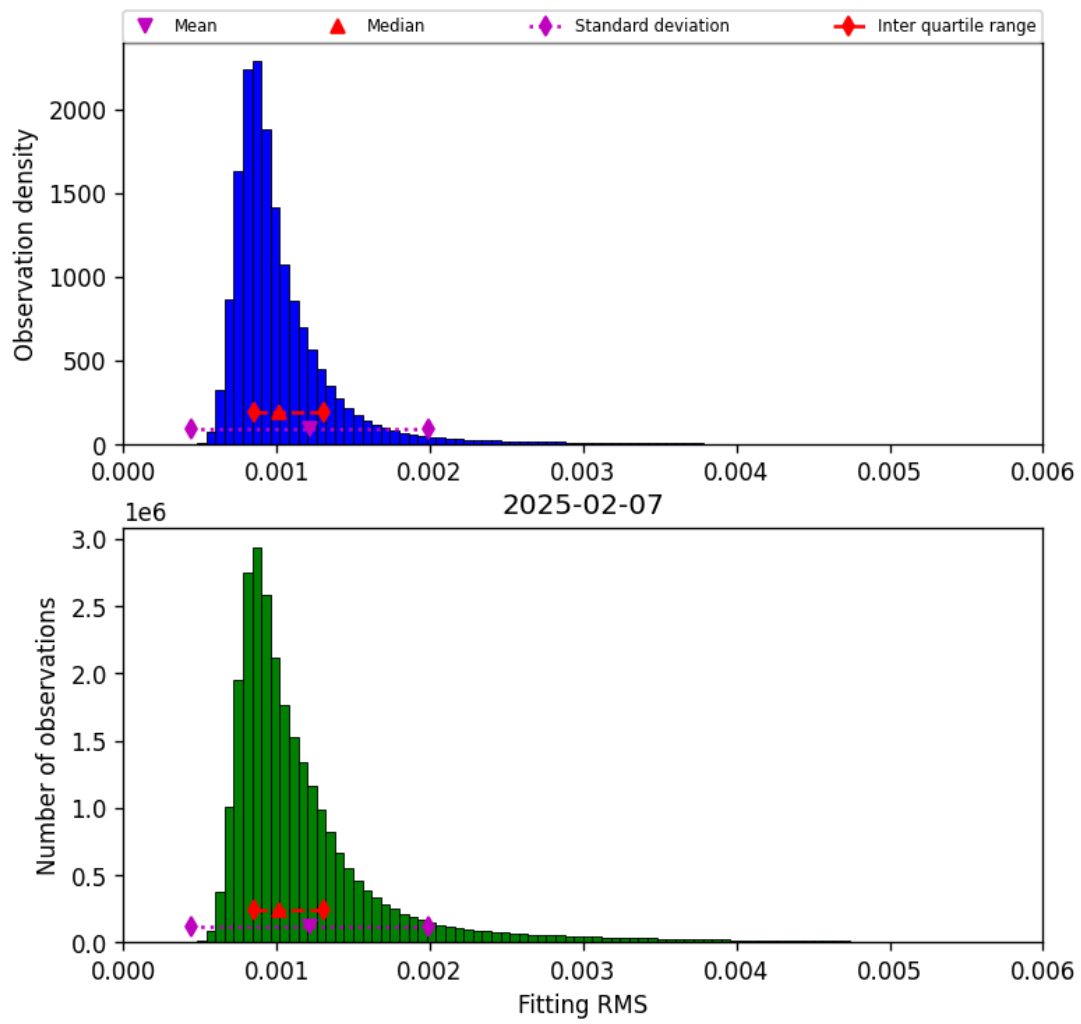
Figure 23: Histogram of “Fitting RMS” for 2025-02-06 to 2025-02-08
