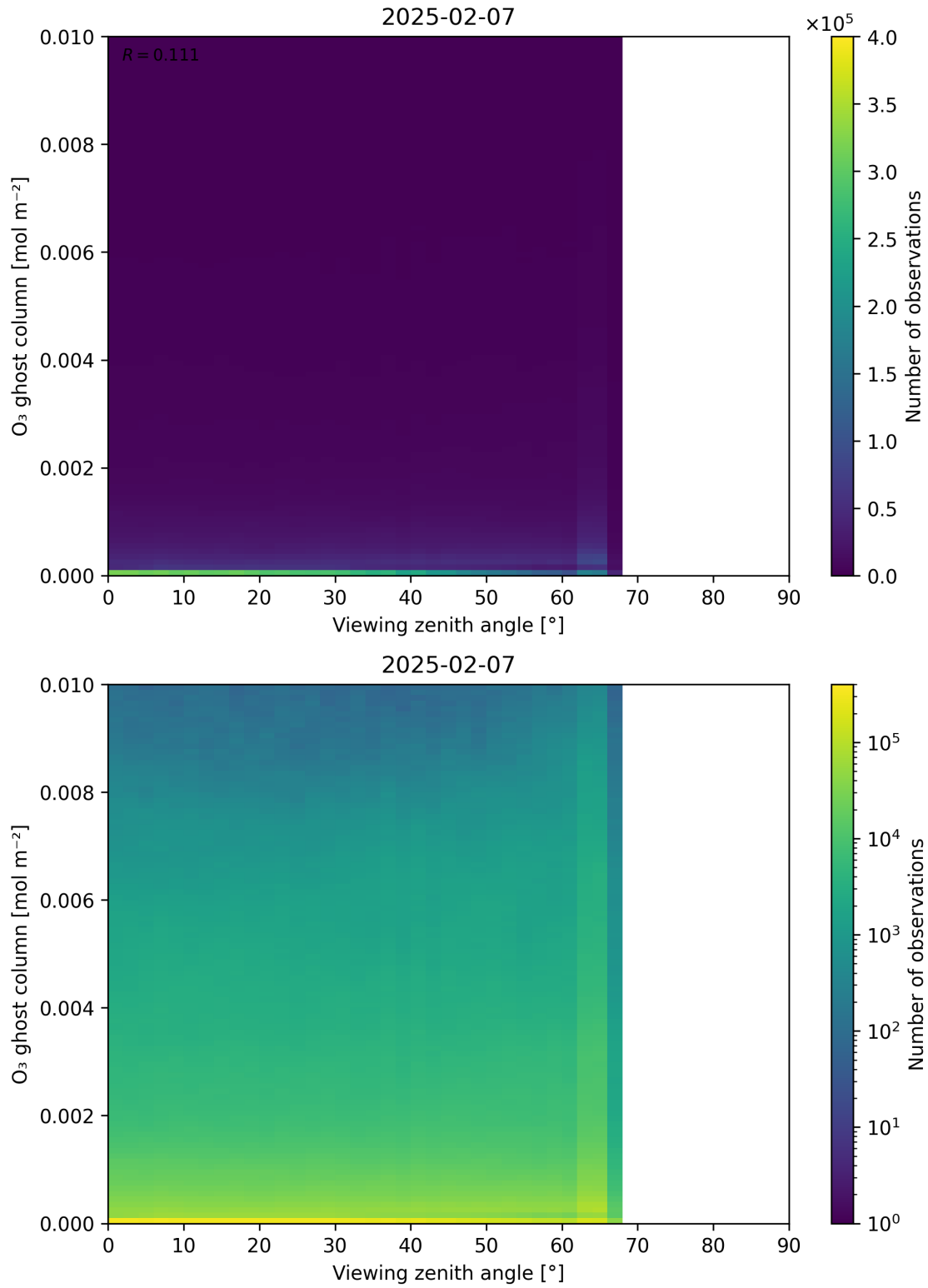
Figure 51: Scatter density plot of “Viewing zenith angle” against “O 3 ghost column” for 2025-02-06 to 2025-02-08.
