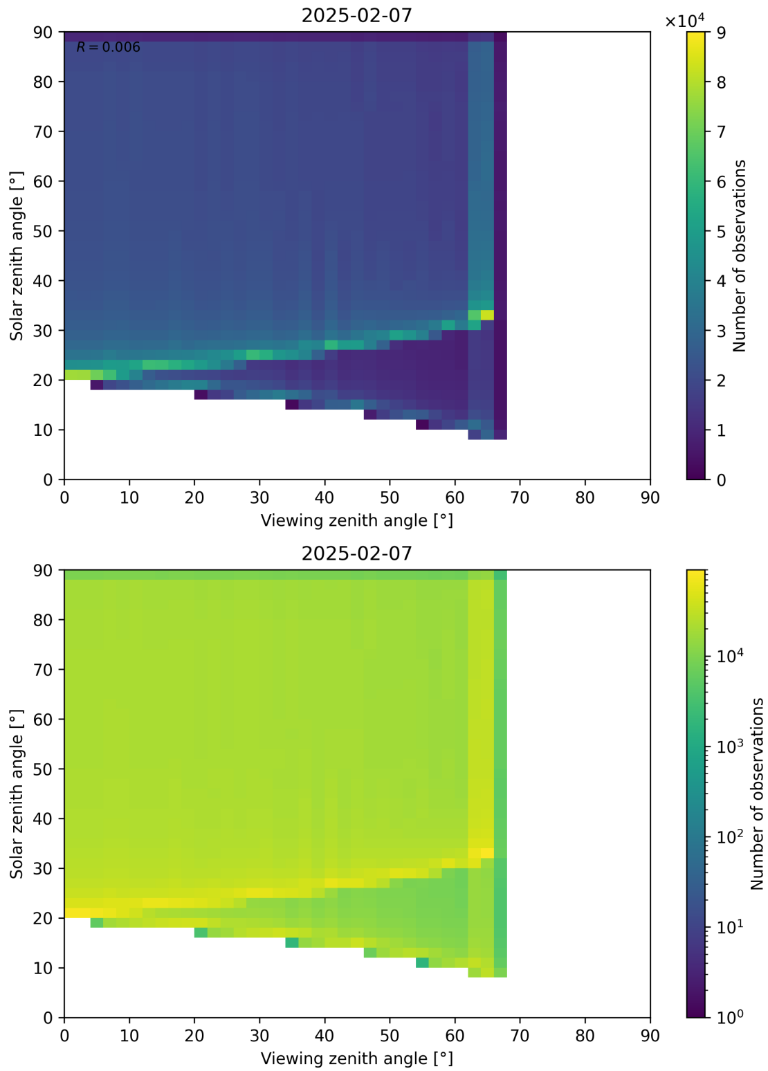
Figure 54: Scatter density plot of “Viewing zenith angle” against “Solar zenith angle” for 2025-02-06 to 2025-02-08.
