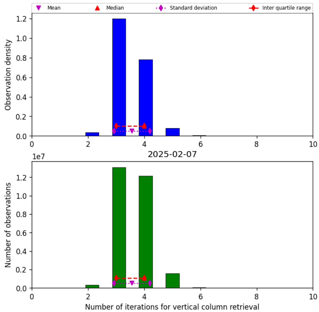
Figure 26: Histogram of “Number of iterations for vertical column retrieval” for 2025-02-06 to 2025-02-08
