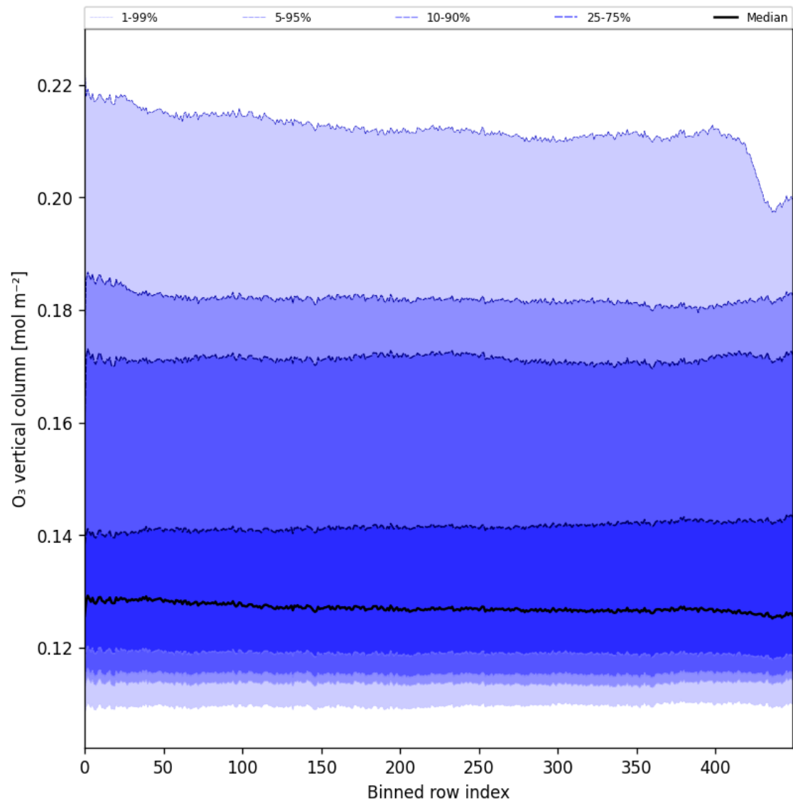
Figure 28: Along track statistics of "O 3 vertical column" for 2025-02-06 to 2025-02-08
