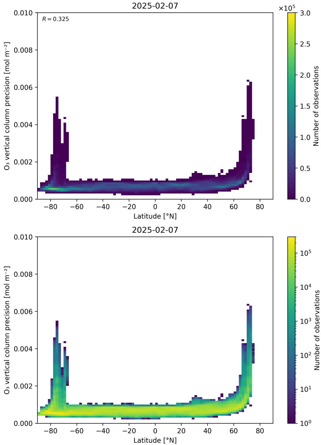
Figure 37: Scatter density plot of “Latitude” against “O 3 vertical column precision” for 2025-02-06 to 2025-02-08.
