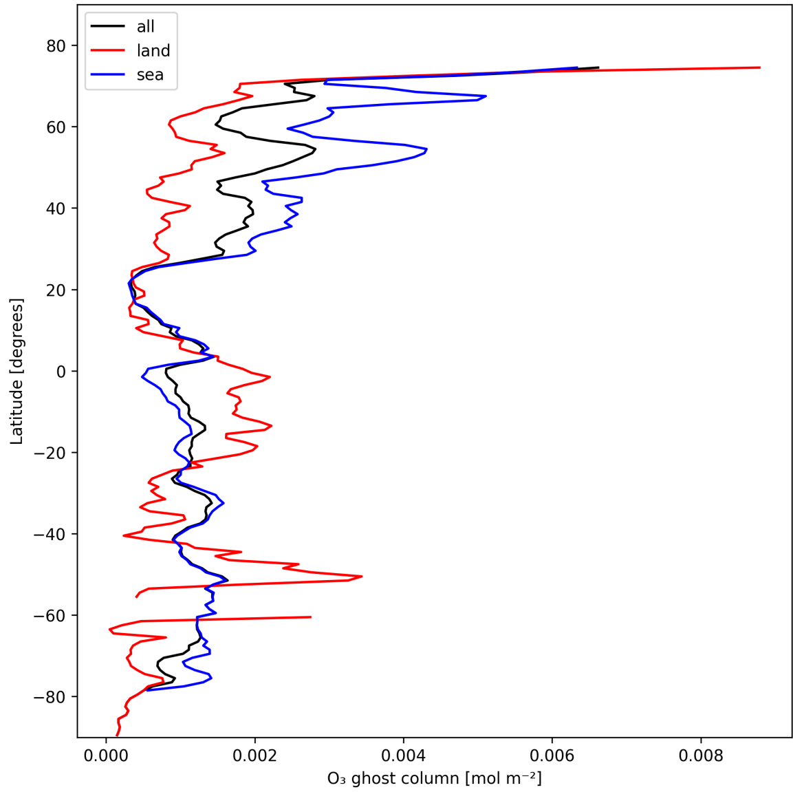
Figure 18: Zonal average of "O 3 ghost column" for 2025-02-06 to 2025-02-08.
