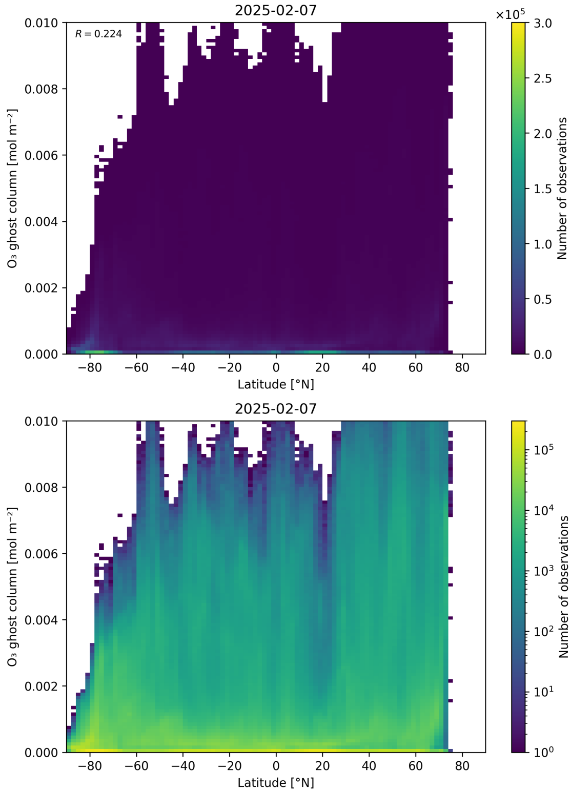
Figure 35: Scatter density plot of “Latitude” against “O 3 ghost column” for 2025-02-06 to 2025-02-08.
