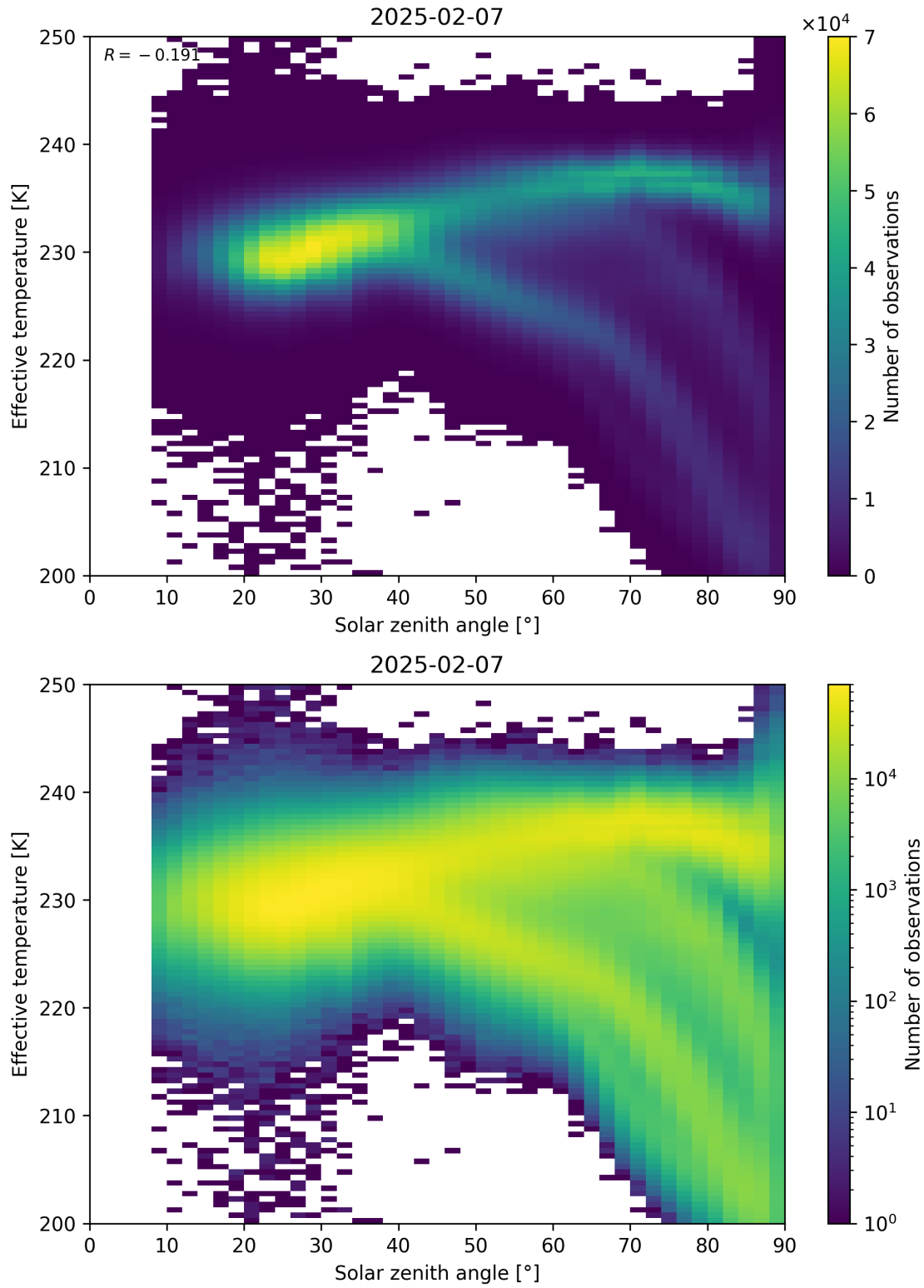
Figure 45: Scatter density plot of “Solar zenith angle” against “Effective temperature” for 2025-02-06 to 2025-02-08.
