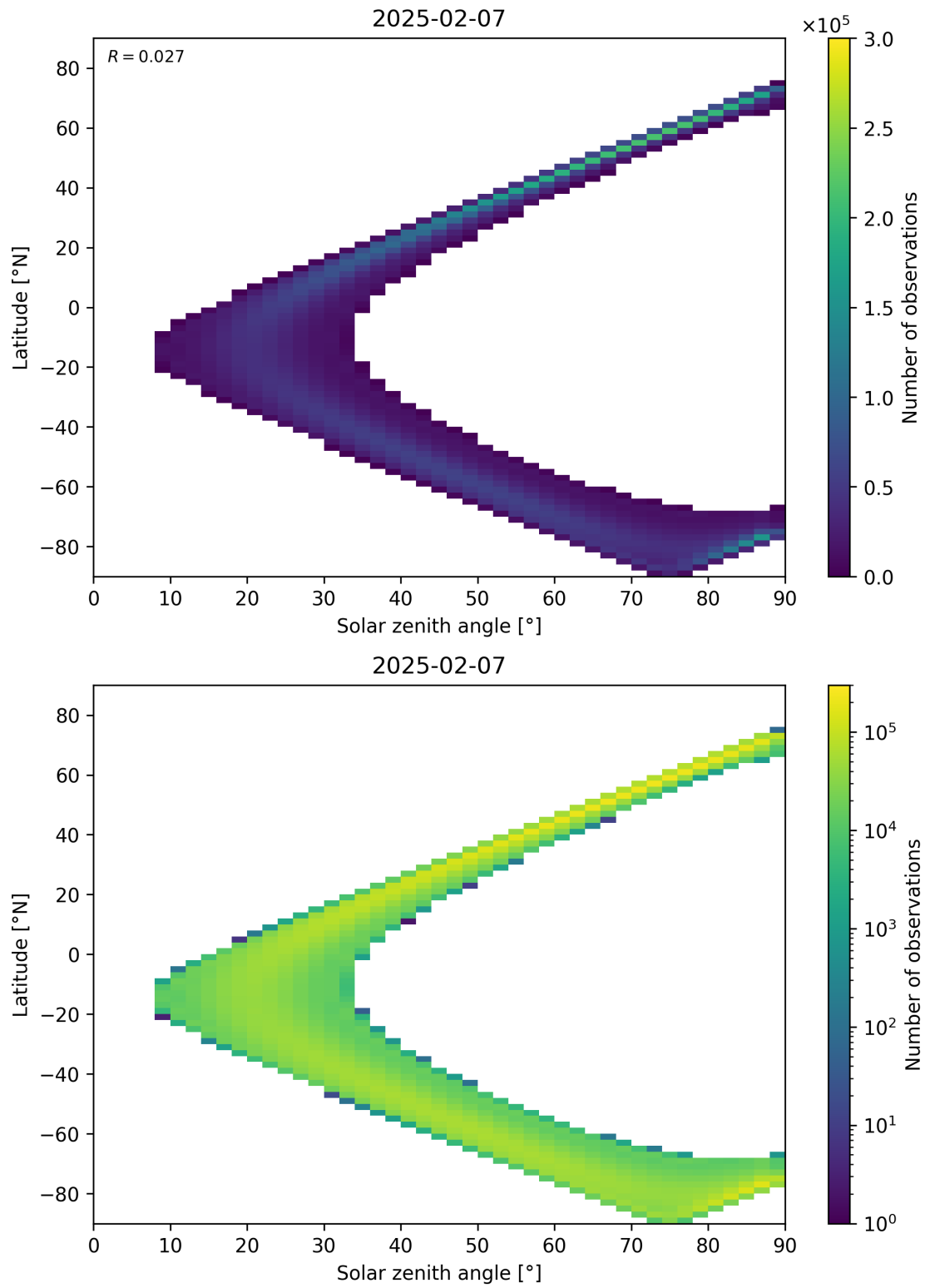
Figure 44: Scatter density plot of “Solar zenith angle” against “Latitude” for 2025-02-06 to 2025-02-08.
