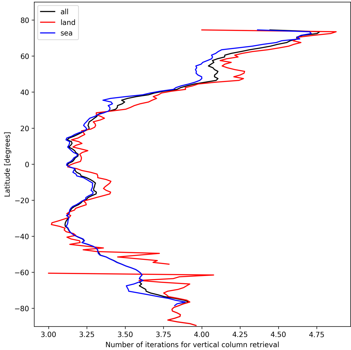
Figure 19: Zonal average of “Number of iterations for vertical column retrieval” for 2025-02-06 to 2025-02-08.
