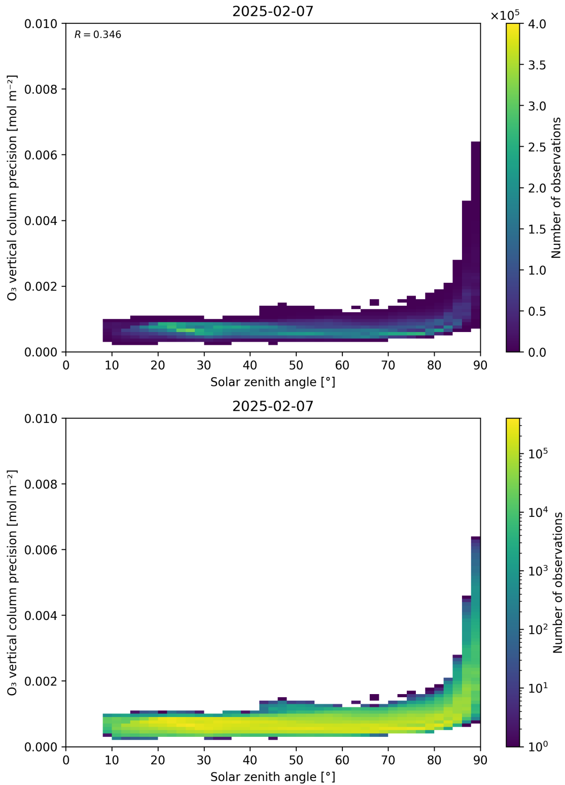
Figure 48: Scatter density plot of “Solar zenith angle” against “O 3 vertical column precision” for 2025-02-06 to 2025-02-08.
