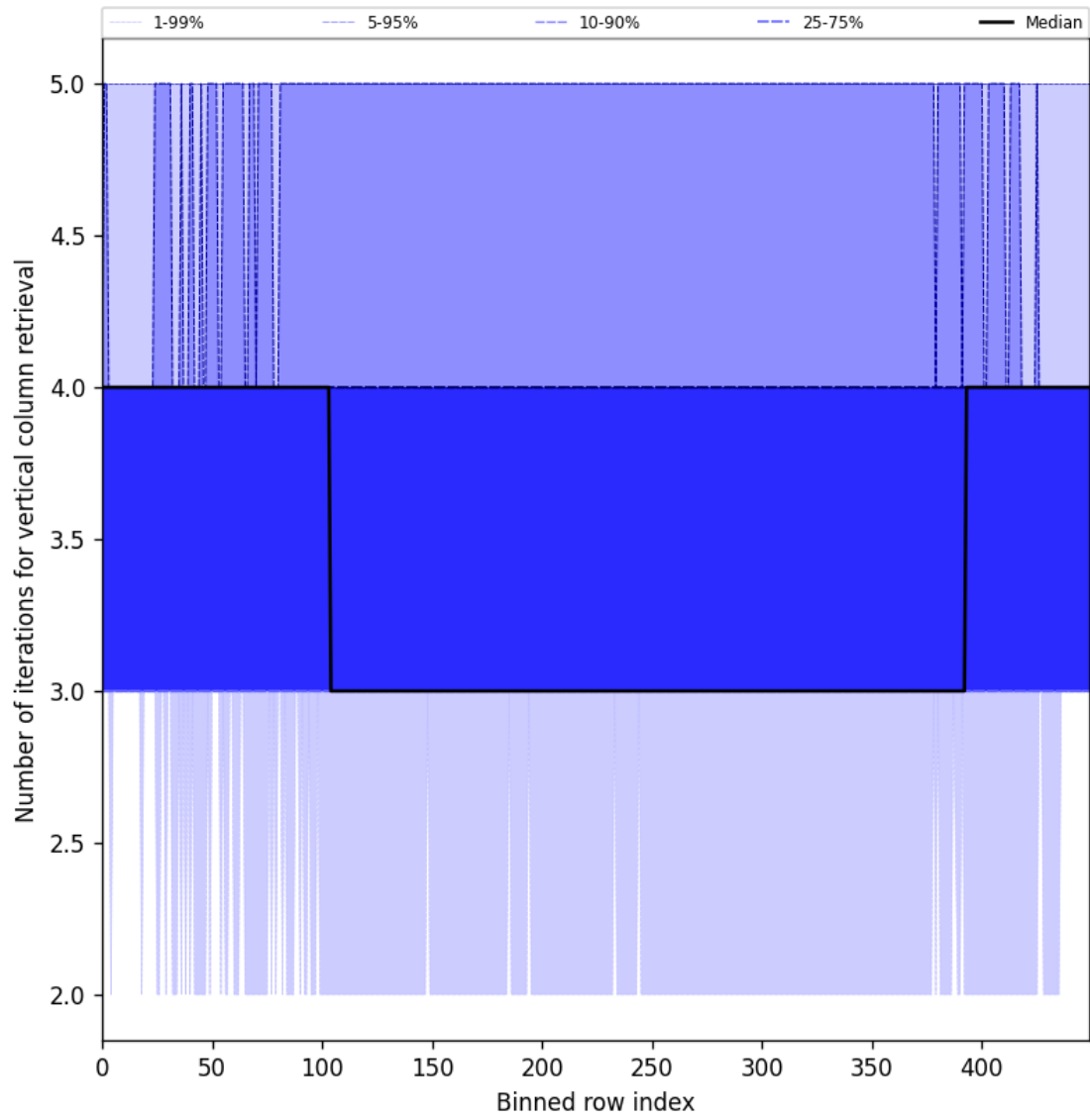
Figure 33: Along track statistics of “Number of iterations for vertical column retrieval” for 2025-02-06 to 2025-02-08
