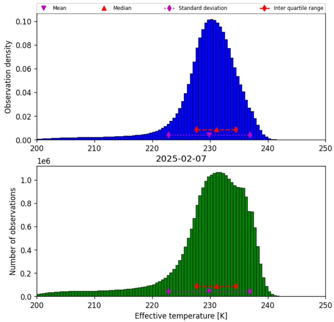
Figure 24: Histogram of “Effective temperature” for 2025-02-06 to 2025-02-08
