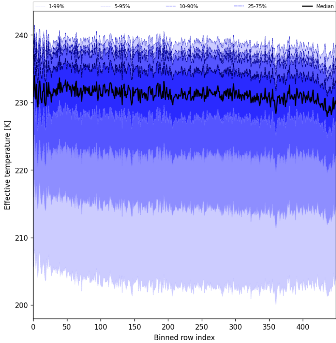
Figure 31: Along track statistics of “Effective temperature” for 2025-02-06 to 2025-02-08
