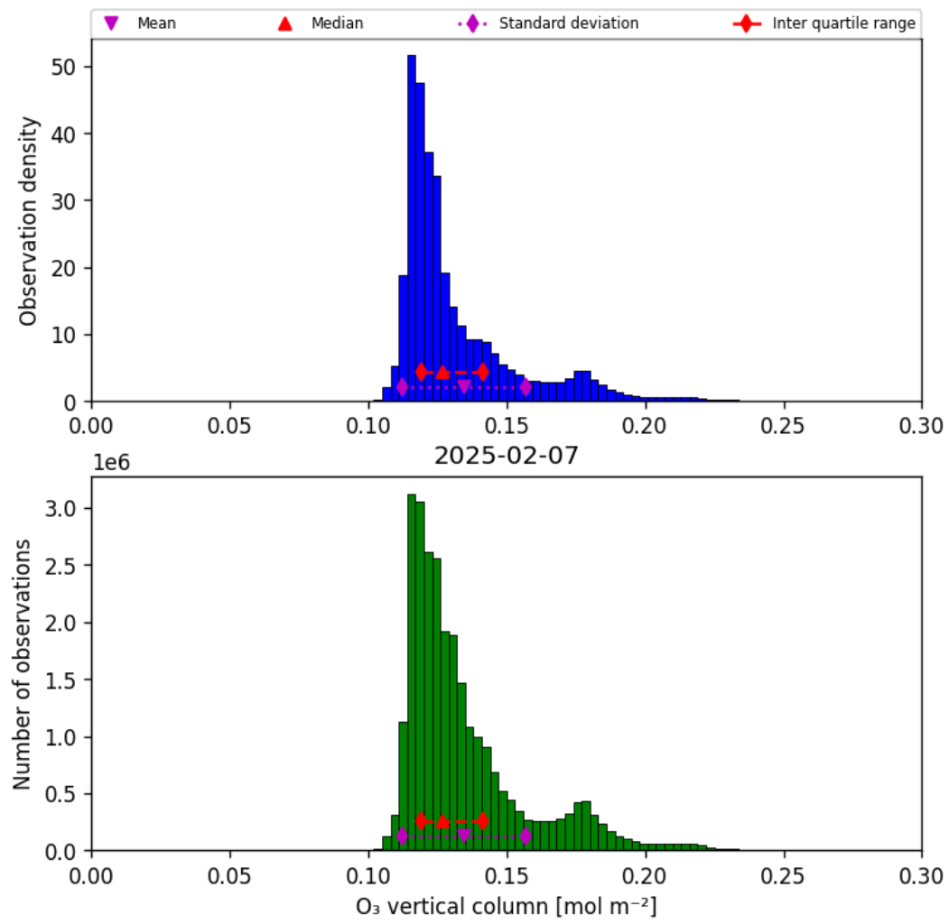
Figure 21: Histogram of “O 3 vertical column” for 2025-02-06 to 2025-02-08
