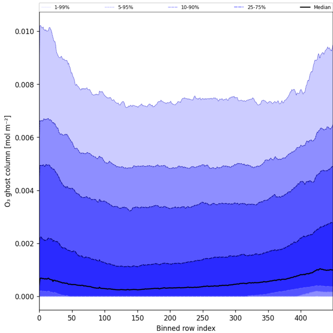
Figure 32: Along track statistics of “O 3 ghost column” for 2025-02-06 to 2025-02-08
