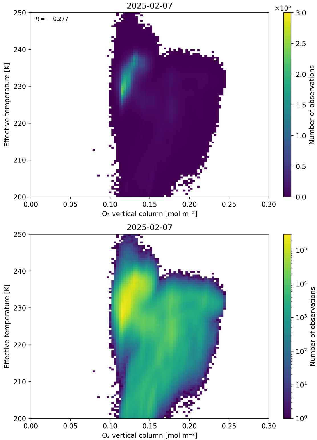
Figure 39: Scatter density plot of “O 3 vertical column” against “Effective temperature” for 2025-02-06 to 2025-02-08.
