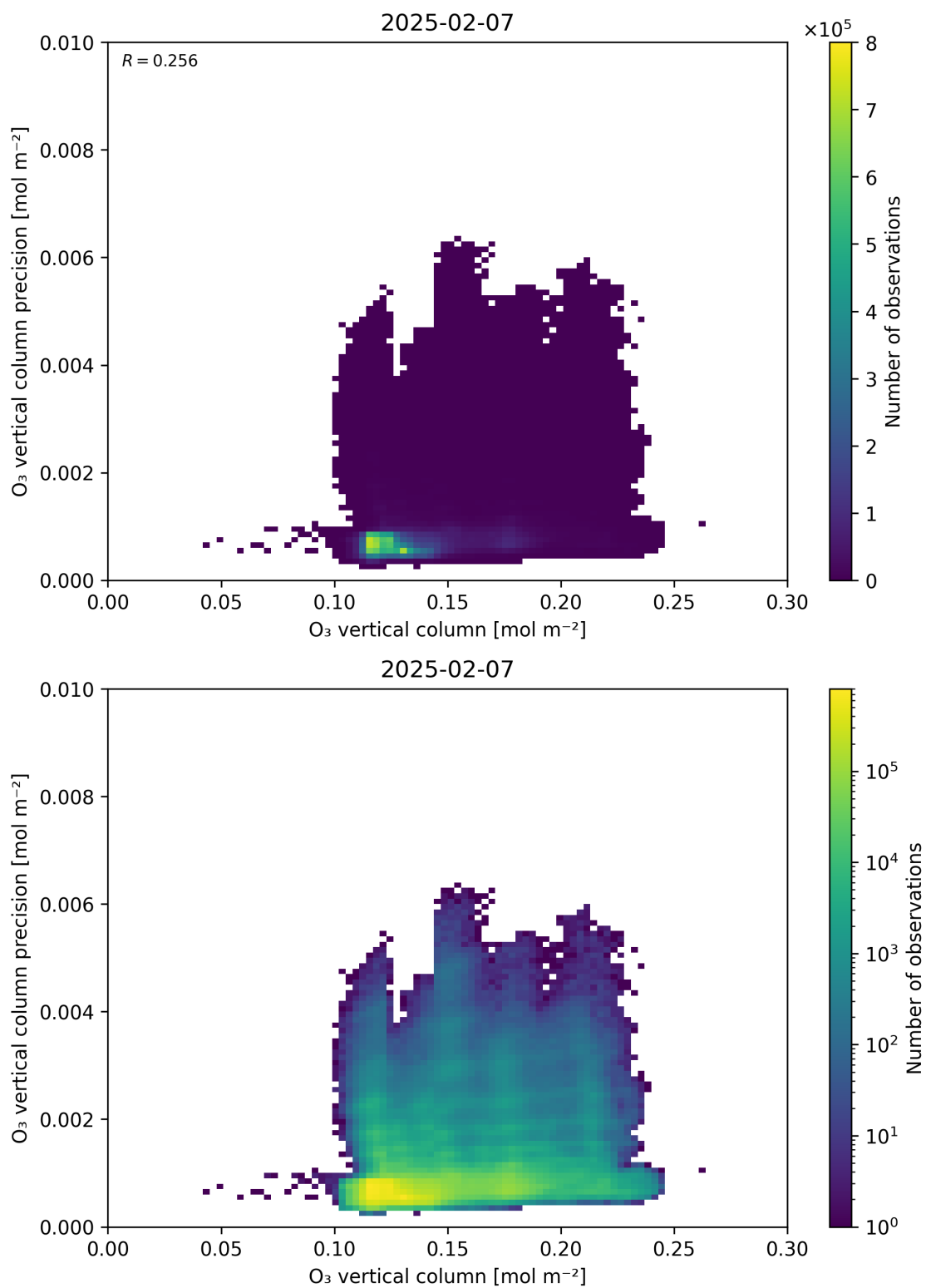
Figure 41: Scatter density plot of “O 3 vertical column” against “O 3 vertical column precision” for 2025-02-06 to 2025-02-08.
