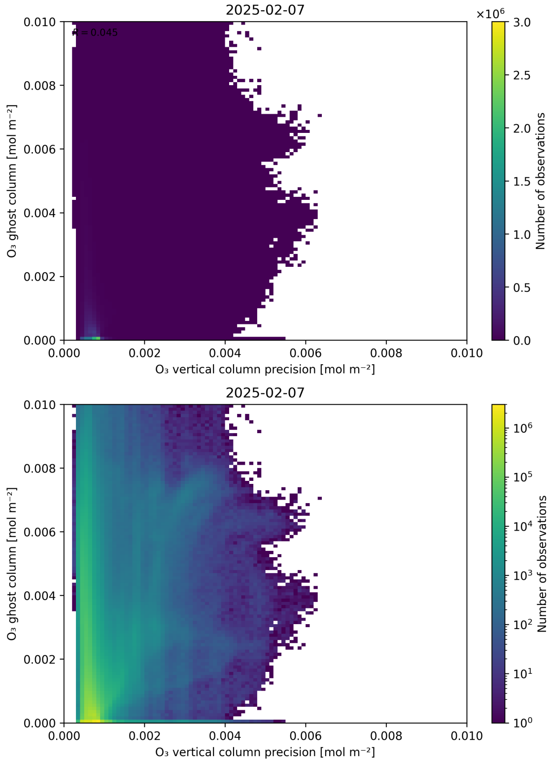
Figure 43: Scatter density plot of “O 3 vertical column precision” against “O 3 ghost column” for 2025-02-06 to 2025-02-08.
