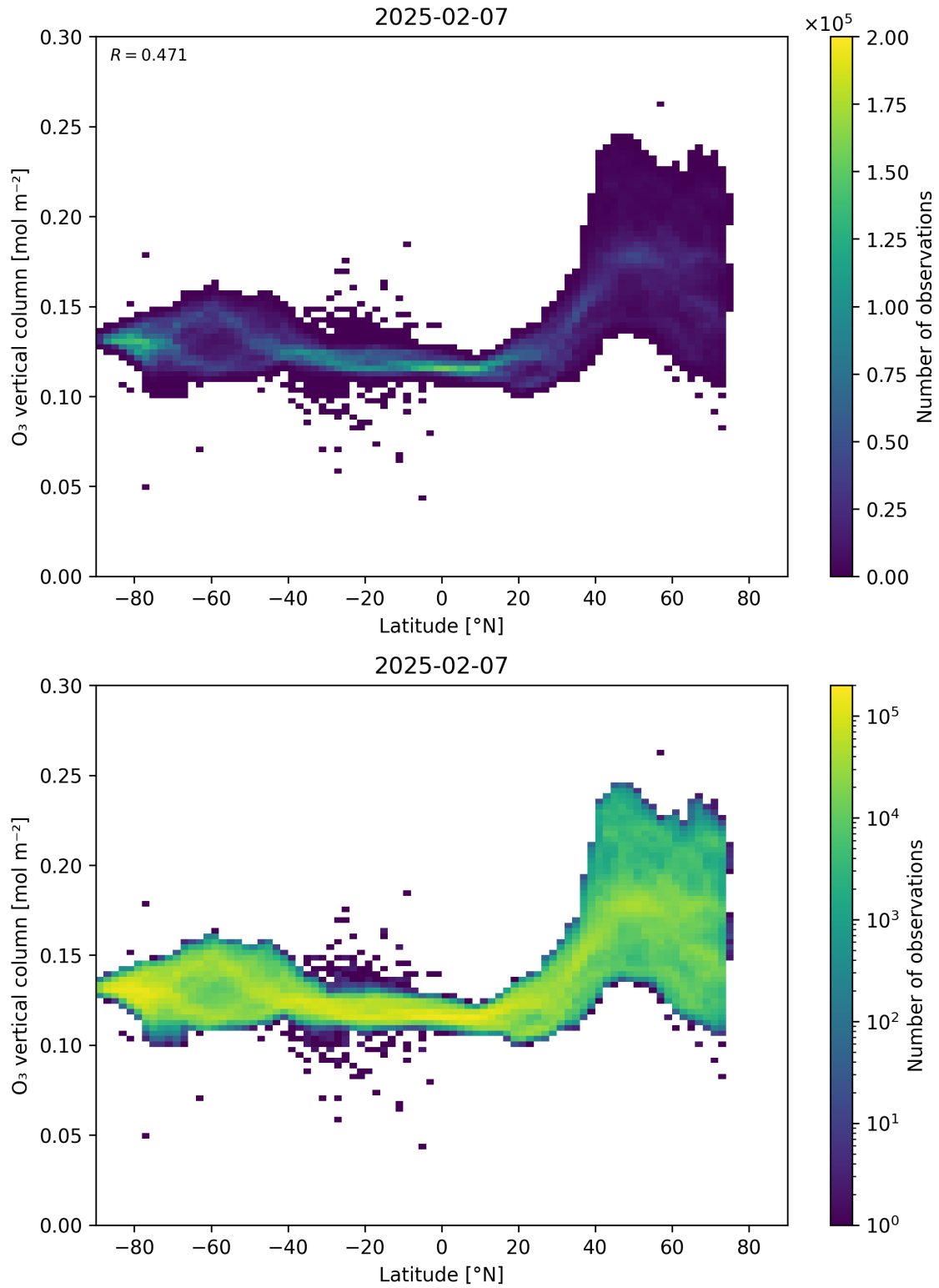
Figure 36: Scatter density plot of “Latitude” against “O 3 vertical column” for 2025-02-06 to 2025-02-08.
