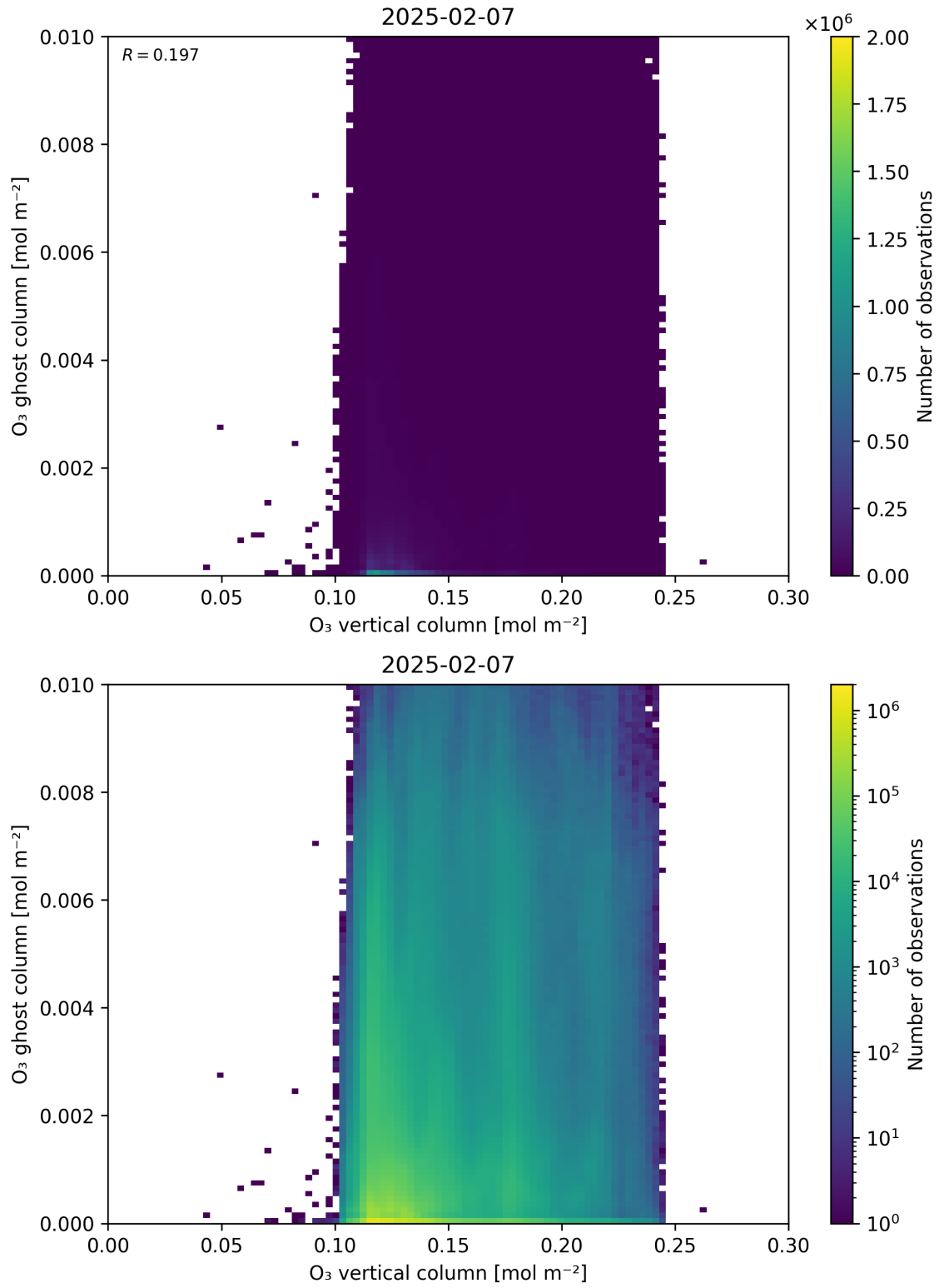
Figure 40: Scatter density plot of “O 3 vertical column” against “O 3 ghost column” for 2025-02-06 to 2025-02-08.
