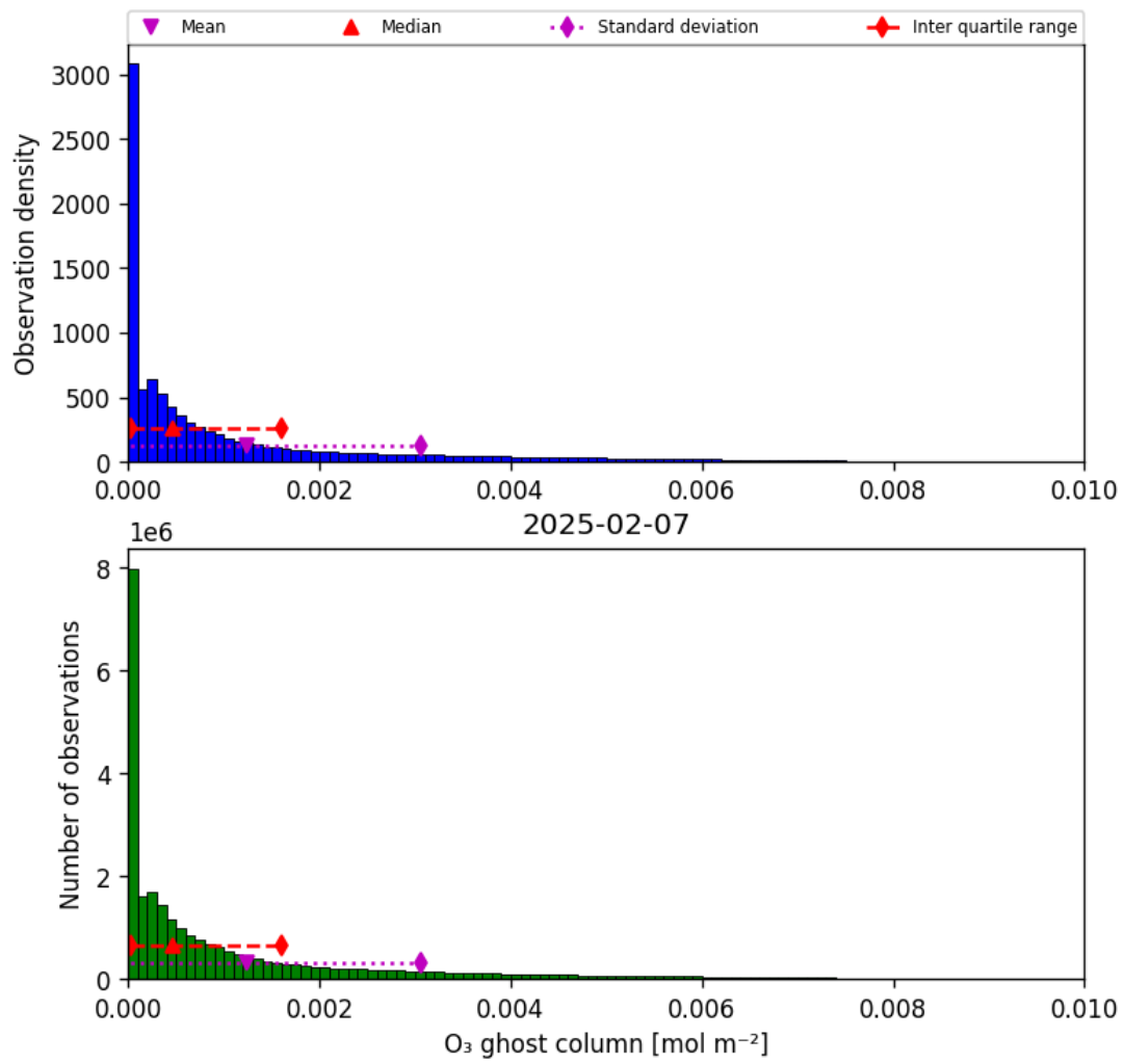
Figure 25: Histogram of “O 3 ghost column” for 2025-02-06 to 2025-02-08
