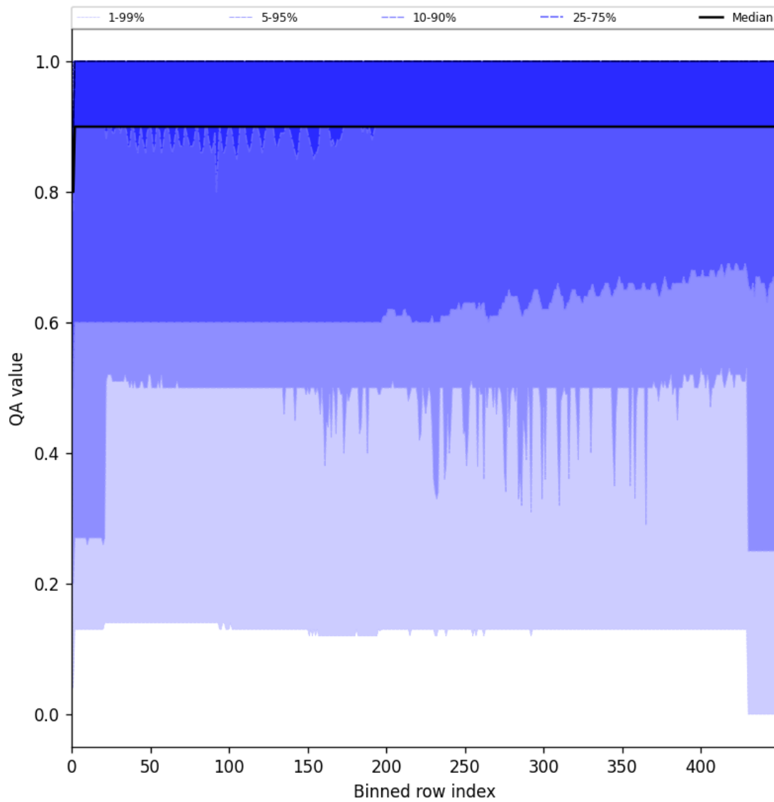
Figure 27: Along track statistics of “QA value” for 2025-02-06 to 2025-02-08
