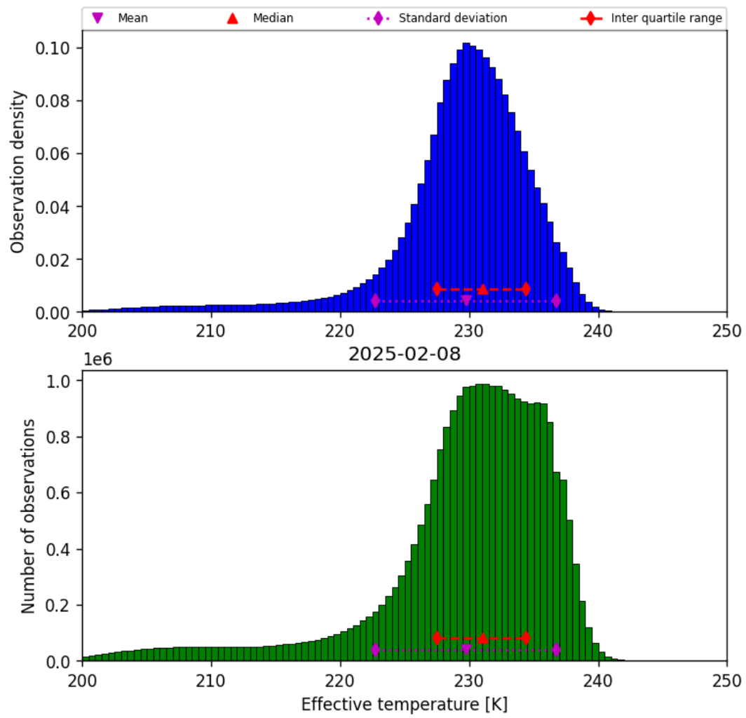
Figure 24: Histogram of “Effective temperature” for 2025-02-08 to 2025-02-09
