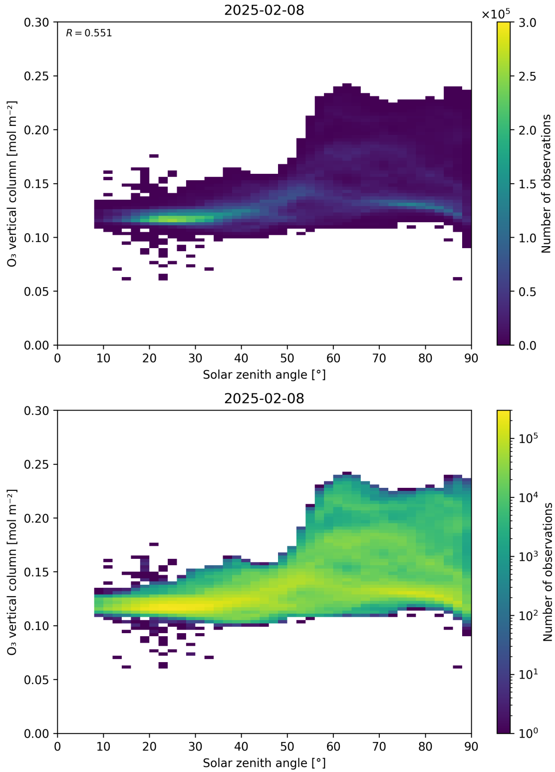
Figure 47: Scatter density plot of “Solar zenith angle” against “O 3 vertical column” for 2025-02-08 to 2025-02-09.
