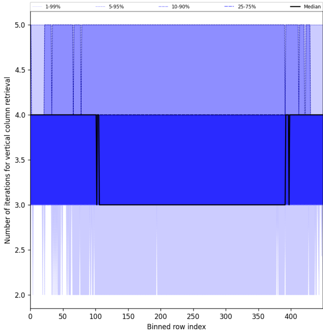
Figure 33: Along track statistics of “Number of iterations for vertical column retrieval” for 2025-02-08 to 2025-02-09
