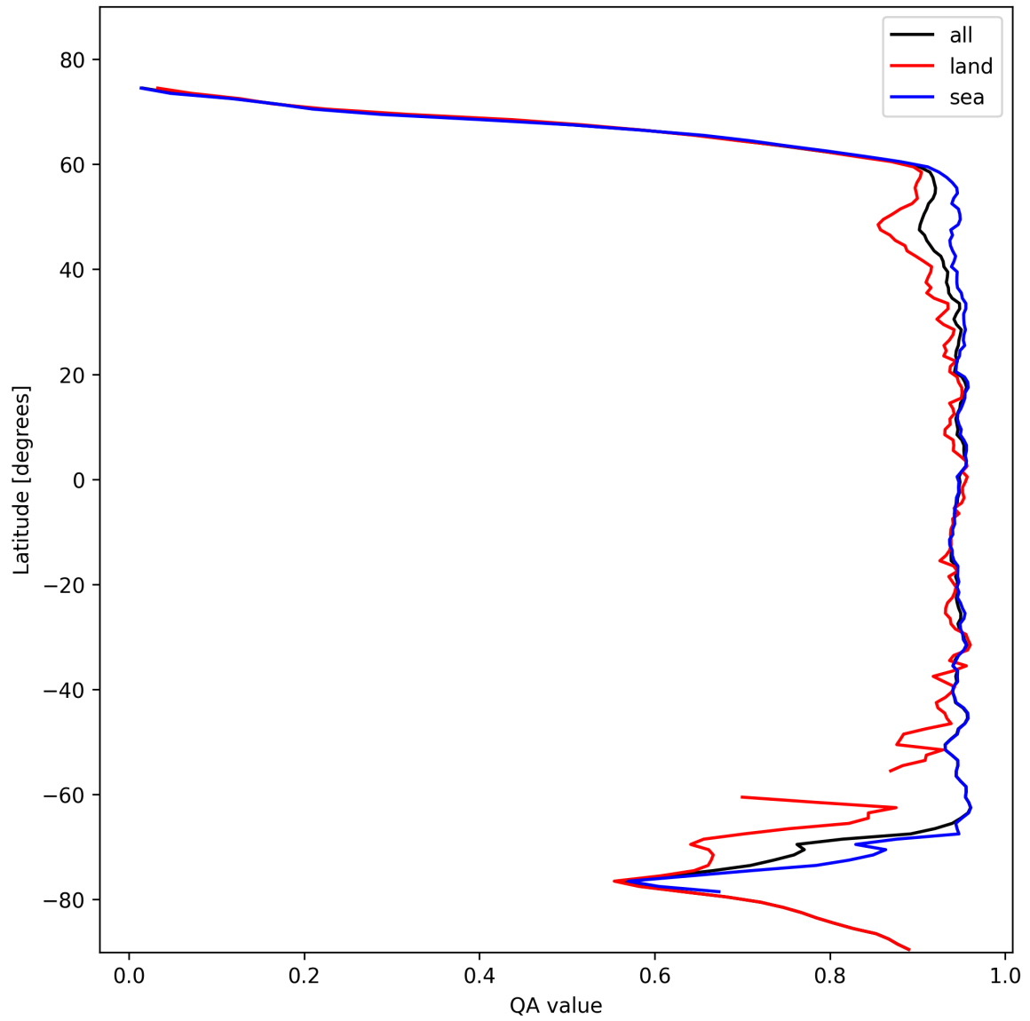
Figure 13: Zonal average of “QA value” for 2025-02-08 to 2025-02-09.
