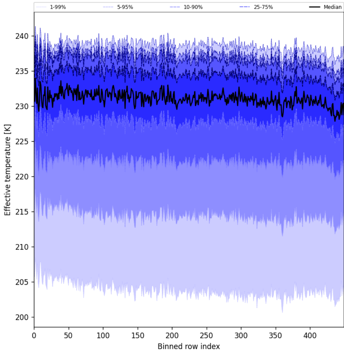
Figure 31: Along track statistics of "Effective temperature" for 2025-02-08 to 2025-02-09
