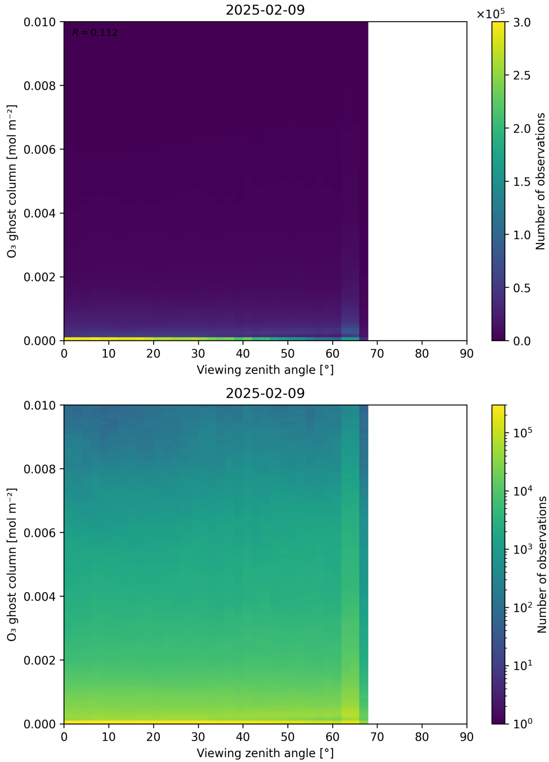
Figure 51: Scatter density plot of “Viewing zenith angle” against “O 3 ghost column” for 2025-02-08 to 2025-02-10.
