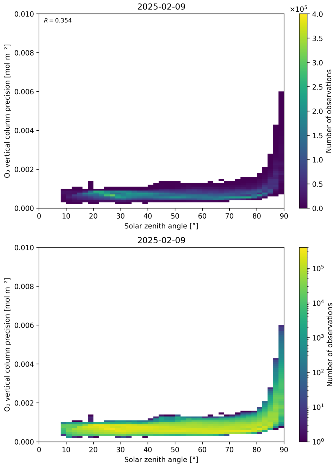
Figure 48: Scatter density plot of “Solar zenith angle” against “O 3 vertical column precision” for 2025-02-08 to 2025-02-10.
