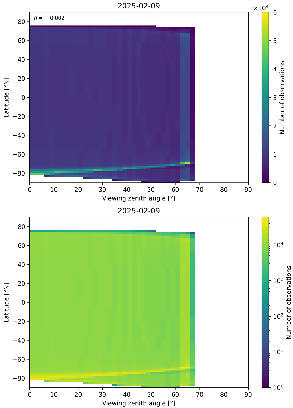
Figure 49: Scatter density plot of “Viewing zenith angle” against “Latitude” for 2025-02-08 to 2025-02-10.
