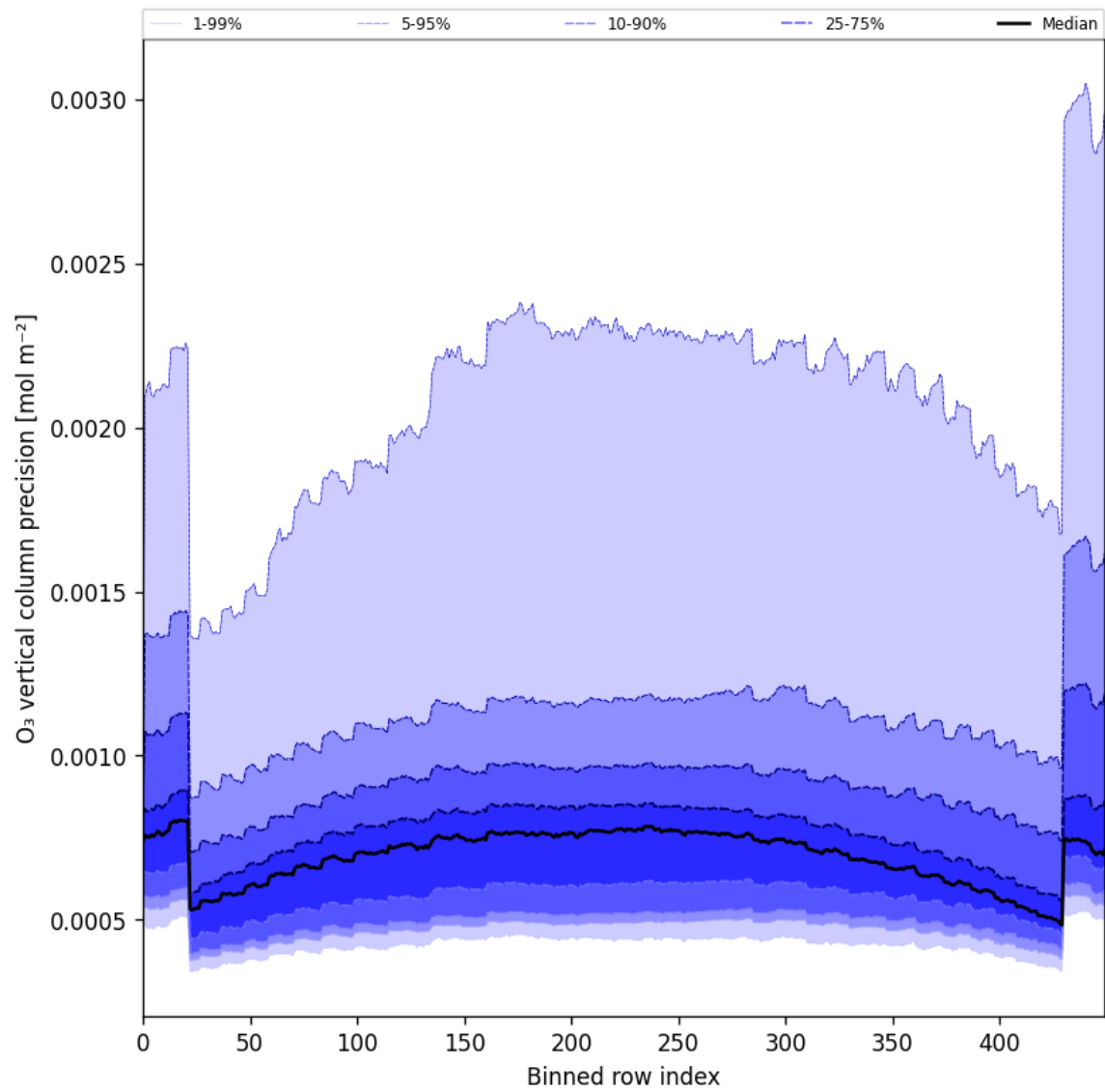
Figure 29: Along track statistics of “O 3 vertical column precision” for 2025-02-08 to 2025-02-10
