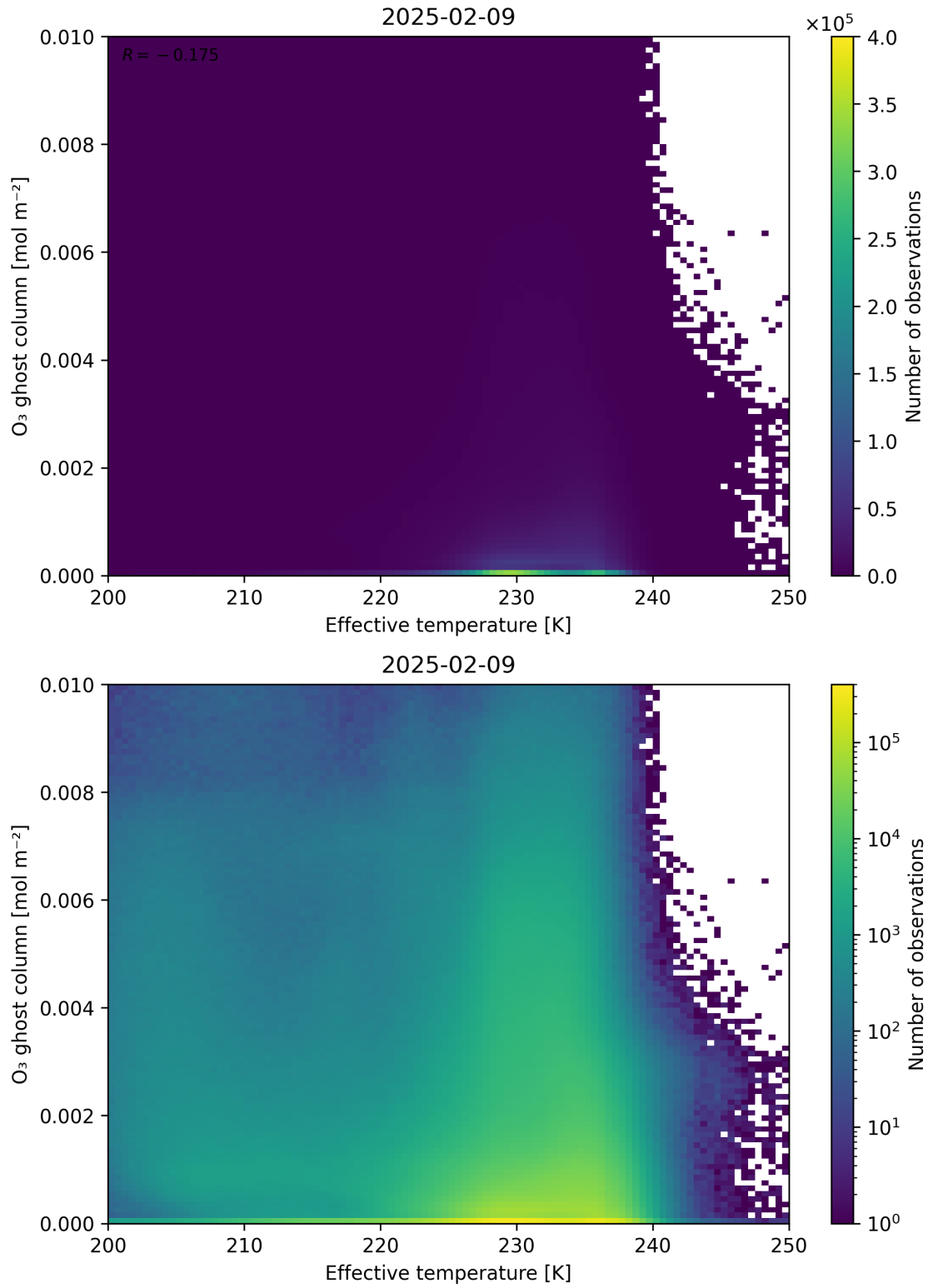
Figure 38: Scatter density plot of “Effective temperature” against “O 3 ghost column” for 2025-02-08 to 2025-02-10.
