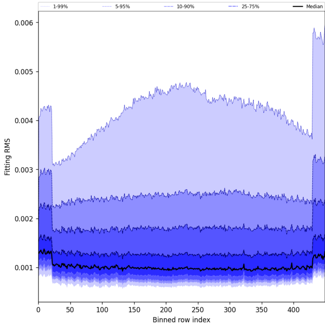
Figure 30: Along track statistics of “Fitting RMS” for 2025-02-08 to 2025-02-10
