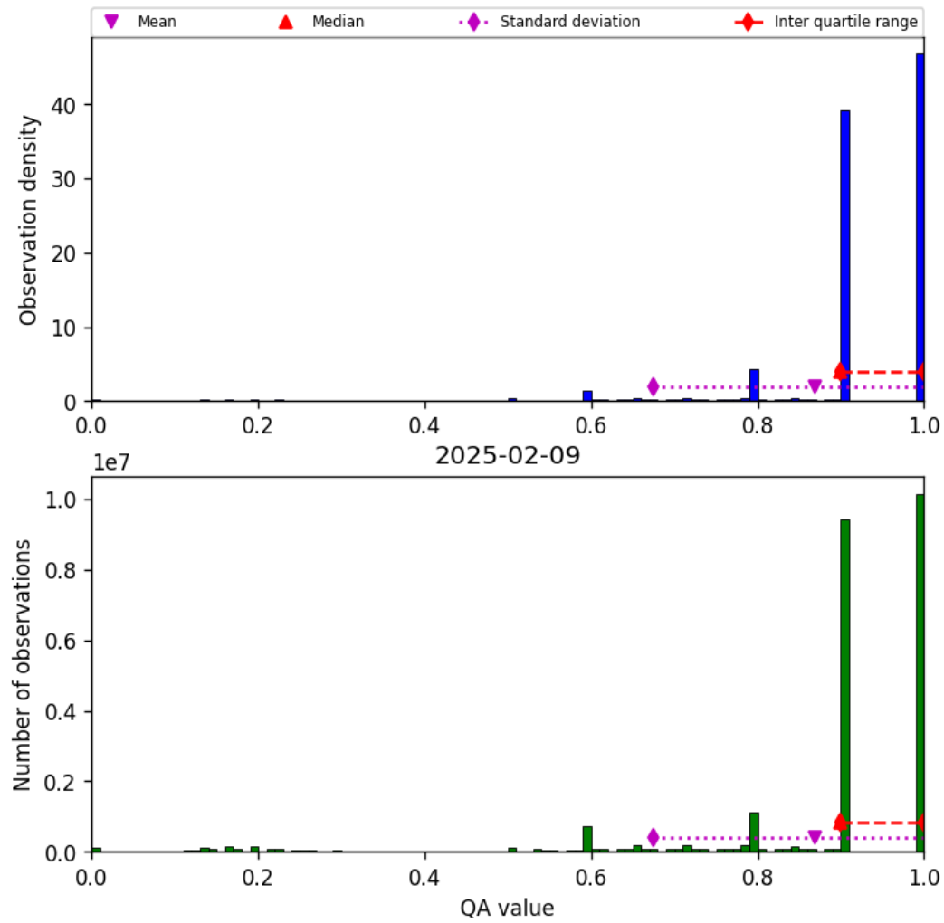
Figure 20: Histogram of “QA value” for 2025-02-08 to 2025-02-10
