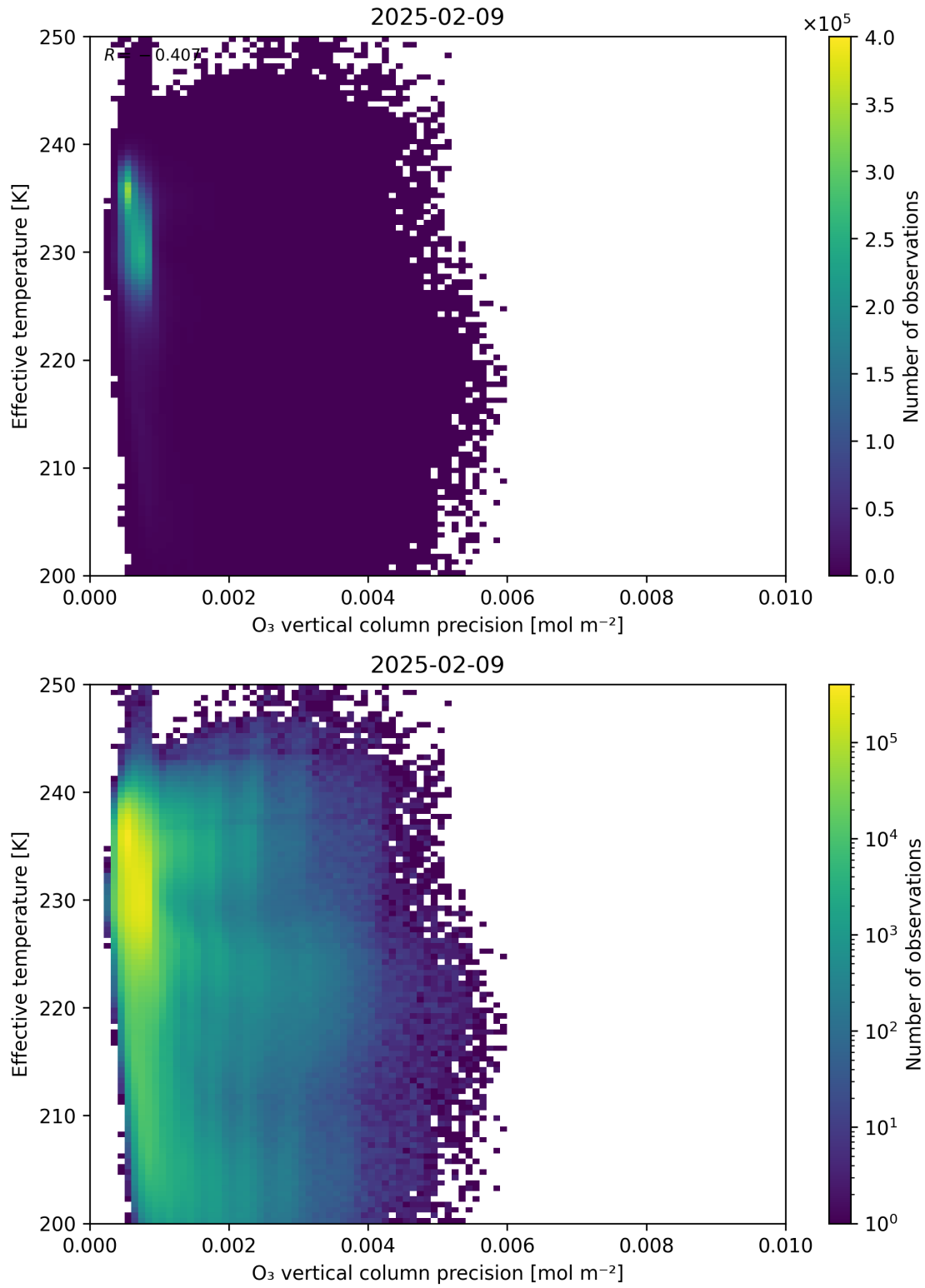
Figure 42: Scatter density plot of “O 3 vertical column precision” against “Effective temperature” for 2025-02-08 to 2025-02-10.
