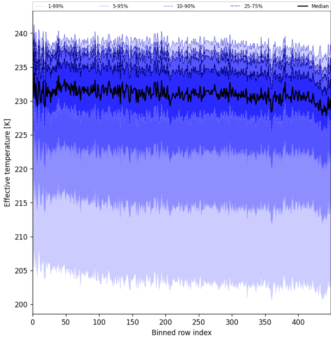
Figure 31: Along track statistics of “Effective temperature” for 2025-02-08 to 2025-02-10
