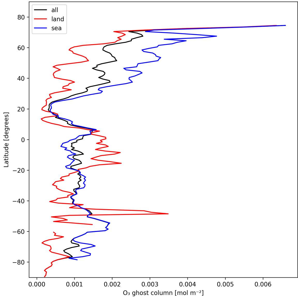
Figure 18: Zonal average of "O 3 ghost column" for 2025-02-08 to 2025-02-10.
