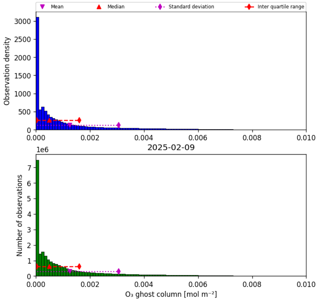
Figure 25: Histogram of "O 3 ghost column" for 2025-02-08 to 2025-02-10
