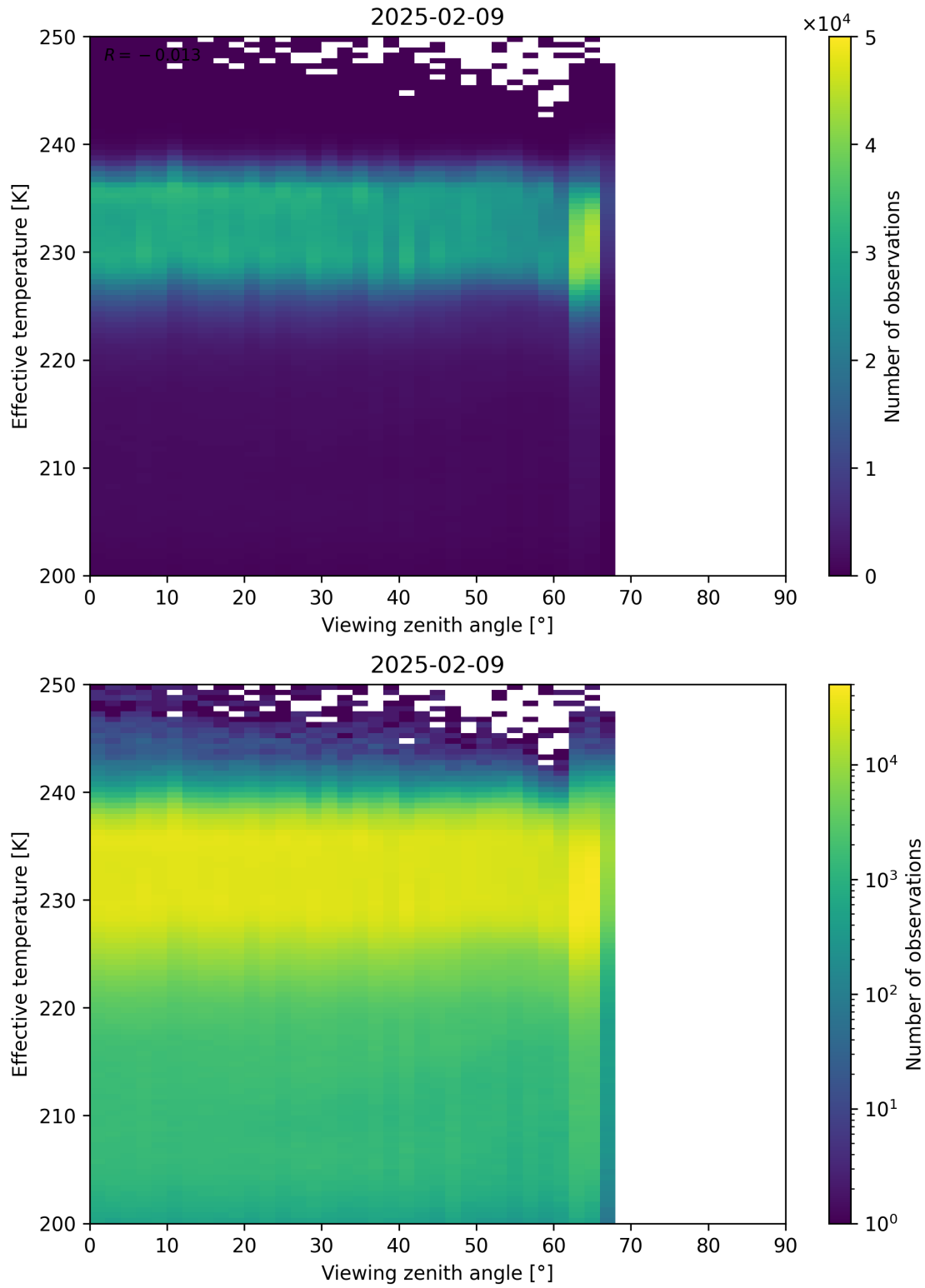
Figure 50: Scatter density plot of “Viewing zenith angle” against “Effective temperature” for 2025-02-08 to 2025-02-10.
