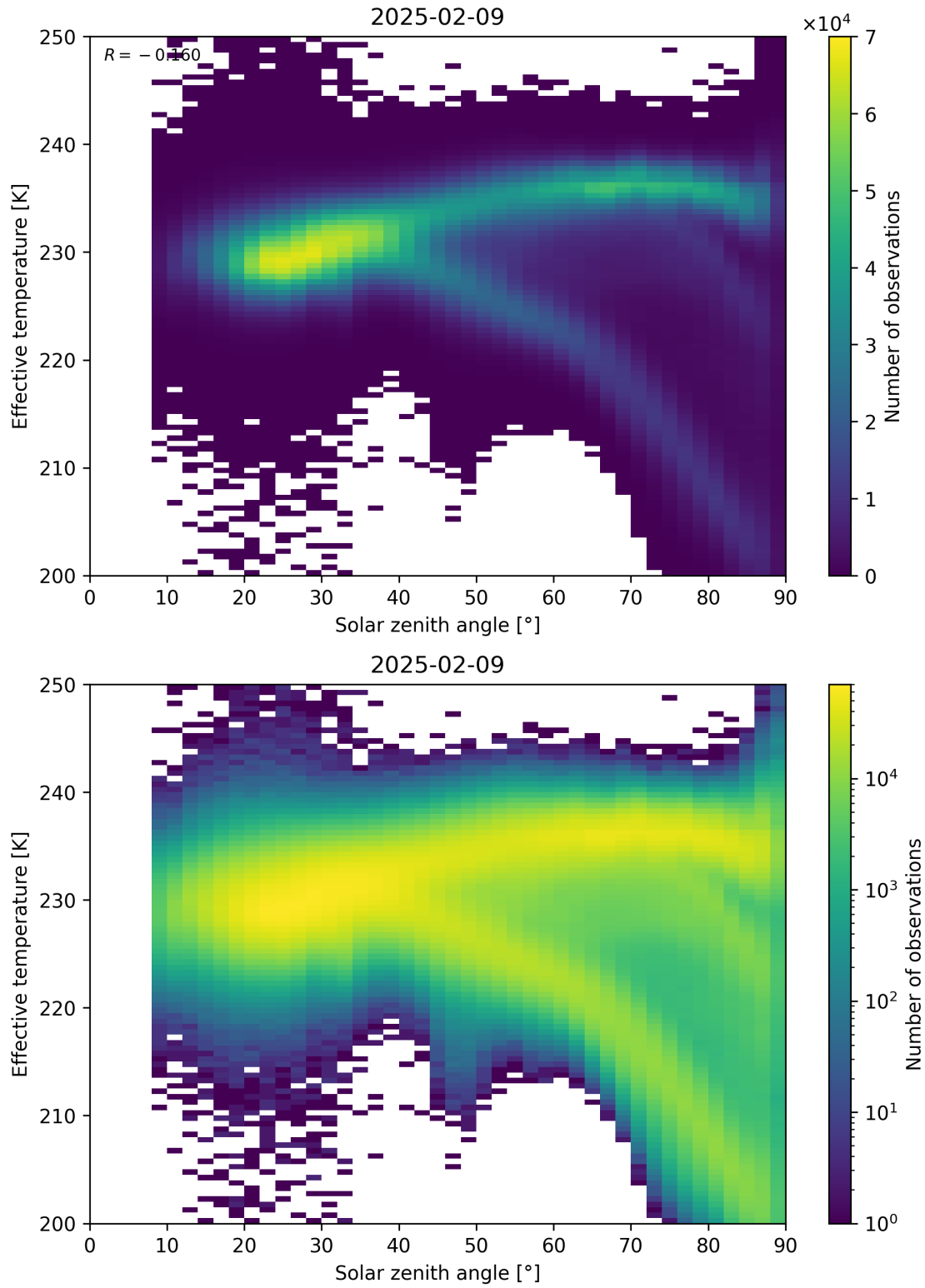
Figure 45: Scatter density plot of “Solar zenith angle” against “Effective temperature” for 2025-02-08 to 2025-02-10.
