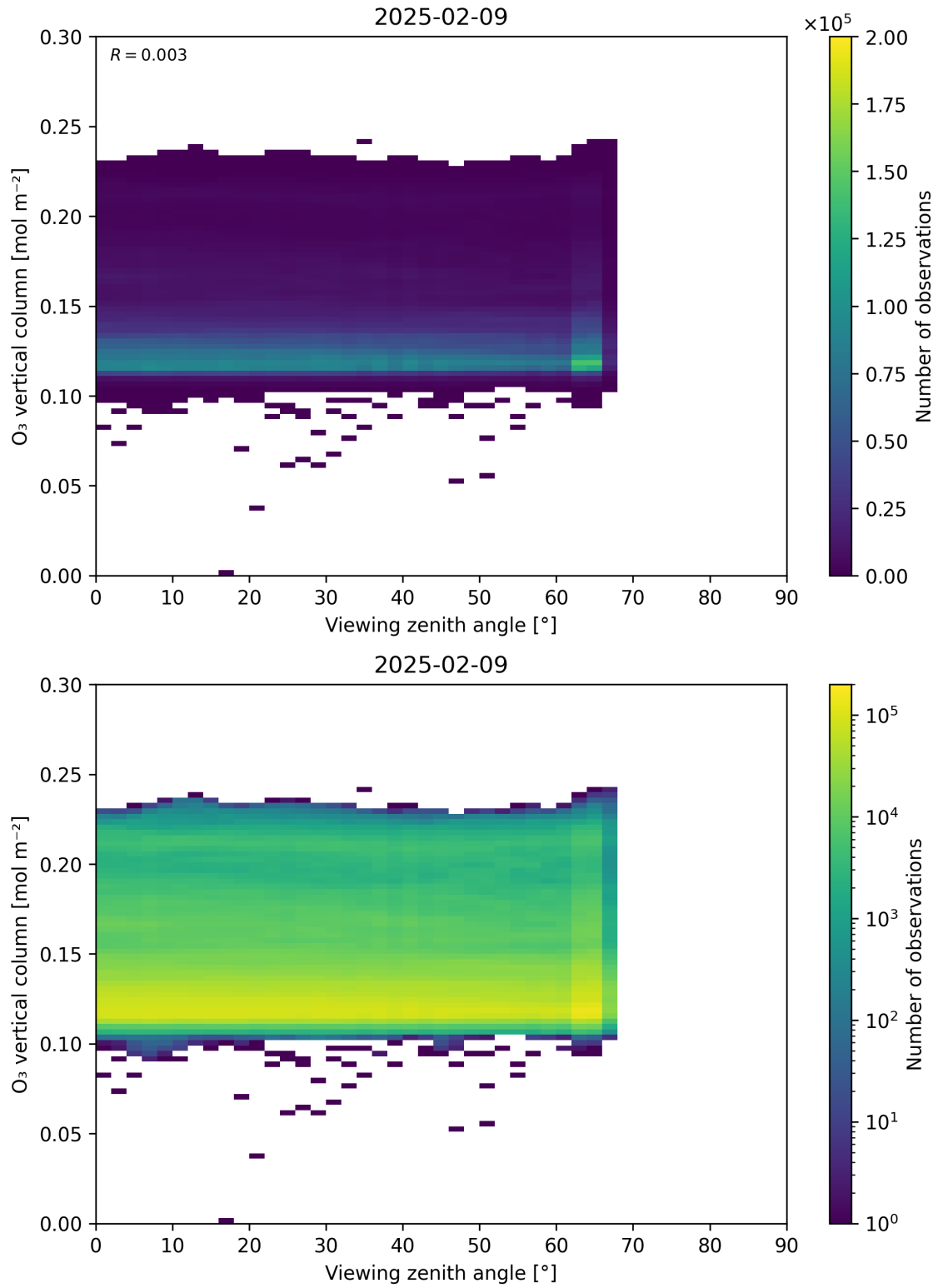
Figure 52: Scatter density plot of “Viewing zenith angle” against “O 3 vertical column” for 2025-02-08 to 2025-02-10.
