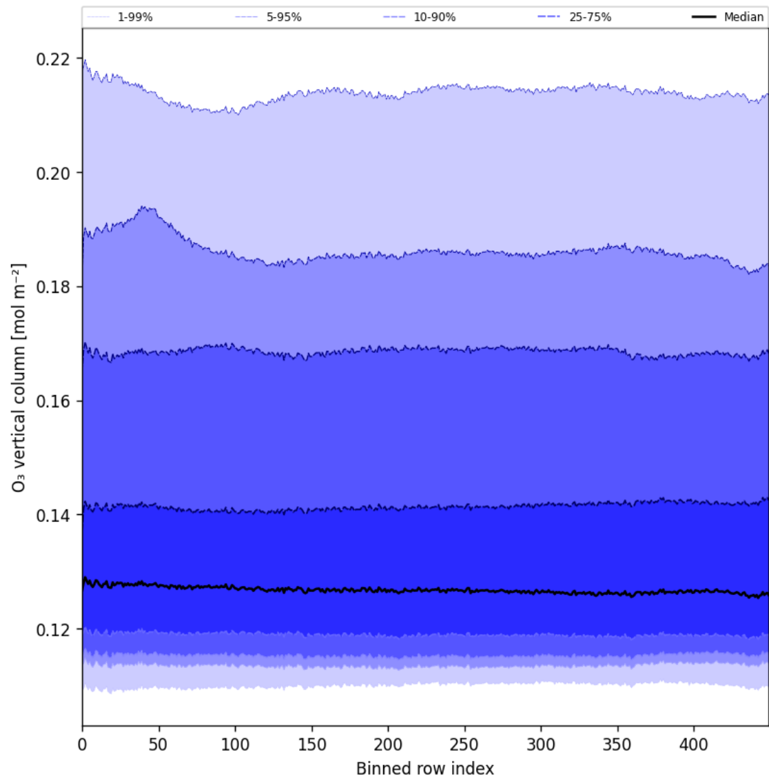
Figure 28: Along track statistics of “O 3 vertical column” for 2025-02-08 to 2025-02-10
