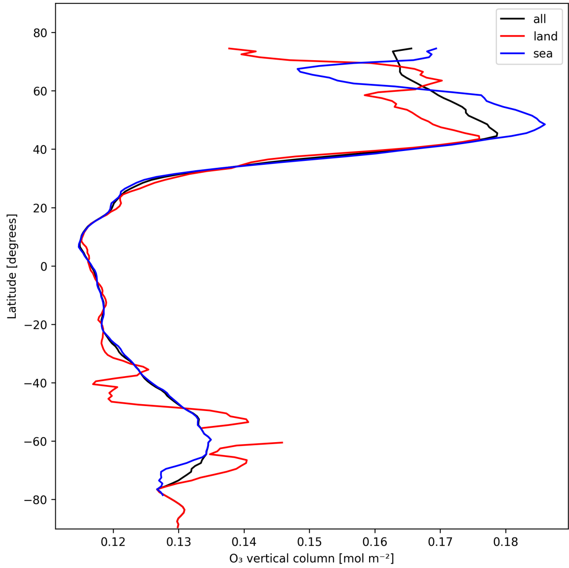
Figure 14: Zonal average of “O 3 vertical column” for 2025-02-08 to 2025-02-10.
