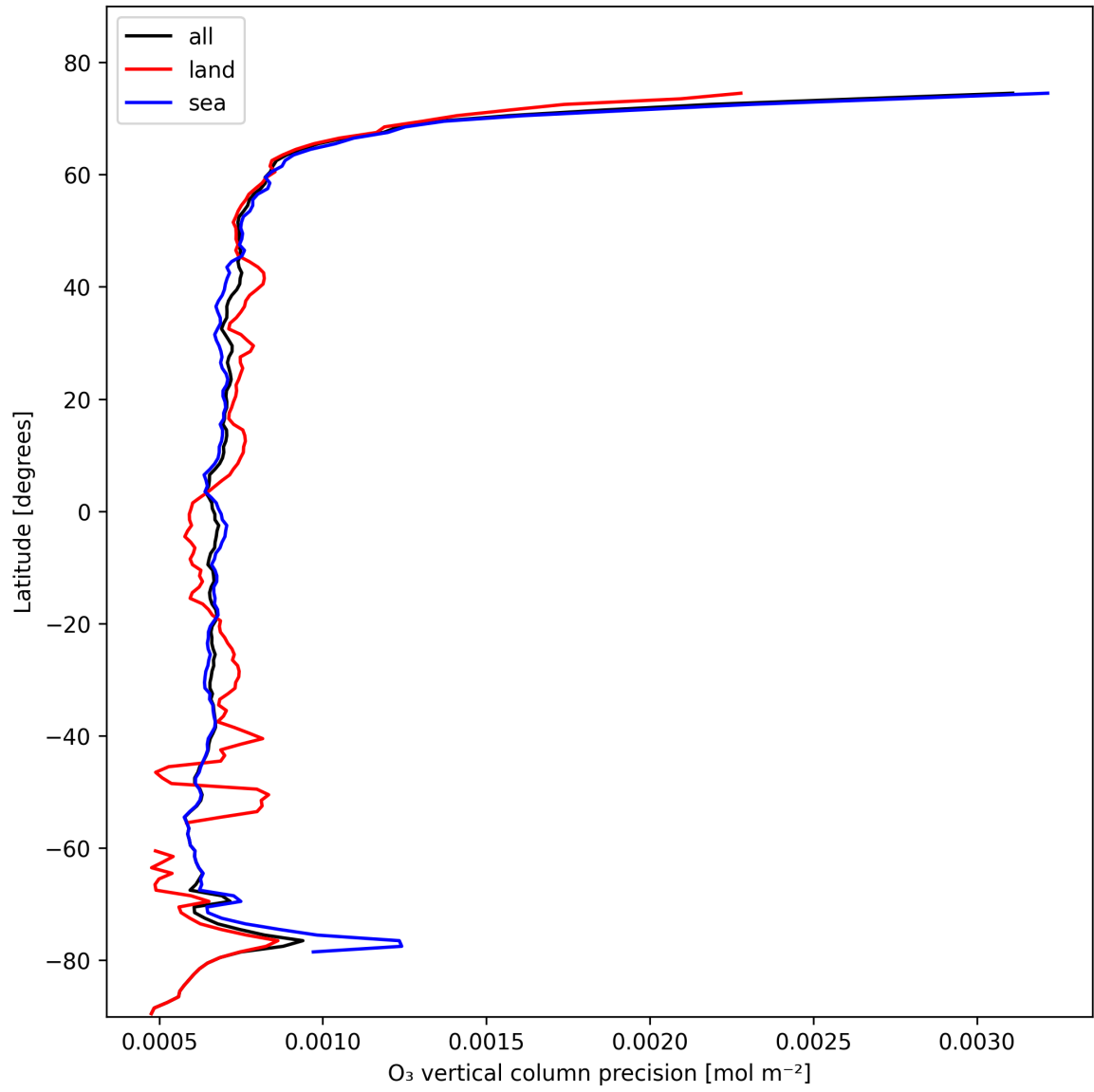
Figure 15: Zonal average of “O 3 vertical column precision” for 2025-02-08 to 2025-02-10.
