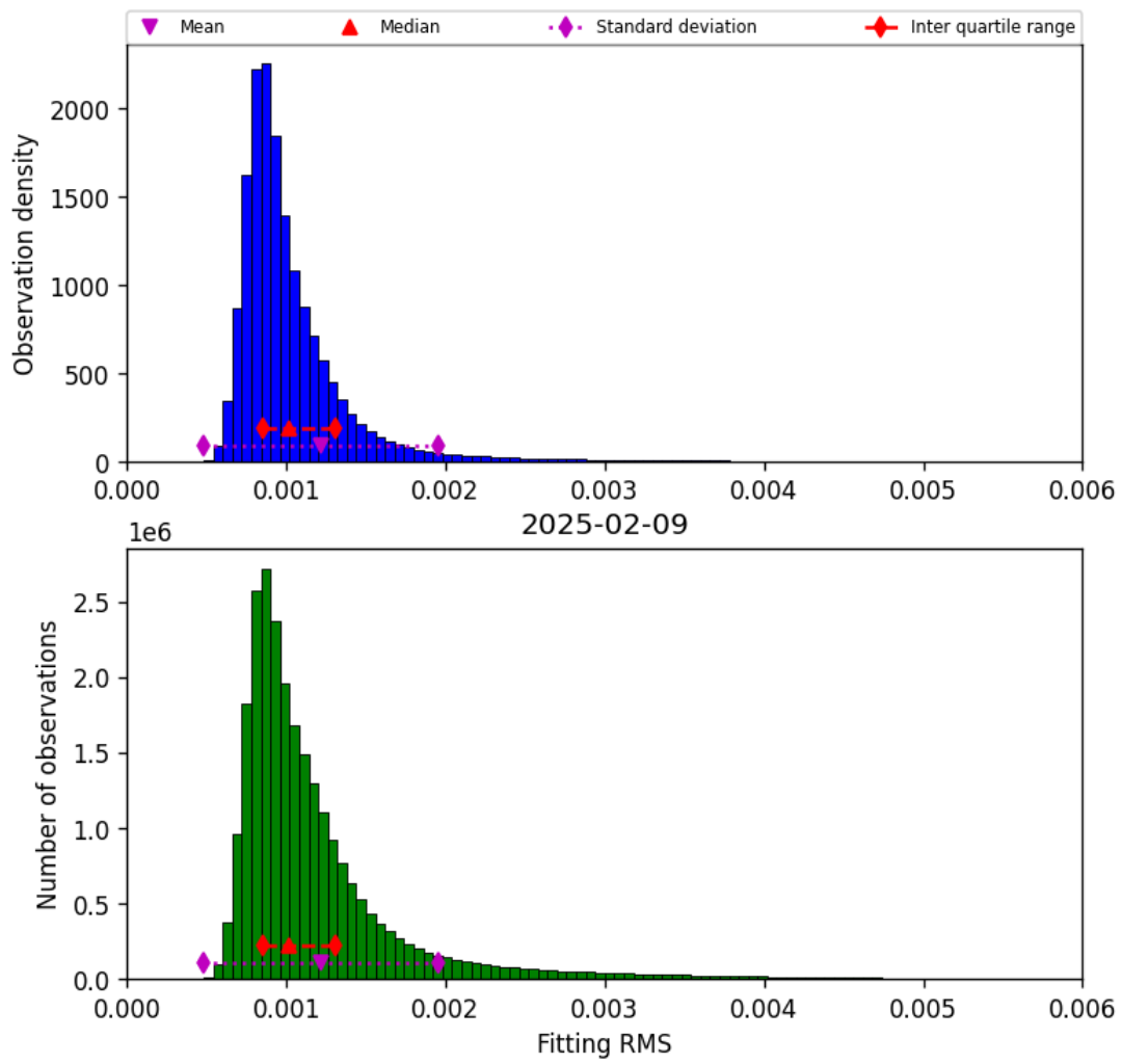
Figure 23: Histogram of “Fitting RMS” for 2025-02-08 to 2025-02-10
