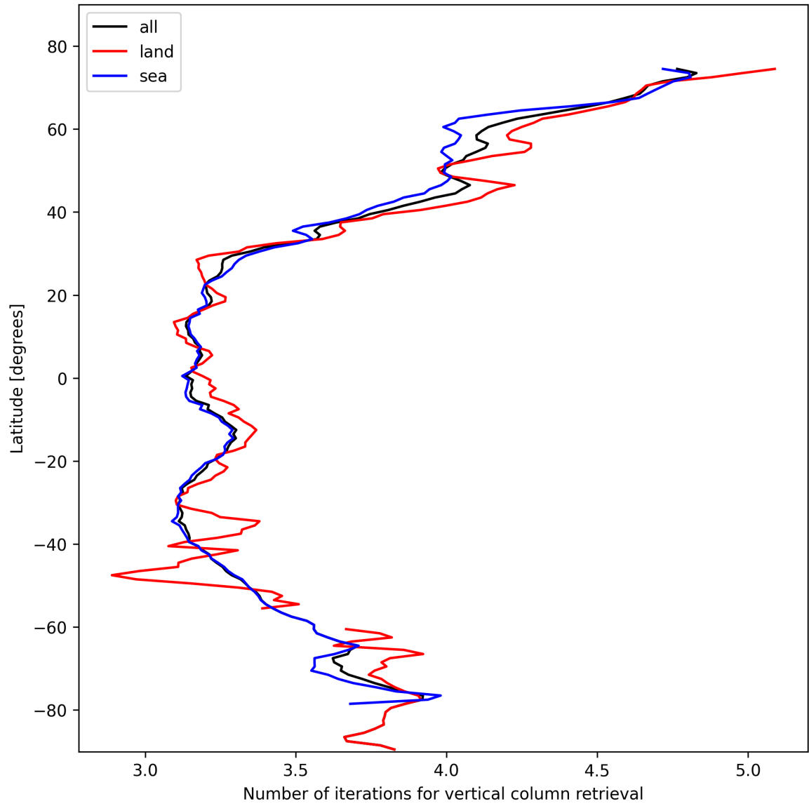
Figure 19: Zonal average of “Number of iterations for vertical column retrieval” for 2025-02-08 to 2025-02-10.
