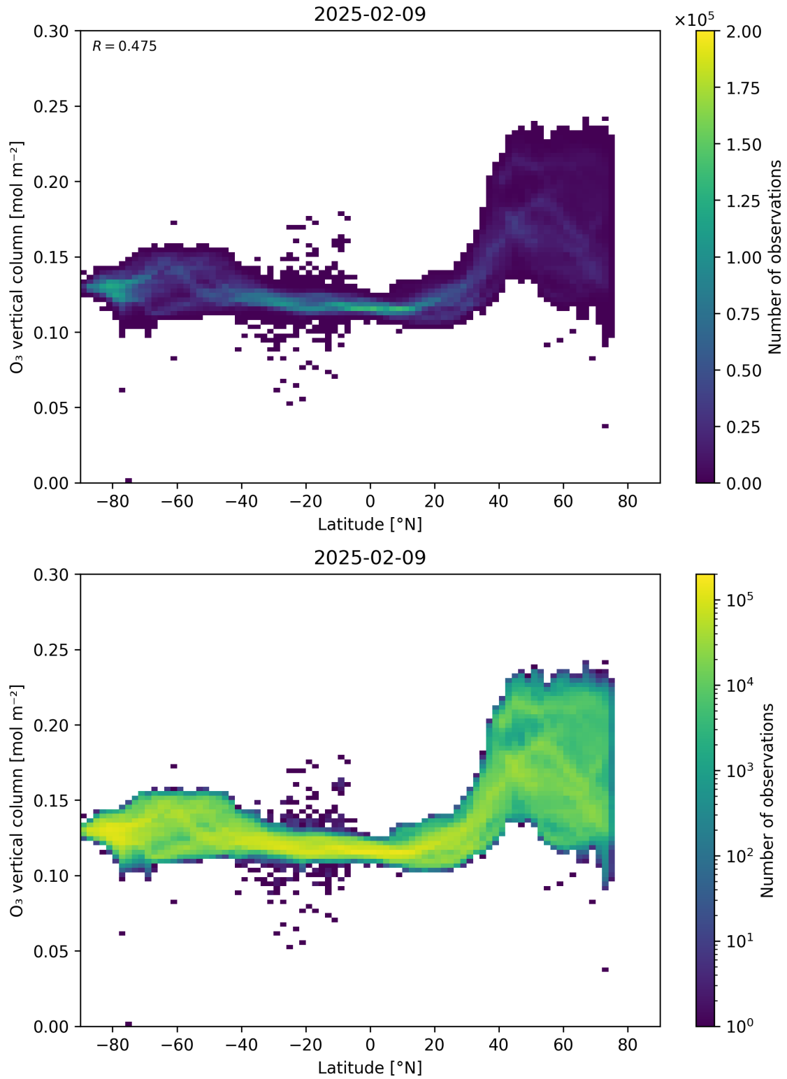
Figure 36: Scatter density plot of “Latitude” against “O 3 vertical column” for 2025-02-08 to 2025-02-10.
