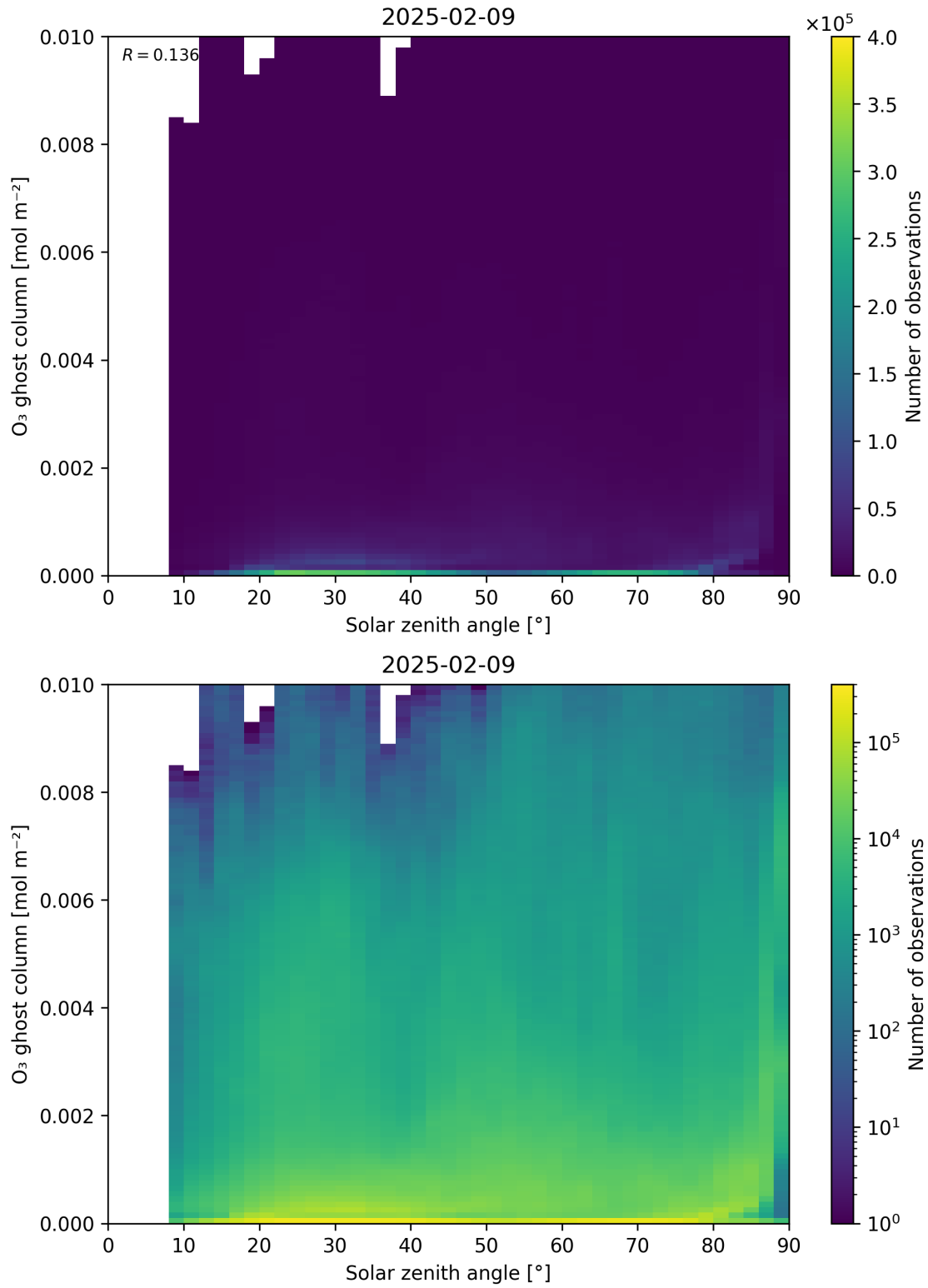
Figure 46: Scatter density plot of “Solar zenith angle” against “O 3 ghost column” for 2025-02-08 to 2025-02-10.
