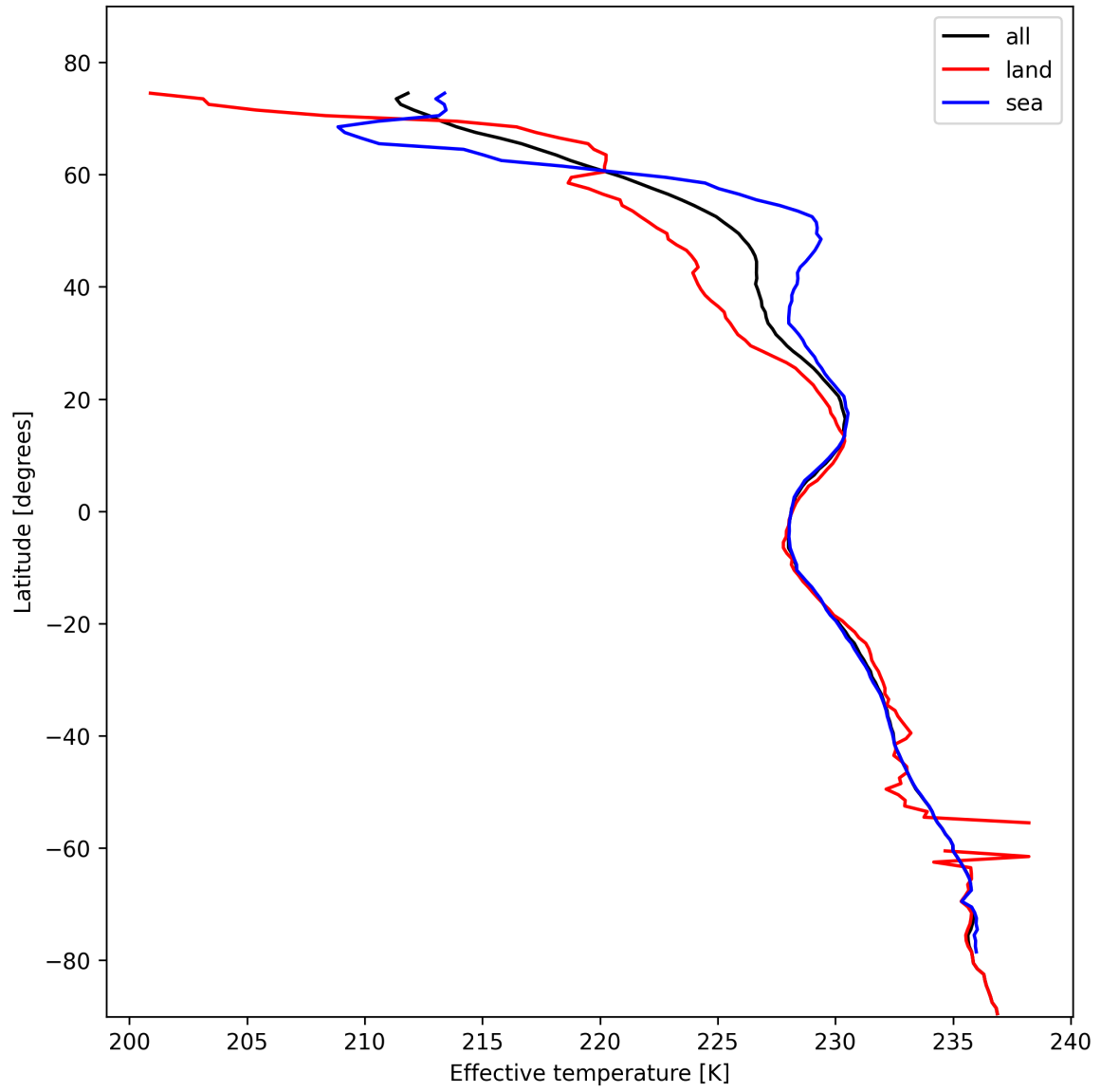
Figure 17: Zonal average of “Effective temperature” for 2025-02-08 to 2025-02-10.
