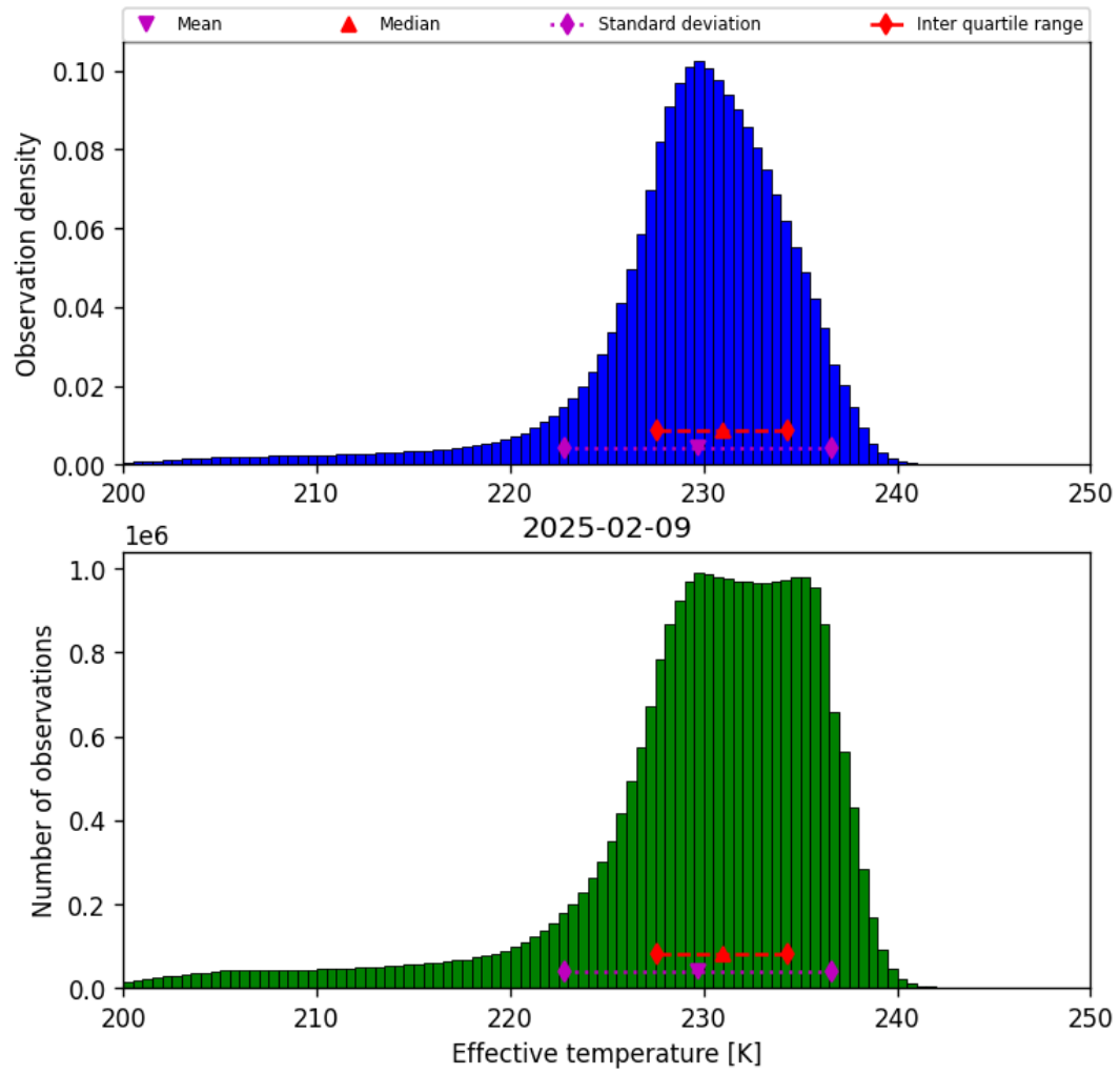
Figure 24: Histogram of “Effective temperature” for 2025-02-08 to 2025-02-10
