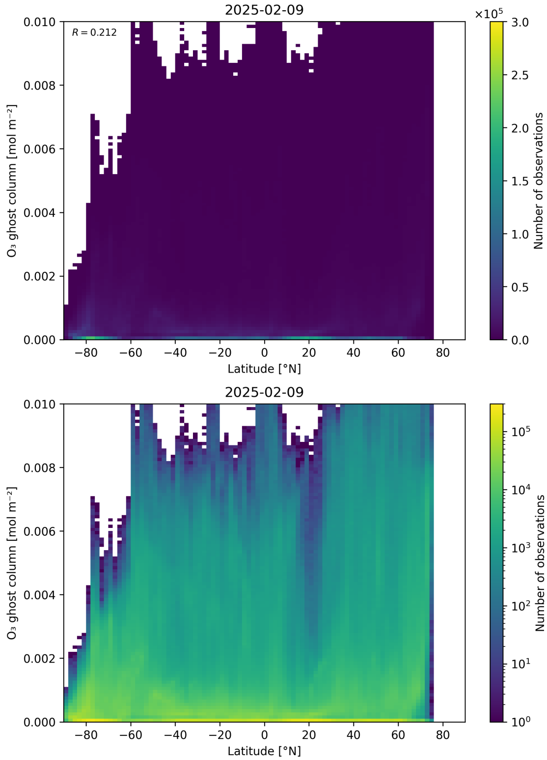
Figure 35: Scatter density plot of “Latitude” against “O 3 ghost column” for 2025-02-08 to 2025-02-10.
