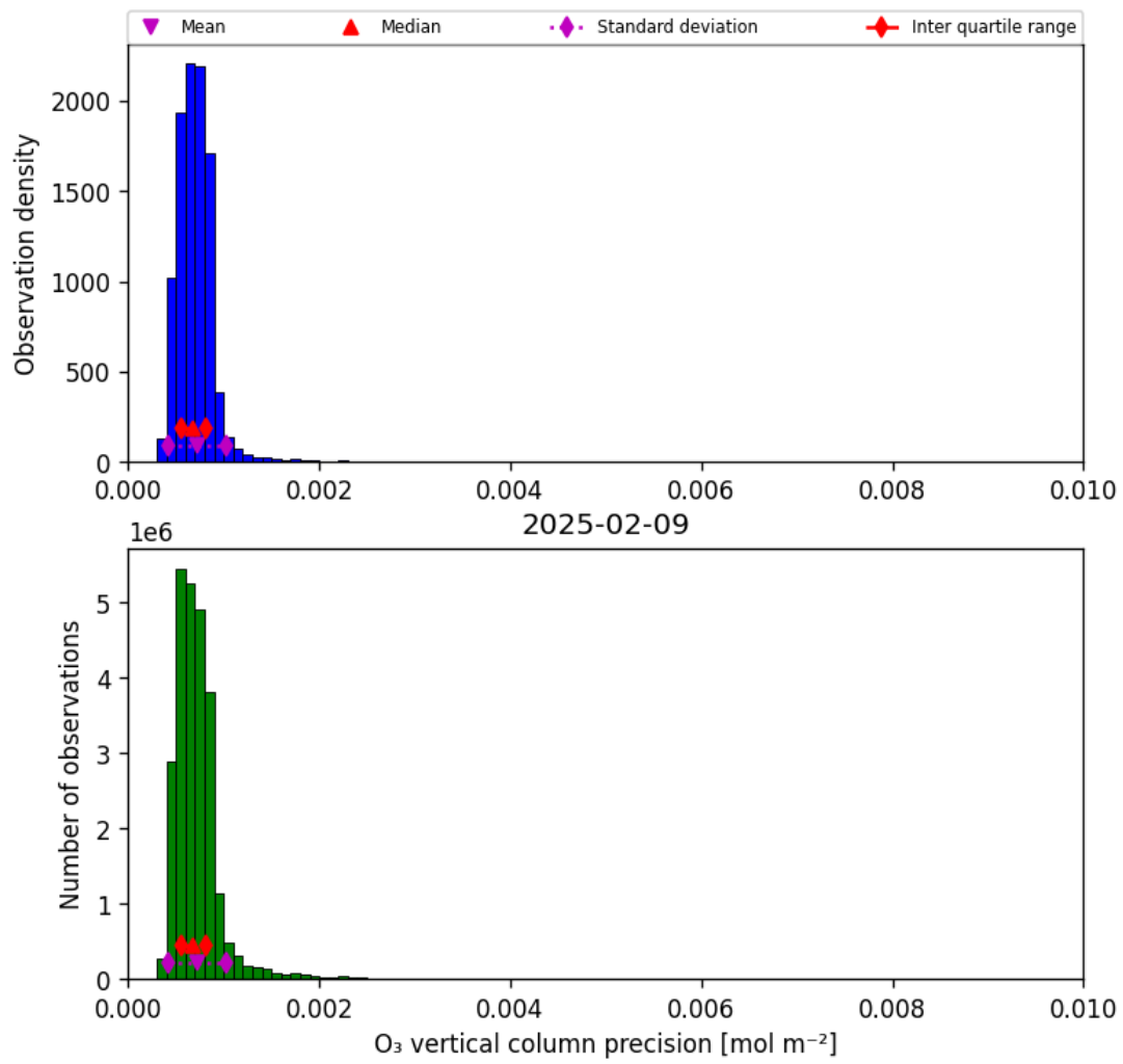
Figure 22: Histogram of “O 3 vertical column precision” for 2025-02-08 to 2025-02-10
