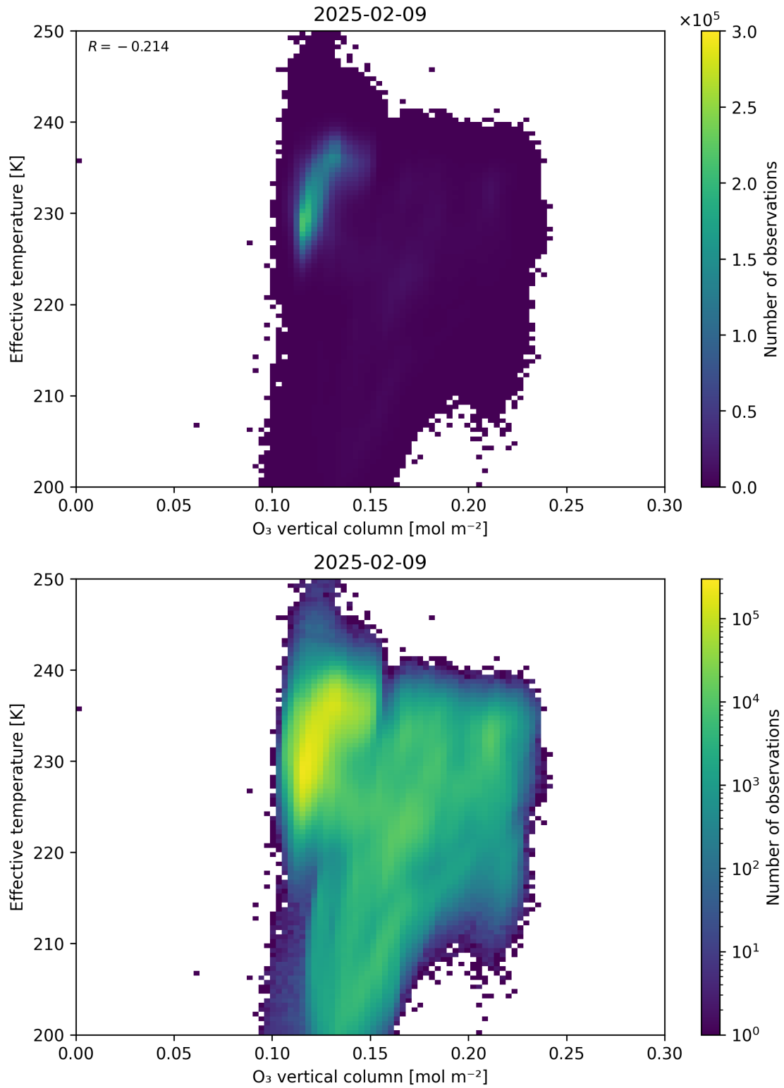
Figure 39: Scatter density plot of “O 3 vertical column” against “Effective temperature” for 2025-02-08 to 2025-02-10.
