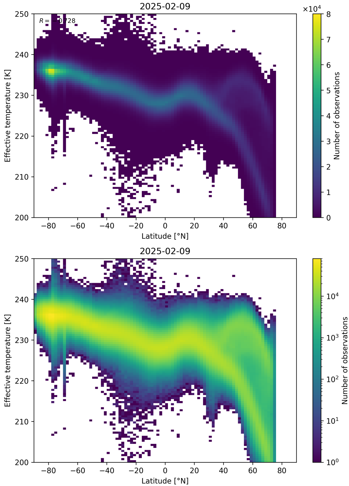
Figure 34: Scatter density plot of “Latitude” against “Effective temperature” for 2025-02-08 to 2025-02-10.
