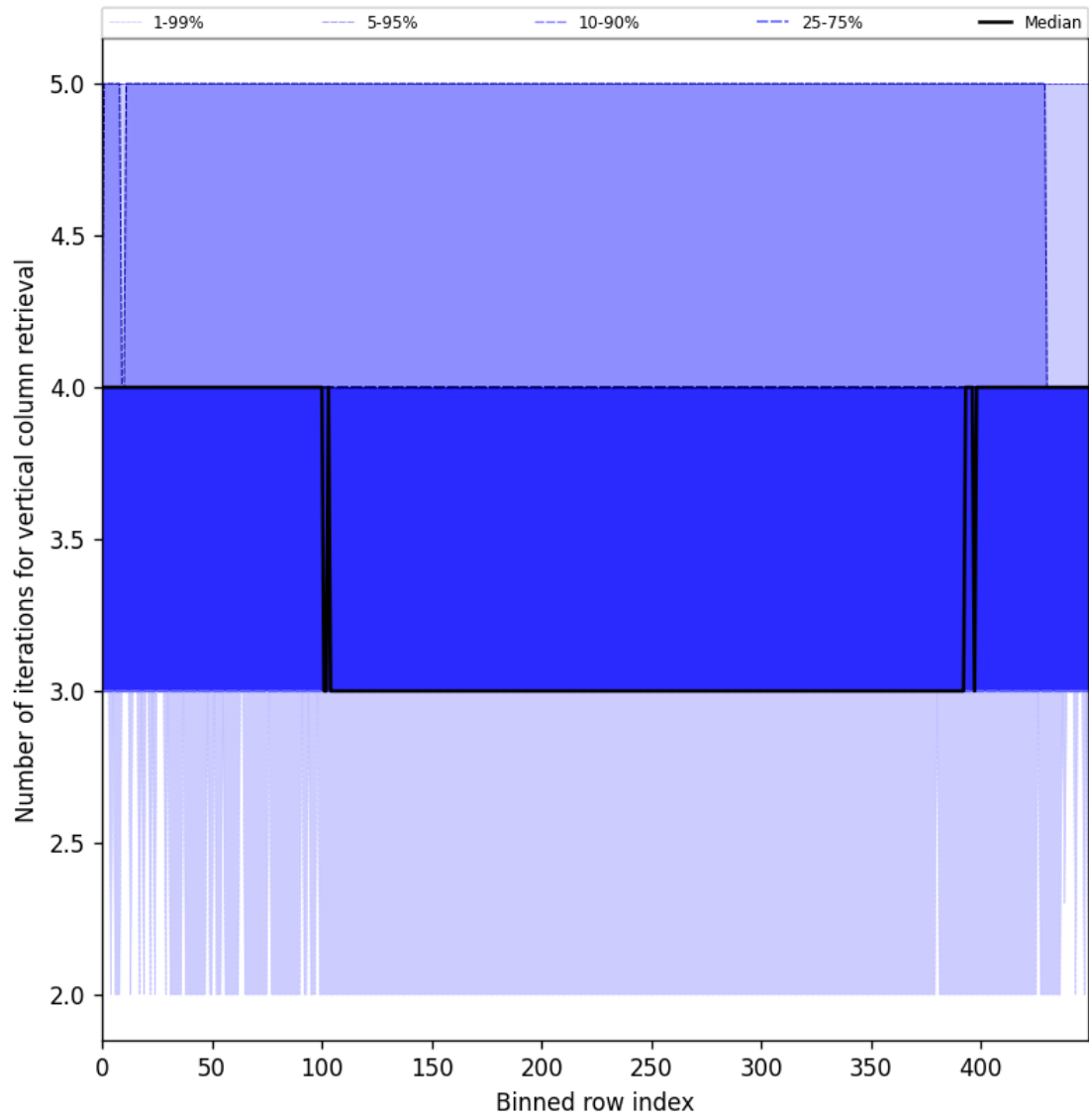
Figure 33: Along track statistics of “Number of iterations for vertical column retrieval” for 2025-02-08 to 2025-02-10
