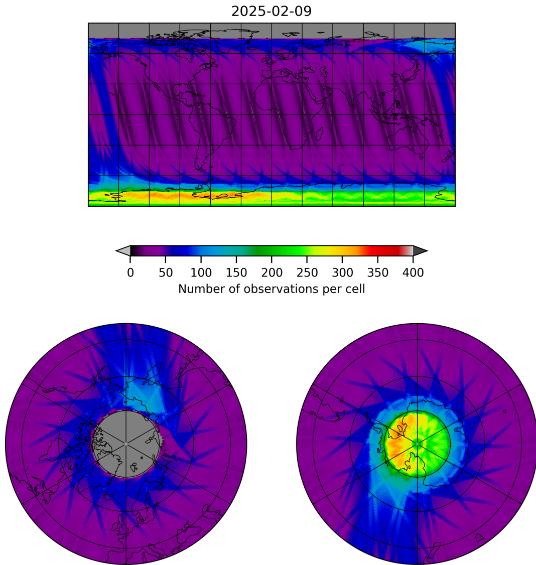
Figure 12: Map of the number of observations for 2025-02-08 to 2025-02-10
