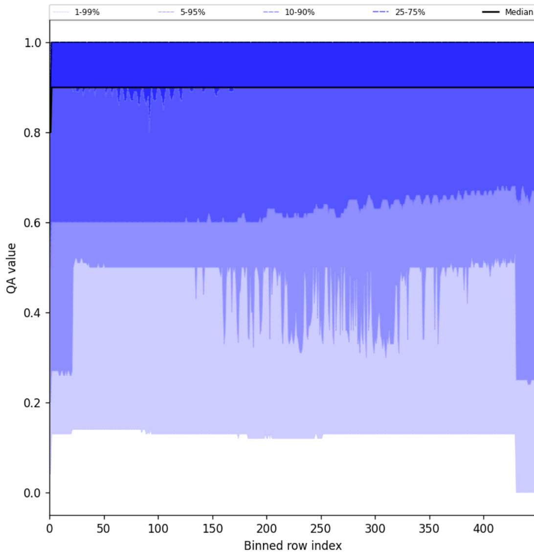
Figure 27: Along track statistics of “QA value” for 2025-02-08 to 2025-02-10
