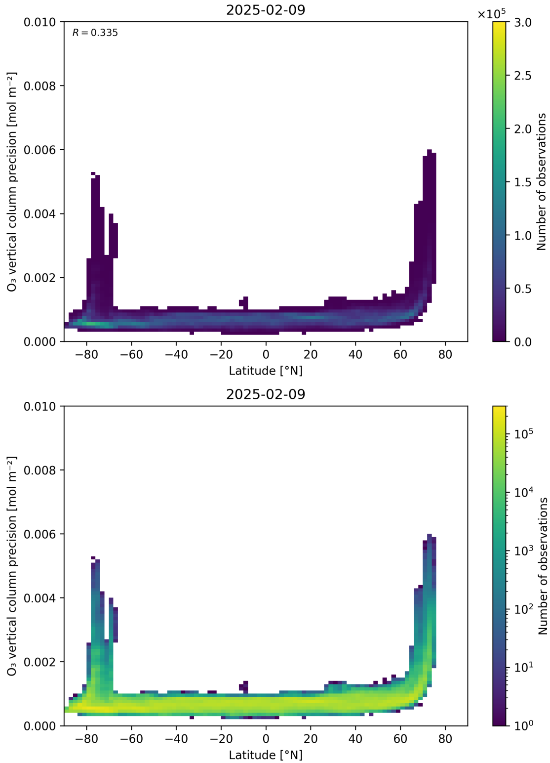
Figure 37: Scatter density plot of “Latitude” against “O 3 vertical column precision” for 2025-02-08 to 2025-02-10.
