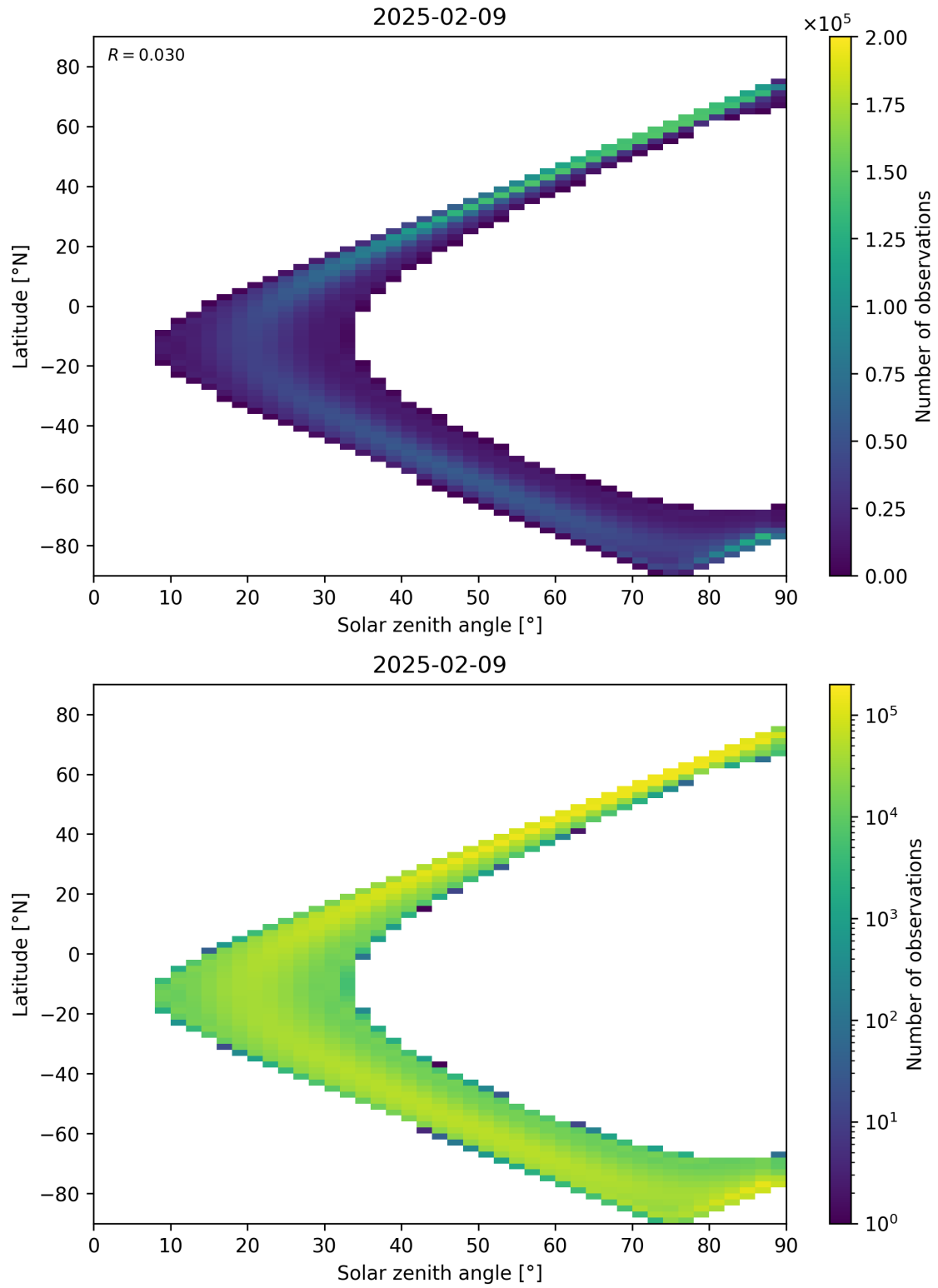
Figure 44: Scatter density plot of “Solar zenith angle” against “Latitude” for 2025-02-08 to 2025-02-10.
