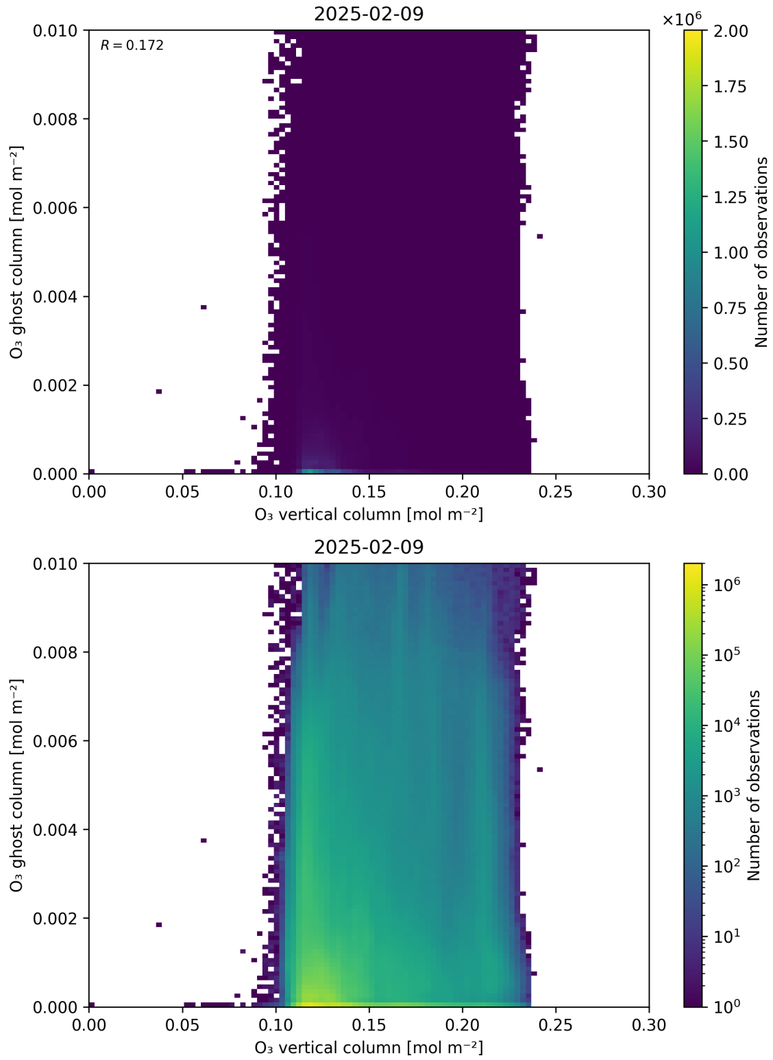
Figure 40: Scatter density plot of “O 3 vertical column” against “O 3 ghost column” for 2025-02-08 to 2025-02-10.
