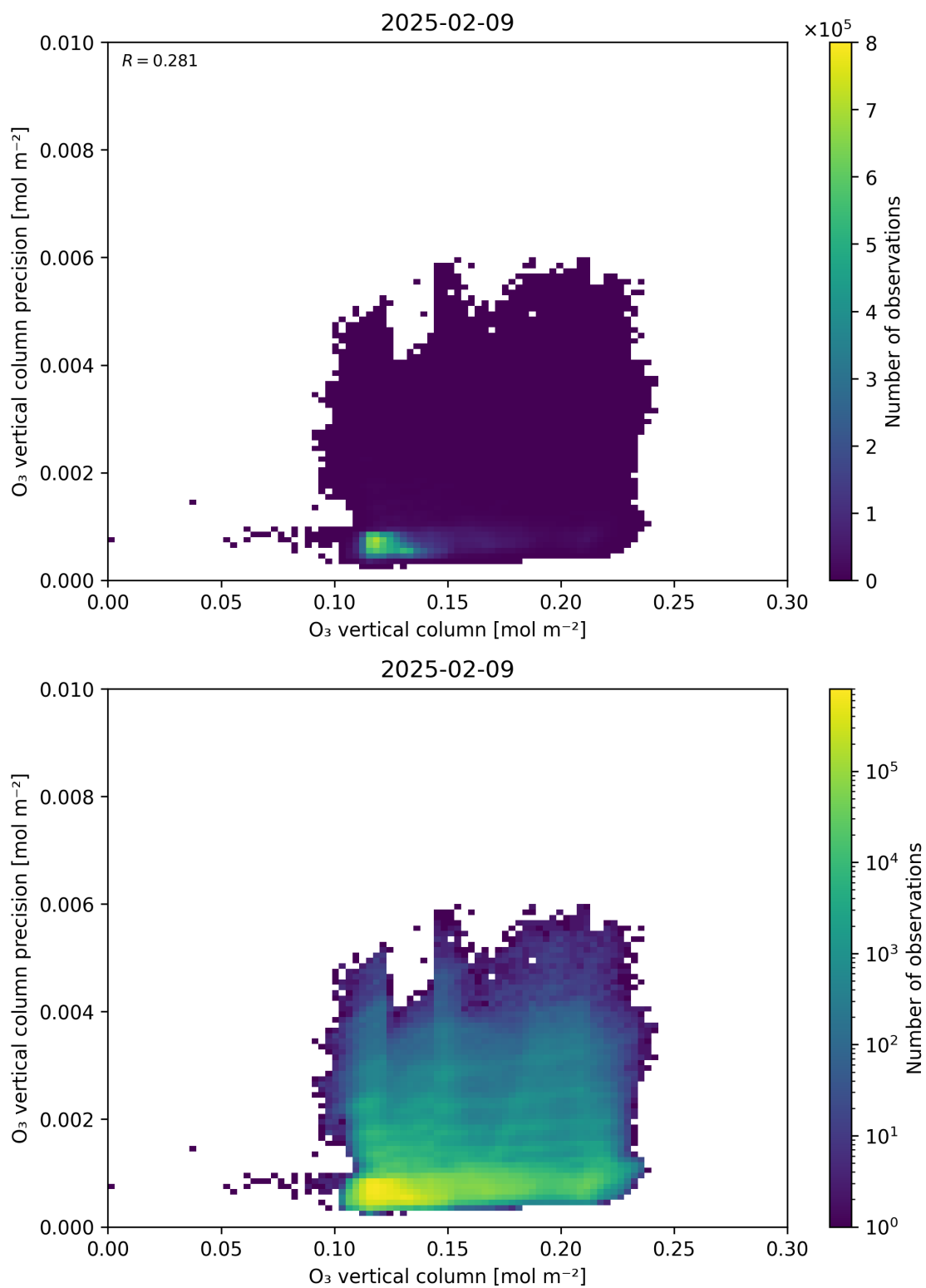
Figure 41: Scatter density plot of “O 3 vertical column” against “O 3 vertical column precision” for 2025-02-08 to 2025-02-10.
