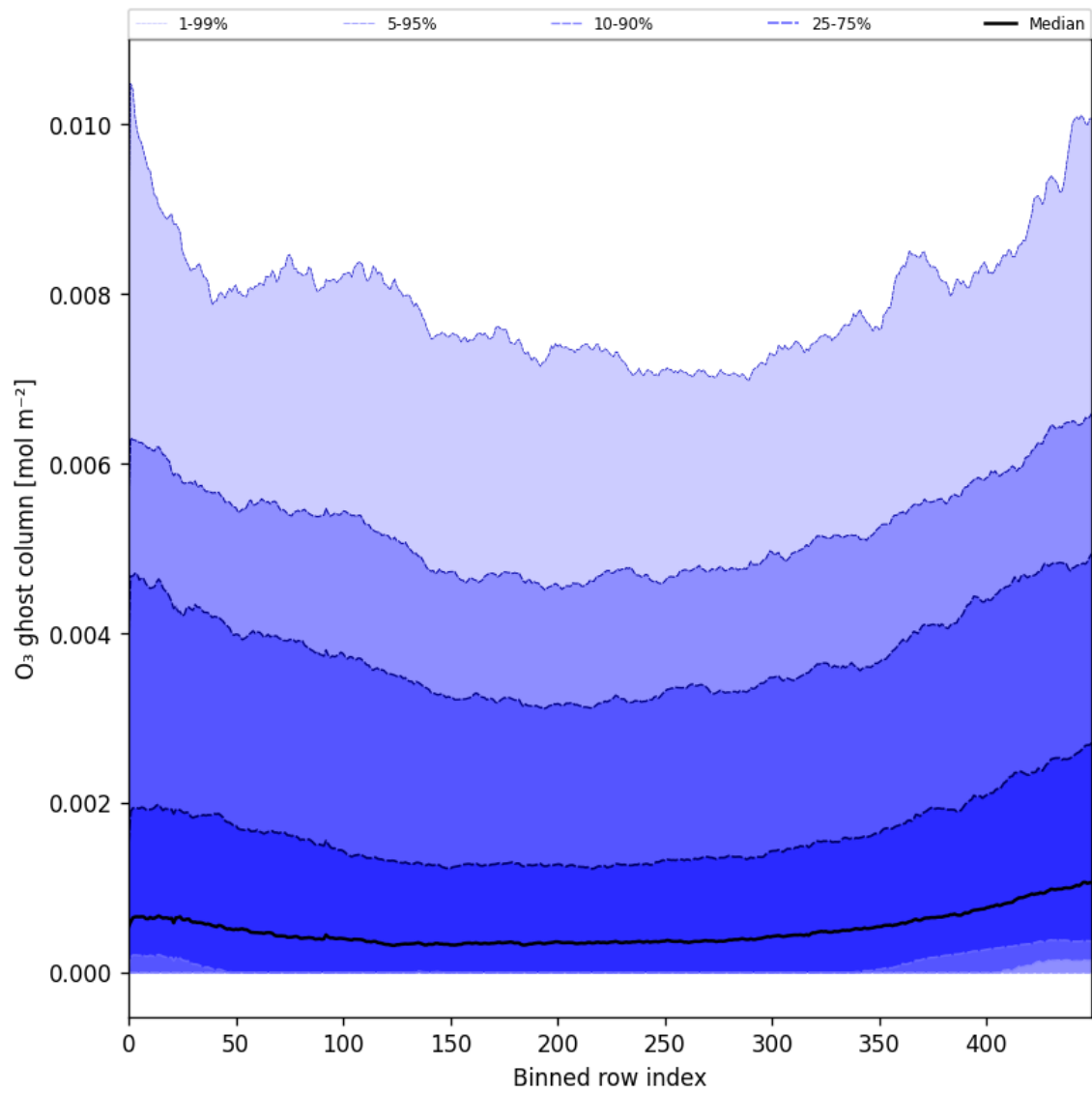
Figure 32: Along track statistics of “O 3 ghost column” for 2025-02-08 to 2025-02-10
