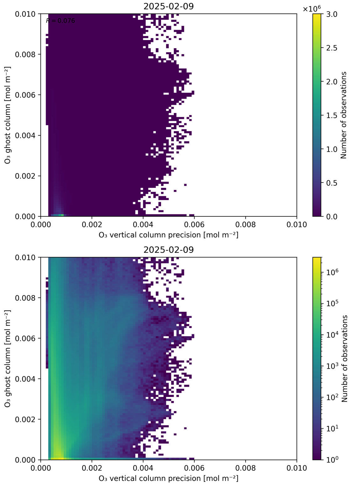
Figure 43: Scatter density plot of “O 3 vertical column precision” against “O 3 ghost column” for 2025-02-08 to 2025-02-10.
