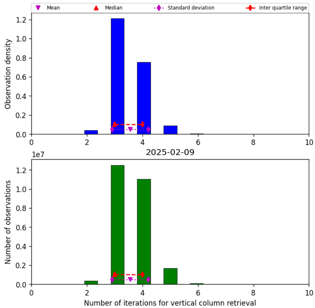
Figure 26: Histogram of “Number of iterations for vertical column retrieval” for 2025-02-08 to 2025-02-10
