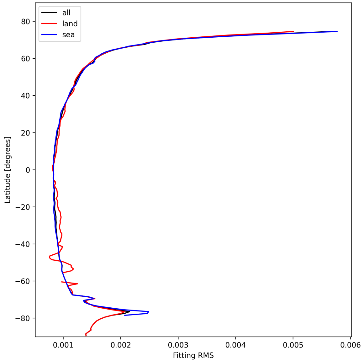
Figure 16: Zonal average of “Fitting RMS” for 2025-02-08 to 2025-02-10.
