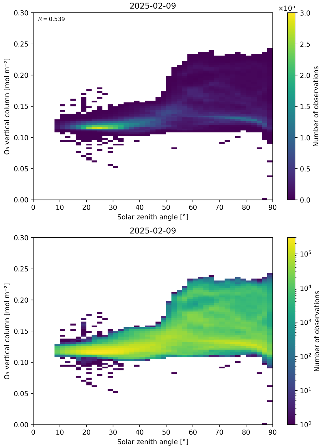
Figure 47: Scatter density plot of “Solar zenith angle” against “O 3 vertical column” for 2025-02-08 to 2025-02-10.
