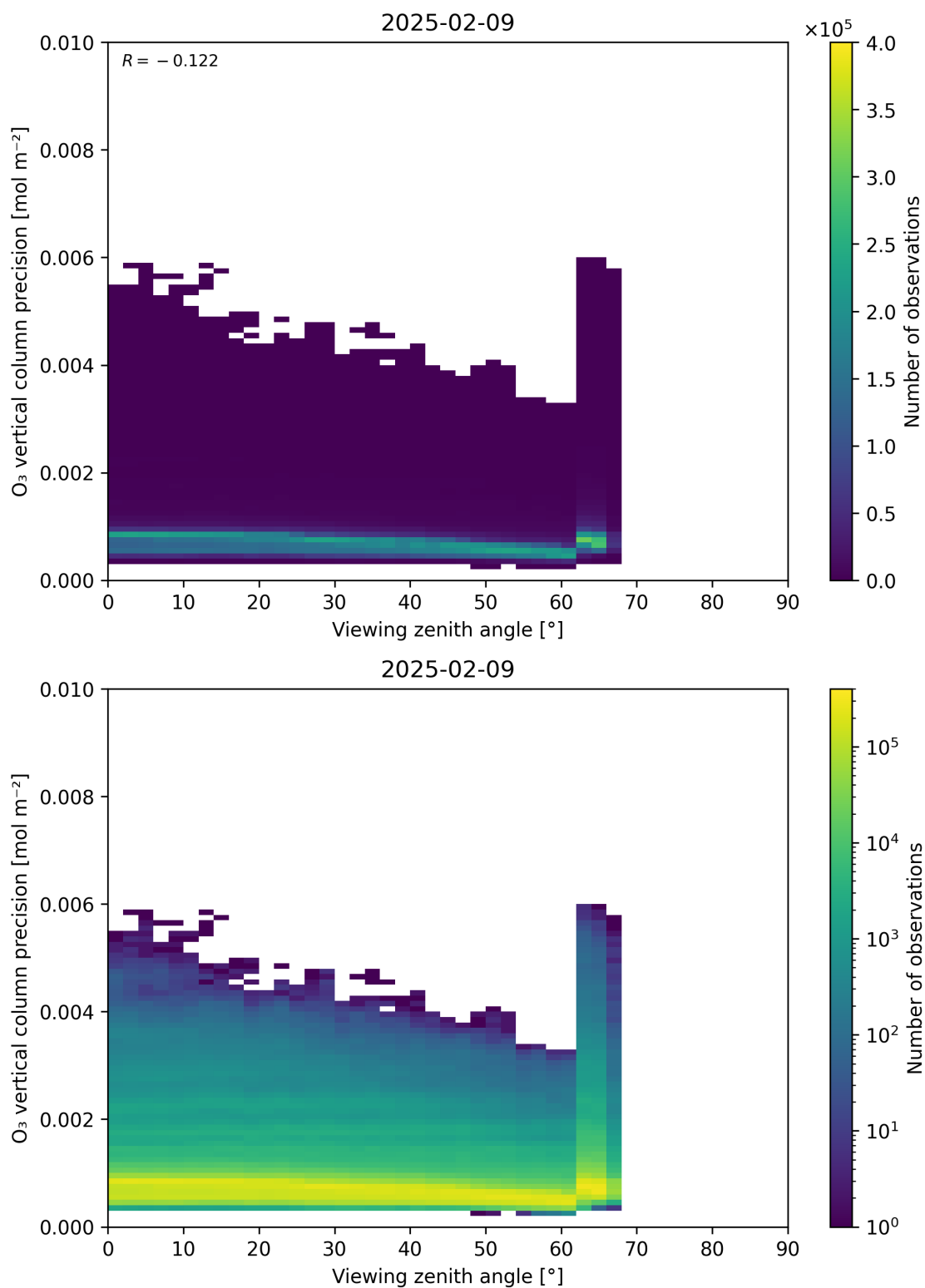
Figure 53: Scatter density plot of “Viewing zenith angle” against “O 3 vertical column precision” for 2025-02-08 to 2025-02-10.
