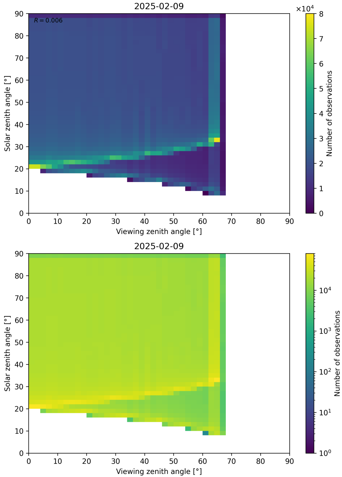
Figure 54: Scatter density plot of “Viewing zenith angle” against “Solar zenith angle” for 2025-02-08 to 2025-02-10.
