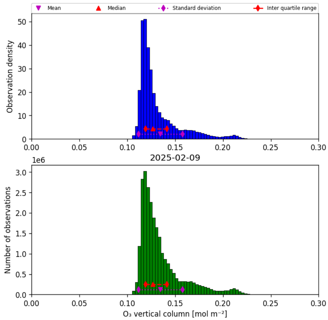
Figure 21: Histogram of “O 3 vertical column” for 2025-02-08 to 2025-02-10
