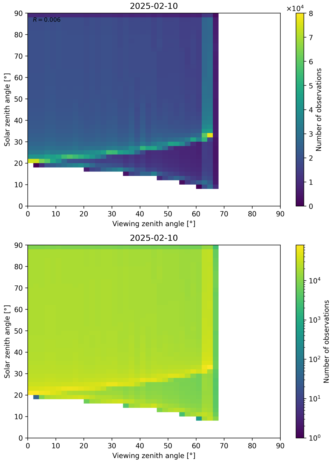
Figure 54: Scatter density plot of “Viewing zenith angle” against “Solar zenith angle” for 2025-02-09 to 2025-02-11.
