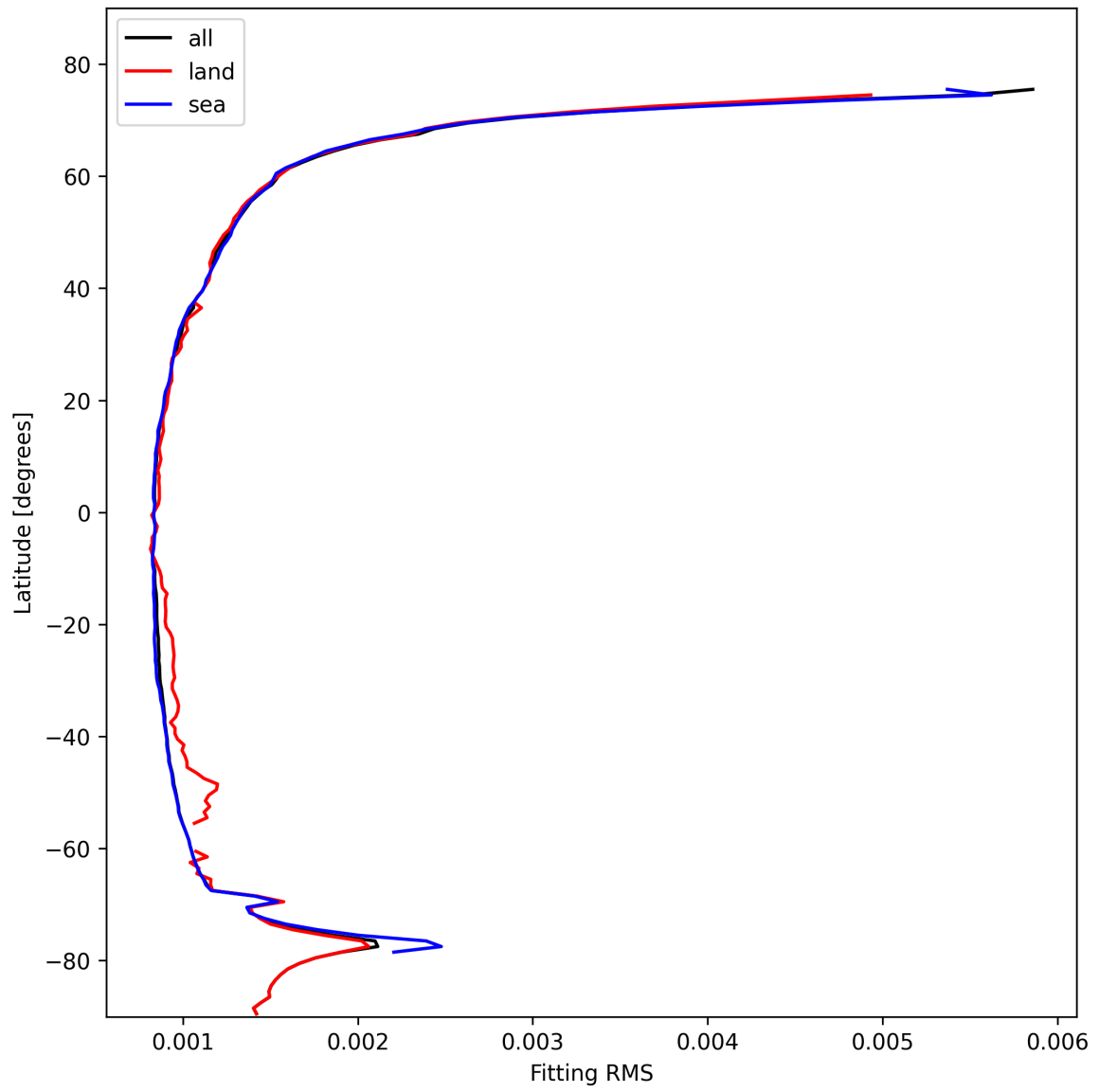
Figure 16: Zonal average of “Fitting RMS” for 2025-02-09 to 2025-02-11.
