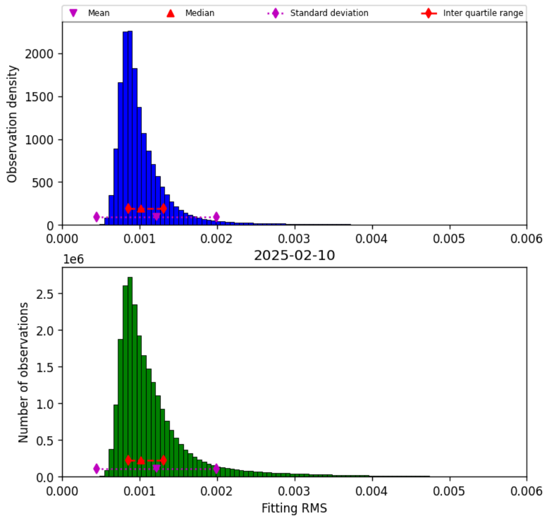
Figure 23: Histogram of “Fitting RMS” for 2025-02-09 to 2025-02-11
