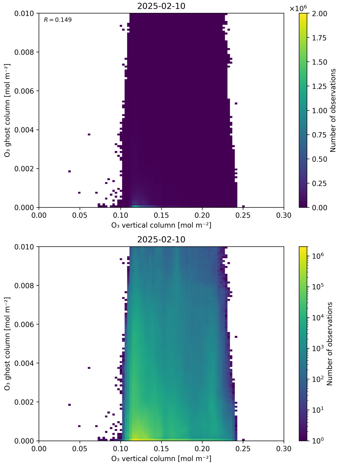
Figure 40: Scatter density plot of “O 3 vertical column” against “O 3 ghost column” for 2025-02-09 to 2025-02-11.
