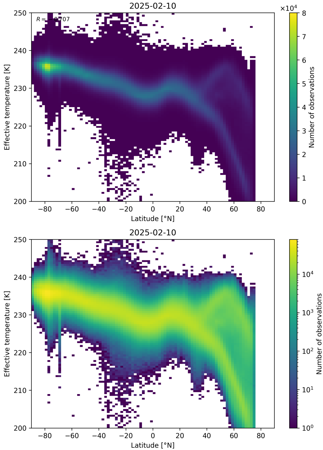
Figure 34: Scatter density plot of “Latitude” against “Effective temperature” for 2025-02-09 to 2025-02-11.
