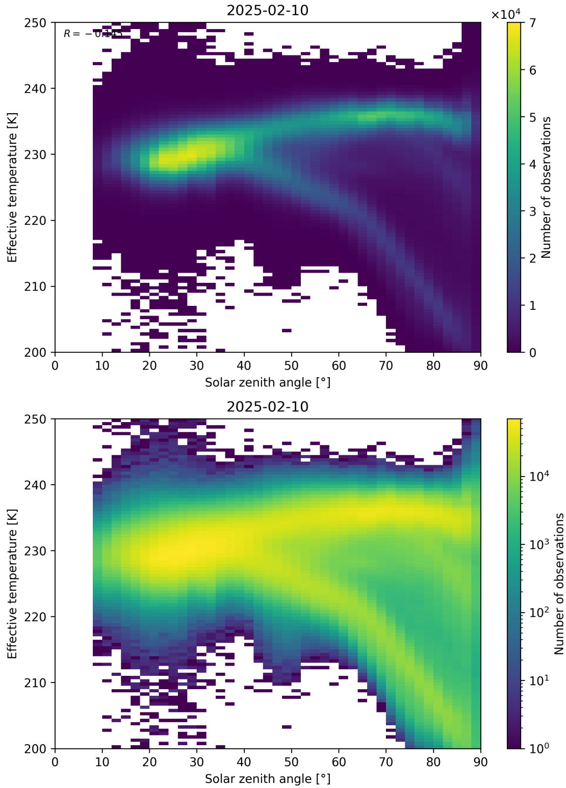
Figure 45: Scatter density plot of “Solar zenith angle” against “Effective temperature” for 2025-02-09 to 2025-02-11.
