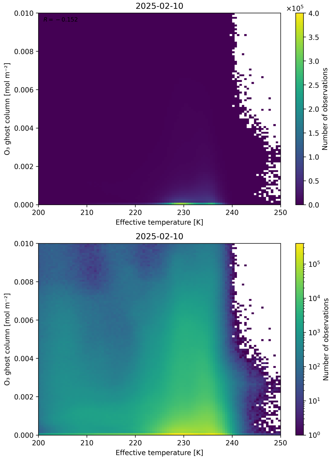
Figure 38: Scatter density plot of “Effective temperature” against “O 3 ghost column” for 2025-02-09 to 2025-02-11.
