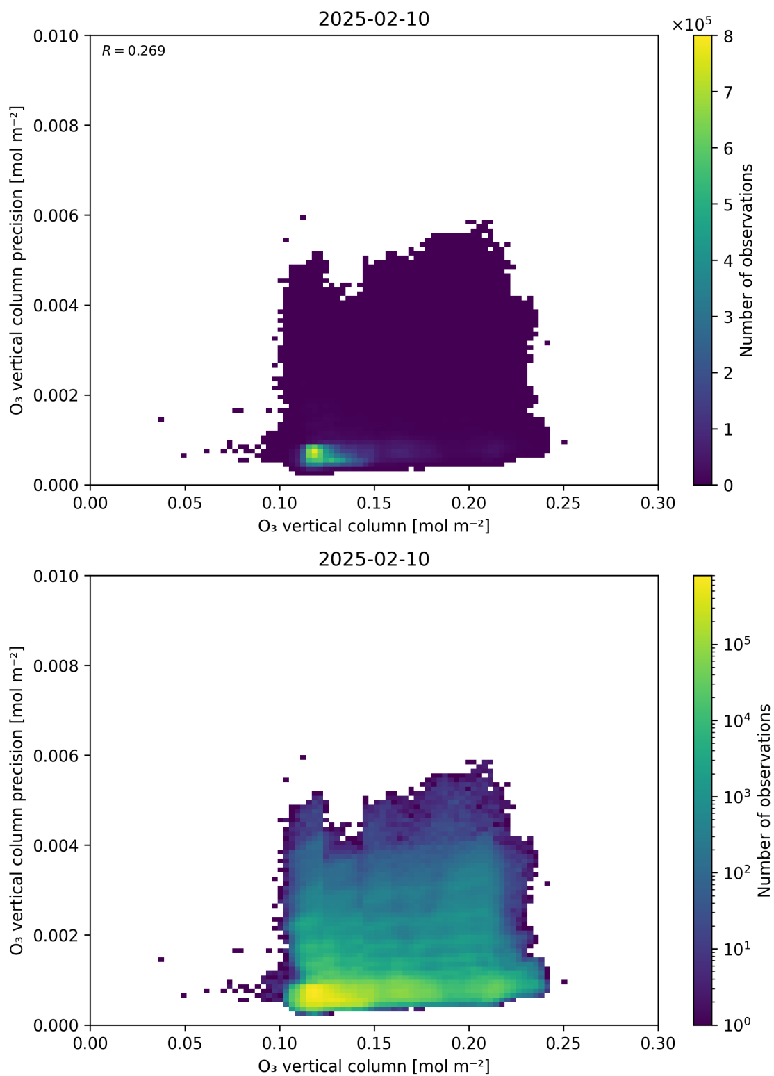
Figure 41: Scatter density plot of “O 3 vertical column” against “O 3 vertical column precision” for 2025-02-09 to 2025-02-11.
