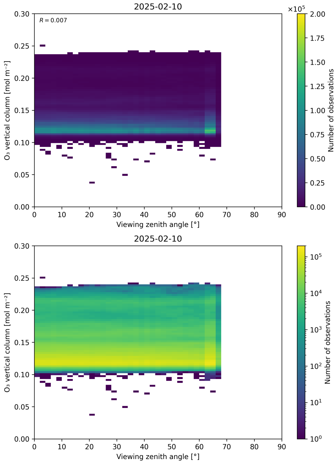
Figure 52: Scatter density plot of “Viewing zenith angle” against “O 3 vertical column” for 2025-02-09 to 2025-02-11.
