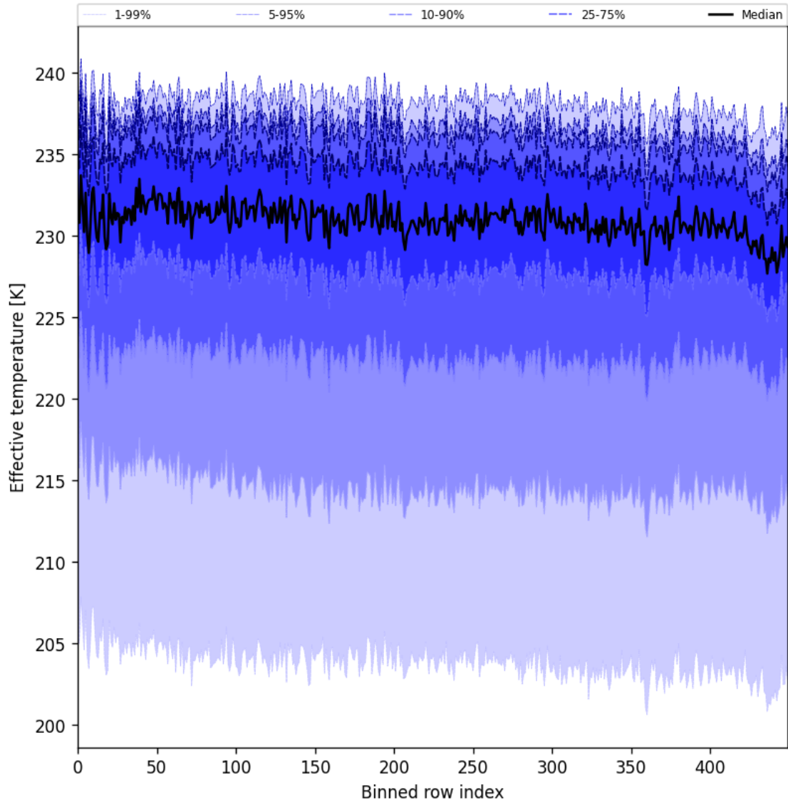
Figure 31: Along track statistics of “Effective temperature” for 2025-02-09 to 2025-02-11
