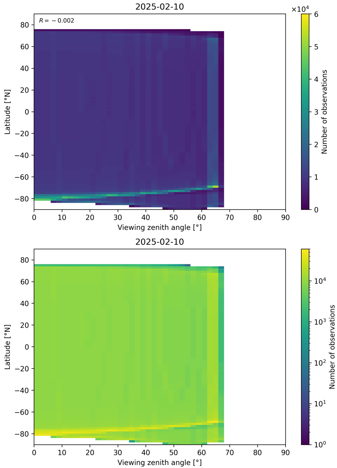
Figure 49: Scatter density plot of “Viewing zenith angle” against “Latitude” for 2025-02-09 to 2025-02-11.
