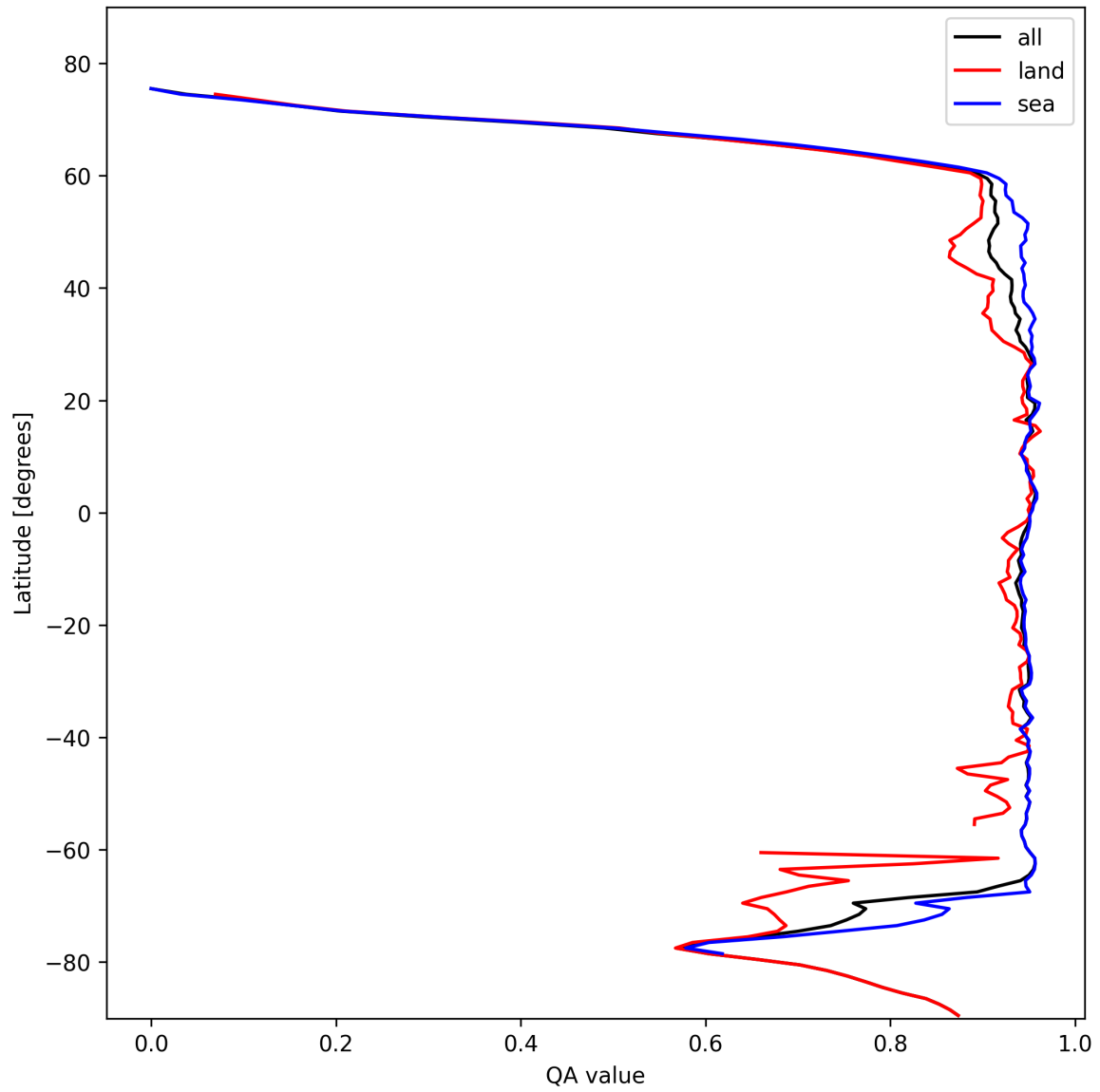
Figure 13: Zonal average of “QA value” for 2025-02-09 to 2025-02-11.
