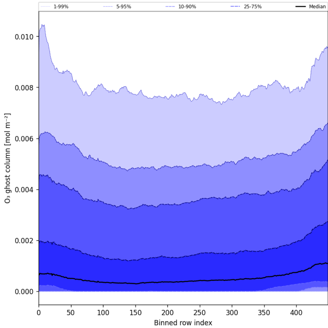
Figure 32: Along track statistics of “O 3 ghost column” for 2025-02-09 to 2025-02-11
