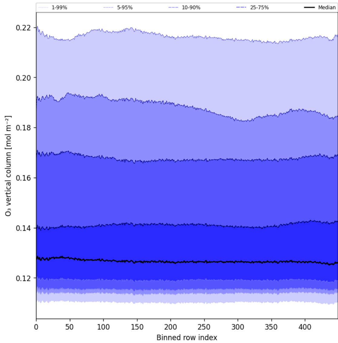
Figure 28: Along track statistics of “O 3 vertical column” for 2025-02-09 to 2025-02-11
