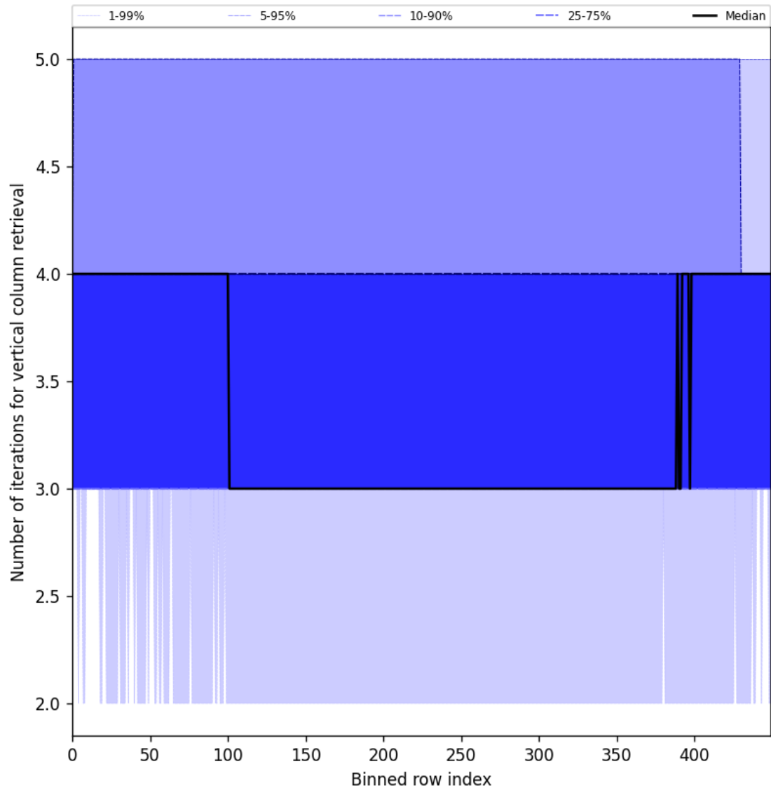
Figure 33: Along track statistics of “Number of iterations for vertical column retrieval” for 2025-02-09 to 2025-02-11
