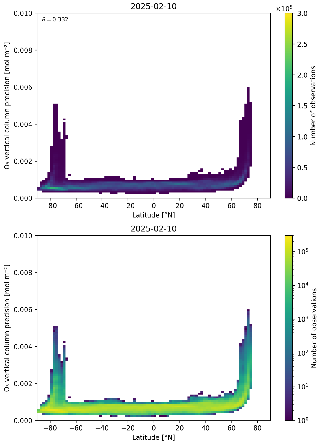
Figure 37: Scatter density plot of “Latitude” against “O 3 vertical column precision” for 2025-02-09 to 2025-02-11.
