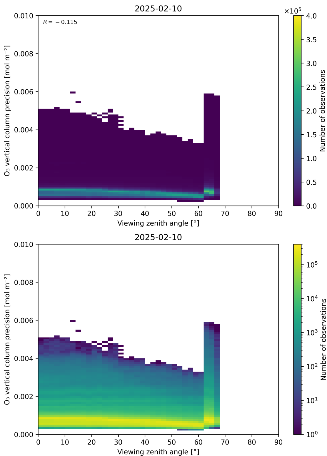
Figure 53: Scatter density plot of “Viewing zenith angle” against “O 3 vertical column precision” for 2025-02-09 to 2025-02-11.
