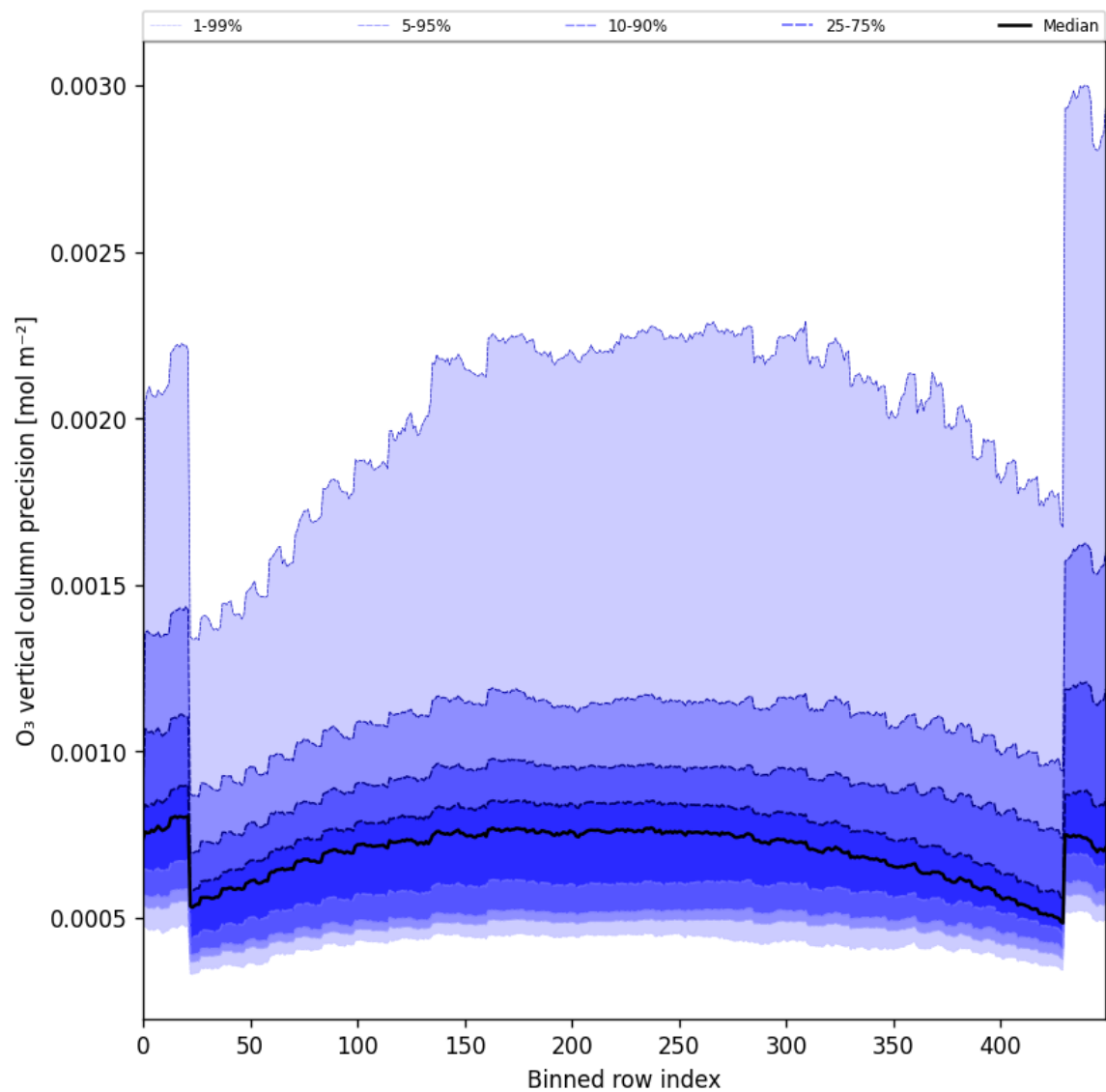
Figure 29: Along track statistics of “O 3 vertical column precision” for 2025-02-09 to 2025-02-11
