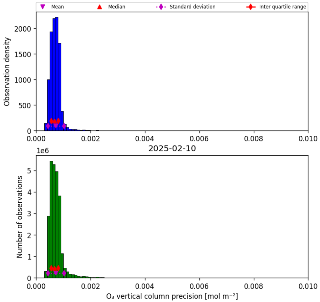
Figure 22: Histogram of “O 3 vertical column precision” for 2025-02-09 to 2025-02-11
