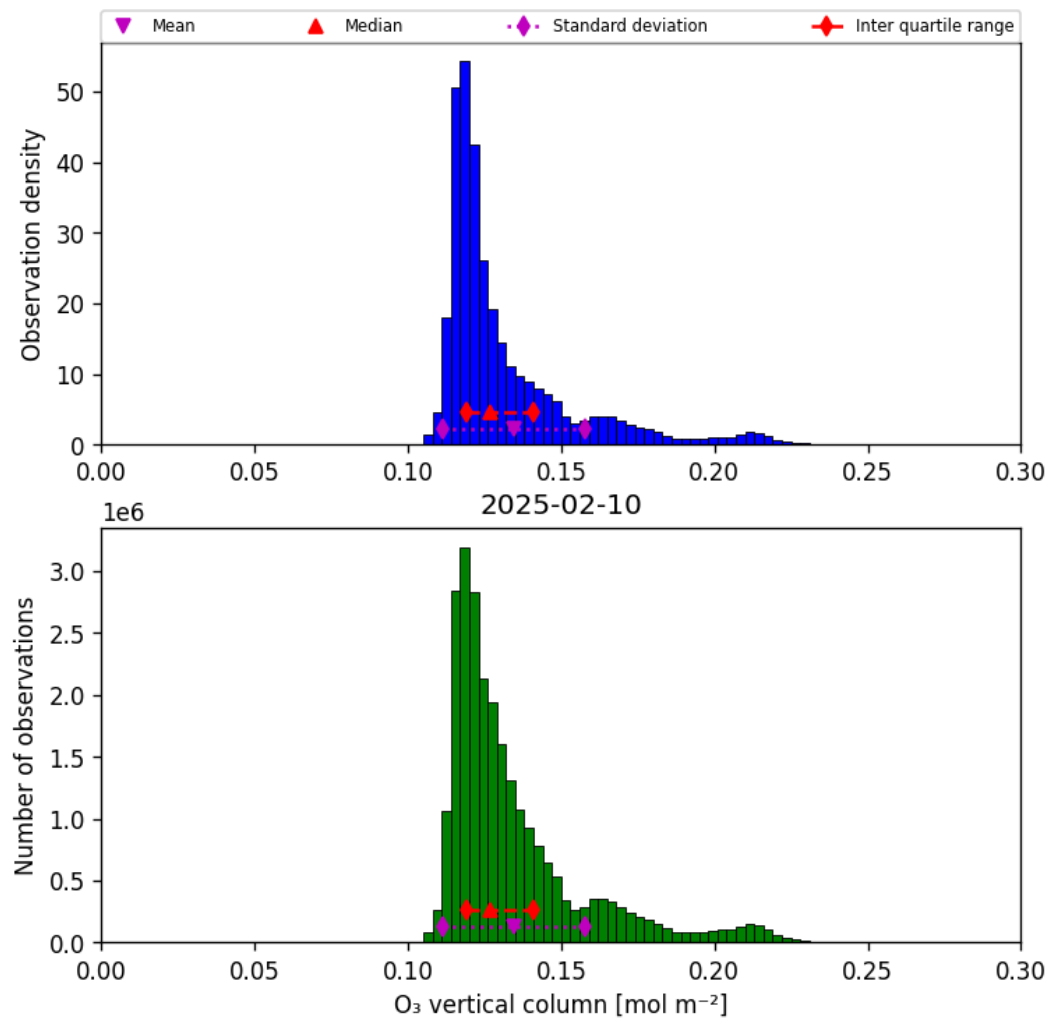
Figure 21: Histogram of “O 3 vertical column” for 2025-02-09 to 2025-02-11
