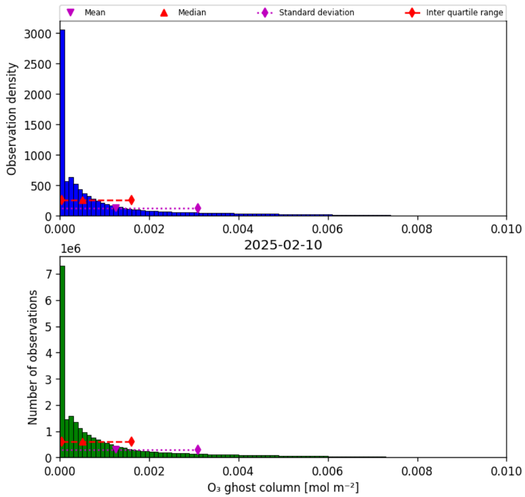
Figure 25: Histogram of "O 3 ghost column" for 2025-02-09 to 2025-02-11
