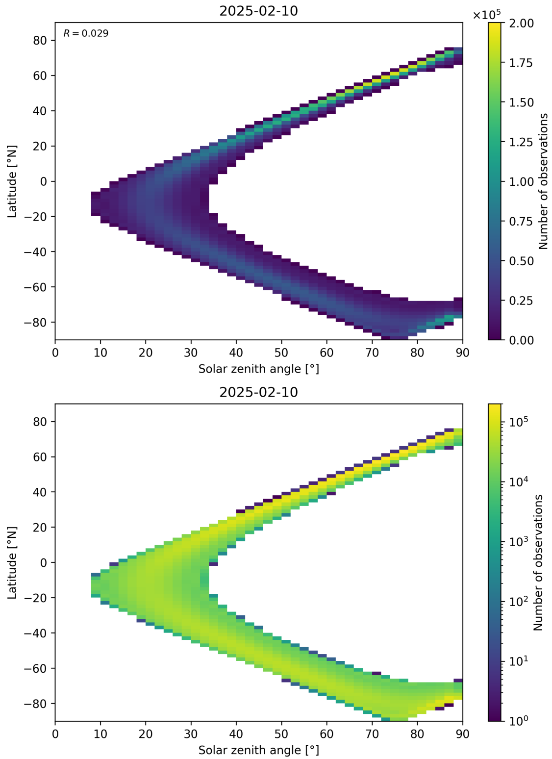
Figure 44: Scatter density plot of “Solar zenith angle” against “Latitude” for 2025-02-09 to 2025-02-11.
