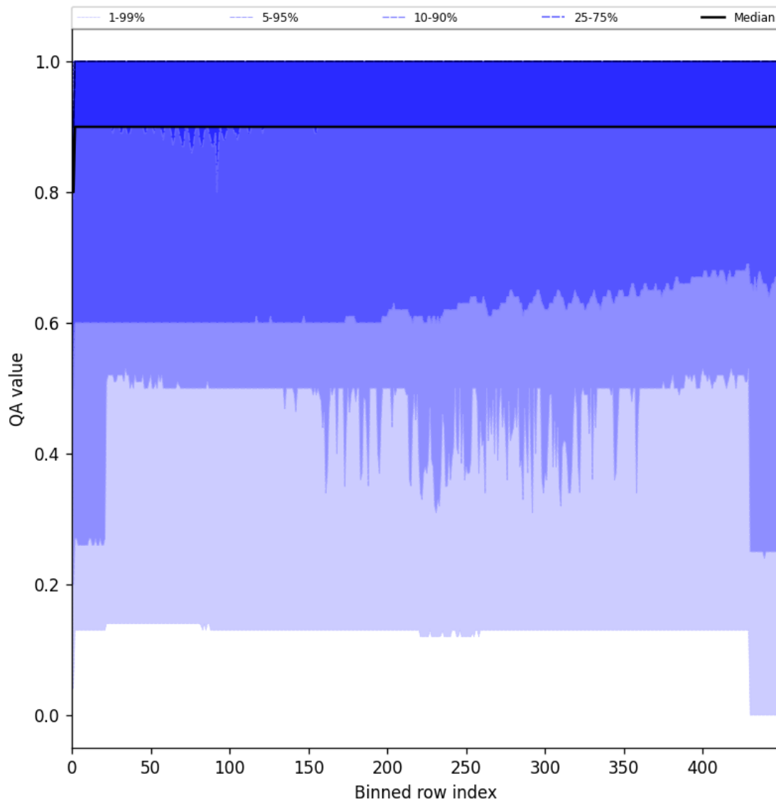
Figure 27: Along track statistics of “QA value” for 2025-02-09 to 2025-02-11
