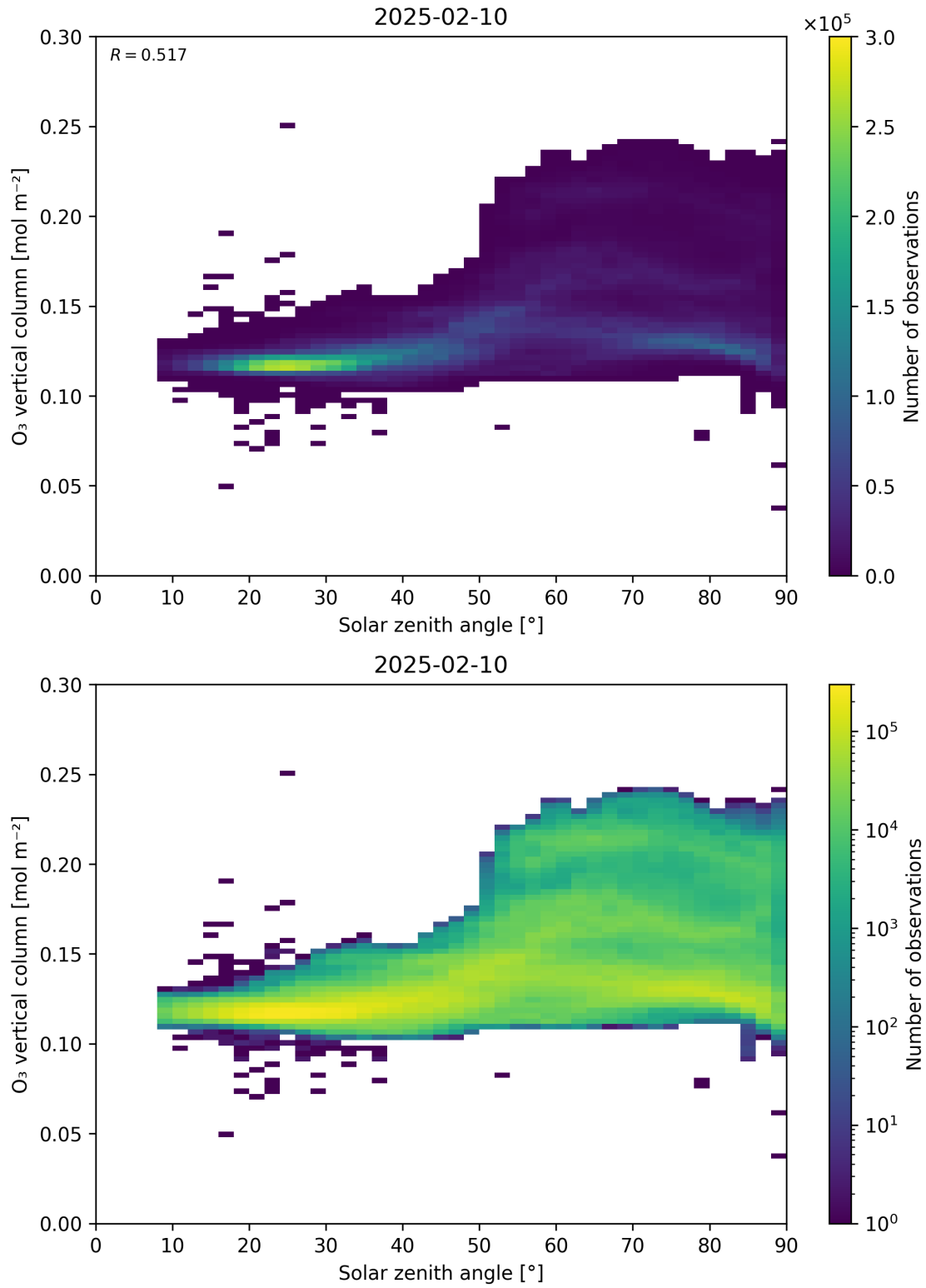
Figure 47: Scatter density plot of “Solar zenith angle” against “O 3 vertical column” for 2025-02-09 to 2025-02-11.
