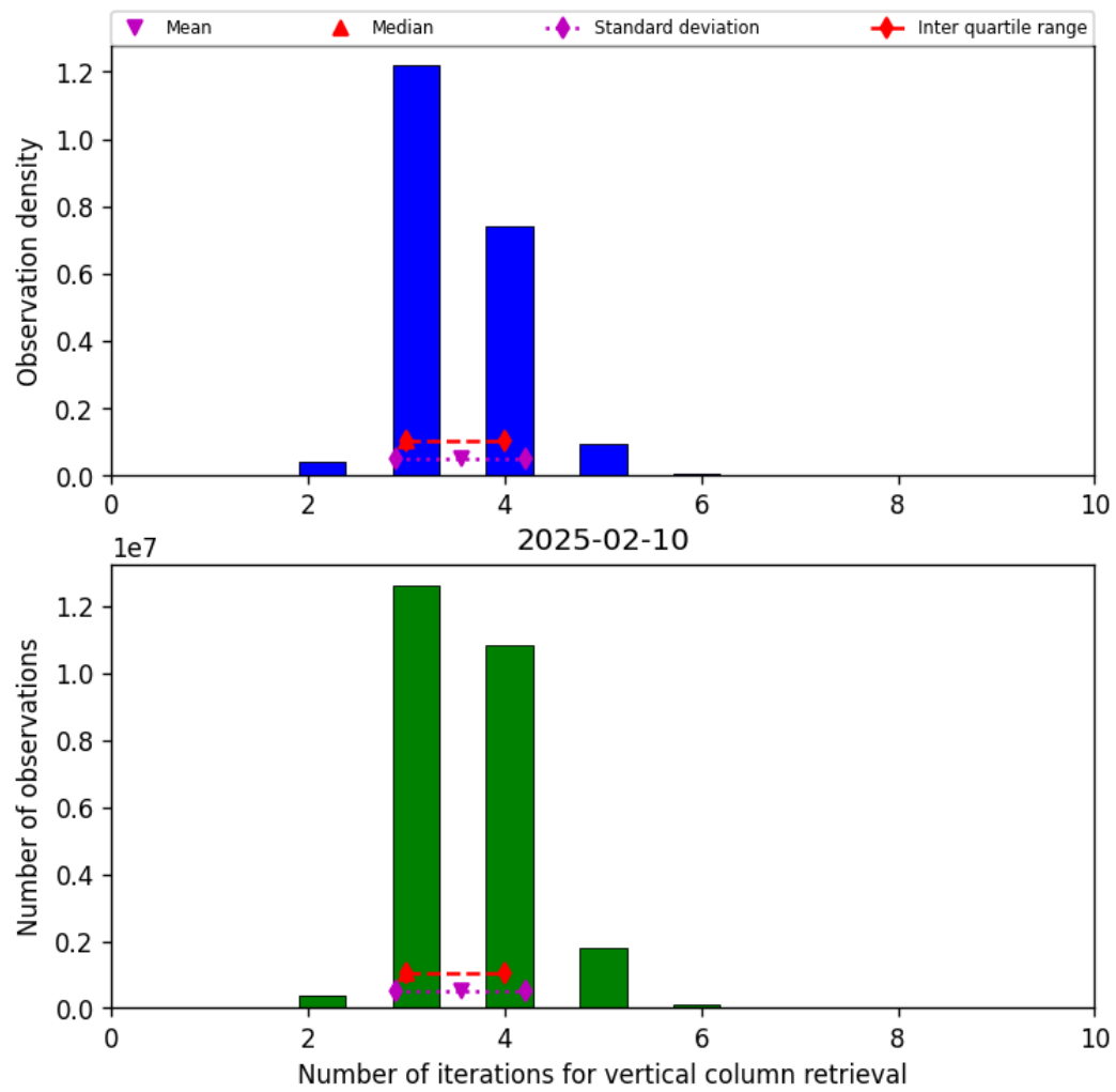
Figure 26: Histogram of “Number of iterations for vertical column retrieval” for 2025-02-09 to 2025-02-11
