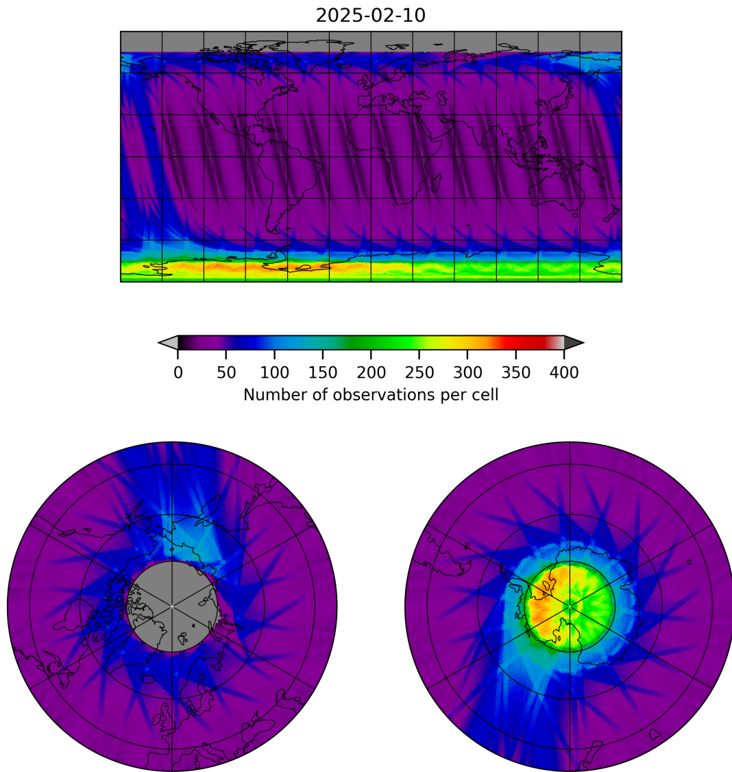
Figure 12: Map of the number of observations for 2025-02-09 to 2025-02-11
