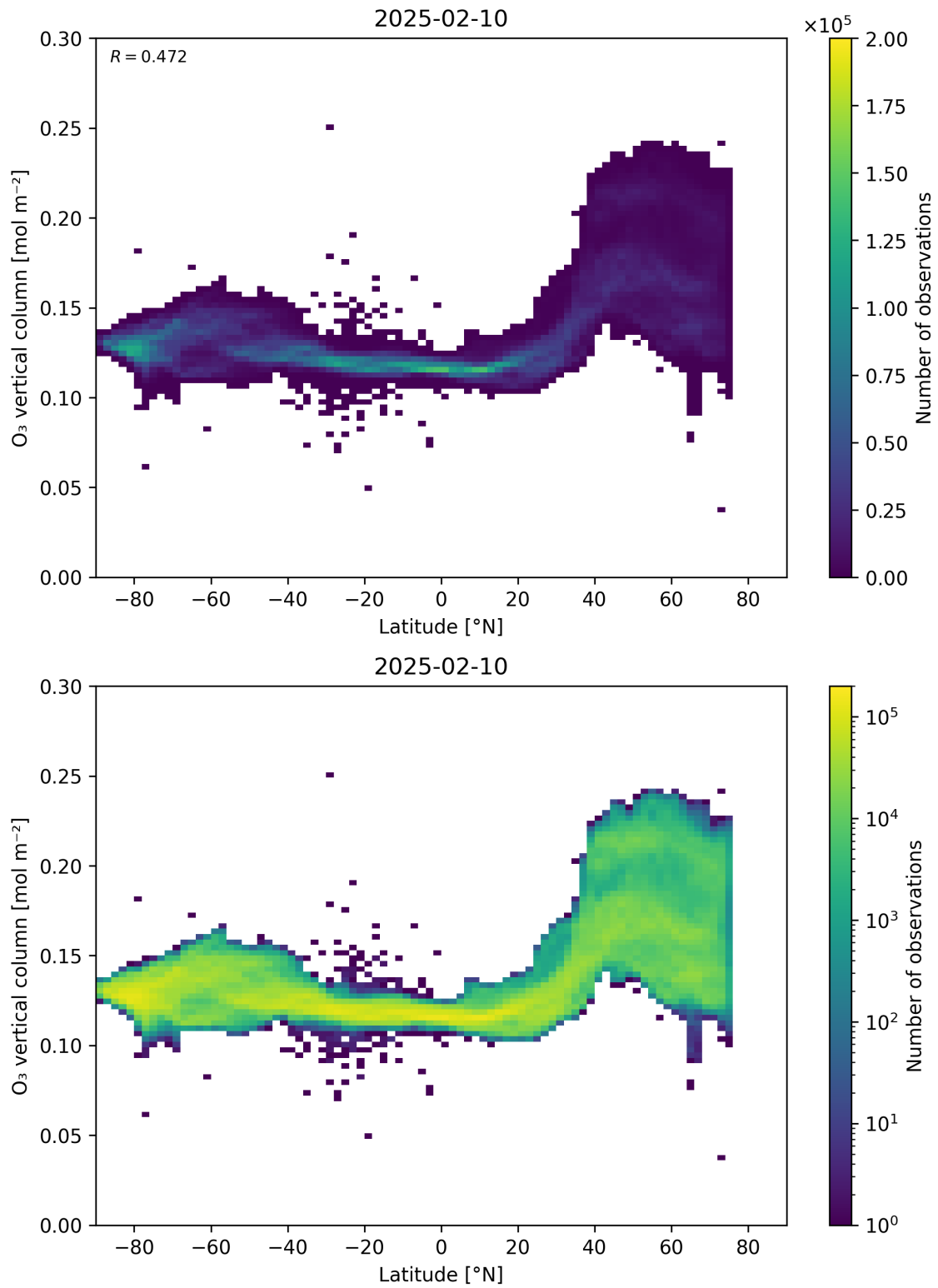
Figure 36: Scatter density plot of “Latitude” against “O 3 vertical column” for 2025-02-09 to 2025-02-11.
