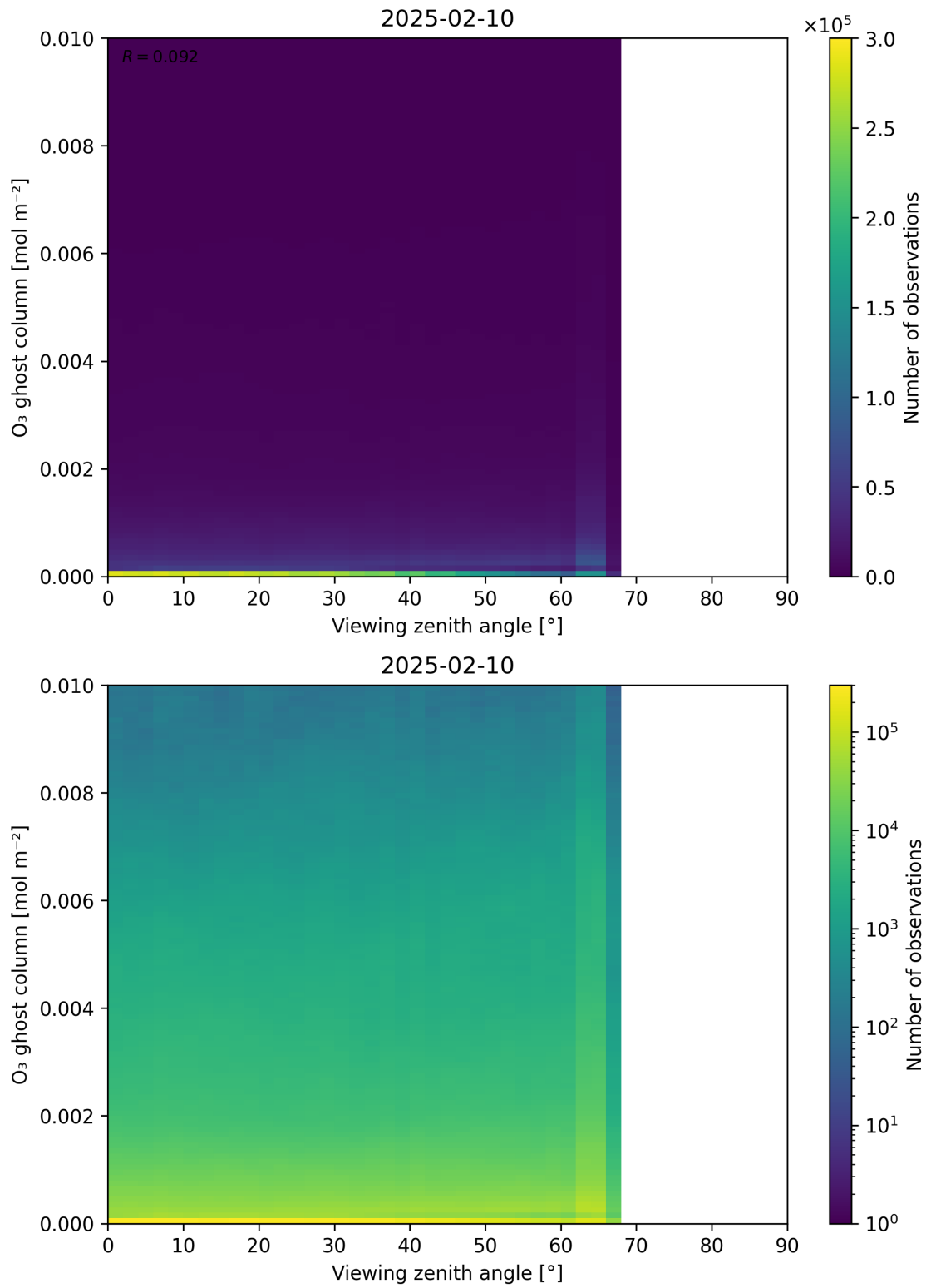
Figure 51: Scatter density plot of “Viewing zenith angle” against “O 3 ghost column” for 2025-02-09 to 2025-02-11.
