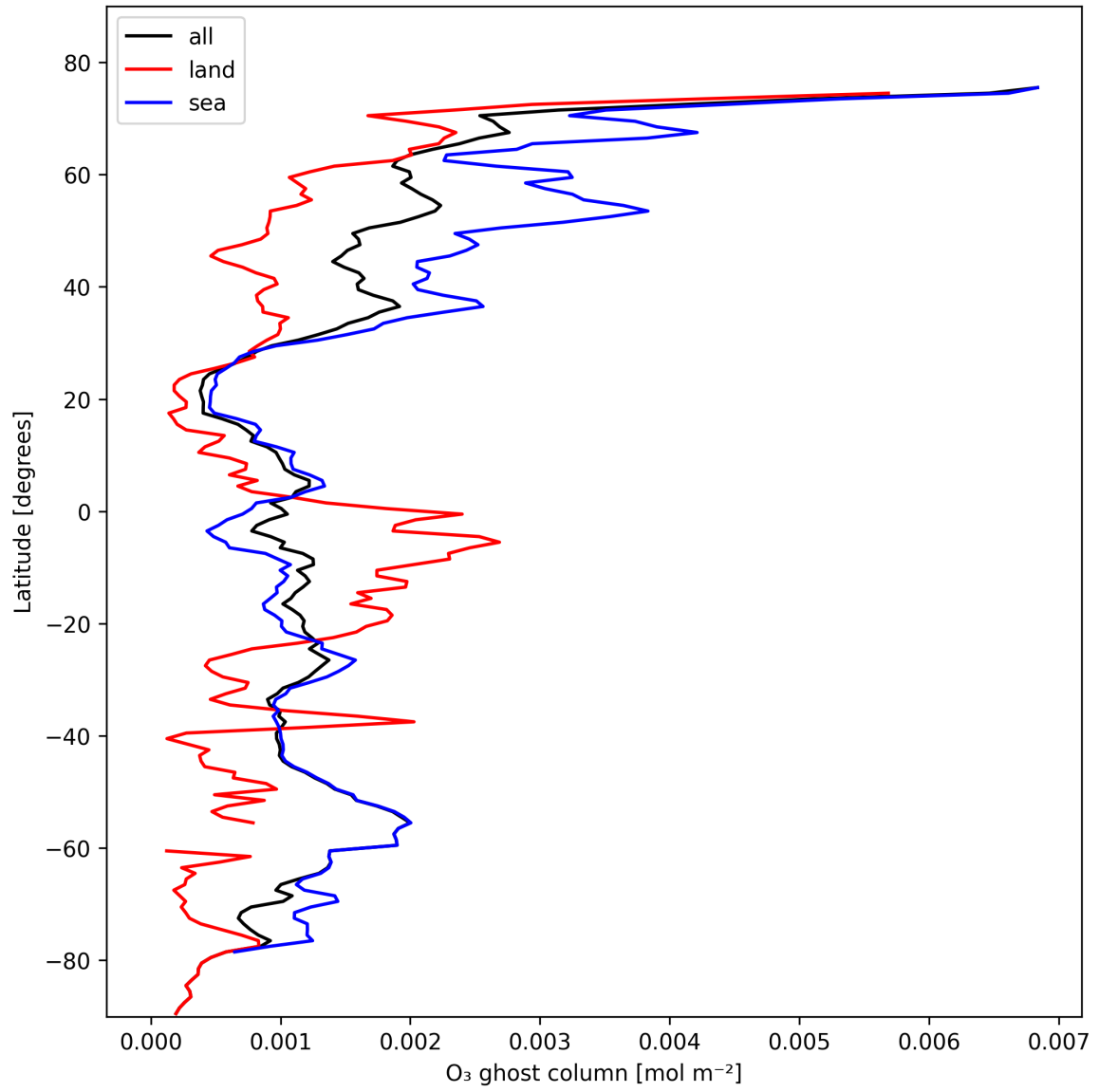
Figure 18: Zonal average of “O 3 ghost column” for 2025-02-09 to 2025-02-11.
