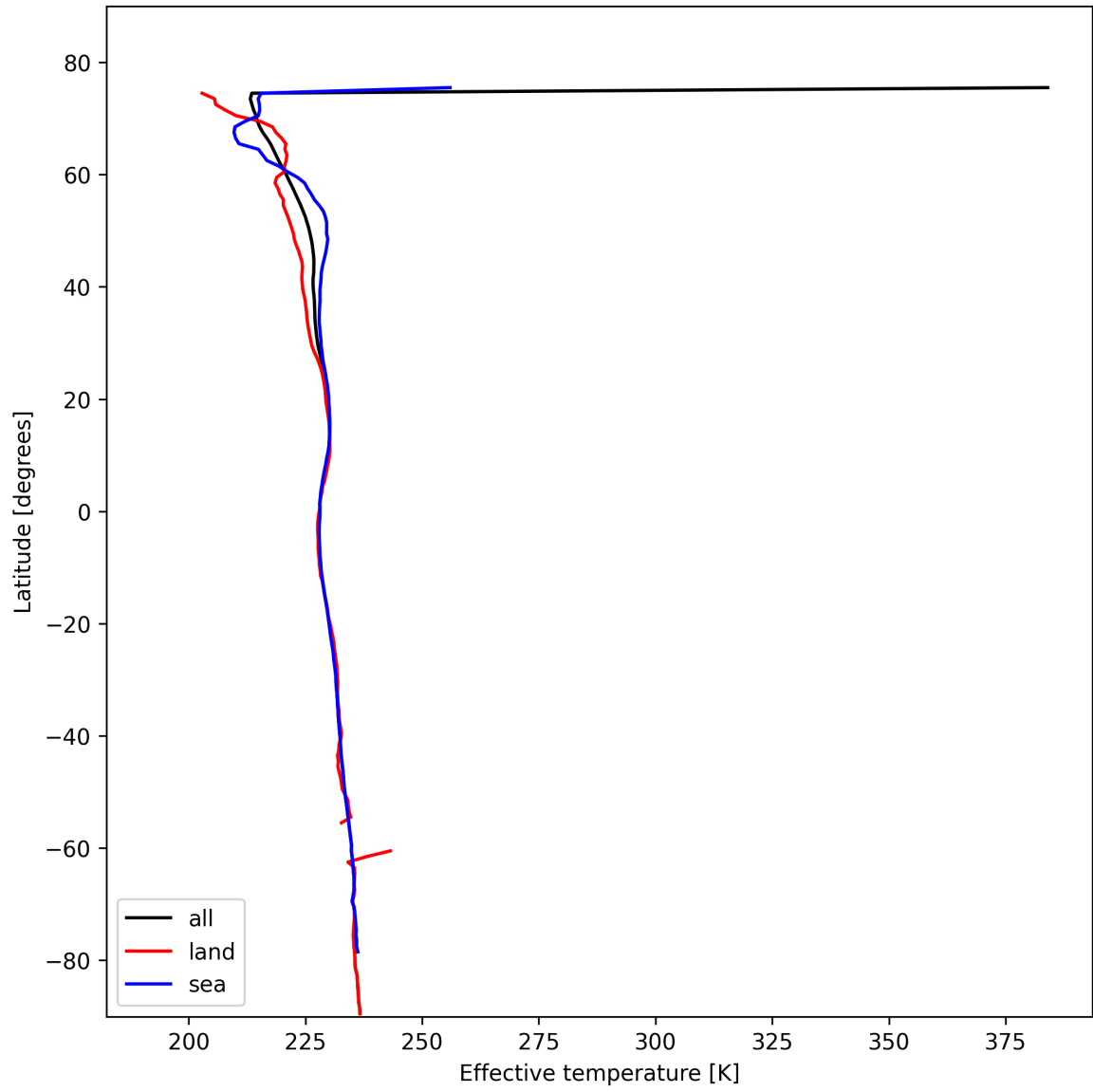
Figure 17: Zonal average of "Effective temperature" for 2025-02-09 to 2025-02-11.
