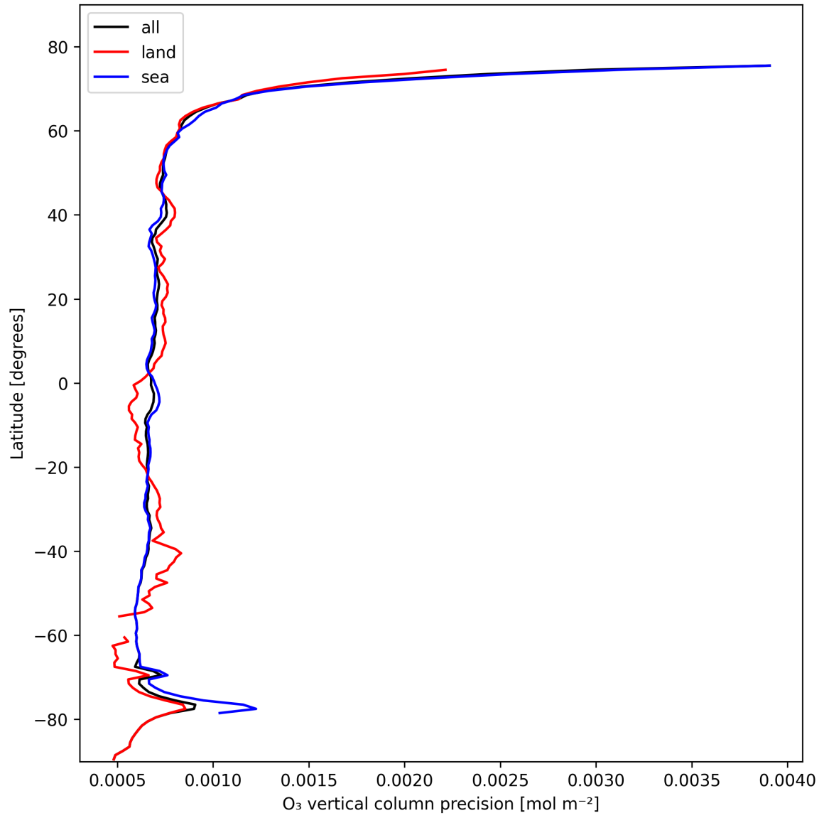
Figure 15: Zonal average of “O 3 vertical column precision” for 2025-02-09 to 2025-02-11.
