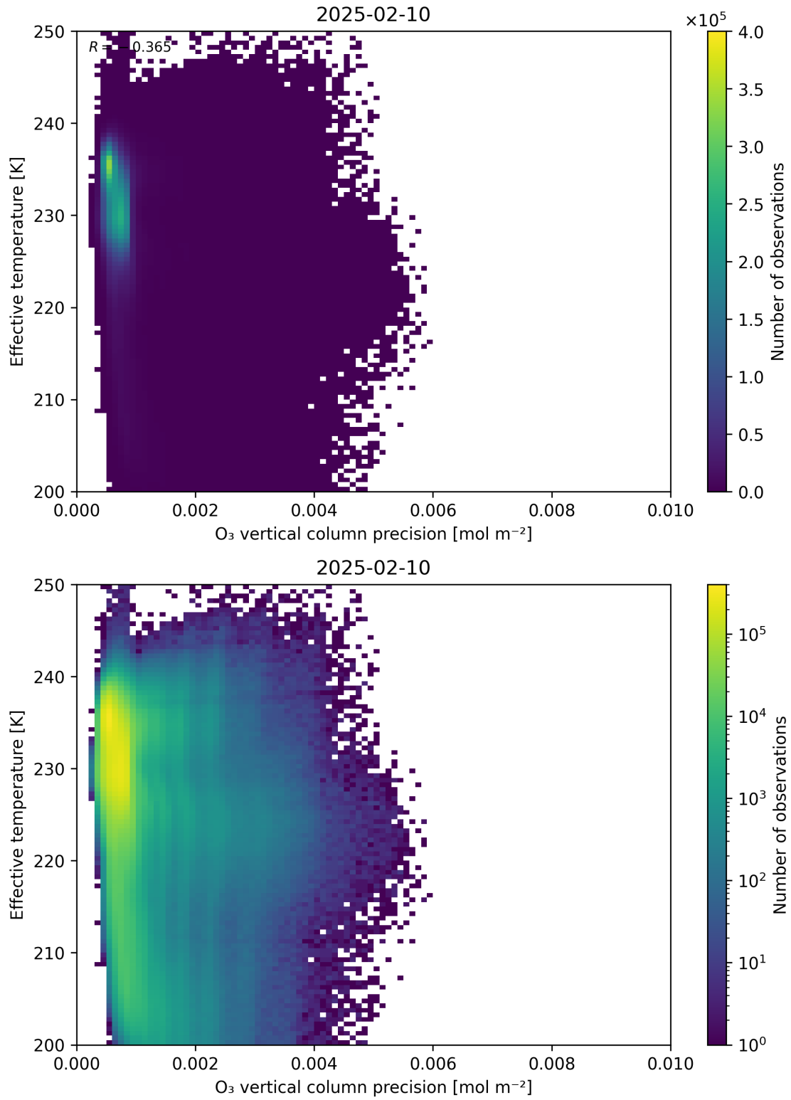
Figure 42: Scatter density plot of “O 3 vertical column precision” against “Effective temperature” for 2025-02-09 to 2025-02-11.
