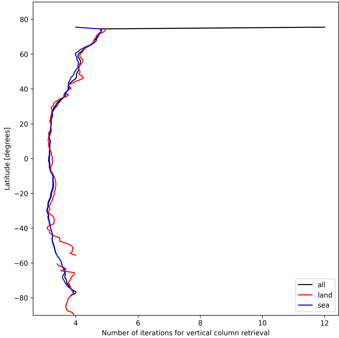
Figure 19: Zonal average of “Number of iterations for vertical column retrieval” for 2025-02-09 to 2025-02-11.
