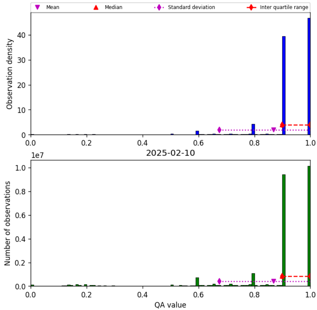
Figure 20: Histogram of “QA value” for 2025-02-09 to 2025-02-11
