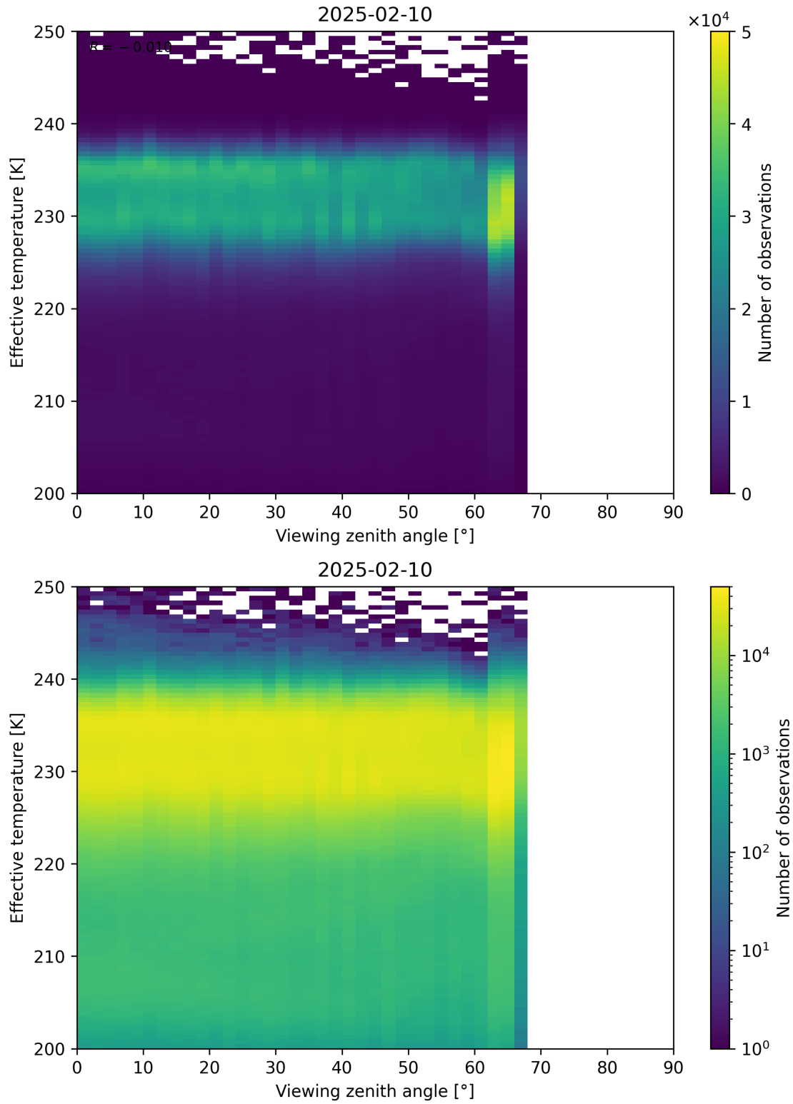
Figure 50: Scatter density plot of “Viewing zenith angle” against “Effective temperature” for 2025-02-09 to 2025-02-11.
