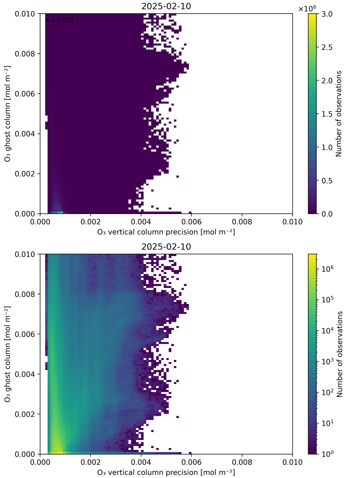
Figure 43: Scatter density plot of “ \text{O}_3 vertical column precision” against “ \text{O}_3 ghost column” for 2025-02-09 to 2025-02-11.
