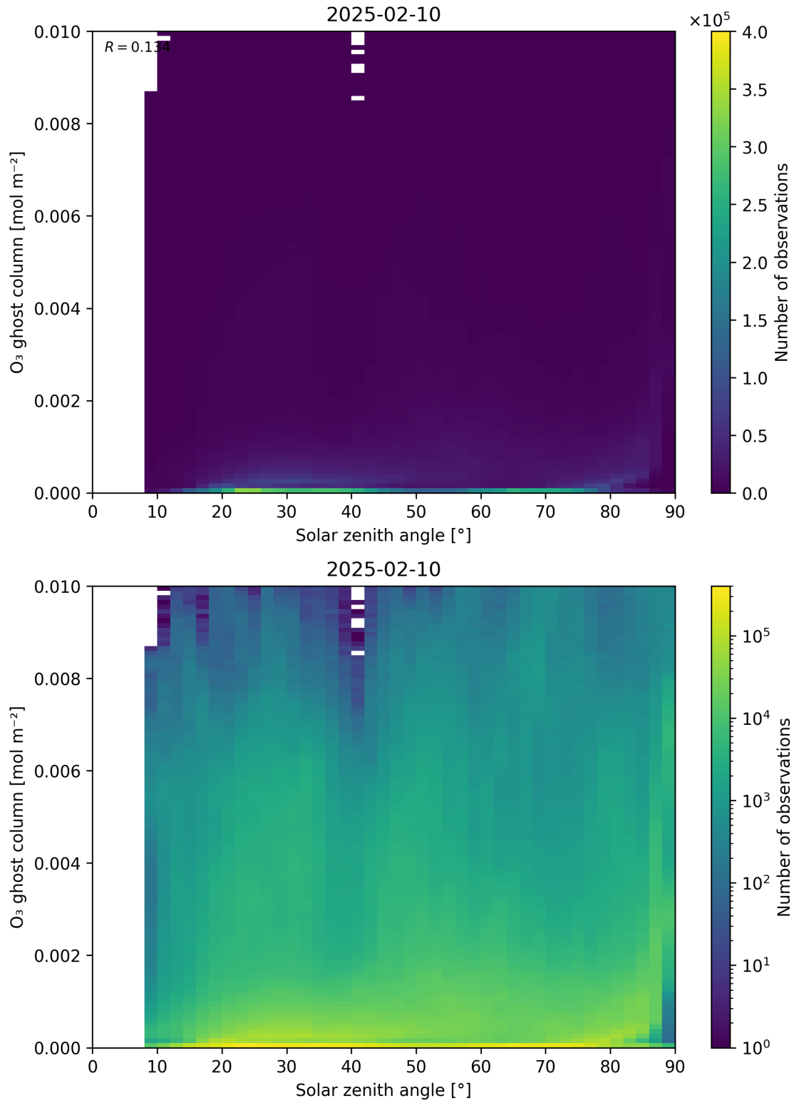
Figure 46: Scatter density plot of “Solar zenith angle” against “O 3 ghost column” for 2025-02-09 to 2025-02-11.
