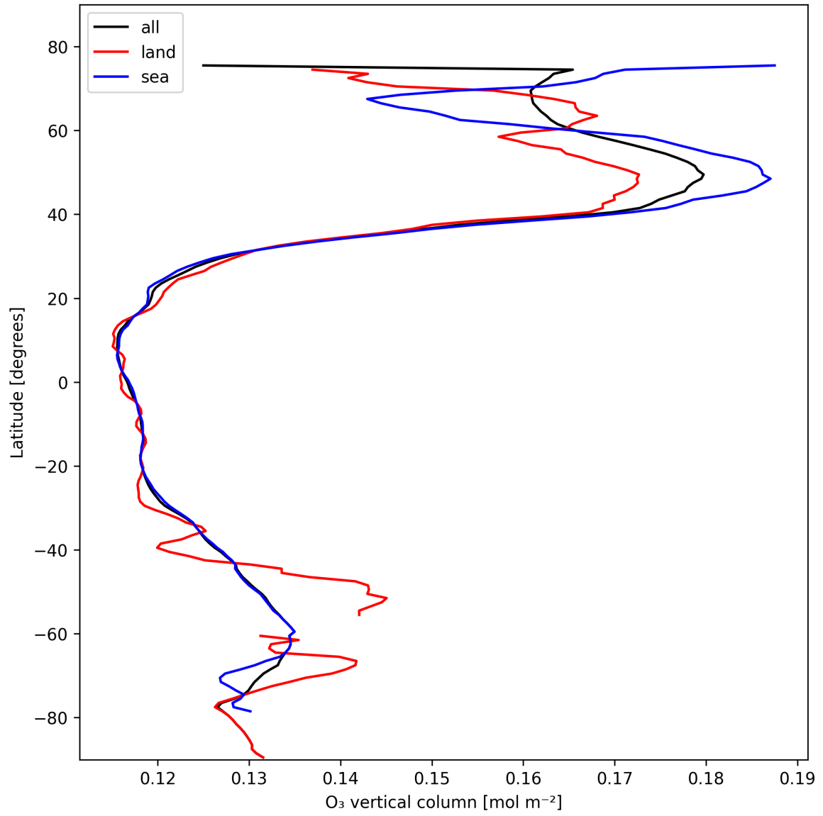
Figure 14: Zonal average of “O 3 vertical column” for 2025-02-09 to 2025-02-11.
