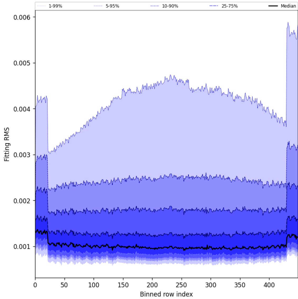
Figure 30: Along track statistics of “Fitting RMS” for 2025-02-09 to 2025-02-11
