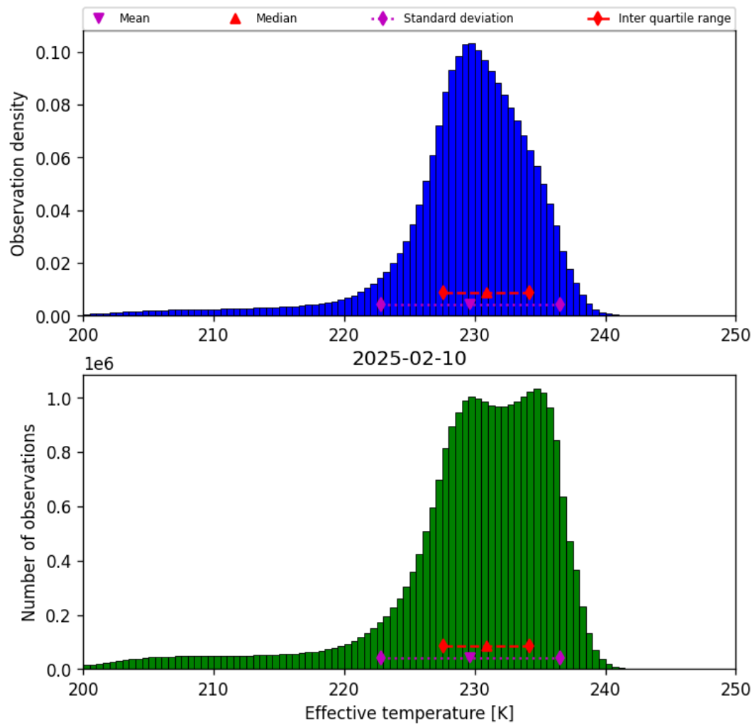
Figure 24: Histogram of “Effective temperature” for 2025-02-09 to 2025-02-11
