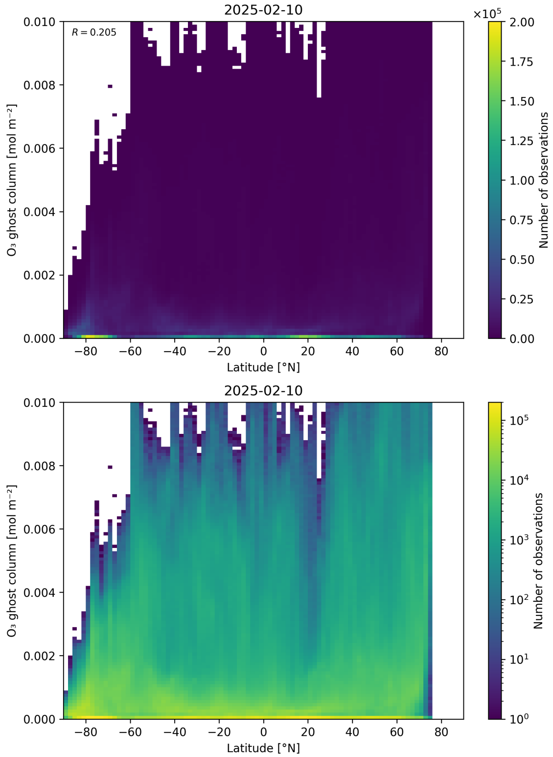
Figure 35: Scatter density plot of “Latitude” against “O 3 ghost column” for 2025-02-09 to 2025-02-11.
