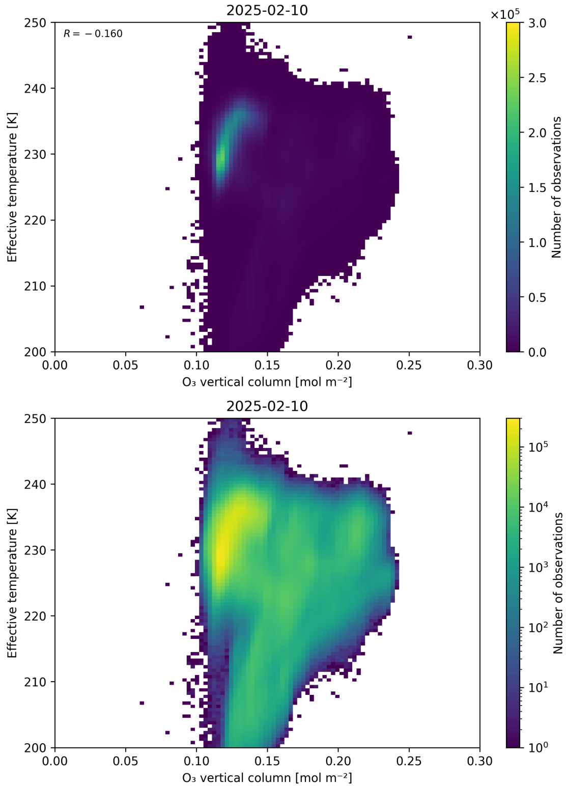
Figure 39: Scatter density plot of “O 3 vertical column” against “Effective temperature” for 2025-02-09 to 2025-02-11.
