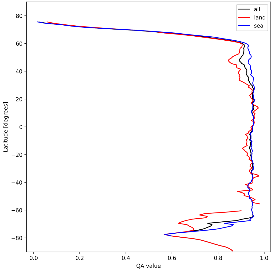
Figure 13: Zonal average of “QA value” for 2025-02-10 to 2025-02-12.
