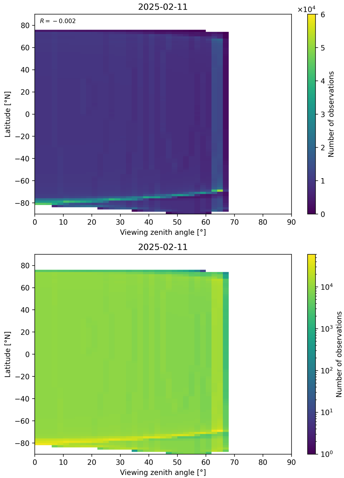
Figure 49: Scatter density plot of “Viewing zenith angle” against “Latitude” for 2025-02-10 to 2025-02-12.
