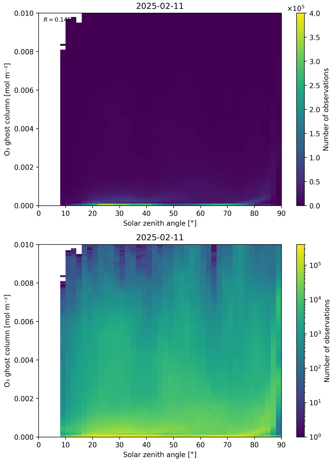
Figure 46: Scatter density plot of “Solar zenith angle” against “O 3 ghost column” for 2025-02-10 to 2025-02-12.
