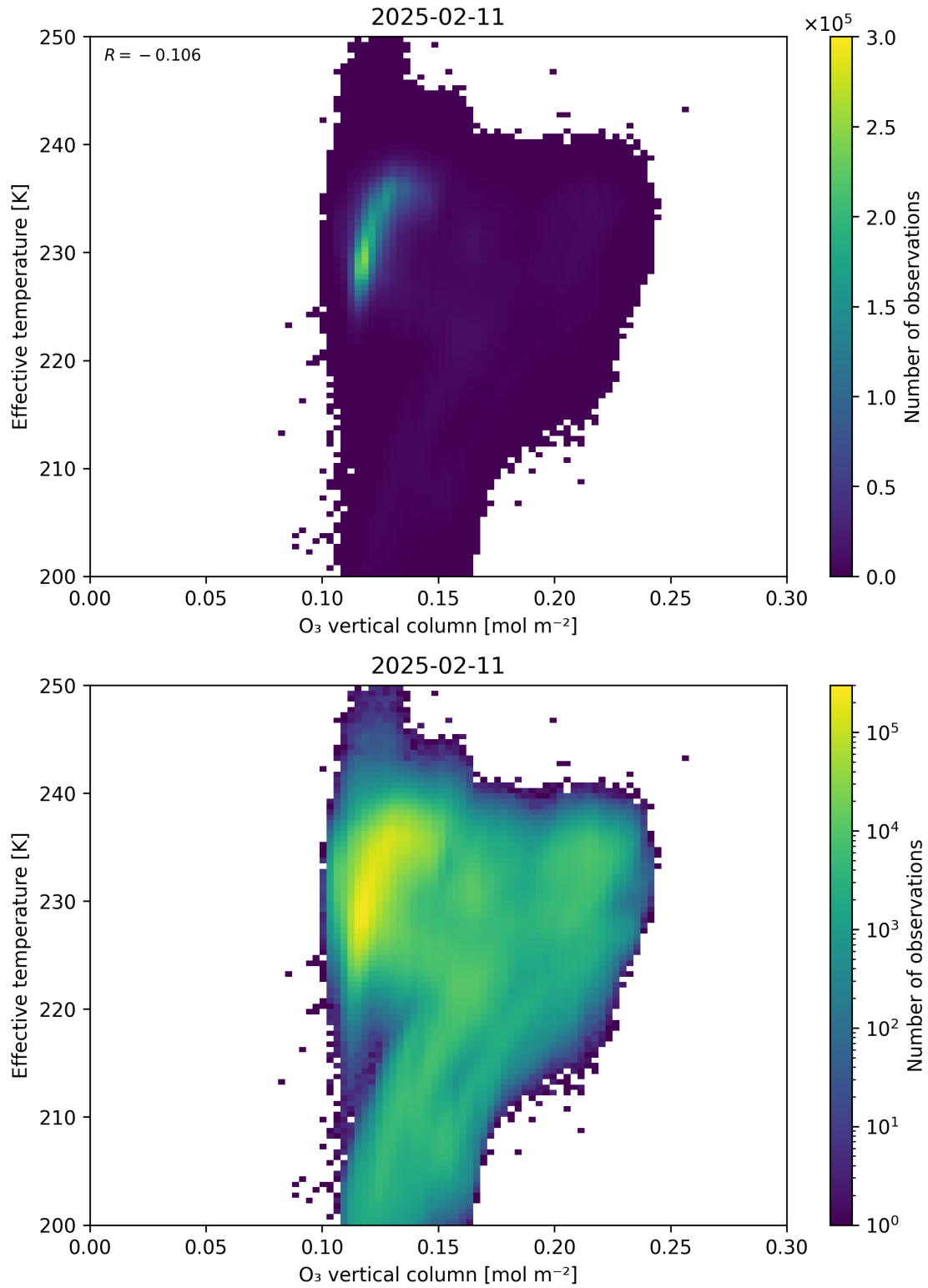
Figure 39: Scatter density plot of “O 3 vertical column” against “Effective temperature” for 2025-02-10 to 2025-02-12.
