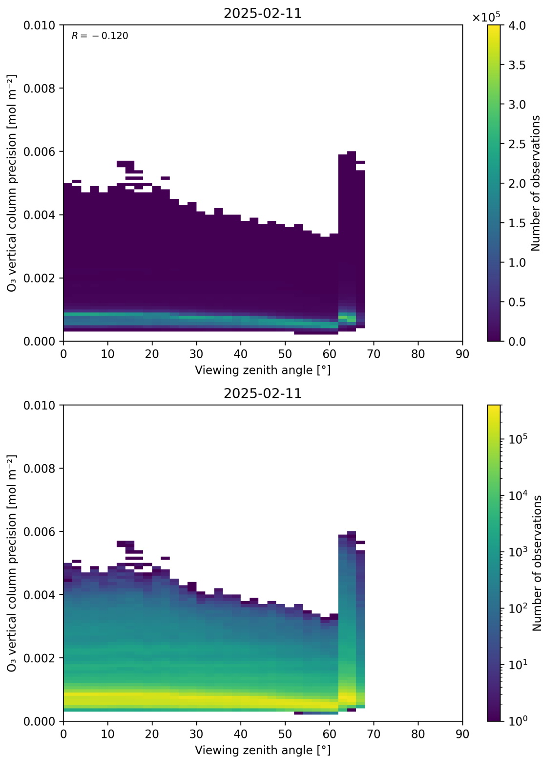
Figure 53: Scatter density plot of “Viewing zenith angle” against “O 3 vertical column precision” for 2025-02-10 to 2025-02-12.
