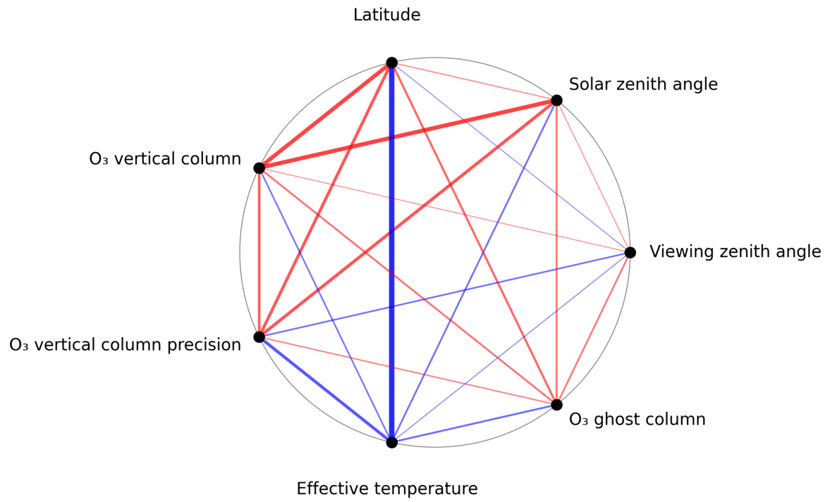
Figure 1: Map of correlation graph for 2025-02-10 to 2025-02-12.
