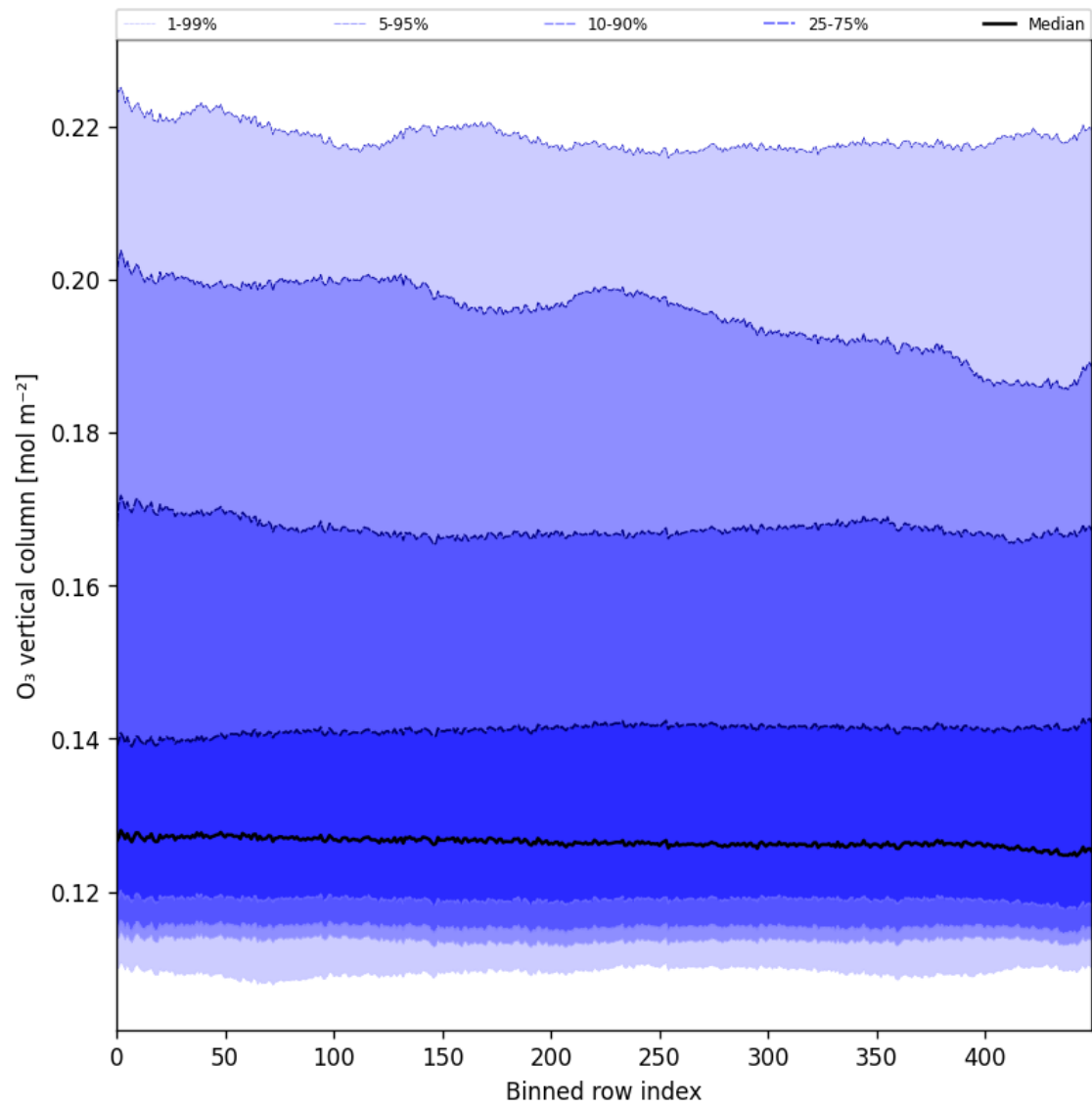
Figure 28: Along track statistics of “O 3 vertical column” for 2025-02-10 to 2025-02-12
