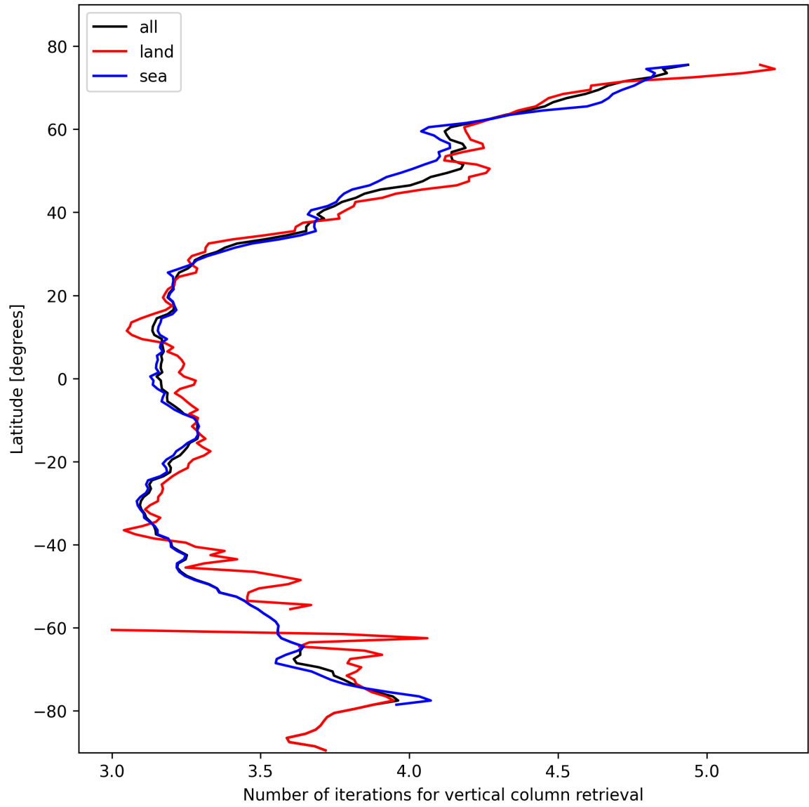
Figure 19: Zonal average of “Number of iterations for vertical column retrieval” for 2025-02-10 to 2025-02-12.
