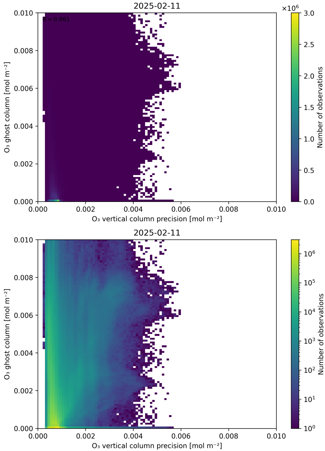
Figure 43: Scatter density plot of “ \text{O}_3 vertical column precision” against “ \text{O}_3 ghost column” for 2025-02-10 to 2025-02-12.
