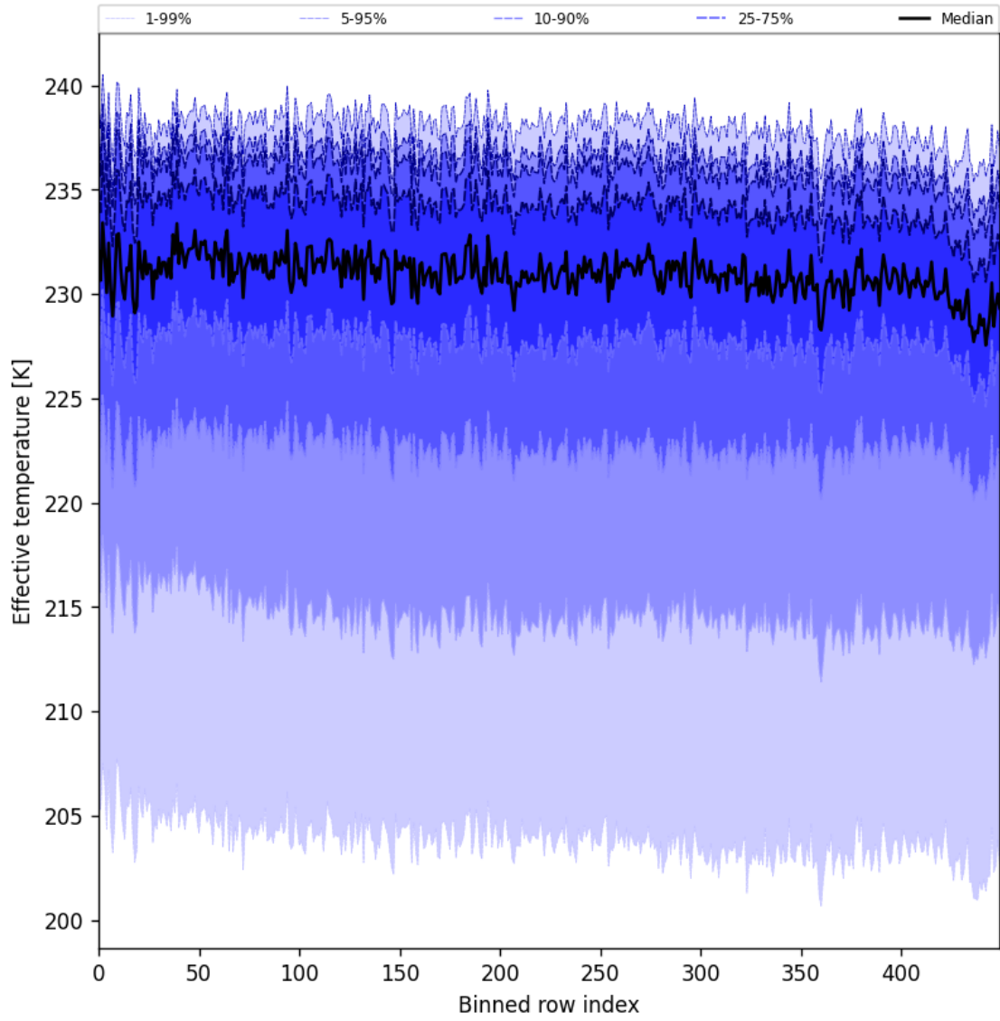
Figure 31: Along track statistics of “Effective temperature” for 2025-02-10 to 2025-02-12
