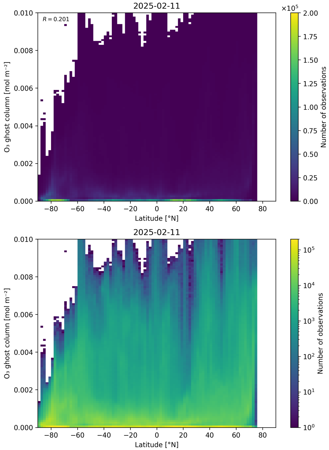
Figure 35: Scatter density plot of “Latitude” against “O 3 ghost column” for 2025-02-10 to 2025-02-12.
