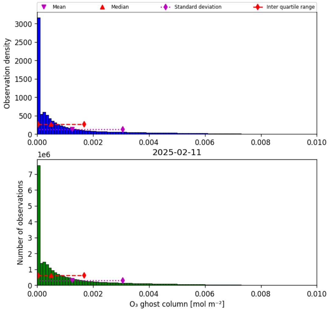
Figure 25: Histogram of “O 3 ghost column” for 2025-02-10 to 2025-02-12
