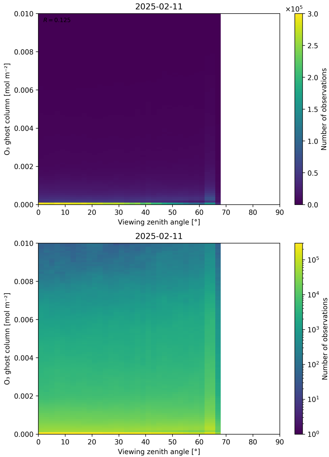
Figure 51: Scatter density plot of “Viewing zenith angle” against “O 3 ghost column” for 2025-02-10 to 2025-02-12.
