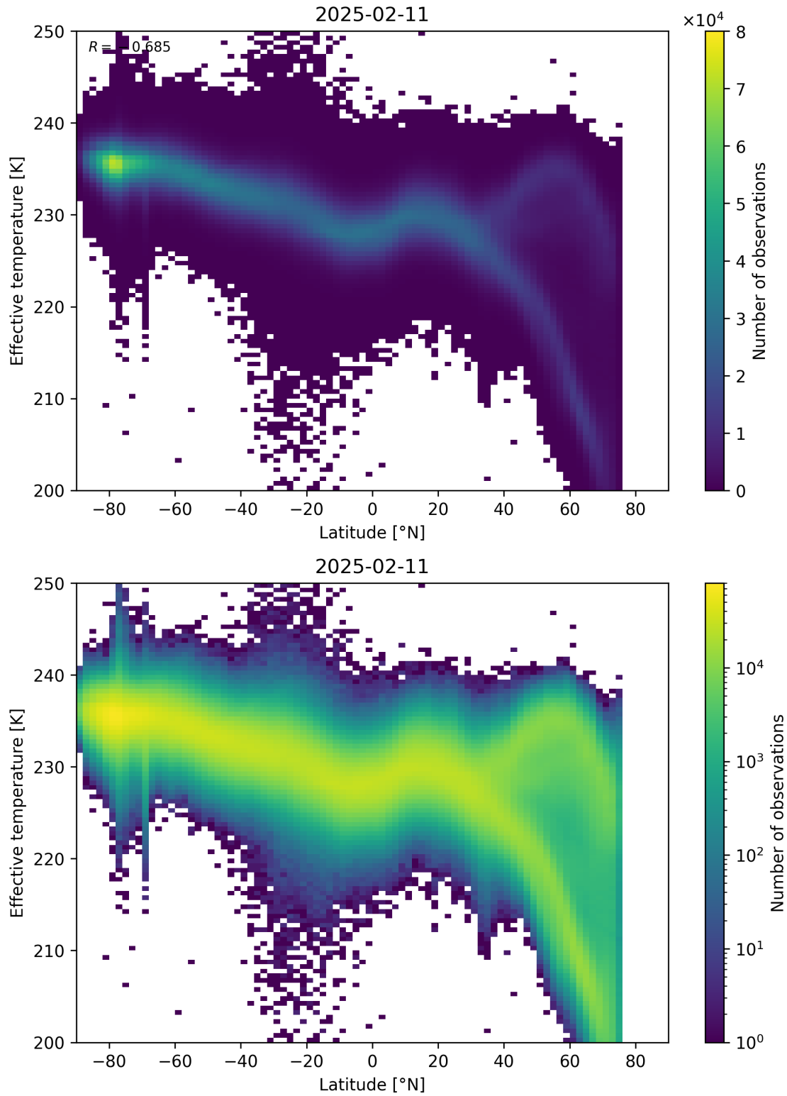
Figure 34: Scatter density plot of “Latitude” against “Effective temperature” for 2025-02-10 to 2025-02-12.
