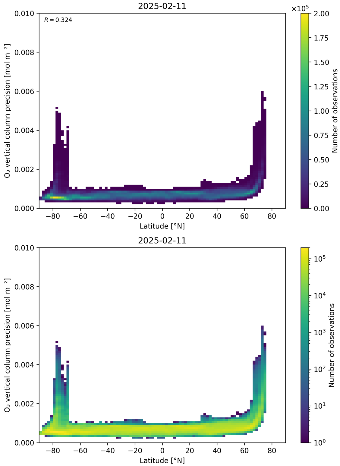
Figure 37: Scatter density plot of “Latitude” against “O 3 vertical column precision” for 2025-02-10 to 2025-02-12.
