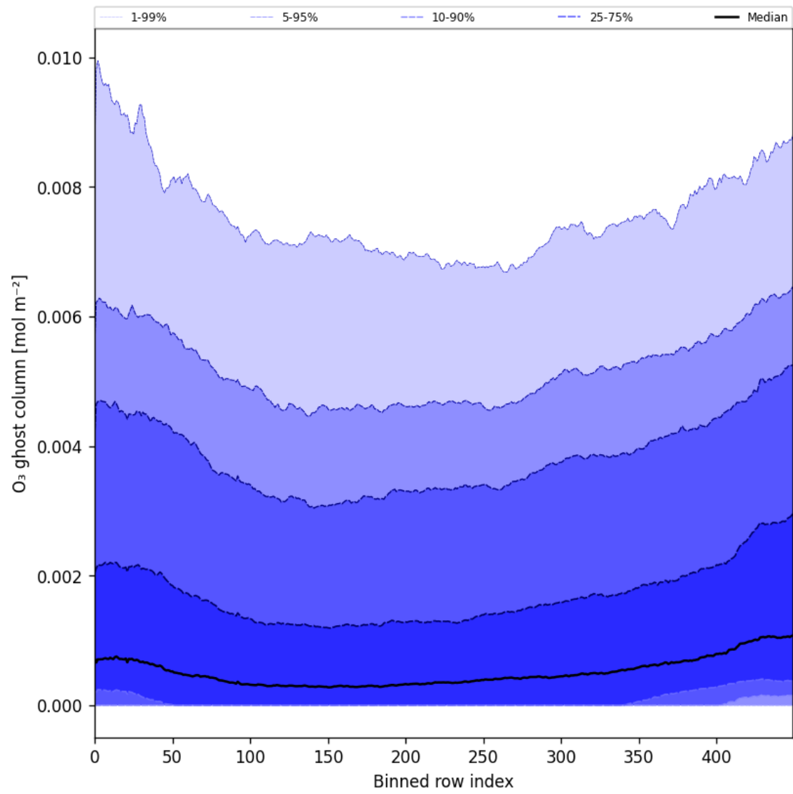
Figure 32: Along track statistics of “O 3 ghost column” for 2025-02-10 to 2025-02-12
