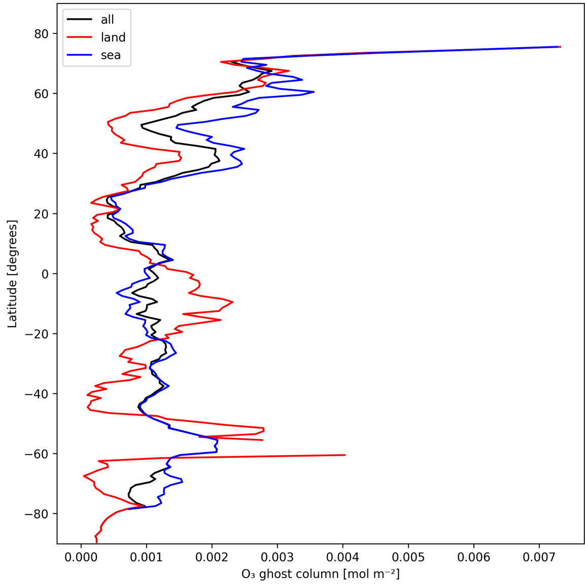
Figure 18: Zonal average of “O 3 ghost column” for 2025-02-10 to 2025-02-12.
