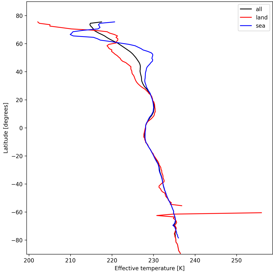
Figure 17: Zonal average of “Effective temperature” for 2025-02-10 to 2025-02-12.
