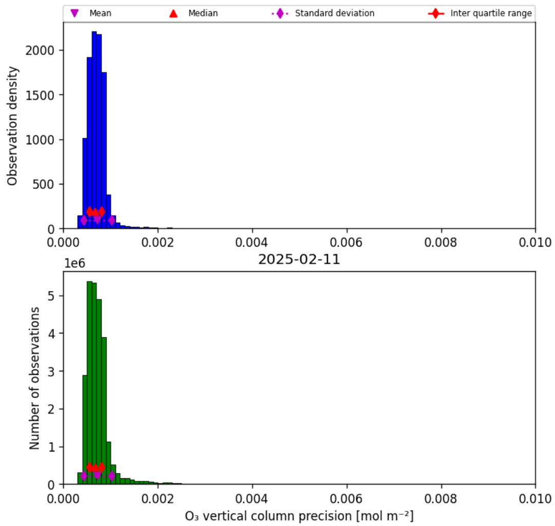
Figure 22: Histogram of “O 3 vertical column precision” for 2025-02-10 to 2025-02-12
