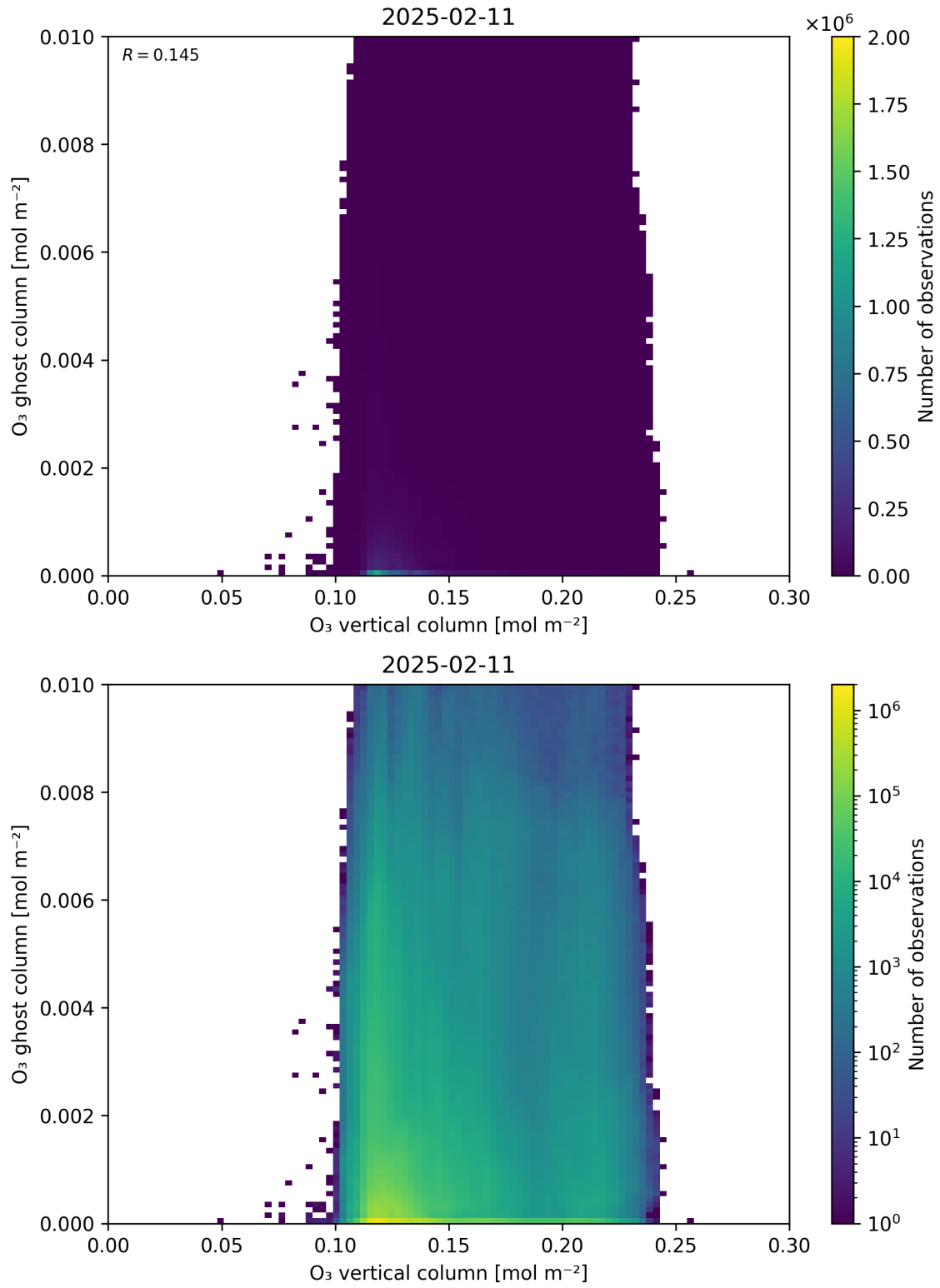
Figure 40: Scatter density plot of “O 3 vertical column” against “O 3 ghost column” for 2025-02-10 to 2025-02-12.
