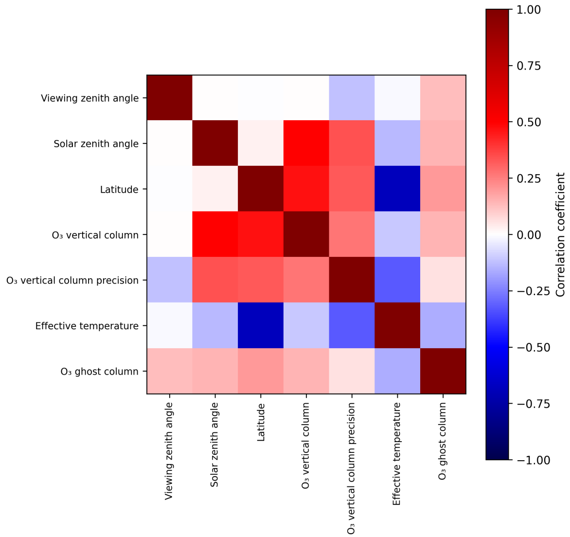
Figure 2: Map of correlation matrix for 2025-02-10 to 2025-02-12.
