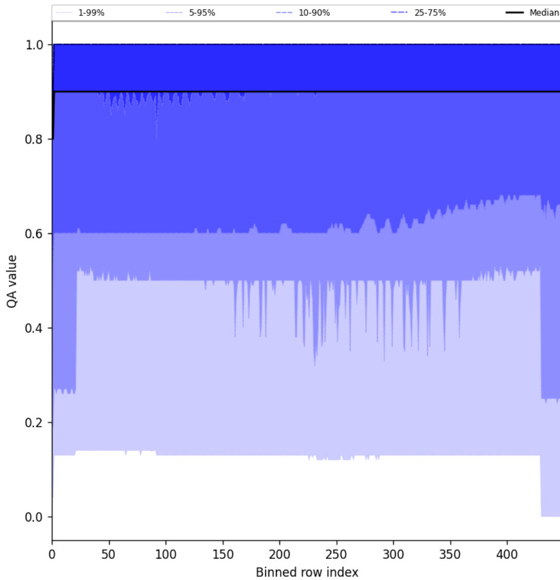
Figure 27: Along track statistics of “QA value” for 2025-02-10 to 2025-02-12
