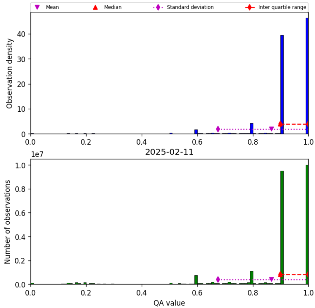
Figure 20: Histogram of “QA value” for 2025-02-10 to 2025-02-12
