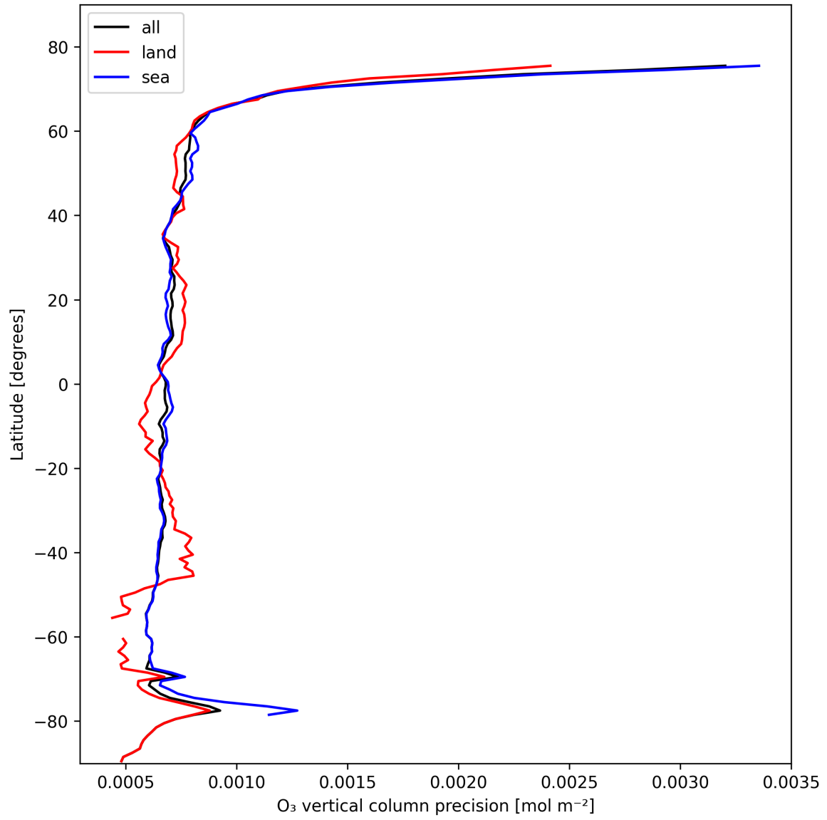
Figure 15: Zonal average of “O 3 vertical column precision” for 2025-02-10 to 2025-02-12.
