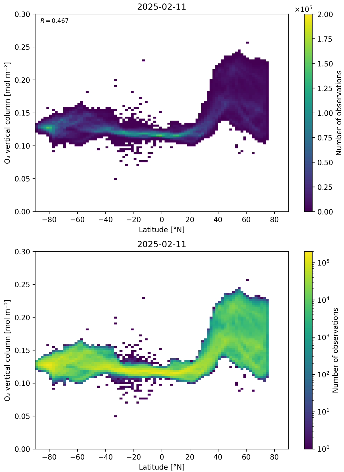
Figure 36: Scatter density plot of “Latitude” against “O 3 vertical column” for 2025-02-10 to 2025-02-12.
