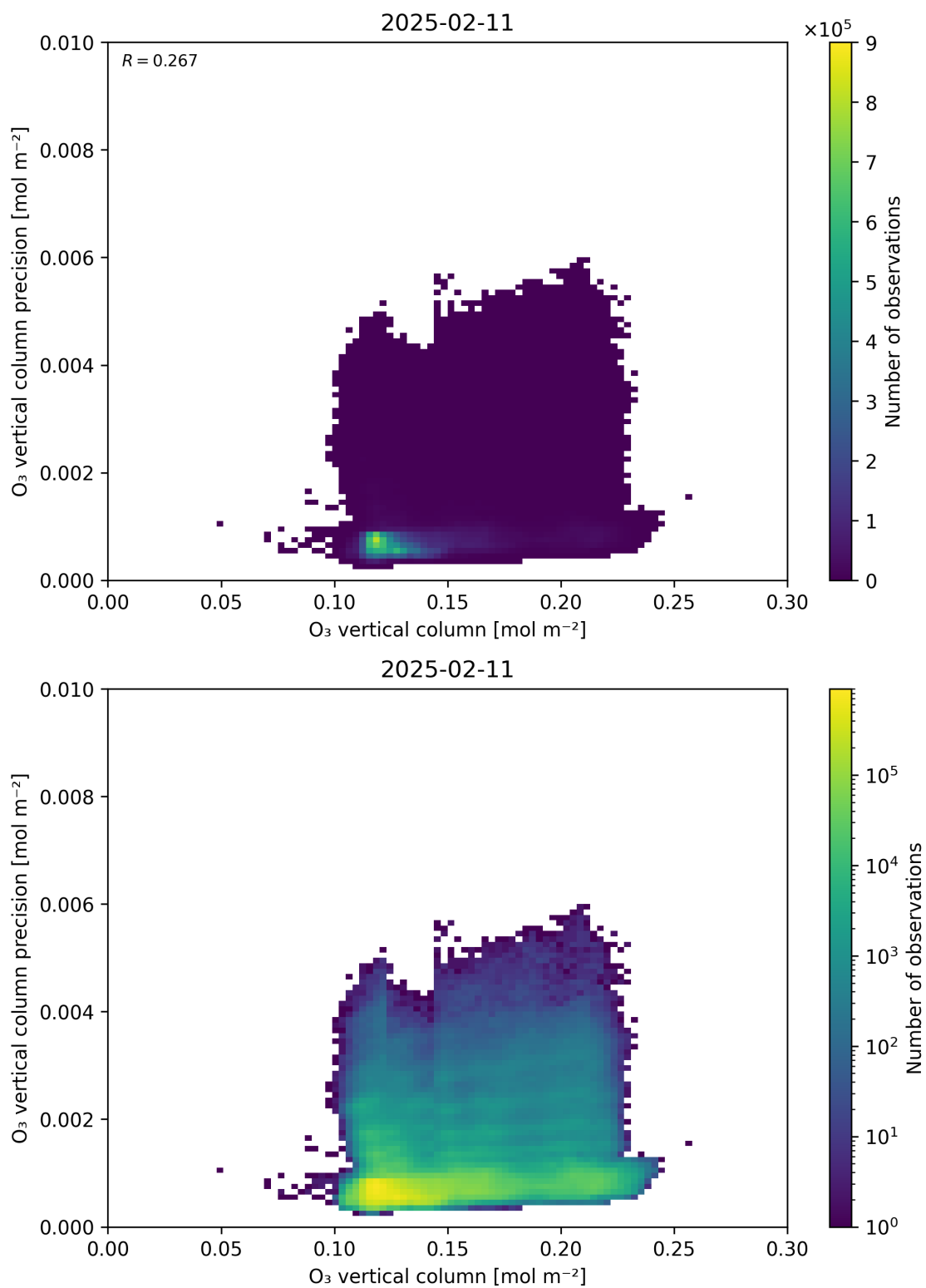
Figure 41: Scatter density plot of “O 3 vertical column” against “O 3 vertical column precision” for 2025-02-10 to 2025-02-12.
