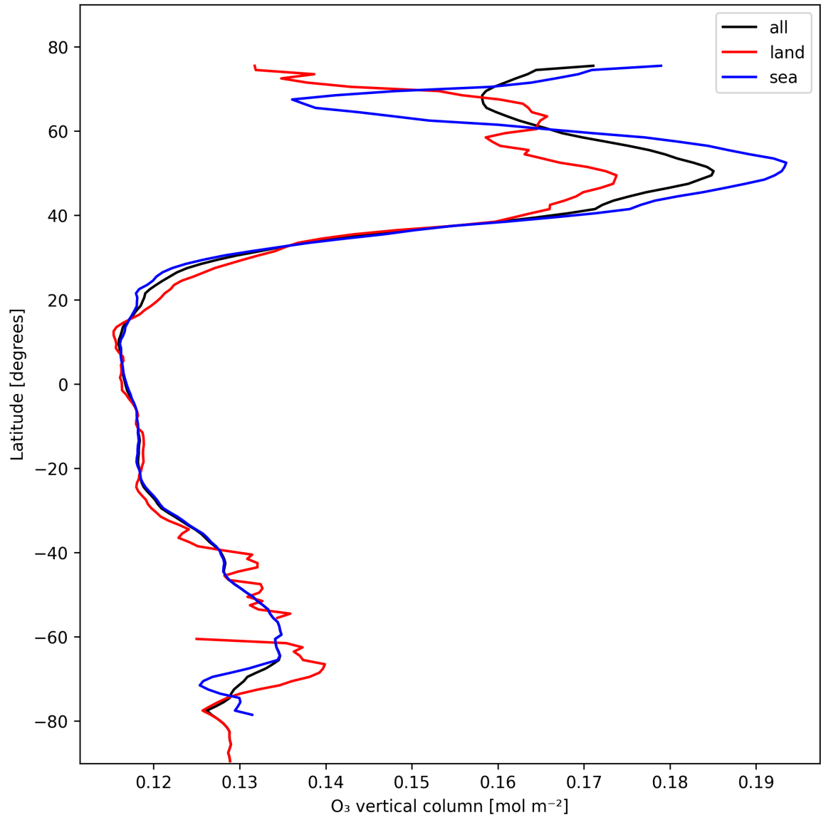
Figure 14: Zonal average of “O 3 vertical column” for 2025-02-10 to 2025-02-12.
