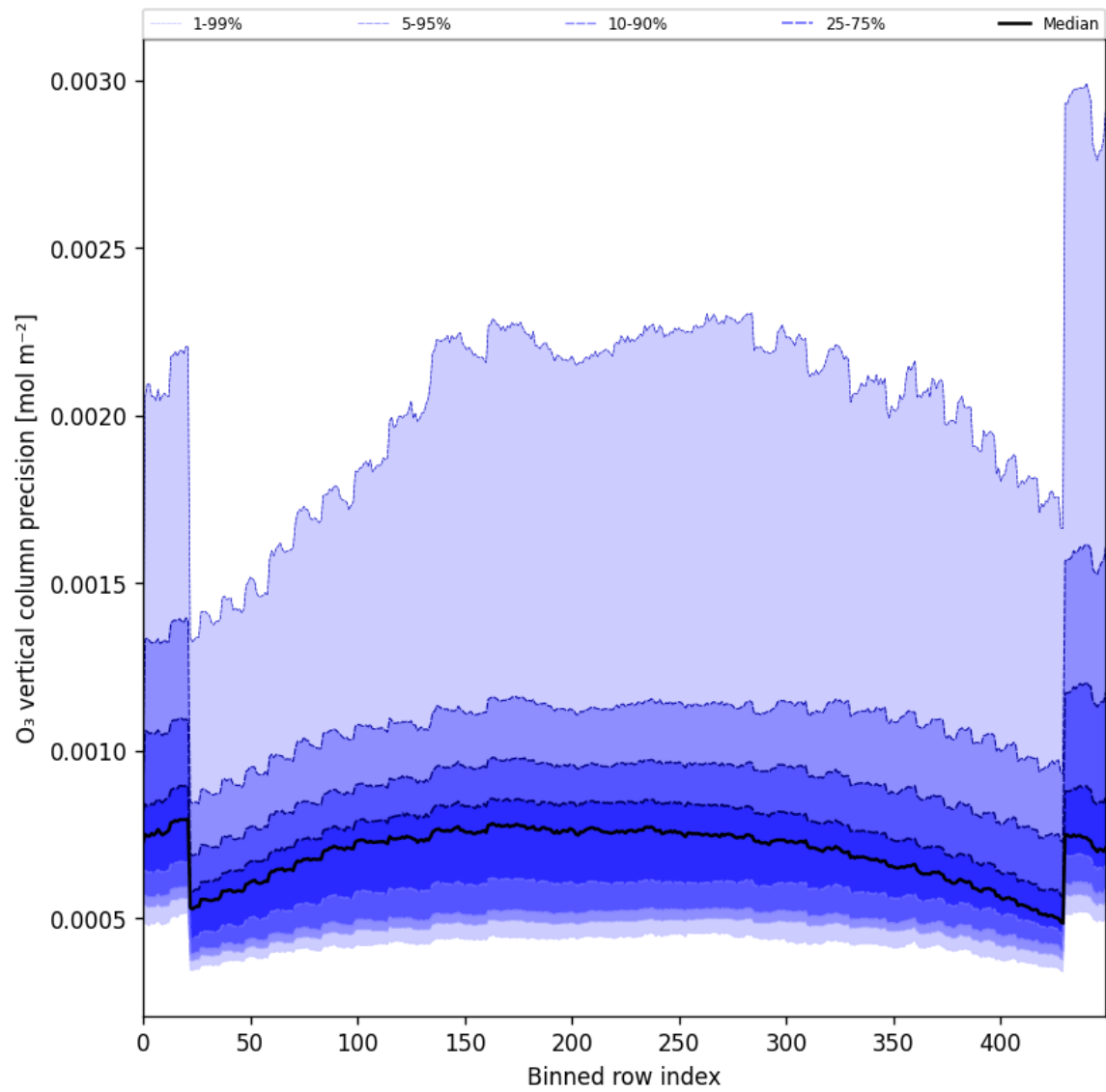
Figure 29: Along track statistics of “O 3 vertical column precision” for 2025-02-10 to 2025-02-12
