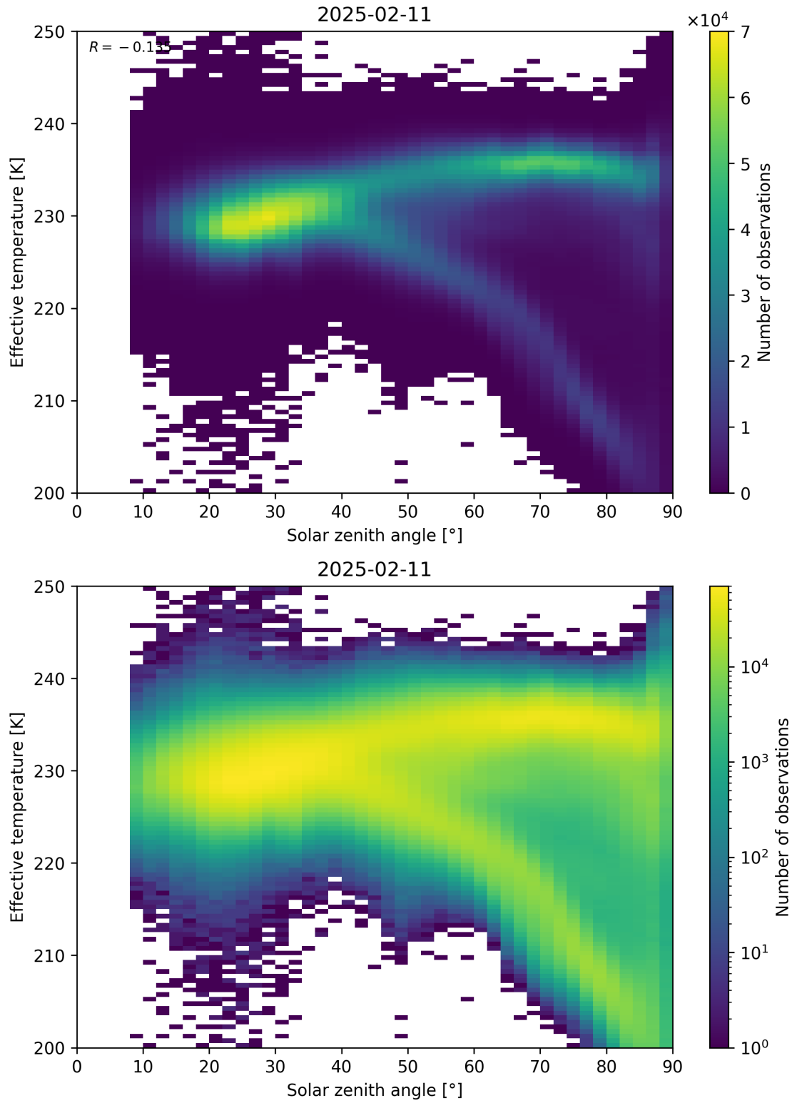
Figure 45: Scatter density plot of “Solar zenith angle” against “Effective temperature” for 2025-02-10 to 2025-02-12.
