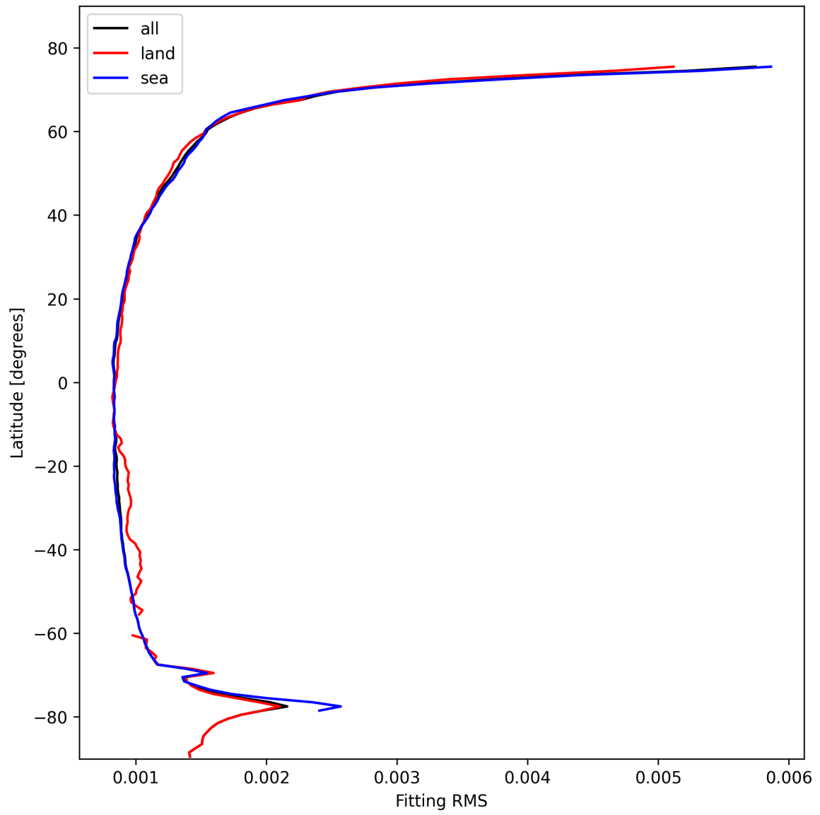
Figure 16: Zonal average of “Fitting RMS” for 2025-02-10 to 2025-02-12.
