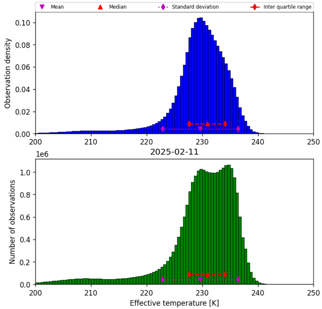
Figure 24: Histogram of “Effective temperature” for 2025-02-10 to 2025-02-12
