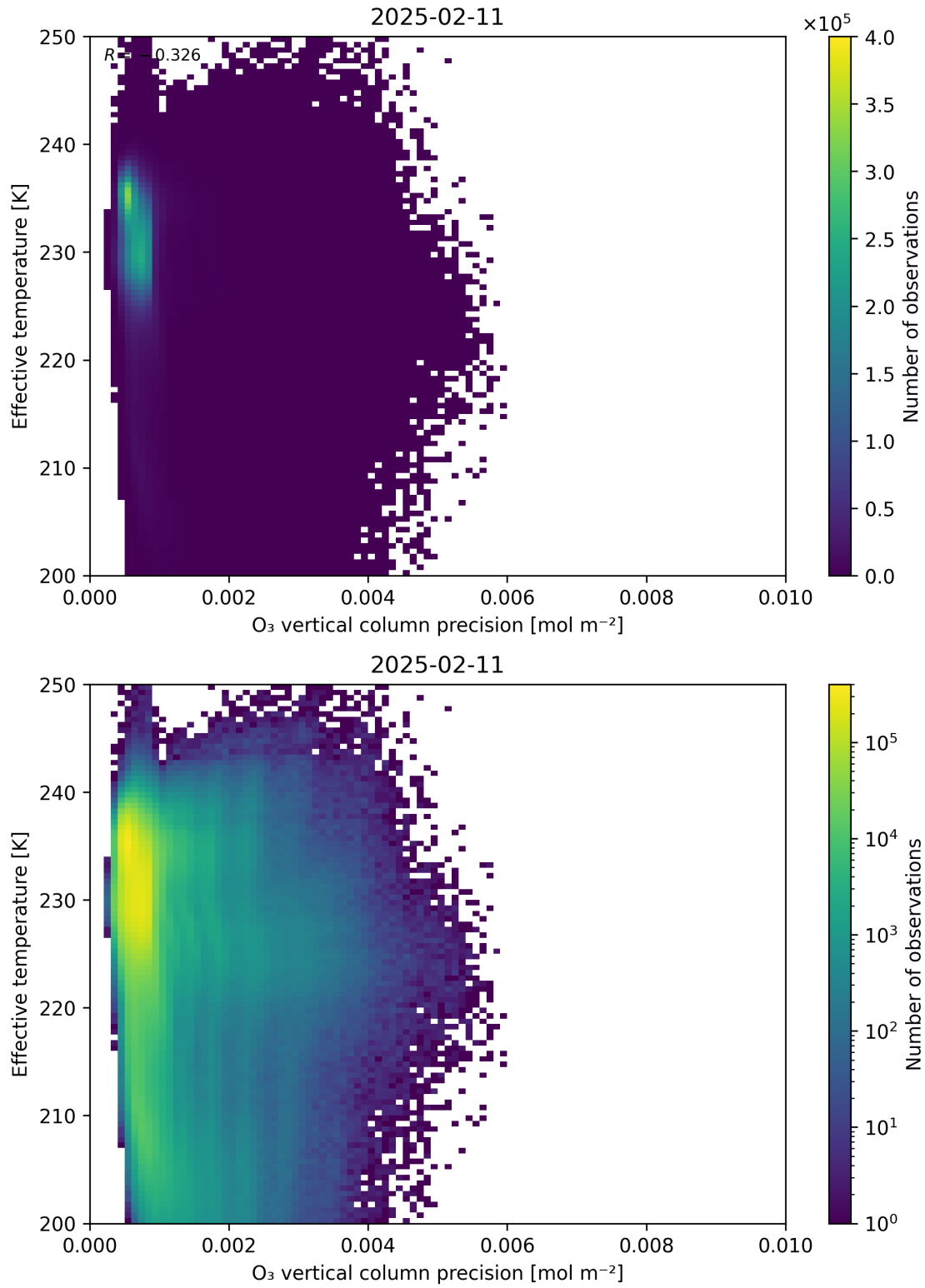
Figure 42: Scatter density plot of “O 3 vertical column precision” against “Effective temperature” for 2025-02-10 to 2025-02-12.
