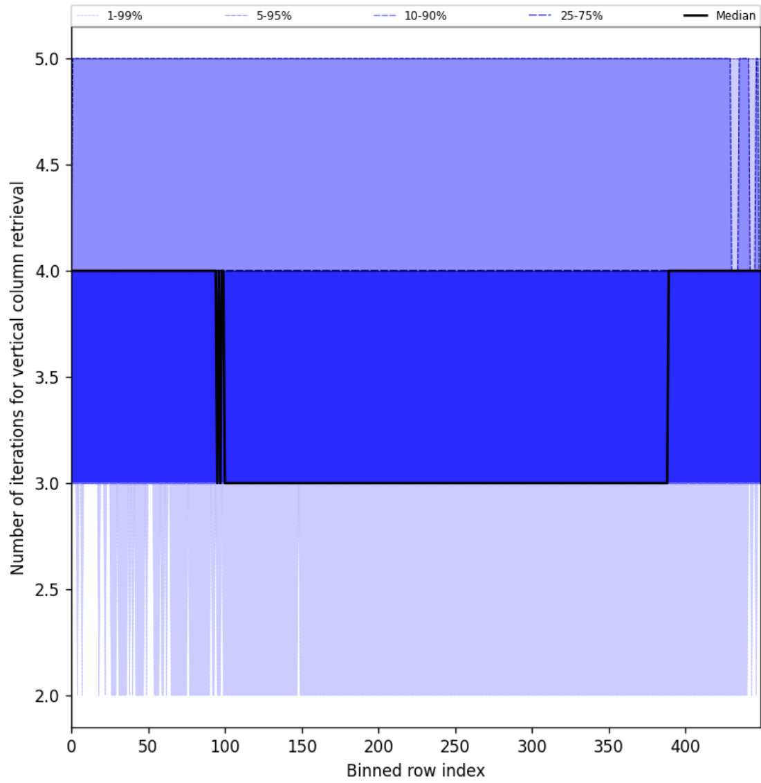
Figure 33: Along track statistics of “Number of iterations for vertical column retrieval” for 2025-02-10 to 2025-02-12
