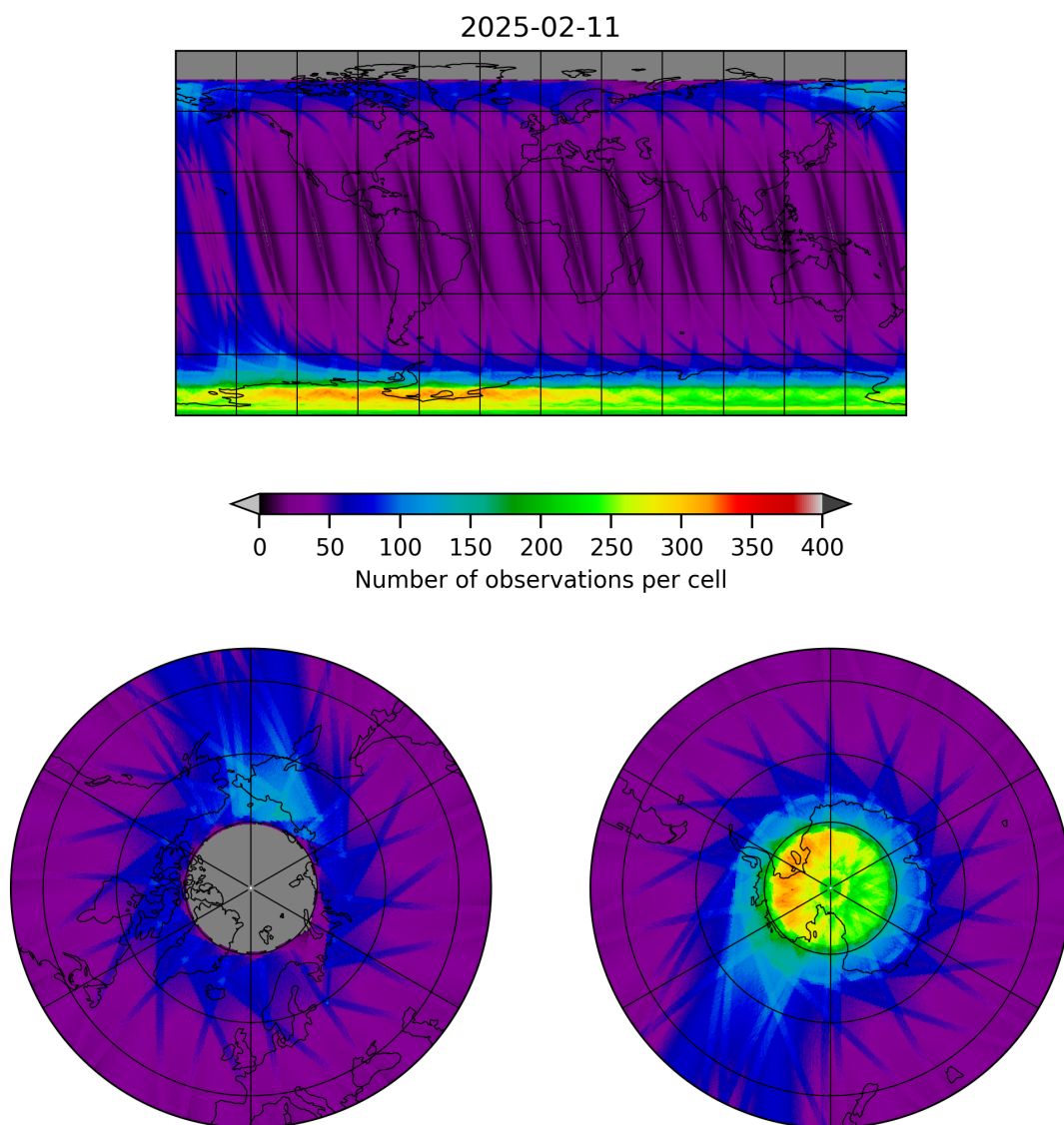
Figure 12: Map of the number of observations for 2025-02-10 to 2025-02-12
