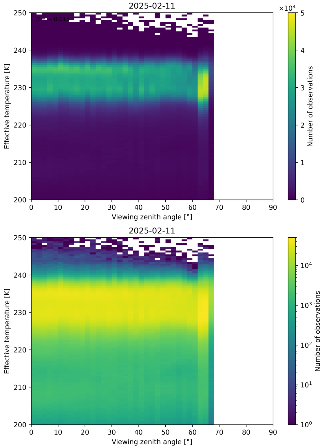
Figure 50: Scatter density plot of “Viewing zenith angle” against “Effective temperature” for 2025-02-10 to 2025-02-12.
