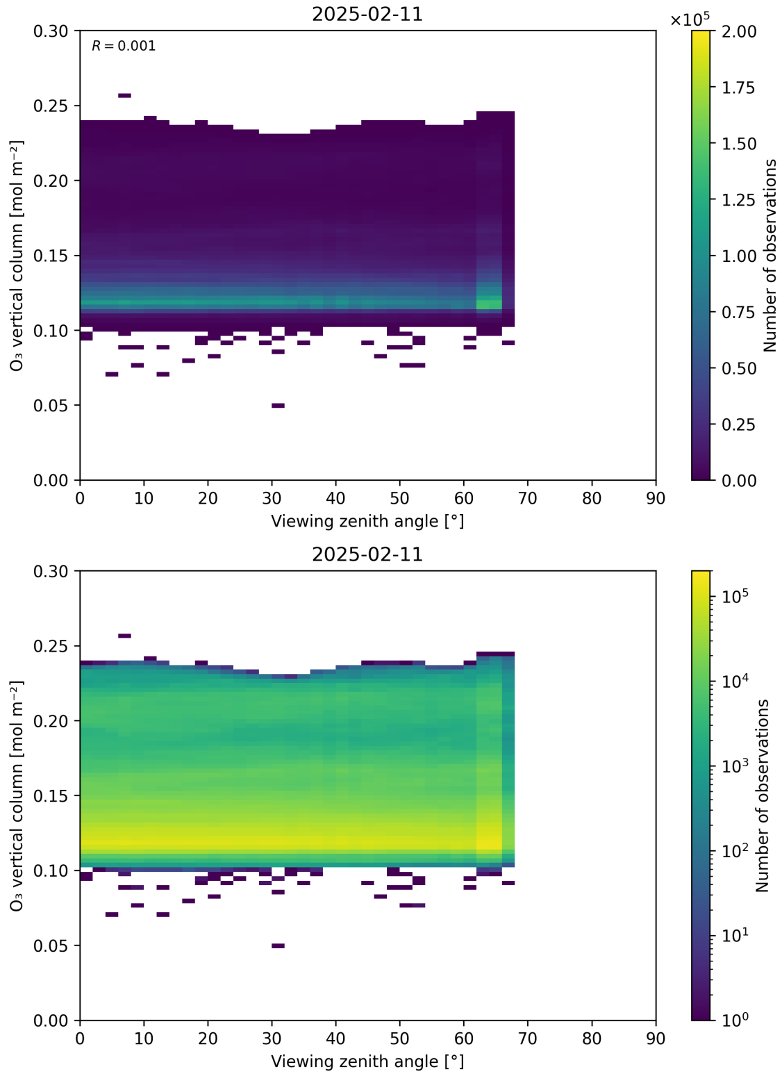
Figure 52: Scatter density plot of “Viewing zenith angle” against “O 3 vertical column” for 2025-02-10 to 2025-02-12.
