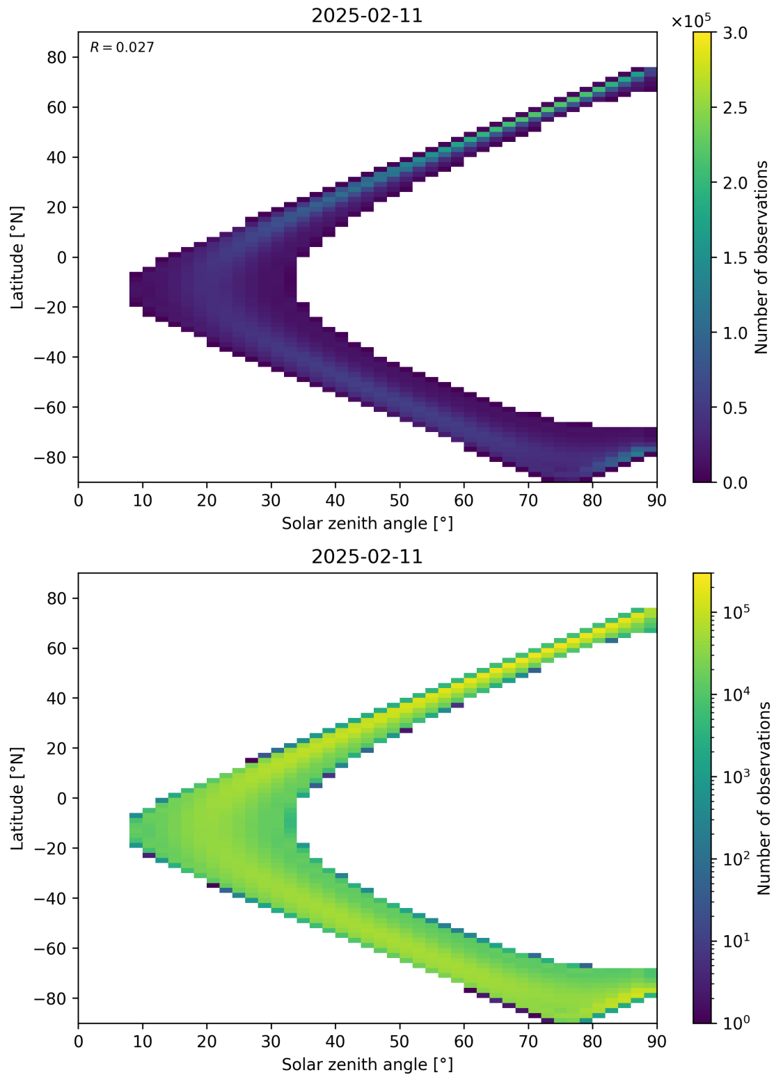
Figure 44: Scatter density plot of “Solar zenith angle” against “Latitude” for 2025-02-10 to 2025-02-12.
