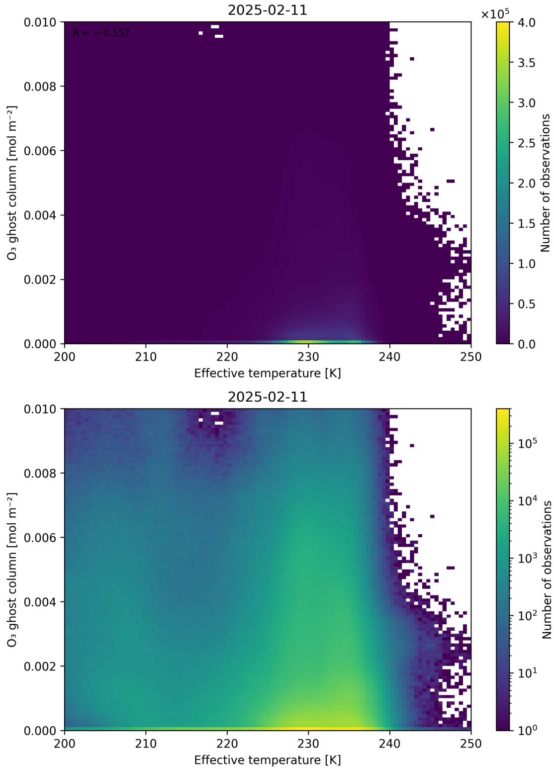
Figure 38: Scatter density plot of “Effective temperature” against “O 3 ghost column” for 2025-02-10 to 2025-02-12.
