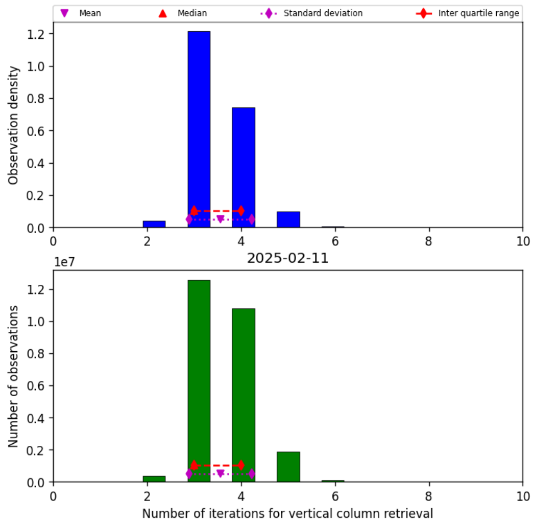
Figure 26: Histogram of “Number of iterations for vertical column retrieval” for 2025-02-10 to 2025-02-12
