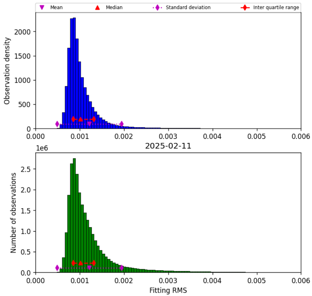
Figure 23: Histogram of “Fitting RMS” for 2025-02-10 to 2025-02-12
