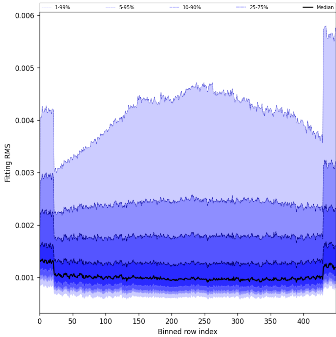
Figure 30: Along track statistics of “Fitting RMS” for 2025-02-10 to 2025-02-12
