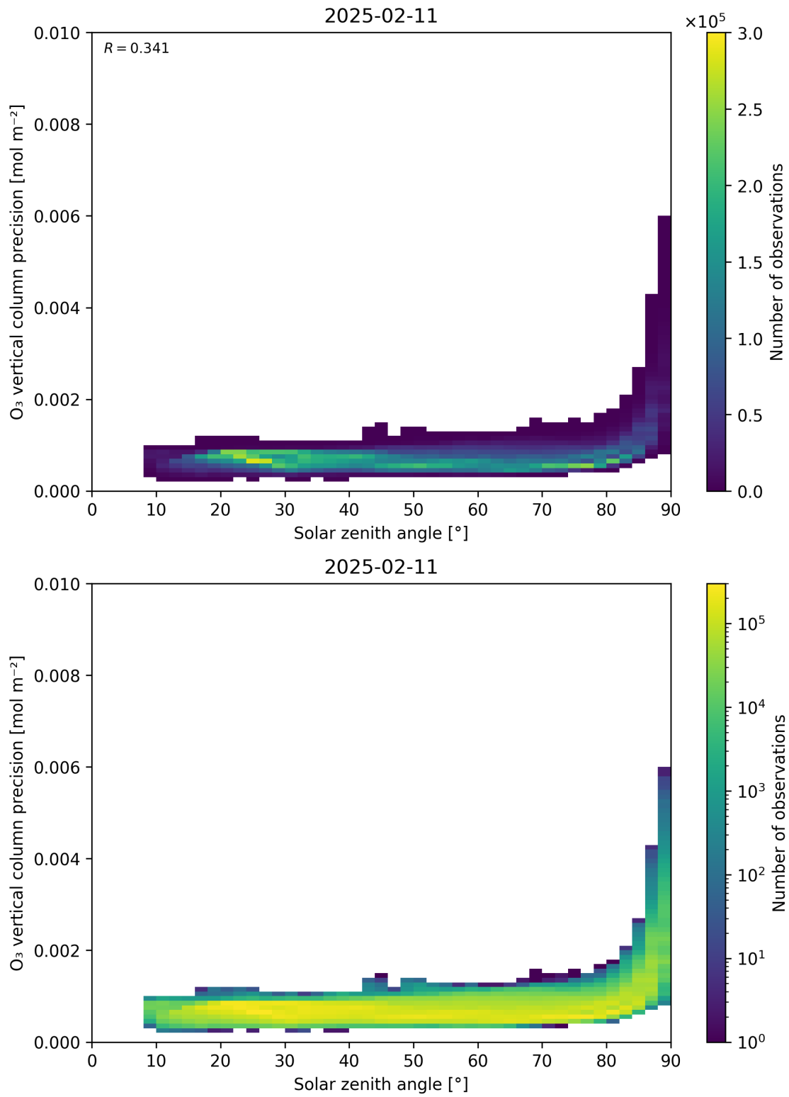
Figure 48: Scatter density plot of “Solar zenith angle” against “O 3 vertical column precision” for 2025-02-10 to 2025-02-12.
