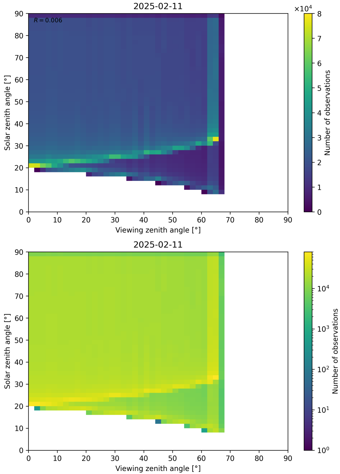
Figure 54: Scatter density plot of “Viewing zenith angle” against “Solar zenith angle” for 2025-02-10 to 2025-02-12.
