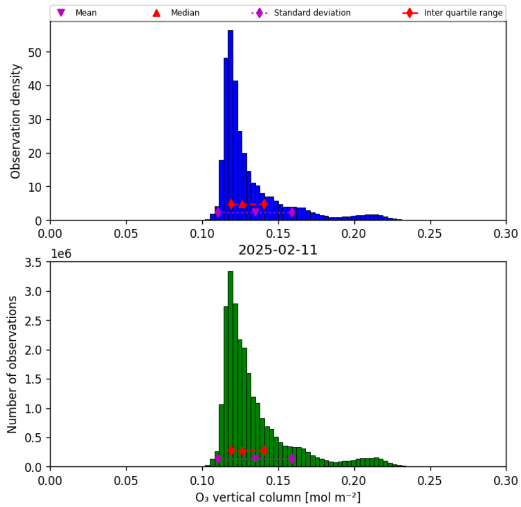
Figure 21: Histogram of “O 3 vertical column” for 2025-02-10 to 2025-02-12
