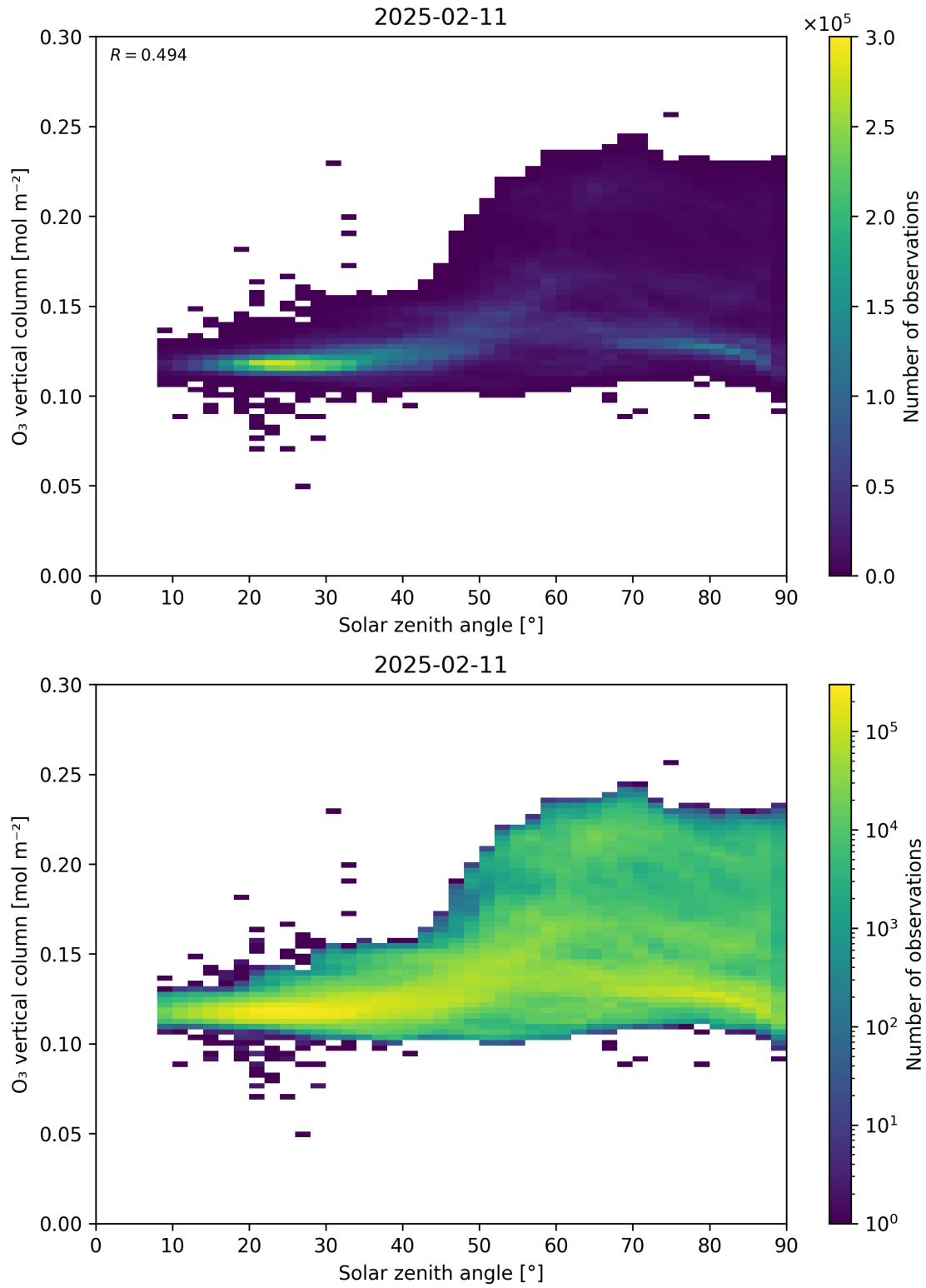
Figure 47: Scatter density plot of “Solar zenith angle” against “O 3 vertical column” for 2025-02-10 to 2025-02-12.
