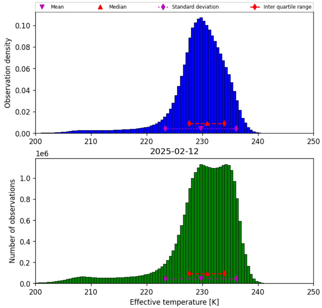
Figure 24: Histogram of “Effective temperature” for 2025-02-11 to 2025-02-13
