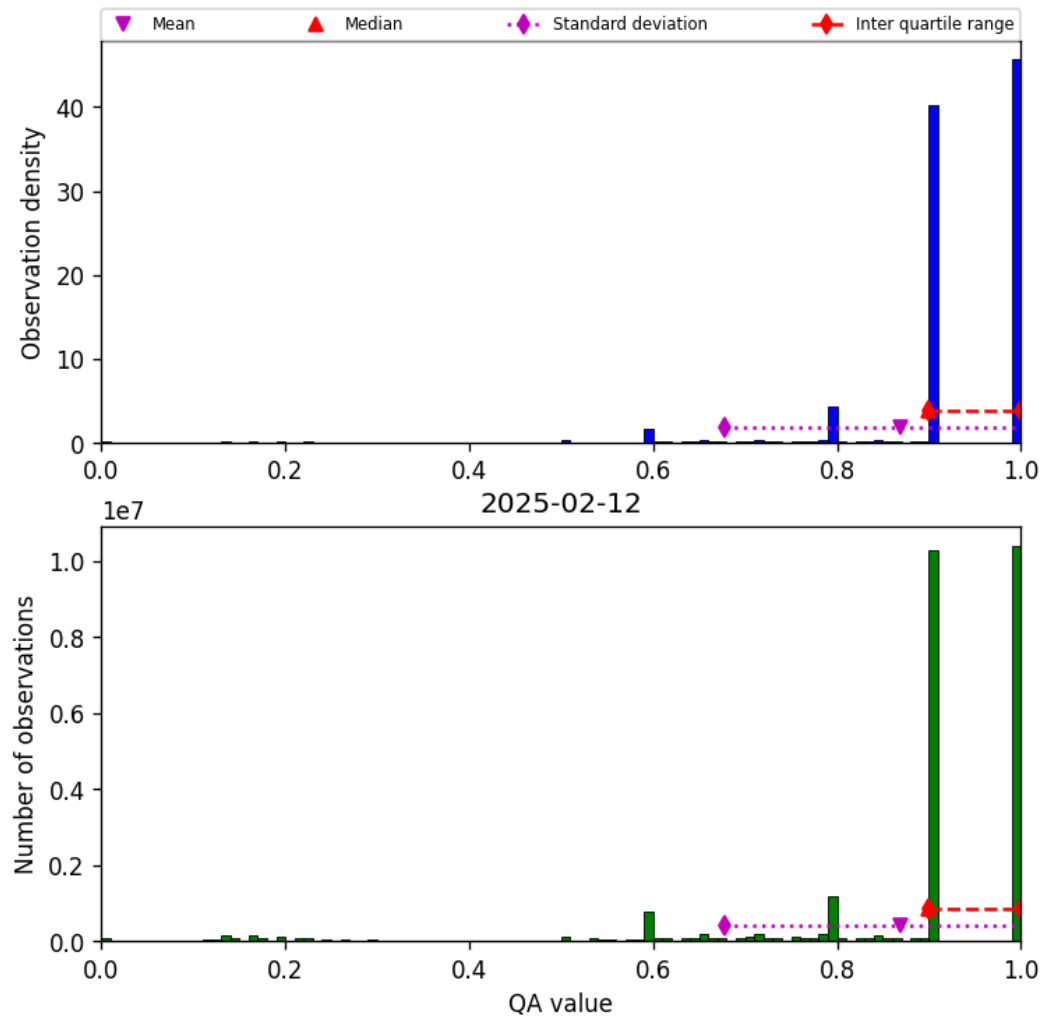
Figure 20: Histogram of “QA value” for 2025-02-11 to 2025-02-13
