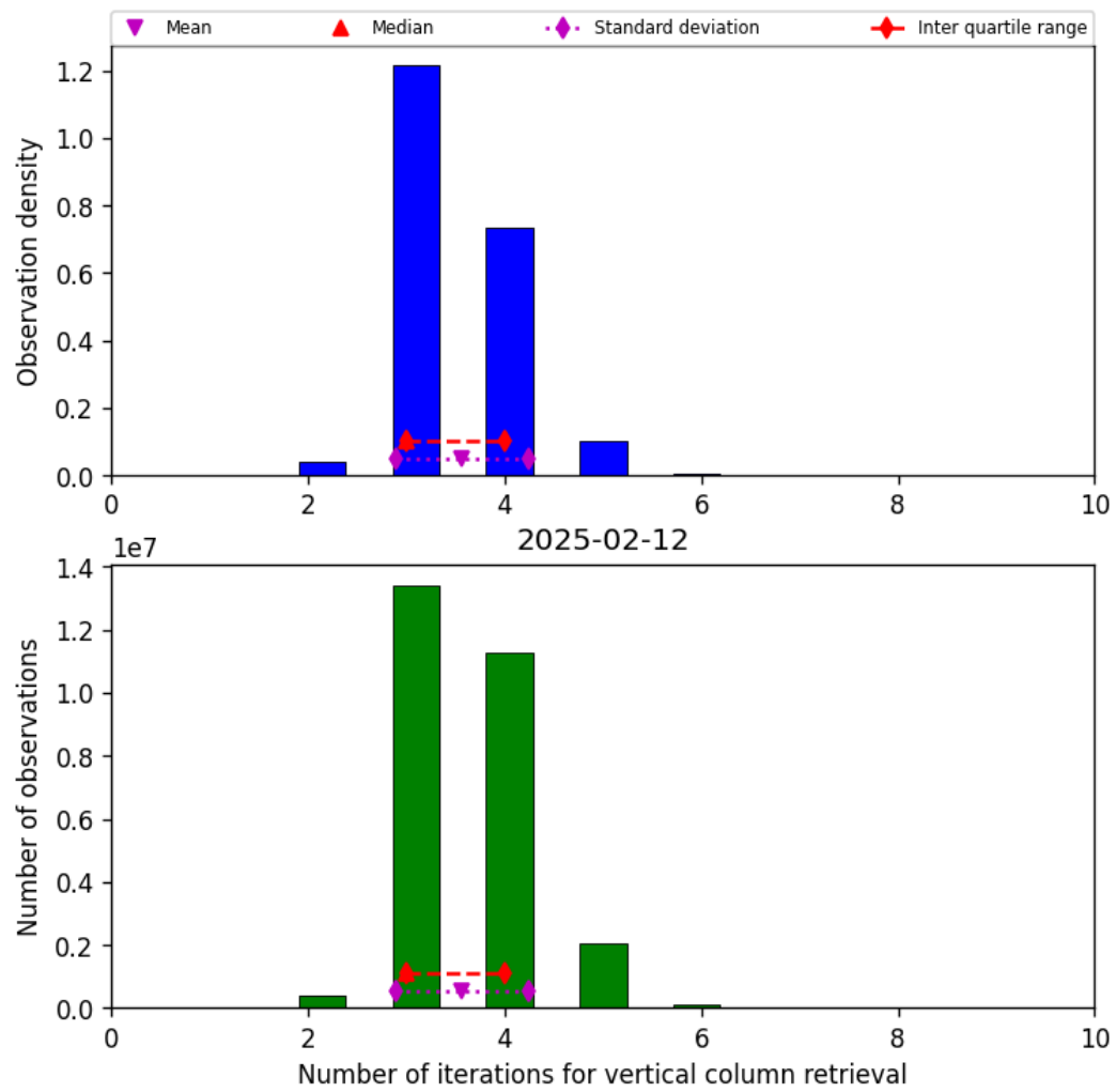
Figure 26: Histogram of “Number of iterations for vertical column retrieval” for 2025-02-11 to 2025-02-13
