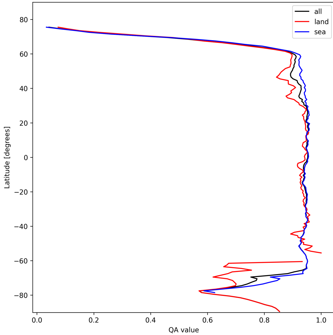
Figure 13: Zonal average of “QA value” for 2025-02-11 to 2025-02-13.
