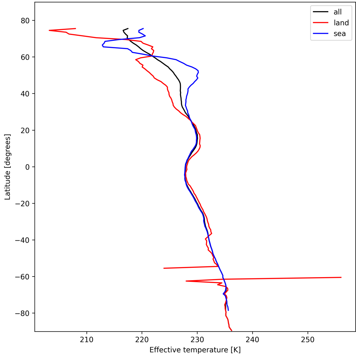
Figure 17: Zonal average of "Effective temperature" for 2025-02-11 to 2025-02-13.
