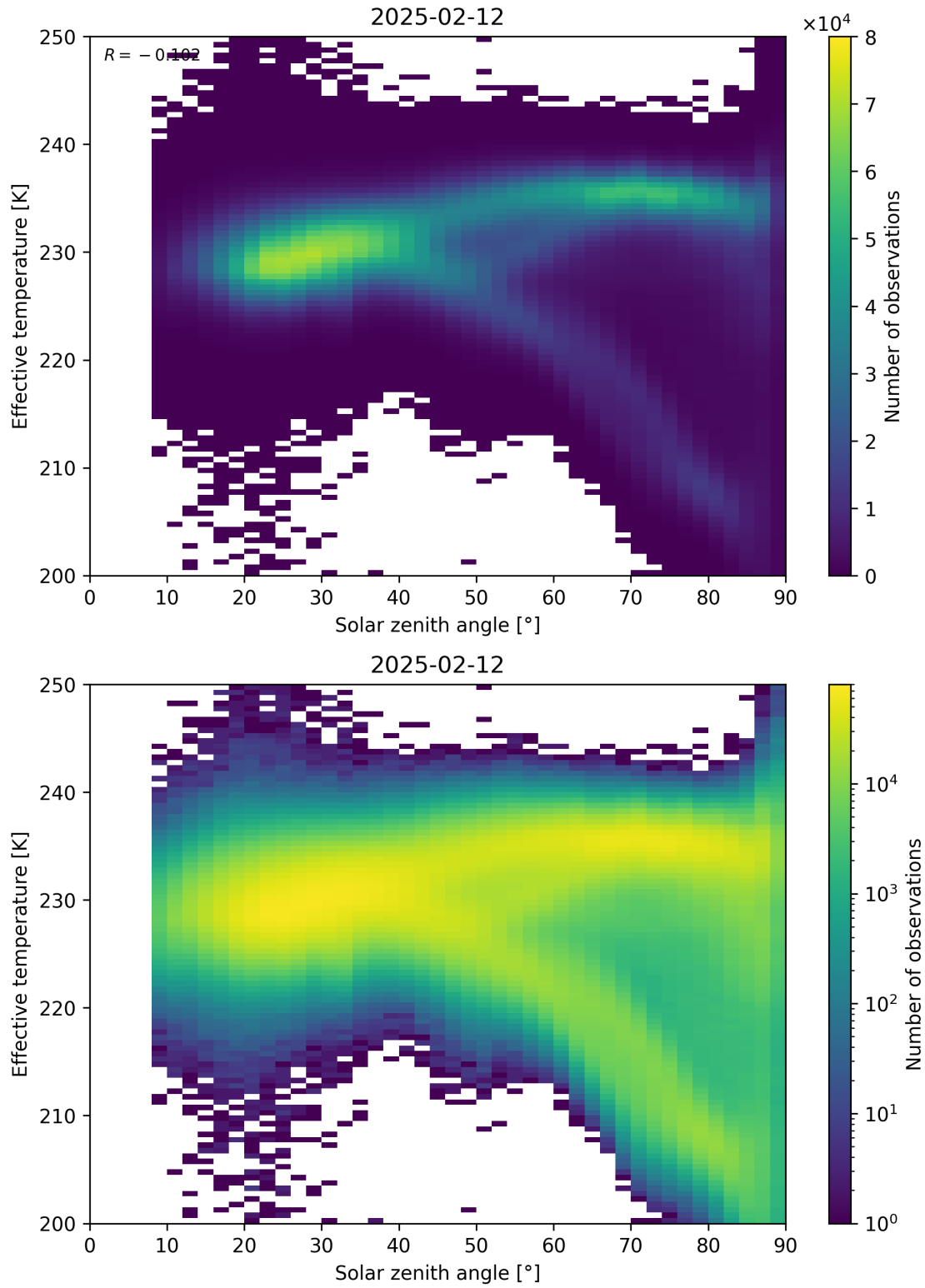
Figure 45: Scatter density plot of “Solar zenith angle” against “Effective temperature” for 2025-02-11 to 2025-02-13.
