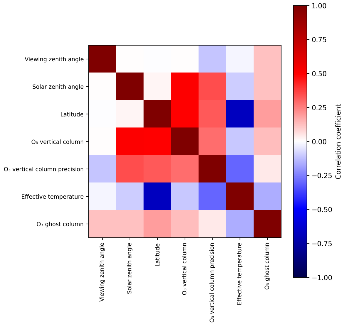
Figure 2: Map of correlation matrix for 2025-02-11 to 2025-02-13.
