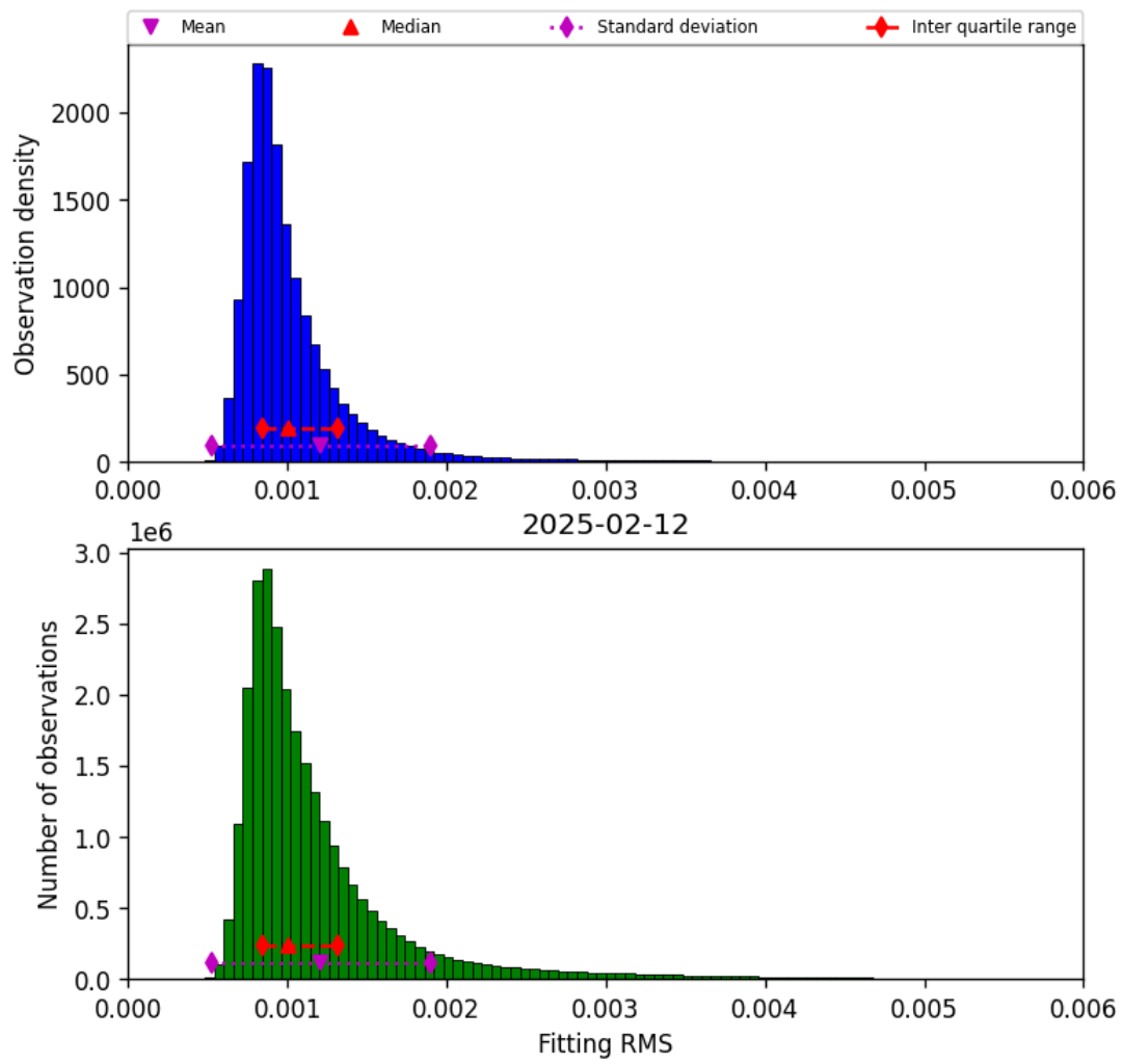
Figure 23: Histogram of “Fitting RMS” for 2025-02-11 to 2025-02-13
