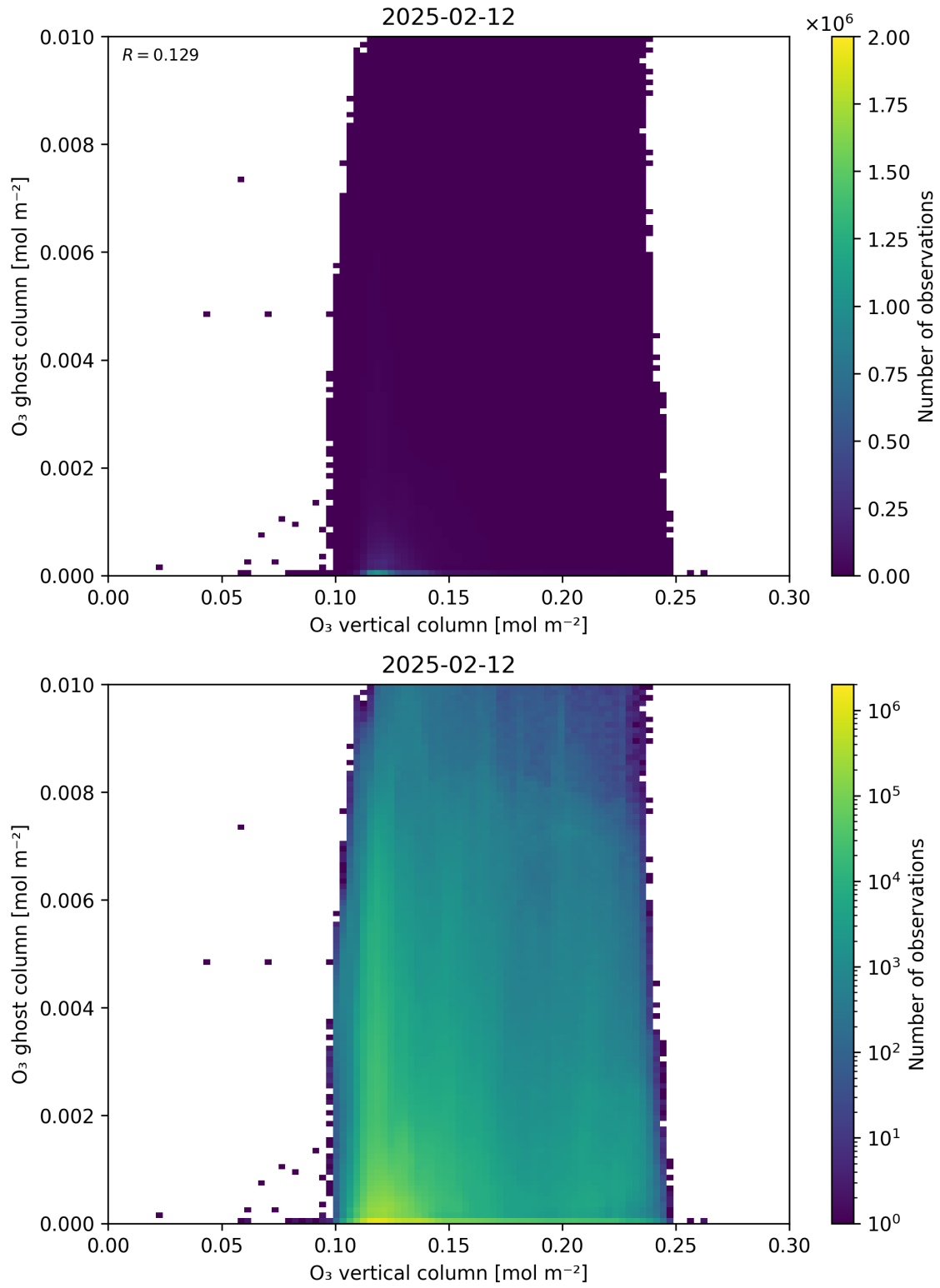
Figure 40: Scatter density plot of “O 3 vertical column” against “O 3 ghost column” for 2025-02-11 to 2025-02-13.
