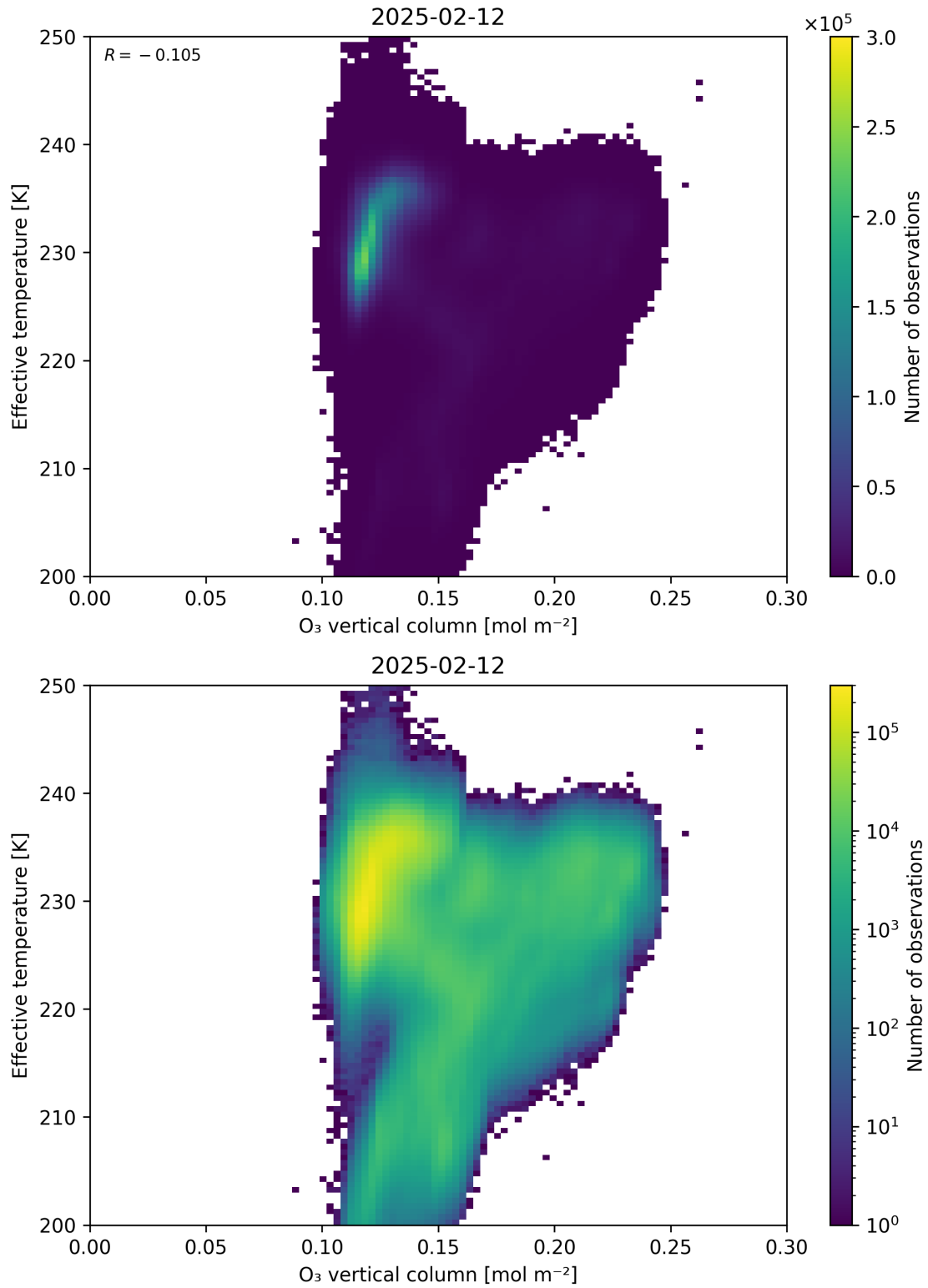
Figure 39: Scatter density plot of “O 3 vertical column” against “Effective temperature” for 2025-02-11 to 2025-02-13.
