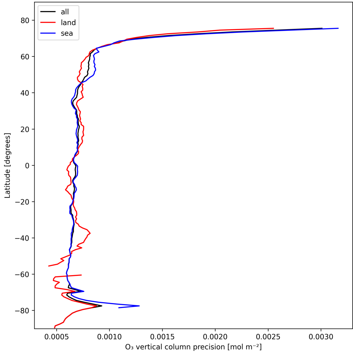
Figure 15: Zonal average of “O 3 vertical column precision” for 2025-02-11 to 2025-02-13.
