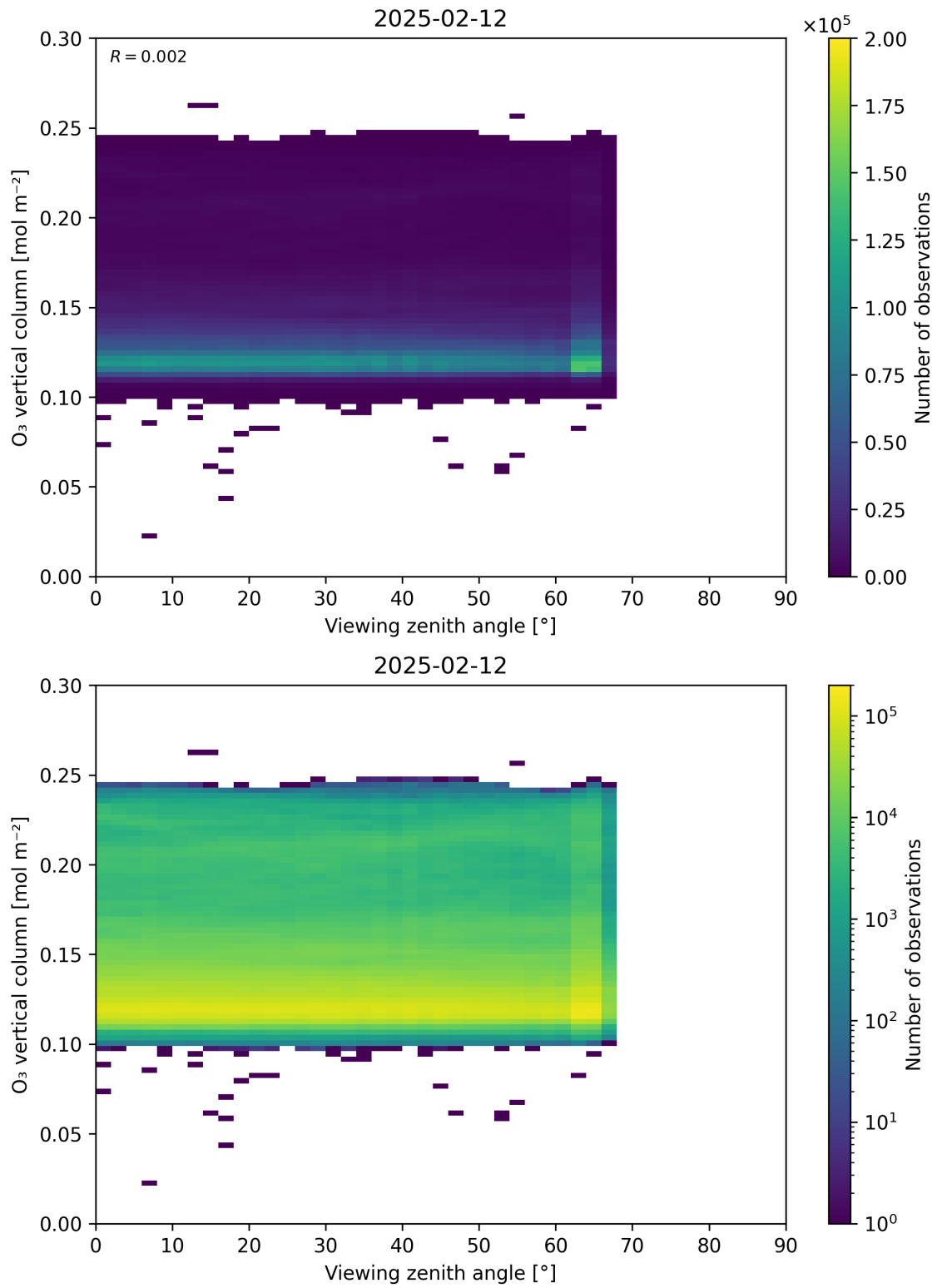
Figure 52: Scatter density plot of “Viewing zenith angle” against “O 3 vertical column” for 2025-02-11 to 2025-02-13.
