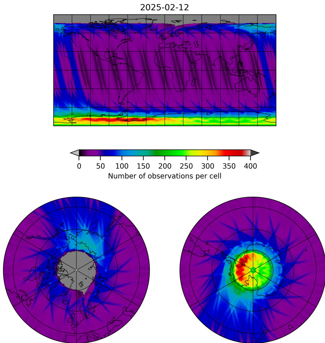
Figure 12: Map of the number of observations for 2025-02-11 to 2025-02-13
