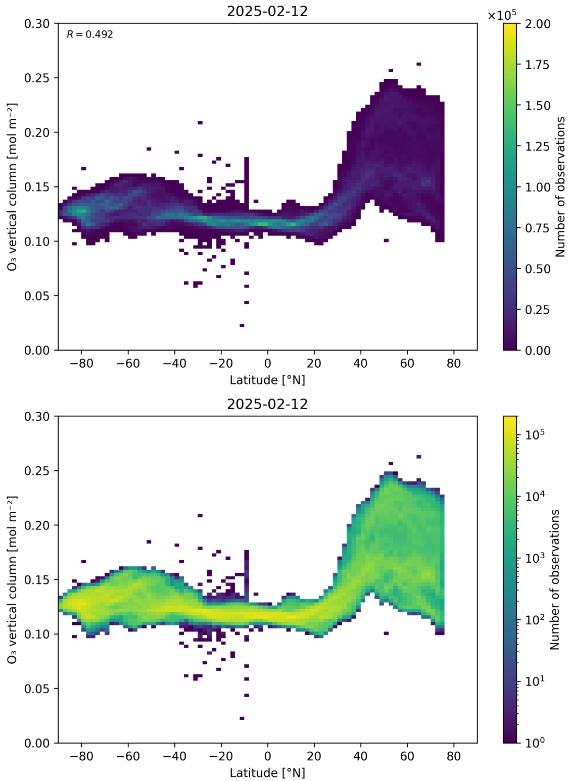
Figure 36: Scatter density plot of “Latitude” against “O 3 vertical column” for 2025-02-11 to 2025-02-13.
