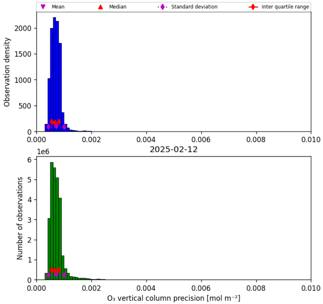
Figure 22: Histogram of “O 3 vertical column precision” for 2025-02-11 to 2025-02-13
