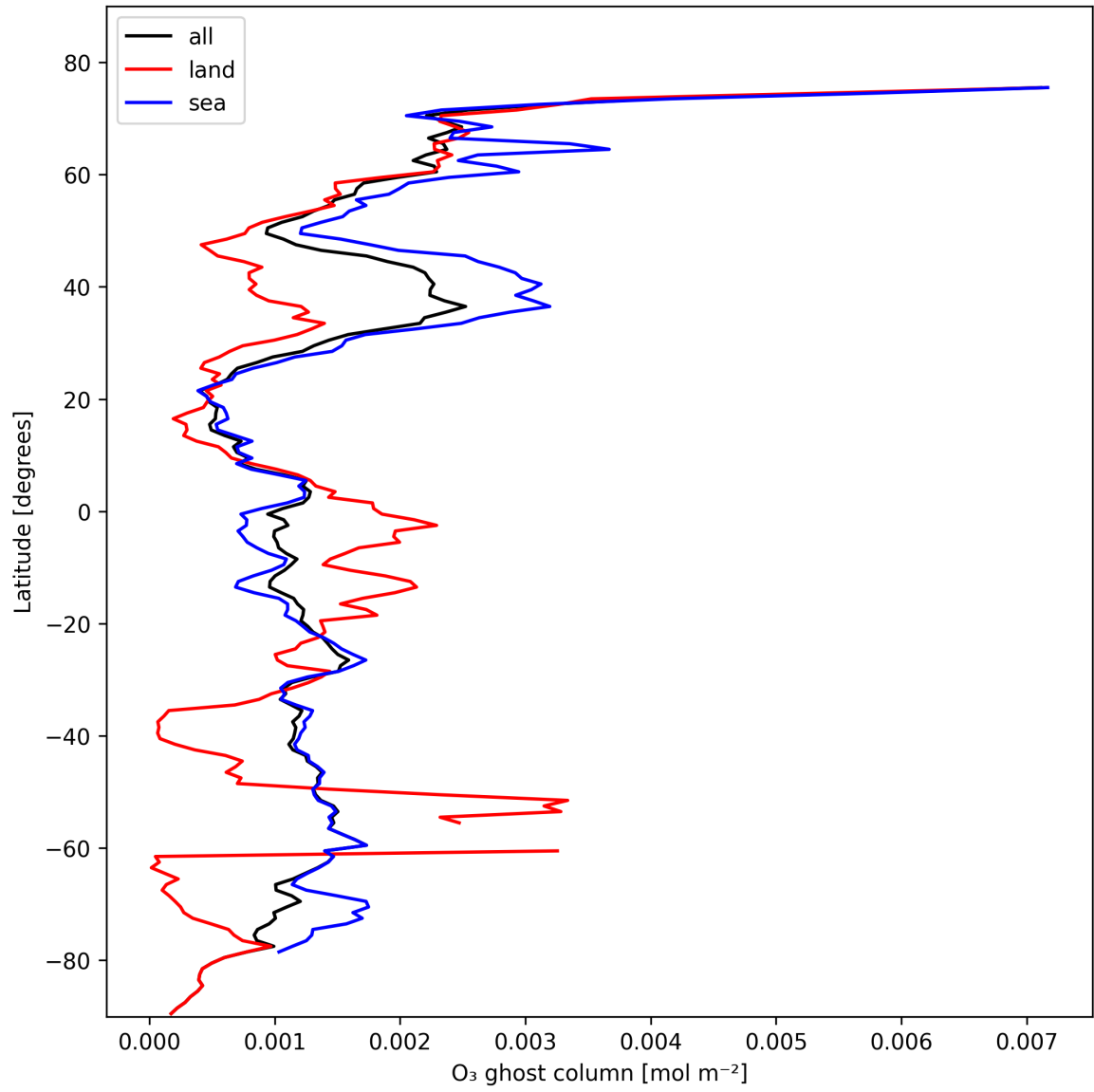
Figure 18: Zonal average of "O 3 ghost column" for 2025-02-11 to 2025-02-13.
