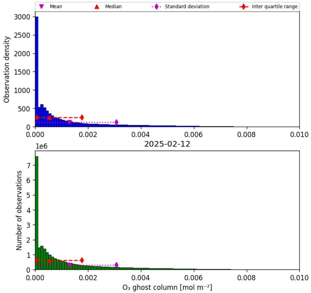
Figure 25: Histogram of “O 3 ghost column” for 2025-02-11 to 2025-02-13
