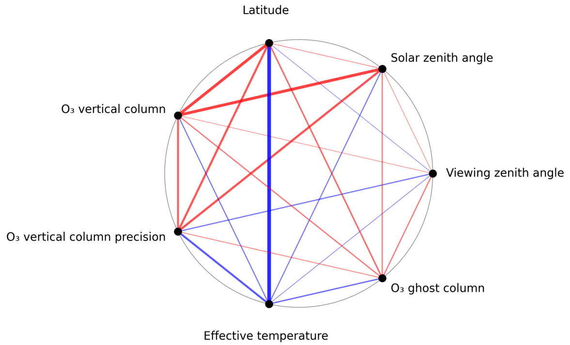
Figure 1: Map of correlation graph for 2025-02-11 to 2025-02-13.
