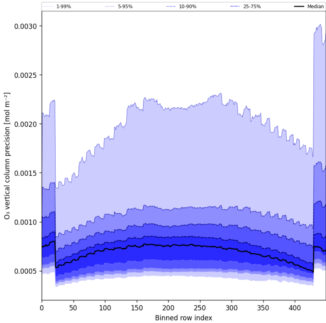
Figure 29: Along track statistics of “O 3 vertical column precision” for 2025-02-11 to 2025-02-13
