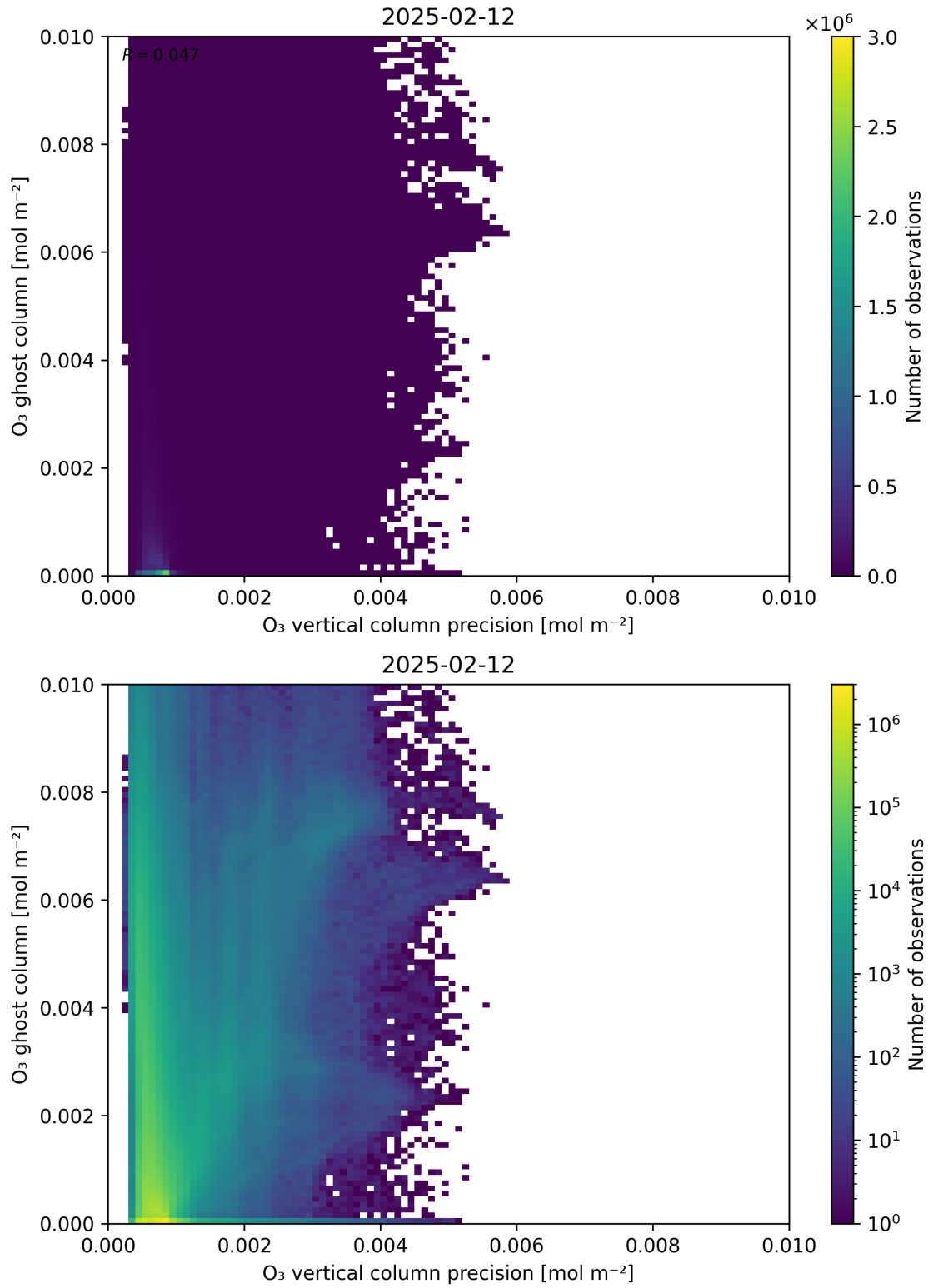
Figure 43: Scatter density plot of “O 3 vertical column precision” against “O 3 ghost column” for 2025-02-11 to 2025-02-13.
