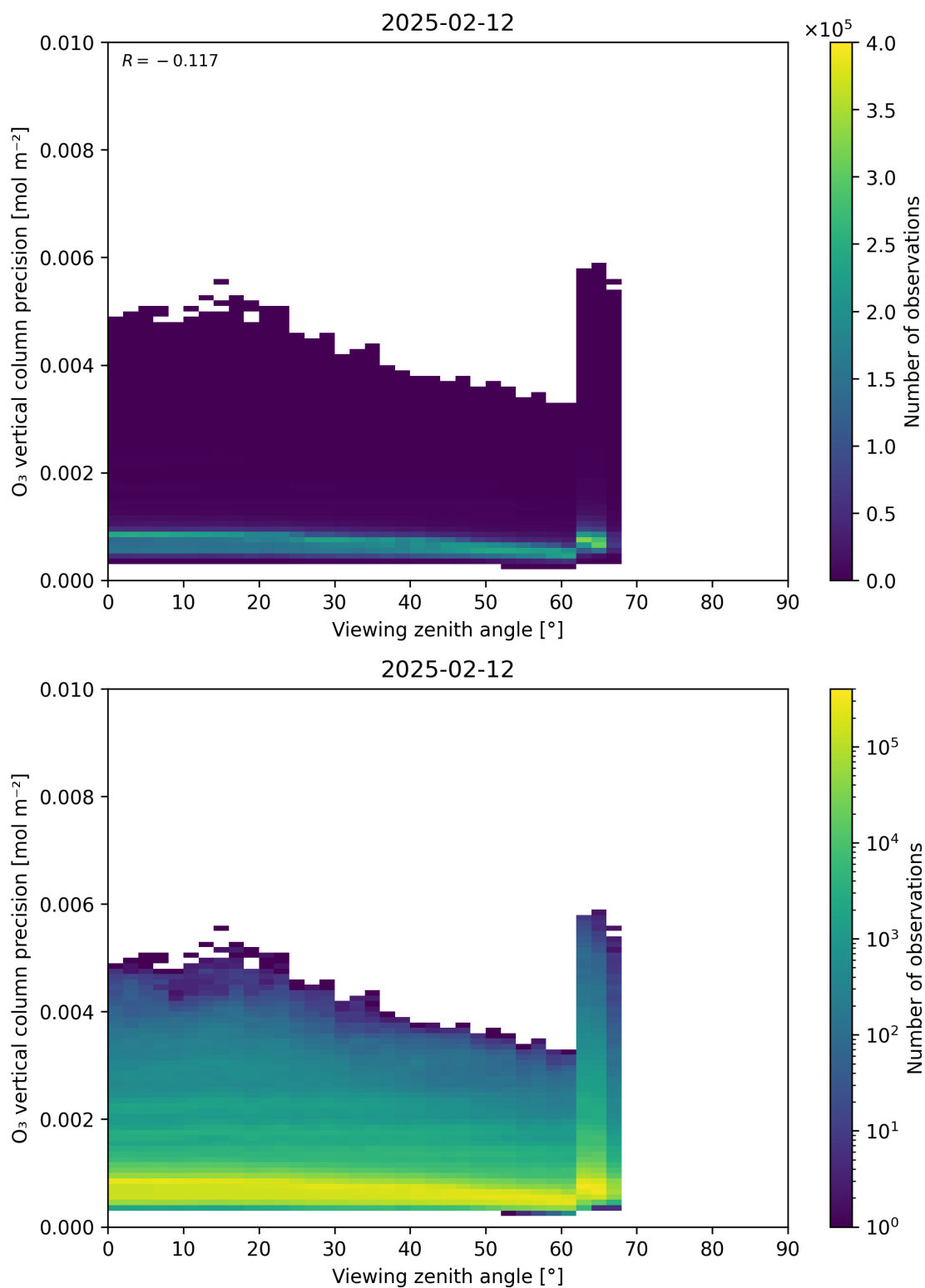
Figure 53: Scatter density plot of “Viewing zenith angle” against “O 3 vertical column precision” for 2025-02-11 to 2025-02-13.
