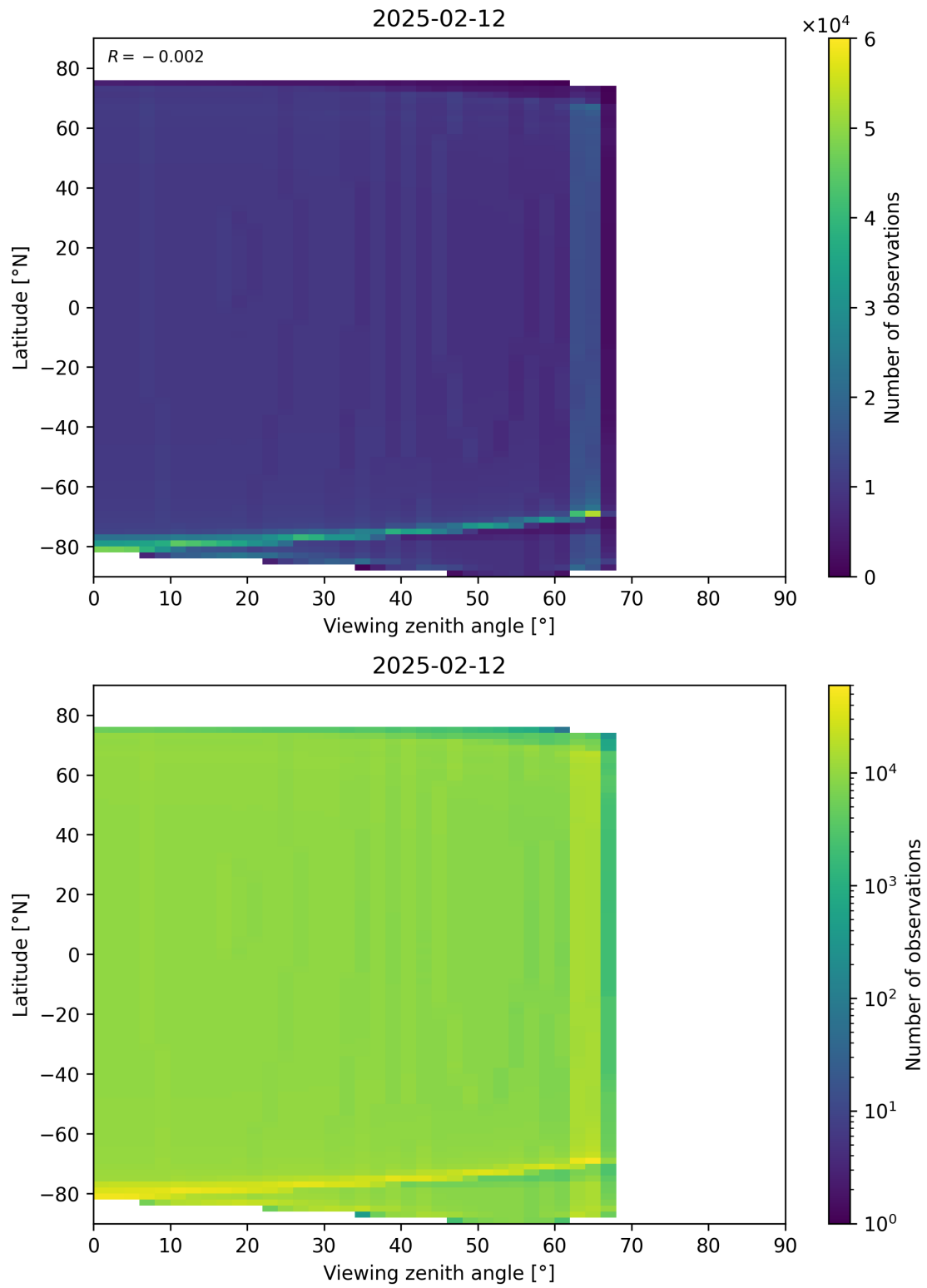
Figure 49: Scatter density plot of “Viewing zenith angle” against “Latitude” for 2025-02-11 to 2025-02-13.
