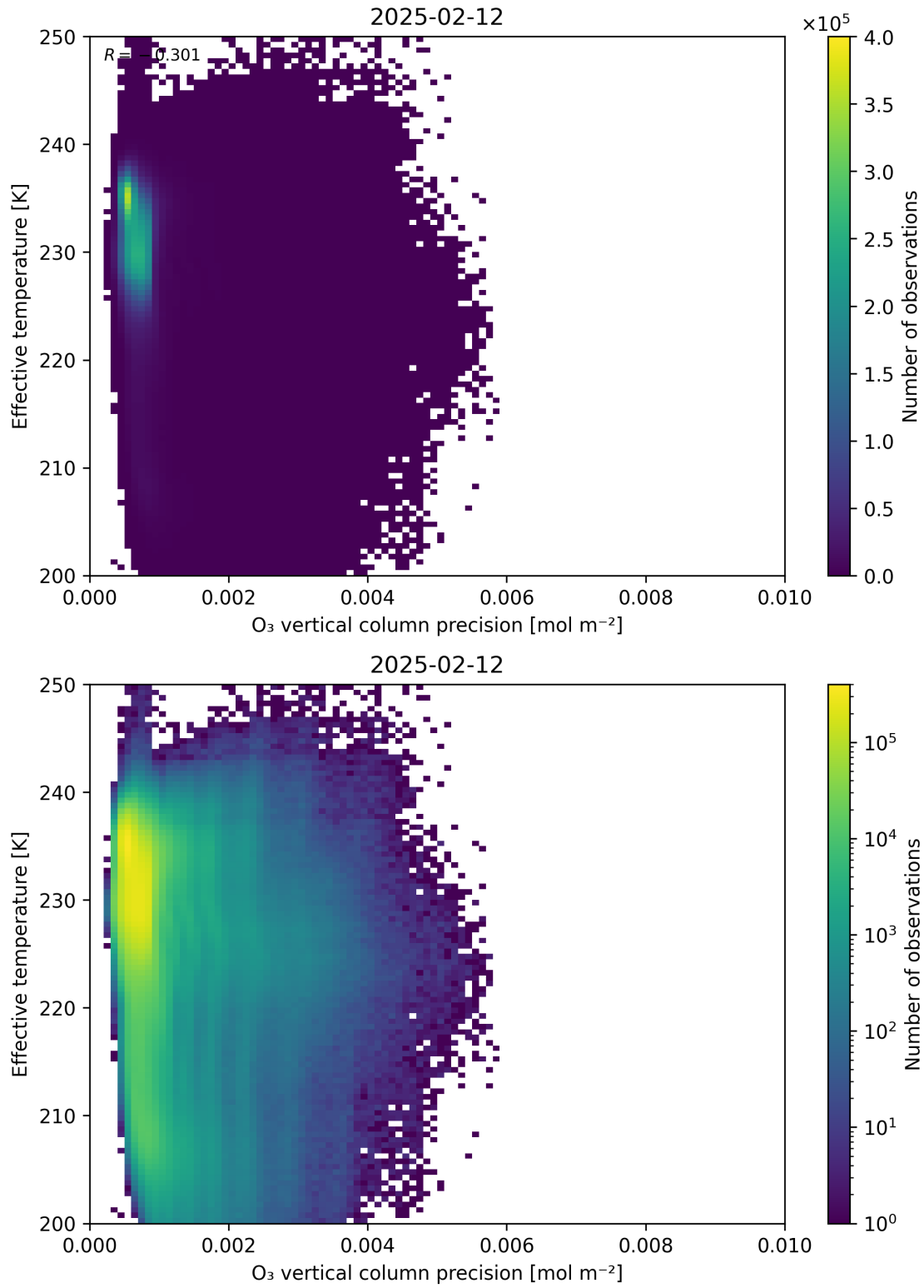
Figure 42: Scatter density plot of “O 3 vertical column precision” against “Effective temperature” for 2025-02-11 to 2025-02-13.
