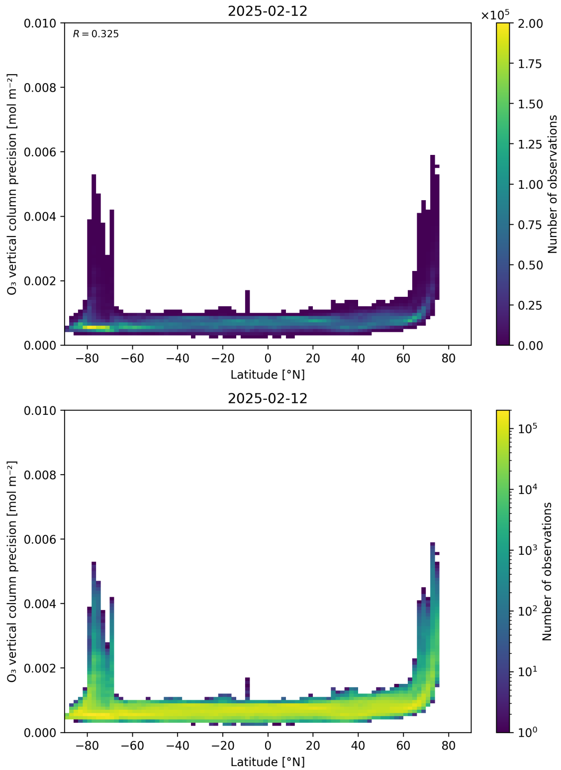
Figure 37: Scatter density plot of “Latitude” against “O 3 vertical column precision” for 2025-02-11 to 2025-02-13.
