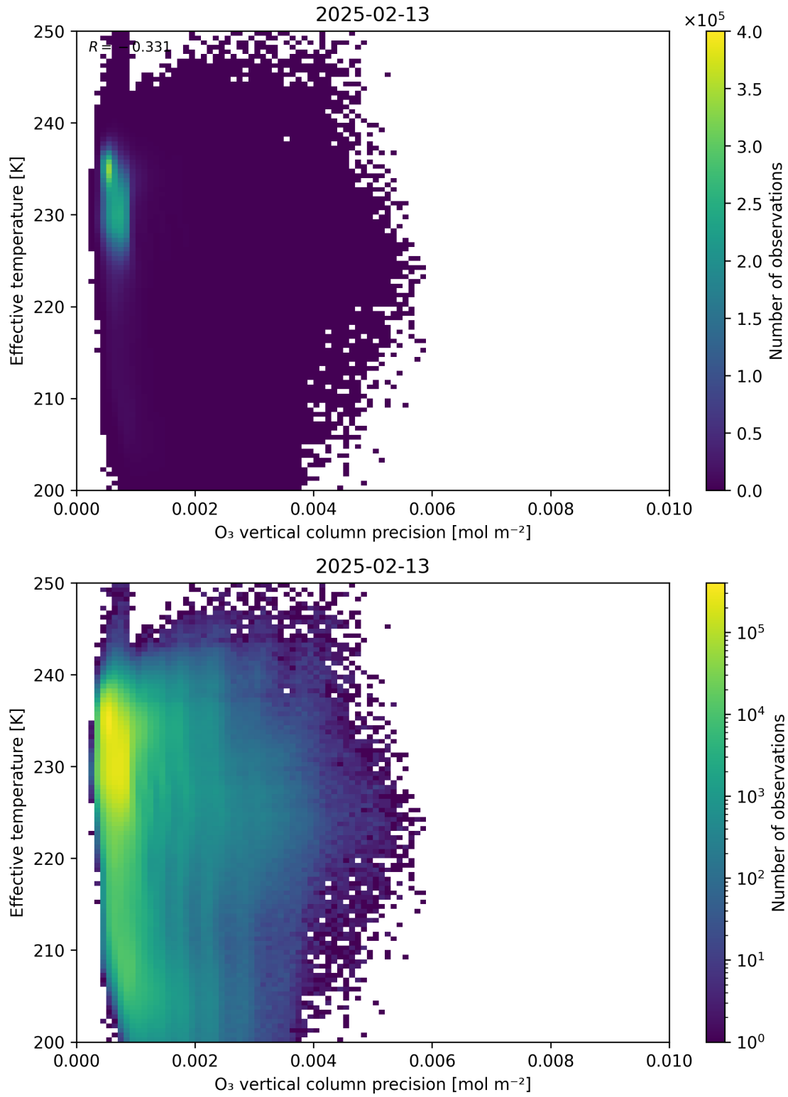
Figure 42: Scatter density plot of “O 3 vertical column precision” against “Effective temperature” for 2025-02-13 to 2025-02-14.
