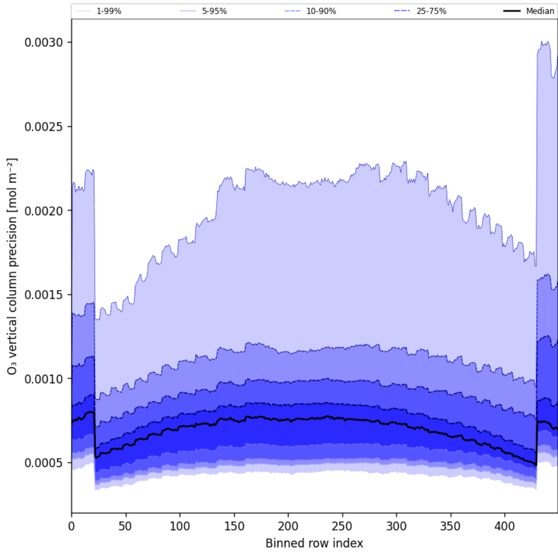
Figure 29: Along track statistics of “O 3 vertical column precision” for 2025-02-13 to 2025-02-14
