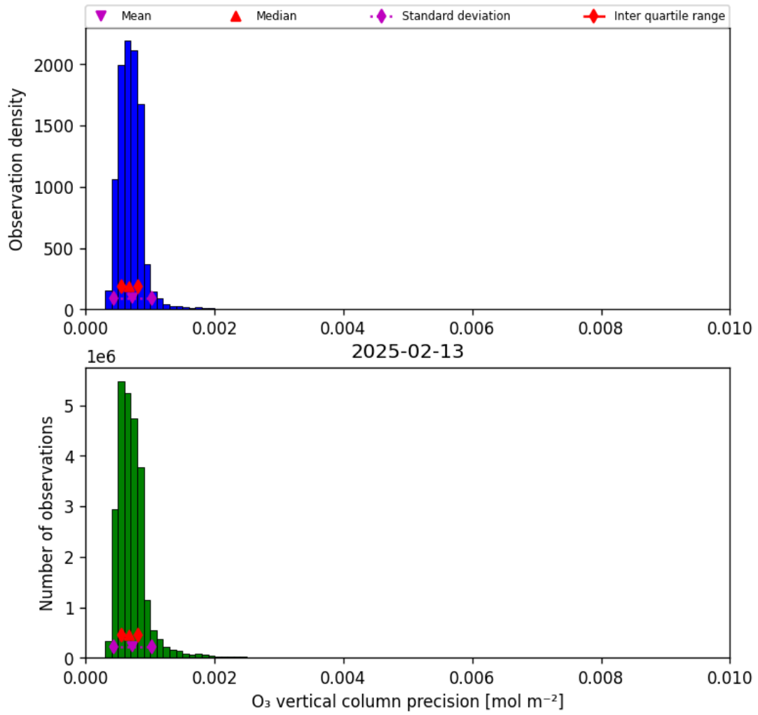
Figure 22: Histogram of “O 3 vertical column precision” for 2025-02-13 to 2025-02-14
