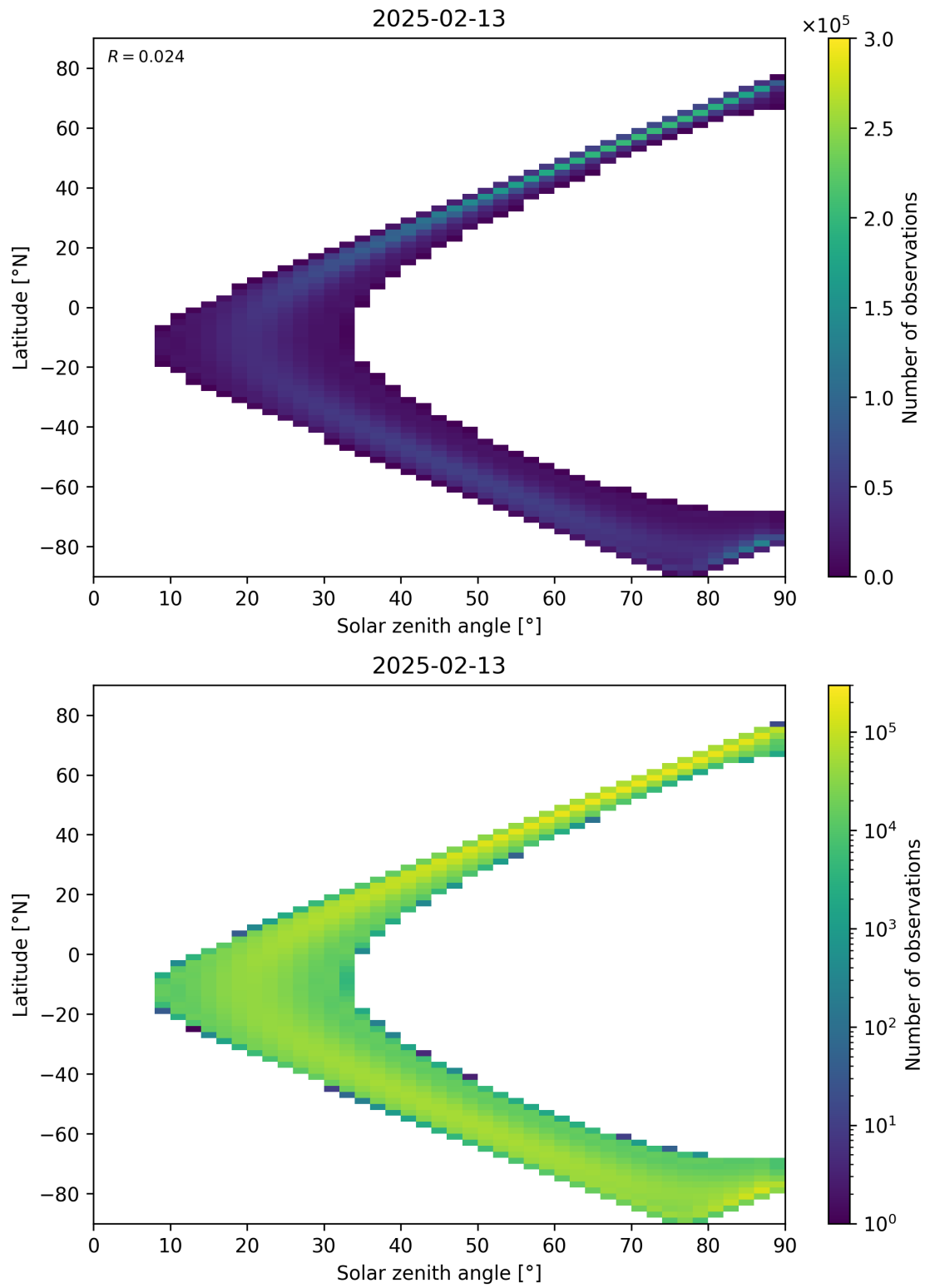
Figure 44: Scatter density plot of “Solar zenith angle” against “Latitude” for 2025-02-13 to 2025-02-14.
