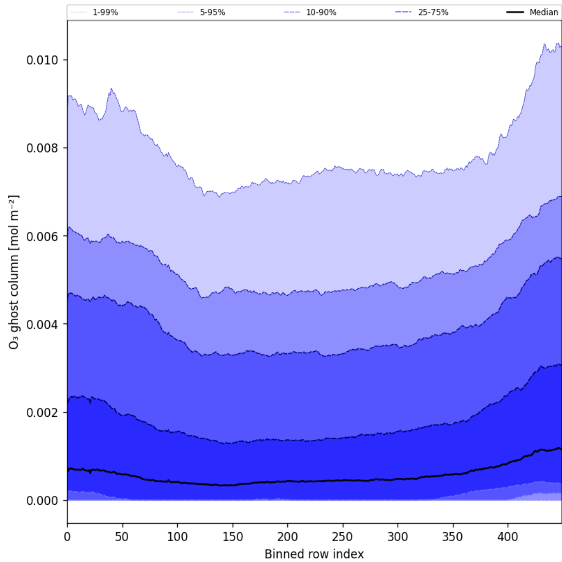
Figure 32: Along track statistics of “O 3 ghost column” for 2025-02-13 to 2025-02-14
