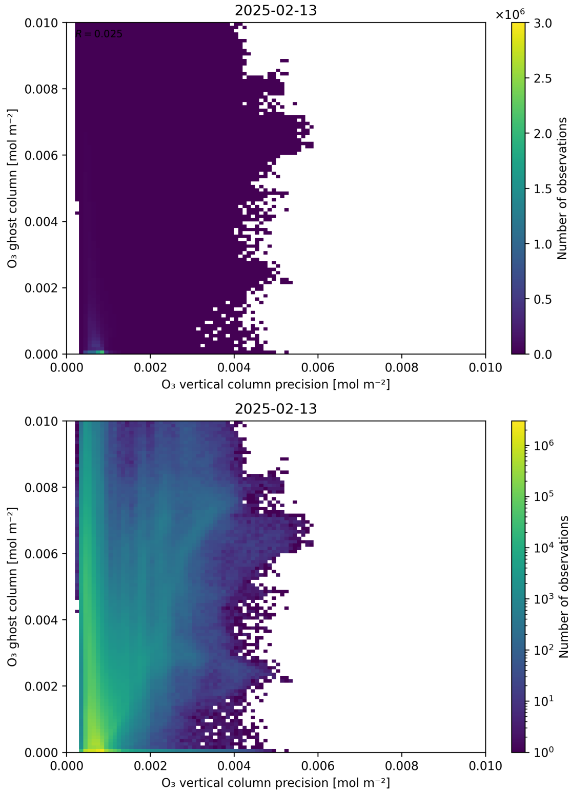
Figure 43: Scatter density plot of “ O_3 vertical column precision” against “ O_3 ghost column” for 2025-02-13 to 2025-02-14.
