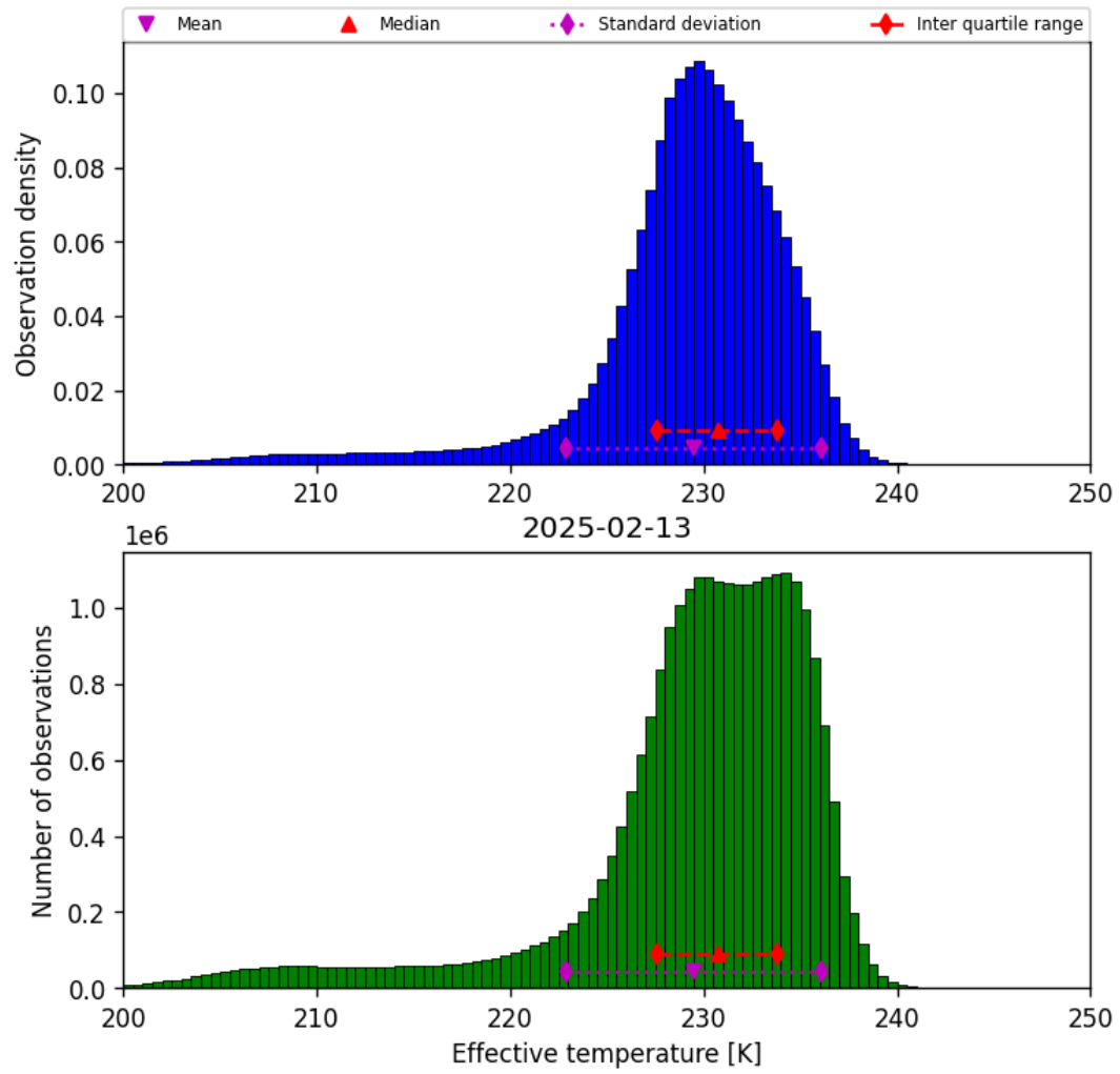
Figure 24: Histogram of “Effective temperature” for 2025-02-13 to 2025-02-14
