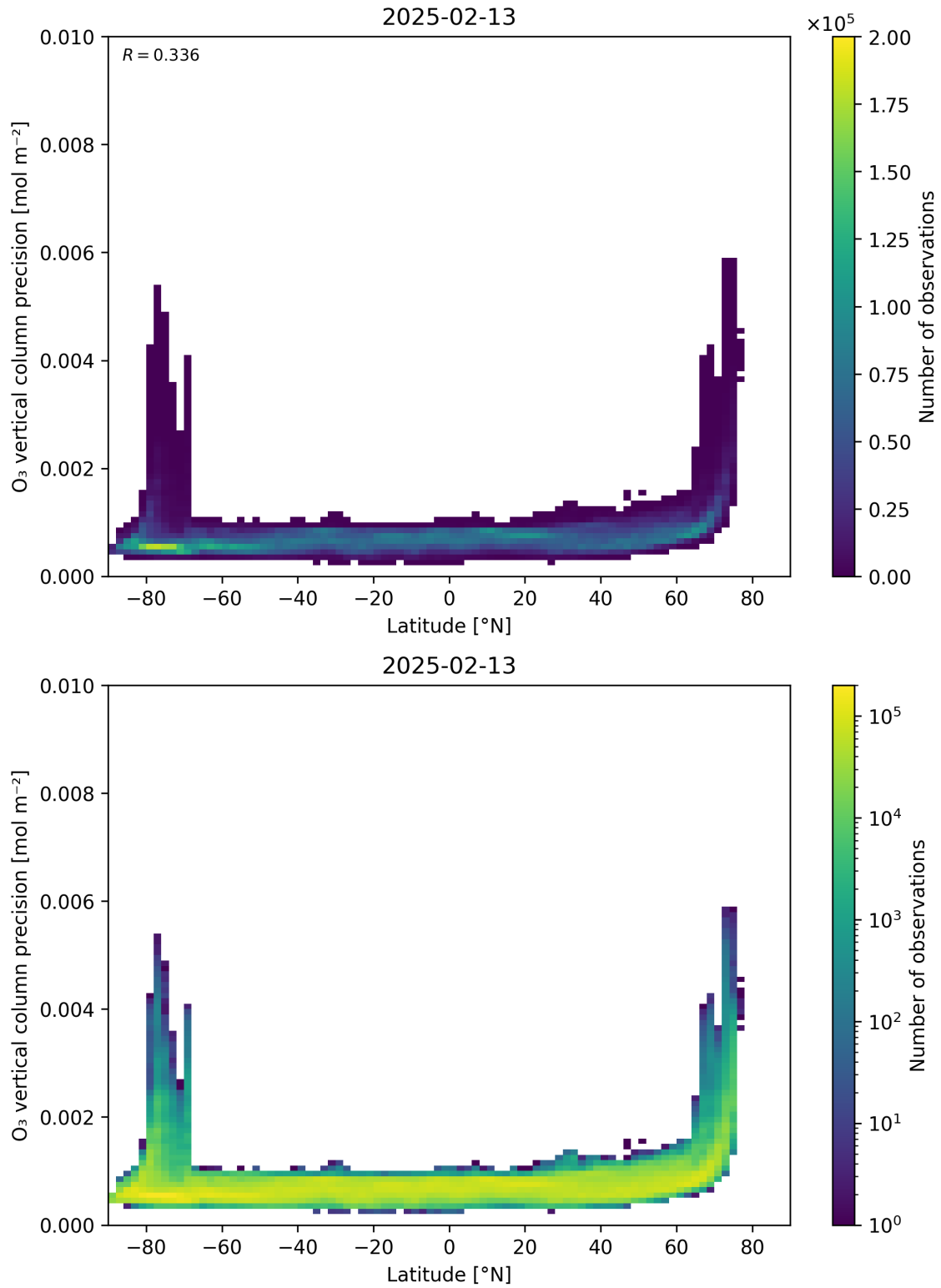
Figure 37: Scatter density plot of “Latitude” against “O 3 vertical column precision” for 2025-02-13 to 2025-02-14.
