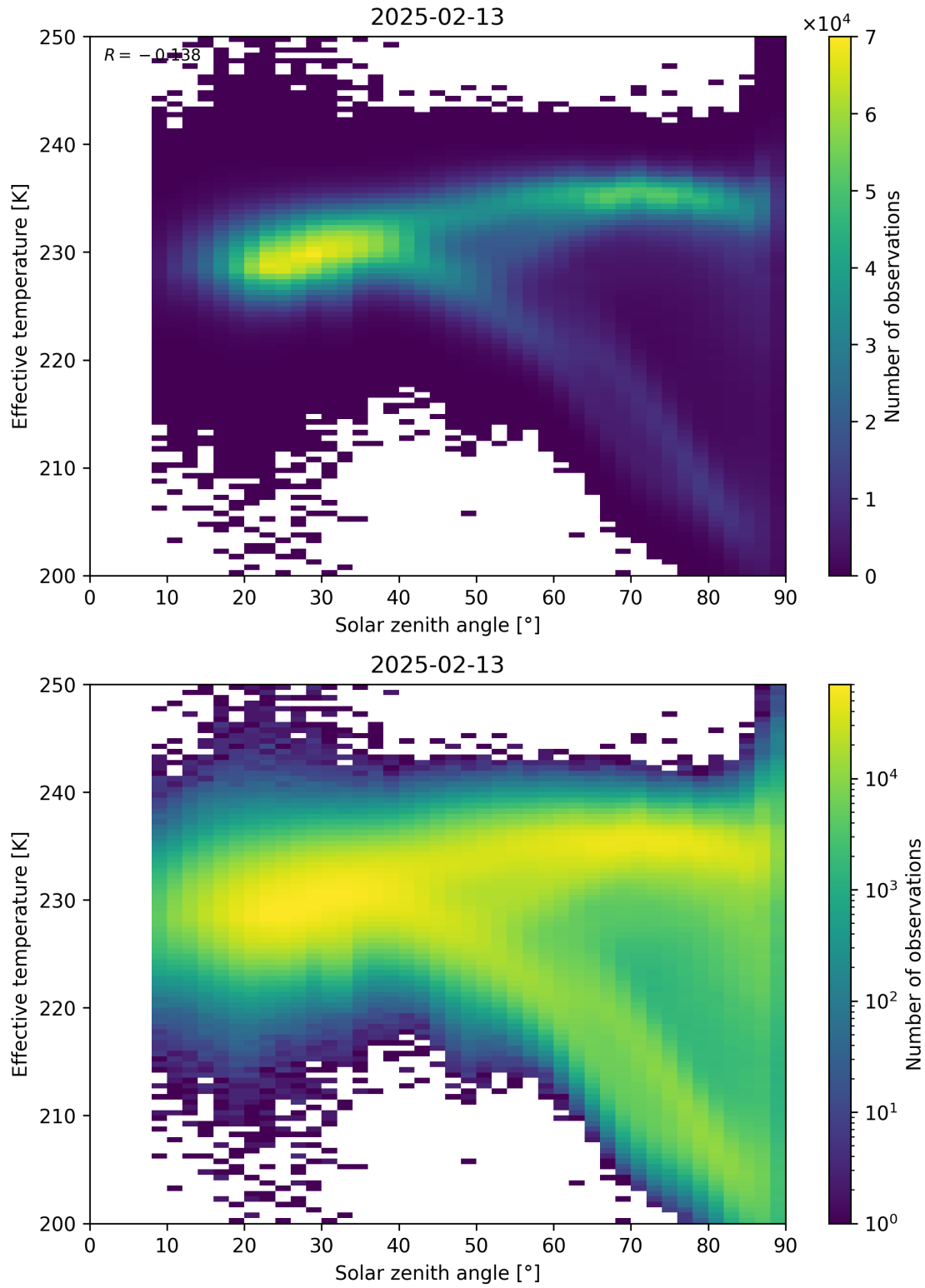
Figure 45: Scatter density plot of “Solar zenith angle” against “Effective temperature” for 2025-02-13 to 2025-02-14.
