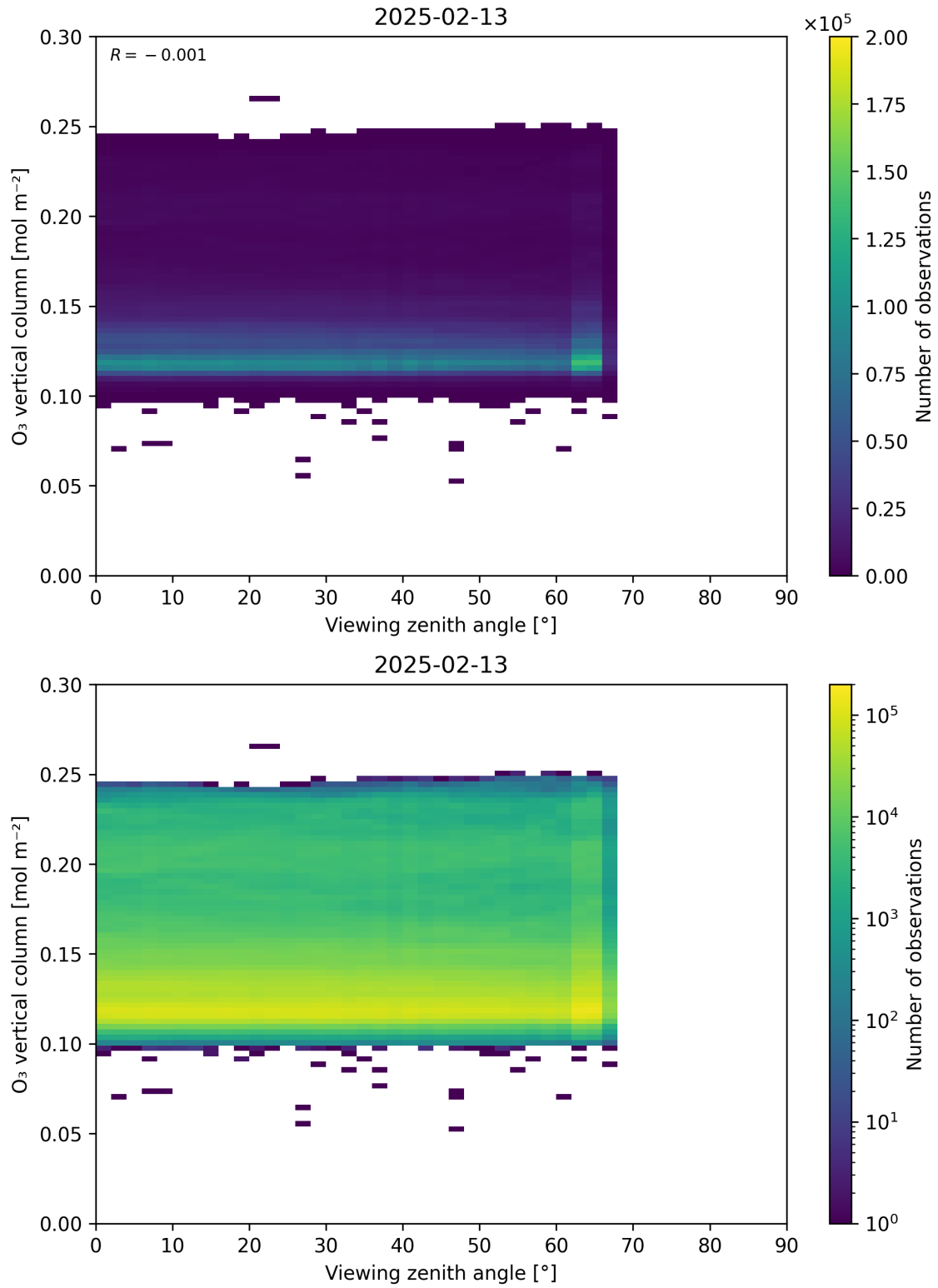
Figure 52: Scatter density plot of “Viewing zenith angle” against “O 3 vertical column” for 2025-02-13 to 2025-02-14.
