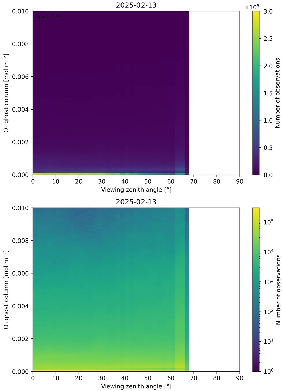
Figure 51: Scatter density plot of “Viewing zenith angle” against “O 3 ghost column” for 2025-02-13 to 2025-02-14.
