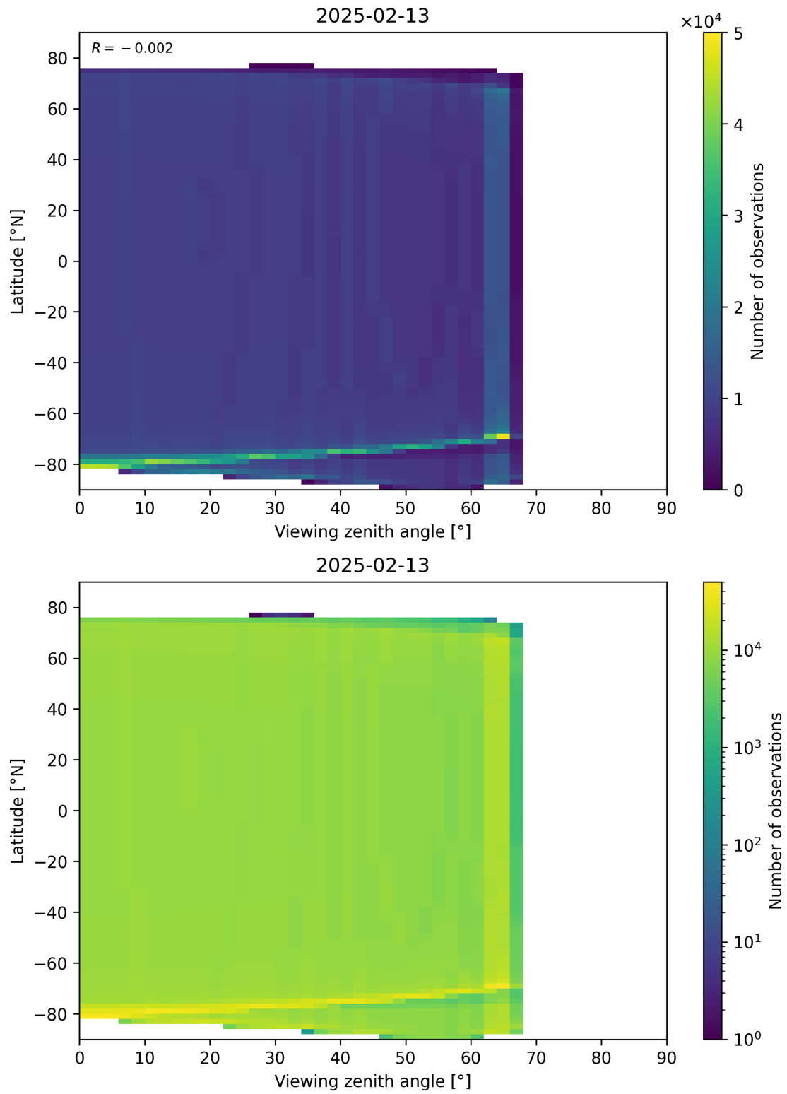
Figure 49: Scatter density plot of “Viewing zenith angle” against “Latitude” for 2025-02-13 to 2025-02-14.
