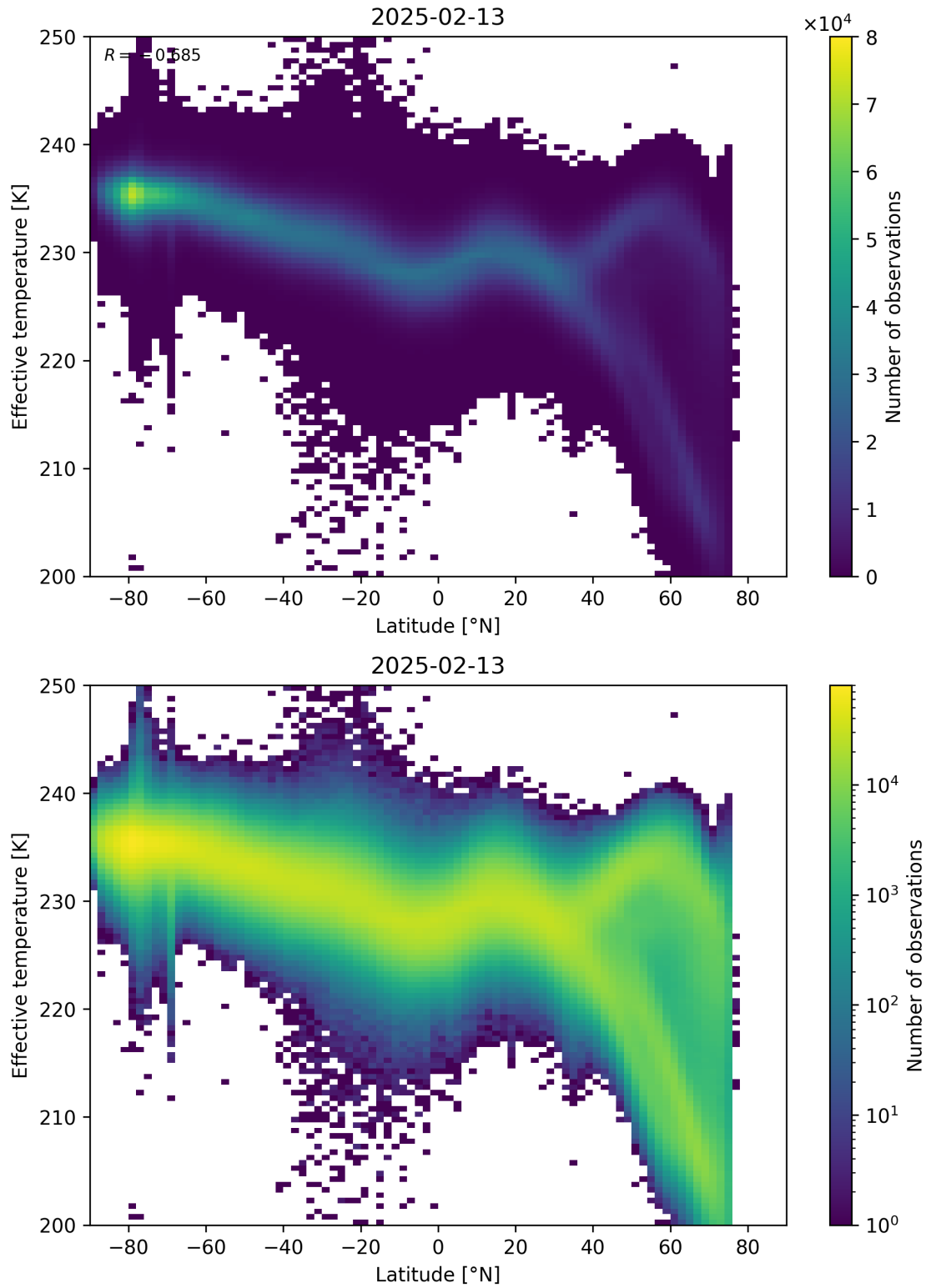
Figure 34: Scatter density plot of “Latitude” against “Effective temperature” for 2025-02-13 to 2025-02-14.
