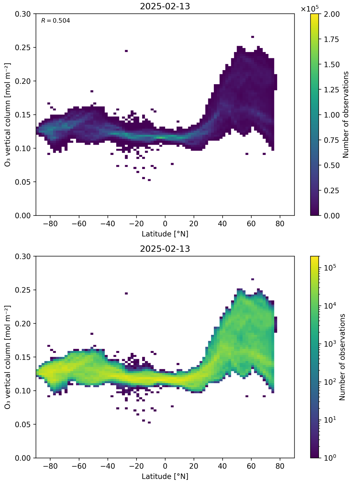
Figure 36: Scatter density plot of “Latitude” against “O 3 vertical column” for 2025-02-13 to 2025-02-14.
