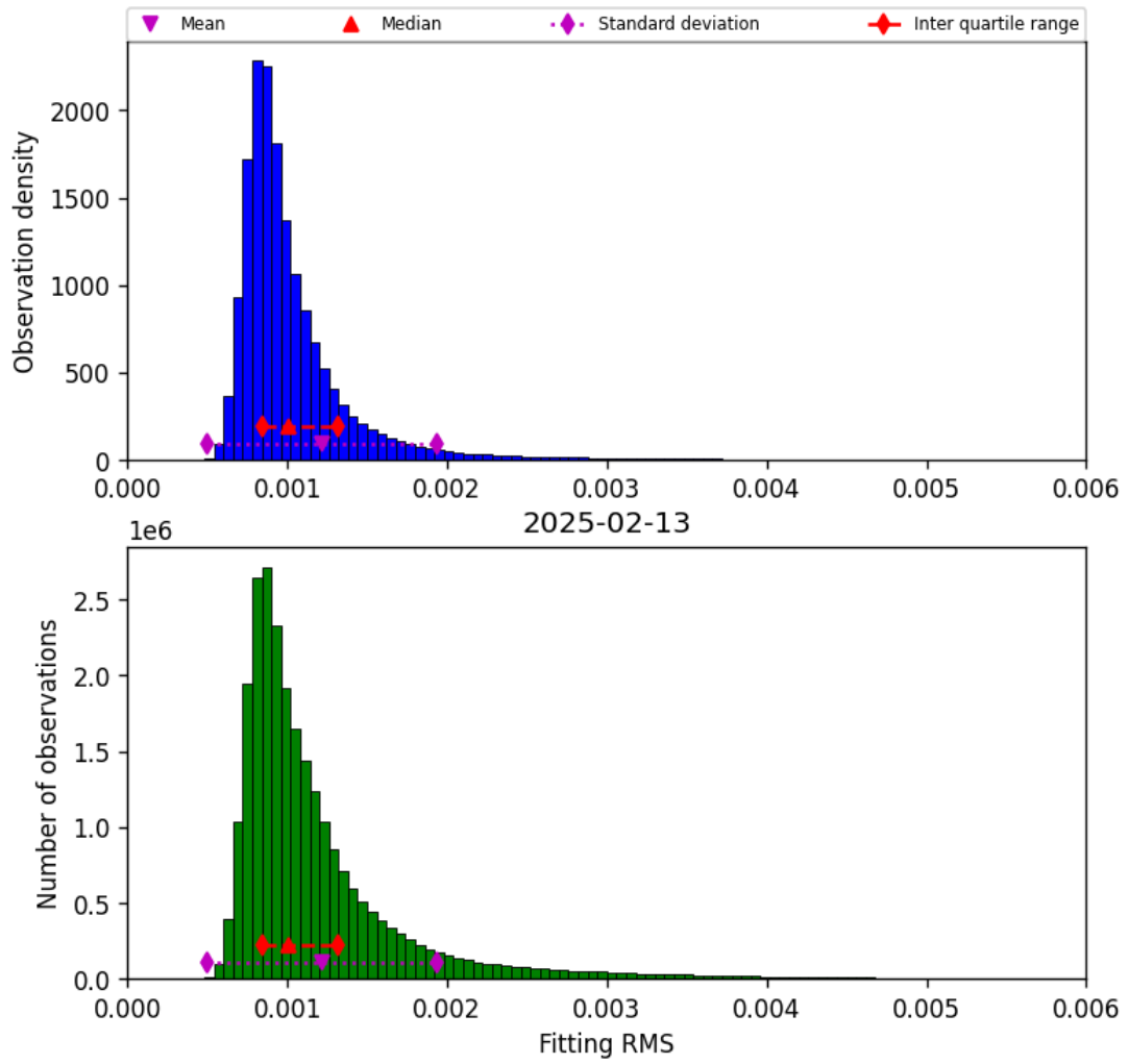
Figure 23: Histogram of “Fitting RMS” for 2025-02-13 to 2025-02-14
