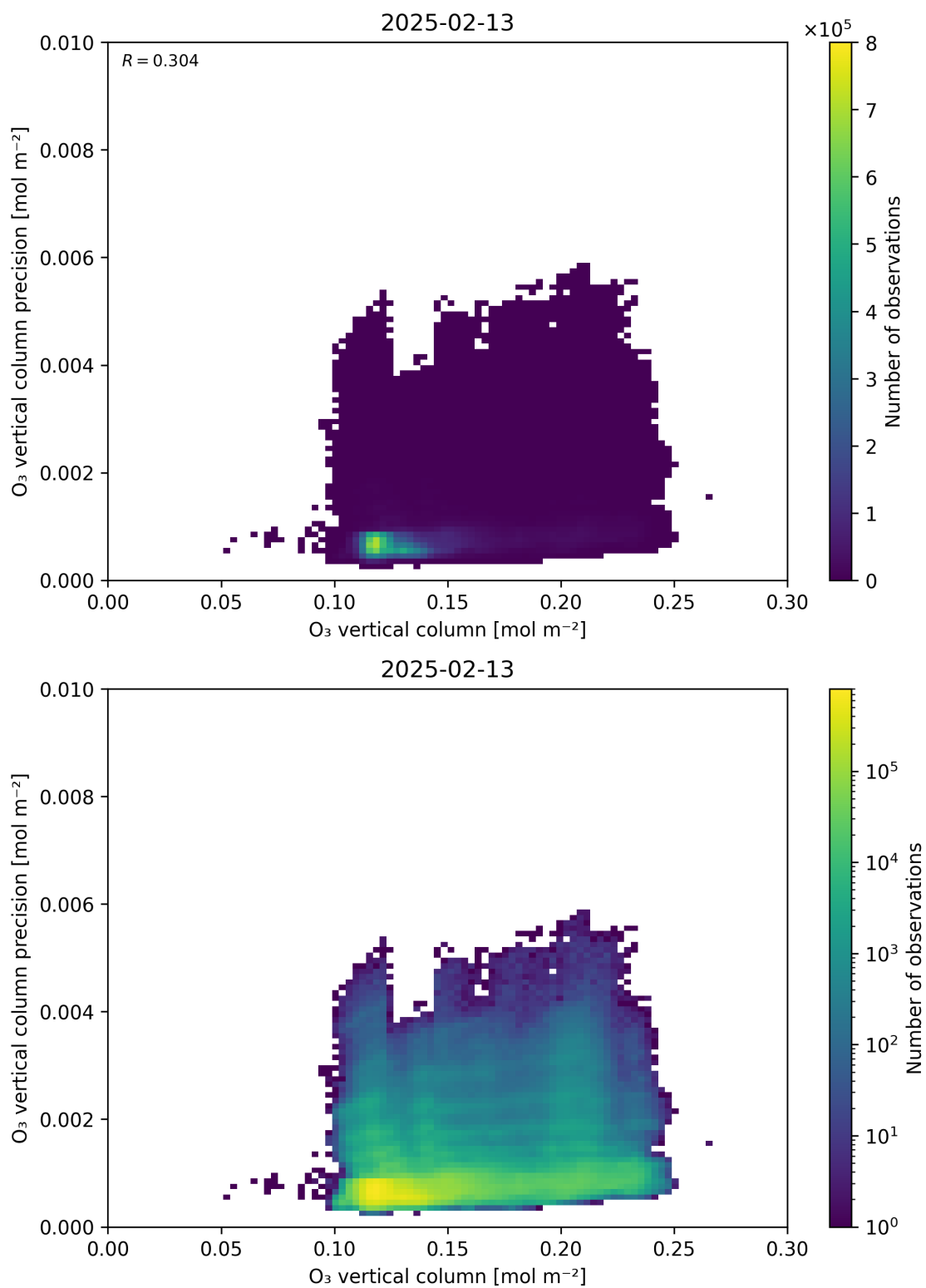
Figure 41: Scatter density plot of “O 3 vertical column” against “O 3 vertical column precision” for 2025-02-13 to 2025-02-14.
