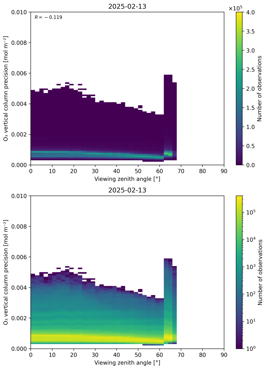
Figure 53: Scatter density plot of “Viewing zenith angle” against “O 3 vertical column precision” for 2025-02-13 to 2025-02-14.
