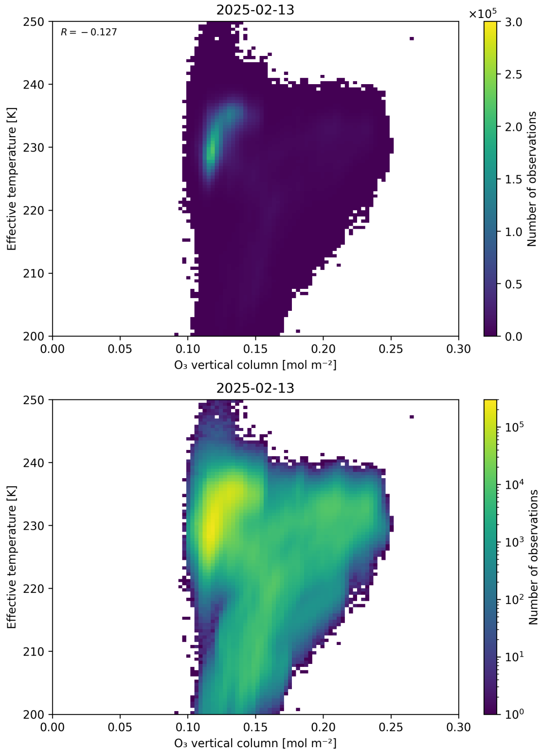
Figure 39: Scatter density plot of “O 3 vertical column” against “Effective temperature” for 2025-02-13 to 2025-02-14.
