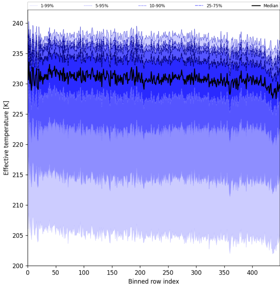
Figure 31: Along track statistics of "Effective temperature" for 2025-02-13 to 2025-02-14
