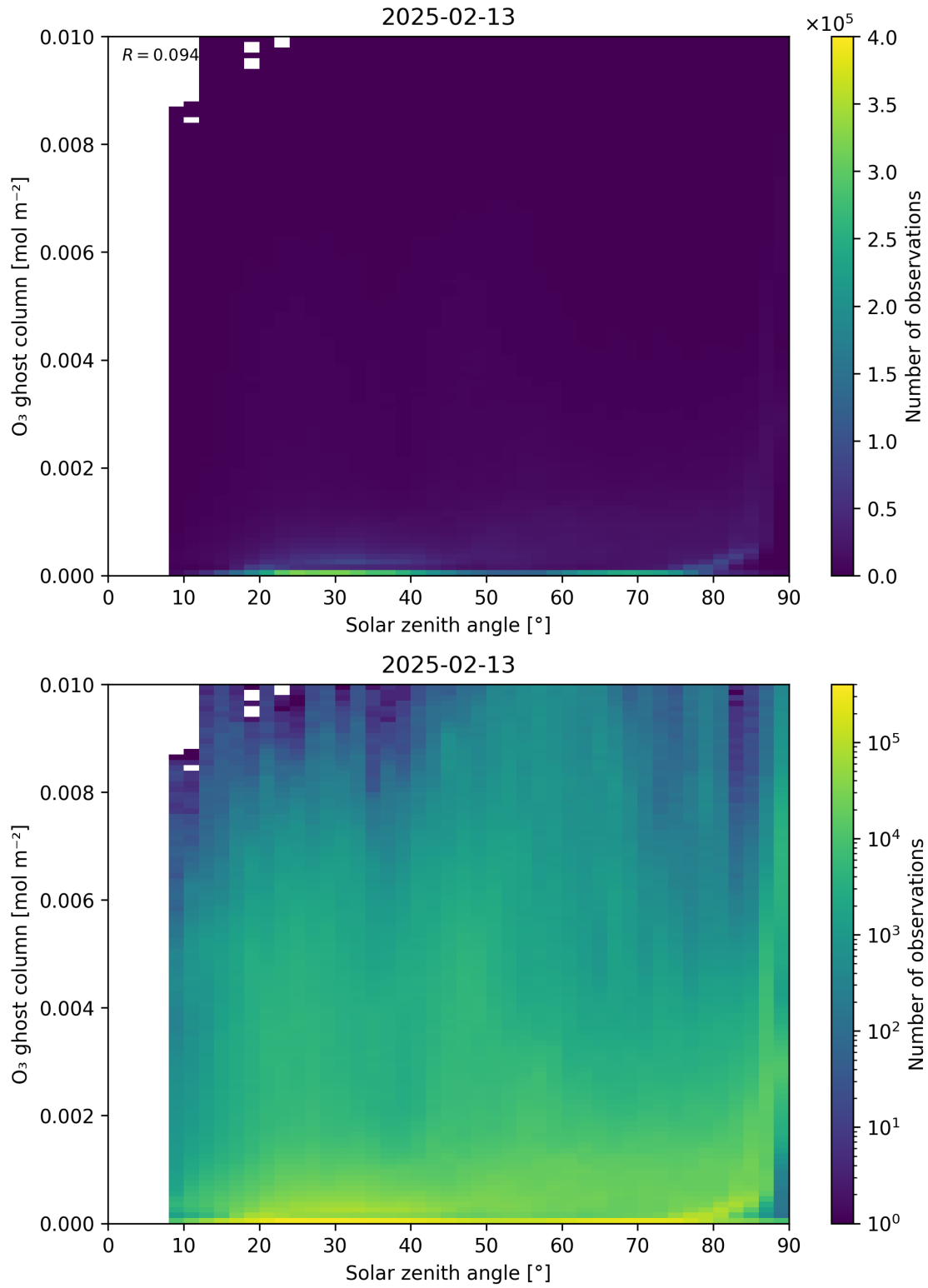
Figure 46: Scatter density plot of “Solar zenith angle” against “O 3 ghost column” for 2025-02-13 to 2025-02-14.
