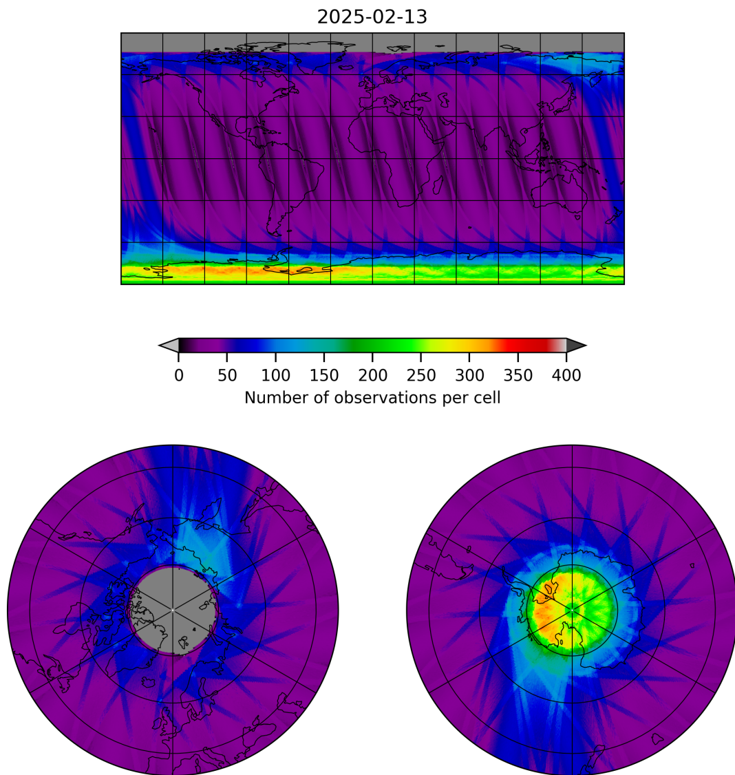
Figure 12: Map of the number of observations for 2025-02-13 to 2025-02-14
