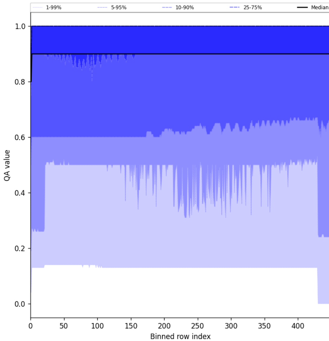
Figure 27: Along track statistics of “QA value” for 2025-02-13 to 2025-02-14
