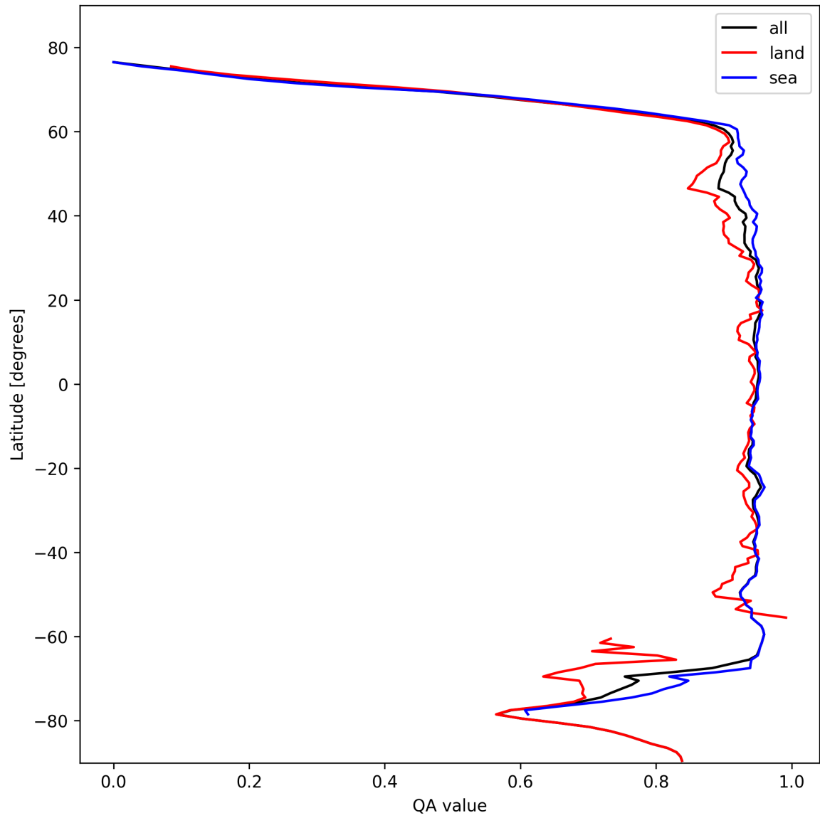
Figure 13: Zonal average of “QA value” for 2025-02-13 to 2025-02-14.
