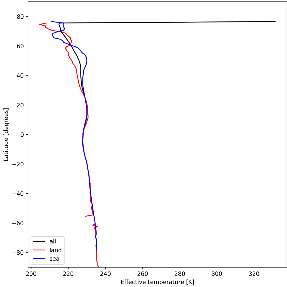
Figure 17: Zonal average of "Effective temperature" for 2025-02-13 to 2025-02-14.
