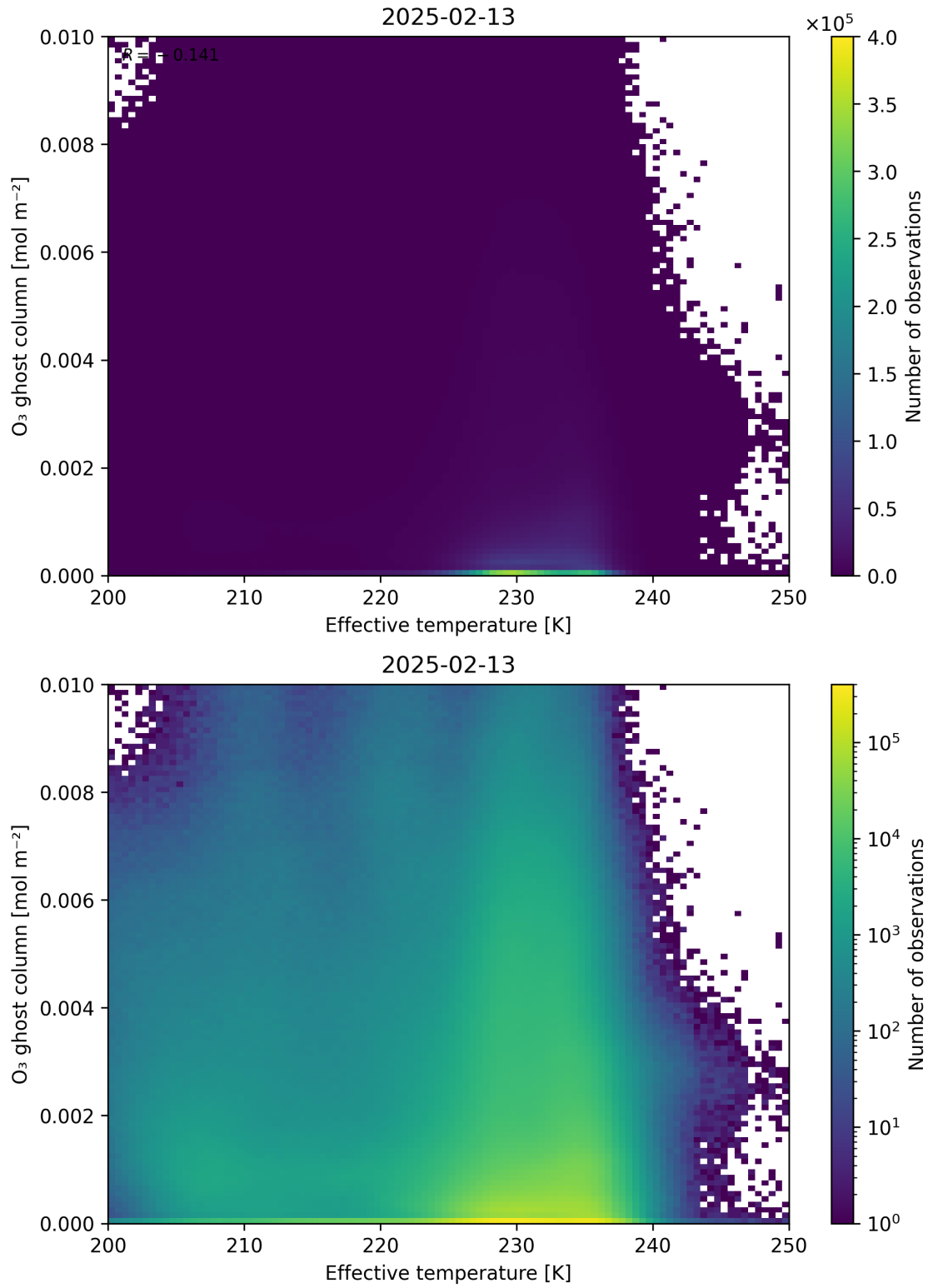
Figure 38: Scatter density plot of “Effective temperature” against “O 3 ghost column” for 2025-02-13 to 2025-02-14.
