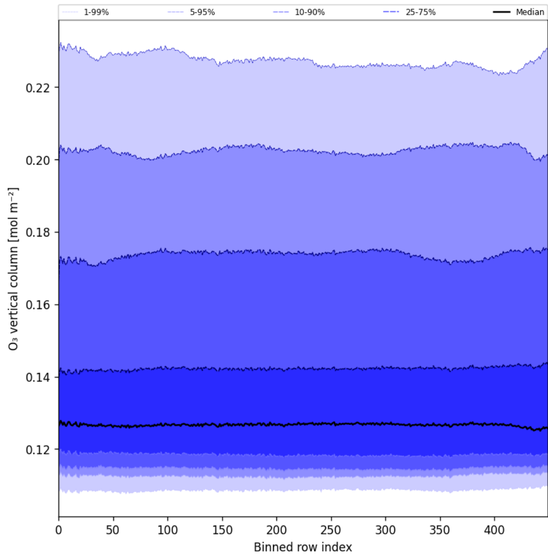
Figure 28: Along track statistics of “O 3 vertical column” for 2025-02-13 to 2025-02-14
