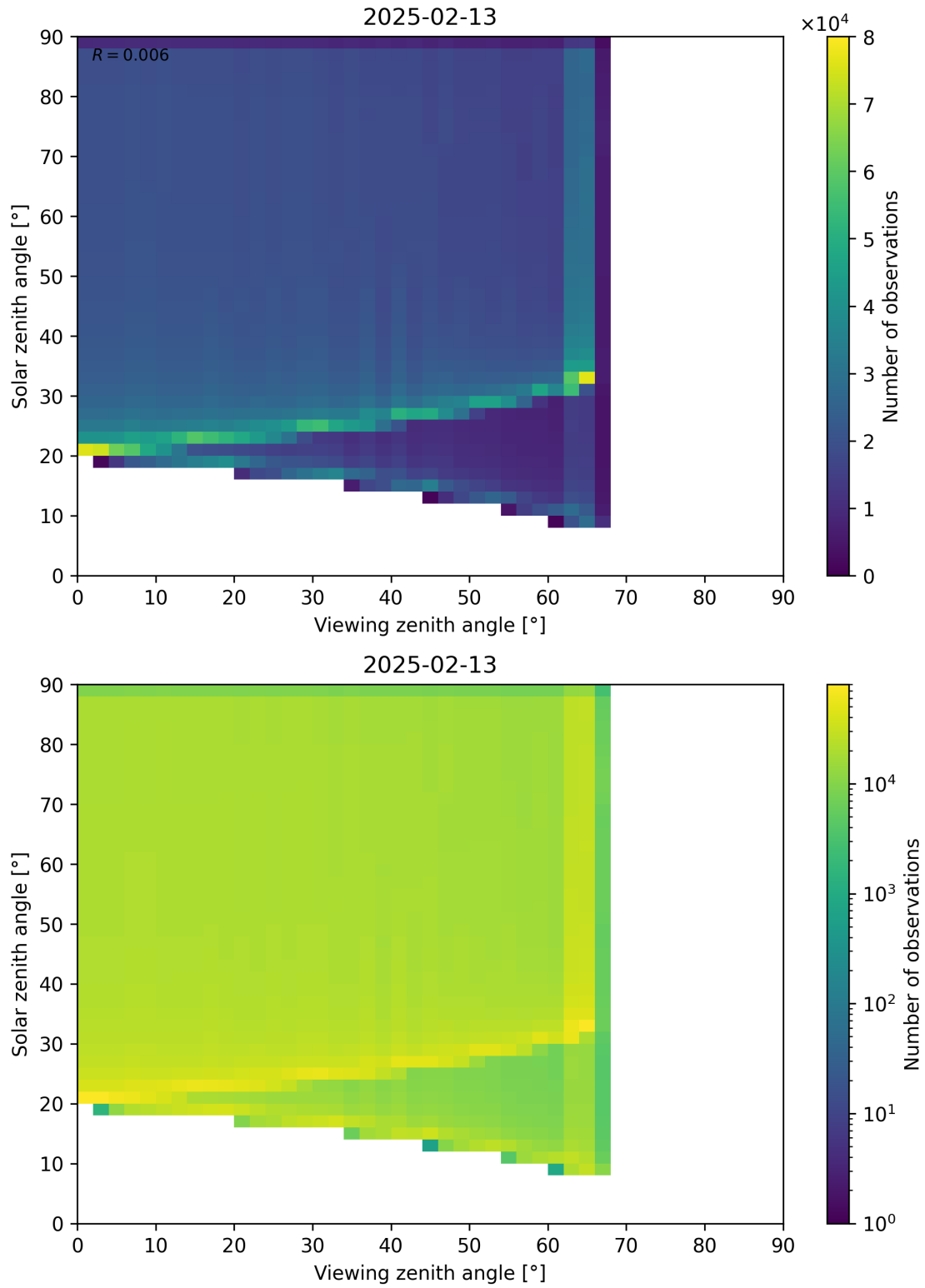
Figure 54: Scatter density plot of “Viewing zenith angle” against “Solar zenith angle” for 2025-02-13 to 2025-02-14.
