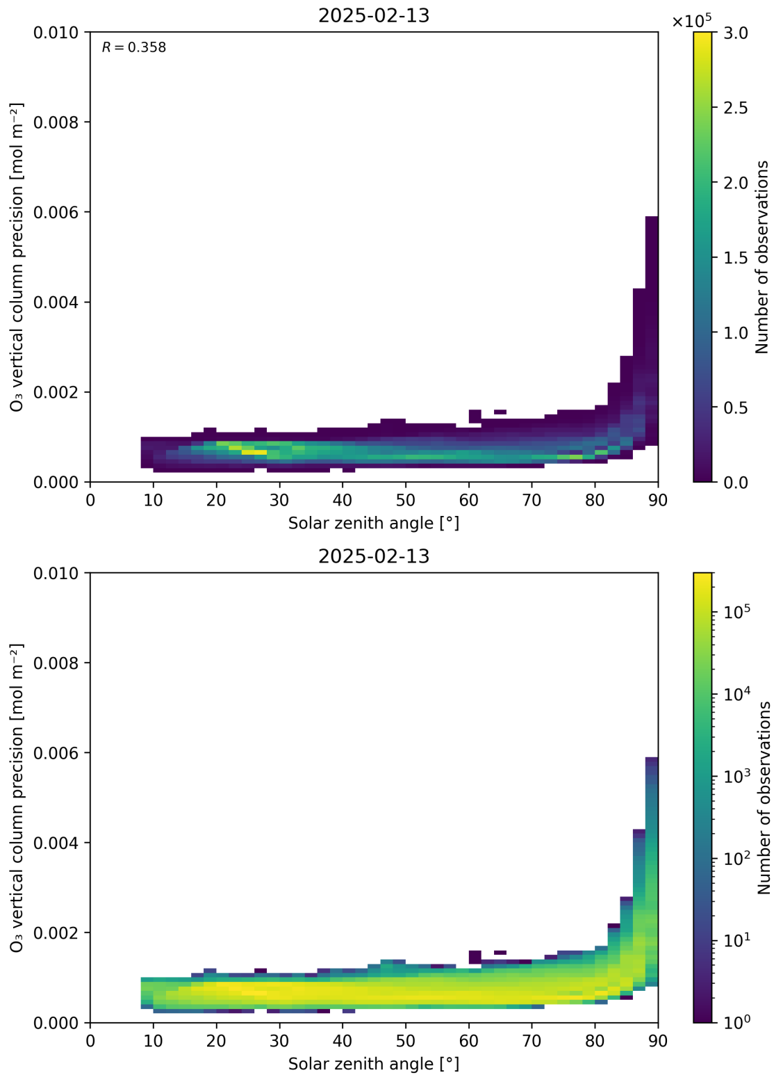
Figure 48: Scatter density plot of “Solar zenith angle” against “O 3 vertical column precision” for 2025-02-13 to 2025-02-14.
