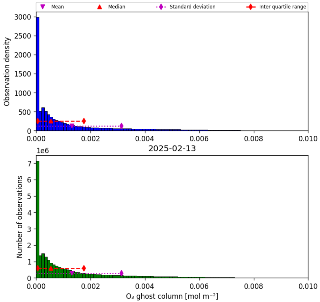
Figure 25: Histogram of “O 3 ghost column” for 2025-02-13 to 2025-02-14
