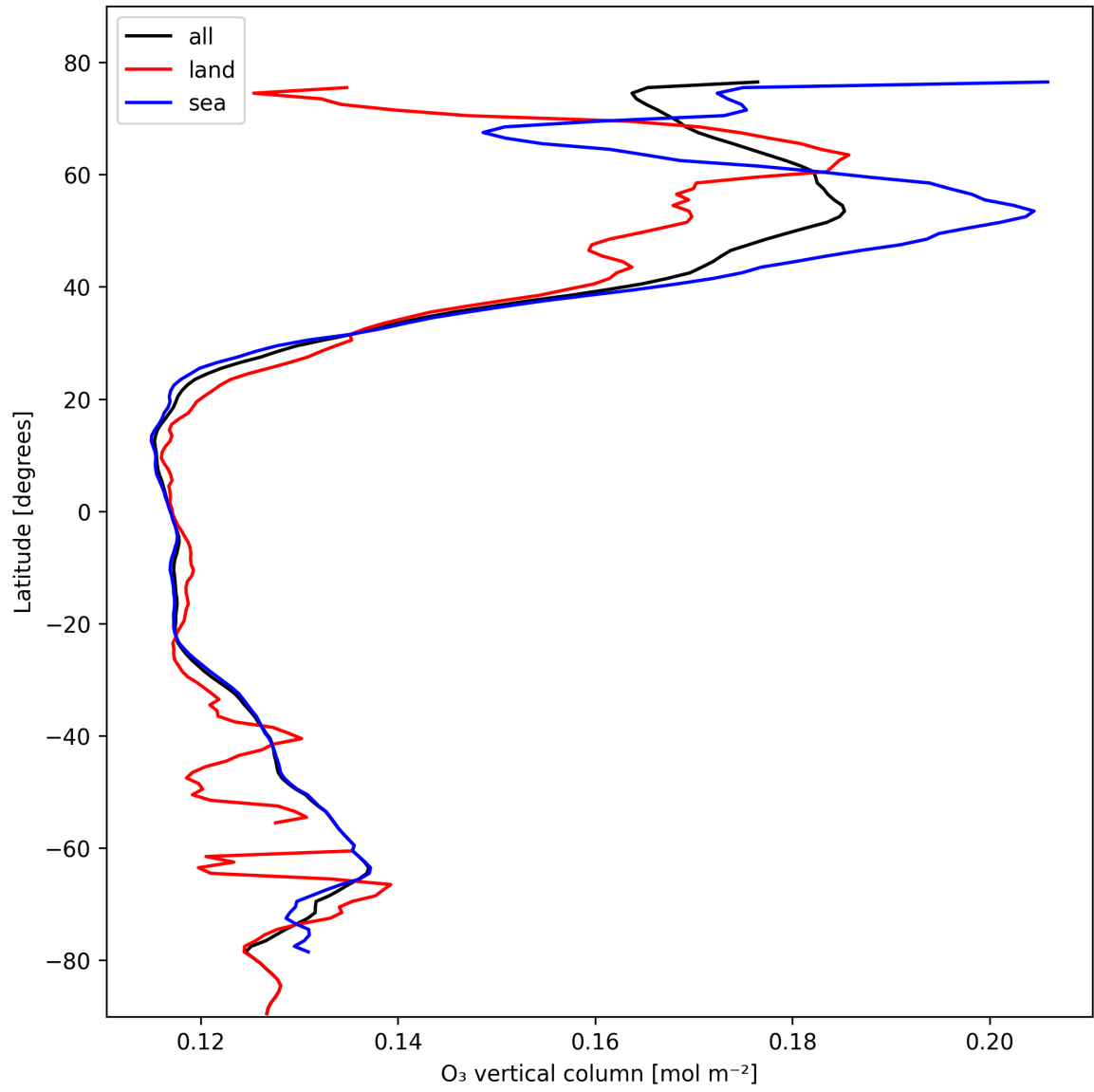
Figure 14: Zonal average of “O 3 vertical column” for 2025-02-13 to 2025-02-14.
