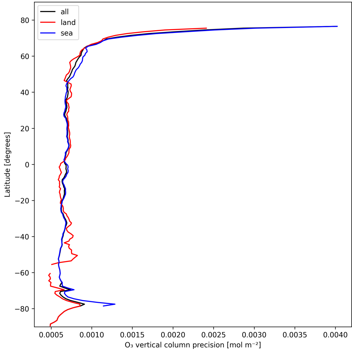
Figure 15: Zonal average of “O 3 vertical column precision” for 2025-02-13 to 2025-02-14.
