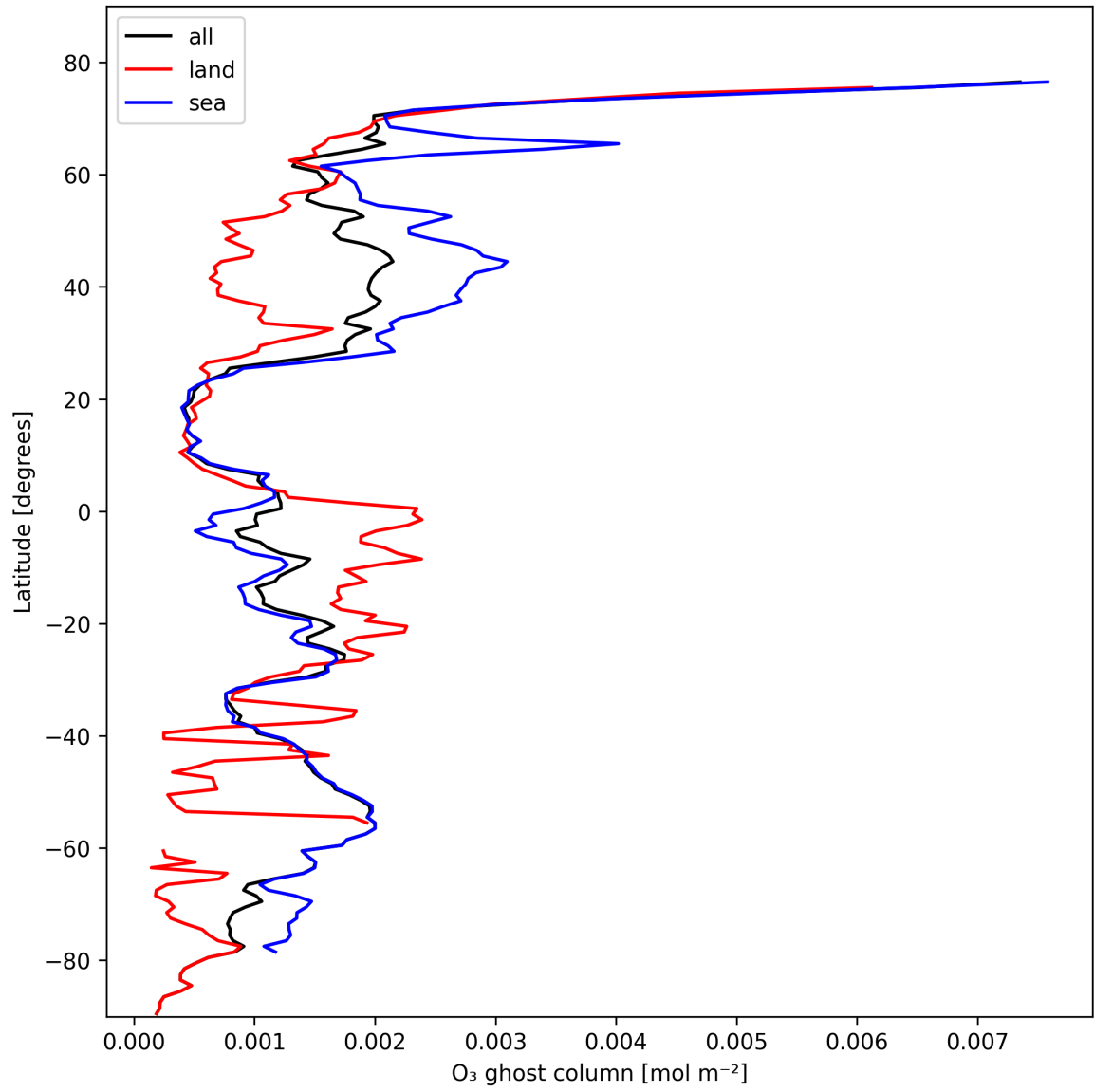
Figure 18: Zonal average of "O 3 ghost column" for 2025-02-13 to 2025-02-14.
