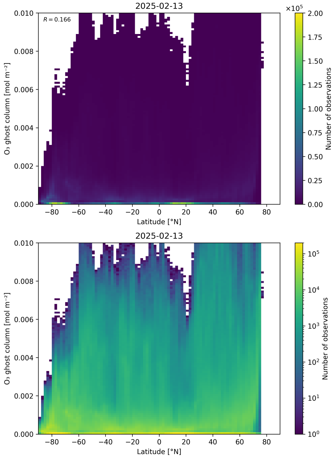
Figure 35: Scatter density plot of “Latitude” against “O 3 ghost column” for 2025-02-13 to 2025-02-14.
