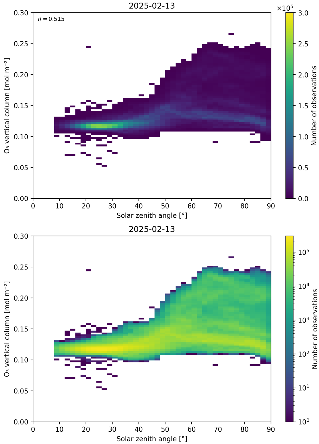
Figure 47: Scatter density plot of “Solar zenith angle” against “O 3 vertical column” for 2025-02-13 to 2025-02-14.
