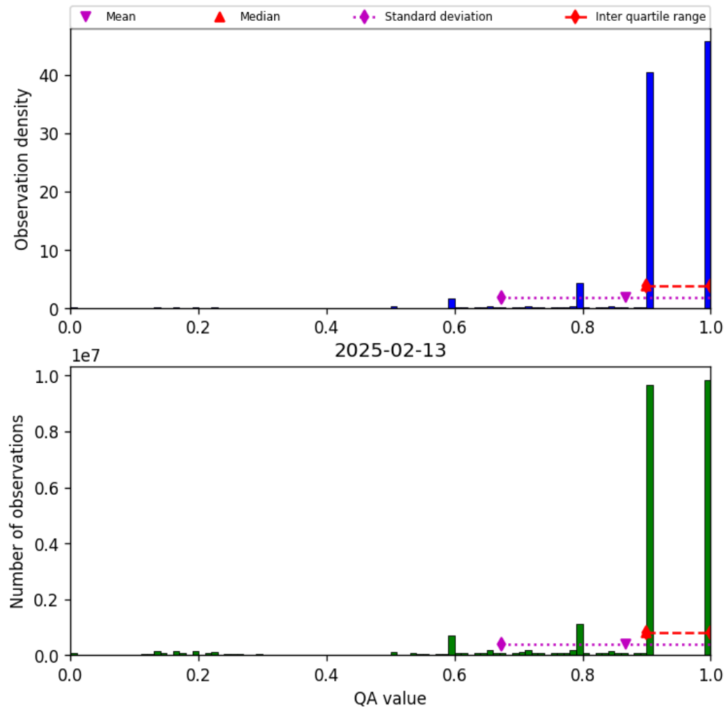
Figure 20: Histogram of “QA value” for 2025-02-13 to 2025-02-14
