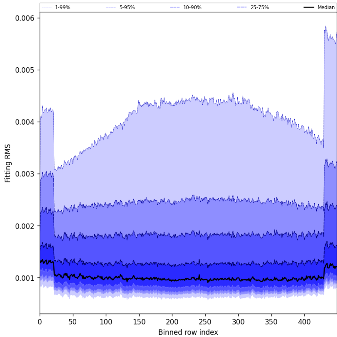
Figure 30: Along track statistics of “Fitting RMS” for 2025-02-13 to 2025-02-14
