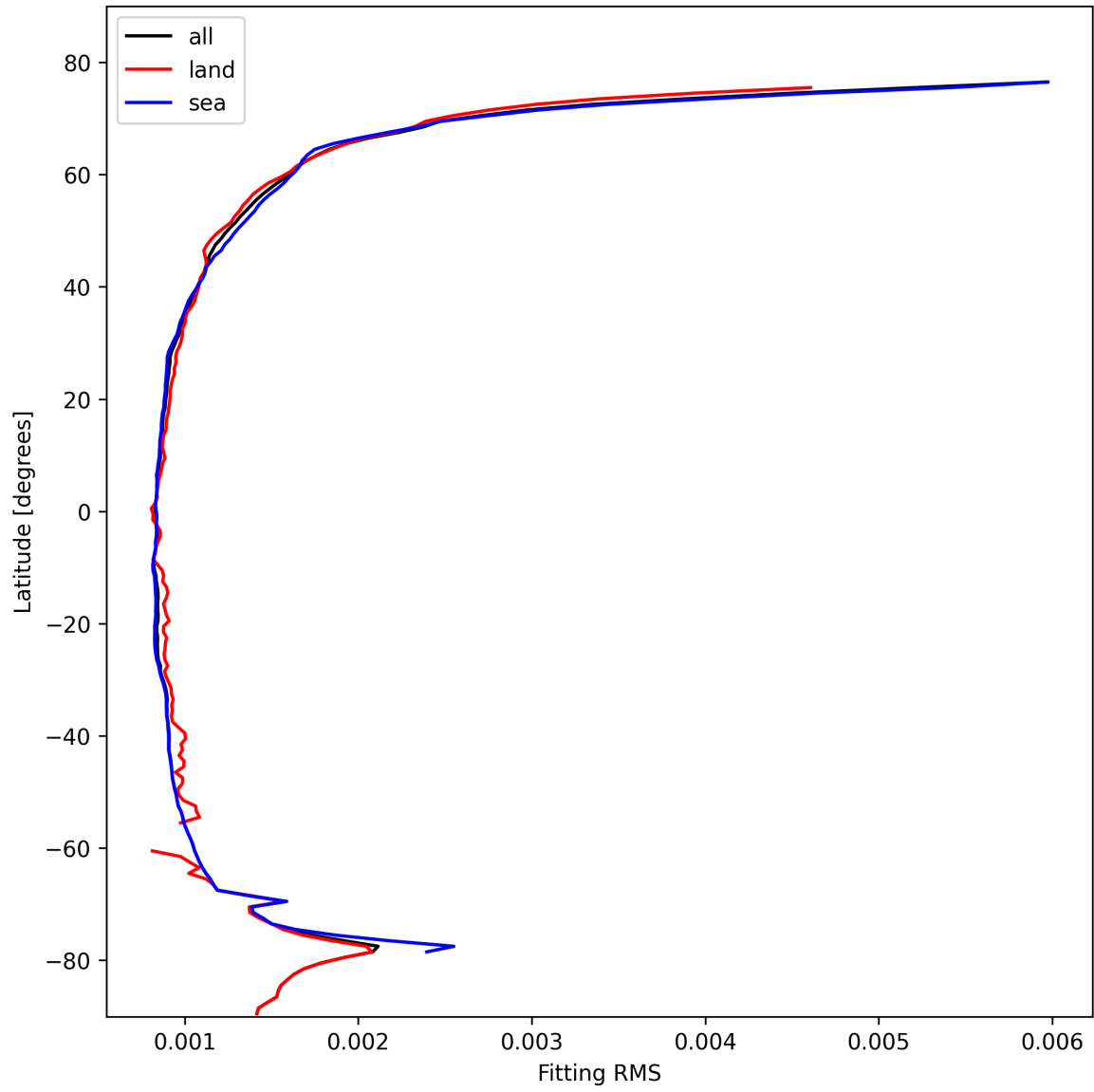
Figure 16: Zonal average of “Fitting RMS” for 2025-02-13 to 2025-02-14.
