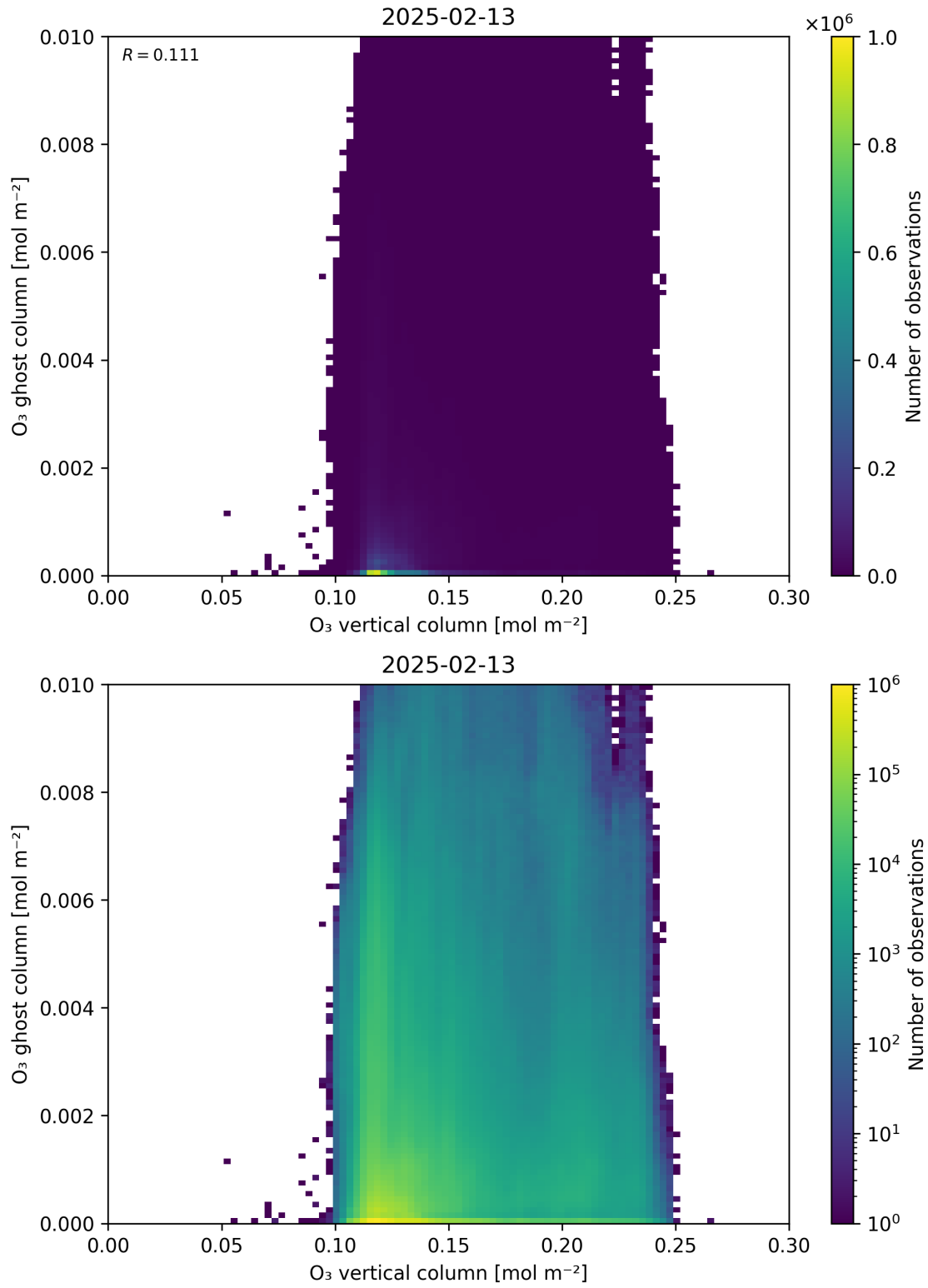
Figure 40: Scatter density plot of “O 3 vertical column” against “O 3 ghost column” for 2025-02-13 to 2025-02-14.
