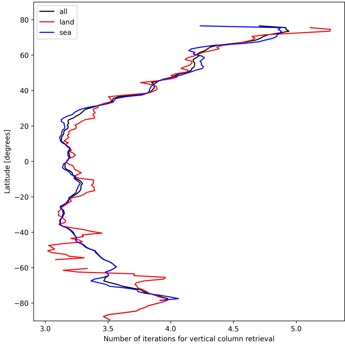
Figure 19: Zonal average of “Number of iterations for vertical column retrieval” for 2025-02-13 to 2025-02-14.
