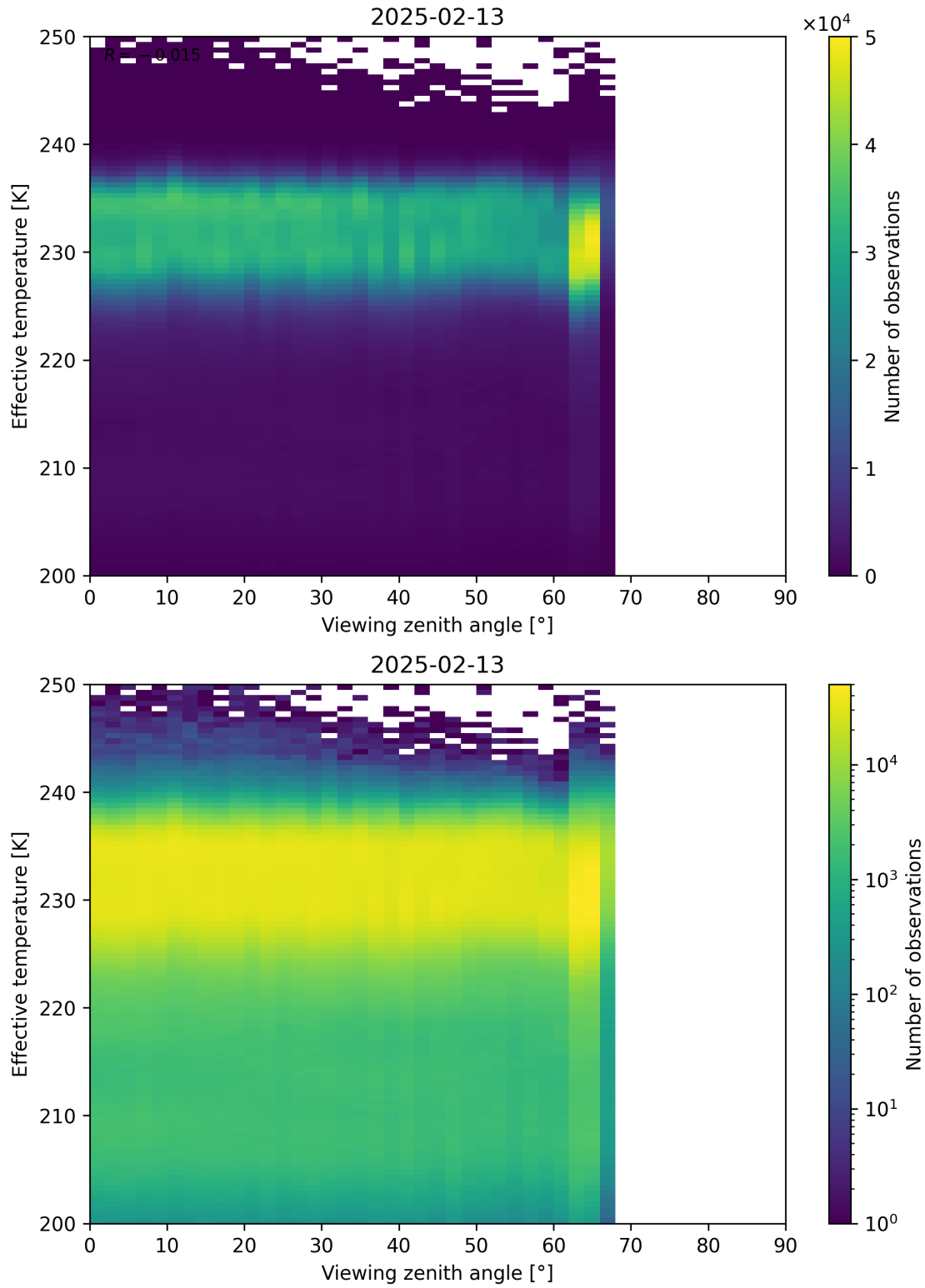
Figure 50: Scatter density plot of “Viewing zenith angle” against “Effective temperature” for 2025-02-13 to 2025-02-14.
