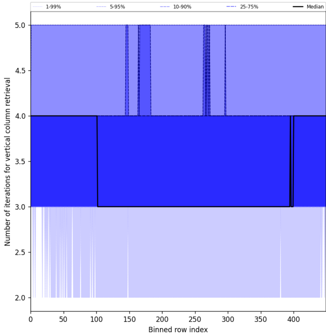
Figure 33: Along track statistics of “Number of iterations for vertical column retrieval” for 2025-02-13 to 2025-02-14
