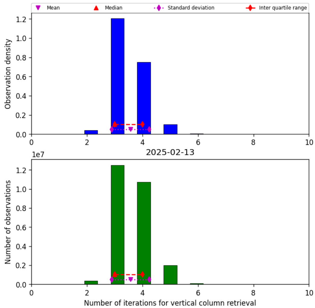
Figure 26: Histogram of “Number of iterations for vertical column retrieval” for 2025-02-13 to 2025-02-14
