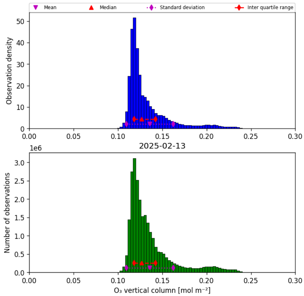
Figure 21: Histogram of “O 3 vertical column” for 2025-02-13 to 2025-02-14
