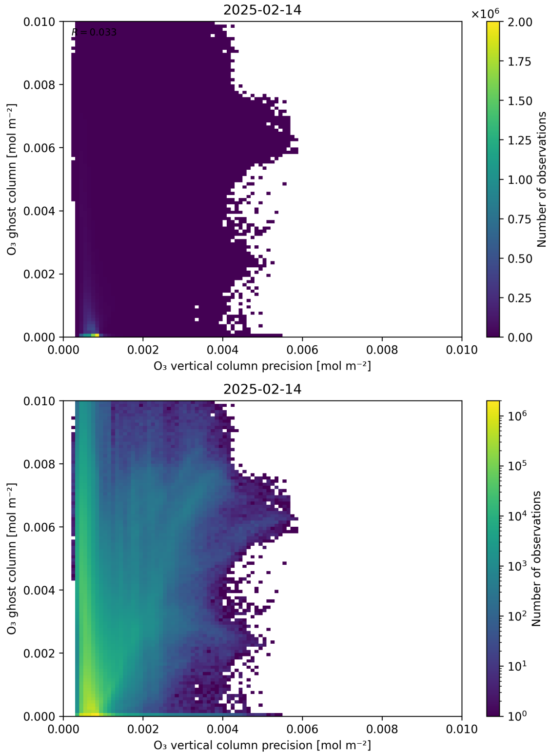
Figure 43: Scatter density plot of “ \text{O}_3 vertical column precision” against “ \text{O}_3 ghost column” for 2025-02-13 to 2025-02-15.
