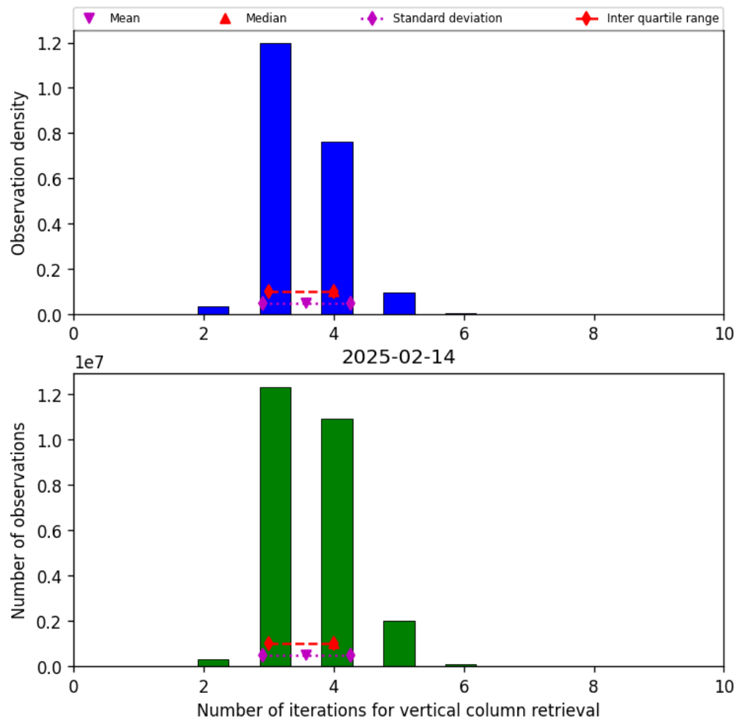
Figure 26: Histogram of “Number of iterations for vertical column retrieval” for 2025-02-13 to 2025-02-15
