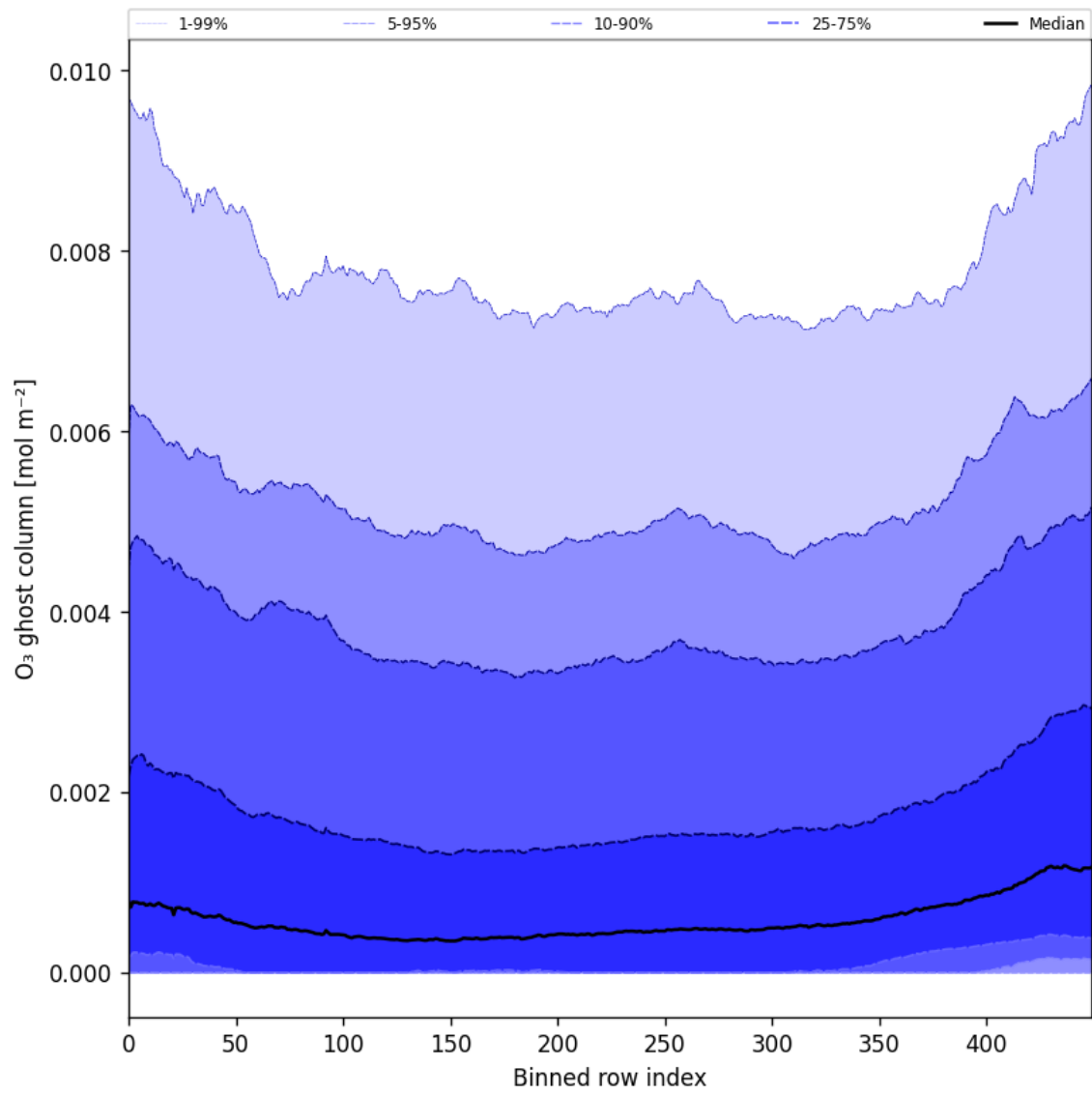
Figure 32: Along track statistics of "O 3 ghost column" for 2025-02-13 to 2025-02-15
