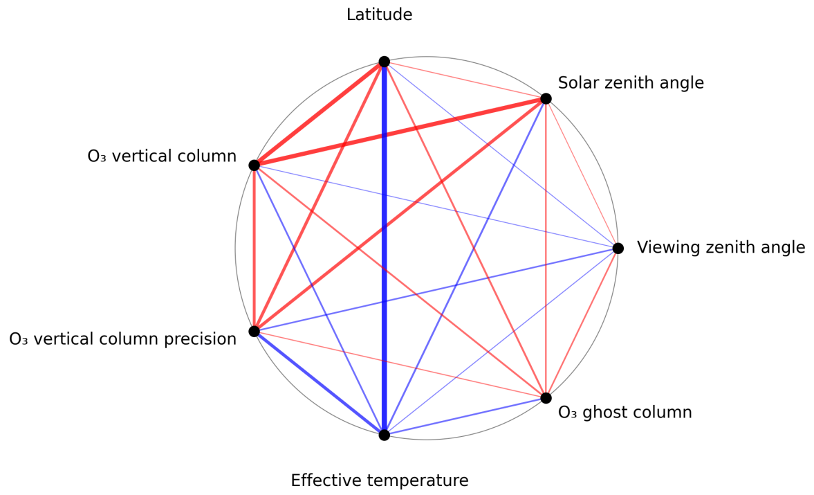
Figure 1: Map of correlation graph for 2025-02-13 to 2025-02-15.
