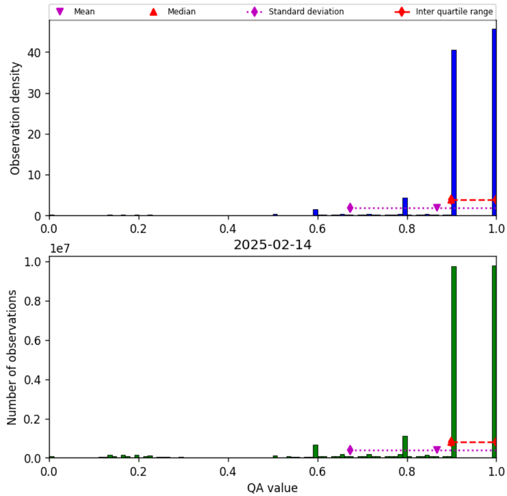
Figure 20: Histogram of “QA value” for 2025-02-13 to 2025-02-15
