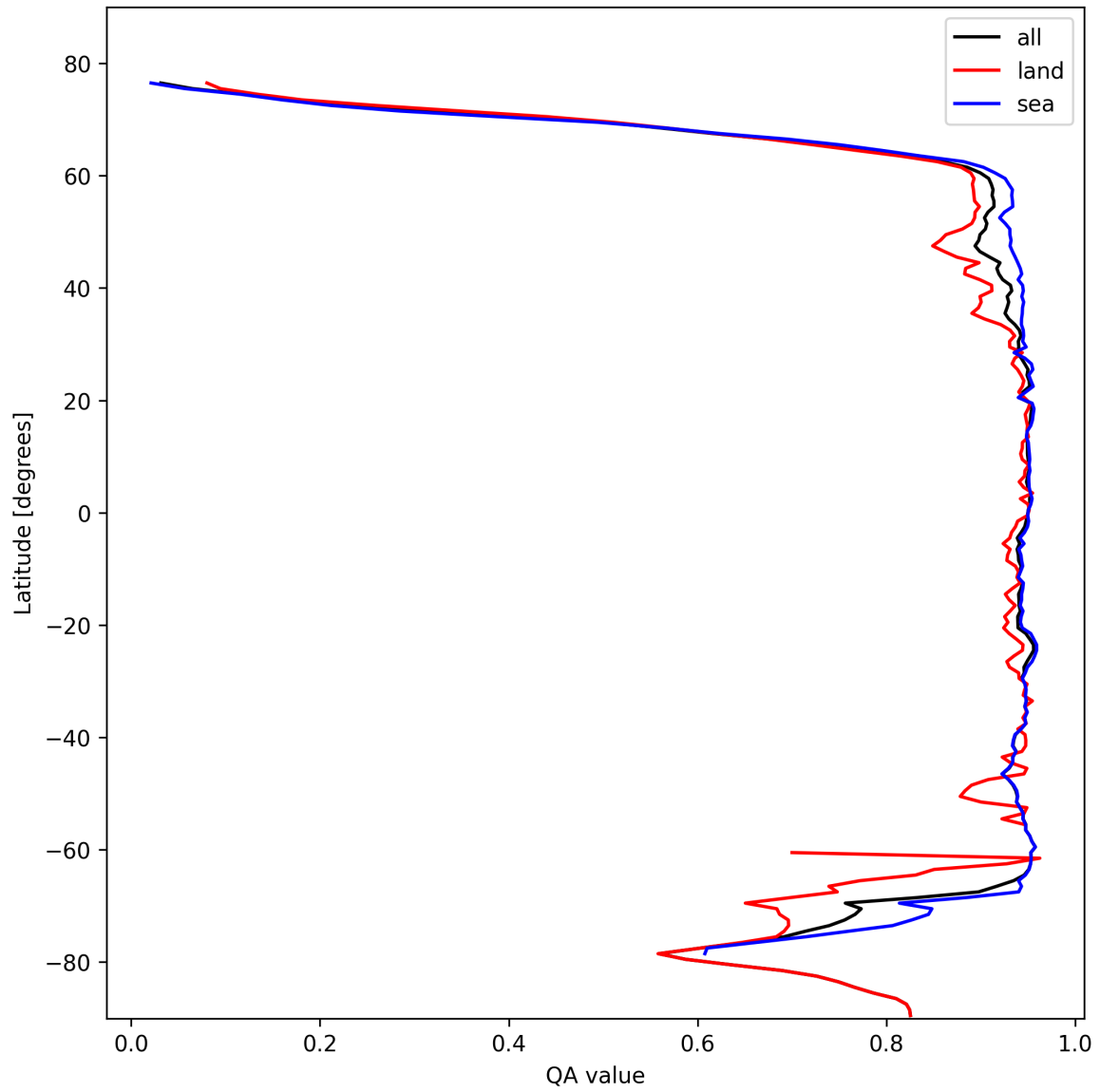
Figure 13: Zonal average of “QA value” for 2025-02-13 to 2025-02-15.
