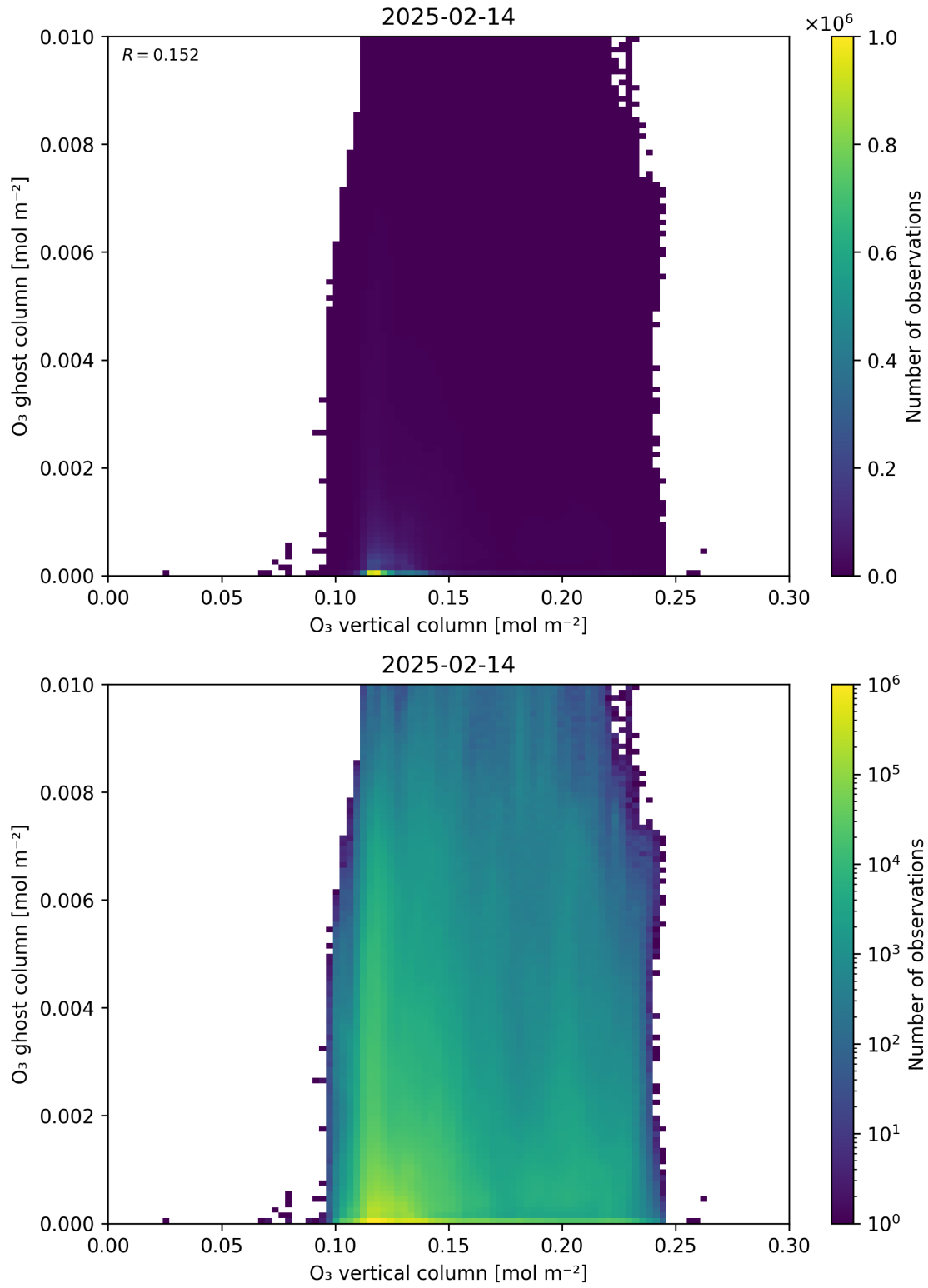
Figure 40: Scatter density plot of “O 3 vertical column” against “O 3 ghost column” for 2025-02-13 to 2025-02-15.
