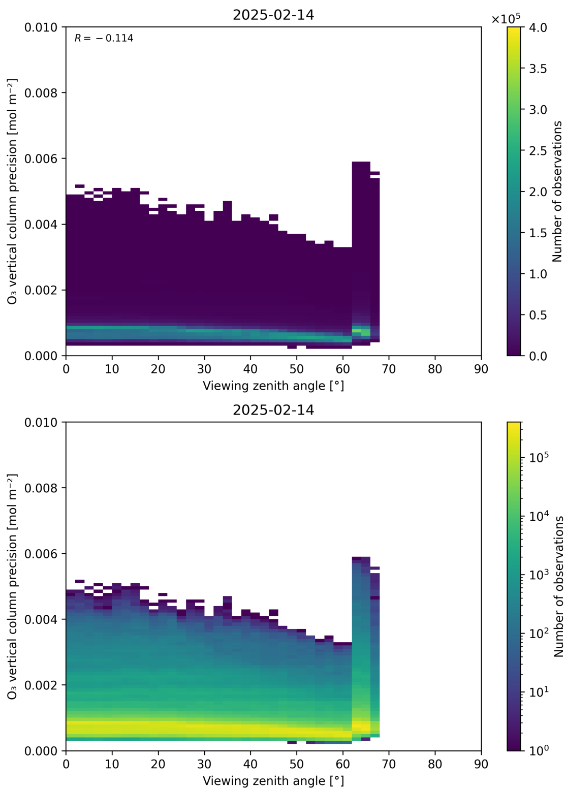
Figure 53: Scatter density plot of “Viewing zenith angle” against “O 3 vertical column precision” for 2025-02-13 to 2025-02-15.
