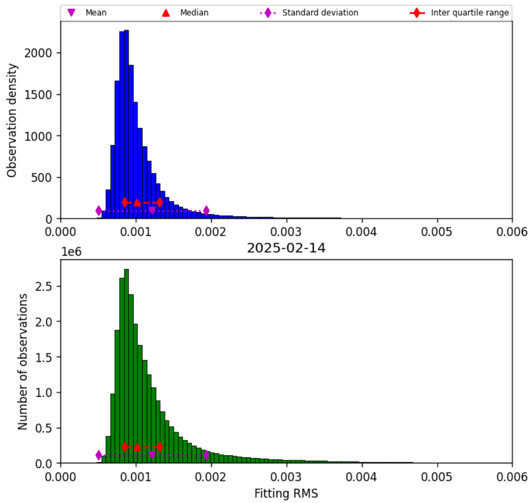
Figure 23: Histogram of “Fitting RMS” for 2025-02-13 to 2025-02-15
