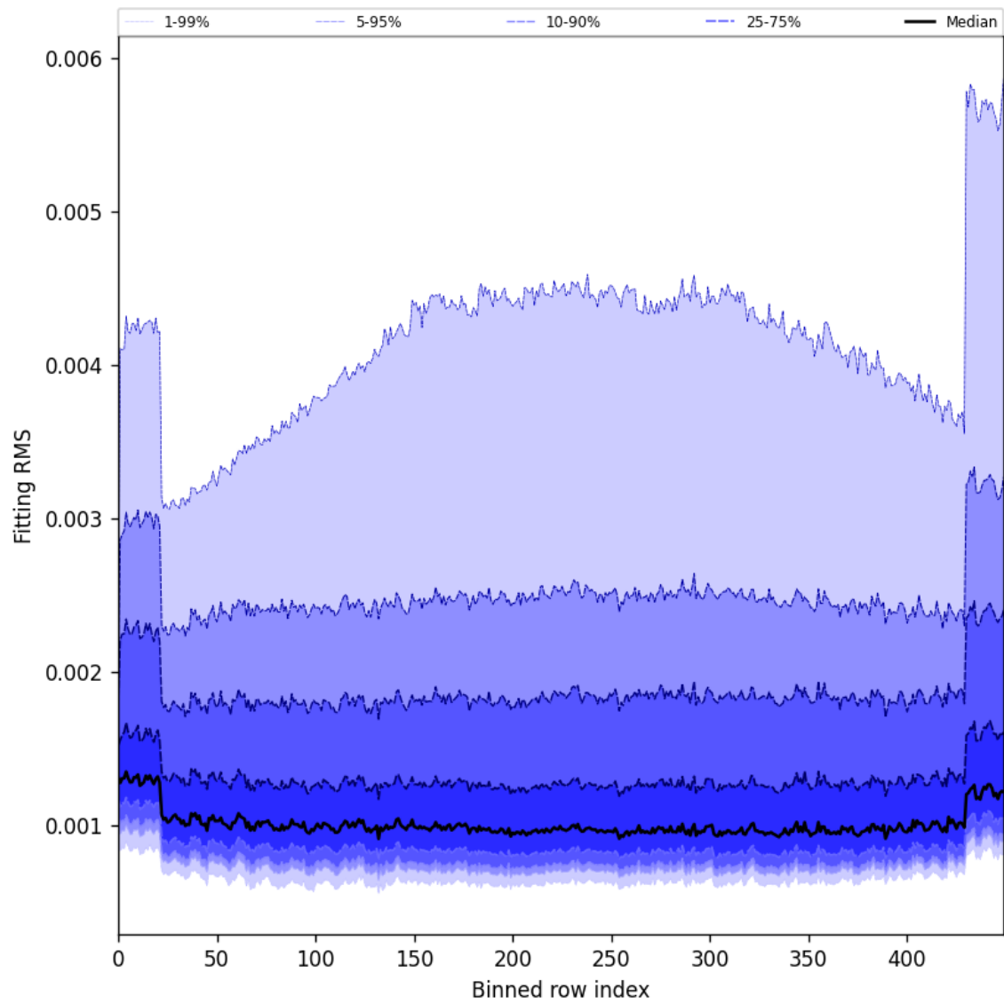
Figure 30: Along track statistics of “Fitting RMS” for 2025-02-13 to 2025-02-15
