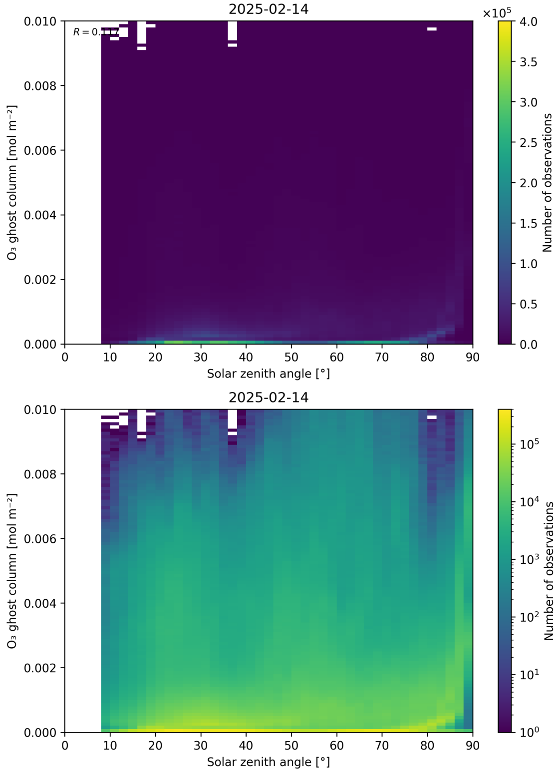
Figure 46: Scatter density plot of “Solar zenith angle” against “O 3 ghost column” for 2025-02-13 to 2025-02-15.
