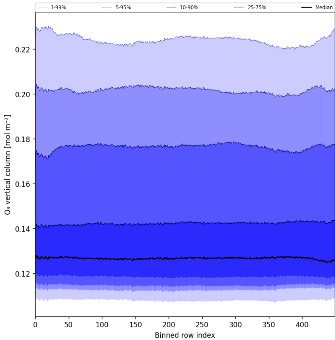
Figure 28: Along track statistics of “O 3 vertical column” for 2025-02-13 to 2025-02-15
