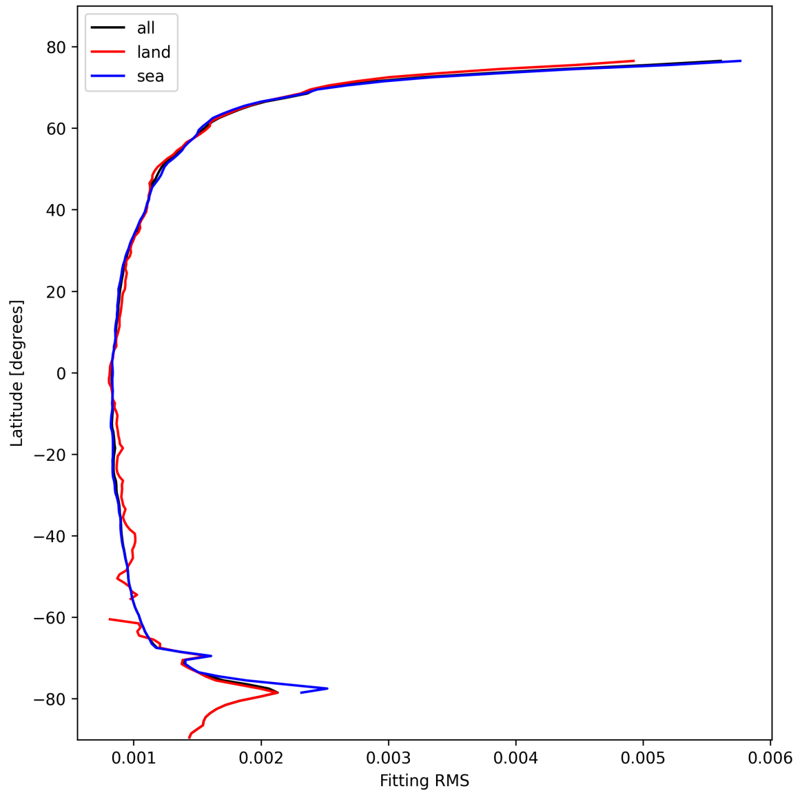
Figure 16: Zonal average of “Fitting RMS” for 2025-02-13 to 2025-02-15.
