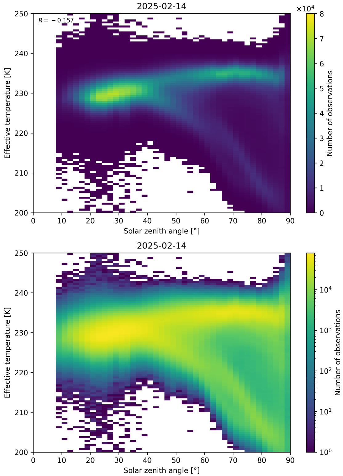
Figure 45: Scatter density plot of “Solar zenith angle” against “Effective temperature” for 2025-02-13 to 2025-02-15.
