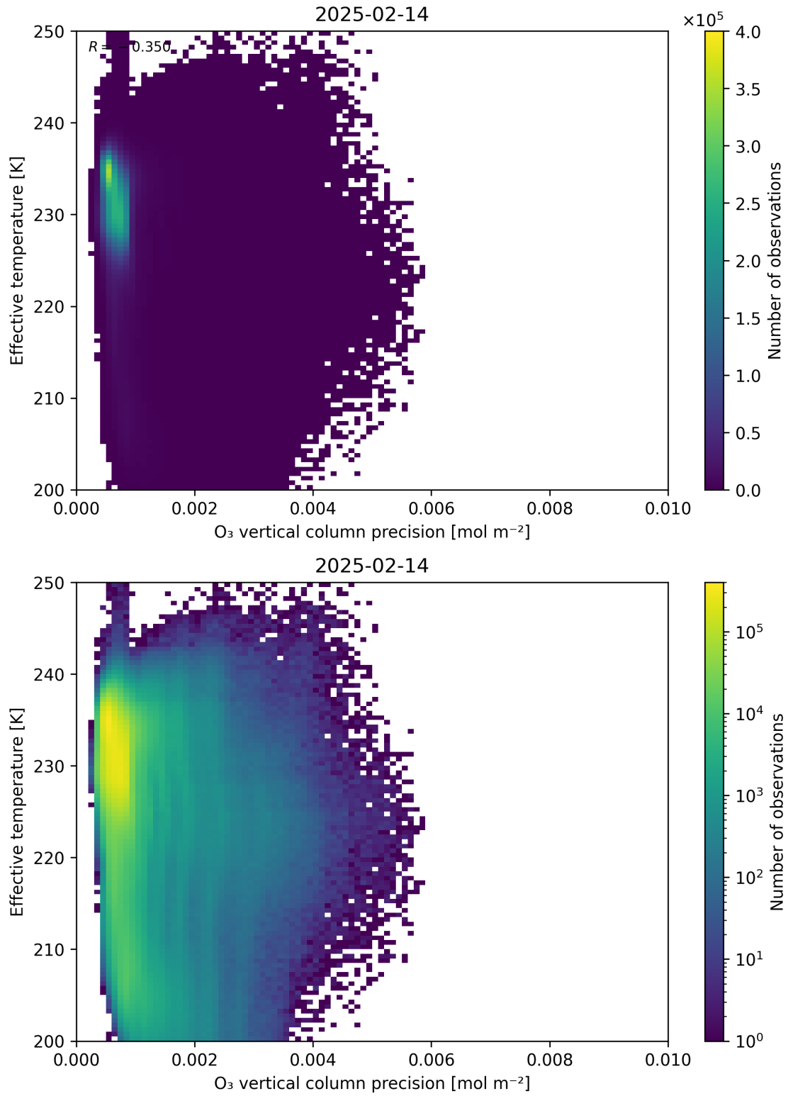
Figure 42: Scatter density plot of “O 3 vertical column precision” against “Effective temperature” for 2025-02-13 to 2025-02-15.
