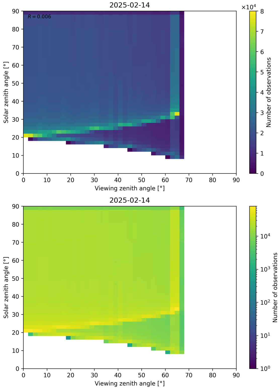
Figure 54: Scatter density plot of “Viewing zenith angle” against “Solar zenith angle” for 2025-02-13 to 2025-02-15.
