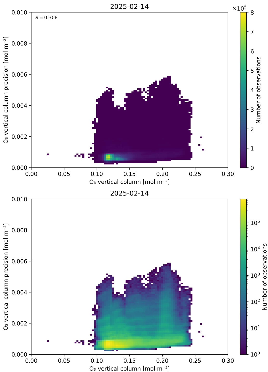
Figure 41: Scatter density plot of “O 3 vertical column” against “O 3 vertical column precision” for 2025-02-13 to 2025-02-15.
