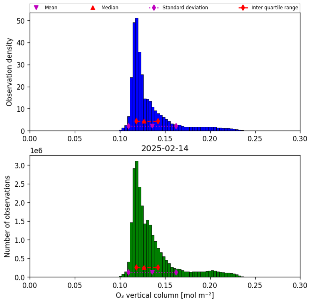
Figure 21: Histogram of “O 3 vertical column” for 2025-02-13 to 2025-02-15
