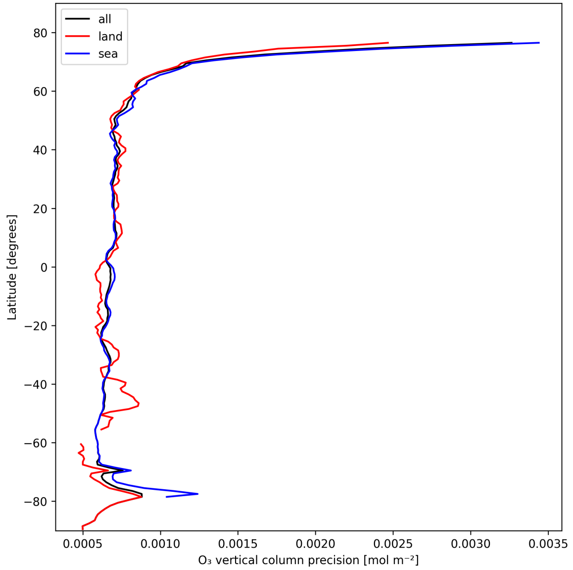
Figure 15: Zonal average of “O 3 vertical column precision” for 2025-02-13 to 2025-02-15.
