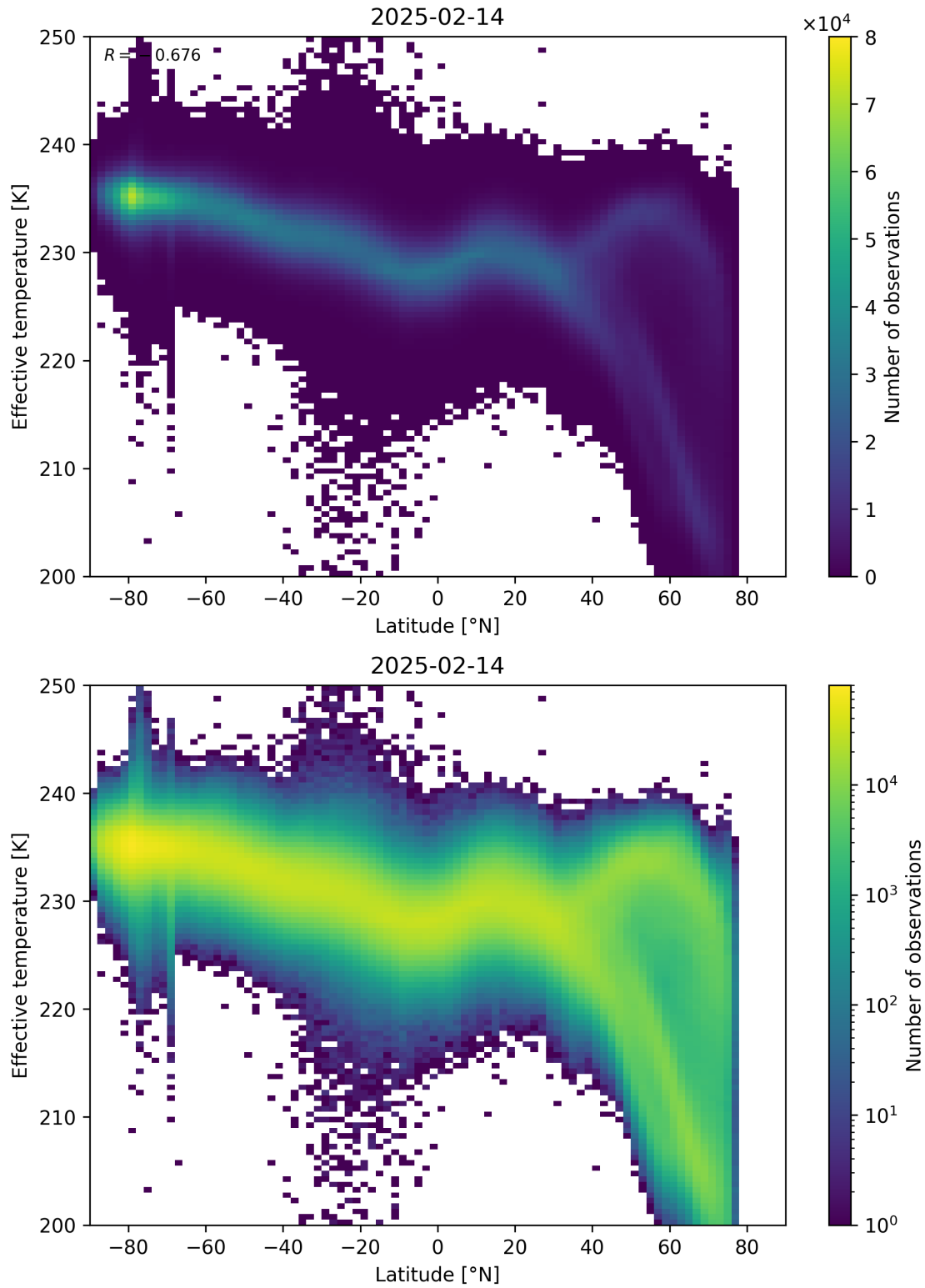
Figure 34: Scatter density plot of “Latitude” against “Effective temperature” for 2025-02-13 to 2025-02-15.
