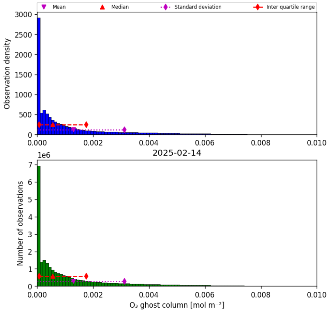
Figure 25: Histogram of “O 3 ghost column” for 2025-02-13 to 2025-02-15
