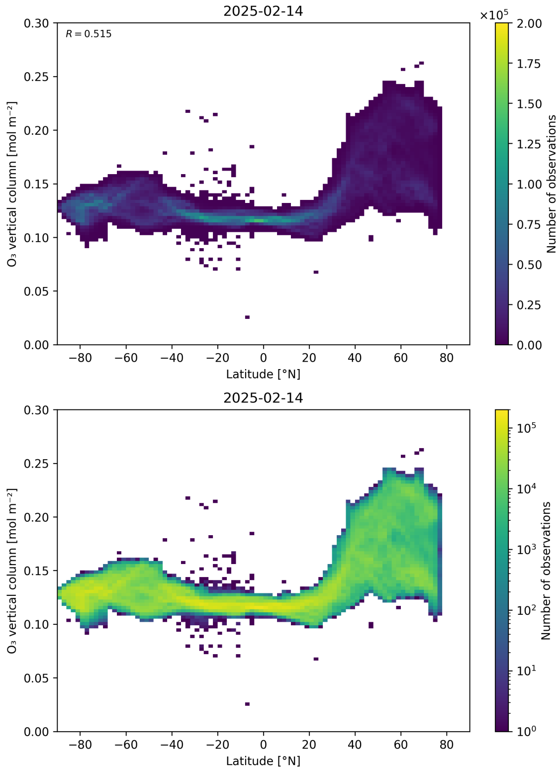
Figure 36: Scatter density plot of “Latitude” against “O 3 vertical column” for 2025-02-13 to 2025-02-15.
