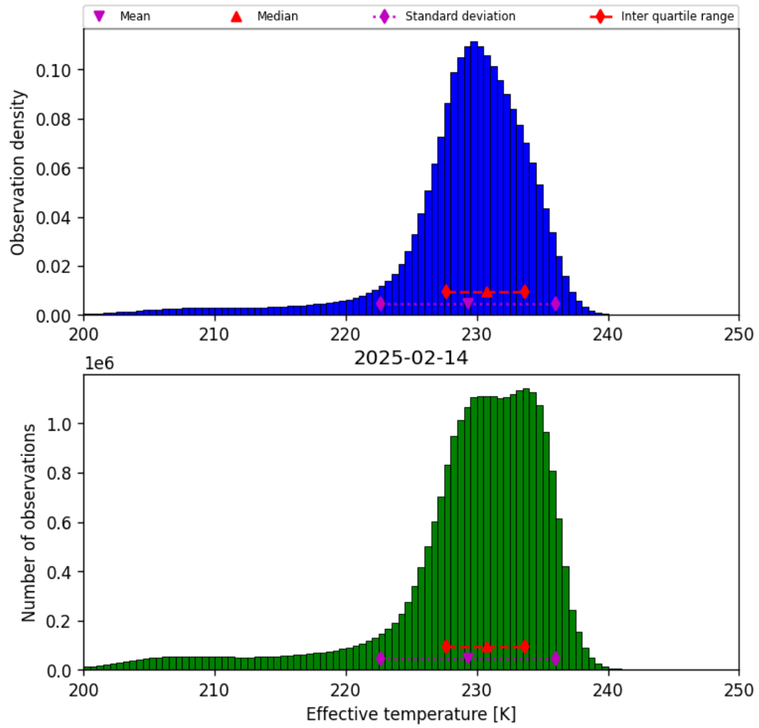
Figure 24: Histogram of “Effective temperature” for 2025-02-13 to 2025-02-15
