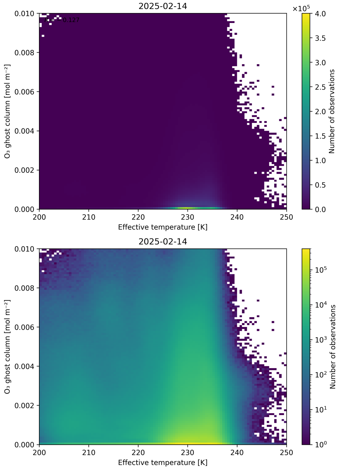
Figure 38: Scatter density plot of “Effective temperature” against “O 3 ghost column” for 2025-02-13 to 2025-02-15.
