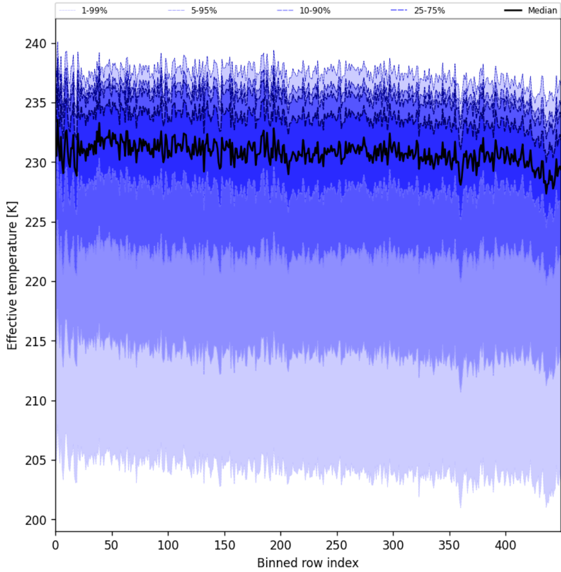
Figure 31: Along track statistics of “Effective temperature” for 2025-02-13 to 2025-02-15
