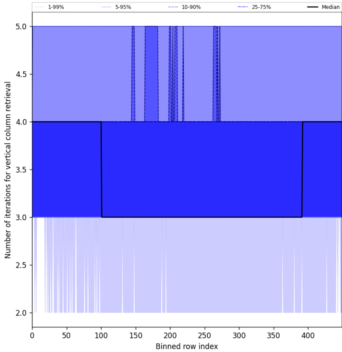
Figure 33: Along track statistics of “Number of iterations for vertical column retrieval” for 2025-02-13 to 2025-02-15
