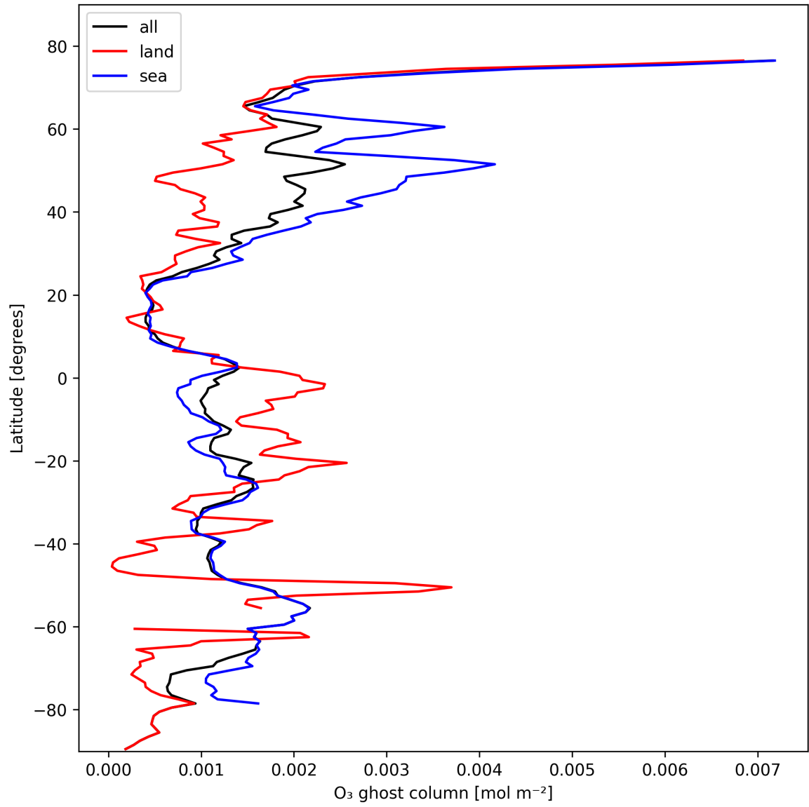
Figure 18: Zonal average of "O 3 ghost column" for 2025-02-13 to 2025-02-15.
