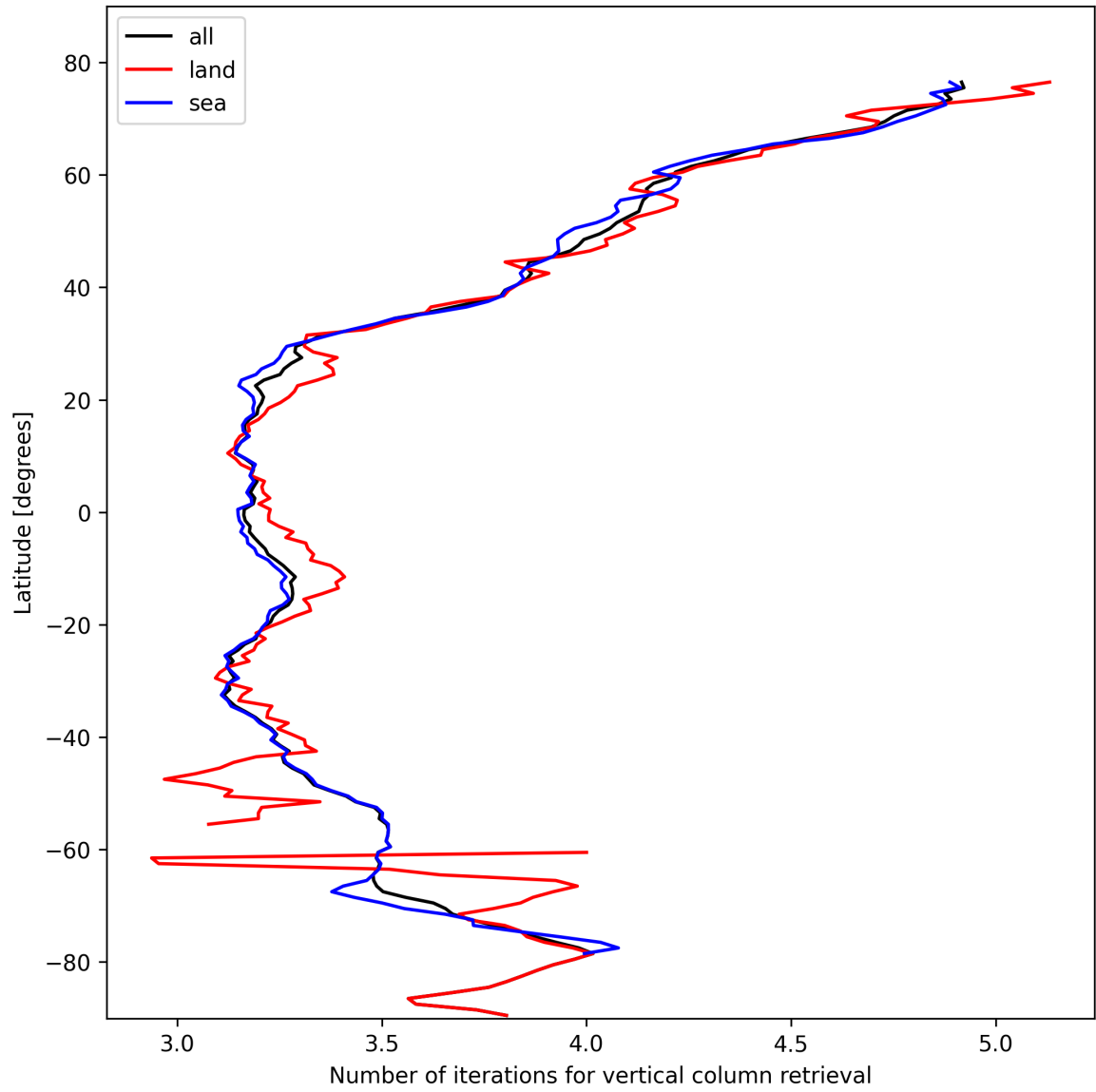
Figure 19: Zonal average of “Number of iterations for vertical column retrieval” for 2025-02-13 to 2025-02-15.
