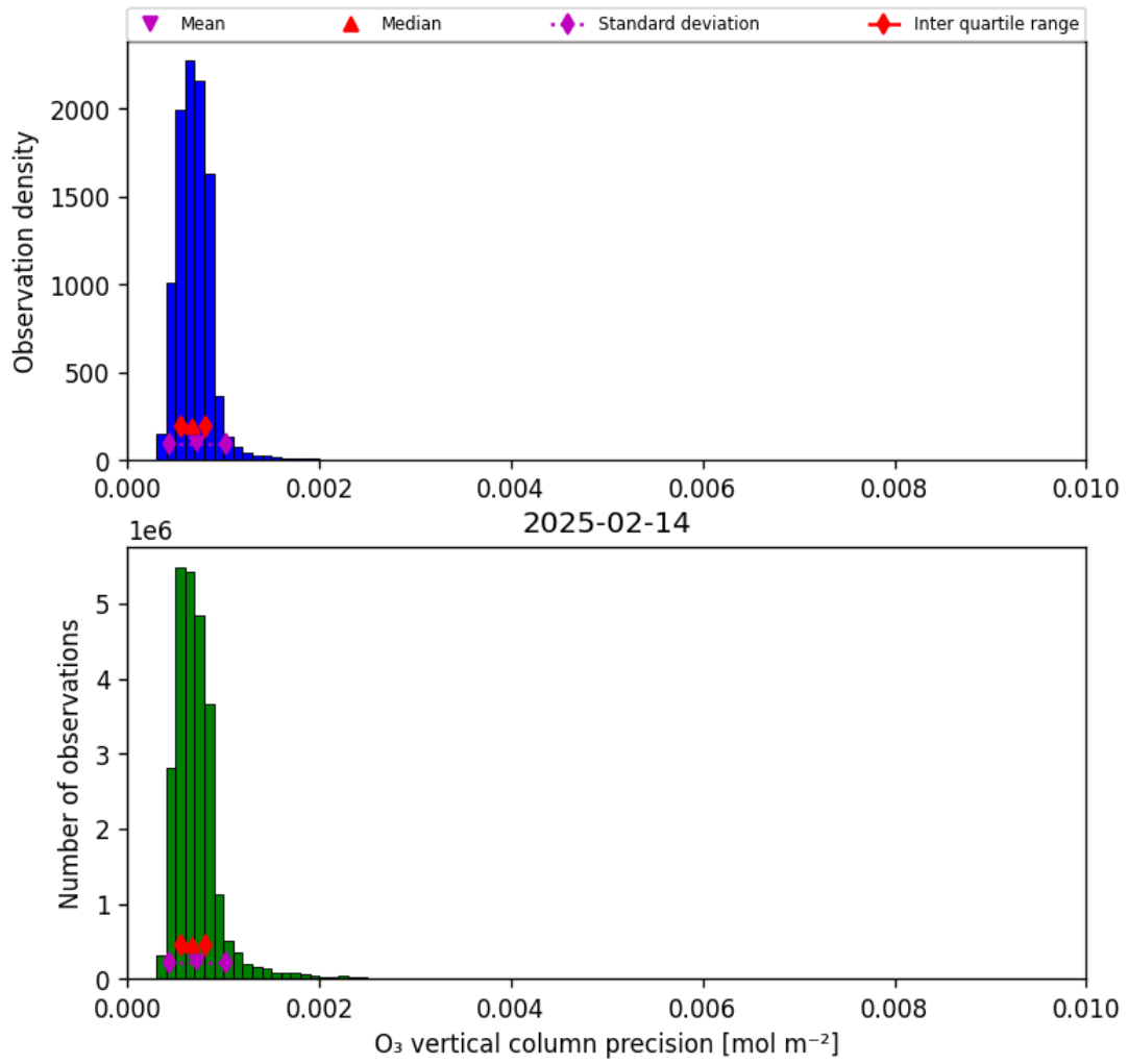
Figure 22: Histogram of “O 3 vertical column precision” for 2025-02-13 to 2025-02-15
