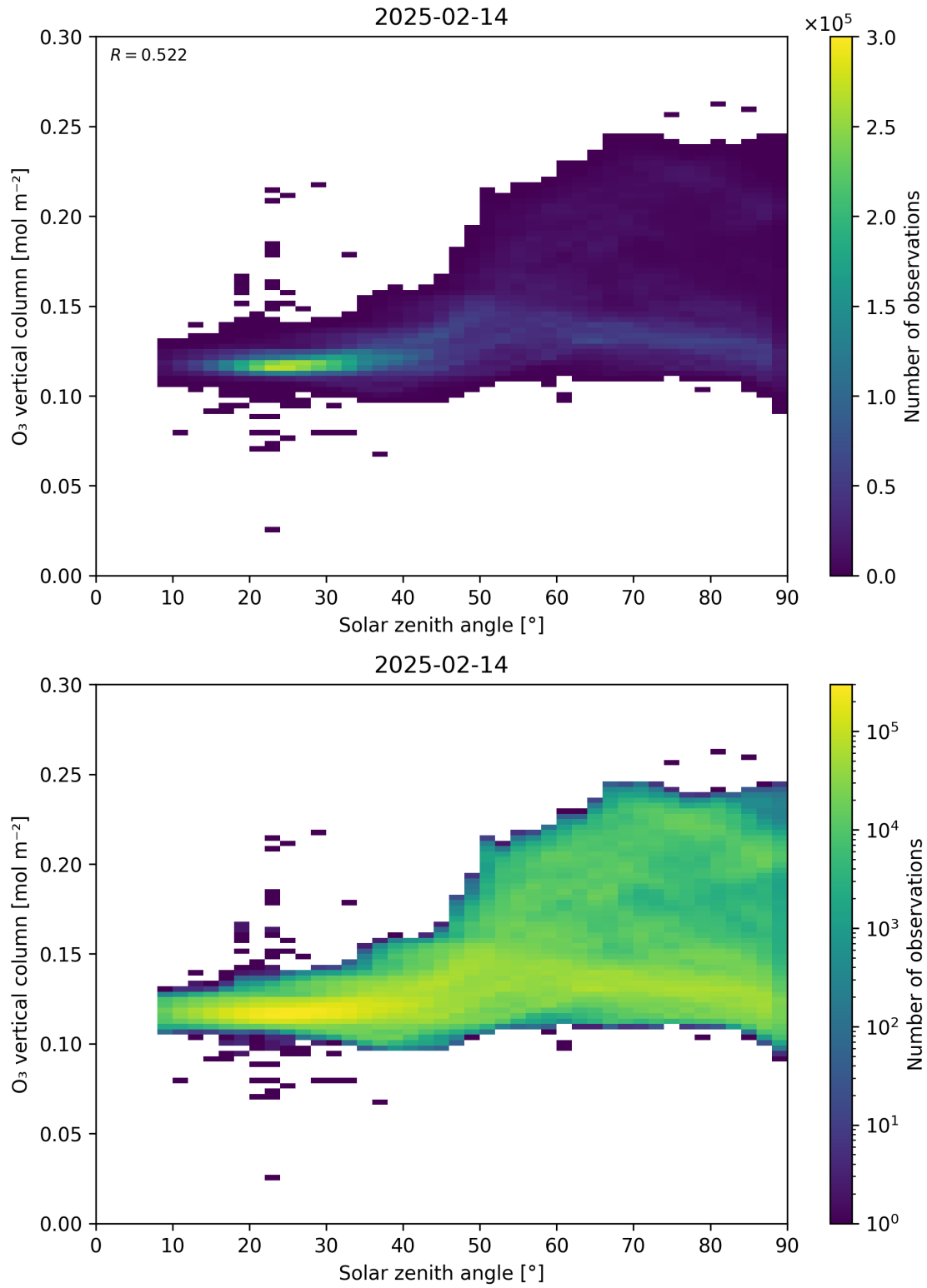
Figure 47: Scatter density plot of “Solar zenith angle” against “O 3 vertical column” for 2025-02-13 to 2025-02-15.
