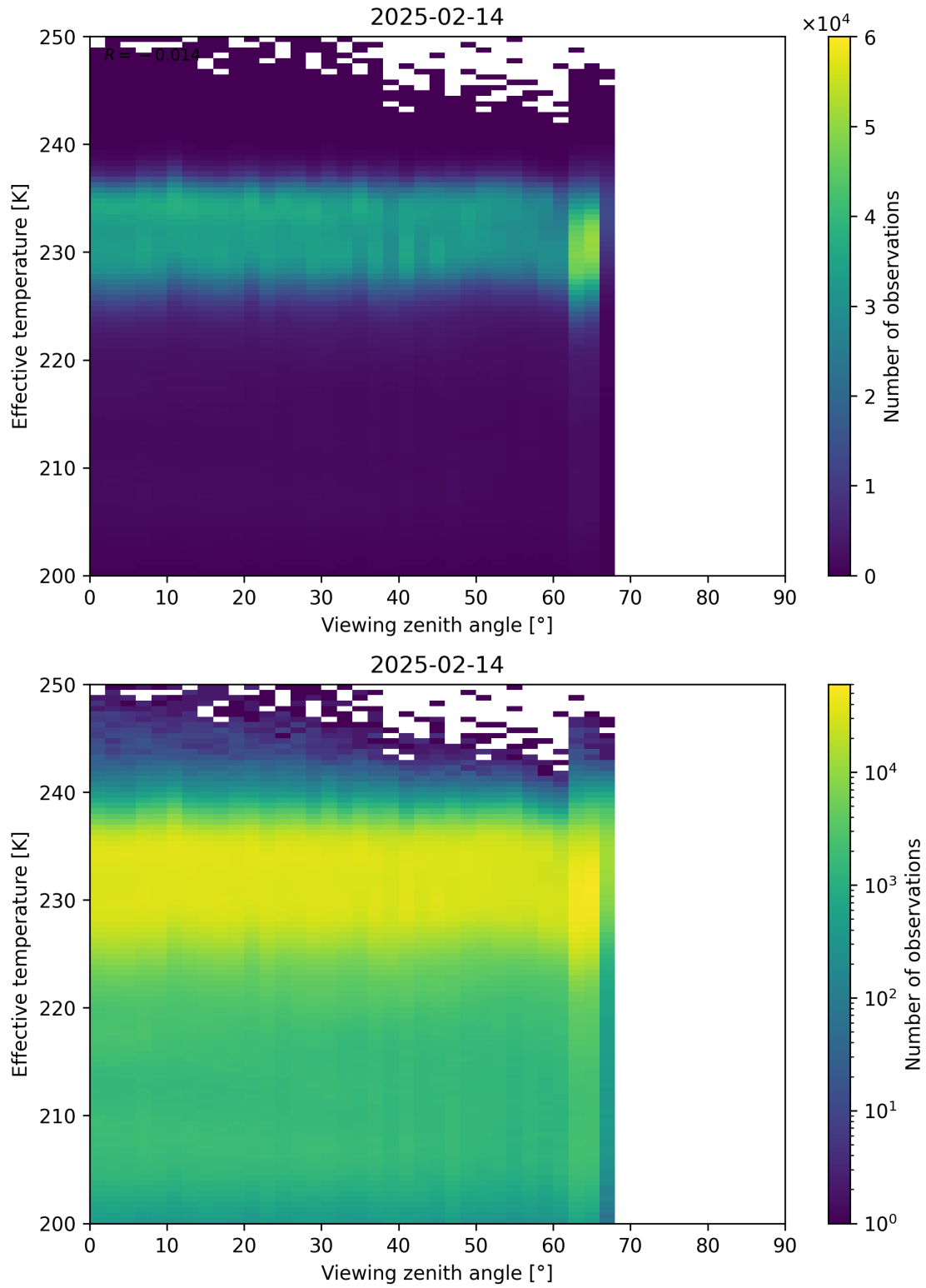
Figure 50: Scatter density plot of “Viewing zenith angle” against “Effective temperature” for 2025-02-13 to 2025-02-15.
