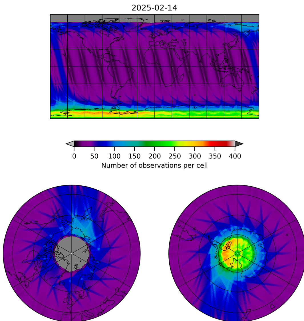
Figure 12: Map of the number of observations for 2025-02-13 to 2025-02-15
