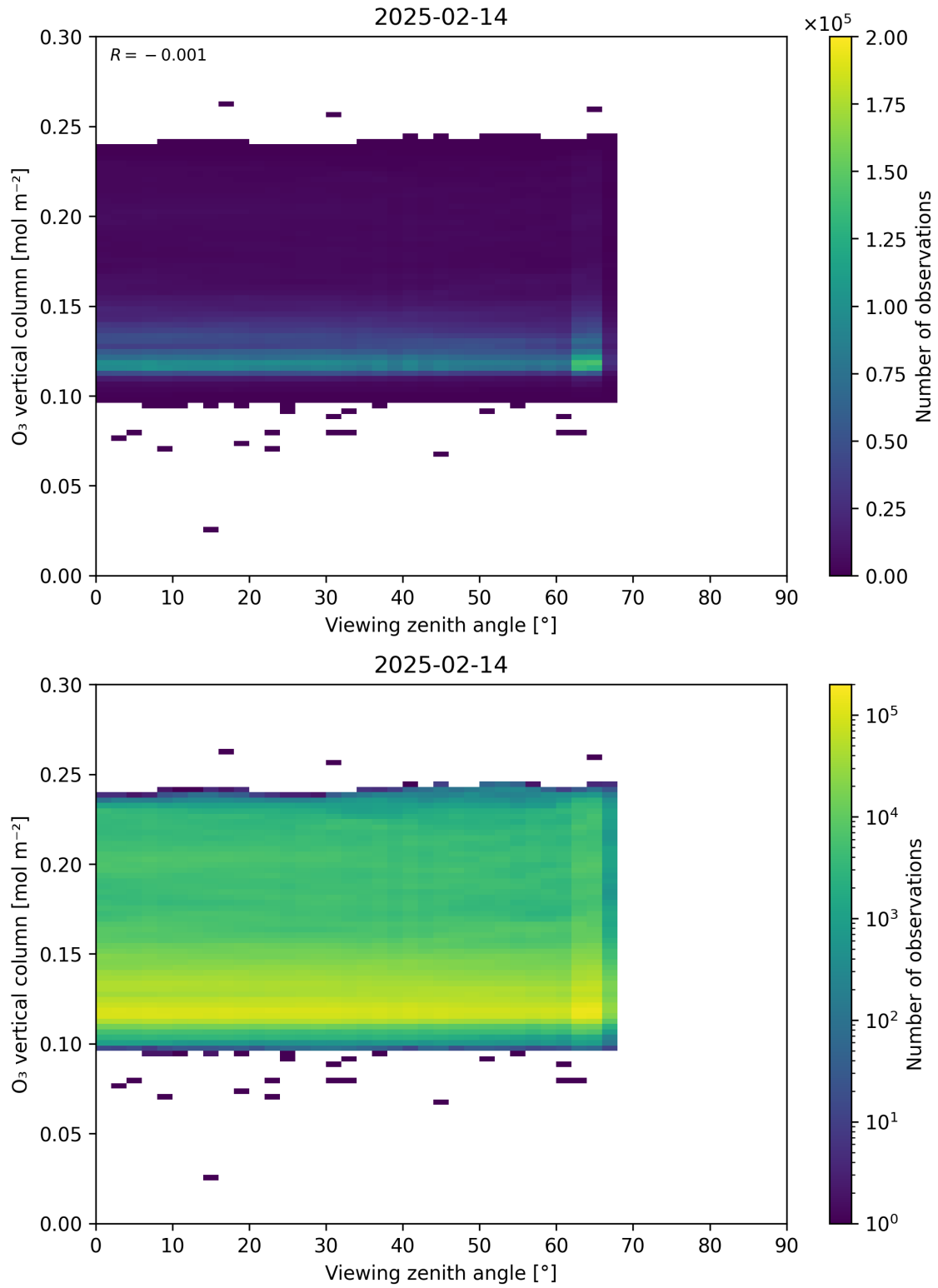
Figure 52: Scatter density plot of “Viewing zenith angle” against “O 3 vertical column” for 2025-02-13 to 2025-02-15.
