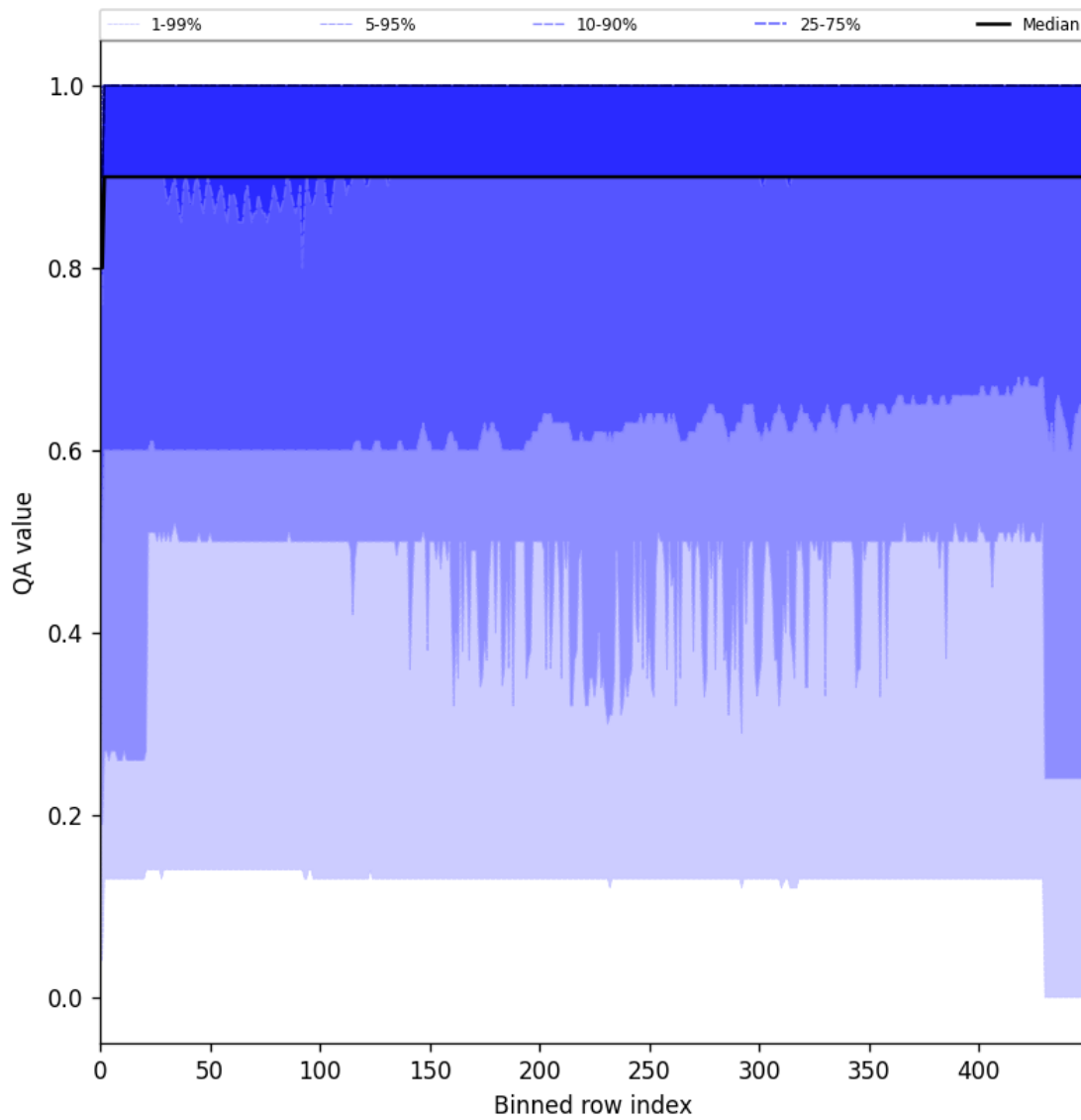
Figure 27: Along track statistics of “QA value” for 2025-02-13 to 2025-02-15
