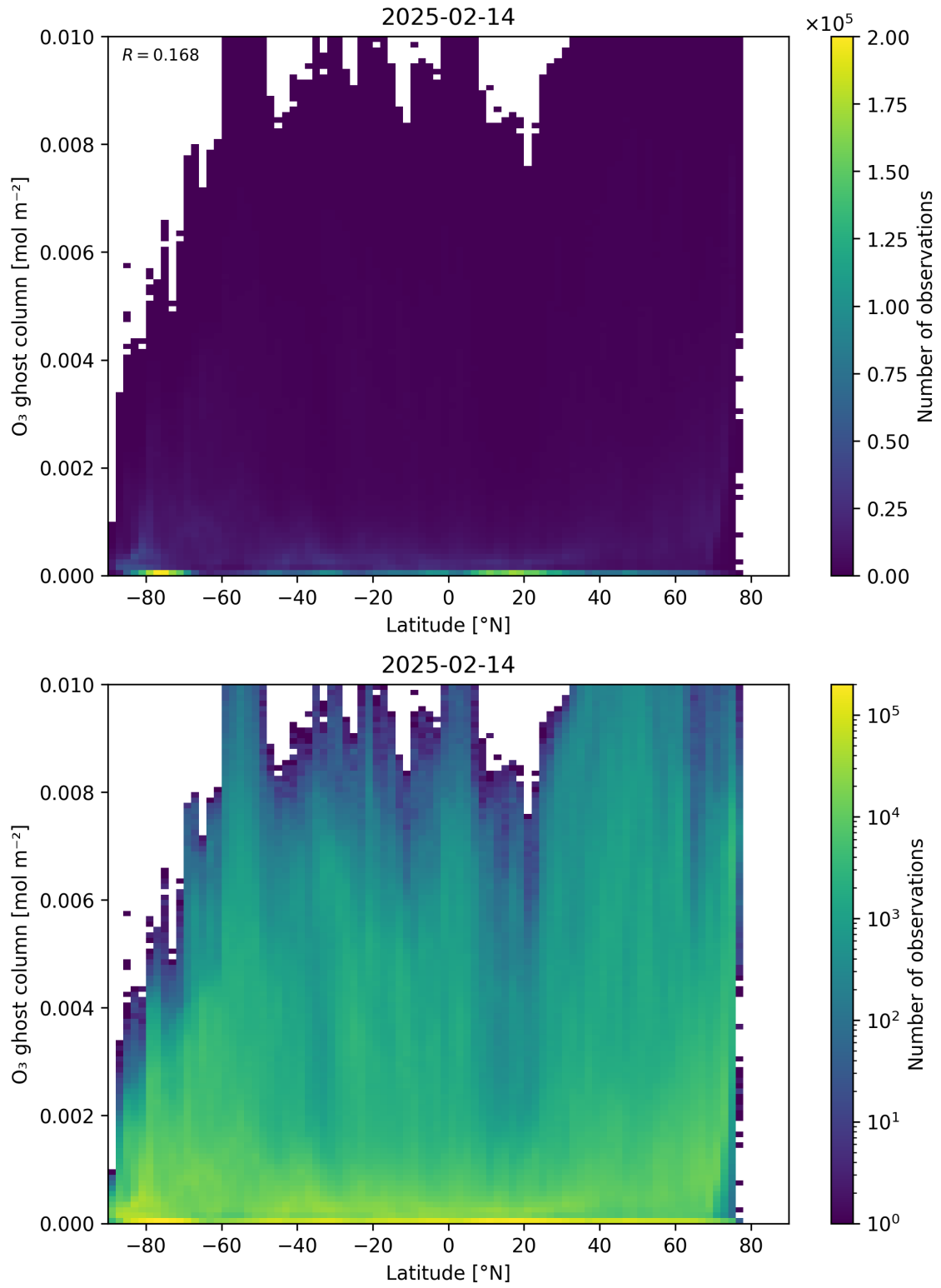
Figure 35: Scatter density plot of “Latitude” against “O 3 ghost column” for 2025-02-13 to 2025-02-15.
