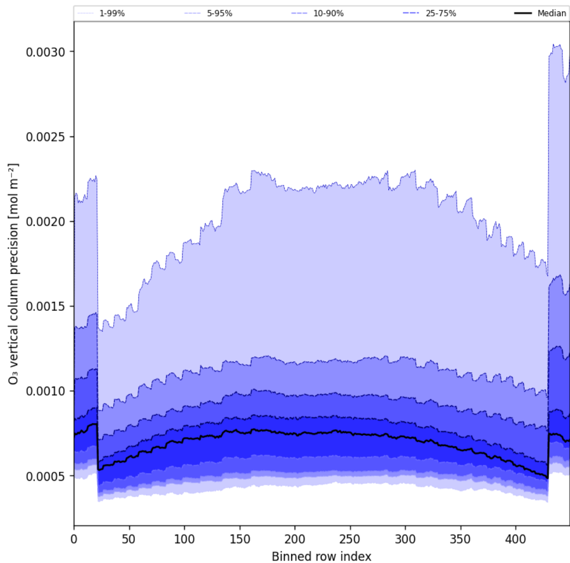
Figure 29: Along track statistics of “O 3 vertical column precision” for 2025-02-13 to 2025-02-15
