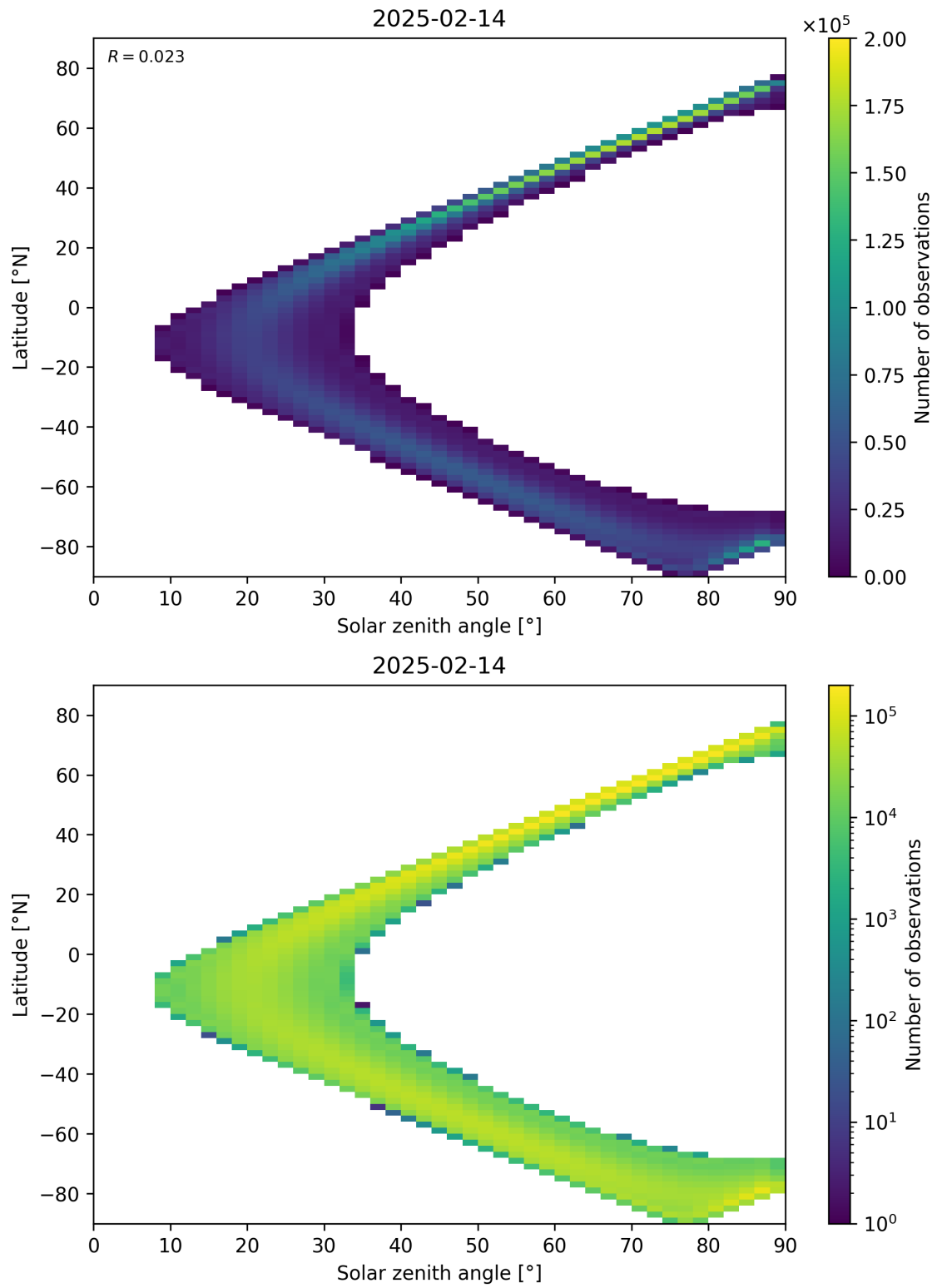
Figure 44: Scatter density plot of “Solar zenith angle” against “Latitude” for 2025-02-13 to 2025-02-15.
