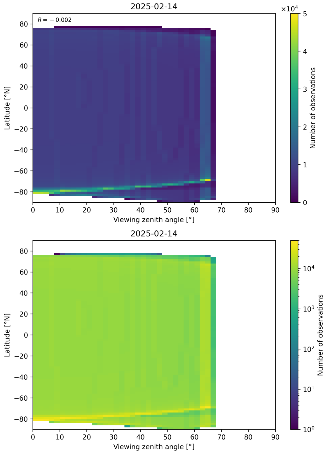
Figure 49: Scatter density plot of “Viewing zenith angle” against “Latitude” for 2025-02-13 to 2025-02-15.
