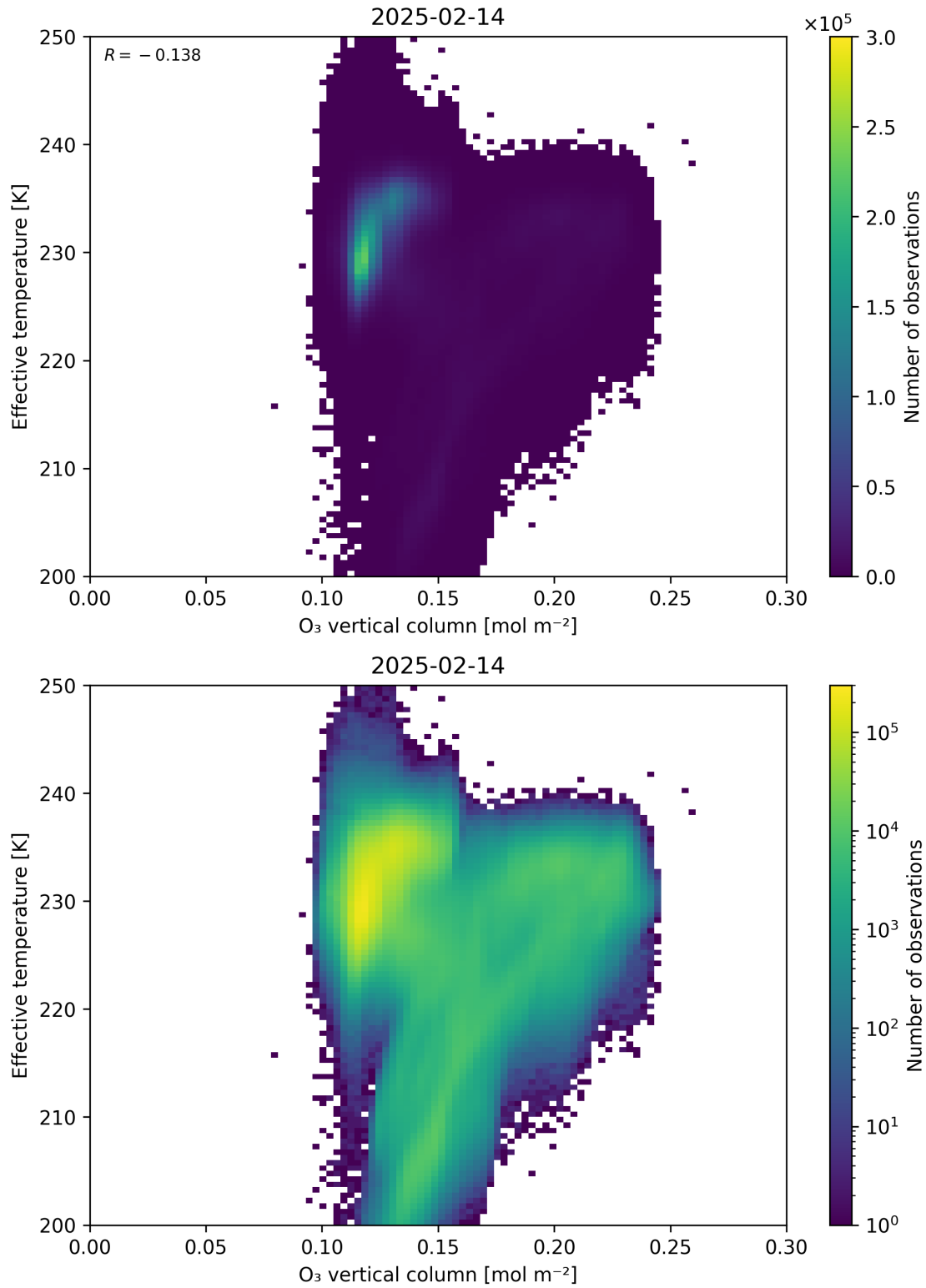
Figure 39: Scatter density plot of “O 3 vertical column” against “Effective temperature” for 2025-02-13 to 2025-02-15.
