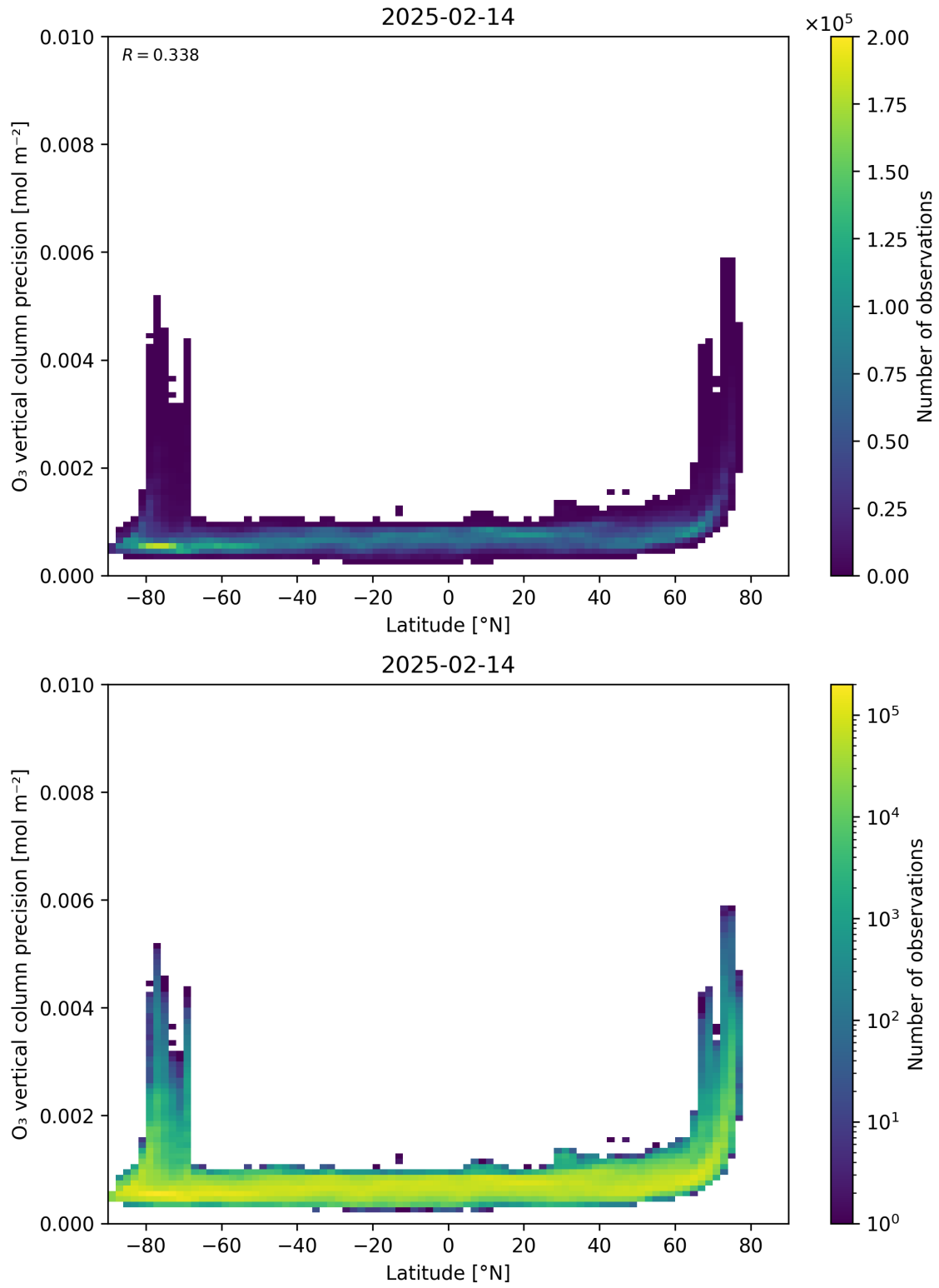
Figure 37: Scatter density plot of “Latitude” against “O 3 vertical column precision” for 2025-02-13 to 2025-02-15.
