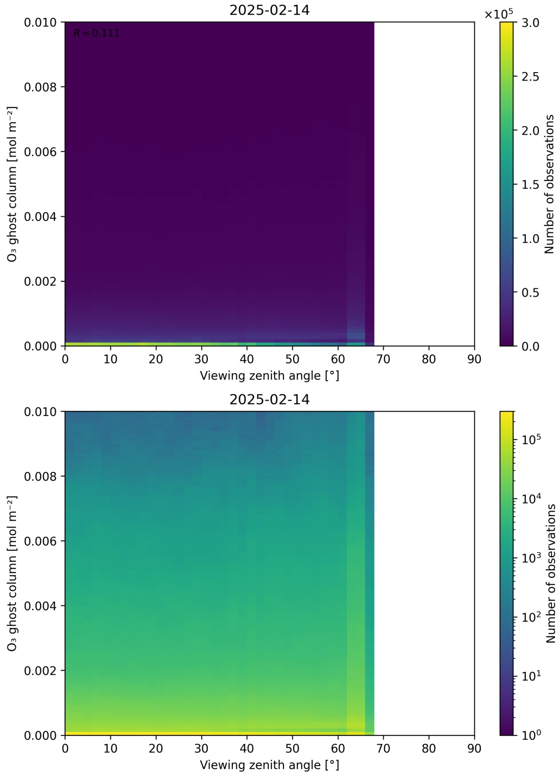
Figure 51: Scatter density plot of “Viewing zenith angle” against “O 3 ghost column” for 2025-02-13 to 2025-02-15.
