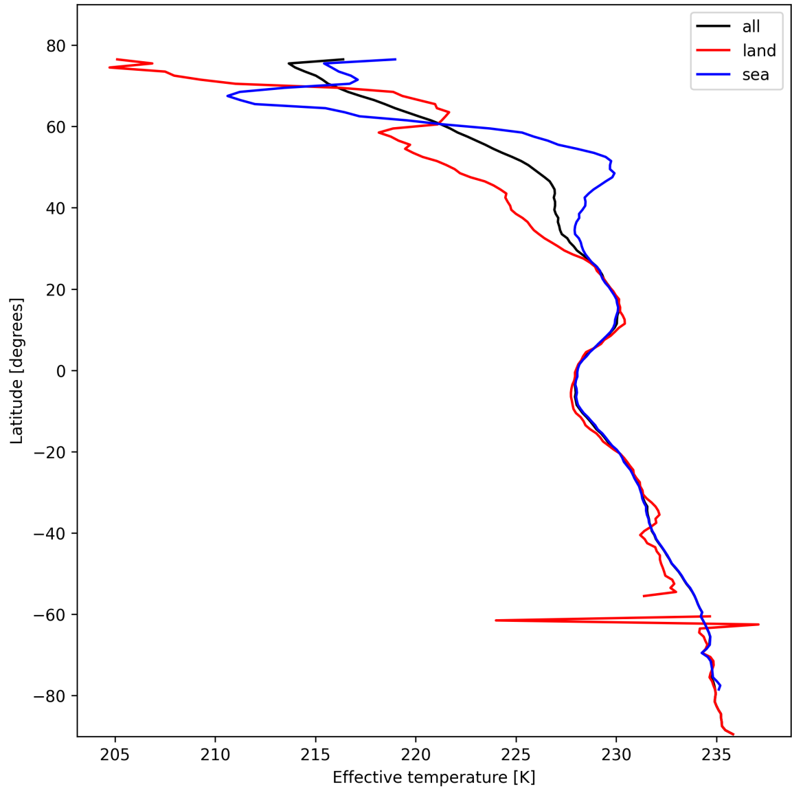
Figure 17: Zonal average of "Effective temperature" for 2025-02-13 to 2025-02-15.
