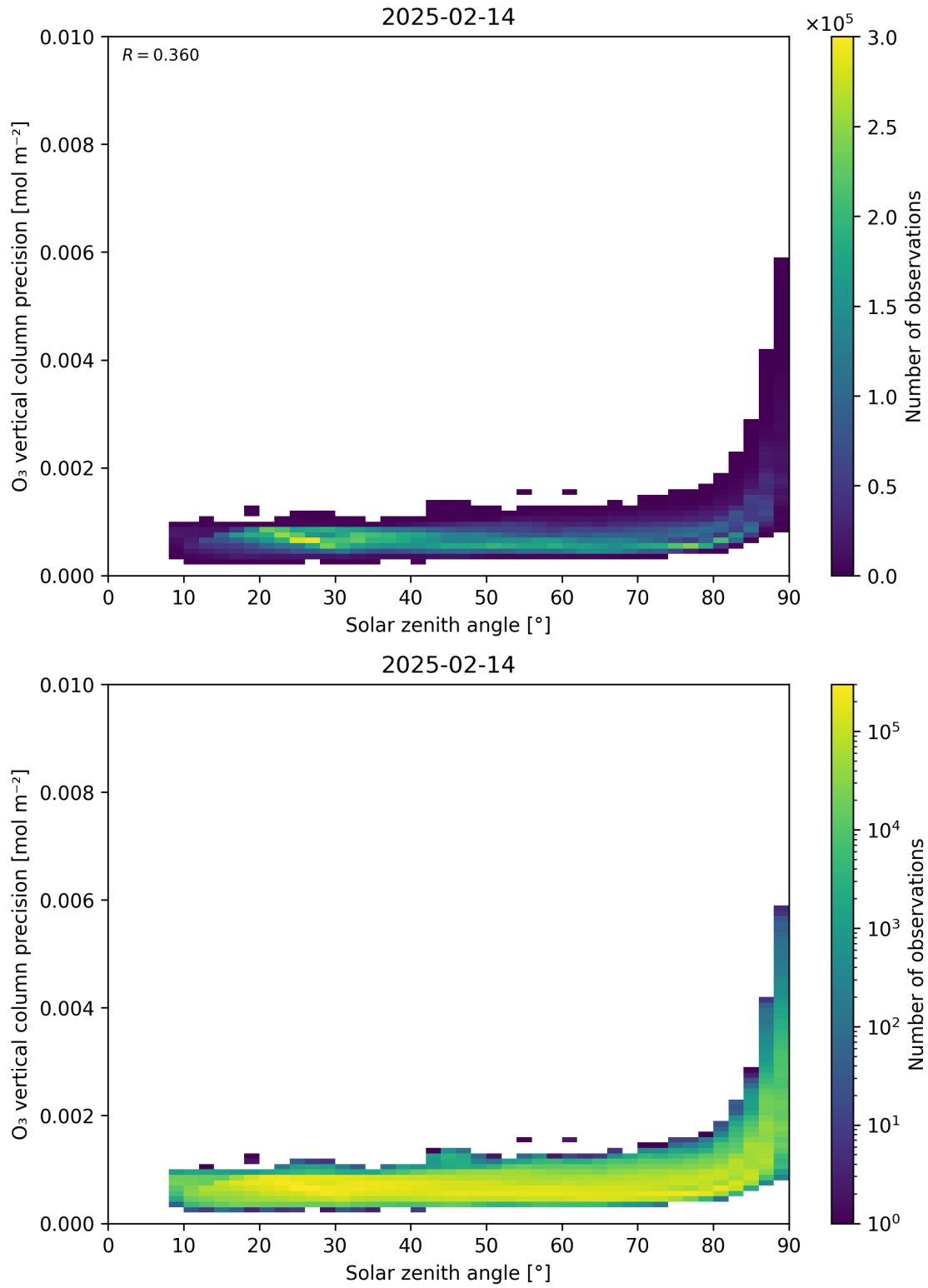
Figure 48: Scatter density plot of “Solar zenith angle” against “O 3 vertical column precision” for 2025-02-13 to 2025-02-15.
