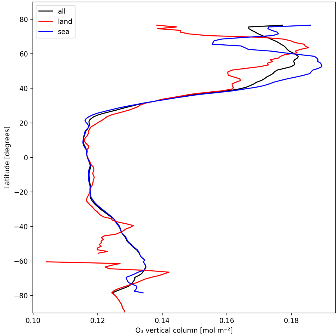
Figure 14: Zonal average of “O 3 vertical column” for 2025-02-13 to 2025-02-15.
