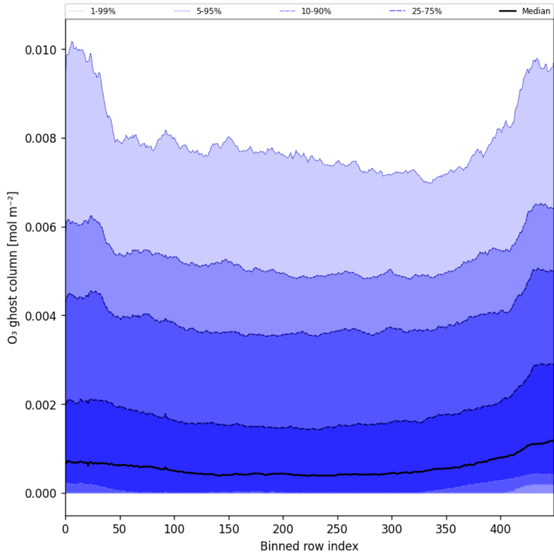
Figure 32: Along track statistics of “O 3 ghost column” for 2025-02-14 to 2025-02-16
