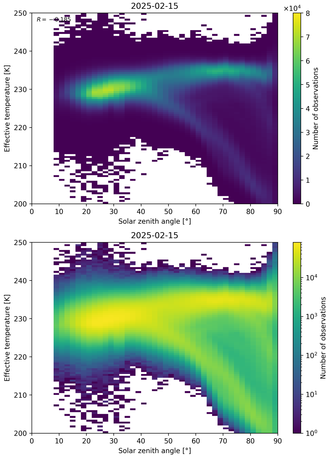
Figure 45: Scatter density plot of “Solar zenith angle” against “Effective temperature” for 2025-02-14 to 2025-02-16.
