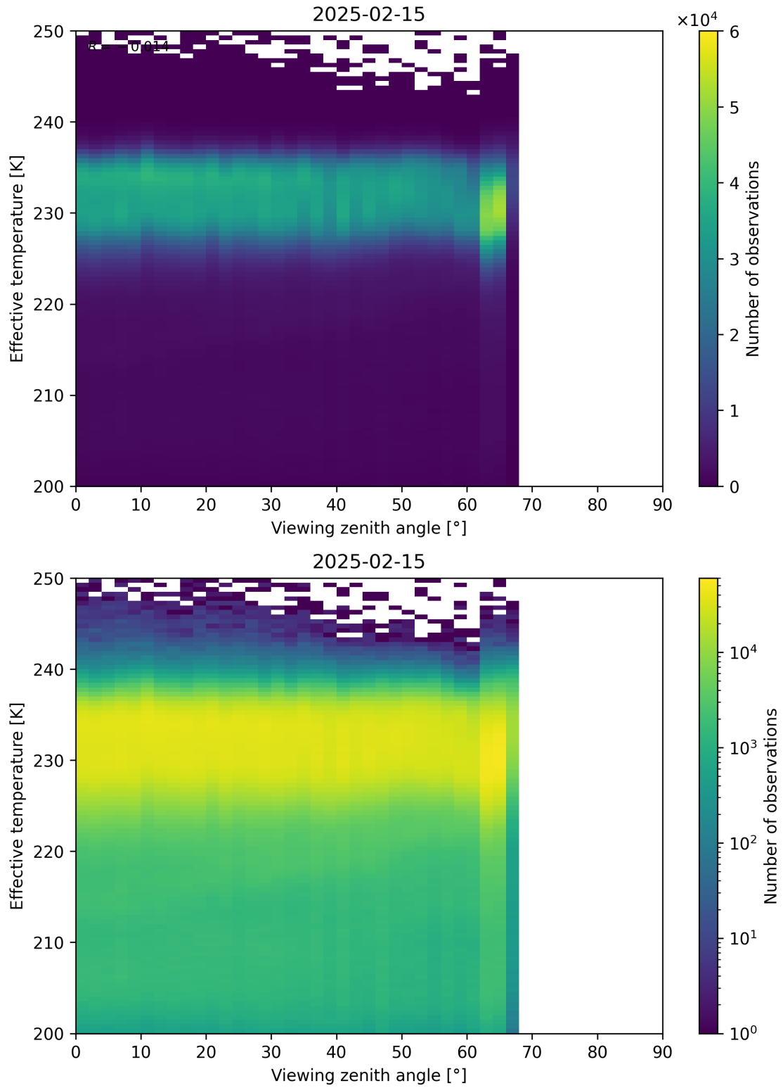
Figure 50: Scatter density plot of “Viewing zenith angle” against “Effective temperature” for 2025-02-14 to 2025-02-16.
