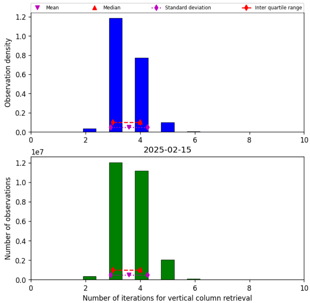
Figure 26: Histogram of “Number of iterations for vertical column retrieval” for 2025-02-14 to 2025-02-16
