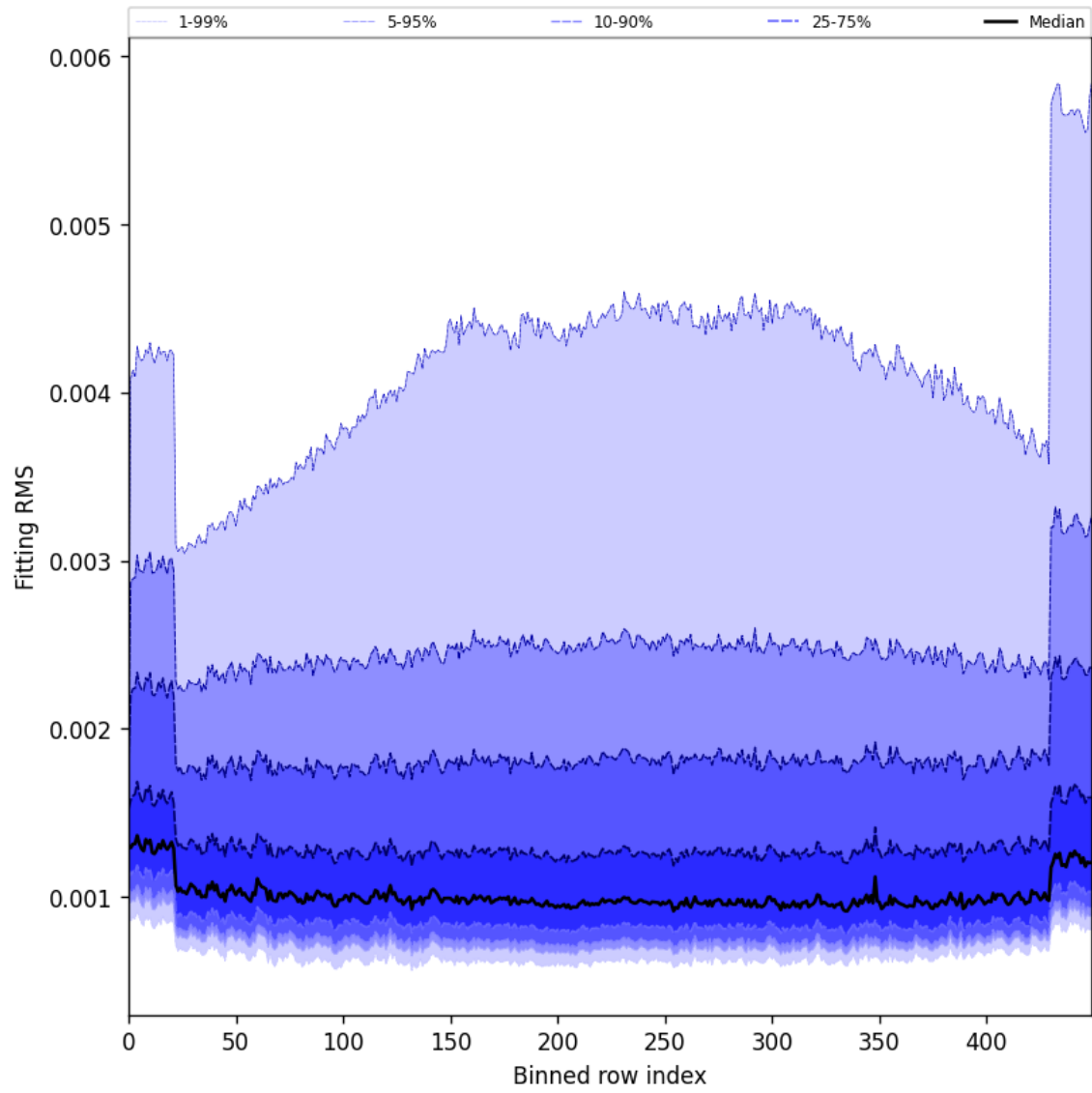
Figure 30: Along track statistics of “Fitting RMS” for 2025-02-14 to 2025-02-16
