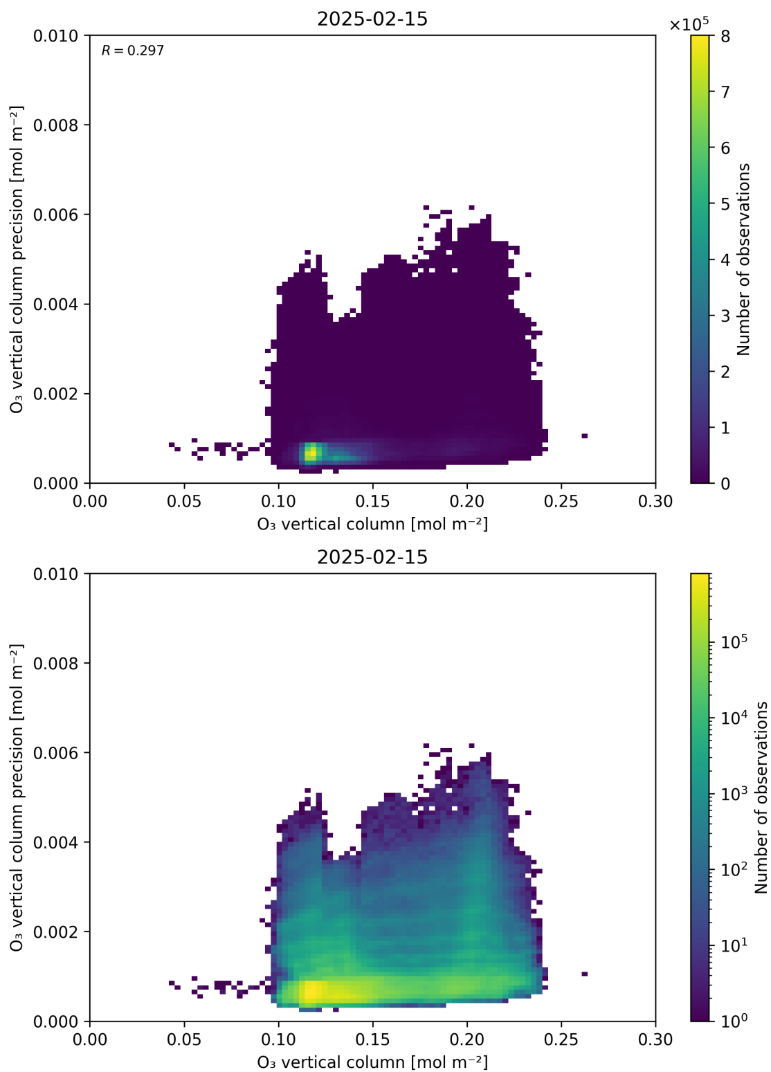
Figure 41: Scatter density plot of “O 3 vertical column” against “O 3 vertical column precision” for 2025-02-14 to 2025-02-16.
