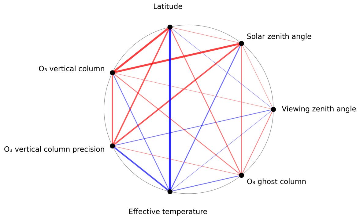
Figure 1: Map of correlation graph for 2025-02-14 to 2025-02-16.
