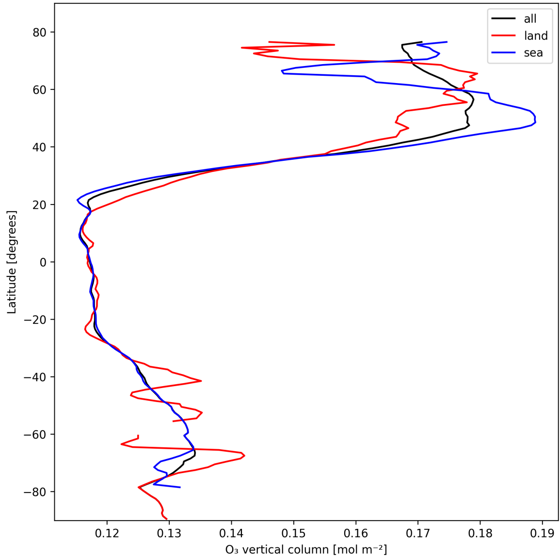
Figure 14: Zonal average of “O 3 vertical column” for 2025-02-14 to 2025-02-16.
