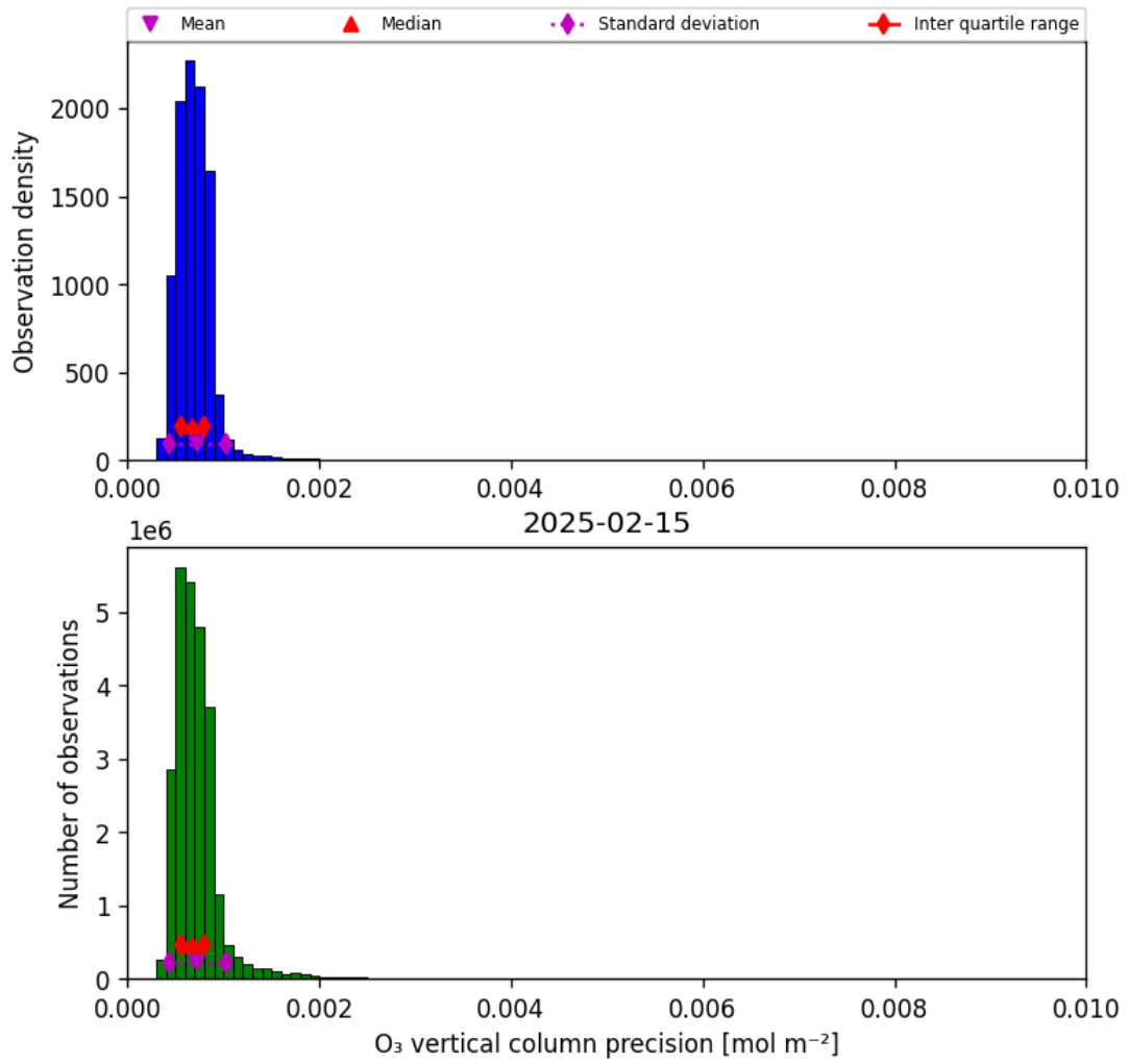
Figure 22: Histogram of “O 3 vertical column precision” for 2025-02-14 to 2025-02-16
