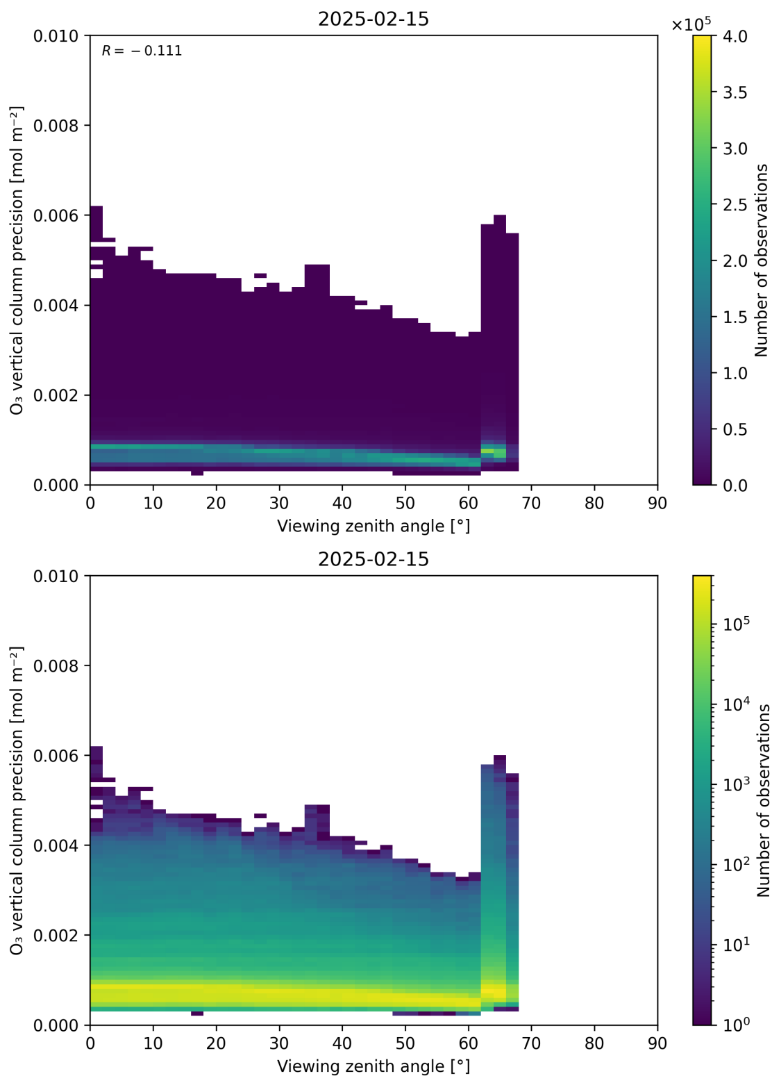
Figure 53: Scatter density plot of “Viewing zenith angle” against “O 3 vertical column precision” for 2025-02-14 to 2025-02-16.
