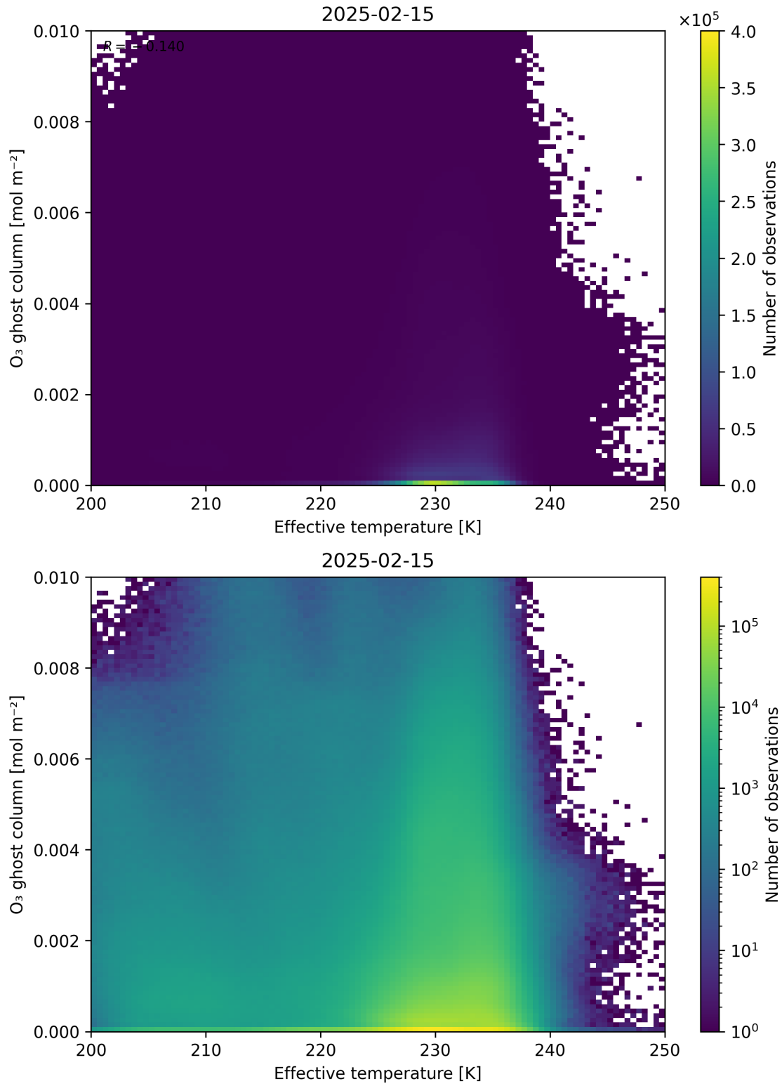
Figure 38: Scatter density plot of “Effective temperature” against “O 3 ghost column” for 2025-02-14 to 2025-02-16.
