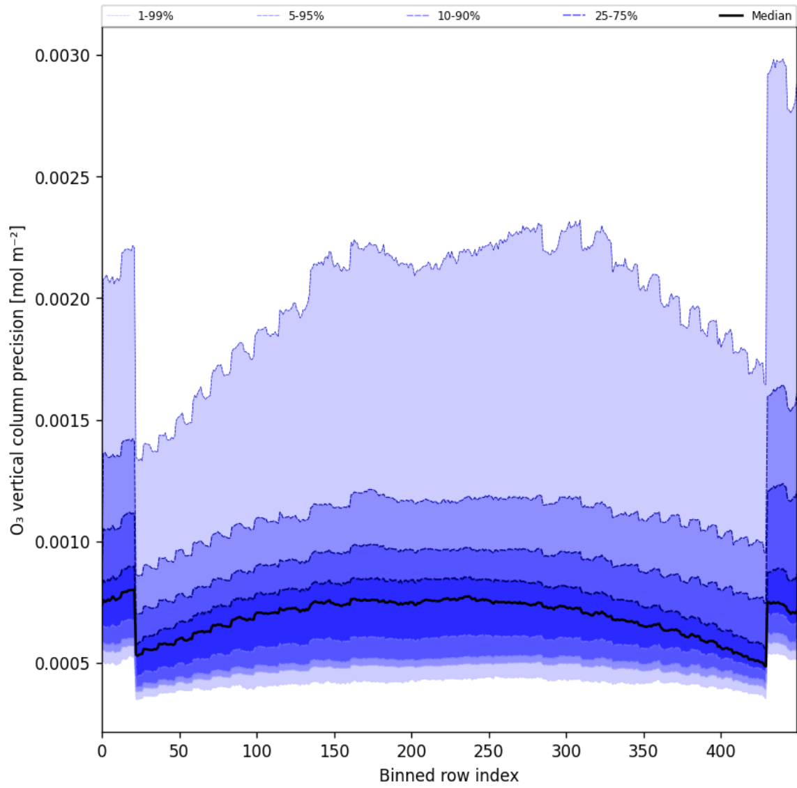
Figure 29: Along track statistics of “O 3 vertical column precision” for 2025-02-14 to 2025-02-16
