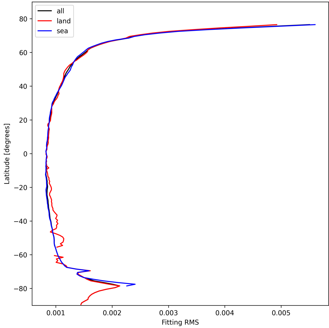
Figure 16: Zonal average of “Fitting RMS” for 2025-02-14 to 2025-02-16.
