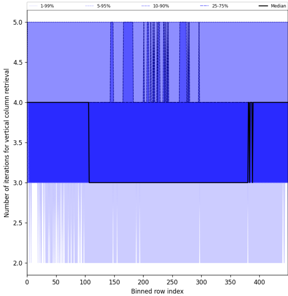
Figure 33: Along track statistics of “Number of iterations for vertical column retrieval” for 2025-02-14 to 2025-02-16
