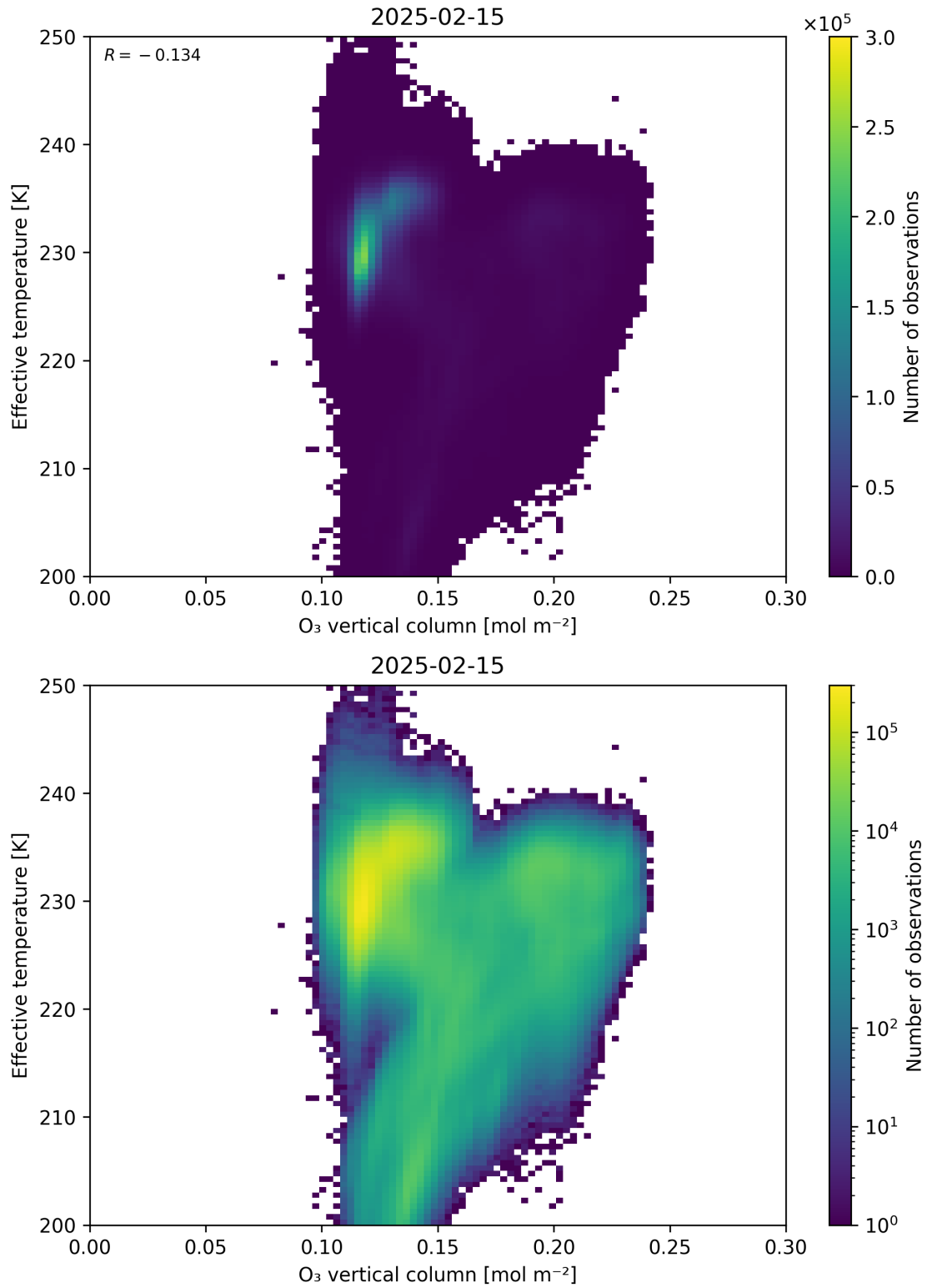
Figure 39: Scatter density plot of “O 3 vertical column” against “Effective temperature” for 2025-02-14 to 2025-02-16.
