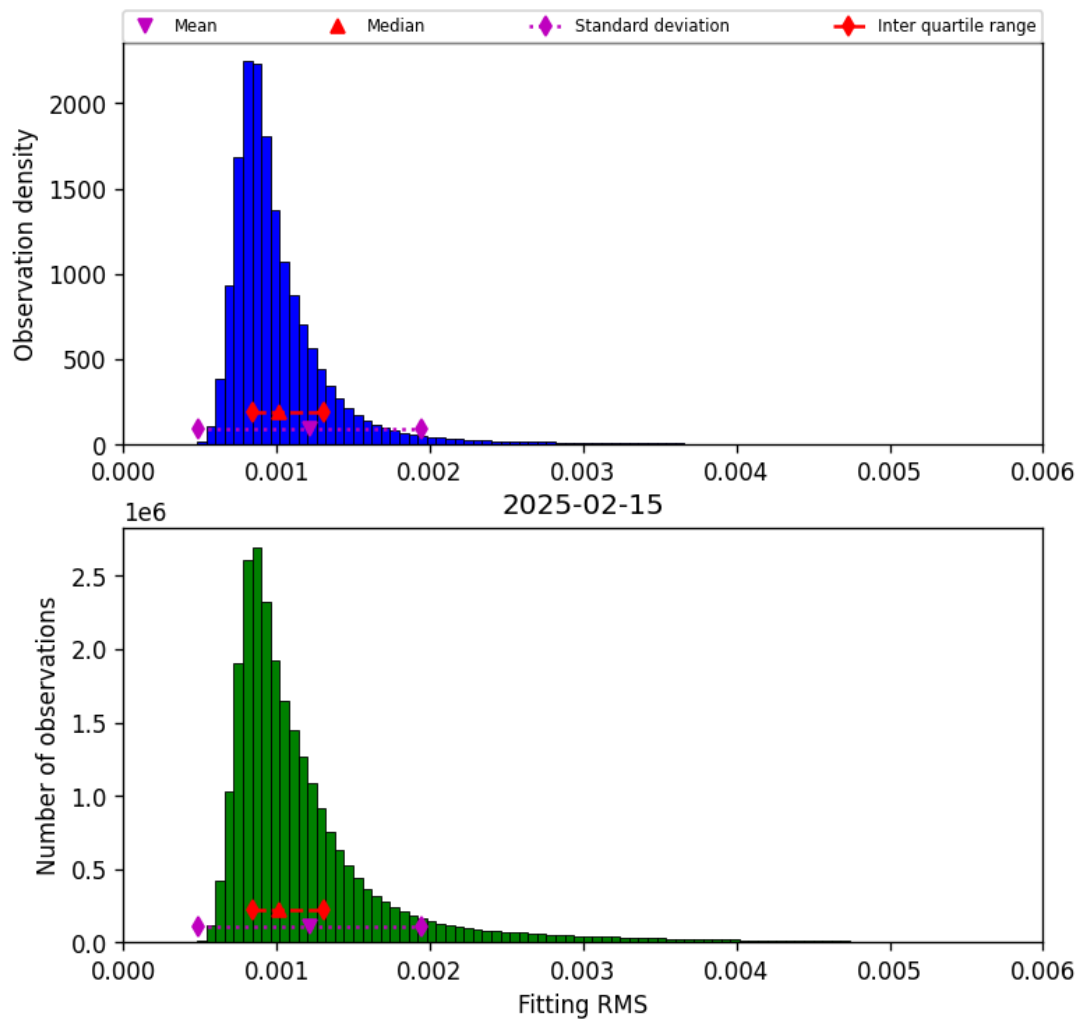
Figure 23: Histogram of “Fitting RMS” for 2025-02-14 to 2025-02-16
