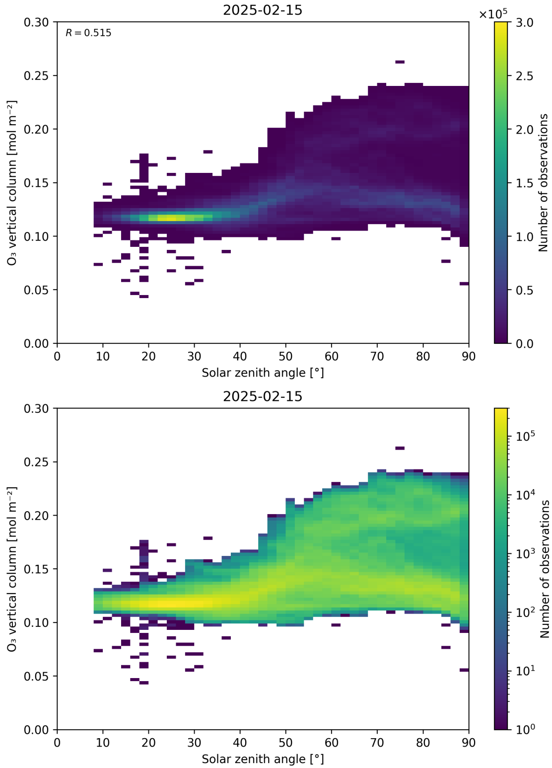
Figure 47: Scatter density plot of “Solar zenith angle” against “O 3 vertical column” for 2025-02-14 to 2025-02-16.
