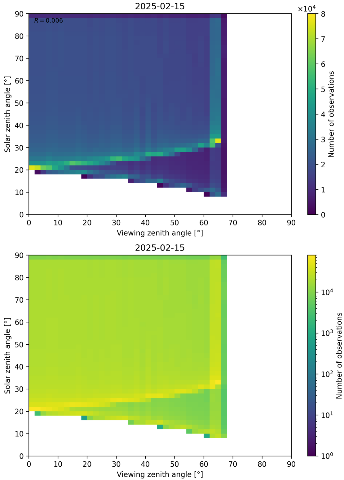
Figure 54: Scatter density plot of “Viewing zenith angle” against “Solar zenith angle” for 2025-02-14 to 2025-02-16.
