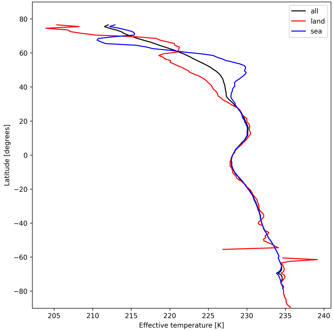
Figure 17: Zonal average of “Effective temperature” for 2025-02-14 to 2025-02-16.
