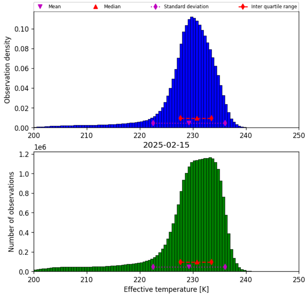
Figure 24: Histogram of “Effective temperature” for 2025-02-14 to 2025-02-16
