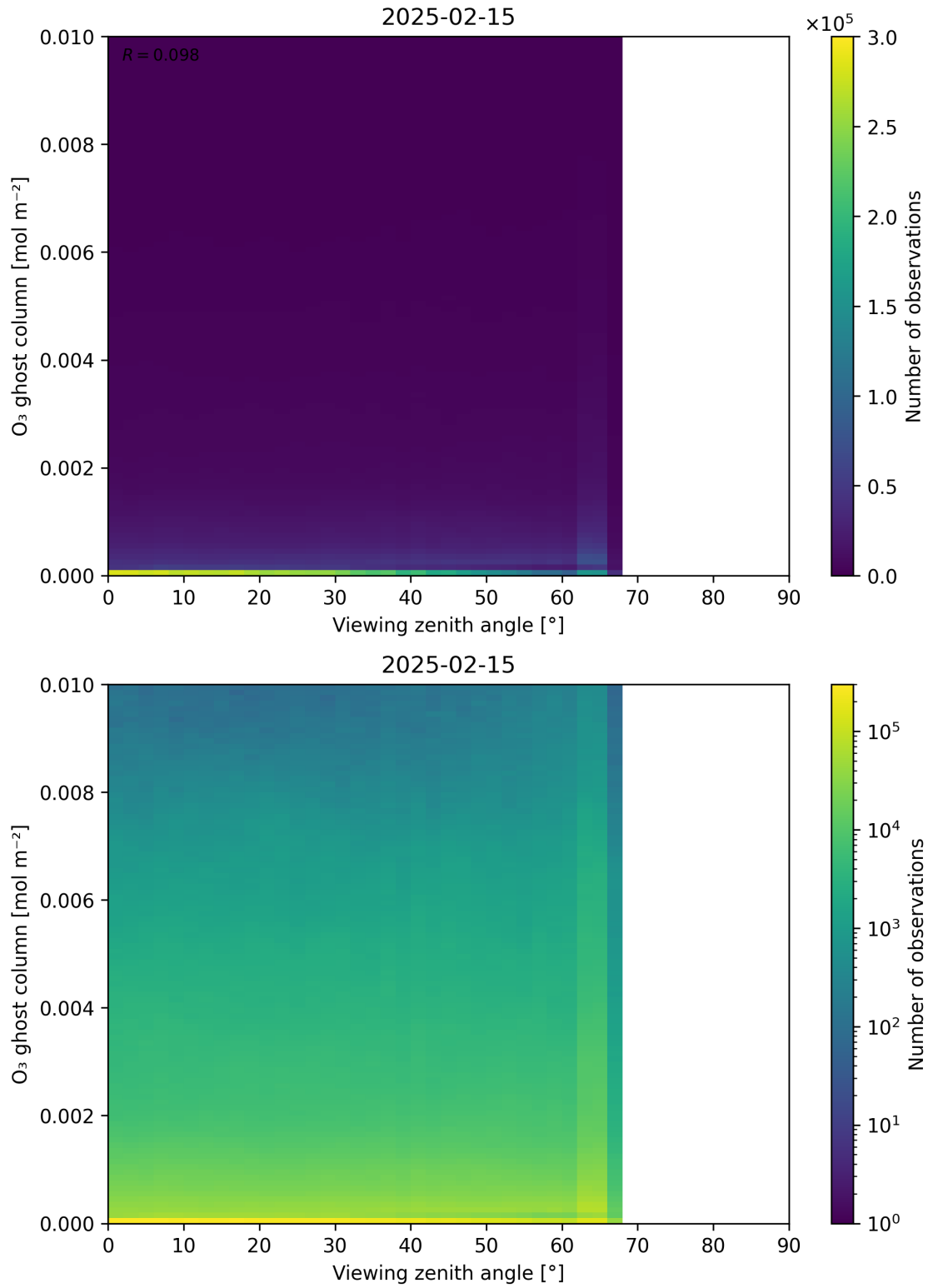
Figure 51: Scatter density plot of “Viewing zenith angle” against “O 3 ghost column” for 2025-02-14 to 2025-02-16.
