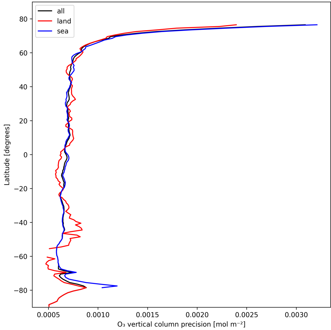
Figure 15: Zonal average of “O 3 vertical column precision” for 2025-02-14 to 2025-02-16.
