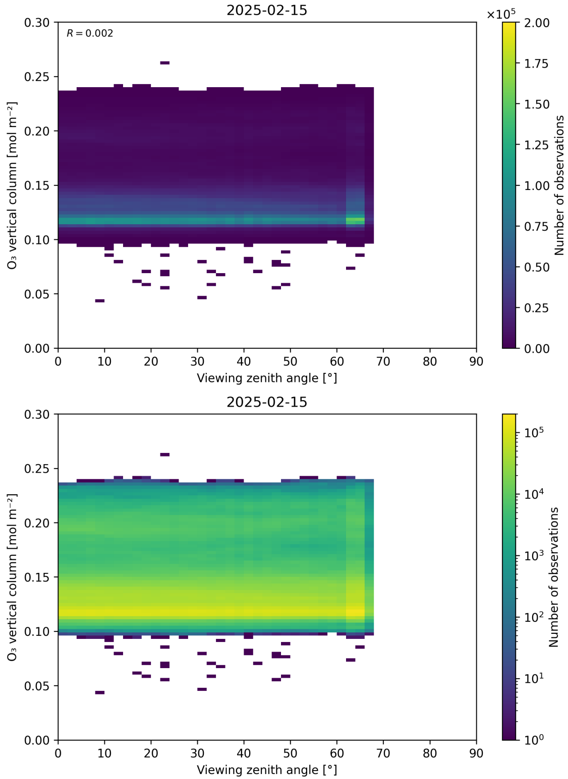
Figure 52: Scatter density plot of “Viewing zenith angle” against “O 3 vertical column” for 2025-02-14 to 2025-02-16.
