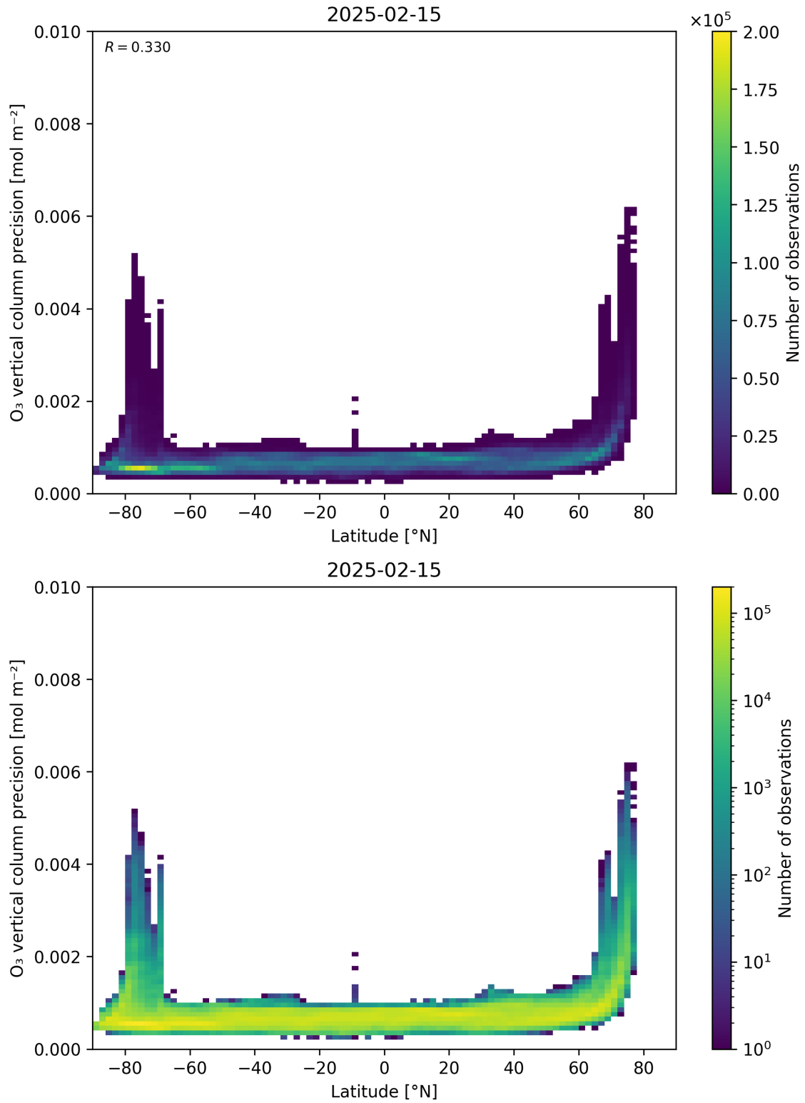
Figure 37: Scatter density plot of “Latitude” against “O 3 vertical column precision” for 2025-02-14 to 2025-02-16.
