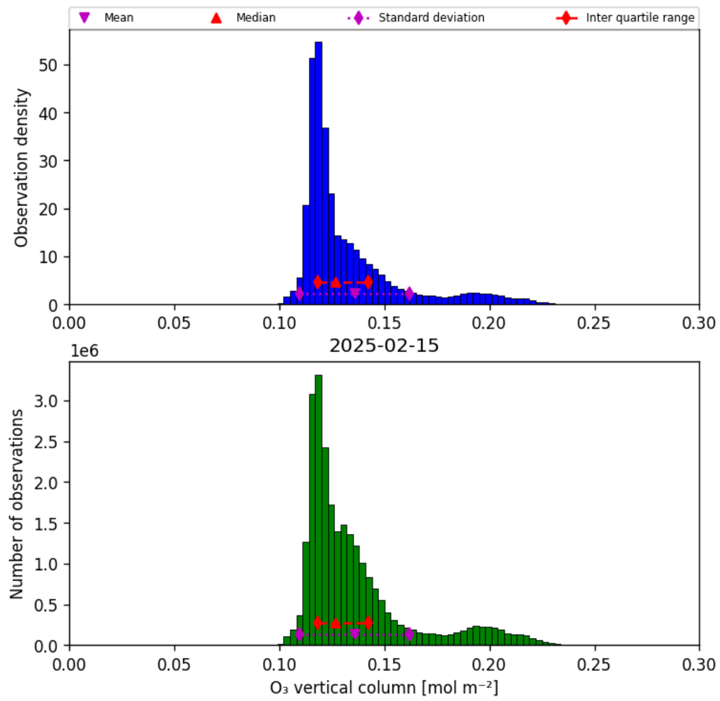
Figure 21: Histogram of “O 3 vertical column” for 2025-02-14 to 2025-02-16
