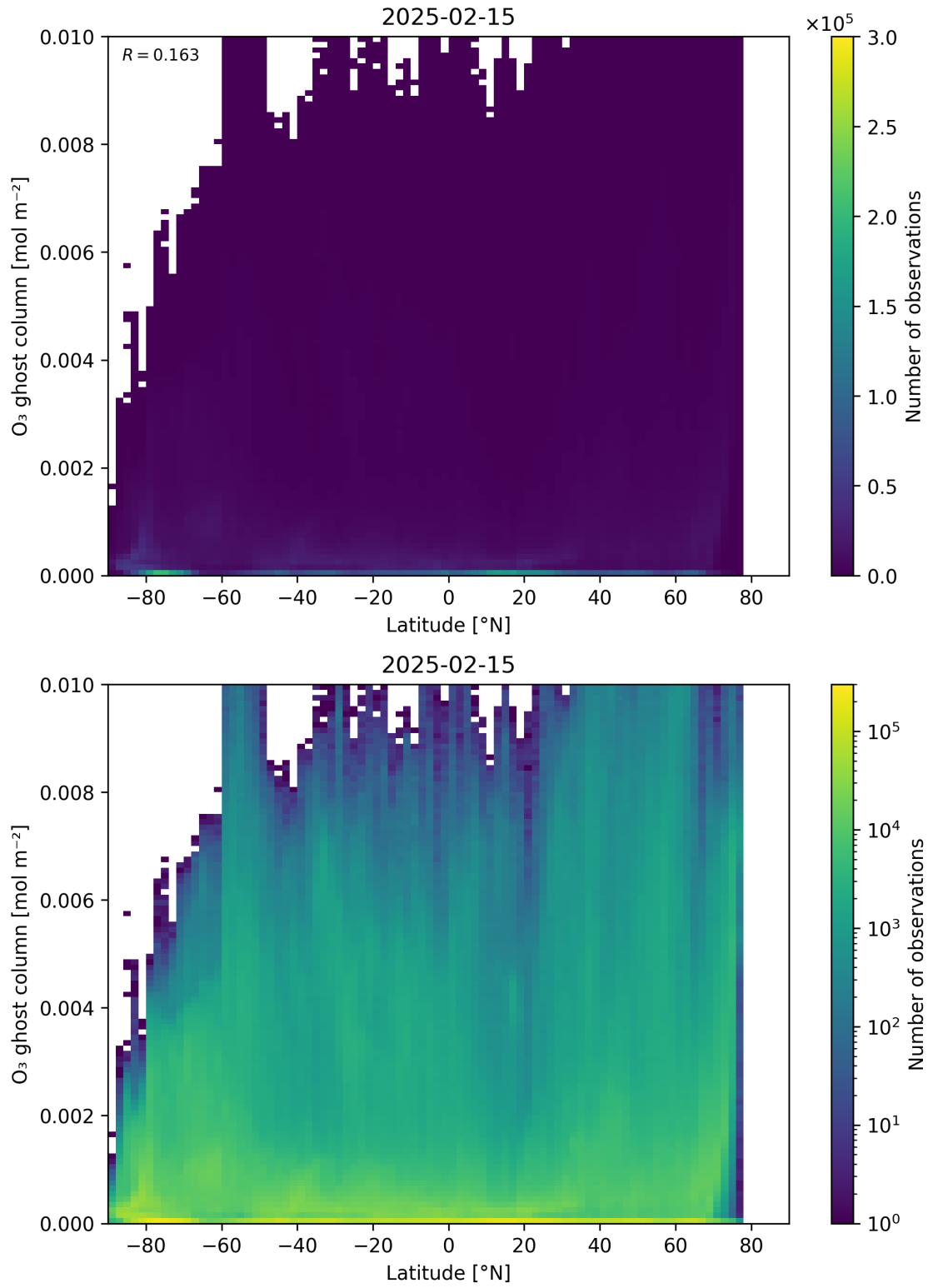
Figure 35: Scatter density plot of “Latitude” against “O 3 ghost column” for 2025-02-14 to 2025-02-16.
