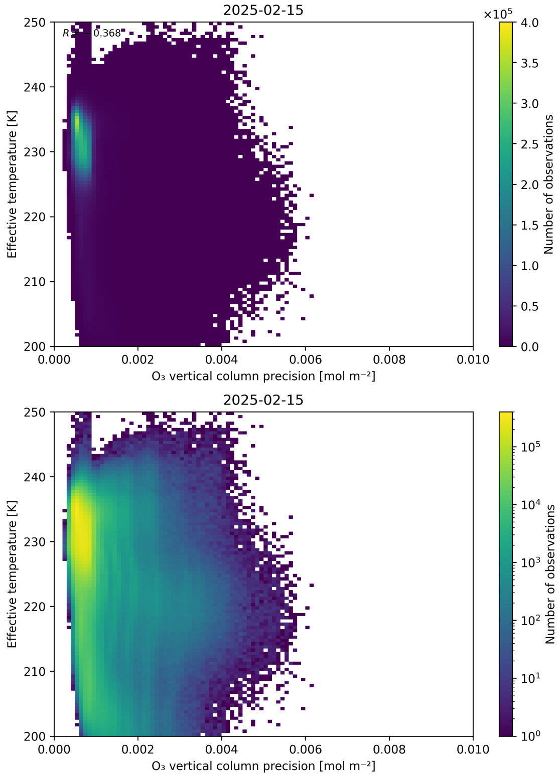
Figure 42: Scatter density plot of “O 3 vertical column precision” against “Effective temperature” for 2025-02-14 to 2025-02-16.
