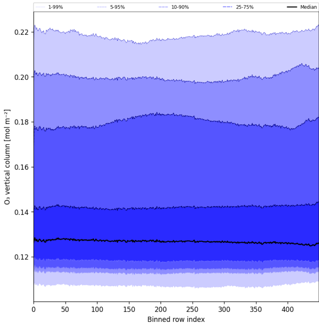
Figure 28: Along track statistics of “O 3 vertical column” for 2025-02-14 to 2025-02-16
