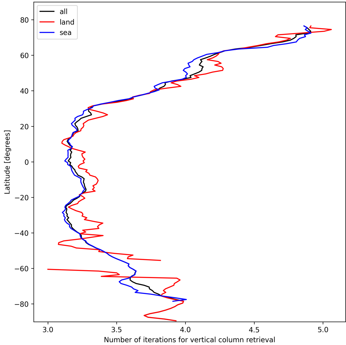
Figure 19: Zonal average of “Number of iterations for vertical column retrieval” for 2025-02-14 to 2025-02-16.
