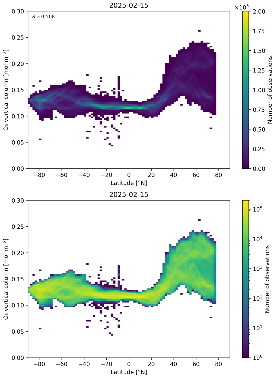
Figure 36: Scatter density plot of “Latitude” against “O 3 vertical column” for 2025-02-14 to 2025-02-16.
