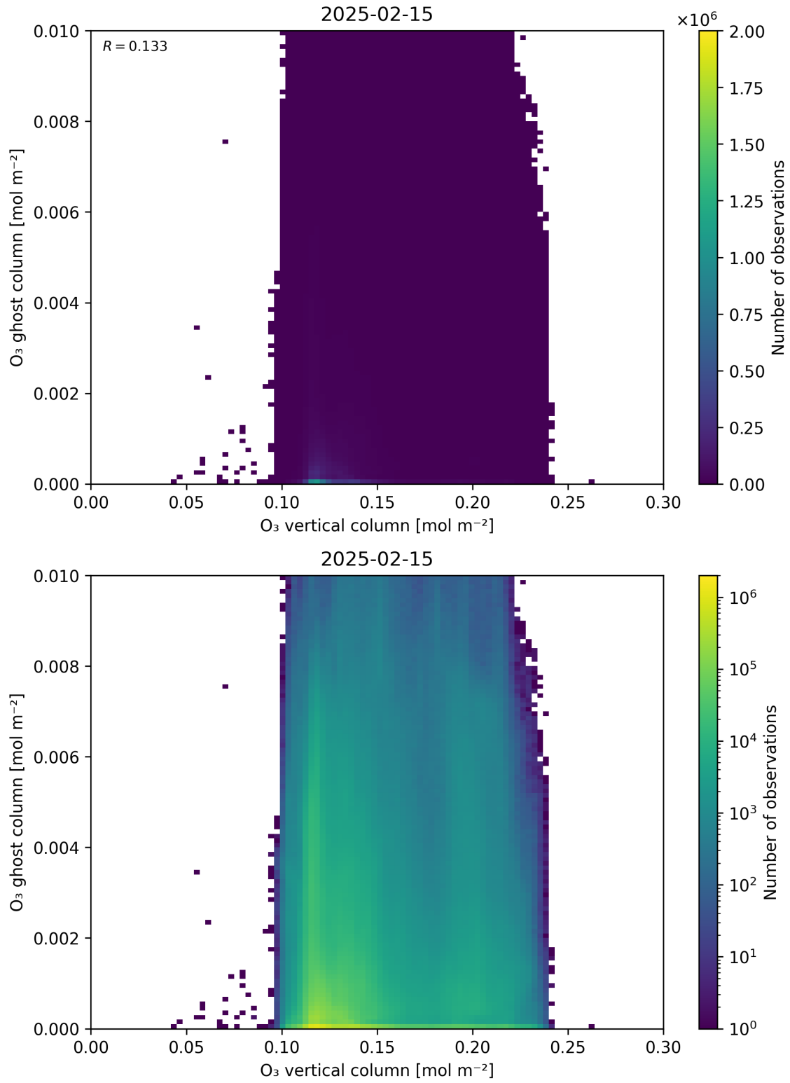
Figure 40: Scatter density plot of “O 3 vertical column” against “O 3 ghost column” for 2025-02-14 to 2025-02-16.
