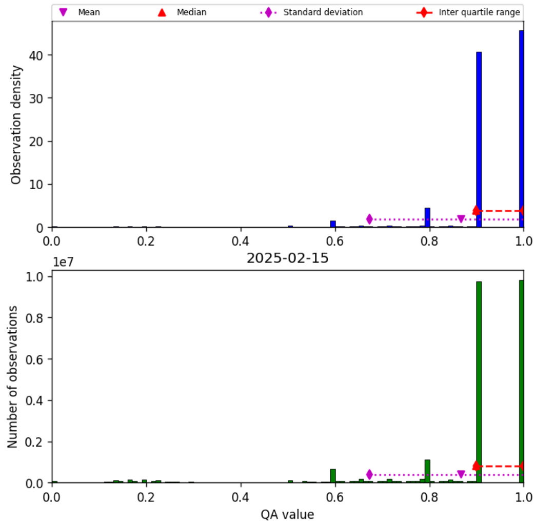
Figure 20: Histogram of “QA value” for 2025-02-14 to 2025-02-16
