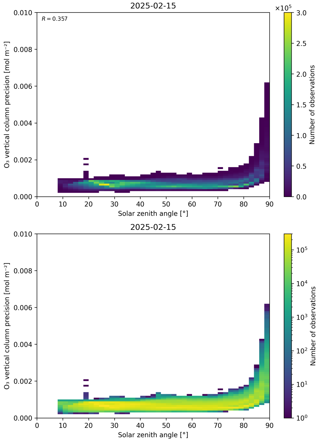
Figure 48: Scatter density plot of “Solar zenith angle” against “O 3 vertical column precision” for 2025-02-14 to 2025-02-16.
