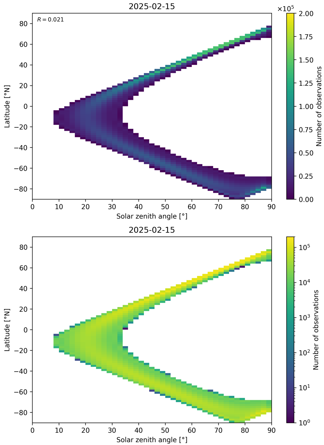
Figure 44: Scatter density plot of “Solar zenith angle” against “Latitude” for 2025-02-14 to 2025-02-16.
