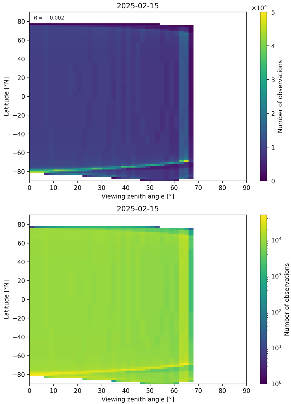
Figure 49: Scatter density plot of “Viewing zenith angle” against “Latitude” for 2025-02-14 to 2025-02-16.
