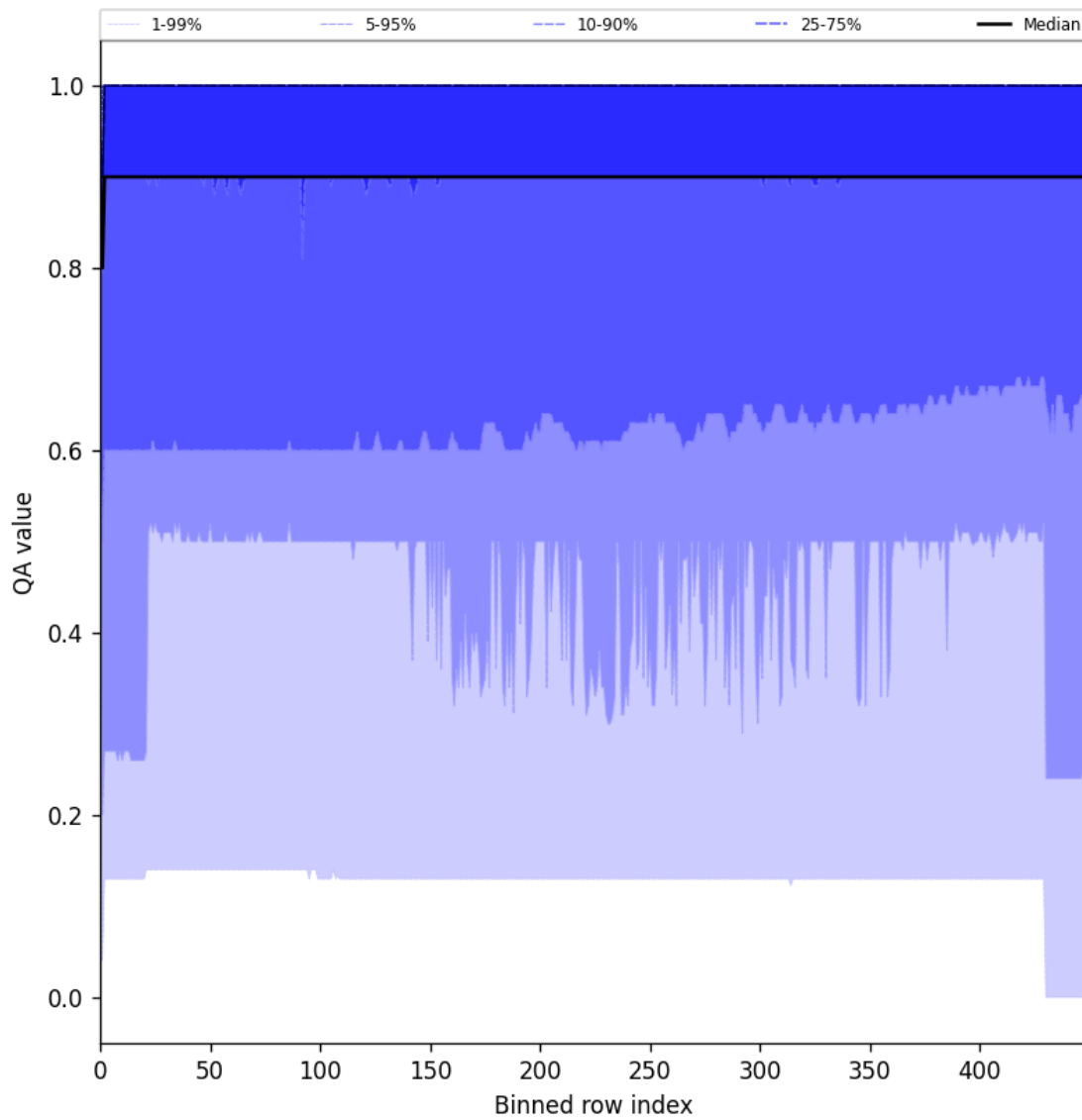
Figure 27: Along track statistics of “QA value” for 2025-02-14 to 2025-02-16
