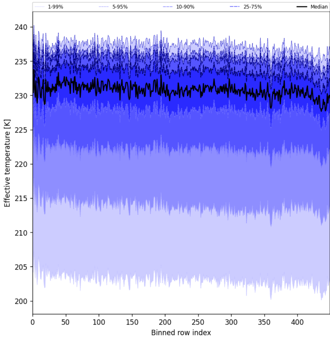
Figure 31: Along track statistics of “Effective temperature” for 2025-02-14 to 2025-02-16
