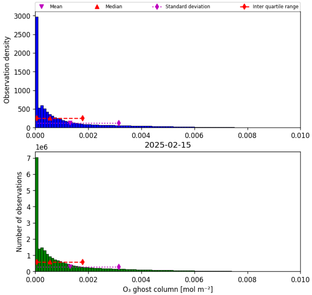
Figure 25: Histogram of “O 3 ghost column” for 2025-02-14 to 2025-02-16
