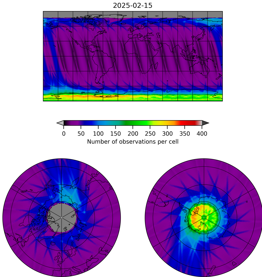
Figure 12: Map of the number of observations for 2025-02-14 to 2025-02-16
