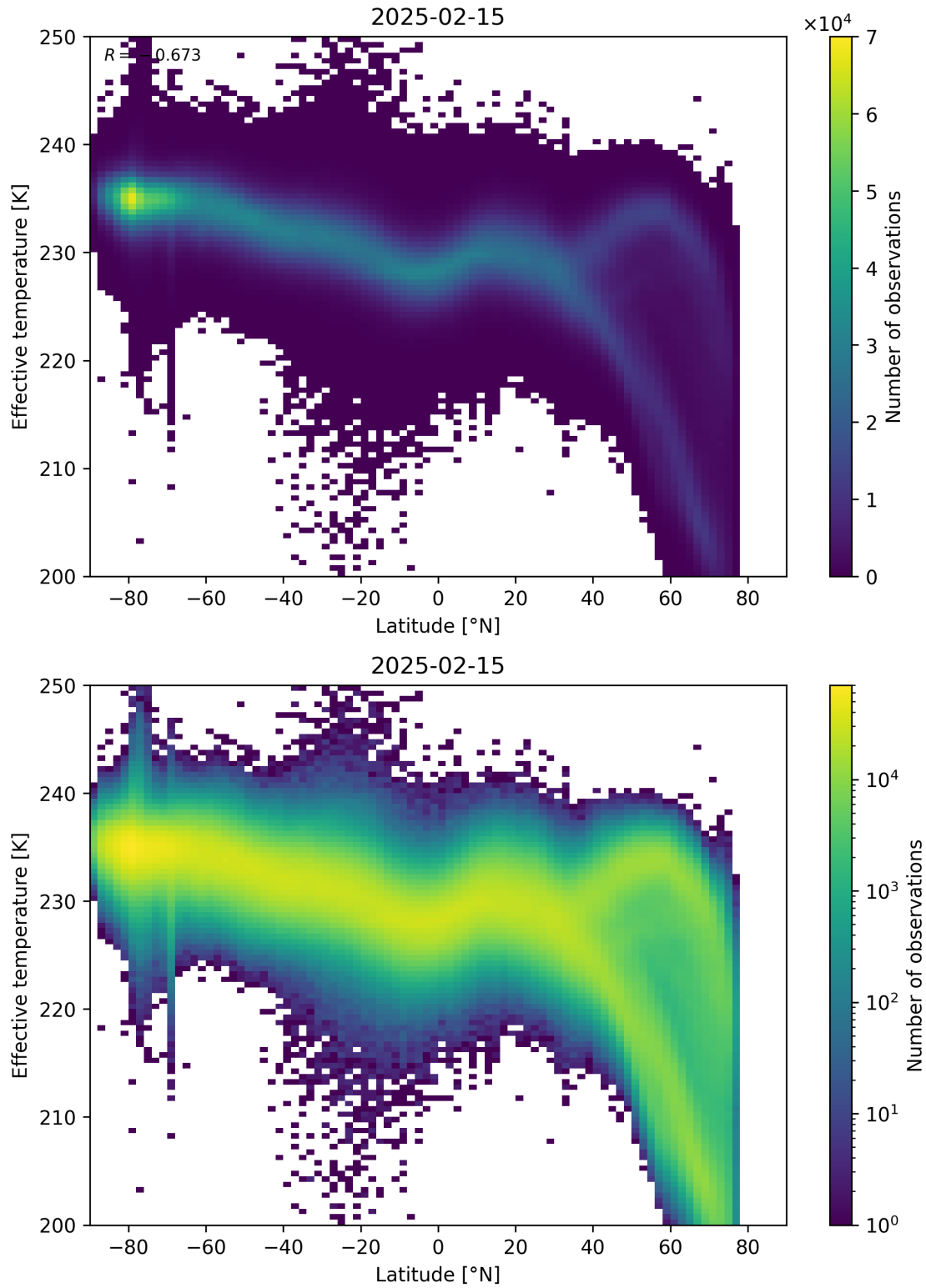
Figure 34: Scatter density plot of “Latitude” against “Effective temperature” for 2025-02-14 to 2025-02-16.
