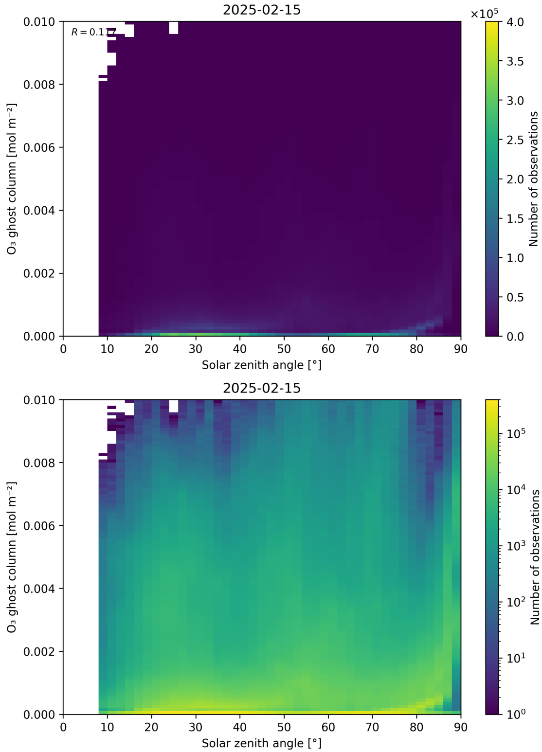
Figure 46: Scatter density plot of “Solar zenith angle” against “O 3 ghost column” for 2025-02-14 to 2025-02-16.
