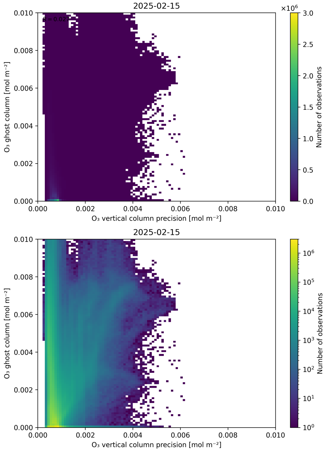
Figure 43: Scatter density plot of “O 3 vertical column precision” against “O 3 ghost column” for 2025-02-14 to 2025-02-16.
