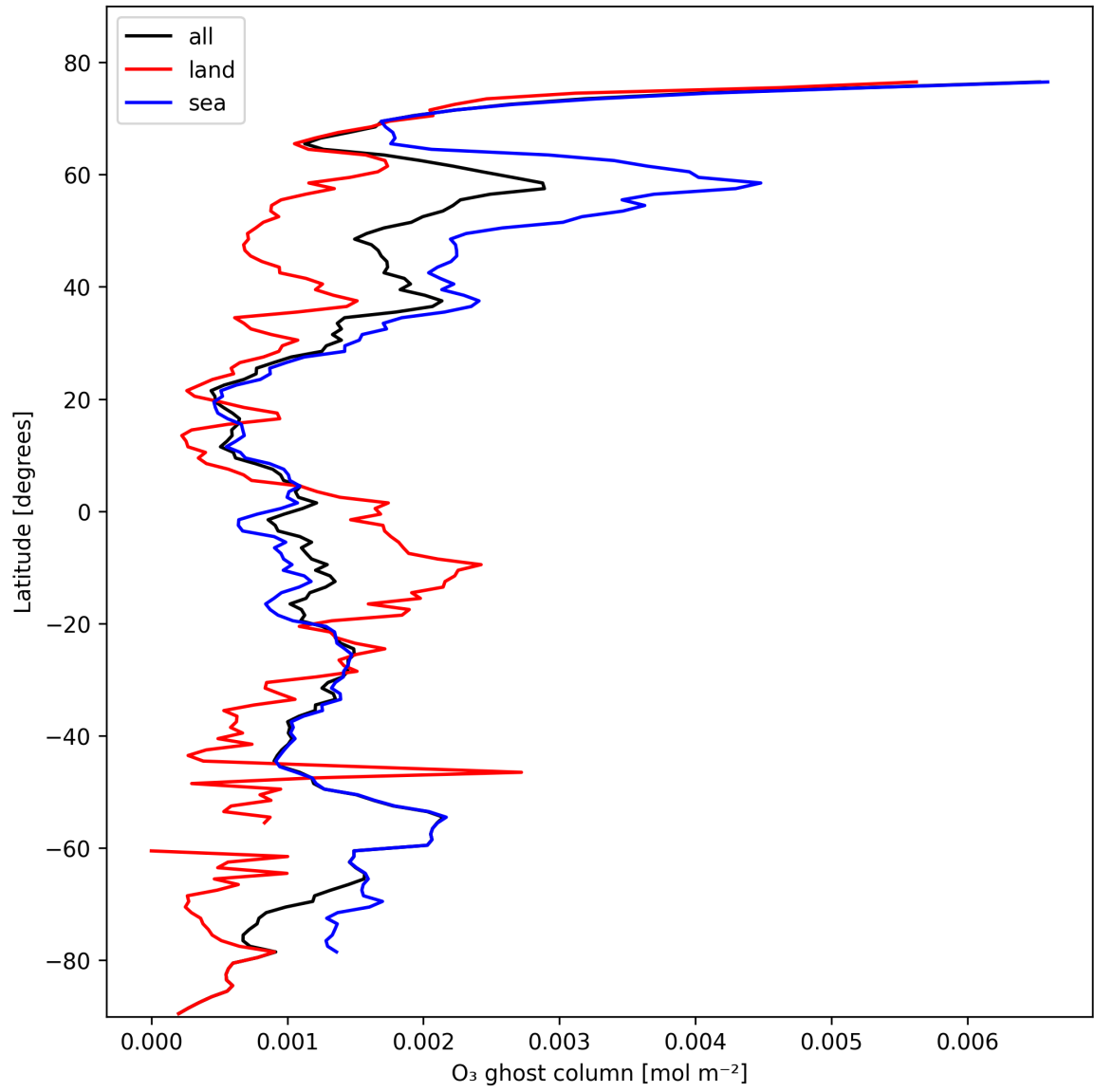
Figure 18: Zonal average of "O 3 ghost column" for 2025-02-14 to 2025-02-16.
