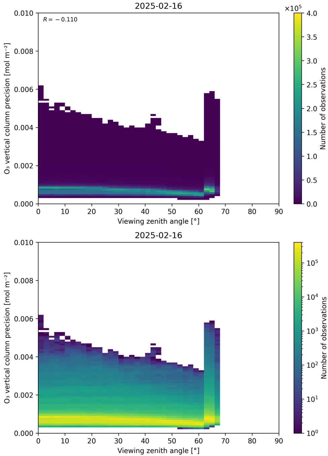
Figure 53: Scatter density plot of “Viewing zenith angle” against “O 3 vertical column precision” for 2025-02-15 to 2025-02-17.
