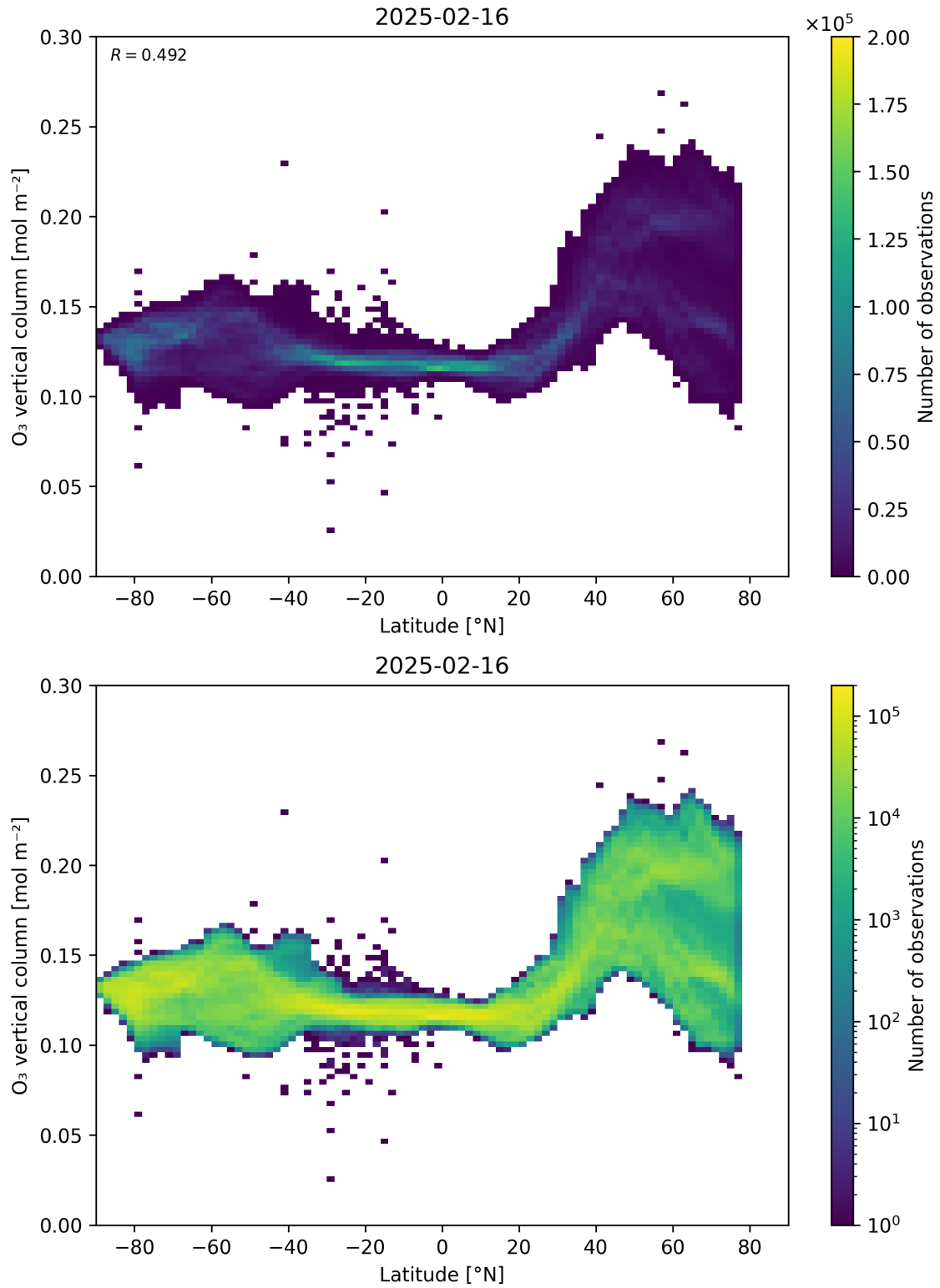
Figure 36: Scatter density plot of “Latitude” against “O 3 vertical column” for 2025-02-15 to 2025-02-17.
