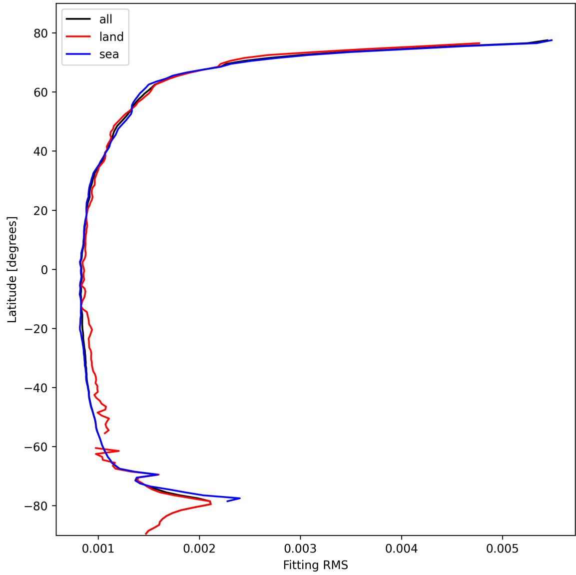
Figure 16: Zonal average of “Fitting RMS” for 2025-02-15 to 2025-02-17.
