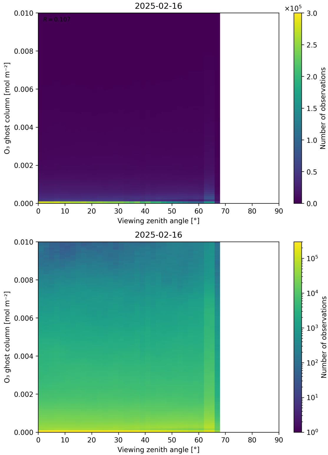
Figure 51: Scatter density plot of “Viewing zenith angle” against “O 3 ghost column” for 2025-02-15 to 2025-02-17.
