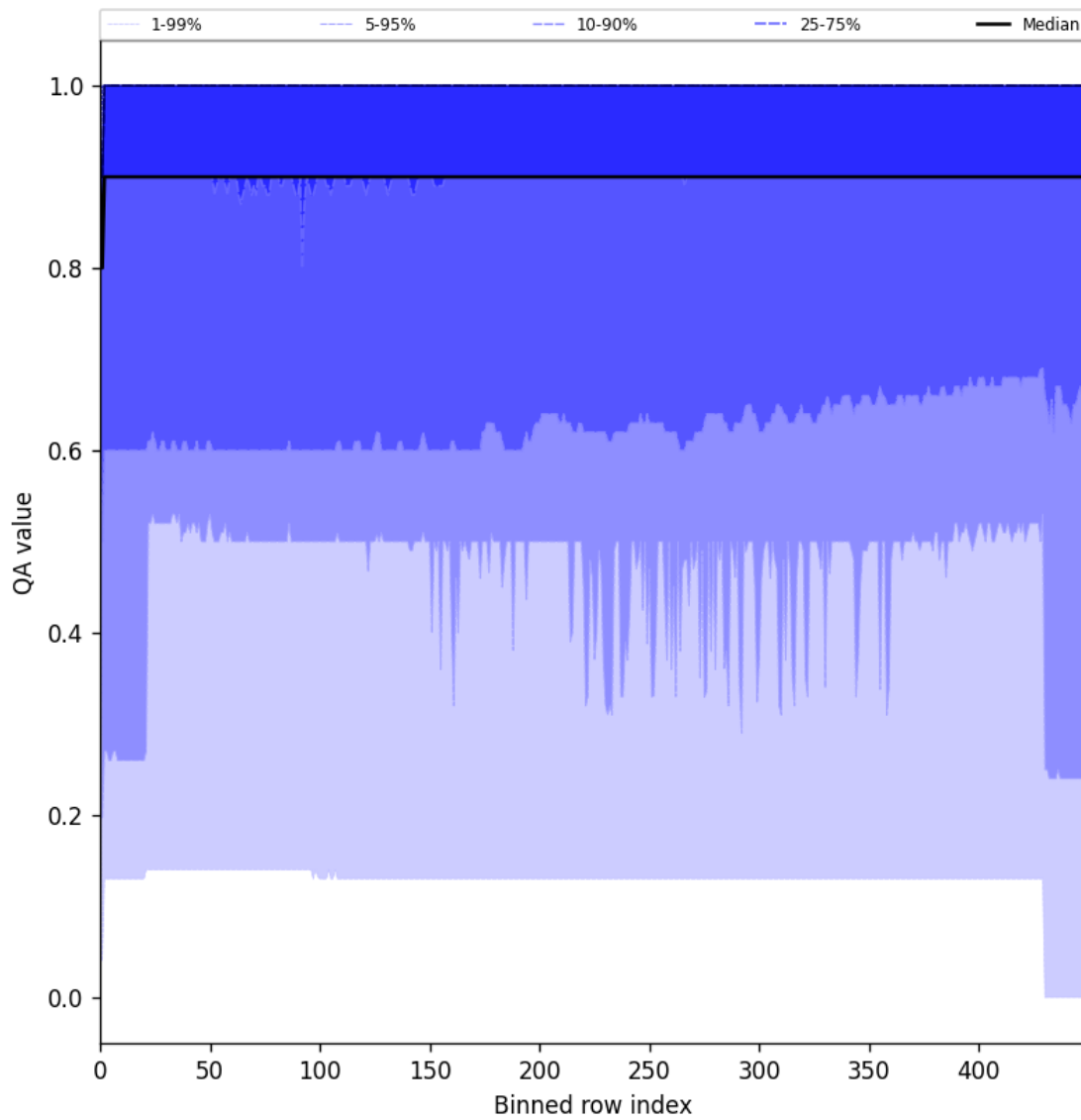
Figure 27: Along track statistics of “QA value” for 2025-02-15 to 2025-02-17
