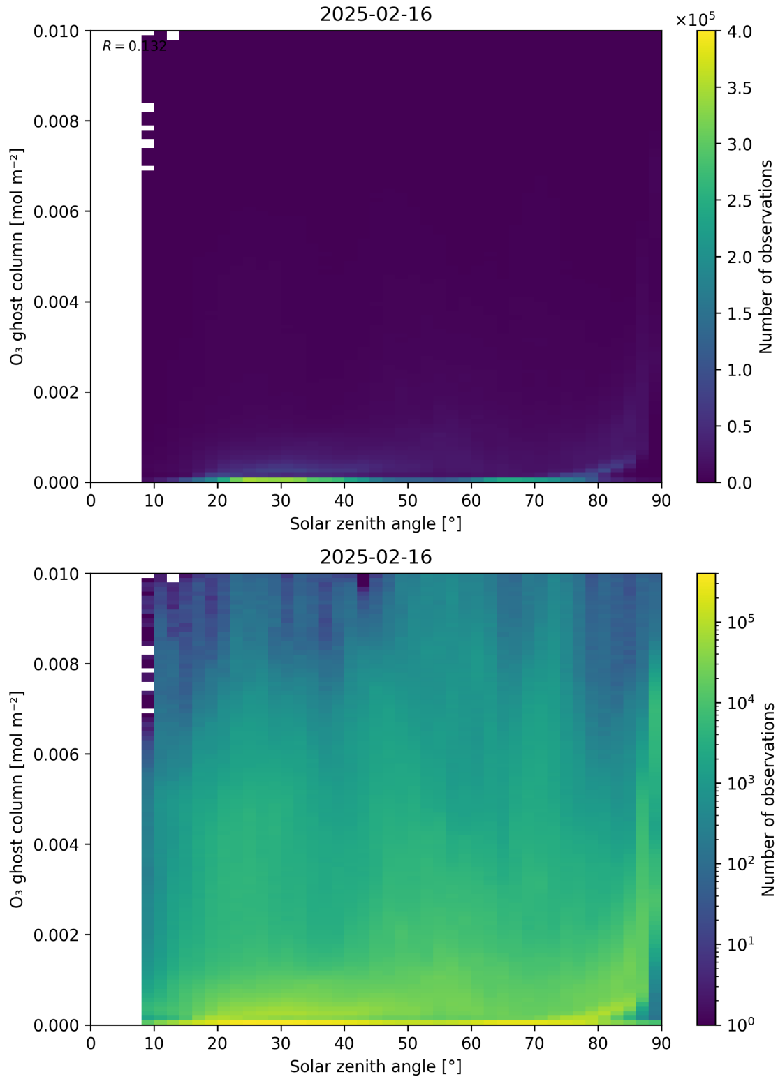
Figure 46: Scatter density plot of “Solar zenith angle” against “O 3 ghost column” for 2025-02-15 to 2025-02-17.
