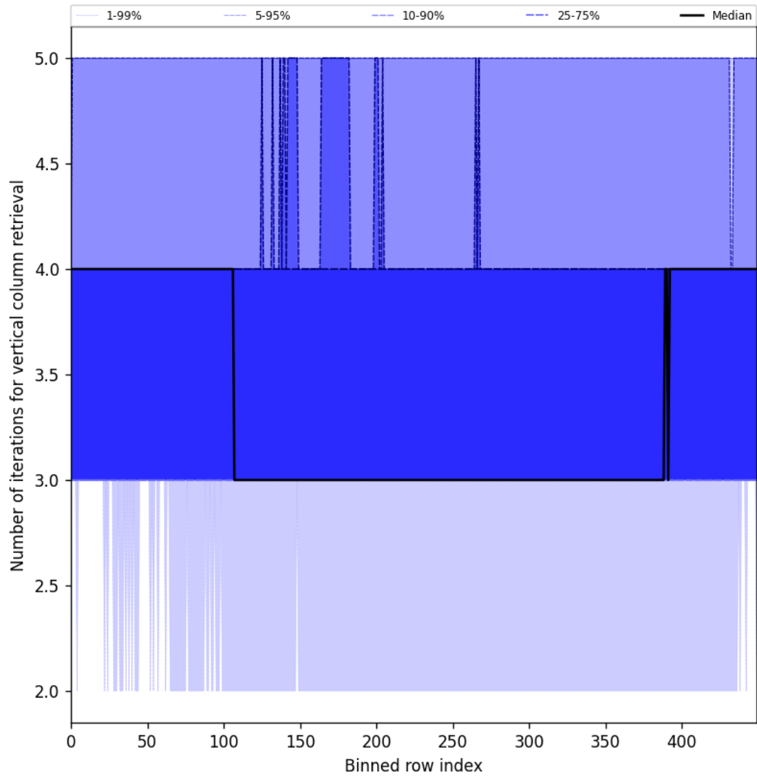
Figure 33: Along track statistics of “Number of iterations for vertical column retrieval” for 2025-02-15 to 2025-02-17
