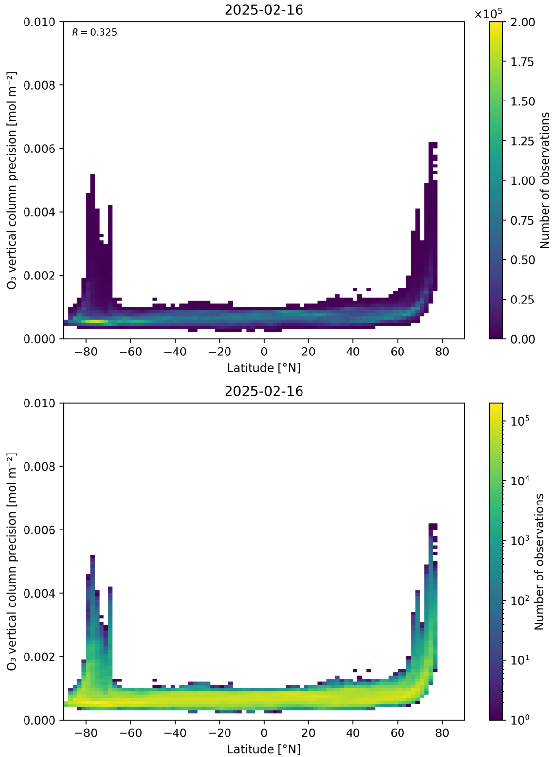
Figure 37: Scatter density plot of “Latitude” against “O 3 vertical column precision” for 2025-02-15 to 2025-02-17.
