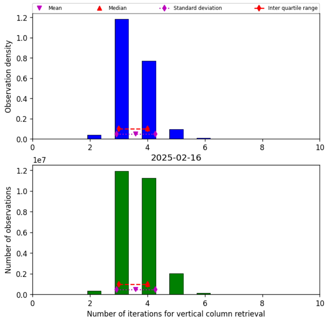
Figure 26: Histogram of “Number of iterations for vertical column retrieval” for 2025-02-15 to 2025-02-17
