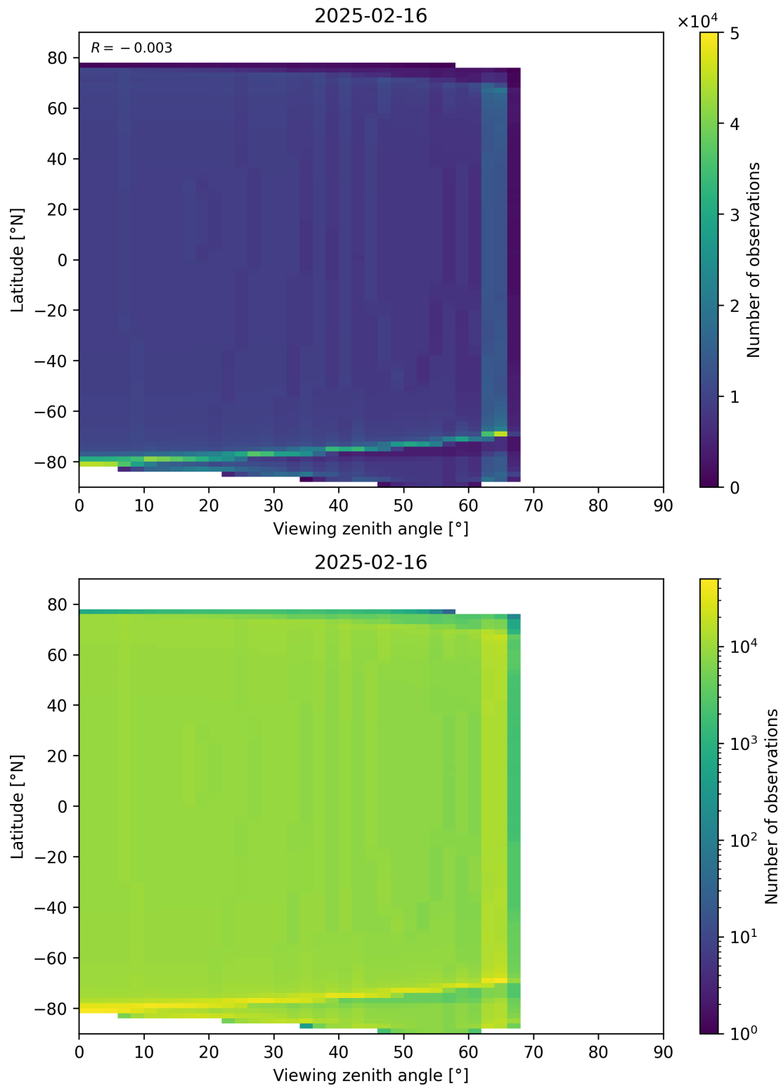
Figure 49: Scatter density plot of “Viewing zenith angle” against “Latitude” for 2025-02-15 to 2025-02-17.
