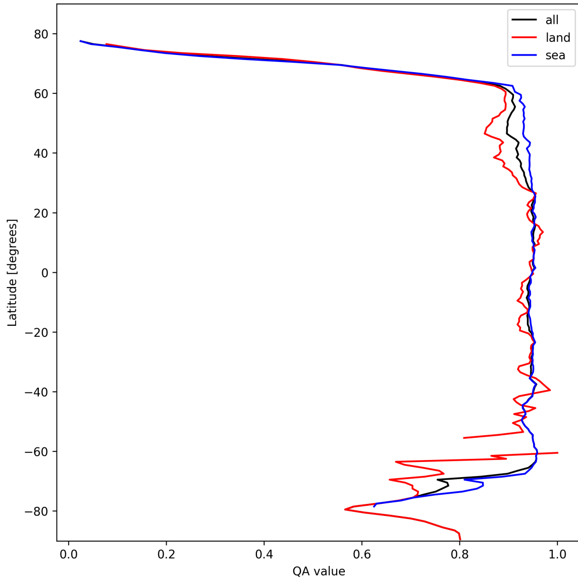
Figure 13: Zonal average of “QA value” for 2025-02-15 to 2025-02-17.
