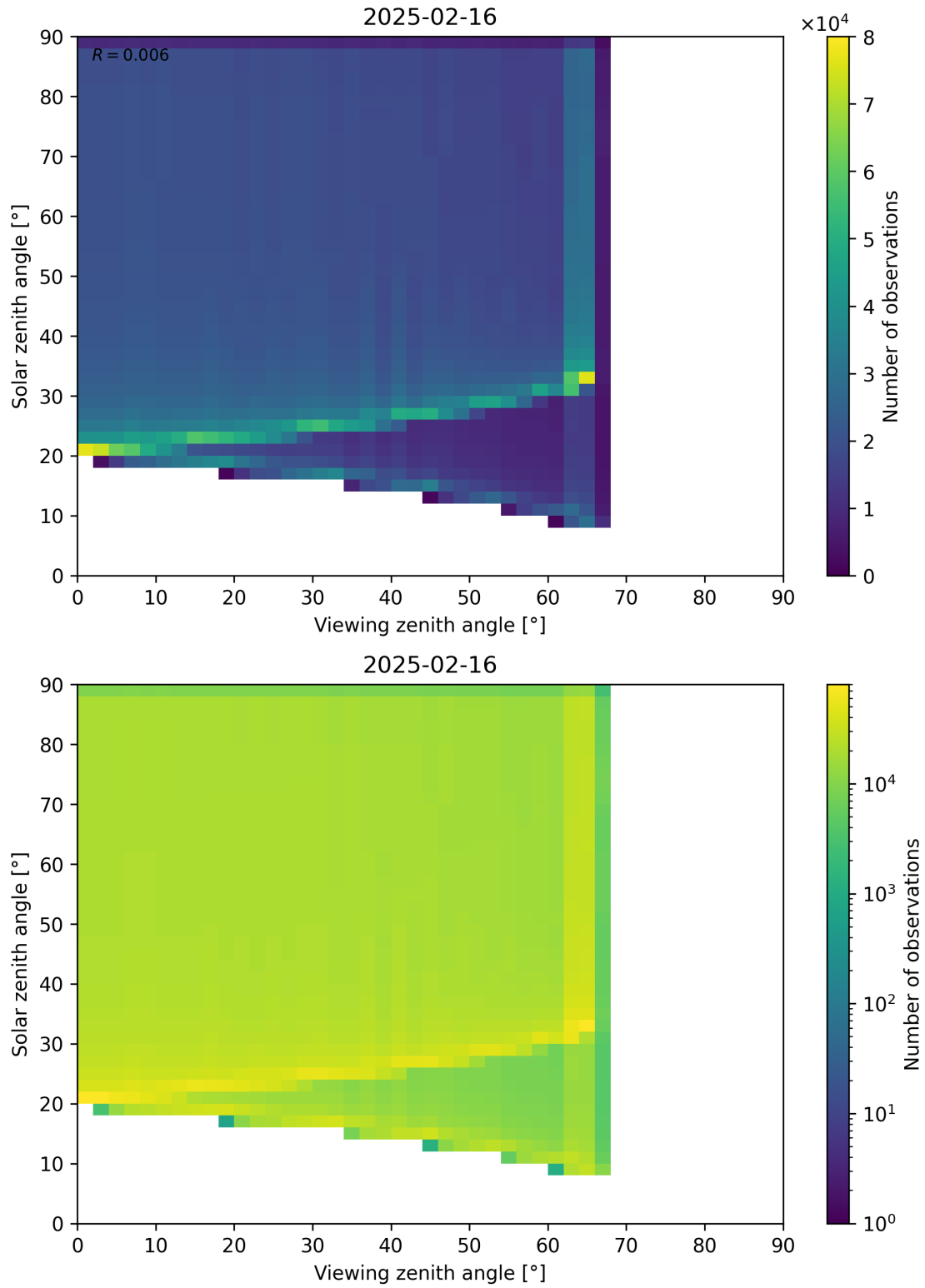
Figure 54: Scatter density plot of “Viewing zenith angle” against “Solar zenith angle” for 2025-02-15 to 2025-02-17.
