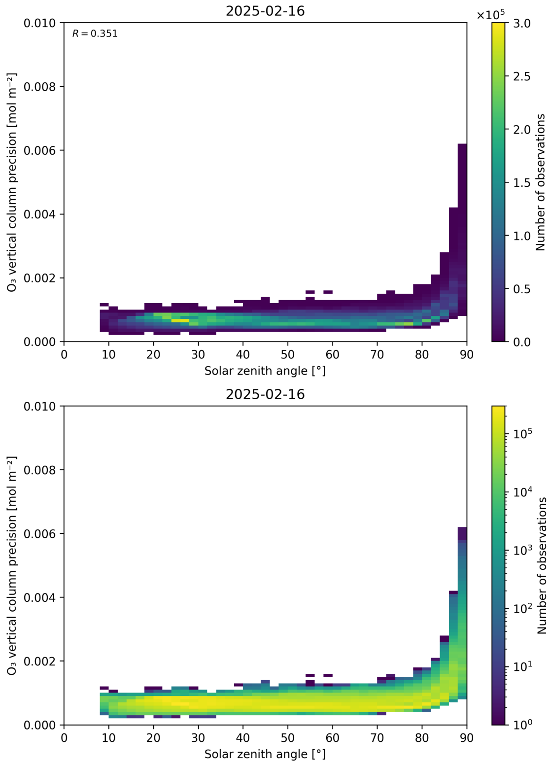
Figure 48: Scatter density plot of “Solar zenith angle” against “O 3 vertical column precision” for 2025-02-15 to 2025-02-17.
