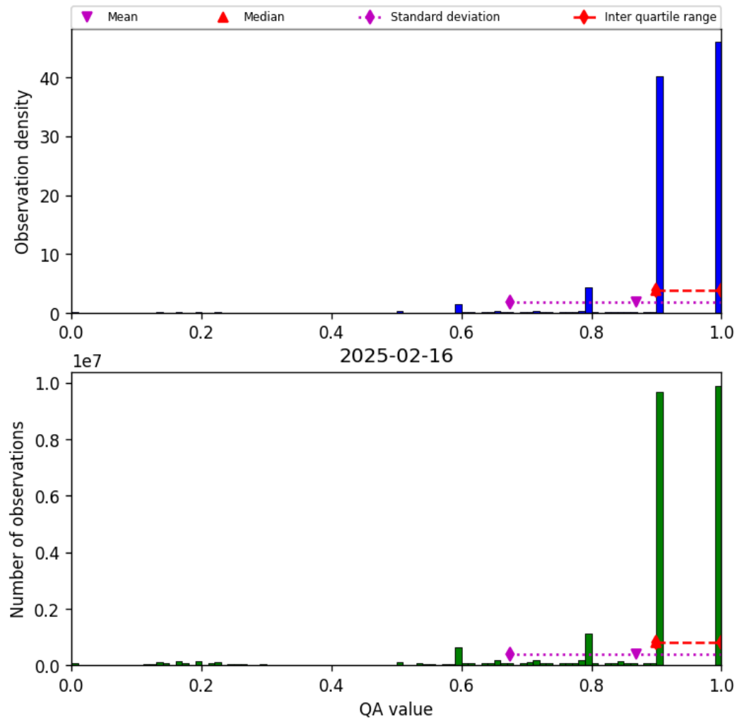
Figure 20: Histogram of “QA value” for 2025-02-15 to 2025-02-17
