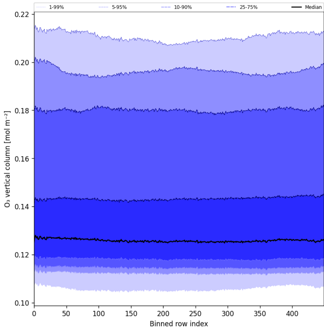
Figure 28: Along track statistics of “O 3 vertical column” for 2025-02-16 to 2025-02-18
