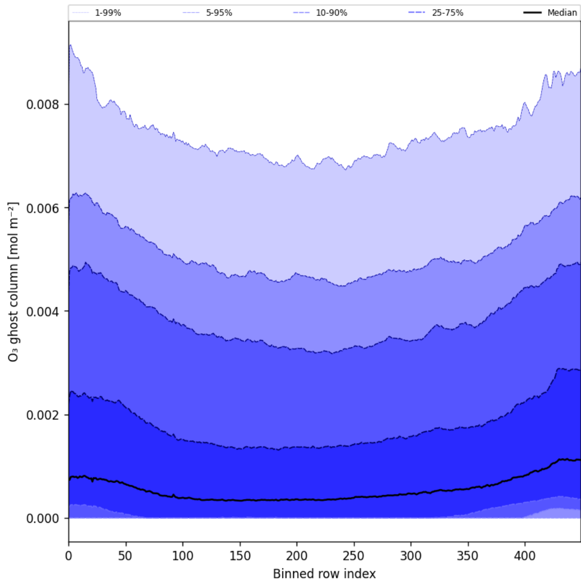
Figure 32: Along track statistics of “O 3 ghost column” for 2025-02-16 to 2025-02-18
