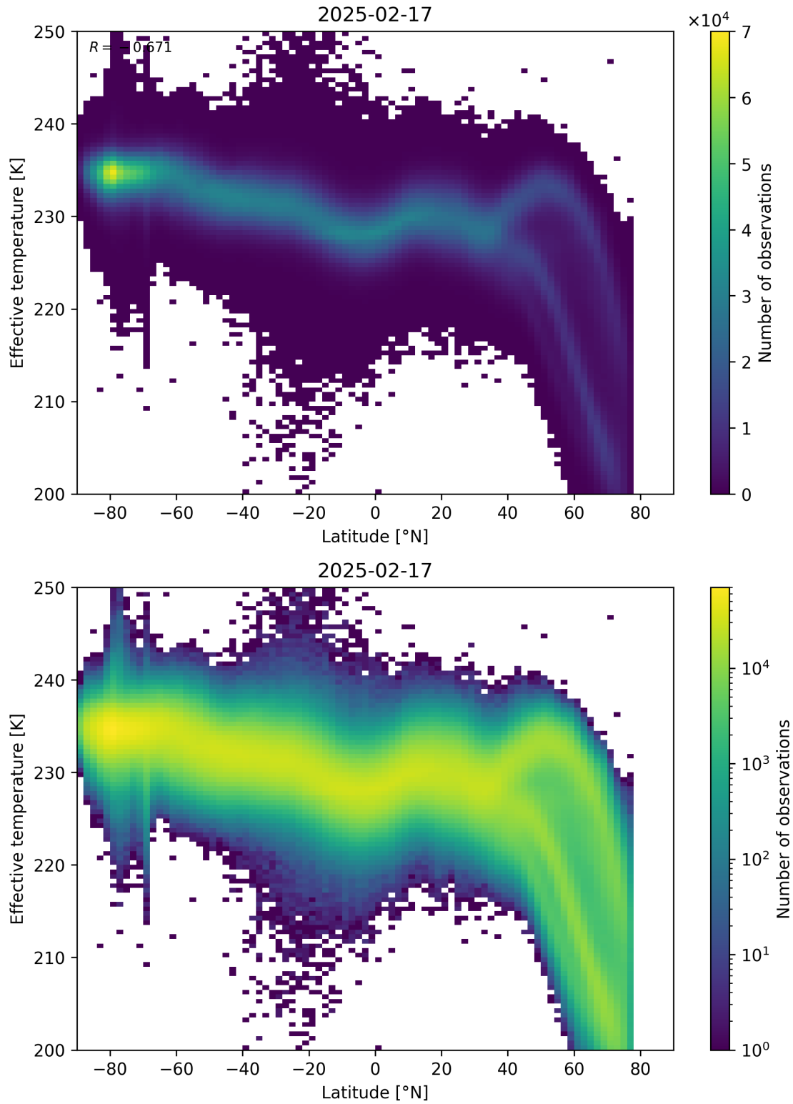
Figure 34: Scatter density plot of “Latitude” against “Effective temperature” for 2025-02-16 to 2025-02-18.
