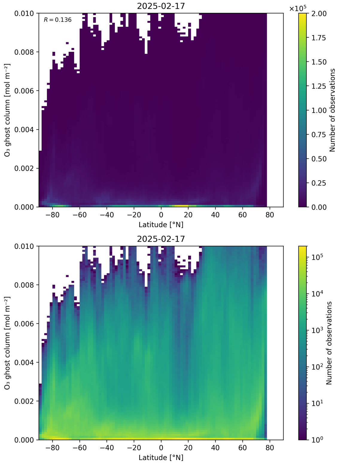
Figure 35: Scatter density plot of “Latitude” against “O 3 ghost column” for 2025-02-16 to 2025-02-18.
