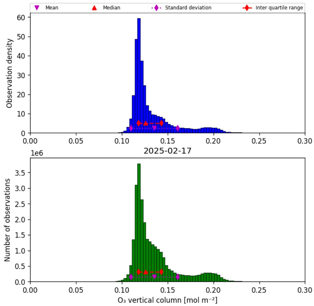
Figure 21: Histogram of “O 3 vertical column” for 2025-02-16 to 2025-02-18
