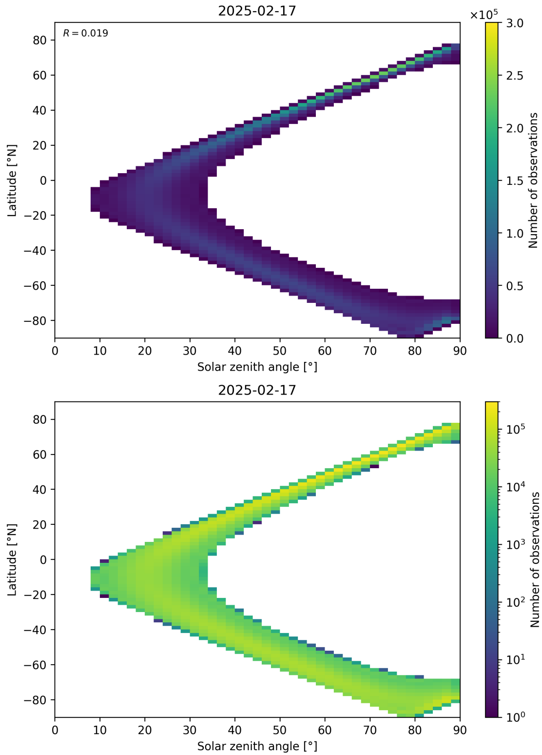
Figure 44: Scatter density plot of “Solar zenith angle” against “Latitude” for 2025-02-16 to 2025-02-18.
