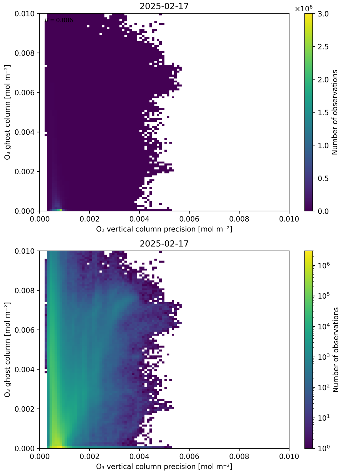
Figure 43: Scatter density plot of “O 3 vertical column precision” against “O 3 ghost column” for 2025-02-16 to 2025-02-18.
