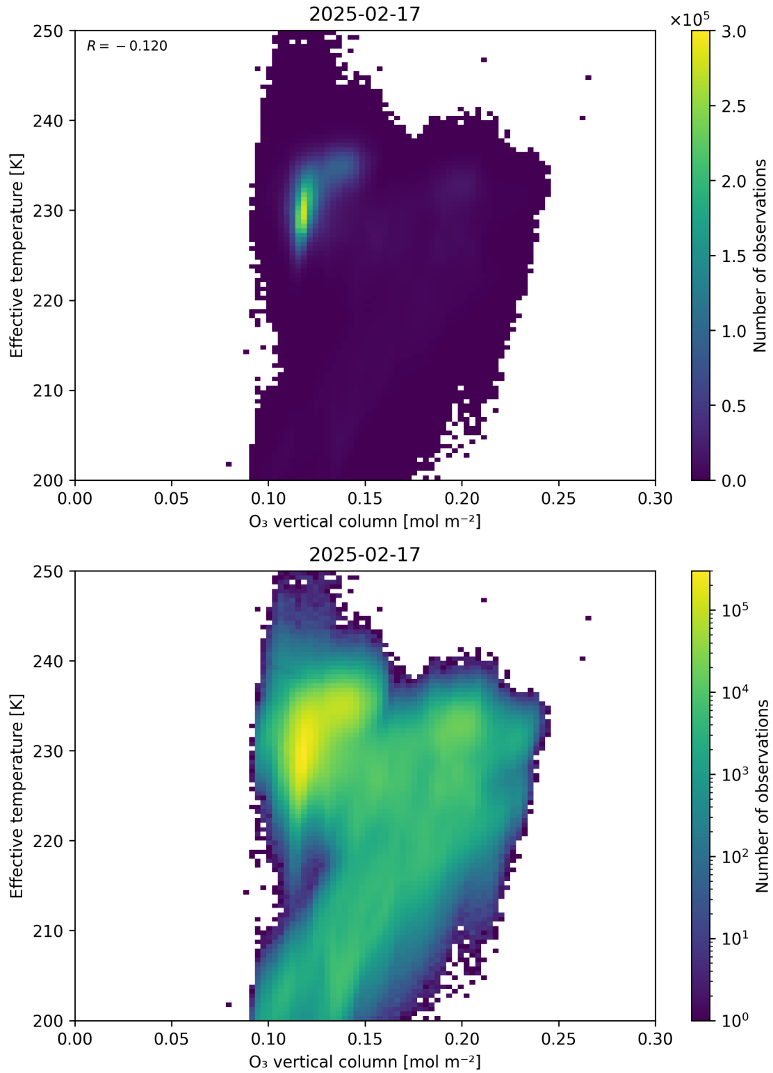
Figure 39: Scatter density plot of “O 3 vertical column” against “Effective temperature” for 2025-02-16 to 2025-02-18.
