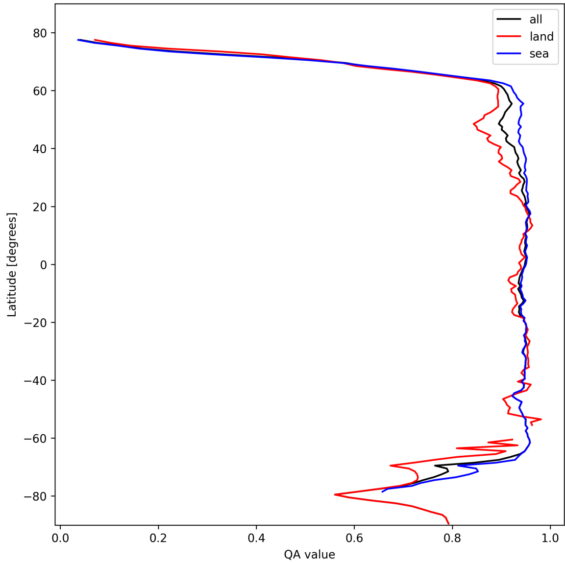
Figure 13: Zonal average of “QA value” for 2025-02-16 to 2025-02-18.
