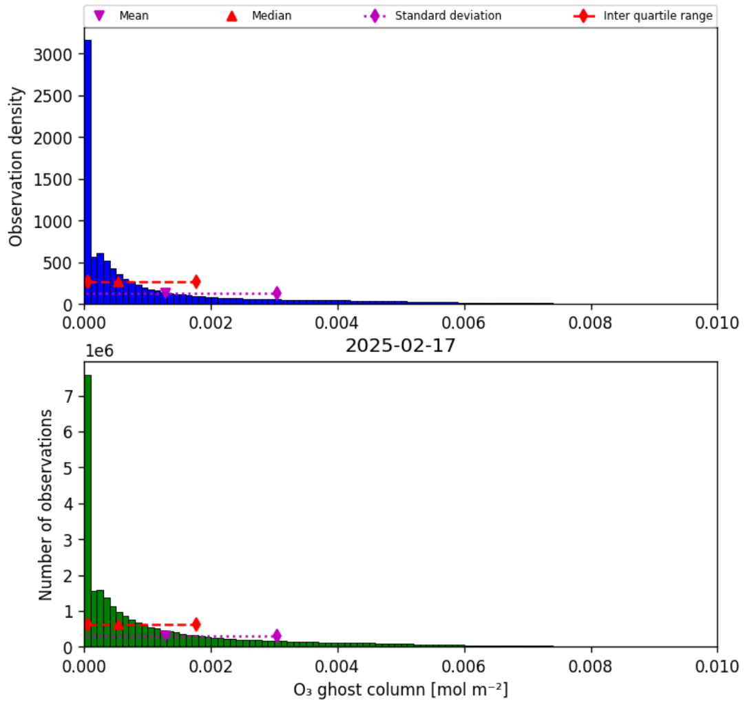
Figure 25: Histogram of “O 3 ghost column” for 2025-02-16 to 2025-02-18
