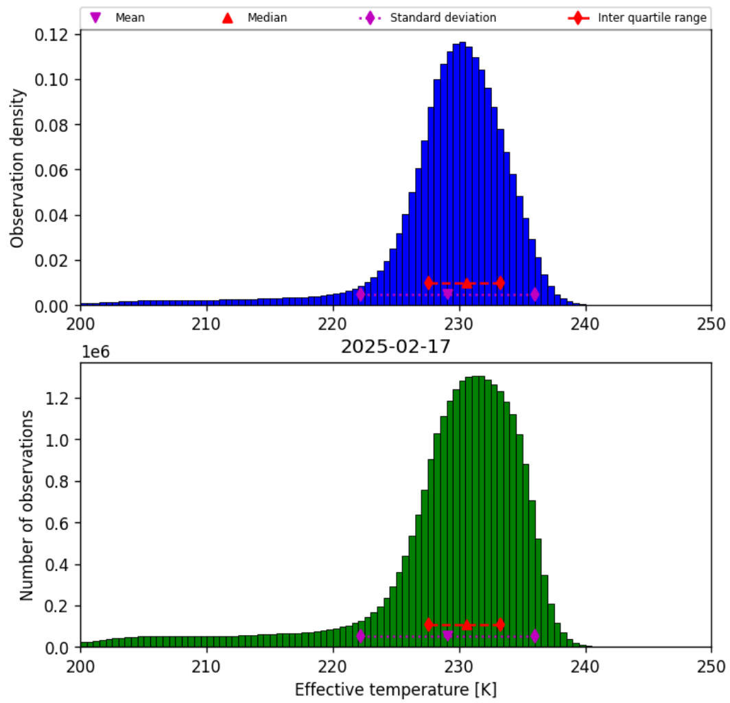
Figure 24: Histogram of “Effective temperature” for 2025-02-16 to 2025-02-18
