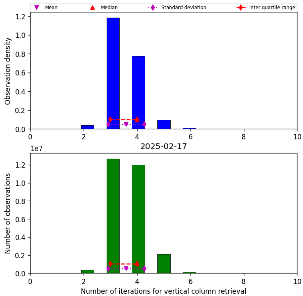
Figure 26: Histogram of “Number of iterations for vertical column retrieval” for 2025-02-16 to 2025-02-18
