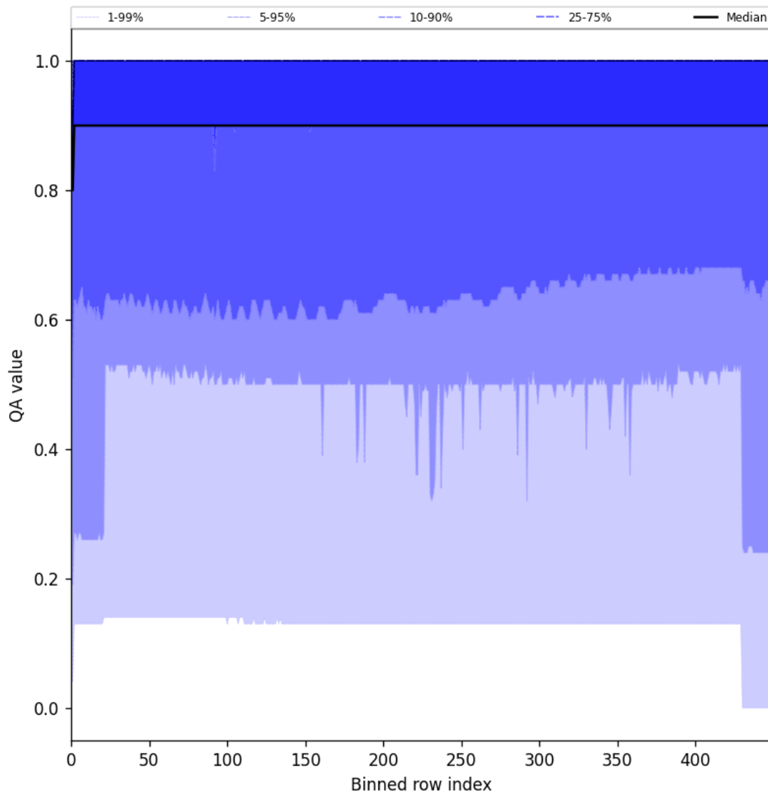
Figure 27: Along track statistics of “QA value” for 2025-02-16 to 2025-02-18
