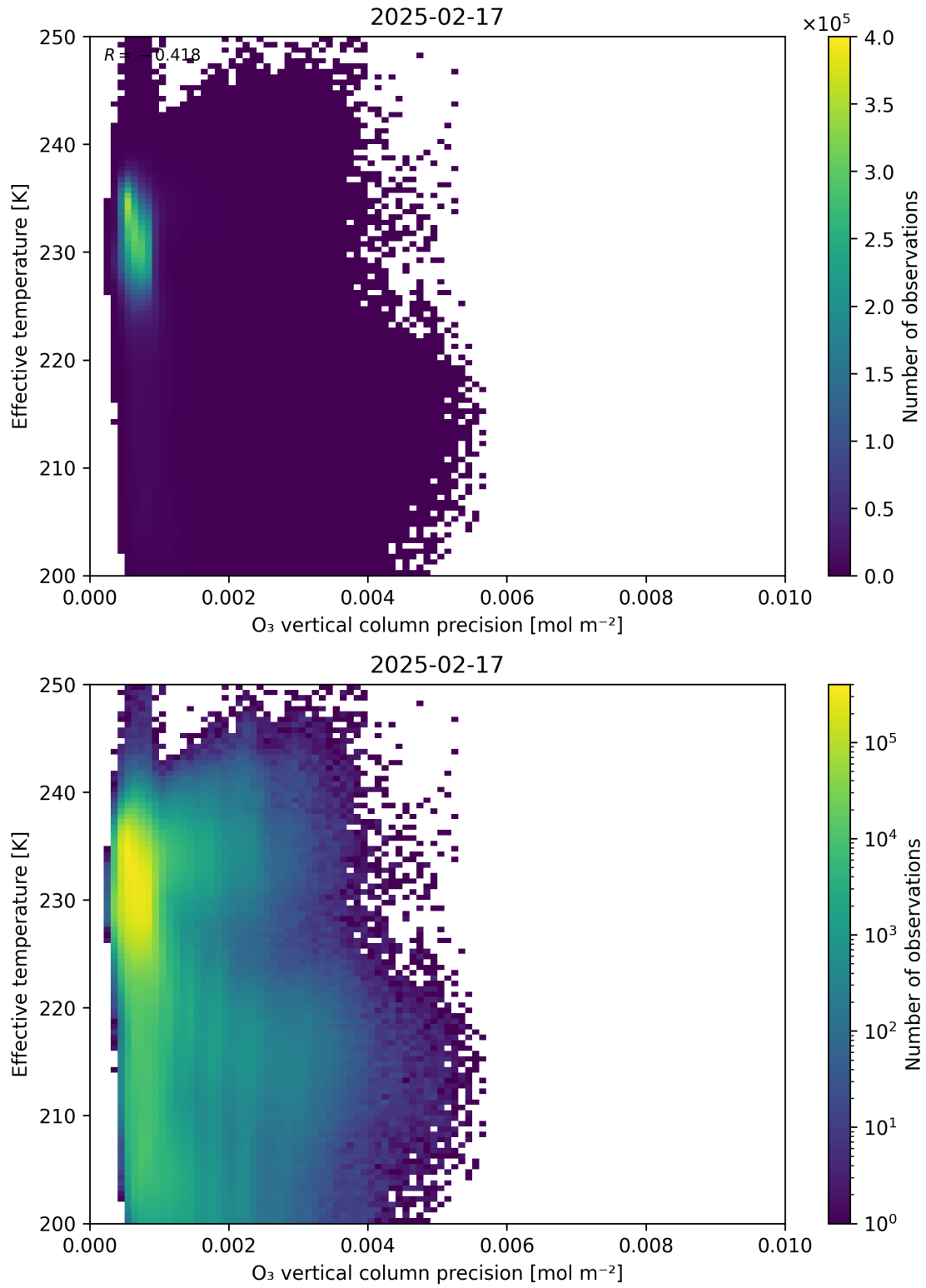
Figure 42: Scatter density plot of “O 3 vertical column precision” against “Effective temperature” for 2025-02-16 to 2025-02-18.
