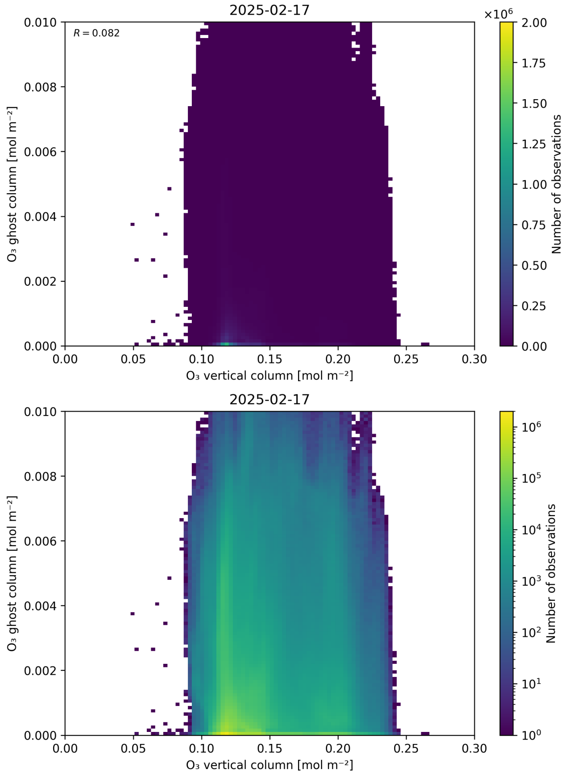
Figure 40: Scatter density plot of “O 3 vertical column” against “O 3 ghost column” for 2025-02-16 to 2025-02-18.
