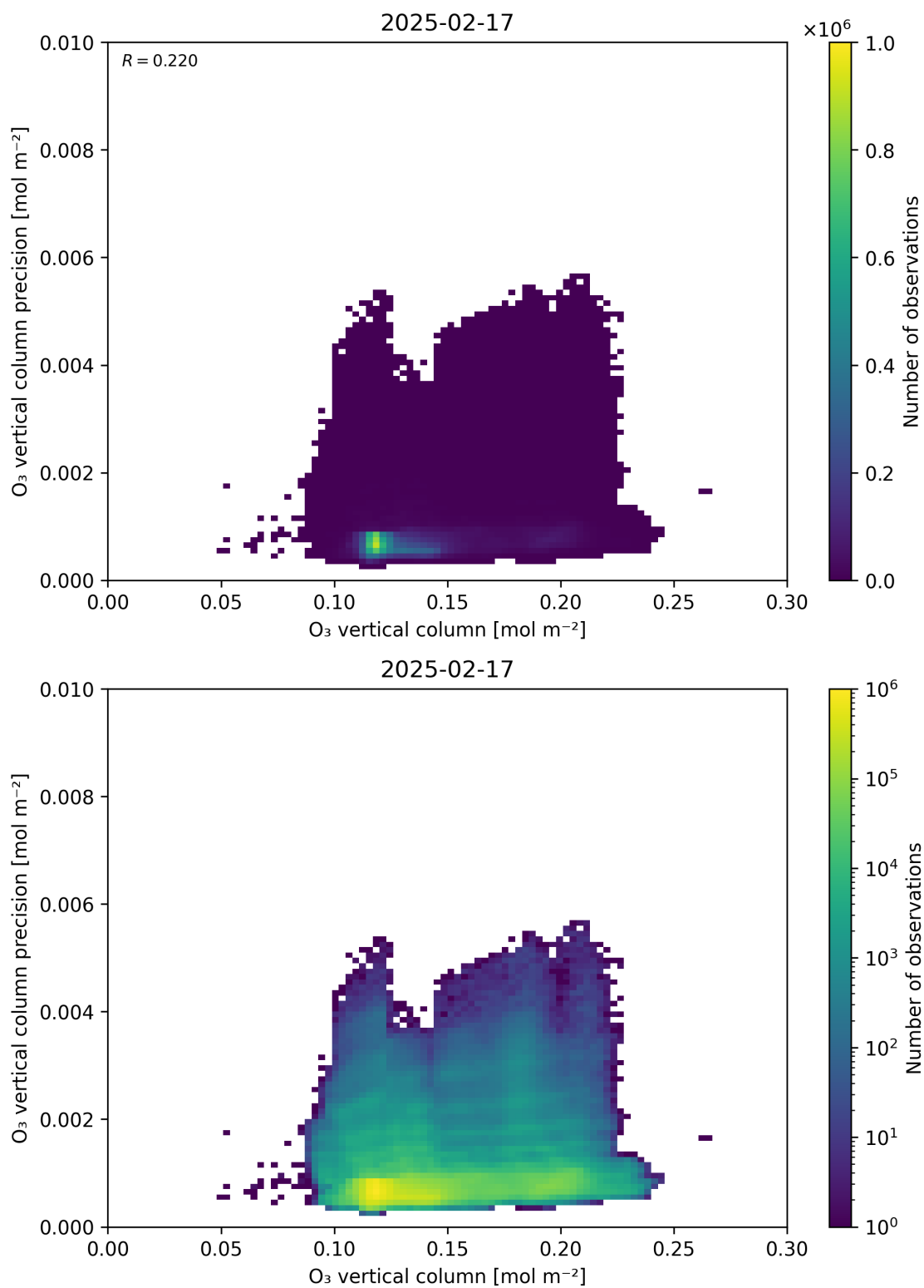
Figure 41: Scatter density plot of “O 3 vertical column” against “O 3 vertical column precision” for 2025-02-16 to 2025-02-18.
