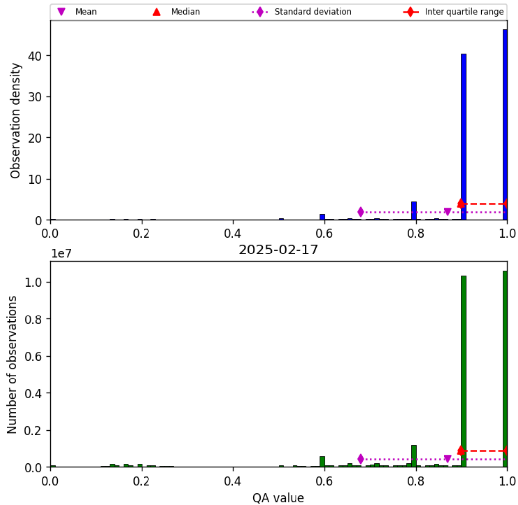
Figure 20: Histogram of “QA value” for 2025-02-16 to 2025-02-18
