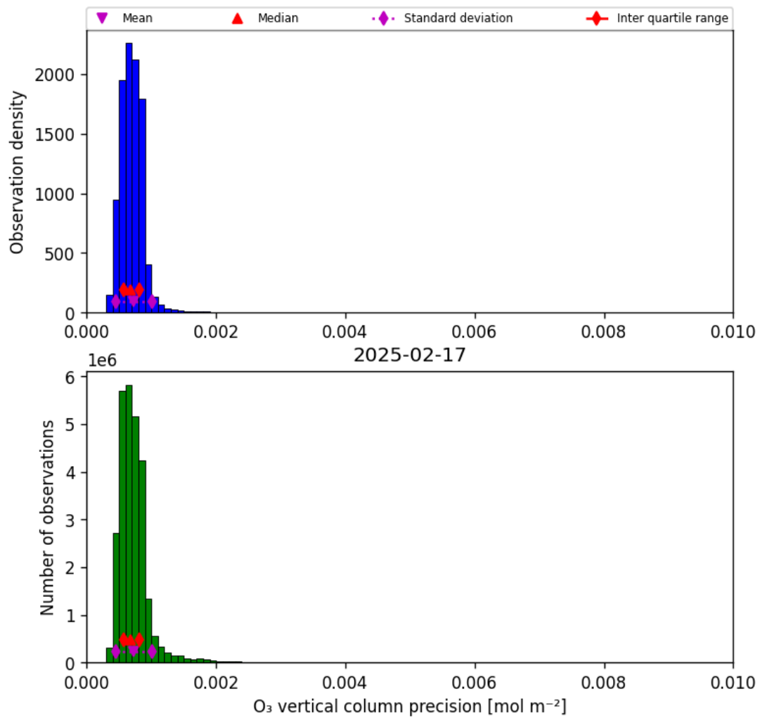
Figure 22: Histogram of “O 3 vertical column precision” for 2025-02-16 to 2025-02-18
