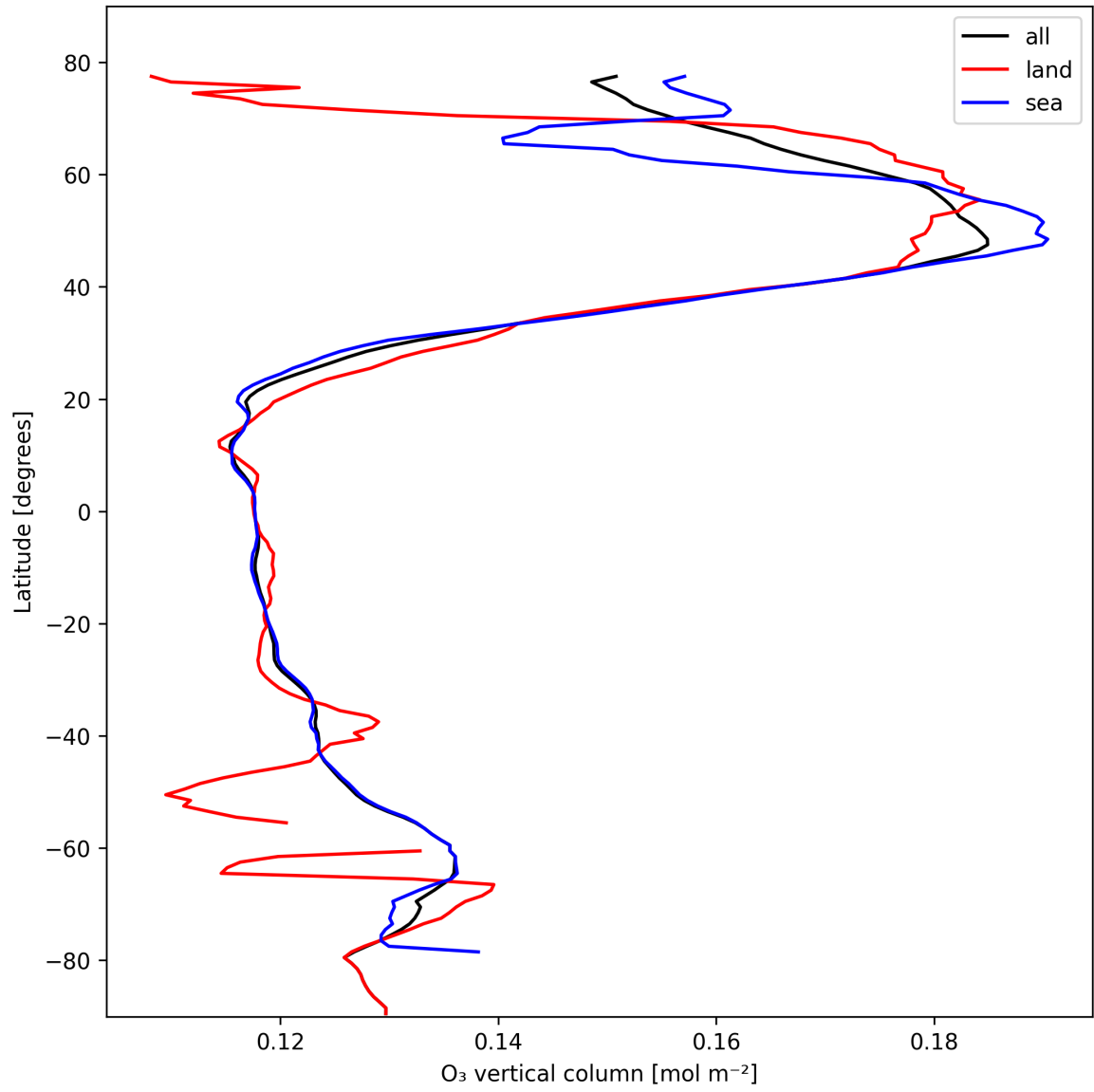
Figure 14: Zonal average of “O 3 vertical column” for 2025-02-16 to 2025-02-18.
