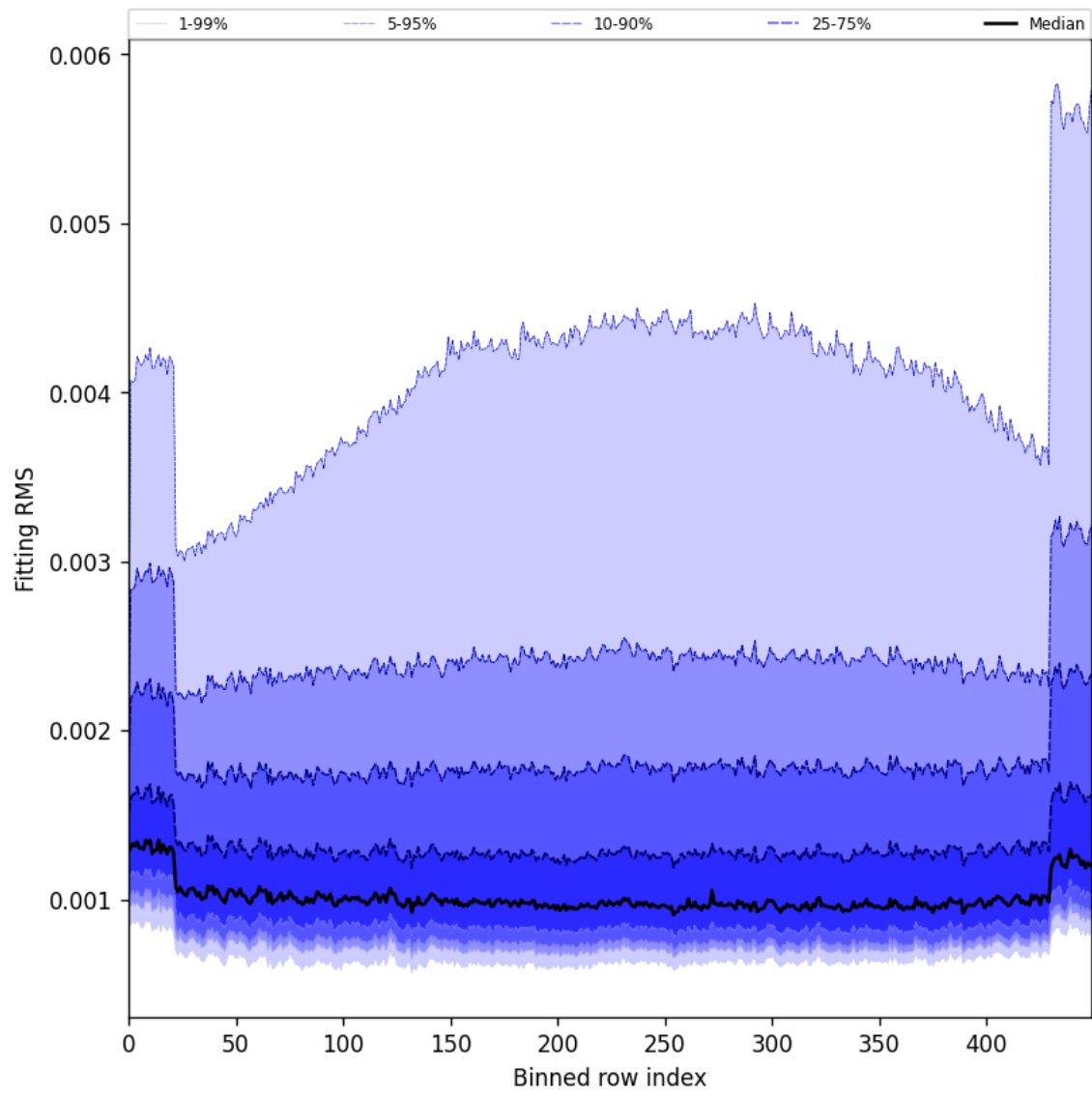
Figure 30: Along track statistics of “Fitting RMS” for 2025-02-16 to 2025-02-18
