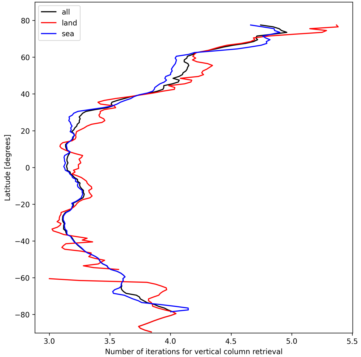
Figure 19: Zonal average of “Number of iterations for vertical column retrieval” for 2025-02-16 to 2025-02-18.
