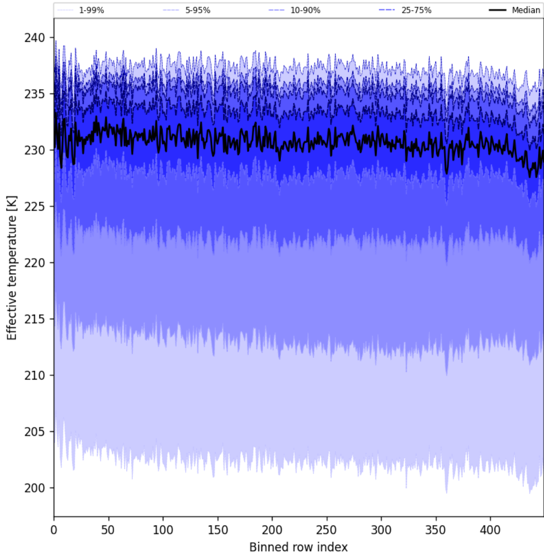
Figure 31: Along track statistics of “Effective temperature” for 2025-02-16 to 2025-02-18
