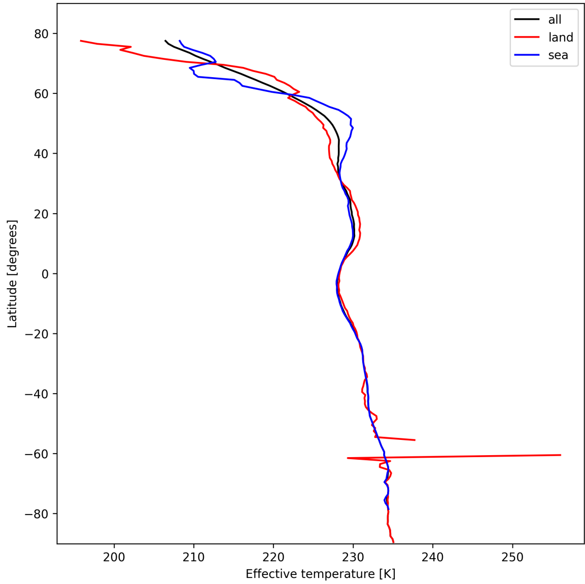
Figure 17: Zonal average of “Effective temperature” for 2025-02-16 to 2025-02-18.
