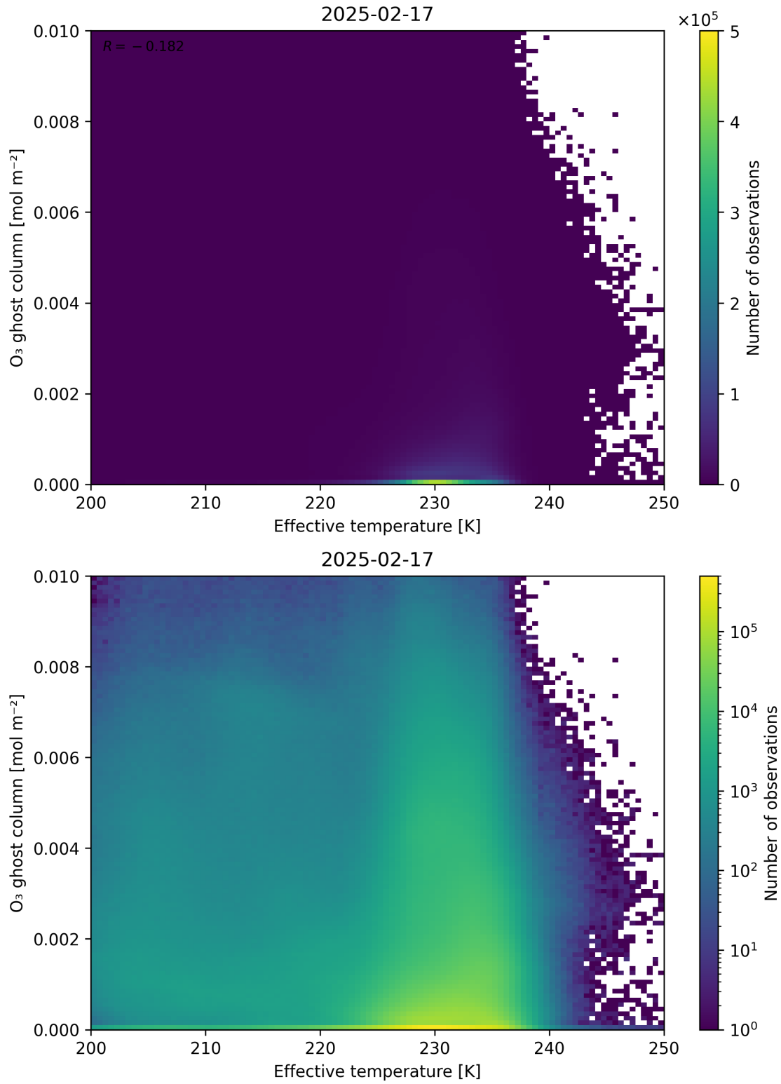
Figure 38: Scatter density plot of “Effective temperature” against “O 3 ghost column” for 2025-02-16 to 2025-02-18.
