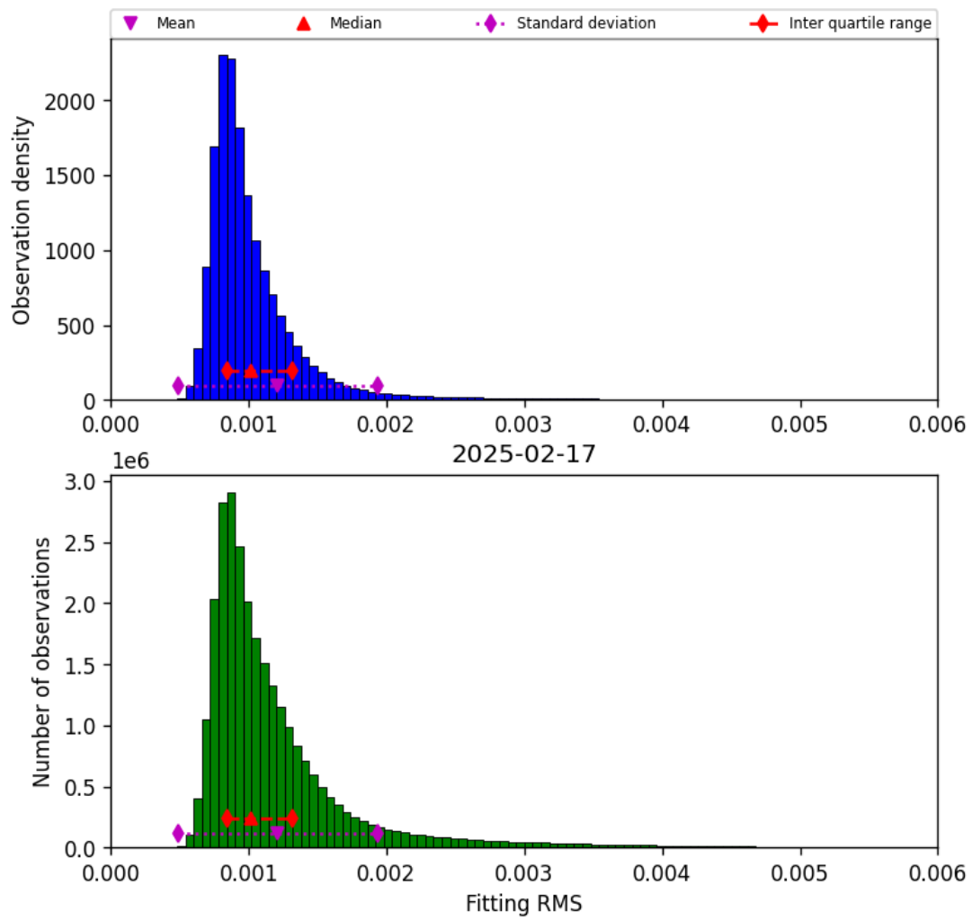
Figure 23: Histogram of “Fitting RMS” for 2025-02-16 to 2025-02-18
