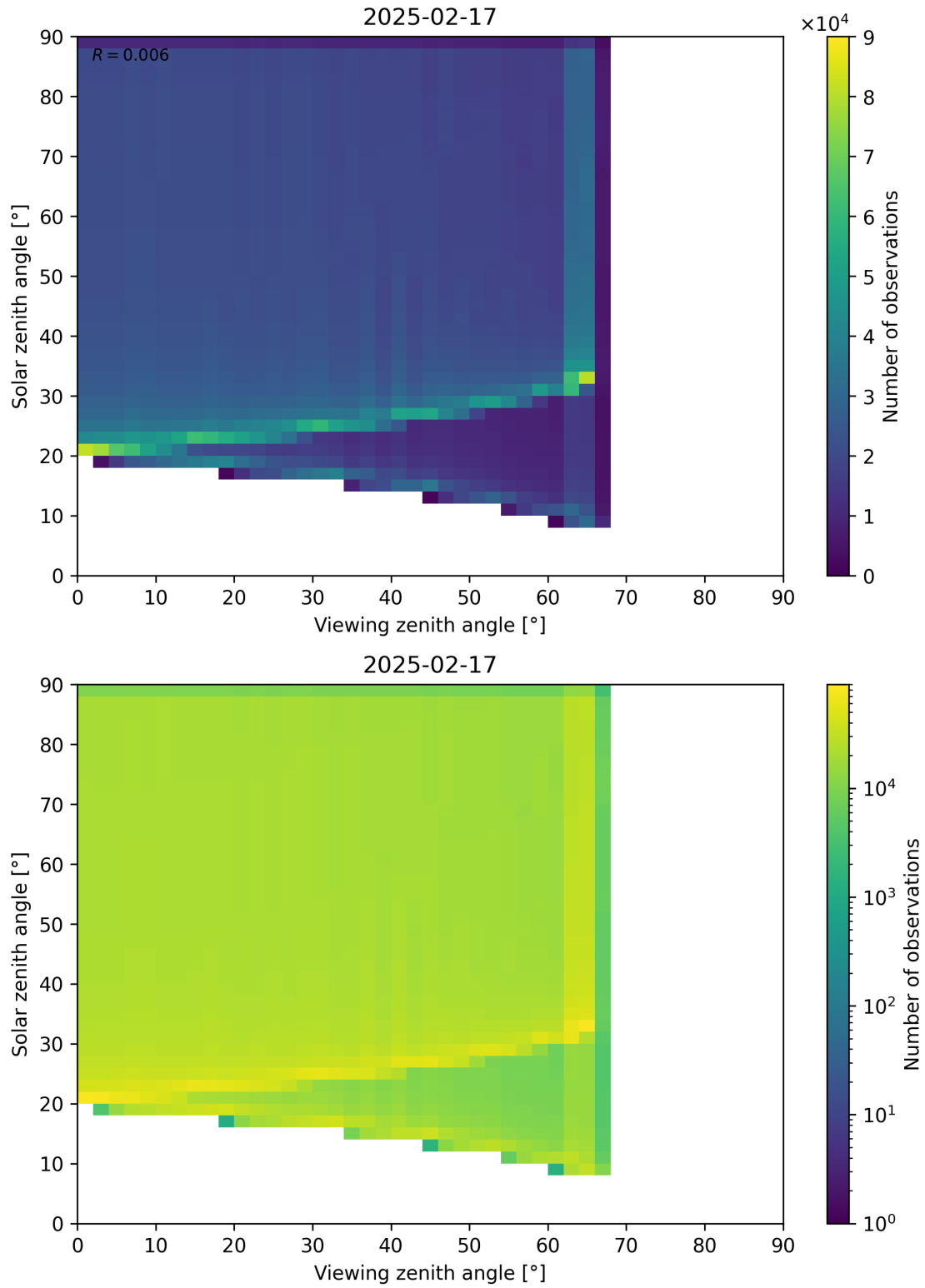
Figure 54: Scatter density plot of “Viewing zenith angle” against “Solar zenith angle” for 2025-02-16 to 2025-02-18.
