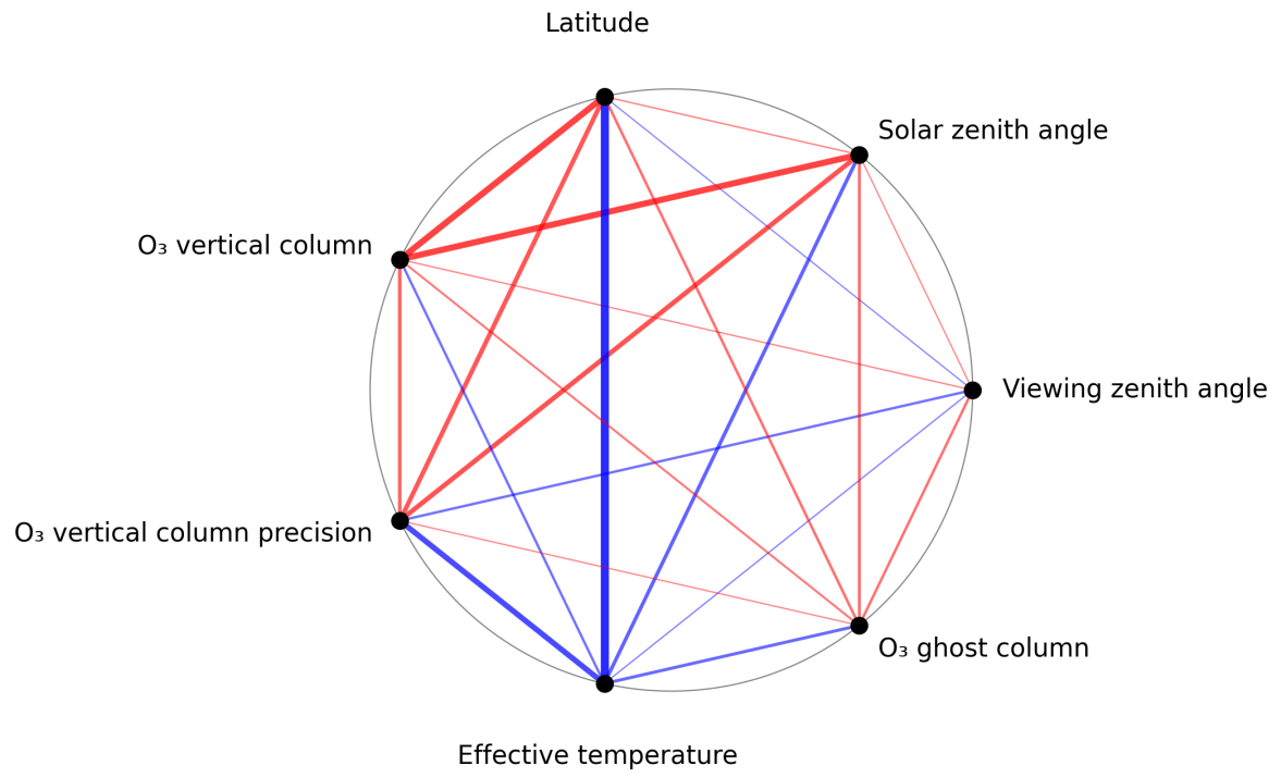
Figure 1: Map of correlation graph for 2025-02-16 to 2025-02-18.
