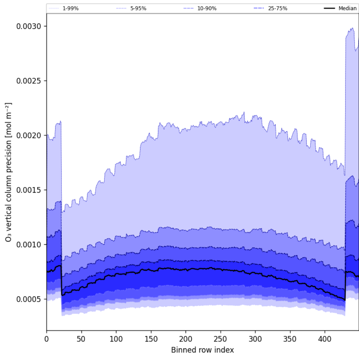
Figure 29: Along track statistics of “O 3 vertical column precision” for 2025-02-16 to 2025-02-18
