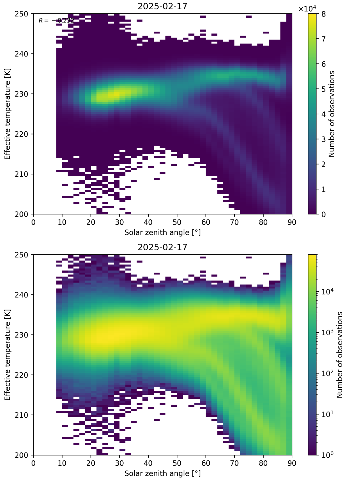
Figure 45: Scatter density plot of “Solar zenith angle” against “Effective temperature” for 2025-02-16 to 2025-02-18.
