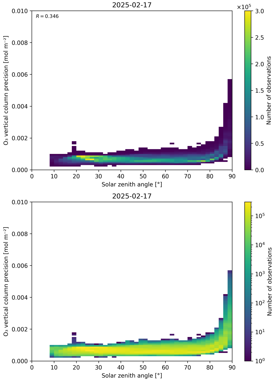
Figure 48: Scatter density plot of “Solar zenith angle” against “O 3 vertical column precision” for 2025-02-16 to 2025-02-18.
