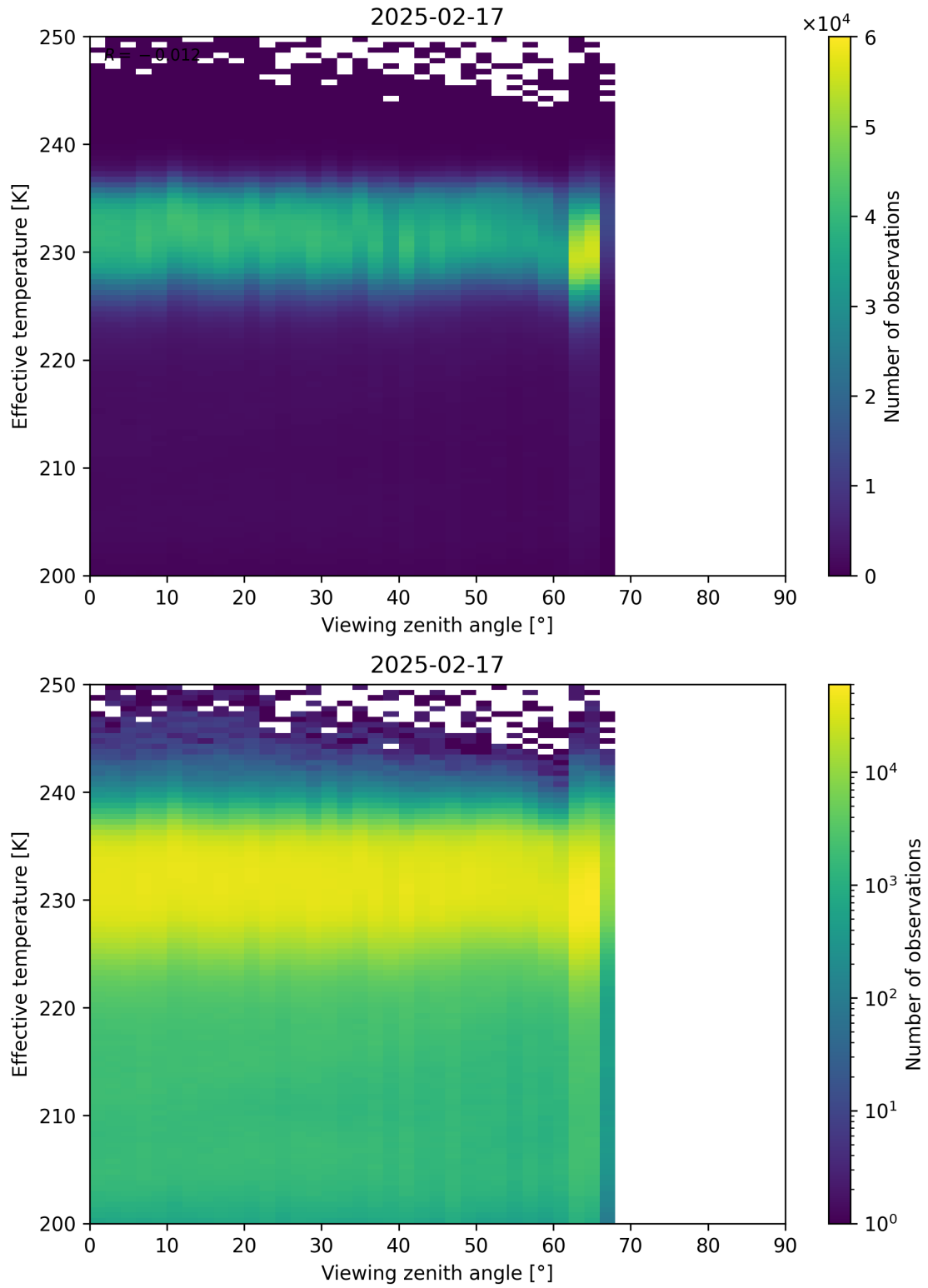
Figure 50: Scatter density plot of “Viewing zenith angle” against “Effective temperature” for 2025-02-16 to 2025-02-18.
