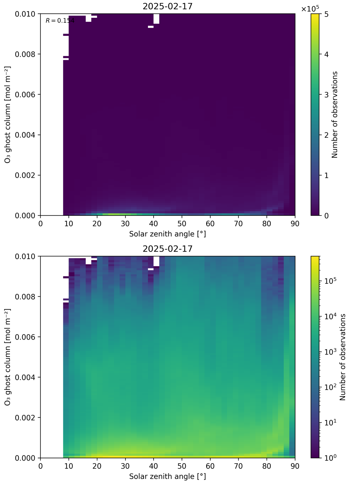
Figure 46: Scatter density plot of “Solar zenith angle” against “O 3 ghost column” for 2025-02-16 to 2025-02-18.
