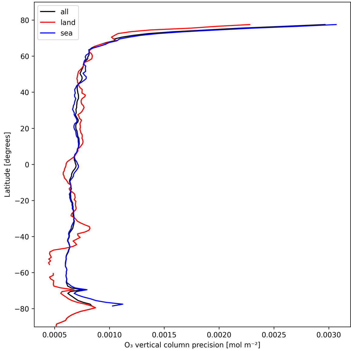
Figure 15: Zonal average of “O 3 vertical column precision” for 2025-02-16 to 2025-02-18.
