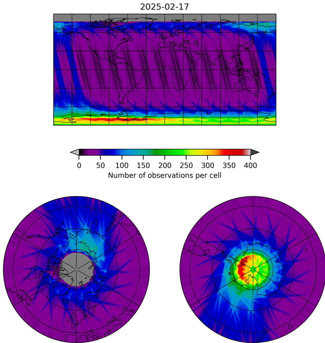
Figure 12: Map of the number of observations for 2025-02-16 to 2025-02-18
