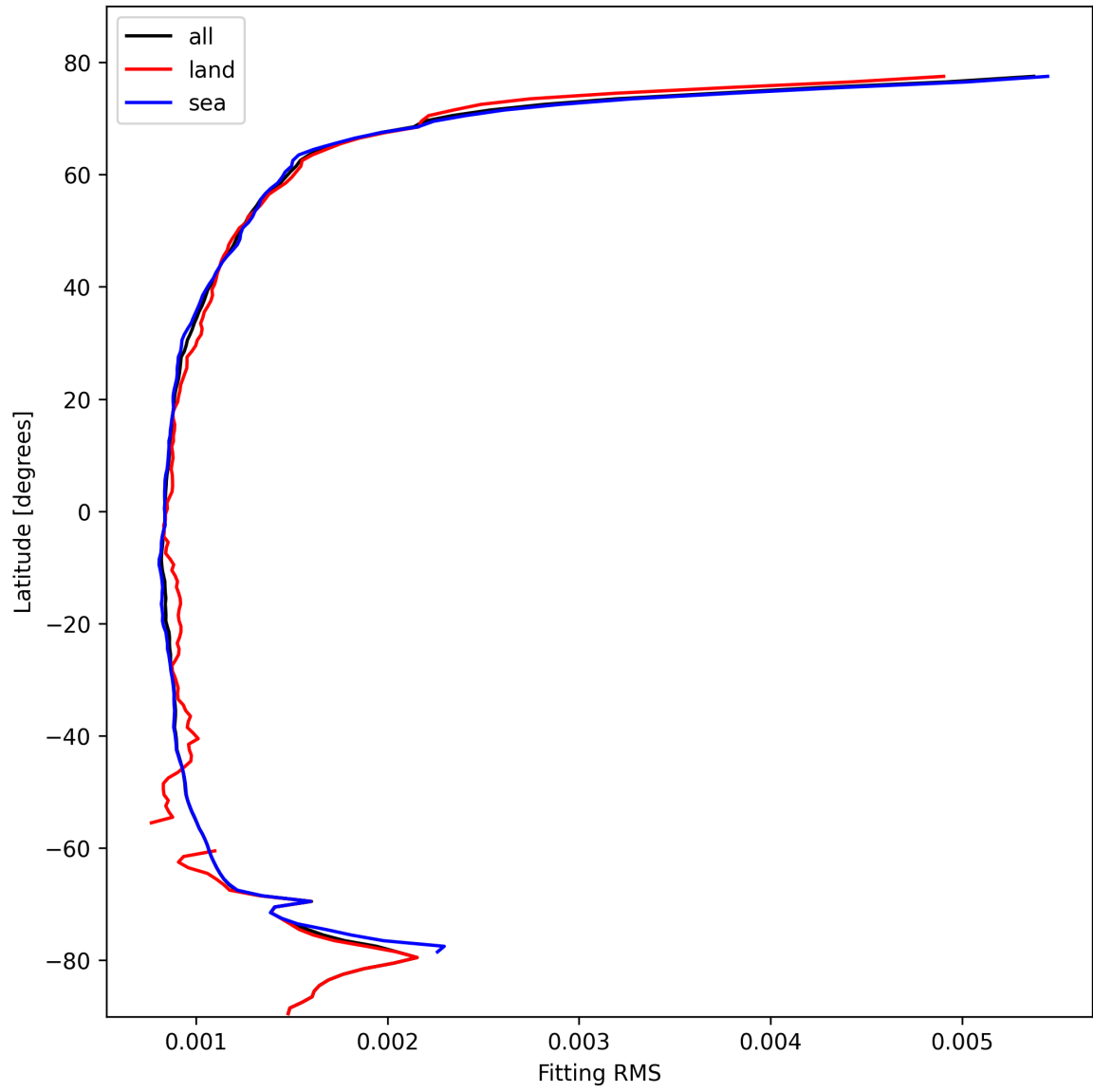
Figure 16: Zonal average of “Fitting RMS” for 2025-02-16 to 2025-02-18.
