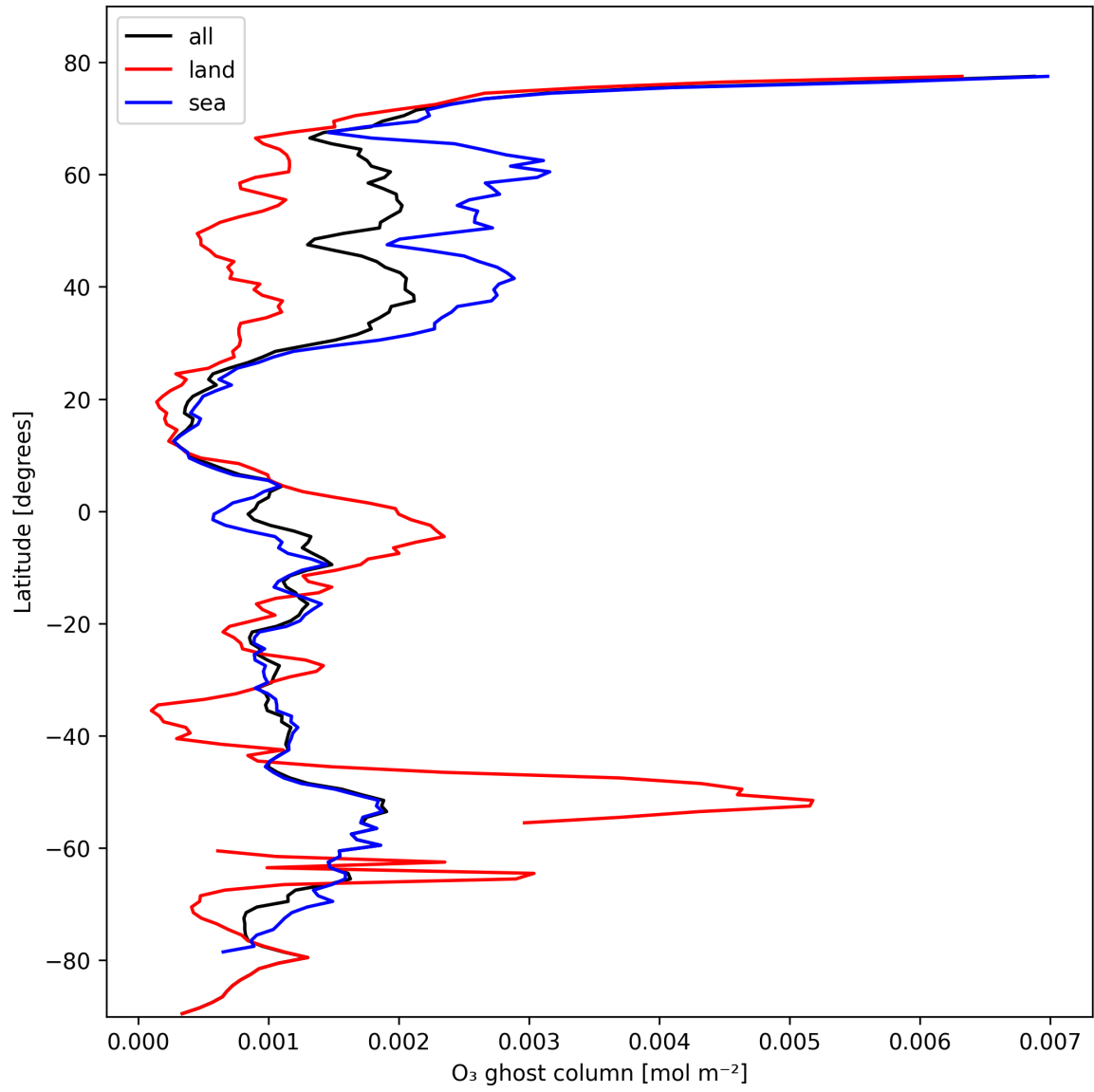
Figure 18: Zonal average of "O 3 ghost column" for 2025-02-16 to 2025-02-18.
