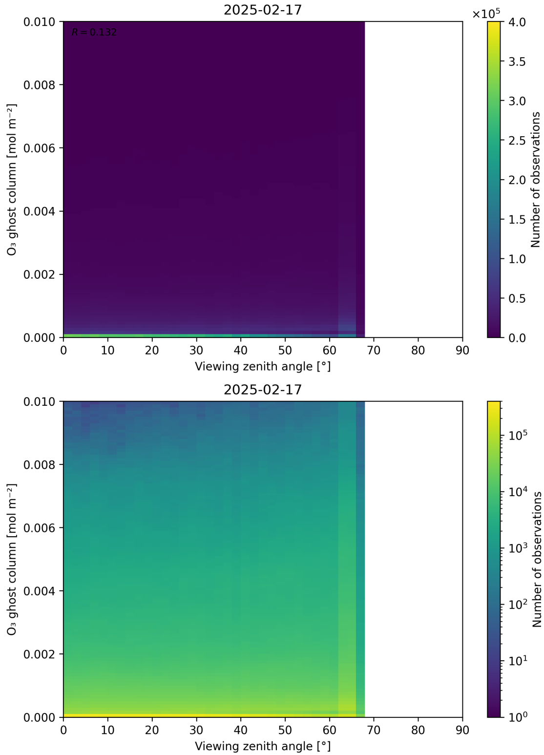
Figure 51: Scatter density plot of “Viewing zenith angle” against “O 3 ghost column” for 2025-02-16 to 2025-02-18.
