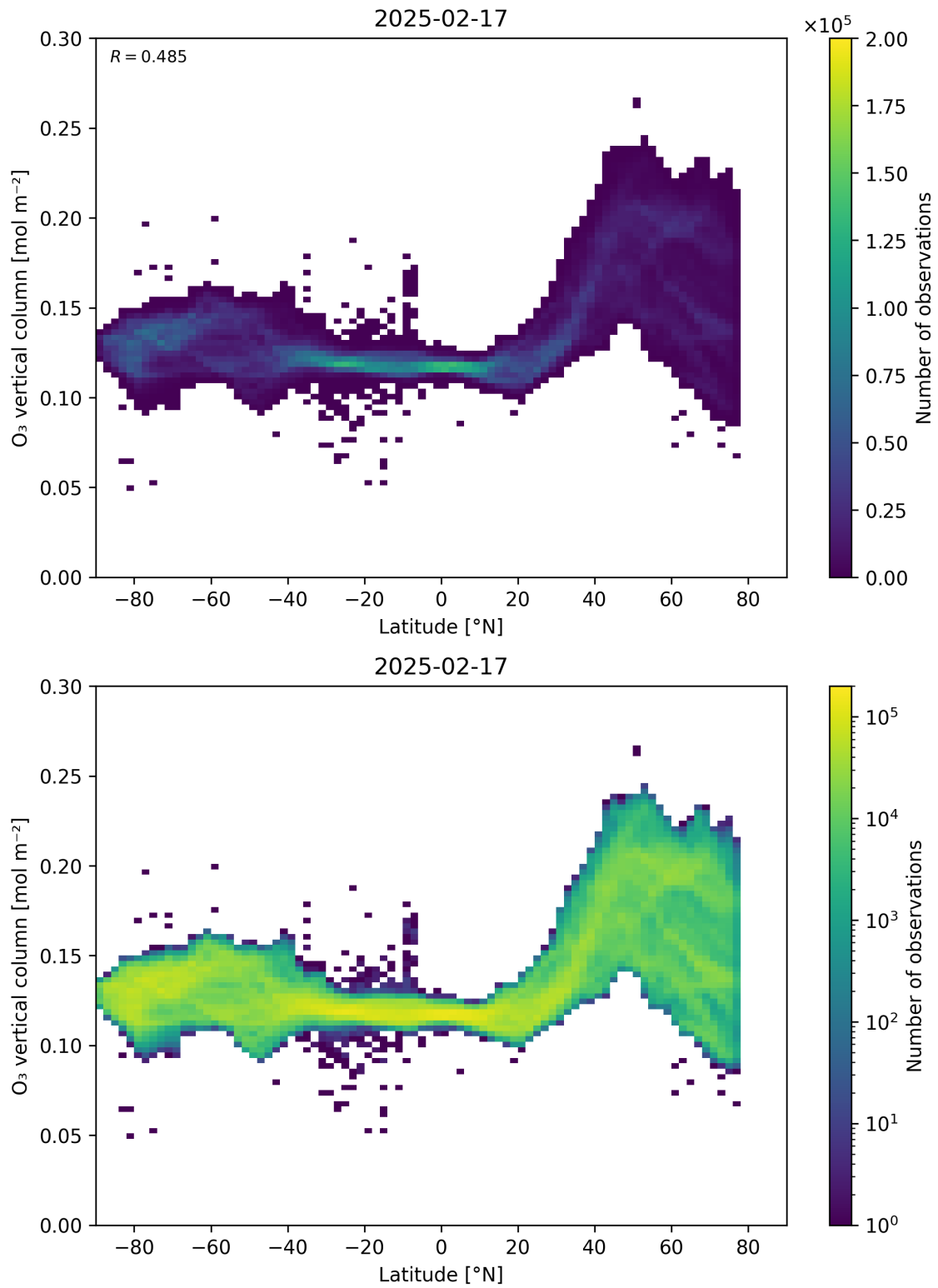
Figure 36: Scatter density plot of “Latitude” against “O 3 vertical column” for 2025-02-16 to 2025-02-18.
