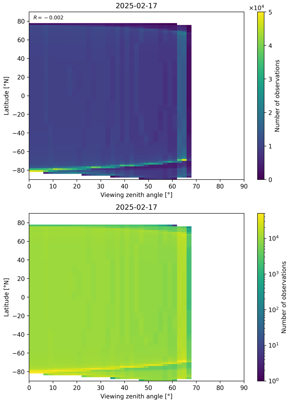
Figure 49: Scatter density plot of “Viewing zenith angle” against “Latitude” for 2025-02-16 to 2025-02-18.
