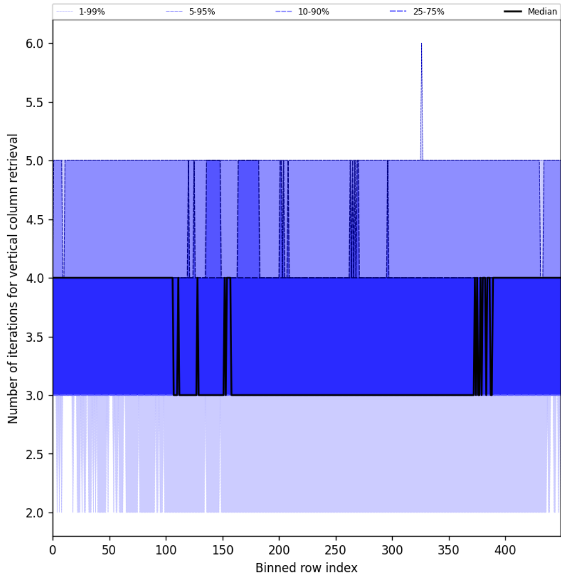
Figure 33: Along track statistics of “Number of iterations for vertical column retrieval” for 2025-02-16 to 2025-02-18
