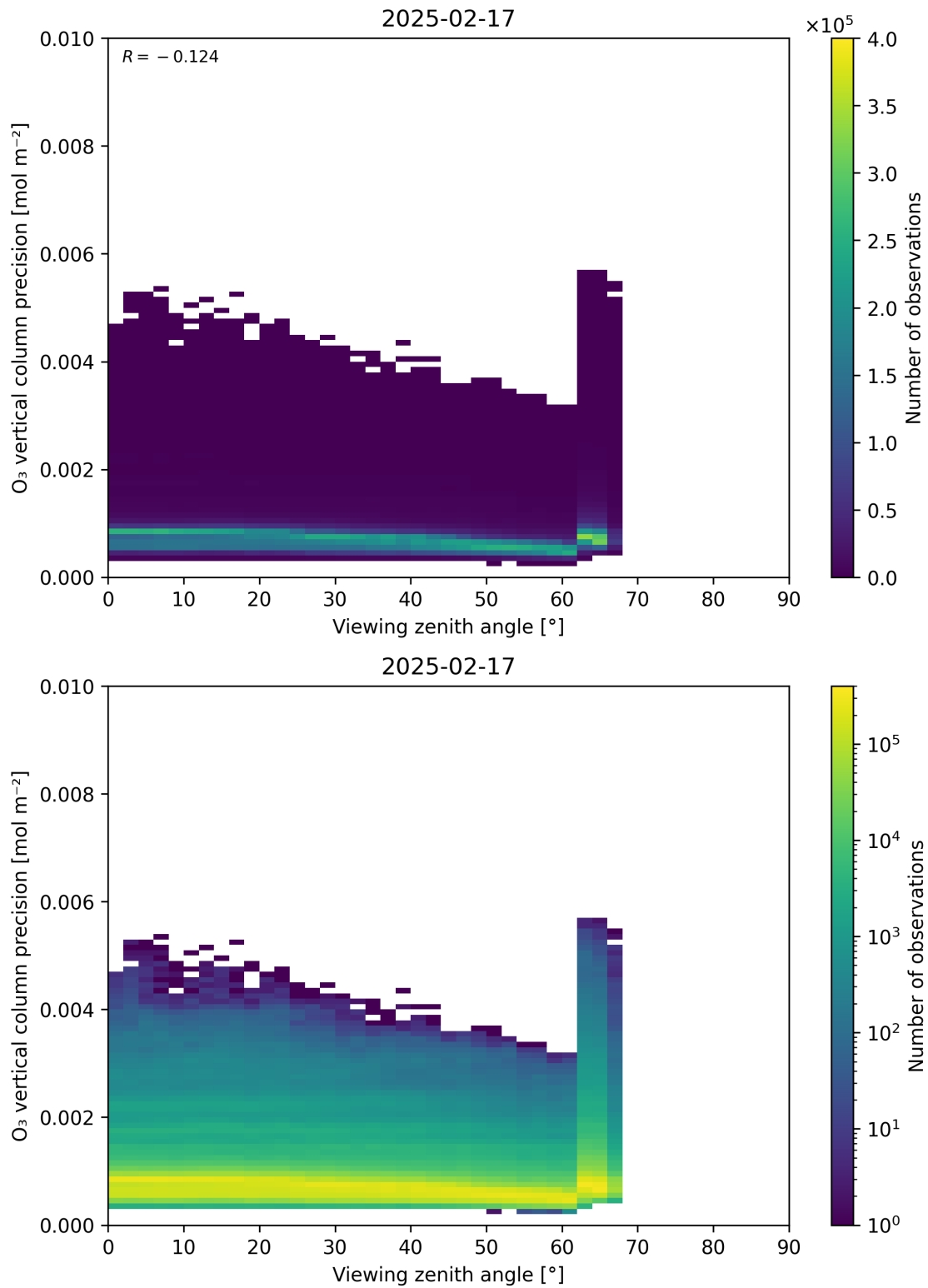
Figure 53: Scatter density plot of “Viewing zenith angle” against “O 3 vertical column precision” for 2025-02-16 to 2025-02-18.
