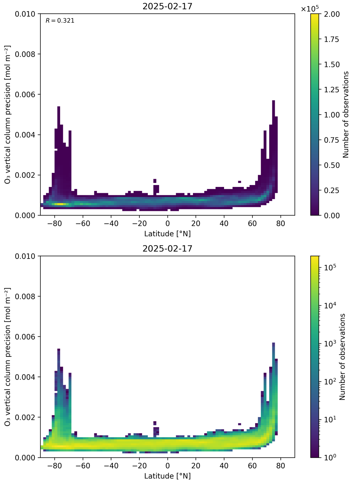
Figure 37: Scatter density plot of “Latitude” against “O 3 vertical column precision” for 2025-02-16 to 2025-02-18.
