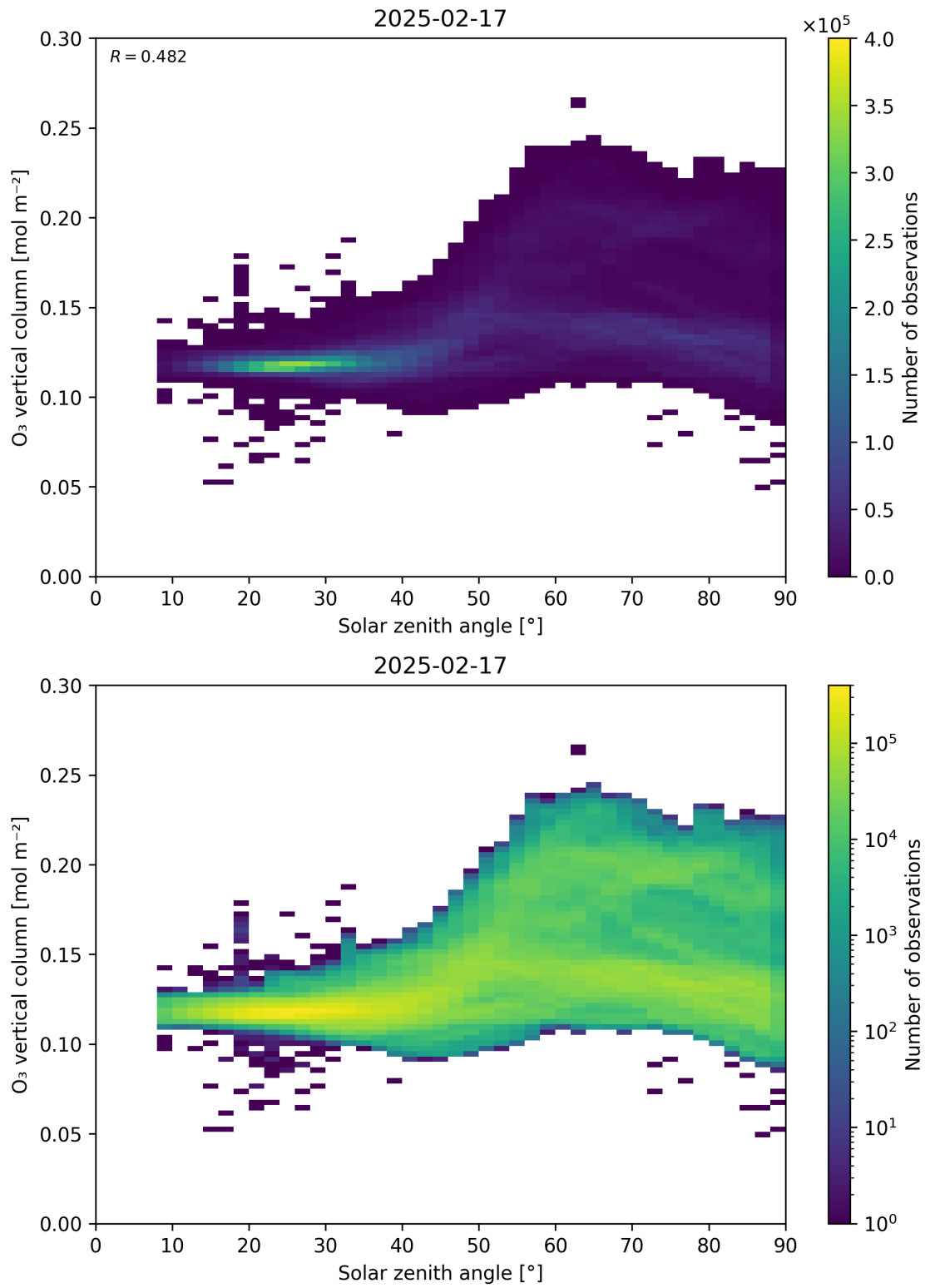
Figure 47: Scatter density plot of “Solar zenith angle” against “O 3 vertical column” for 2025-02-16 to 2025-02-18.
