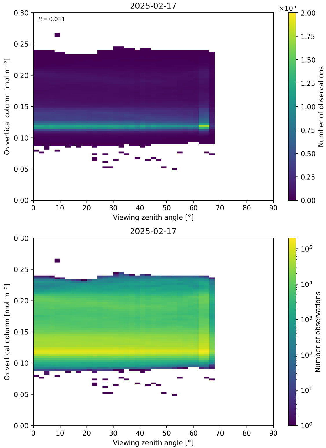
Figure 52: Scatter density plot of “Viewing zenith angle” against “O 3 vertical column” for 2025-02-16 to 2025-02-18.
