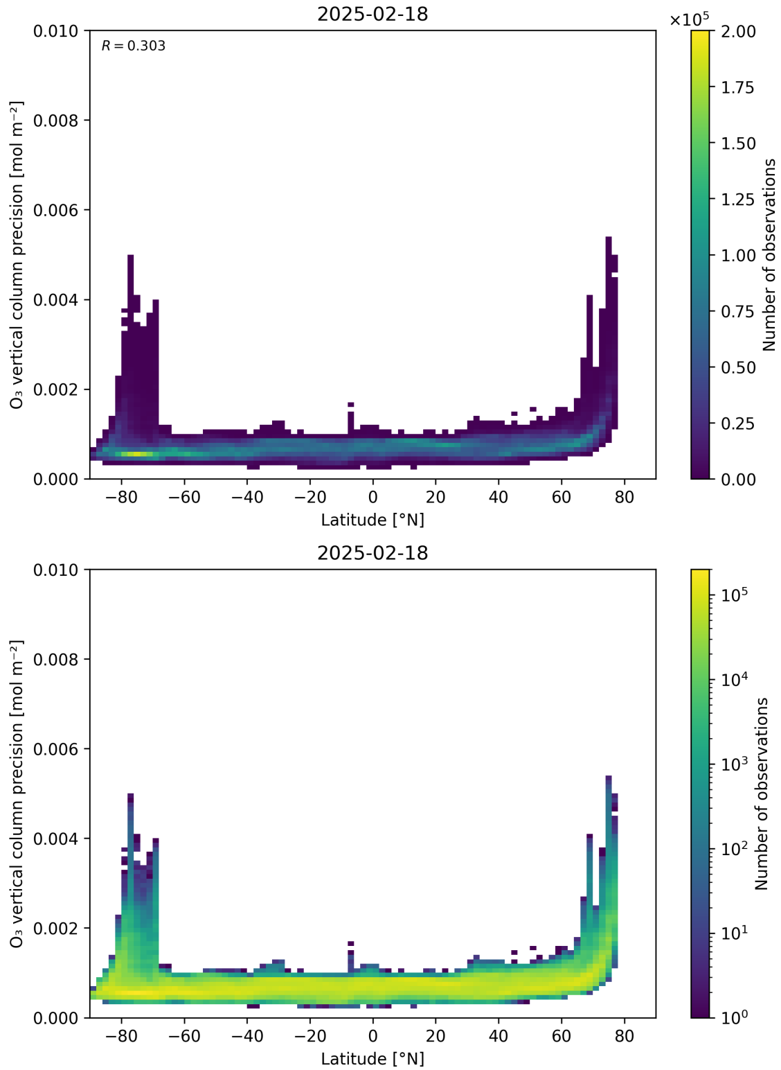
Figure 37: Scatter density plot of “Latitude” against “O 3 vertical column precision” for 2025-02-18 to 2025-02-19.
