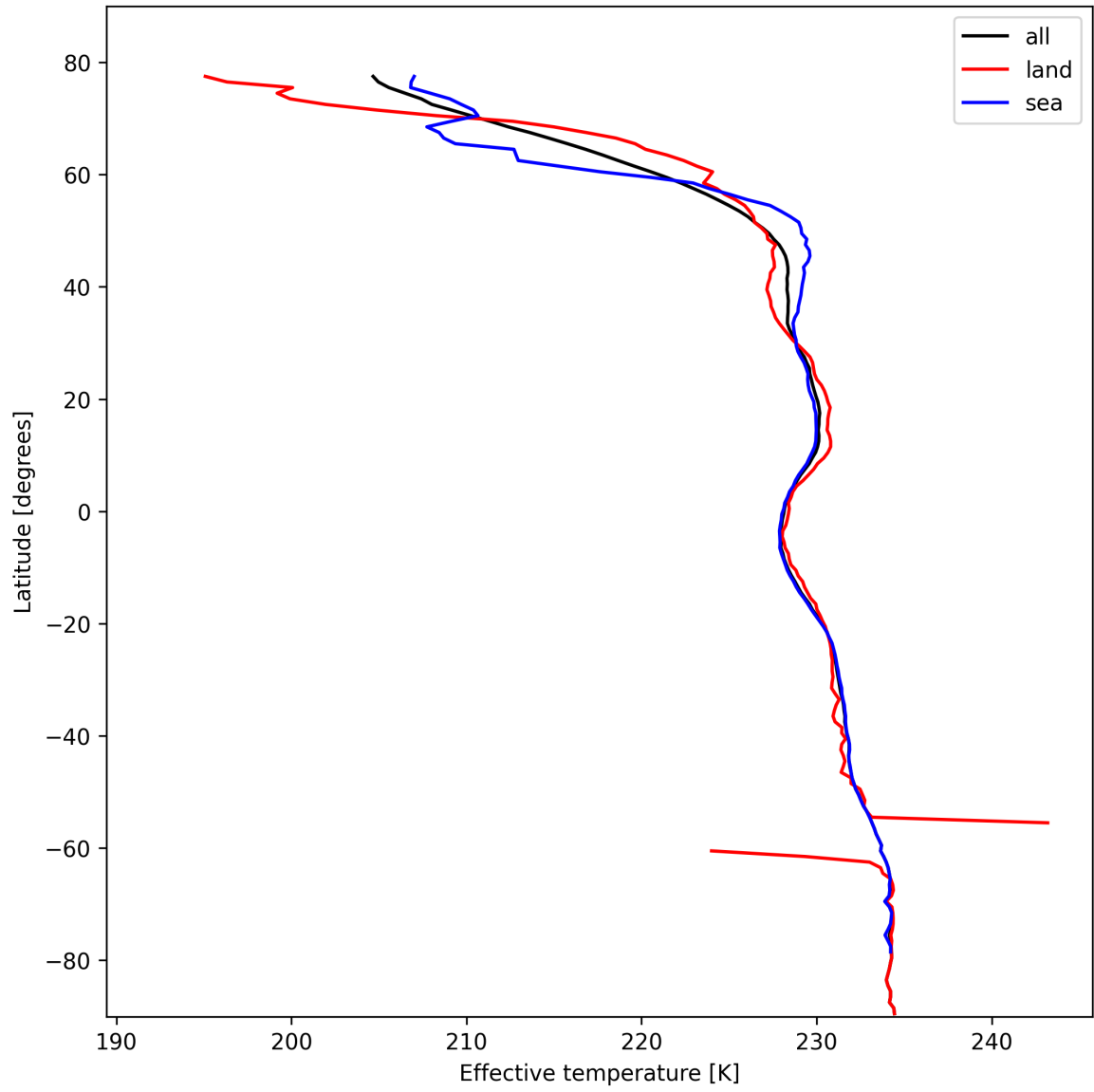
Figure 17: Zonal average of "Effective temperature" for 2025-02-18 to 2025-02-19.
