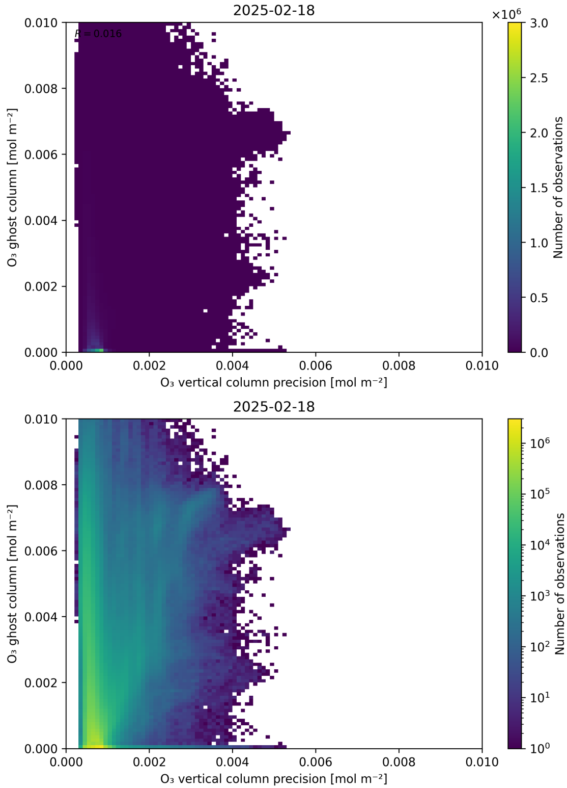
Figure 43: Scatter density plot of “O 3 vertical column precision” against “O 3 ghost column” for 2025-02-18 to 2025-02-19.
