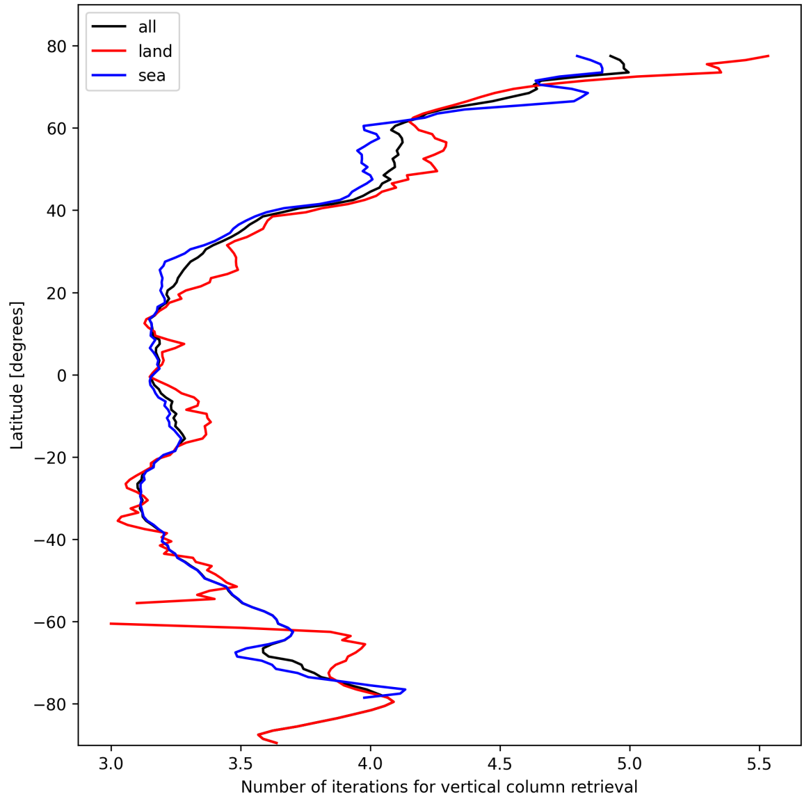
Figure 19: Zonal average of “Number of iterations for vertical column retrieval” for 2025-02-18 to 2025-02-19.
