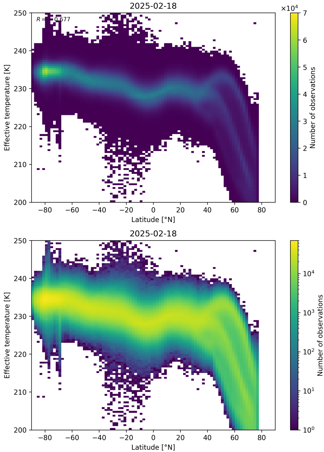
Figure 34: Scatter density plot of “Latitude” against “Effective temperature” for 2025-02-18 to 2025-02-19.
