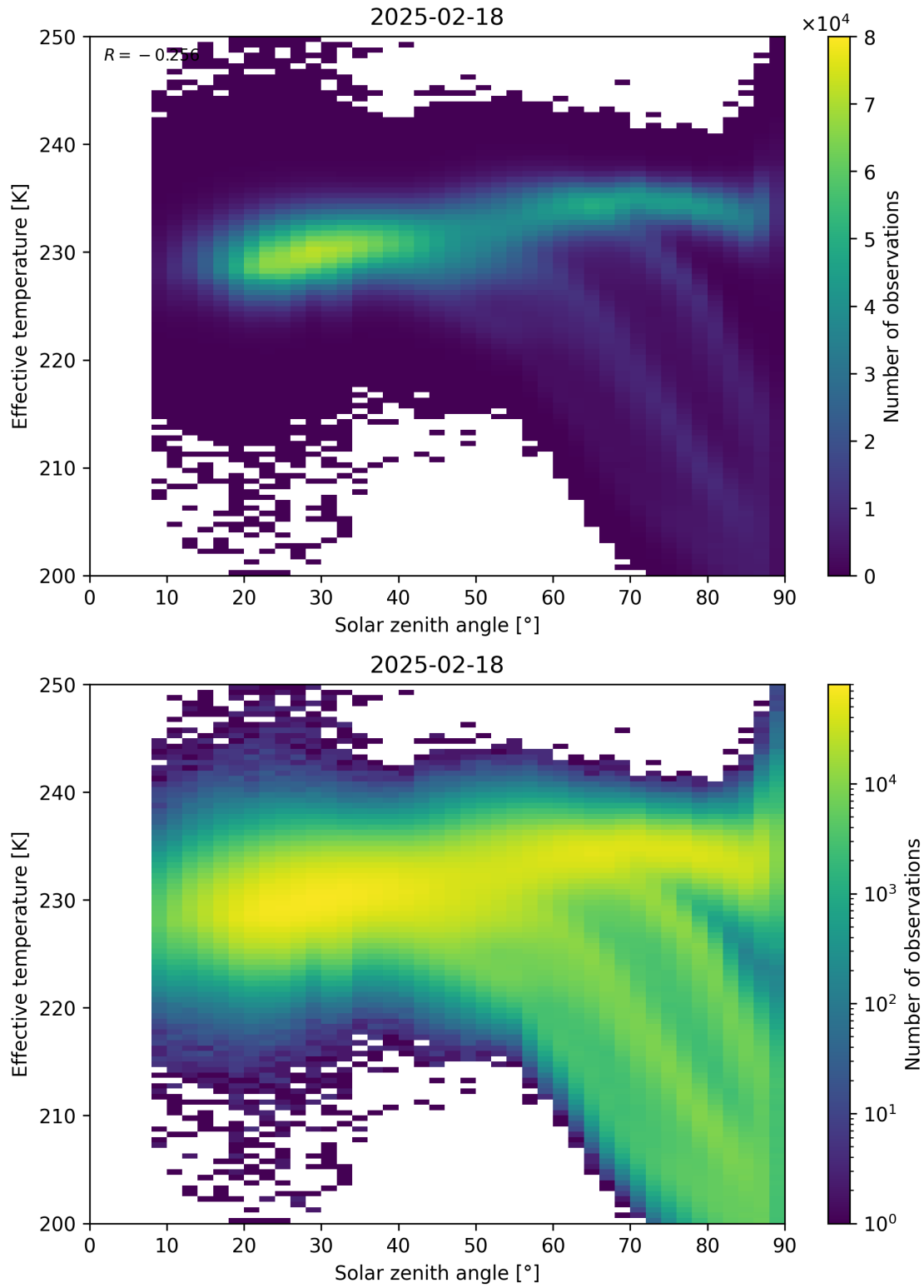
Figure 45: Scatter density plot of “Solar zenith angle” against “Effective temperature” for 2025-02-18 to 2025-02-19.
