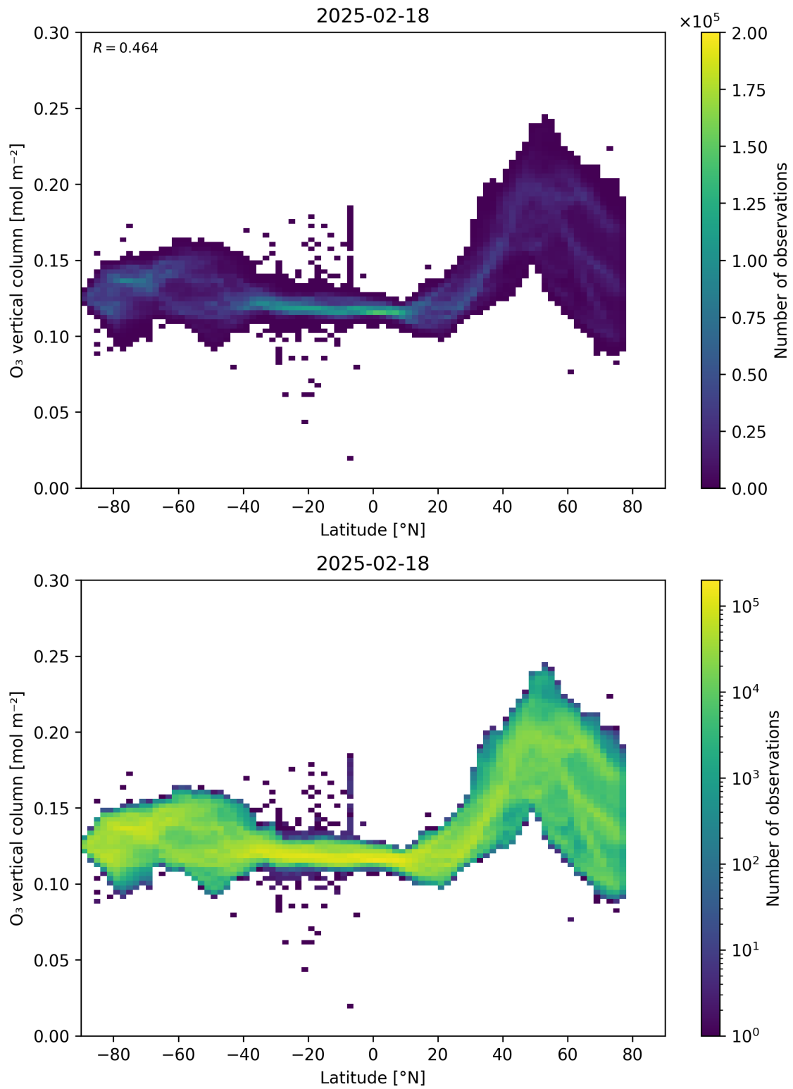
Figure 36: Scatter density plot of “Latitude” against “O 3 vertical column” for 2025-02-18 to 2025-02-19.
