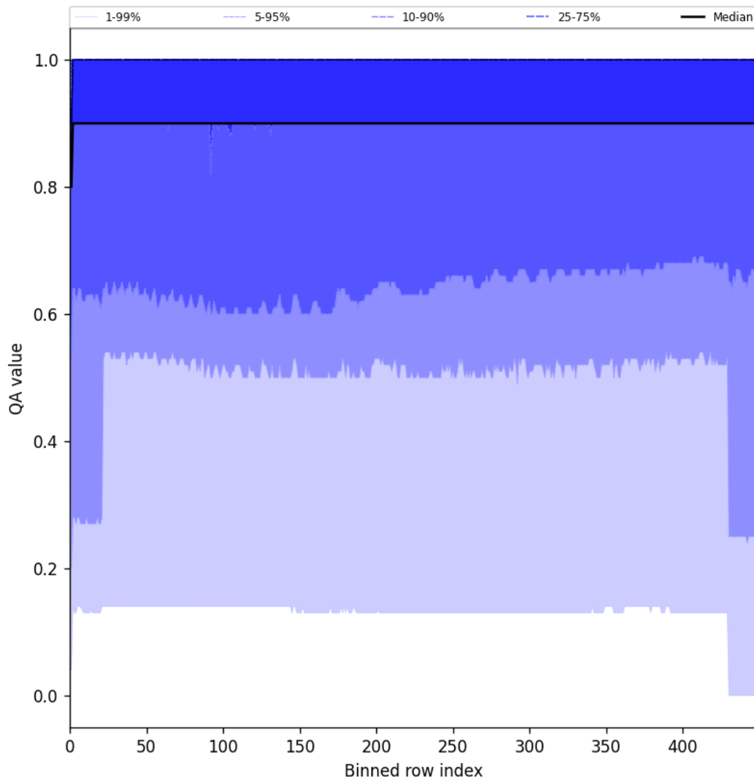
Figure 27: Along track statistics of “QA value” for 2025-02-18 to 2025-02-19
