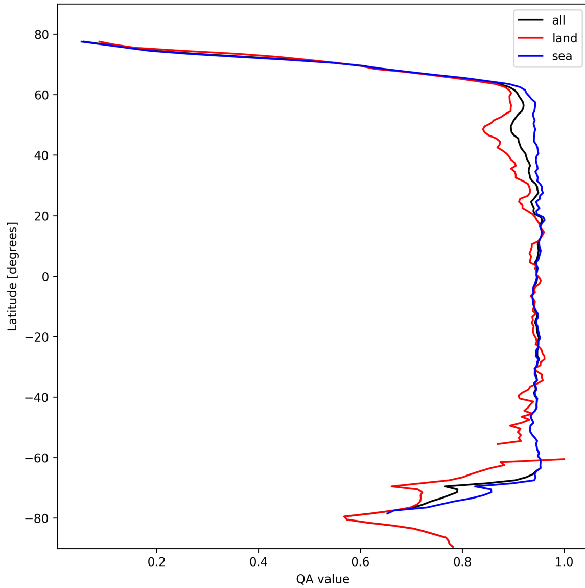
Figure 13: Zonal average of “QA value” for 2025-02-18 to 2025-02-19.
