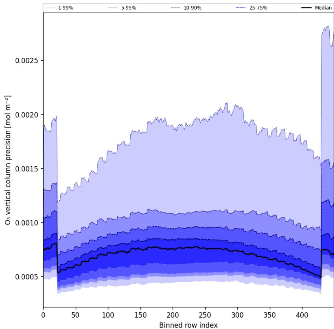
Figure 29: Along track statistics of “O 3 vertical column precision” for 2025-02-18 to 2025-02-19
