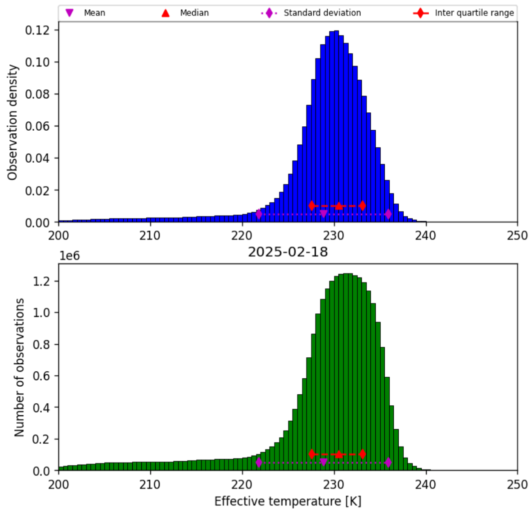
Figure 24: Histogram of “Effective temperature” for 2025-02-18 to 2025-02-19
