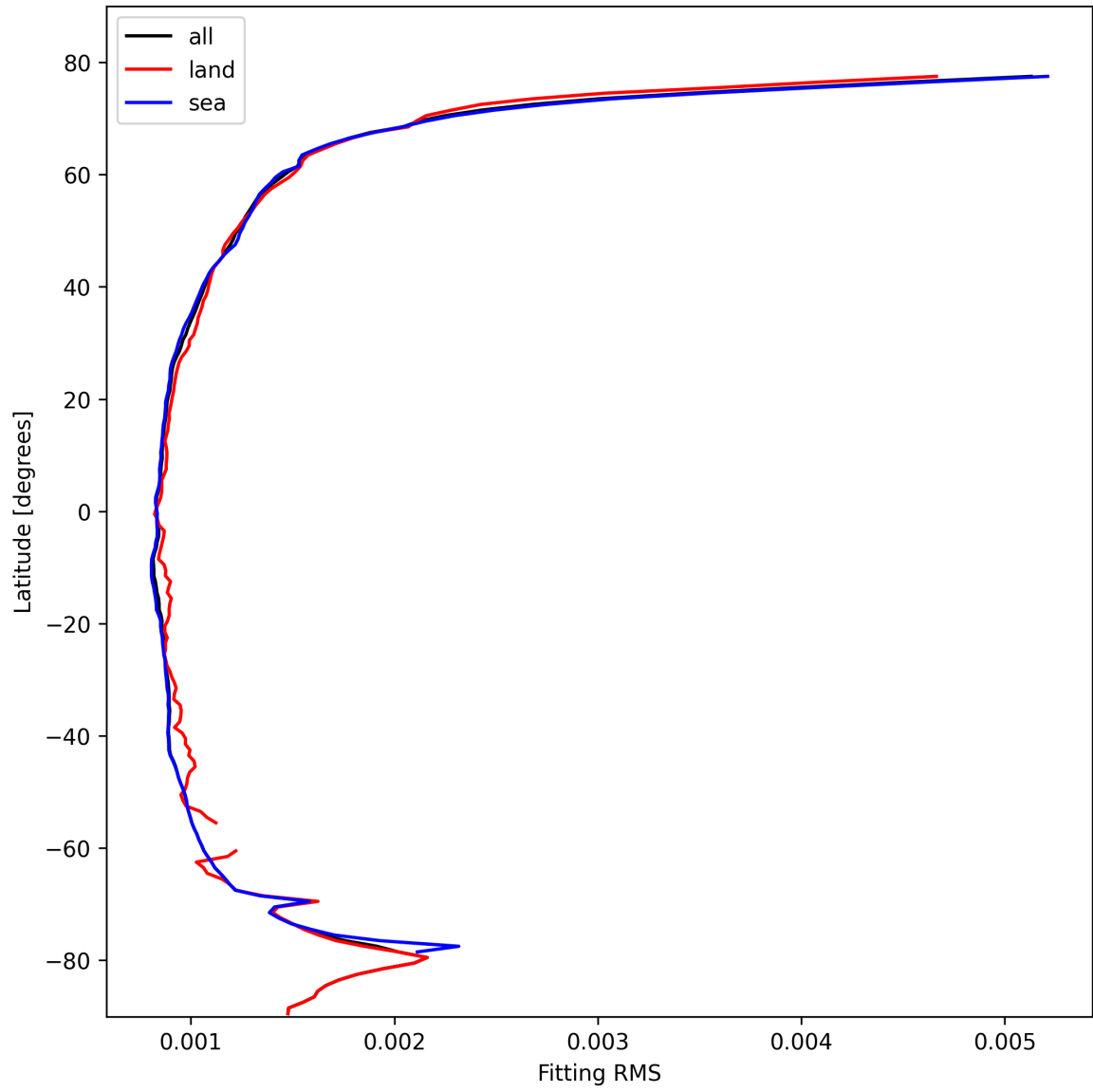
Figure 16: Zonal average of “Fitting RMS” for 2025-02-18 to 2025-02-19.
