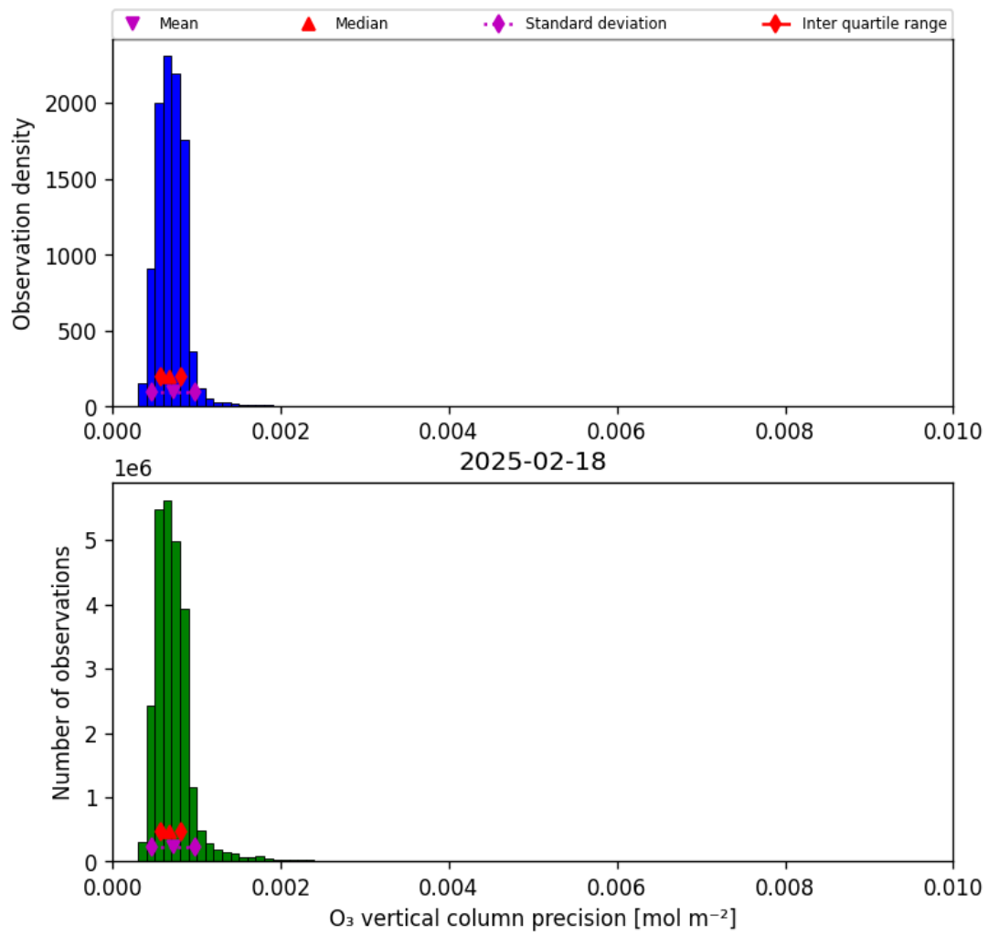
Figure 22: Histogram of “O 3 vertical column precision” for 2025-02-18 to 2025-02-19
