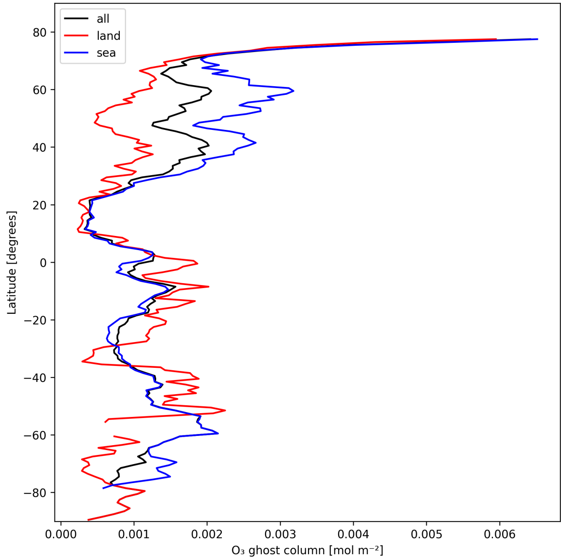
Figure 18: Zonal average of "O 3 ghost column" for 2025-02-18 to 2025-02-19.
