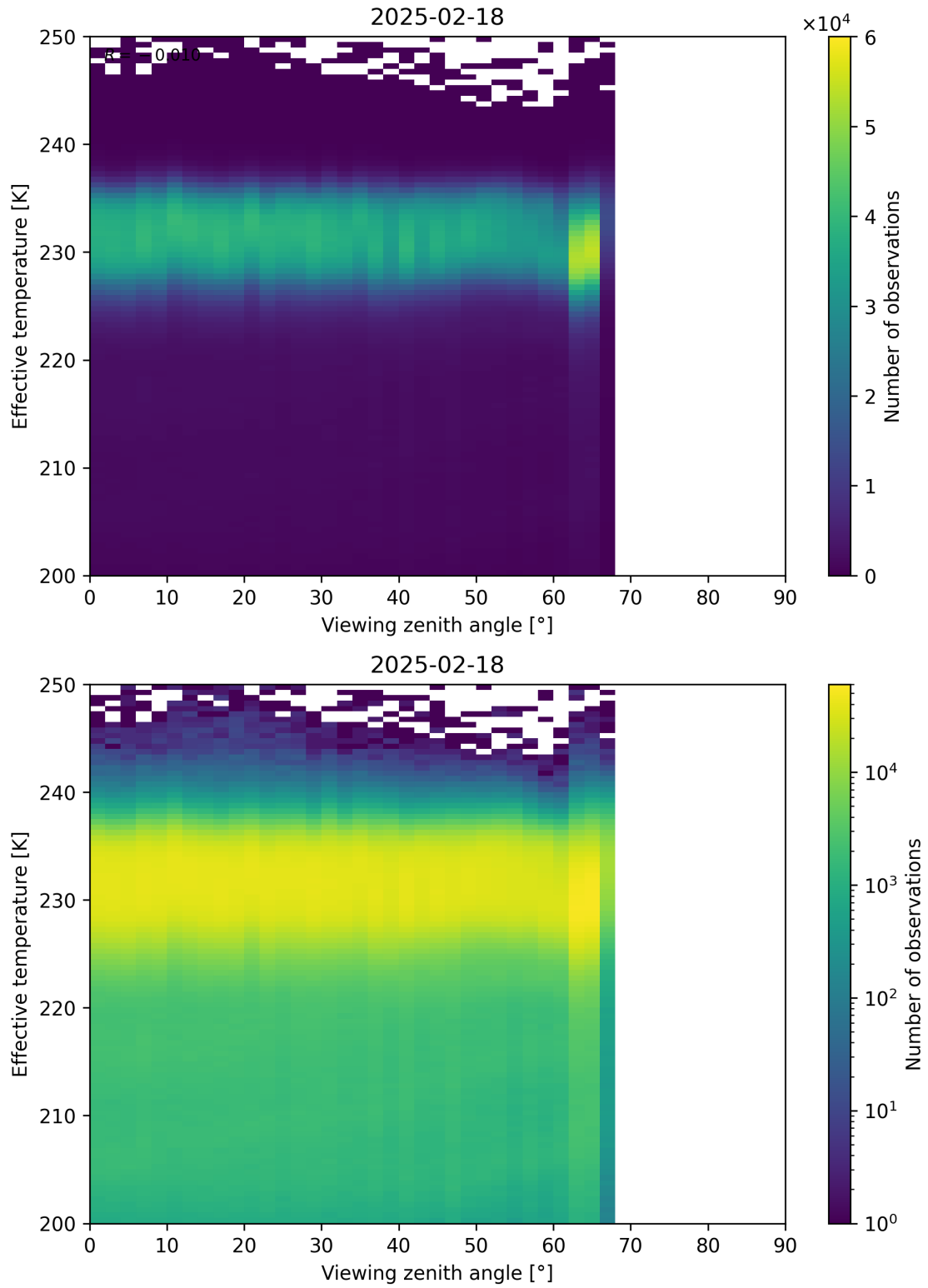
Figure 50: Scatter density plot of “Viewing zenith angle” against “Effective temperature” for 2025-02-18 to 2025-02-19.
