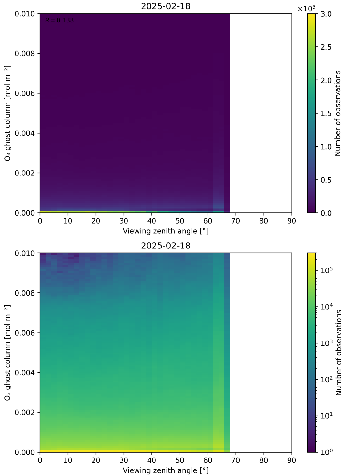
Figure 51: Scatter density plot of “Viewing zenith angle” against “O 3 ghost column” for 2025-02-18 to 2025-02-19.
