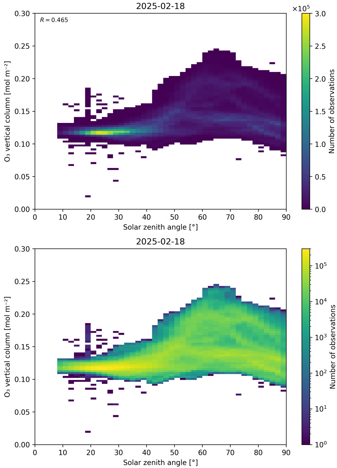
Figure 47: Scatter density plot of “Solar zenith angle” against “O 3 vertical column” for 2025-02-18 to 2025-02-19.
