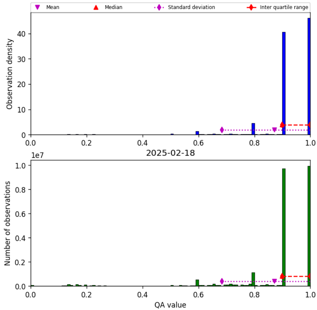
Figure 20: Histogram of “QA value” for 2025-02-18 to 2025-02-19
