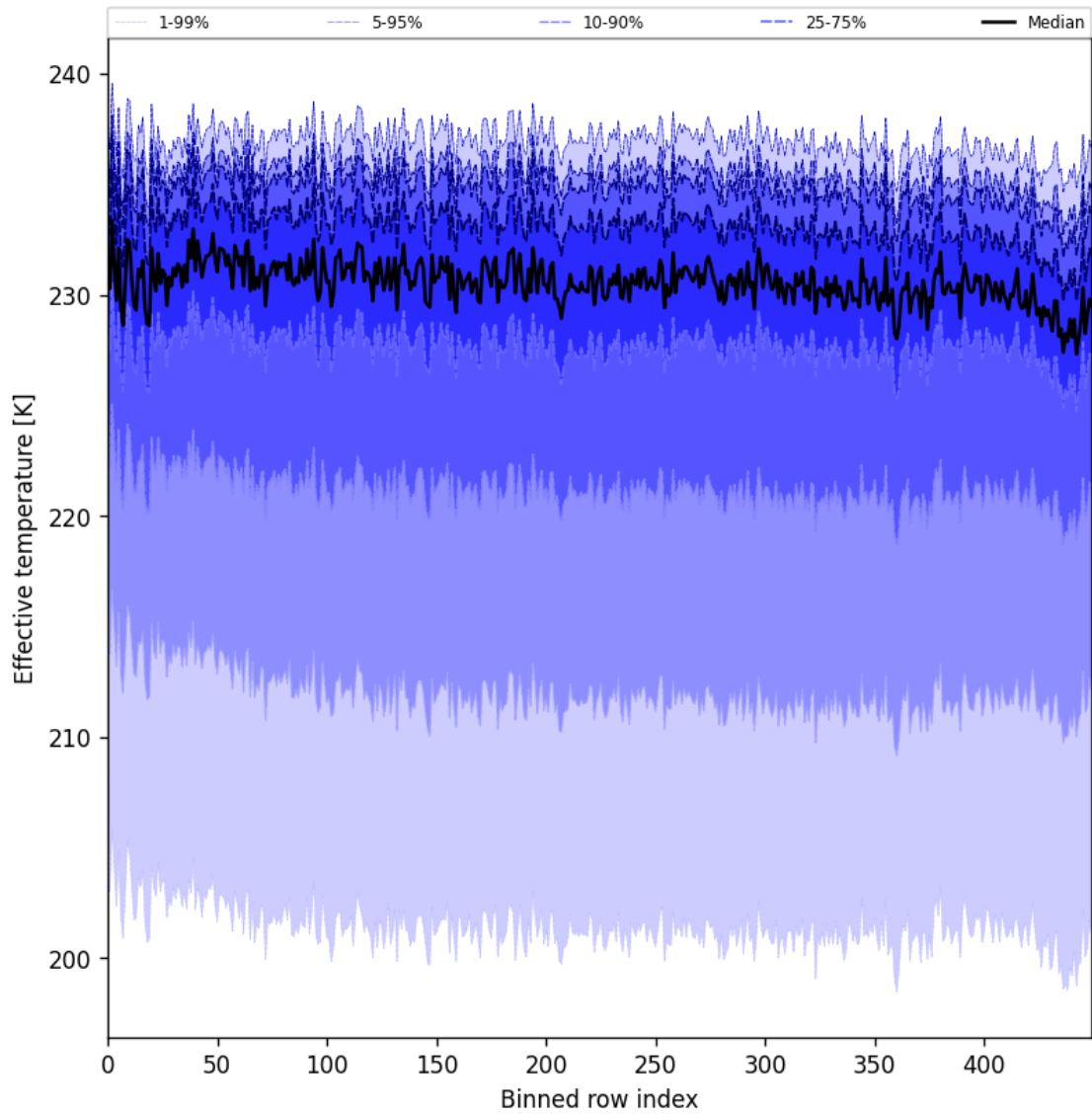
Figure 31: Along track statistics of “Effective temperature” for 2025-02-18 to 2025-02-19
