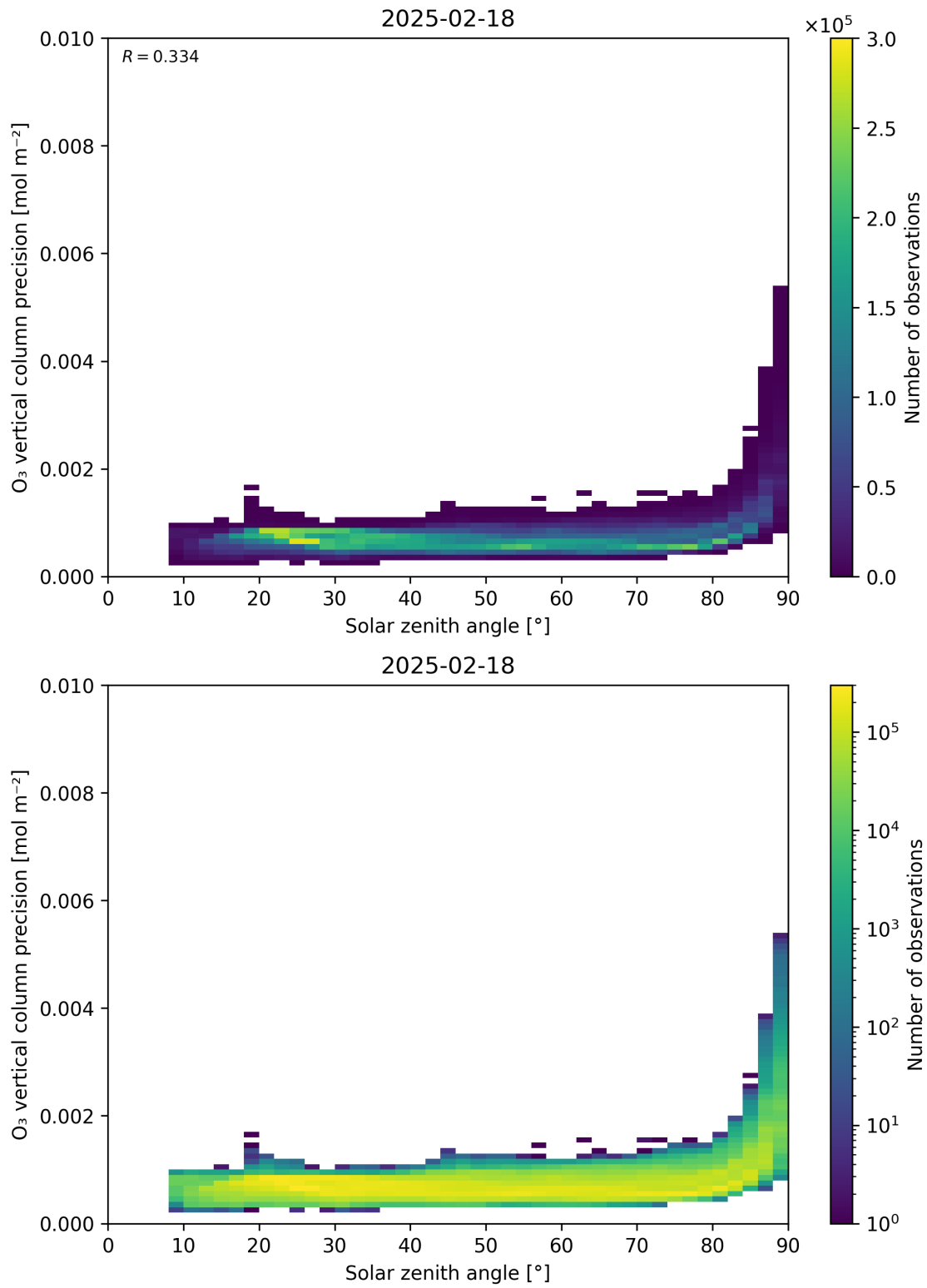
Figure 48: Scatter density plot of “Solar zenith angle” against “O 3 vertical column precision” for 2025-02-18 to 2025-02-19.
