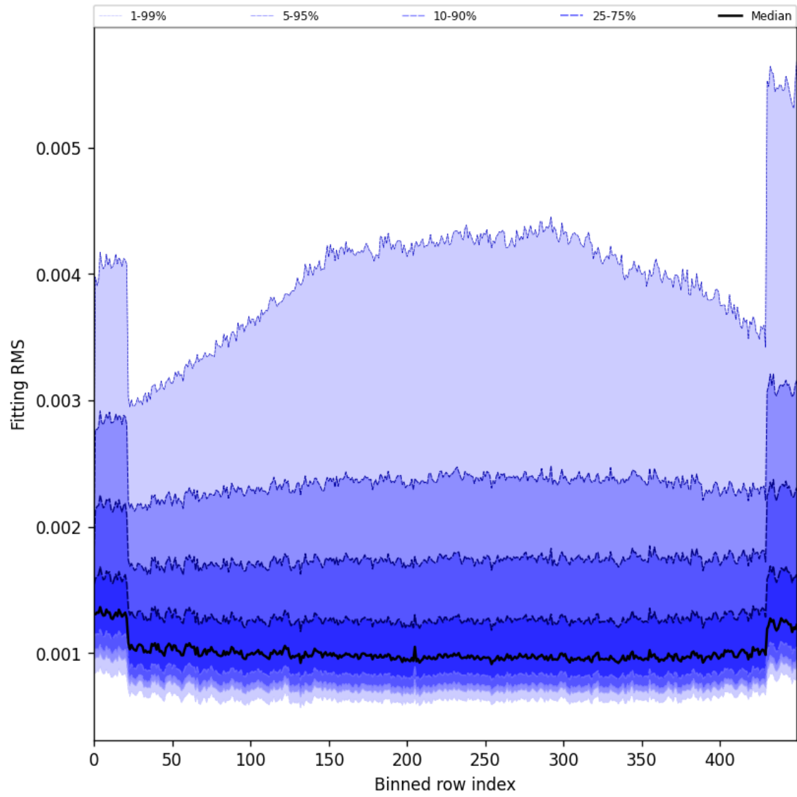
Figure 30: Along track statistics of “Fitting RMS” for 2025-02-18 to 2025-02-19
