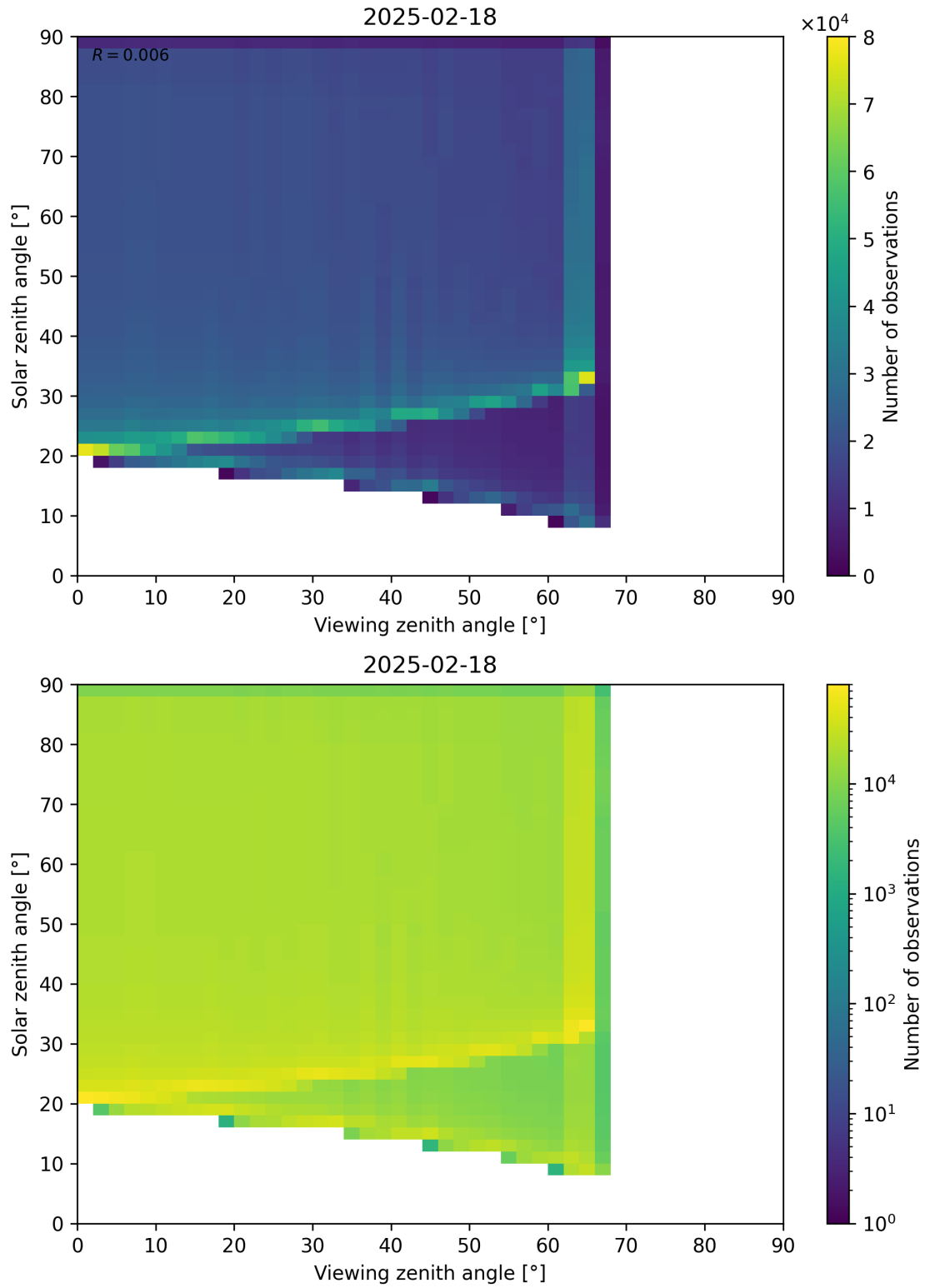
Figure 54: Scatter density plot of “Viewing zenith angle” against “Solar zenith angle” for 2025-02-18 to 2025-02-19.
