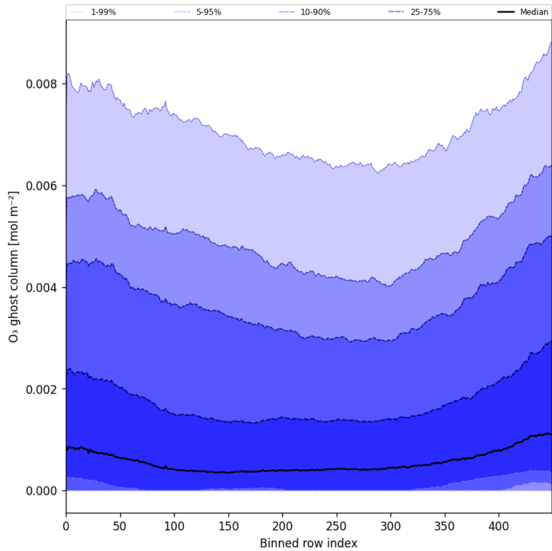
Figure 32: Along track statistics of “O 3 ghost column” for 2025-02-18 to 2025-02-19
