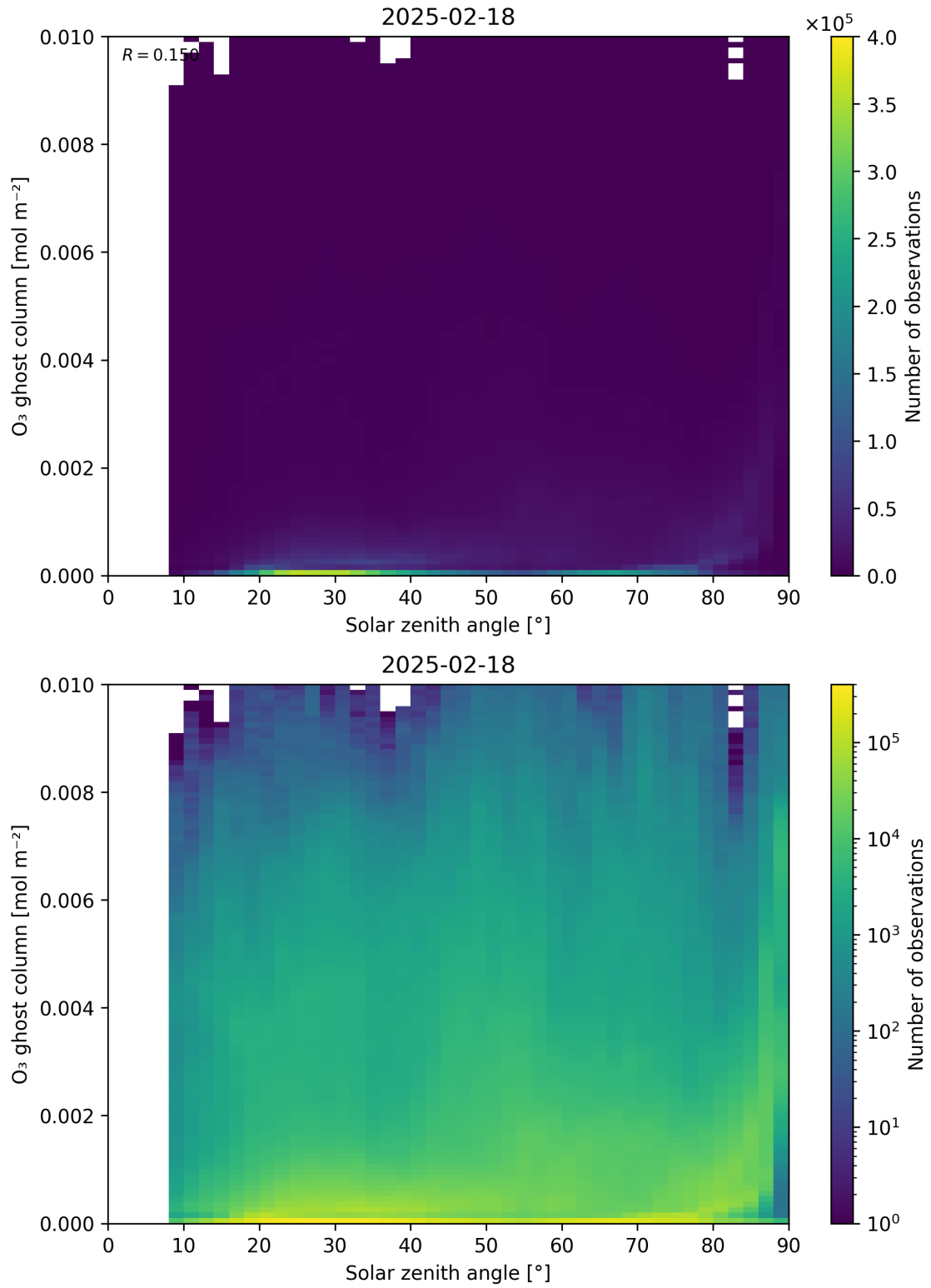
Figure 46: Scatter density plot of “Solar zenith angle” against “O 3 ghost column” for 2025-02-18 to 2025-02-19.
