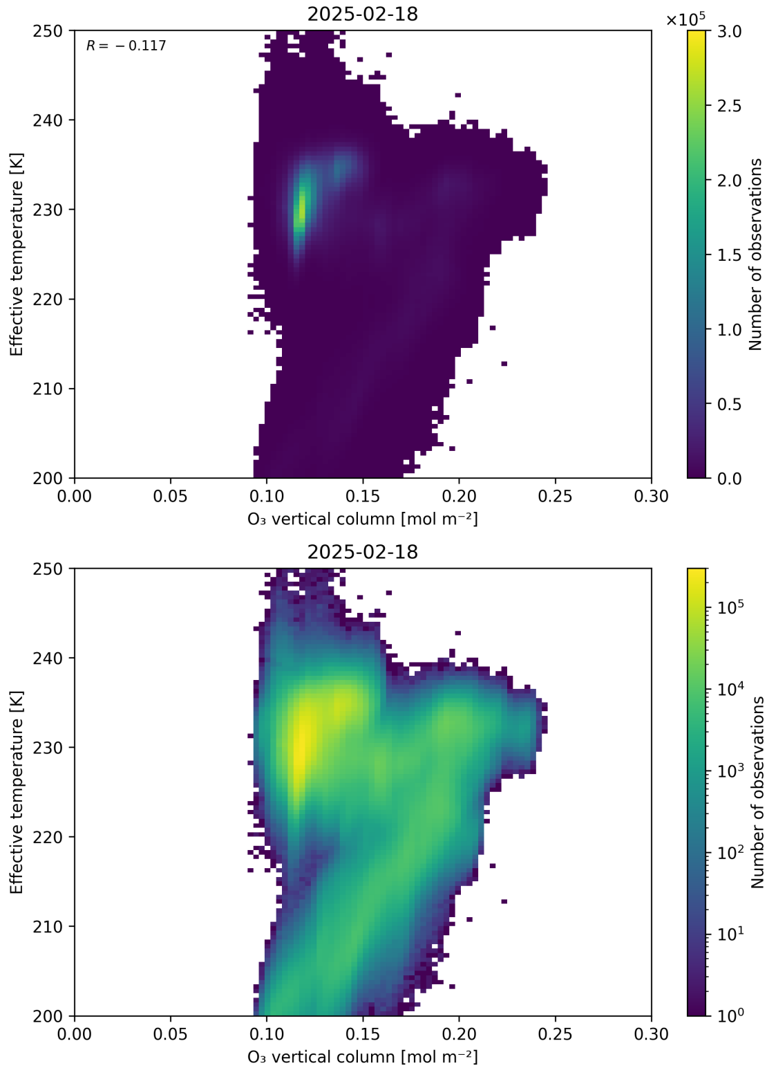
Figure 39: Scatter density plot of “O 3 vertical column” against “Effective temperature” for 2025-02-18 to 2025-02-19.
