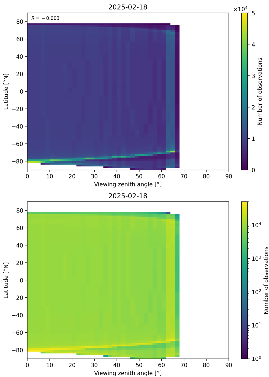
Figure 49: Scatter density plot of “Viewing zenith angle” against “Latitude” for 2025-02-18 to 2025-02-19.
