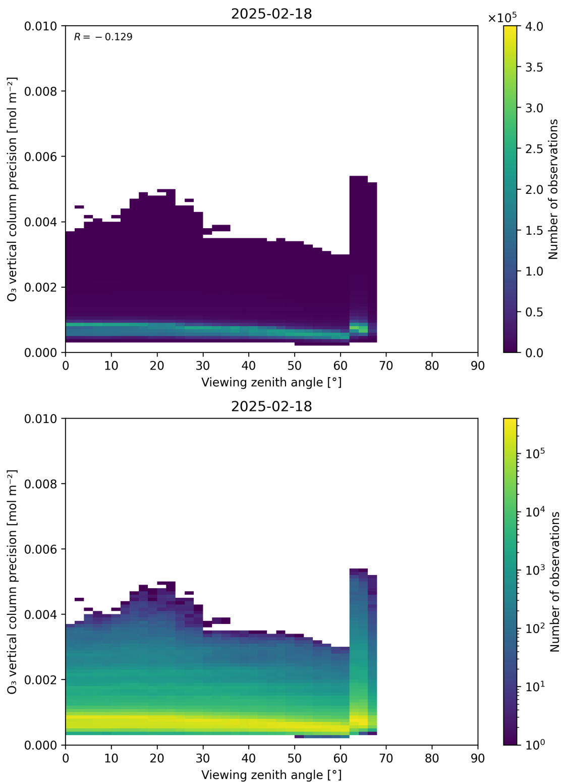
Figure 53: Scatter density plot of “Viewing zenith angle” against “O 3 vertical column precision” for 2025-02-18 to 2025-02-19.
