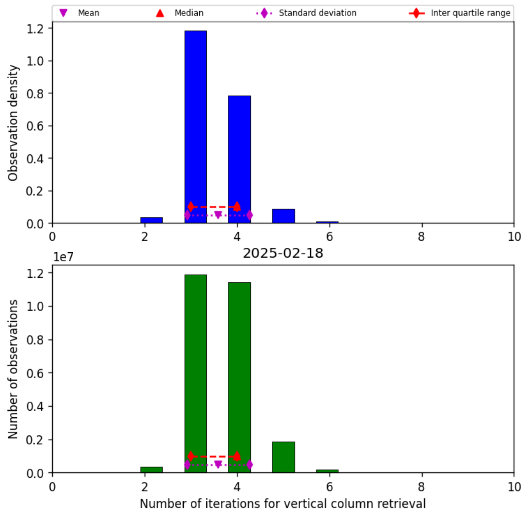
Figure 26: Histogram of “Number of iterations for vertical column retrieval” for 2025-02-18 to 2025-02-19
