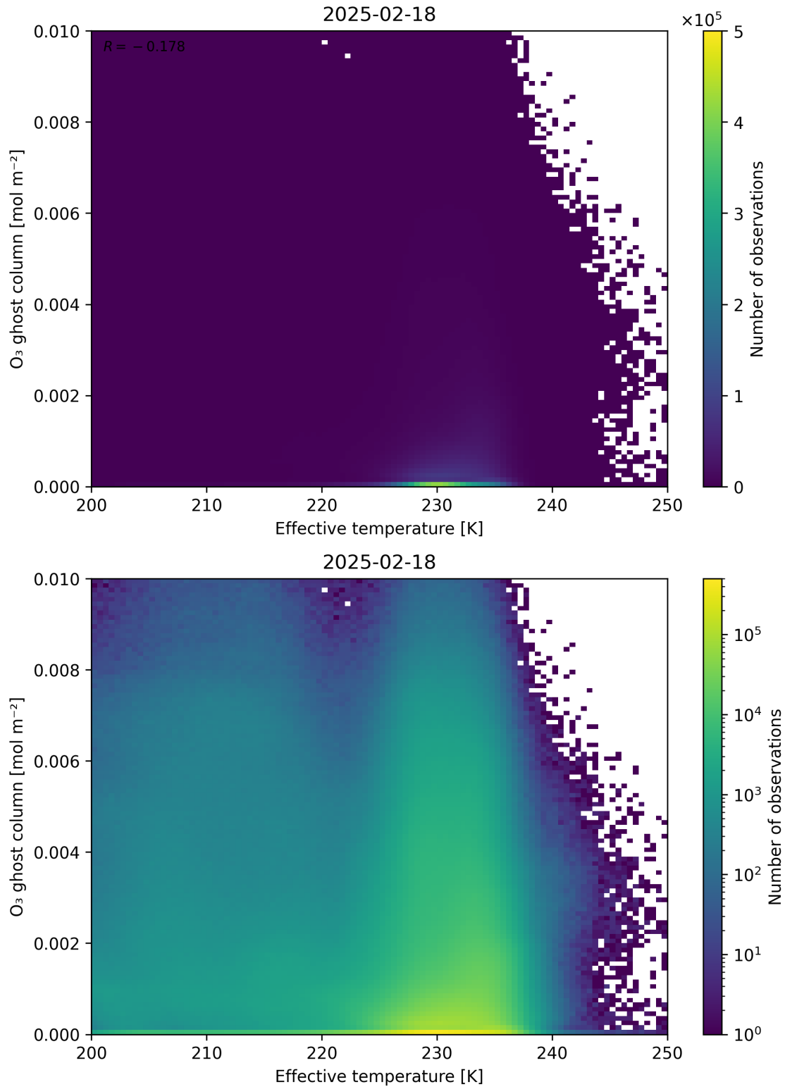
Figure 38: Scatter density plot of “Effective temperature” against “O 3 ghost column” for 2025-02-18 to 2025-02-19.
