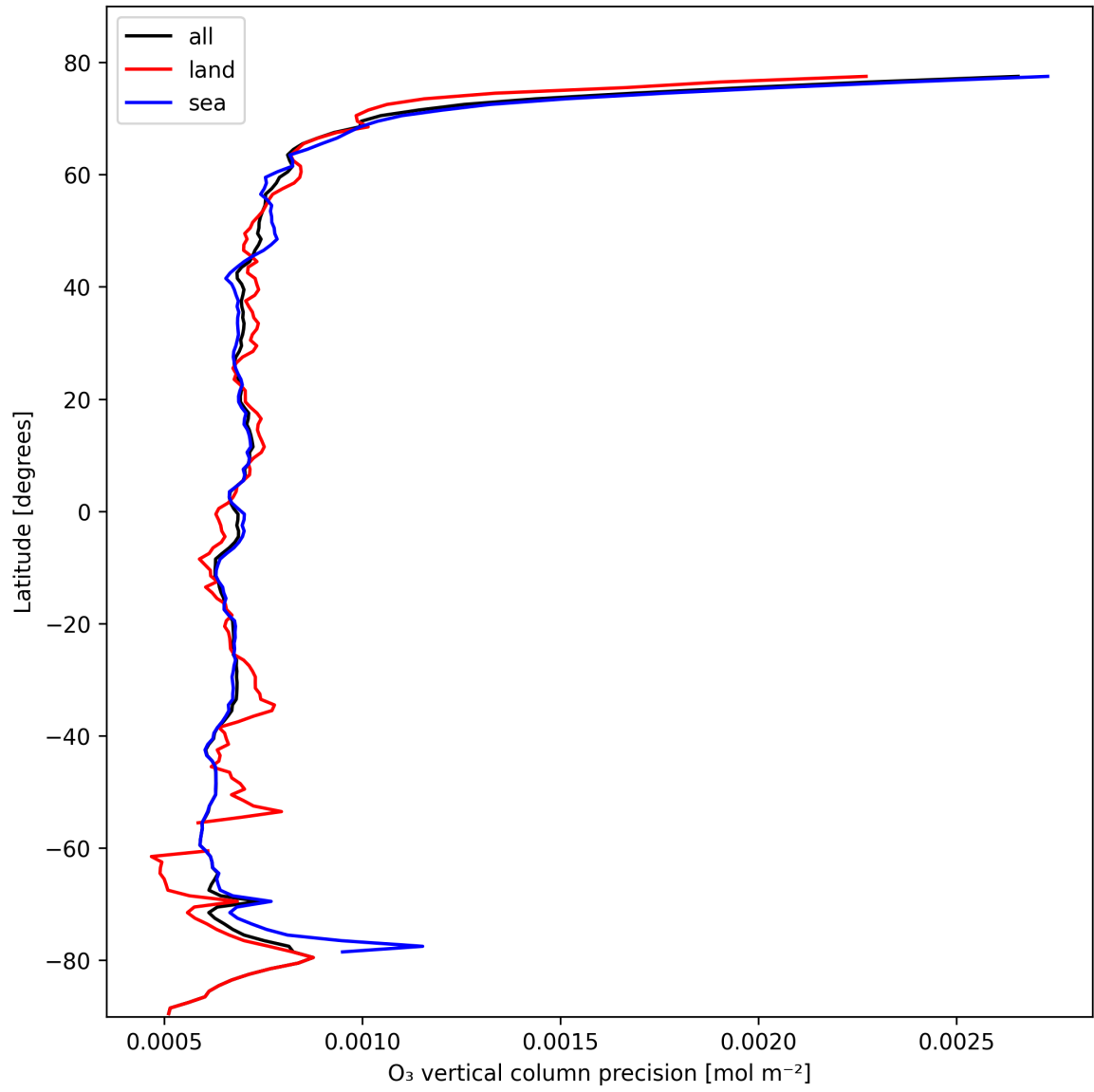
Figure 15: Zonal average of “O 3 vertical column precision” for 2025-02-18 to 2025-02-19.
