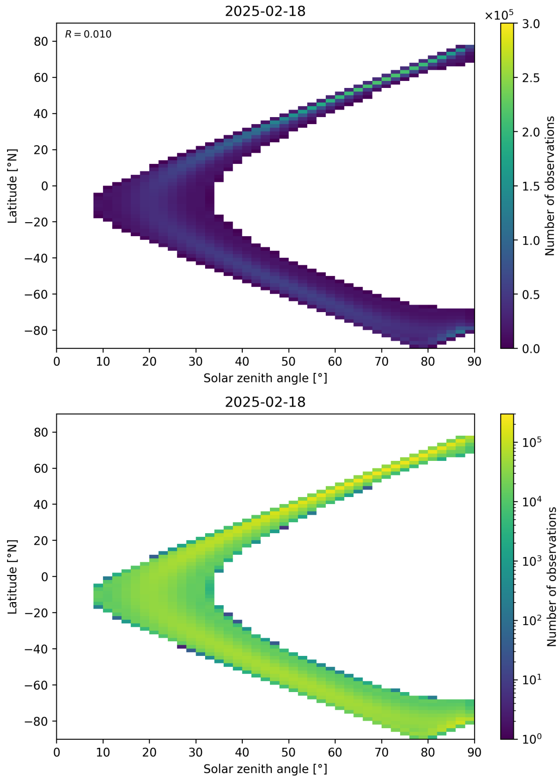
Figure 44: Scatter density plot of “Solar zenith angle” against “Latitude” for 2025-02-18 to 2025-02-19.
