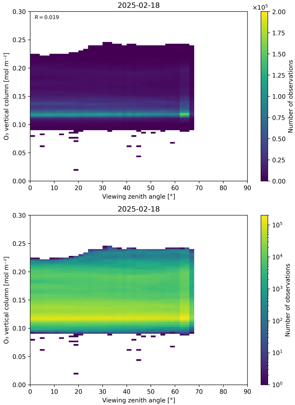
Figure 52: Scatter density plot of “Viewing zenith angle” against “O 3 vertical column” for 2025-02-18 to 2025-02-19.
