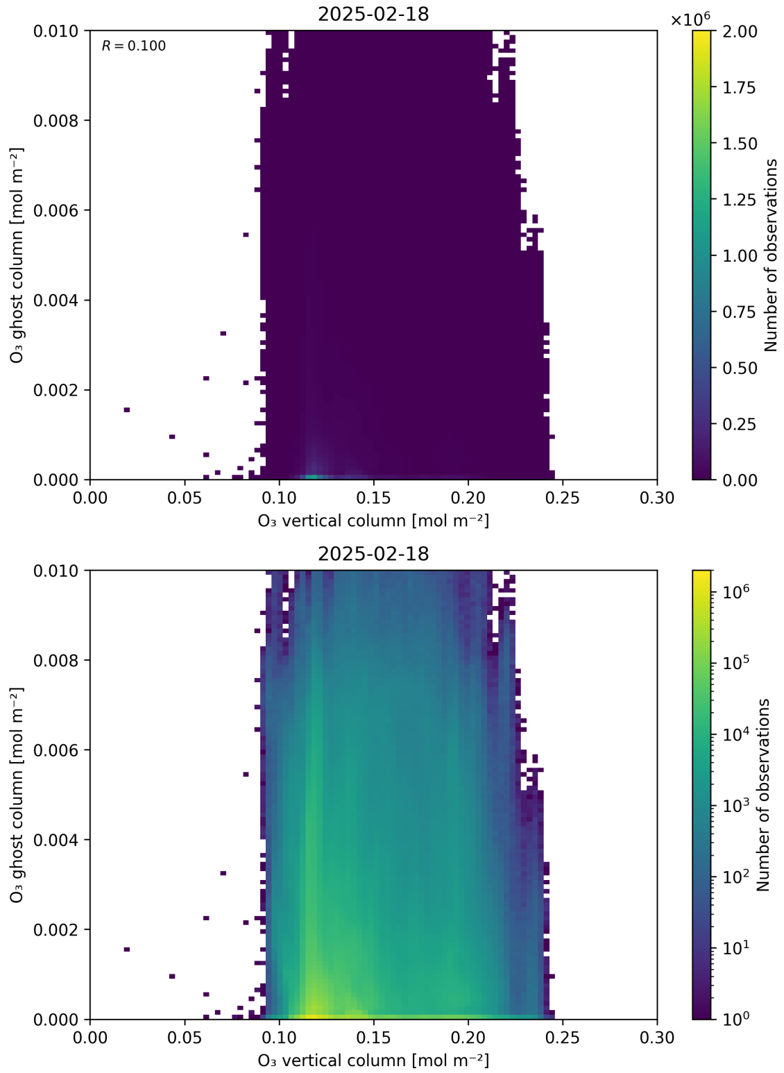
Figure 40: Scatter density plot of “O 3 vertical column” against “O 3 ghost column” for 2025-02-18 to 2025-02-19.
