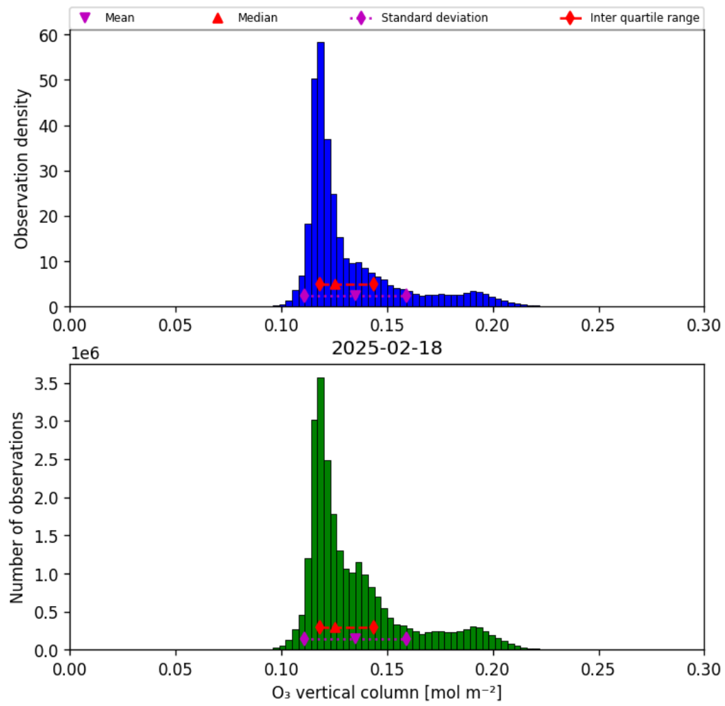
Figure 21: Histogram of “O 3 vertical column” for 2025-02-18 to 2025-02-19
