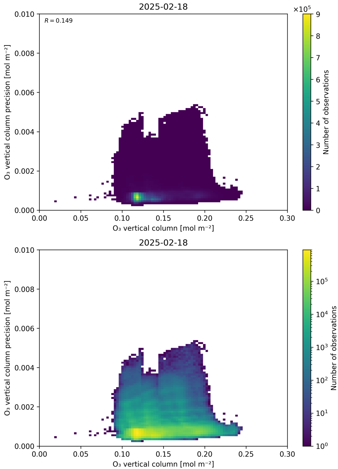
Figure 41: Scatter density plot of “O 3 vertical column” against “O 3 vertical column precision” for 2025-02-18 to 2025-02-19.
