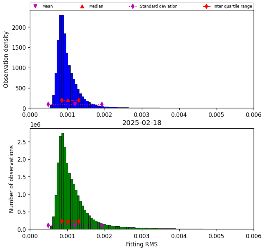
Figure 23: Histogram of “Fitting RMS” for 2025-02-18 to 2025-02-19
