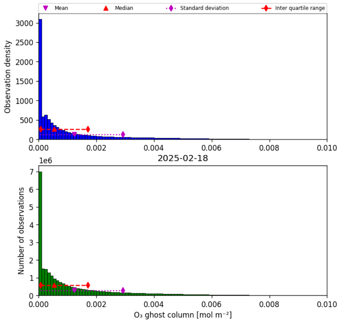
Figure 25: Histogram of “O 3 ghost column” for 2025-02-18 to 2025-02-19
