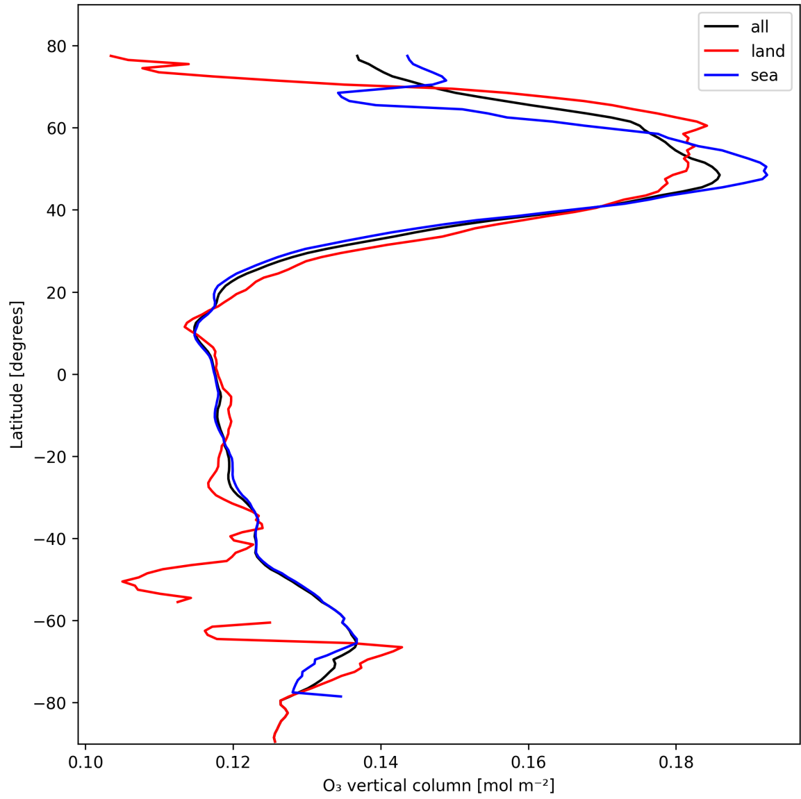
Figure 14: Zonal average of “O 3 vertical column” for 2025-02-18 to 2025-02-19.
