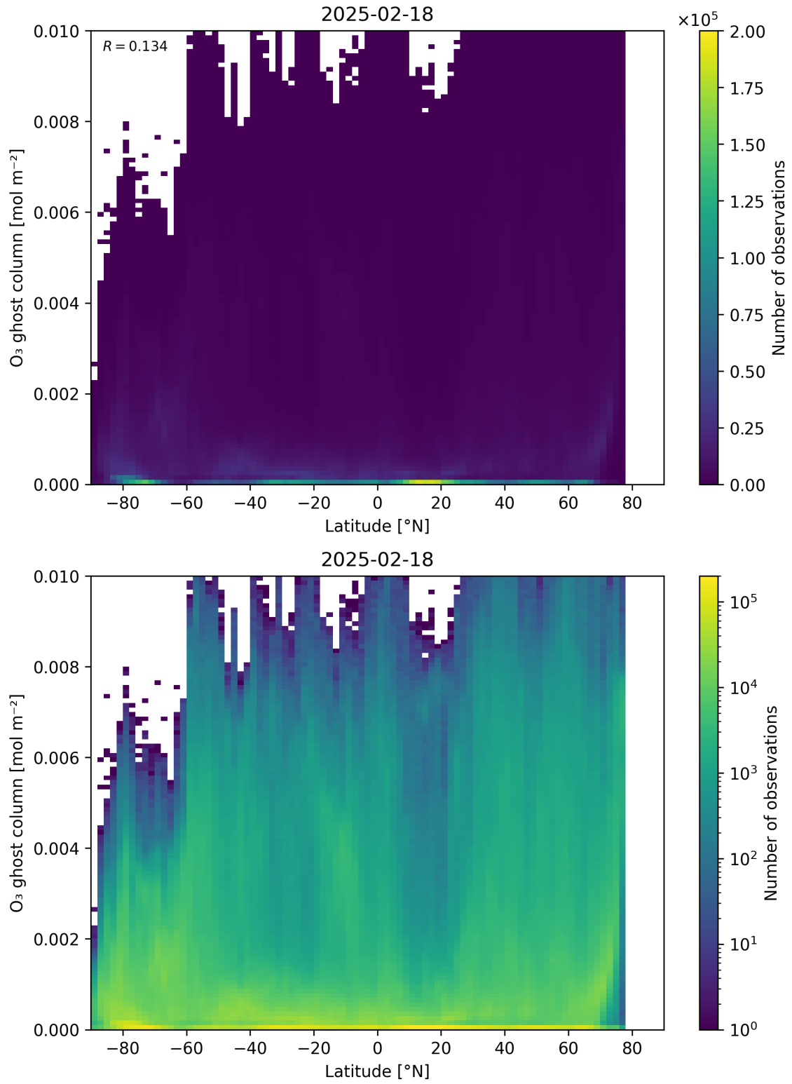
Figure 35: Scatter density plot of “Latitude” against “O 3 ghost column” for 2025-02-18 to 2025-02-19.
