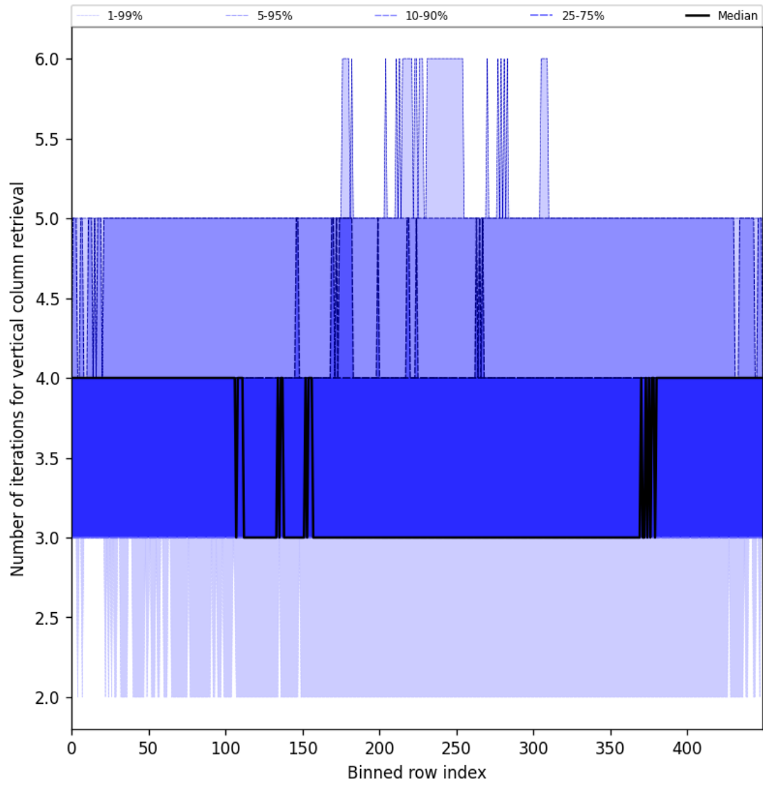
Figure 33: Along track statistics of “Number of iterations for vertical column retrieval” for 2025-02-18 to 2025-02-19
