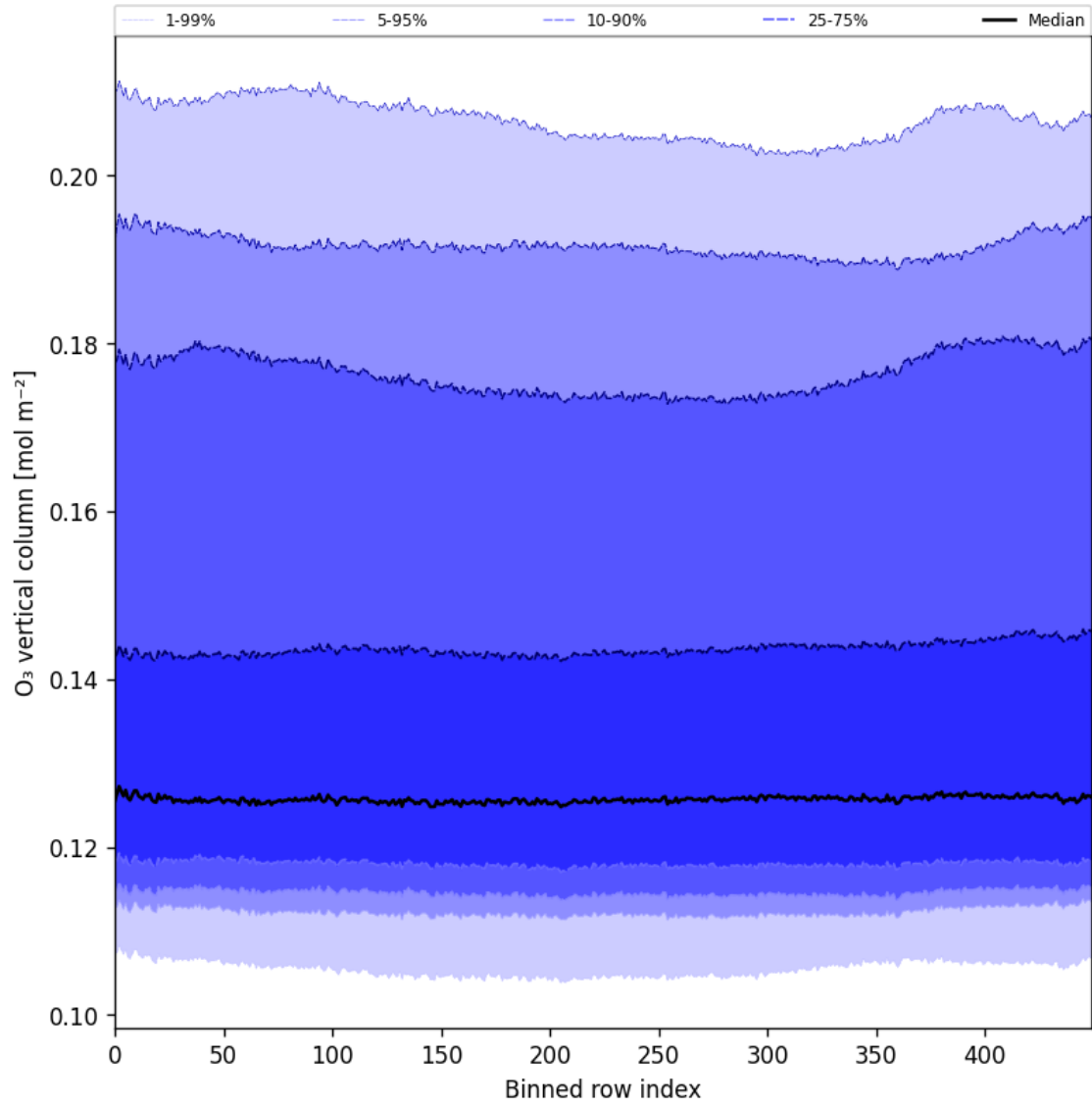
Figure 28: Along track statistics of “O 3 vertical column” for 2025-02-18 to 2025-02-19
