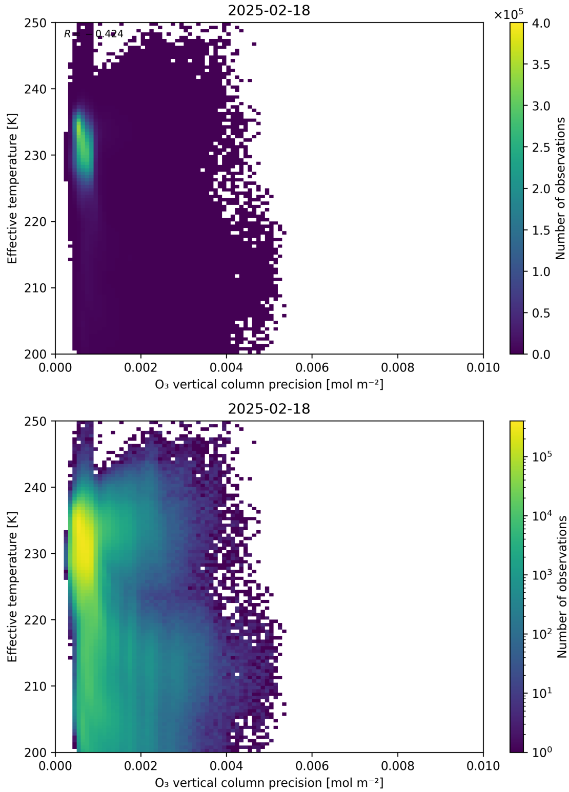
Figure 42: Scatter density plot of “O 3 vertical column precision” against “Effective temperature” for 2025-02-18 to 2025-02-19.
