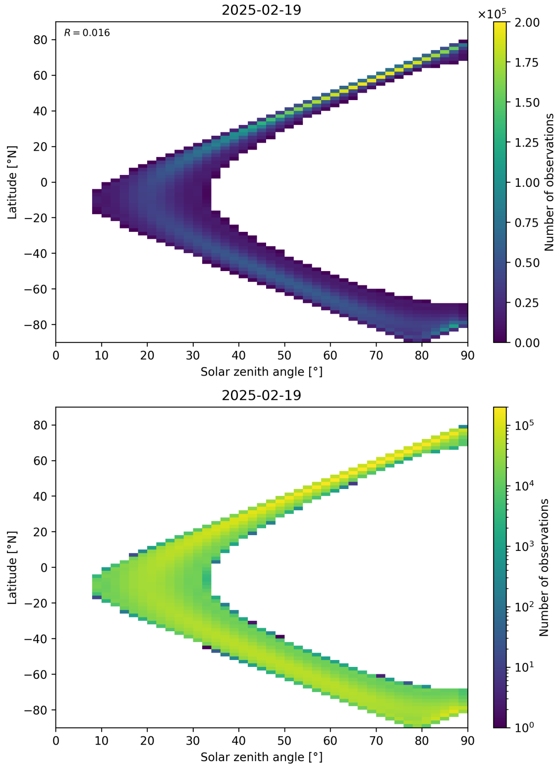
Figure 44: Scatter density plot of “Solar zenith angle” against “Latitude” for 2025-02-19 to 2025-02-20.
