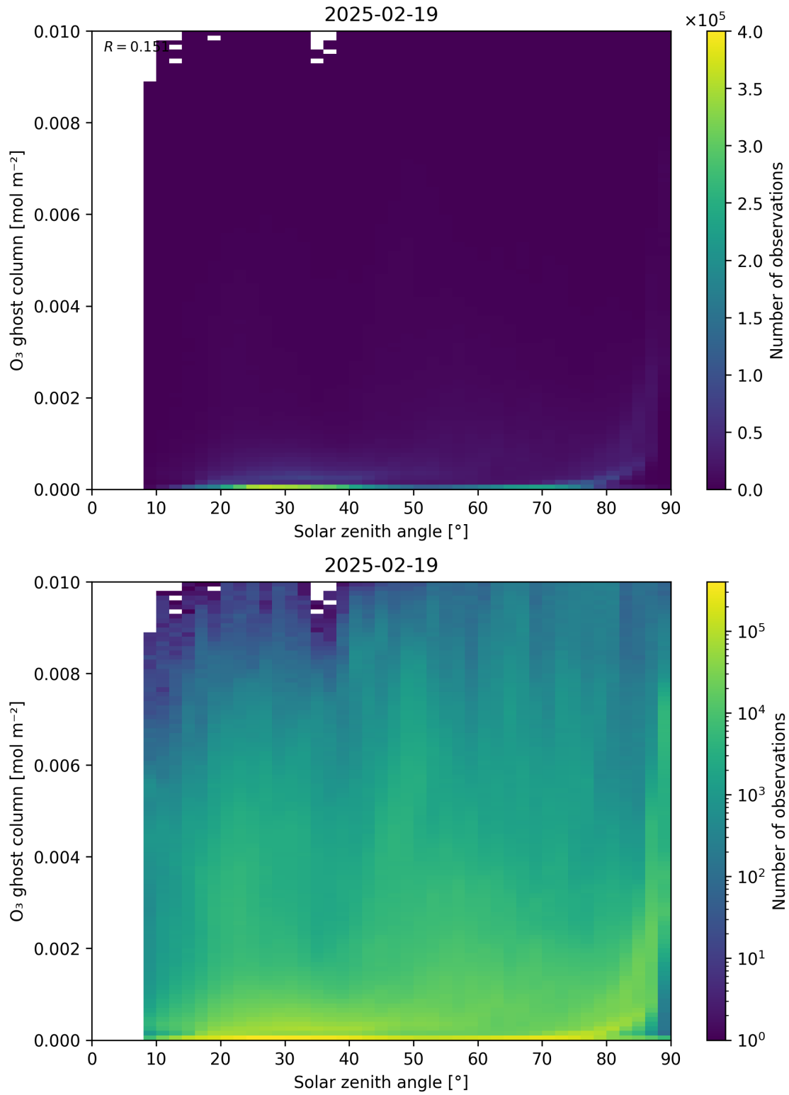
Figure 46: Scatter density plot of “Solar zenith angle” against “O 3 ghost column” for 2025-02-19 to 2025-02-20.
