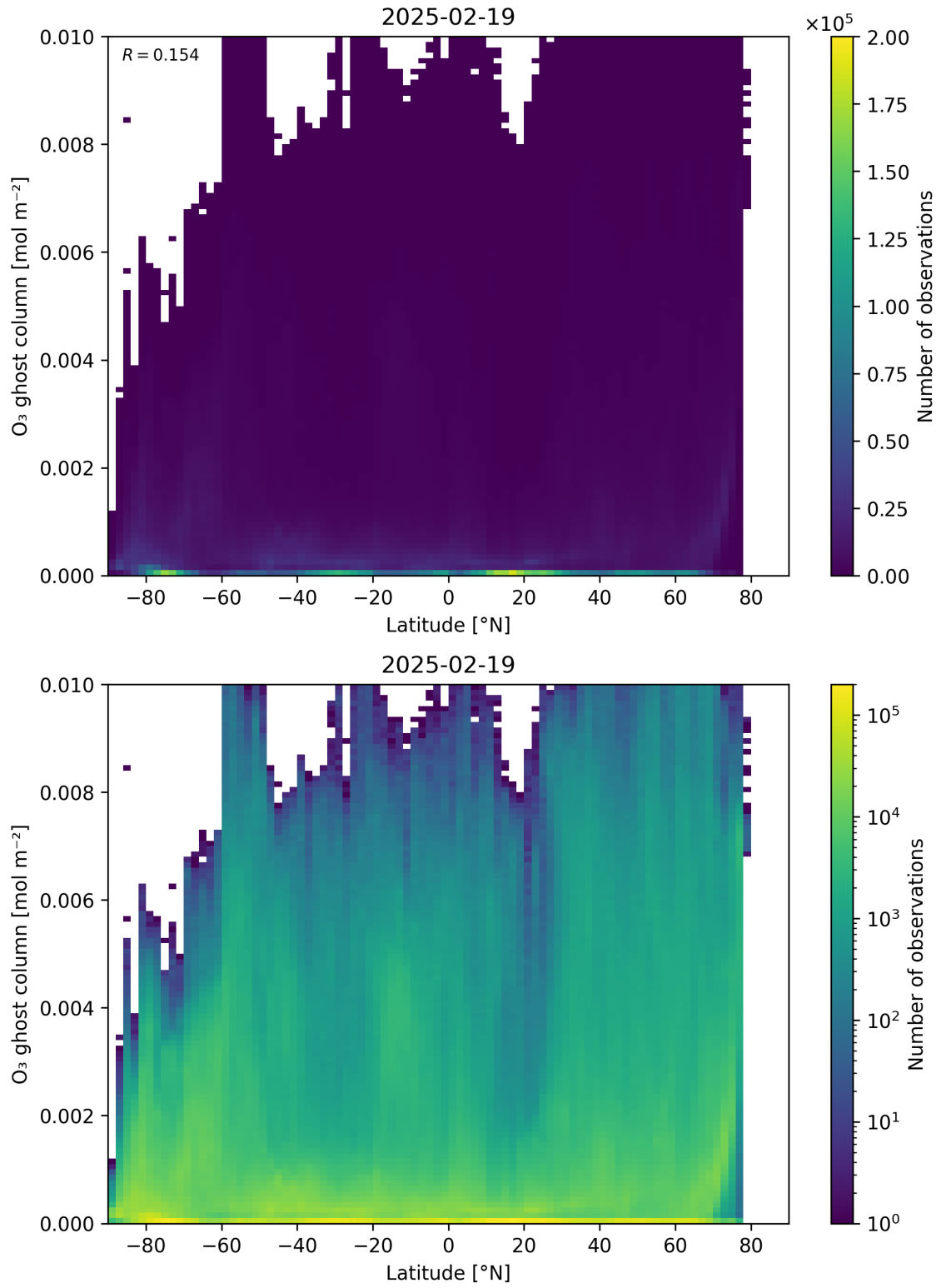
Figure 35: Scatter density plot of “Latitude” against “O 3 ghost column” for 2025-02-19 to 2025-02-20.
