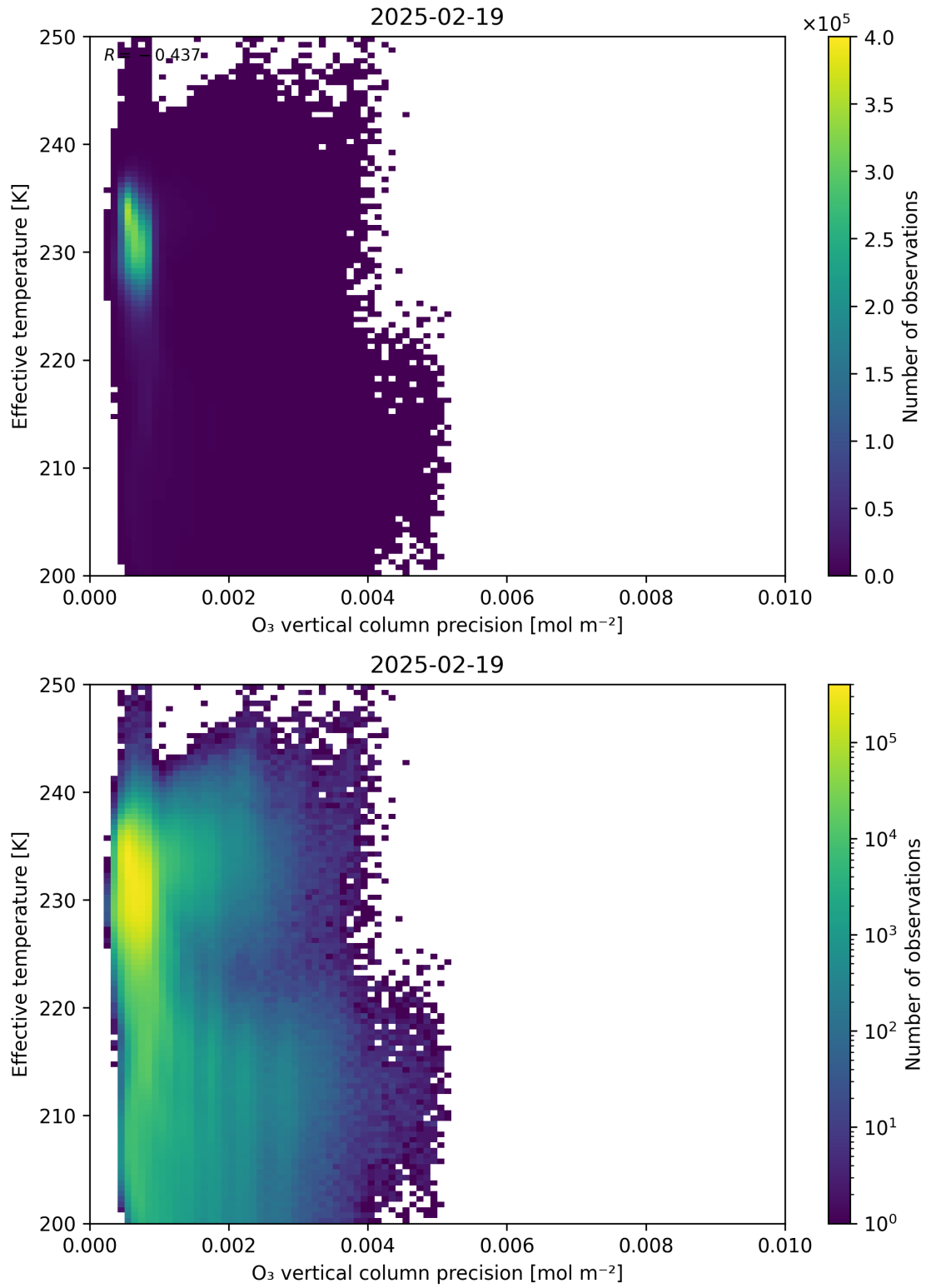
Figure 42: Scatter density plot of “O 3 vertical column precision” against “Effective temperature” for 2025-02-19 to 2025-02-20.
