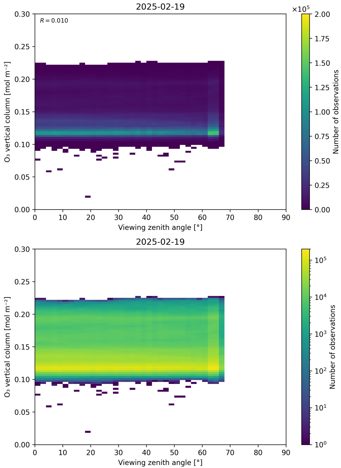
Figure 52: Scatter density plot of “Viewing zenith angle” against “O 3 vertical column” for 2025-02-19 to 2025-02-20.
