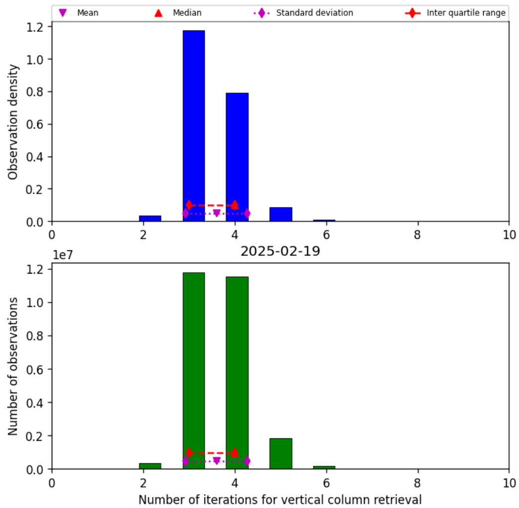
Figure 26: Histogram of “Number of iterations for vertical column retrieval” for 2025-02-19 to 2025-02-20
