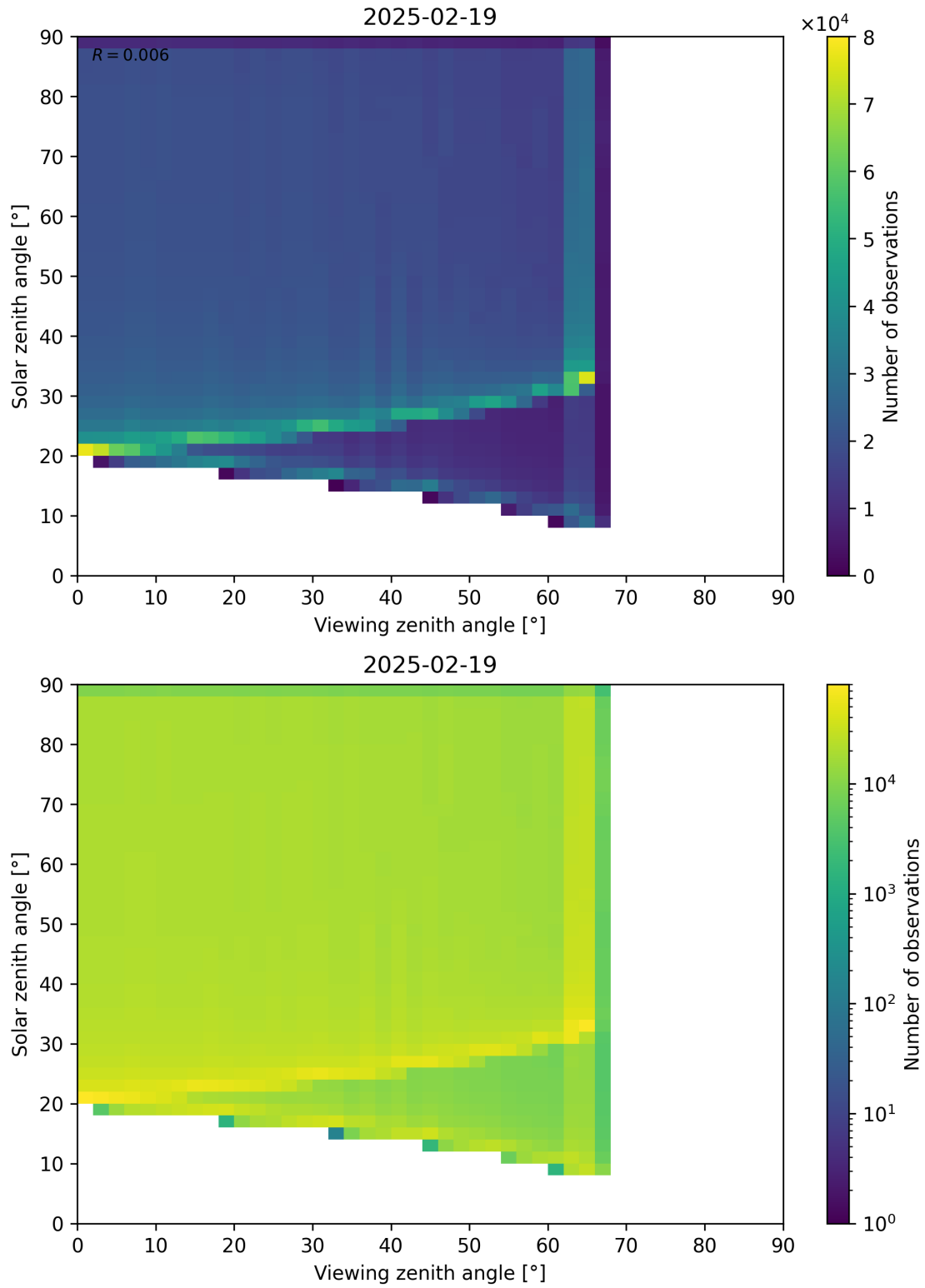
Figure 54: Scatter density plot of “Viewing zenith angle” against “Solar zenith angle” for 2025-02-19 to 2025-02-20.
