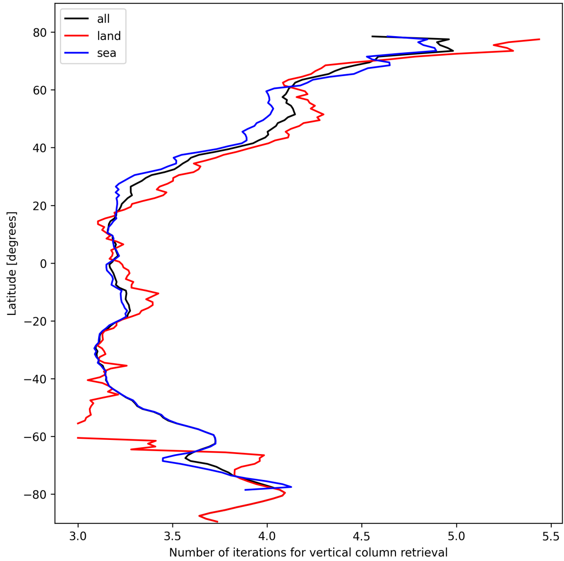
Figure 19: Zonal average of “Number of iterations for vertical column retrieval” for 2025-02-19 to 2025-02-20.
