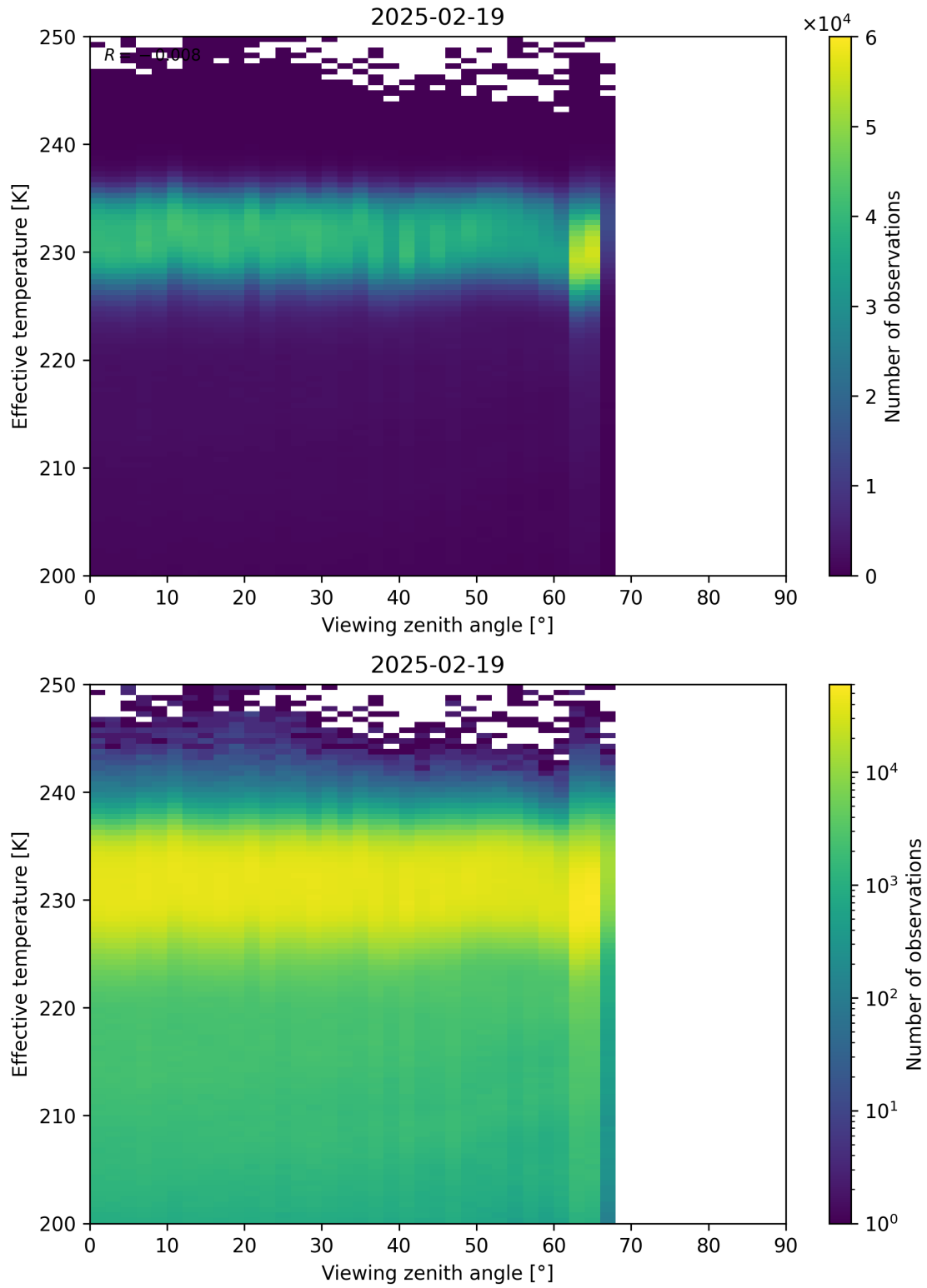
Figure 50: Scatter density plot of “Viewing zenith angle” against “Effective temperature” for 2025-02-19 to 2025-02-20.
