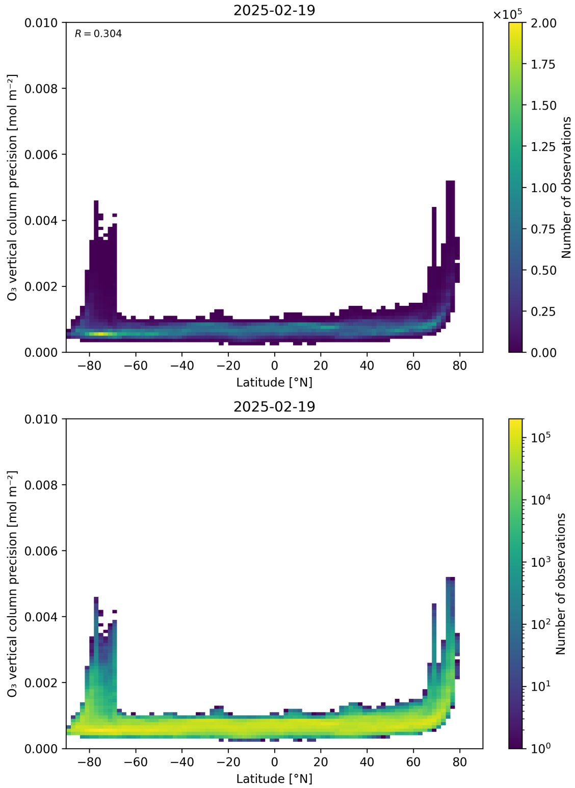
Figure 37: Scatter density plot of “Latitude” against “O 3 vertical column precision” for 2025-02-19 to 2025-02-20.
