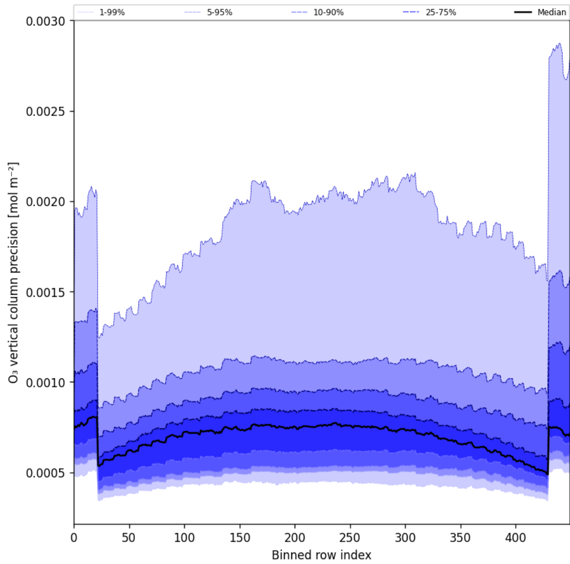
Figure 29: Along track statistics of “O 3 vertical column precision” for 2025-02-19 to 2025-02-20
