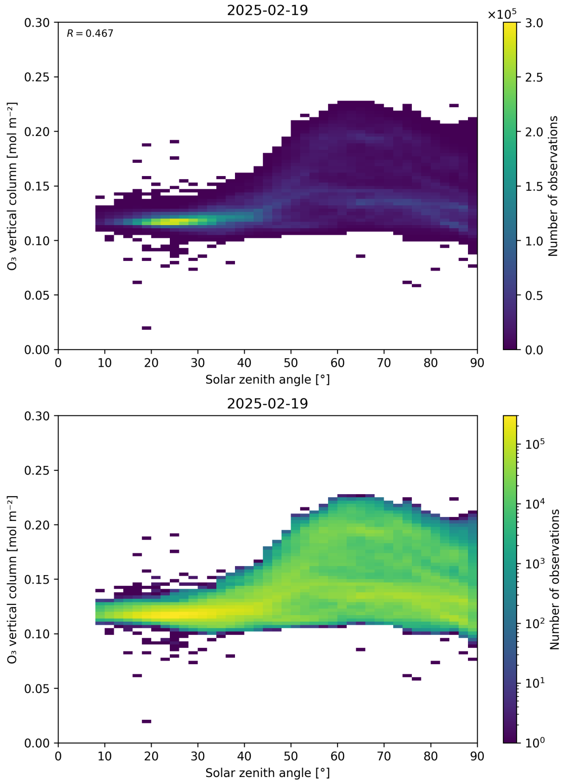
Figure 47: Scatter density plot of “Solar zenith angle” against “O 3 vertical column” for 2025-02-19 to 2025-02-20.
