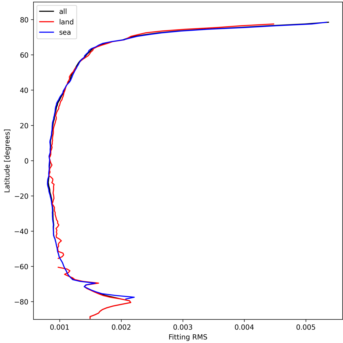
Figure 16: Zonal average of “Fitting RMS” for 2025-02-19 to 2025-02-20.
