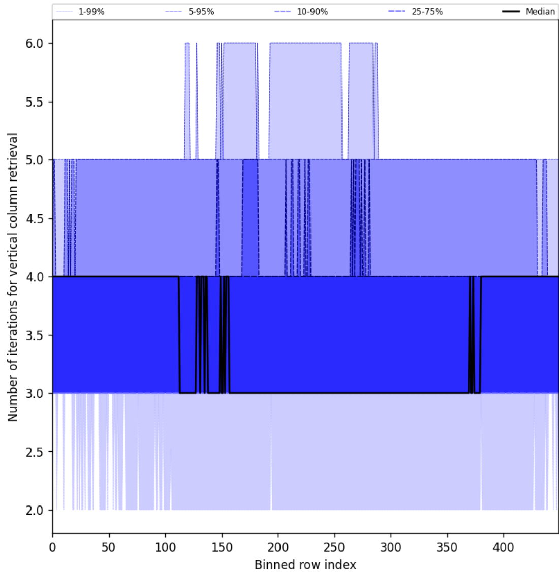
Figure 33: Along track statistics of “Number of iterations for vertical column retrieval” for 2025-02-19 to 2025-02-20
