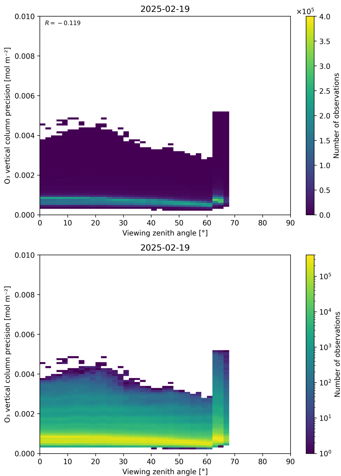
Figure 53: Scatter density plot of “Viewing zenith angle” against “O 3 vertical column precision” for 2025-02-19 to 2025-02-20.
