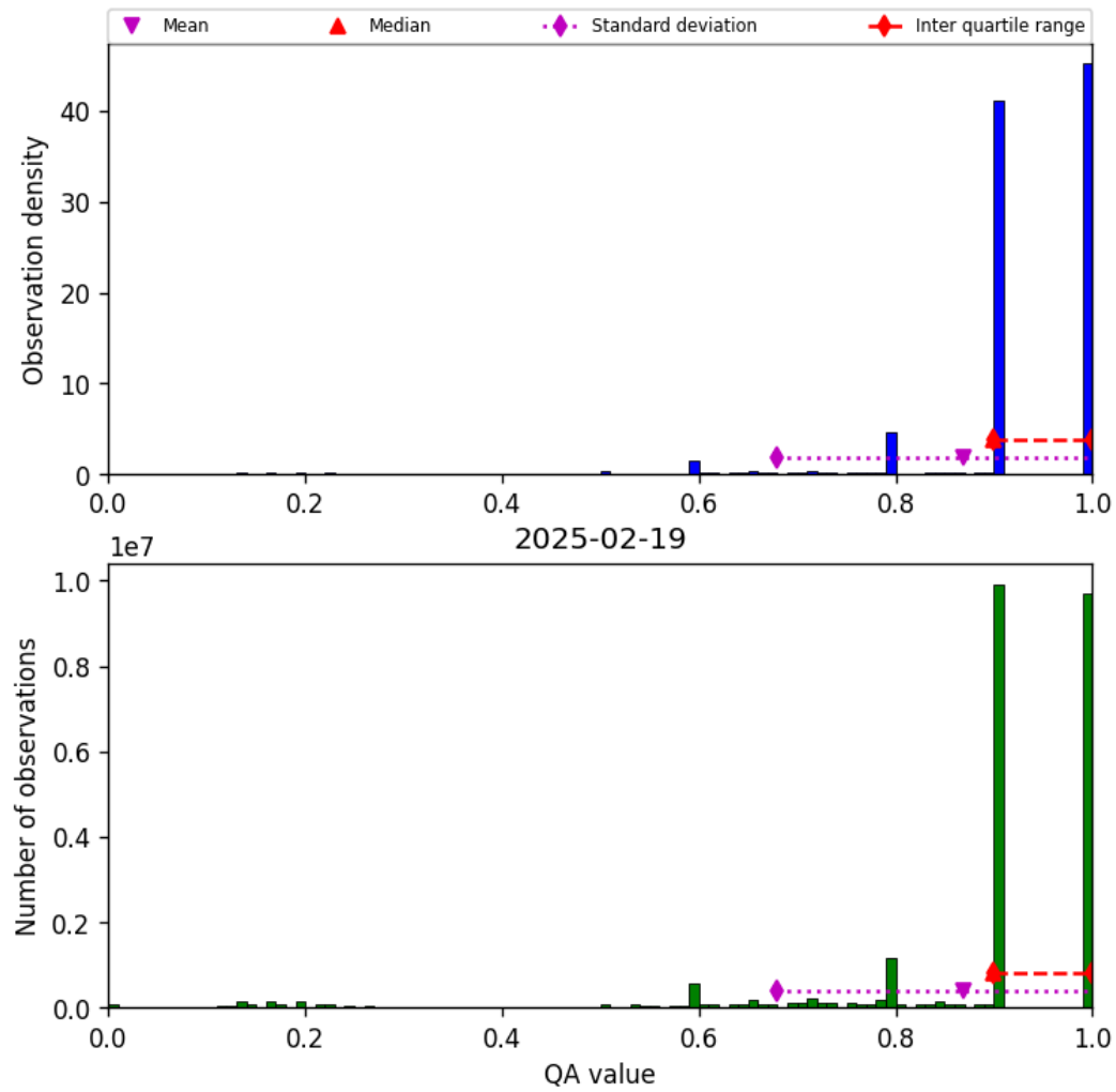
Figure 20: Histogram of “QA value” for 2025-02-19 to 2025-02-20
