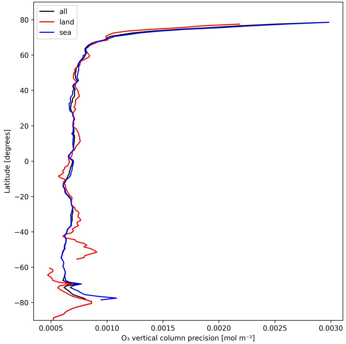
Figure 15: Zonal average of "O 3 vertical column precision" for 2025-02-19 to 2025-02-20.
