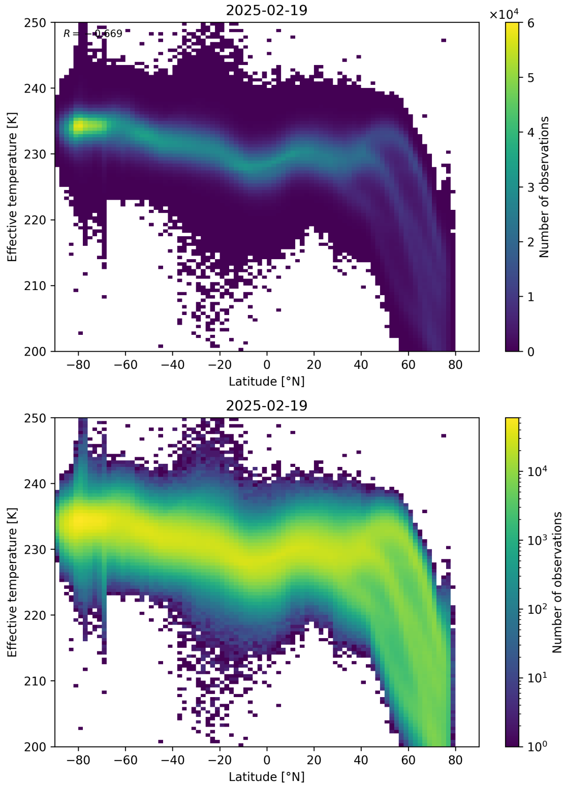
Figure 34: Scatter density plot of “Latitude” against “Effective temperature” for 2025-02-19 to 2025-02-20.
