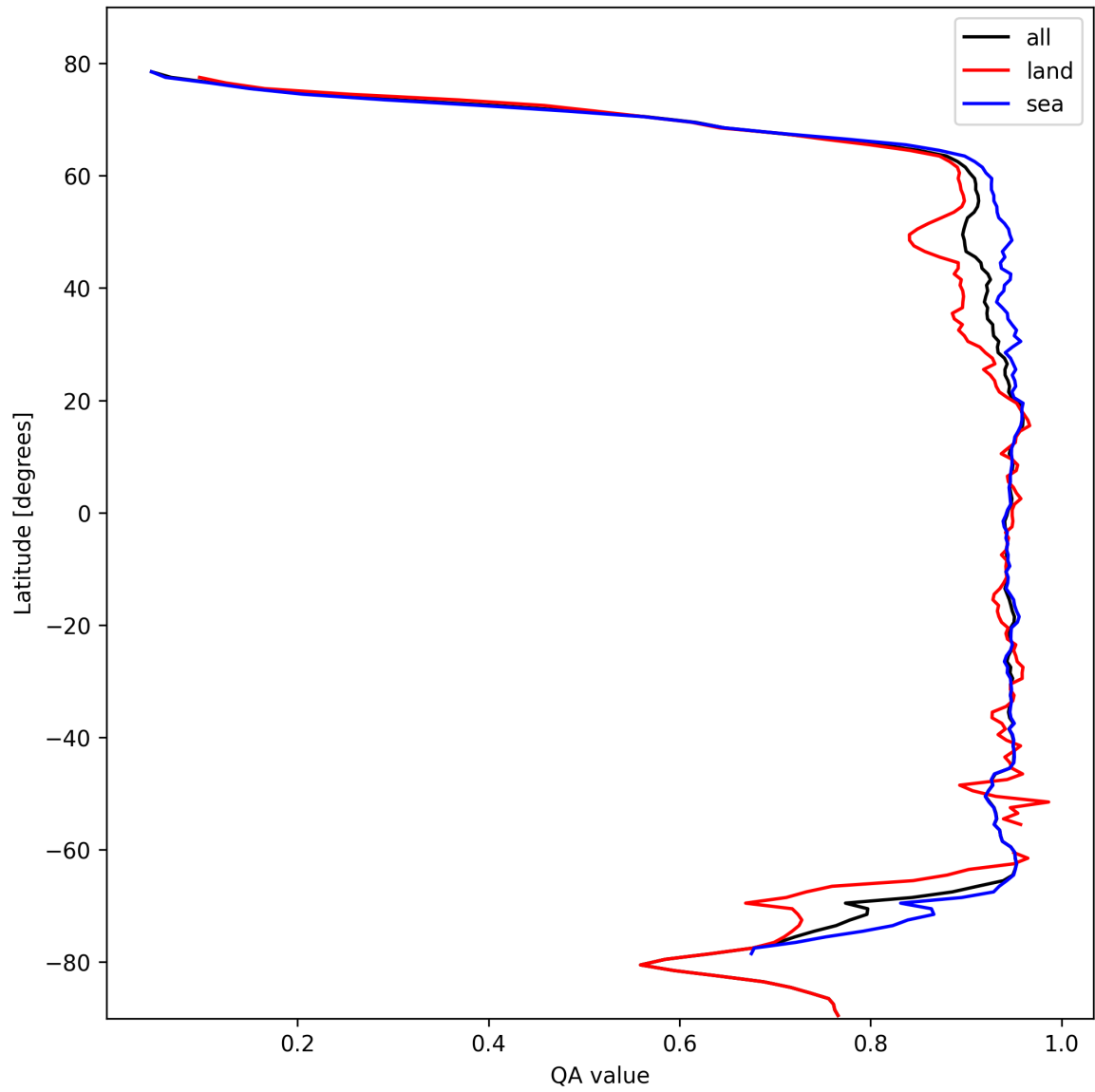
Figure 13: Zonal average of “QA value” for 2025-02-19 to 2025-02-20.
