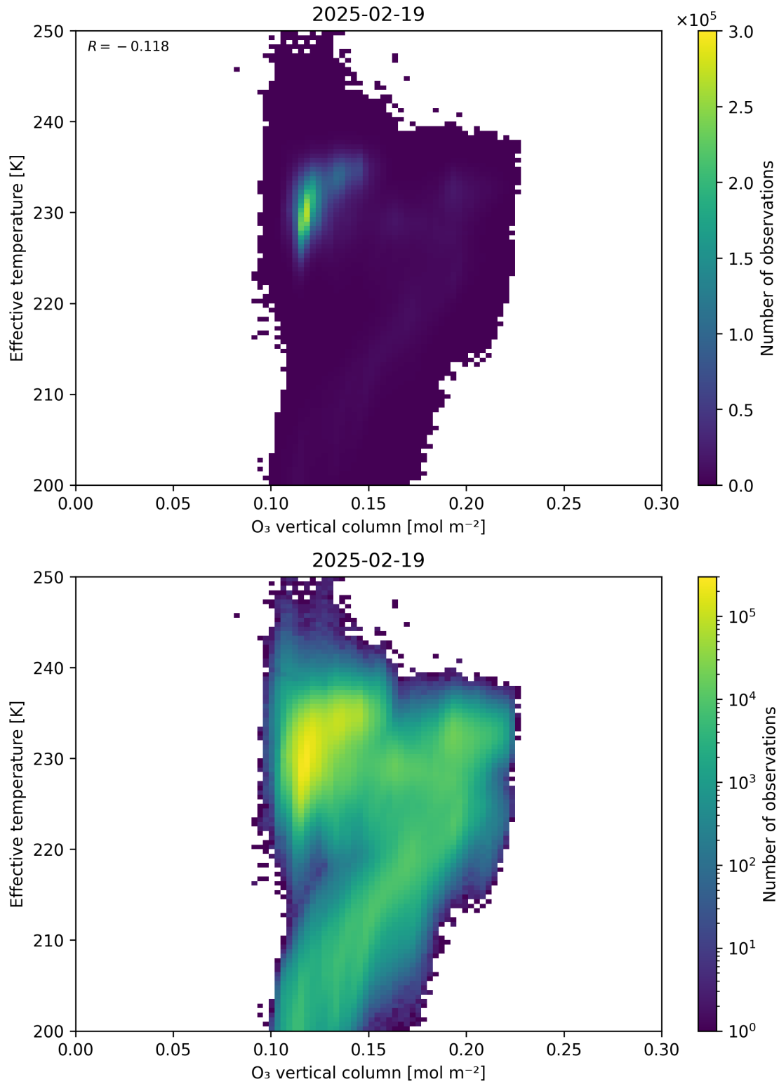
Figure 39: Scatter density plot of “O 3 vertical column” against “Effective temperature” for 2025-02-19 to 2025-02-20.
