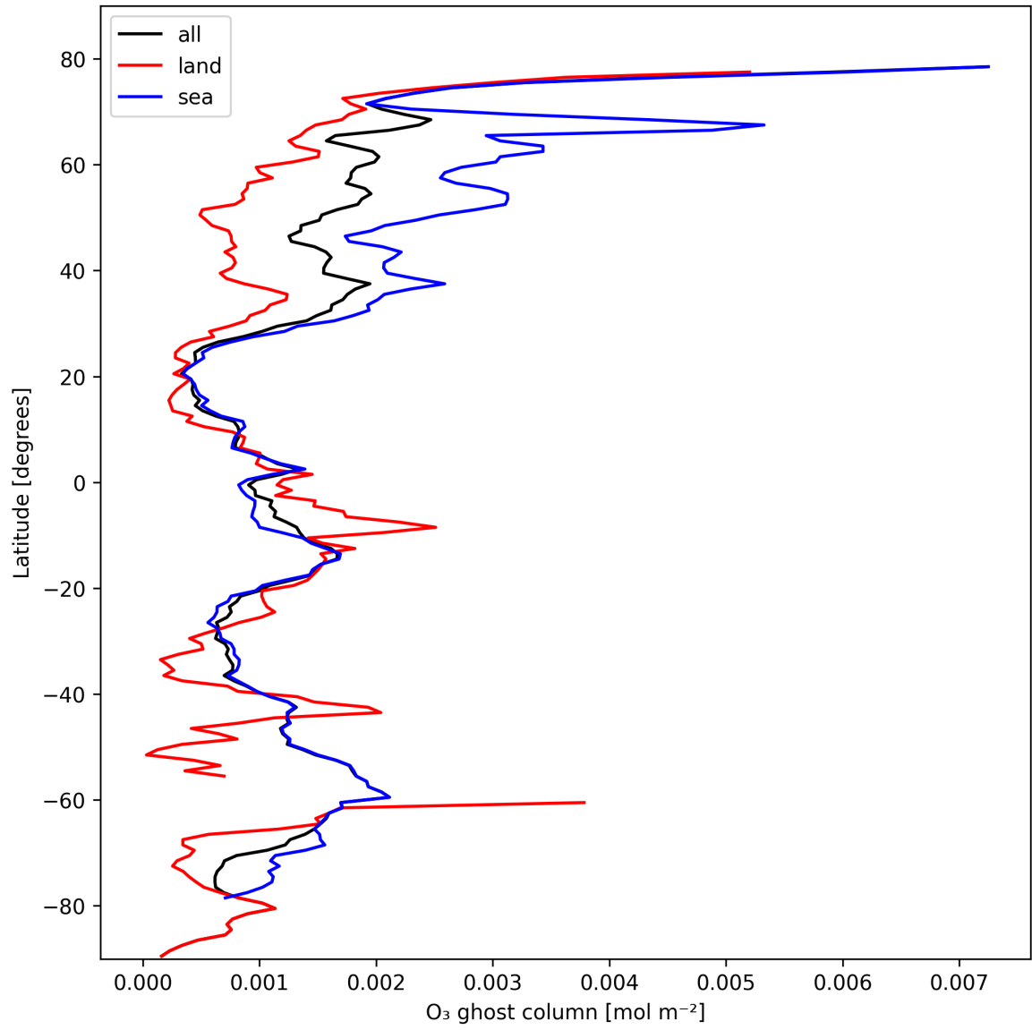
Figure 18: Zonal average of “O 3 ghost column” for 2025-02-19 to 2025-02-20.
