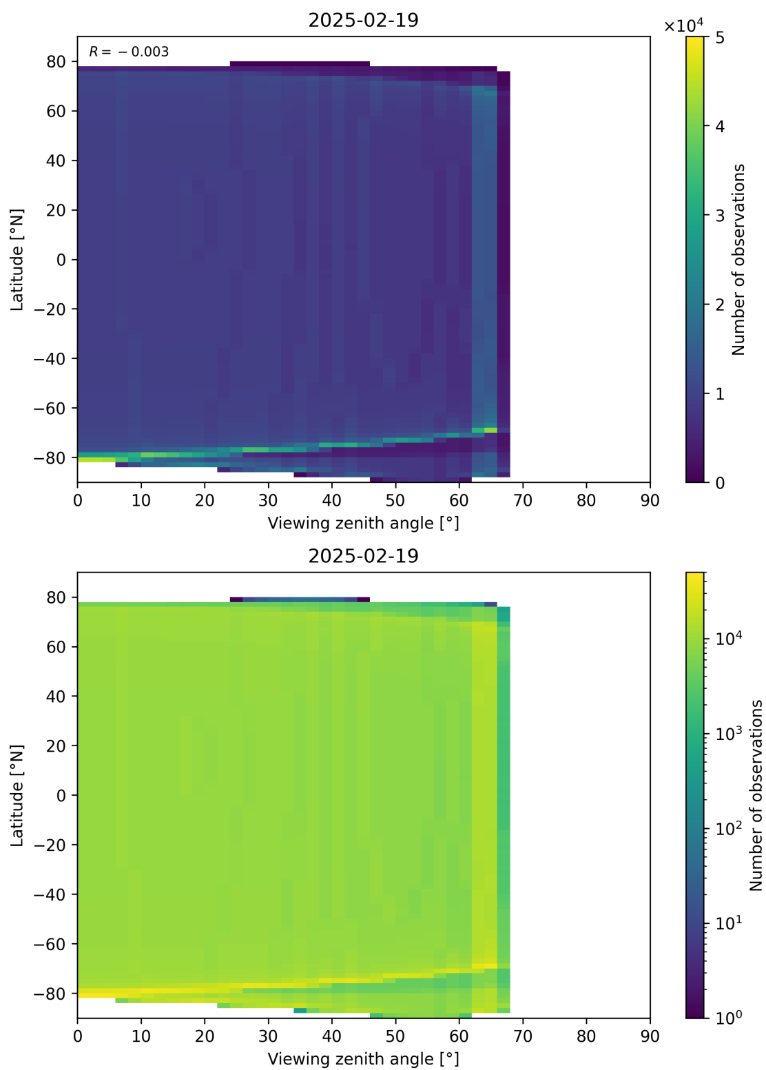
Figure 49: Scatter density plot of “Viewing zenith angle” against “Latitude” for 2025-02-19 to 2025-02-20.
