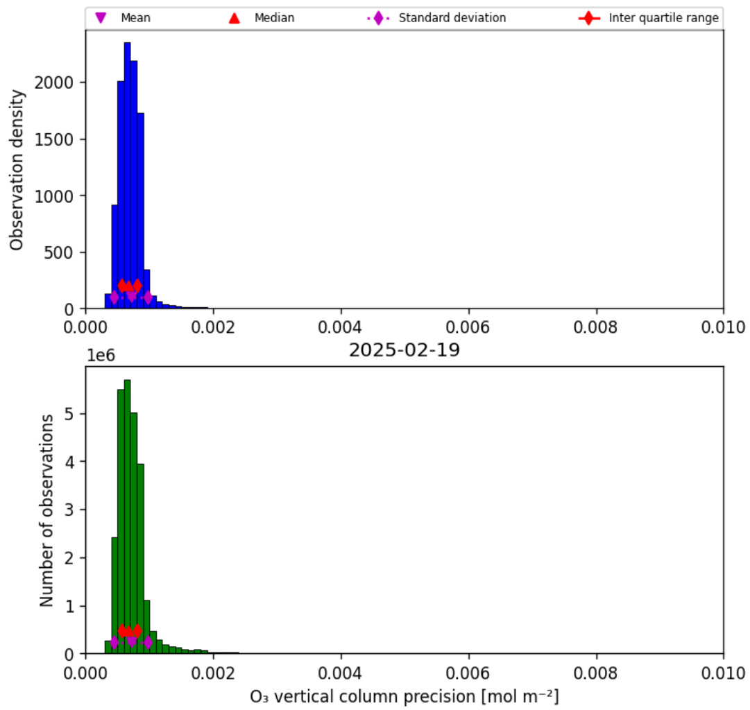
Figure 22: Histogram of “O 3 vertical column precision” for 2025-02-19 to 2025-02-20
