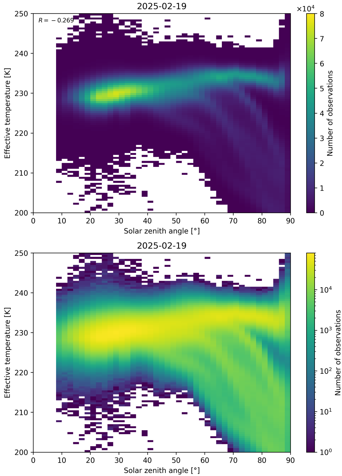
Figure 45: Scatter density plot of “Solar zenith angle” against “Effective temperature” for 2025-02-19 to 2025-02-20.
