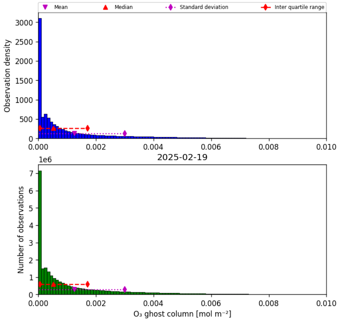
Figure 25: Histogram of “O 3 ghost column” for 2025-02-19 to 2025-02-20
