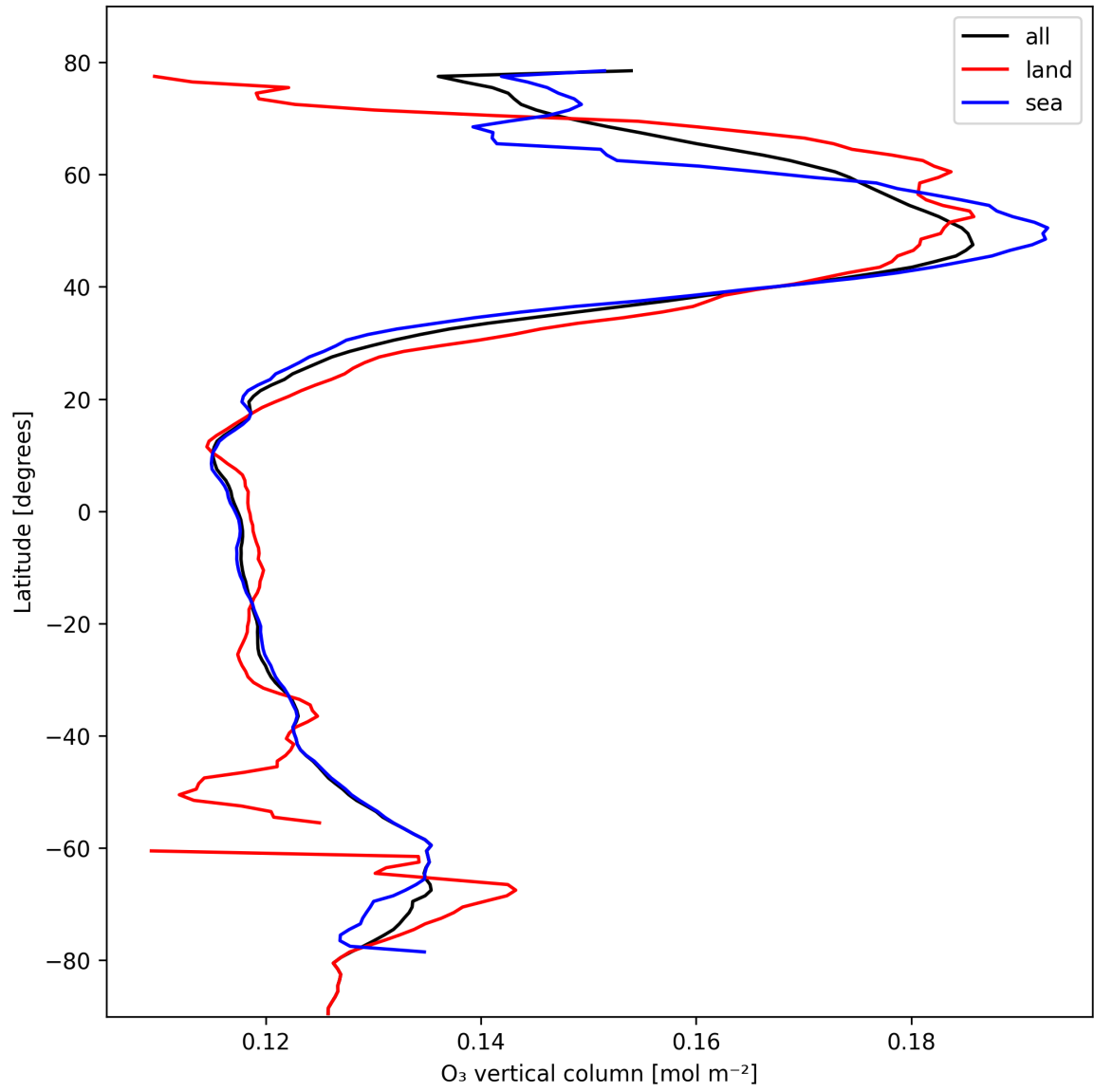
Figure 14: Zonal average of “O 3 vertical column” for 2025-02-19 to 2025-02-20.
