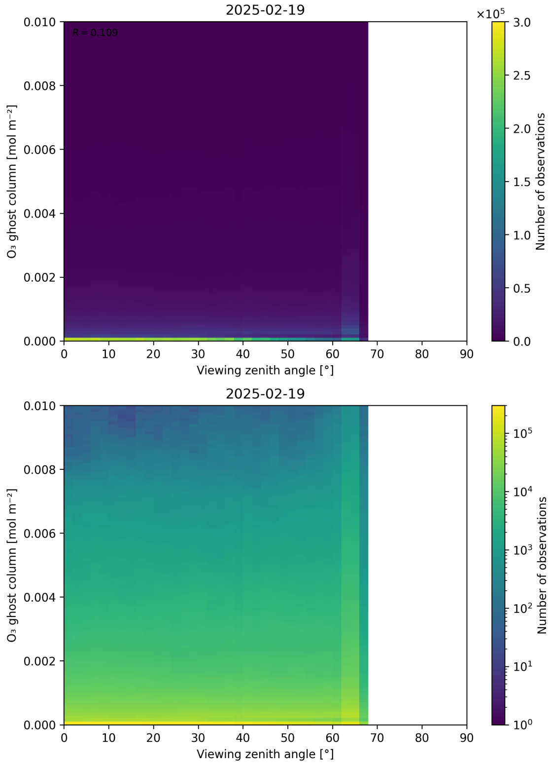
Figure 51: Scatter density plot of “Viewing zenith angle” against “O 3 ghost column” for 2025-02-19 to 2025-02-20.
