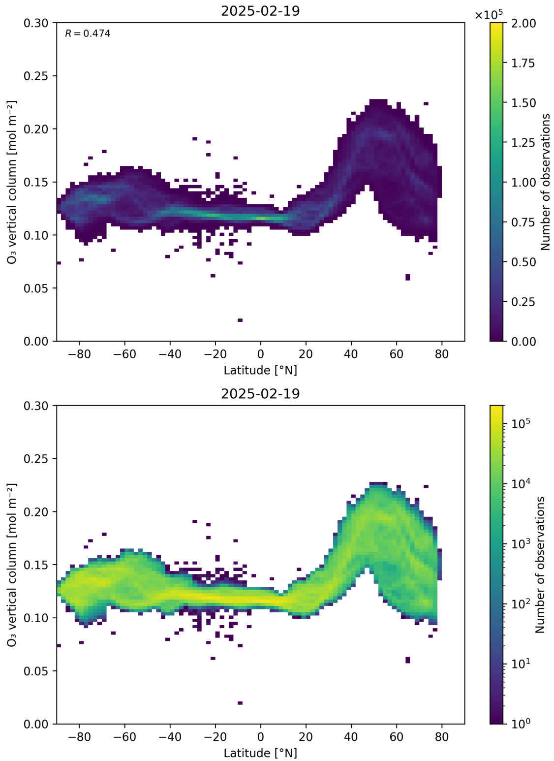
Figure 36: Scatter density plot of “Latitude” against “O 3 vertical column” for 2025-02-19 to 2025-02-20.
