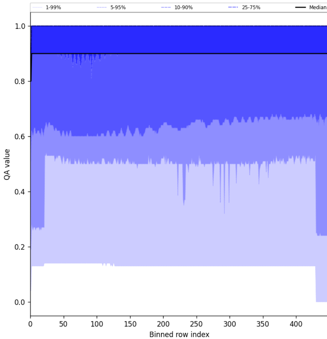
Figure 27: Along track statistics of “QA value” for 2025-02-19 to 2025-02-20
