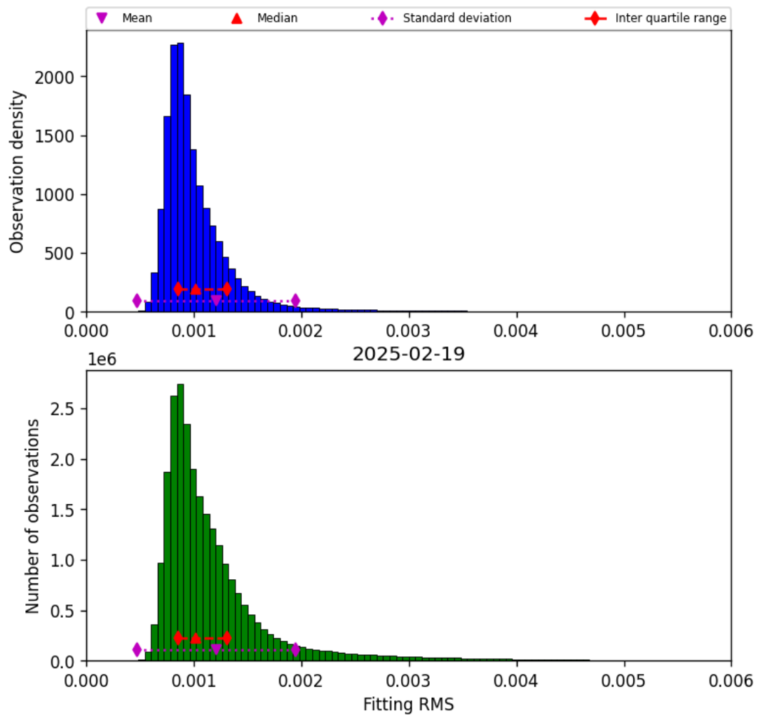
Figure 23: Histogram of “Fitting RMS” for 2025-02-19 to 2025-02-20
