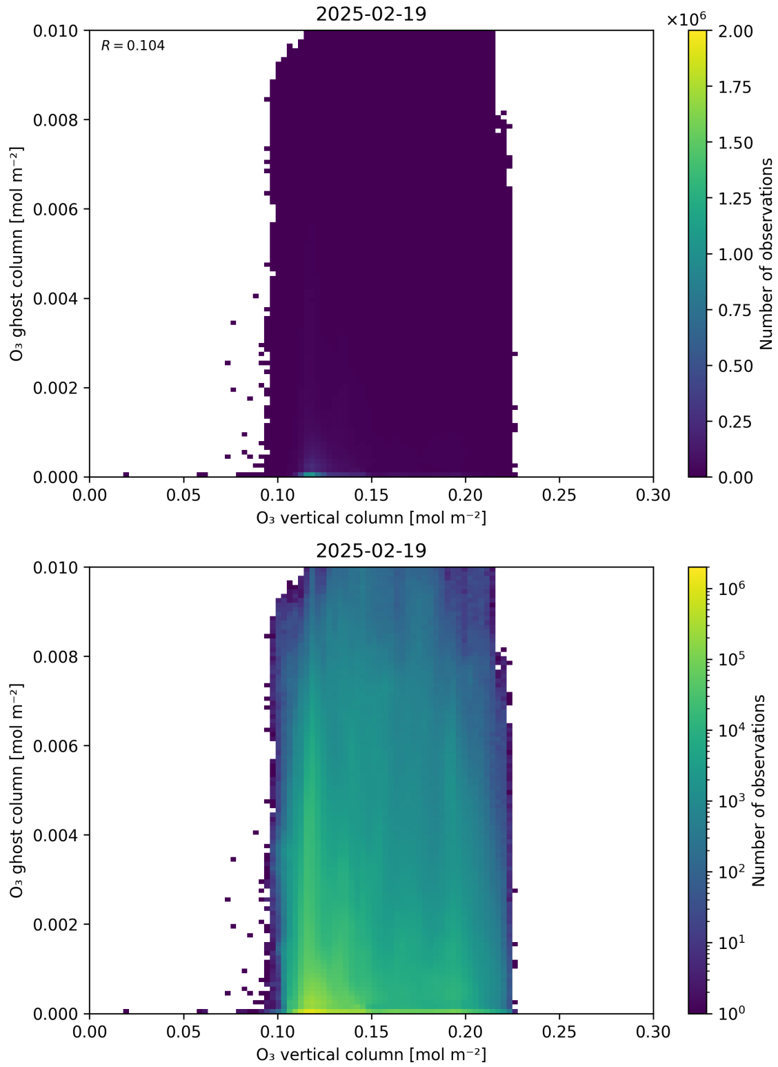
Figure 40: Scatter density plot of “O 3 vertical column” against “O 3 ghost column” for 2025-02-19 to 2025-02-20.
