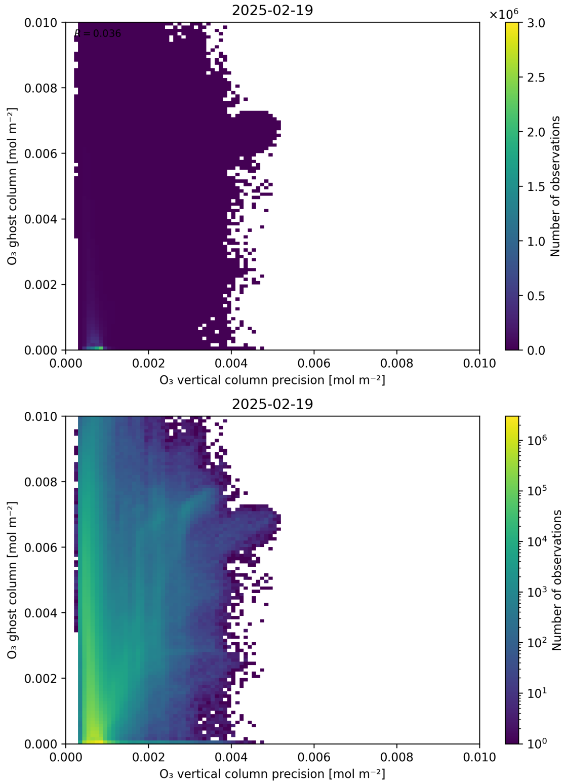
Figure 43: Scatter density plot of “ \text{O}_3 vertical column precision” against “ \text{O}_3 ghost column” for 2025-02-19 to 2025-02-20.
