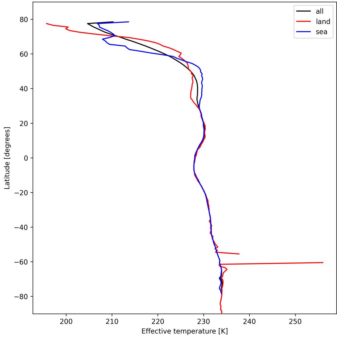
Figure 17: Zonal average of “Effective temperature” for 2025-02-19 to 2025-02-20.
