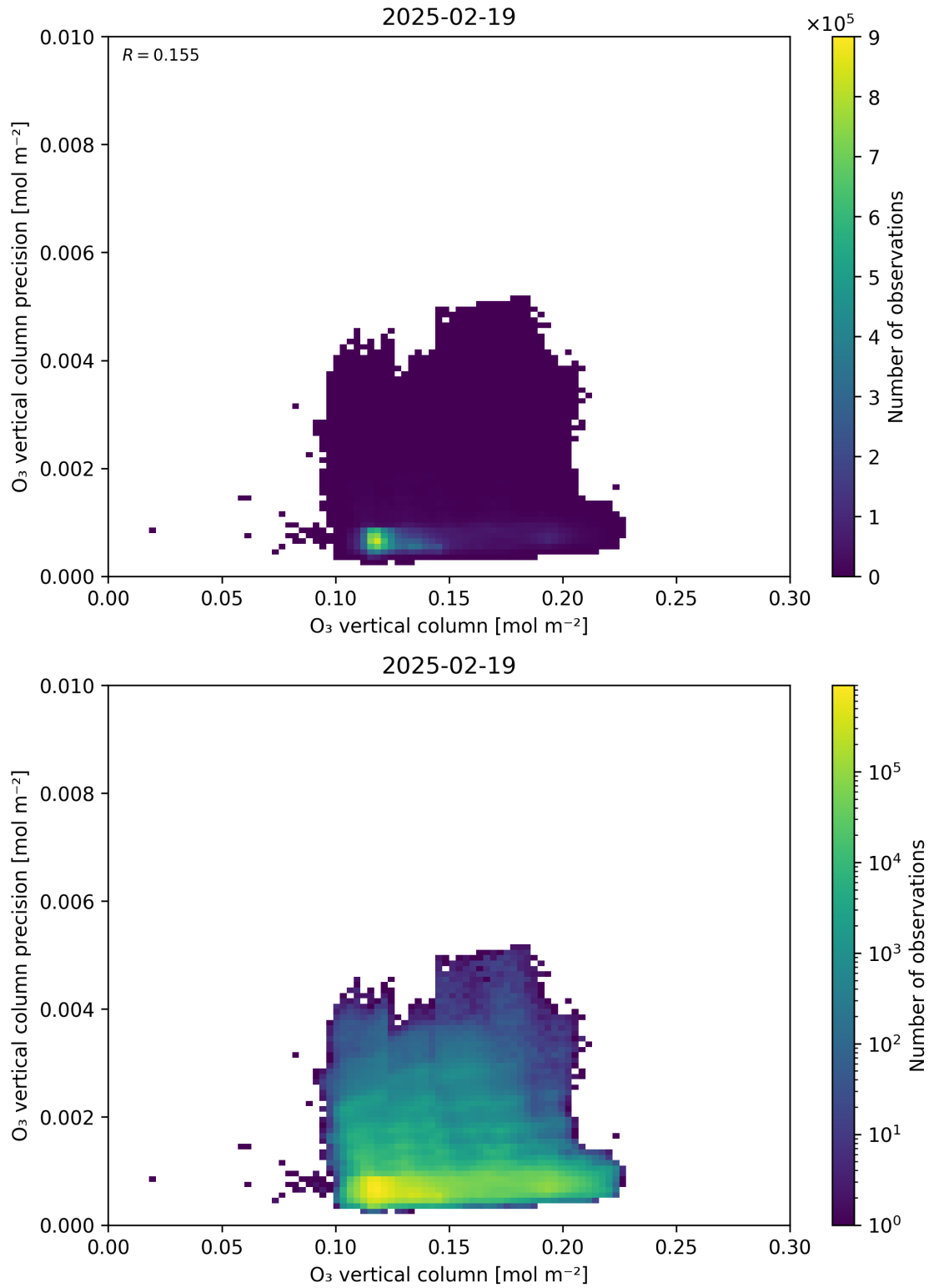
Figure 41: Scatter density plot of “O 3 vertical column” against “O 3 vertical column precision” for 2025-02-19 to 2025-02-20.
