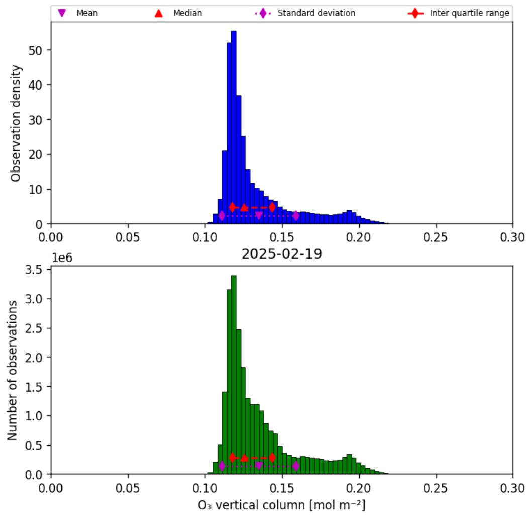
Figure 21: Histogram of “O 3 vertical column” for 2025-02-19 to 2025-02-20
