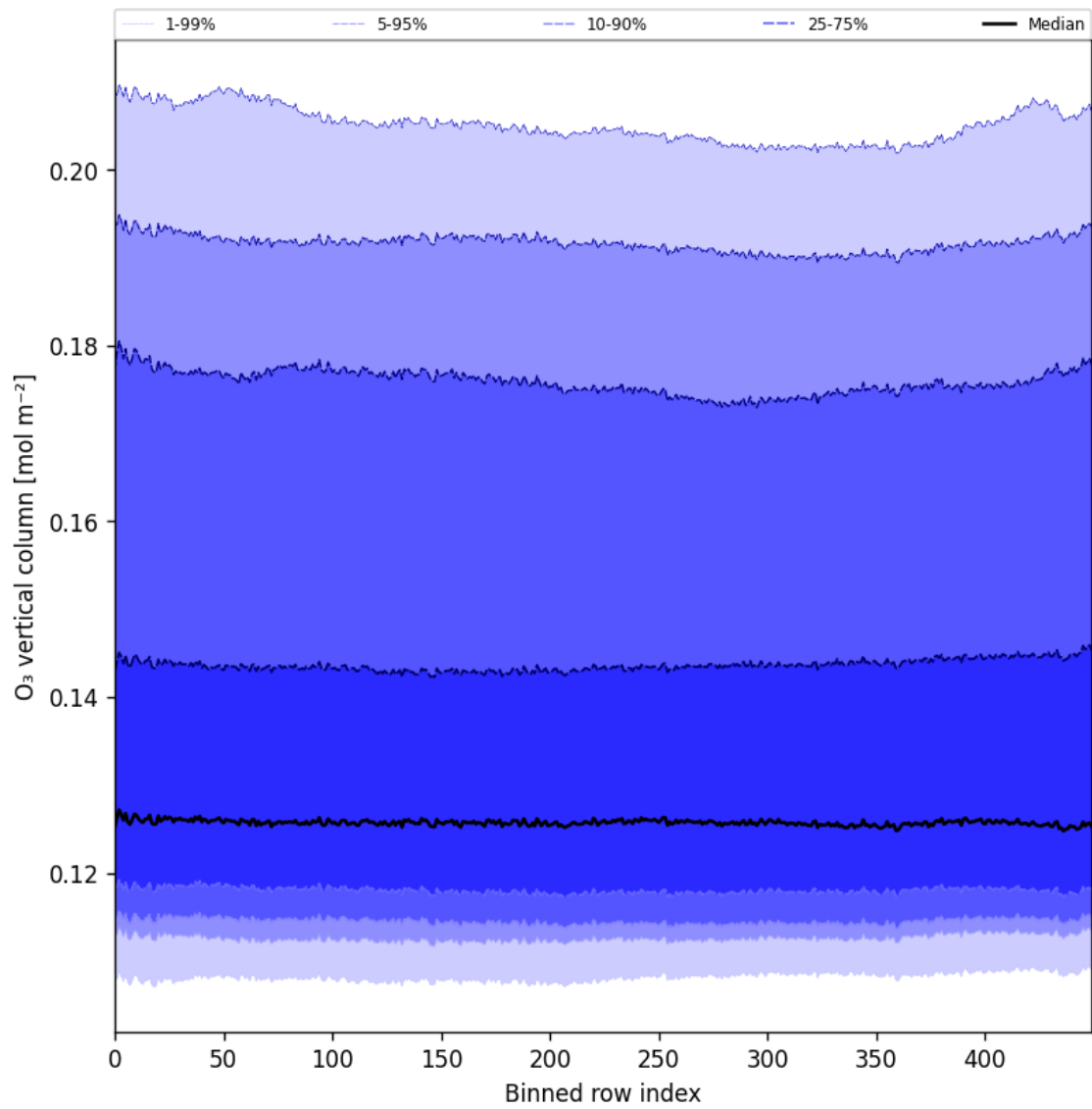
Figure 28: Along track statistics of “O 3 vertical column” for 2025-02-19 to 2025-02-20
