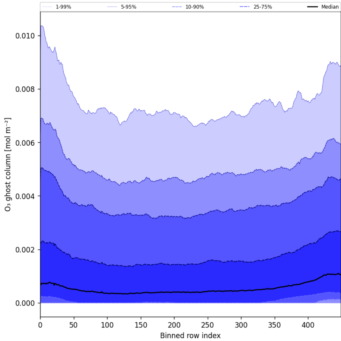
Figure 32: Along track statistics of “O 3 ghost column” for 2025-02-19 to 2025-02-20
