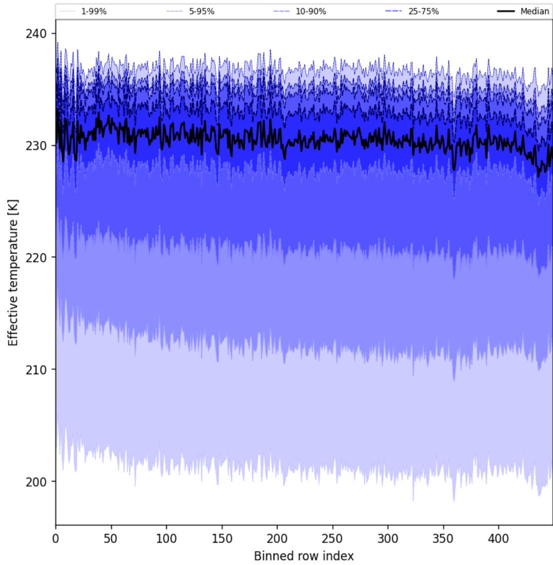
Figure 31: Along track statistics of “Effective temperature” for 2025-02-19 to 2025-02-20
