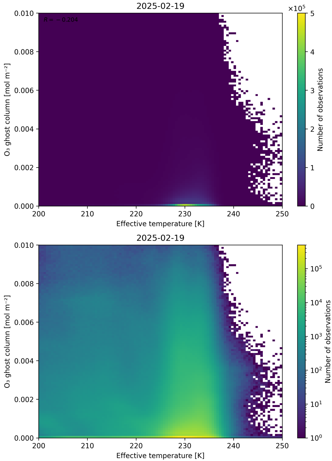
Figure 38: Scatter density plot of “Effective temperature” against “O 3 ghost column” for 2025-02-19 to 2025-02-20.
