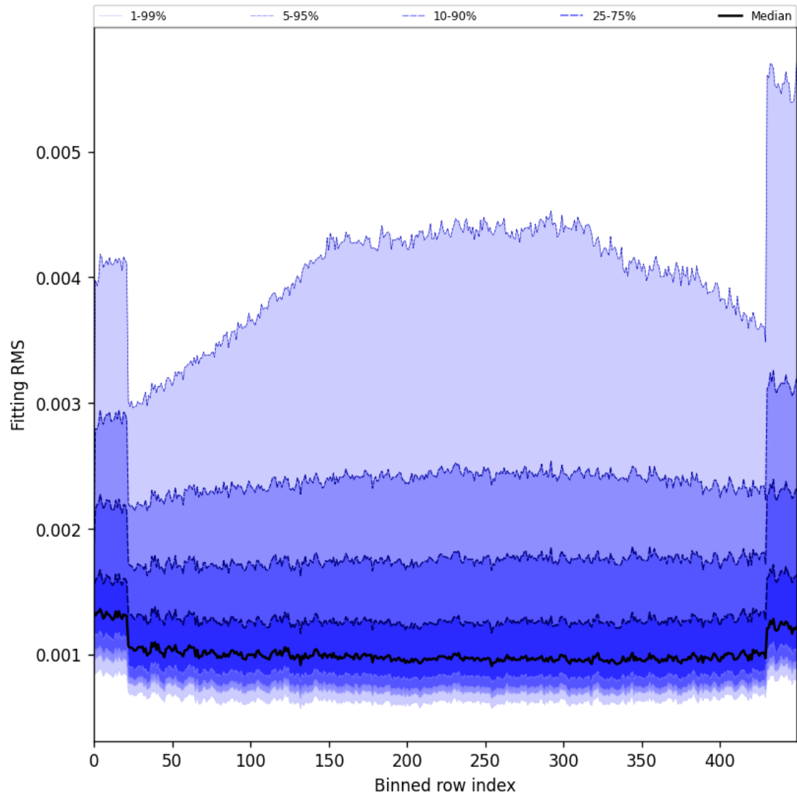
Figure 30: Along track statistics of “Fitting RMS” for 2025-02-19 to 2025-02-20
