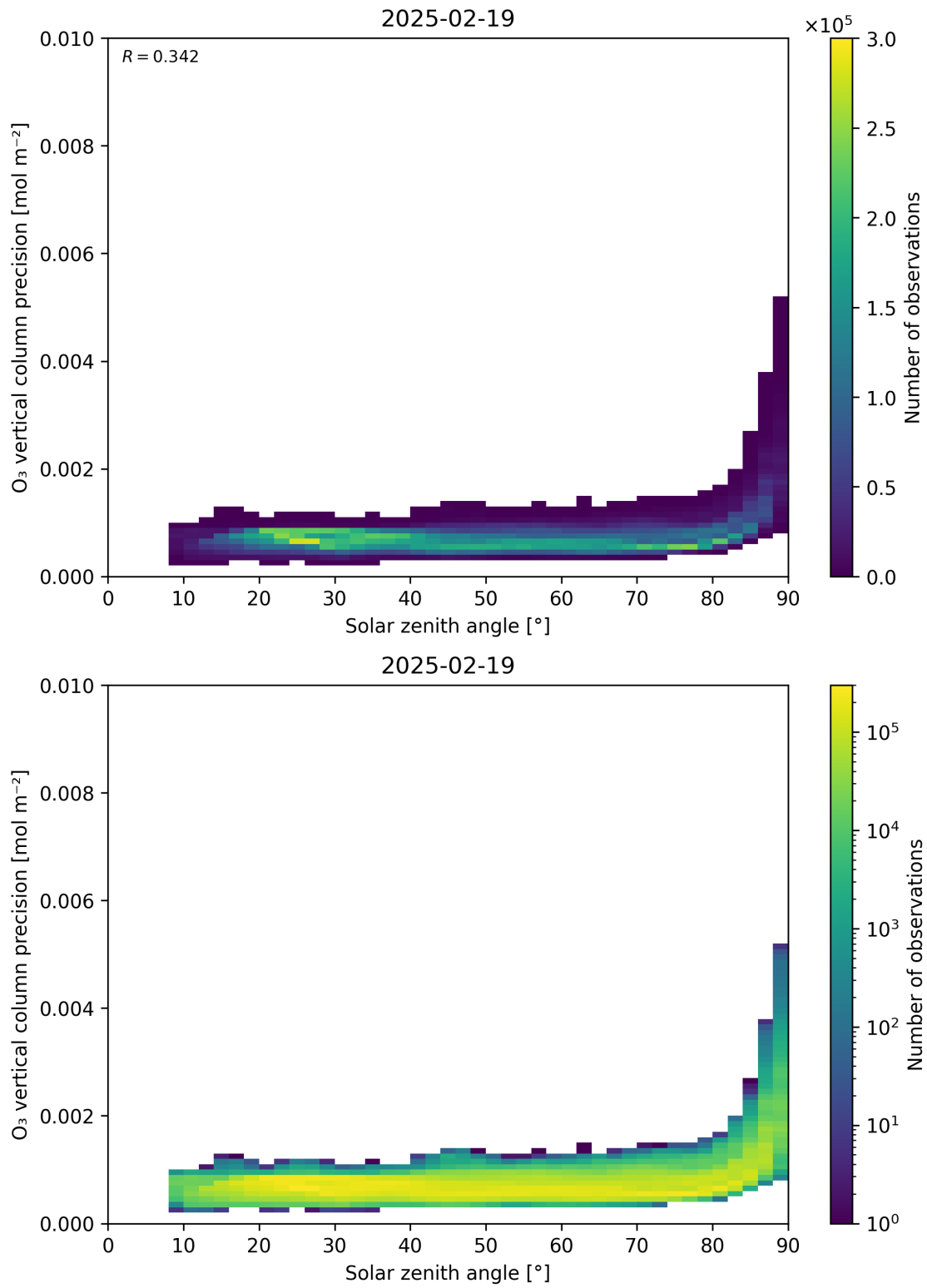
Figure 48: Scatter density plot of “Solar zenith angle” against “O 3 vertical column precision” for 2025-02-19 to 2025-02-20.
