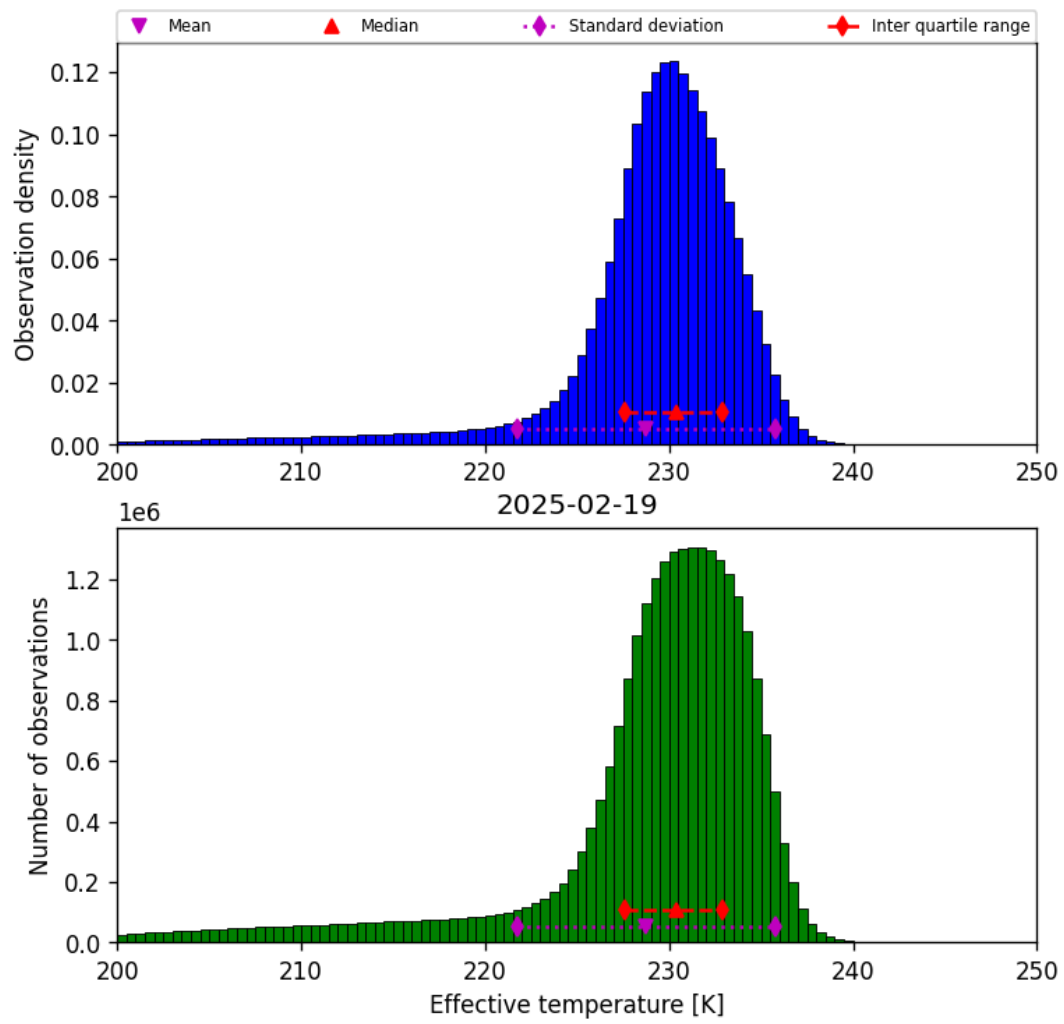
Figure 24: Histogram of “Effective temperature” for 2025-02-19 to 2025-02-20
