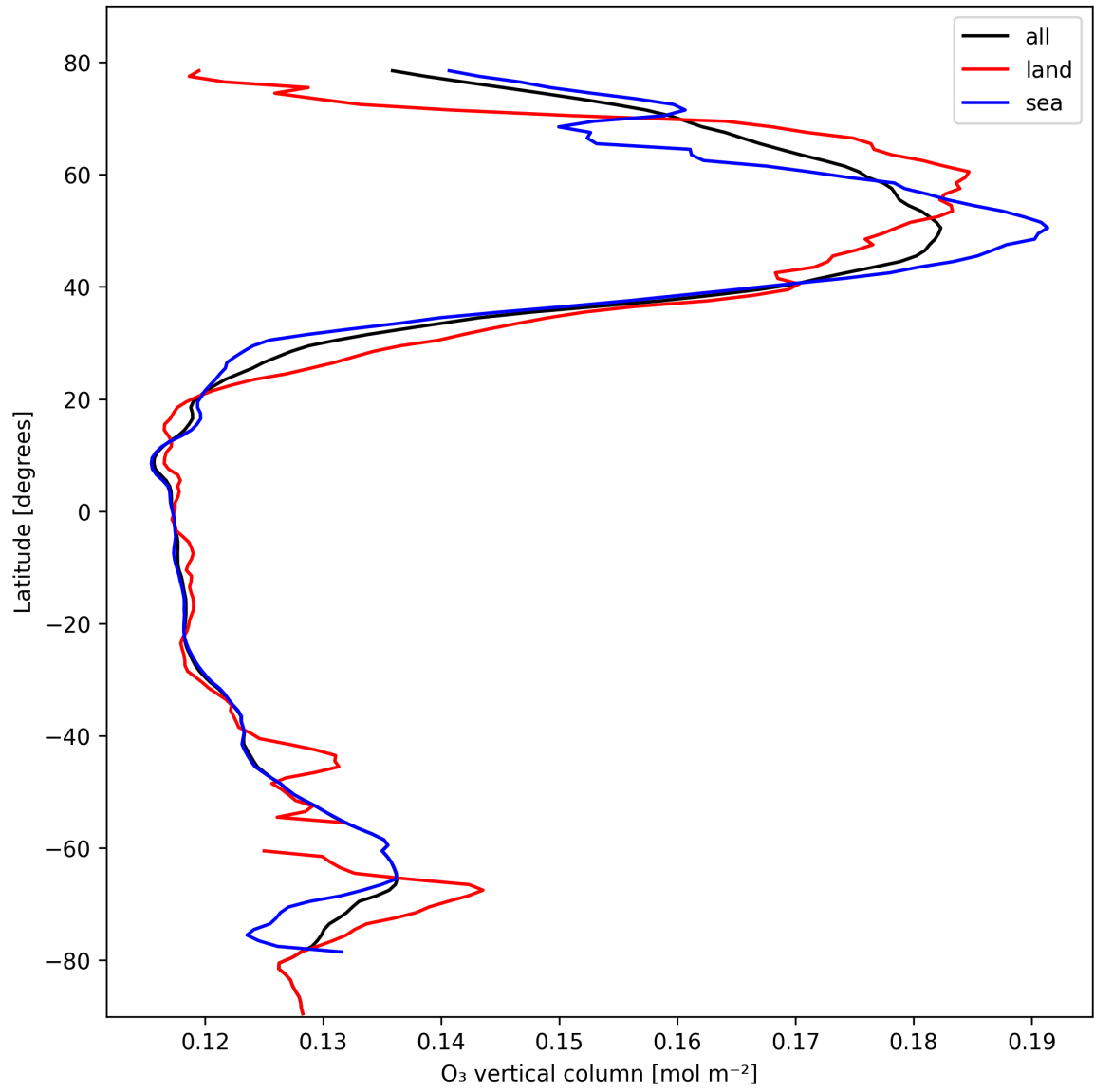
Figure 14: Zonal average of “O 3 vertical column” for 2025-02-20 to 2025-02-22.
