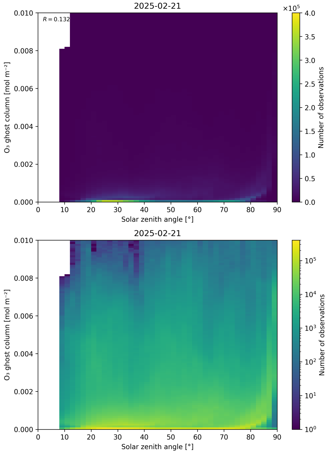
Figure 46: Scatter density plot of “Solar zenith angle” against “O 3 ghost column” for 2025-02-20 to 2025-02-22.
