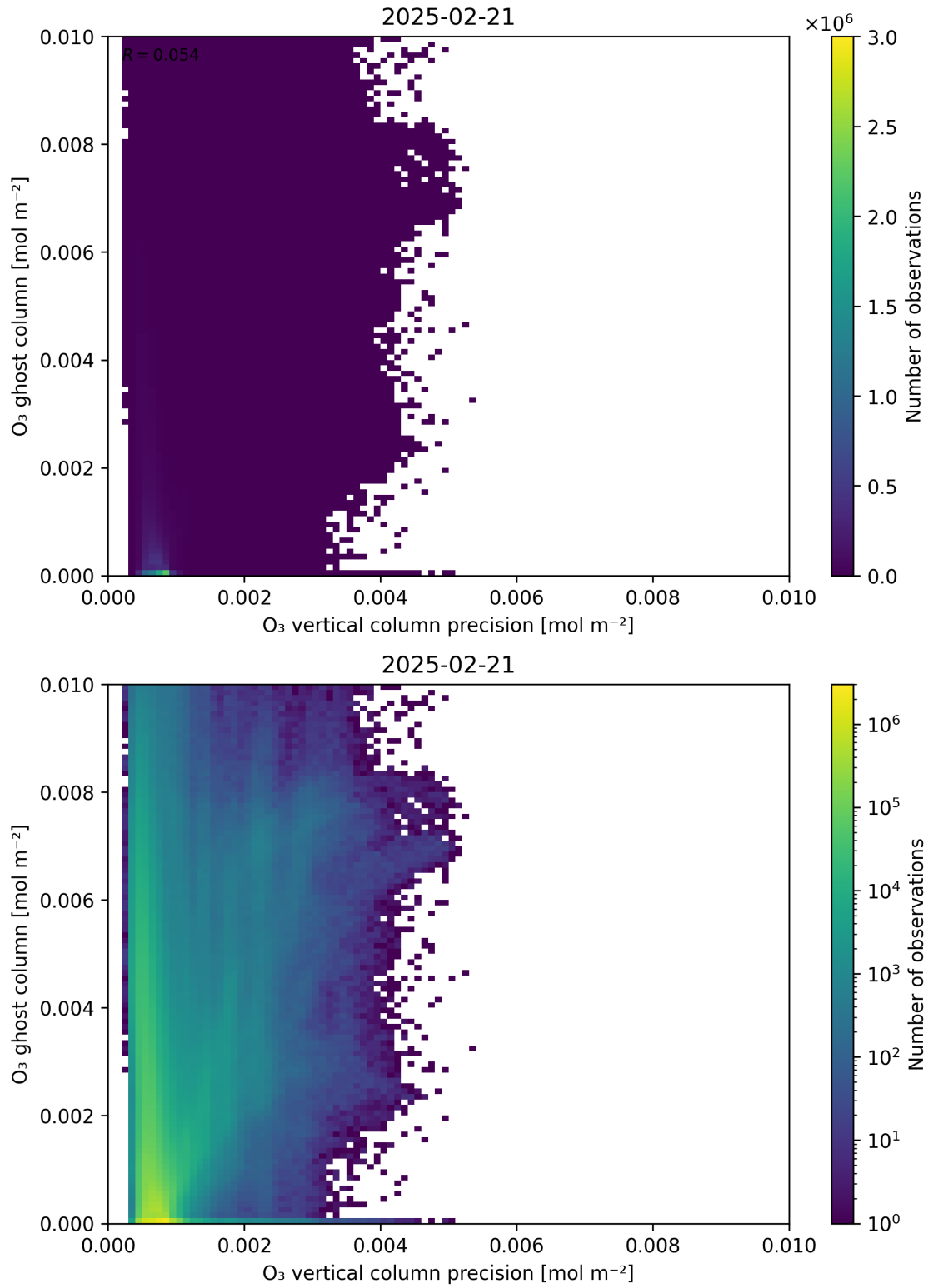
Figure 43: Scatter density plot of “O 3 vertical column precision” against “O 3 ghost column” for 2025-02-20 to 2025-02-22.
