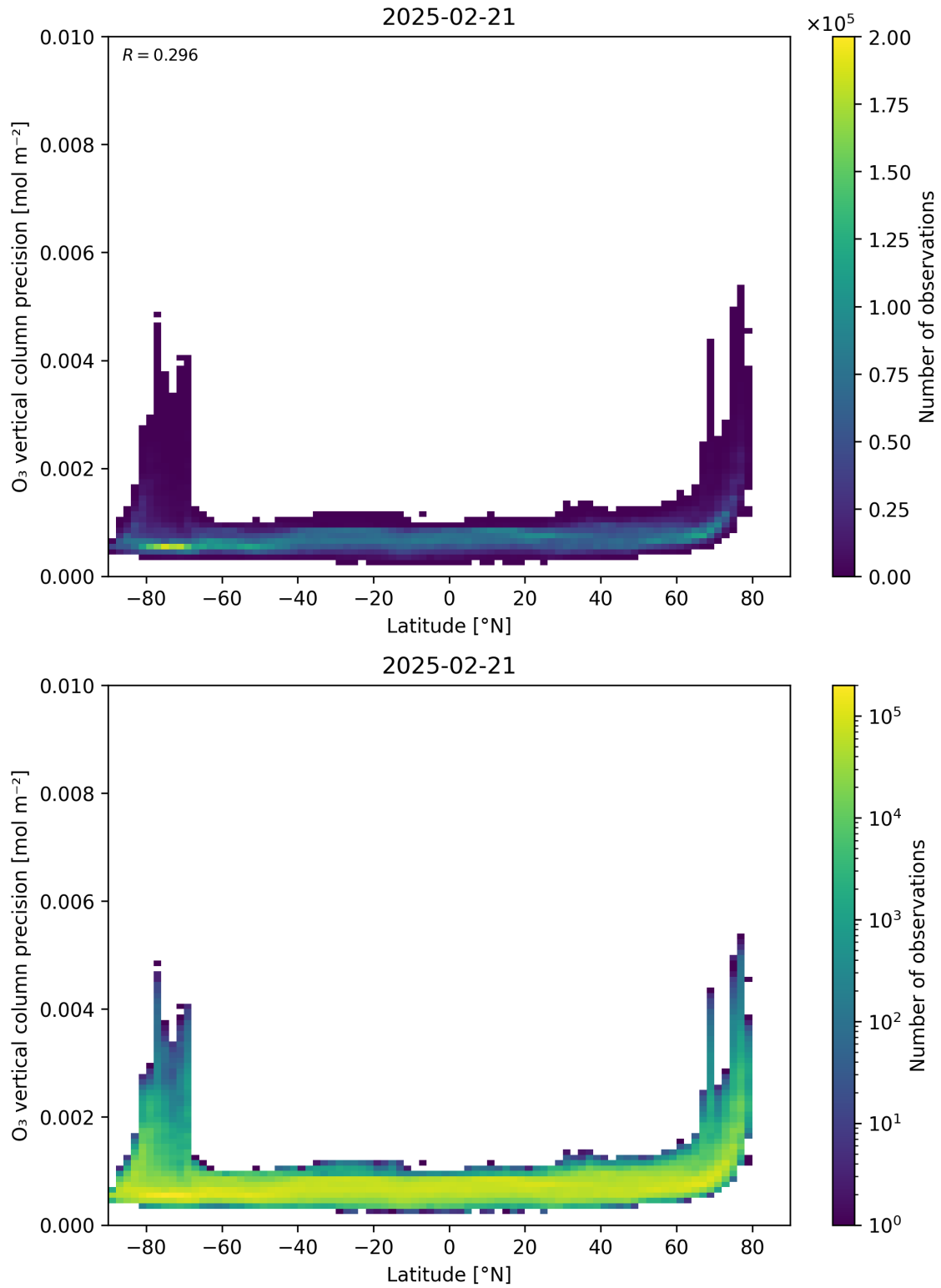
Figure 37: Scatter density plot of “Latitude” against “O 3 vertical column precision” for 2025-02-20 to 2025-02-22.
