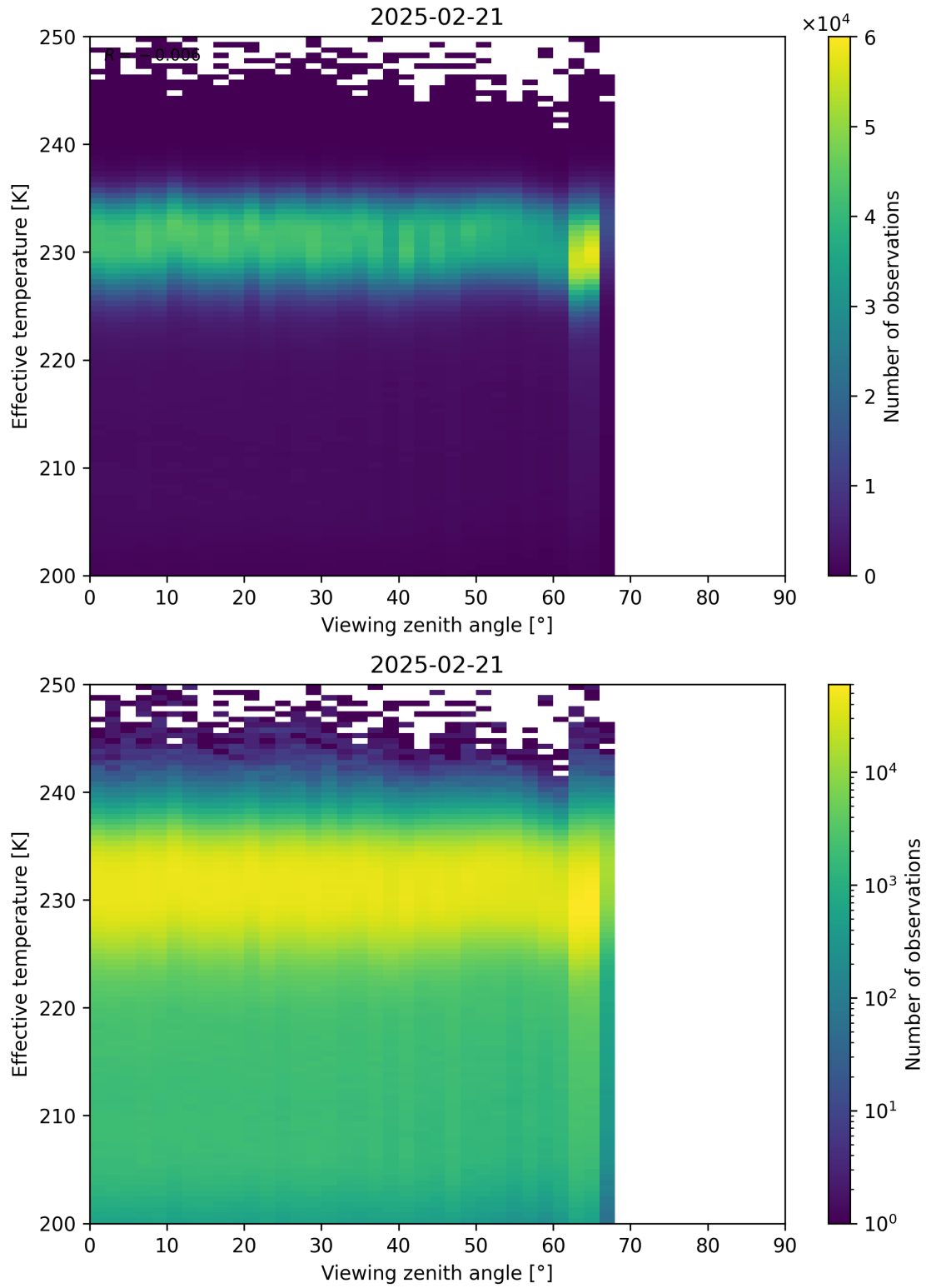
Figure 50: Scatter density plot of “Viewing zenith angle” against “Effective temperature” for 2025-02-20 to 2025-02-22.
