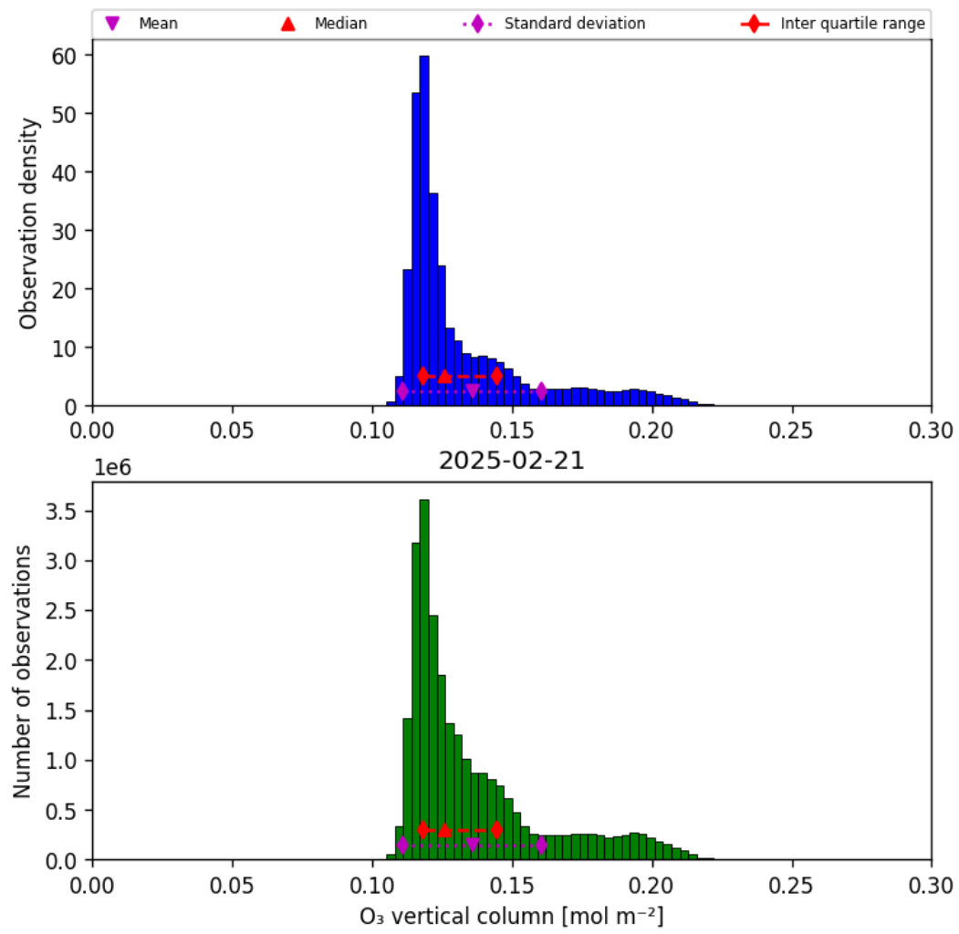
Figure 21: Histogram of “O 3 vertical column” for 2025-02-20 to 2025-02-22
