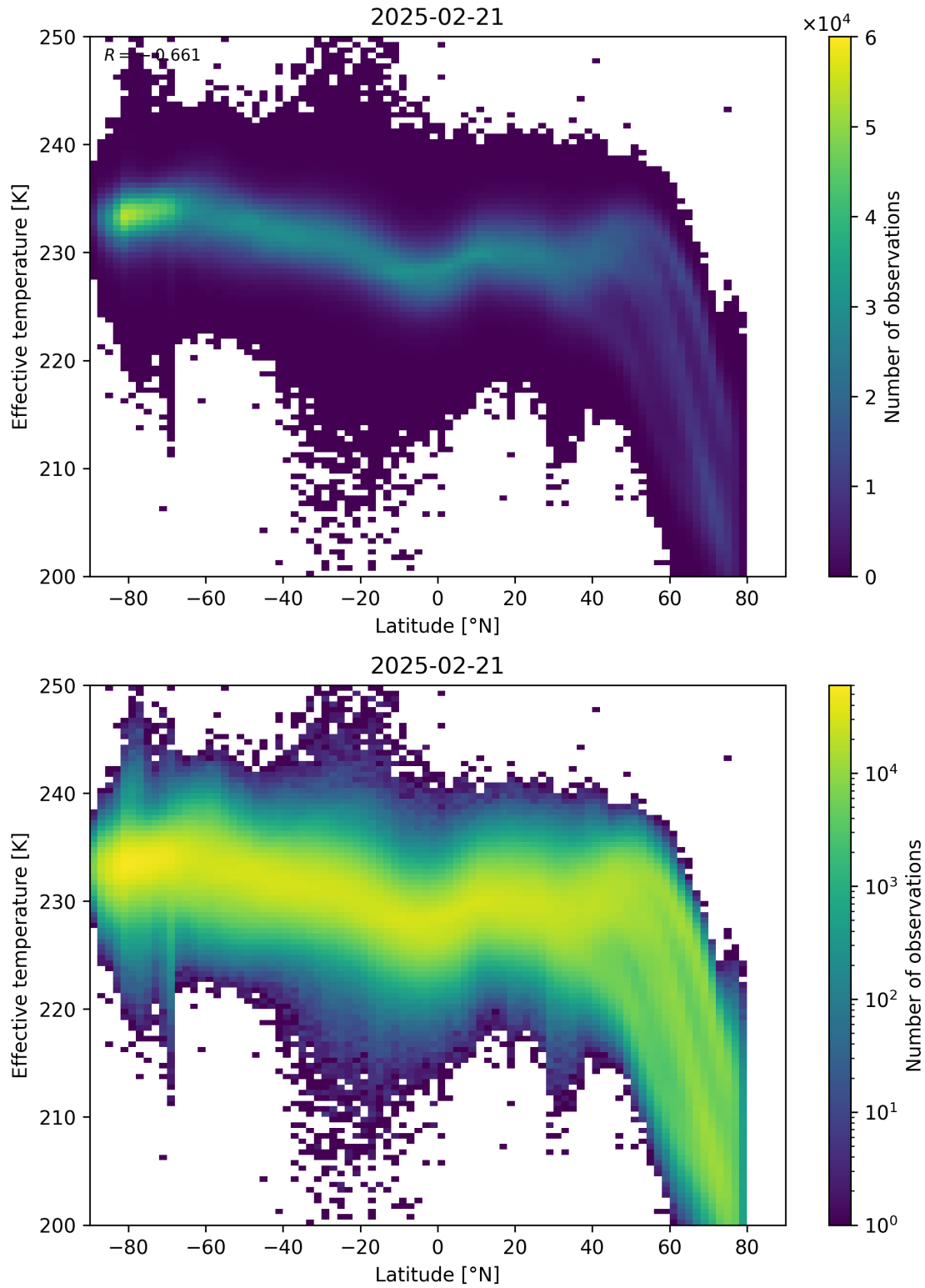
Figure 34: Scatter density plot of “Latitude” against “Effective temperature” for 2025-02-20 to 2025-02-22.
