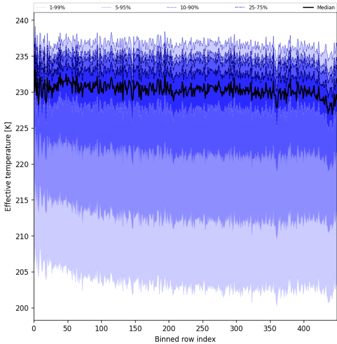
Figure 31: Along track statistics of “Effective temperature” for 2025-02-20 to 2025-02-22
