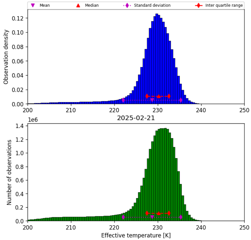
Figure 24: Histogram of “Effective temperature” for 2025-02-20 to 2025-02-22
