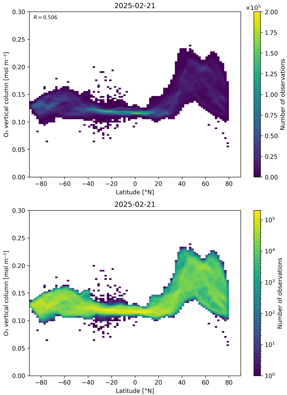
Figure 36: Scatter density plot of “Latitude” against “O 3 vertical column” for 2025-02-20 to 2025-02-22.
