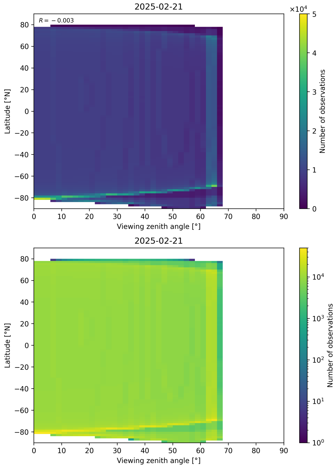
Figure 49: Scatter density plot of “Viewing zenith angle” against “Latitude” for 2025-02-20 to 2025-02-22.
