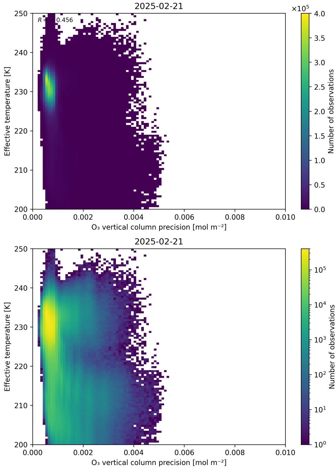
Figure 42: Scatter density plot of “O 3 vertical column precision” against “Effective temperature” for 2025-02-20 to 2025-02-22.
