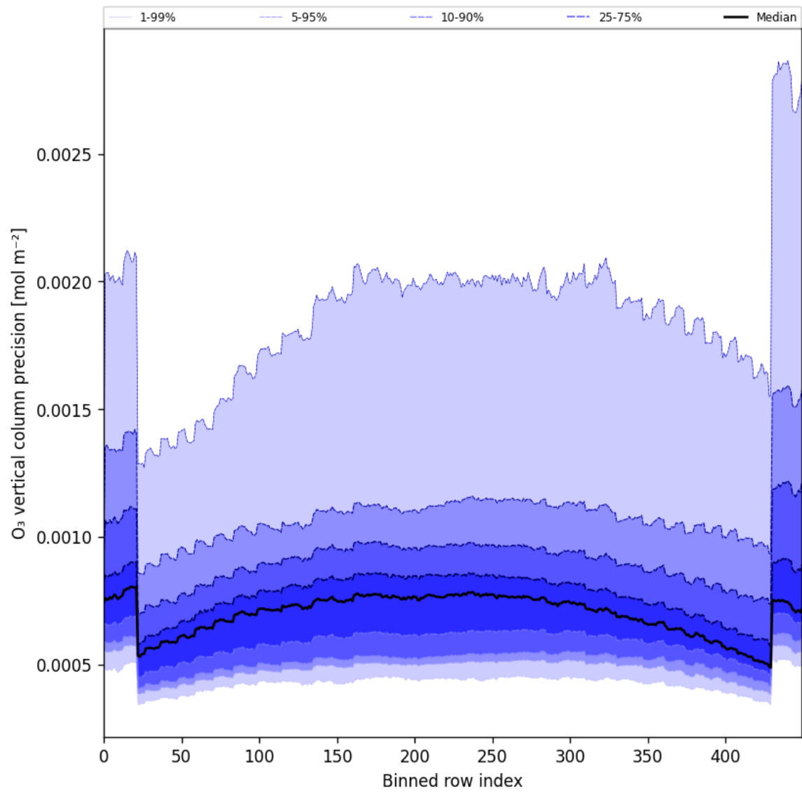
Figure 29: Along track statistics of “O 3 vertical column precision” for 2025-02-20 to 2025-02-22
