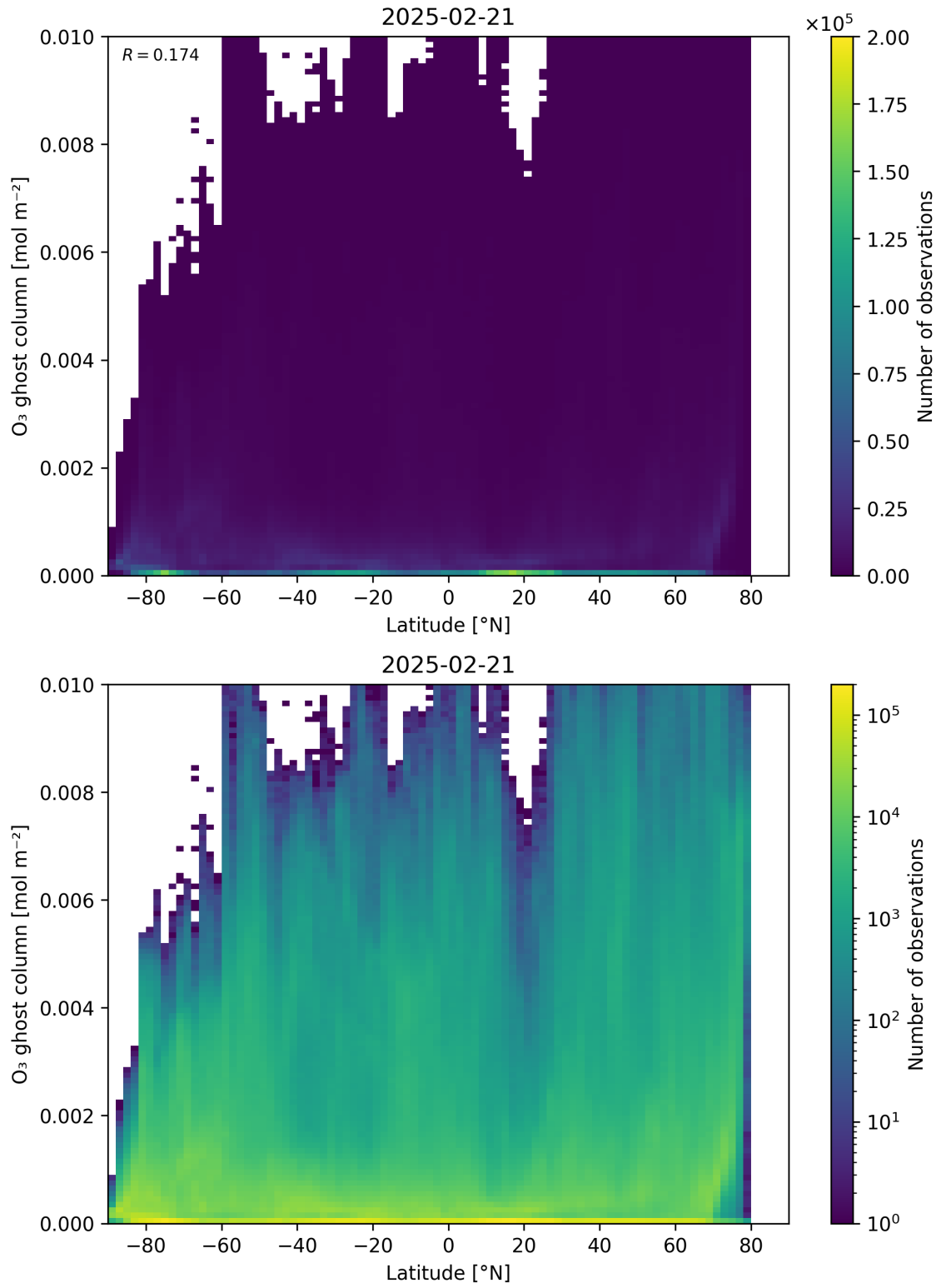
Figure 35: Scatter density plot of “Latitude” against “O 3 ghost column” for 2025-02-20 to 2025-02-22.
