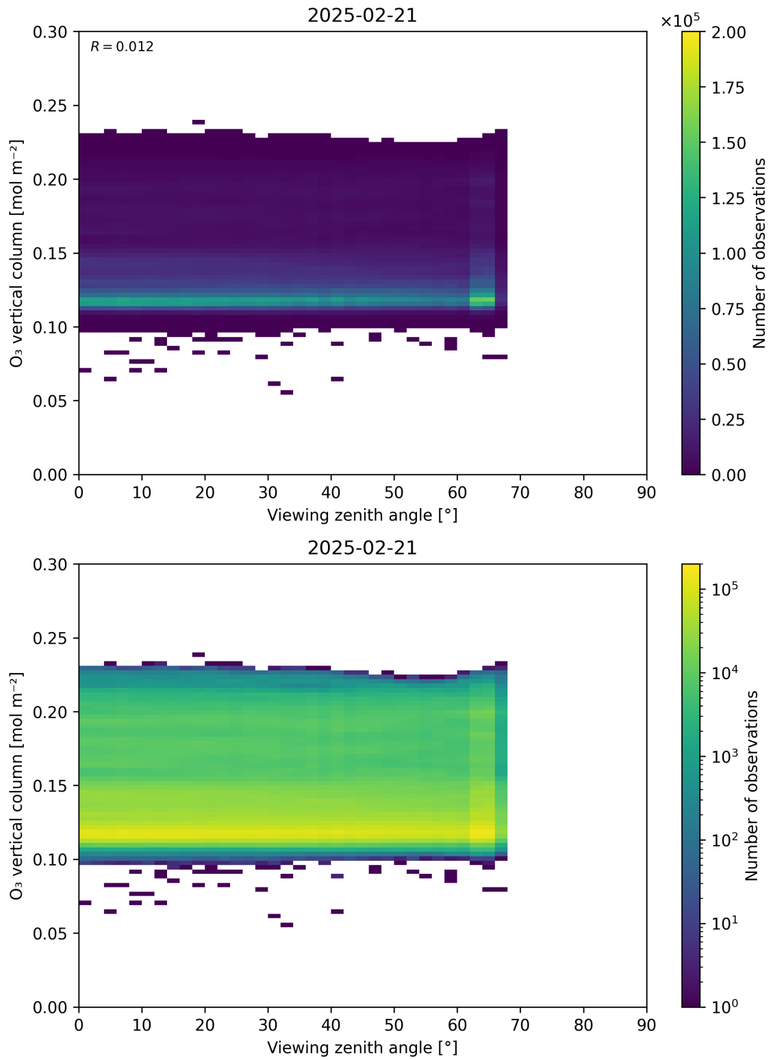
Figure 52: Scatter density plot of “Viewing zenith angle” against “O 3 vertical column” for 2025-02-20 to 2025-02-22.
