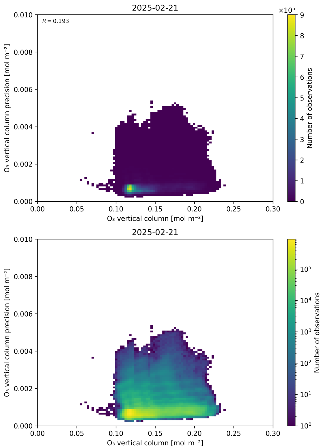
Figure 41: Scatter density plot of “O 3 vertical column” against “O 3 vertical column precision” for 2025-02-20 to 2025-02-22.
