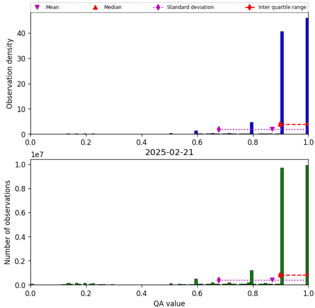
Figure 20: Histogram of “QA value” for 2025-02-20 to 2025-02-22
