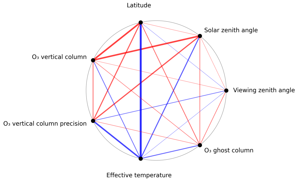
Figure 1: Map of correlation graph for 2025-02-20 to 2025-02-22.
