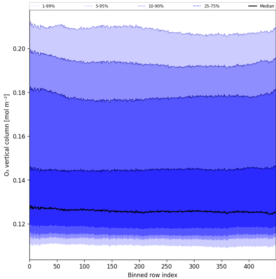
Figure 28: Along track statistics of “O 3 vertical column” for 2025-02-20 to 2025-02-22
