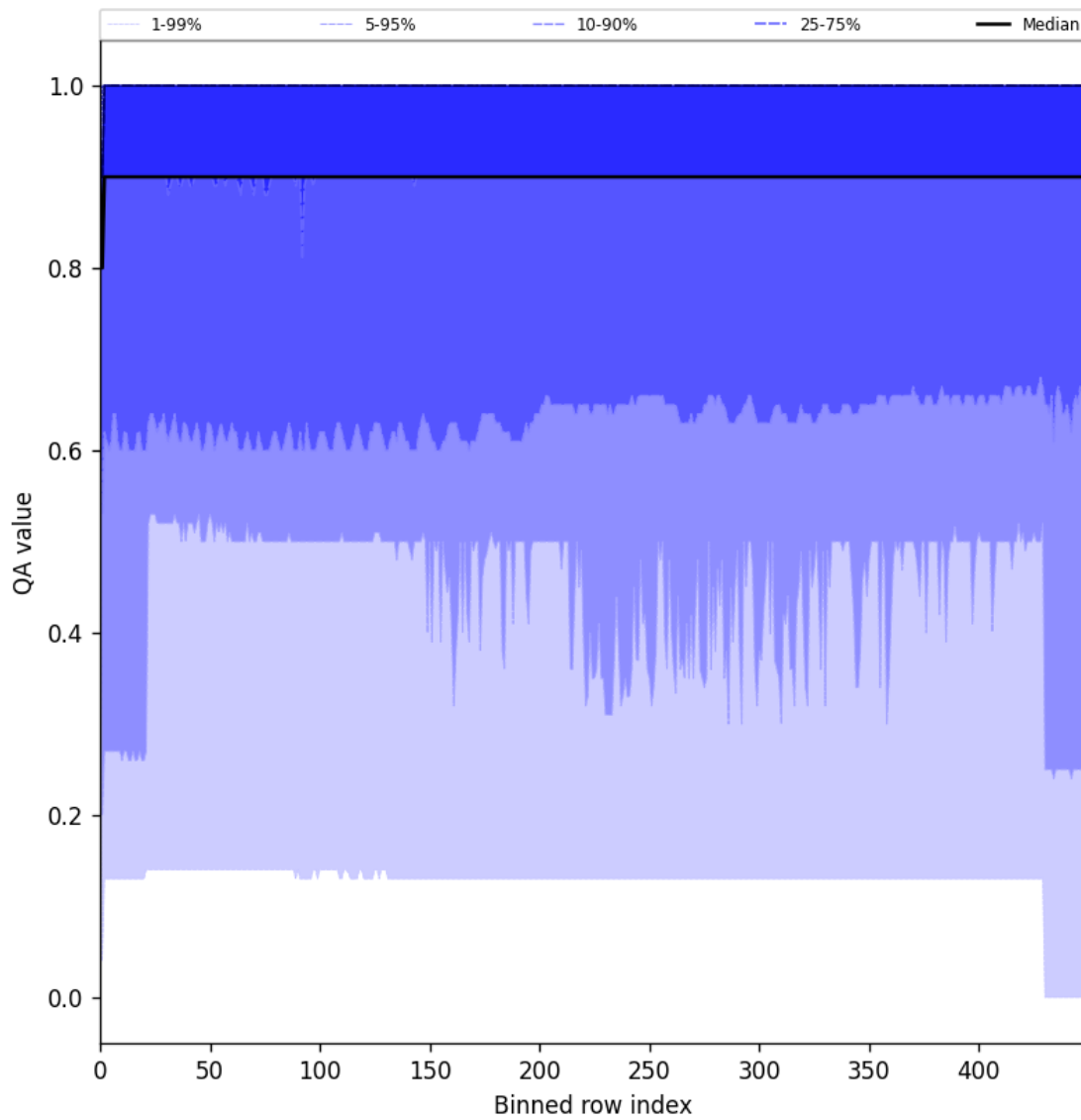
Figure 27: Along track statistics of “QA value” for 2025-02-20 to 2025-02-22
