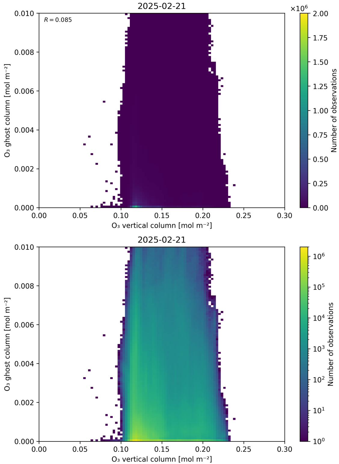
Figure 40: Scatter density plot of “O 3 vertical column” against “O 3 ghost column” for 2025-02-20 to 2025-02-22.
