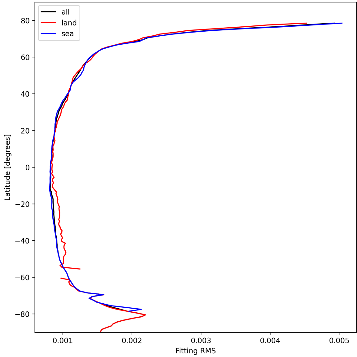
Figure 16: Zonal average of “Fitting RMS” for 2025-02-20 to 2025-02-22.
