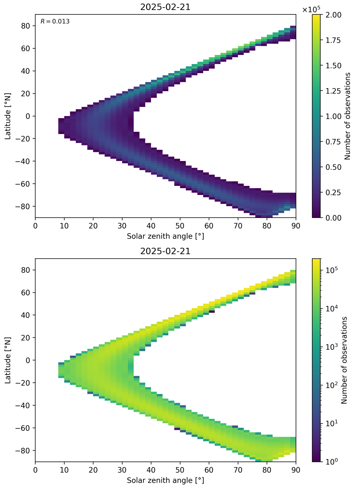
Figure 44: Scatter density plot of “Solar zenith angle” against “Latitude” for 2025-02-20 to 2025-02-22.
