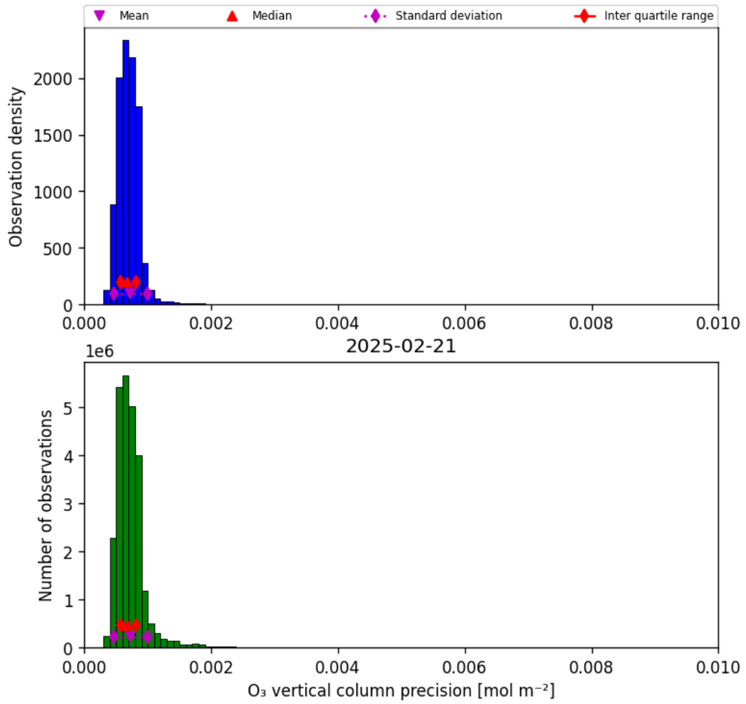
Figure 22: Histogram of “O 3 vertical column precision” for 2025-02-20 to 2025-02-22
