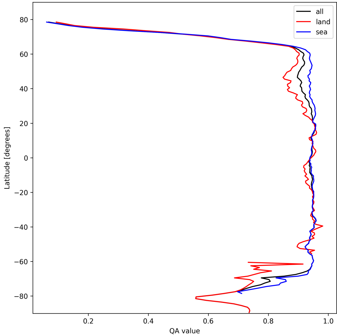
Figure 13: Zonal average of “QA value” for 2025-02-20 to 2025-02-22.
