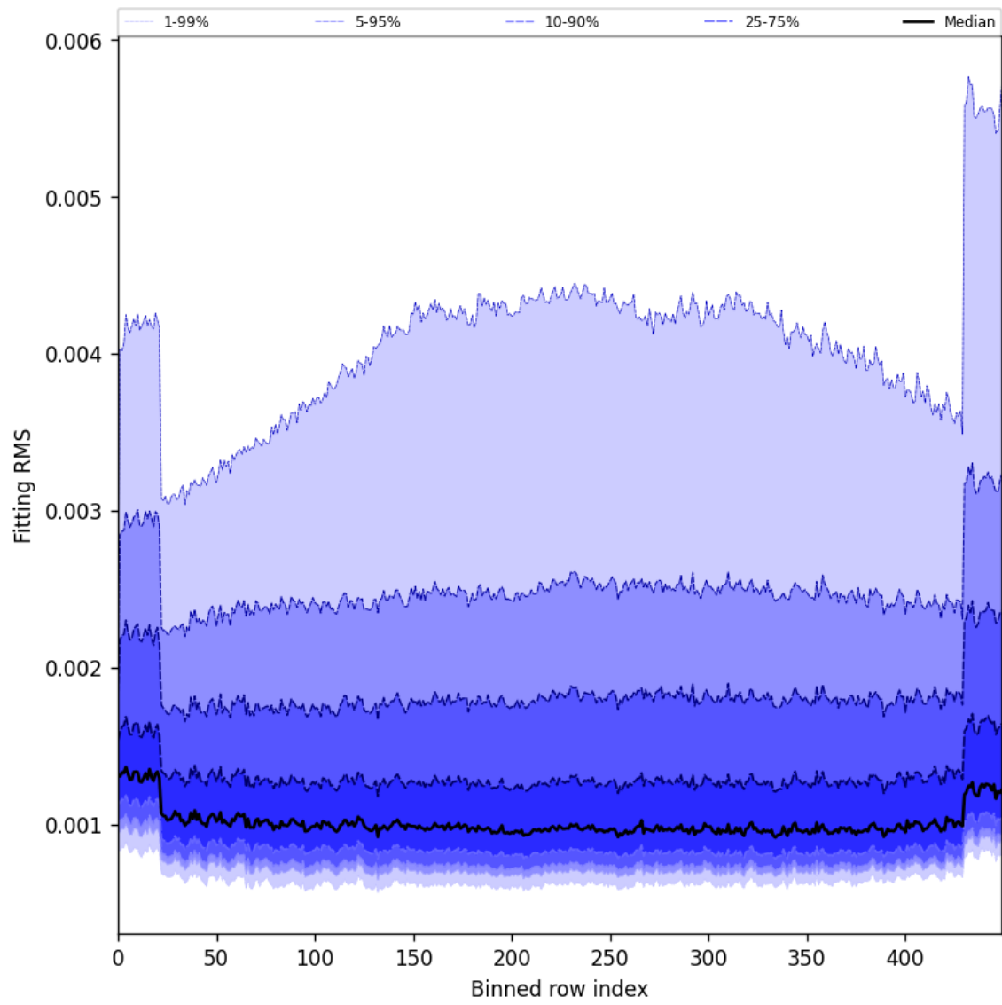
Figure 30: Along track statistics of “Fitting RMS” for 2025-02-20 to 2025-02-22
