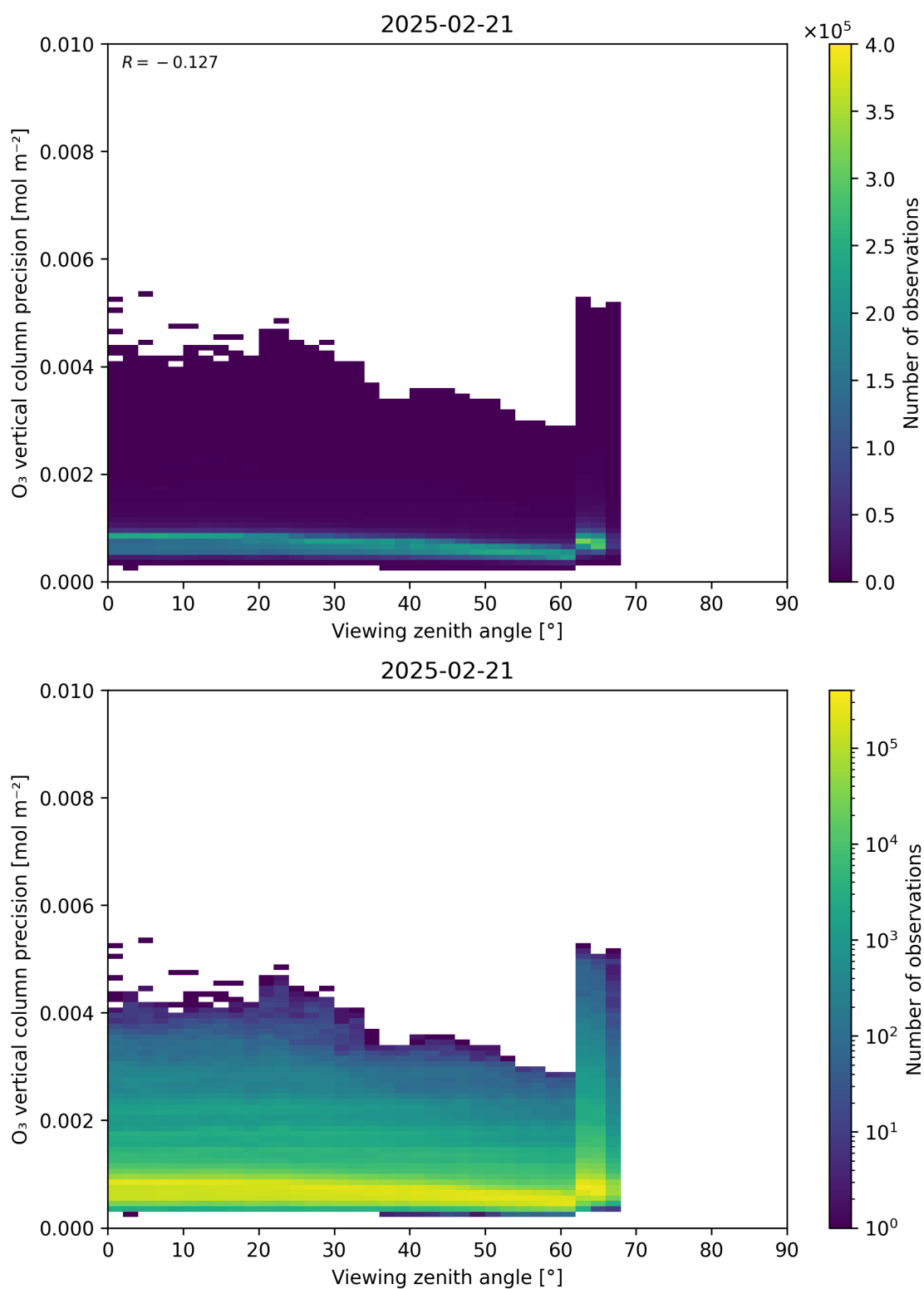
Figure 53: Scatter density plot of “Viewing zenith angle” against “O 3 vertical column precision” for 2025-02-20 to 2025-02-22.
