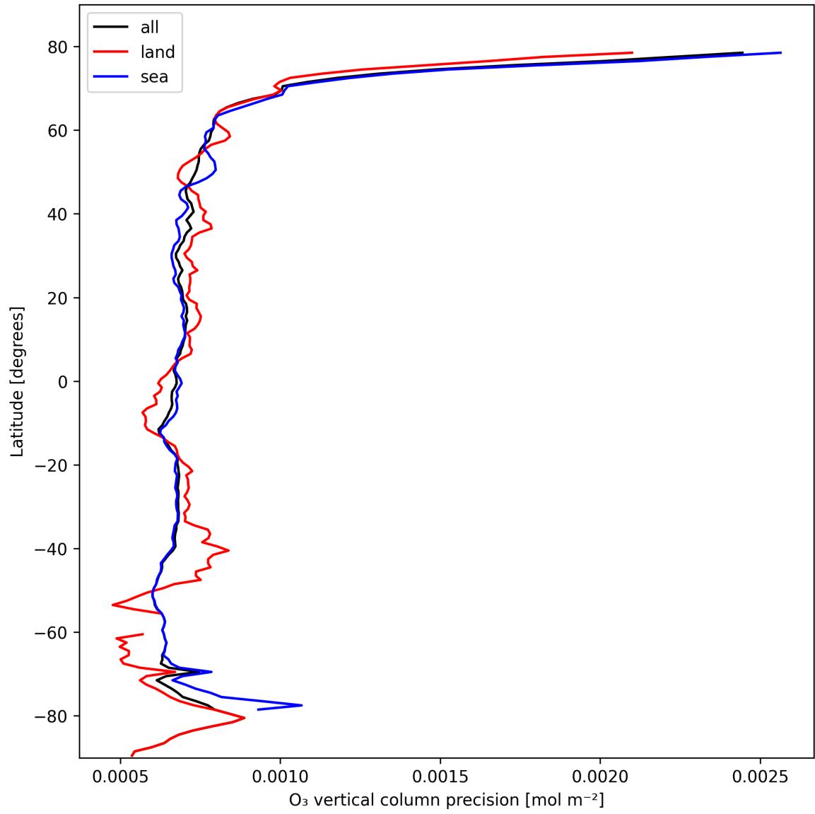
Figure 15: Zonal average of “O 3 vertical column precision” for 2025-02-20 to 2025-02-22.
