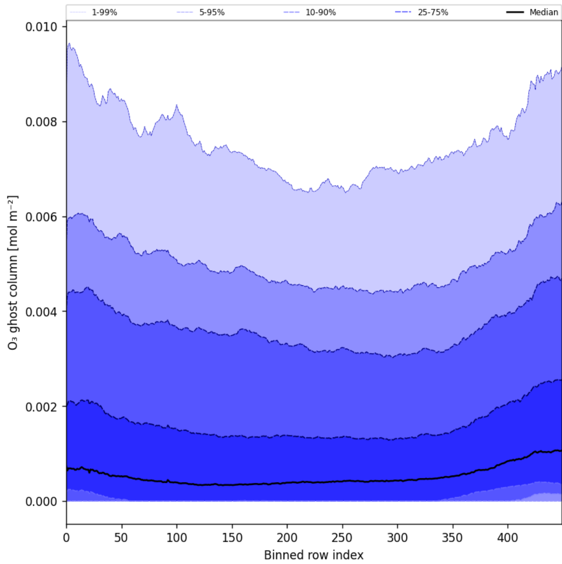
Figure 32: Along track statistics of “O 3 ghost column” for 2025-02-20 to 2025-02-22
