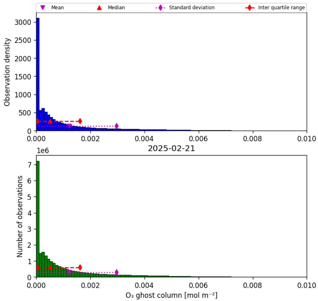
Figure 25: Histogram of "O 3 ghost column" for 2025-02-20 to 2025-02-22
