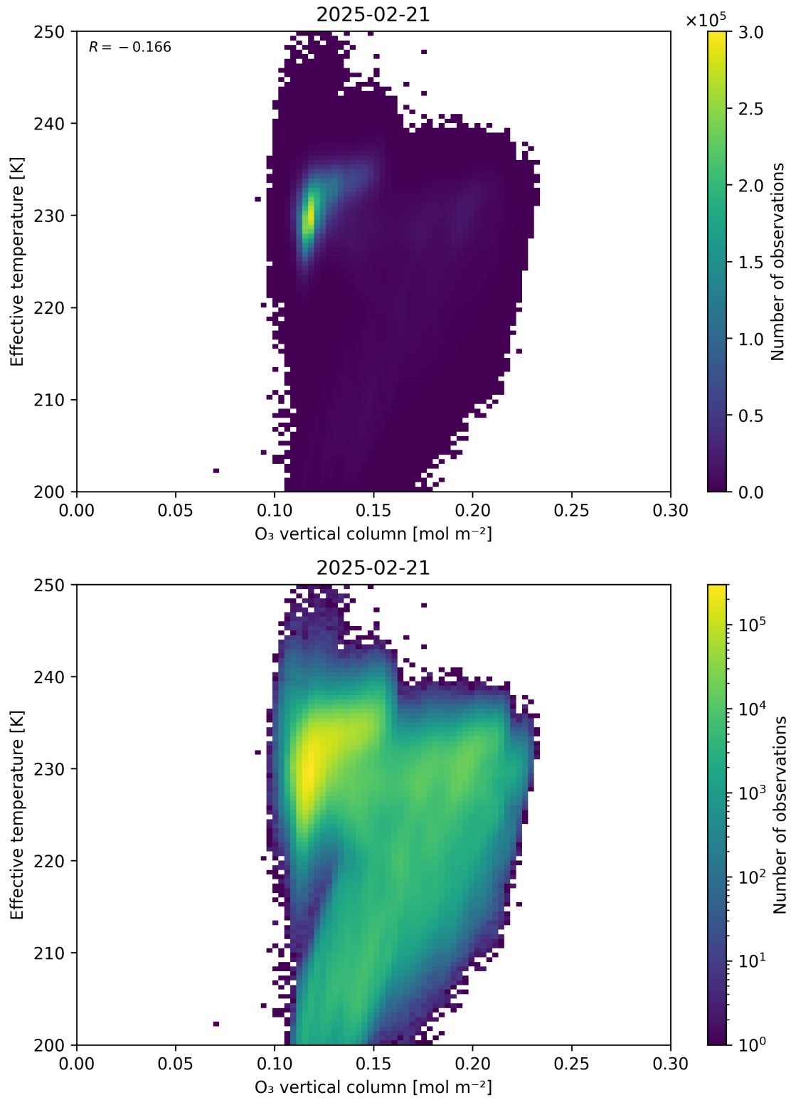
Figure 39: Scatter density plot of “O 3 vertical column” against “Effective temperature” for 2025-02-20 to 2025-02-22.
