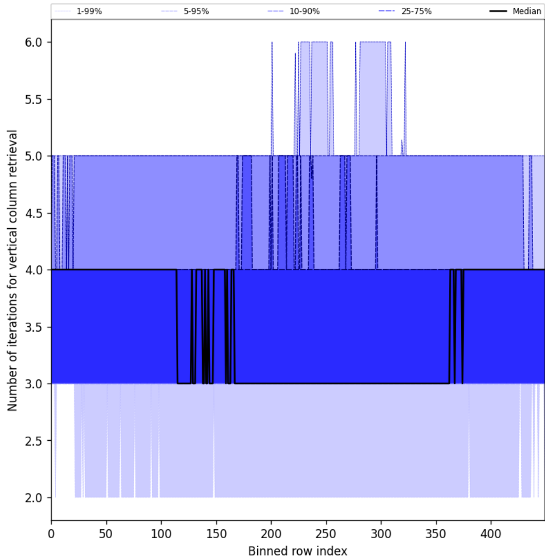
Figure 33: Along track statistics of “Number of iterations for vertical column retrieval” for 2025-02-20 to 2025-02-22
