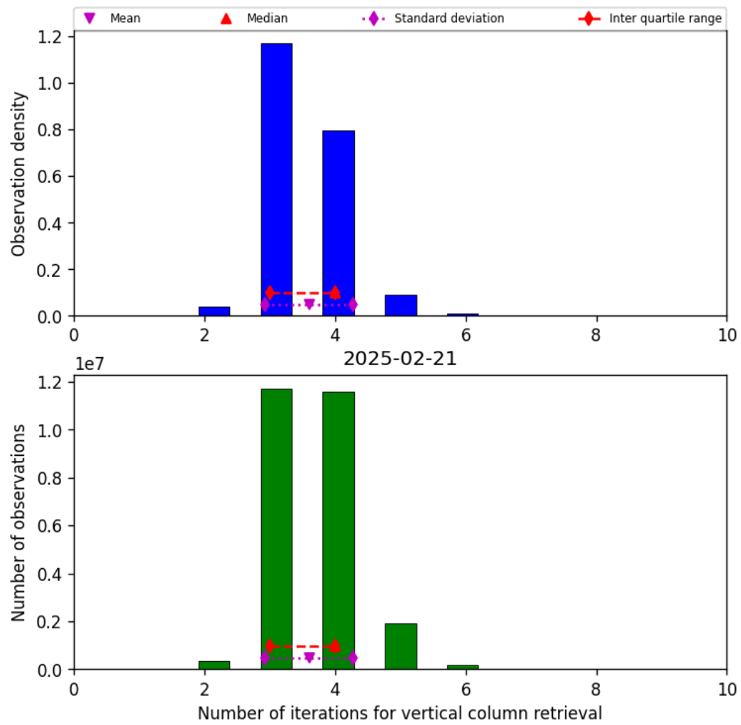
Figure 26: Histogram of “Number of iterations for vertical column retrieval” for 2025-02-20 to 2025-02-22
