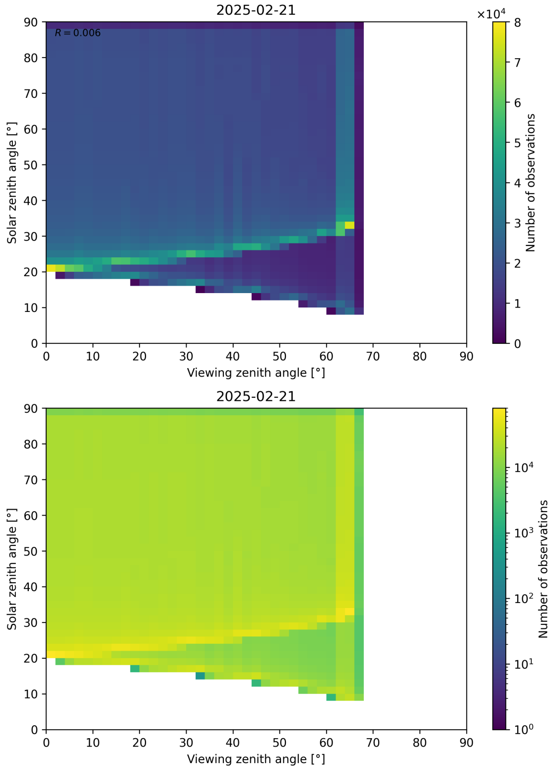
Figure 54: Scatter density plot of “Viewing zenith angle” against “Solar zenith angle” for 2025-02-20 to 2025-02-22.
