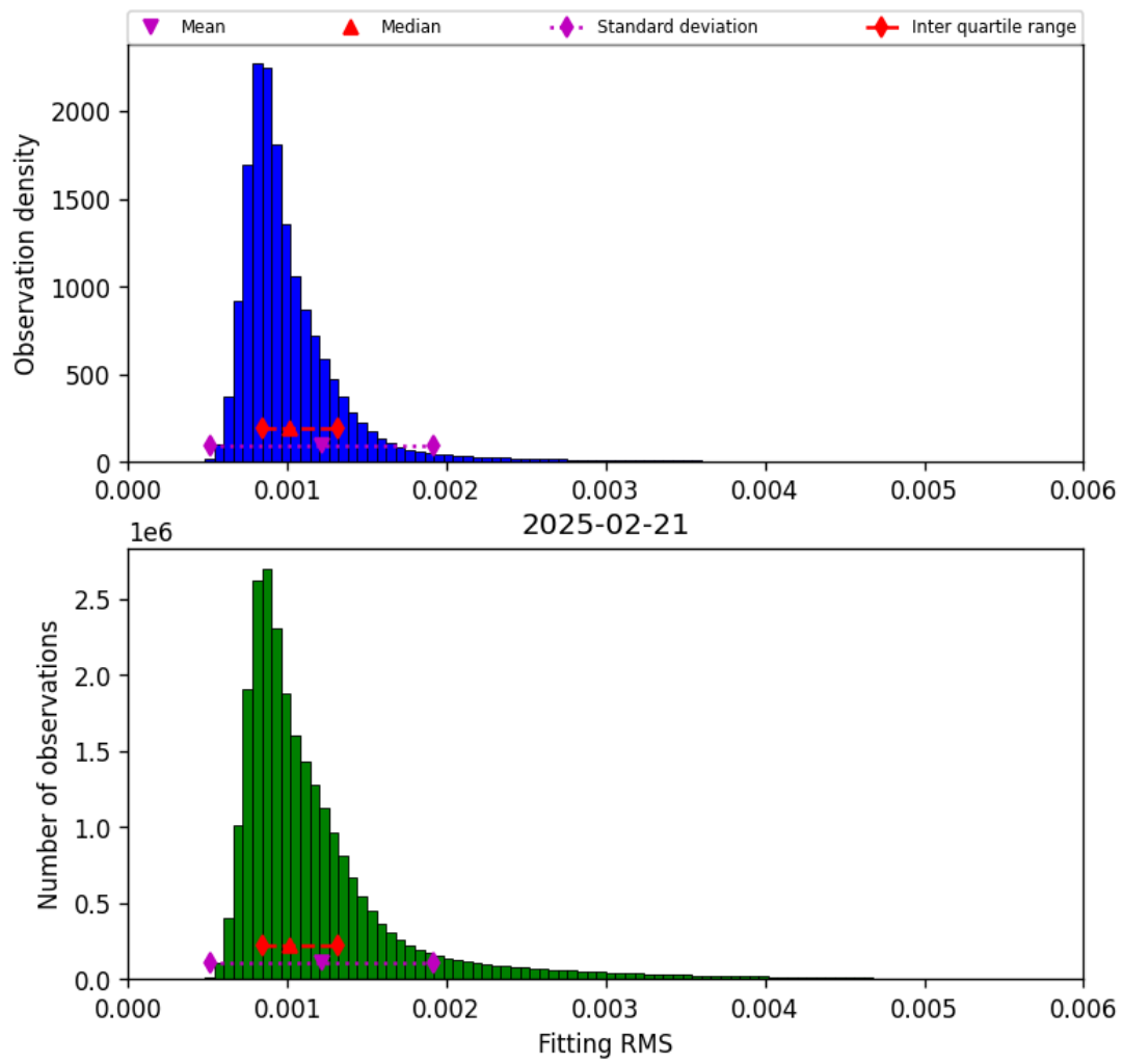
Figure 23: Histogram of “Fitting RMS” for 2025-02-20 to 2025-02-22
