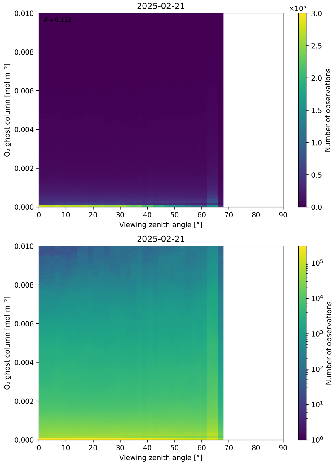
Figure 51: Scatter density plot of “Viewing zenith angle” against “O 3 ghost column” for 2025-02-20 to 2025-02-22.
