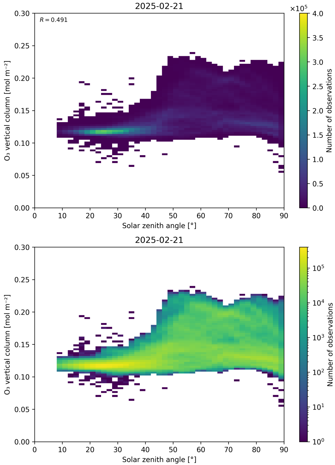
Figure 47: Scatter density plot of “Solar zenith angle” against “O 3 vertical column” for 2025-02-20 to 2025-02-22.
