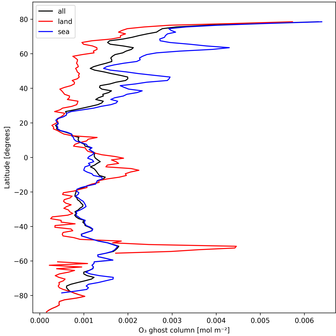
Figure 18: Zonal average of "O 3 ghost column" for 2025-02-20 to 2025-02-22.
