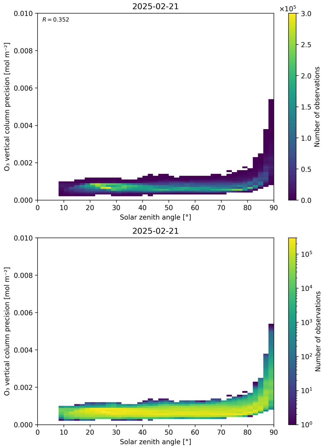
Figure 48: Scatter density plot of “Solar zenith angle” against “O 3 vertical column precision” for 2025-02-20 to 2025-02-22.
