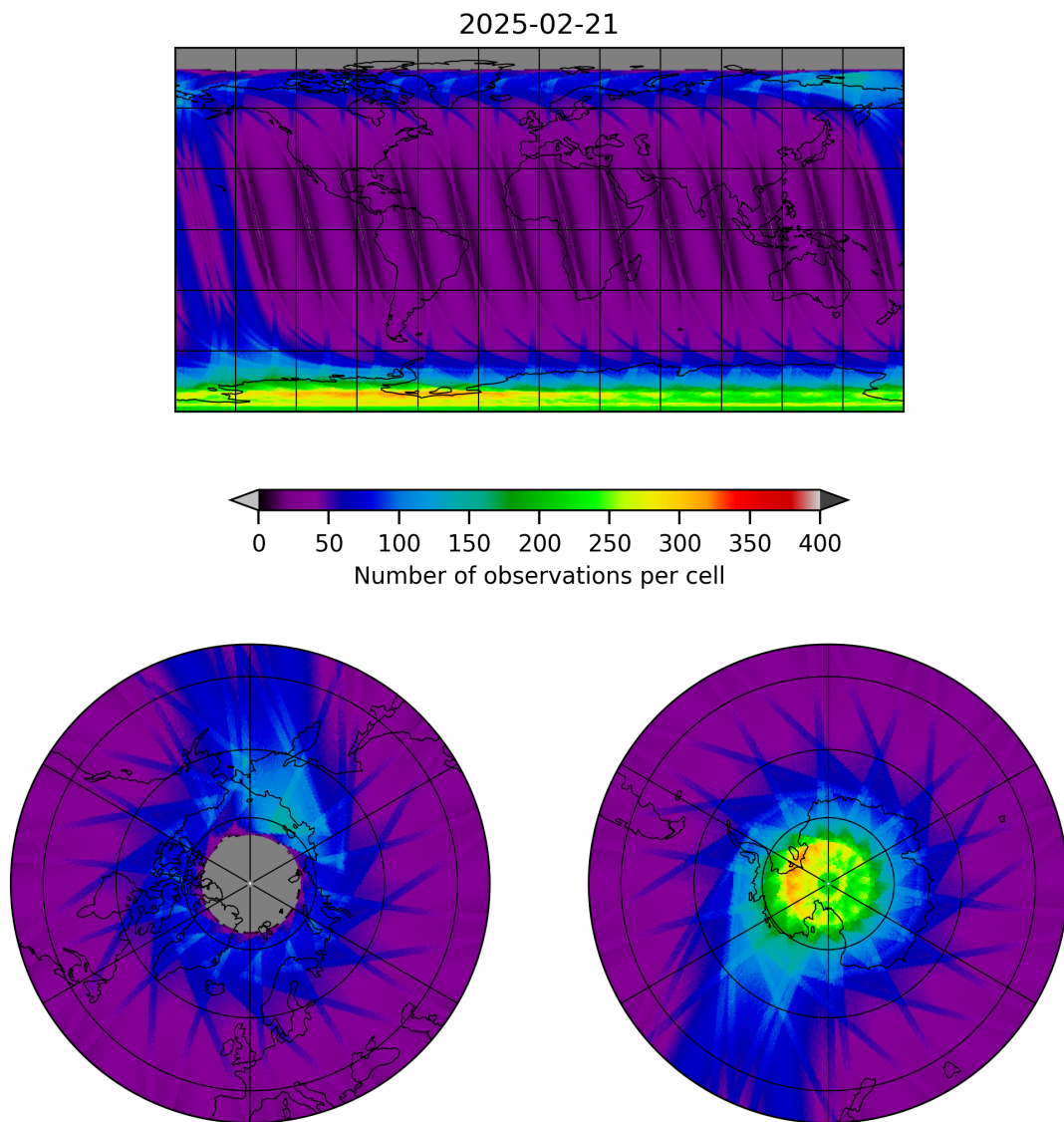
Figure 12: Map of the number of observations for 2025-02-20 to 2025-02-22
