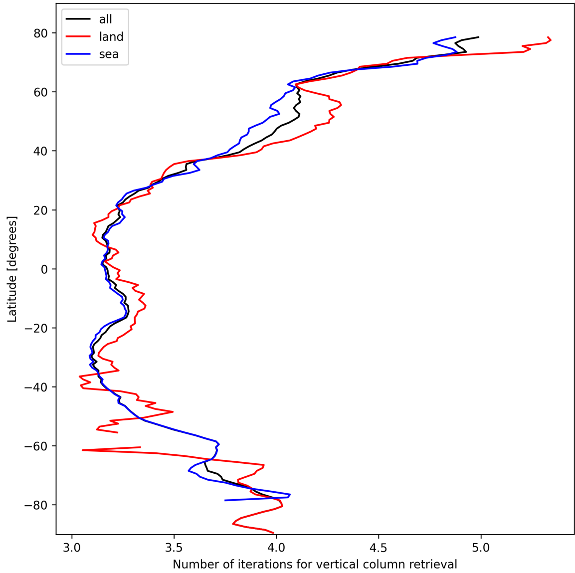
Figure 19: Zonal average of “Number of iterations for vertical column retrieval” for 2025-02-20 to 2025-02-22.
