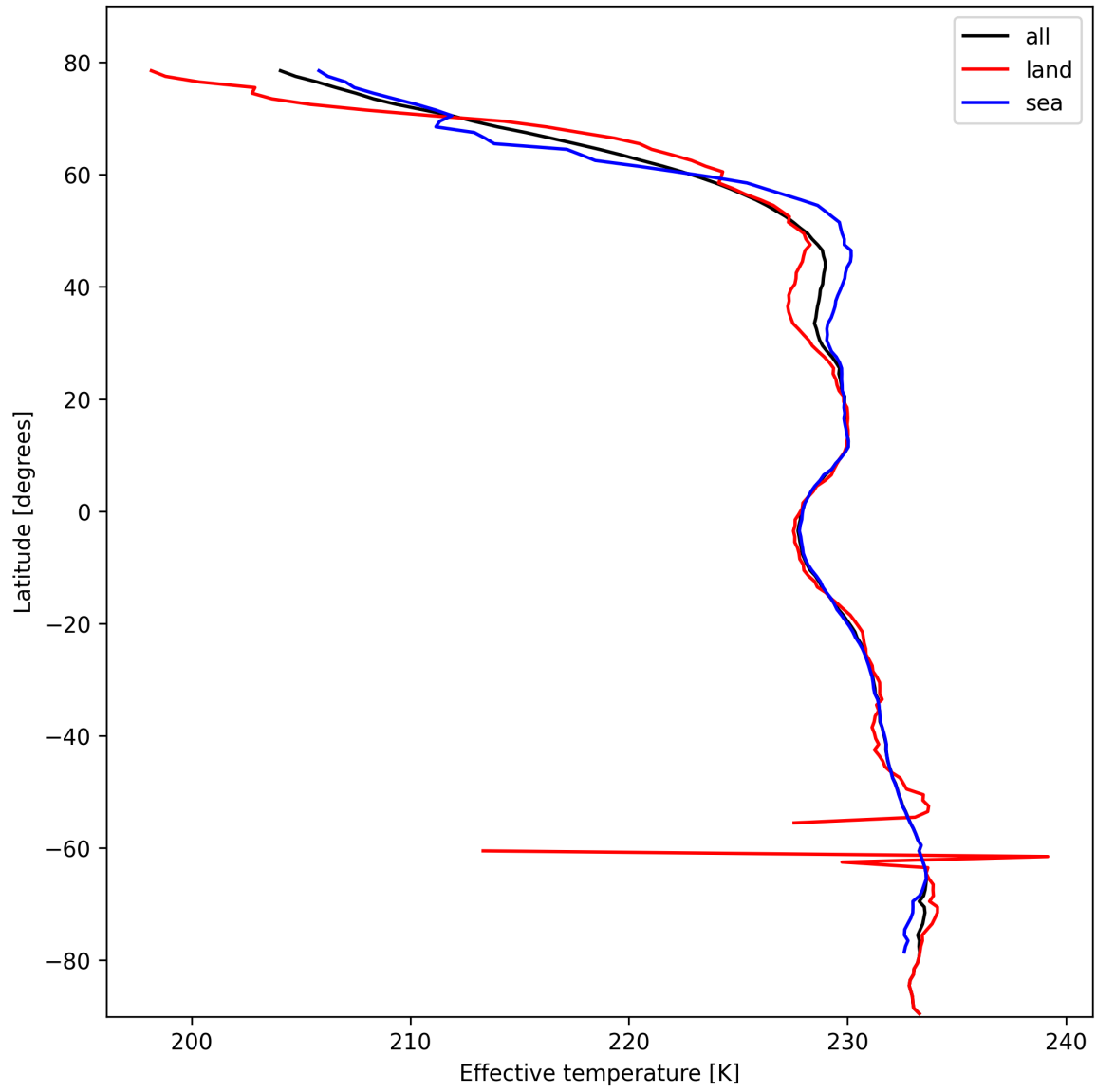
Figure 17: Zonal average of “Effective temperature” for 2025-02-20 to 2025-02-22.
