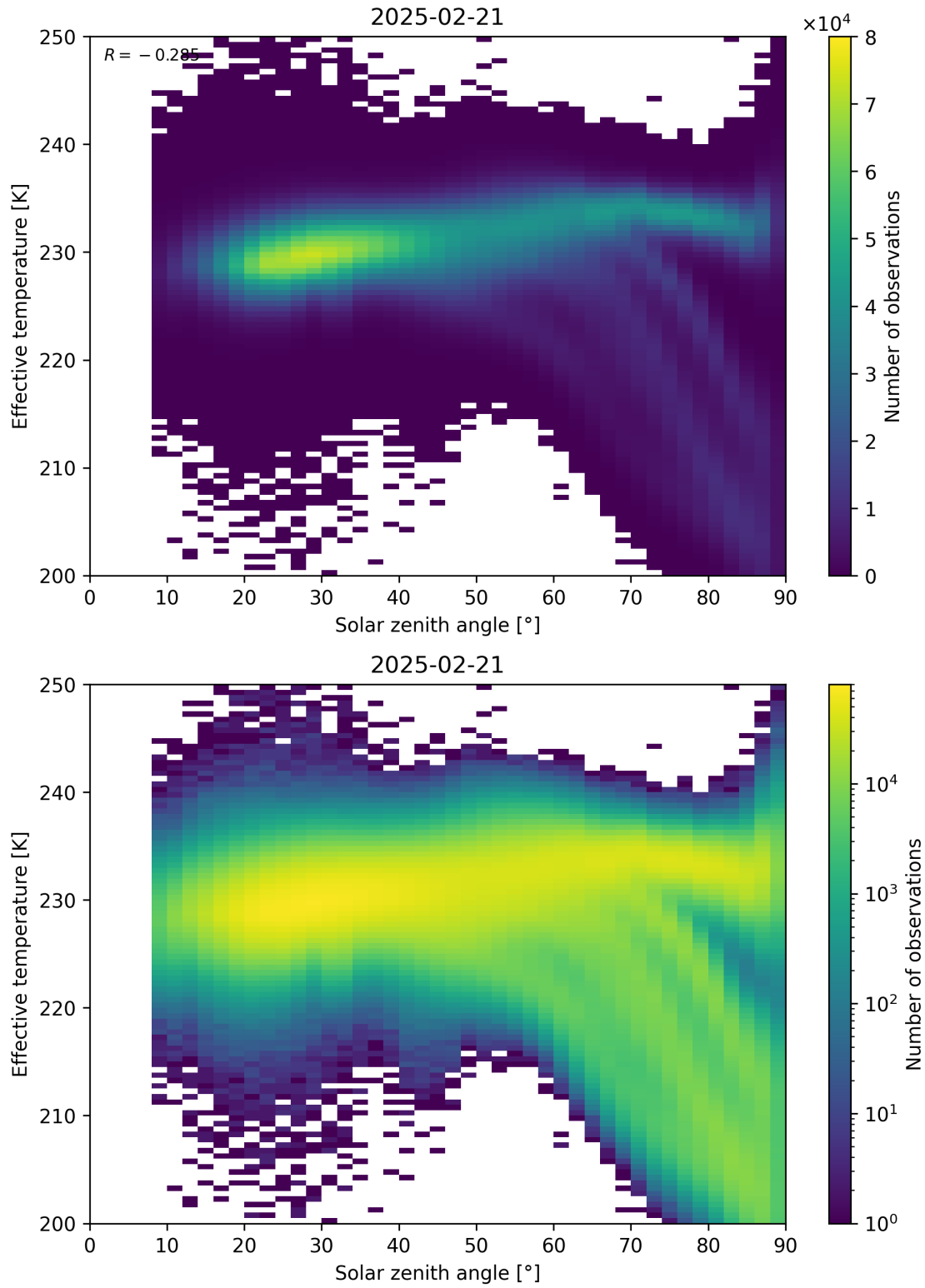
Figure 45: Scatter density plot of “Solar zenith angle” against “Effective temperature” for 2025-02-20 to 2025-02-22.
