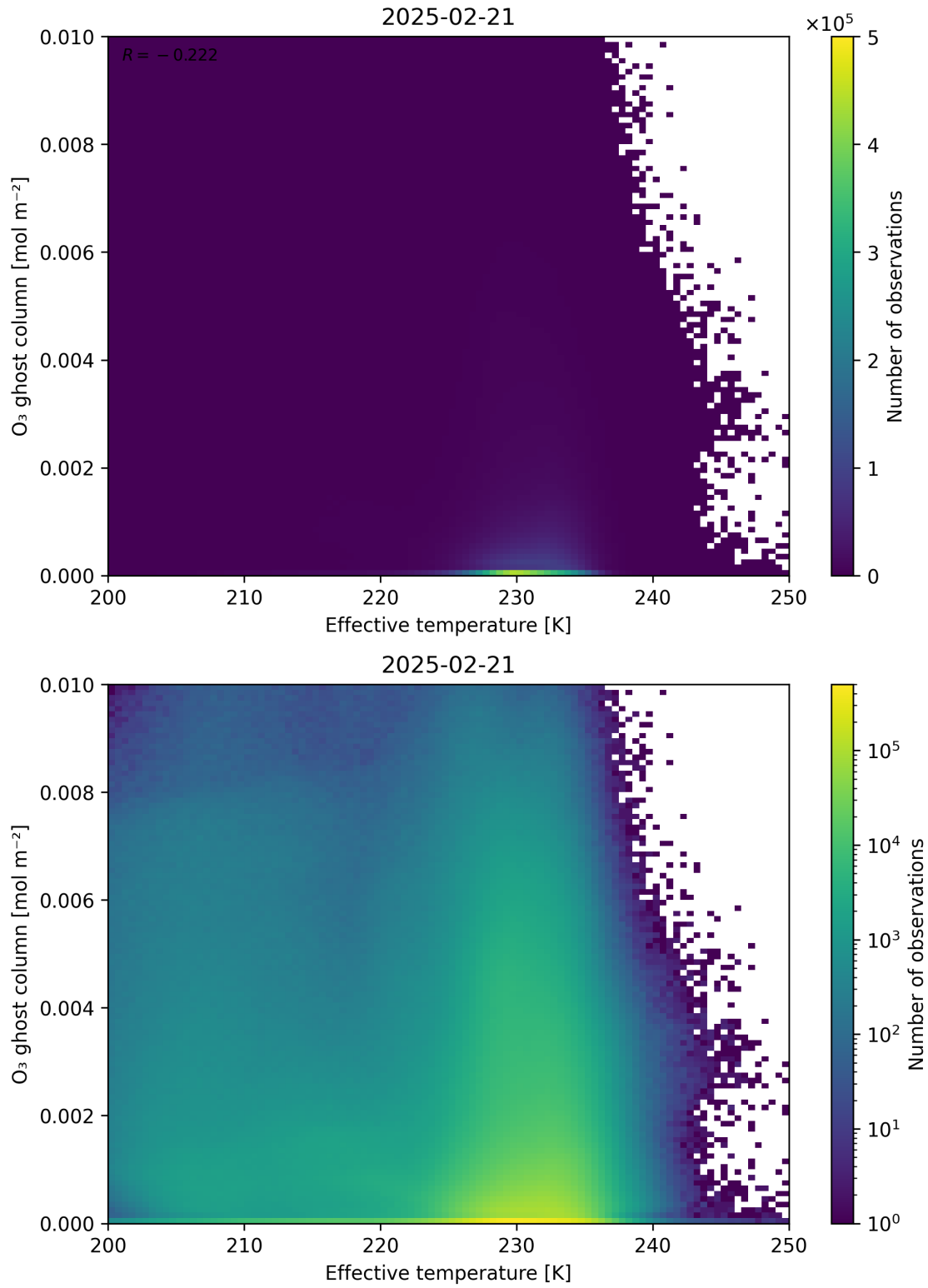
Figure 38: Scatter density plot of “Effective temperature” against “O 3 ghost column” for 2025-02-20 to 2025-02-22.
