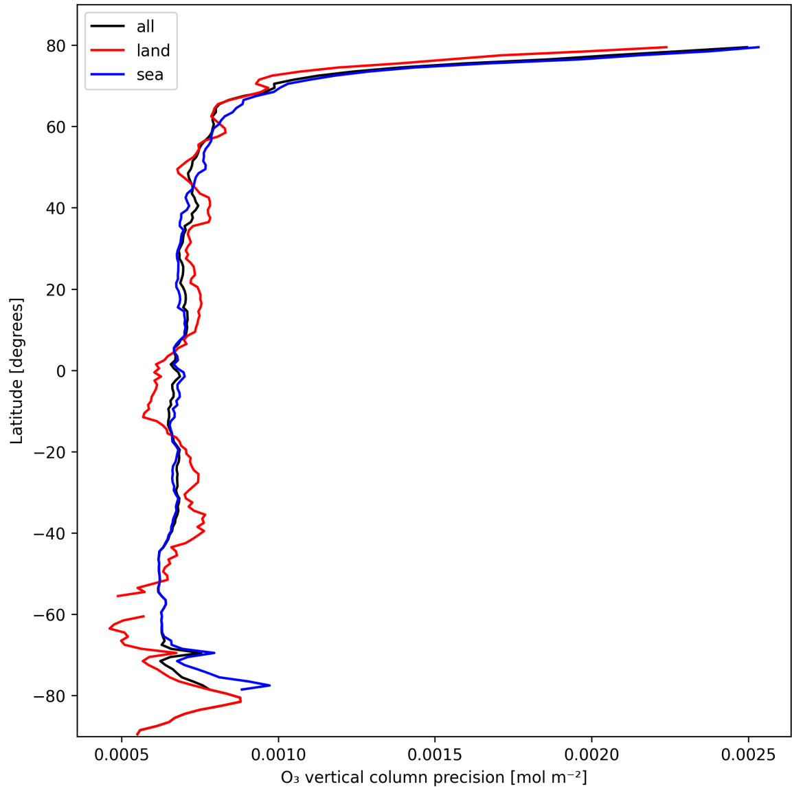
Figure 15: Zonal average of “O 3 vertical column precision” for 2025-02-21 to 2025-02-23.
