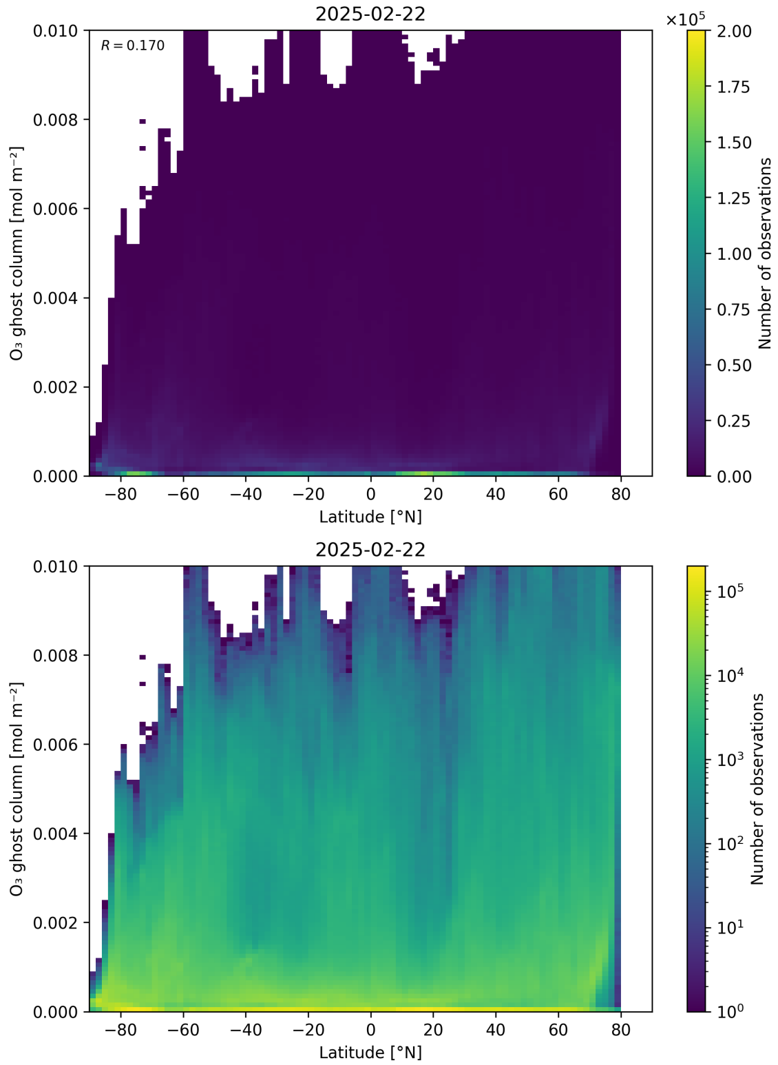
Figure 35: Scatter density plot of “Latitude” against “O 3 ghost column” for 2025-02-21 to 2025-02-23.
