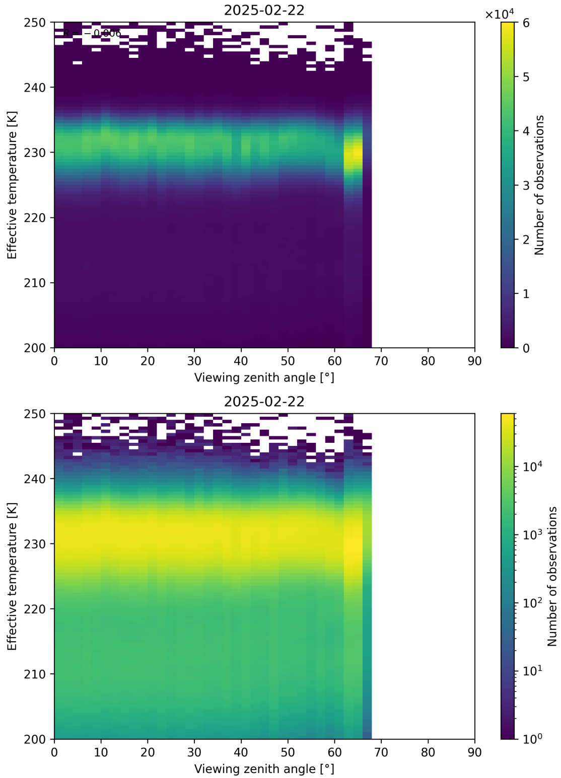
Figure 50: Scatter density plot of “Viewing zenith angle” against “Effective temperature” for 2025-02-21 to 2025-02-23.
