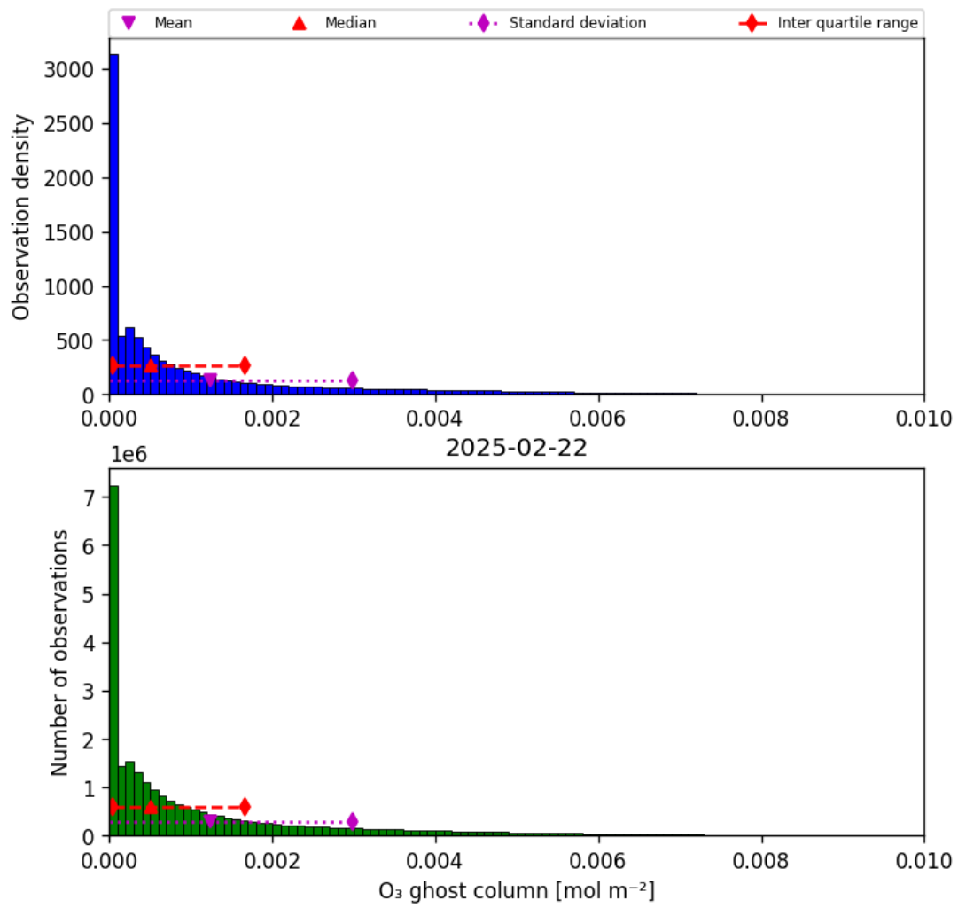
Figure 25: Histogram of "O 3 ghost column" for 2025-02-21 to 2025-02-23
