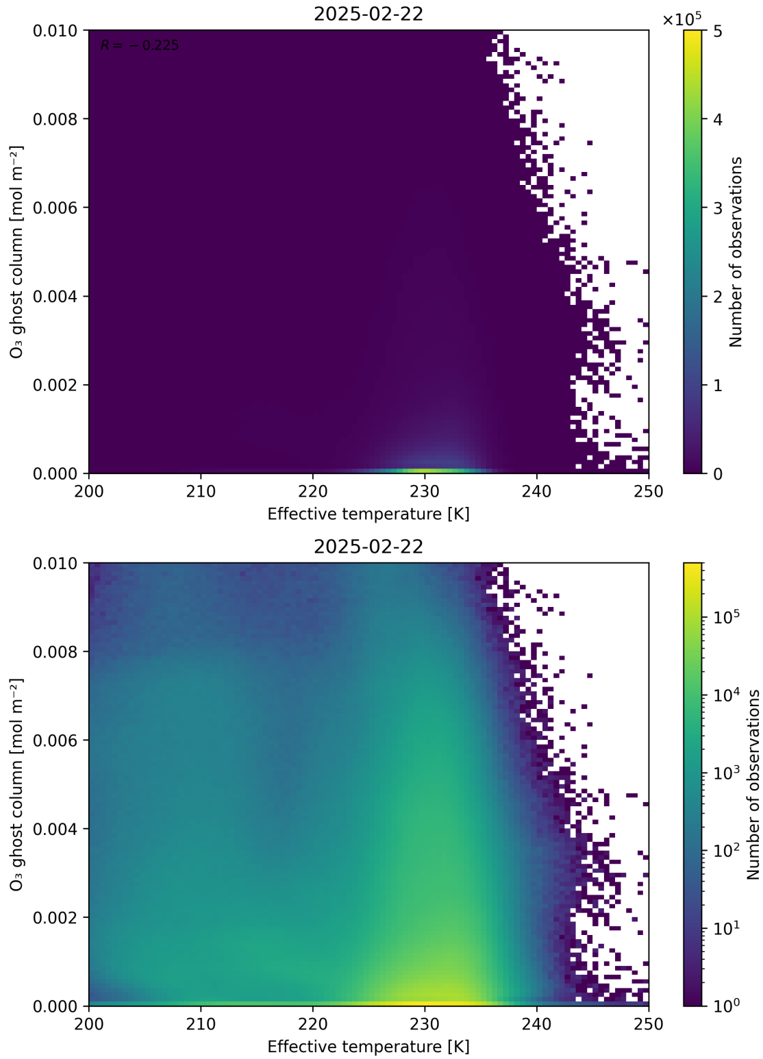
Figure 38: Scatter density plot of “Effective temperature” against “O 3 ghost column” for 2025-02-21 to 2025-02-23.
