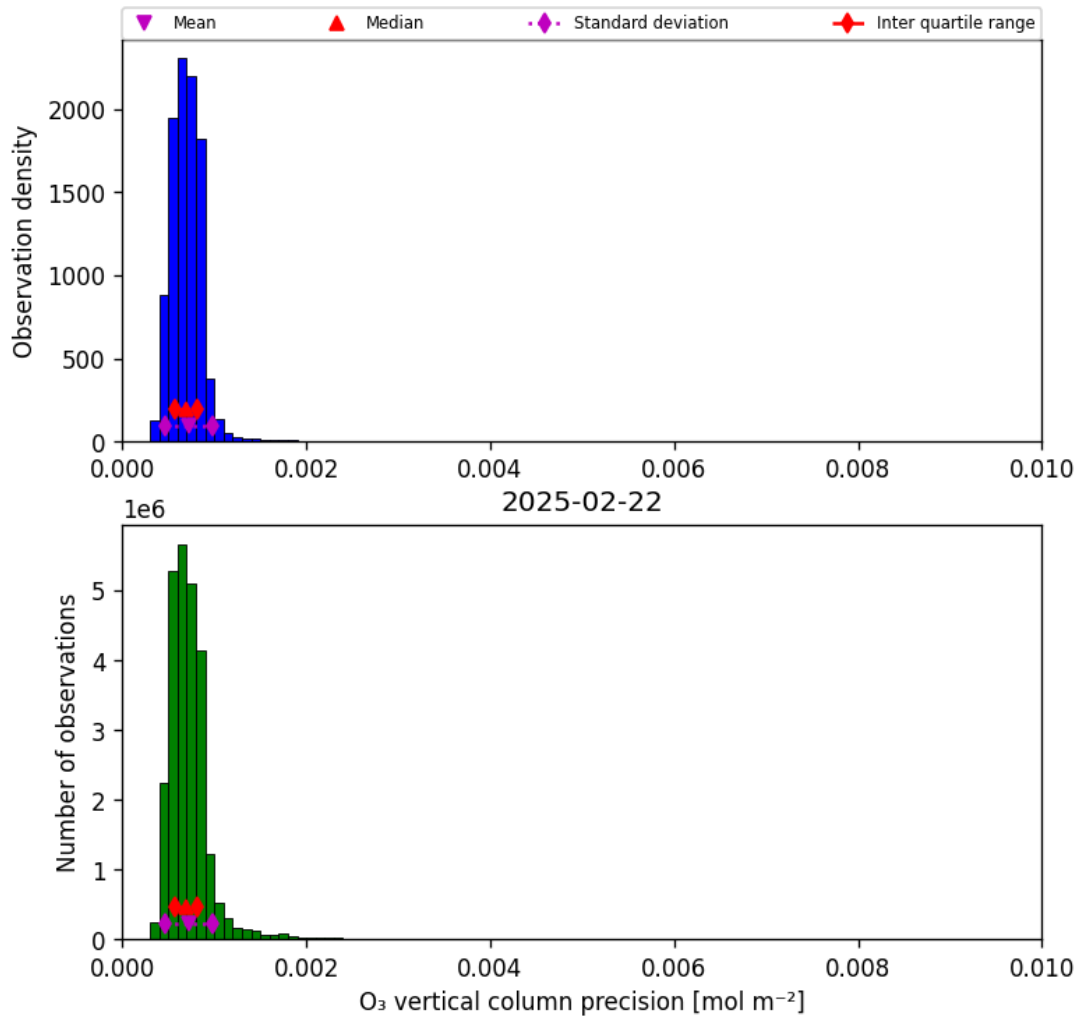
Figure 22: Histogram of “O 3 vertical column precision” for 2025-02-21 to 2025-02-23
