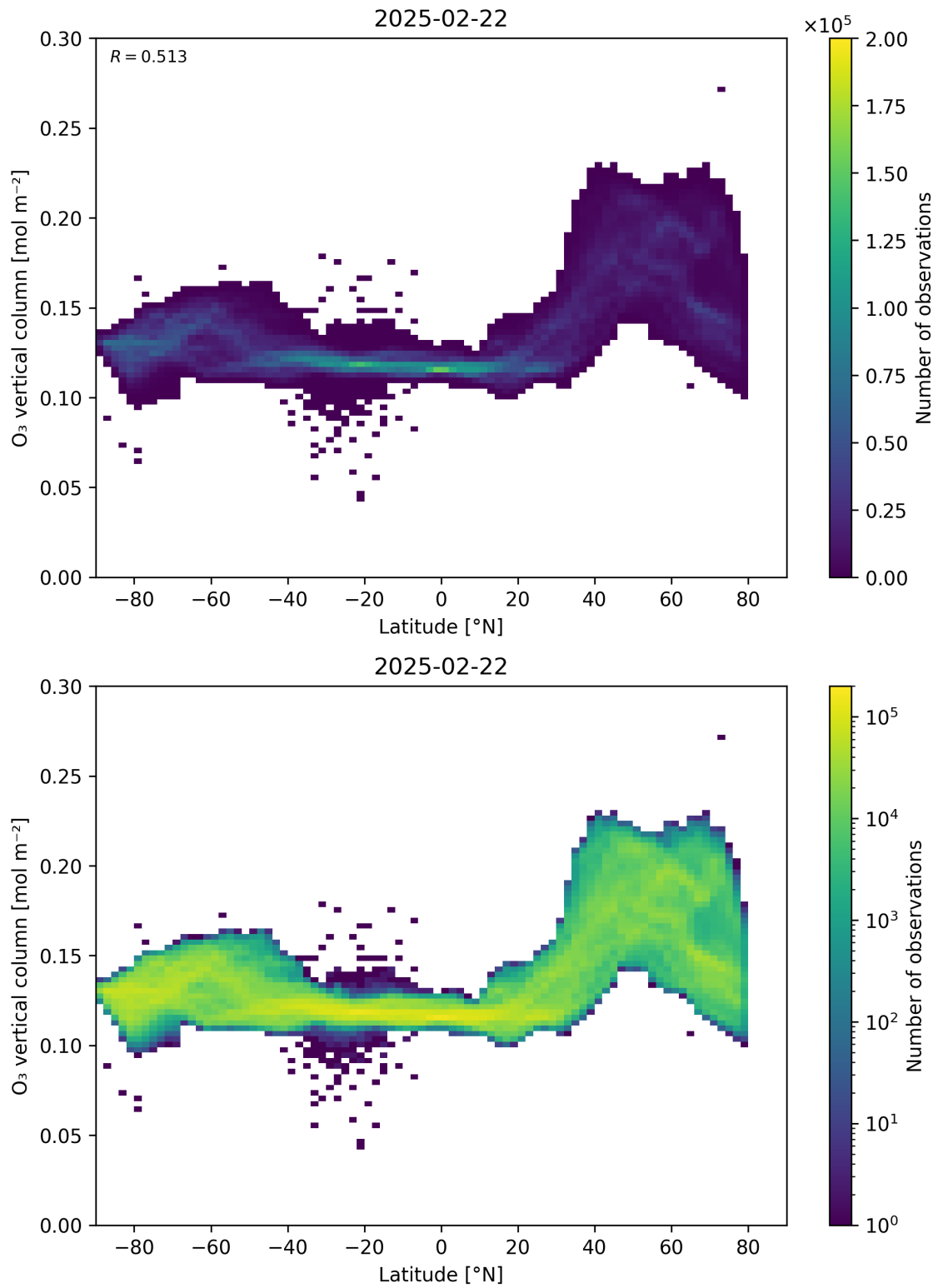
Figure 36: Scatter density plot of “Latitude” against “O 3 vertical column” for 2025-02-21 to 2025-02-23.
