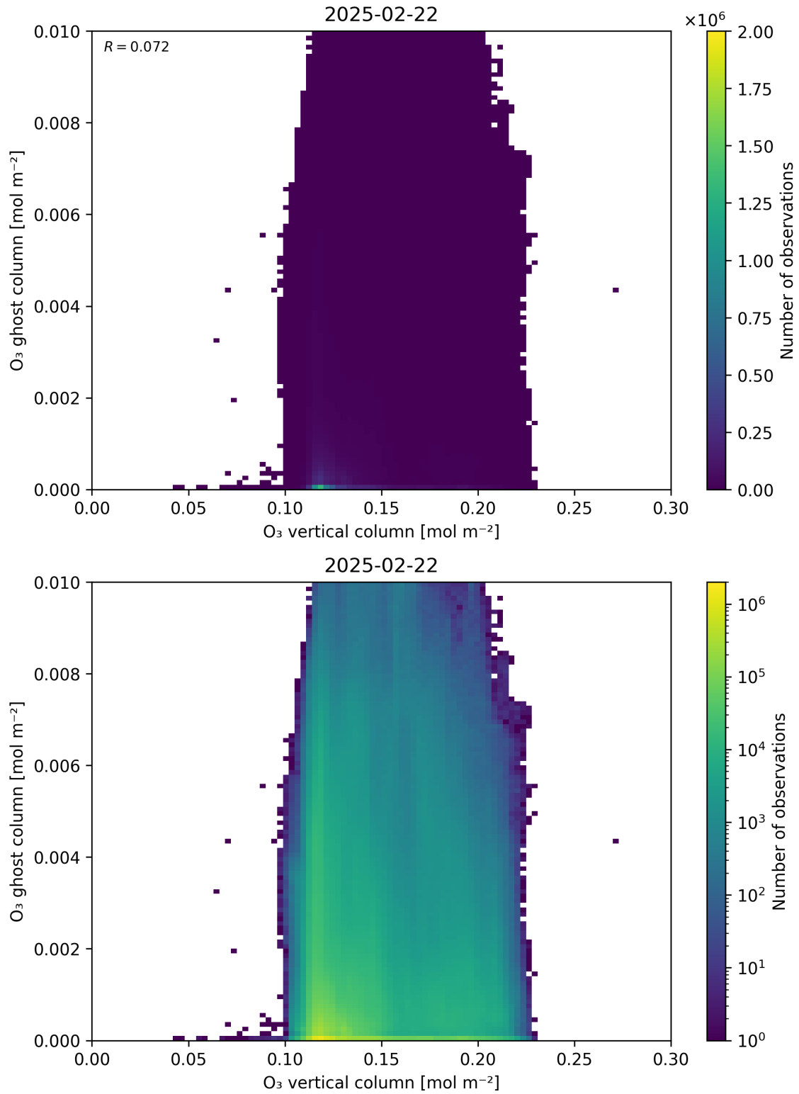
Figure 40: Scatter density plot of “O 3 vertical column” against “O 3 ghost column” for 2025-02-21 to 2025-02-23.
