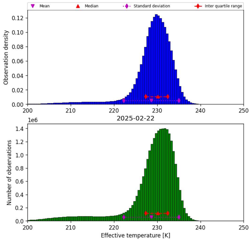
Figure 24: Histogram of “Effective temperature” for 2025-02-21 to 2025-02-23
