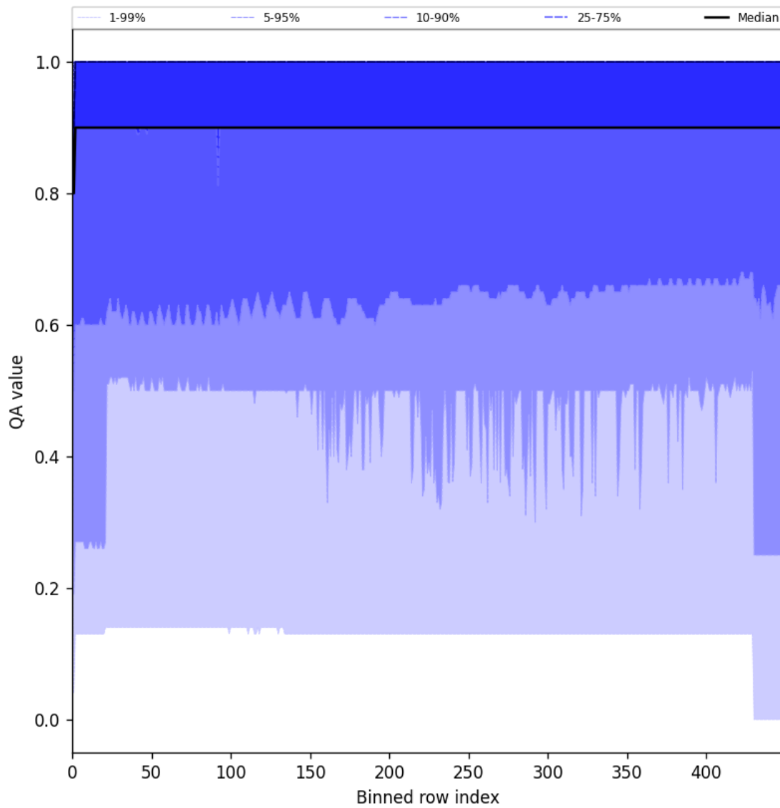
Figure 27: Along track statistics of “QA value” for 2025-02-21 to 2025-02-23
