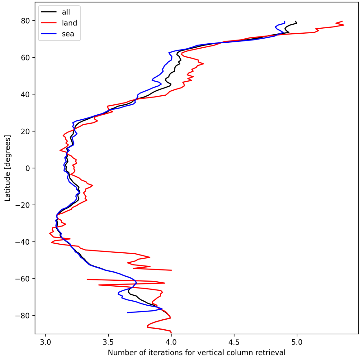
Figure 19: Zonal average of “Number of iterations for vertical column retrieval” for 2025-02-21 to 2025-02-23.
