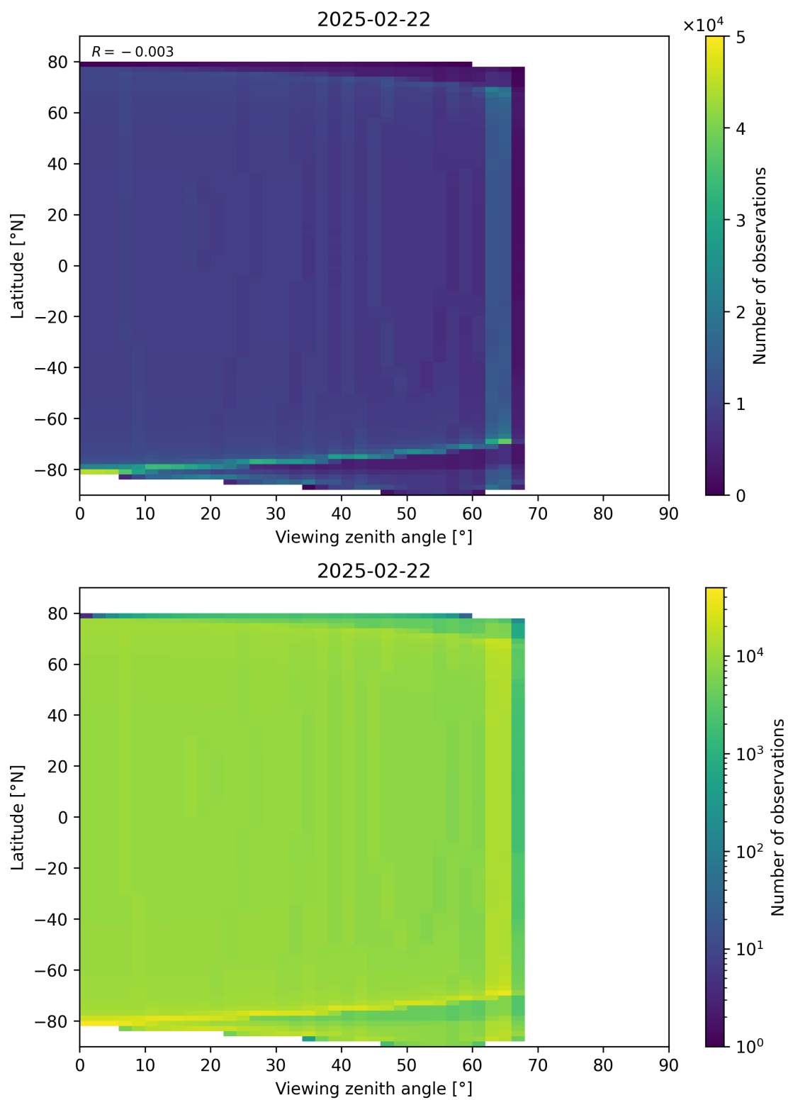
Figure 49: Scatter density plot of “Viewing zenith angle” against “Latitude” for 2025-02-21 to 2025-02-23.
