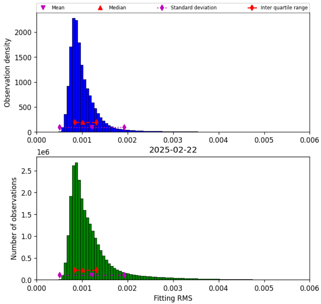
Figure 23: Histogram of “Fitting RMS” for 2025-02-21 to 2025-02-23
