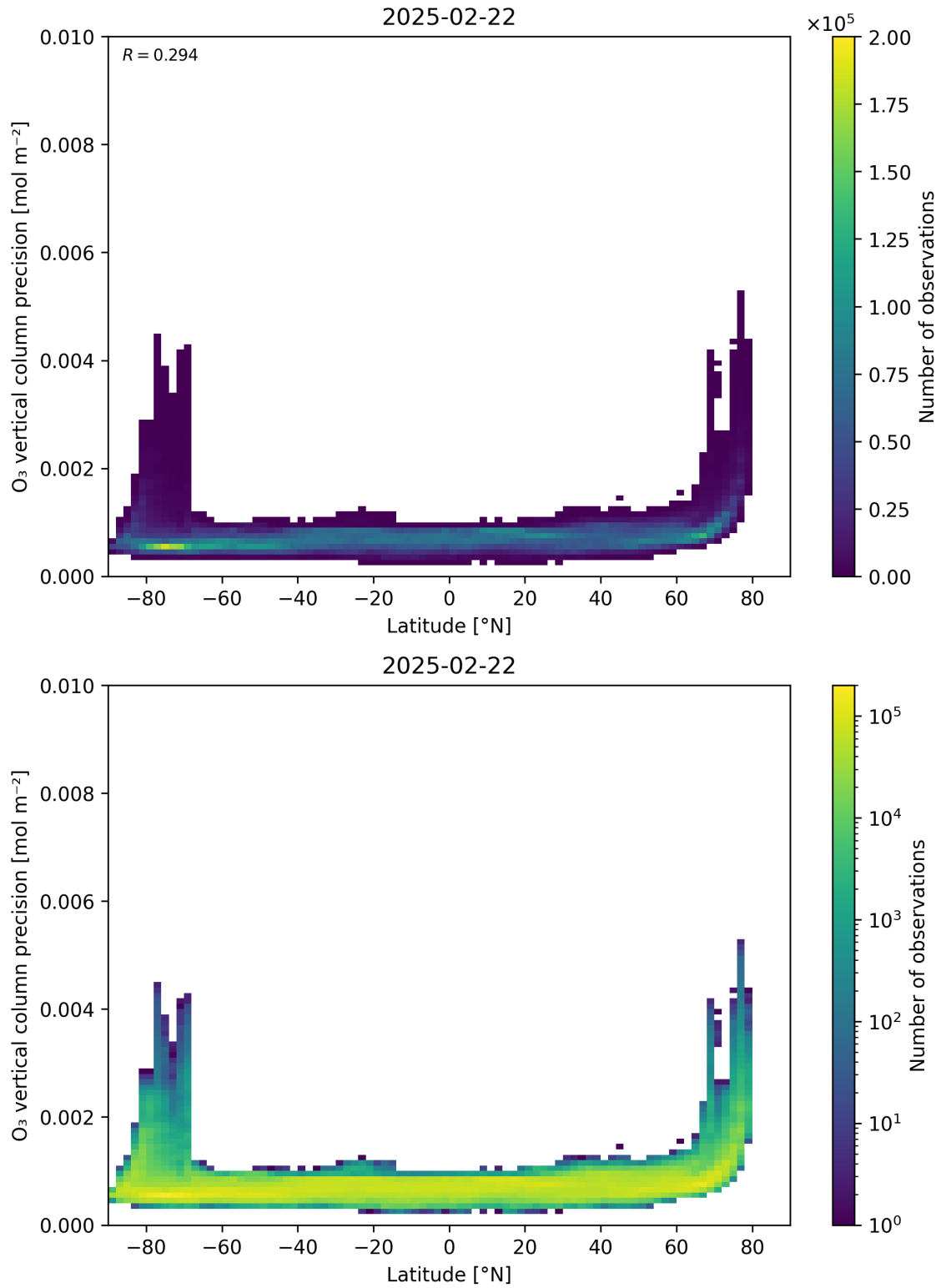
Figure 37: Scatter density plot of “Latitude” against “O 3 vertical column precision” for 2025-02-21 to 2025-02-23.
