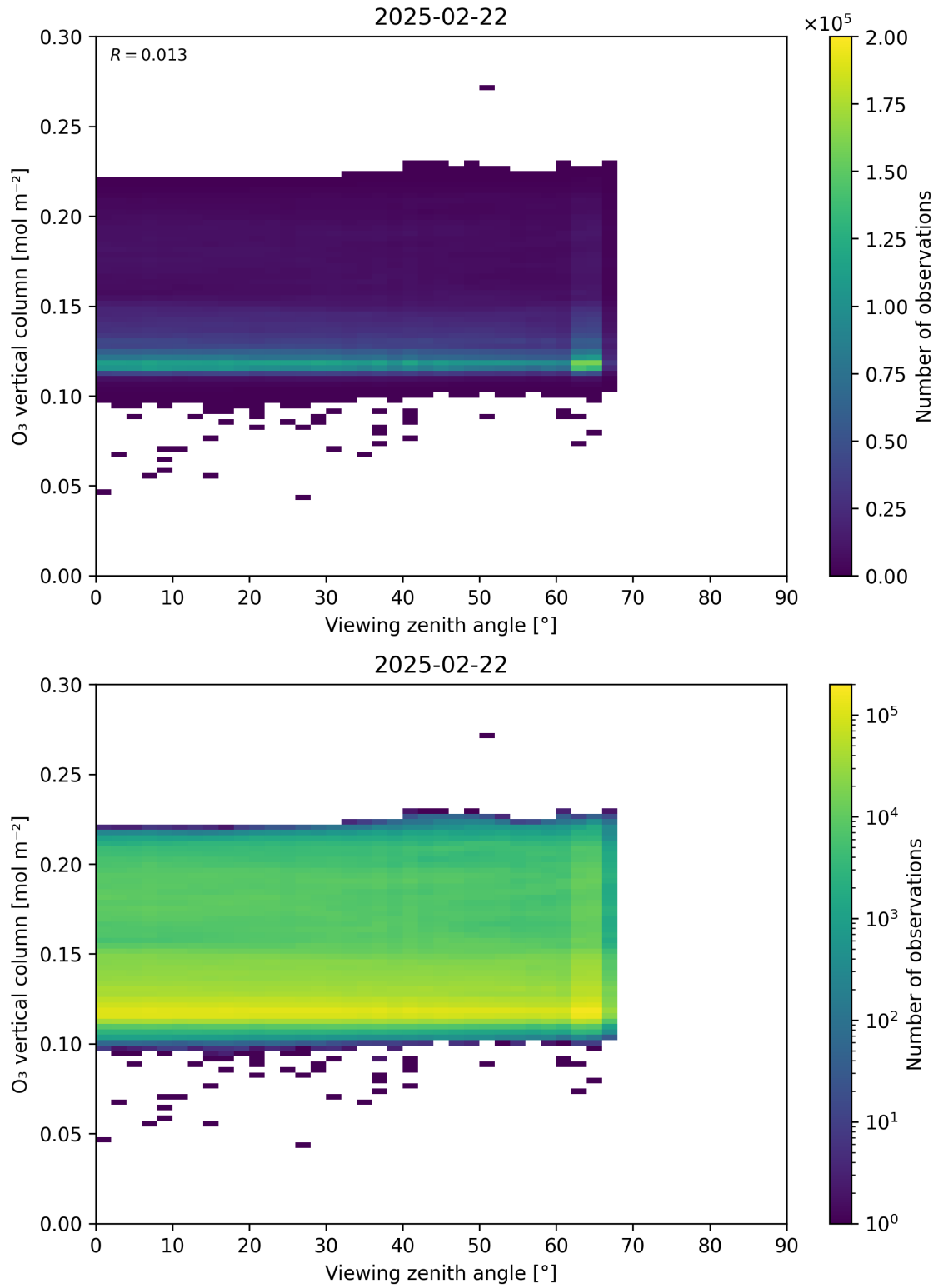
Figure 52: Scatter density plot of “Viewing zenith angle” against “O 3 vertical column” for 2025-02-21 to 2025-02-23.
