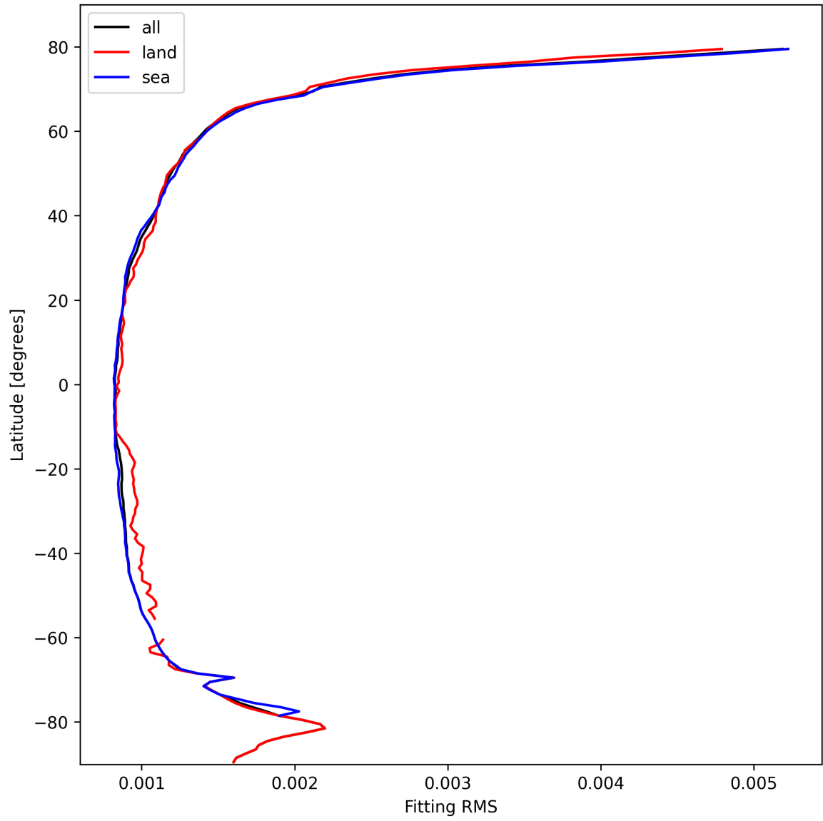
Figure 16: Zonal average of “Fitting RMS” for 2025-02-21 to 2025-02-23.
