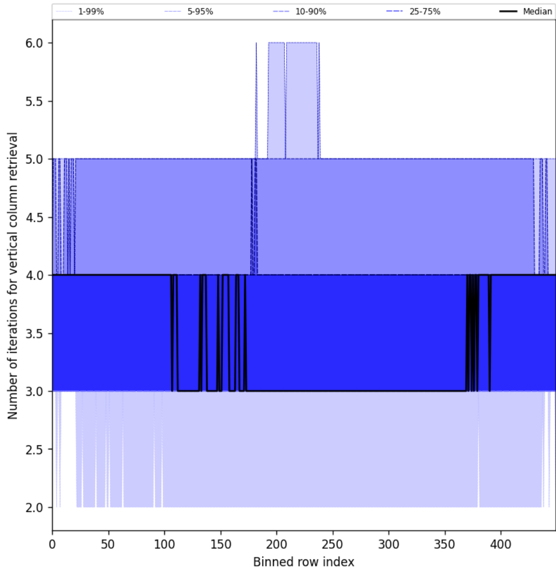
Figure 33: Along track statistics of “Number of iterations for vertical column retrieval” for 2025-02-21 to 2025-02-23
