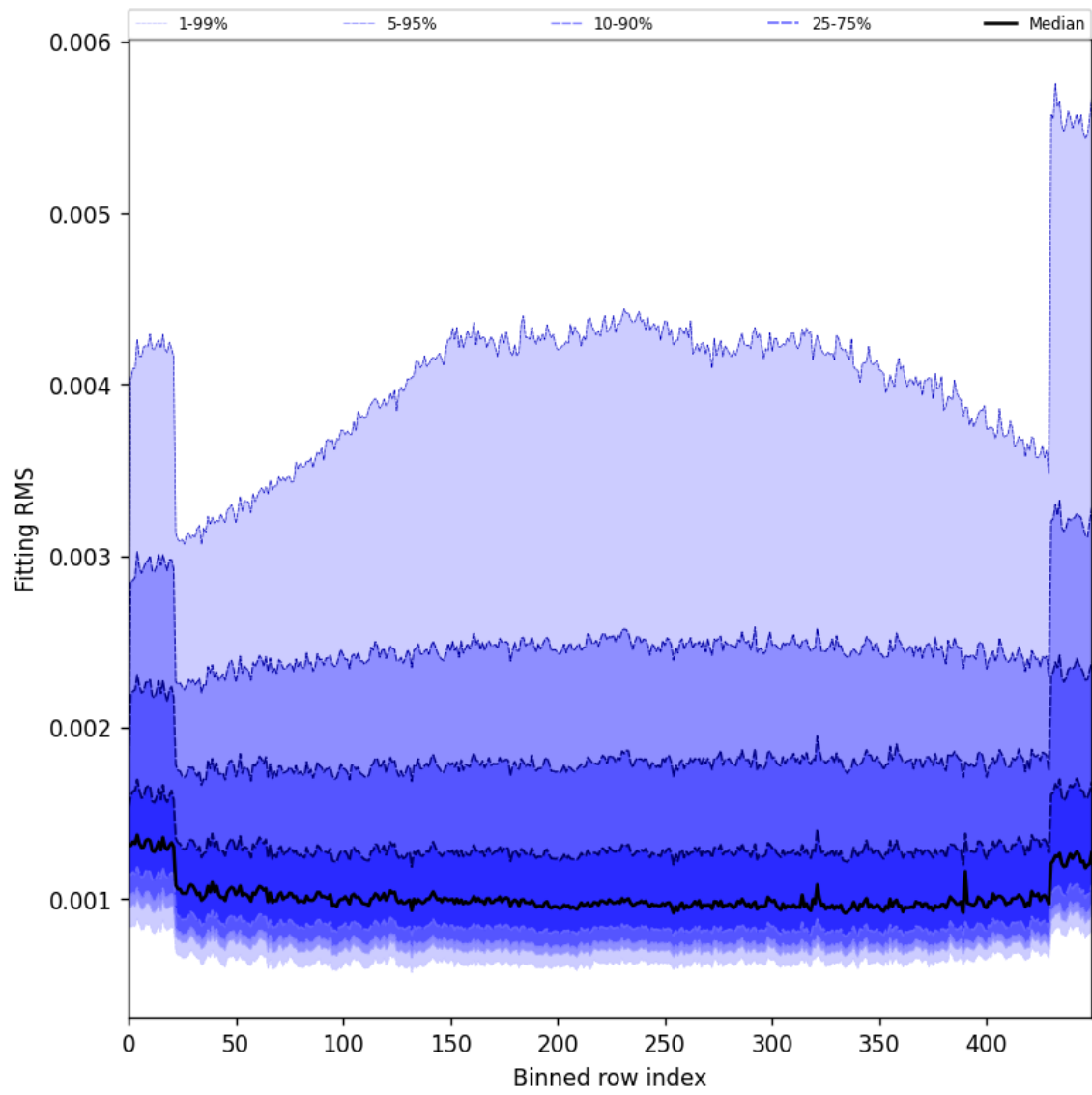
Figure 30: Along track statistics of “Fitting RMS” for 2025-02-21 to 2025-02-23
