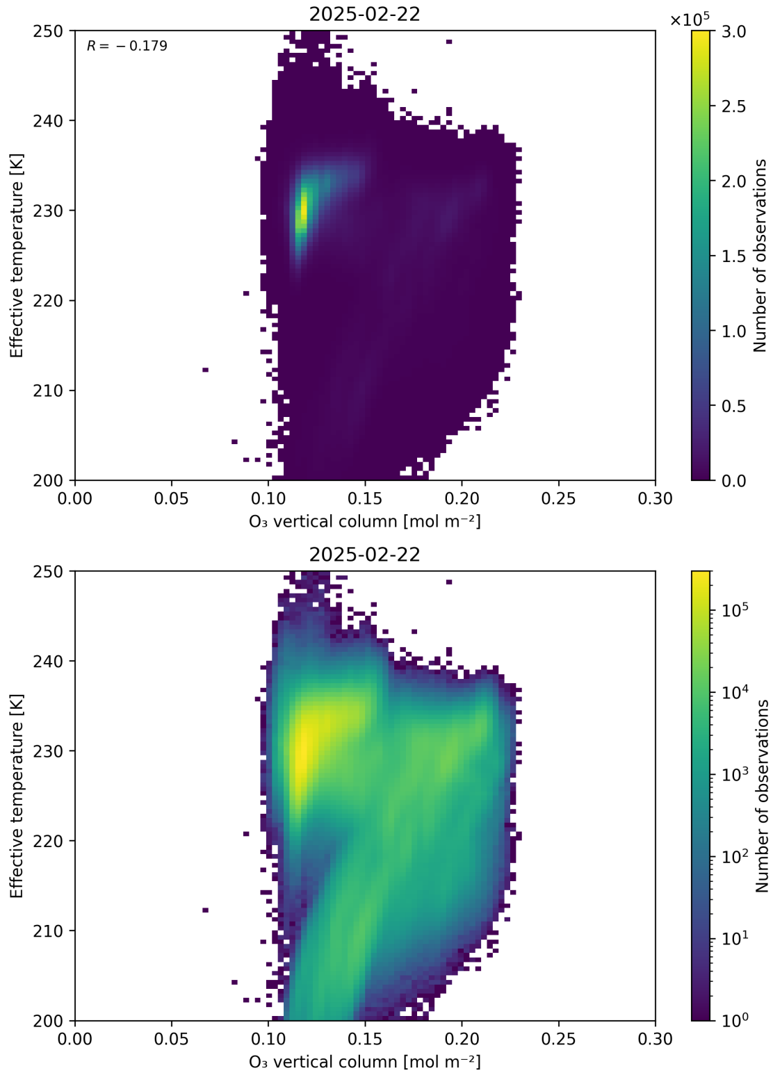
Figure 39: Scatter density plot of “O 3 vertical column” against “Effective temperature” for 2025-02-21 to 2025-02-23.
