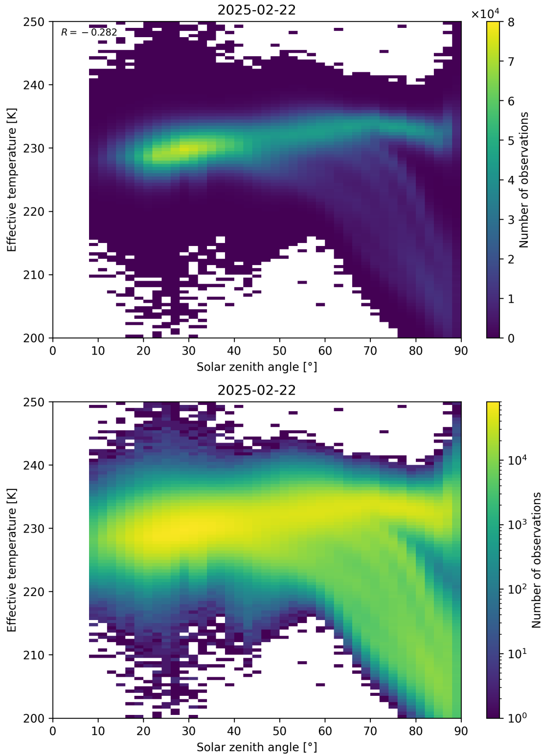
Figure 45: Scatter density plot of “Solar zenith angle” against “Effective temperature” for 2025-02-21 to 2025-02-23.
