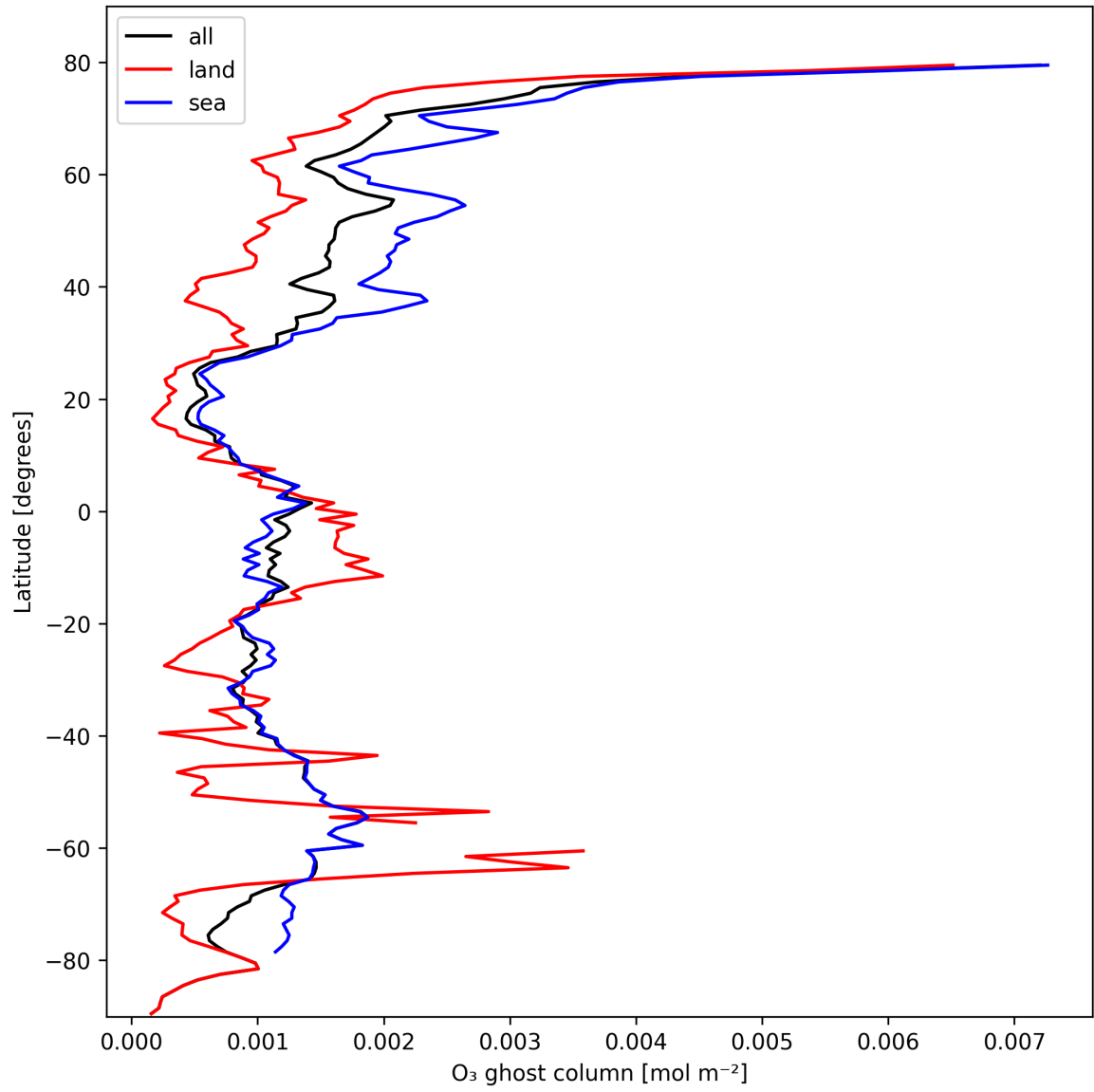
Figure 18: Zonal average of "O 3 ghost column" for 2025-02-21 to 2025-02-23.
