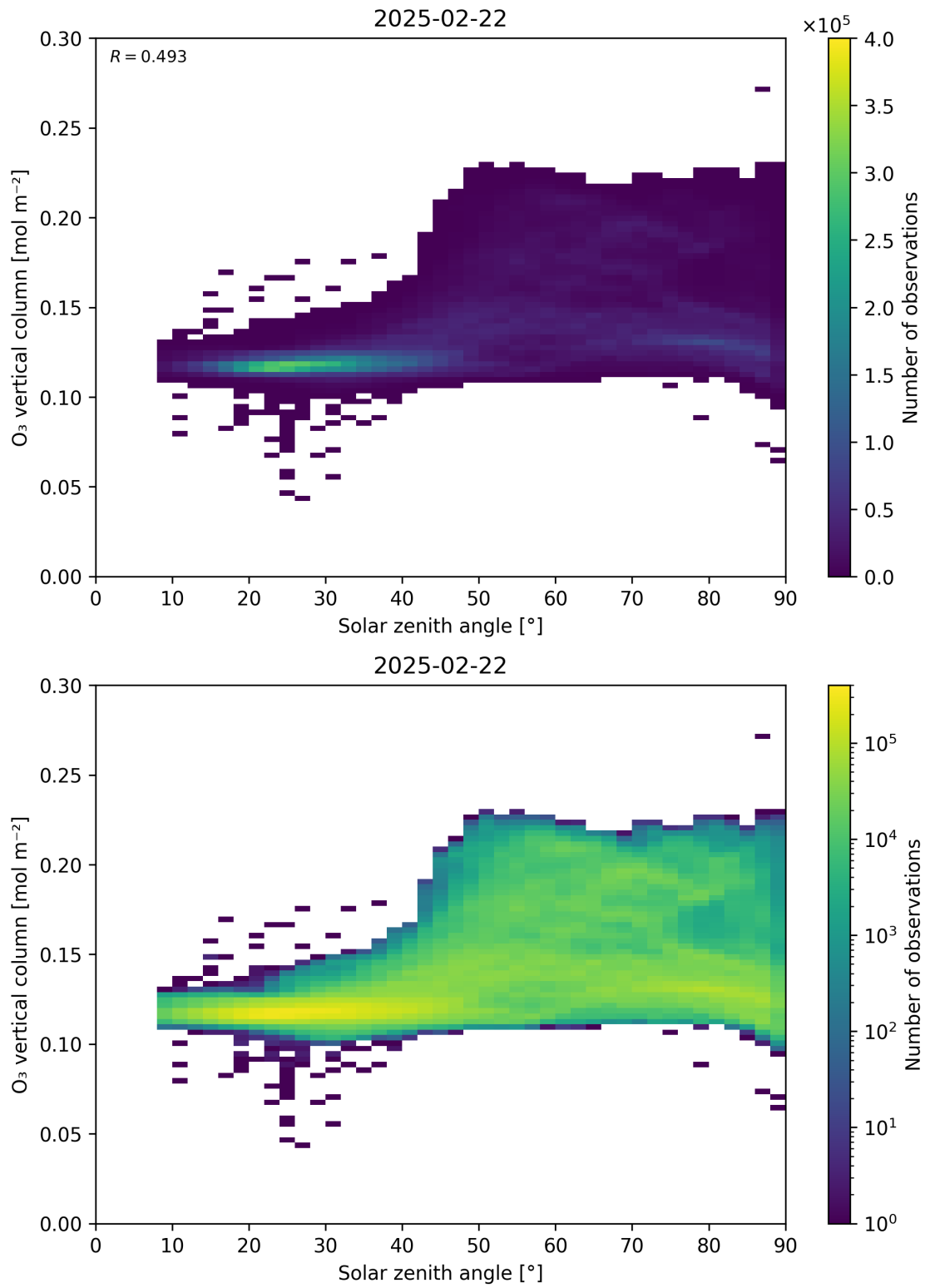
Figure 47: Scatter density plot of “Solar zenith angle” against “O 3 vertical column” for 2025-02-21 to 2025-02-23.
