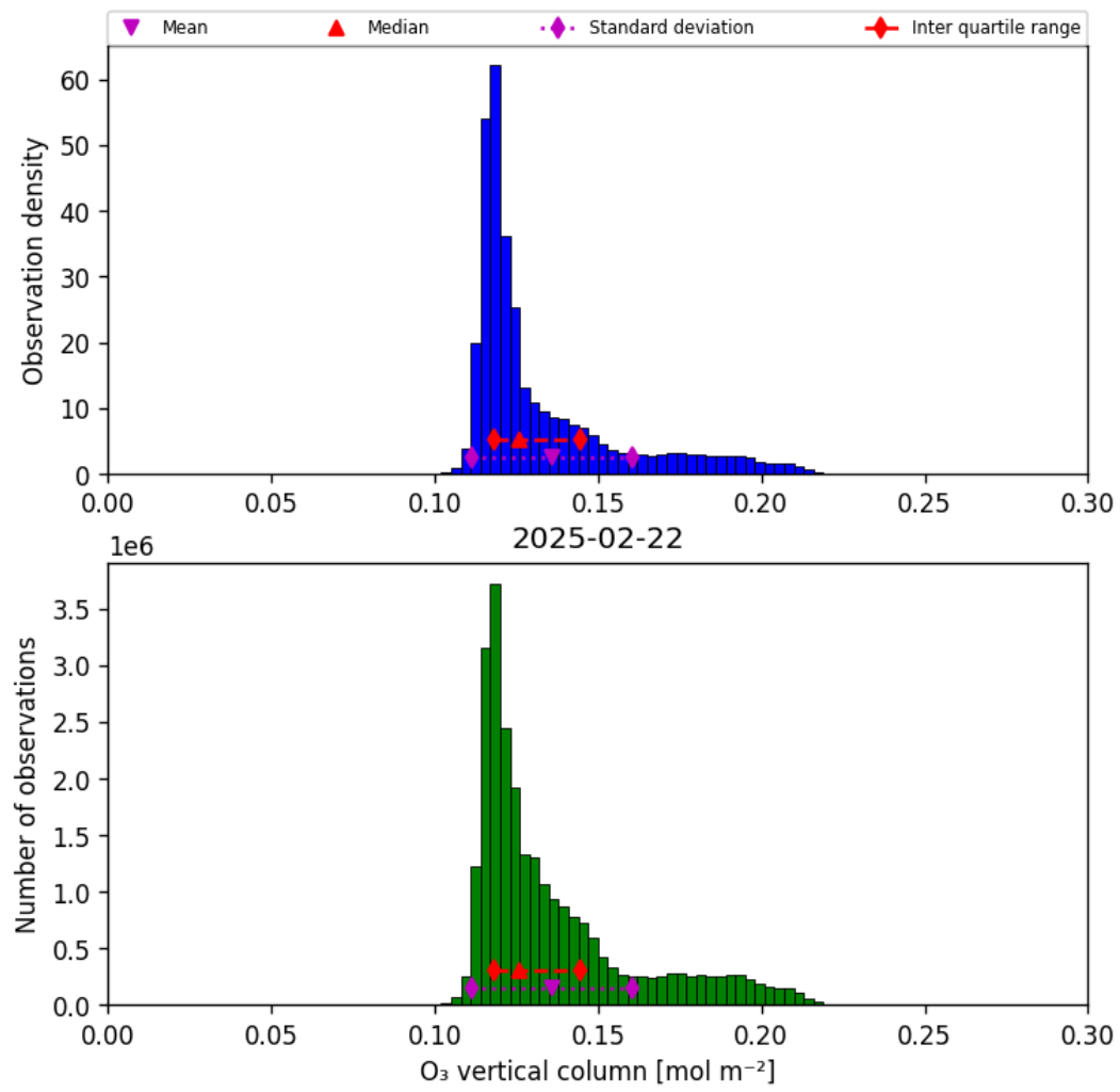
Figure 21: Histogram of “O 3 vertical column” for 2025-02-21 to 2025-02-23
