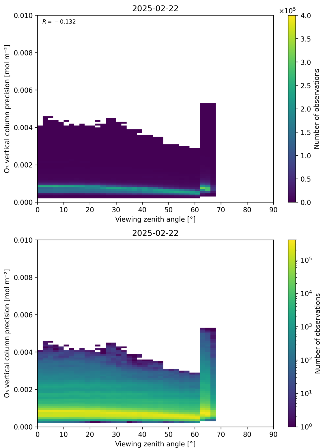
Figure 53: Scatter density plot of “Viewing zenith angle” against “O 3 vertical column precision” for 2025-02-21 to 2025-02-23.
