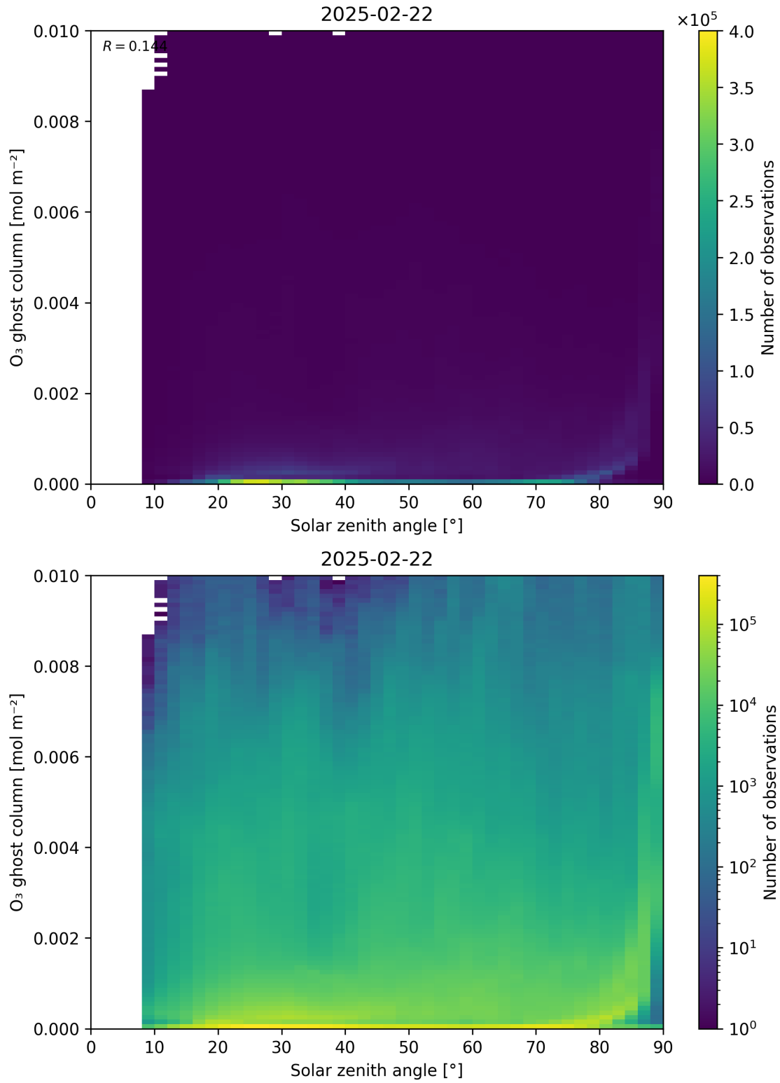
Figure 46: Scatter density plot of “Solar zenith angle” against “O 3 ghost column” for 2025-02-21 to 2025-02-23.
