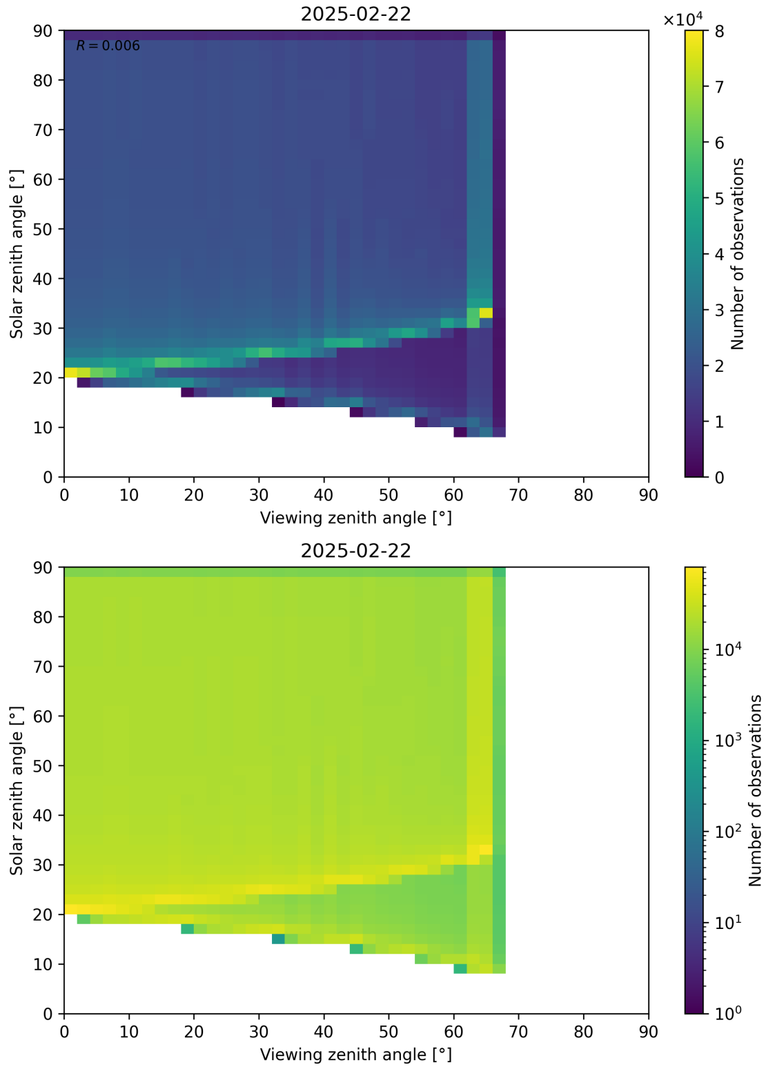
Figure 54: Scatter density plot of “Viewing zenith angle” against “Solar zenith angle” for 2025-02-21 to 2025-02-23.
