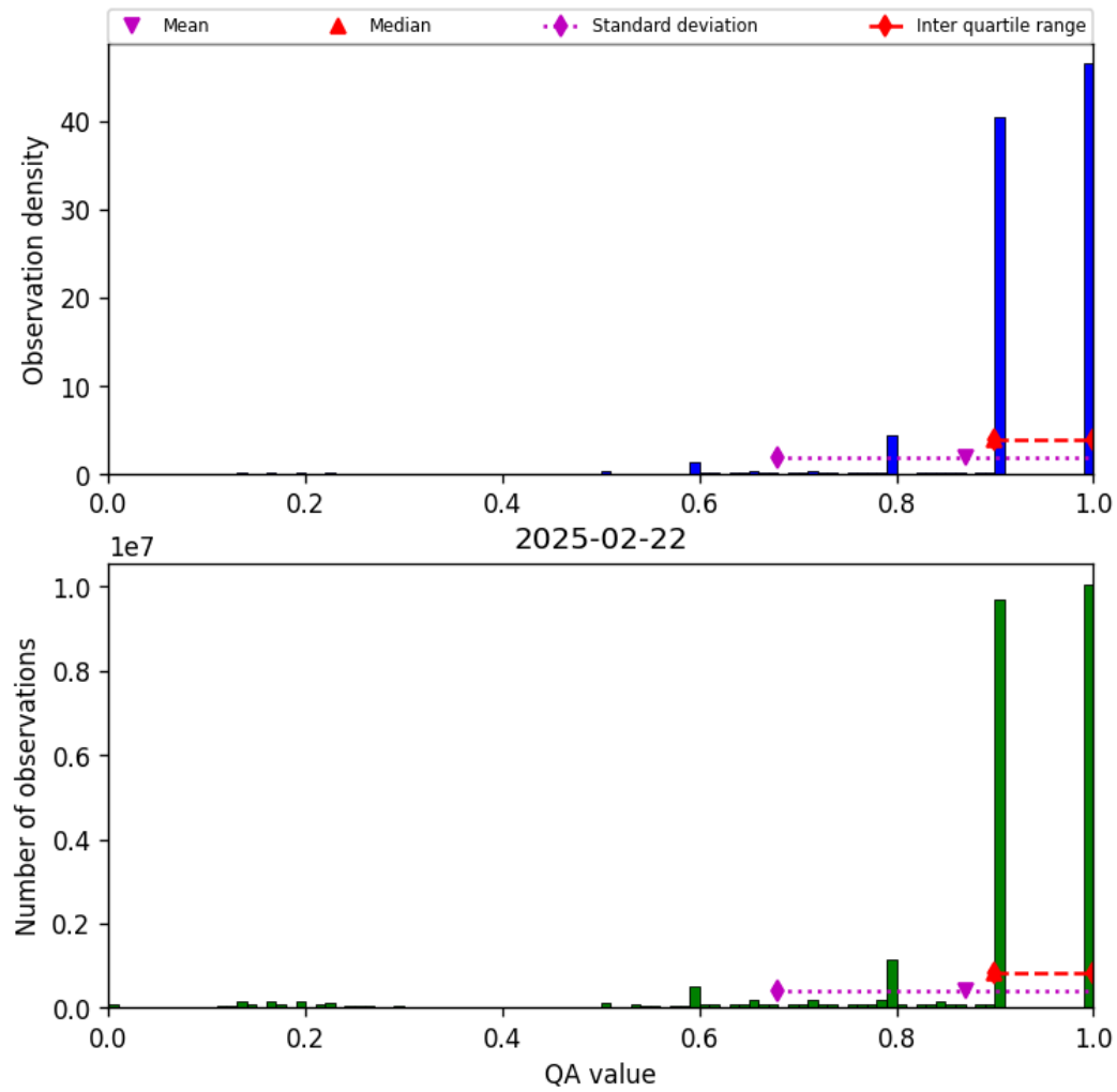
Figure 20: Histogram of “QA value” for 2025-02-21 to 2025-02-23
