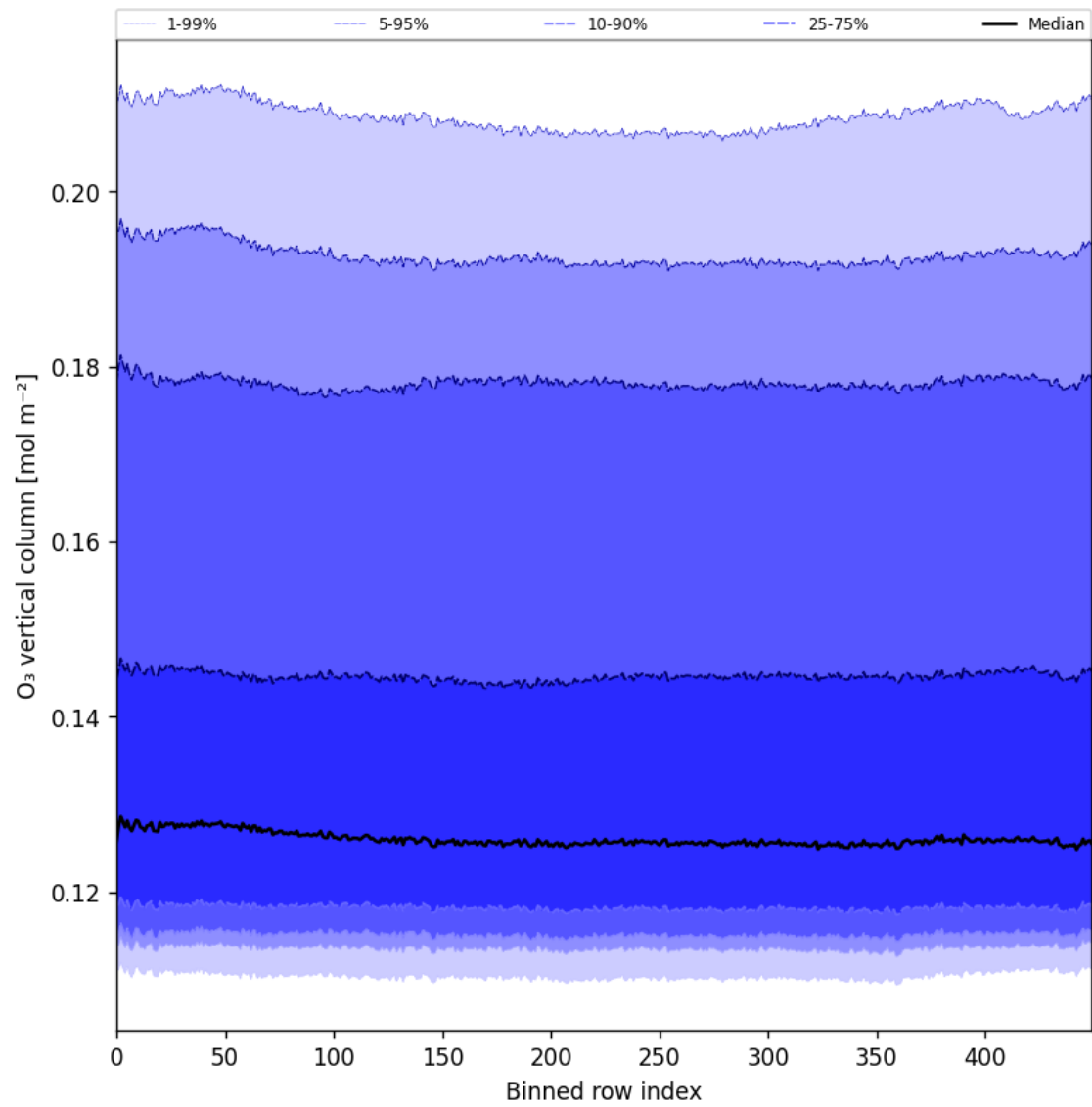
Figure 28: Along track statistics of “O 3 vertical column” for 2025-02-21 to 2025-02-23
