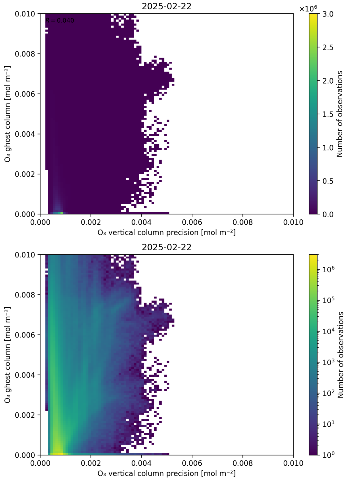
Figure 43: Scatter density plot of “ O_3 vertical column precision” against “ O_3 ghost column” for 2025-02-21 to 2025-02-23.
