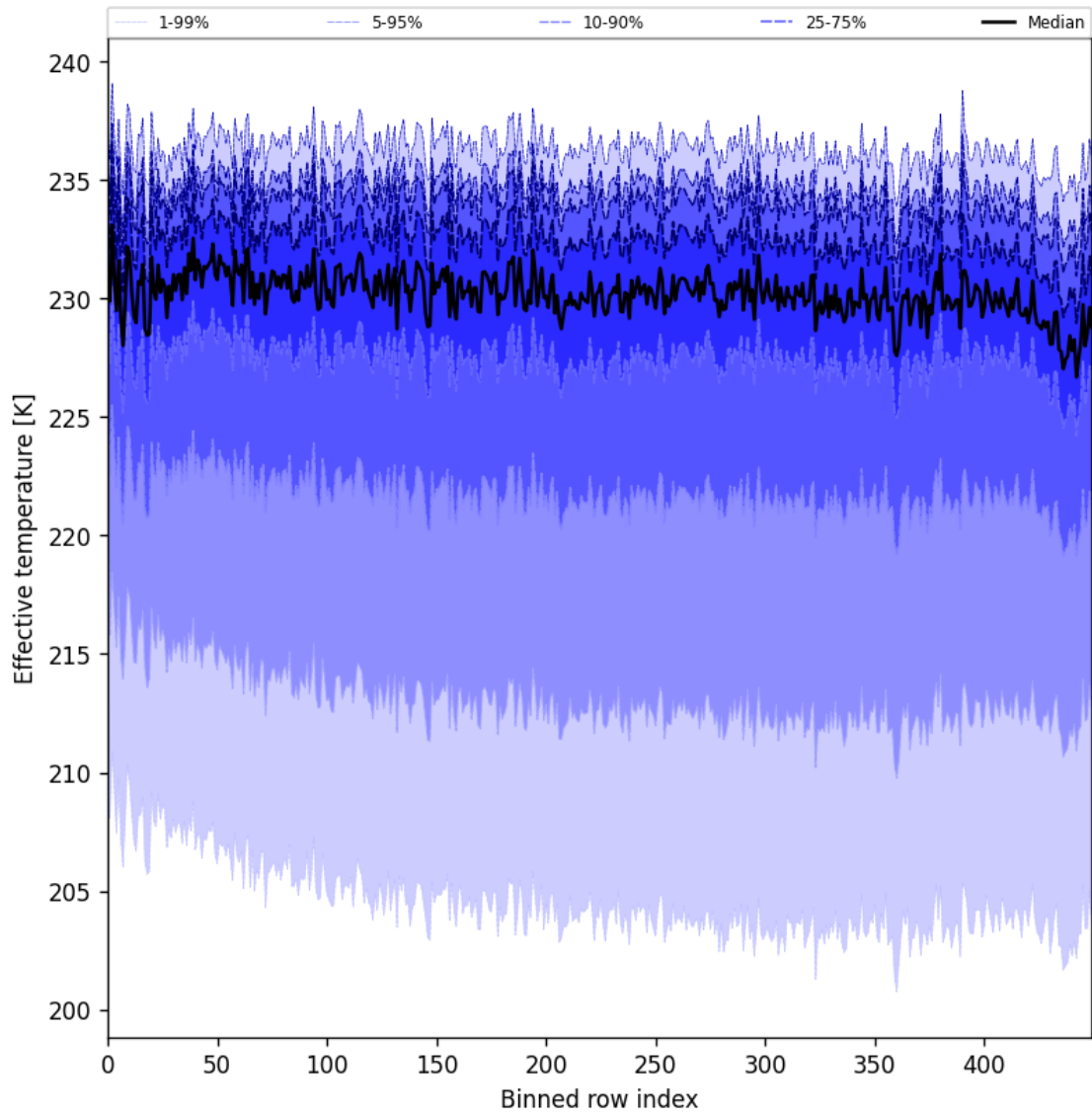
Figure 31: Along track statistics of “Effective temperature” for 2025-02-21 to 2025-02-23
