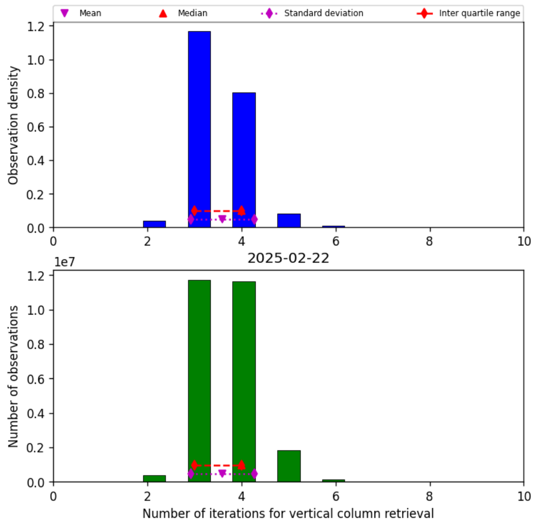
Figure 26: Histogram of “Number of iterations for vertical column retrieval” for 2025-02-21 to 2025-02-23
