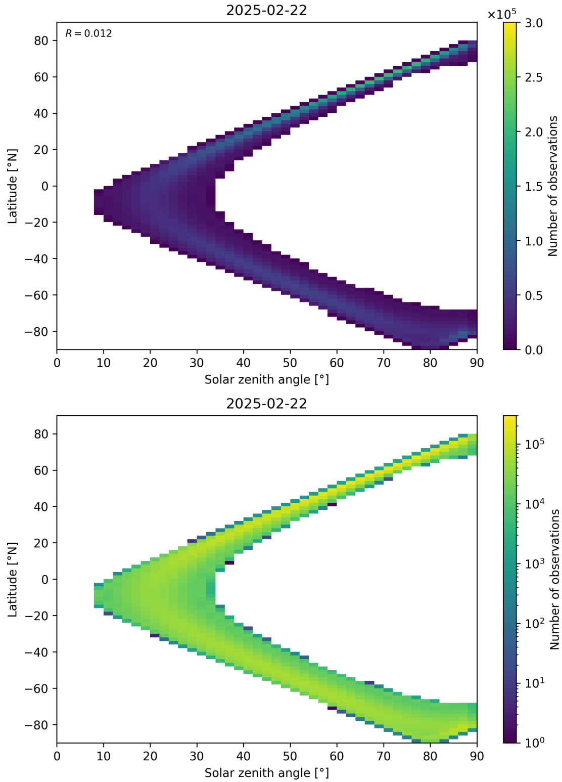
Figure 44: Scatter density plot of “Solar zenith angle” against “Latitude” for 2025-02-21 to 2025-02-23.
