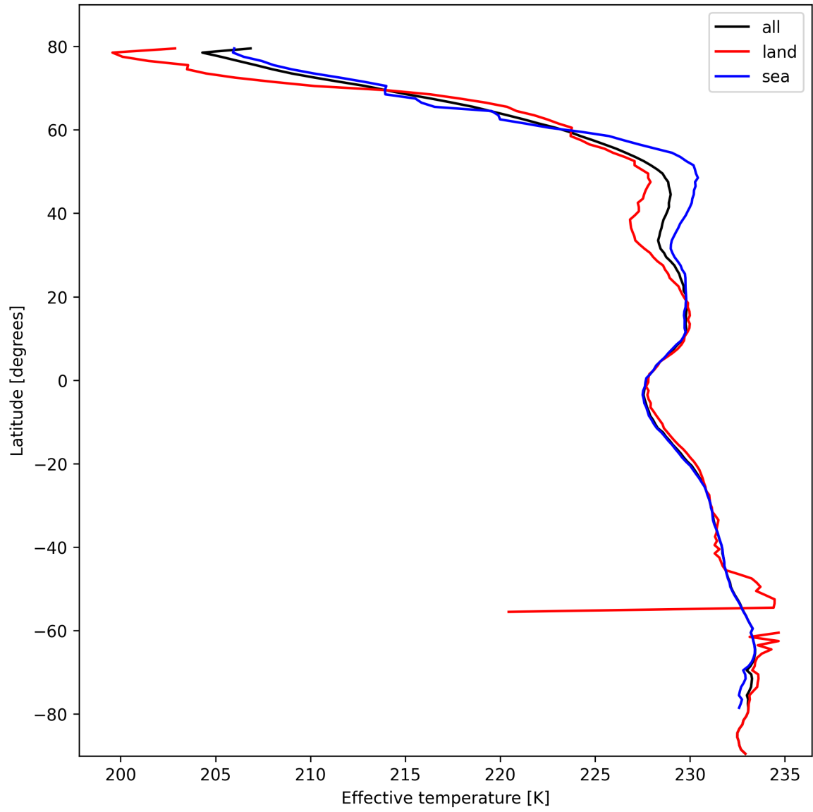
Figure 17: Zonal average of "Effective temperature" for 2025-02-21 to 2025-02-23.
