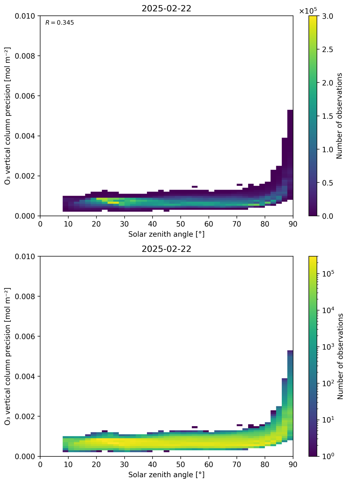
Figure 48: Scatter density plot of “Solar zenith angle” against “O 3 vertical column precision” for 2025-02-21 to 2025-02-23.
