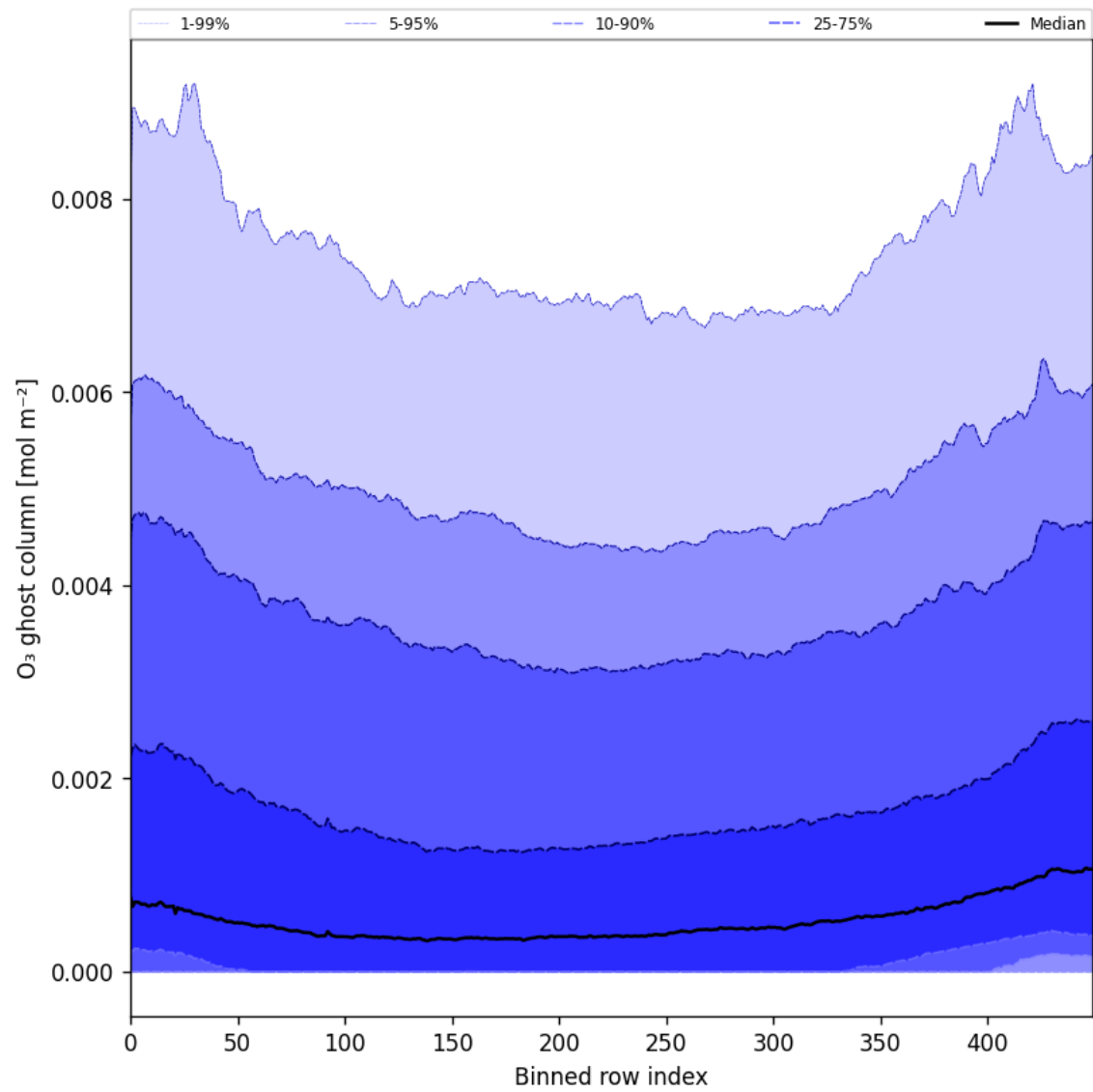
Figure 32: Along track statistics of “O 3 ghost column” for 2025-02-21 to 2025-02-23
