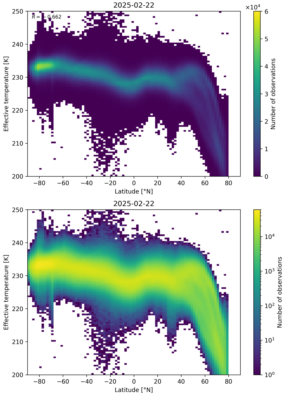
Figure 34: Scatter density plot of “Latitude” against “Effective temperature” for 2025-02-21 to 2025-02-23.
