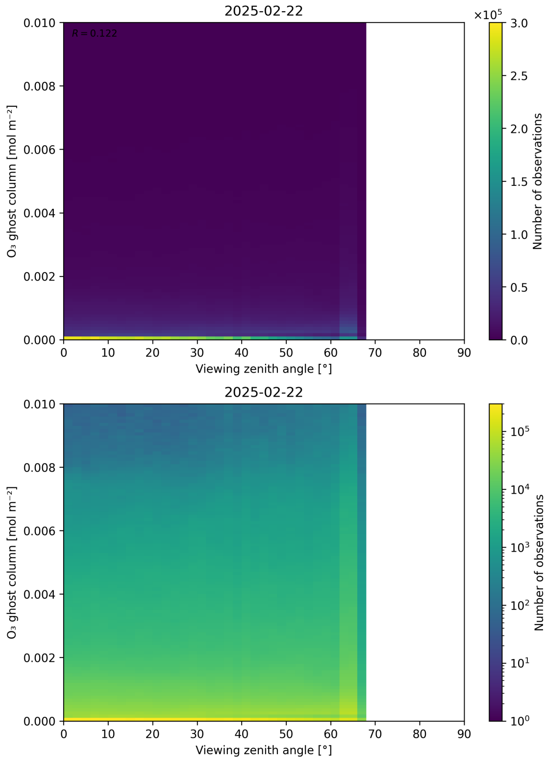
Figure 51: Scatter density plot of “Viewing zenith angle” against “O 3 ghost column” for 2025-02-21 to 2025-02-23.
