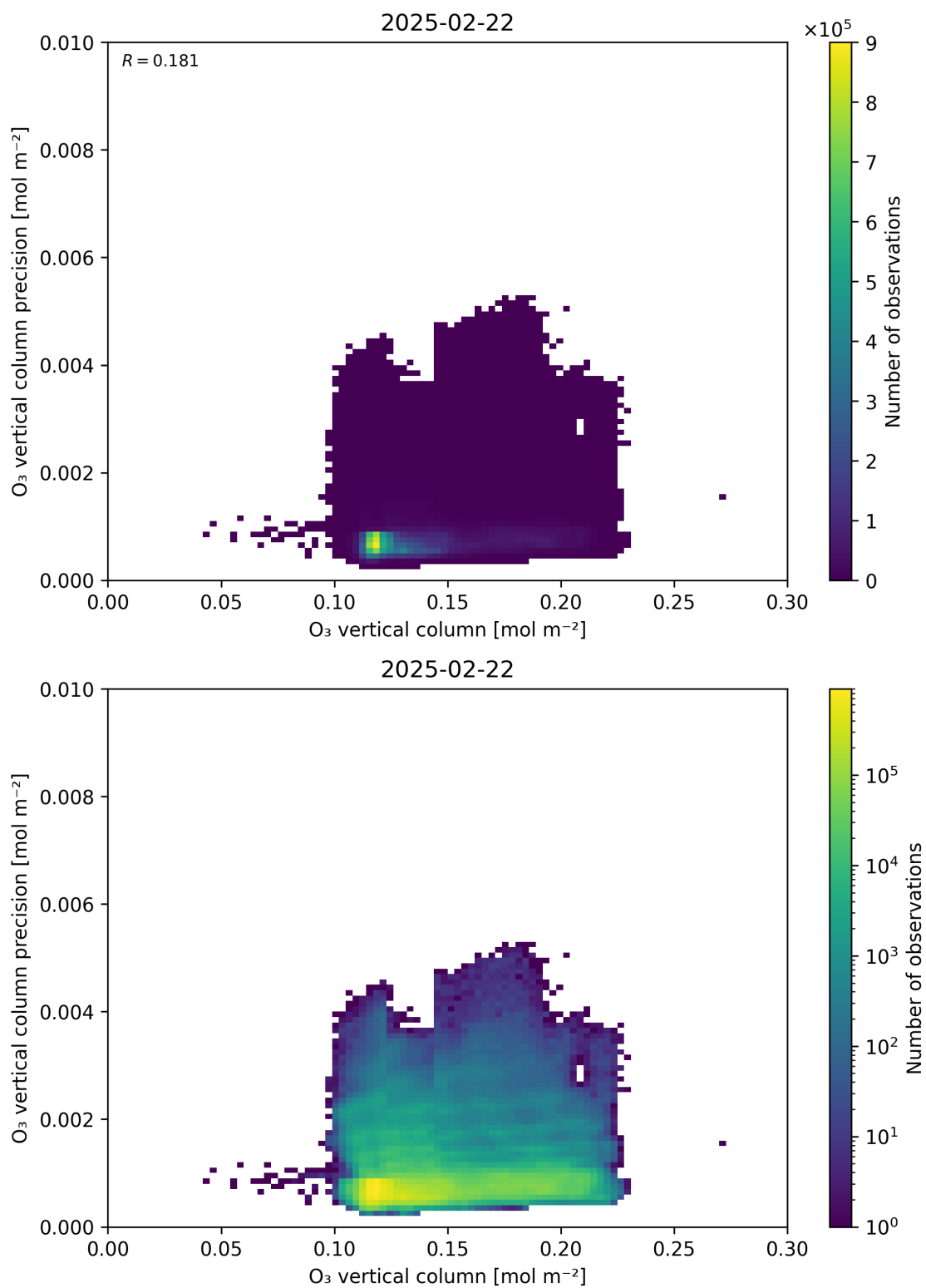
Figure 41: Scatter density plot of “O 3 vertical column” against “O 3 vertical column precision” for 2025-02-21 to 2025-02-23.
