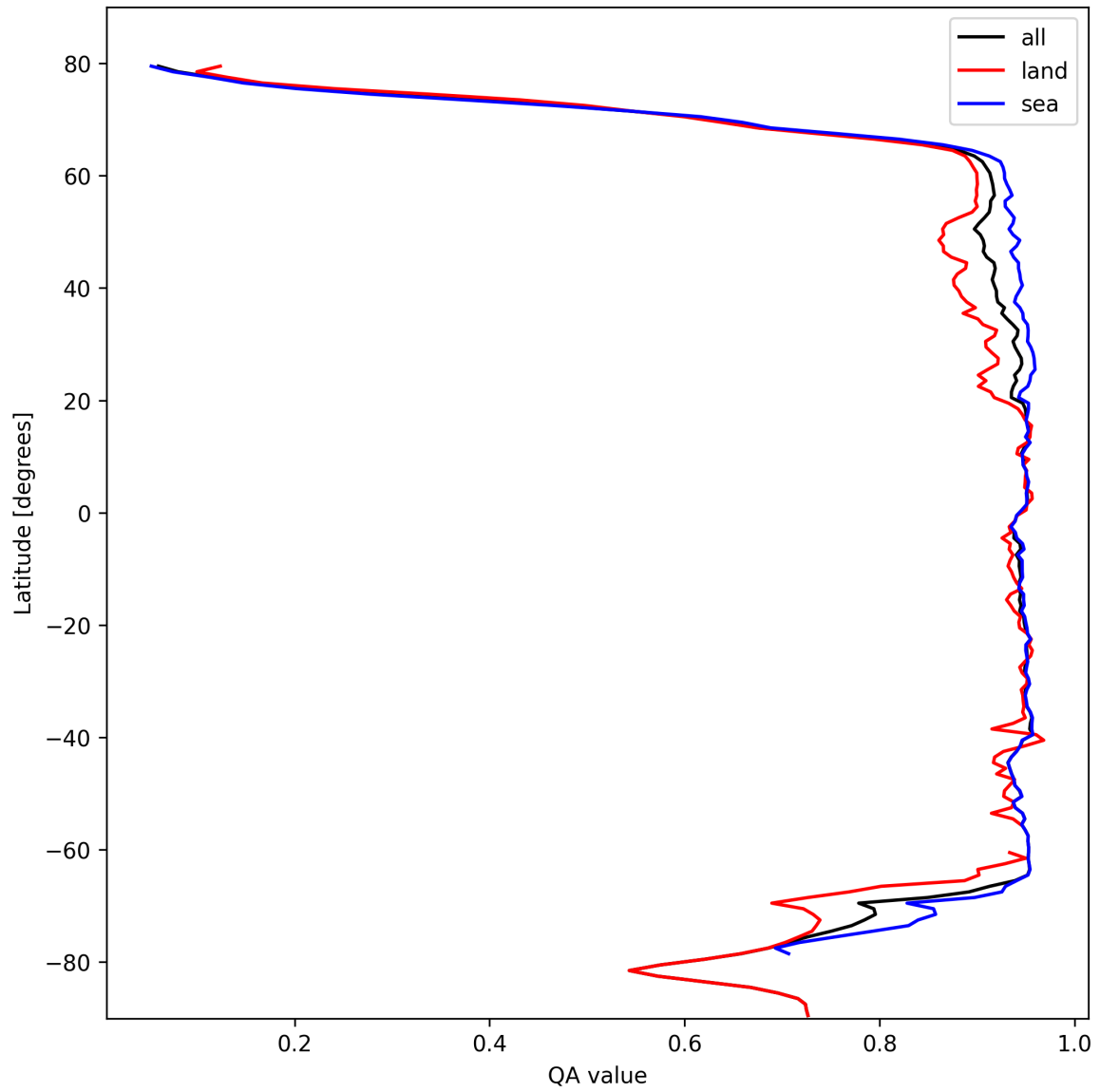
Figure 13: Zonal average of “QA value” for 2025-02-21 to 2025-02-23.
