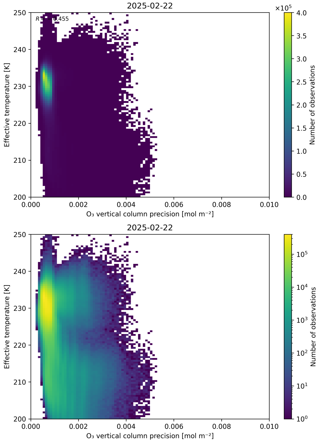
Figure 42: Scatter density plot of “O 3 vertical column precision” against “Effective temperature” for 2025-02-21 to 2025-02-23.
