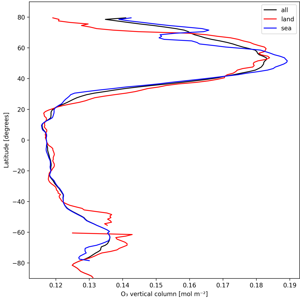
Figure 14: Zonal average of “O 3 vertical column” for 2025-02-21 to 2025-02-23.
