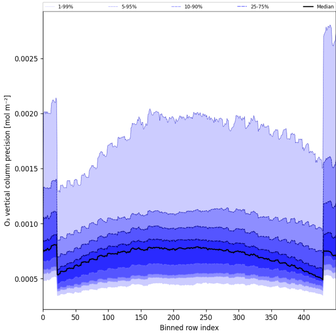
Figure 29: Along track statistics of “O 3 vertical column precision” for 2025-02-21 to 2025-02-23
