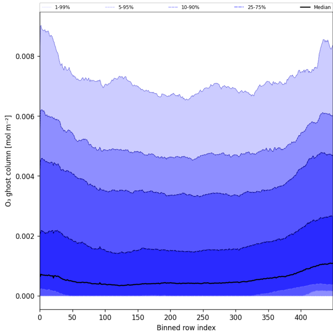
Figure 32: Along track statistics of “O 3 ghost column” for 2025-02-24 to 2025-02-25
