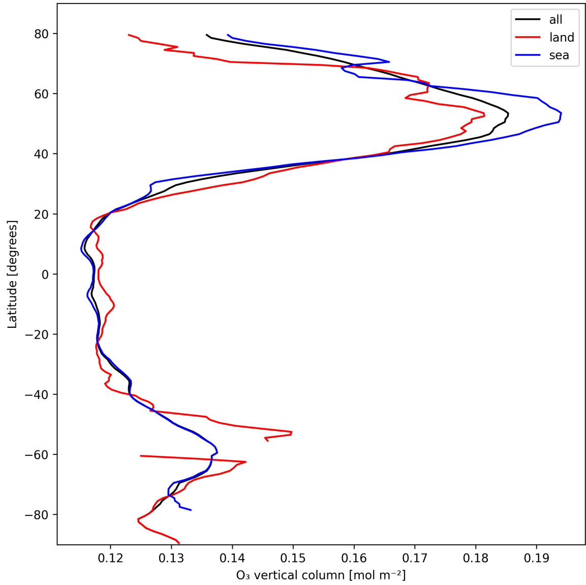
Figure 14: Zonal average of “O 3 vertical column” for 2025-02-24 to 2025-02-25.
