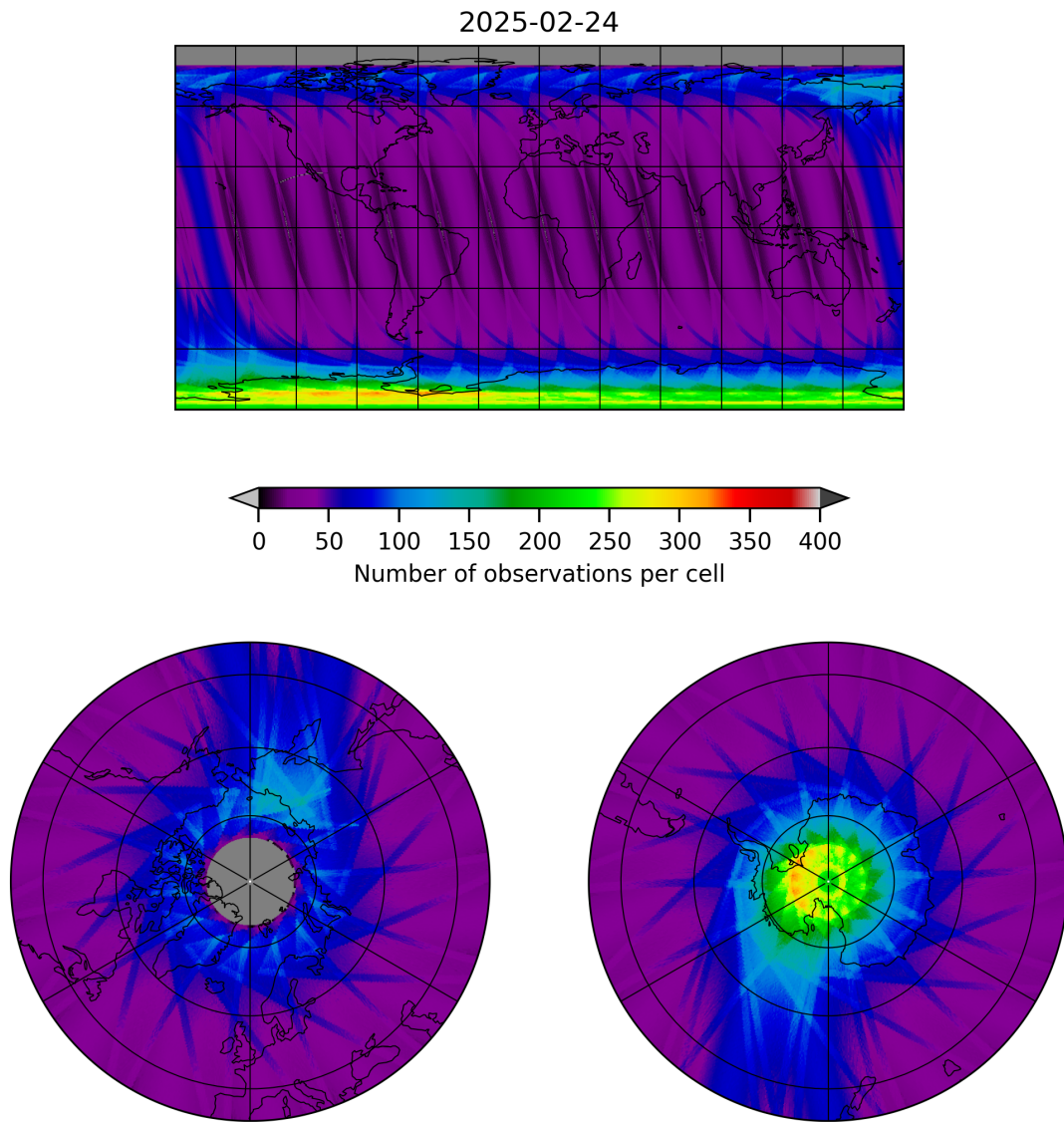
Figure 12: Map of the number of observations for 2025-02-24 to 2025-02-25
