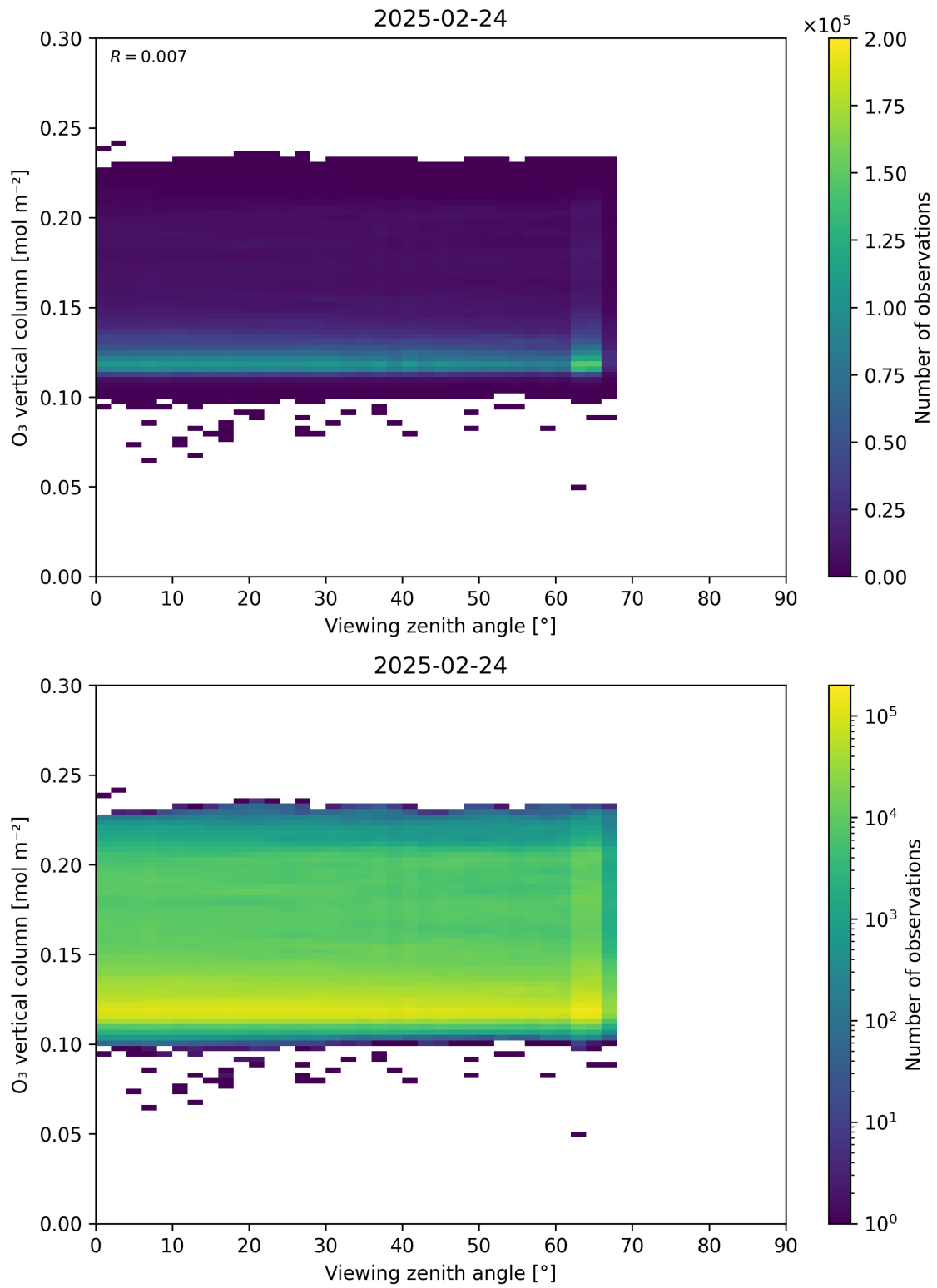
Figure 52: Scatter density plot of “Viewing zenith angle” against “O 3 vertical column” for 2025-02-24 to 2025-02-25.
