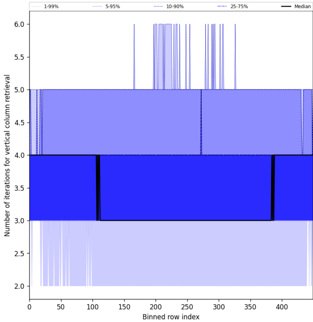
Figure 33: Along track statistics of “Number of iterations for vertical column retrieval” for 2025-02-24 to 2025-02-25
