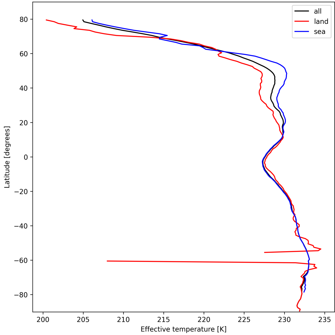
Figure 17: Zonal average of “Effective temperature” for 2025-02-24 to 2025-02-25.
