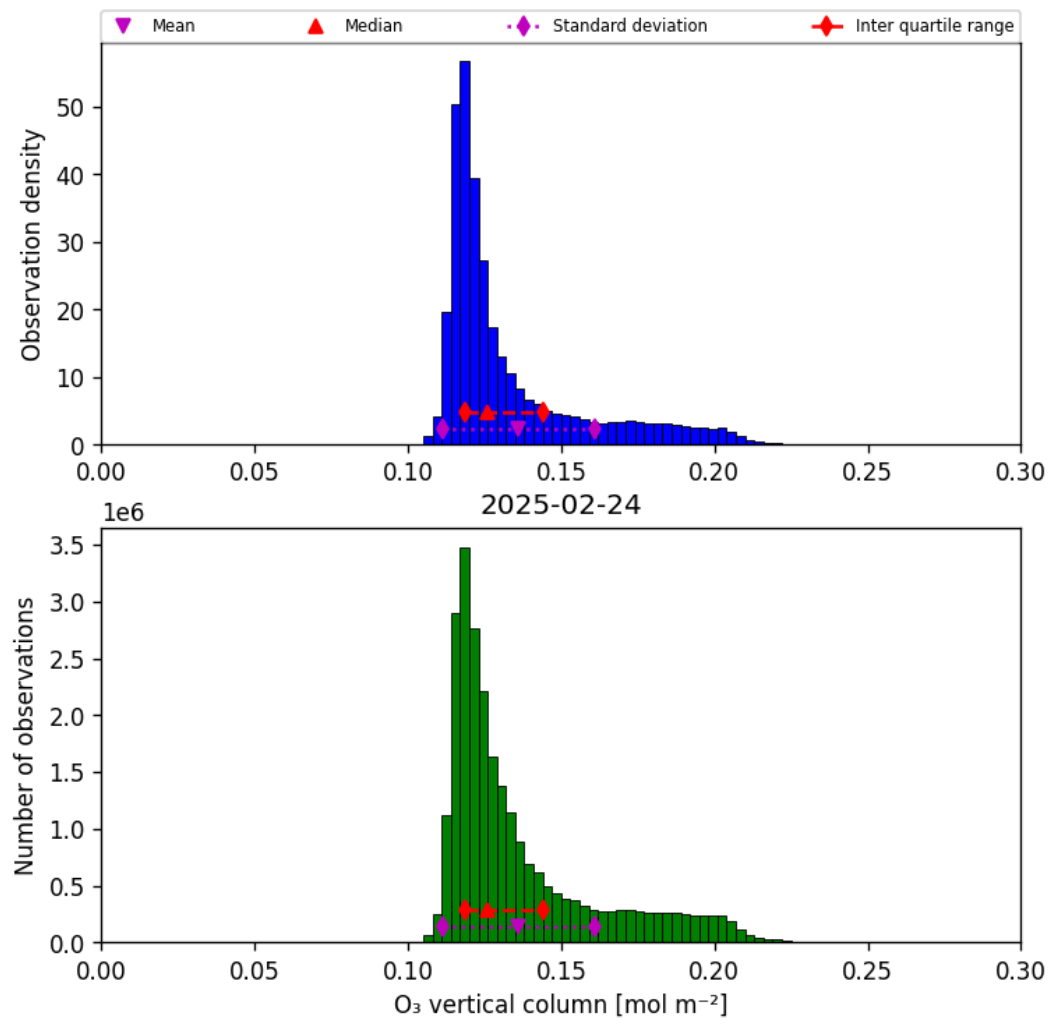
Figure 21: Histogram of “O 3 vertical column” for 2025-02-24 to 2025-02-25
