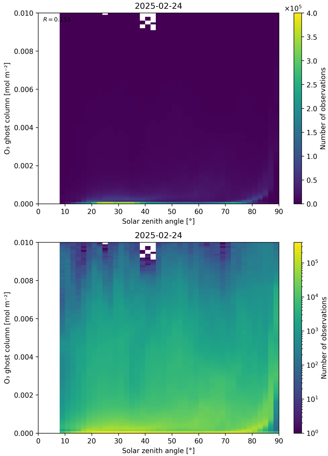
Figure 46: Scatter density plot of “Solar zenith angle” against “O 3 ghost column” for 2025-02-24 to 2025-02-25.
