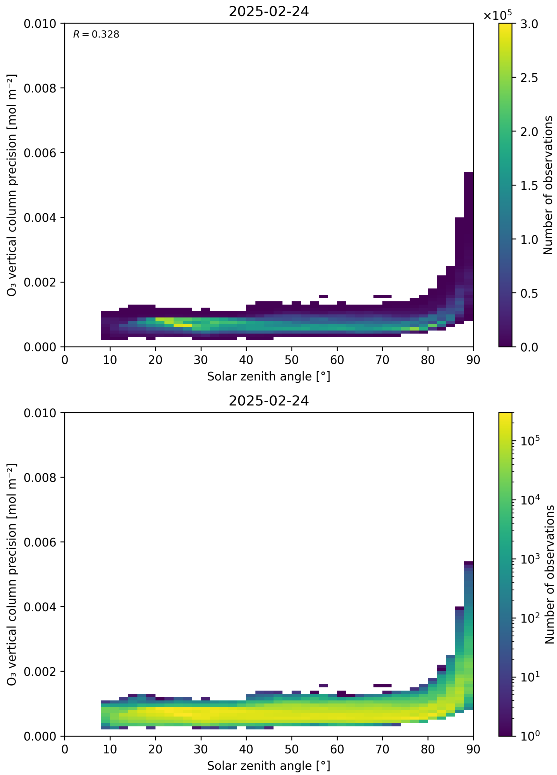
Figure 48: Scatter density plot of “Solar zenith angle” against “O 3 vertical column precision” for 2025-02-24 to 2025-02-25.
