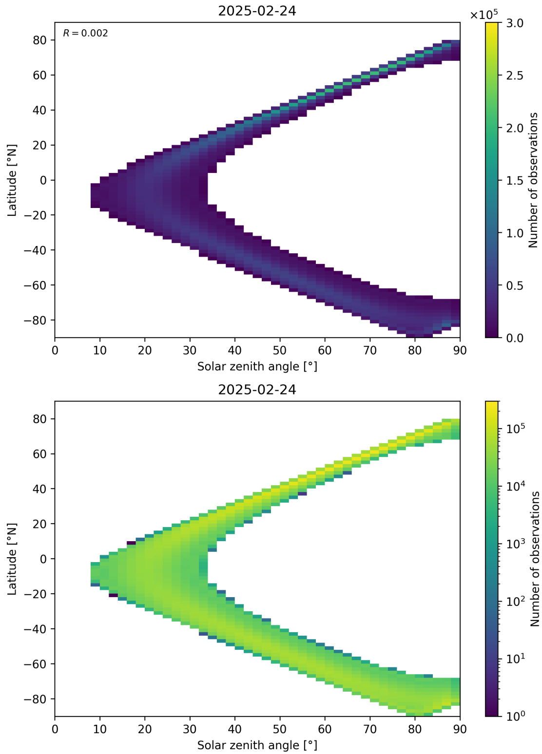
Figure 44: Scatter density plot of “Solar zenith angle” against “Latitude” for 2025-02-24 to 2025-02-25.
