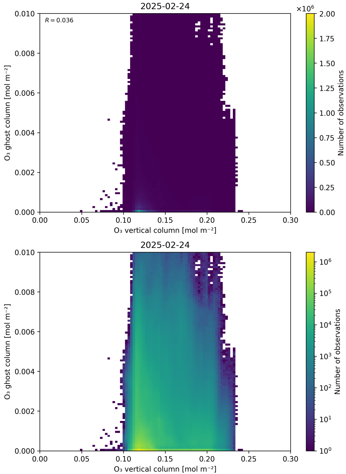
Figure 40: Scatter density plot of “O 3 vertical column” against “O 3 ghost column” for 2025-02-24 to 2025-02-25.
