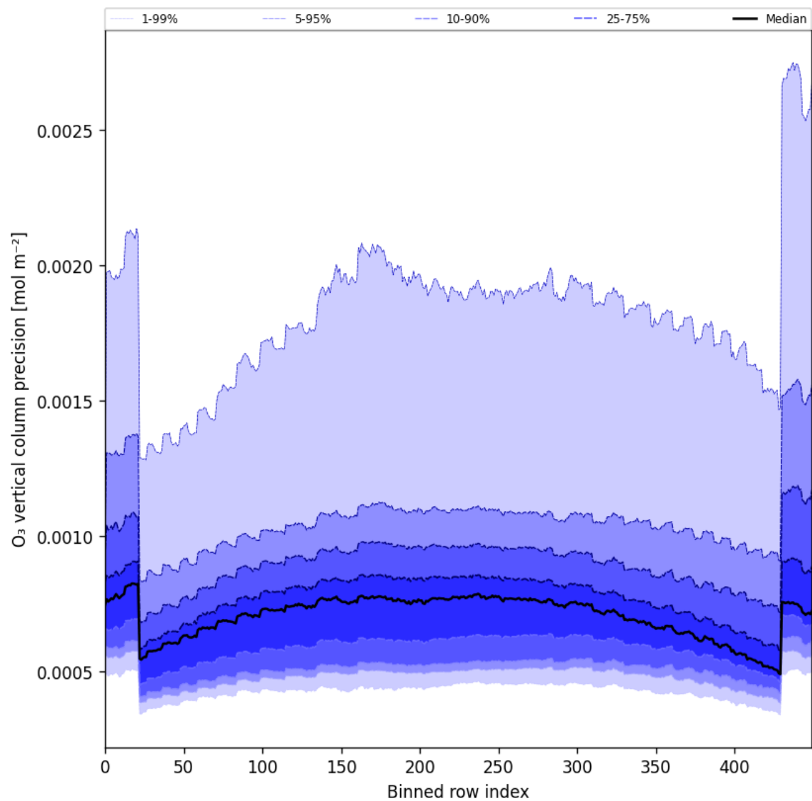
Figure 29: Along track statistics of “O 3 vertical column precision” for 2025-02-24 to 2025-02-25
