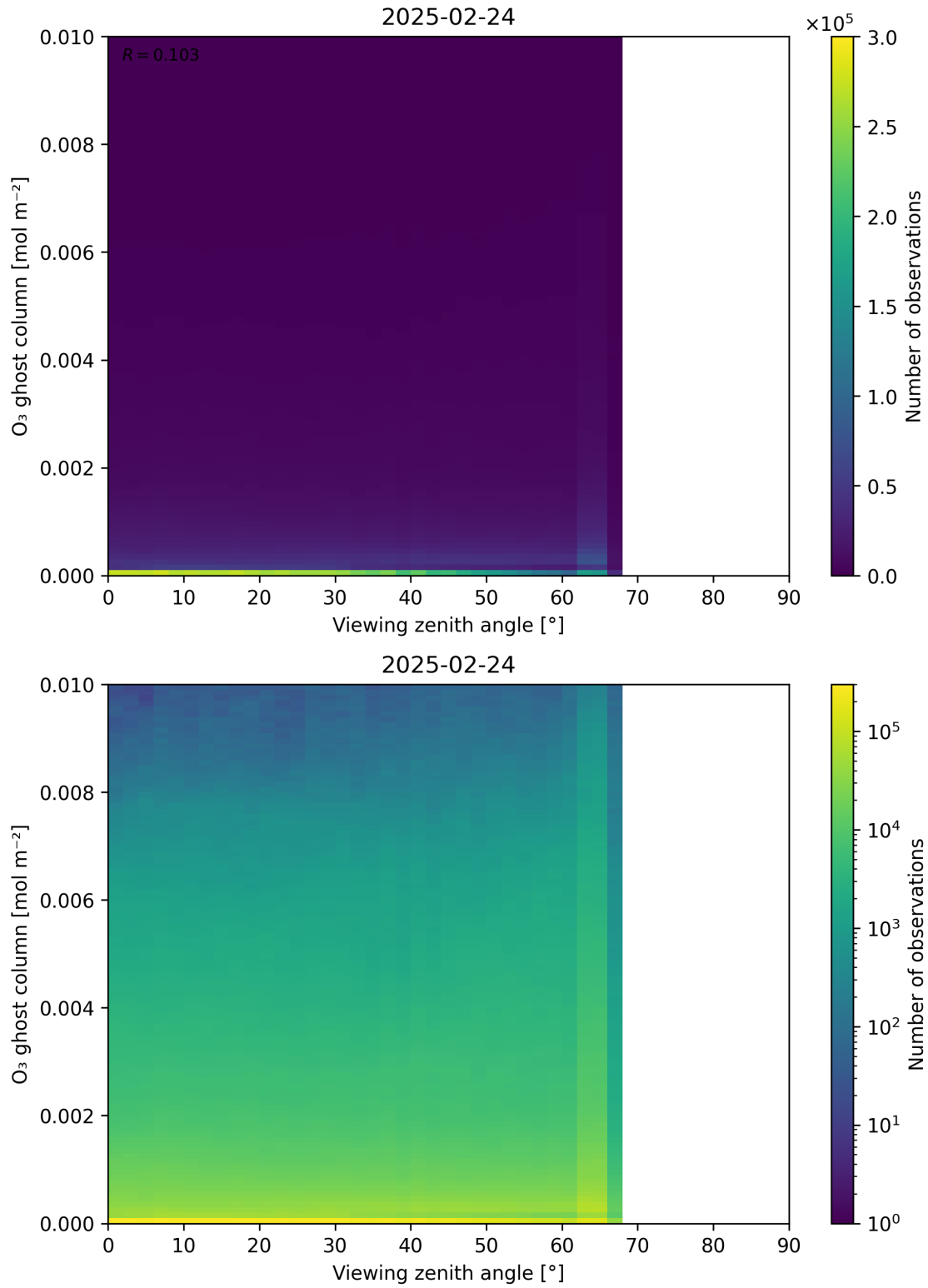
Figure 51: Scatter density plot of “Viewing zenith angle” against “O 3 ghost column” for 2025-02-24 to 2025-02-25.
