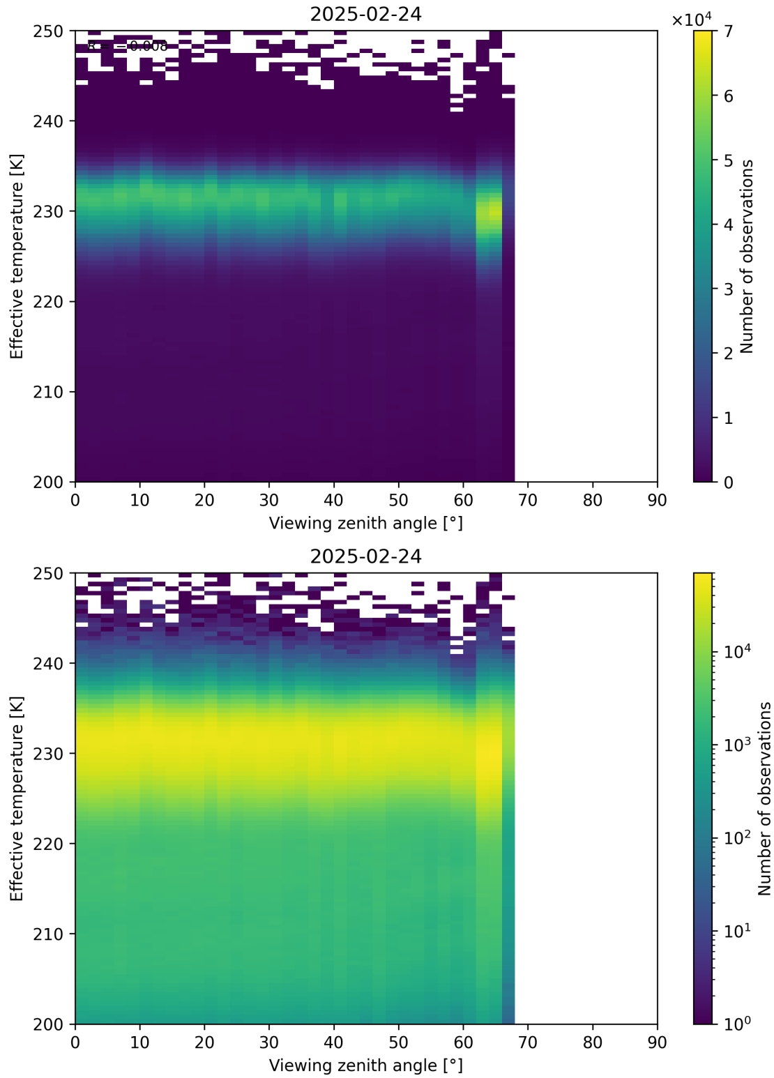
Figure 50: Scatter density plot of “Viewing zenith angle” against “Effective temperature” for 2025-02-24 to 2025-02-25.
