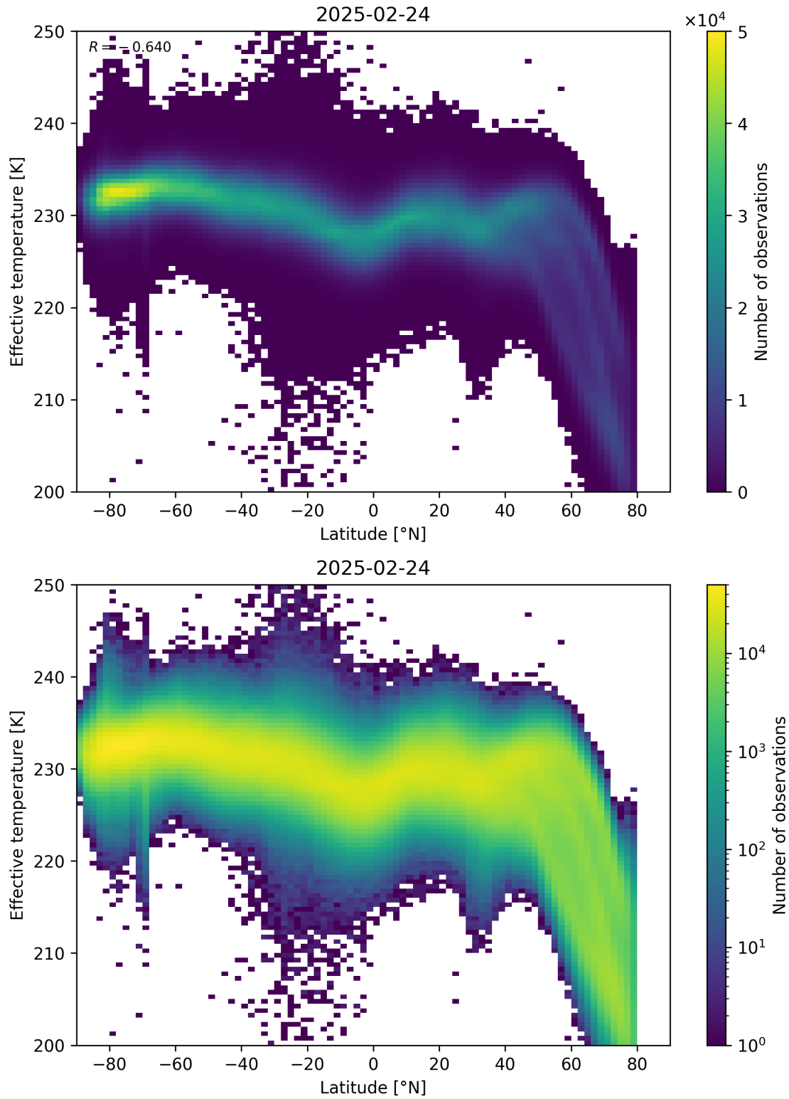
Figure 34: Scatter density plot of “Latitude” against “Effective temperature” for 2025-02-24 to 2025-02-25.
