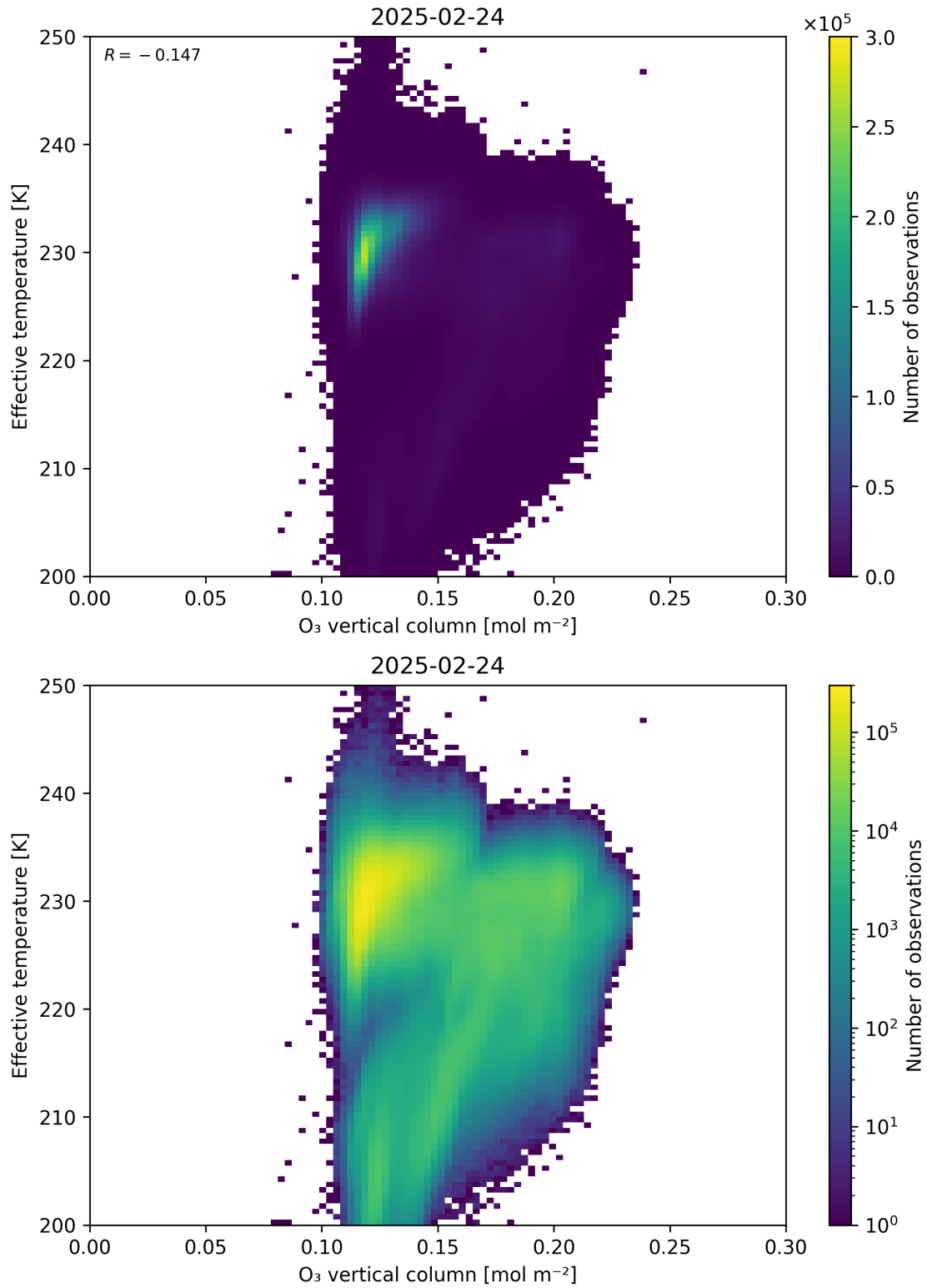
Figure 39: Scatter density plot of “O 3 vertical column” against “Effective temperature” for 2025-02-24 to 2025-02-25.
