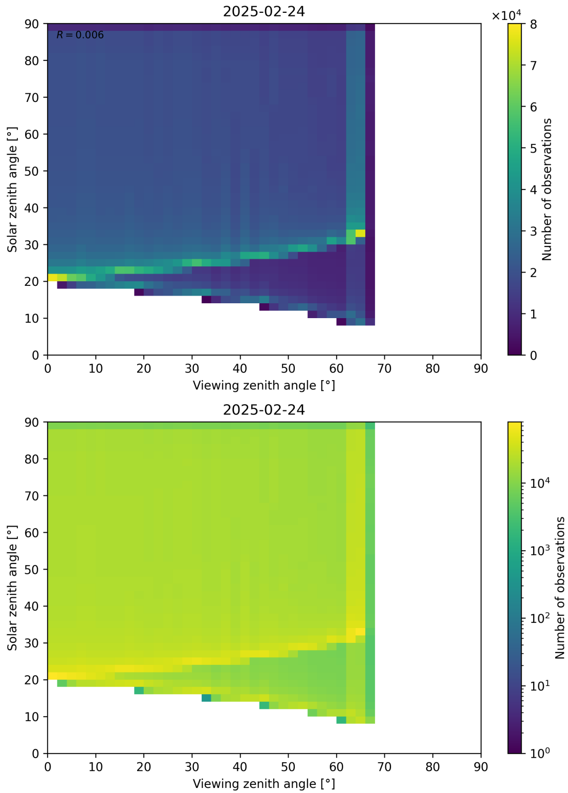
Figure 54: Scatter density plot of “Viewing zenith angle” against “Solar zenith angle” for 2025-02-24 to 2025-02-25.
