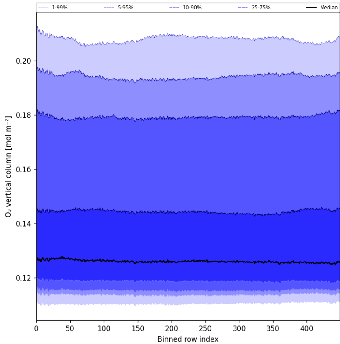
Figure 28: Along track statistics of “O 3 vertical column” for 2025-02-24 to 2025-02-25
