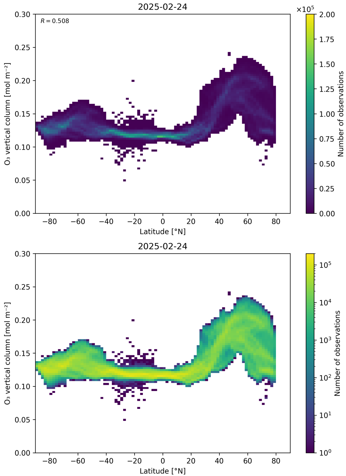
Figure 36: Scatter density plot of “Latitude” against “O 3 vertical column” for 2025-02-24 to 2025-02-25.
