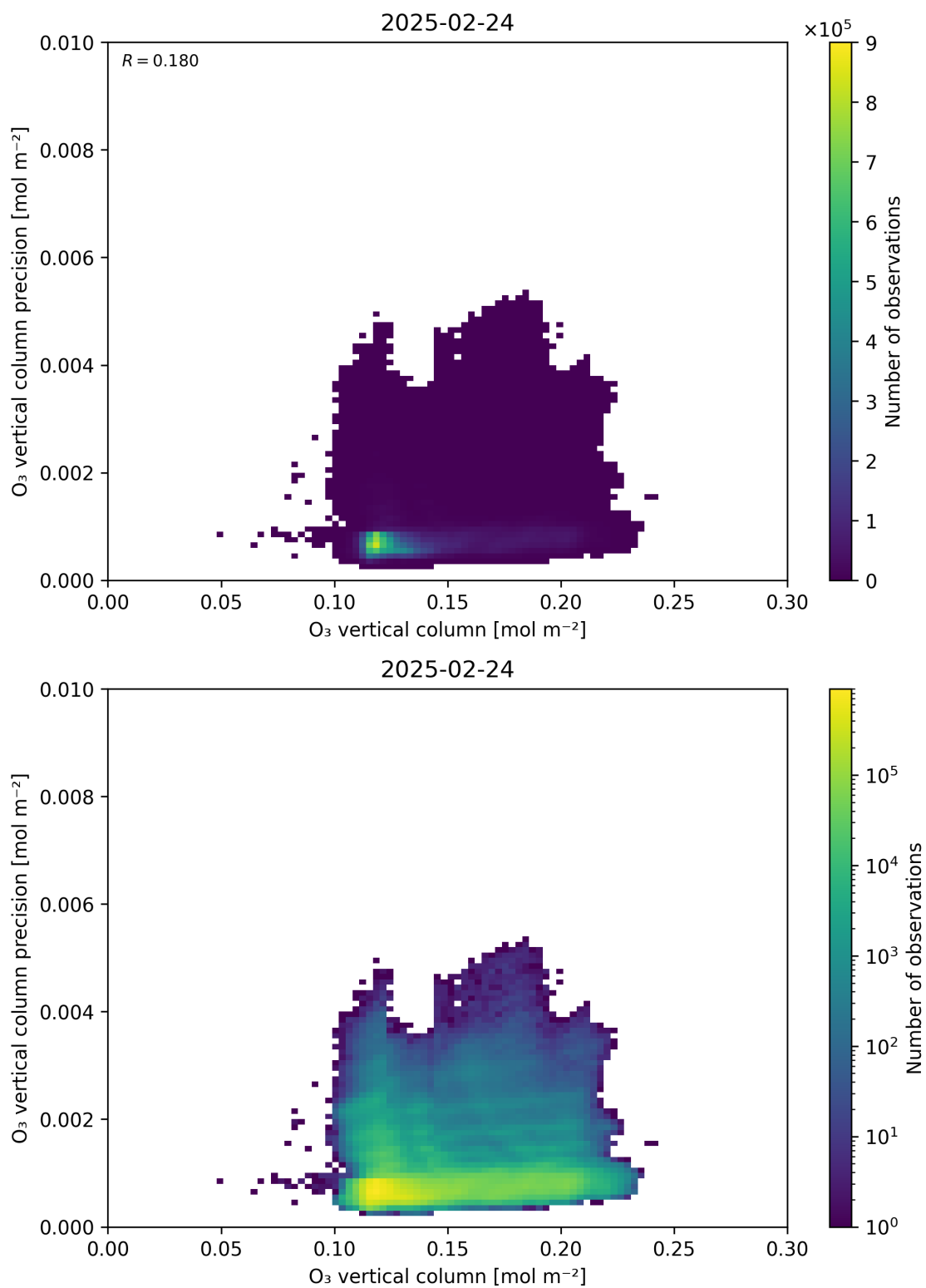
Figure 41: Scatter density plot of “O 3 vertical column” against “O 3 vertical column precision” for 2025-02-24 to 2025-02-25.
