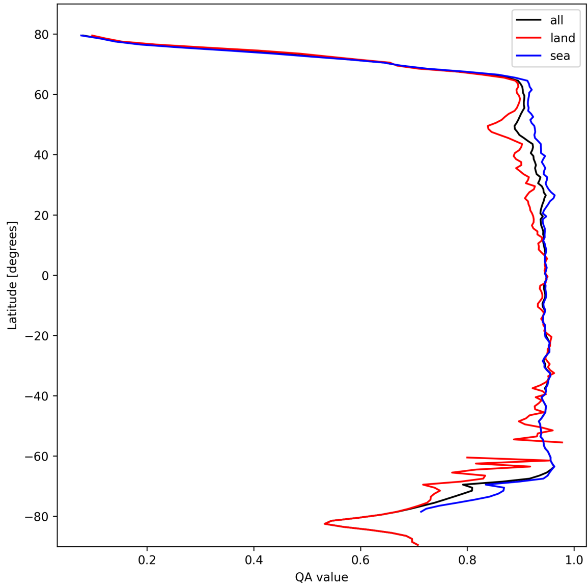
Figure 13: Zonal average of “QA value” for 2025-02-24 to 2025-02-25.
