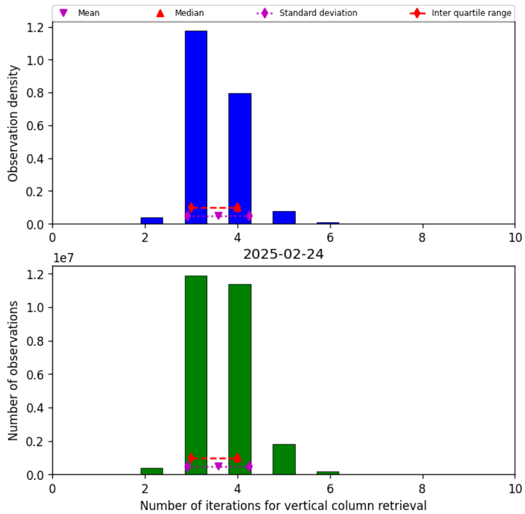
Figure 26: Histogram of “Number of iterations for vertical column retrieval” for 2025-02-24 to 2025-02-25
