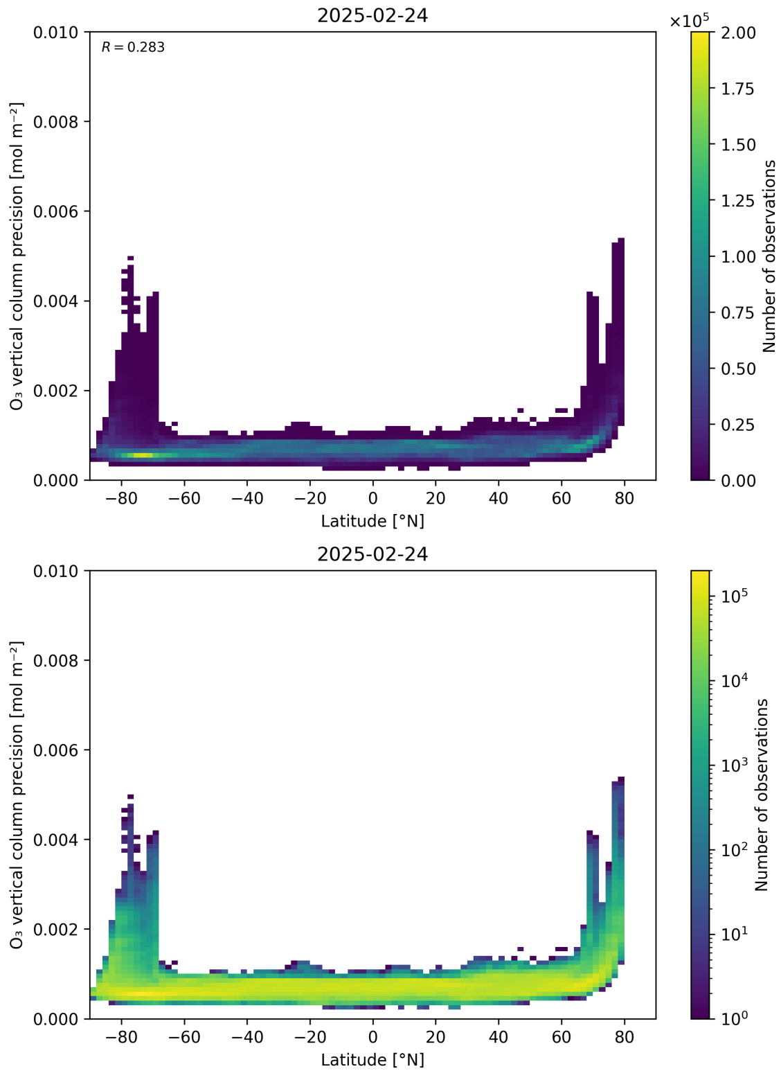
Figure 37: Scatter density plot of “Latitude” against “O 3 vertical column precision” for 2025-02-24 to 2025-02-25.
