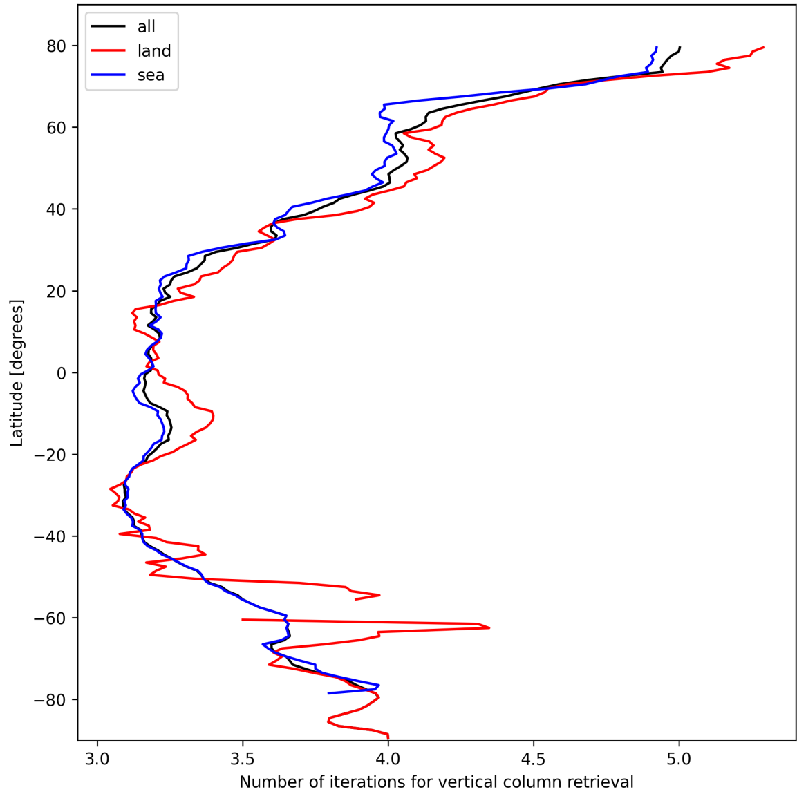
Figure 19: Zonal average of “Number of iterations for vertical column retrieval” for 2025-02-24 to 2025-02-25.
