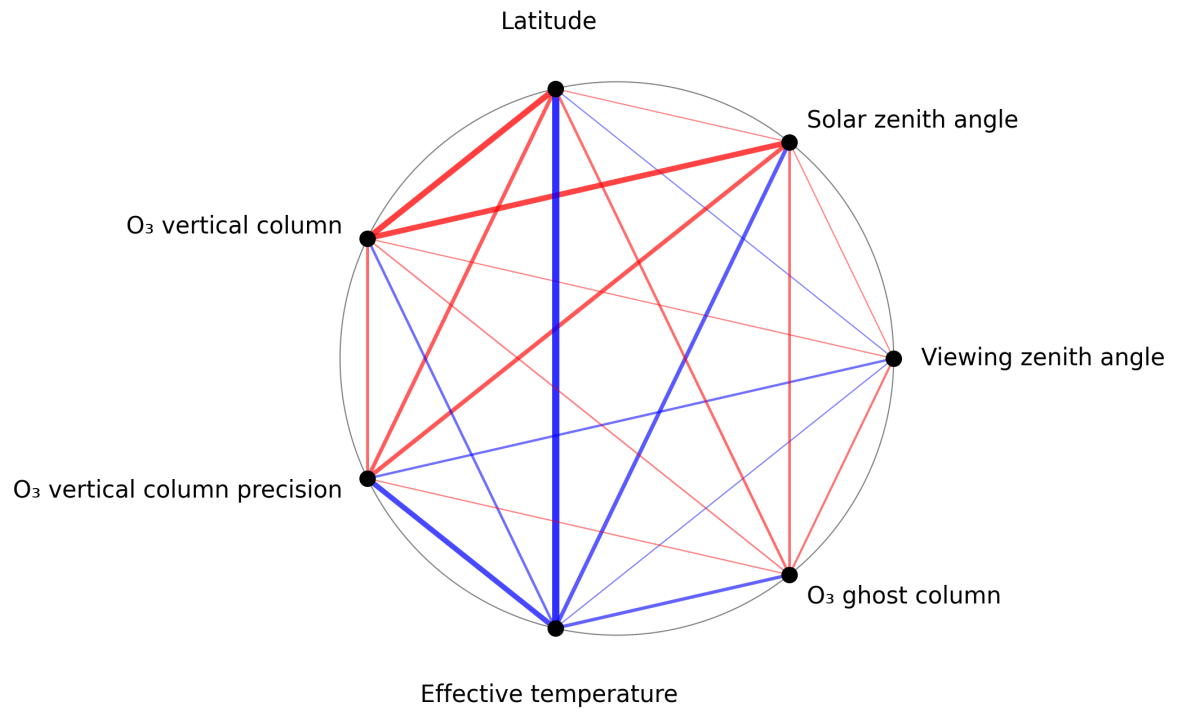
Figure 1: Map of correlation graph for 2025-02-24 to 2025-02-25.
