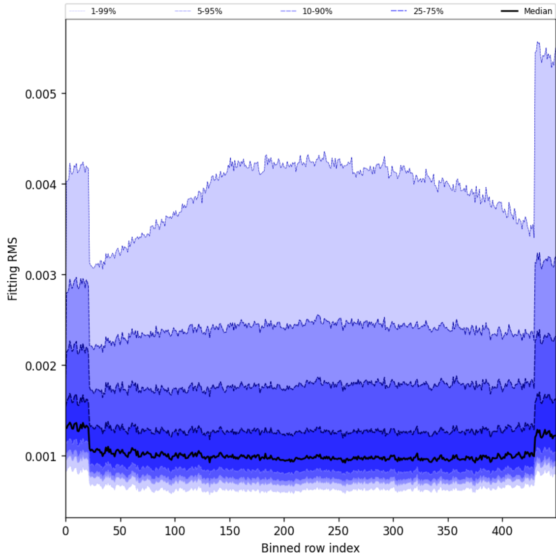
Figure 30: Along track statistics of “Fitting RMS” for 2025-02-24 to 2025-02-25
