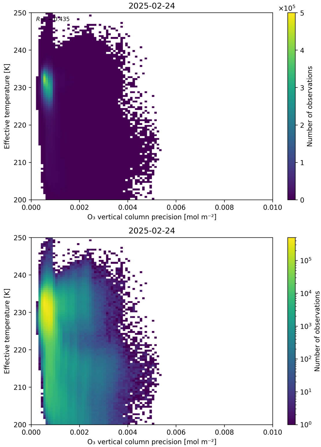
Figure 42: Scatter density plot of “O 3 vertical column precision” against “Effective temperature” for 2025-02-24 to 2025-02-25.
