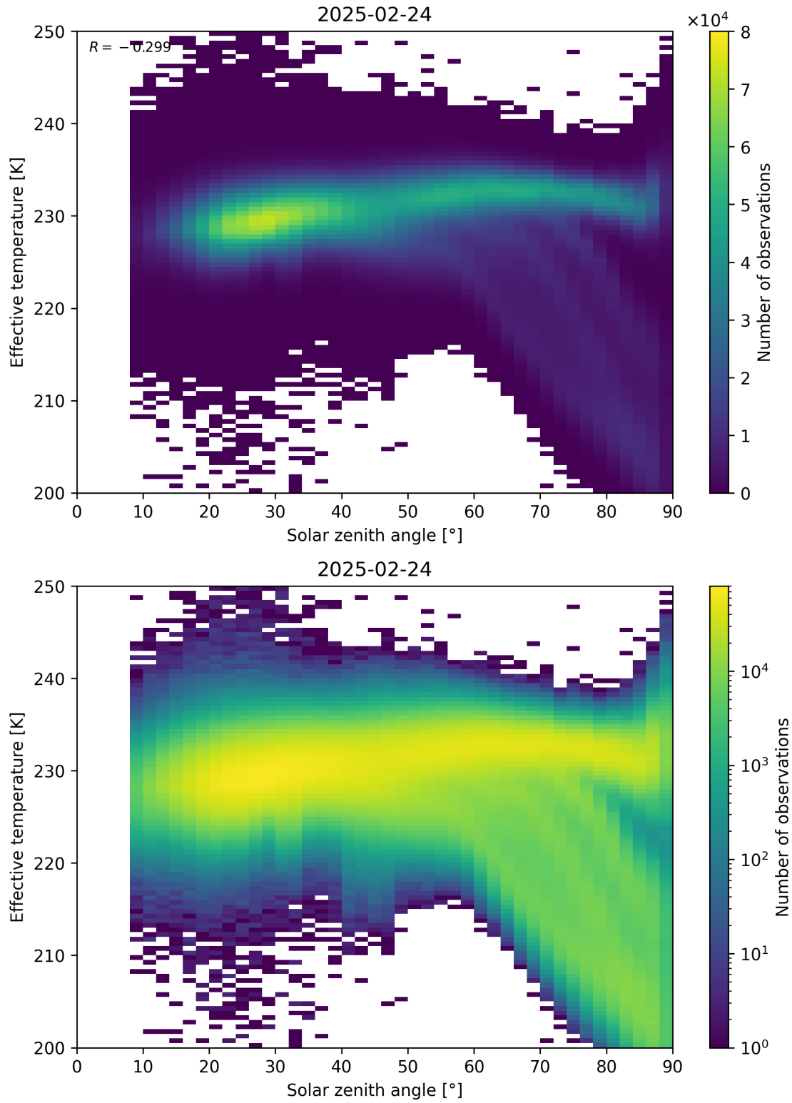
Figure 45: Scatter density plot of “Solar zenith angle” against “Effective temperature” for 2025-02-24 to 2025-02-25.
