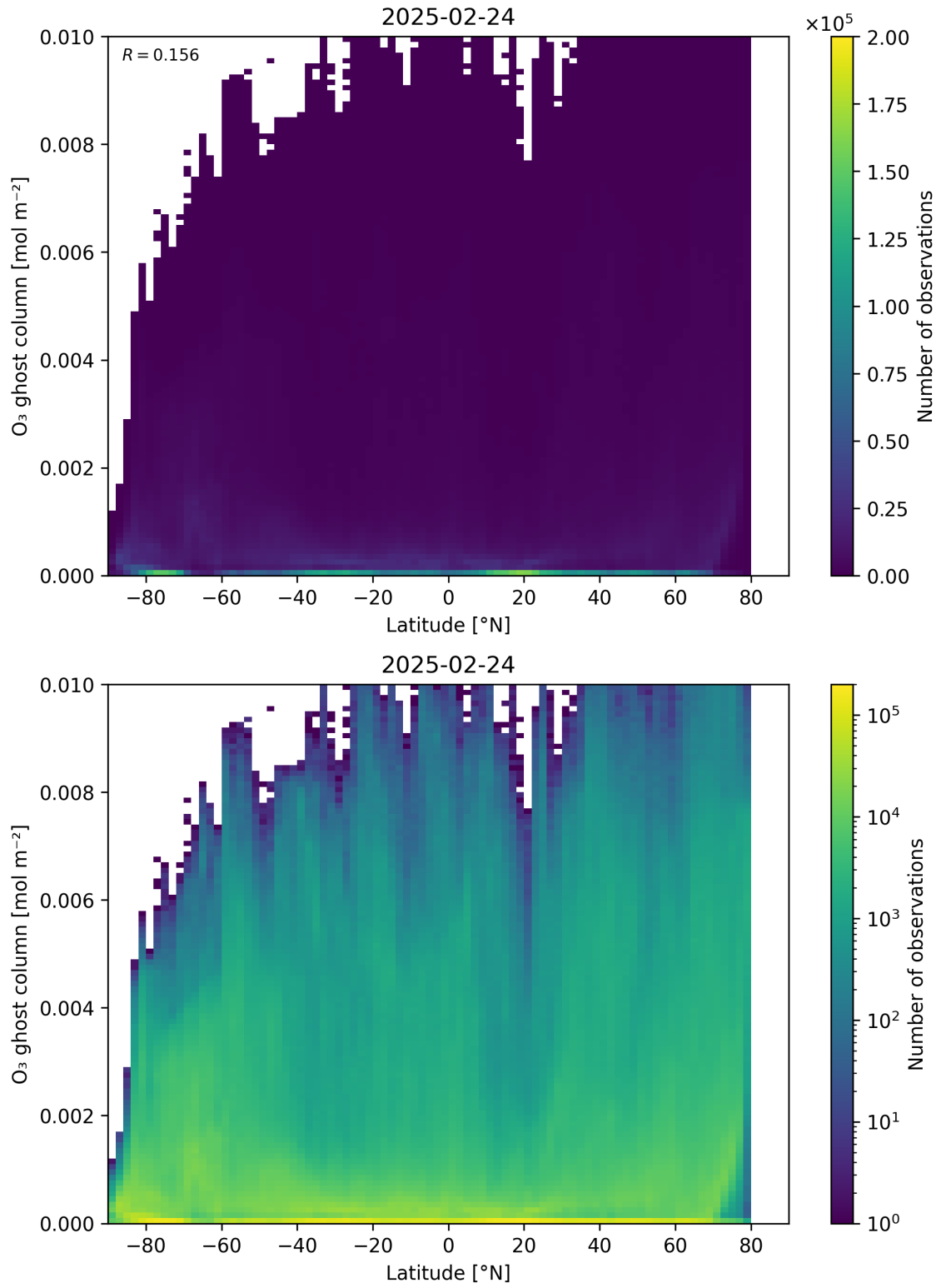
Figure 35: Scatter density plot of “Latitude” against “O 3 ghost column” for 2025-02-24 to 2025-02-25.
