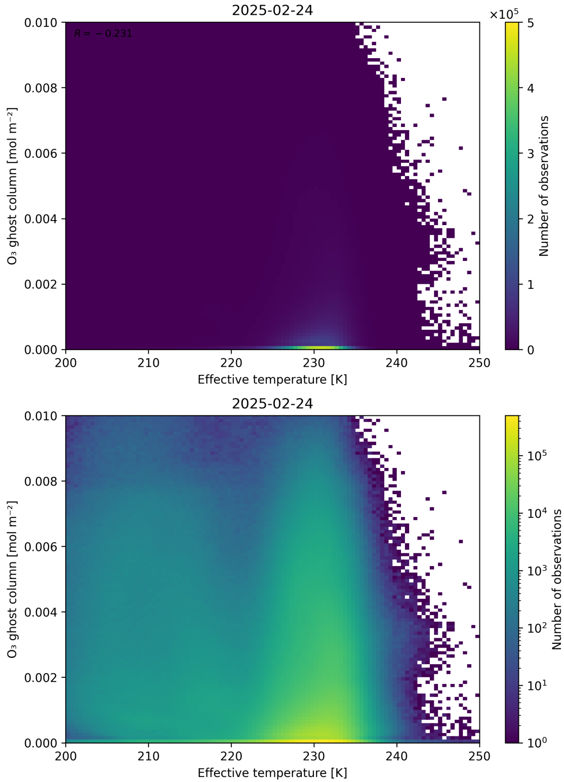
Figure 38: Scatter density plot of “Effective temperature” against “O 3 ghost column” for 2025-02-24 to 2025-02-25.
