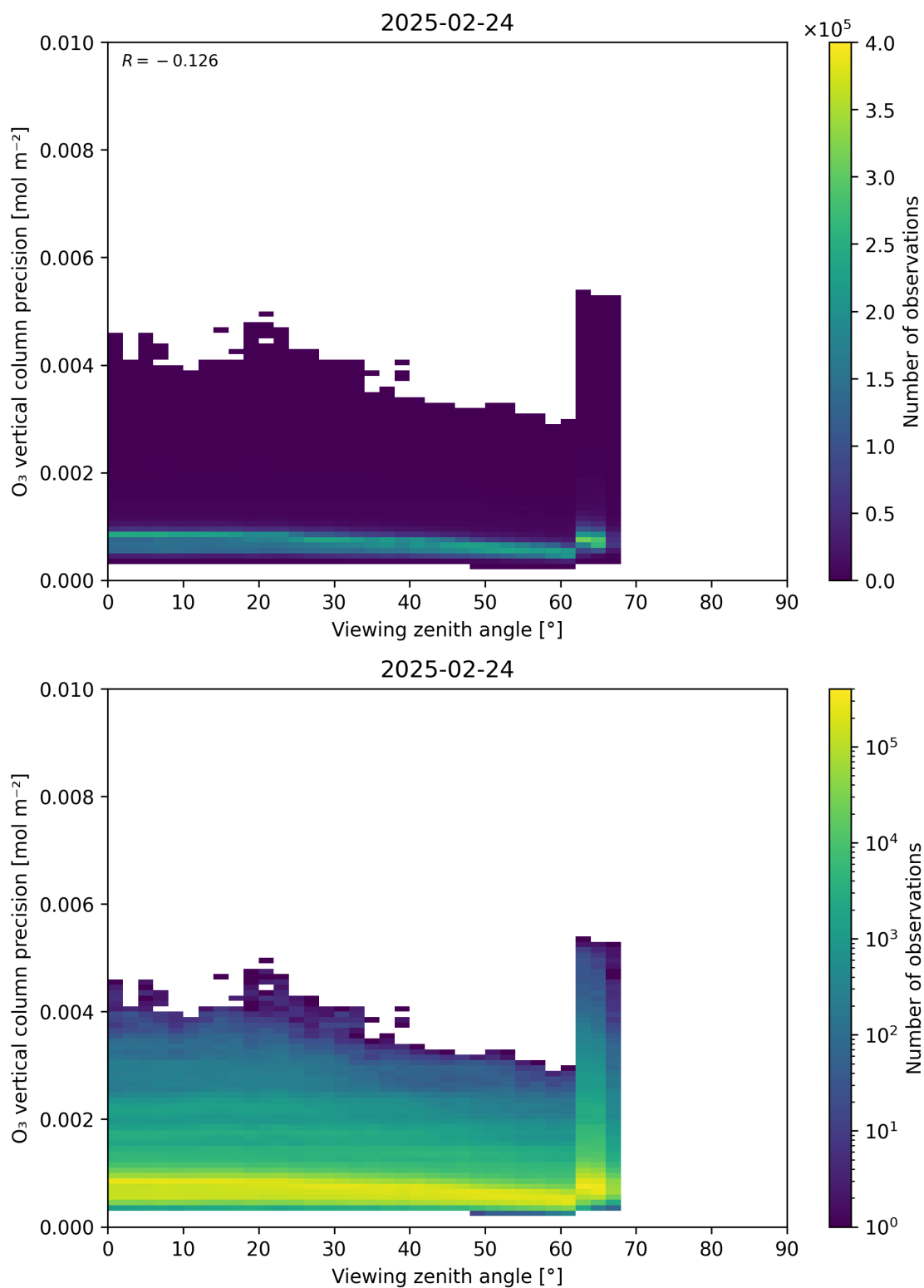
Figure 53: Scatter density plot of “Viewing zenith angle” against “O 3 vertical column precision” for 2025-02-24 to 2025-02-25.
