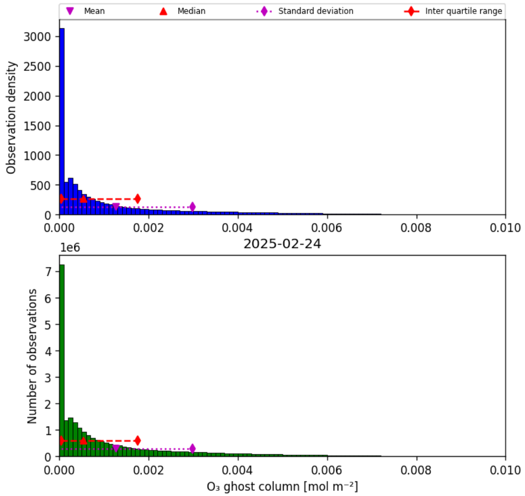
Figure 25: Histogram of “O 3 ghost column” for 2025-02-24 to 2025-02-25
