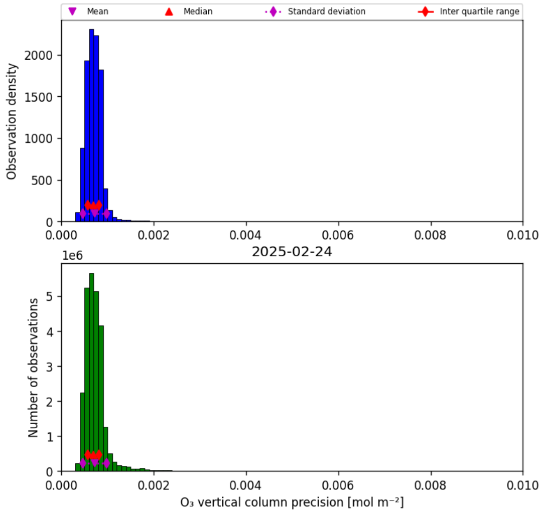
Figure 22: Histogram of “O 3 vertical column precision” for 2025-02-24 to 2025-02-25
