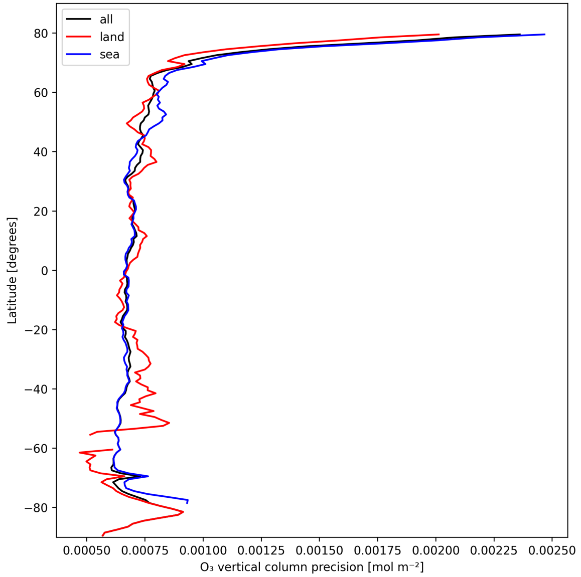
Figure 15: Zonal average of “O 3 vertical column precision” for 2025-02-24 to 2025-02-25.
