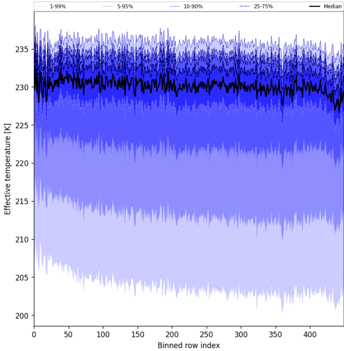
Figure 31: Along track statistics of “Effective temperature” for 2025-02-24 to 2025-02-25
