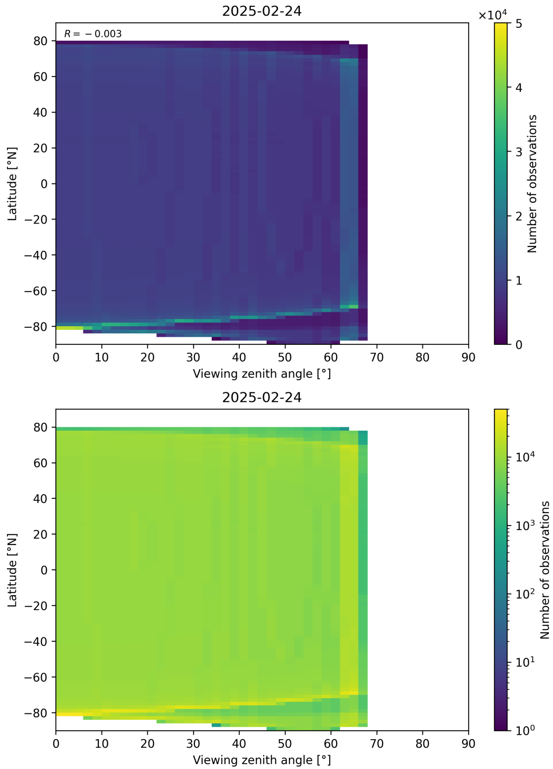
Figure 49: Scatter density plot of “Viewing zenith angle” against “Latitude” for 2025-02-24 to 2025-02-25.
