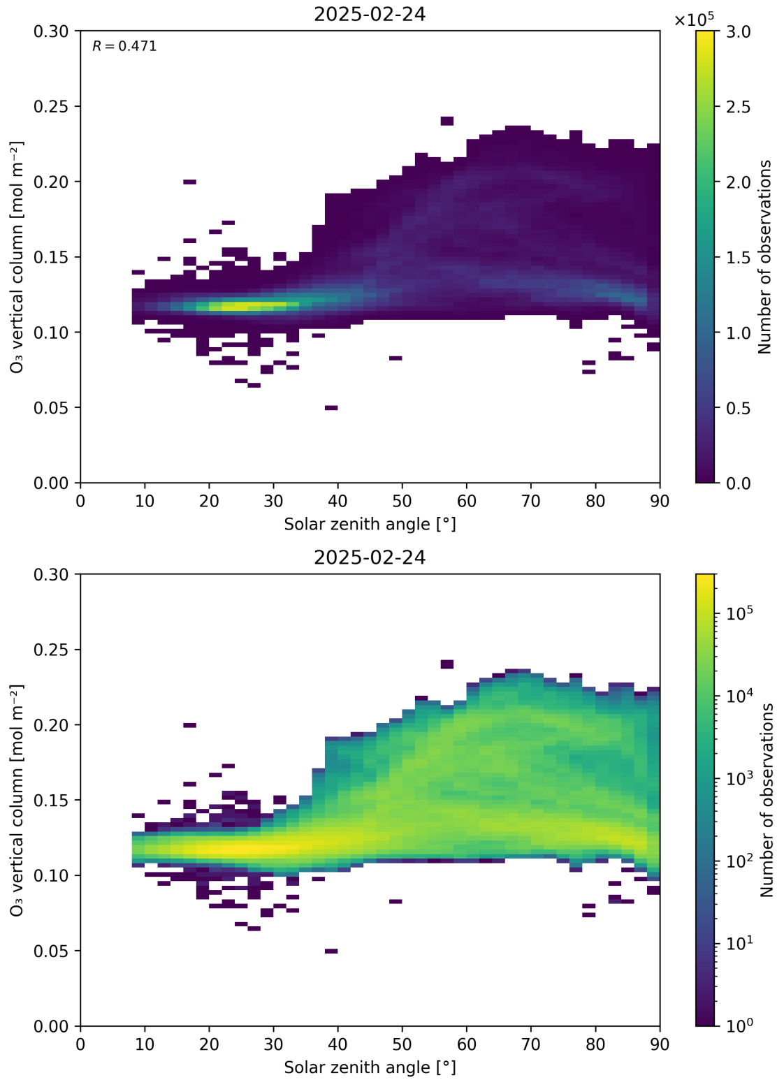
Figure 47: Scatter density plot of “Solar zenith angle” against “O 3 vertical column” for 2025-02-24 to 2025-02-25.
