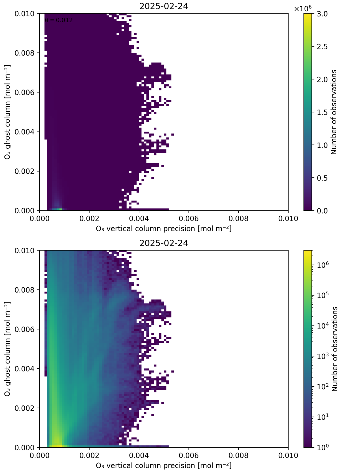
Figure 43: Scatter density plot of “O 3 vertical column precision” against “O 3 ghost column” for 2025-02-24 to 2025-02-25.
