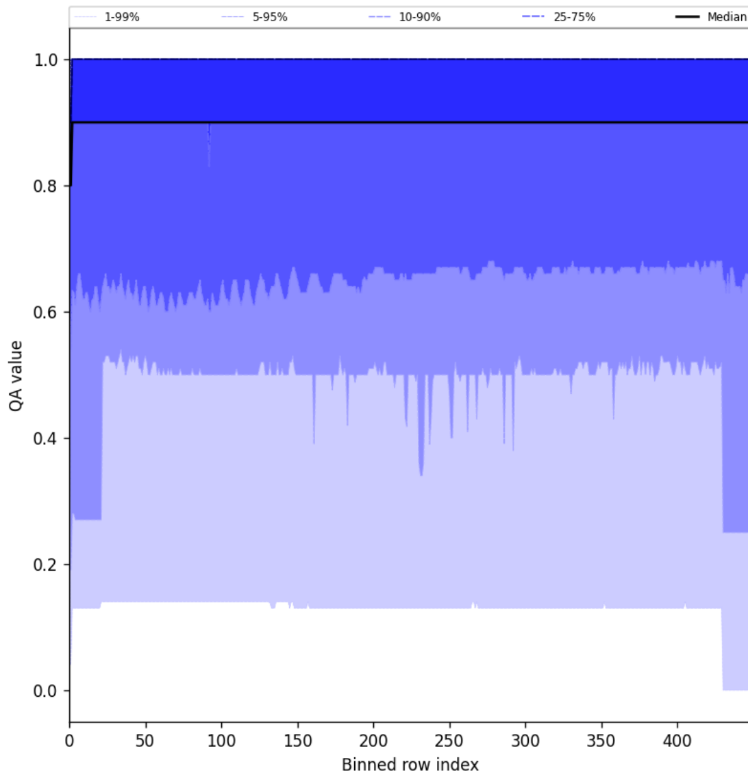
Figure 27: Along track statistics of “QA value” for 2025-02-24 to 2025-02-25
