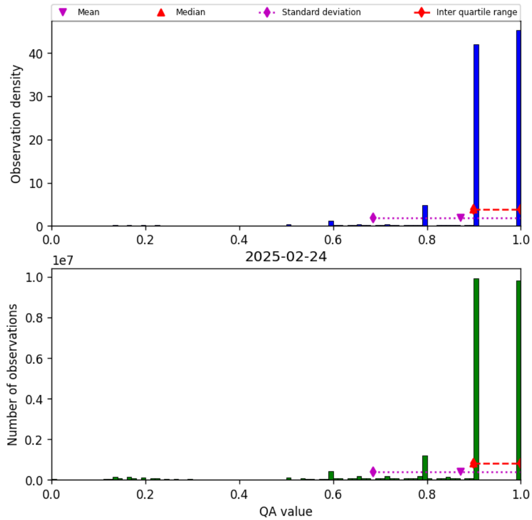
Figure 20: Histogram of “QA value” for 2025-02-24 to 2025-02-25
