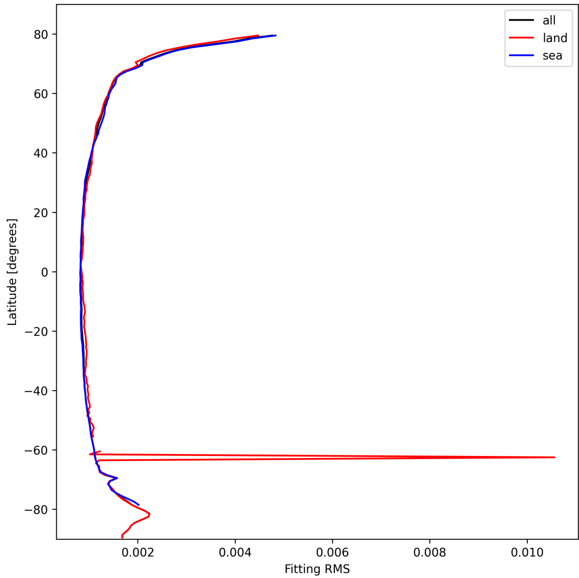
Figure 16: Zonal average of “Fitting RMS” for 2025-02-24 to 2025-02-25.
