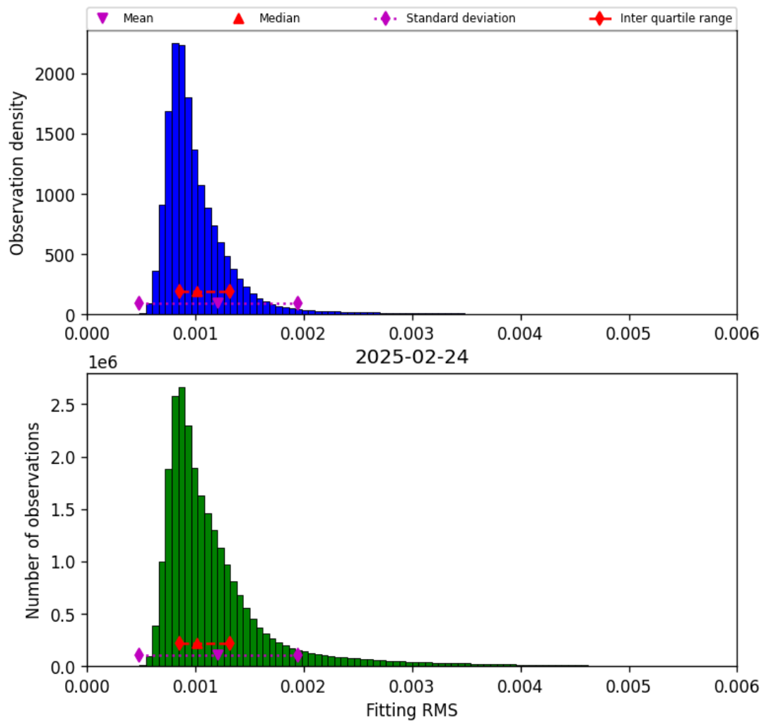
Figure 23: Histogram of “Fitting RMS” for 2025-02-24 to 2025-02-25
