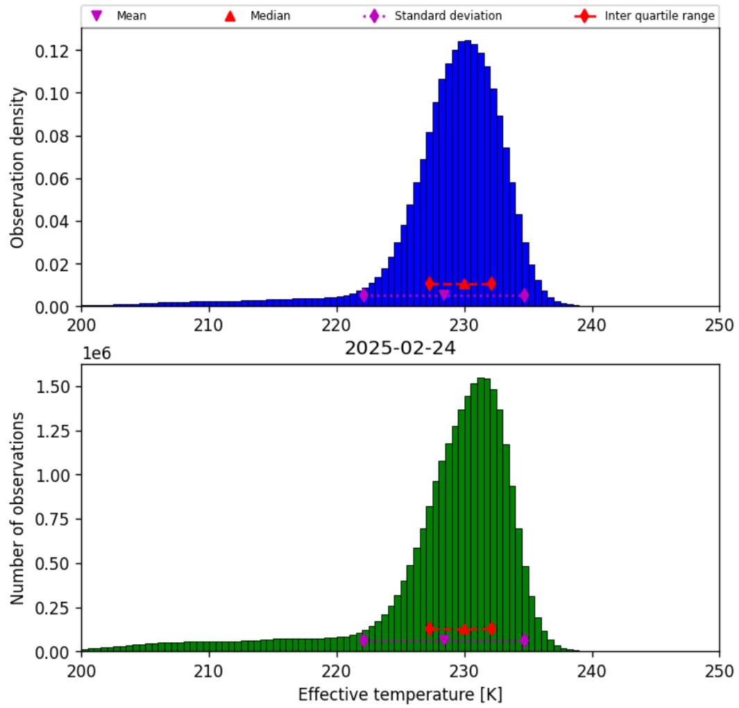
Figure 24: Histogram of “Effective temperature” for 2025-02-24 to 2025-02-25
