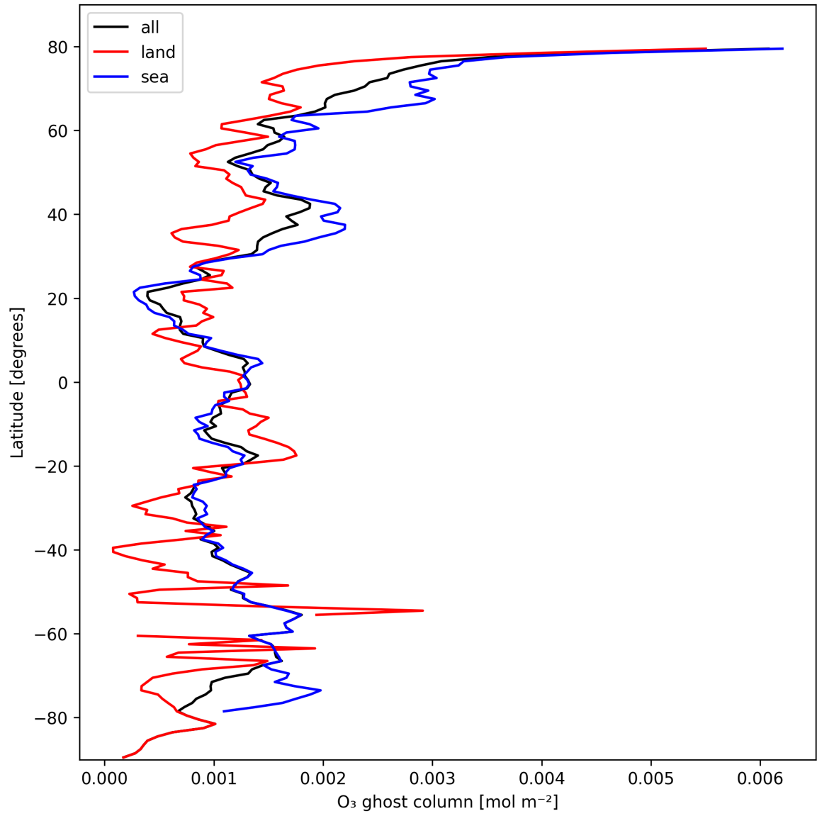
Figure 18: Zonal average of "O 3 ghost column" for 2025-02-24 to 2025-02-25.
