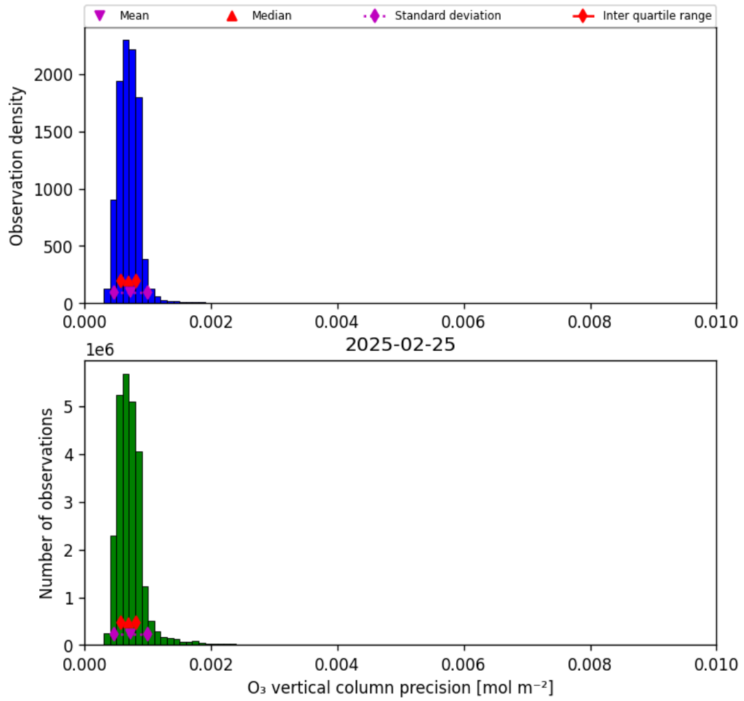
Figure 22: Histogram of “O 3 vertical column precision” for 2025-02-24 to 2025-02-26
