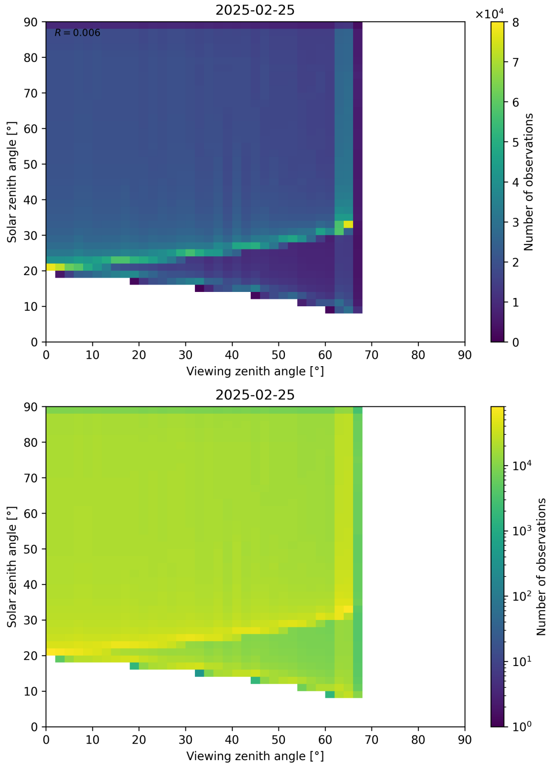
Figure 54: Scatter density plot of “Viewing zenith angle” against “Solar zenith angle” for 2025-02-24 to 2025-02-26.
