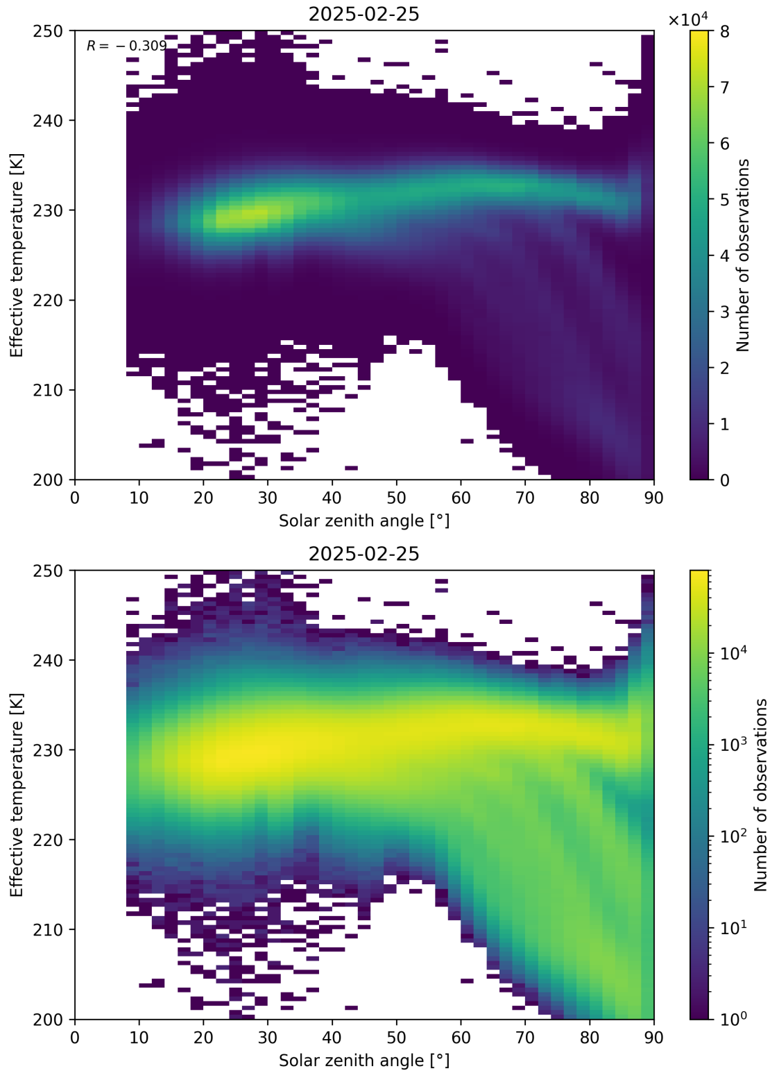
Figure 45: Scatter density plot of “Solar zenith angle” against “Effective temperature” for 2025-02-24 to 2025-02-26.
