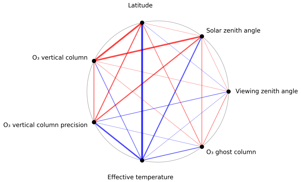
Figure 1: Map of correlation graph for 2025-02-24 to 2025-02-26.
