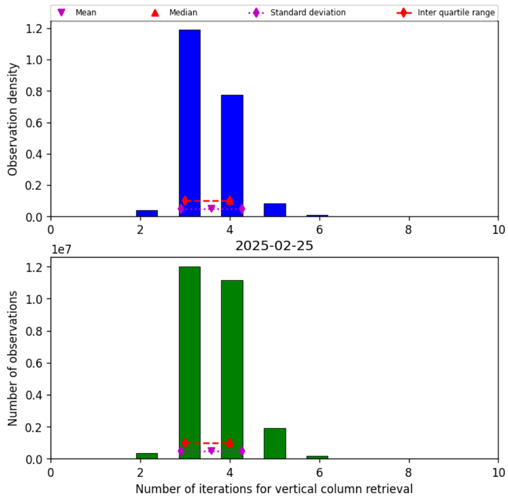
Figure 26: Histogram of “Number of iterations for vertical column retrieval” for 2025-02-24 to 2025-02-26
