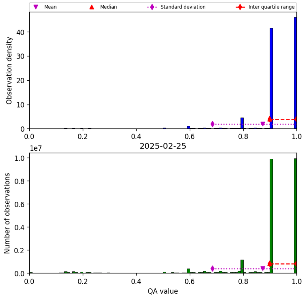
Figure 20: Histogram of “QA value” for 2025-02-24 to 2025-02-26
