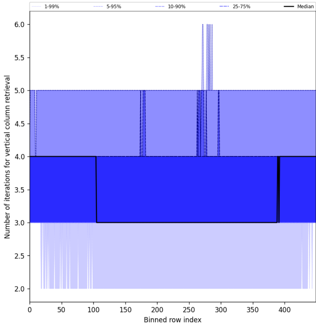
Figure 33: Along track statistics of “Number of iterations for vertical column retrieval” for 2025-02-24 to 2025-02-26
