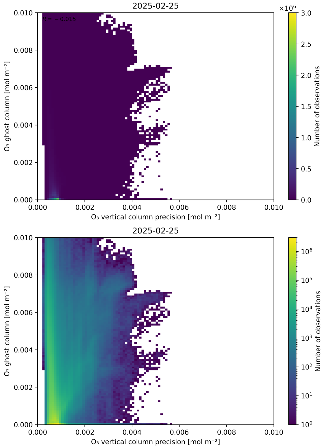
Figure 43: Scatter density plot of “ \text{O}_3 vertical column precision” against “ \text{O}_3 ghost column” for 2025-02-24 to 2025-02-26.
