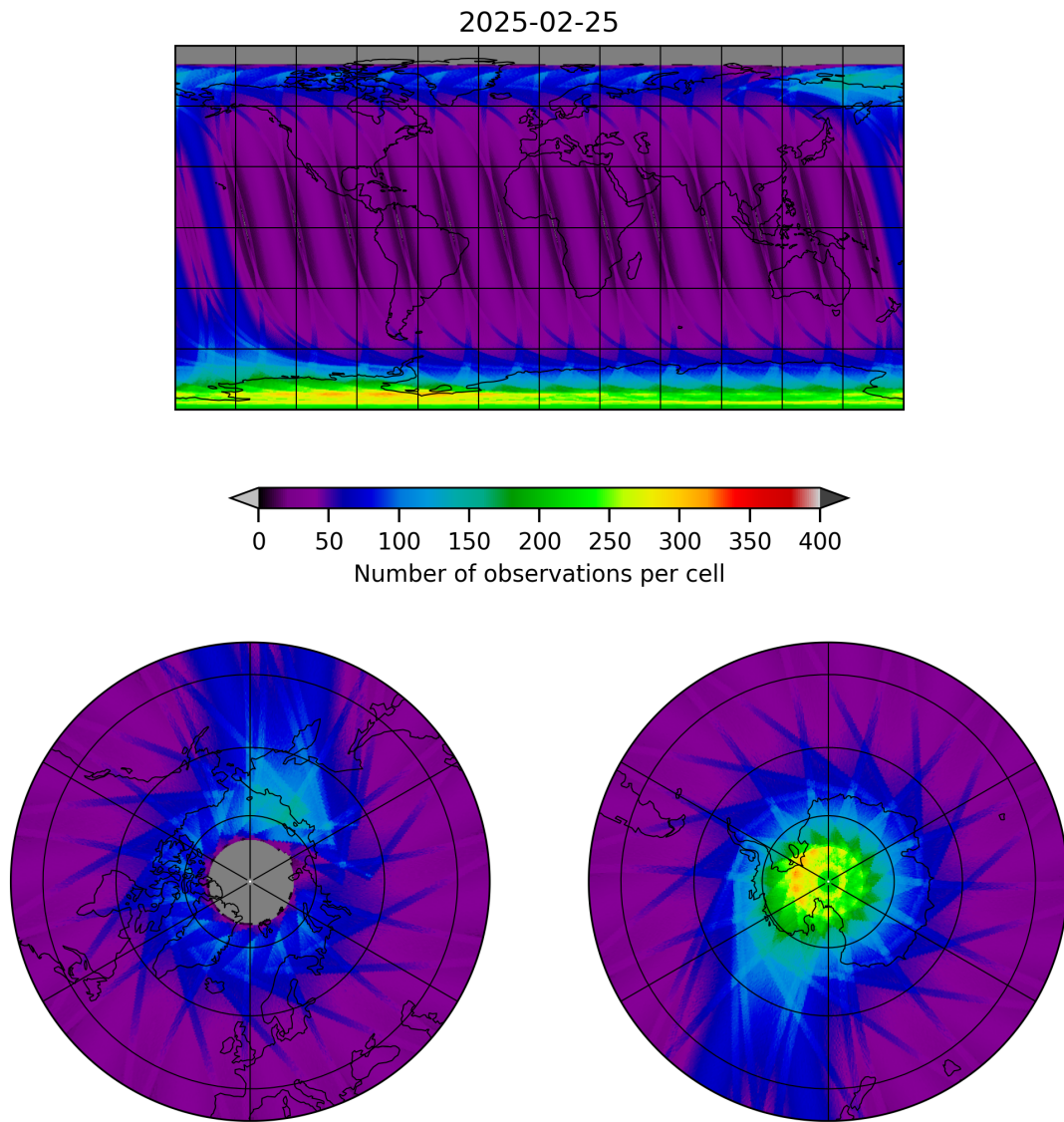
Figure 12: Map of the number of observations for 2025-02-24 to 2025-02-26
