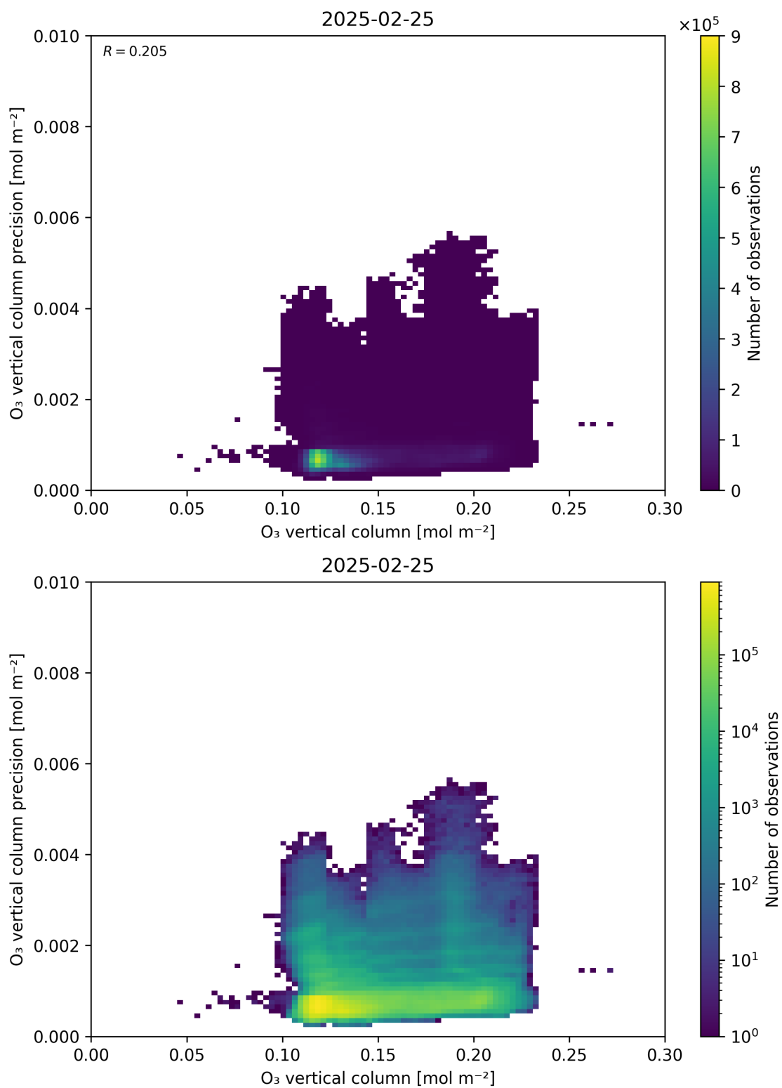
Figure 41: Scatter density plot of “O 3 vertical column” against “O 3 vertical column precision” for 2025-02-24 to 2025-02-26.
