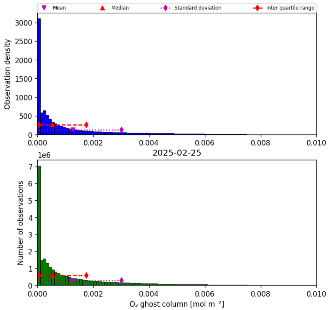
Figure 25: Histogram of “O 3 ghost column” for 2025-02-24 to 2025-02-26
