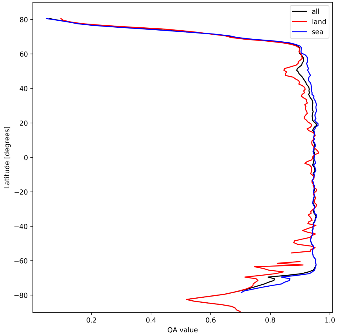
Figure 13: Zonal average of “QA value” for 2025-02-24 to 2025-02-26.
