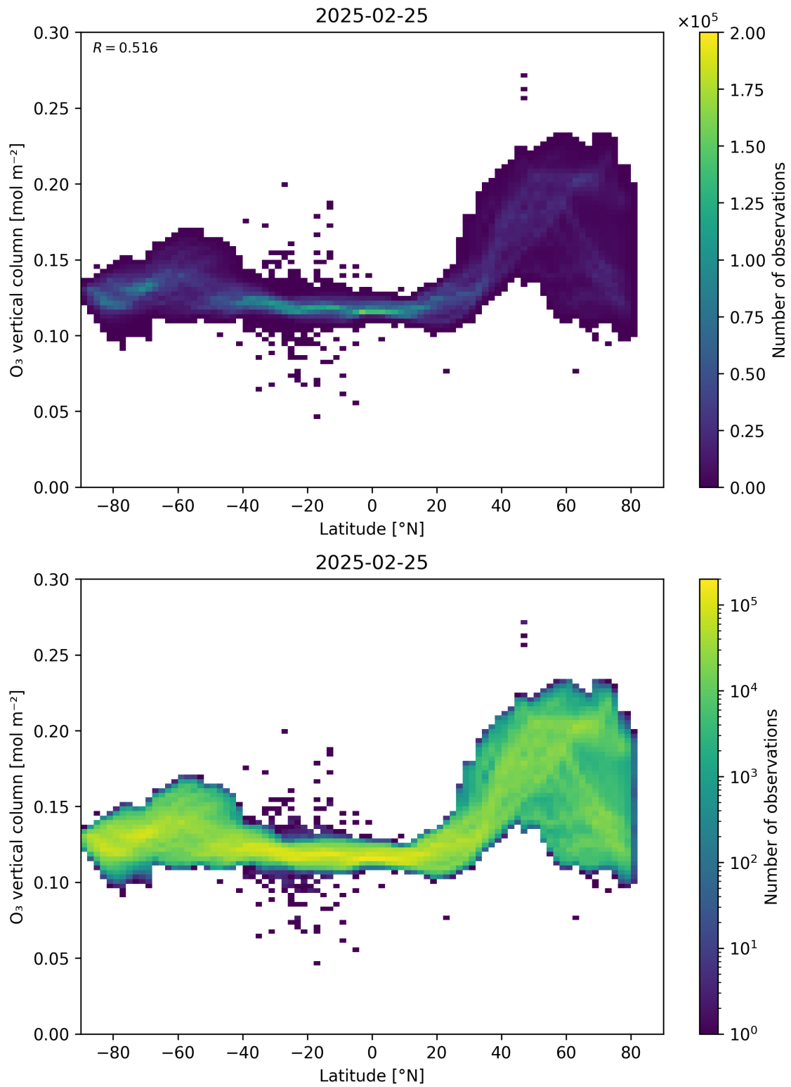
Figure 36: Scatter density plot of “Latitude” against “O 3 vertical column” for 2025-02-24 to 2025-02-26.
