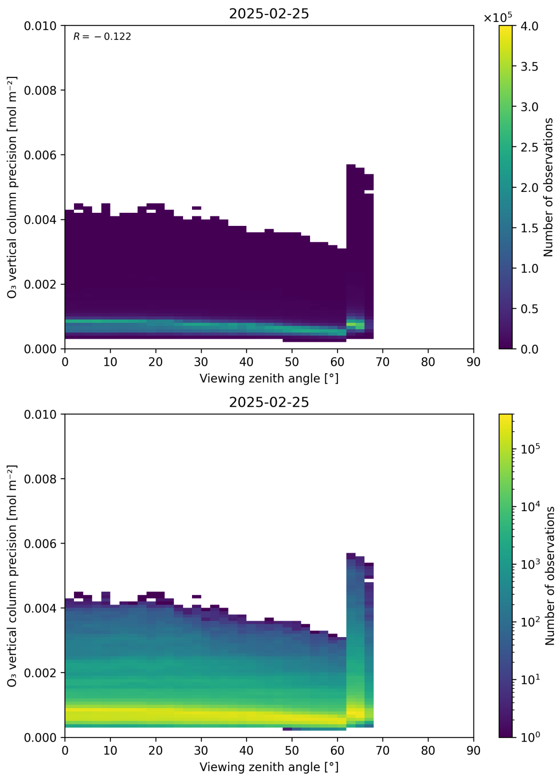
Figure 53: Scatter density plot of “Viewing zenith angle” against “O 3 vertical column precision” for 2025-02-24 to 2025-02-26.
