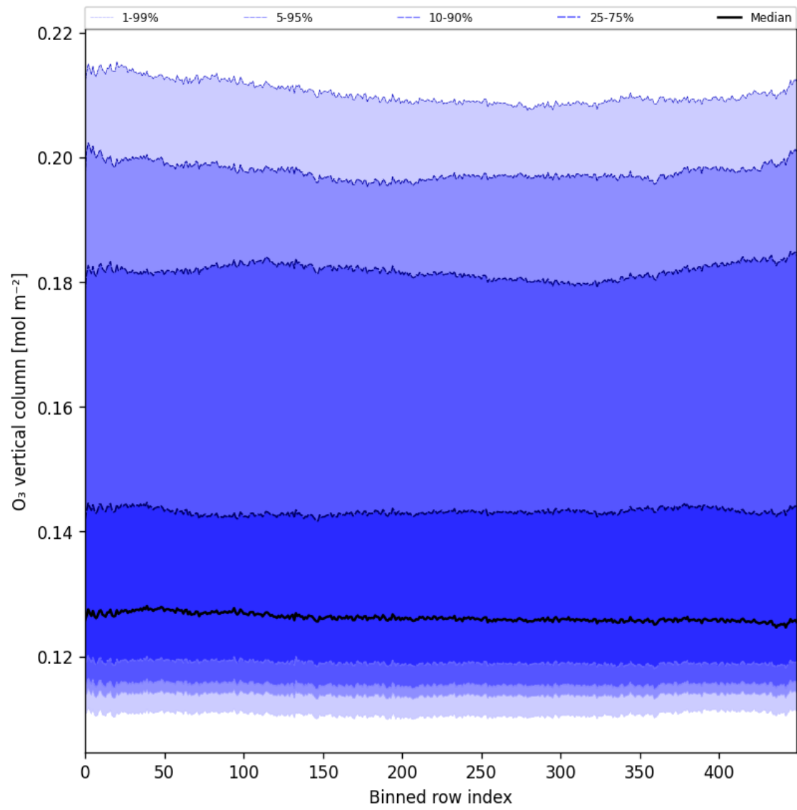
Figure 28: Along track statistics of “O 3 vertical column” for 2025-02-24 to 2025-02-26
