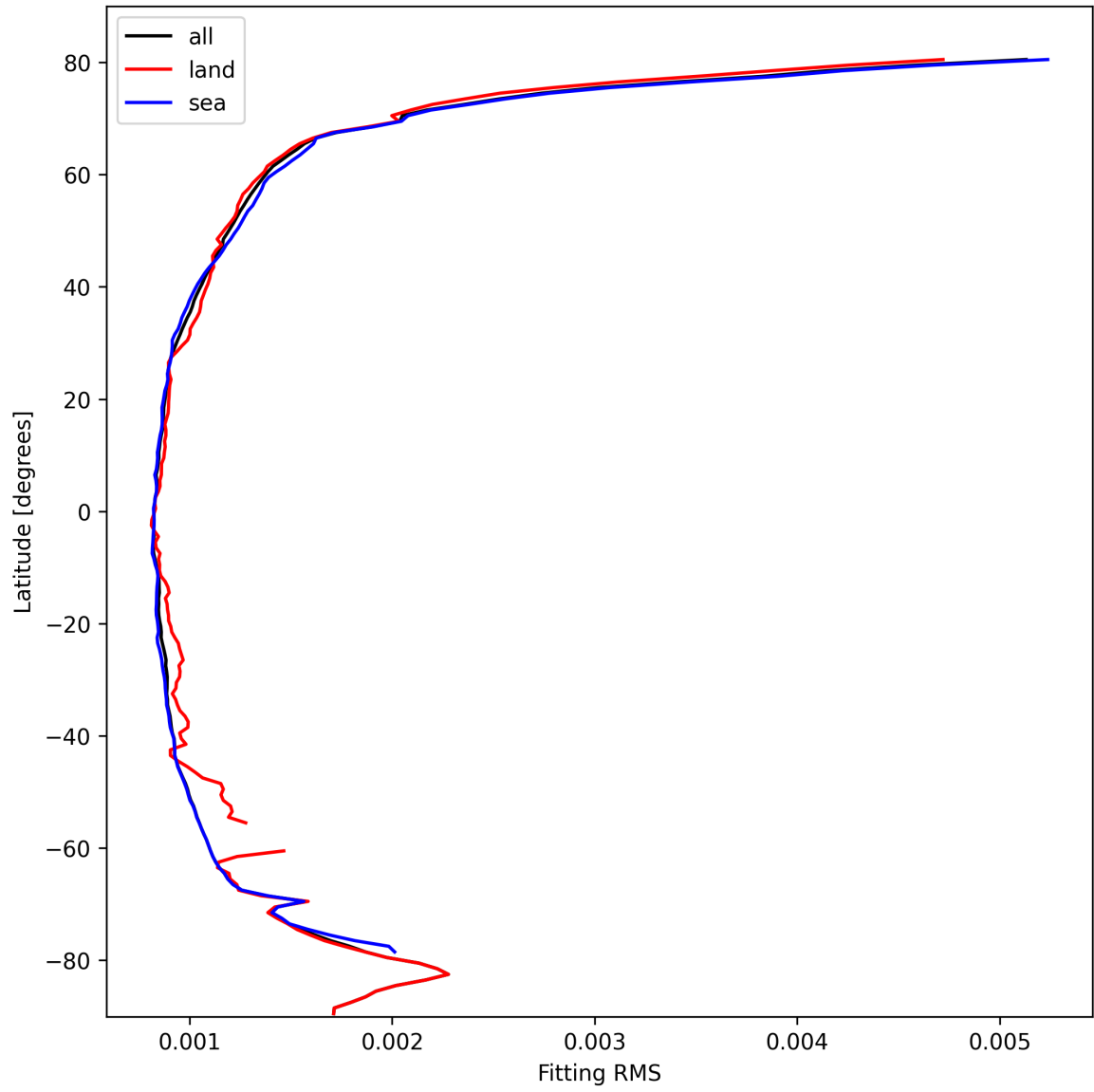
Figure 16: Zonal average of “Fitting RMS” for 2025-02-24 to 2025-02-26.
