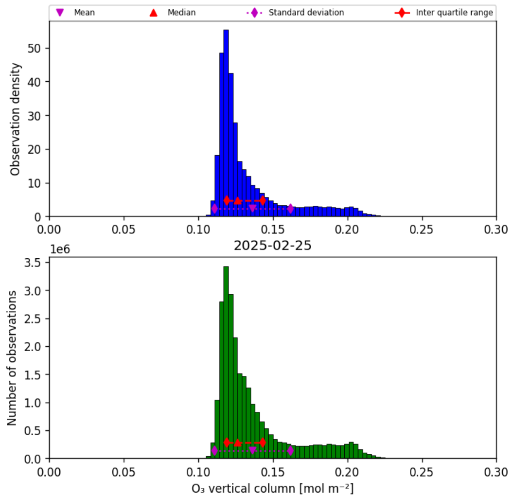
Figure 21: Histogram of “O 3 vertical column” for 2025-02-24 to 2025-02-26
