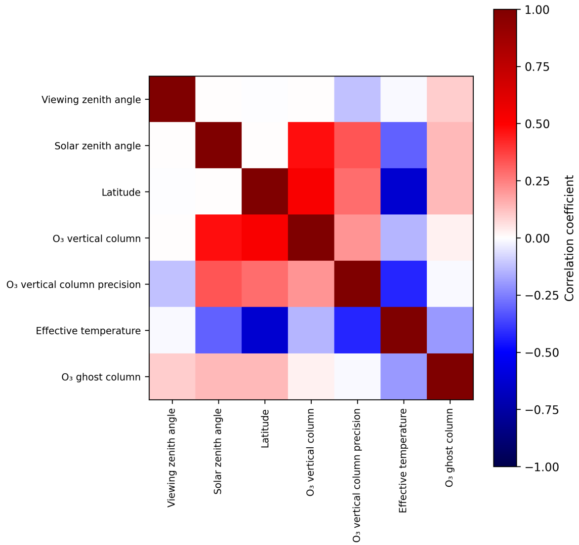
Figure 2: Map of correlation matrix for 2025-02-24 to 2025-02-26.
