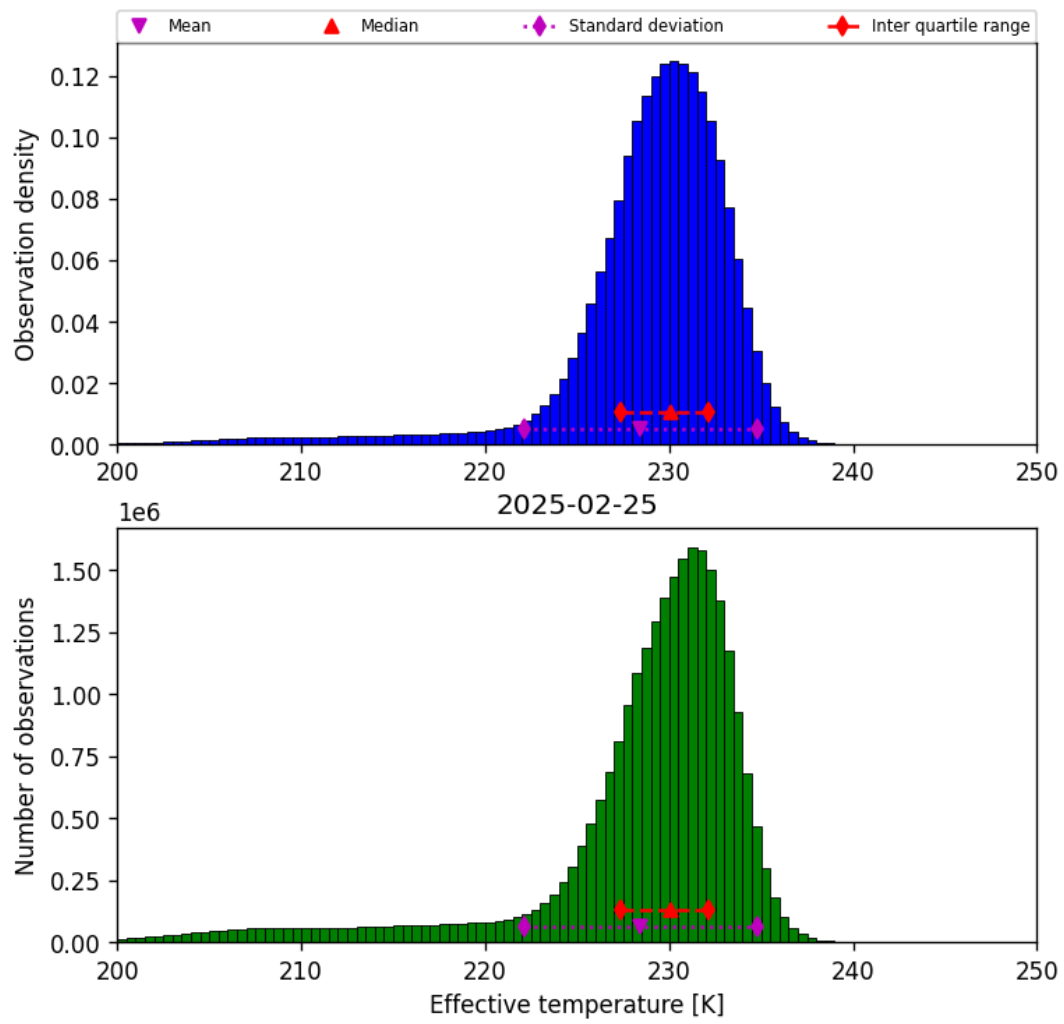
Figure 24: Histogram of “Effective temperature” for 2025-02-24 to 2025-02-26
