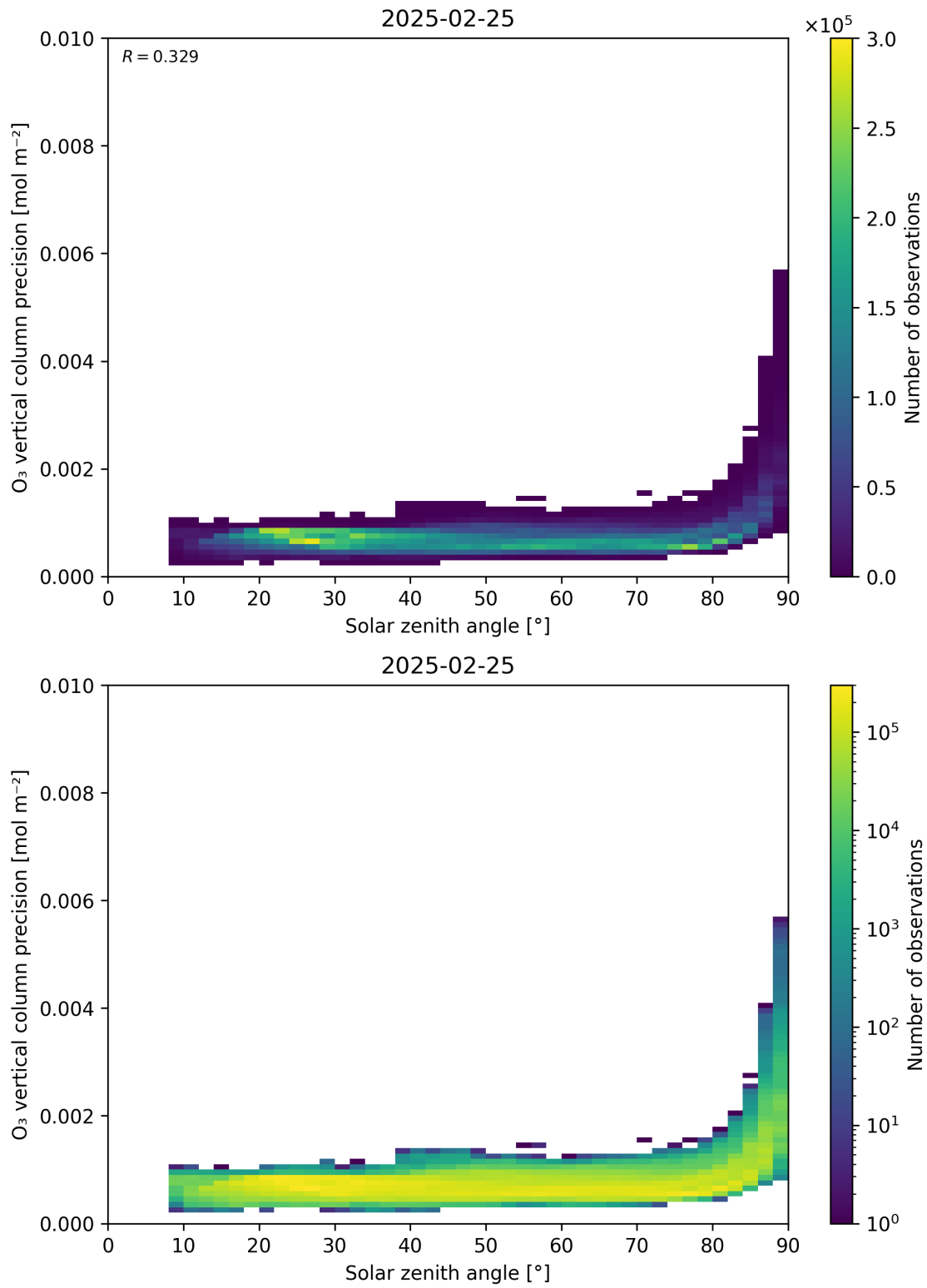
Figure 48: Scatter density plot of “Solar zenith angle” against “O 3 vertical column precision” for 2025-02-24 to 2025-02-26.
