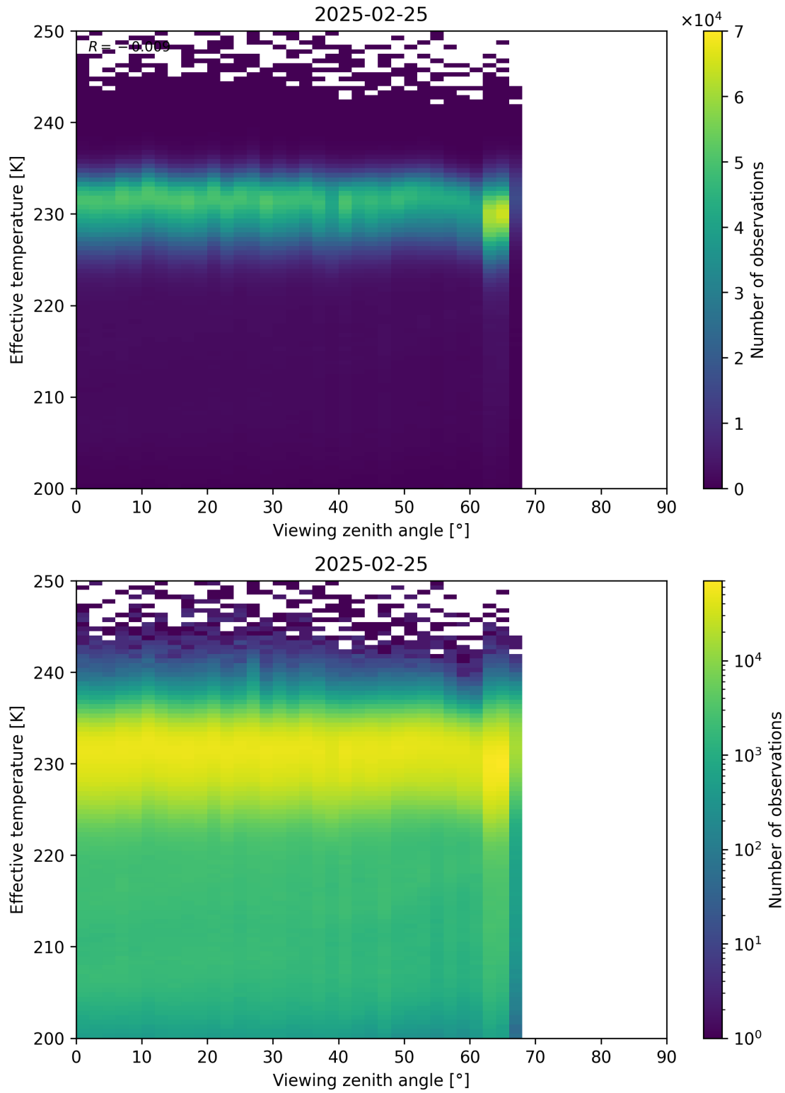
Figure 50: Scatter density plot of “Viewing zenith angle” against “Effective temperature” for 2025-02-24 to 2025-02-26.
