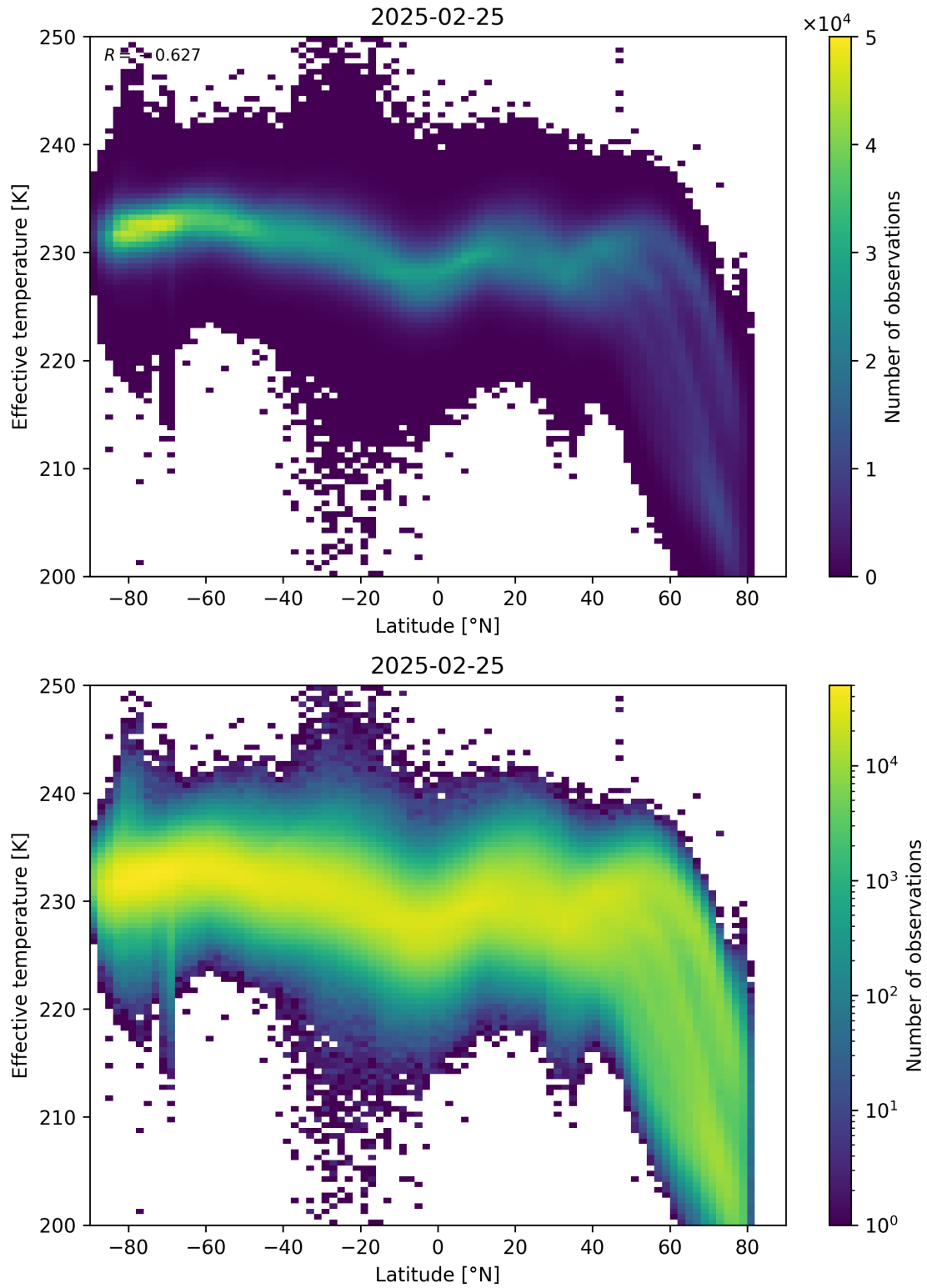
Figure 34: Scatter density plot of “Latitude” against “Effective temperature” for 2025-02-24 to 2025-02-26.
