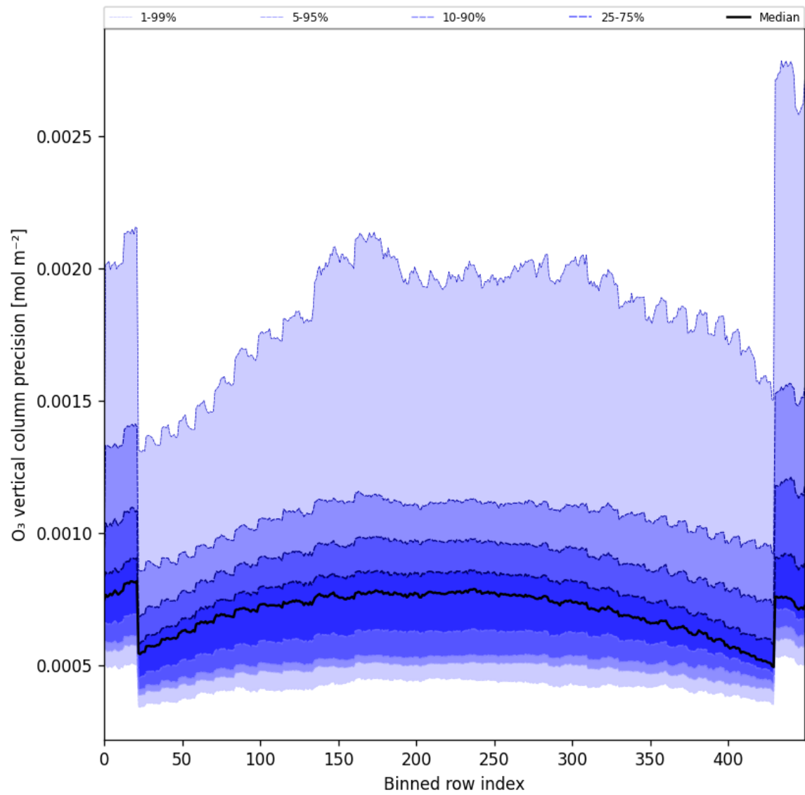
Figure 29: Along track statistics of “O 3 vertical column precision” for 2025-02-24 to 2025-02-26
