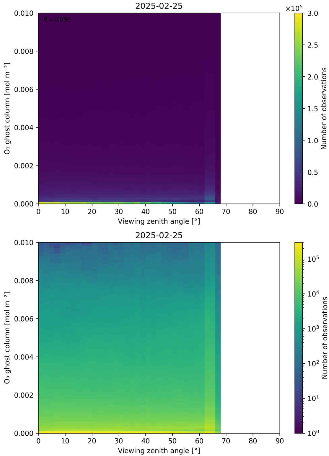
Figure 51: Scatter density plot of “Viewing zenith angle” against “O 3 ghost column” for 2025-02-24 to 2025-02-26.
