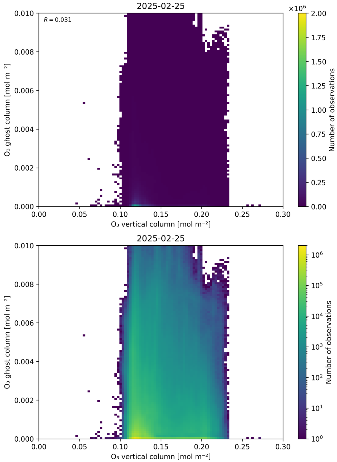
Figure 40: Scatter density plot of “O 3 vertical column” against “O 3 ghost column” for 2025-02-24 to 2025-02-26.
