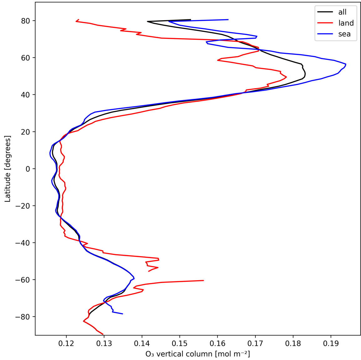
Figure 14: Zonal average of “O 3 vertical column” for 2025-02-24 to 2025-02-26.
