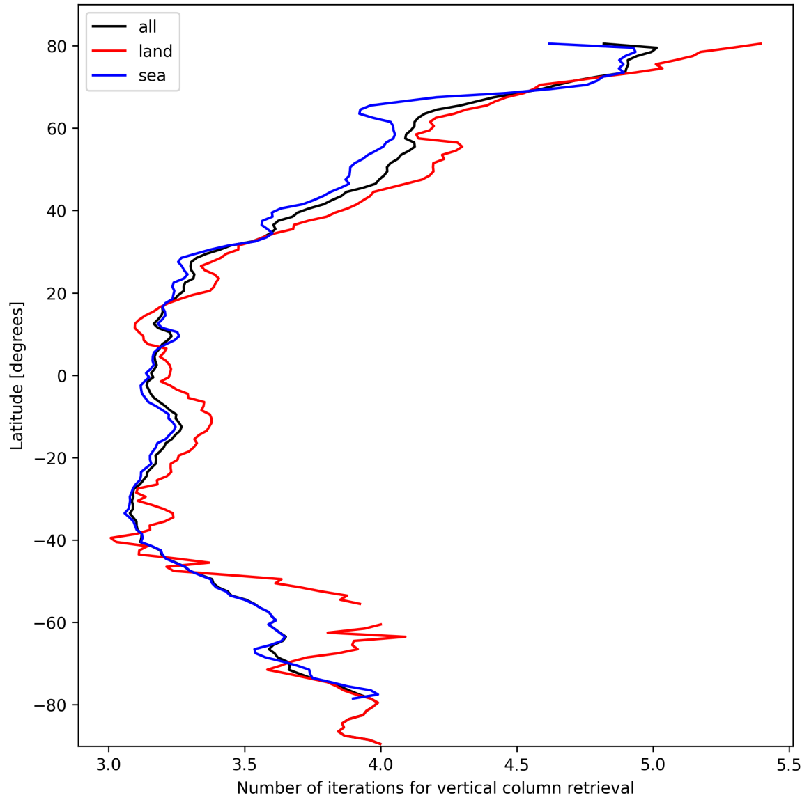
Figure 19: Zonal average of “Number of iterations for vertical column retrieval” for 2025-02-24 to 2025-02-26.
