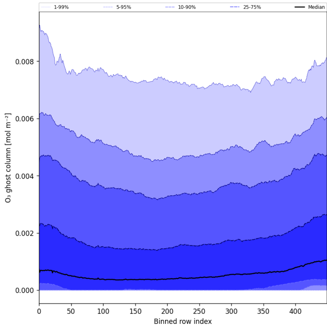
Figure 32: Along track statistics of “O 3 ghost column” for 2025-02-24 to 2025-02-26
