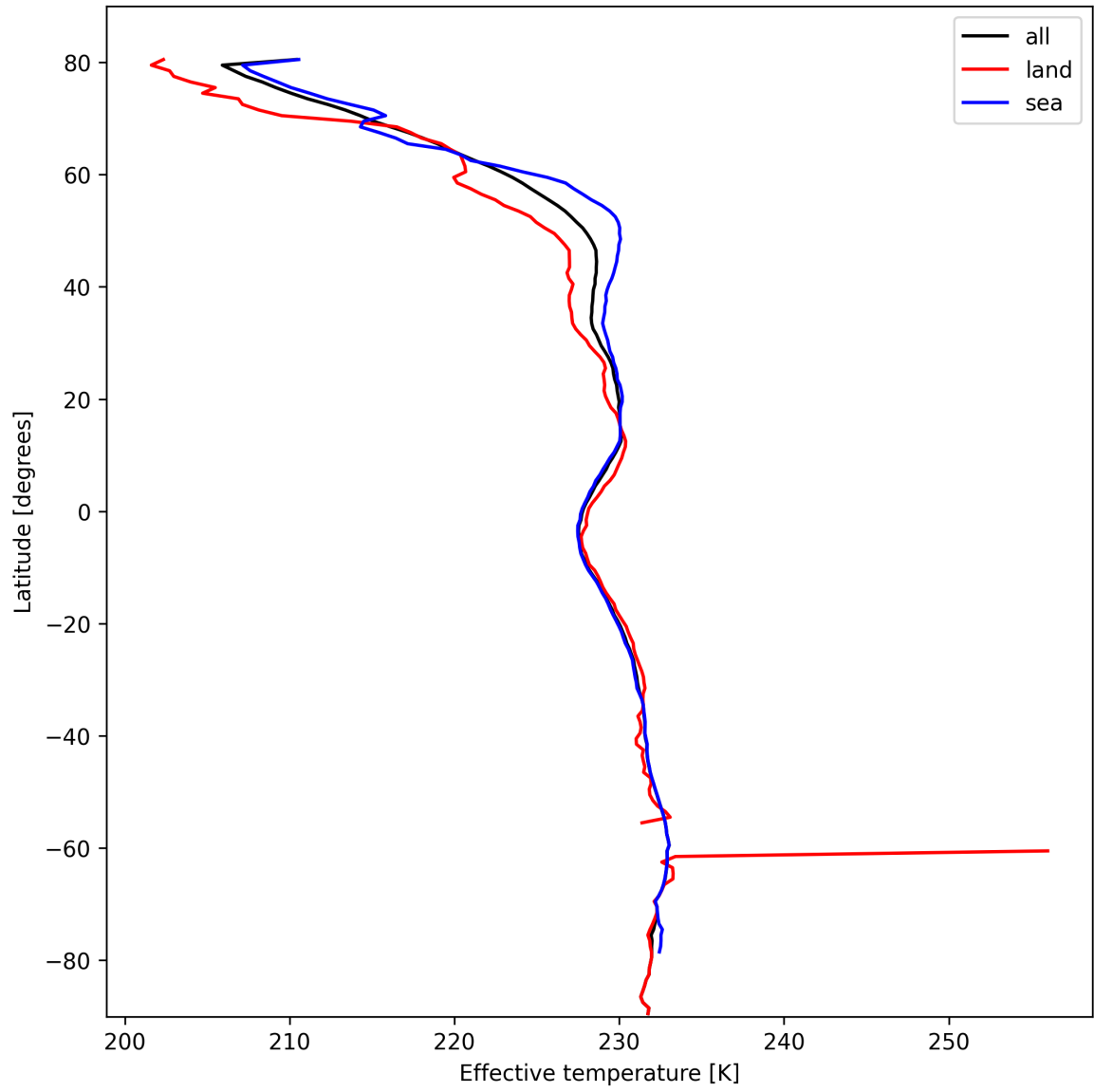
Figure 17: Zonal average of “Effective temperature” for 2025-02-24 to 2025-02-26.
