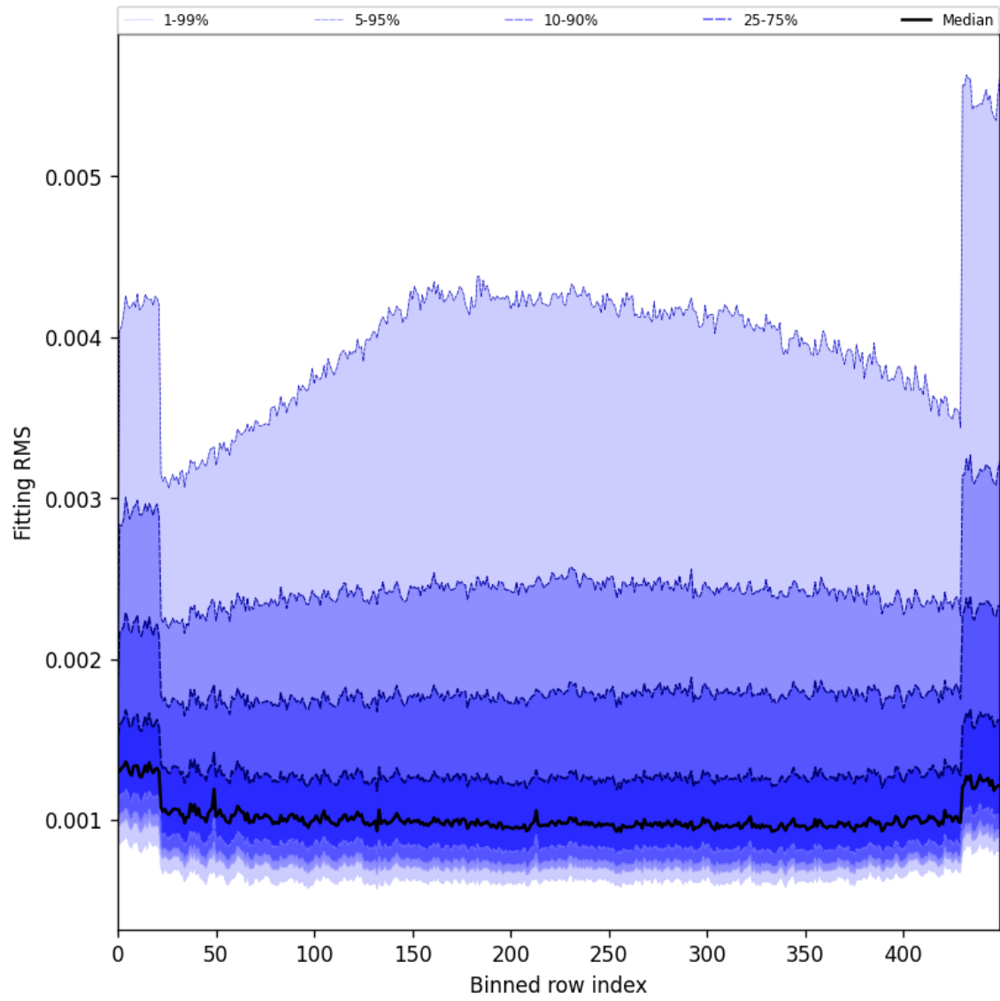
Figure 30: Along track statistics of “Fitting RMS” for 2025-02-24 to 2025-02-26
