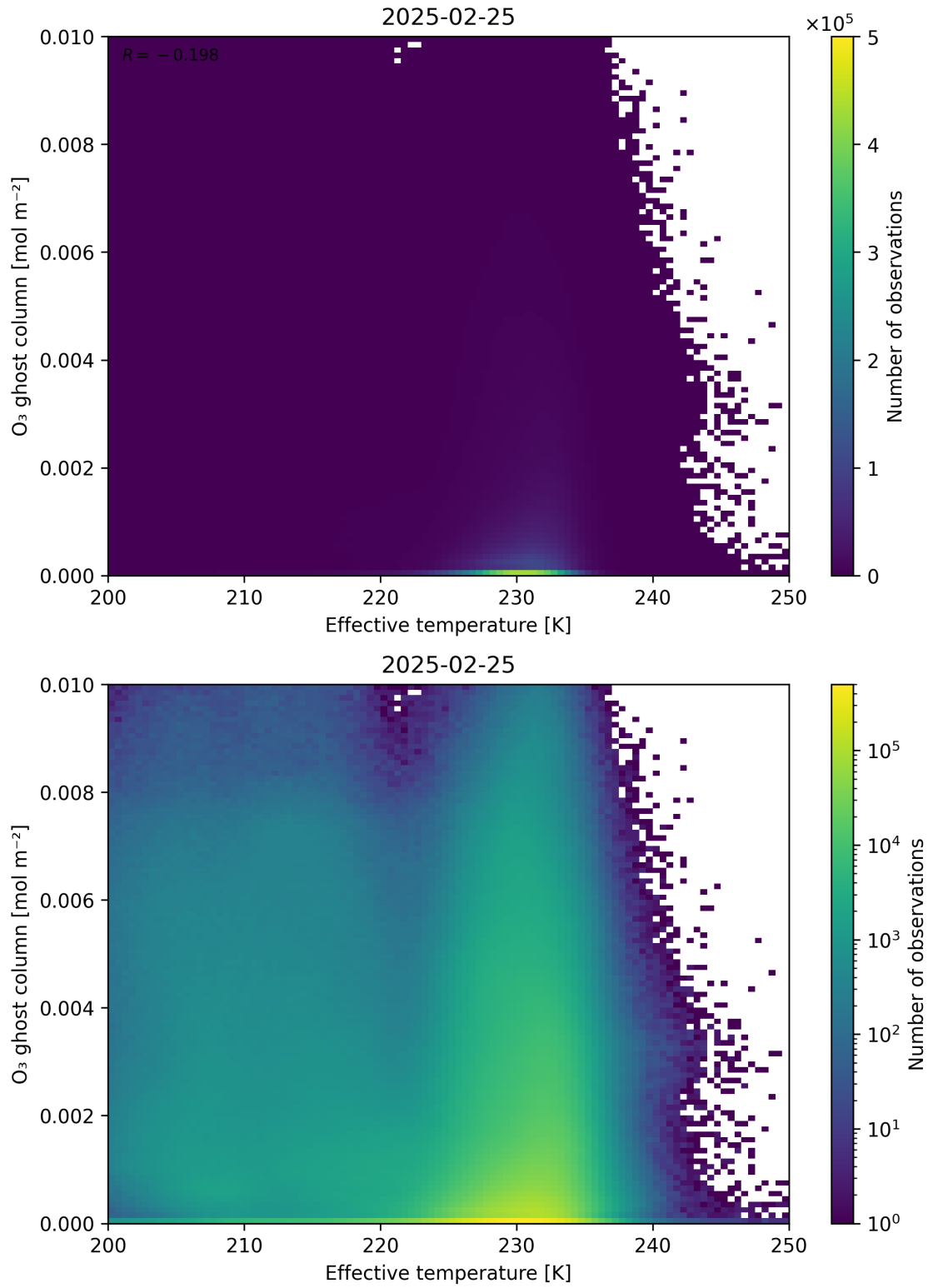
Figure 38: Scatter density plot of “Effective temperature” against “O 3 ghost column” for 2025-02-24 to 2025-02-26.
