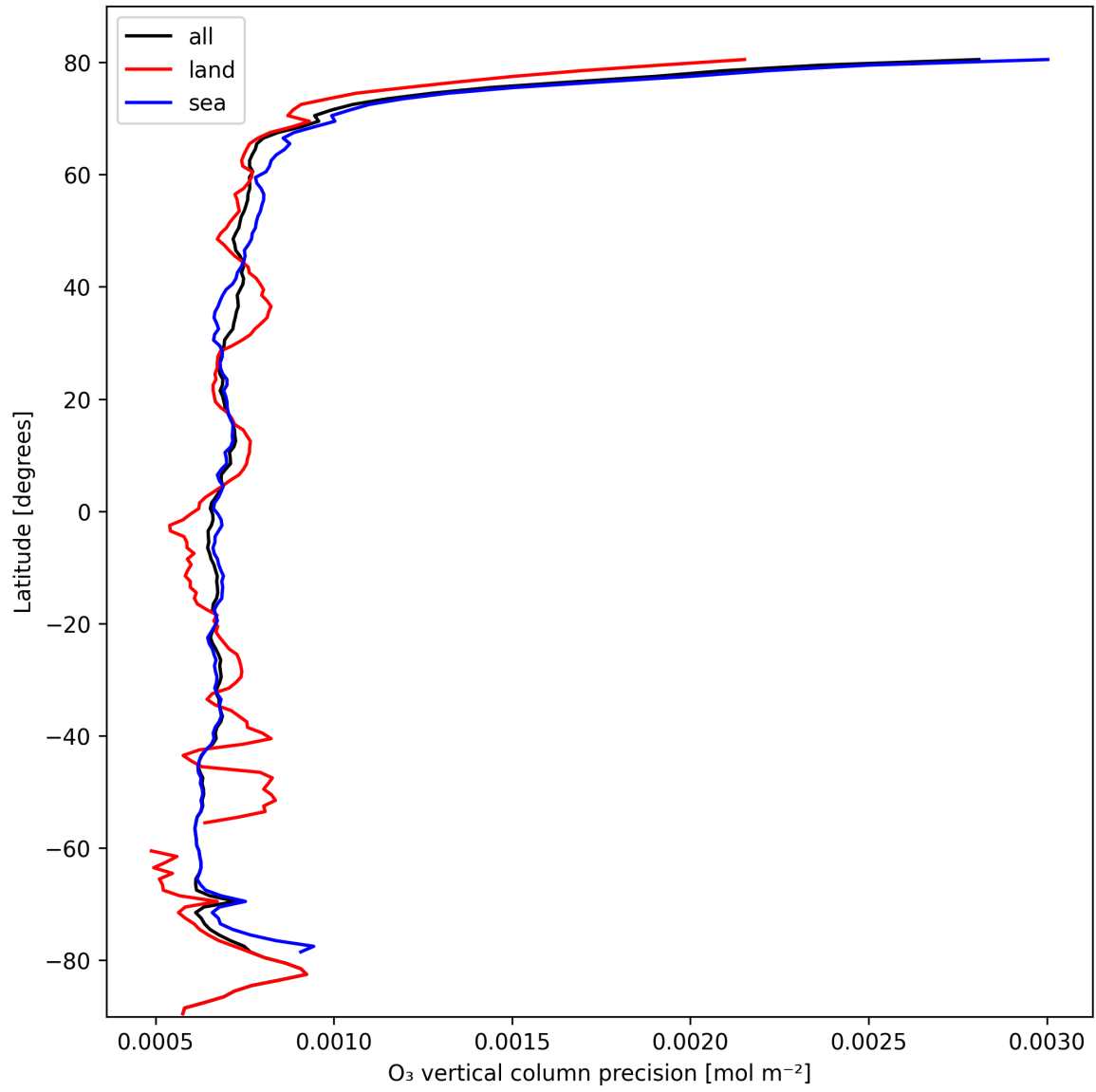
Figure 15: Zonal average of “O 3 vertical column precision” for 2025-02-24 to 2025-02-26.
