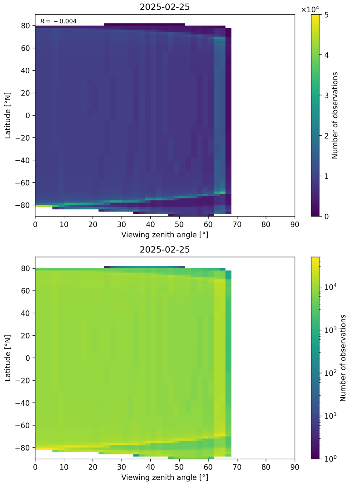
Figure 49: Scatter density plot of “Viewing zenith angle” against “Latitude” for 2025-02-24 to 2025-02-26.
