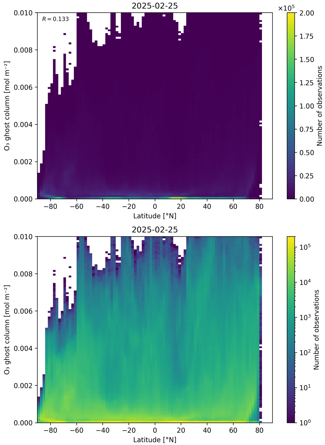
Figure 35: Scatter density plot of “Latitude” against “O 3 ghost column” for 2025-02-24 to 2025-02-26.
