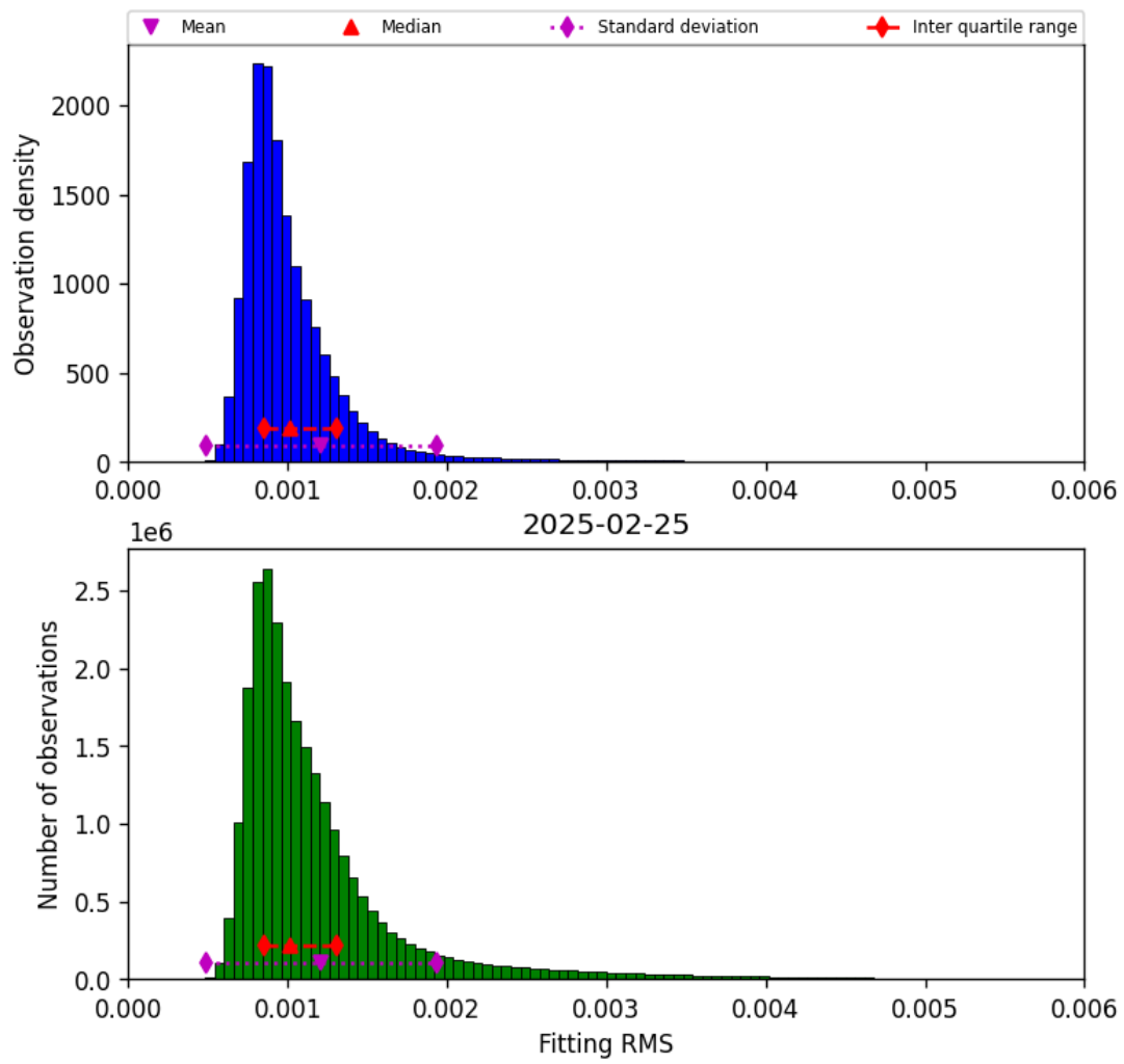
Figure 23: Histogram of “Fitting RMS” for 2025-02-24 to 2025-02-26
