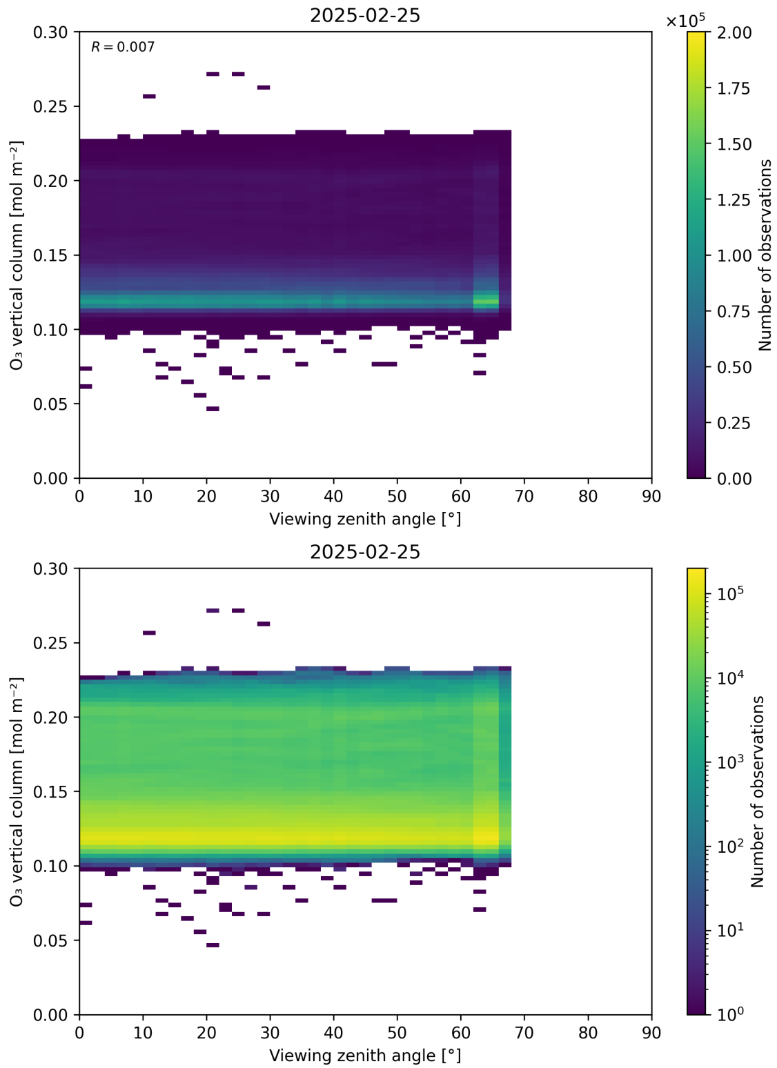
Figure 52: Scatter density plot of “Viewing zenith angle” against “O 3 vertical column” for 2025-02-24 to 2025-02-26.
