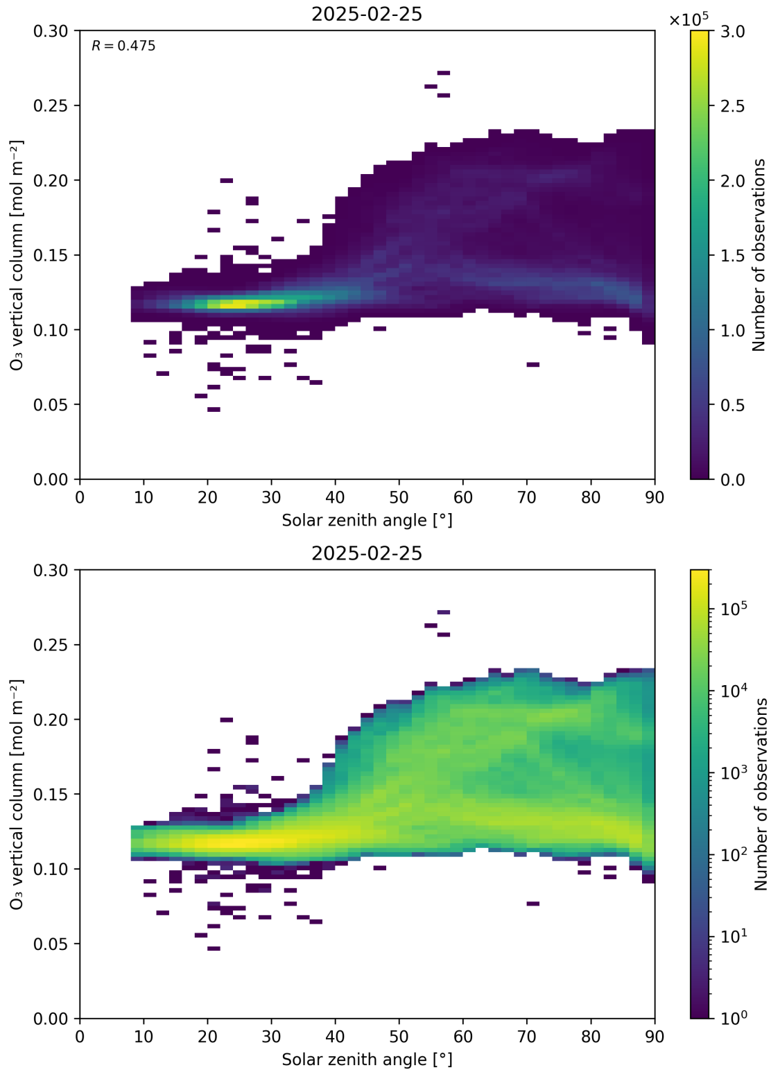
Figure 47: Scatter density plot of “Solar zenith angle” against “O 3 vertical column” for 2025-02-24 to 2025-02-26.
