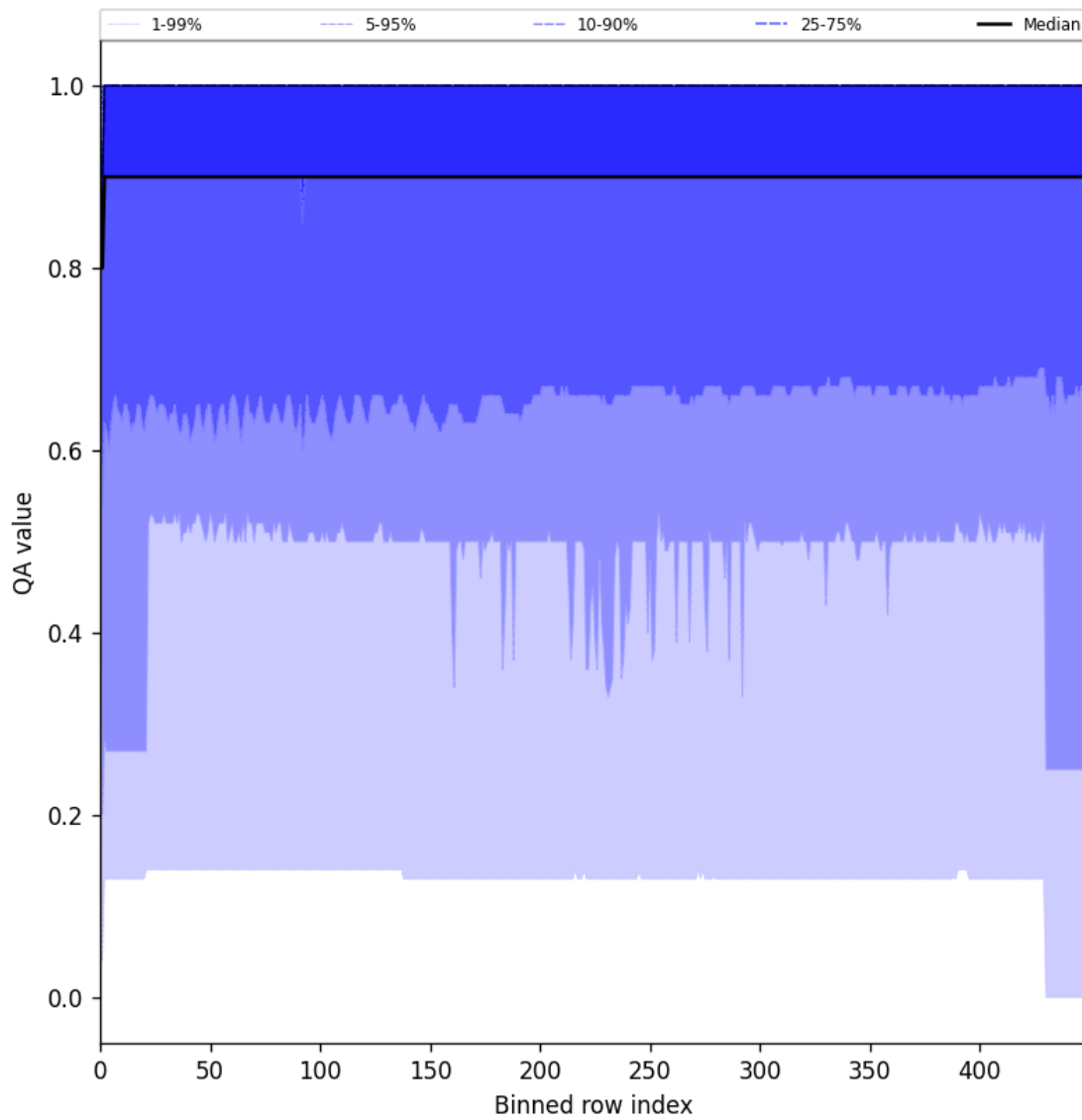
Figure 27: Along track statistics of “QA value” for 2025-02-24 to 2025-02-26
