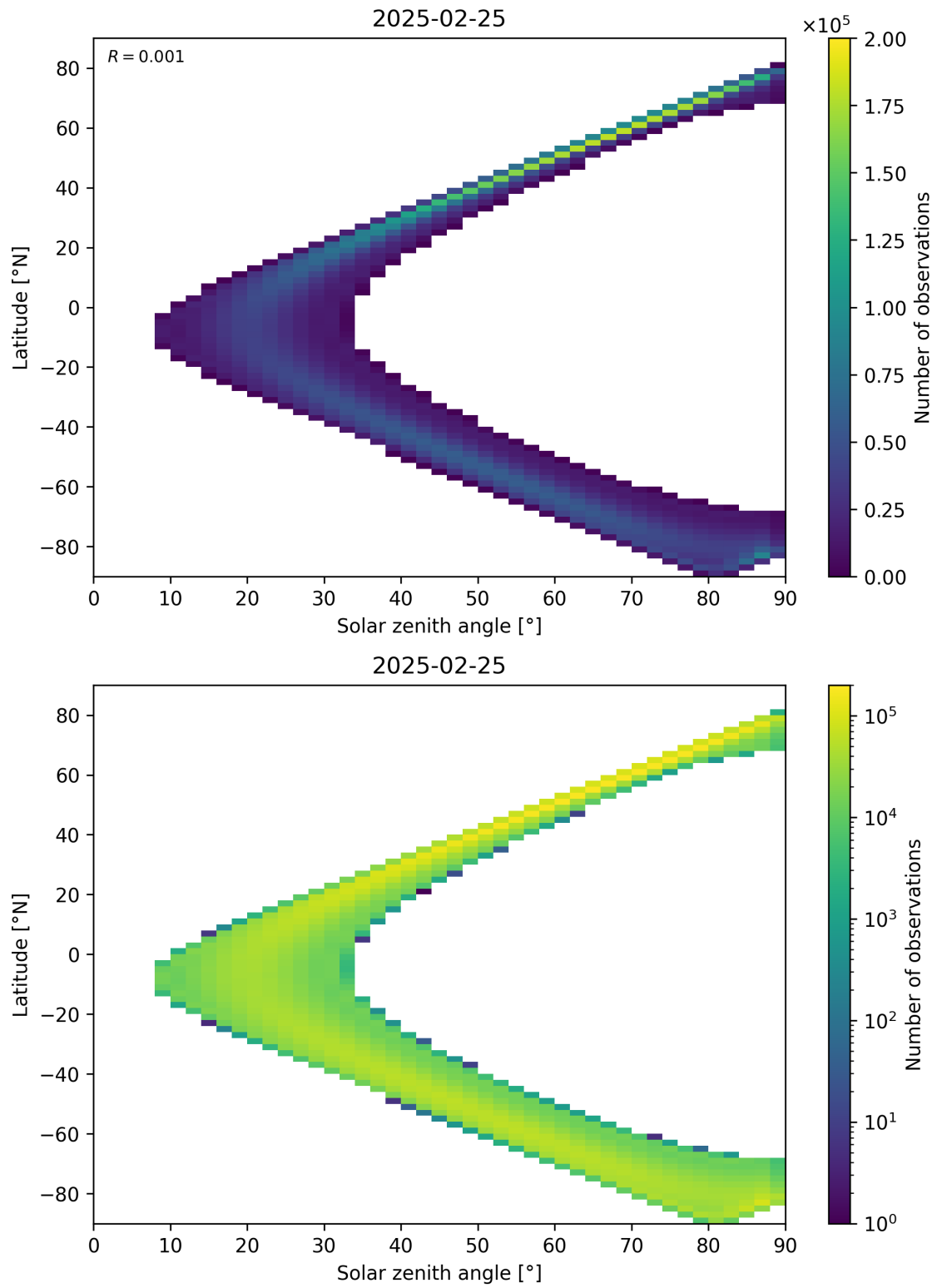
Figure 44: Scatter density plot of “Solar zenith angle” against “Latitude” for 2025-02-24 to 2025-02-26.
