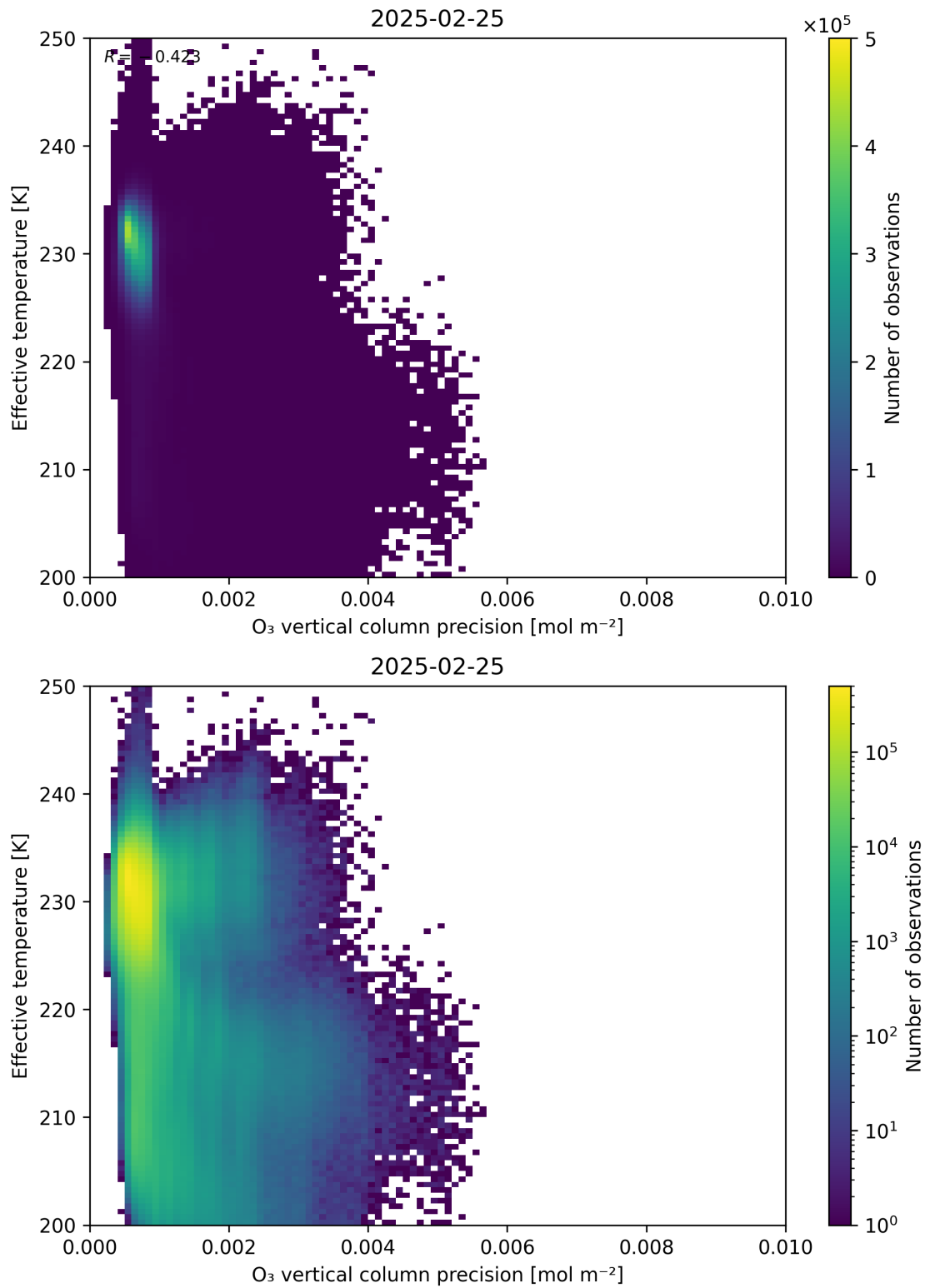
Figure 42: Scatter density plot of “O 3 vertical column precision” against “Effective temperature” for 2025-02-24 to 2025-02-26.
