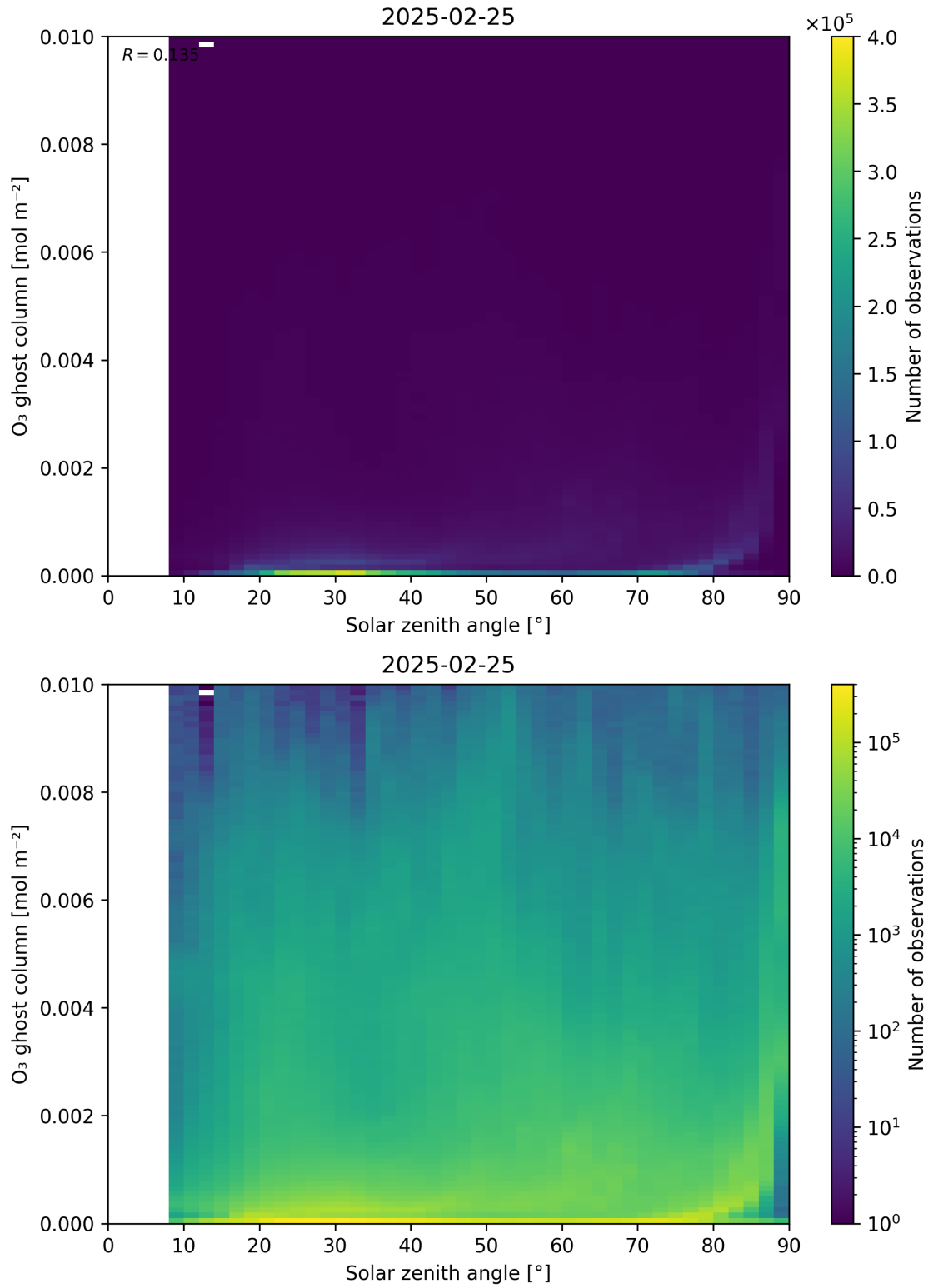
Figure 46: Scatter density plot of “Solar zenith angle” against “O 3 ghost column” for 2025-02-24 to 2025-02-26.
