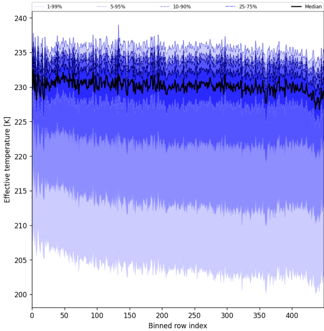
Figure 31: Along track statistics of “Effective temperature” for 2025-02-24 to 2025-02-26
