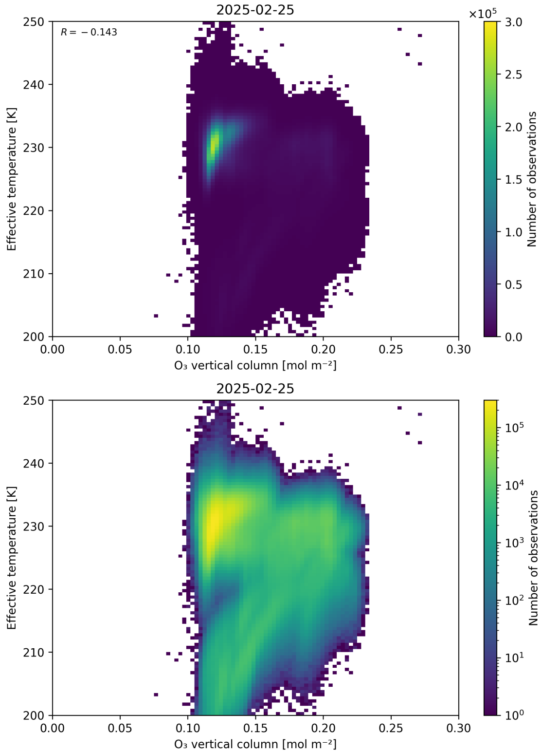
Figure 39: Scatter density plot of “O 3 vertical column” against “Effective temperature” for 2025-02-24 to 2025-02-26.
