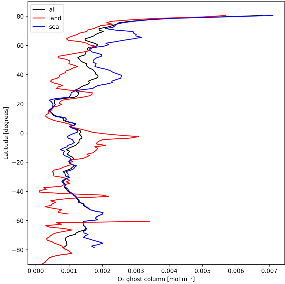
Figure 18: Zonal average of "O 3 ghost column" for 2025-02-24 to 2025-02-26.
