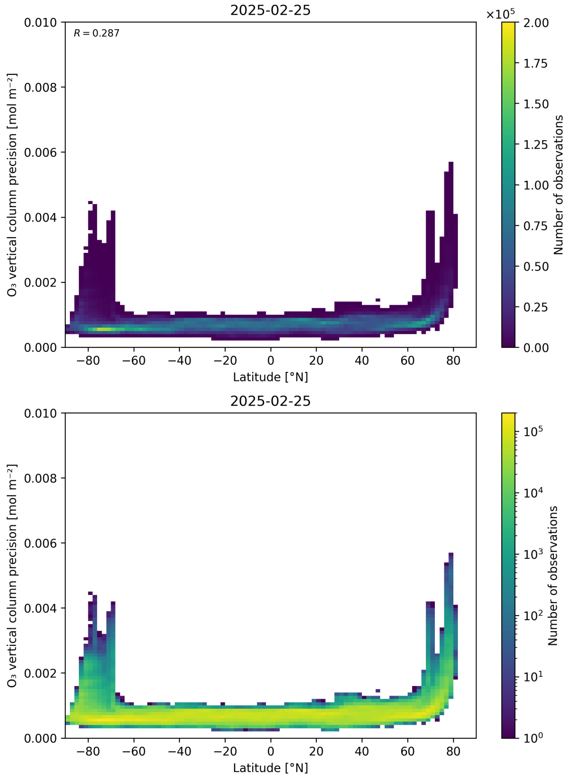
Figure 37: Scatter density plot of “Latitude” against “O 3 vertical column precision” for 2025-02-24 to 2025-02-26.
