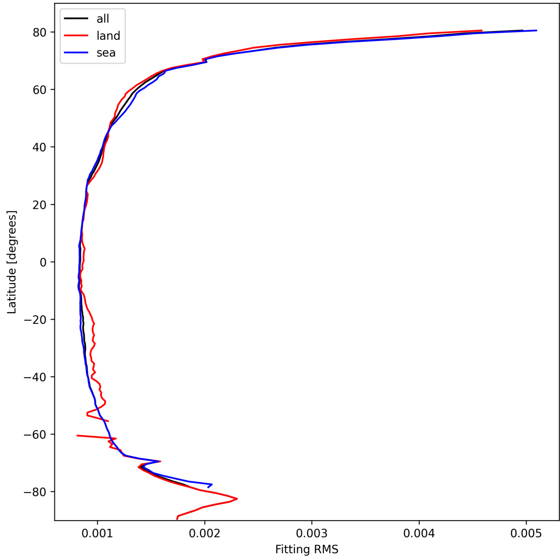
Figure 16: Zonal average of “Fitting RMS” for 2025-02-25 to 2025-02-27.
