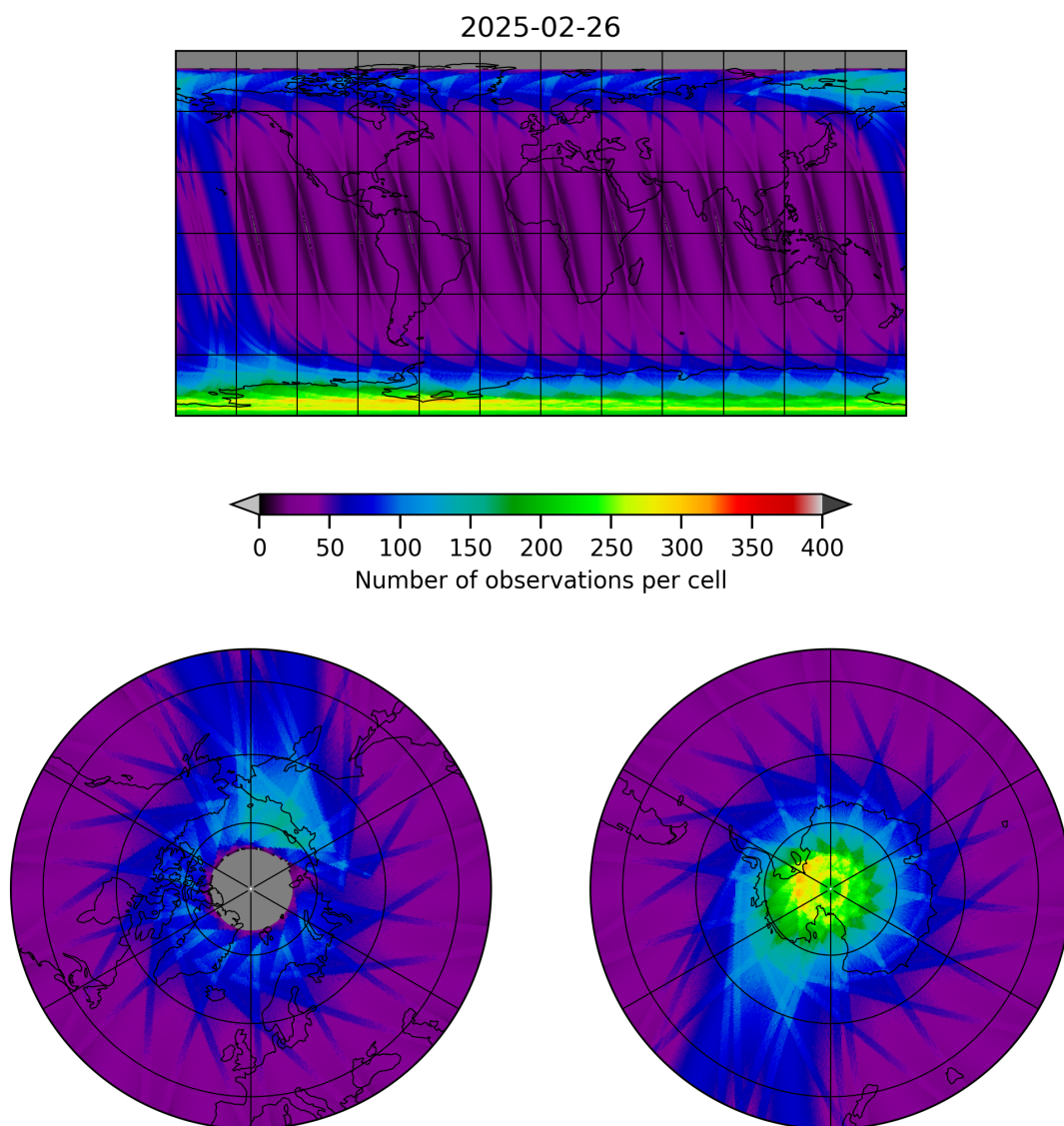
Figure 12: Map of the number of observations for 2025-02-25 to 2025-02-27
