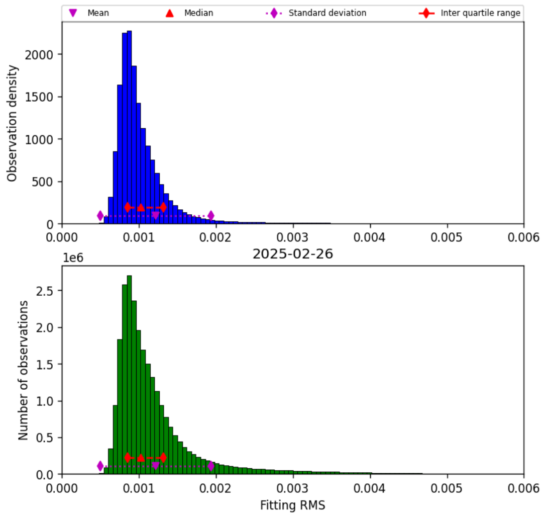
Figure 23: Histogram of “Fitting RMS” for 2025-02-25 to 2025-02-27
