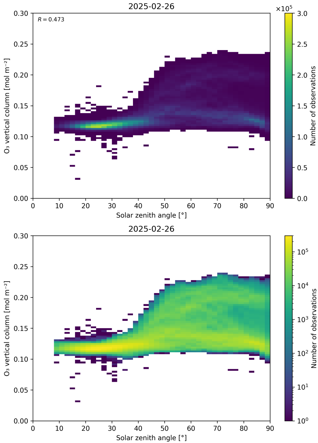
Figure 47: Scatter density plot of “Solar zenith angle” against “O 3 vertical column” for 2025-02-25 to 2025-02-27.
