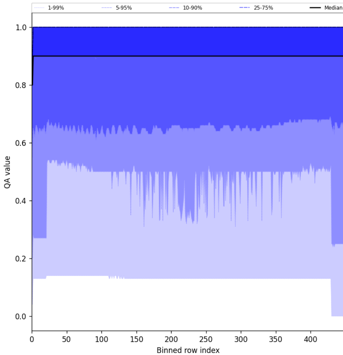
Figure 27: Along track statistics of “QA value” for 2025-02-25 to 2025-02-27
