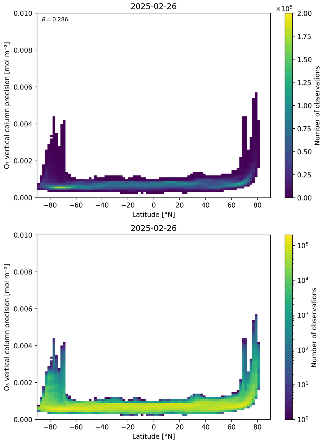
Figure 37: Scatter density plot of “Latitude” against “O 3 vertical column precision” for 2025-02-25 to 2025-02-27.
