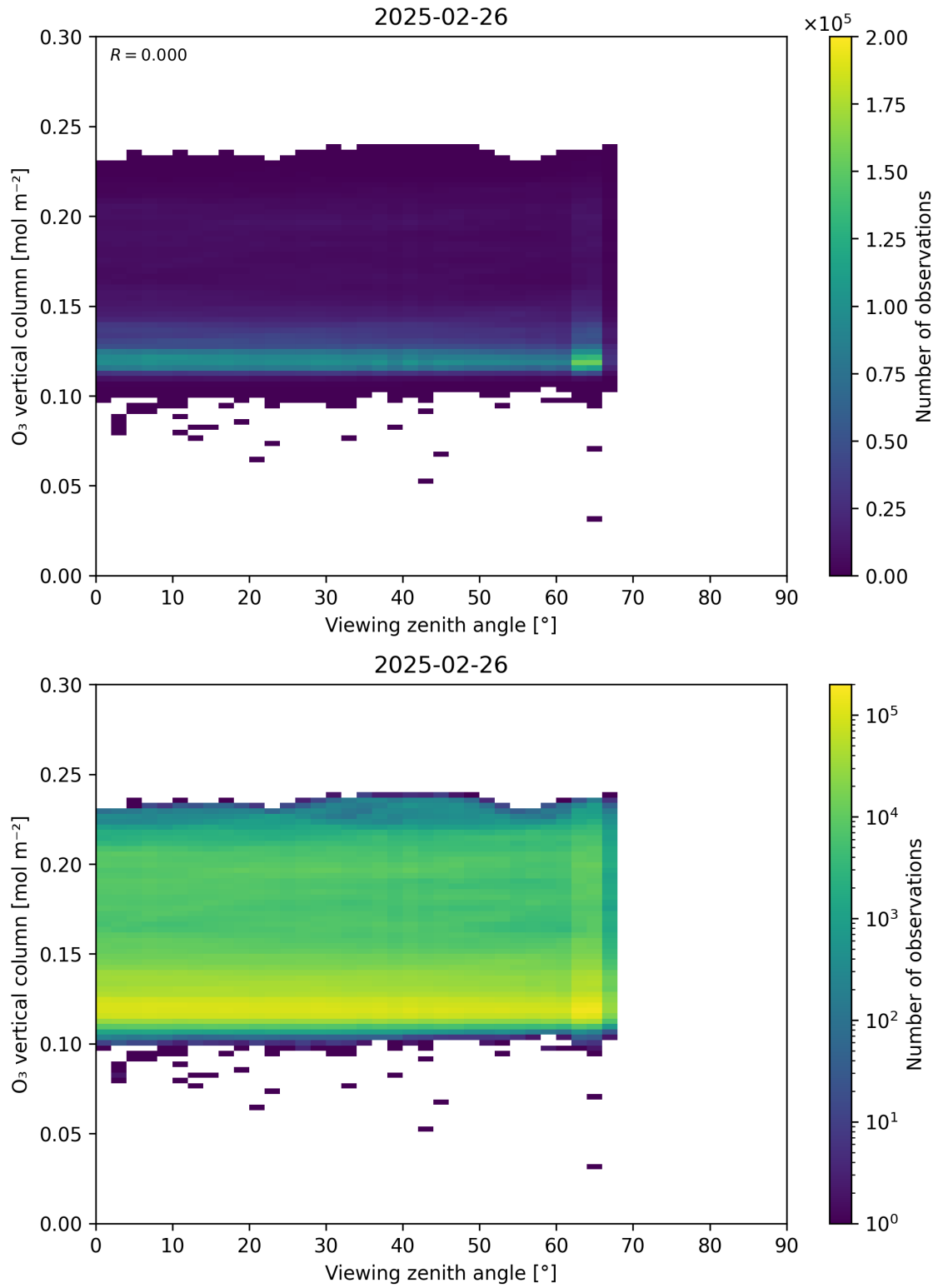
Figure 52: Scatter density plot of “Viewing zenith angle” against “O 3 vertical column” for 2025-02-25 to 2025-02-27.
