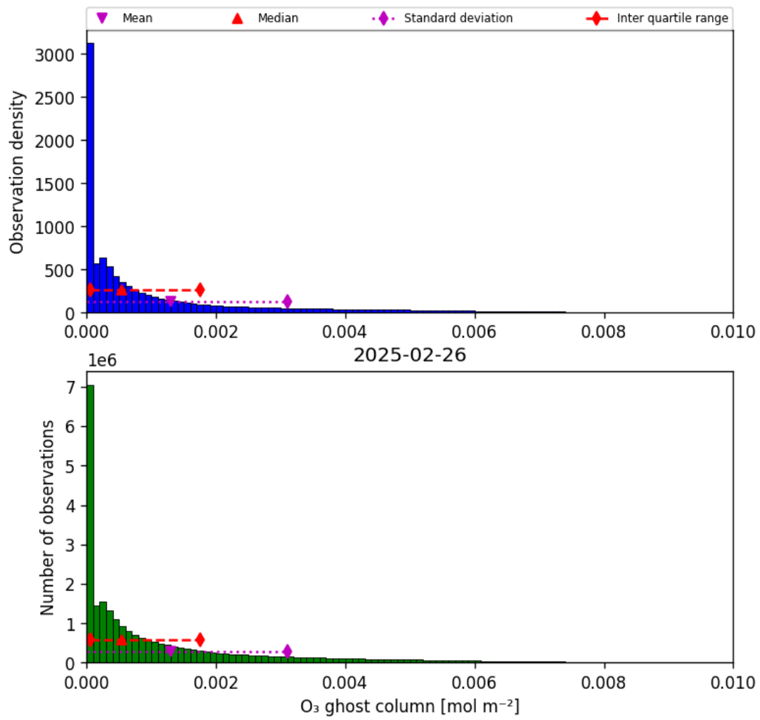
Figure 25: Histogram of “O 3 ghost column” for 2025-02-25 to 2025-02-27
