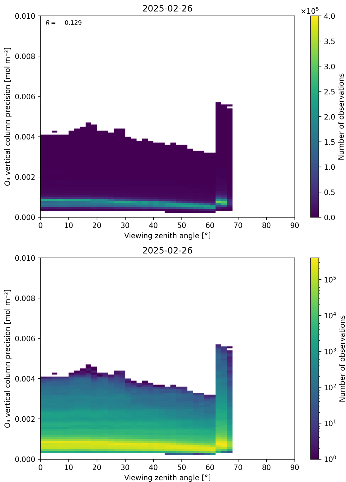
Figure 53: Scatter density plot of “Viewing zenith angle” against “O 3 vertical column precision” for 2025-02-25 to 2025-02-27.
