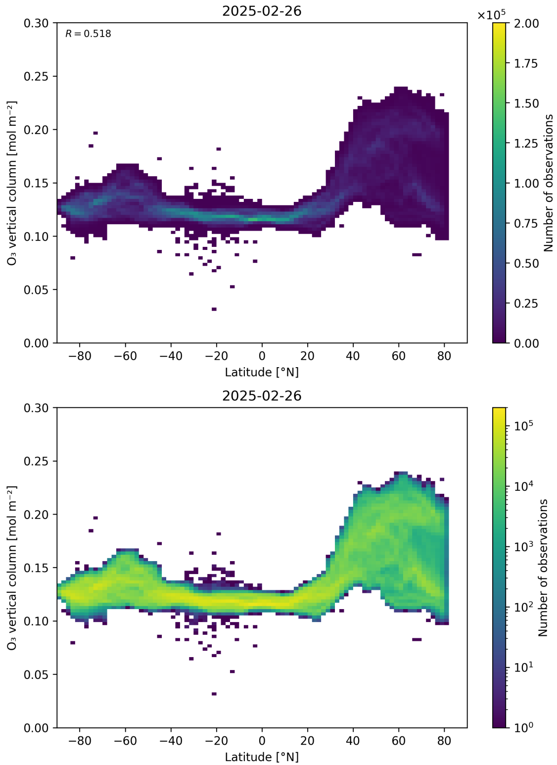
Figure 36: Scatter density plot of “Latitude” against “O 3 vertical column” for 2025-02-25 to 2025-02-27.
