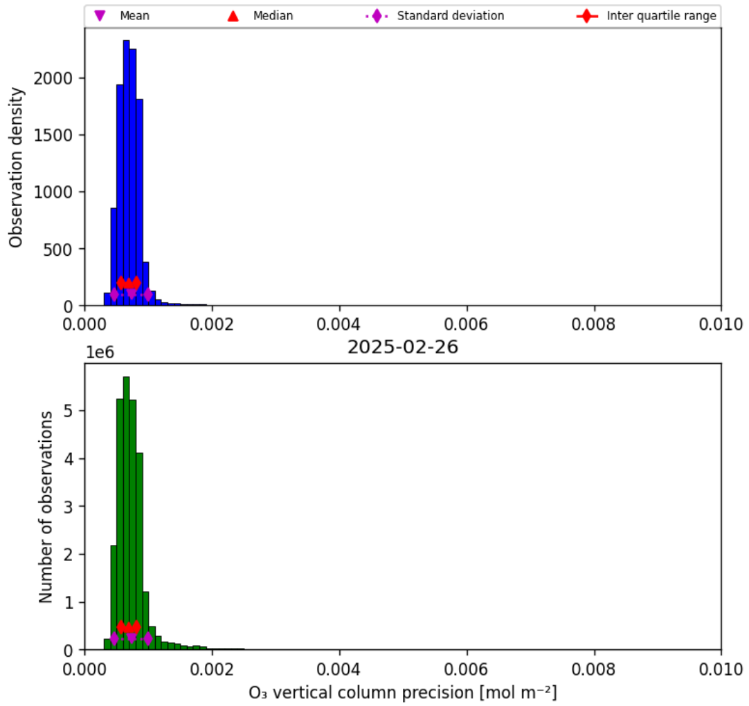
Figure 22: Histogram of “O 3 vertical column precision” for 2025-02-25 to 2025-02-27
