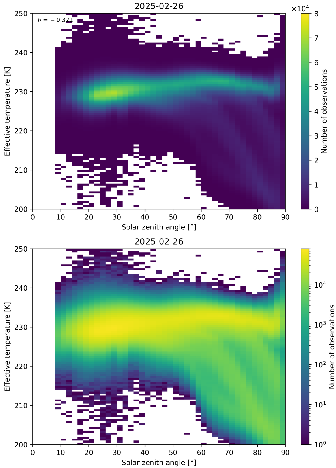
Figure 45: Scatter density plot of “Solar zenith angle” against “Effective temperature” for 2025-02-25 to 2025-02-27.
