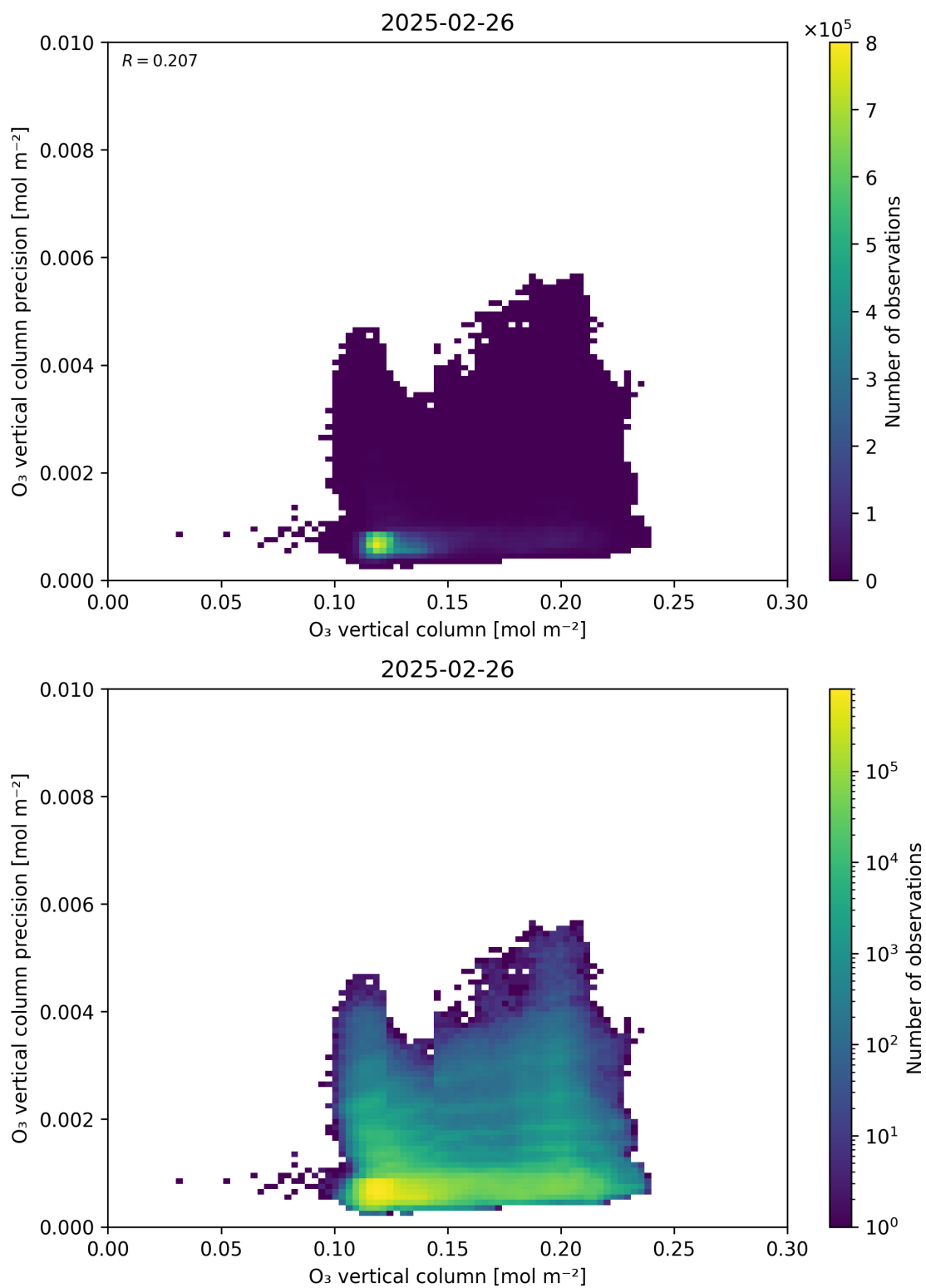
Figure 41: Scatter density plot of “O 3 vertical column” against “O 3 vertical column precision” for 2025-02-25 to 2025-02-27.
