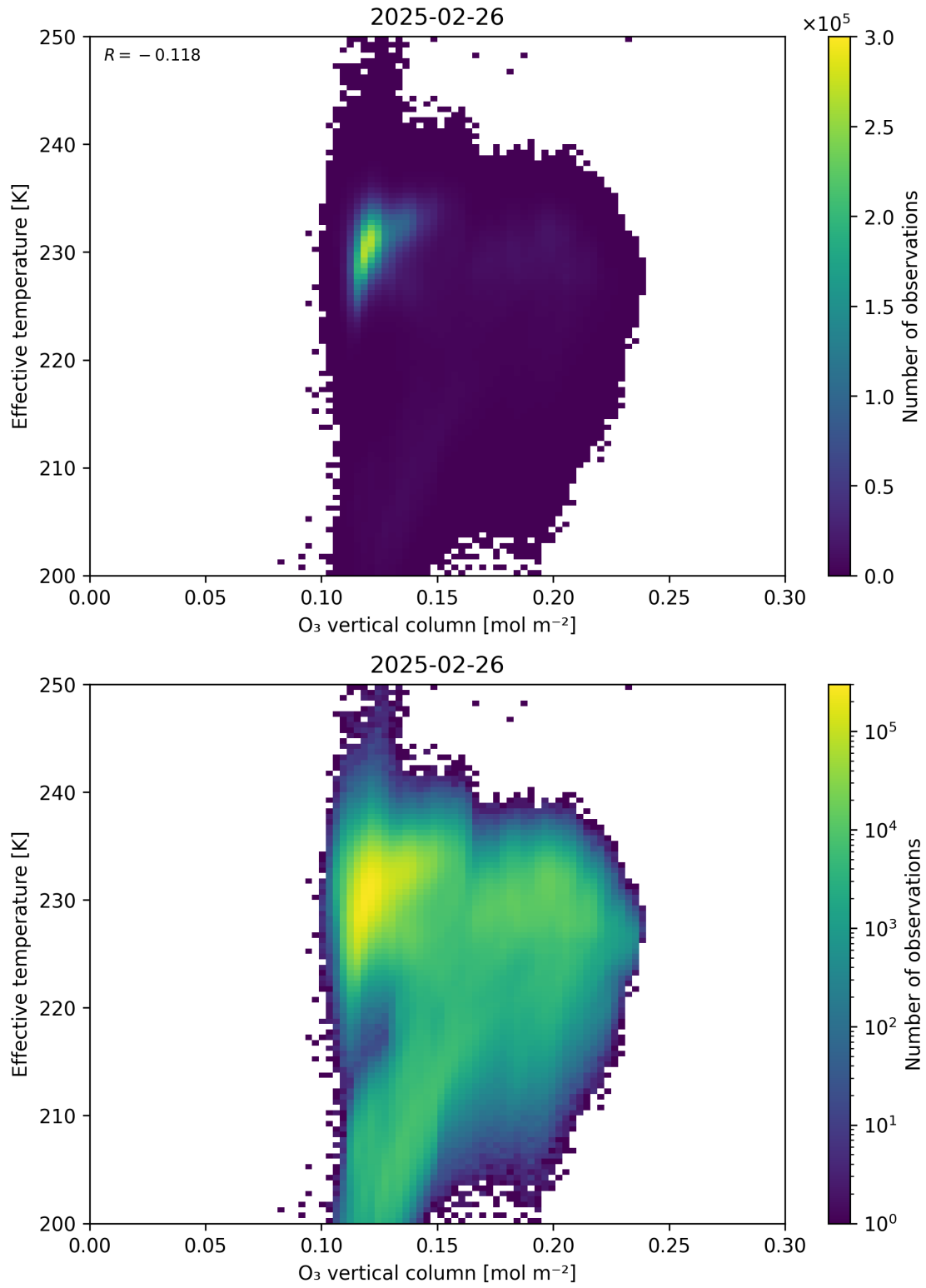
Figure 39: Scatter density plot of “O 3 vertical column” against “Effective temperature” for 2025-02-25 to 2025-02-27.
