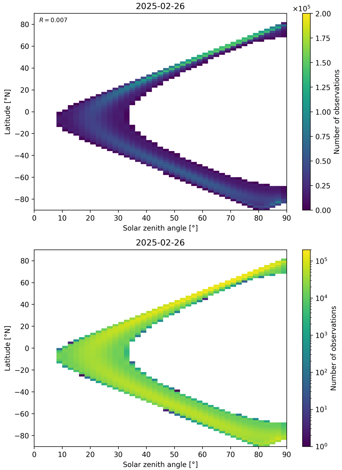
Figure 44: Scatter density plot of “Solar zenith angle” against “Latitude” for 2025-02-25 to 2025-02-27.
