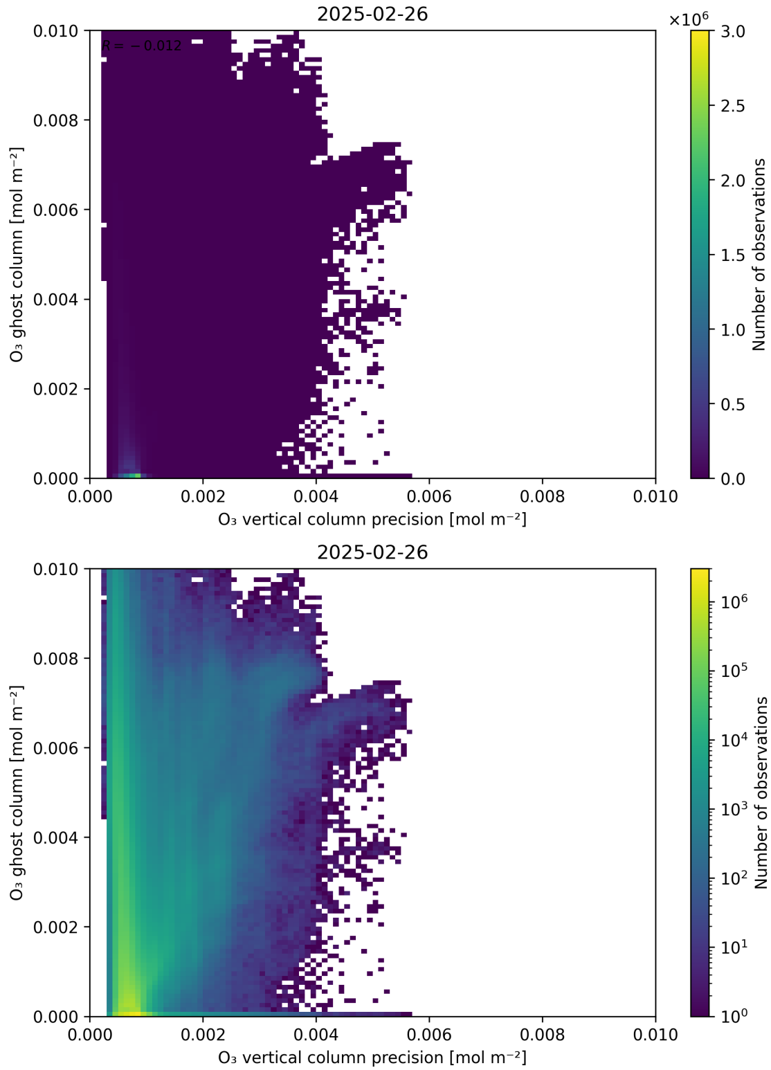
Figure 43: Scatter density plot of “ O_3 vertical column precision” against “ O_3 ghost column” for 2025-02-25 to 2025-02-27.
