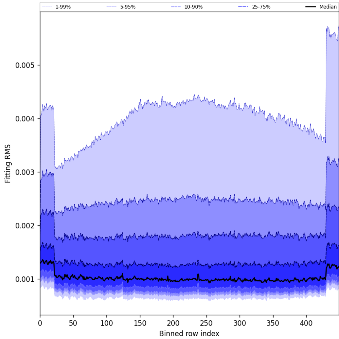
Figure 30: Along track statistics of “Fitting RMS” for 2025-02-25 to 2025-02-27
