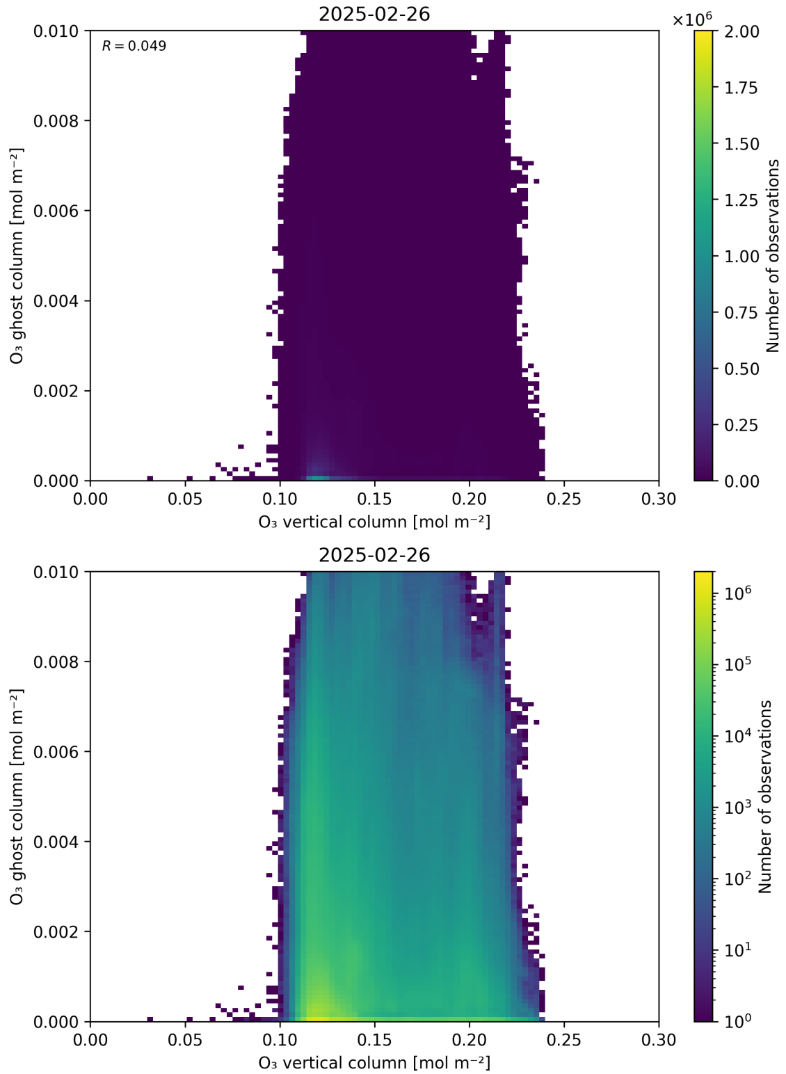
Figure 40: Scatter density plot of “O 3 vertical column” against “O 3 ghost column” for 2025-02-25 to 2025-02-27.
