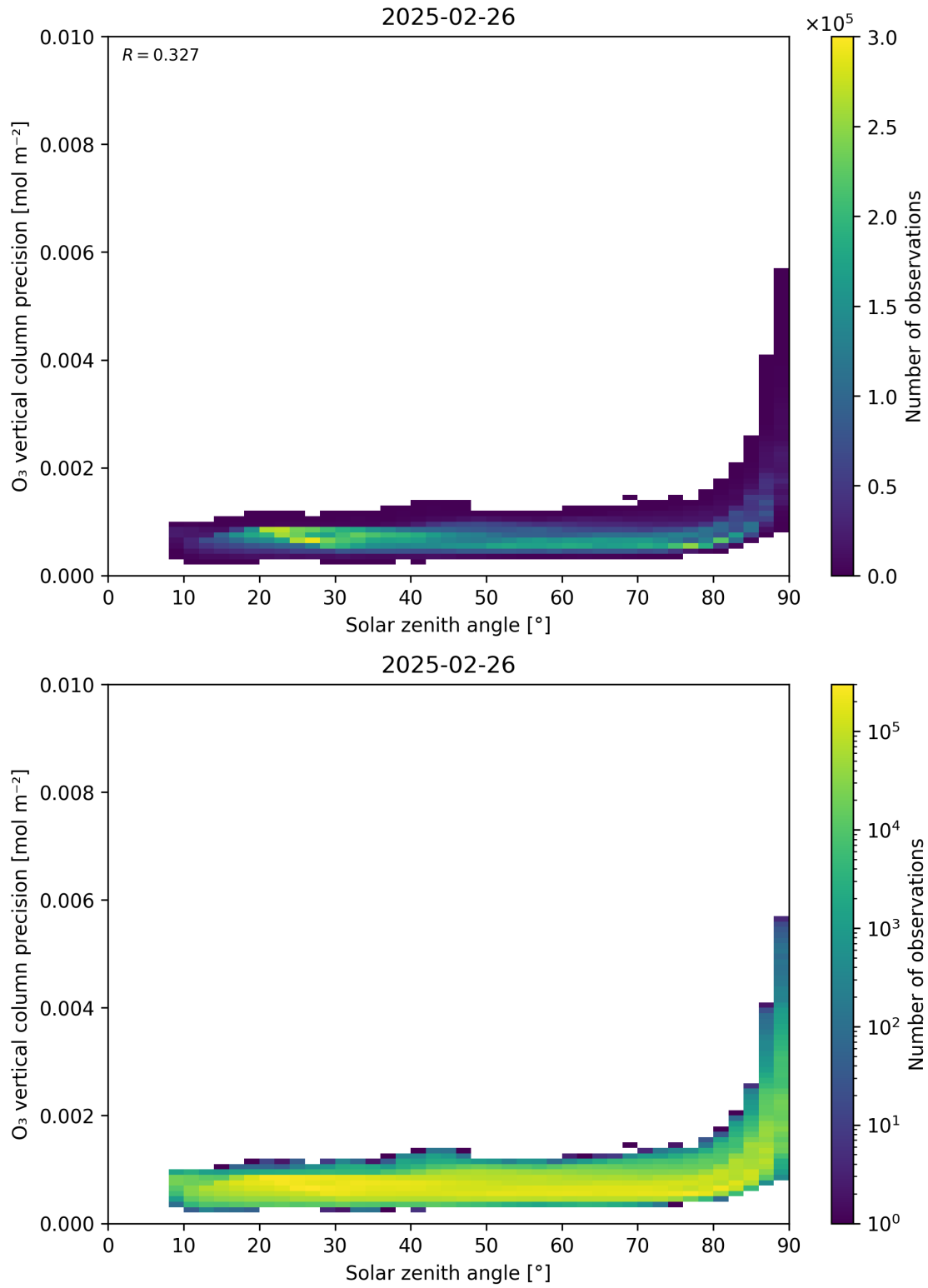
Figure 48: Scatter density plot of “Solar zenith angle” against “O 3 vertical column precision” for 2025-02-25 to 2025-02-27.
