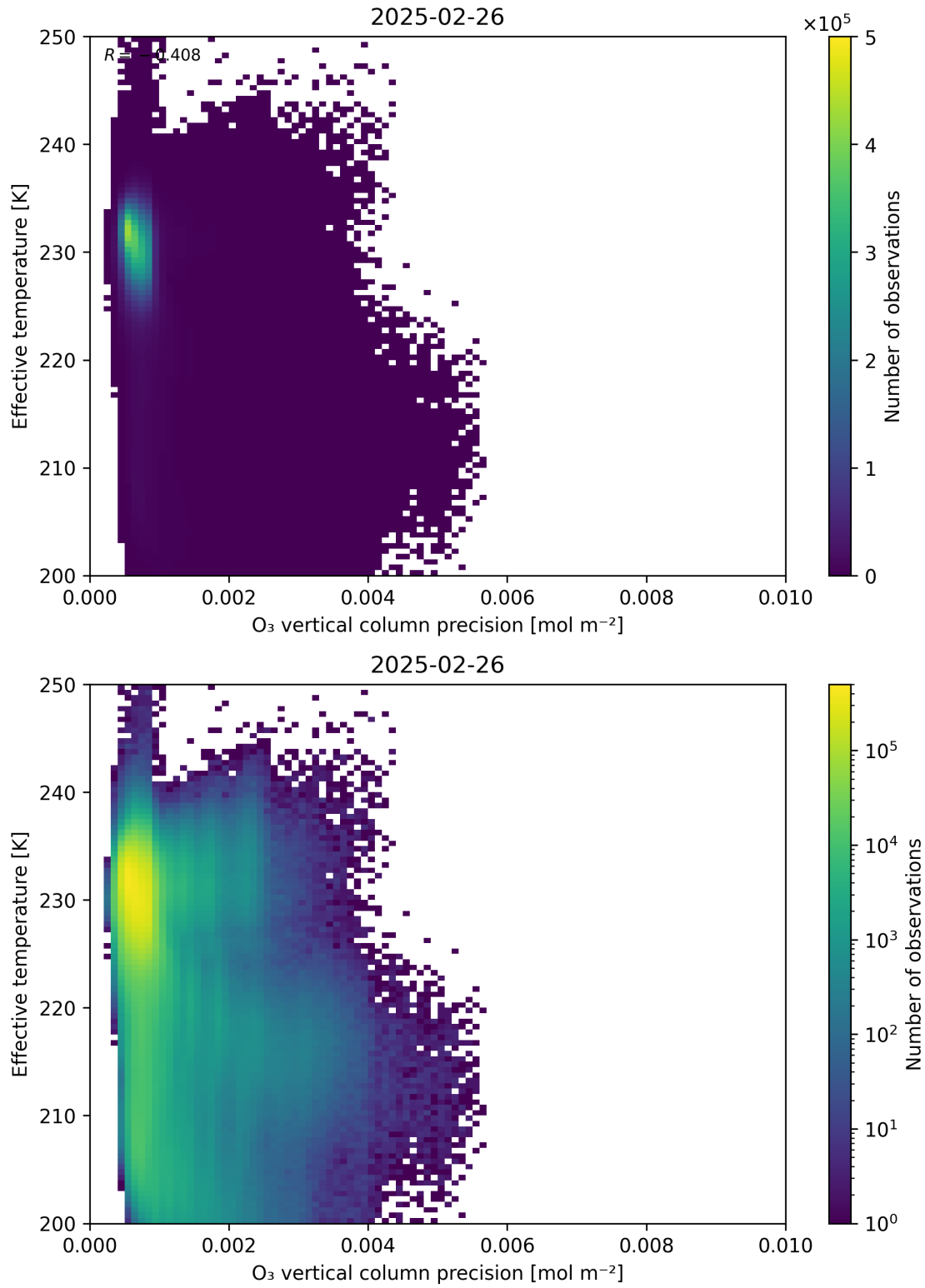
Figure 42: Scatter density plot of “O 3 vertical column precision” against “Effective temperature” for 2025-02-25 to 2025-02-27.
