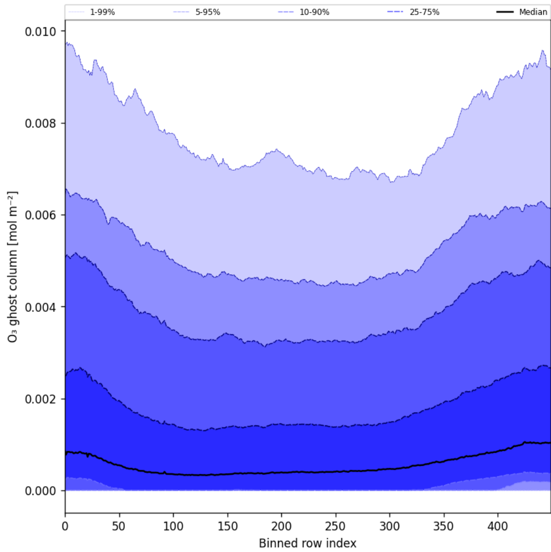
Figure 32: Along track statistics of “O 3 ghost column” for 2025-02-25 to 2025-02-27
