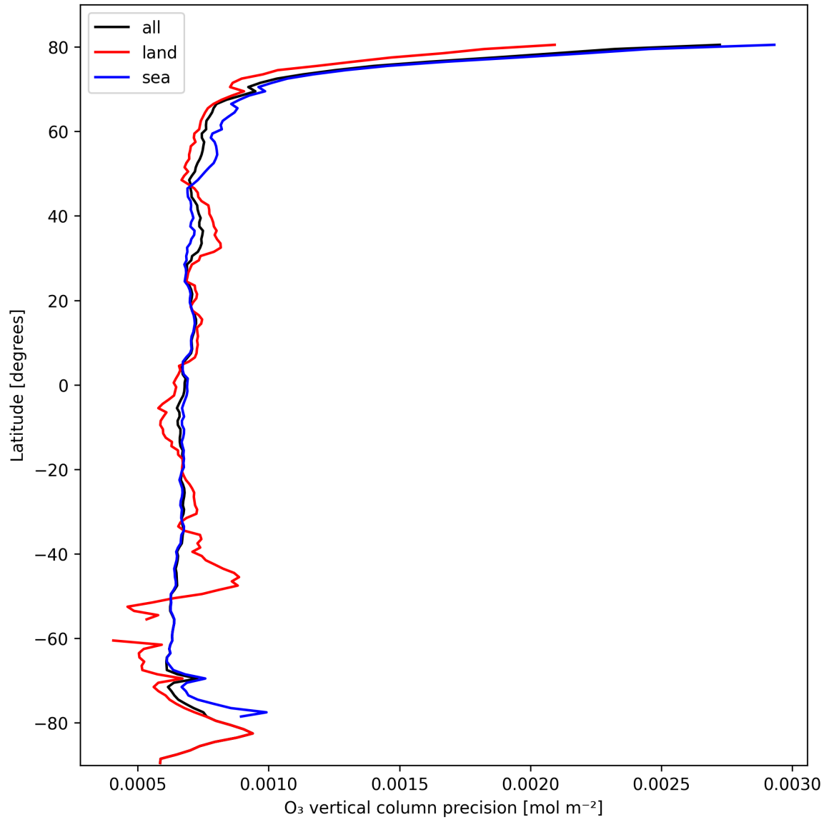
Figure 15: Zonal average of “O 3 vertical column precision” for 2025-02-25 to 2025-02-27.
