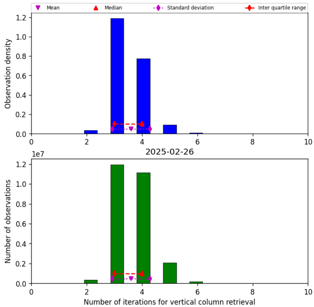
Figure 26: Histogram of “Number of iterations for vertical column retrieval” for 2025-02-25 to 2025-02-27
