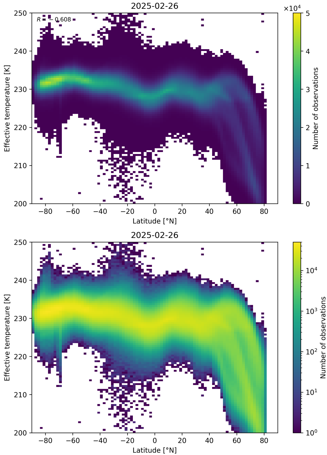
Figure 34: Scatter density plot of “Latitude” against “Effective temperature” for 2025-02-25 to 2025-02-27.
