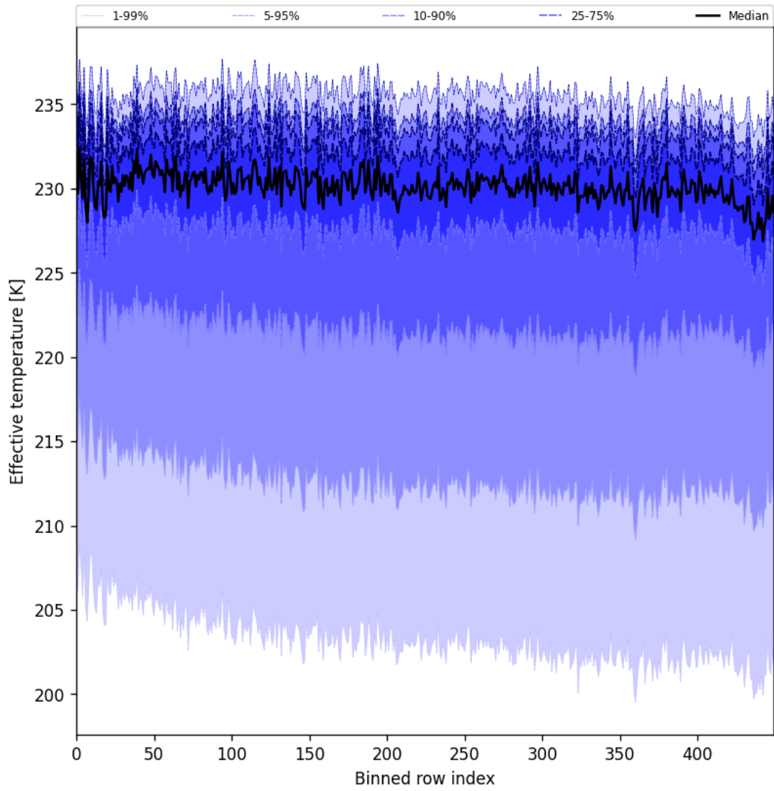
Figure 31: Along track statistics of “Effective temperature” for 2025-02-25 to 2025-02-27
