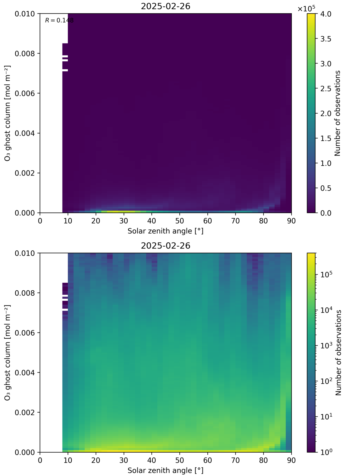
Figure 46: Scatter density plot of “Solar zenith angle” against “O 3 ghost column” for 2025-02-25 to 2025-02-27.
