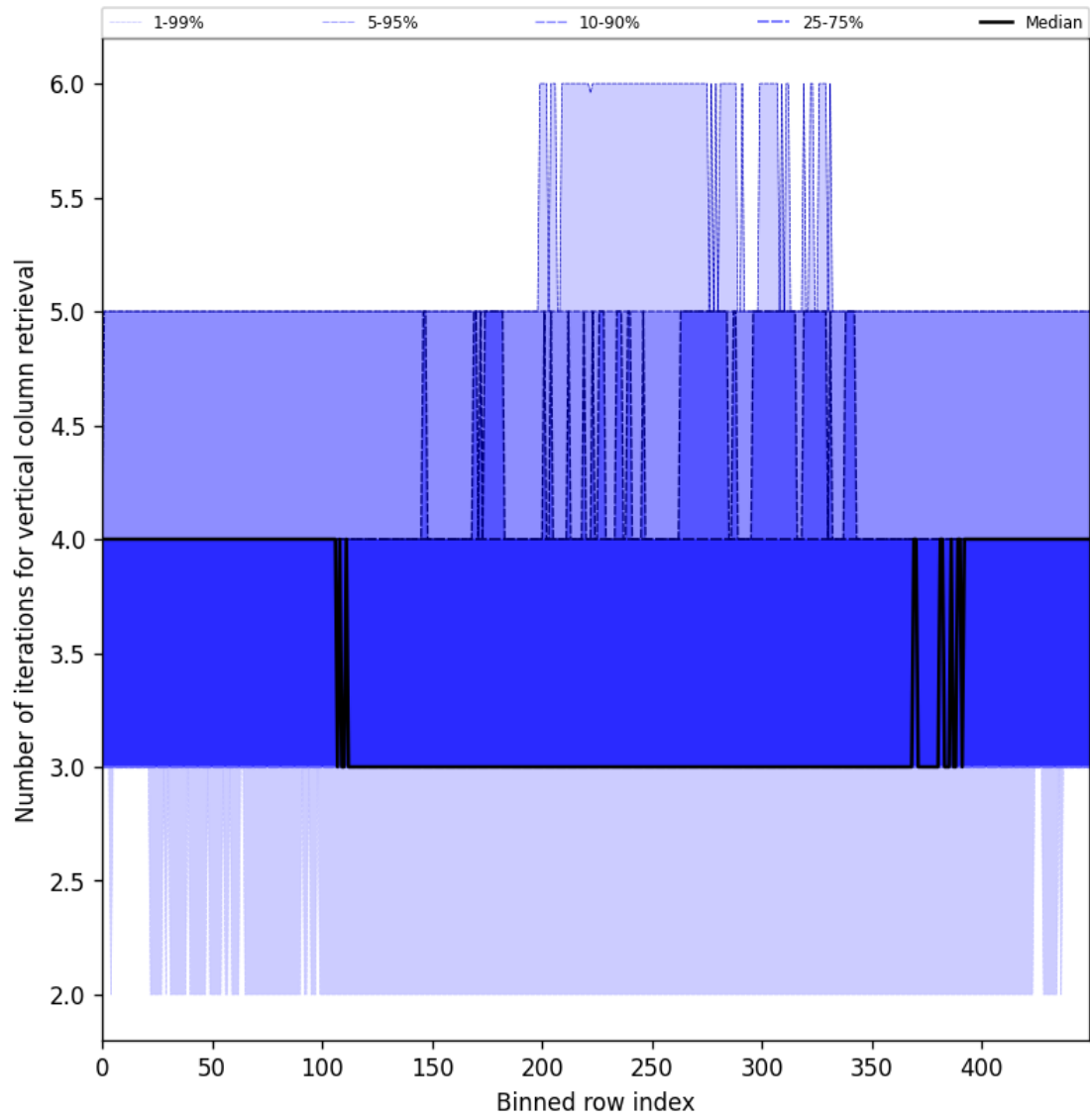
Figure 33: Along track statistics of “Number of iterations for vertical column retrieval” for 2025-02-25 to 2025-02-27
