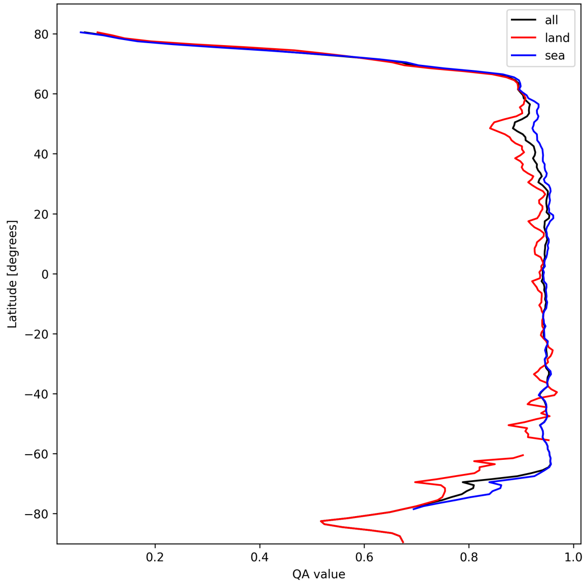
Figure 13: Zonal average of “QA value” for 2025-02-25 to 2025-02-27.
