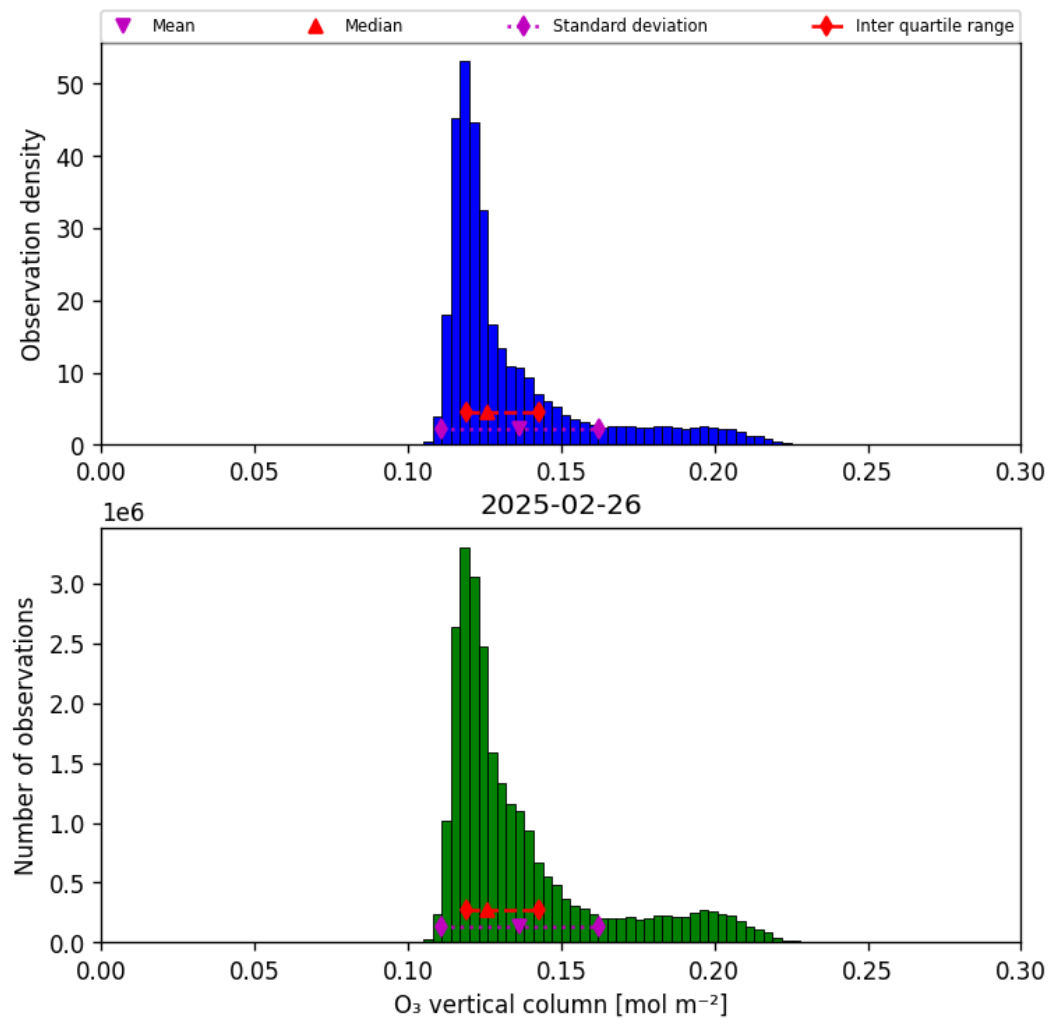
Figure 21: Histogram of “O 3 vertical column” for 2025-02-25 to 2025-02-27
