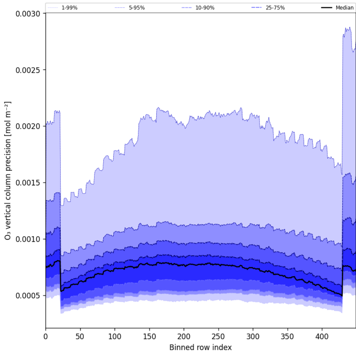
Figure 29: Along track statistics of “O 3 vertical column precision” for 2025-02-25 to 2025-02-27
