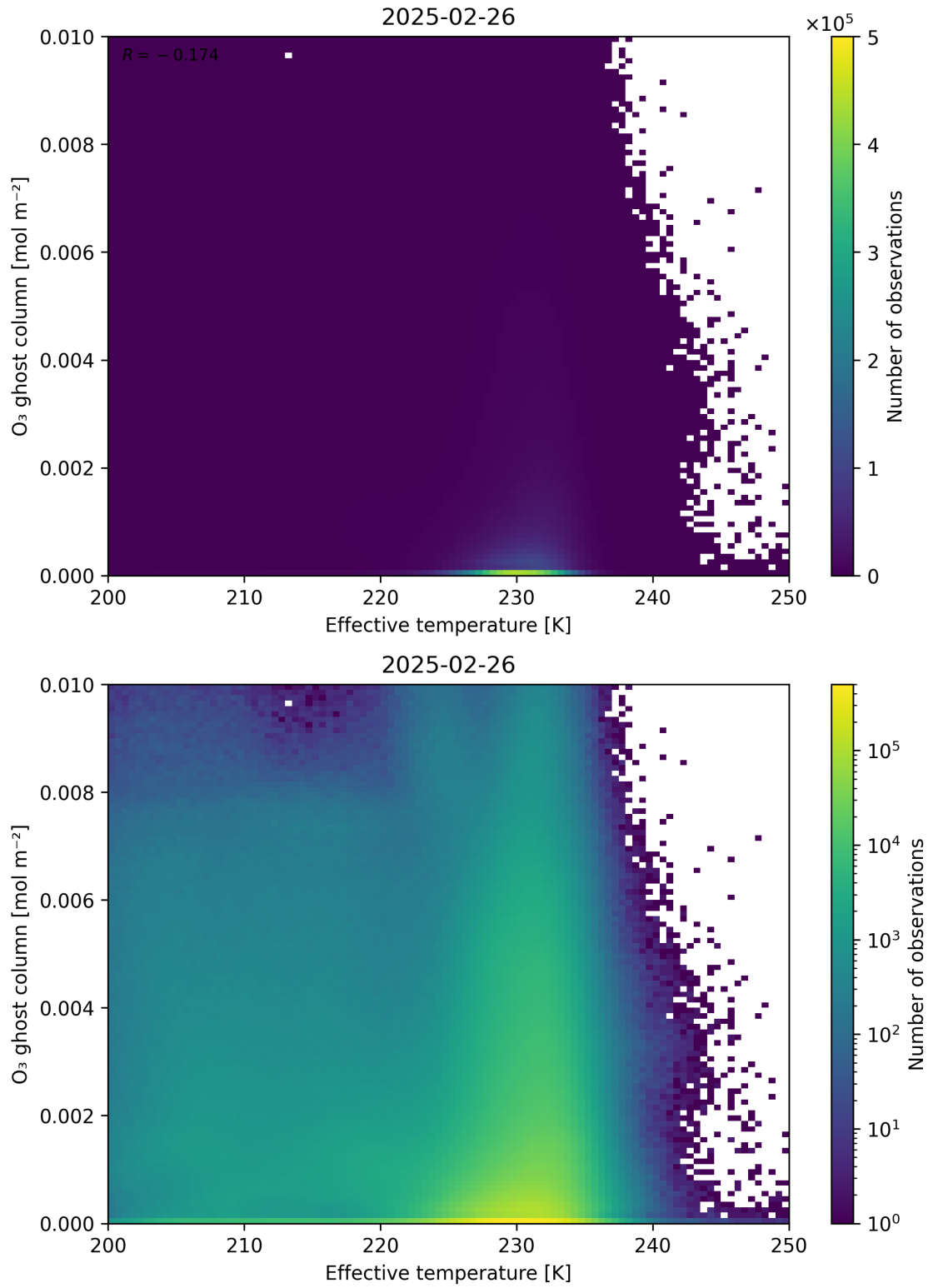
Figure 38: Scatter density plot of “Effective temperature” against “O 3 ghost column” for 2025-02-25 to 2025-02-27.
