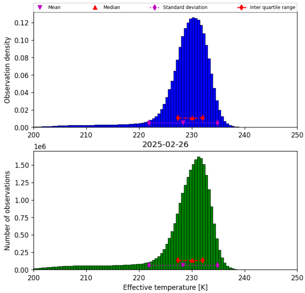
Figure 24: Histogram of “Effective temperature” for 2025-02-25 to 2025-02-27
