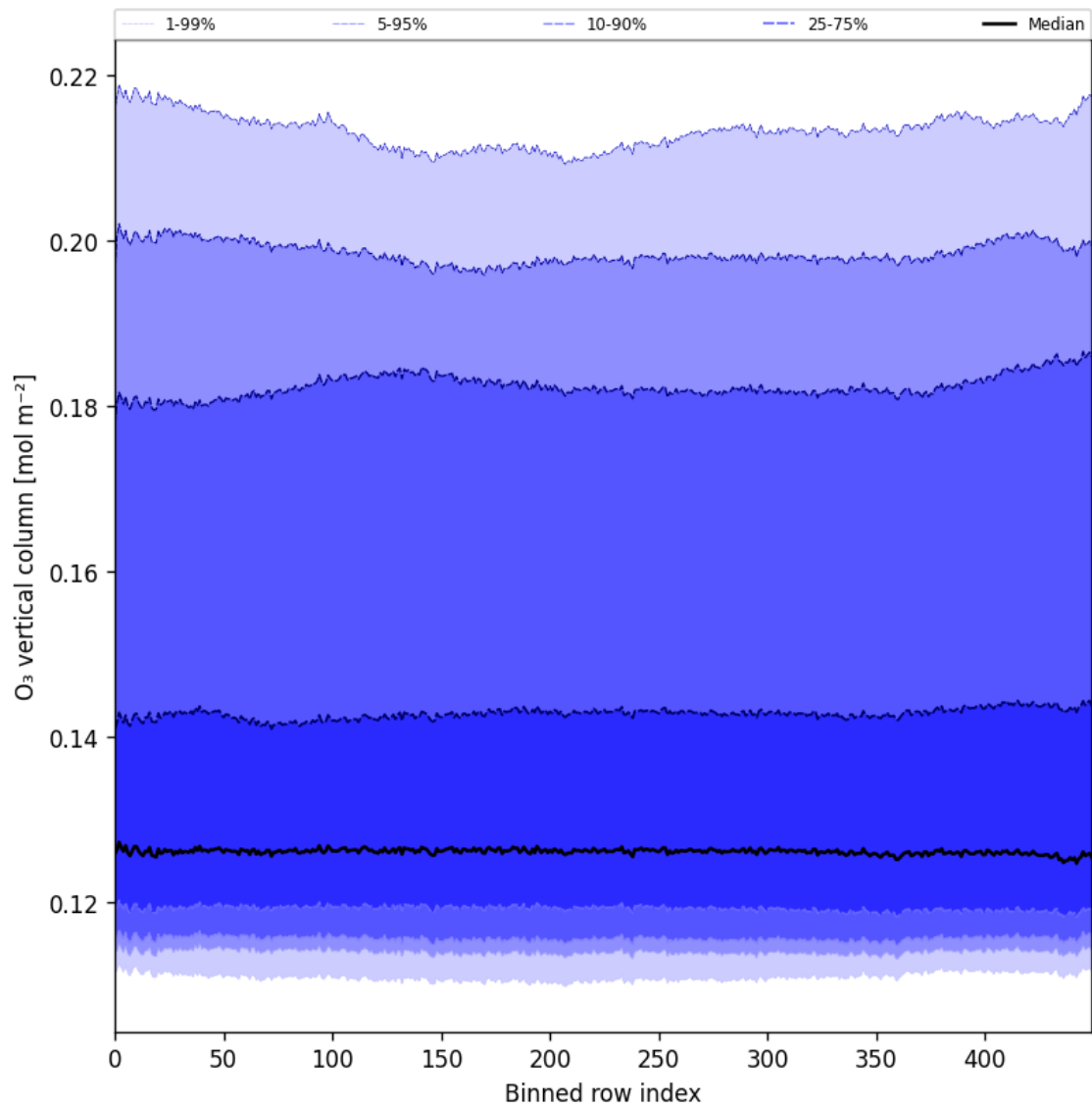
Figure 28: Along track statistics of “O 3 vertical column” for 2025-02-25 to 2025-02-27
