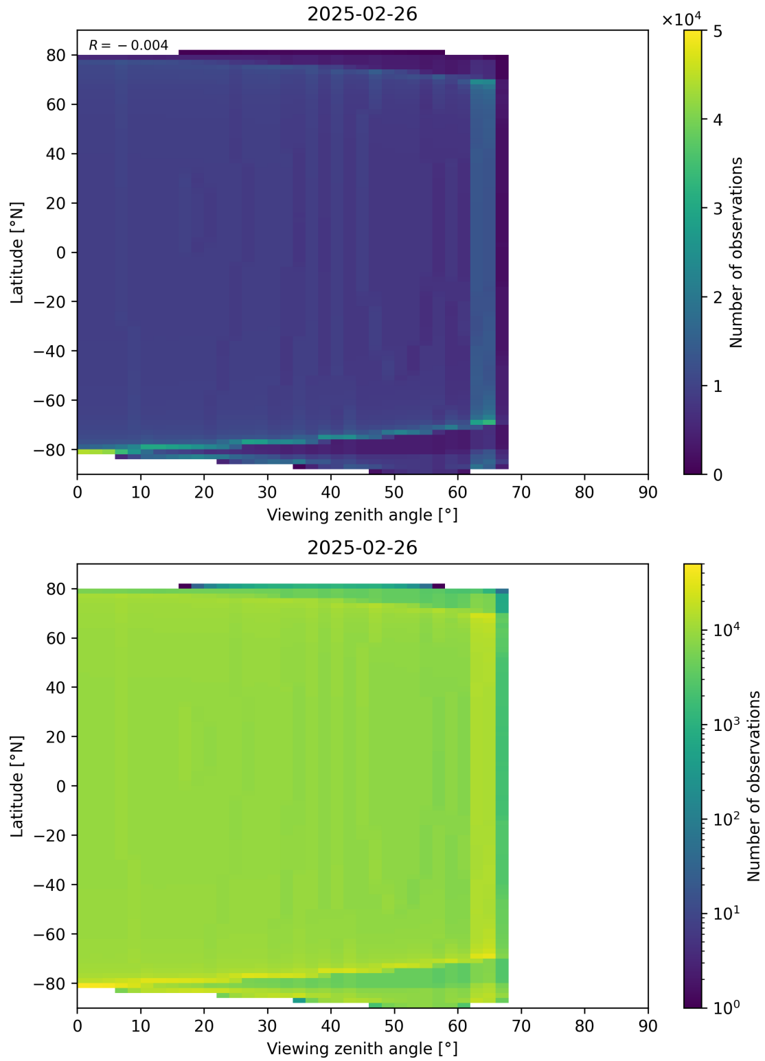
Figure 49: Scatter density plot of “Viewing zenith angle” against “Latitude” for 2025-02-25 to 2025-02-27.
