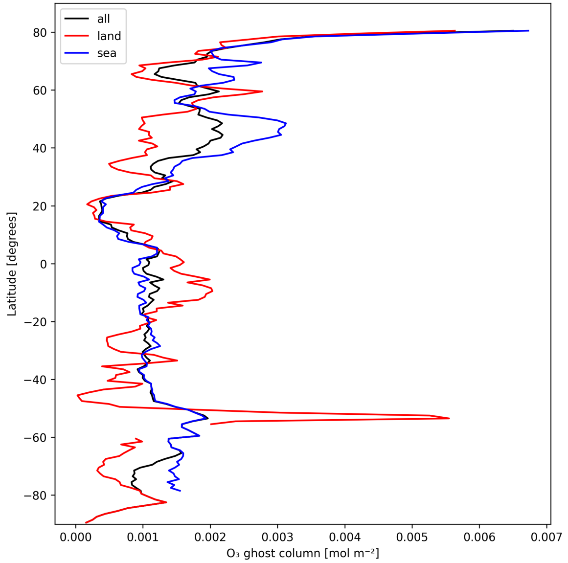
Figure 18: Zonal average of “O 3 ghost column” for 2025-02-25 to 2025-02-27.
