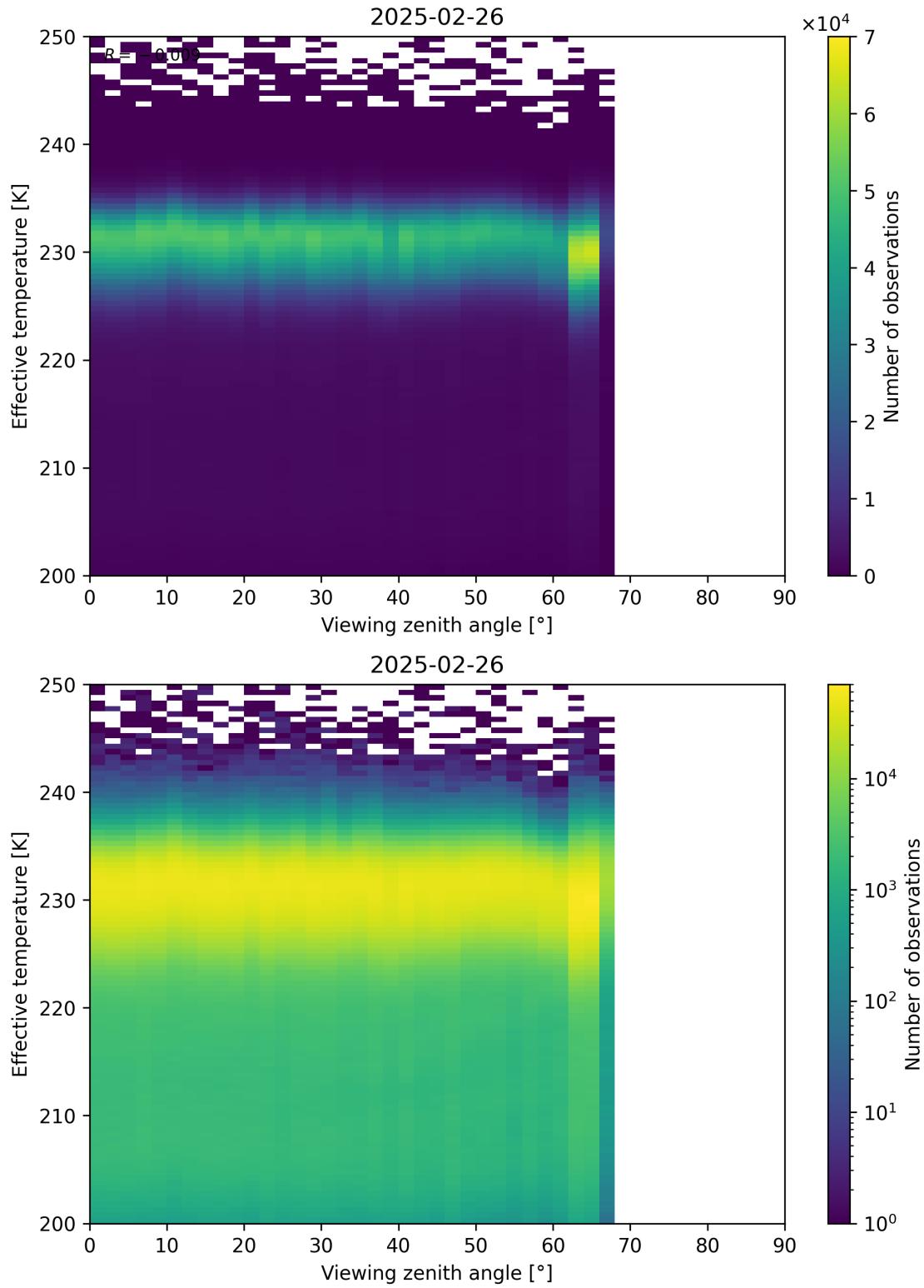
Figure 50: Scatter density plot of “Viewing zenith angle” against “Effective temperature” for 2025-02-25 to 2025-02-27.
