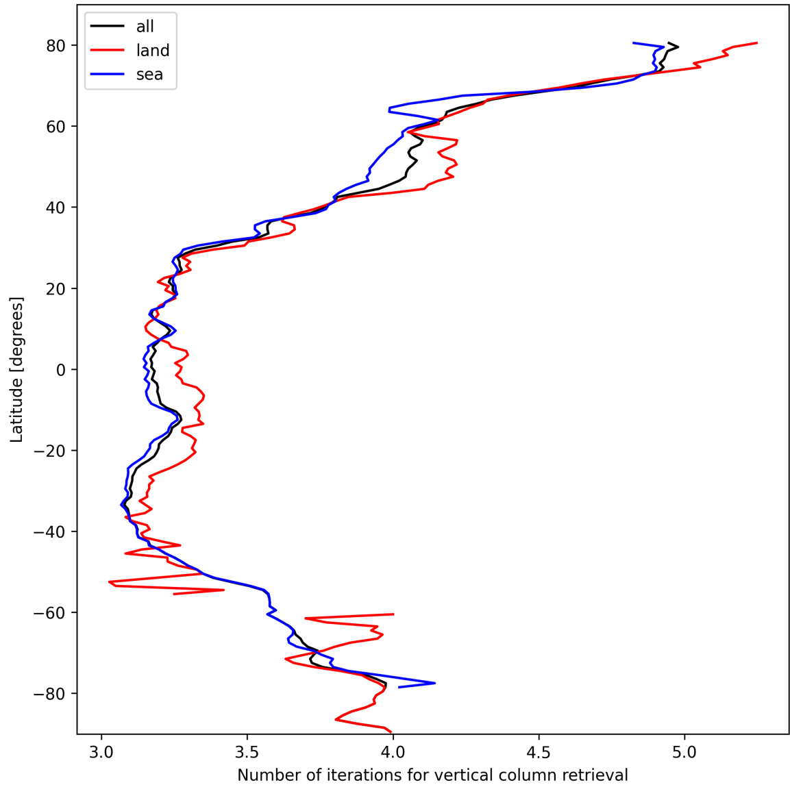
Figure 19: Zonal average of “Number of iterations for vertical column retrieval” for 2025-02-25 to 2025-02-27.
