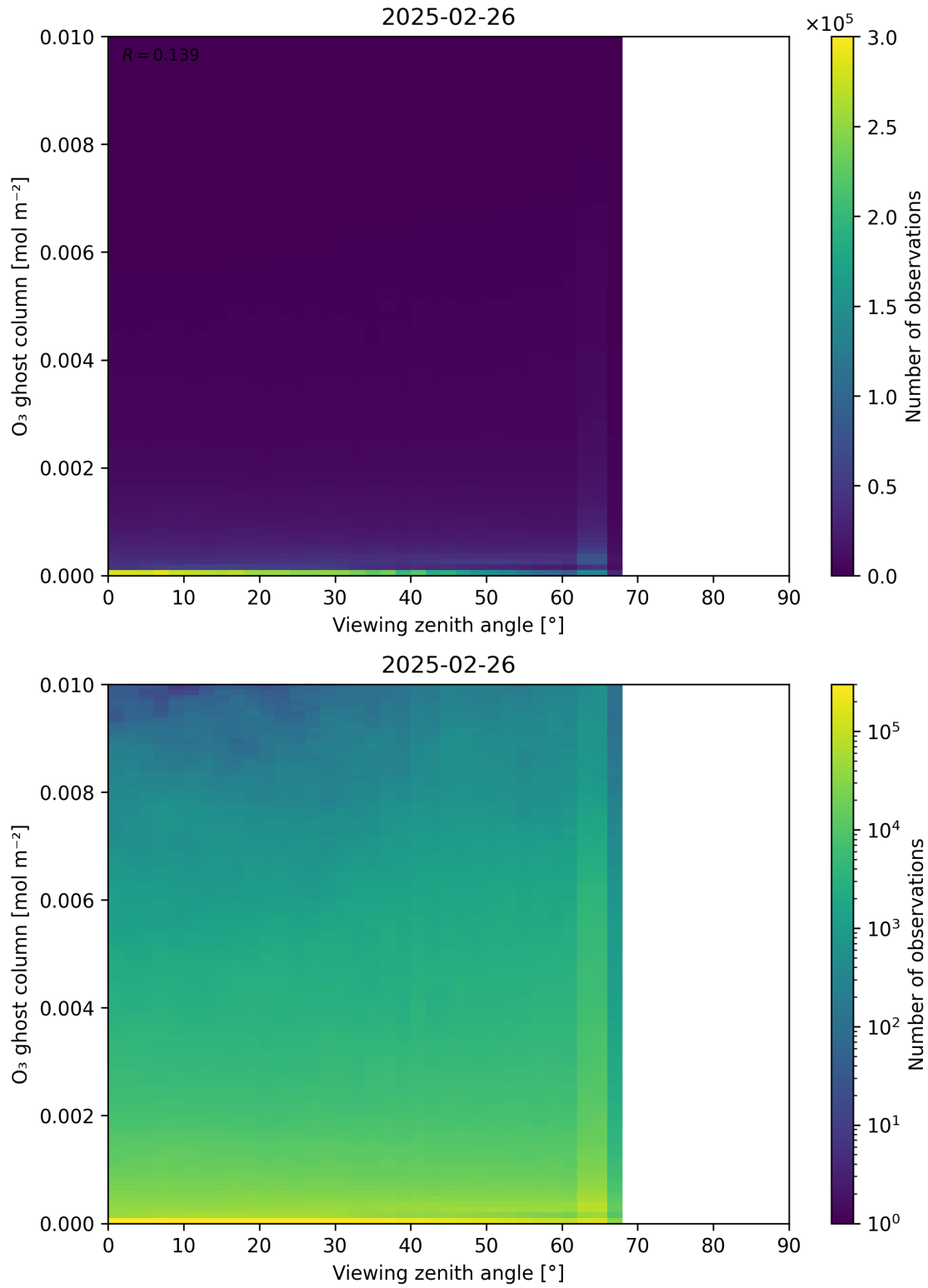
Figure 51: Scatter density plot of “Viewing zenith angle” against “O 3 ghost column” for 2025-02-25 to 2025-02-27.
