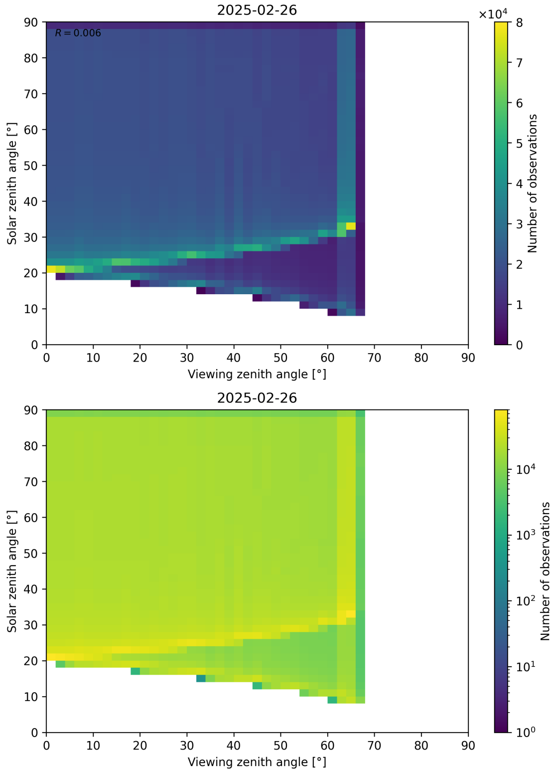
Figure 54: Scatter density plot of “Viewing zenith angle” against “Solar zenith angle” for 2025-02-25 to 2025-02-27.
