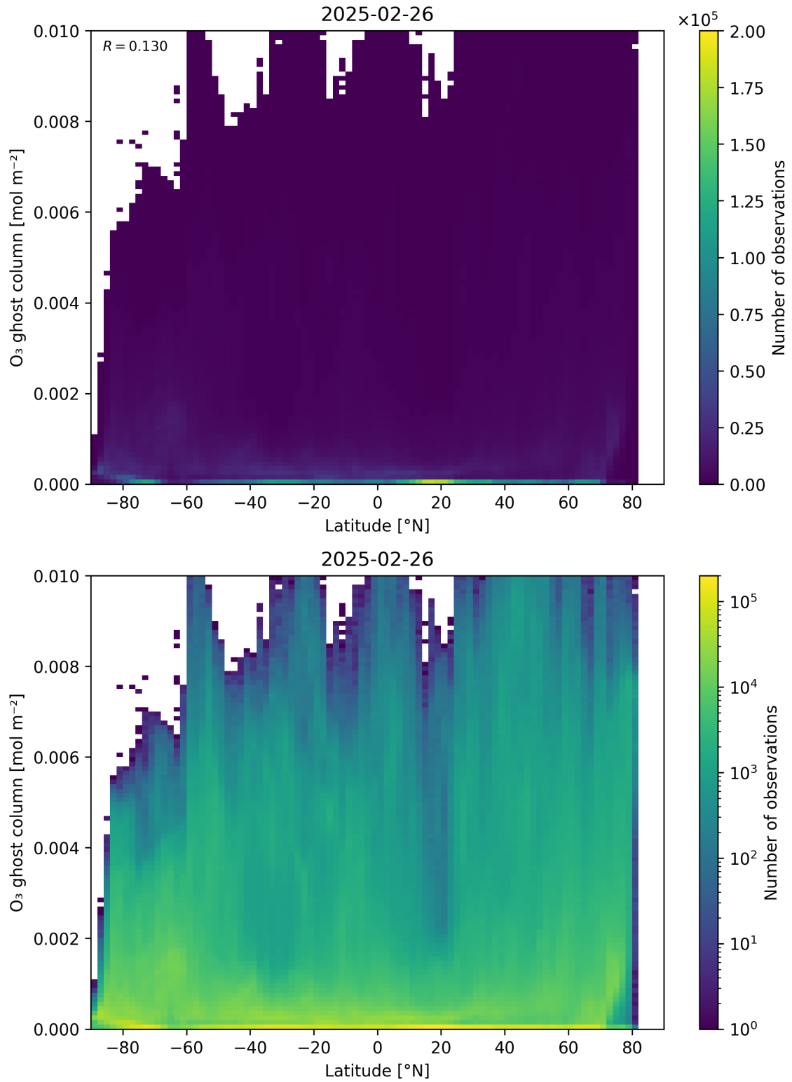
Figure 35: Scatter density plot of “Latitude” against “O 3 ghost column” for 2025-02-25 to 2025-02-27.
