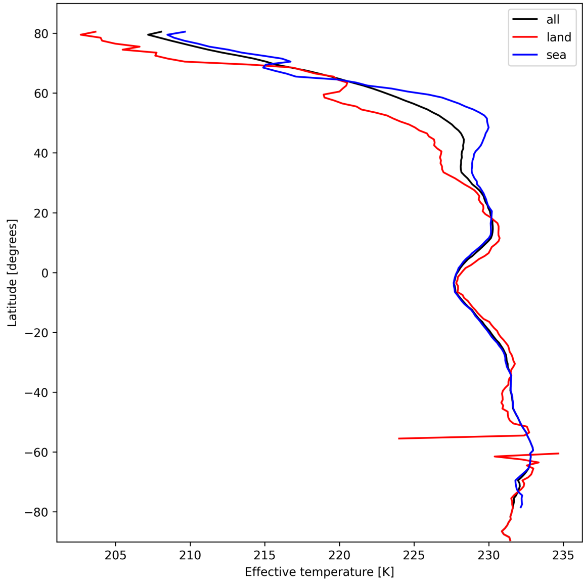
Figure 17: Zonal average of "Effective temperature" for 2025-02-25 to 2025-02-27.
