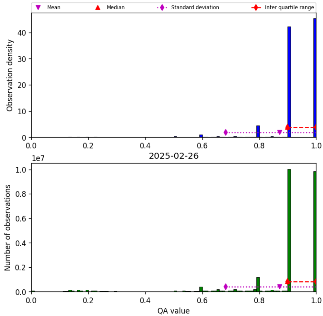
Figure 20: Histogram of “QA value” for 2025-02-25 to 2025-02-27
