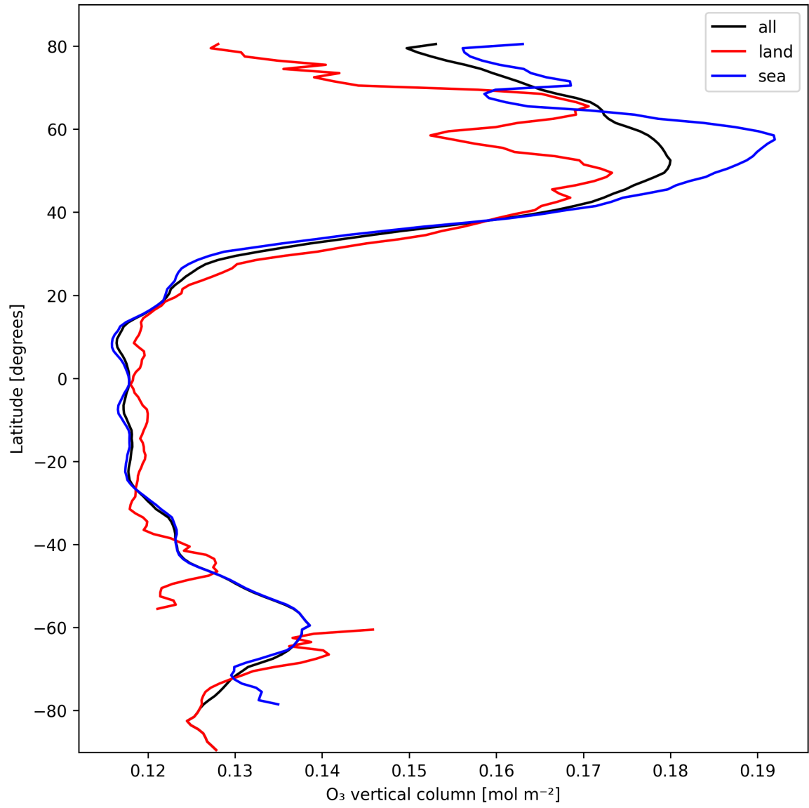
Figure 14: Zonal average of “O 3 vertical column” for 2025-02-25 to 2025-02-27.
