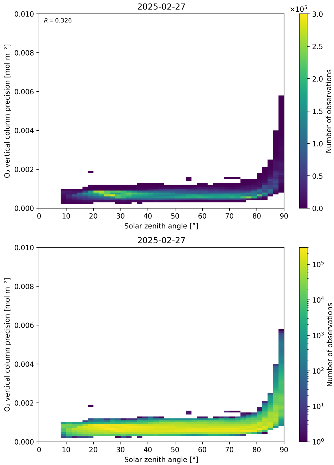
Figure 48: Scatter density plot of “Solar zenith angle” against “O 3 vertical column precision” for 2025-02-26 to 2025-02-28.
