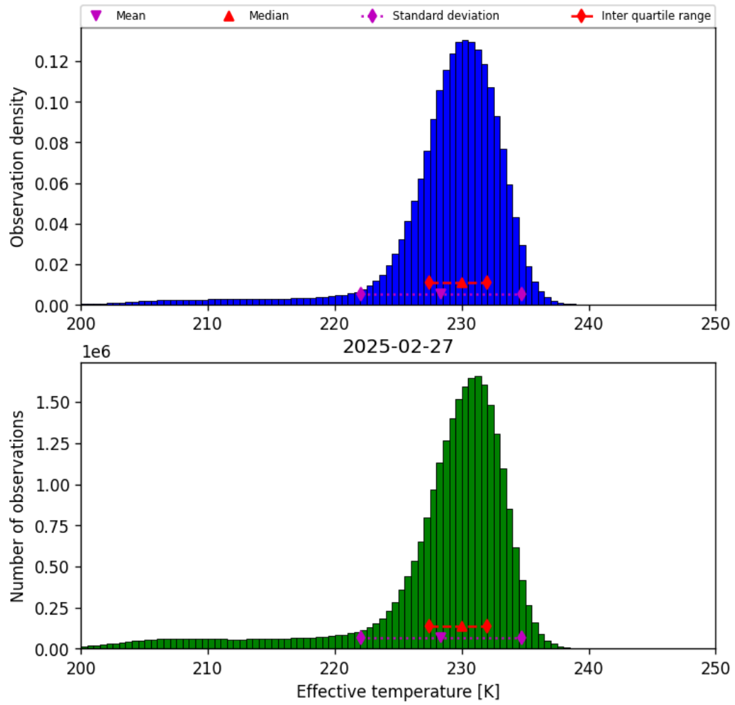
Figure 24: Histogram of “Effective temperature” for 2025-02-26 to 2025-02-28
