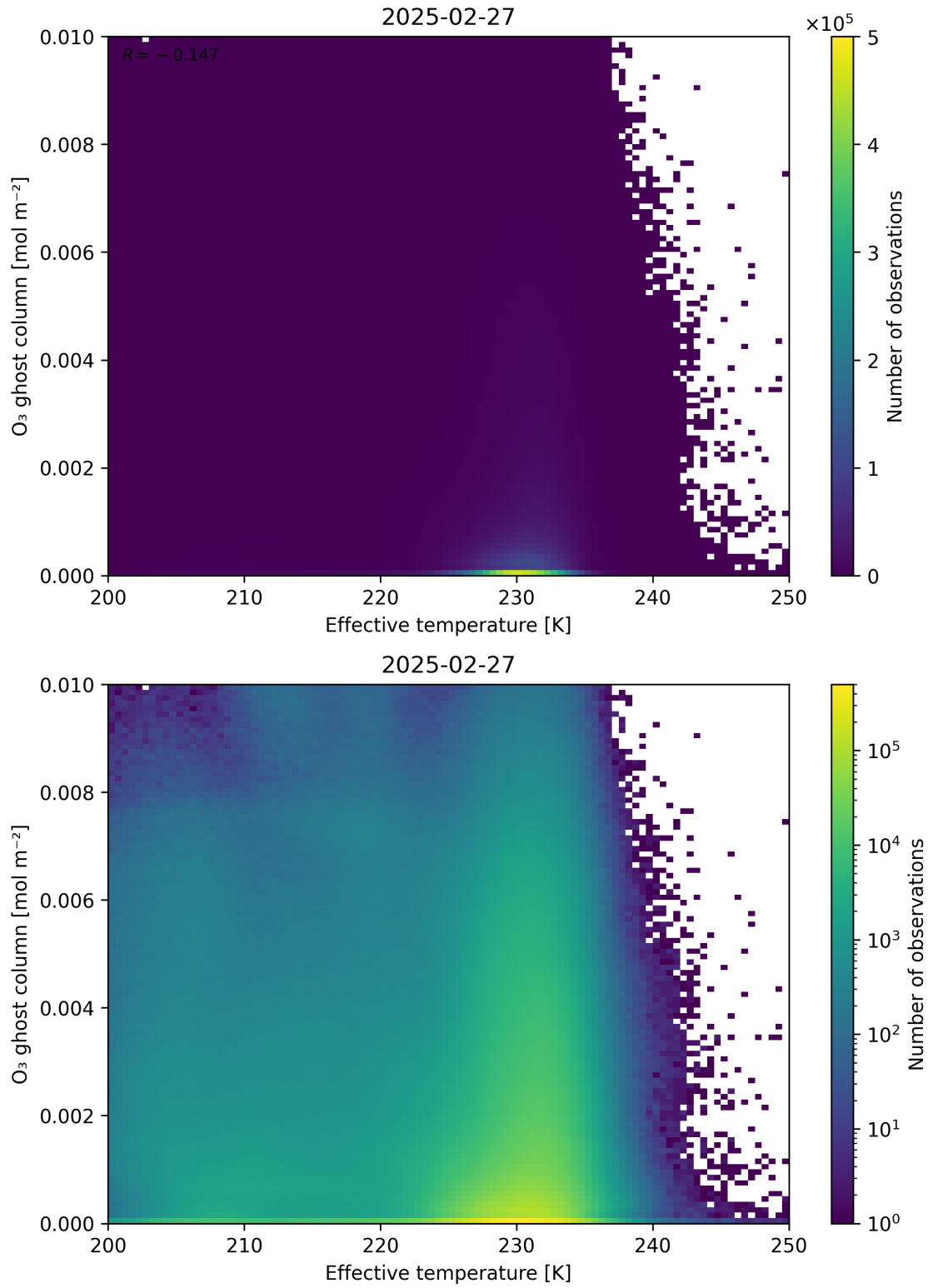
Figure 38: Scatter density plot of “Effective temperature” against “O 3 ghost column” for 2025-02-26 to 2025-02-28.
