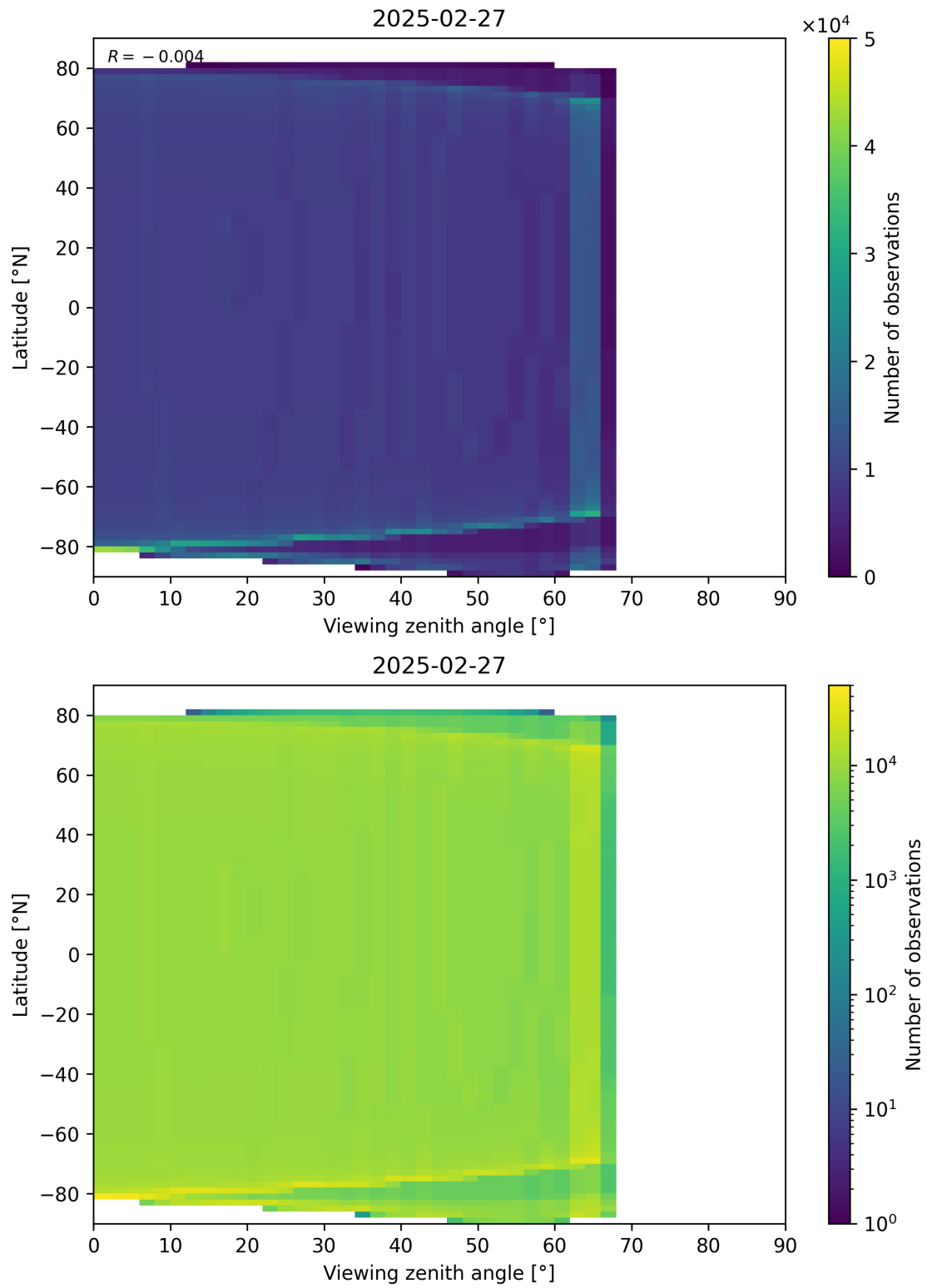
Figure 49: Scatter density plot of “Viewing zenith angle” against “Latitude” for 2025-02-26 to 2025-02-28.
