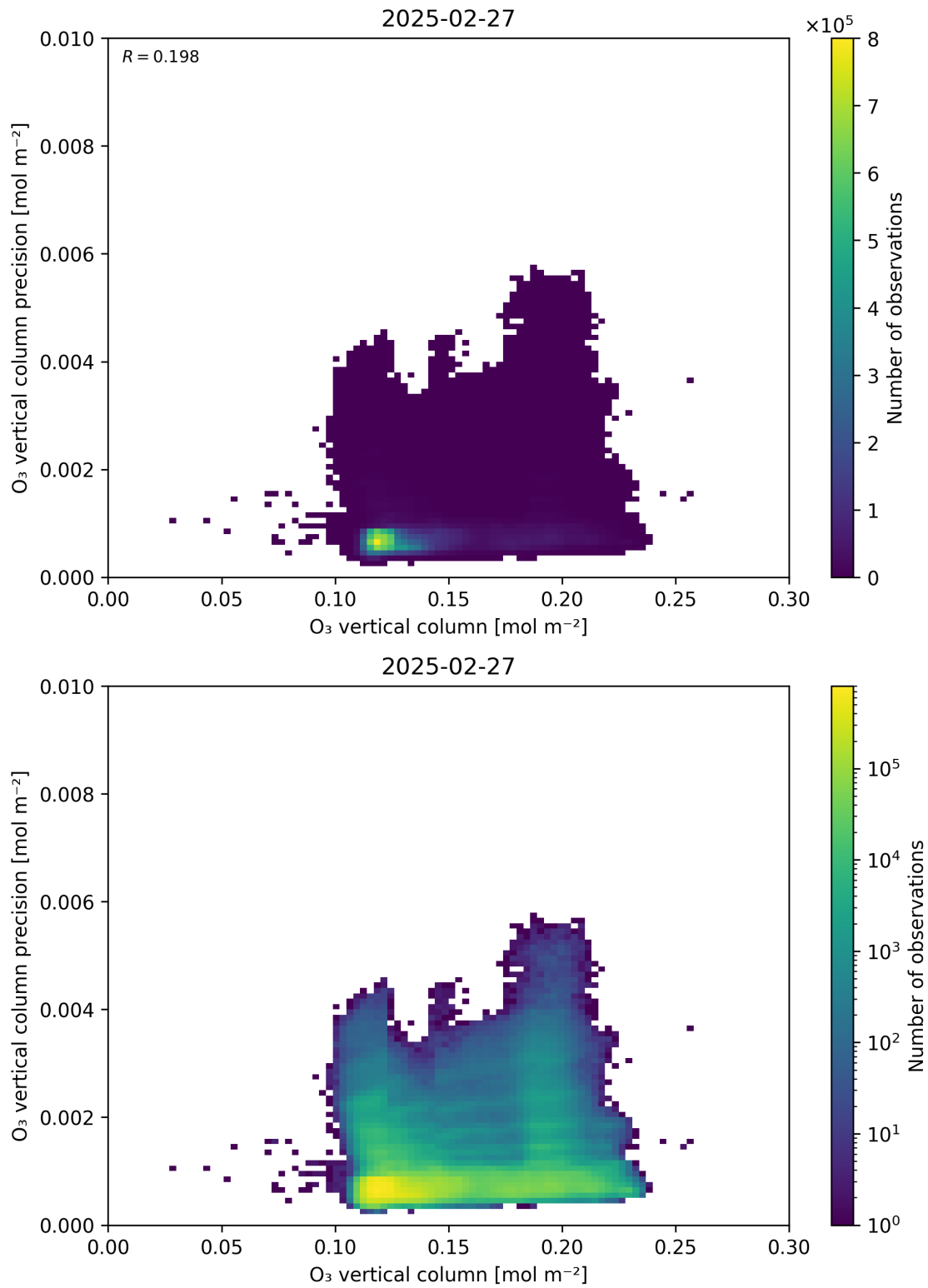
Figure 41: Scatter density plot of “O 3 vertical column” against “O 3 vertical column precision” for 2025-02-26 to 2025-02-28.
