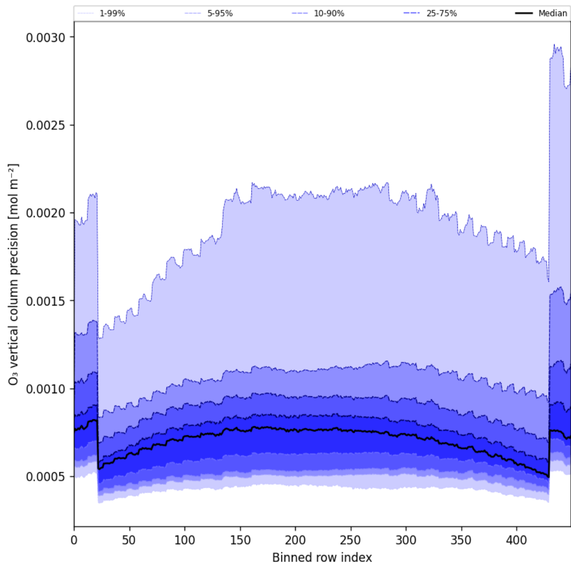
Figure 29: Along track statistics of “O 3 vertical column precision” for 2025-02-26 to 2025-02-28
