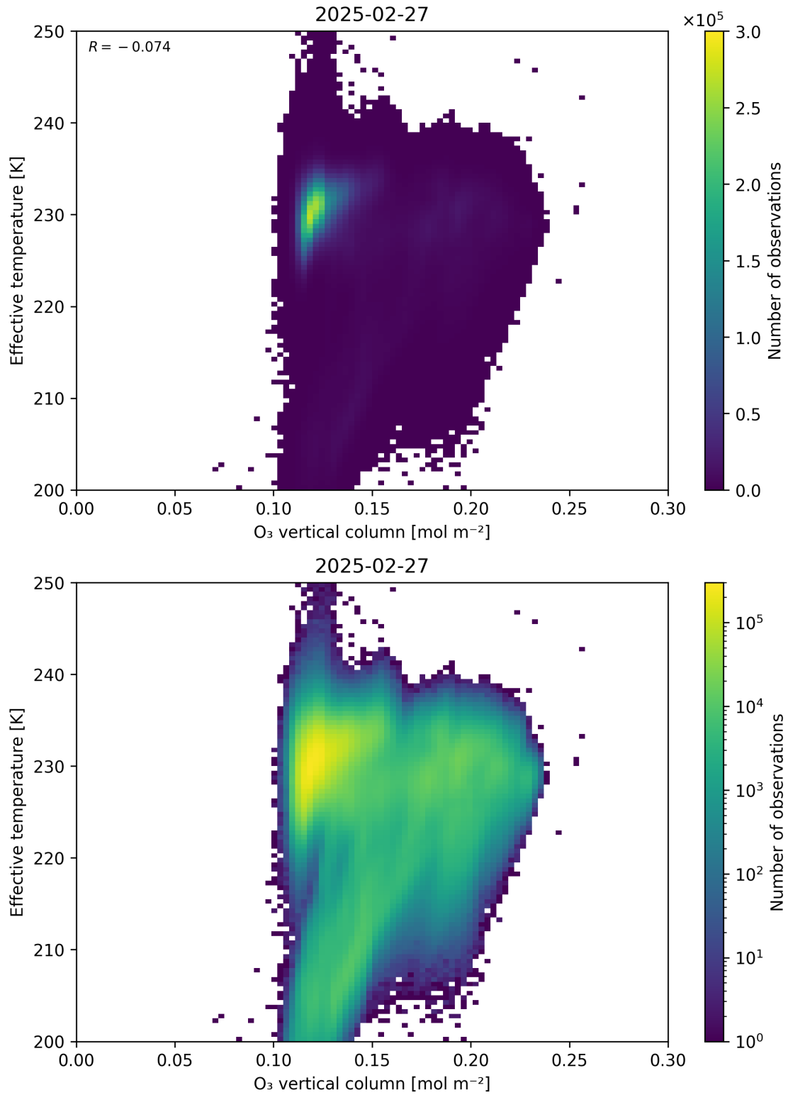
Figure 39: Scatter density plot of “O 3 vertical column” against “Effective temperature” for 2025-02-26 to 2025-02-28.
