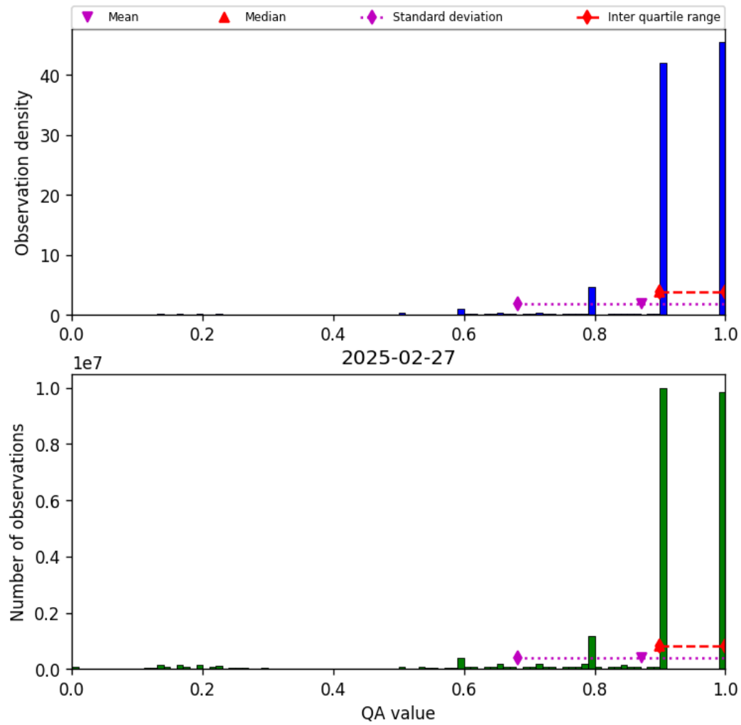
Figure 20: Histogram of “QA value” for 2025-02-26 to 2025-02-28
