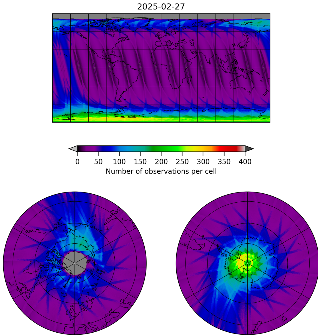
Figure 12: Map of the number of observations for 2025-02-26 to 2025-02-28
