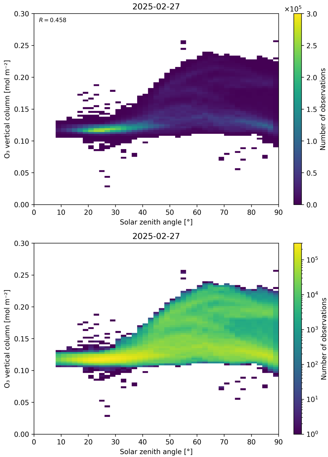
Figure 47: Scatter density plot of “Solar zenith angle” against “O 3 vertical column” for 2025-02-26 to 2025-02-28.
