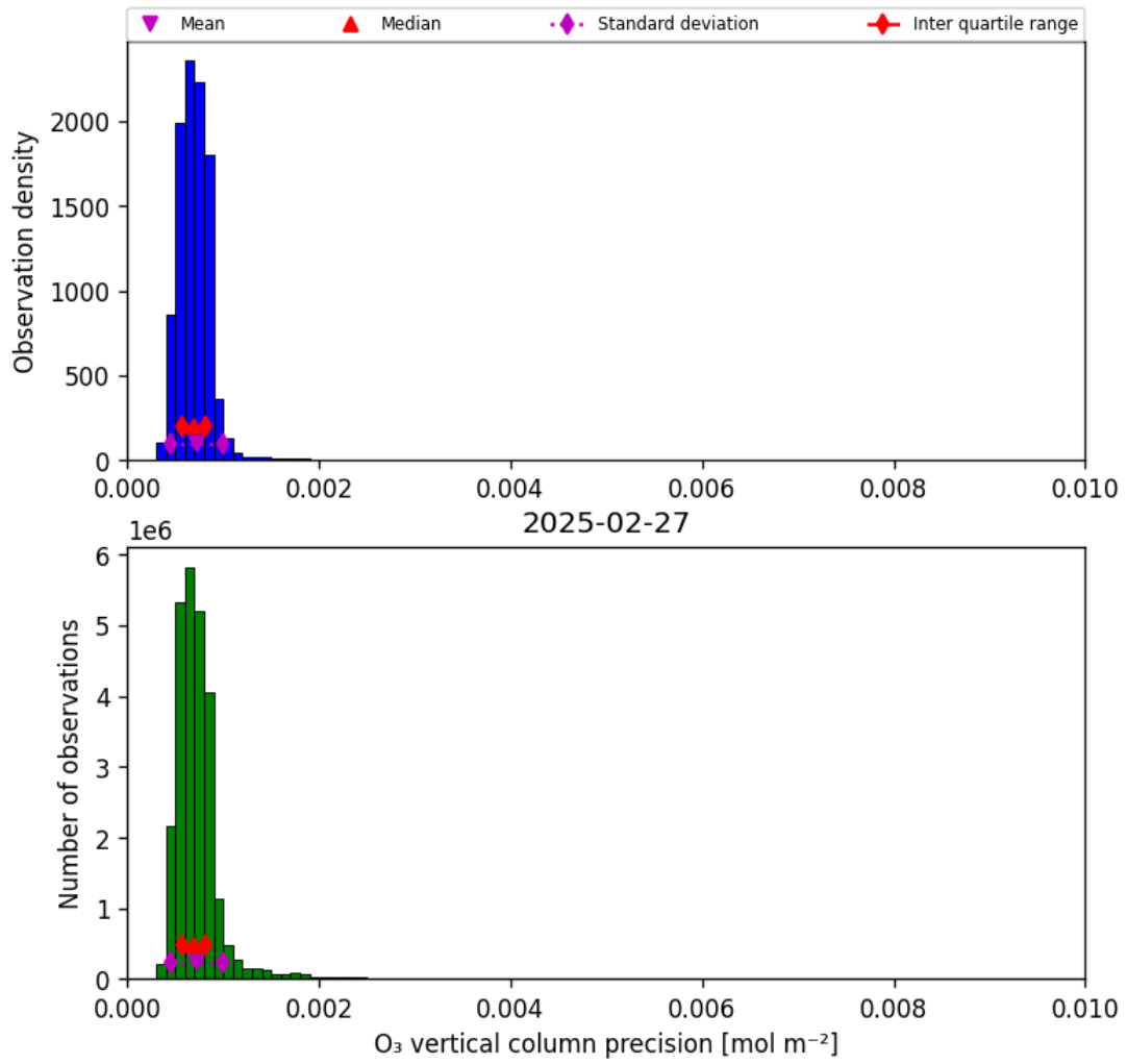
Figure 22: Histogram of “O 3 vertical column precision” for 2025-02-26 to 2025-02-28
