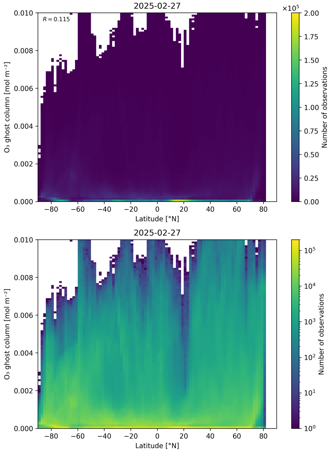
Figure 35: Scatter density plot of “Latitude” against “O 3 ghost column” for 2025-02-26 to 2025-02-28.
