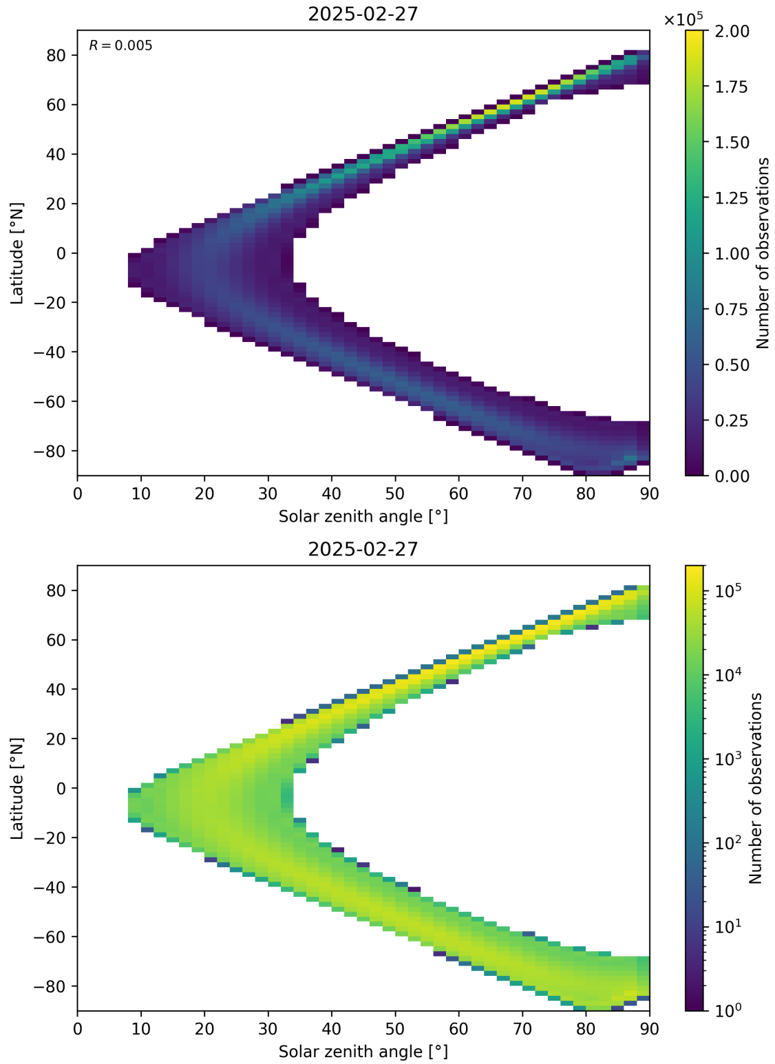
Figure 44: Scatter density plot of “Solar zenith angle” against “Latitude” for 2025-02-26 to 2025-02-28.
