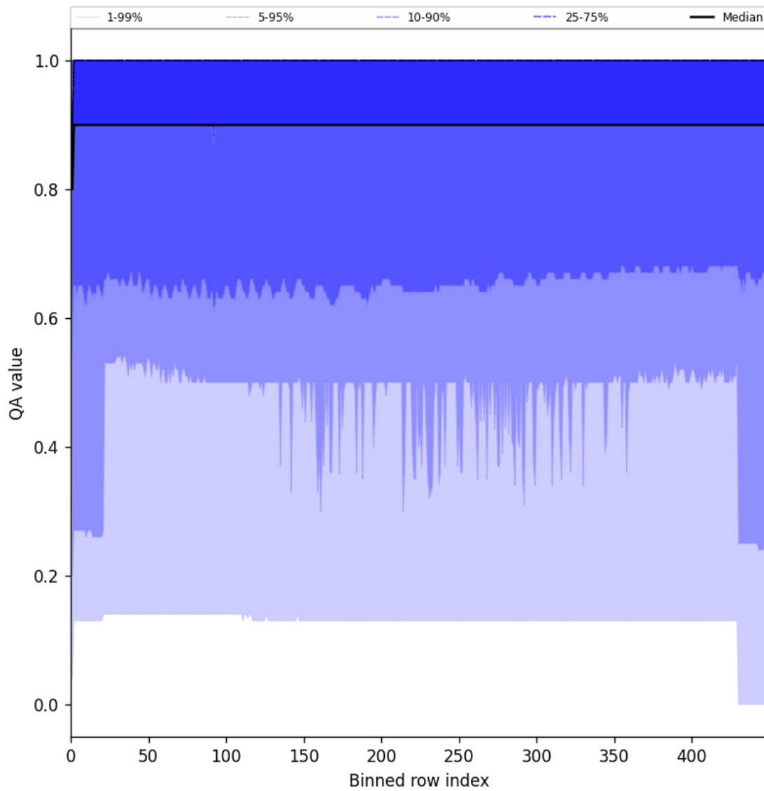
Figure 27: Along track statistics of “QA value” for 2025-02-26 to 2025-02-28
