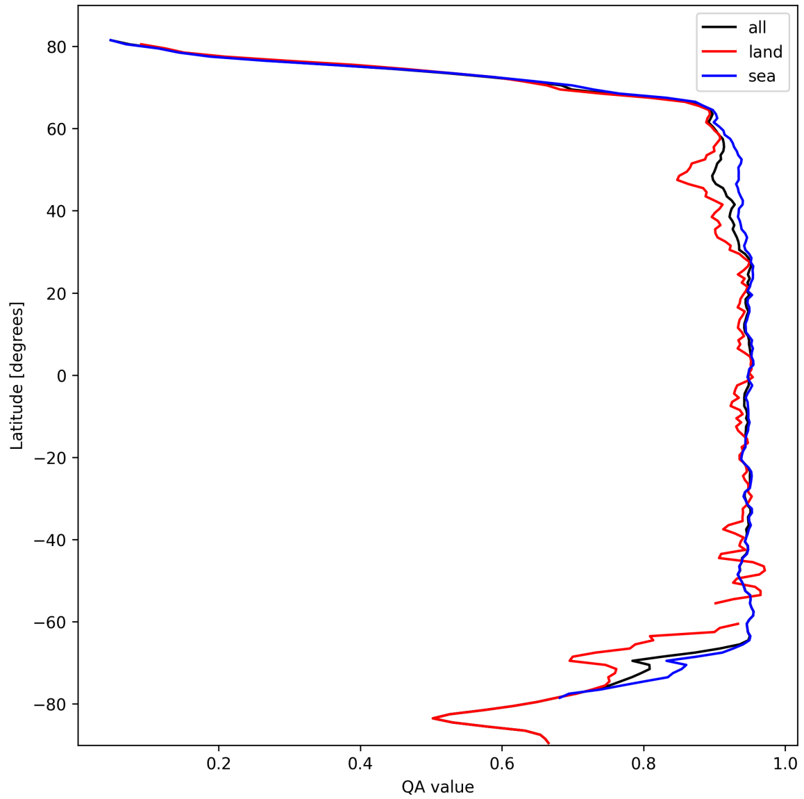
Figure 13: Zonal average of “QA value” for 2025-02-26 to 2025-02-28.
