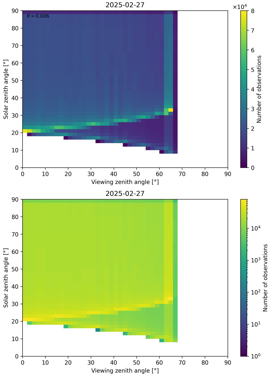
Figure 54: Scatter density plot of “Viewing zenith angle” against “Solar zenith angle” for 2025-02-26 to 2025-02-28.
