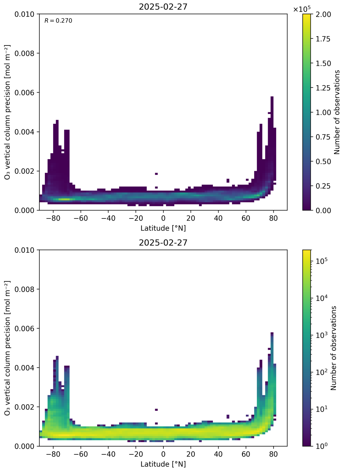
Figure 37: Scatter density plot of “Latitude” against “O 3 vertical column precision” for 2025-02-26 to 2025-02-28.
