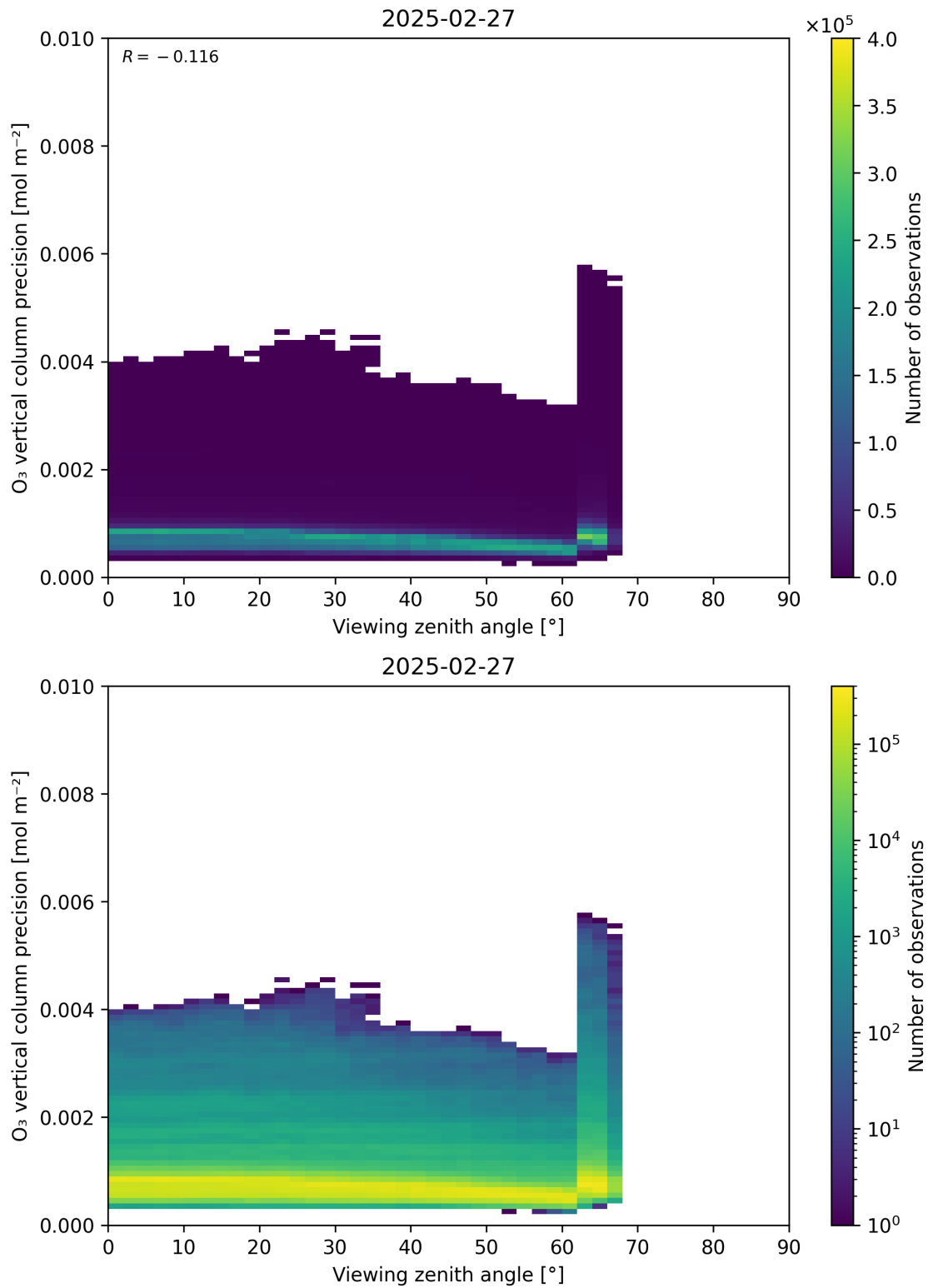
Figure 53: Scatter density plot of “Viewing zenith angle” against “O 3 vertical column precision” for 2025-02-26 to 2025-02-28.
