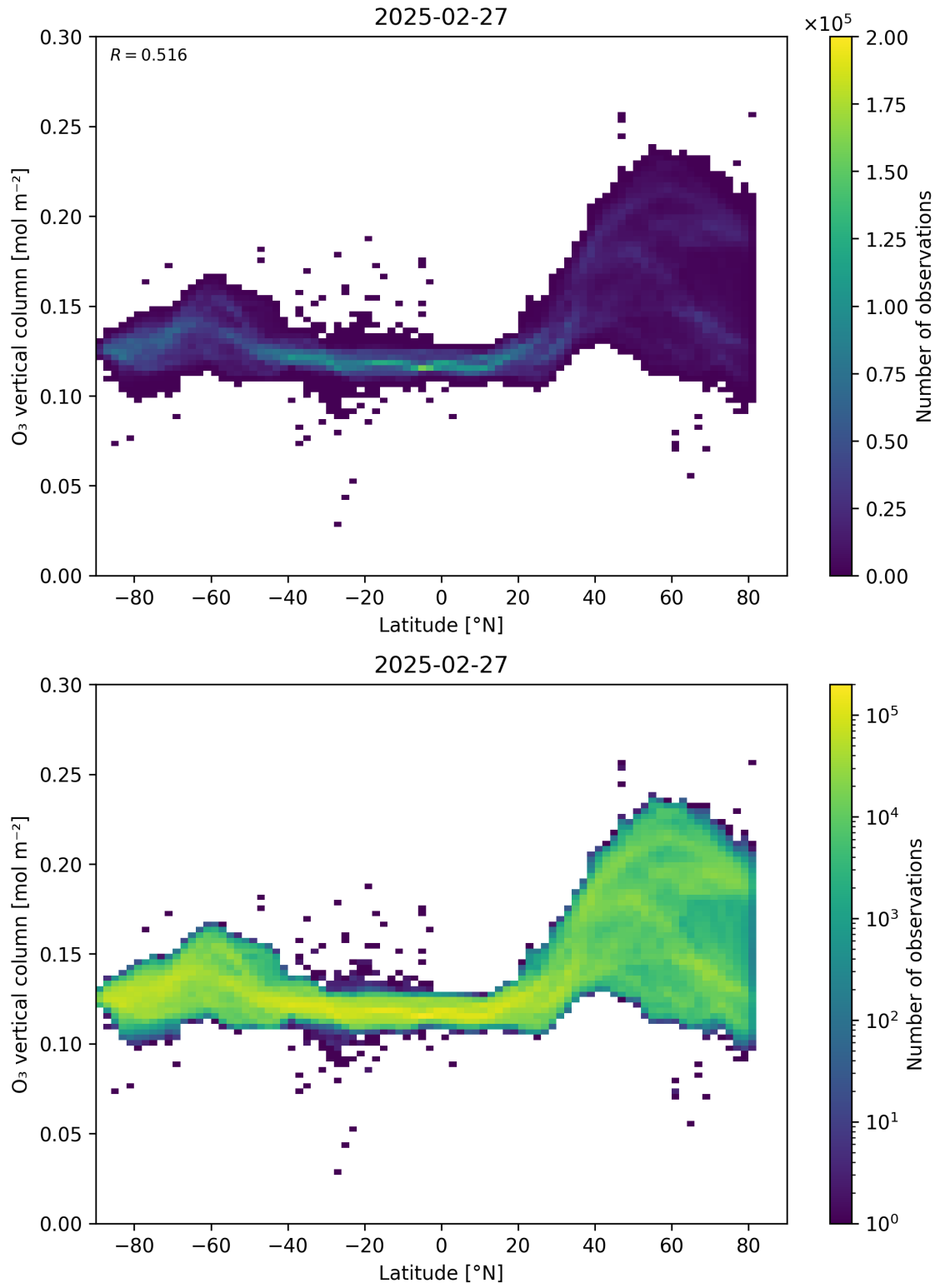
Figure 36: Scatter density plot of “Latitude” against “O 3 vertical column” for 2025-02-26 to 2025-02-28.
