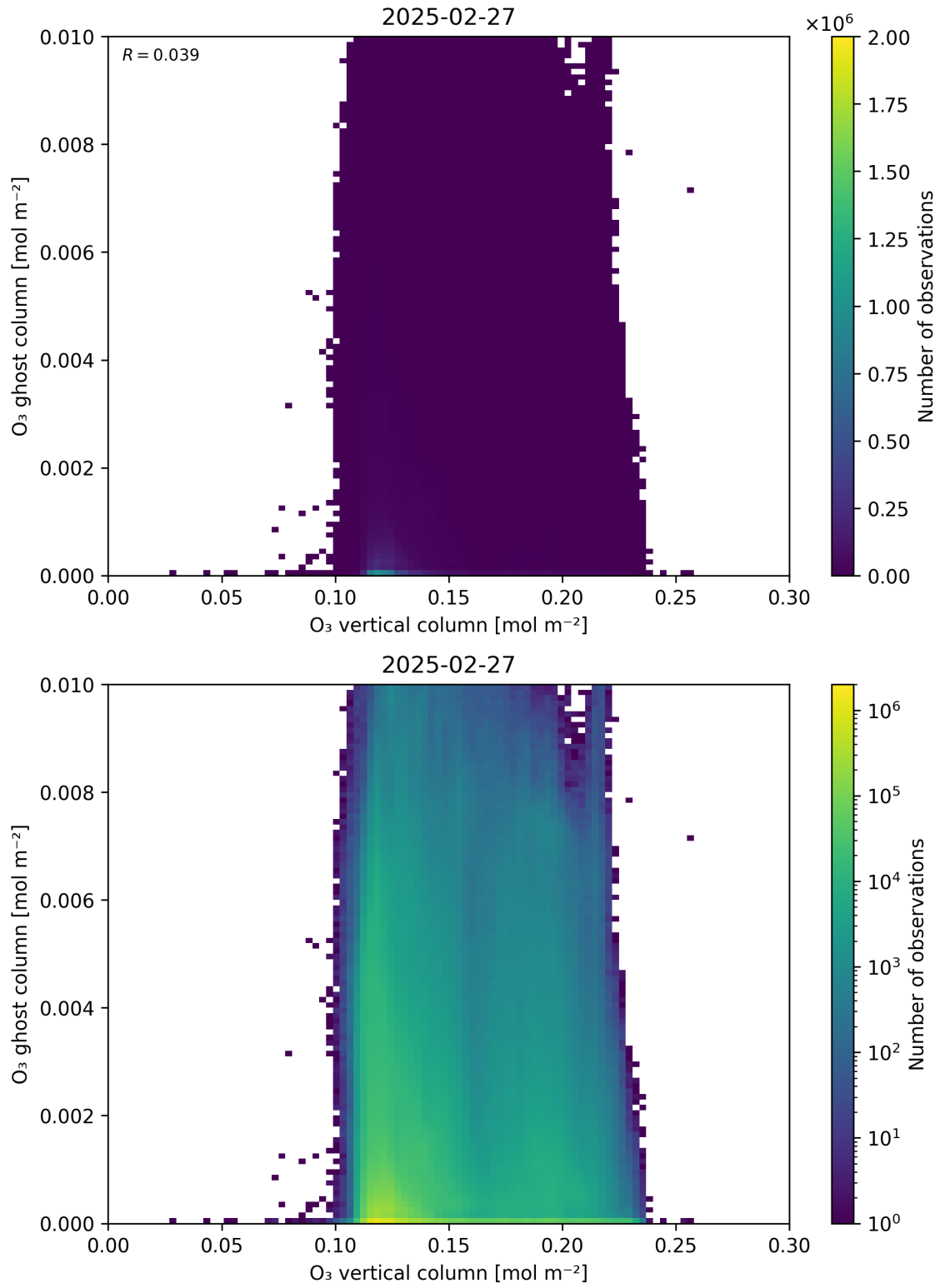
Figure 40: Scatter density plot of “O 3 vertical column” against “O 3 ghost column” for 2025-02-26 to 2025-02-28.
