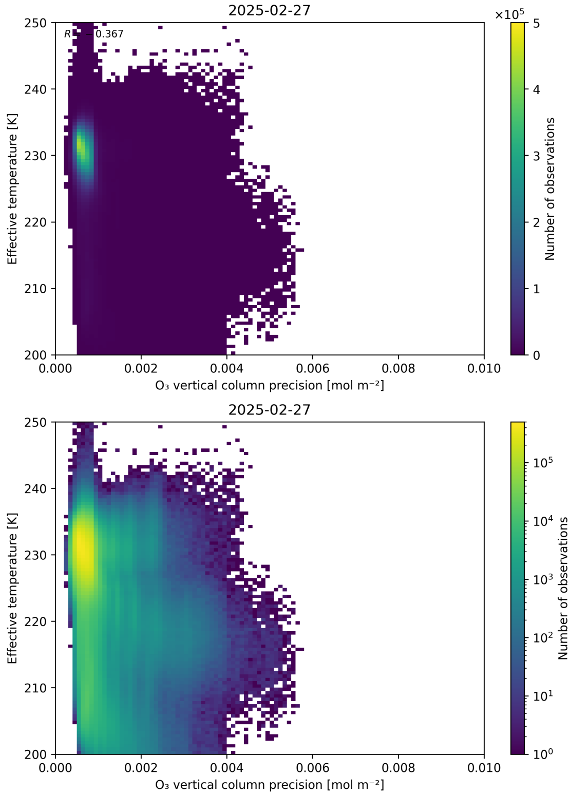
Figure 42: Scatter density plot of “ O_3 vertical column precision” against “Effective temperature” for 2025-02-26 to 2025-02-28.
