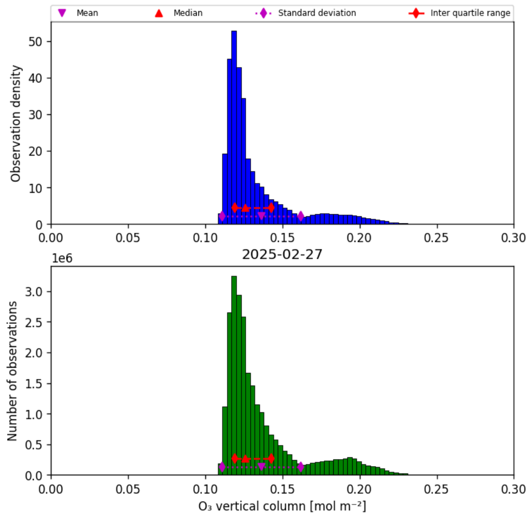
Figure 21: Histogram of “O 3 vertical column” for 2025-02-26 to 2025-02-28
