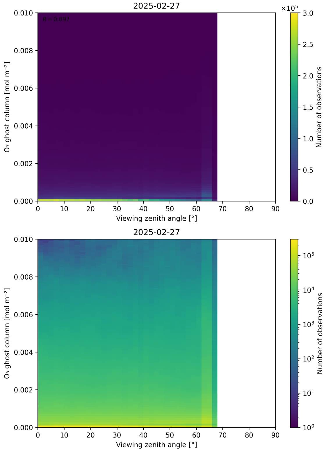
Figure 51: Scatter density plot of “Viewing zenith angle” against “O 3 ghost column” for 2025-02-26 to 2025-02-28.
