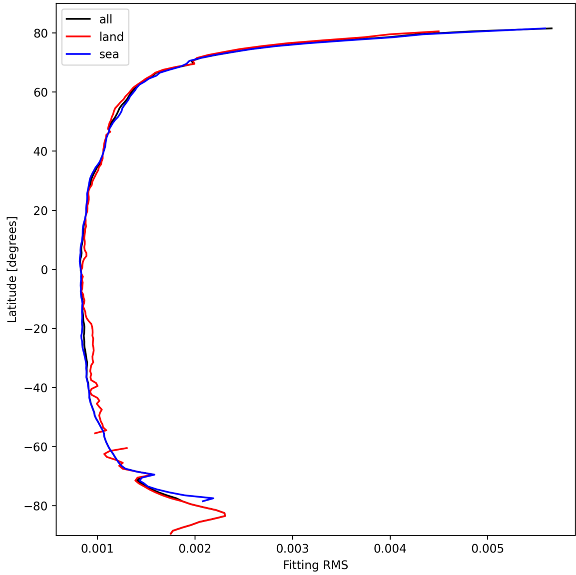
Figure 16: Zonal average of “Fitting RMS” for 2025-02-26 to 2025-02-28.
