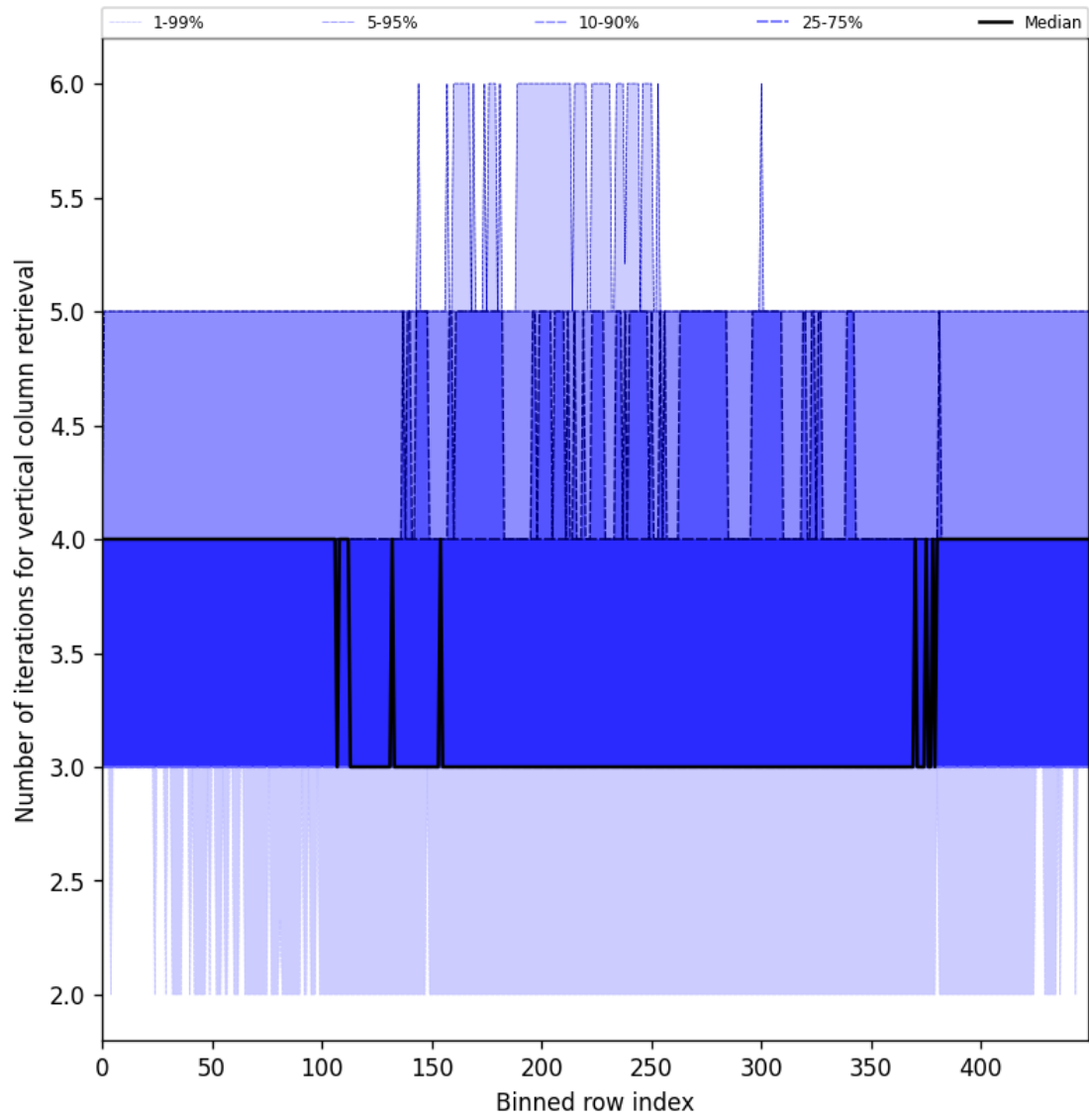
Figure 33: Along track statistics of “Number of iterations for vertical column retrieval” for 2025-02-26 to 2025-02-28
