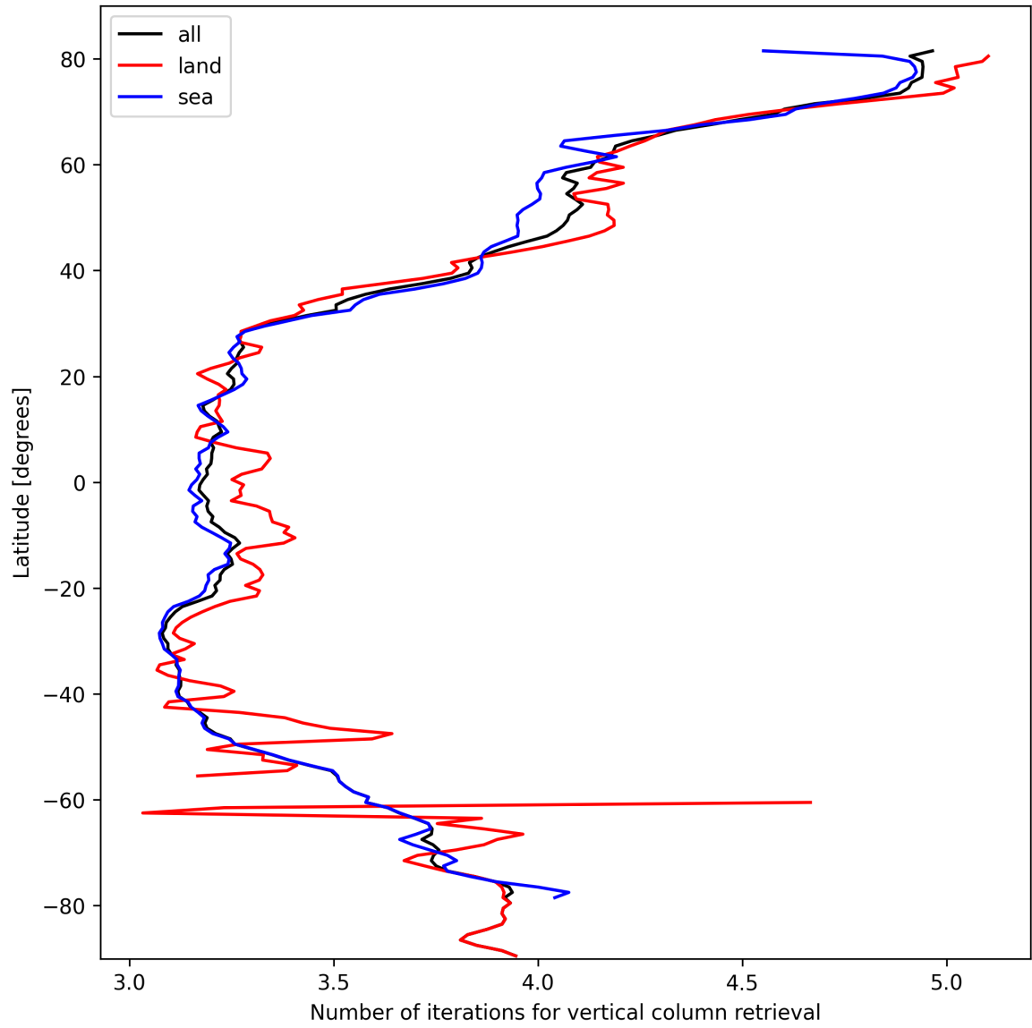
Figure 19: Zonal average of “Number of iterations for vertical column retrieval” for 2025-02-26 to 2025-02-28.
