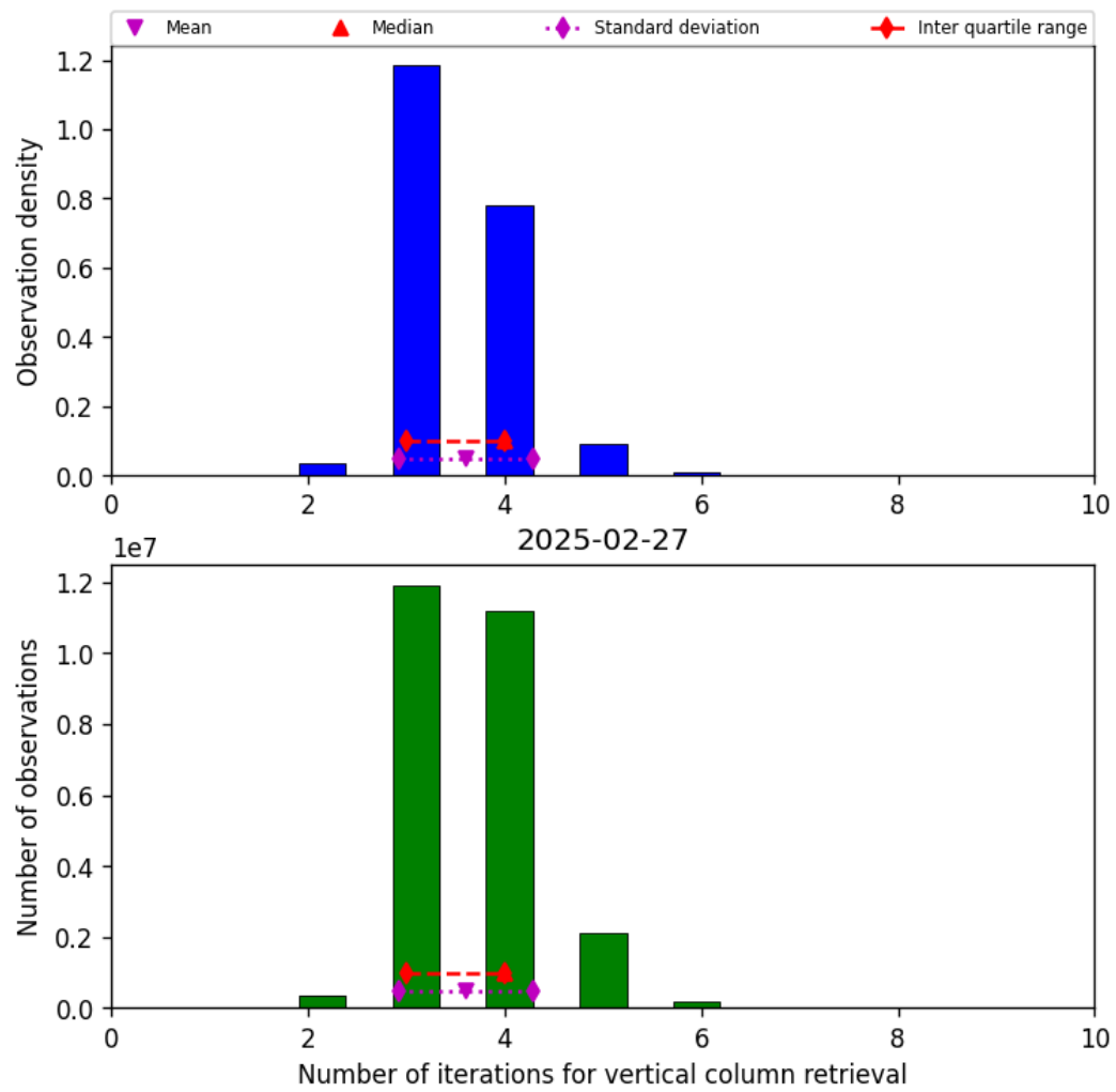
Figure 26: Histogram of “Number of iterations for vertical column retrieval” for 2025-02-26 to 2025-02-28
