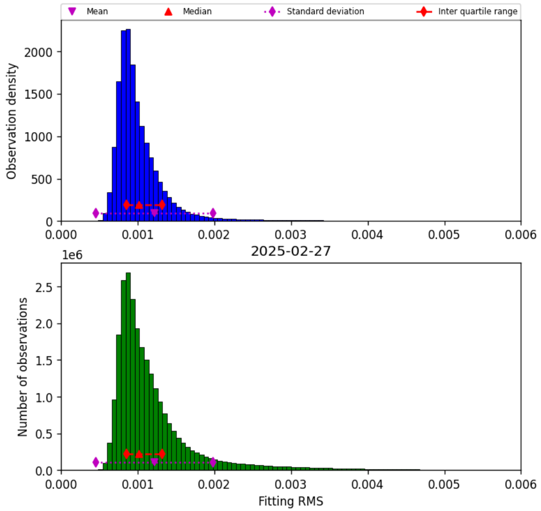
Figure 23: Histogram of “Fitting RMS” for 2025-02-26 to 2025-02-28
