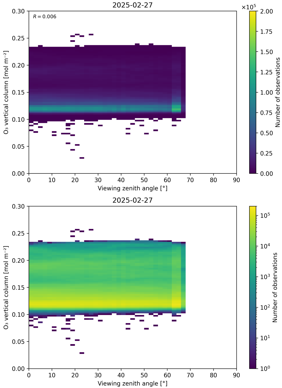
Figure 52: Scatter density plot of “Viewing zenith angle” against “O 3 vertical column” for 2025-02-26 to 2025-02-28.
