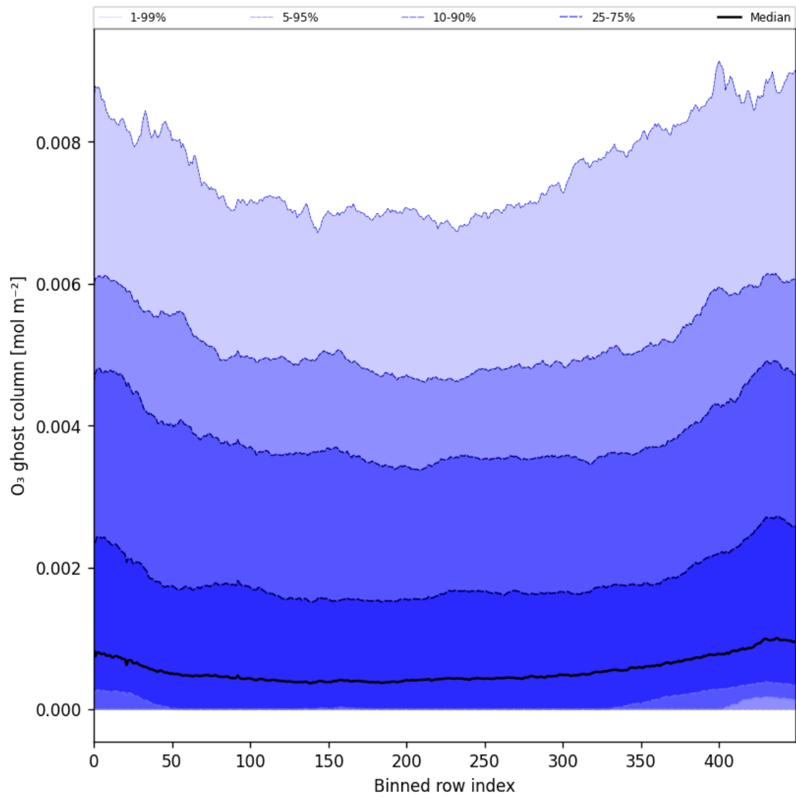
Figure 32: Along track statistics of “O 3 ghost column” for 2025-02-26 to 2025-02-28
