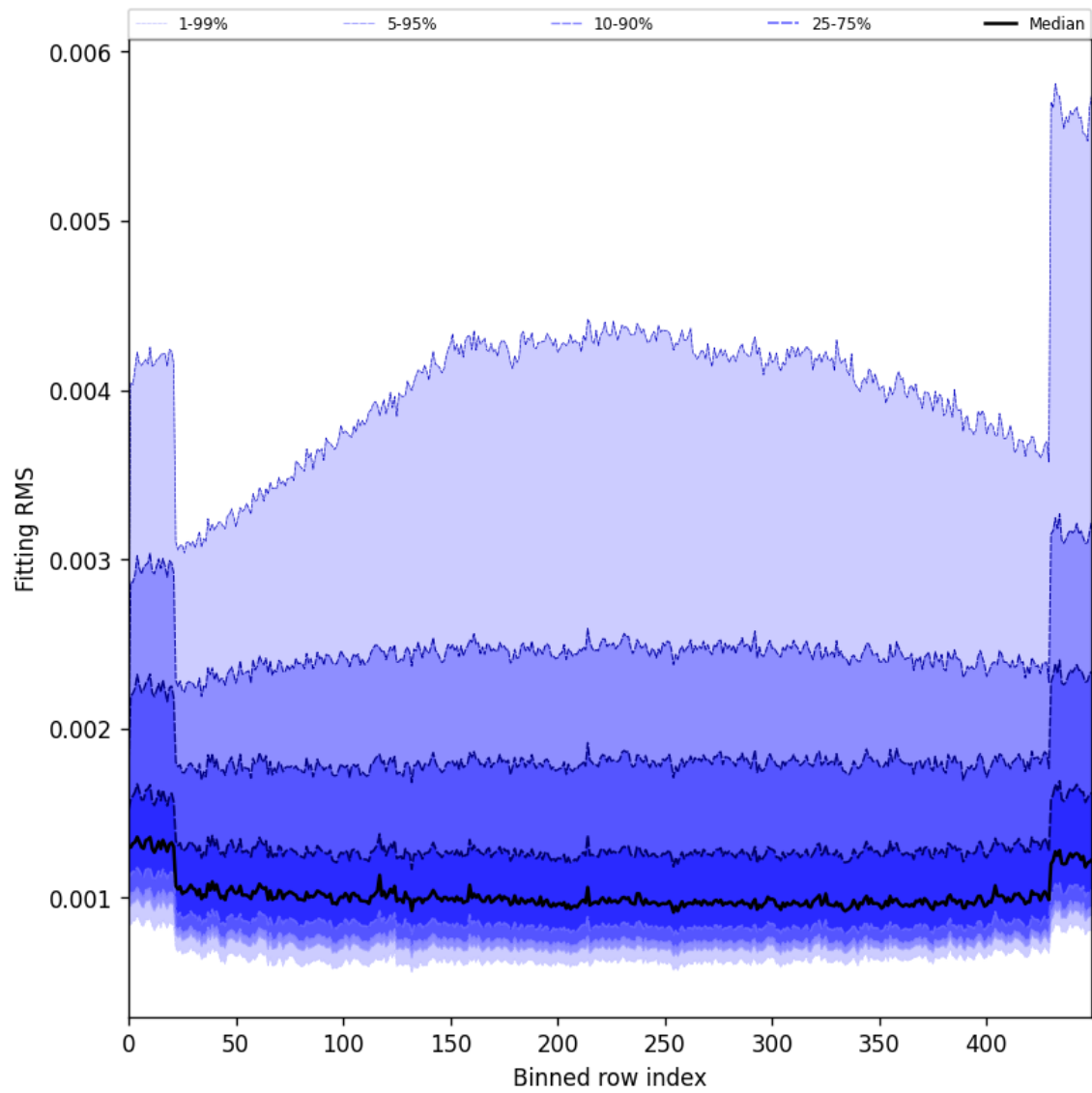
Figure 30: Along track statistics of “Fitting RMS” for 2025-02-26 to 2025-02-28
