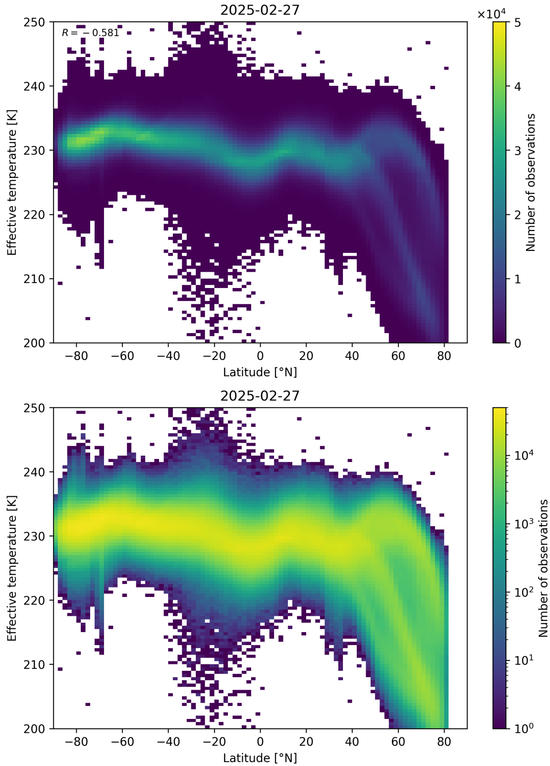
Figure 34: Scatter density plot of “Latitude” against “Effective temperature” for 2025-02-26 to 2025-02-28.
