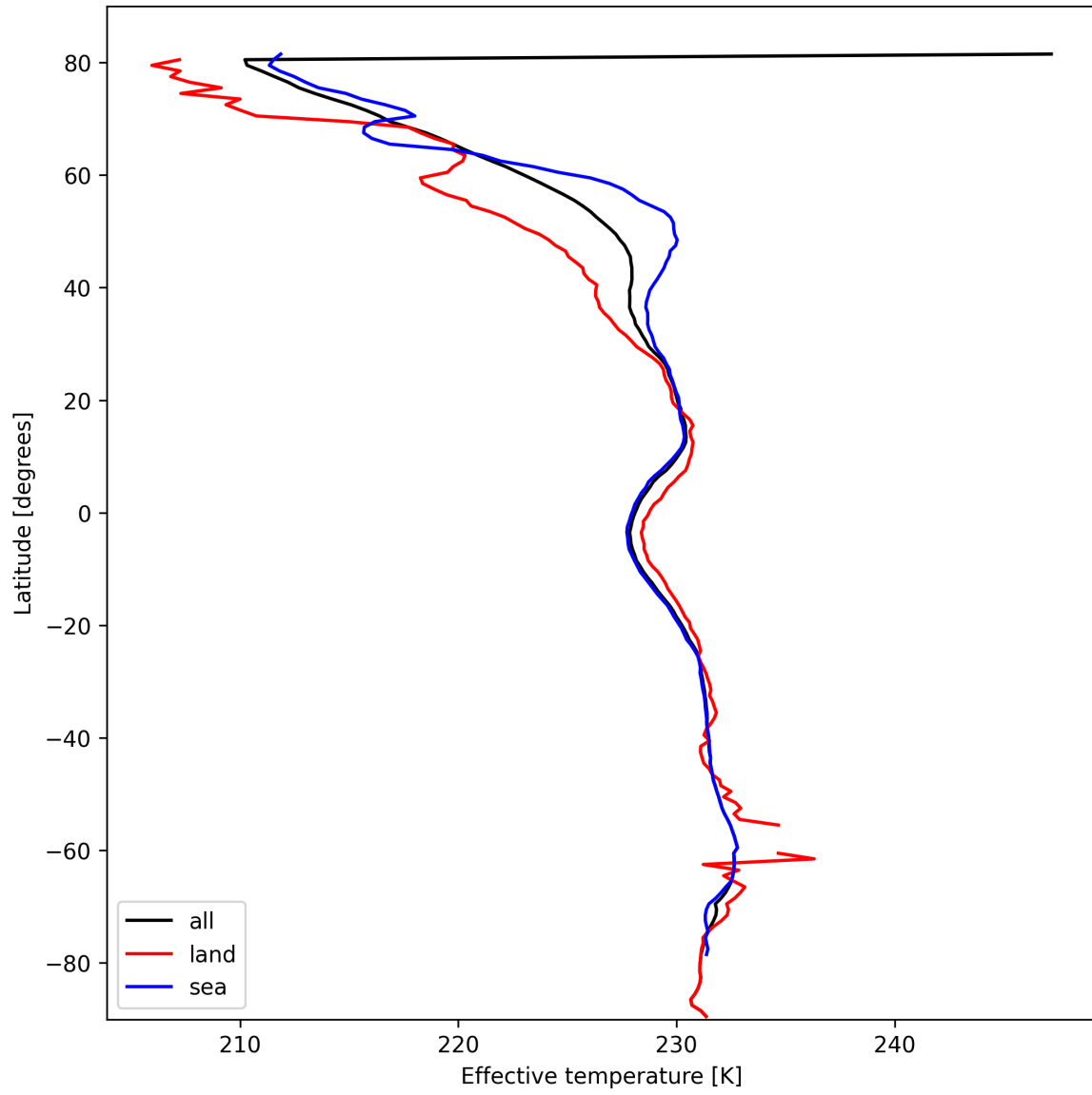
Figure 17: Zonal average of “Effective temperature” for 2025-02-26 to 2025-02-28.
