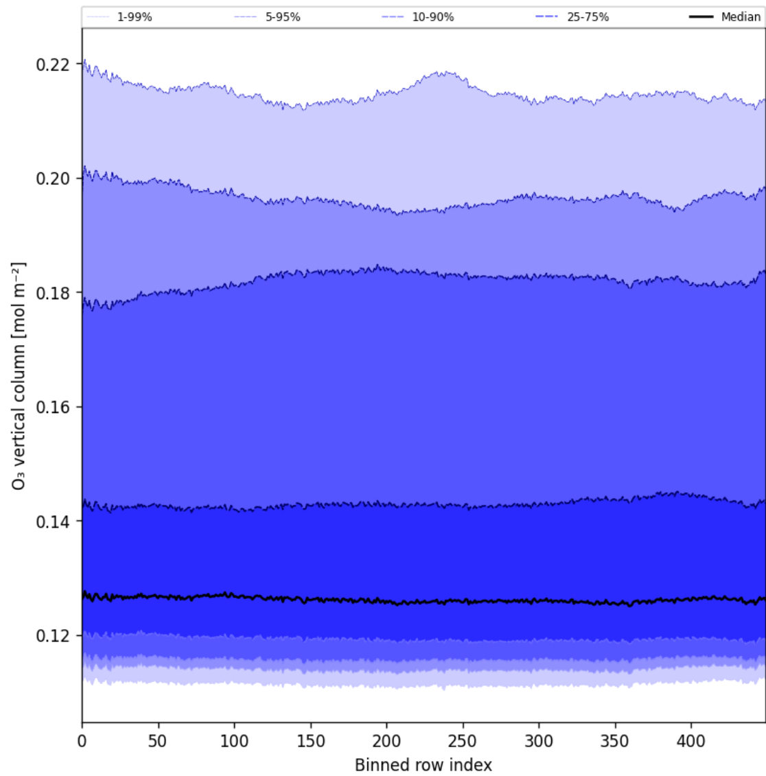
Figure 28: Along track statistics of “O 3 vertical column” for 2025-02-26 to 2025-02-28
