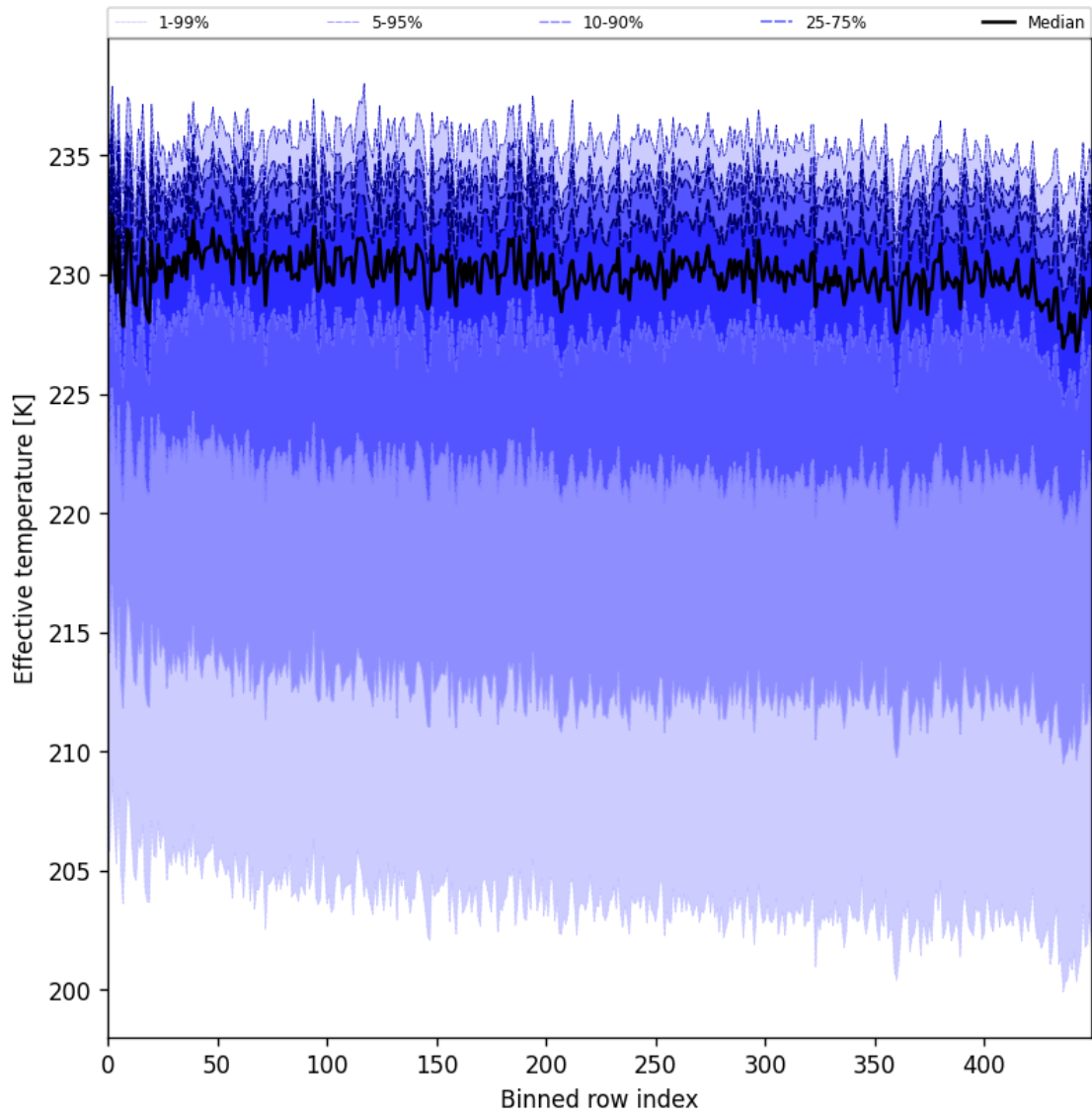
Figure 31: Along track statistics of "Effective temperature" for 2025-02-26 to 2025-02-28
