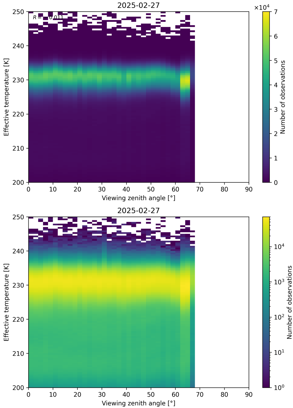
Figure 50: Scatter density plot of “Viewing zenith angle” against “Effective temperature” for 2025-02-26 to 2025-02-28.
