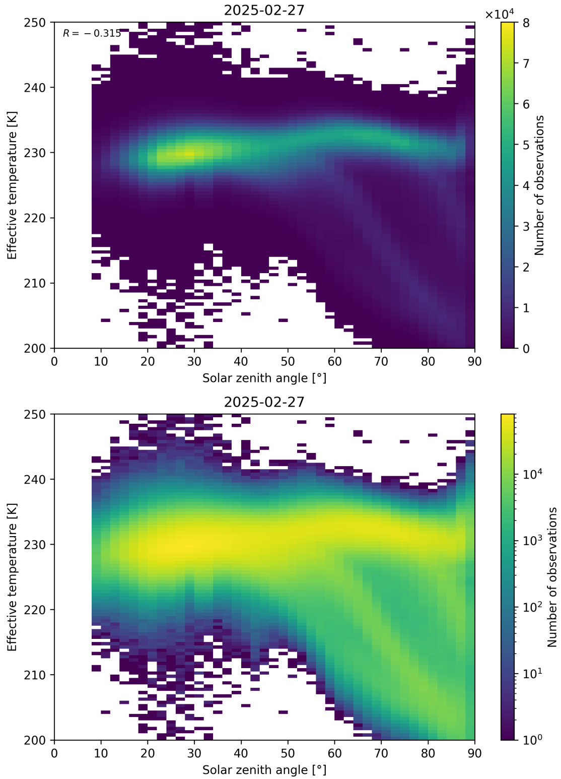
Figure 45: Scatter density plot of “Solar zenith angle” against “Effective temperature” for 2025-02-26 to 2025-02-28.
