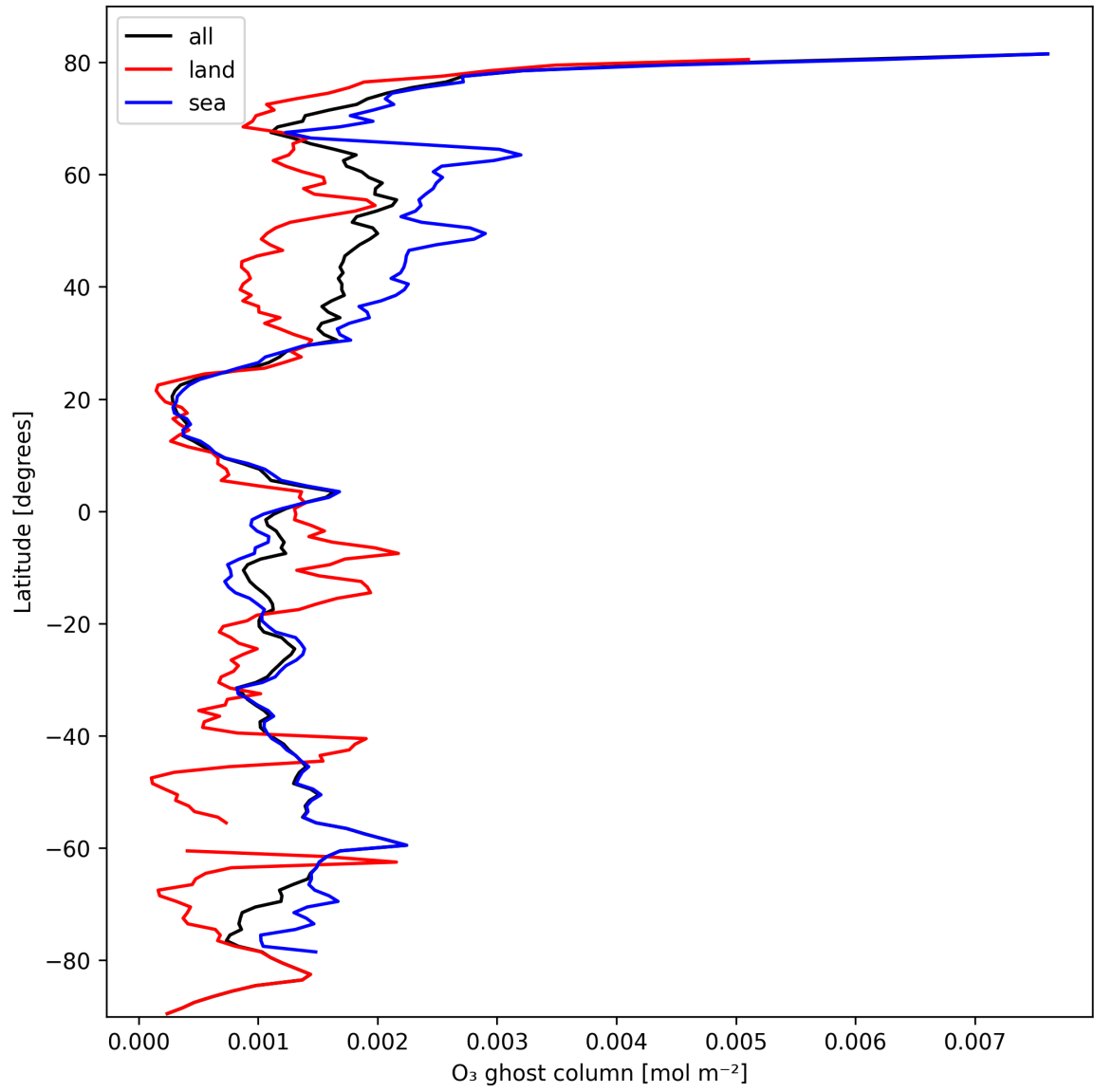
Figure 18: Zonal average of “O 3 ghost column” for 2025-02-26 to 2025-02-28.
