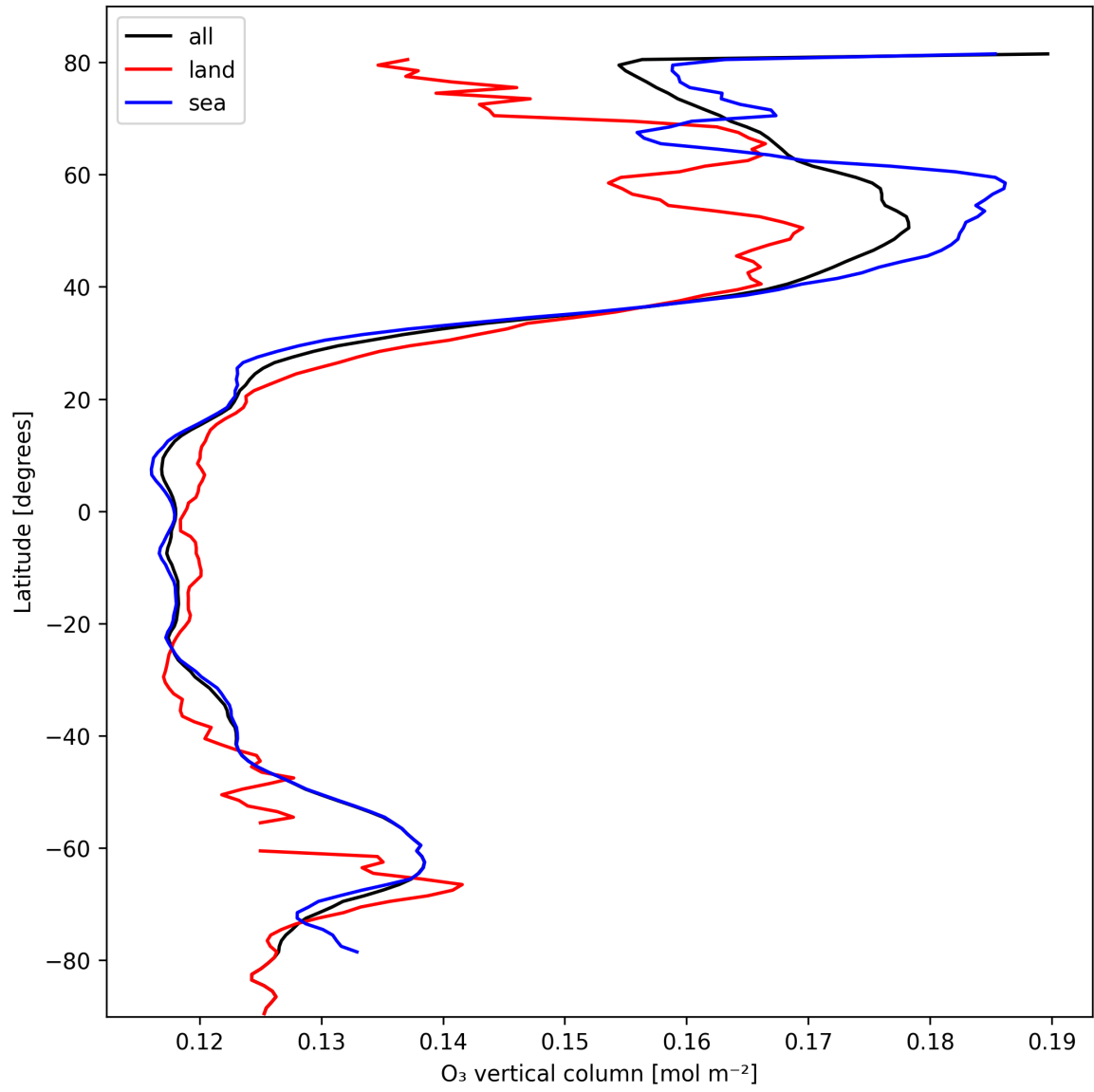
Figure 14: Zonal average of “O 3 vertical column” for 2025-02-26 to 2025-02-28.
