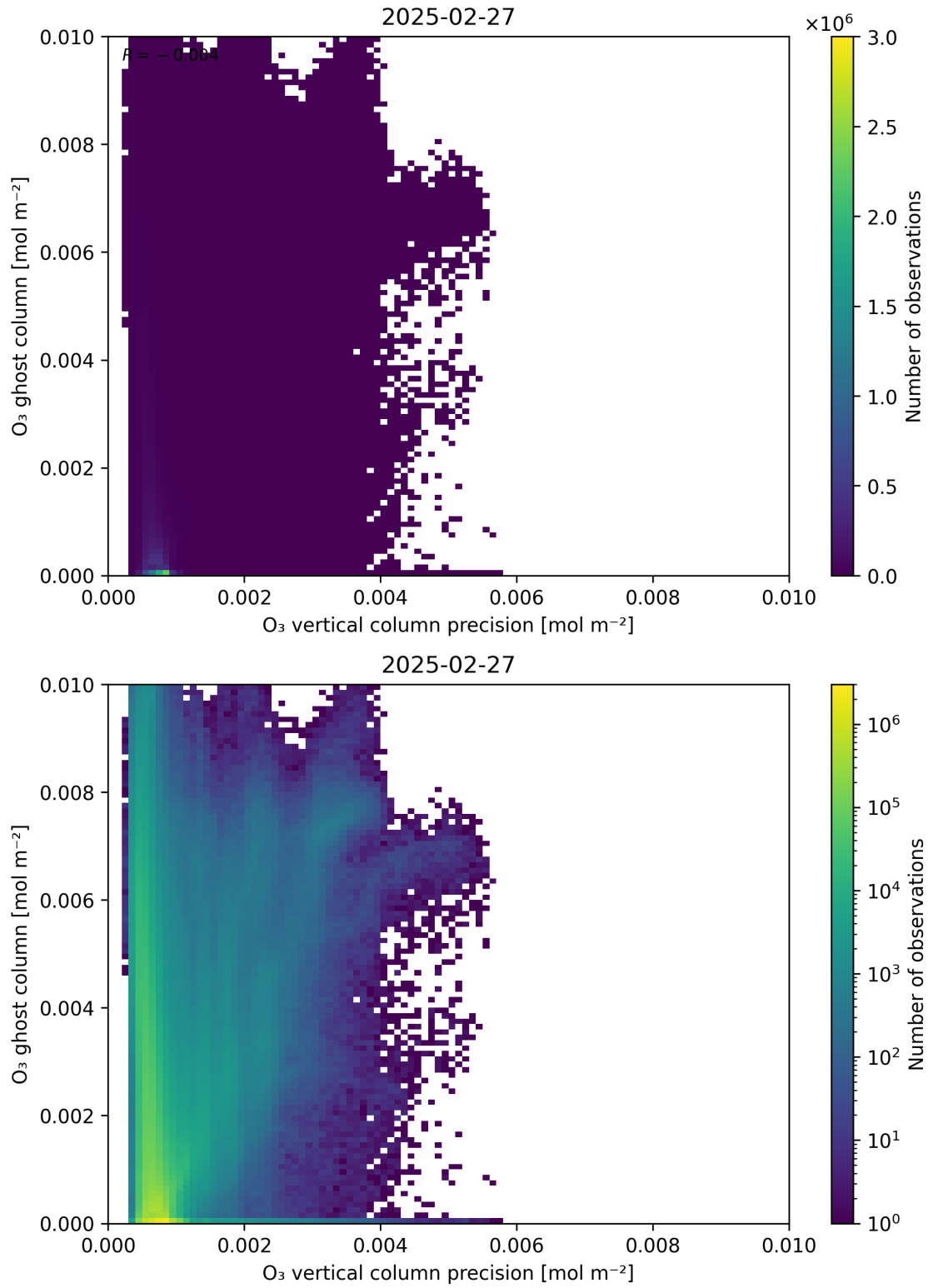
Figure 43: Scatter density plot of “ \text{O}_3 vertical column precision” against “ \text{O}_3 ghost column” for 2025-02-26 to 2025-02-28.
