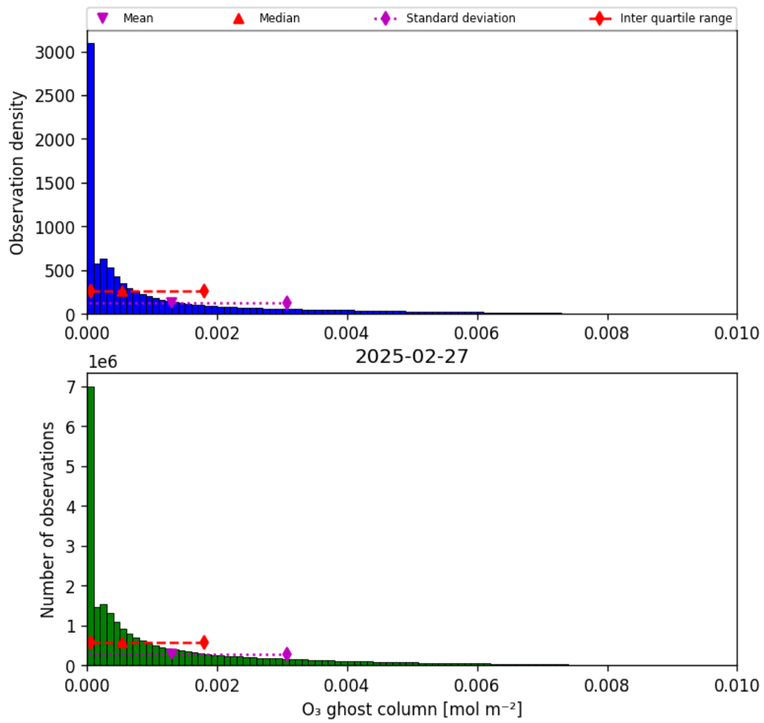
Figure 25: Histogram of “O 3 ghost column” for 2025-02-26 to 2025-02-28
