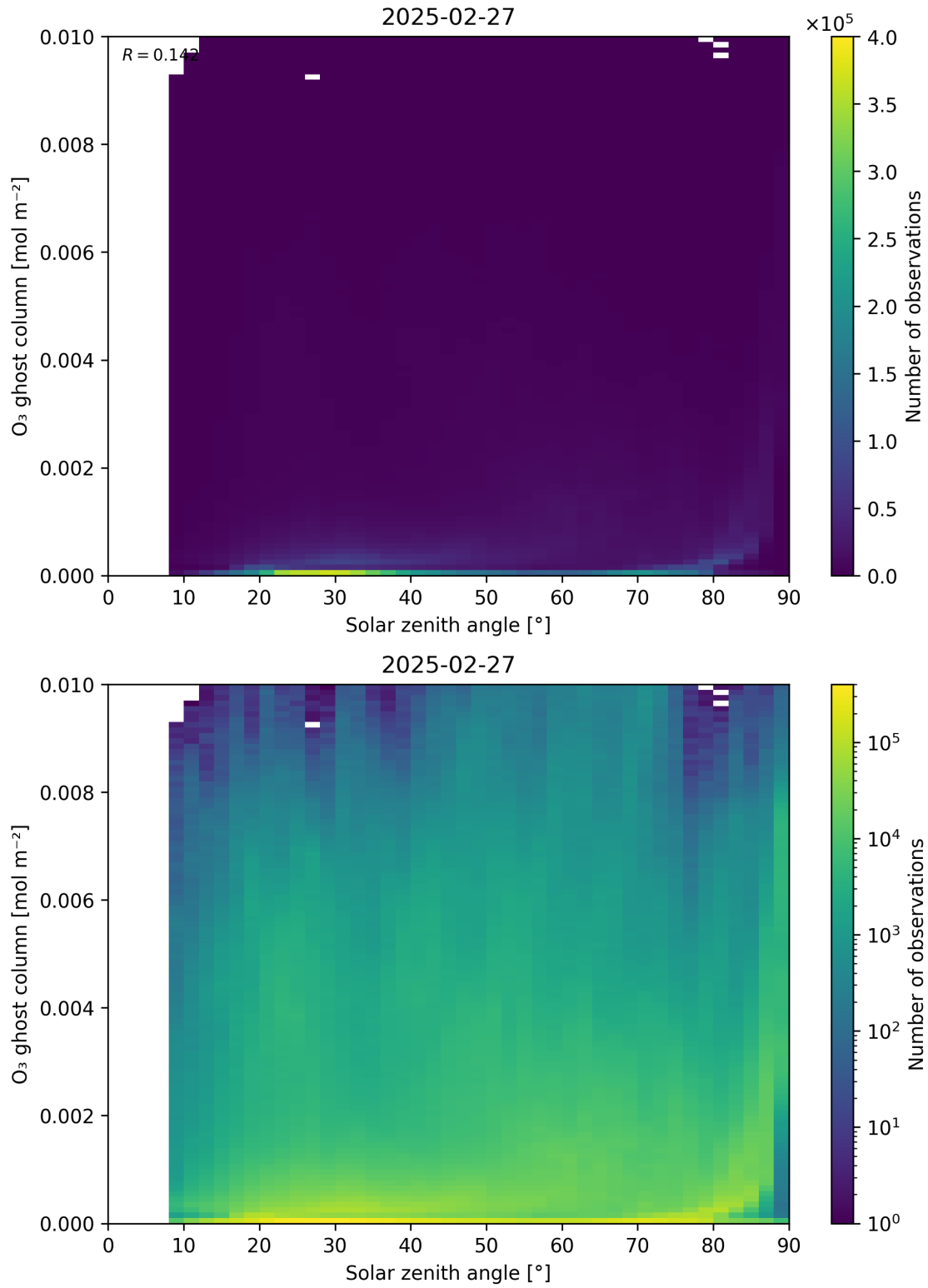
Figure 46: Scatter density plot of “Solar zenith angle” against “O 3 ghost column” for 2025-02-26 to 2025-02-28.
