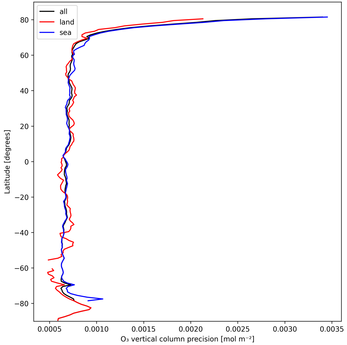
Figure 15: Zonal average of “O 3 vertical column precision” for 2025-02-26 to 2025-02-28.
