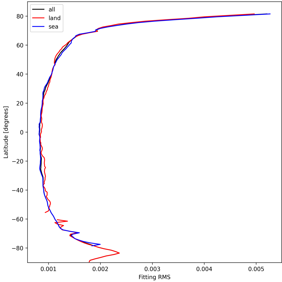
Figure 16: Zonal average of “Fitting RMS” for 2025-02-27 to 2025-03-01.
