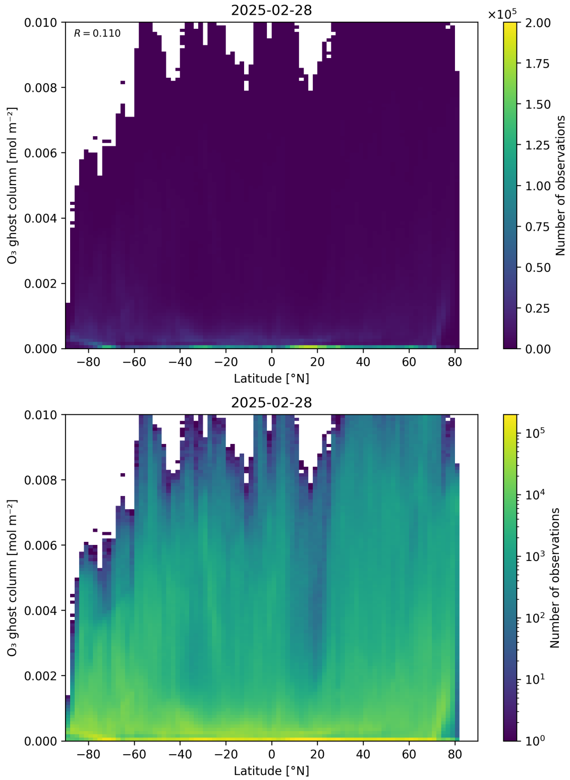
Figure 35: Scatter density plot of “Latitude” against “O 3 ghost column” for 2025-02-27 to 2025-03-01.
