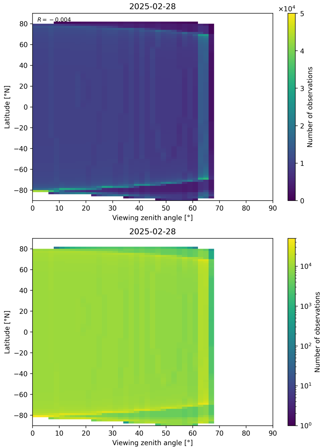
Figure 49: Scatter density plot of “Viewing zenith angle” against “Latitude” for 2025-02-27 to 2025-03-01.
