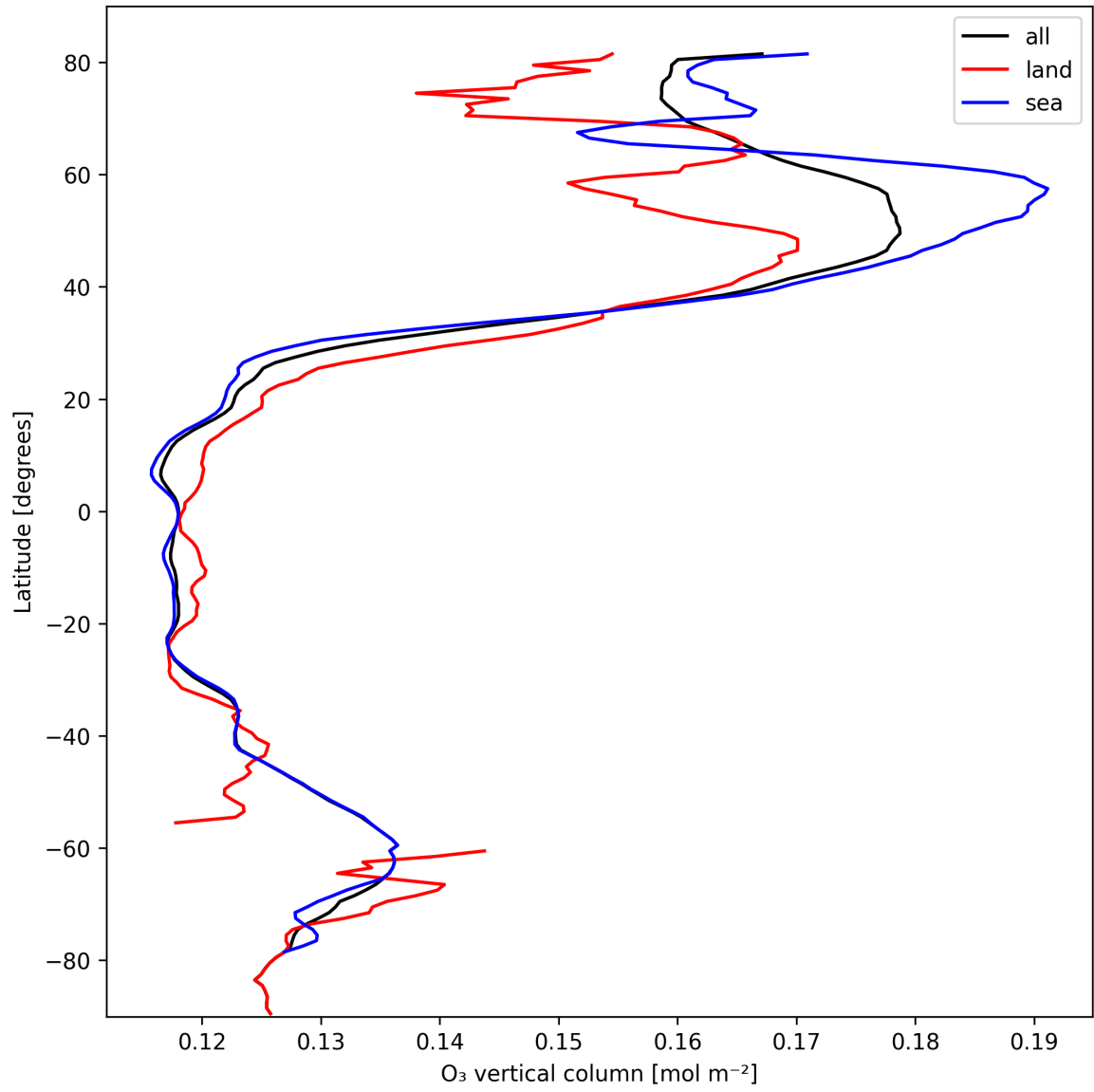
Figure 14: Zonal average of “O 3 vertical column” for 2025-02-27 to 2025-03-01.
