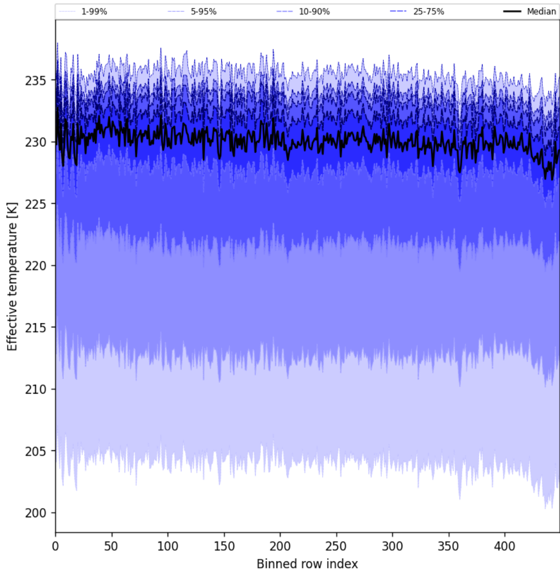
Figure 31: Along track statistics of “Effective temperature” for 2025-02-27 to 2025-03-01
