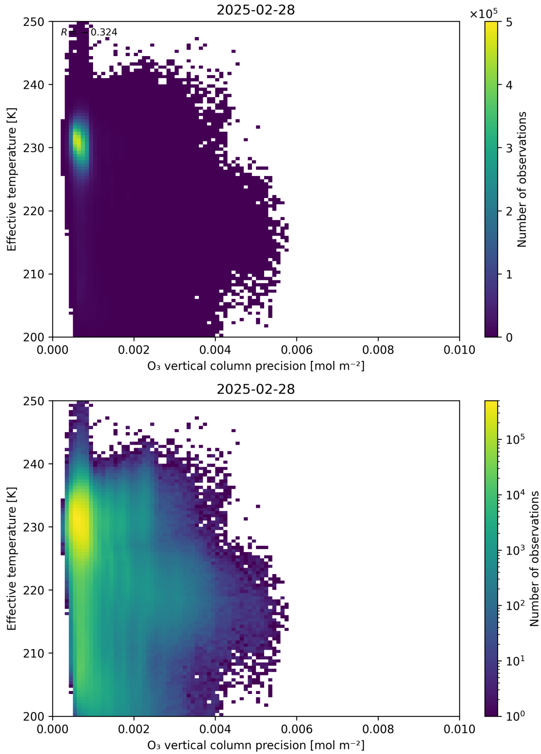
Figure 42: Scatter density plot of “O 3 vertical column precision” against “Effective temperature” for 2025-02-27 to 2025-03-01.
