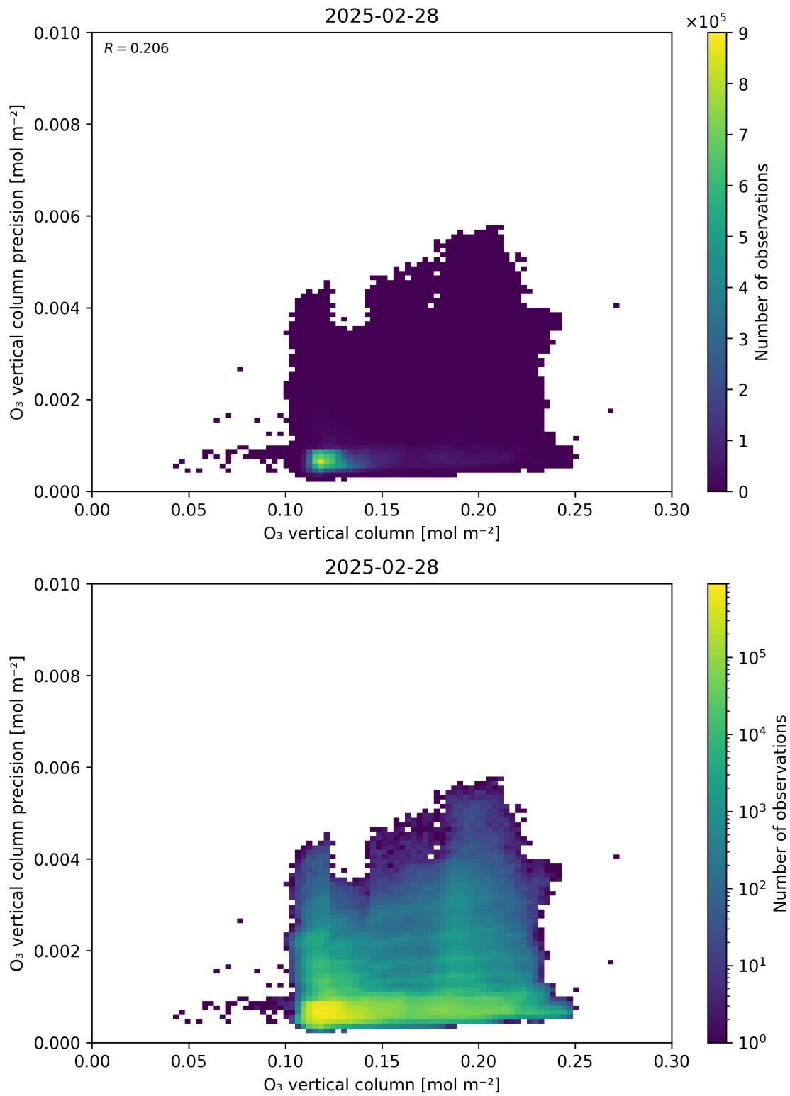
Figure 41: Scatter density plot of “O 3 vertical column” against “O 3 vertical column precision” for 2025-02-27 to 2025-03-01.
