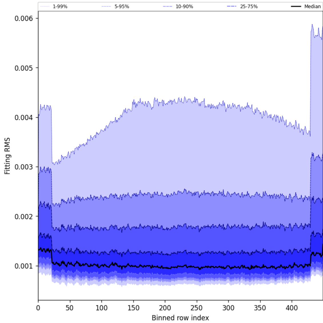
Figure 30: Along track statistics of “Fitting RMS” for 2025-02-27 to 2025-03-01
