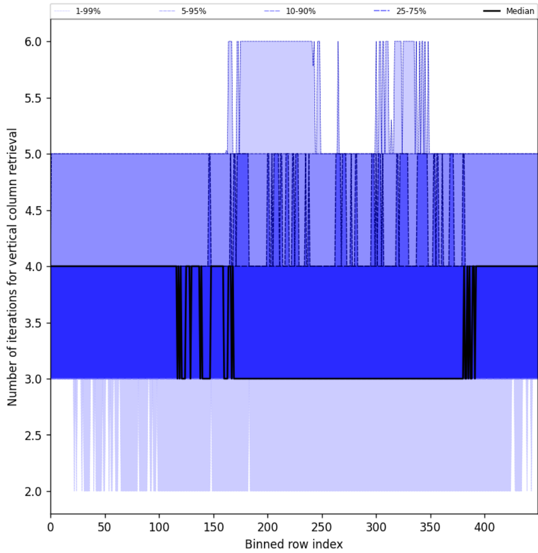
Figure 33: Along track statistics of “Number of iterations for vertical column retrieval” for 2025-02-27 to 2025-03-01
