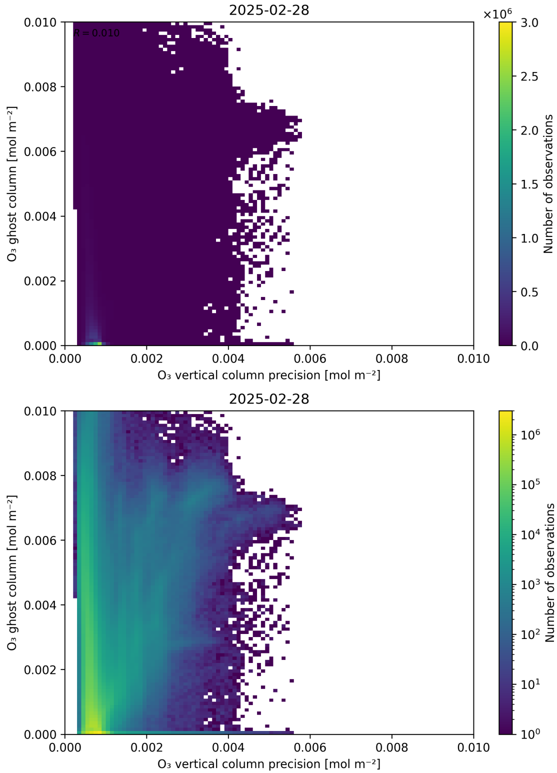
Figure 43: Scatter density plot of “O 3 vertical column precision” against “O 3 ghost column” for 2025-02-27 to 2025-03-01.
