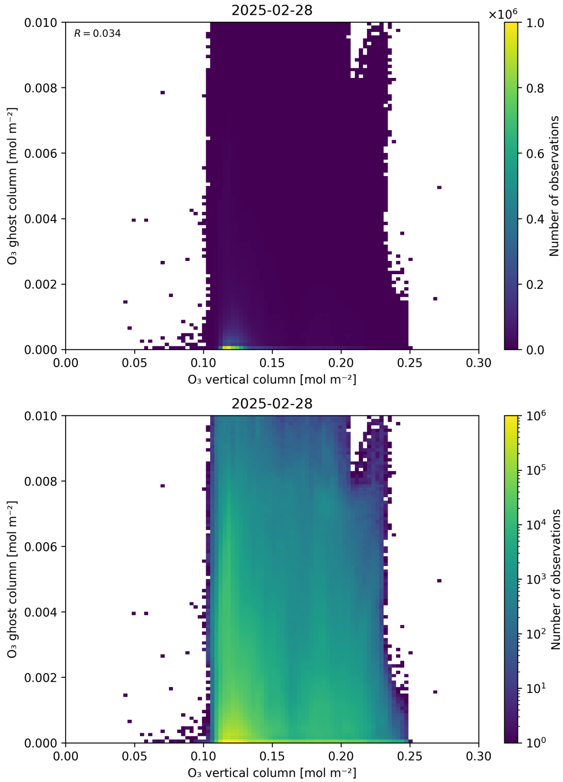
Figure 40: Scatter density plot of “ O_3 vertical column” against “ O_3 ghost column” for 2025-02-27 to 2025-03-01.
