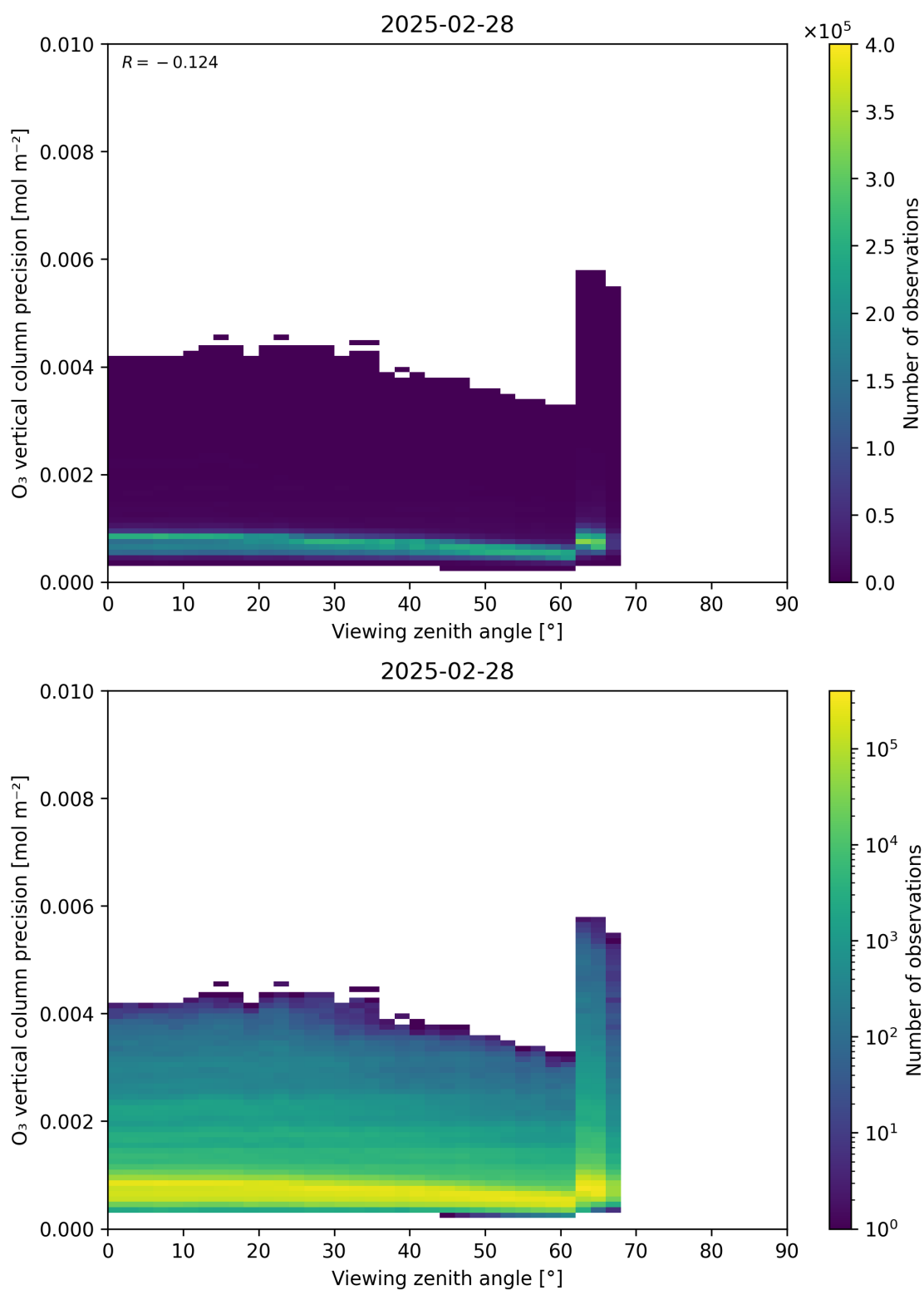
Figure 53: Scatter density plot of “Viewing zenith angle” against “O 3 vertical column precision” for 2025-02-27 to 2025-03-01.
