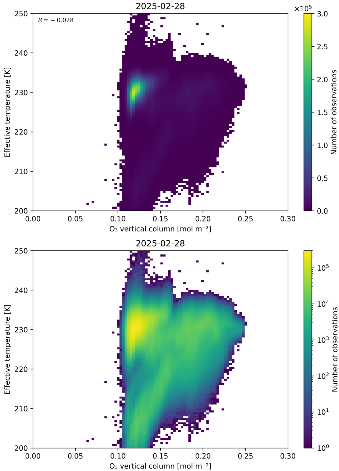
Figure 39: Scatter density plot of “O 3 vertical column” against “Effective temperature” for 2025-02-27 to 2025-03-01.
