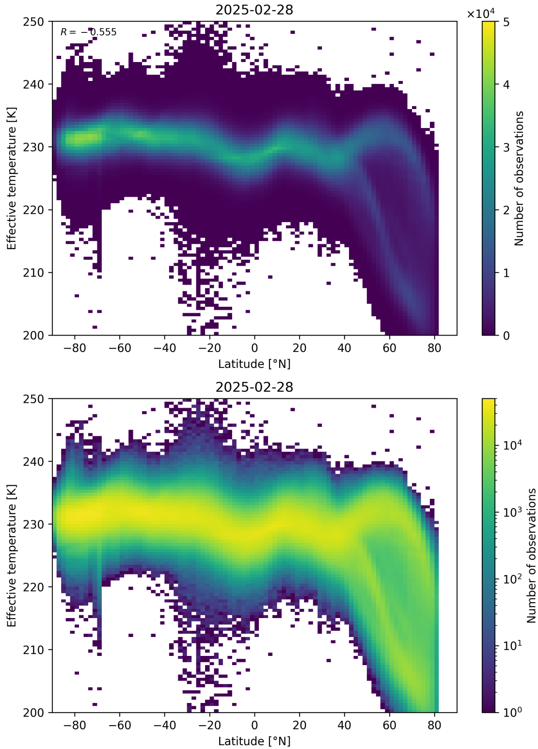
Figure 34: Scatter density plot of “Latitude” against “Effective temperature” for 2025-02-27 to 2025-03-01.
