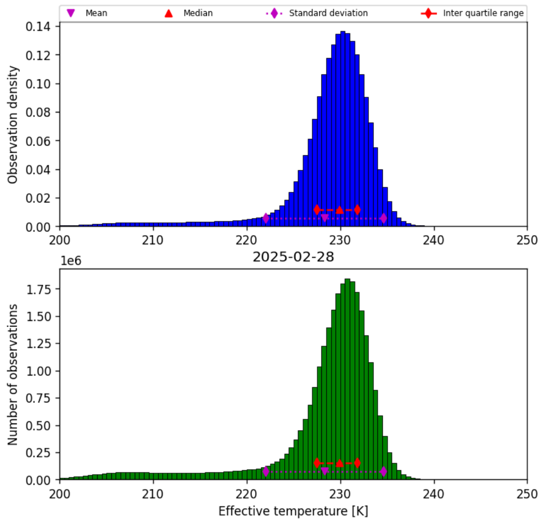
Figure 24: Histogram of “Effective temperature” for 2025-02-27 to 2025-03-01
