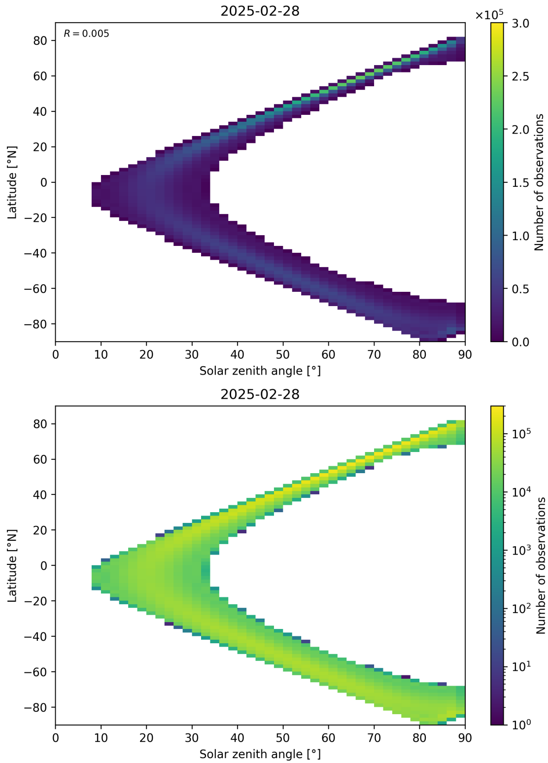
Figure 44: Scatter density plot of “Solar zenith angle” against “Latitude” for 2025-02-27 to 2025-03-01.
