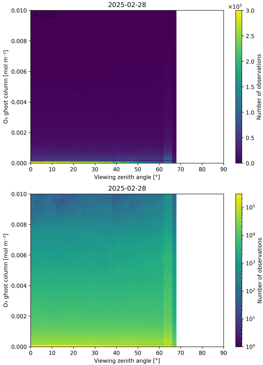
Figure 51: Scatter density plot of “Viewing zenith angle” against “O 3 ghost column” for 2025-02-27 to 2025-03-01.
