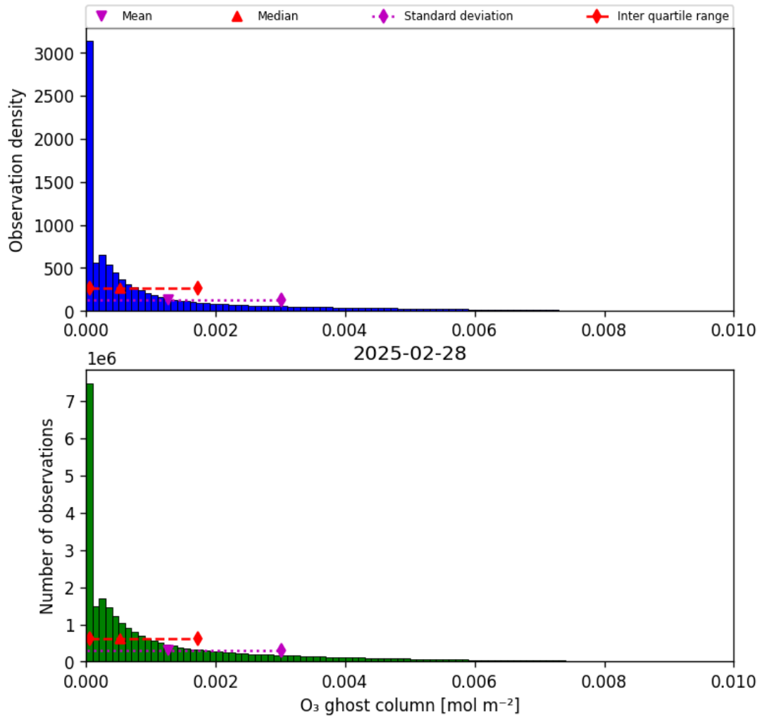
Figure 25: Histogram of "O 3 ghost column" for 2025-02-27 to 2025-03-01
