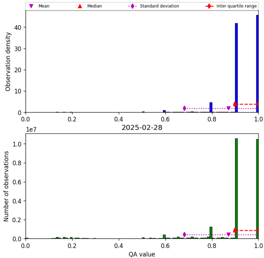
Figure 20: Histogram of “QA value” for 2025-02-27 to 2025-03-01
