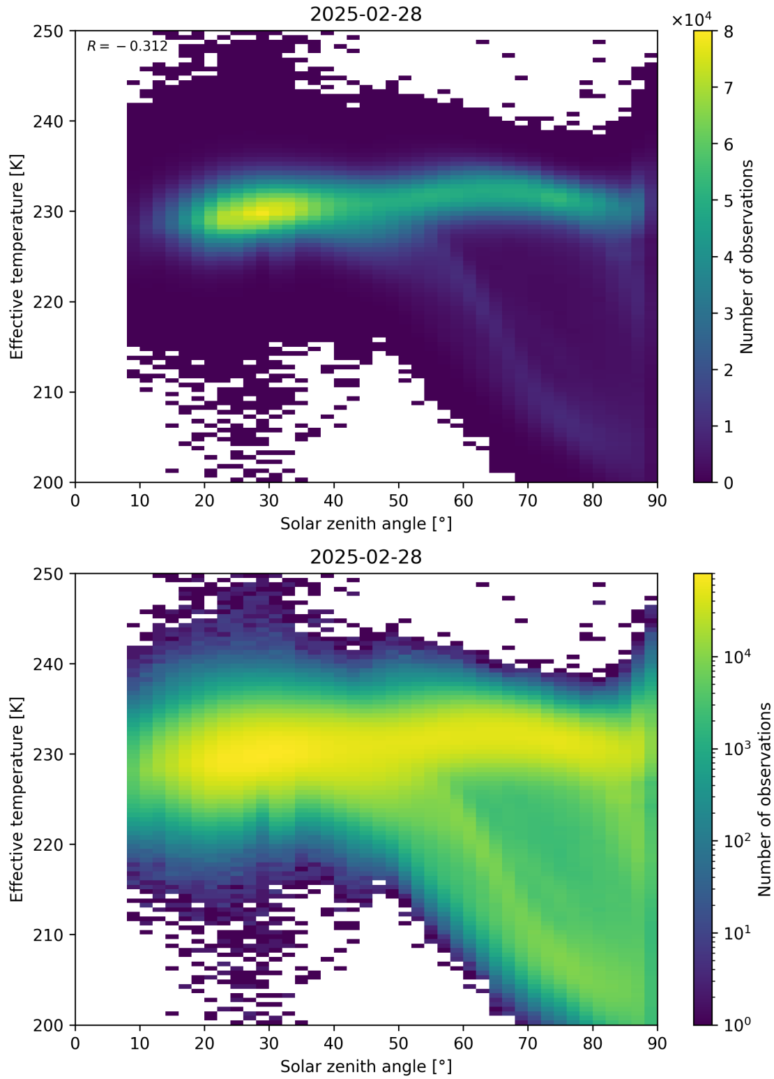
Figure 45: Scatter density plot of “Solar zenith angle” against “Effective temperature” for 2025-02-27 to 2025-03-01.
