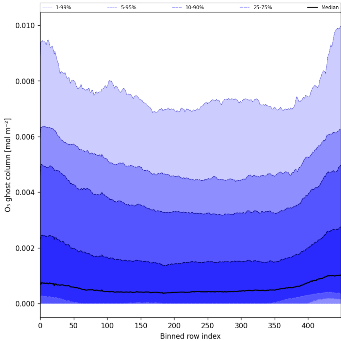
Figure 32: Along track statistics of “O 3 ghost column” for 2025-02-27 to 2025-03-01
