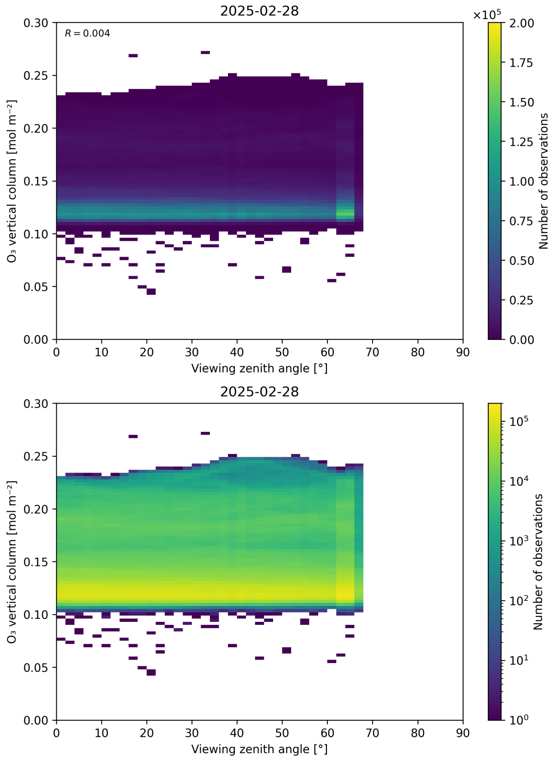
Figure 52: Scatter density plot of “Viewing zenith angle” against “O 3 vertical column” for 2025-02-27 to 2025-03-01.
