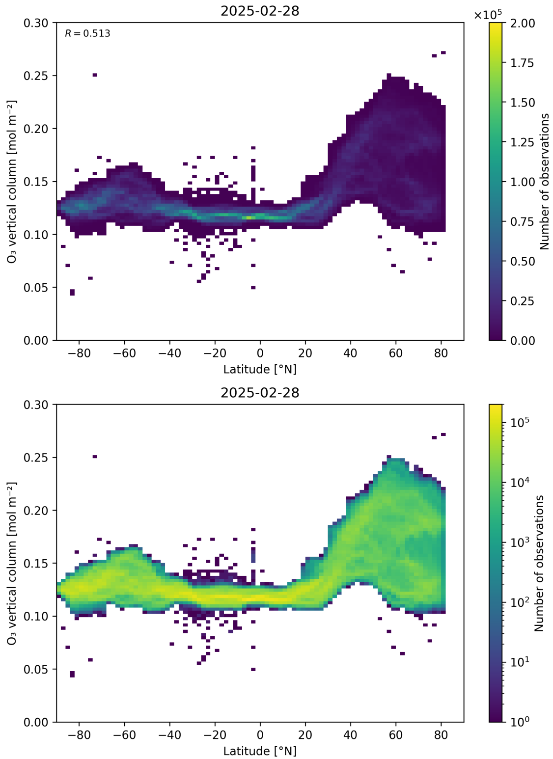
Figure 36: Scatter density plot of “Latitude” against “O 3 vertical column” for 2025-02-27 to 2025-03-01.
