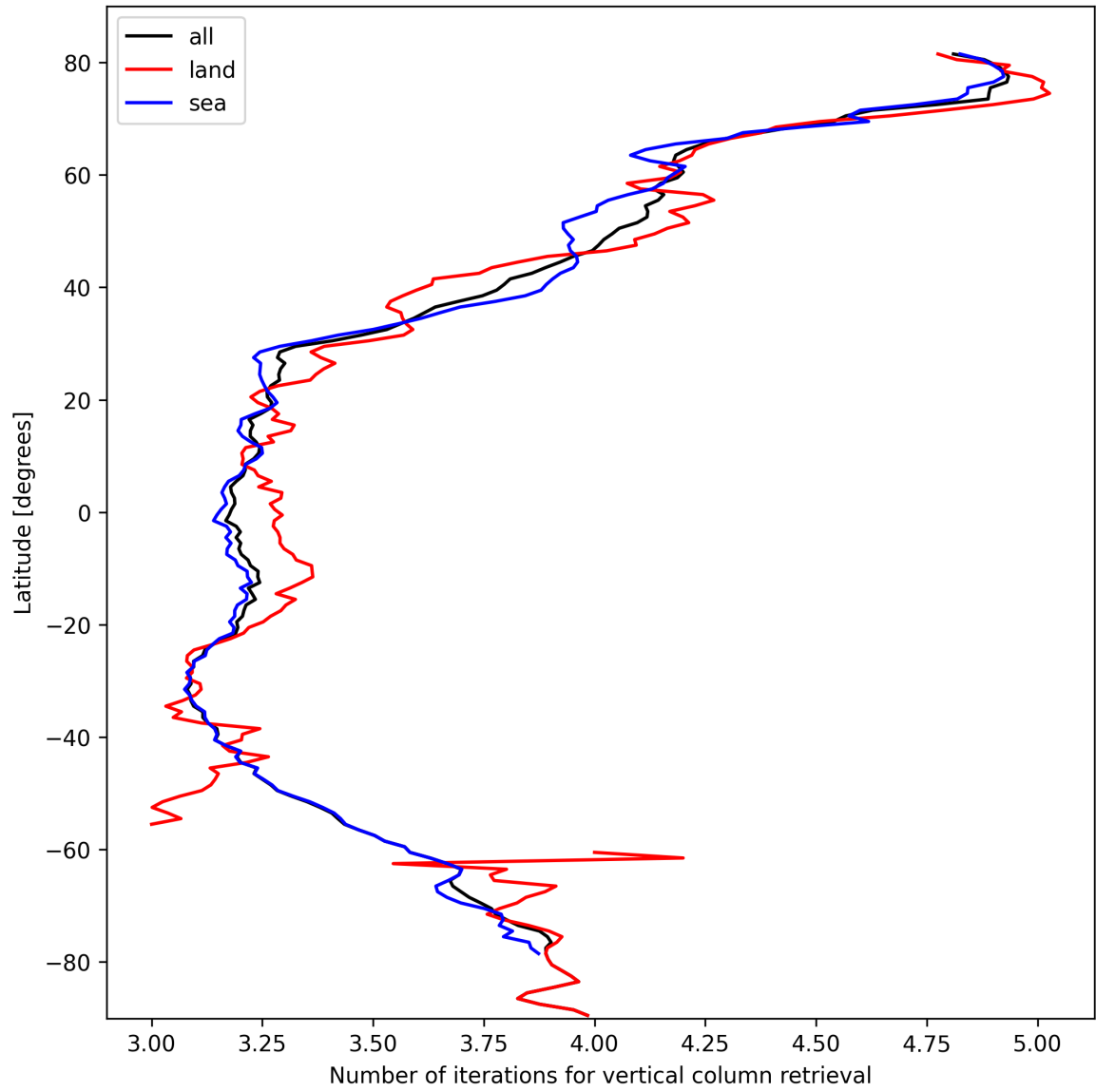
Figure 19: Zonal average of “Number of iterations for vertical column retrieval” for 2025-02-27 to 2025-03-01.
