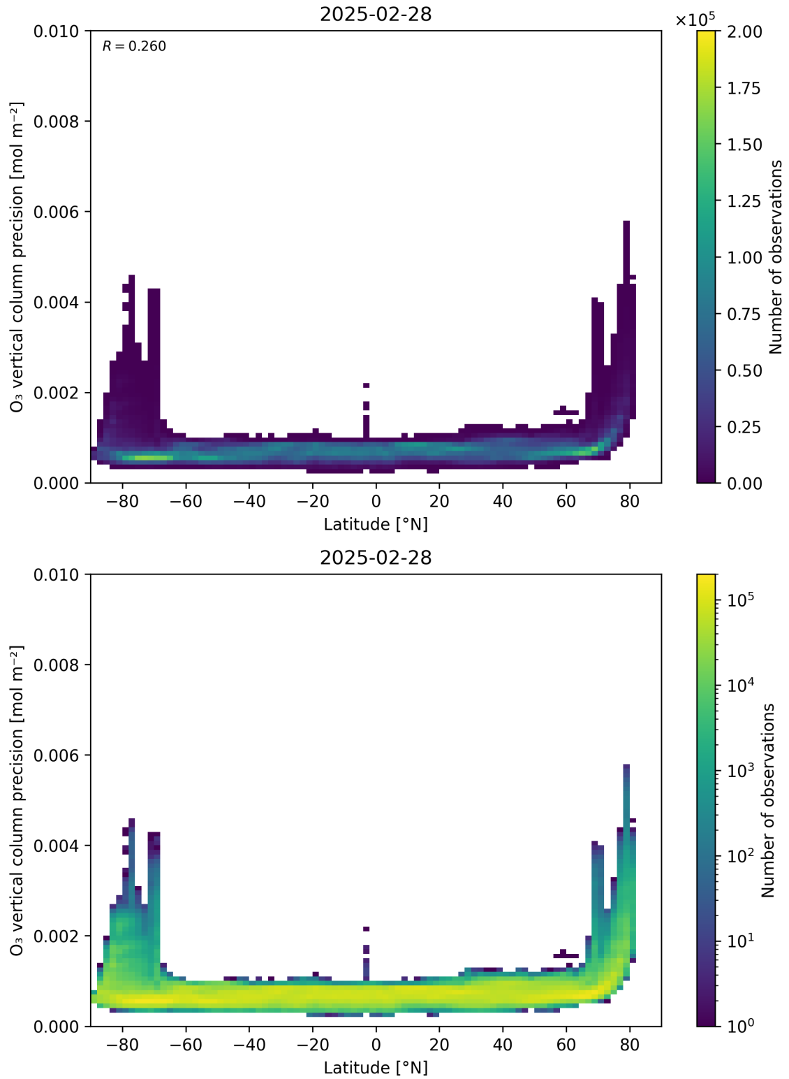
Figure 37: Scatter density plot of “Latitude” against “O 3 vertical column precision” for 2025-02-27 to 2025-03-01.
