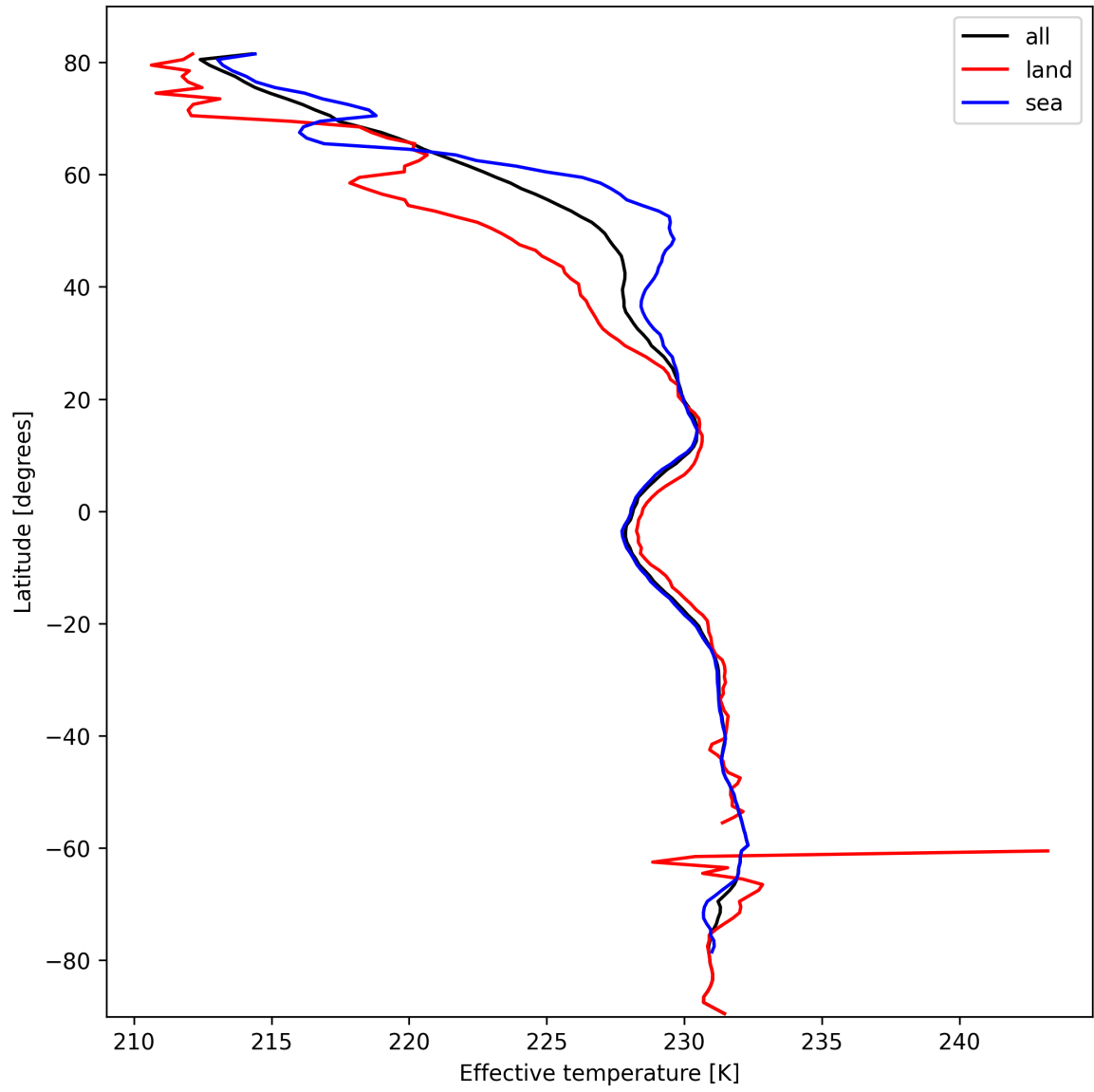
Figure 17: Zonal average of “Effective temperature” for 2025-02-27 to 2025-03-01.
