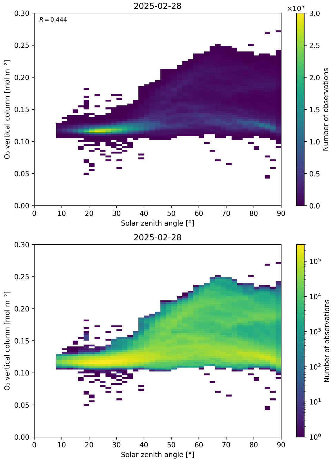
Figure 47: Scatter density plot of “Solar zenith angle” against “O 3 vertical column” for 2025-02-27 to 2025-03-01.
