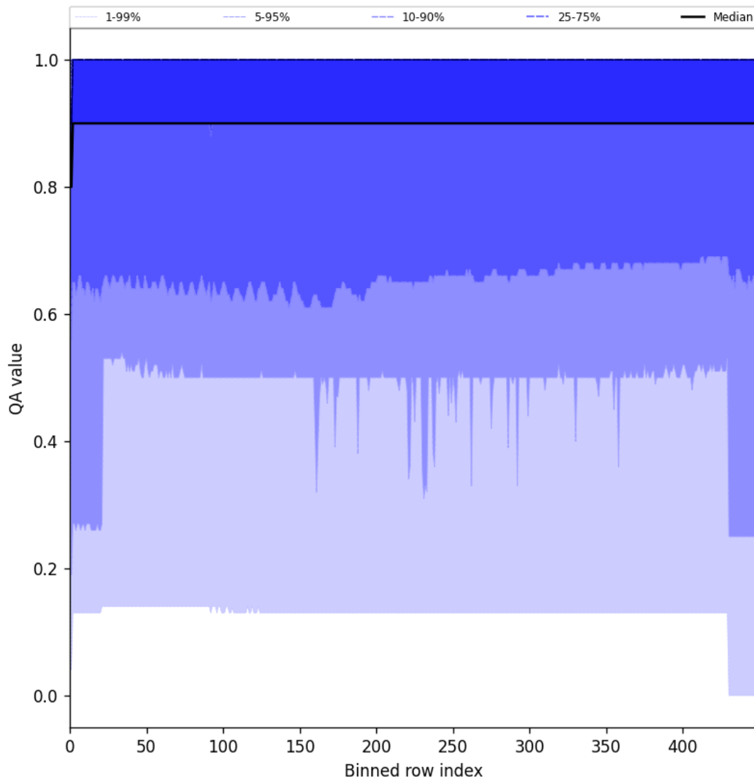
Figure 27: Along track statistics of “QA value” for 2025-02-27 to 2025-03-01
