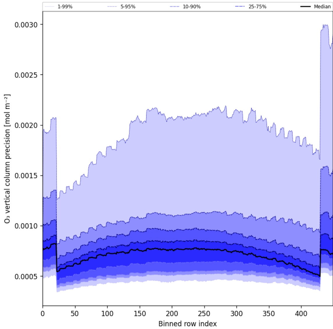
Figure 29: Along track statistics of “O 3 vertical column precision” for 2025-02-27 to 2025-03-01
