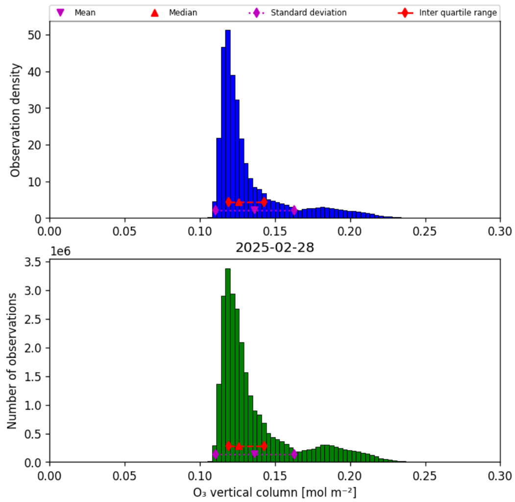
Figure 21: Histogram of “O 3 vertical column” for 2025-02-27 to 2025-03-01
