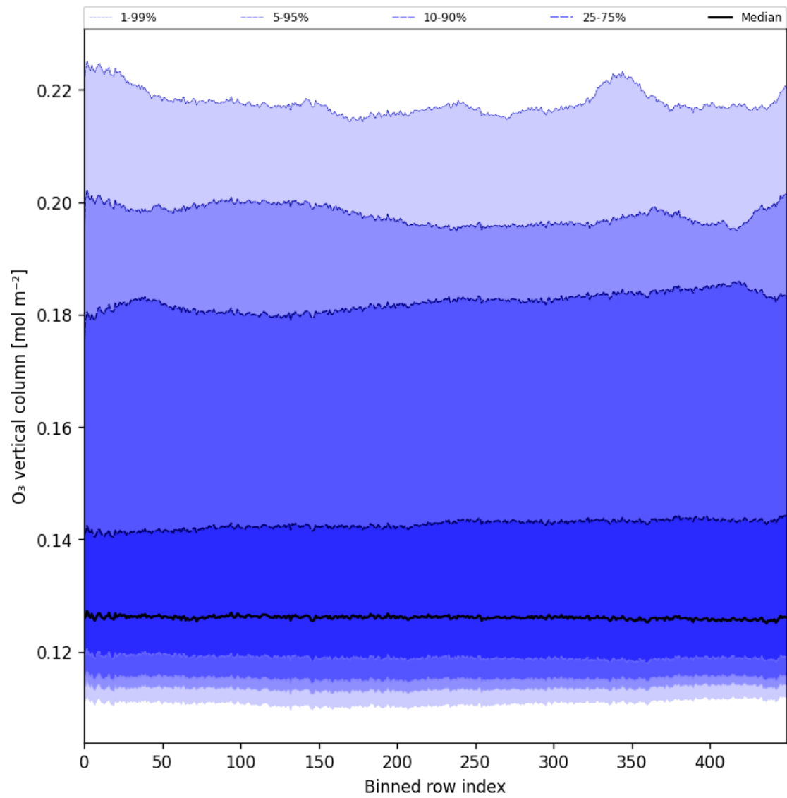
Figure 28: Along track statistics of “O 3 vertical column” for 2025-02-27 to 2025-03-01
