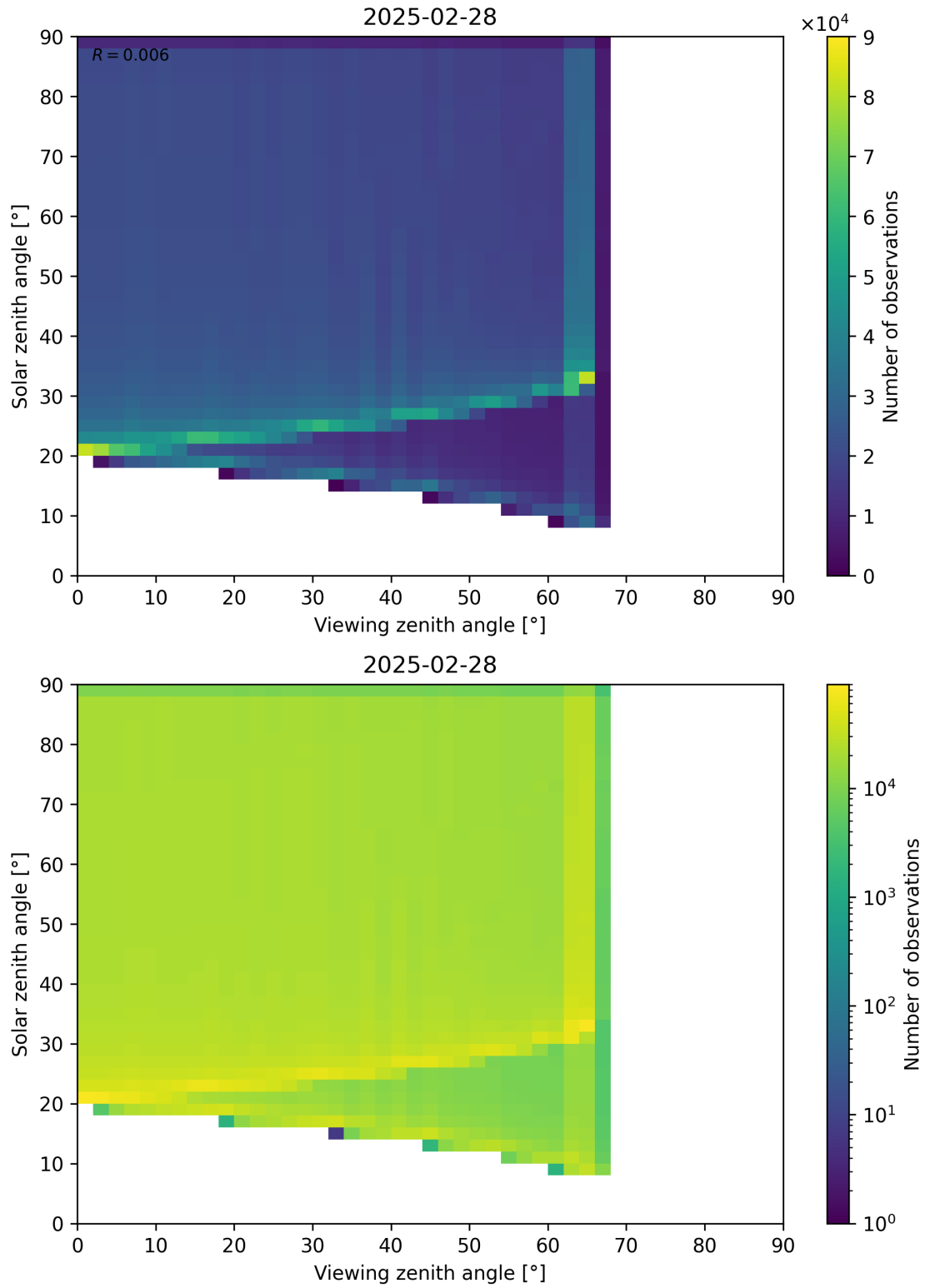
Figure 54: Scatter density plot of “Viewing zenith angle” against “Solar zenith angle” for 2025-02-27 to 2025-03-01.
