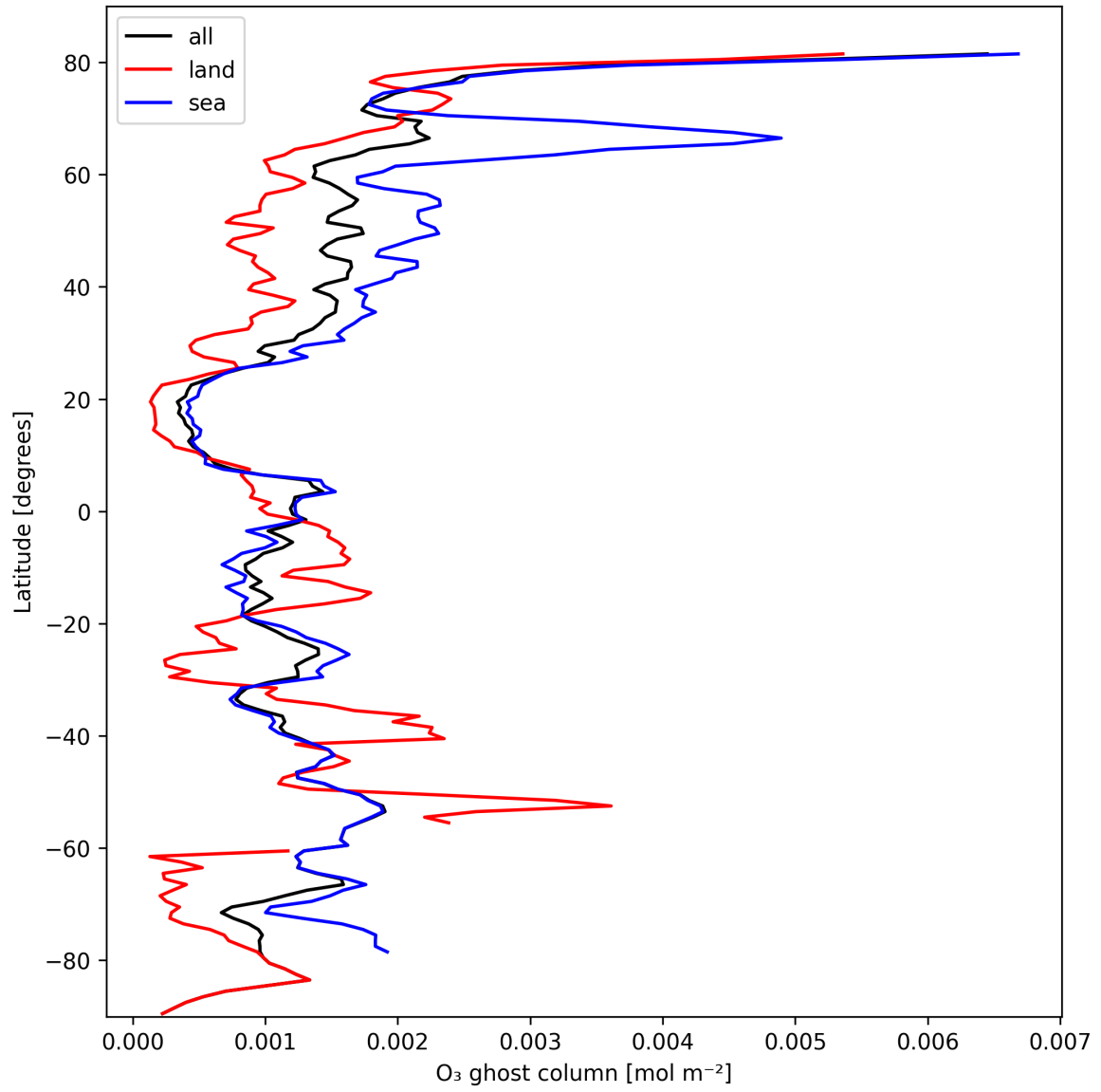
Figure 18: Zonal average of "O 3 ghost column" for 2025-02-27 to 2025-03-01.
