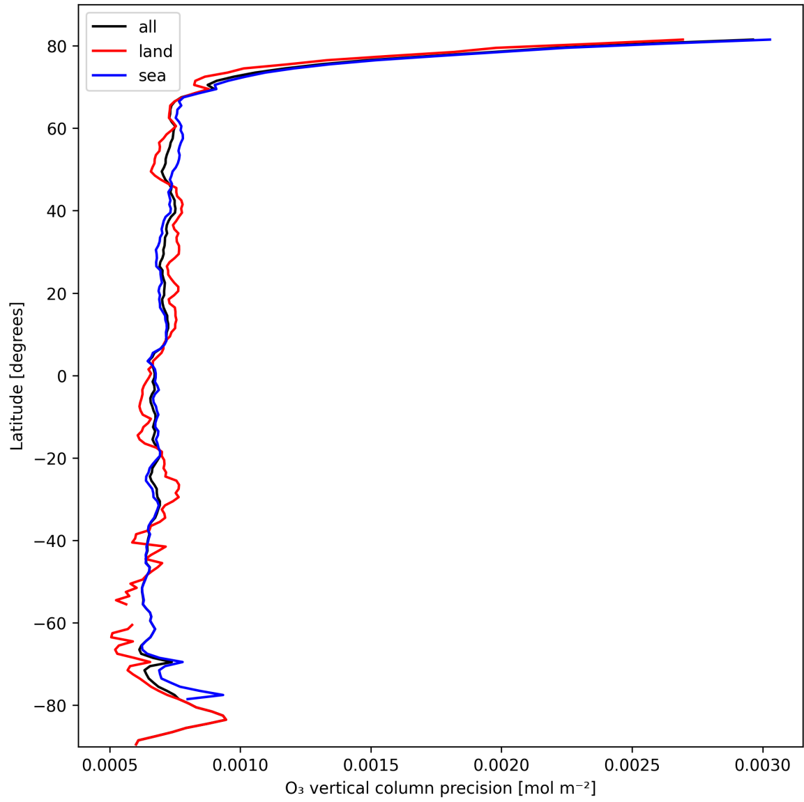
Figure 15: Zonal average of “O 3 vertical column precision” for 2025-02-27 to 2025-03-01.
