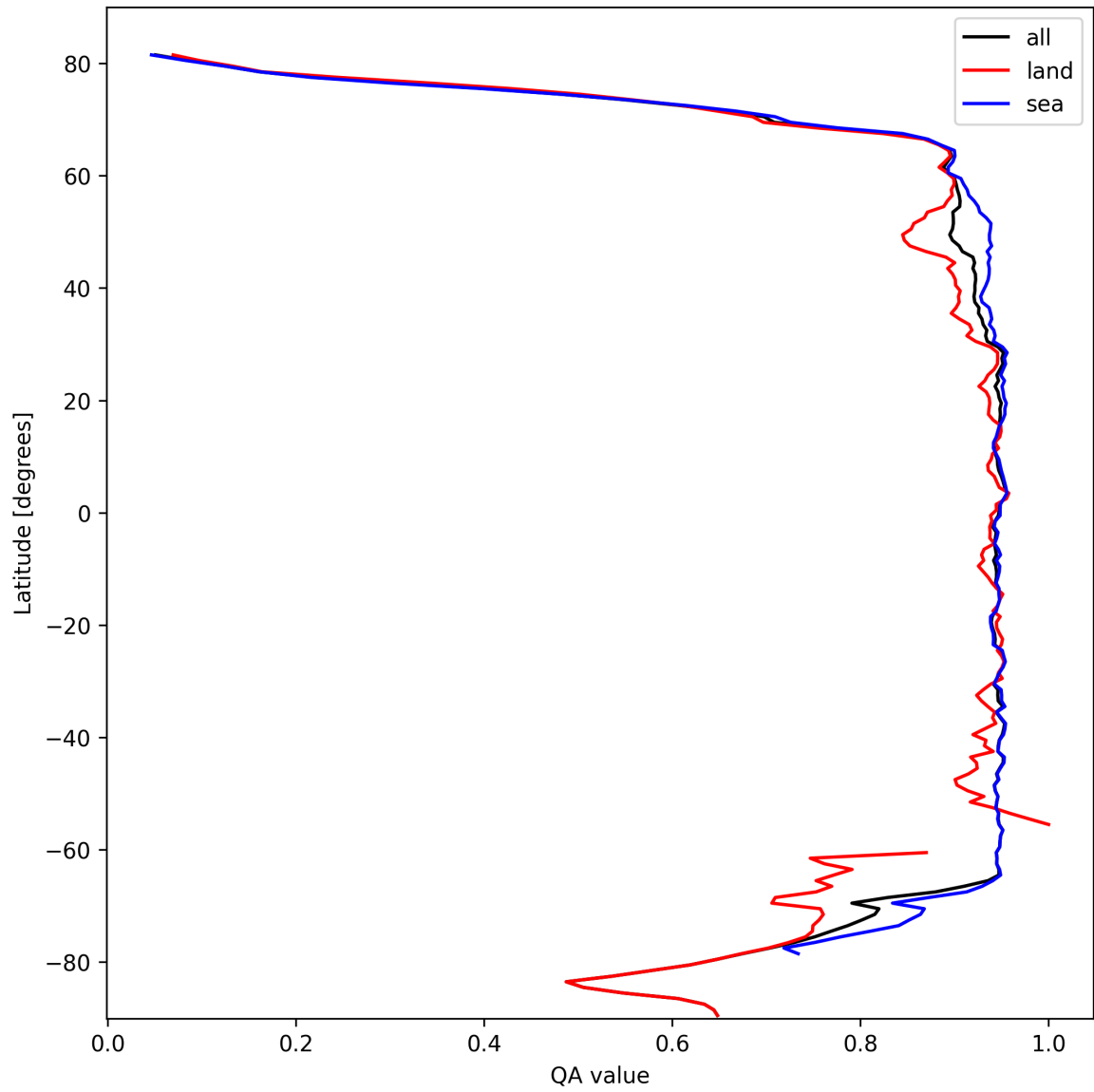
Figure 13: Zonal average of “QA value” for 2025-02-27 to 2025-03-01.
