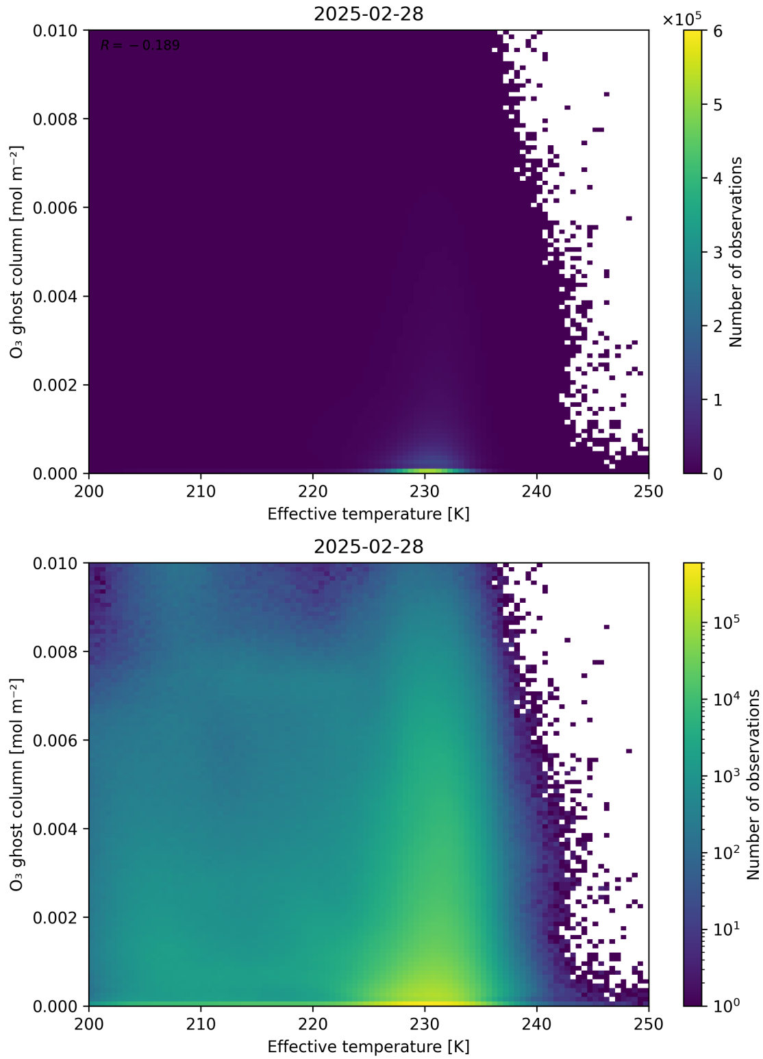
Figure 38: Scatter density plot of “Effective temperature” against “O 3 ghost column” for 2025-02-27 to 2025-03-01.
