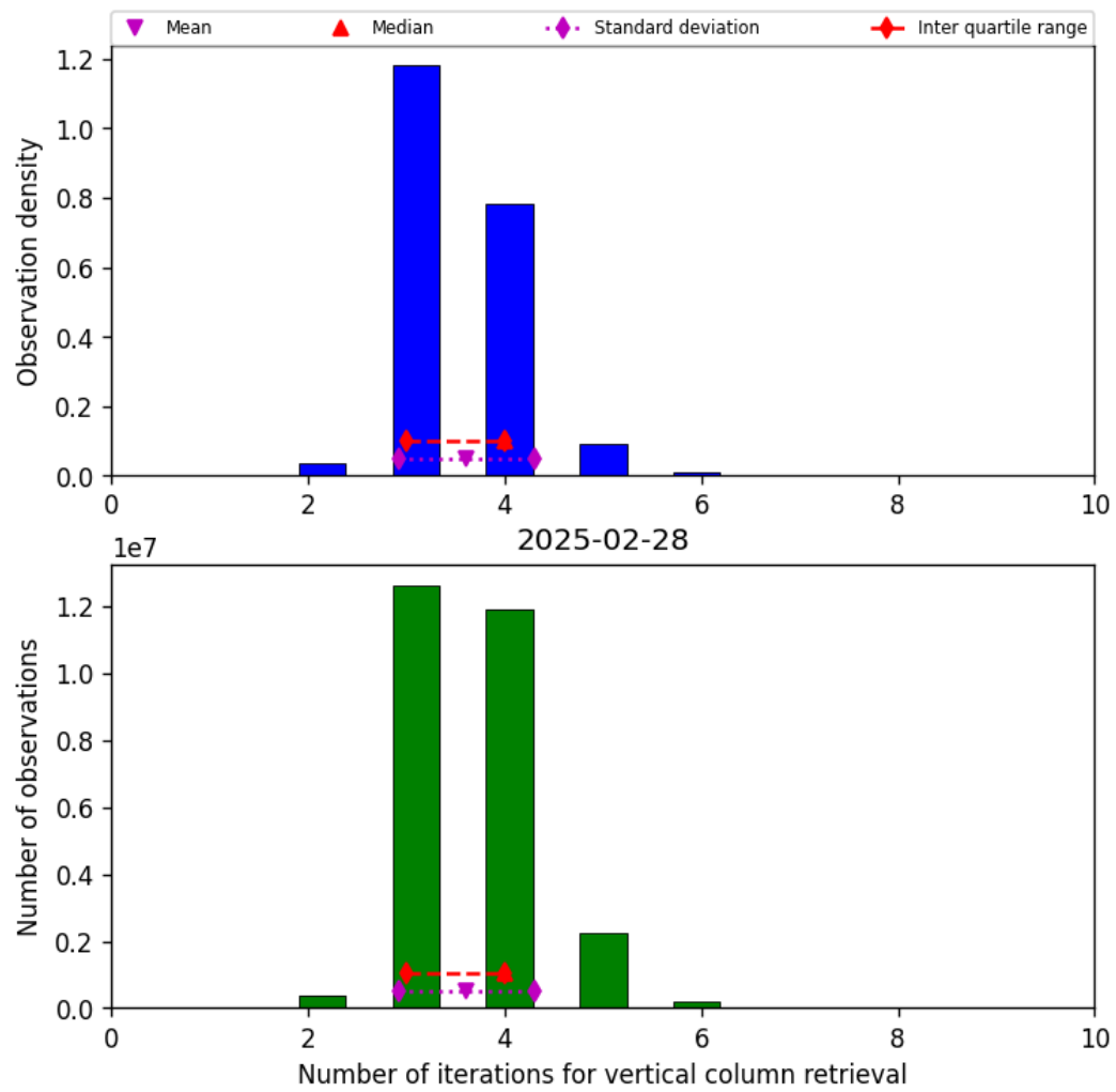
Figure 26: Histogram of “Number of iterations for vertical column retrieval” for 2025-02-27 to 2025-03-01
