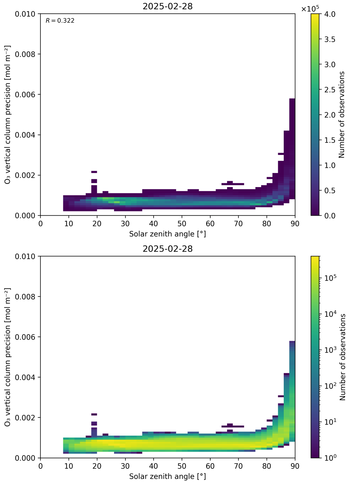
Figure 48: Scatter density plot of “Solar zenith angle” against “O 3 vertical column precision” for 2025-02-27 to 2025-03-01.
