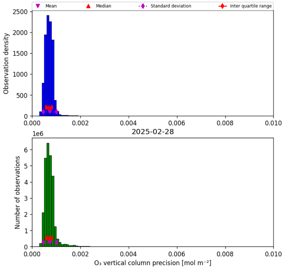
Figure 22: Histogram of “O 3 vertical column precision” for 2025-02-27 to 2025-03-01
