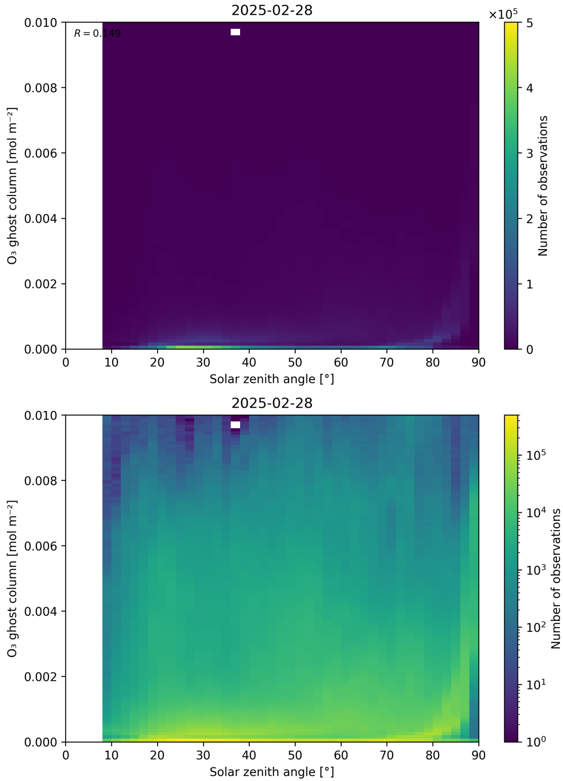
Figure 46: Scatter density plot of “Solar zenith angle” against “O 3 ghost column” for 2025-02-27 to 2025-03-01.
