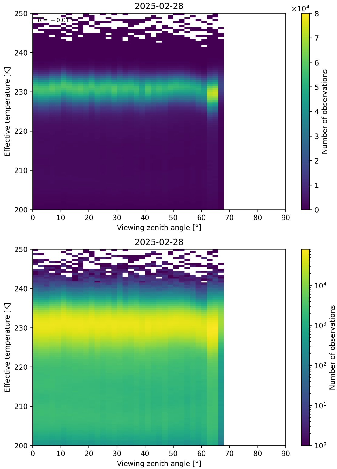
Figure 50: Scatter density plot of “Viewing zenith angle” against “Effective temperature” for 2025-02-27 to 2025-03-01.
