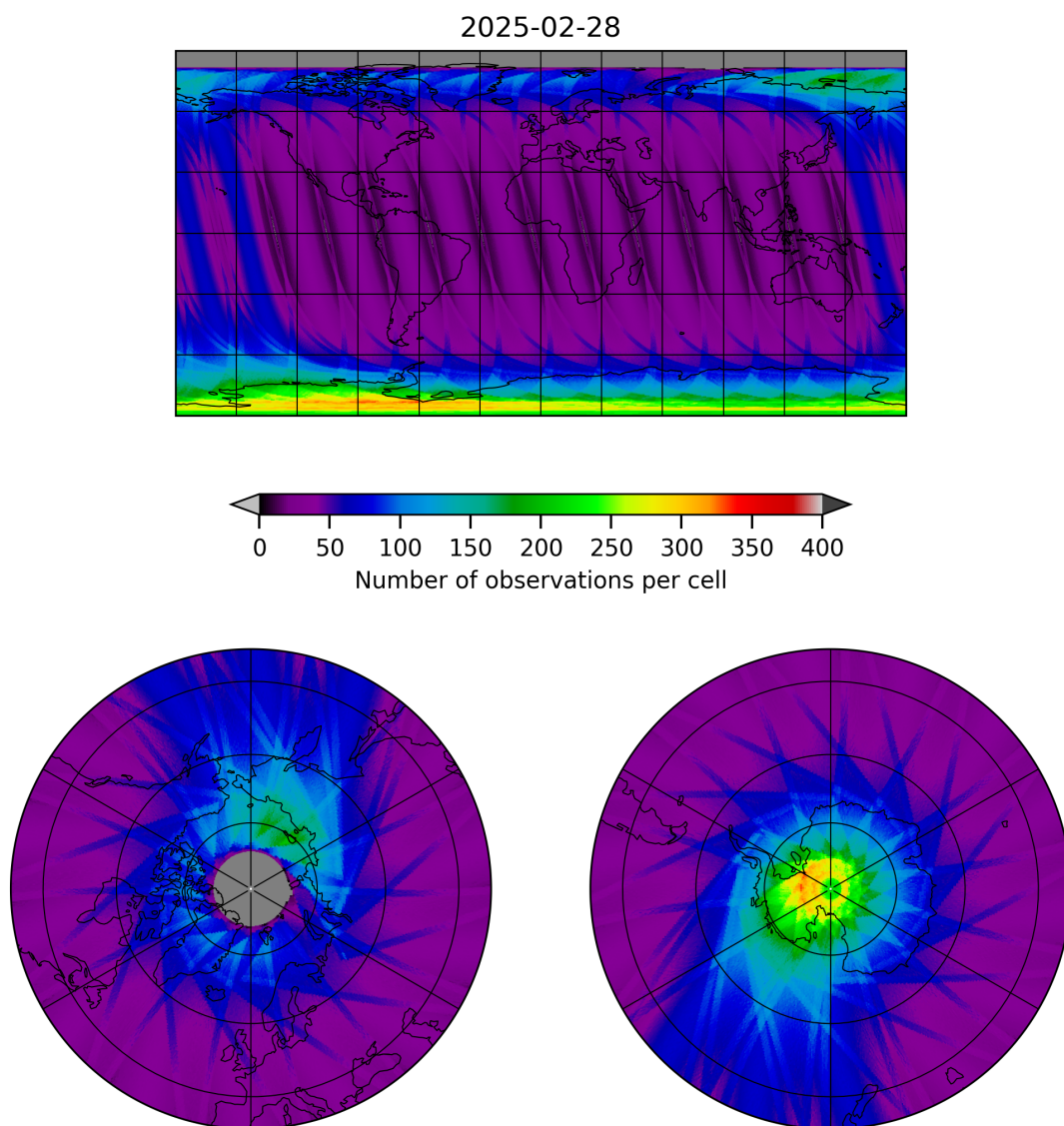
Figure 12: Map of the number of observations for 2025-02-27 to 2025-03-01
