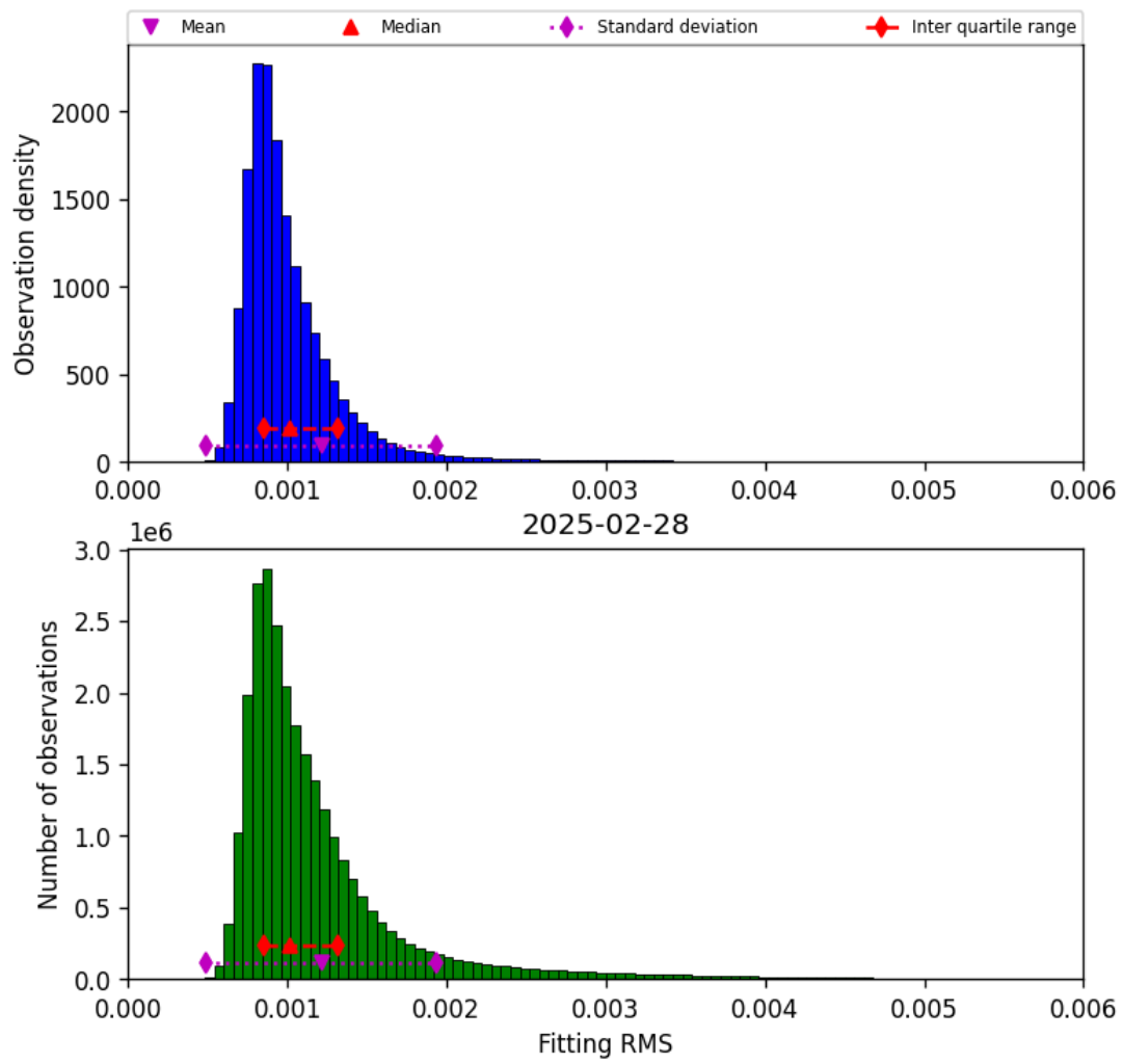
Figure 23: Histogram of “Fitting RMS” for 2025-02-27 to 2025-03-01
