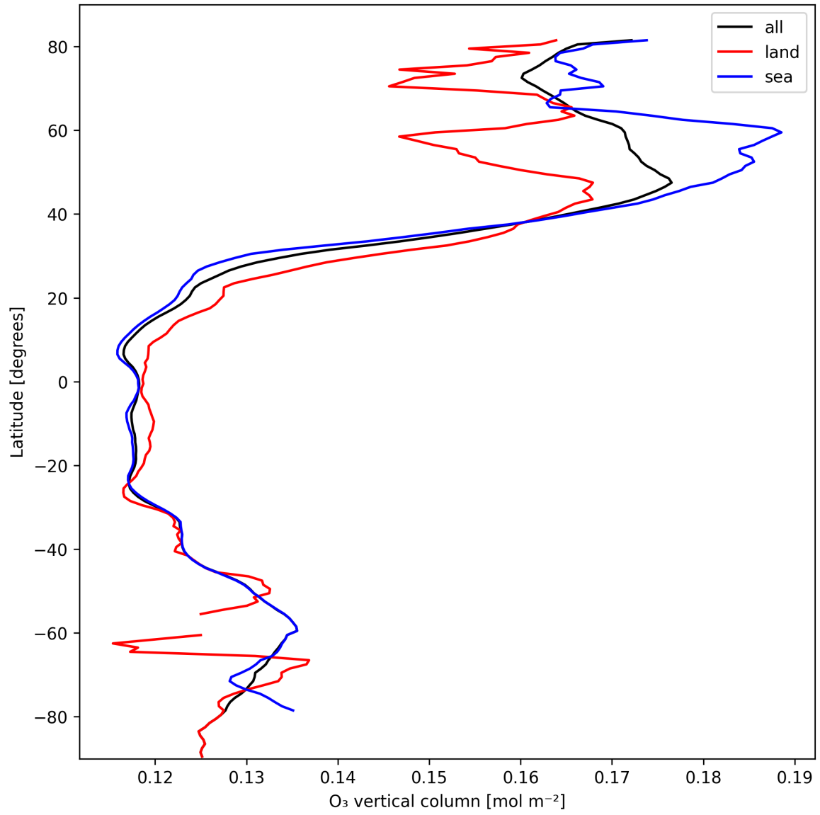
Figure 14: Zonal average of “O 3 vertical column” for 2025-03-01 to 2025-03-02.
