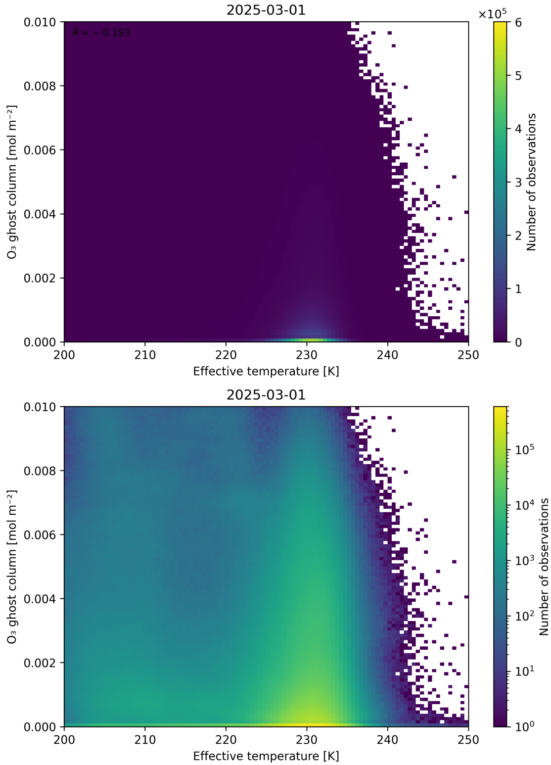
Figure 38: Scatter density plot of “Effective temperature” against “O 3 ghost column” for 2025-03-01 to 2025-03-02.
