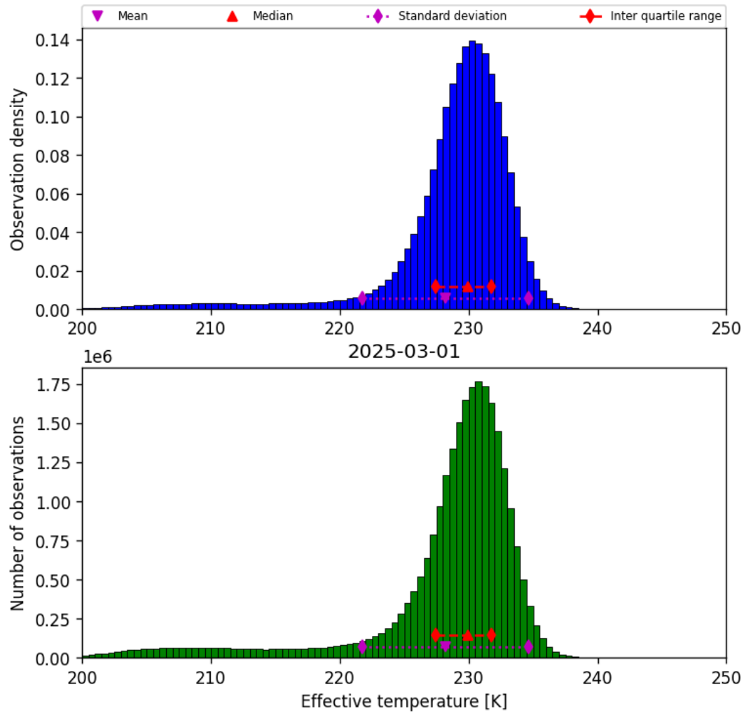
Figure 24: Histogram of “Effective temperature” for 2025-03-01 to 2025-03-02
