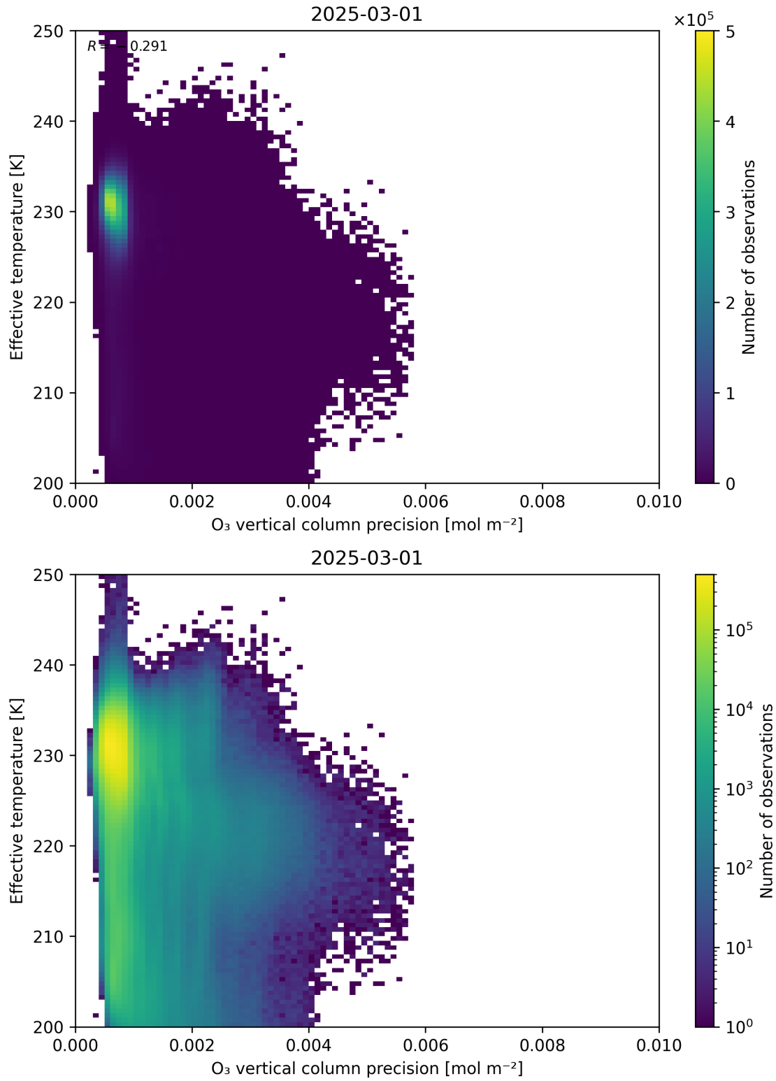
Figure 42: Scatter density plot of “O 3 vertical column precision” against “Effective temperature” for 2025-03-01 to 2025-03-02.
