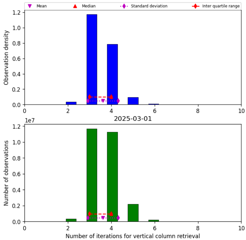
Figure 26: Histogram of “Number of iterations for vertical column retrieval” for 2025-03-01 to 2025-03-02
