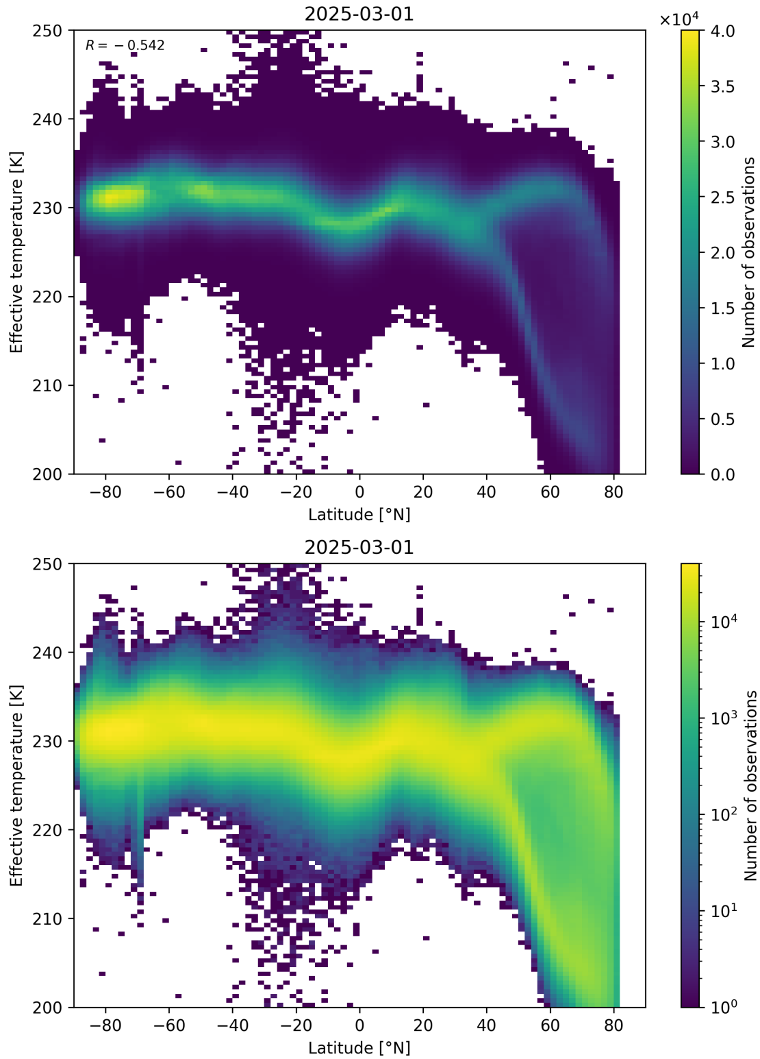
Figure 34: Scatter density plot of “Latitude” against “Effective temperature” for 2025-03-01 to 2025-03-02.
