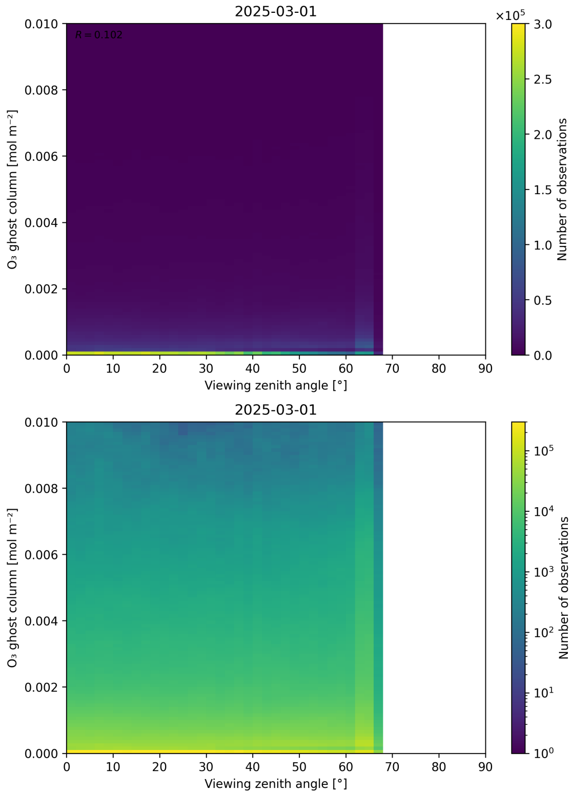
Figure 51: Scatter density plot of “Viewing zenith angle” against “O 3 ghost column” for 2025-03-01 to 2025-03-02.
