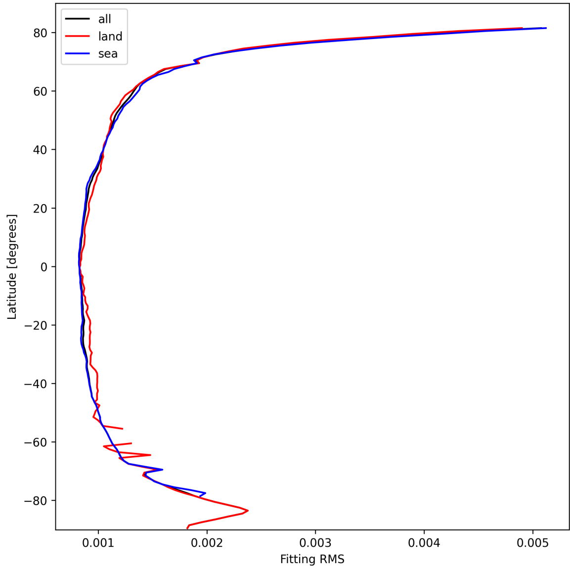
Figure 16: Zonal average of “Fitting RMS” for 2025-03-01 to 2025-03-02.
