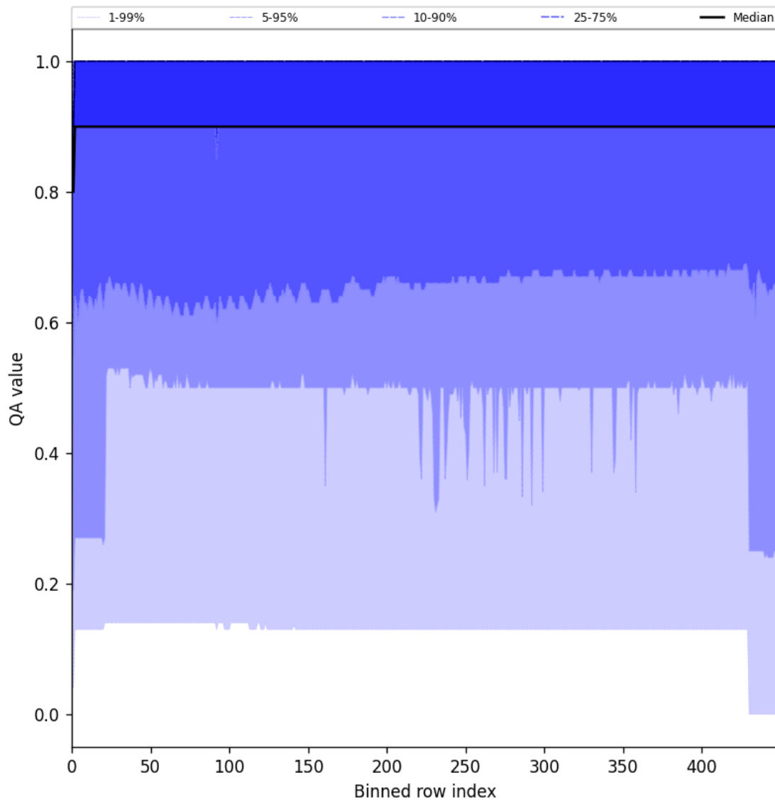
Figure 27: Along track statistics of “QA value” for 2025-03-01 to 2025-03-02
