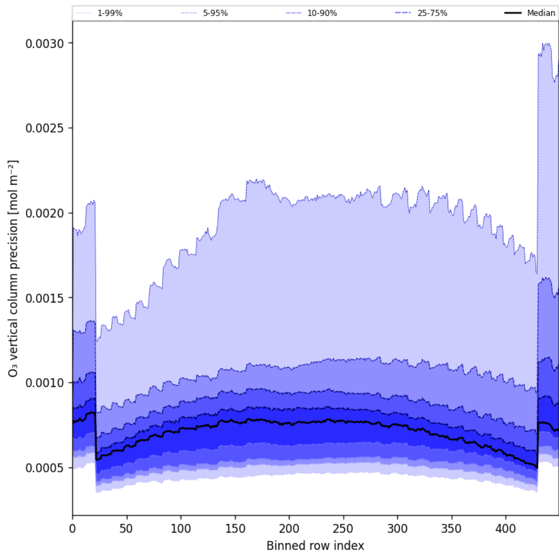
Figure 29: Along track statistics of “O 3 vertical column precision” for 2025-03-01 to 2025-03-02
