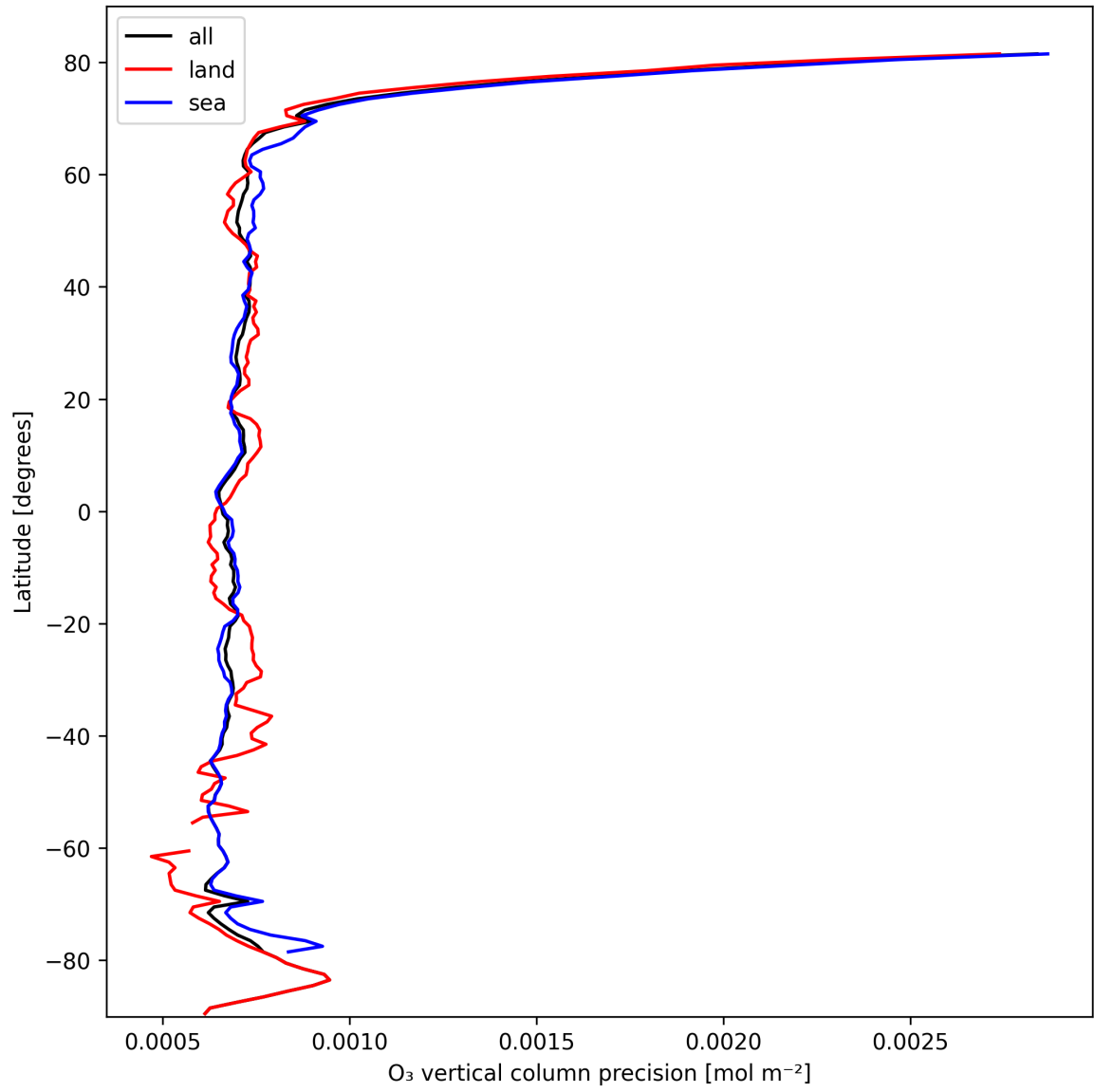
Figure 15: Zonal average of “O 3 vertical column precision” for 2025-03-01 to 2025-03-02.
