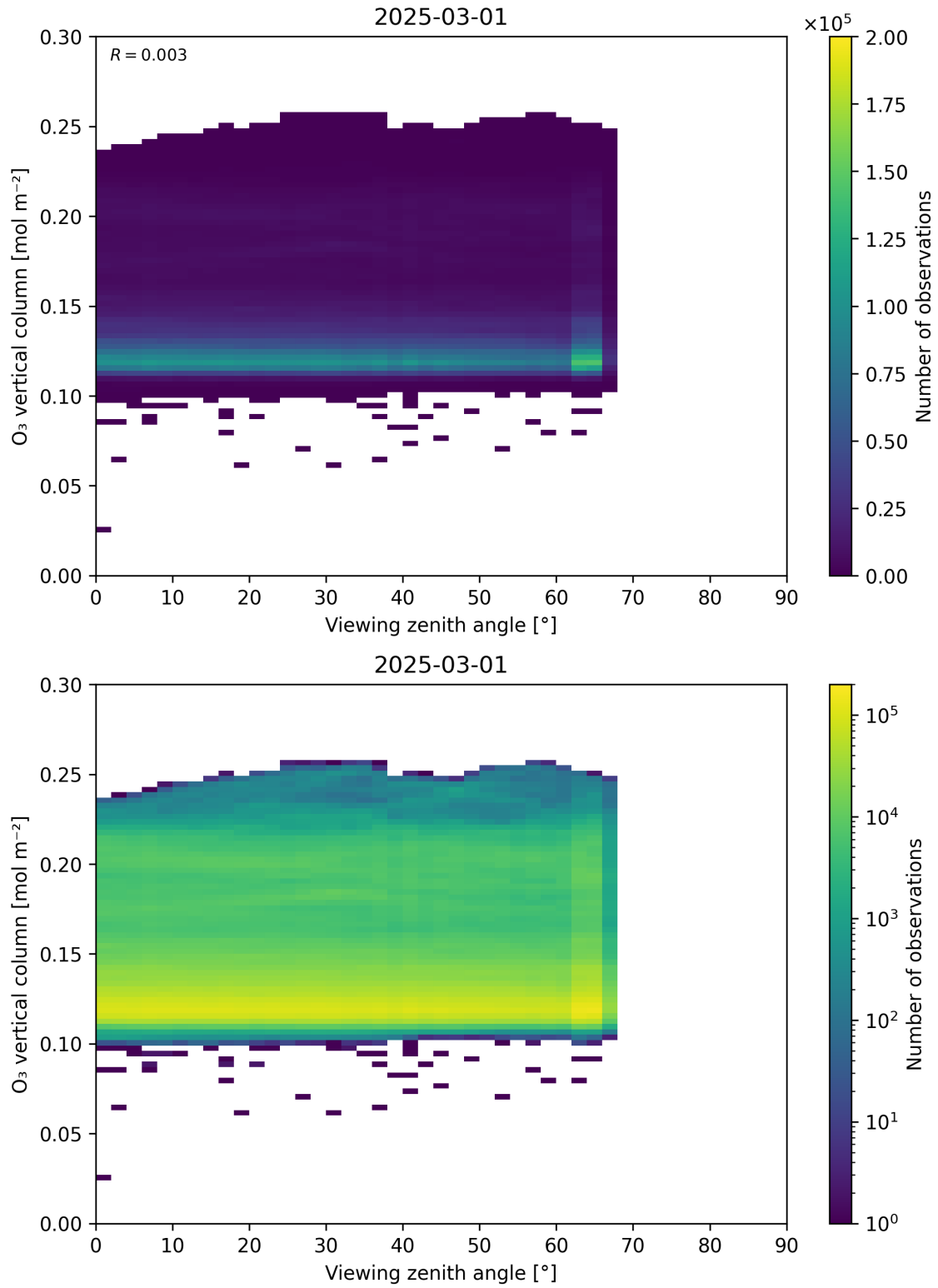
Figure 52: Scatter density plot of “Viewing zenith angle” against “O 3 vertical column” for 2025-03-01 to 2025-03-02.
