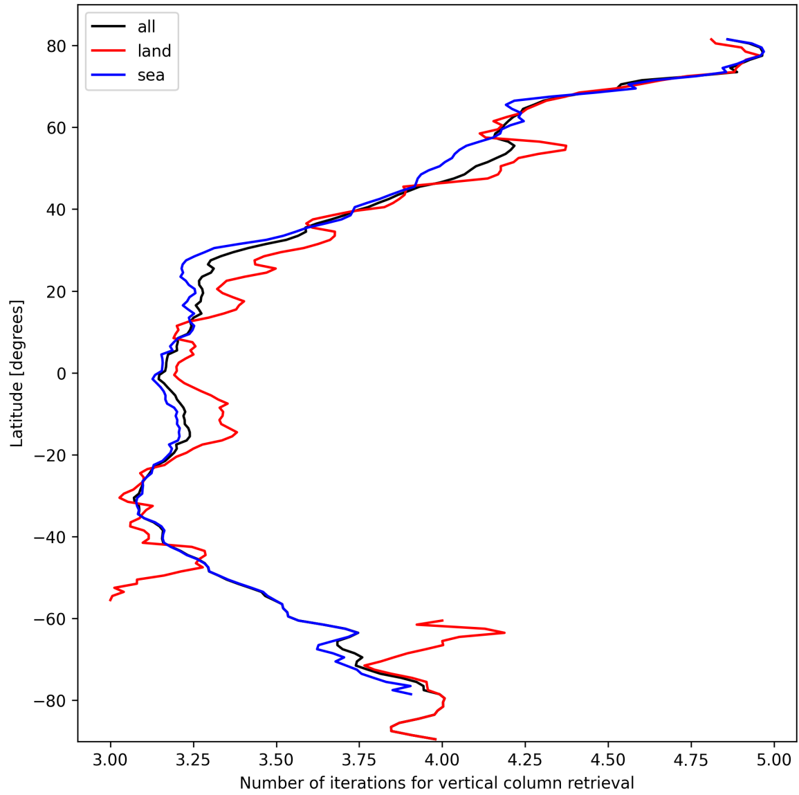
Figure 19: Zonal average of “Number of iterations for vertical column retrieval” for 2025-03-01 to 2025-03-02.
