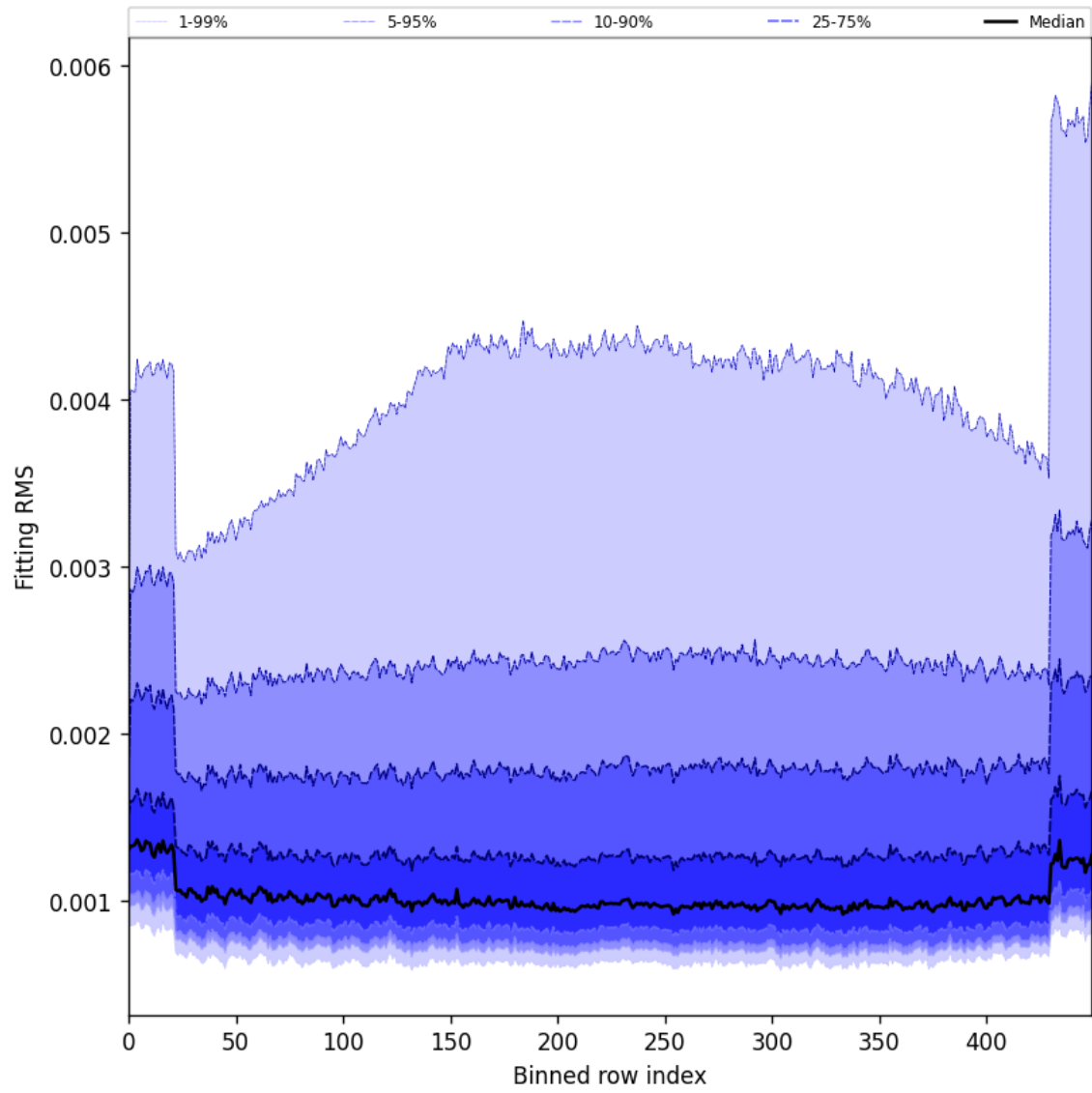
Figure 30: Along track statistics of “Fitting RMS” for 2025-03-01 to 2025-03-02
