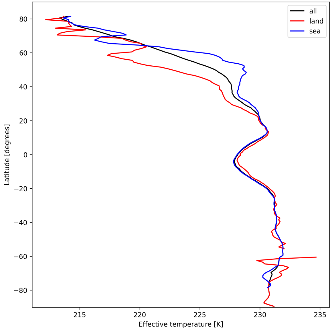
Figure 17: Zonal average of “Effective temperature” for 2025-03-01 to 2025-03-02.
