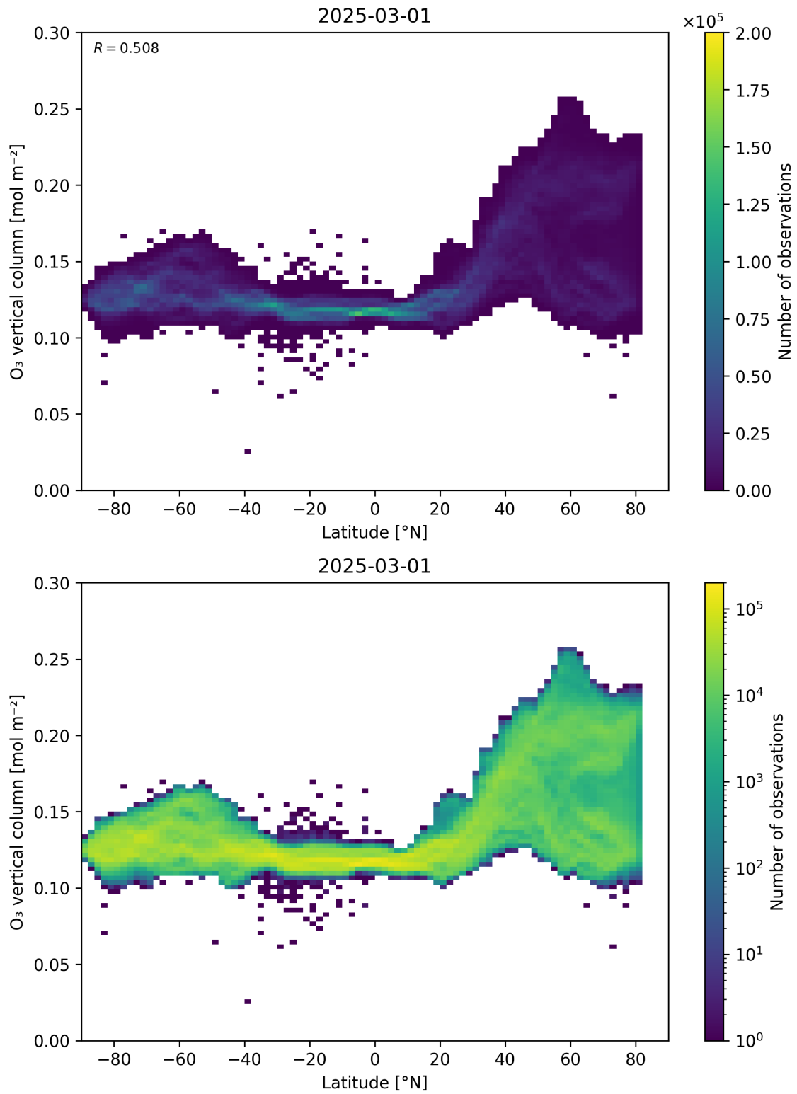
Figure 36: Scatter density plot of “Latitude” against “O 3 vertical column” for 2025-03-01 to 2025-03-02.
