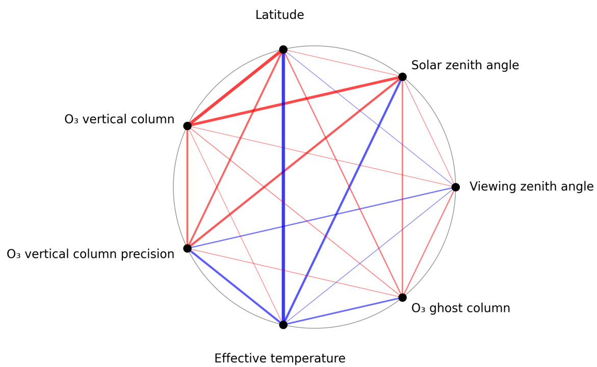
Figure 1: Map of correlation graph for 2025-03-01 to 2025-03-02.
