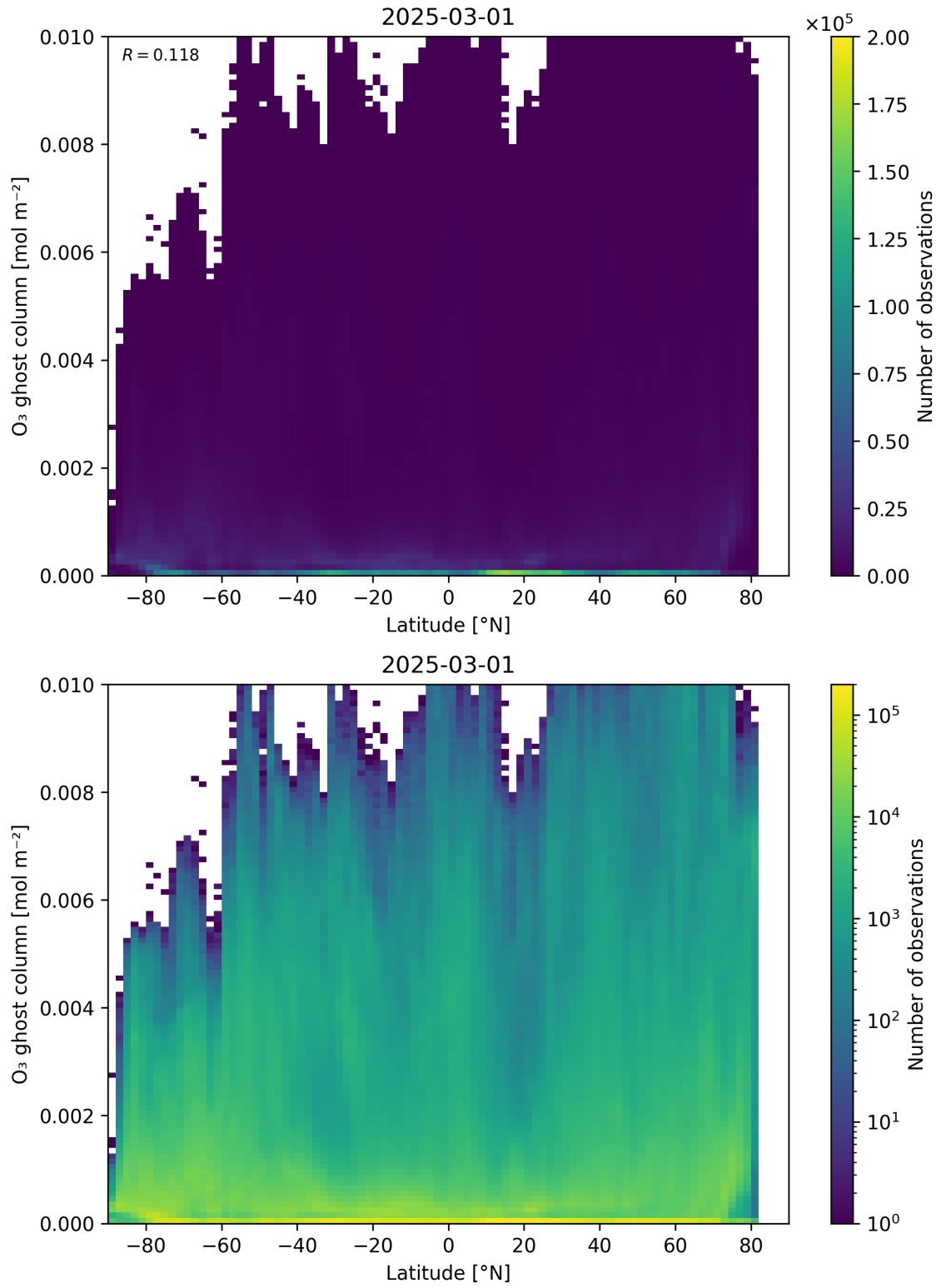
Figure 35: Scatter density plot of “Latitude” against “O 3 ghost column” for 2025-03-01 to 2025-03-02.
