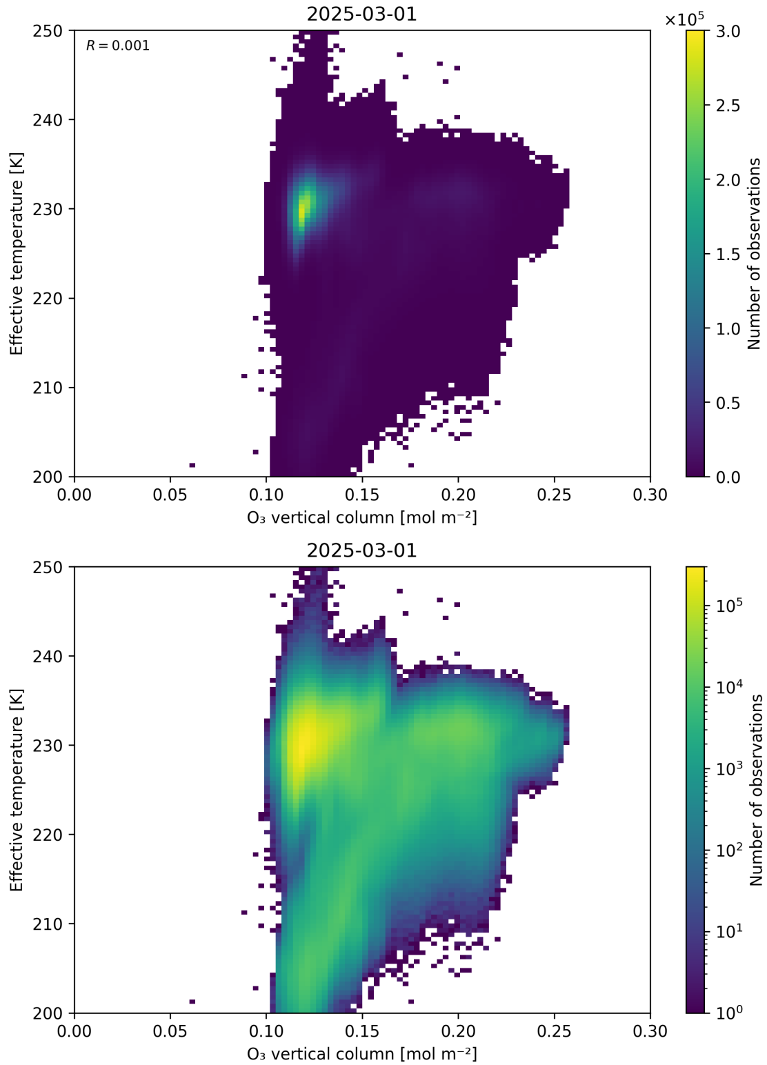
Figure 39: Scatter density plot of “O 3 vertical column” against “Effective temperature” for 2025-03-01 to 2025-03-02.
