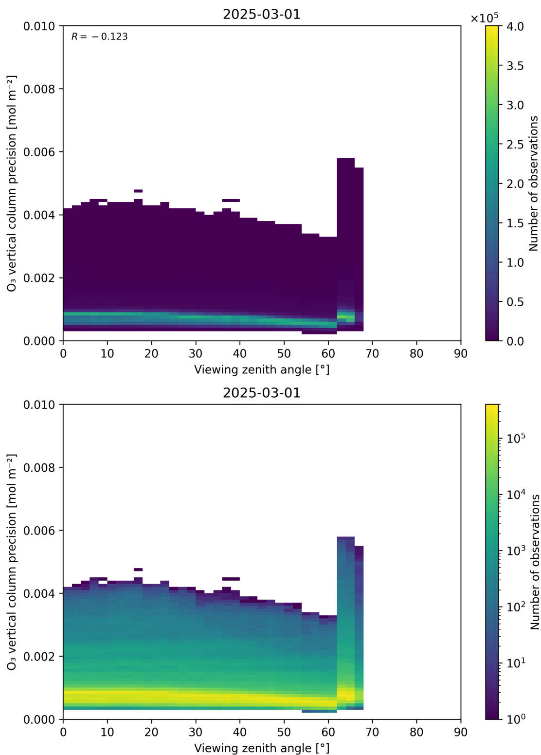
Figure 53: Scatter density plot of “Viewing zenith angle” against “O 3 vertical column precision” for 2025-03-01 to 2025-03-02.
