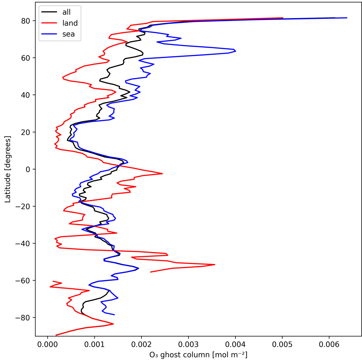
Figure 18: Zonal average of "O 3 ghost column" for 2025-03-01 to 2025-03-02.
