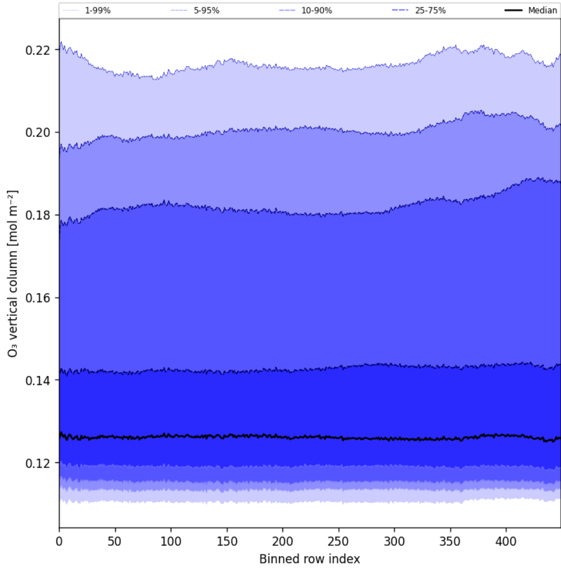
Figure 28: Along track statistics of "O 3 vertical column" for 2025-03-01 to 2025-03-02
