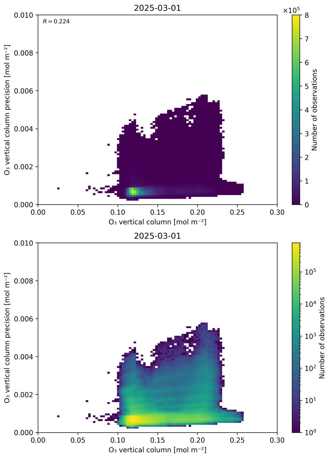
Figure 41: Scatter density plot of “O 3 vertical column” against “O 3 vertical column precision” for 2025-03-01 to 2025-03-02.
