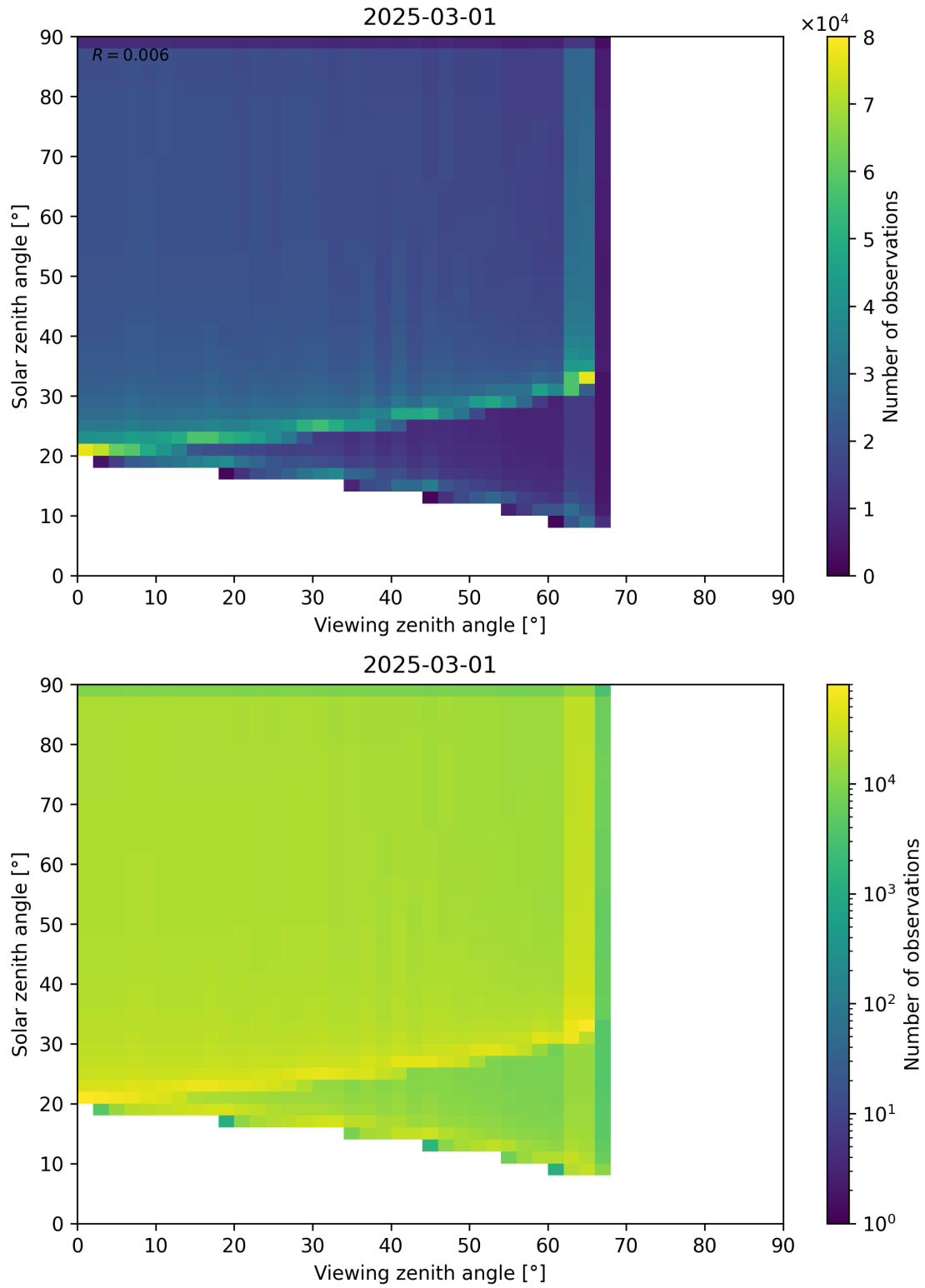
Figure 54: Scatter density plot of “Viewing zenith angle” against “Solar zenith angle” for 2025-03-01 to 2025-03-02.
