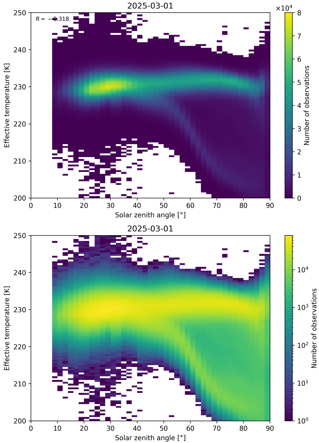
Figure 45: Scatter density plot of “Solar zenith angle” against “Effective temperature” for 2025-03-01 to 2025-03-02.
