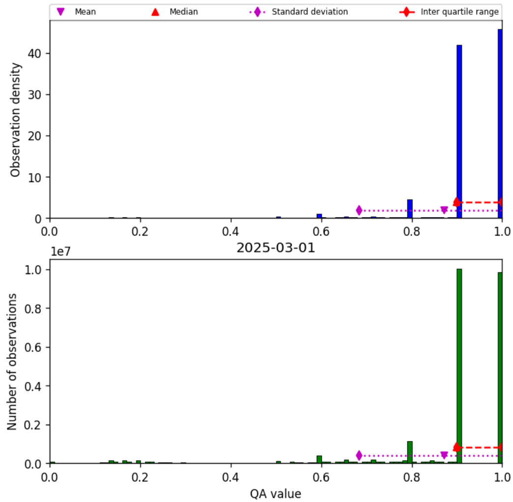
Figure 20: Histogram of “QA value” for 2025-03-01 to 2025-03-02
