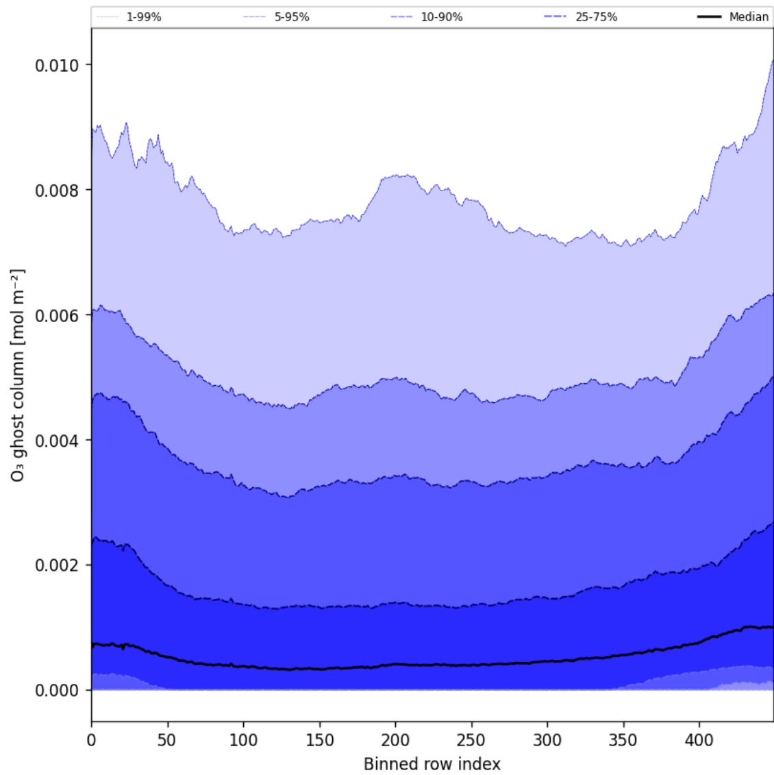
Figure 32: Along track statistics of “O 3 ghost column” for 2025-03-01 to 2025-03-02
