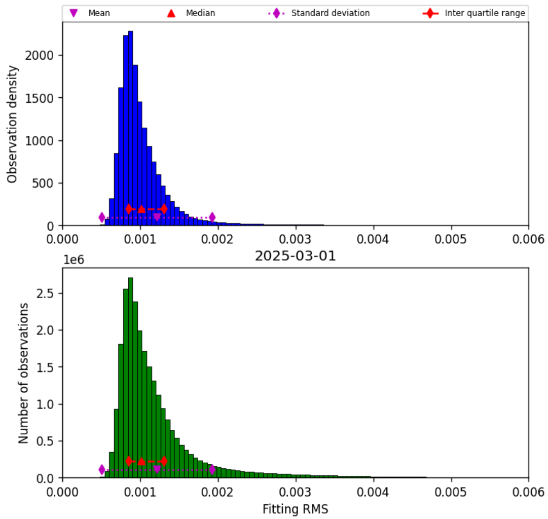
Figure 23: Histogram of “Fitting RMS” for 2025-03-01 to 2025-03-02
