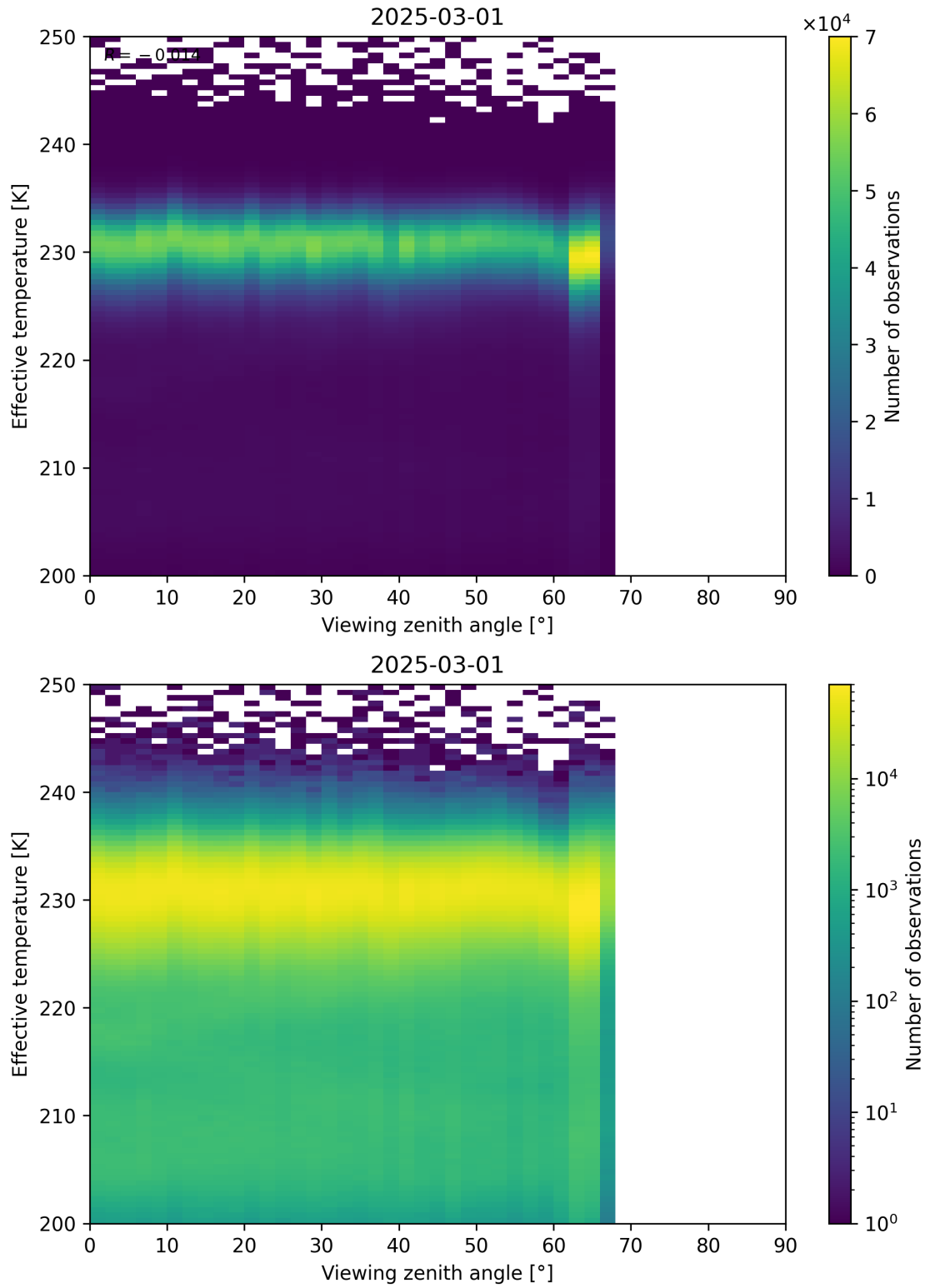
Figure 50: Scatter density plot of “Viewing zenith angle” against “Effective temperature” for 2025-03-01 to 2025-03-02.
