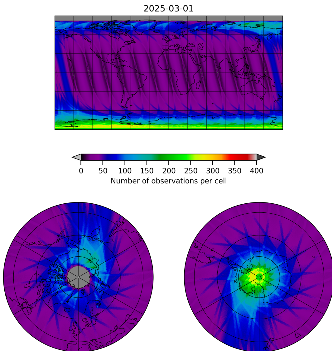
Figure 12: Map of the number of observations for 2025-03-01 to 2025-03-02
