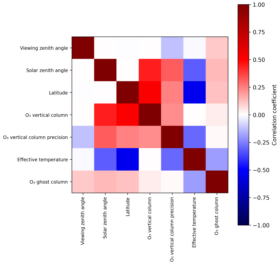
Figure 2: Map of correlation matrix for 2025-03-01 to 2025-03-02.
