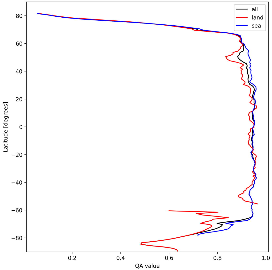
Figure 13: Zonal average of “QA value” for 2025-03-01 to 2025-03-02.
