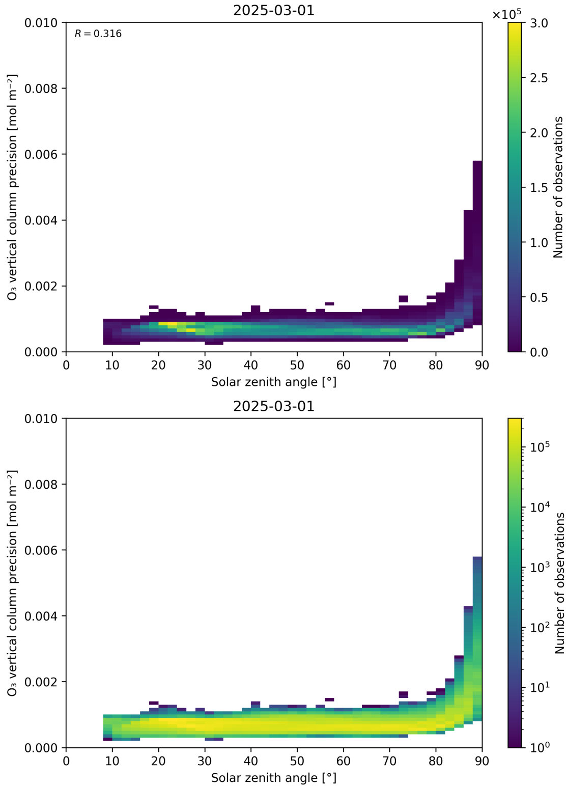
Figure 48: Scatter density plot of “Solar zenith angle” against “O 3 vertical column precision” for 2025-03-01 to 2025-03-02.
