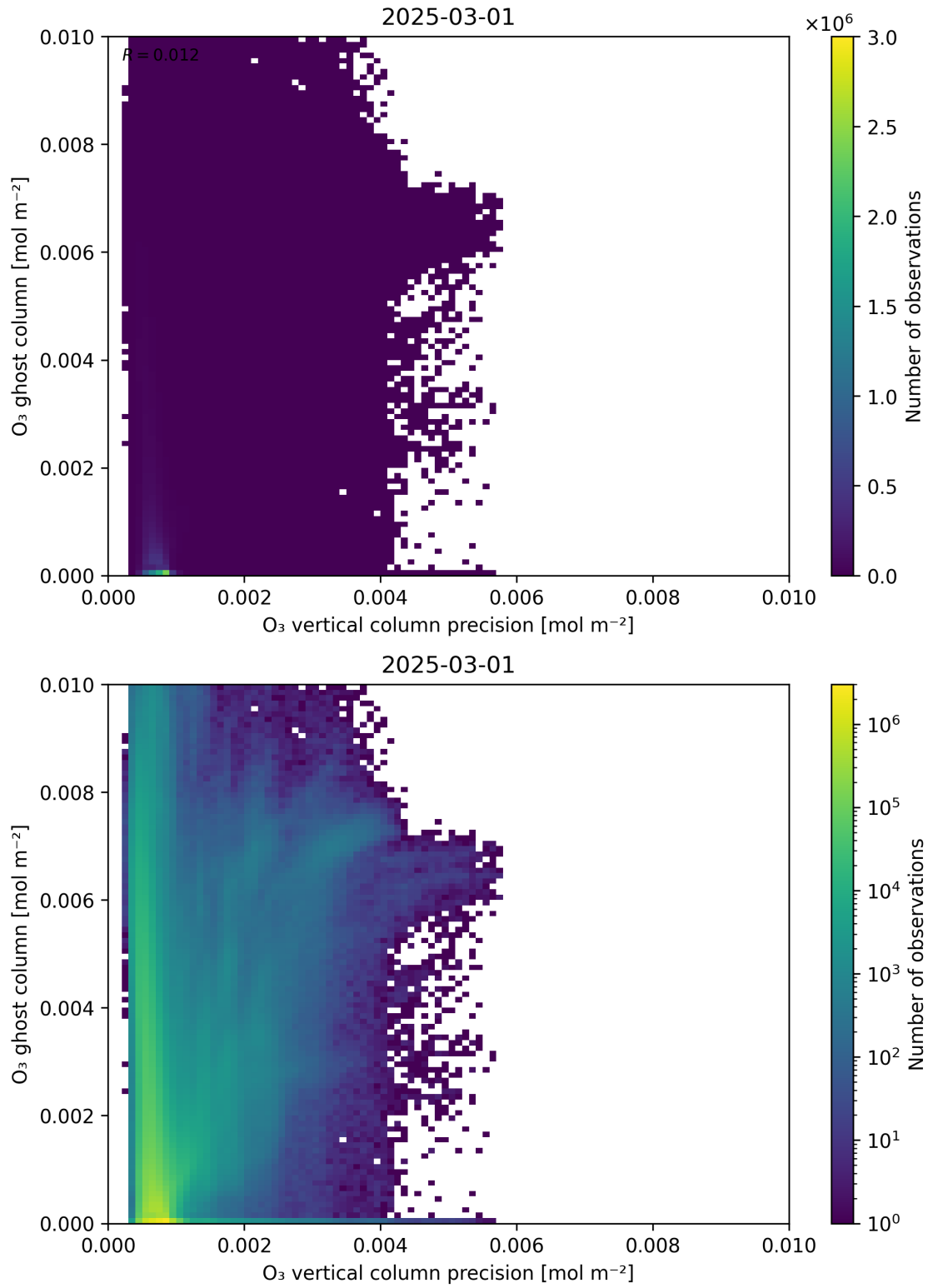
Figure 43: Scatter density plot of “O 3 vertical column precision” against “O 3 ghost column” for 2025-03-01 to 2025-03-02.
