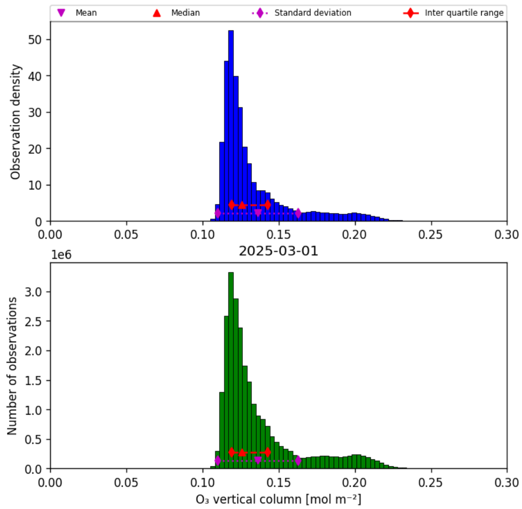
Figure 21: Histogram of “O 3 vertical column” for 2025-03-01 to 2025-03-02
