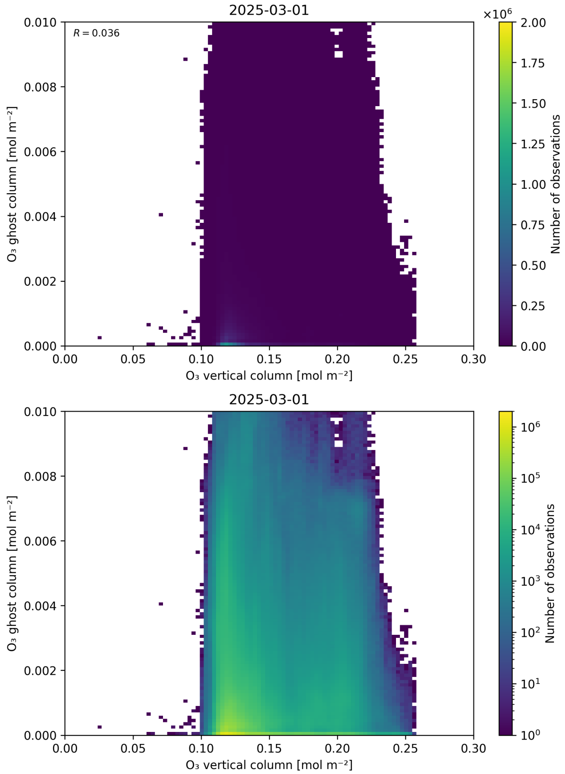
Figure 40: Scatter density plot of “O 3 vertical column” against “O 3 ghost column” for 2025-03-01 to 2025-03-02.
