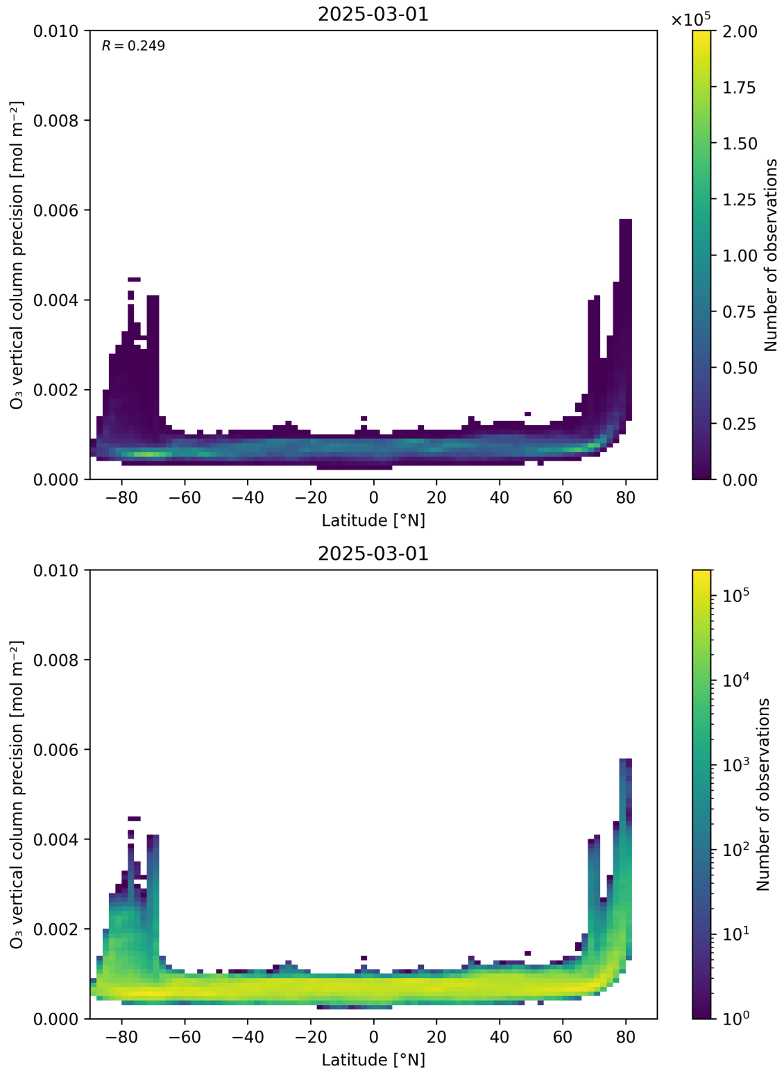
Figure 37: Scatter density plot of “Latitude” against “O 3 vertical column precision” for 2025-03-01 to 2025-03-02.
