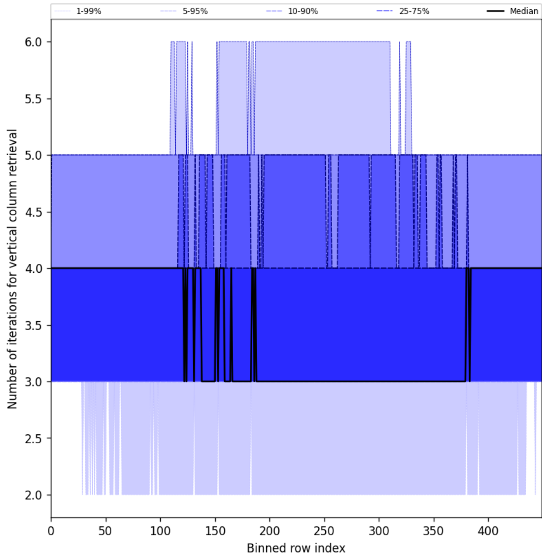
Figure 33: Along track statistics of “Number of iterations for vertical column retrieval” for 2025-03-01 to 2025-03-02
