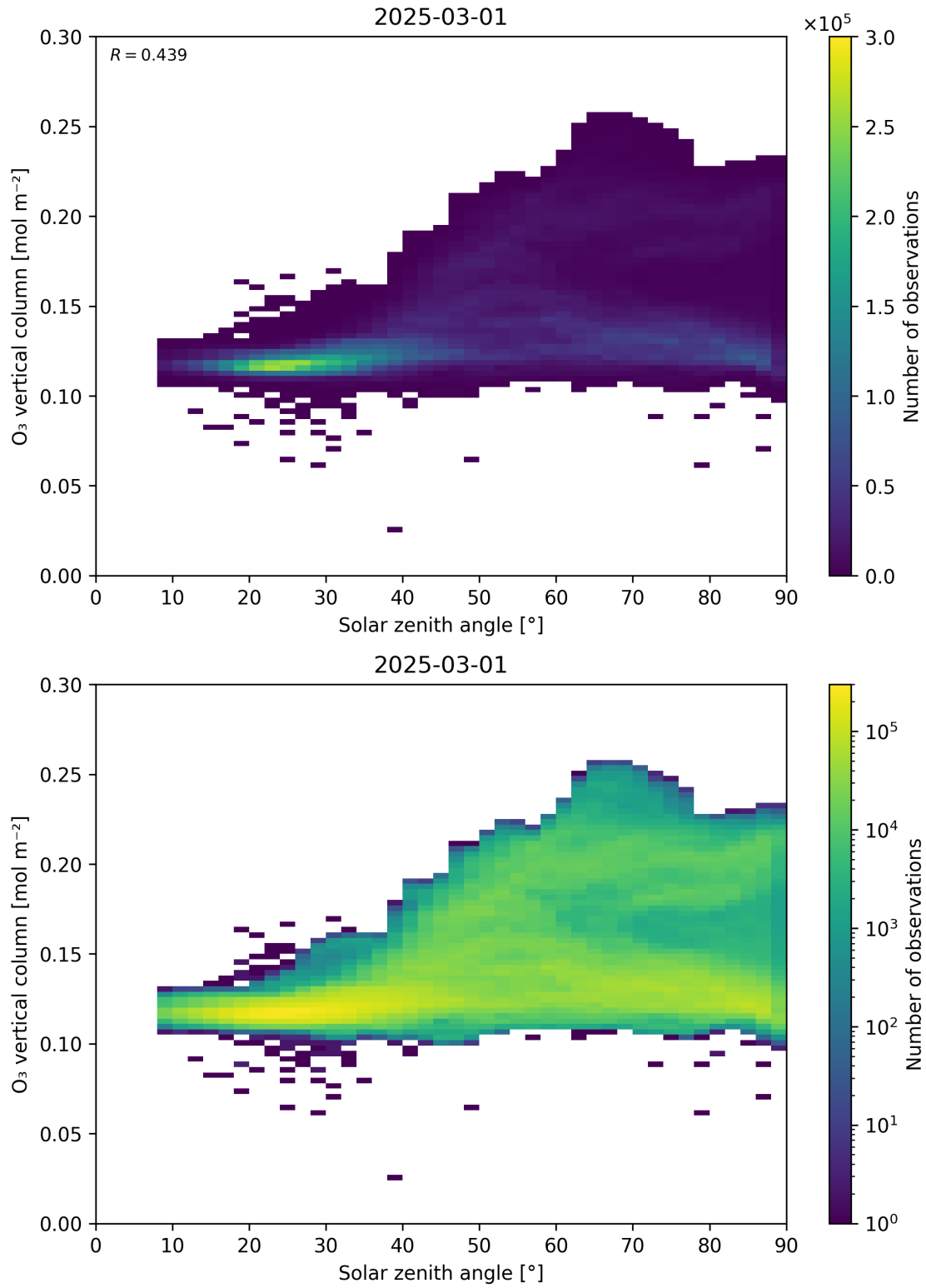
Figure 47: Scatter density plot of “Solar zenith angle” against “O 3 vertical column” for 2025-03-01 to 2025-03-02.
