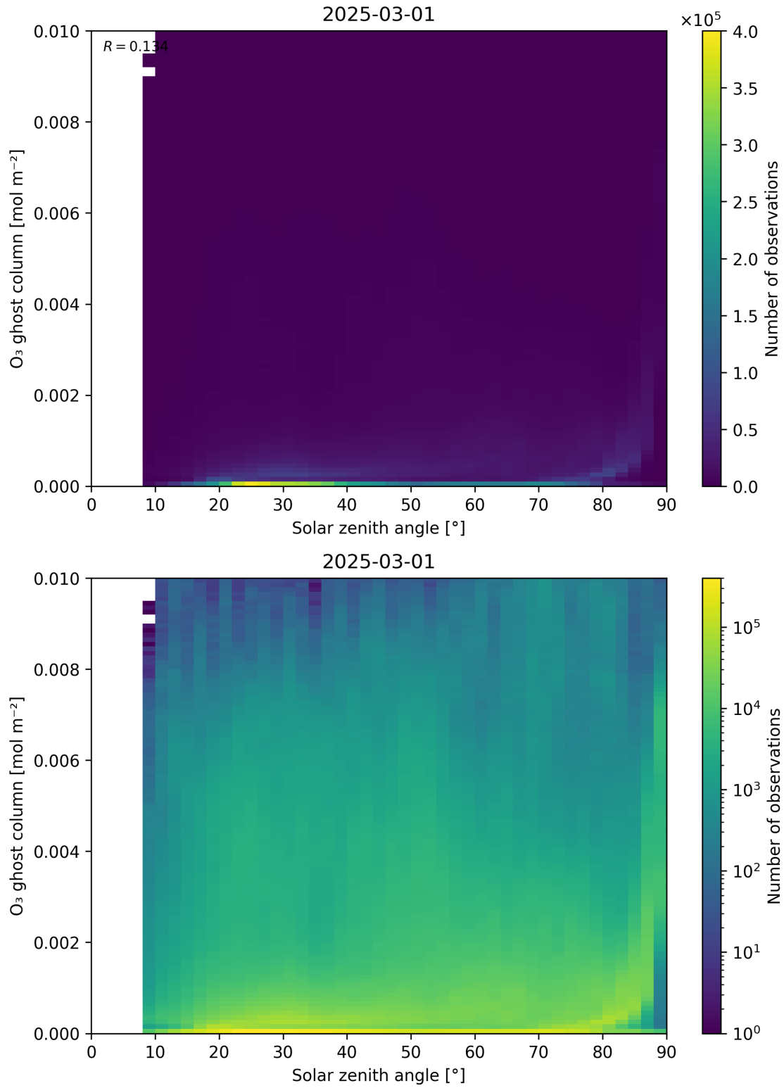
Figure 46: Scatter density plot of “Solar zenith angle” against “O 3 ghost column” for 2025-03-01 to 2025-03-02.
