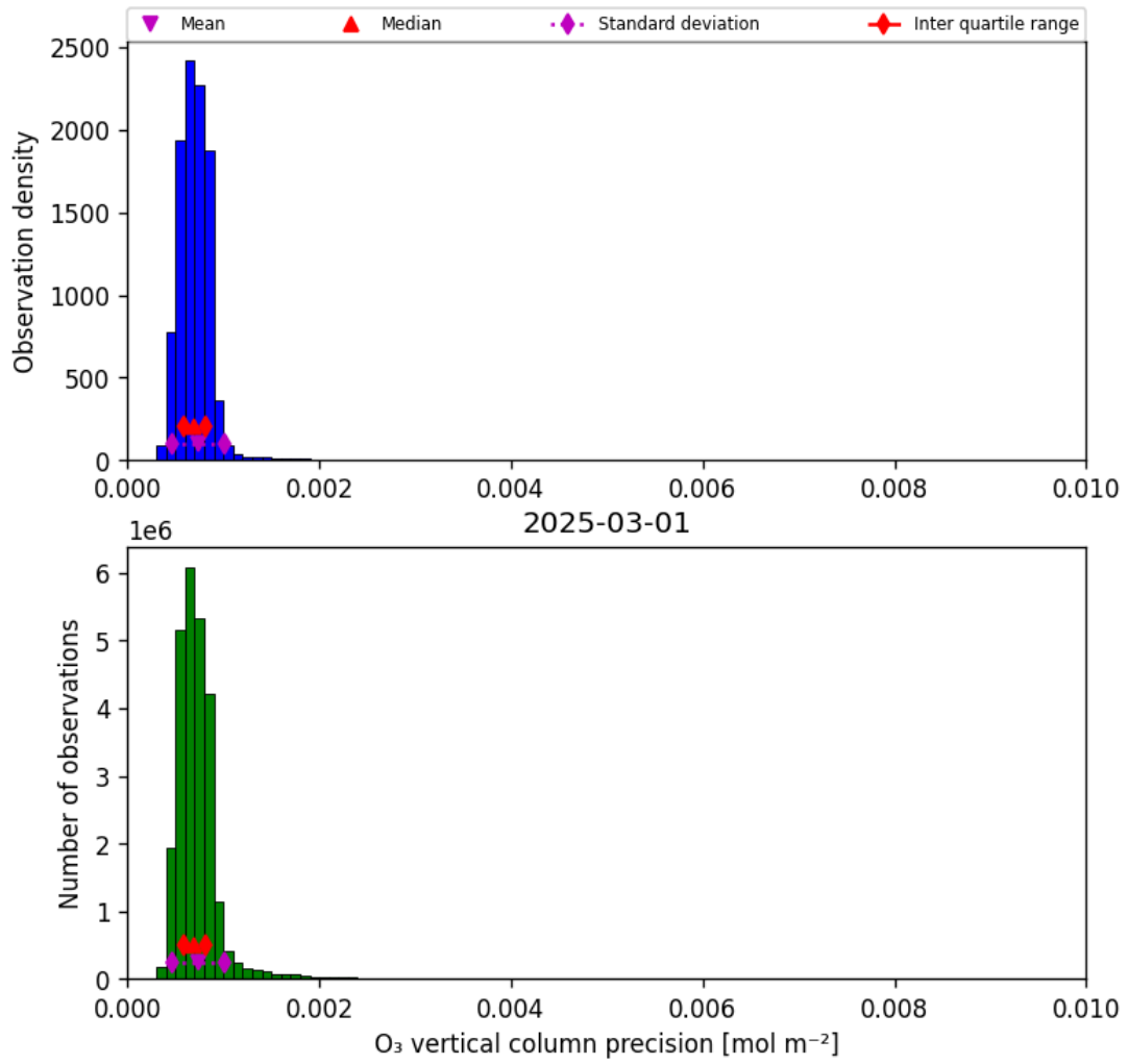
Figure 22: Histogram of “O 3 vertical column precision” for 2025-03-01 to 2025-03-02
