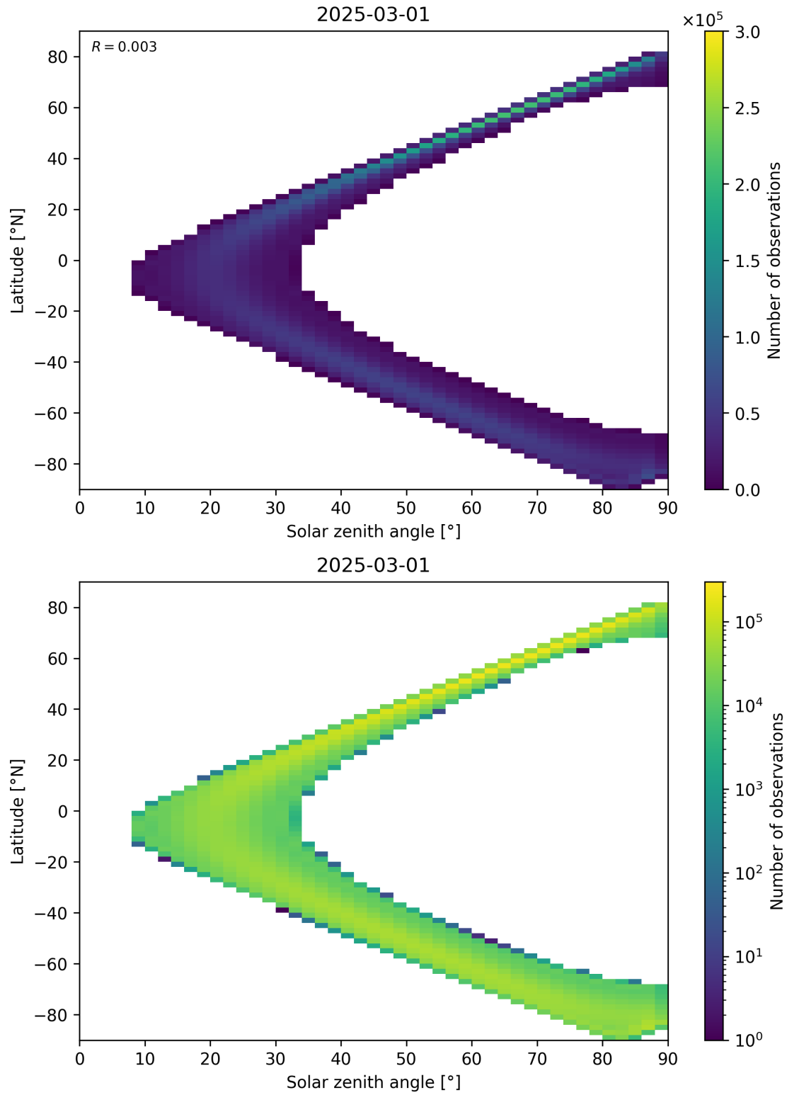
Figure 44: Scatter density plot of “Solar zenith angle” against “Latitude” for 2025-03-01 to 2025-03-02.
