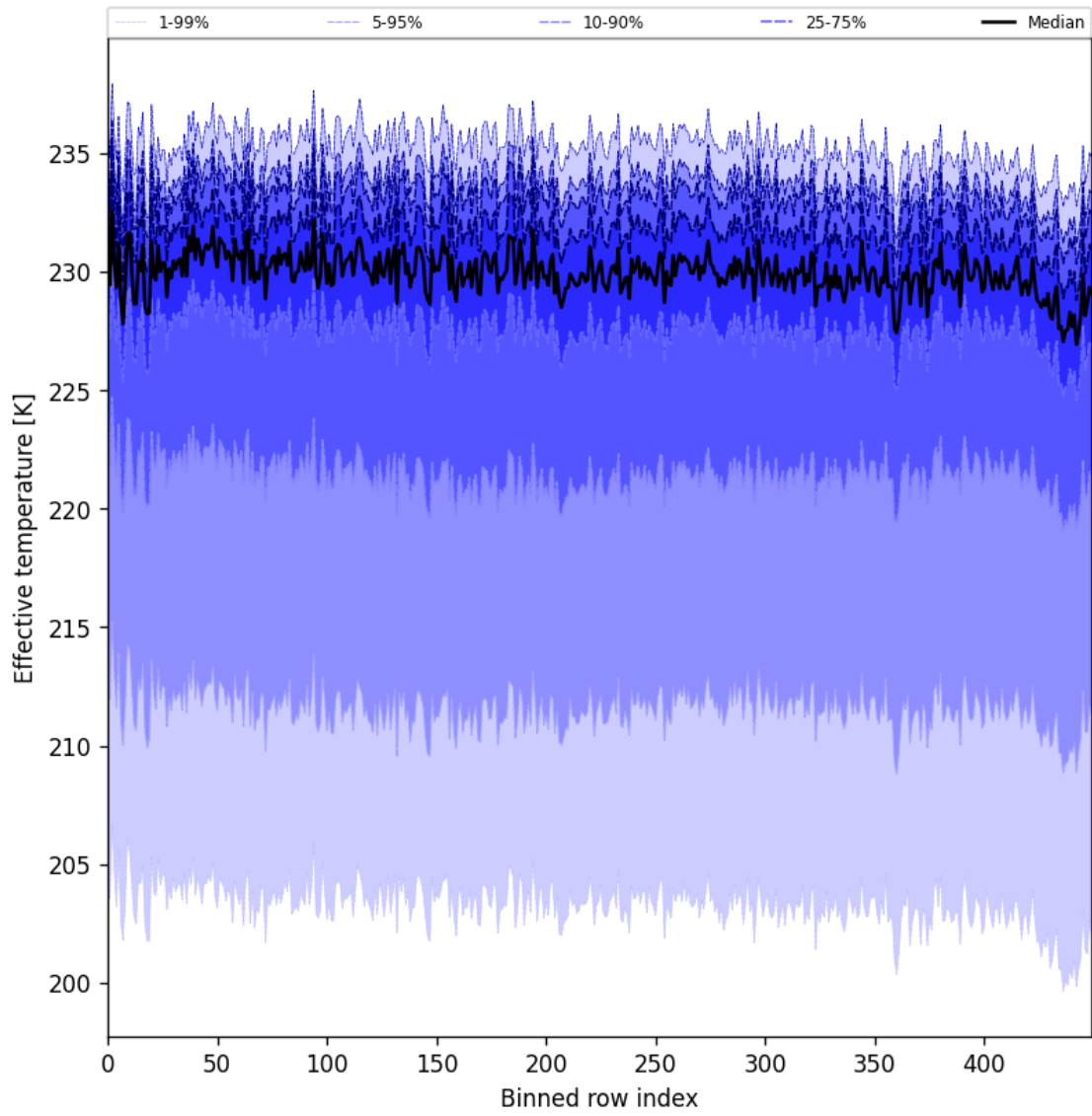
Figure 31: Along track statistics of "Effective temperature" for 2025-03-01 to 2025-03-02
