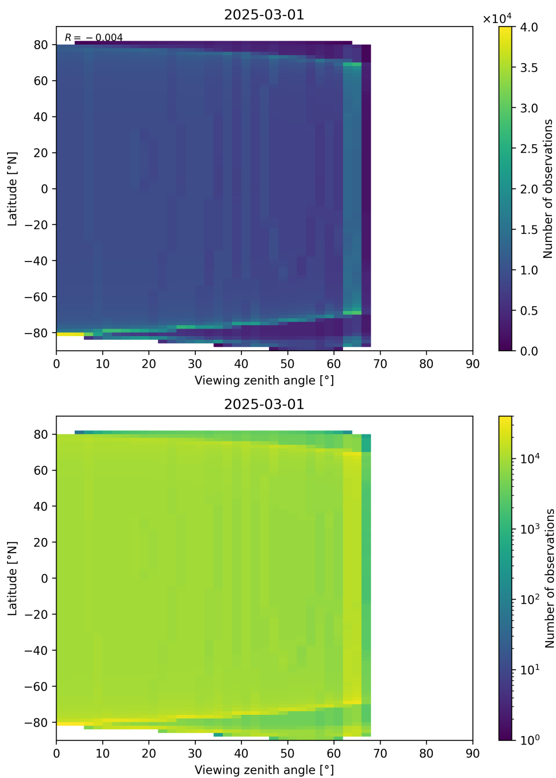
Figure 49: Scatter density plot of “Viewing zenith angle” against “Latitude” for 2025-03-01 to 2025-03-02.
