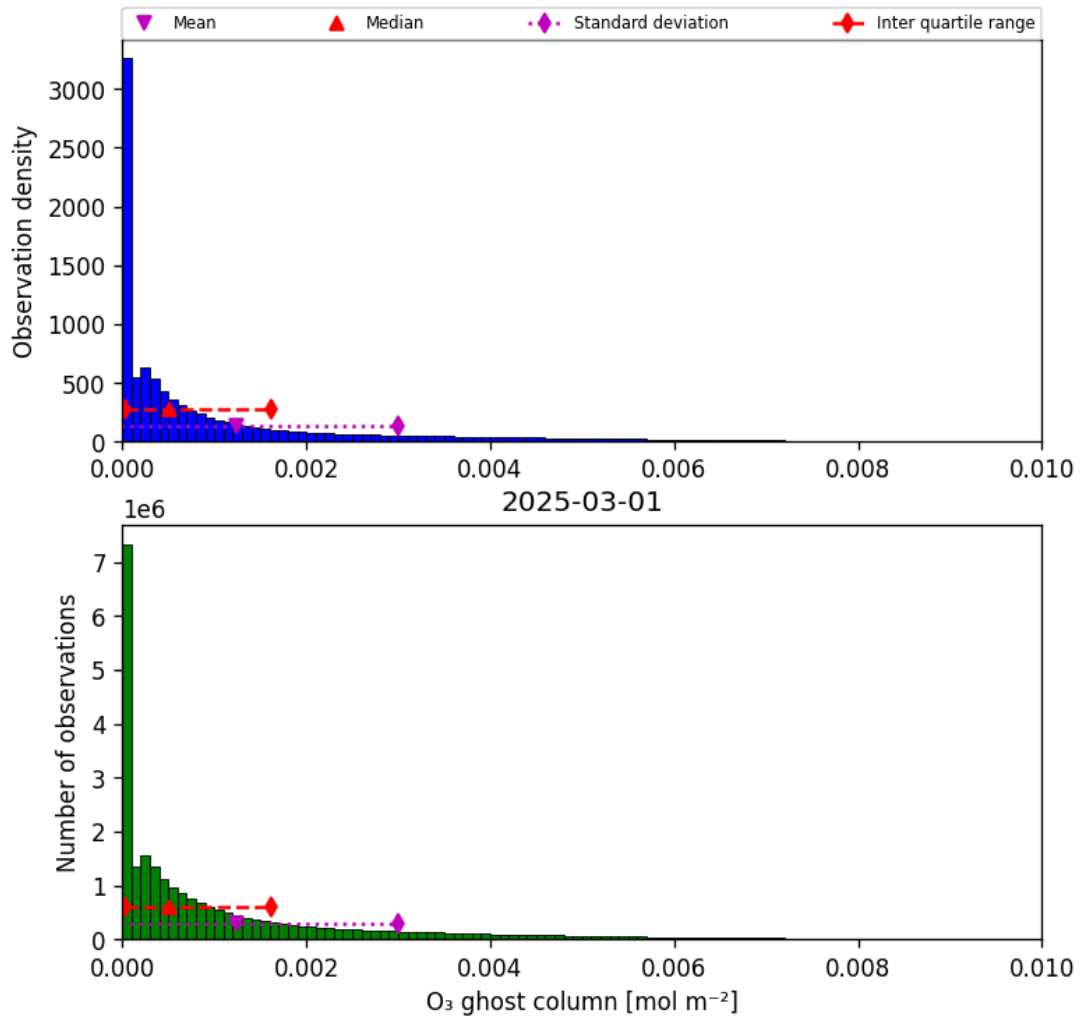
Figure 25: Histogram of “O 3 ghost column” for 2025-03-01 to 2025-03-02
