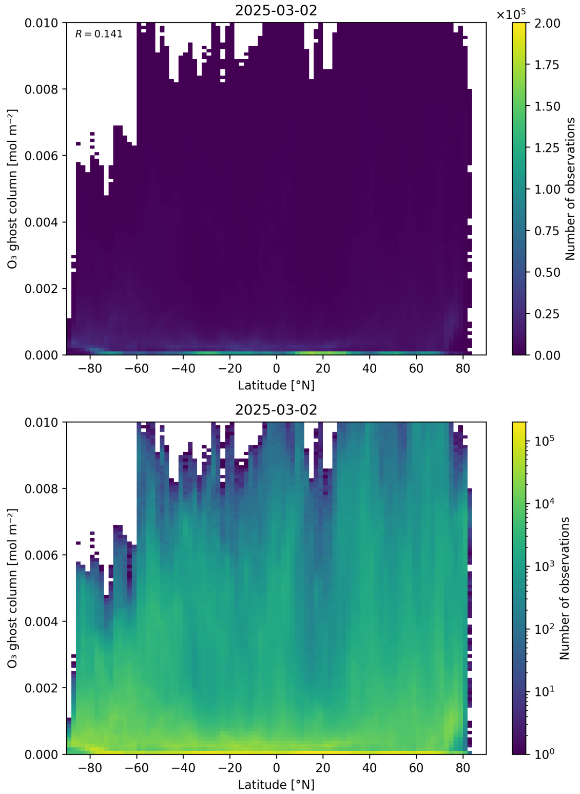
Figure 35: Scatter density plot of “Latitude” against “O 3 ghost column” for 2025-03-01 to 2025-03-03.
