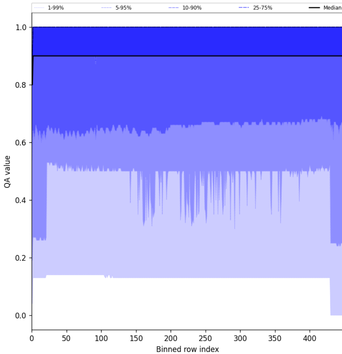
Figure 27: Along track statistics of “QA value” for 2025-03-01 to 2025-03-03
