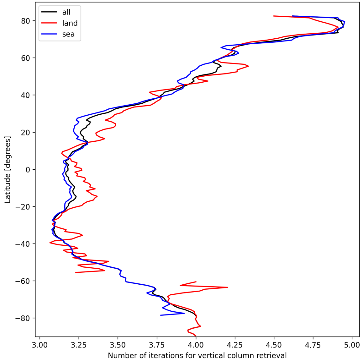
Figure 19: Zonal average of “Number of iterations for vertical column retrieval” for 2025-03-01 to 2025-03-03.
