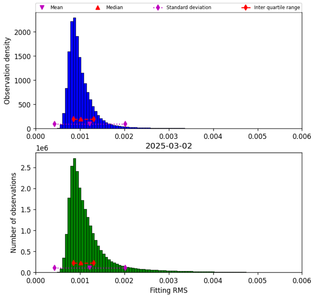
Figure 23: Histogram of “Fitting RMS” for 2025-03-01 to 2025-03-03
