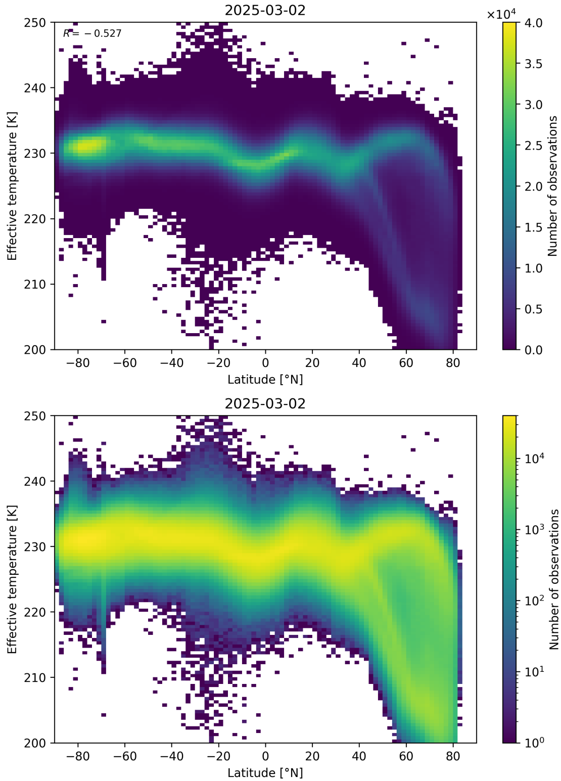
Figure 34: Scatter density plot of “Latitude” against “Effective temperature” for 2025-03-01 to 2025-03-03.
