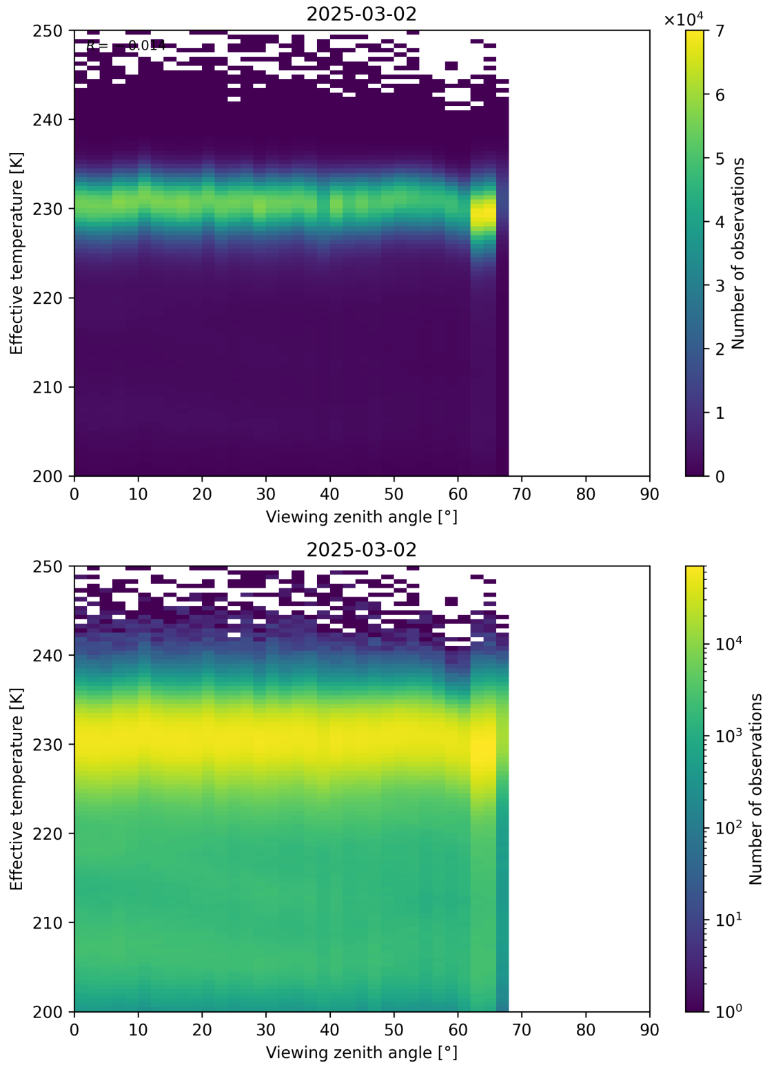
Figure 50: Scatter density plot of “Viewing zenith angle” against “Effective temperature” for 2025-03-01 to 2025-03-03.
