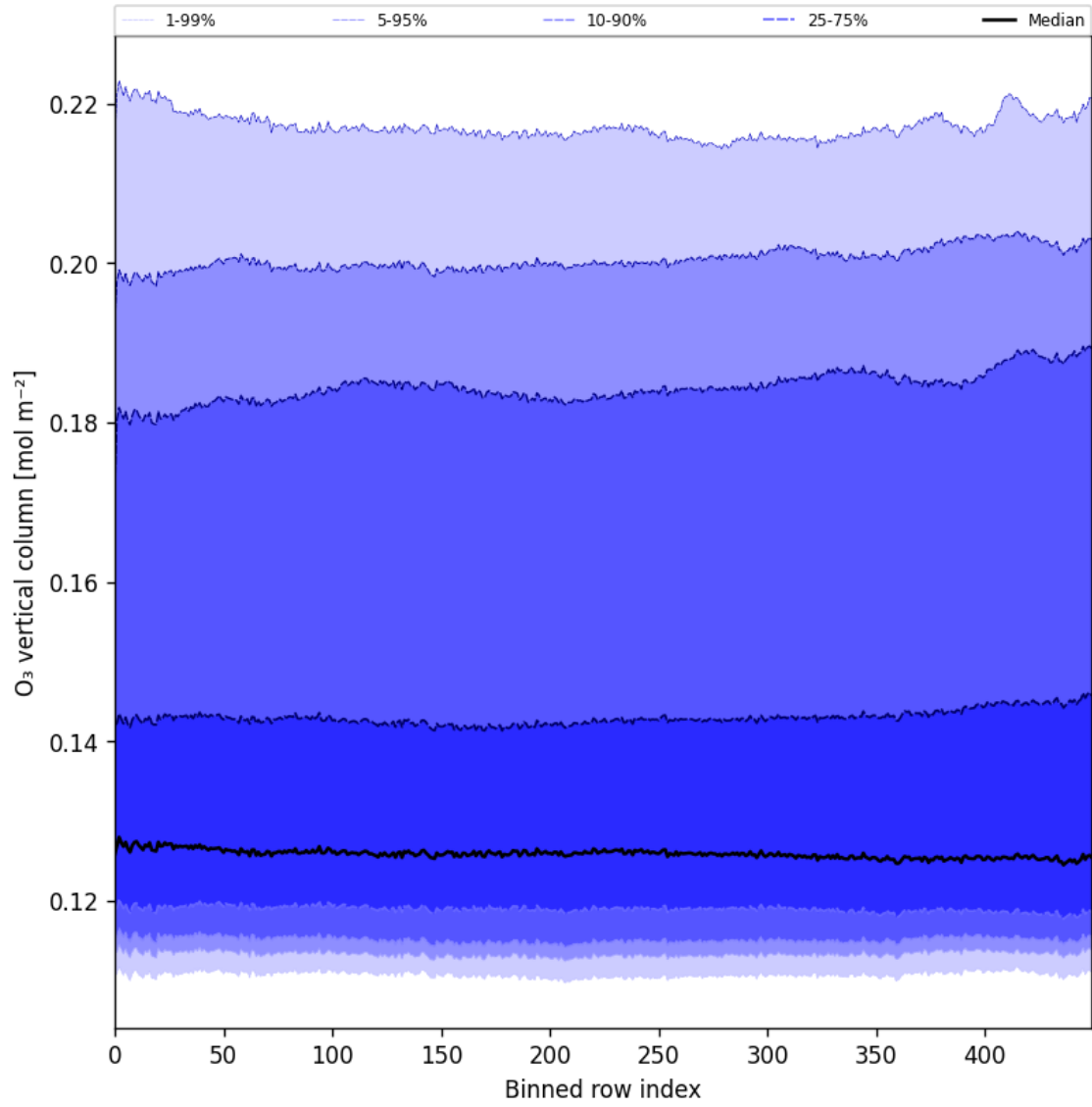
Figure 28: Along track statistics of “O 3 vertical column” for 2025-03-01 to 2025-03-03
