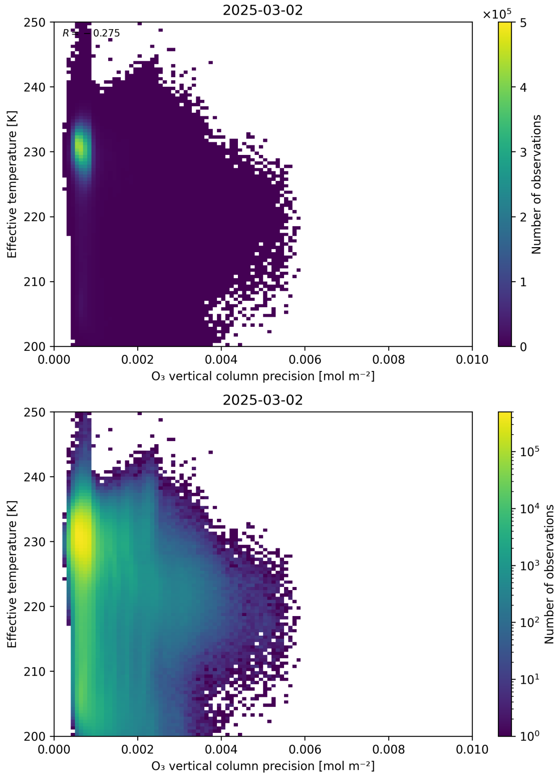
Figure 42: Scatter density plot of “O 3 vertical column precision” against “Effective temperature” for 2025-03-01 to 2025-03-03.
