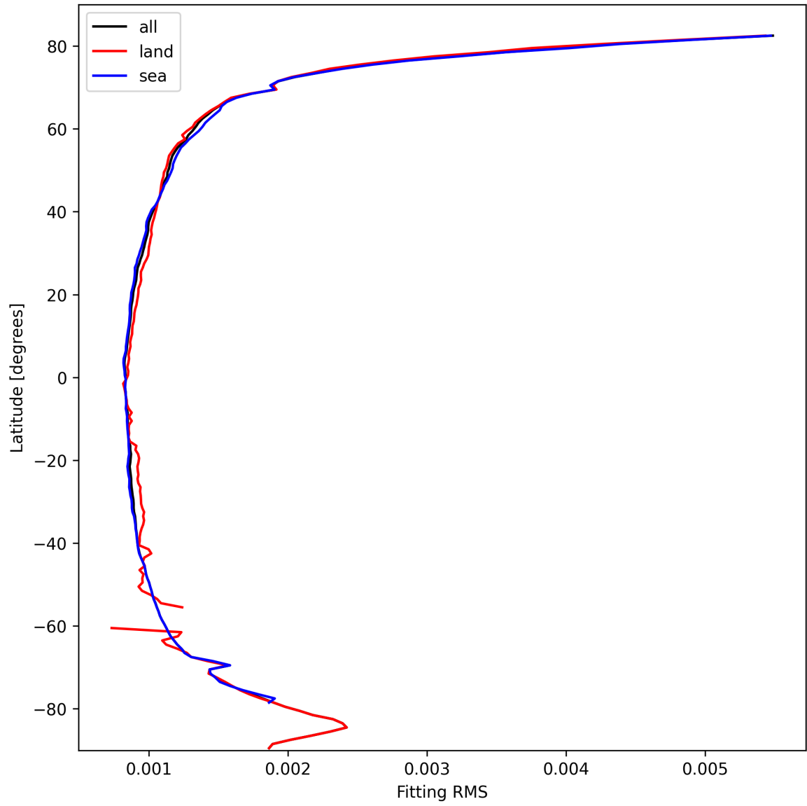
Figure 16: Zonal average of “Fitting RMS” for 2025-03-01 to 2025-03-03.
