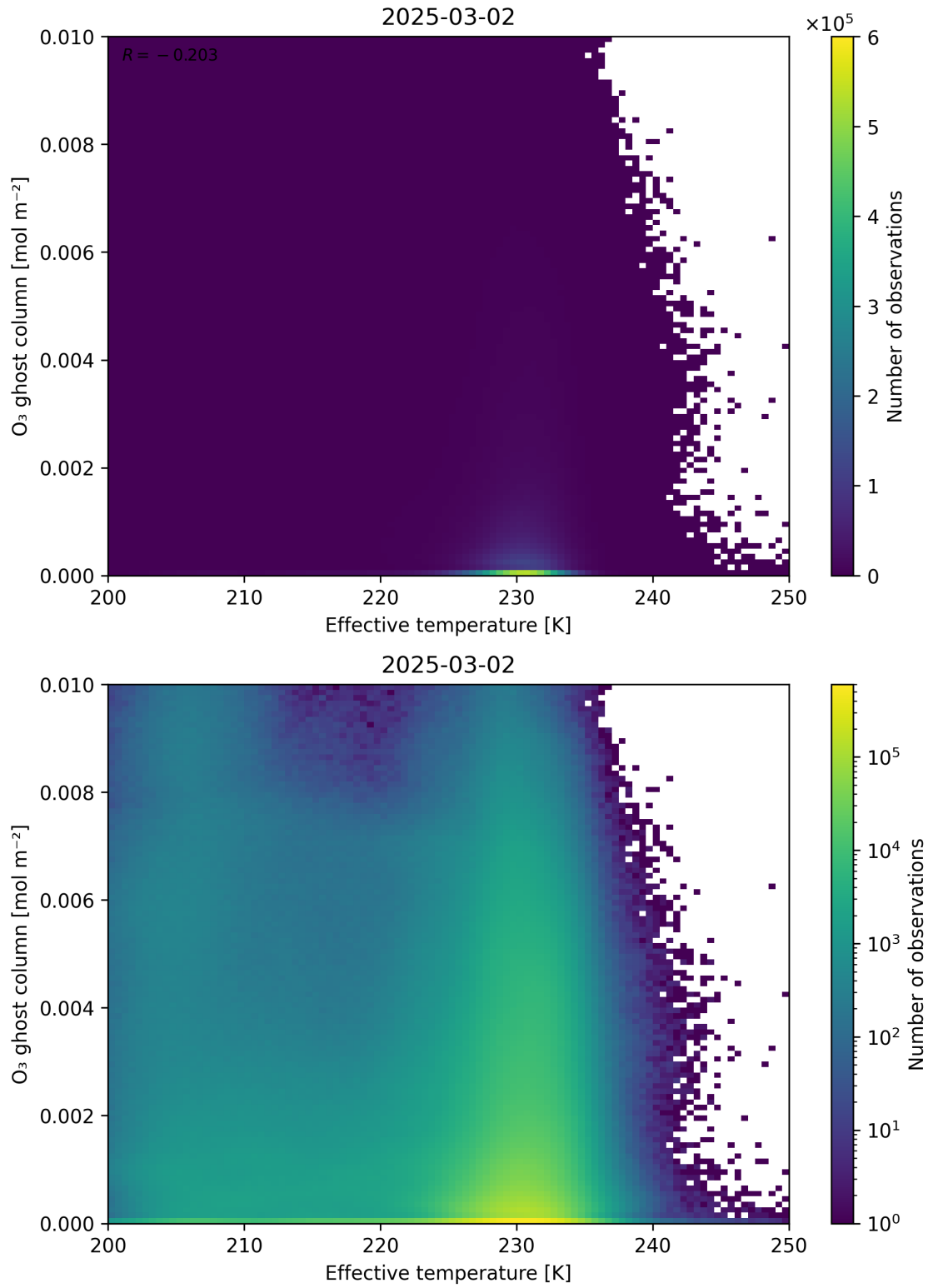
Figure 38: Scatter density plot of “Effective temperature” against “O 3 ghost column” for 2025-03-01 to 2025-03-03.
