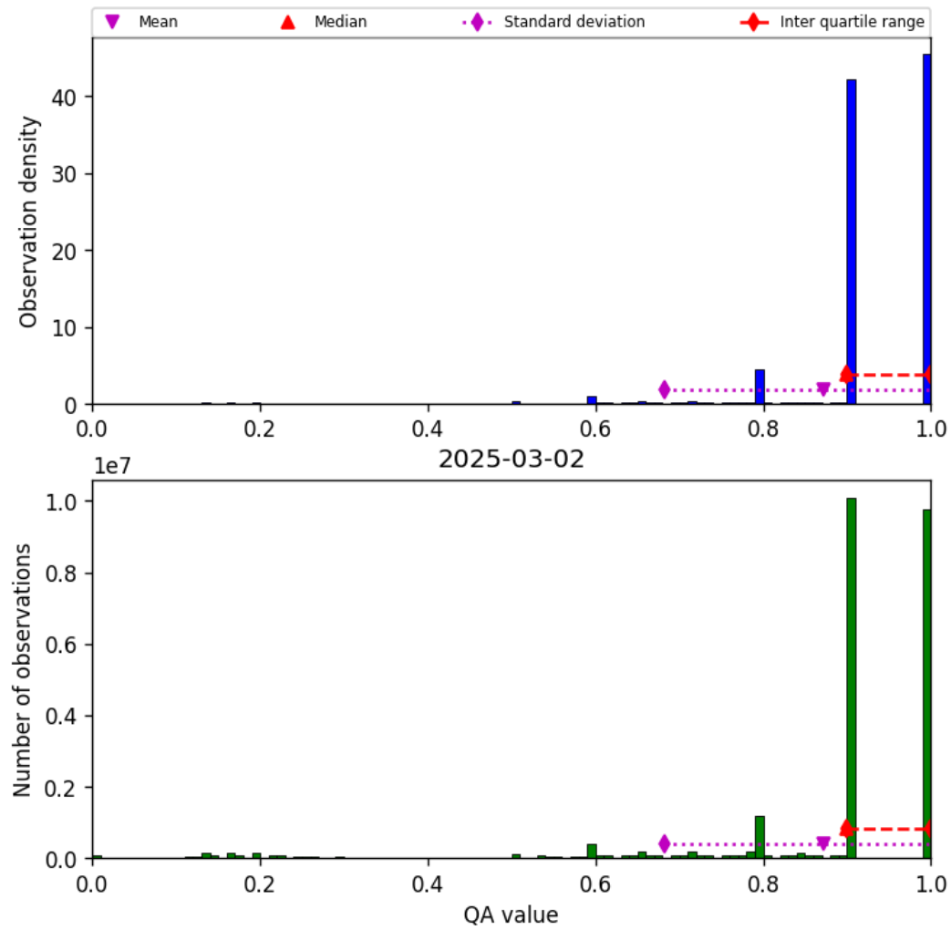
Figure 20: Histogram of “QA value” for 2025-03-01 to 2025-03-03
