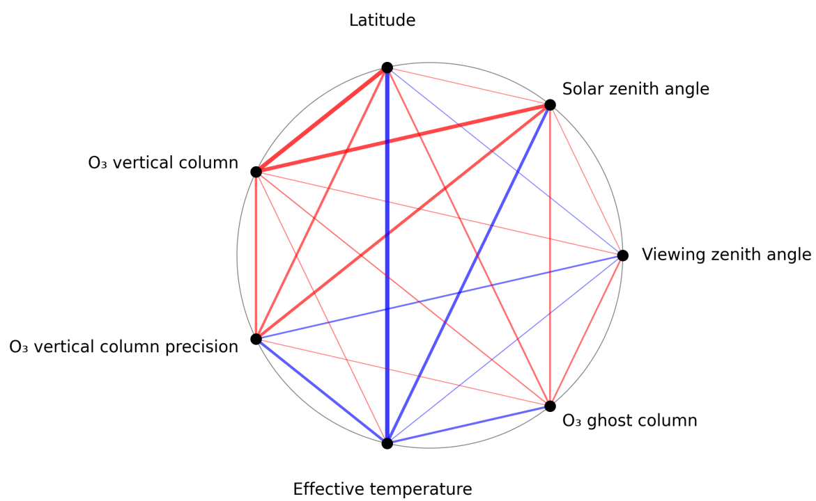
Figure 1: Map of correlation graph for 2025-03-01 to 2025-03-03.
