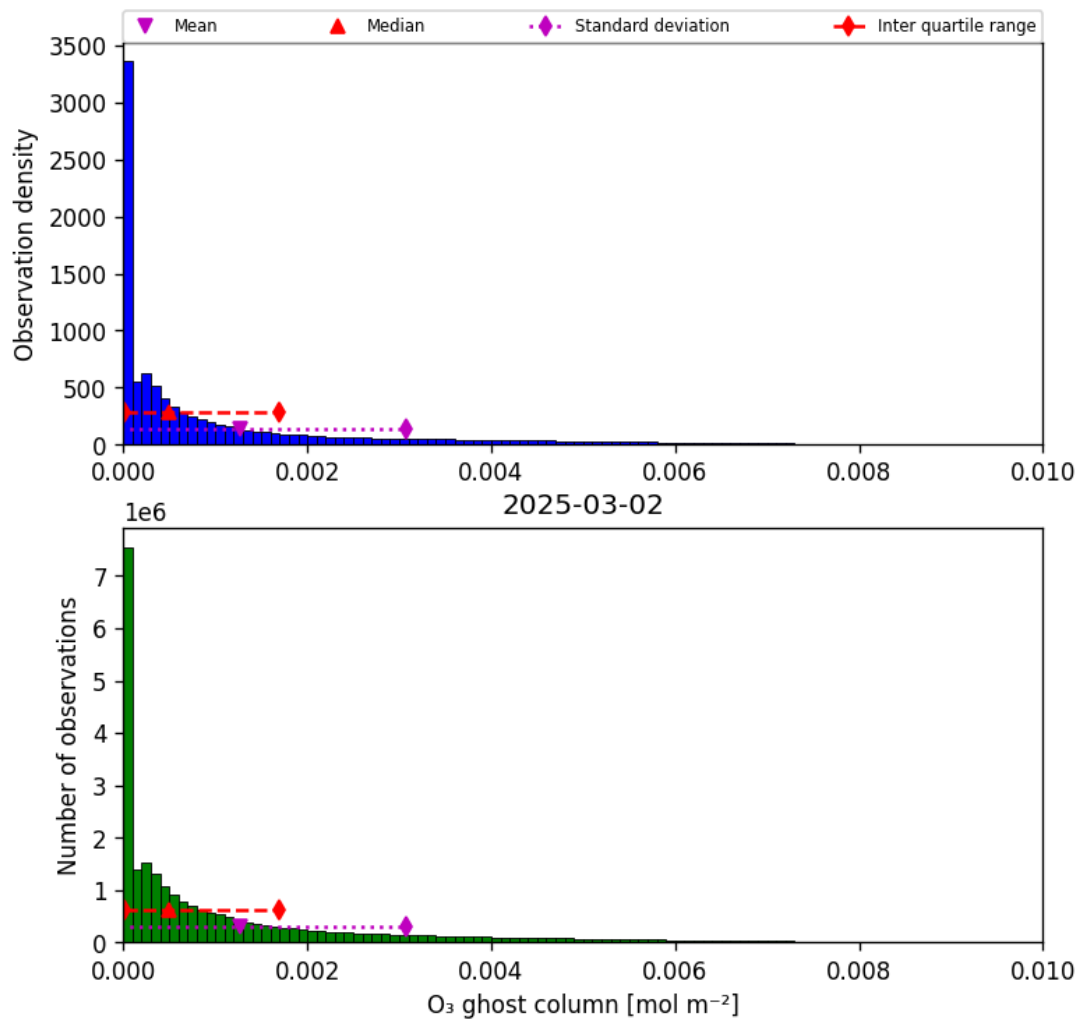
Figure 25: Histogram of “O 3 ghost column” for 2025-03-01 to 2025-03-03
