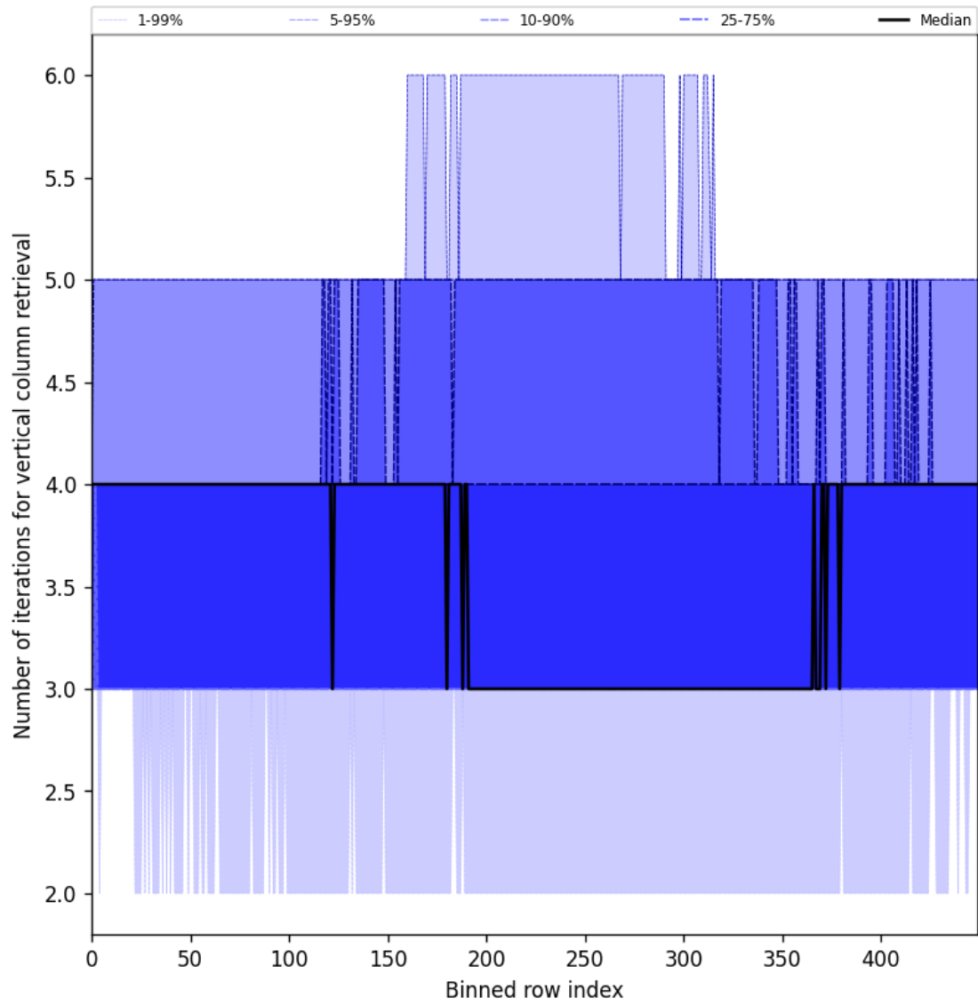
Figure 33: Along track statistics of “Number of iterations for vertical column retrieval” for 2025-03-01 to 2025-03-03
