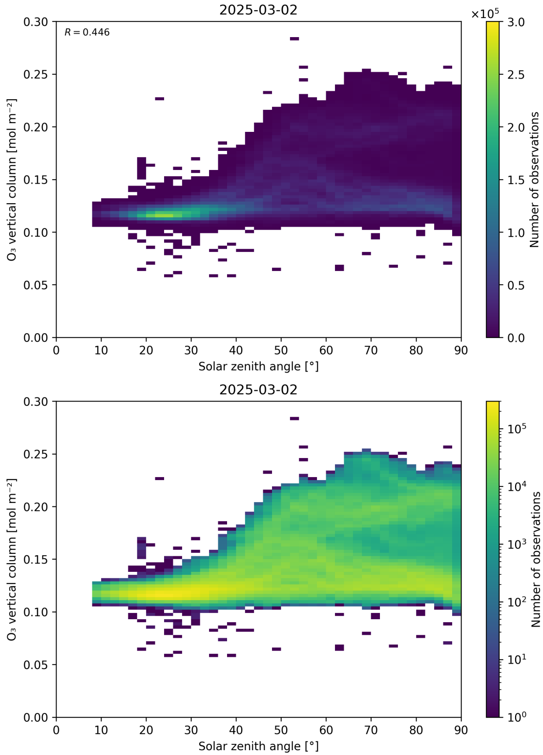
Figure 47: Scatter density plot of “Solar zenith angle” against “O 3 vertical column” for 2025-03-01 to 2025-03-03.
