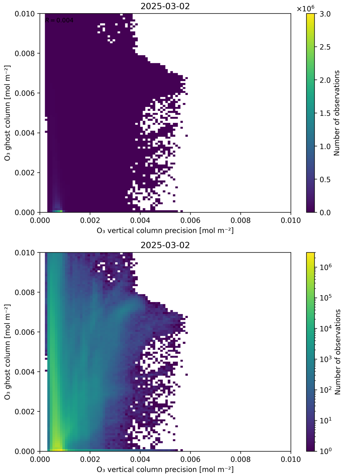
Figure 43: Scatter density plot of “O 3 vertical column precision” against “O 3 ghost column” for 2025-03-01 to 2025-03-03.
