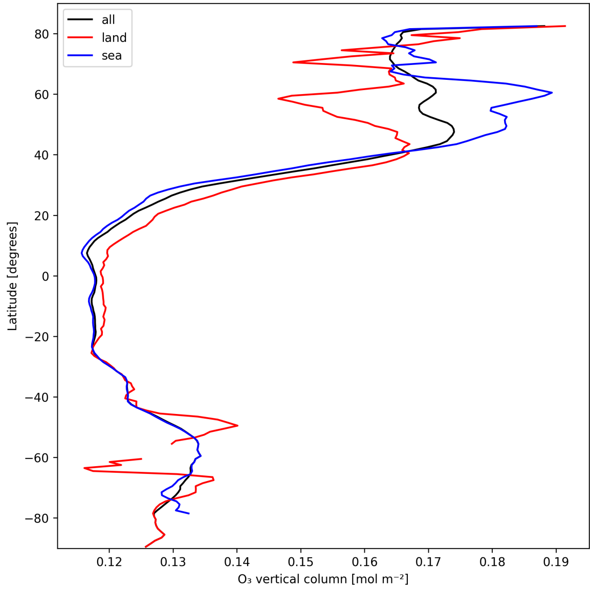
Figure 14: Zonal average of “O 3 vertical column” for 2025-03-01 to 2025-03-03.
