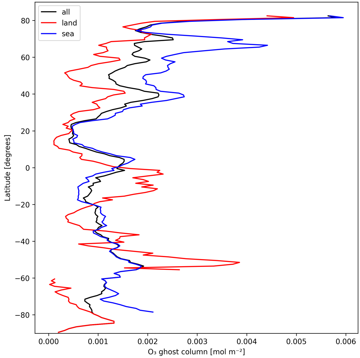
Figure 18: Zonal average of “O 3 ghost column” for 2025-03-01 to 2025-03-03.
