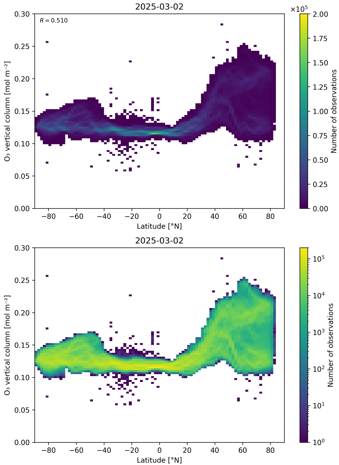
Figure 36: Scatter density plot of “Latitude” against “O 3 vertical column” for 2025-03-01 to 2025-03-03.
