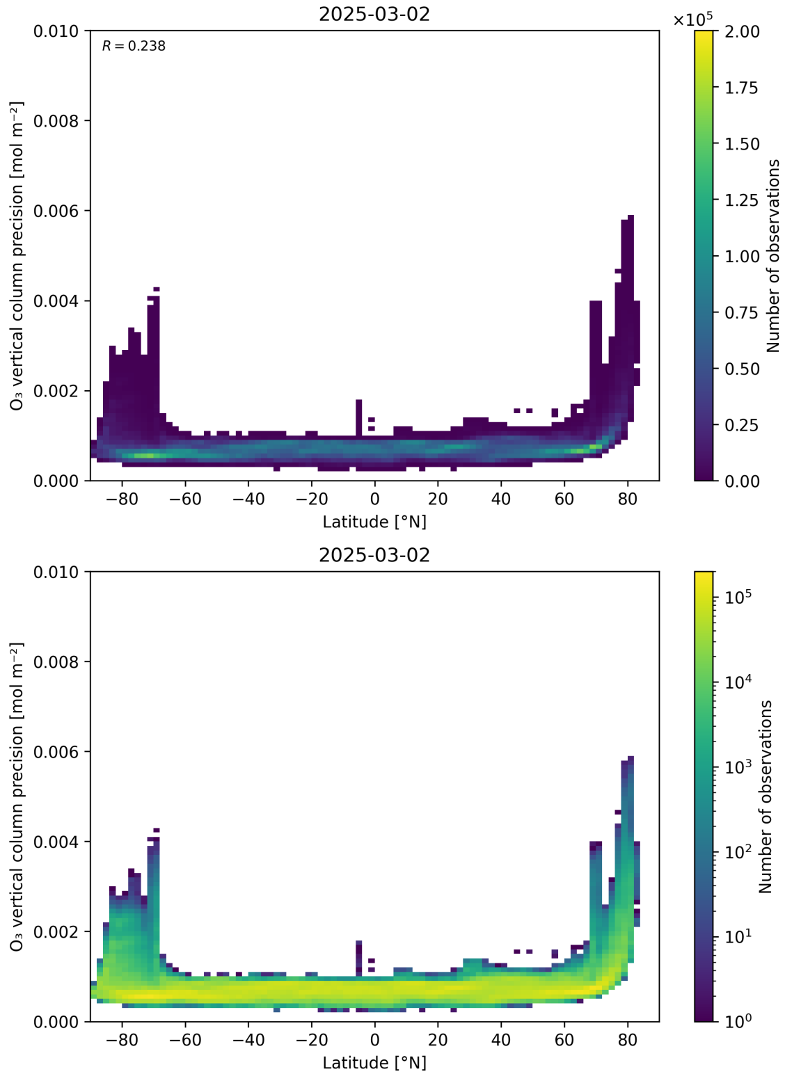
Figure 37: Scatter density plot of “Latitude” against “O 3 vertical column precision” for 2025-03-01 to 2025-03-03.
