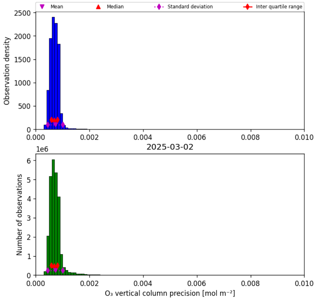
Figure 22: Histogram of “O 3 vertical column precision” for 2025-03-01 to 2025-03-03
