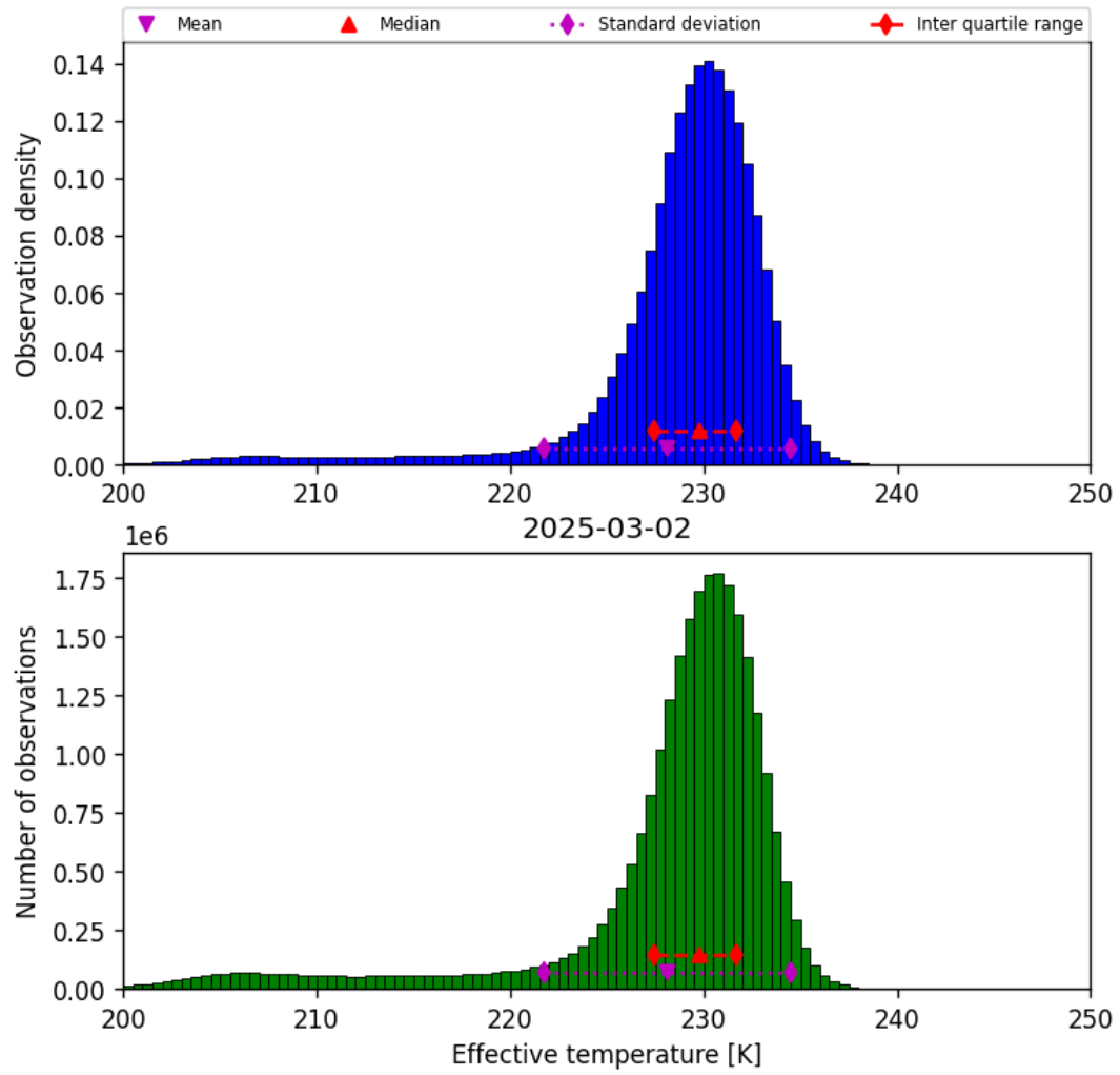
Figure 24: Histogram of “Effective temperature” for 2025-03-01 to 2025-03-03
