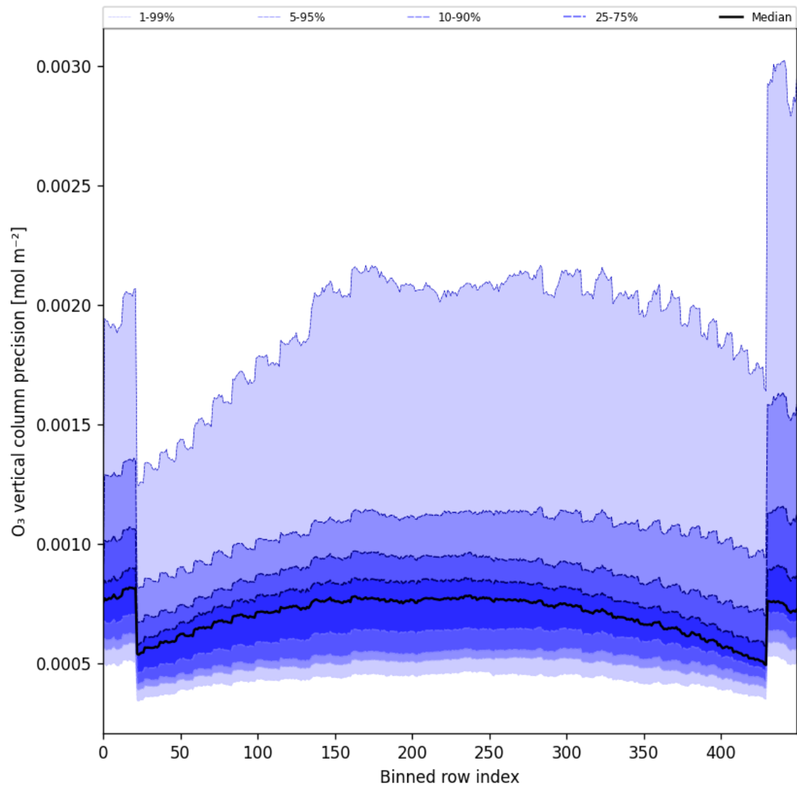
Figure 29: Along track statistics of “O 3 vertical column precision” for 2025-03-01 to 2025-03-03
