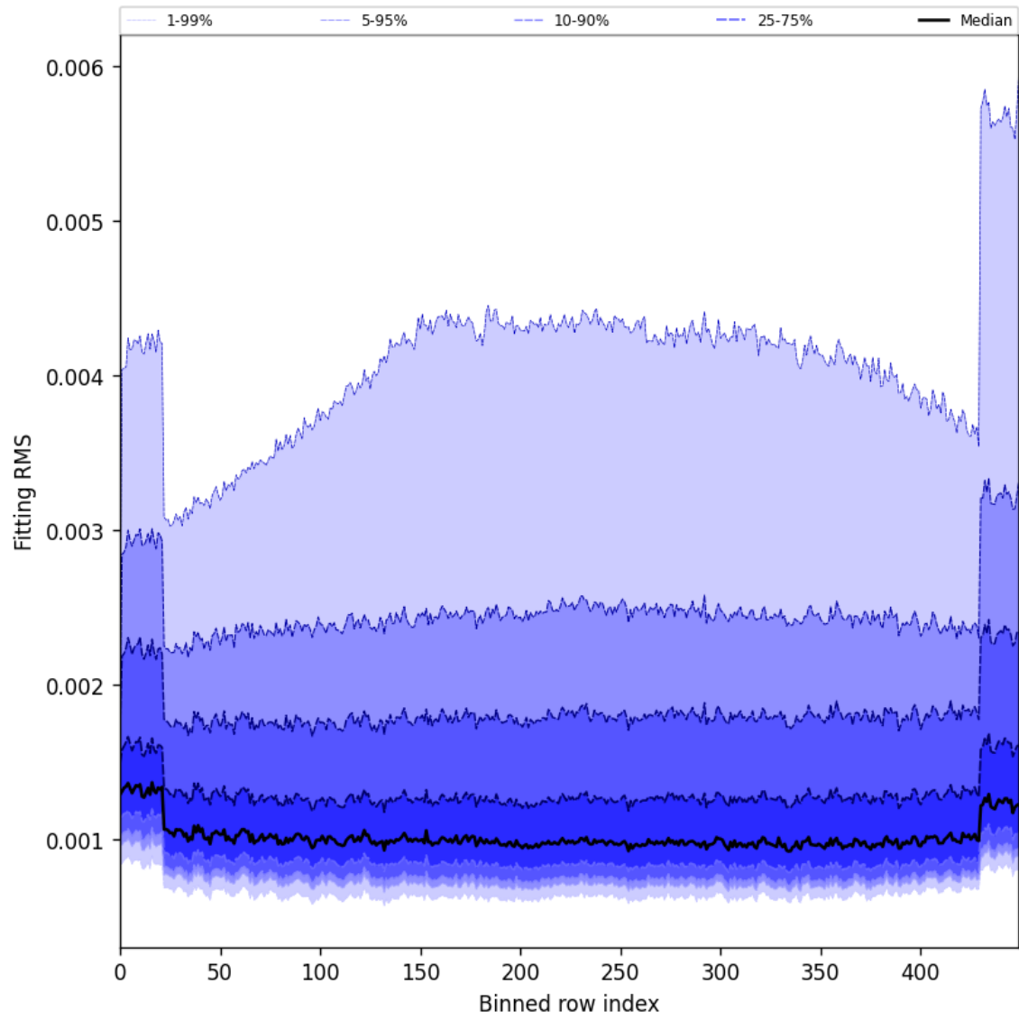
Figure 30: Along track statistics of “Fitting RMS” for 2025-03-01 to 2025-03-03
