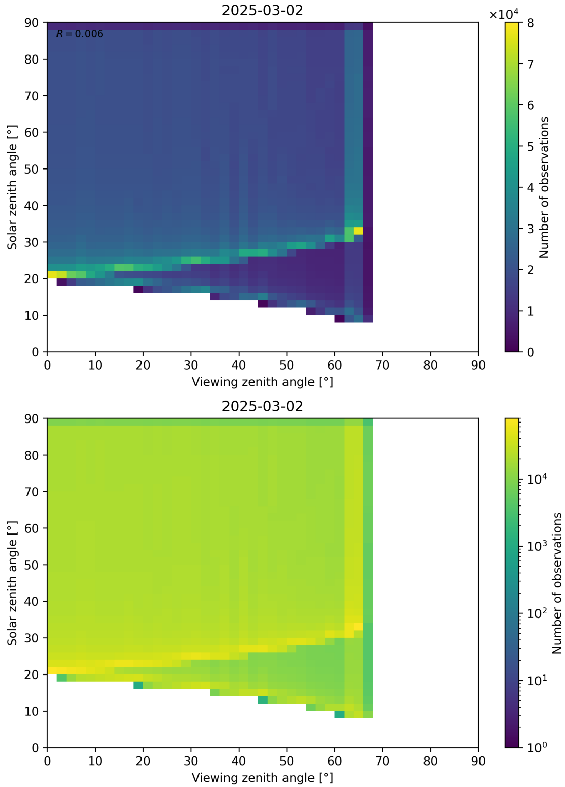
Figure 54: Scatter density plot of “Viewing zenith angle” against “Solar zenith angle” for 2025-03-01 to 2025-03-03.
