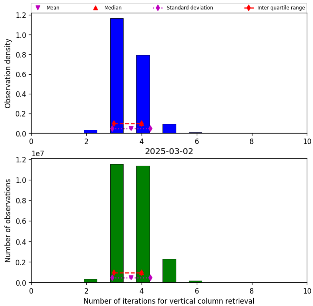
Figure 26: Histogram of “Number of iterations for vertical column retrieval” for 2025-03-01 to 2025-03-03
