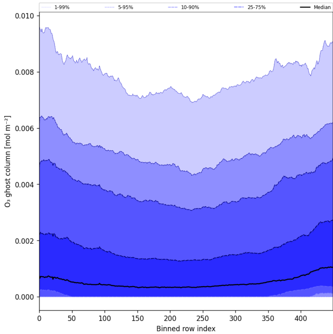
Figure 32: Along track statistics of “O 3 ghost column” for 2025-03-01 to 2025-03-03
