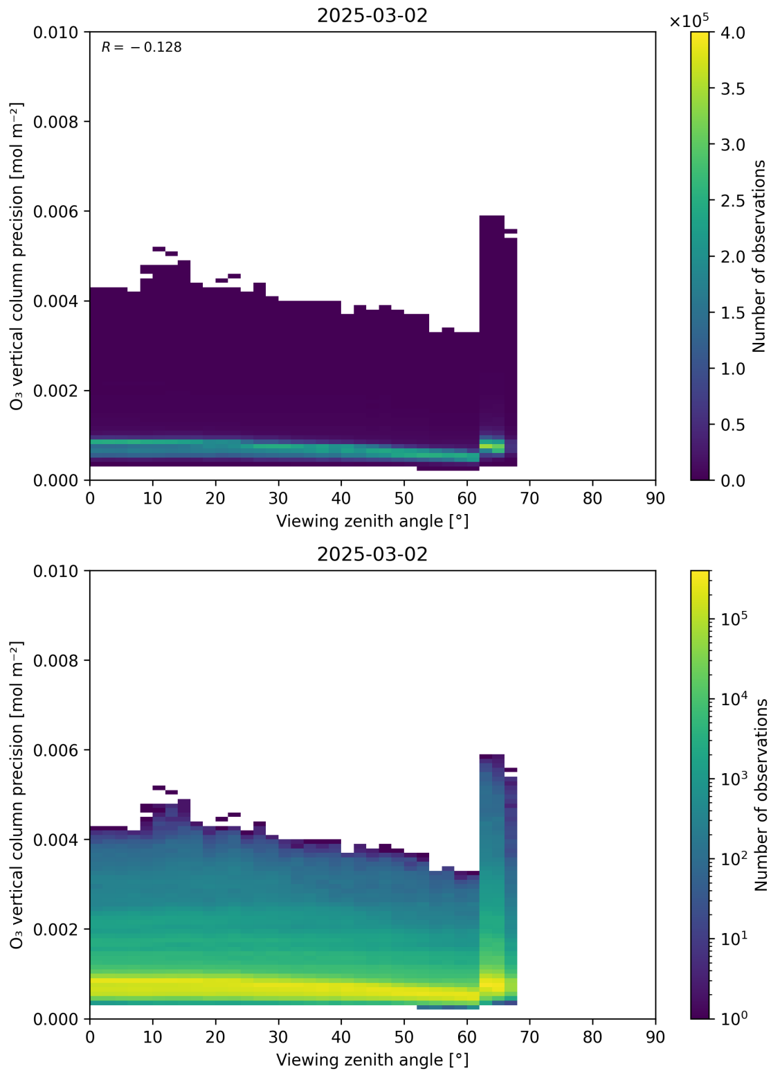
Figure 53: Scatter density plot of “Viewing zenith angle” against “O 3 vertical column precision” for 2025-03-01 to 2025-03-03.
