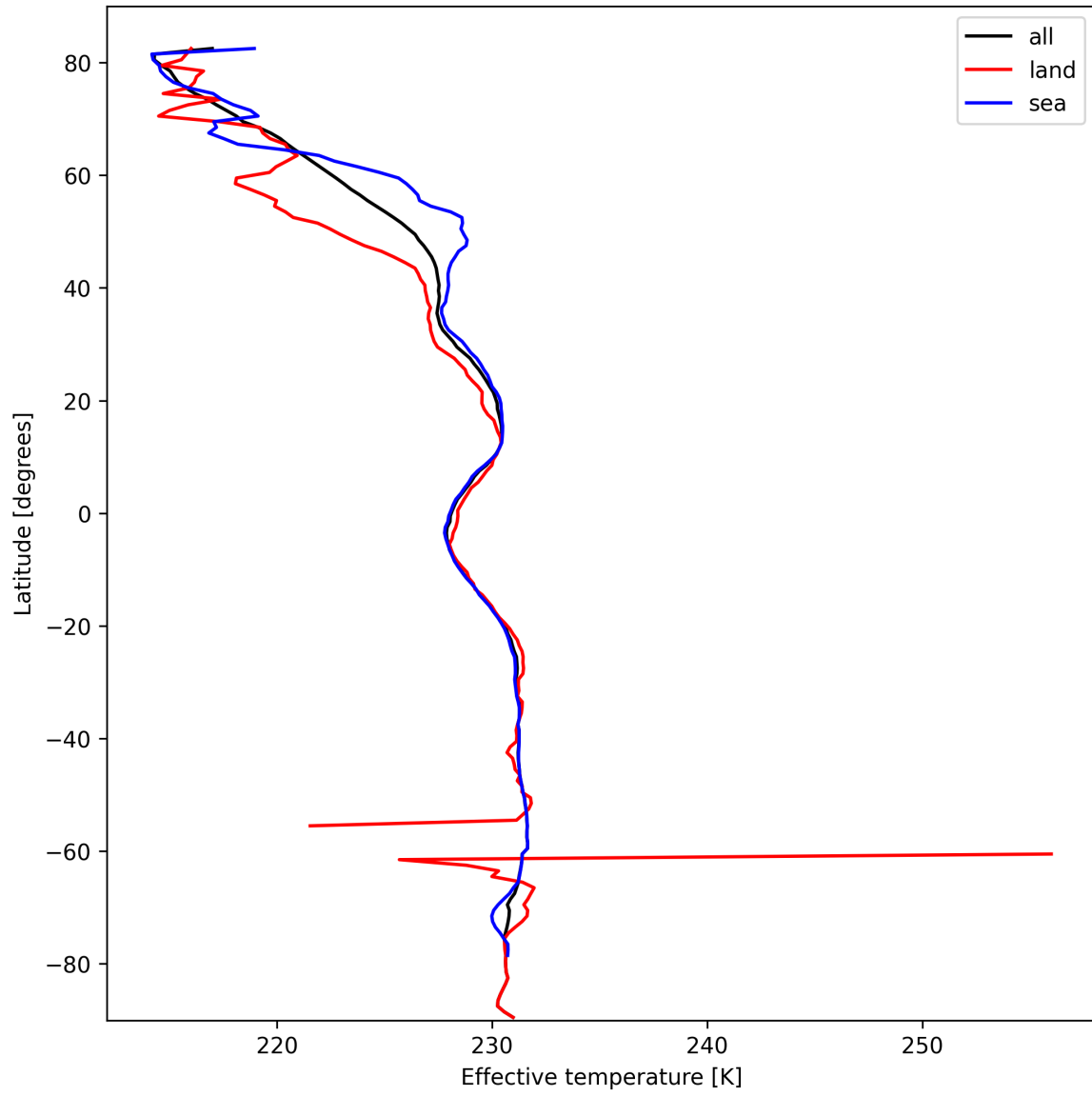
Figure 17: Zonal average of “Effective temperature” for 2025-03-01 to 2025-03-03.
