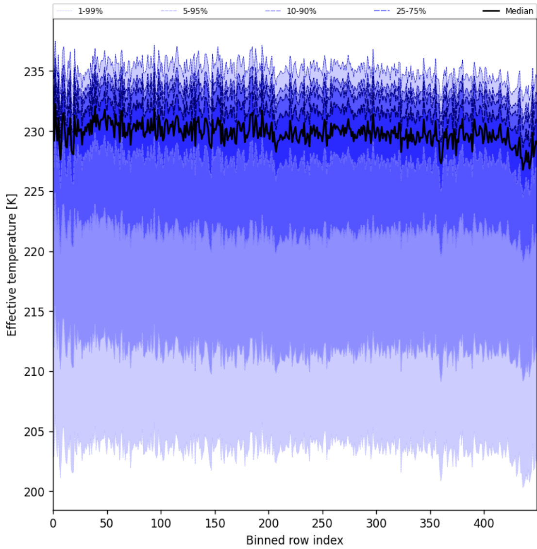
Figure 31: Along track statistics of “Effective temperature” for 2025-03-01 to 2025-03-03
