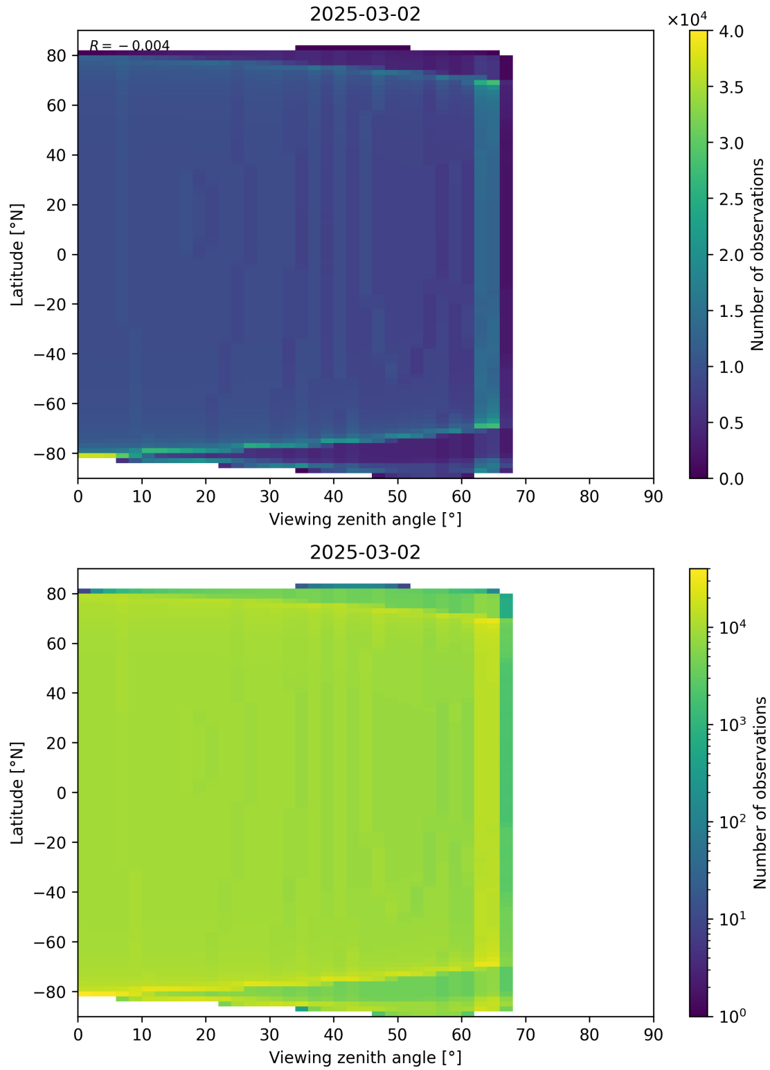
Figure 49: Scatter density plot of “Viewing zenith angle” against “Latitude” for 2025-03-01 to 2025-03-03.
