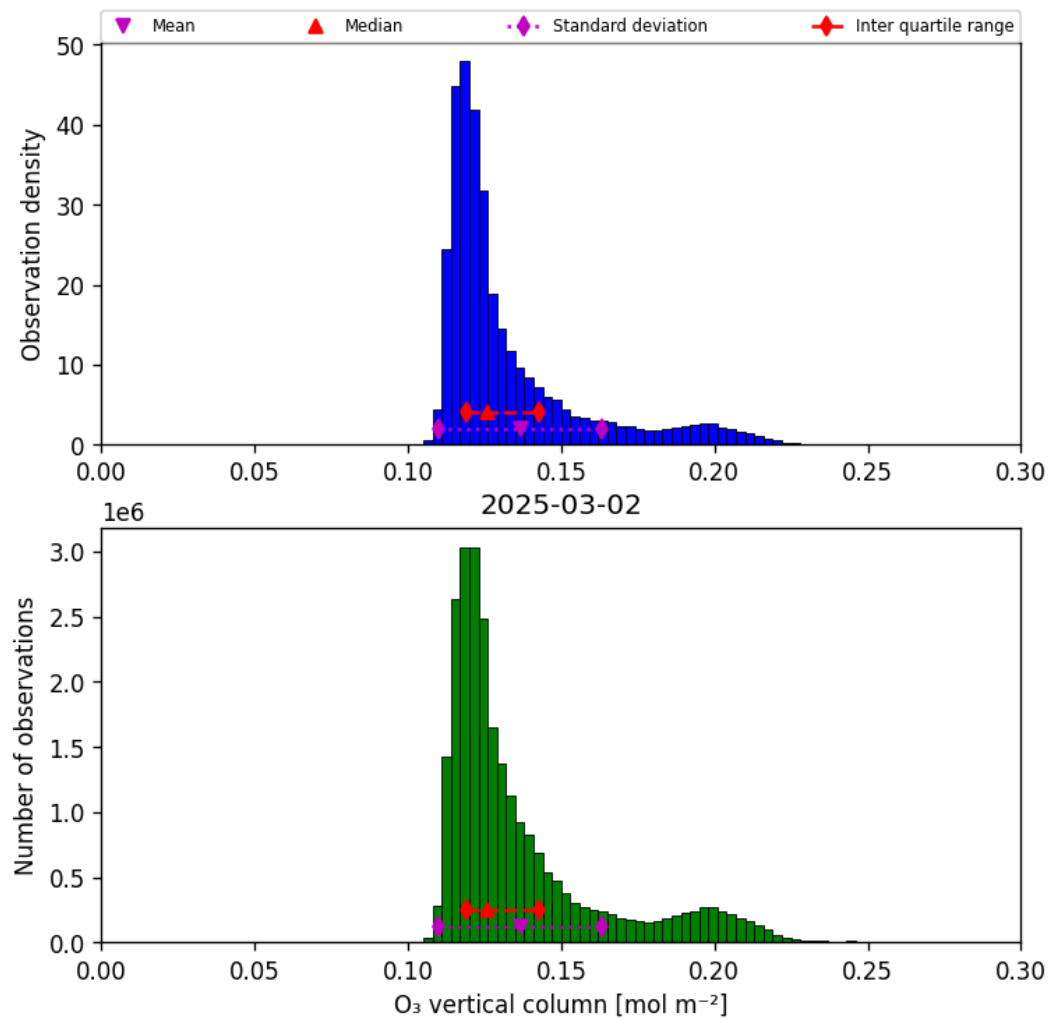
Figure 21: Histogram of “O 3 vertical column” for 2025-03-01 to 2025-03-03
