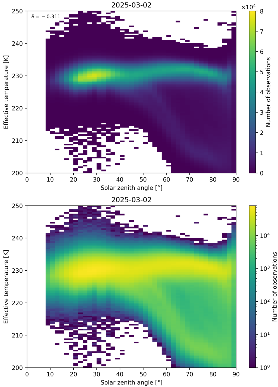
Figure 45: Scatter density plot of “Solar zenith angle” against “Effective temperature” for 2025-03-01 to 2025-03-03.
