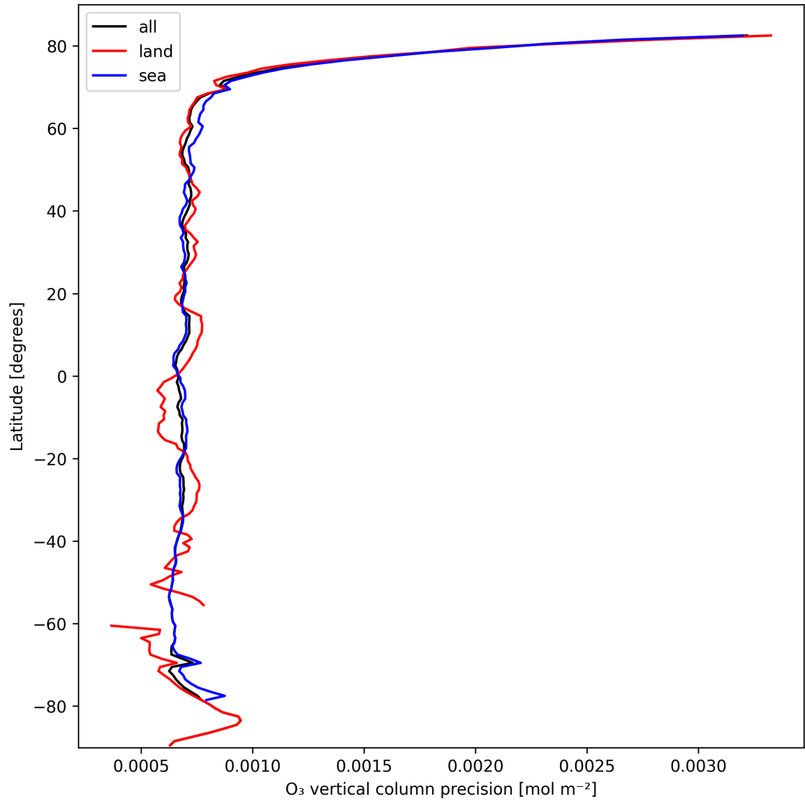
Figure 15: Zonal average of “O 3 vertical column precision” for 2025-03-01 to 2025-03-03.
