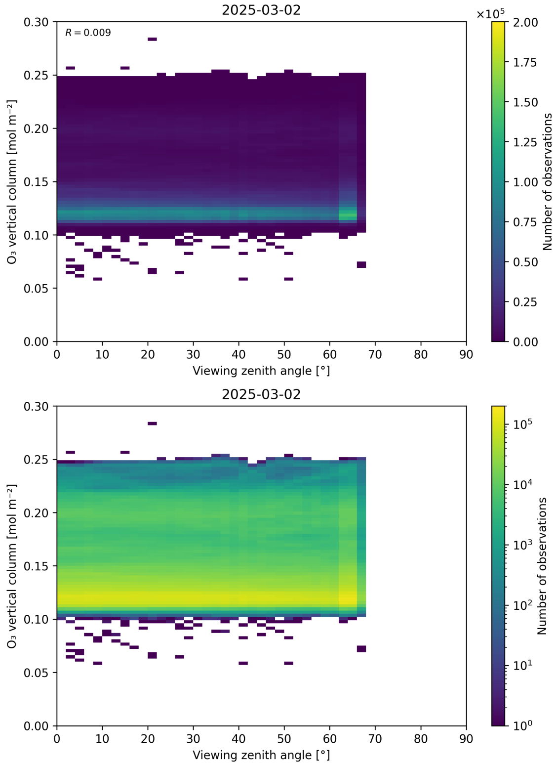
Figure 52: Scatter density plot of “Viewing zenith angle” against “O 3 vertical column” for 2025-03-01 to 2025-03-03.
