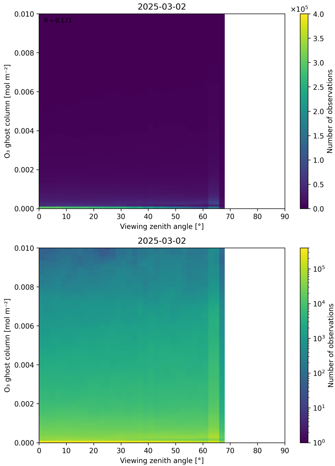
Figure 51: Scatter density plot of “Viewing zenith angle” against “O 3 ghost column” for 2025-03-01 to 2025-03-03.
