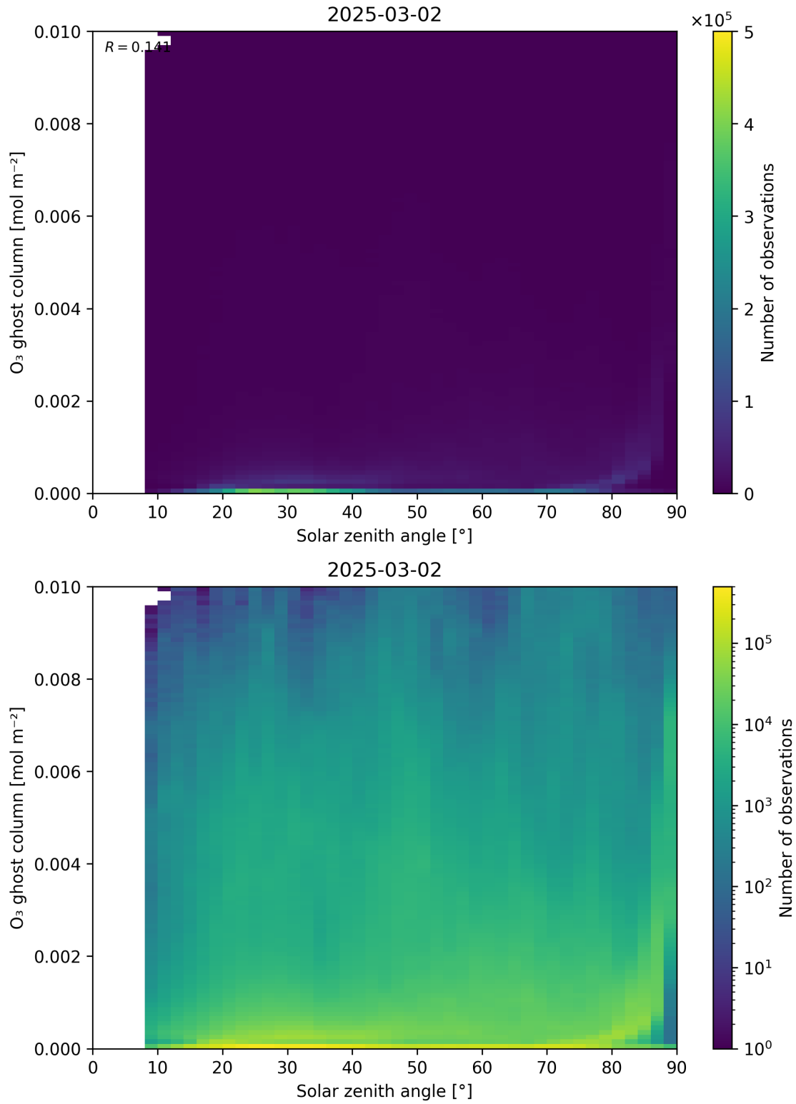
Figure 46: Scatter density plot of “Solar zenith angle” against “O 3 ghost column” for 2025-03-01 to 2025-03-03.
