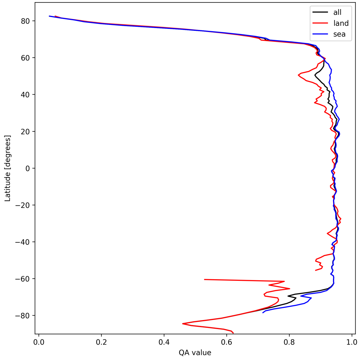
Figure 13: Zonal average of “QA value” for 2025-03-01 to 2025-03-03.
