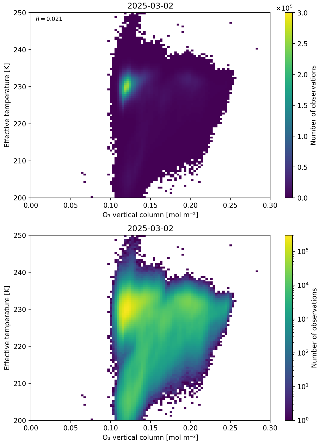
Figure 39: Scatter density plot of “O 3 vertical column” against “Effective temperature” for 2025-03-01 to 2025-03-03.
