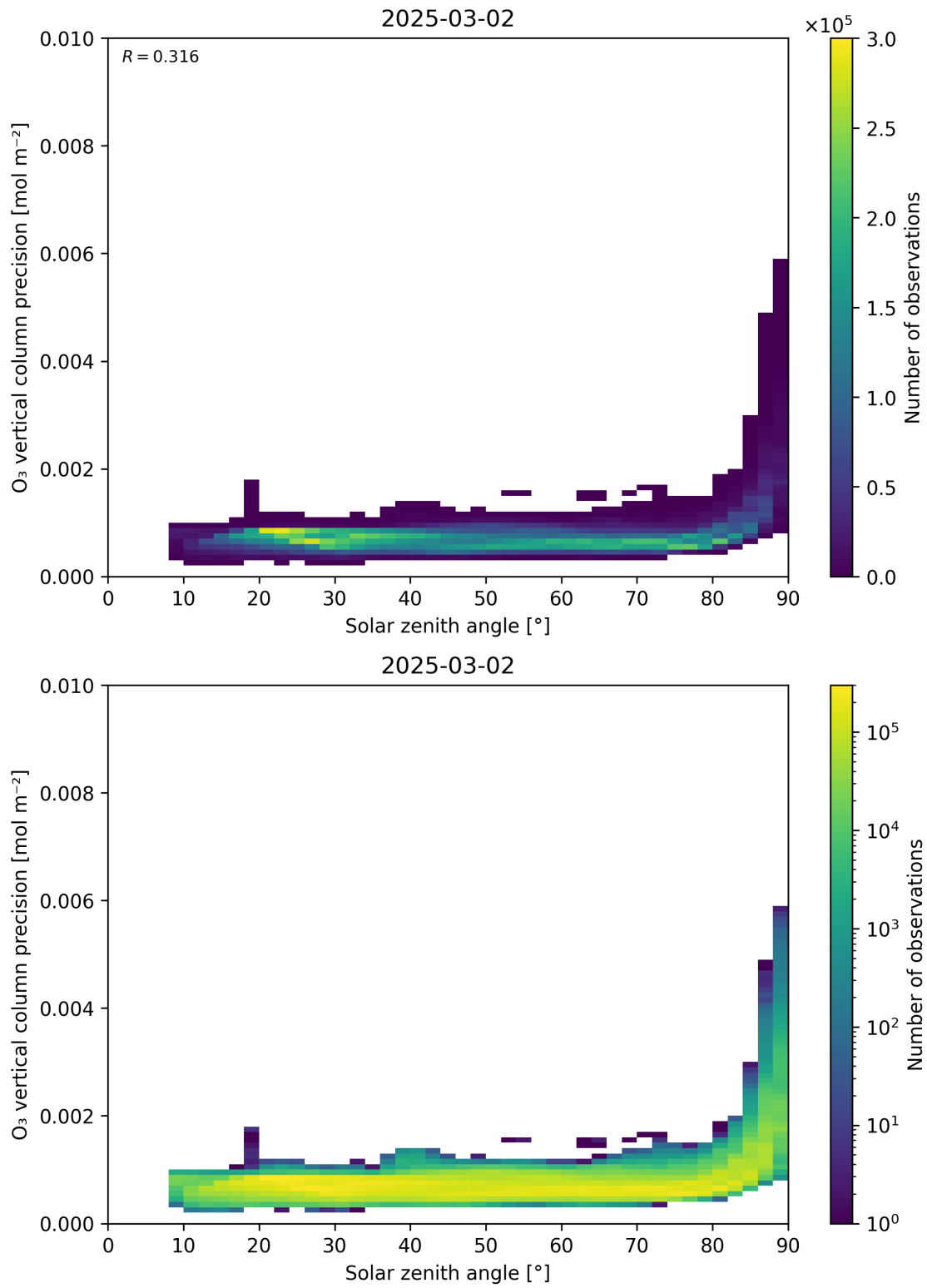
Figure 48: Scatter density plot of “Solar zenith angle” against “O 3 vertical column precision” for 2025-03-01 to 2025-03-03.
