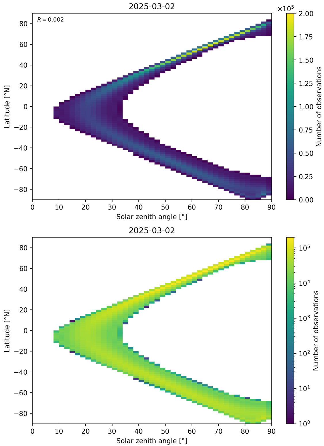
Figure 44: Scatter density plot of “Solar zenith angle” against “Latitude” for 2025-03-01 to 2025-03-03.
