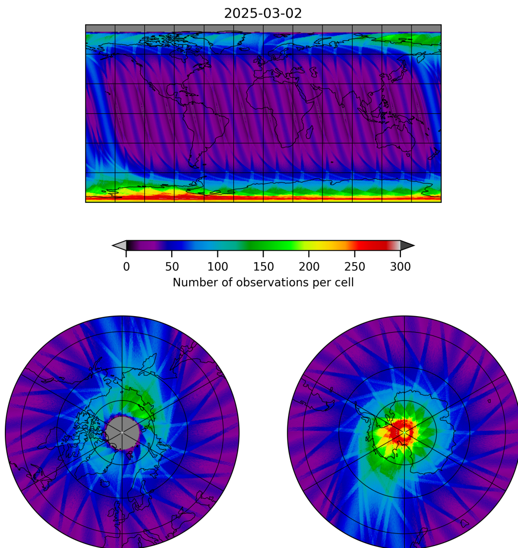
Figure 12: Map of the number of observations for 2025-03-01 to 2025-03-03
