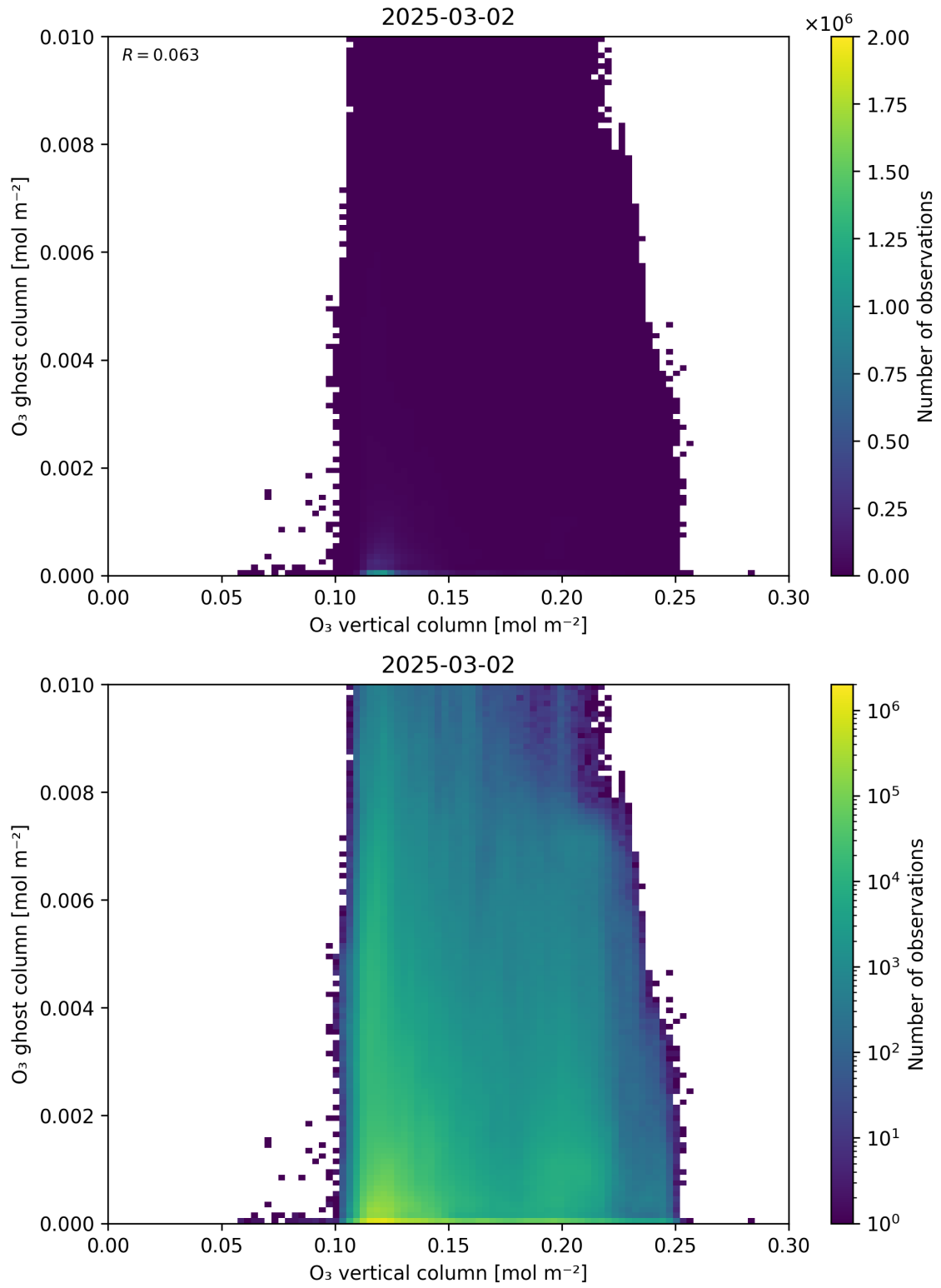
Figure 40: Scatter density plot of “O 3 vertical column” against “O 3 ghost column” for 2025-03-01 to 2025-03-03.
