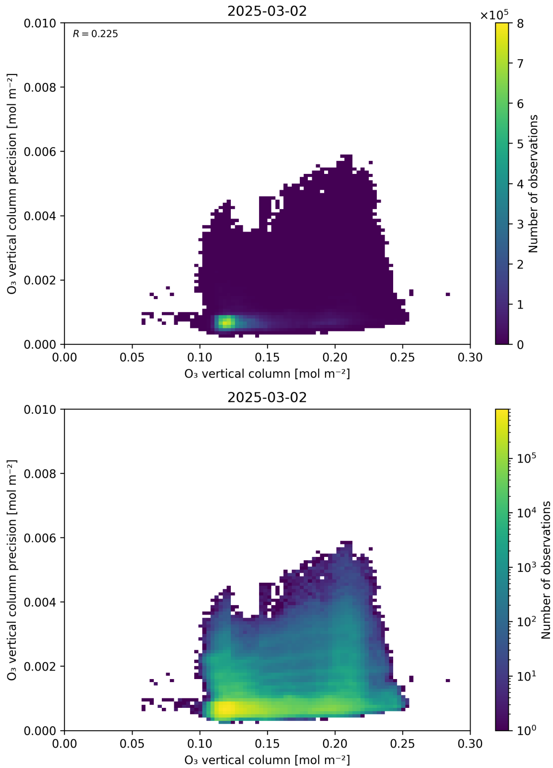
Figure 41: Scatter density plot of “O 3 vertical column” against “O 3 vertical column precision” for 2025-03-01 to 2025-03-03.
