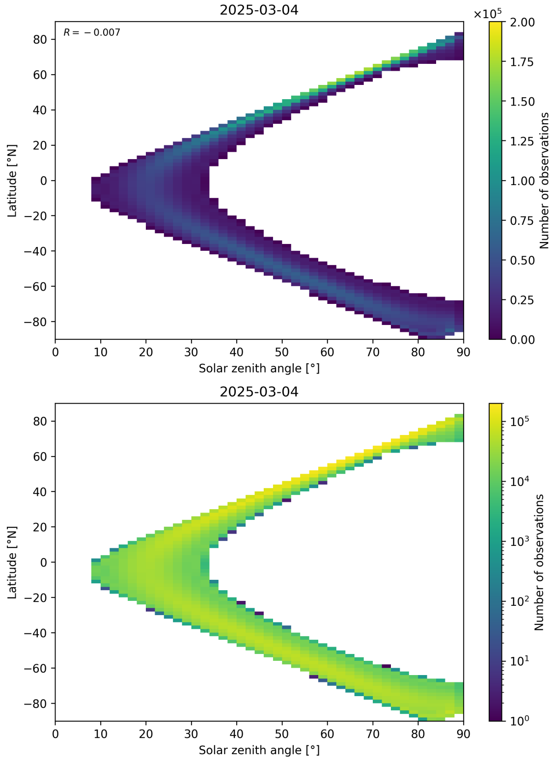
Figure 44: Scatter density plot of “Solar zenith angle” against “Latitude” for 2025-03-03 to 2025-03-05.
