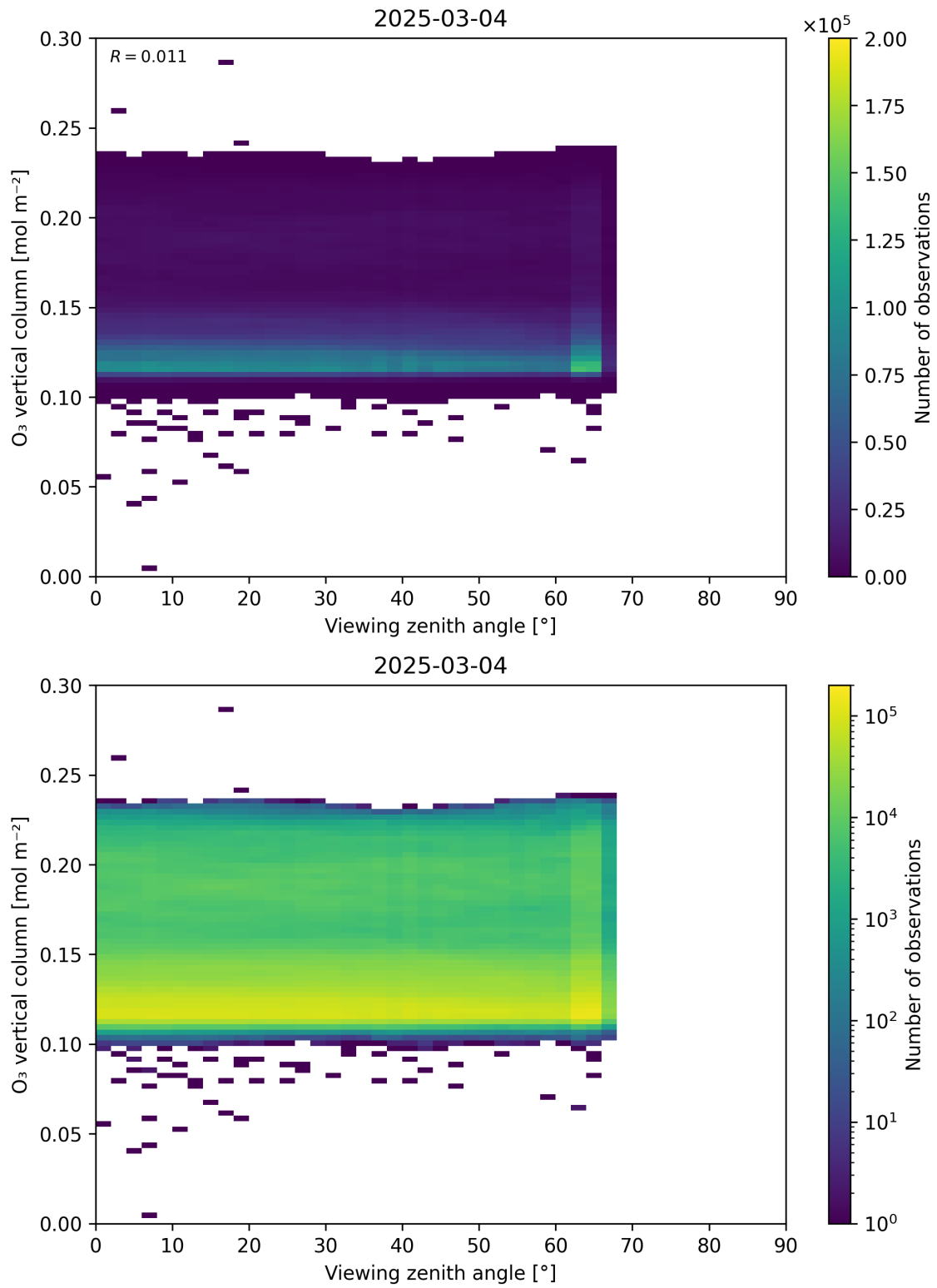
Figure 52: Scatter density plot of “Viewing zenith angle” against “O 3 vertical column” for 2025-03-03 to 2025-03-05.
