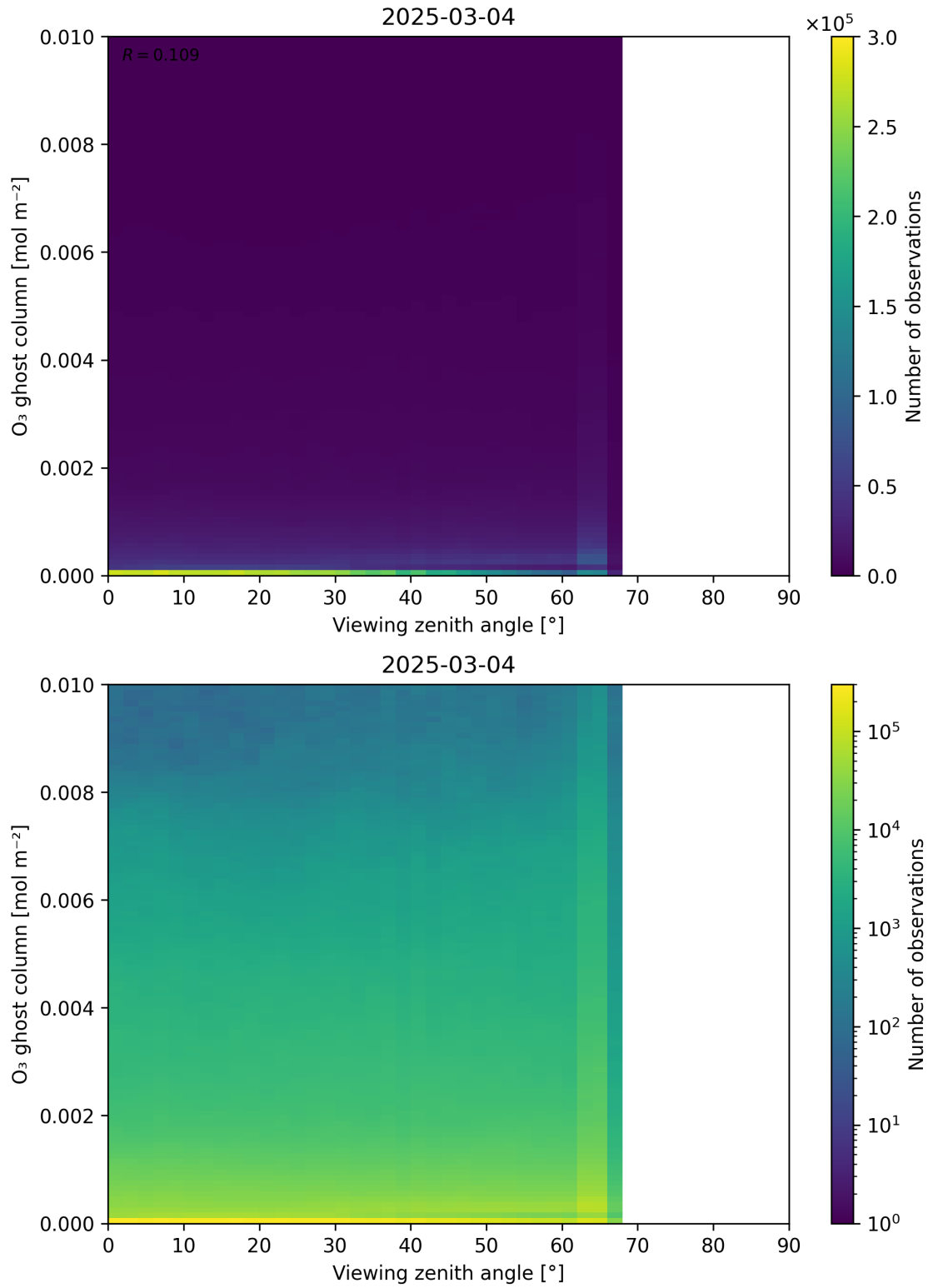
Figure 51: Scatter density plot of “Viewing zenith angle” against “O 3 ghost column” for 2025-03-03 to 2025-03-05.
