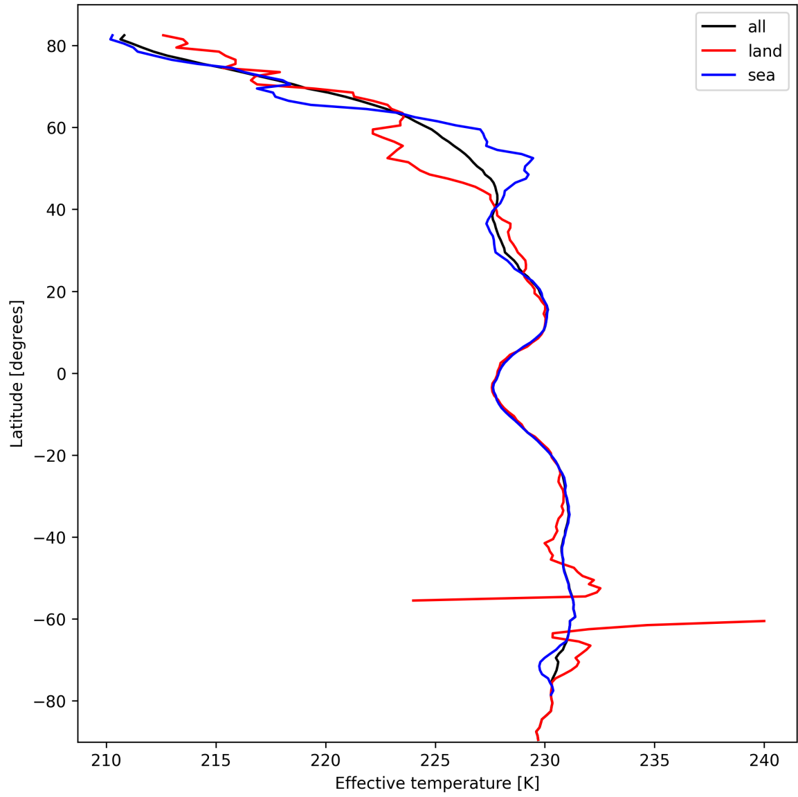
Figure 17: Zonal average of “Effective temperature” for 2025-03-03 to 2025-03-05.
