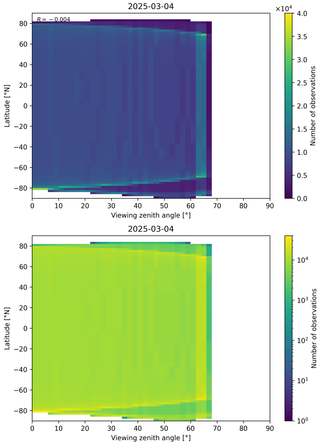
Figure 49: Scatter density plot of “Viewing zenith angle” against “Latitude” for 2025-03-03 to 2025-03-05.
