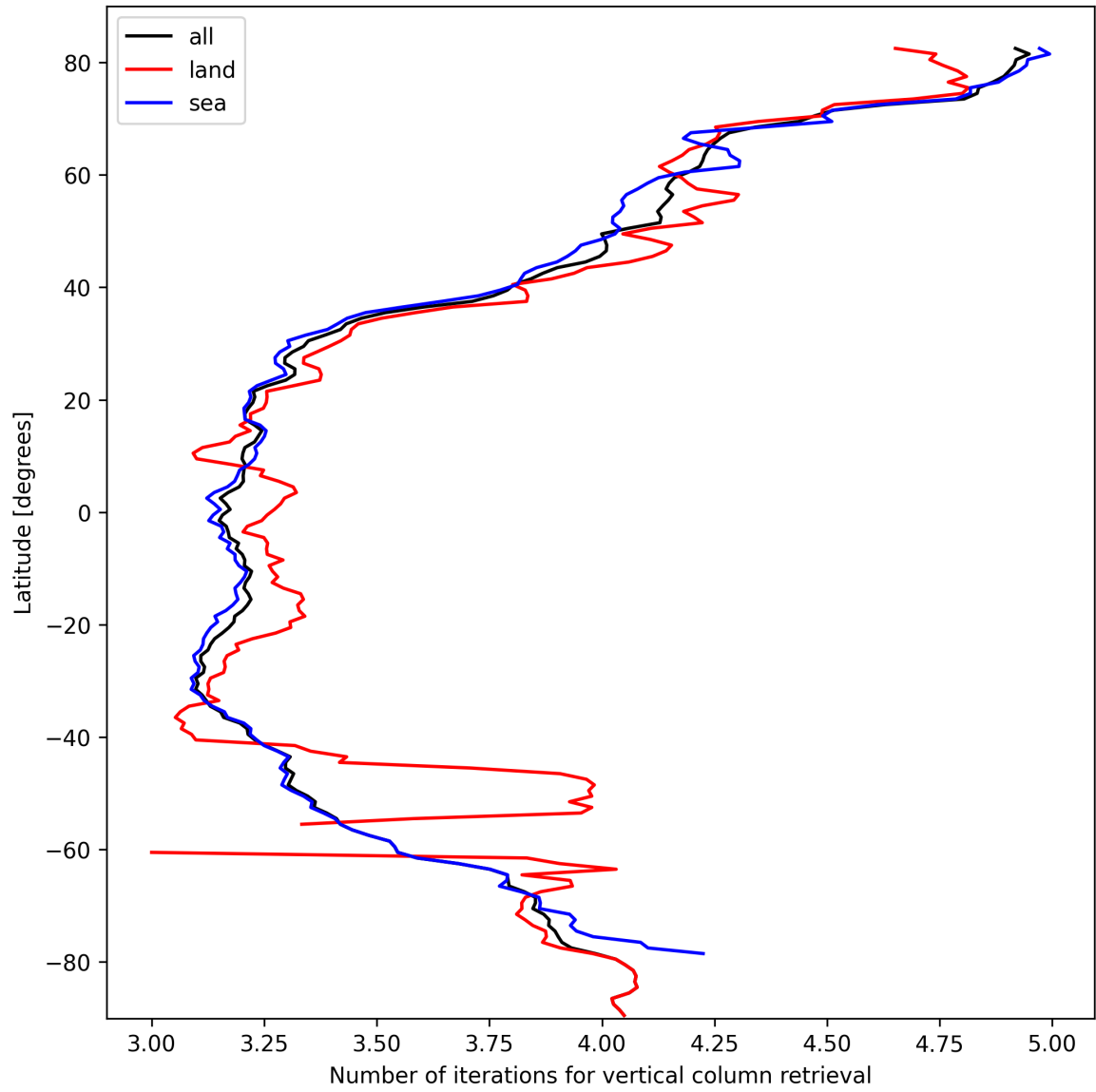
Figure 19: Zonal average of “Number of iterations for vertical column retrieval” for 2025-03-03 to 2025-03-05.
