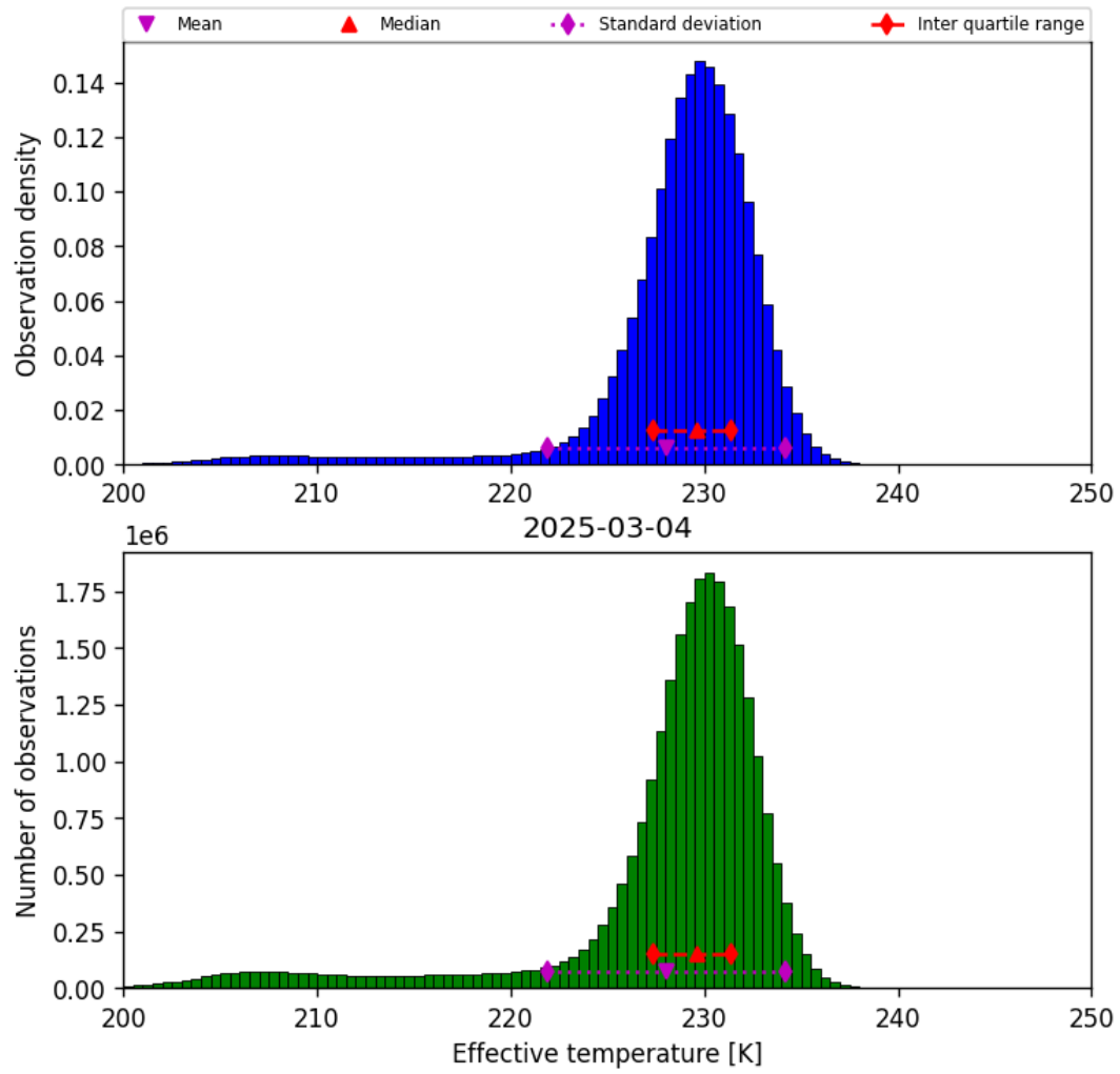
Figure 24: Histogram of “Effective temperature” for 2025-03-03 to 2025-03-05
