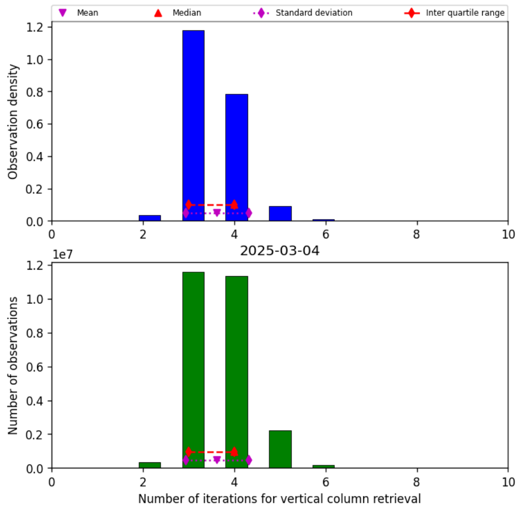
Figure 26: Histogram of “Number of iterations for vertical column retrieval” for 2025-03-03 to 2025-03-05
