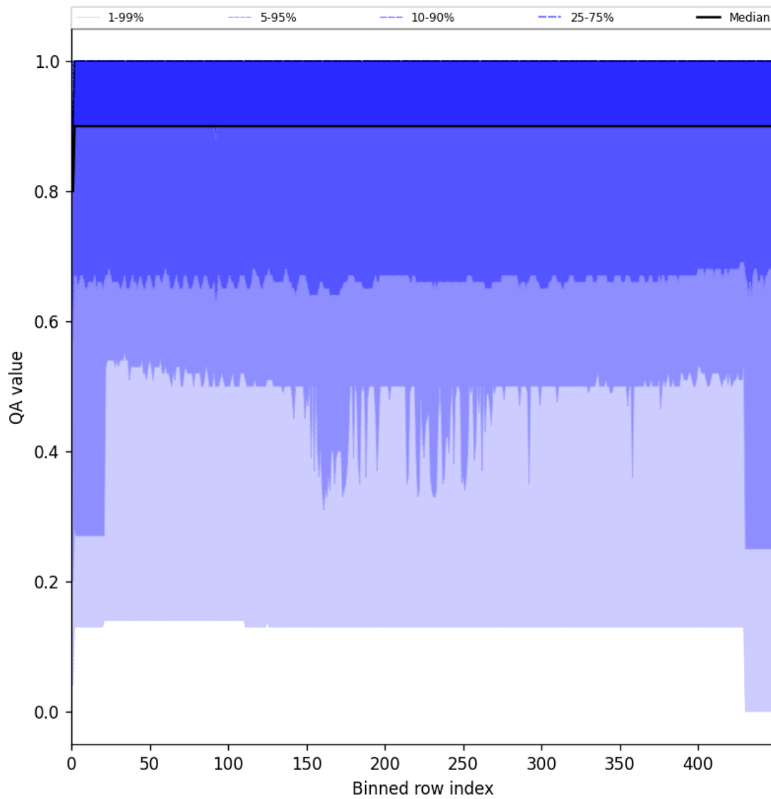
Figure 27: Along track statistics of “QA value” for 2025-03-03 to 2025-03-05
