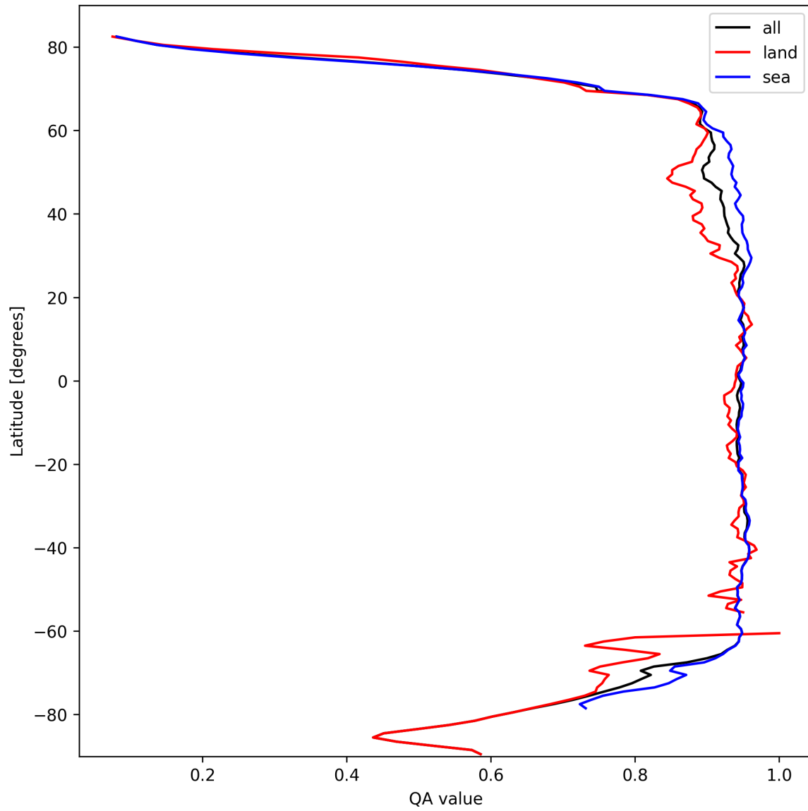
Figure 13: Zonal average of “QA value” for 2025-03-03 to 2025-03-05.
