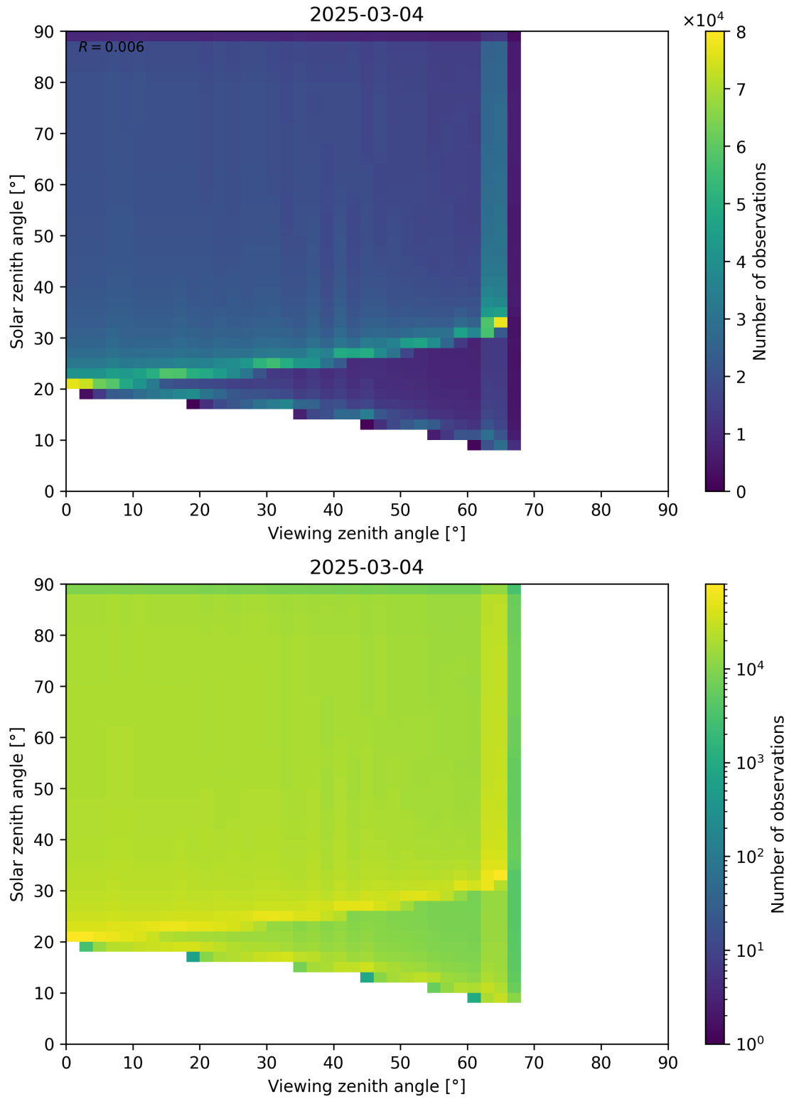
Figure 54: Scatter density plot of “Viewing zenith angle” against “Solar zenith angle” for 2025-03-03 to 2025-03-05.
