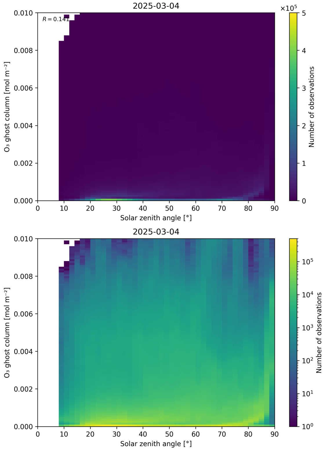
Figure 46: Scatter density plot of “Solar zenith angle” against “O 3 ghost column” for 2025-03-03 to 2025-03-05.
