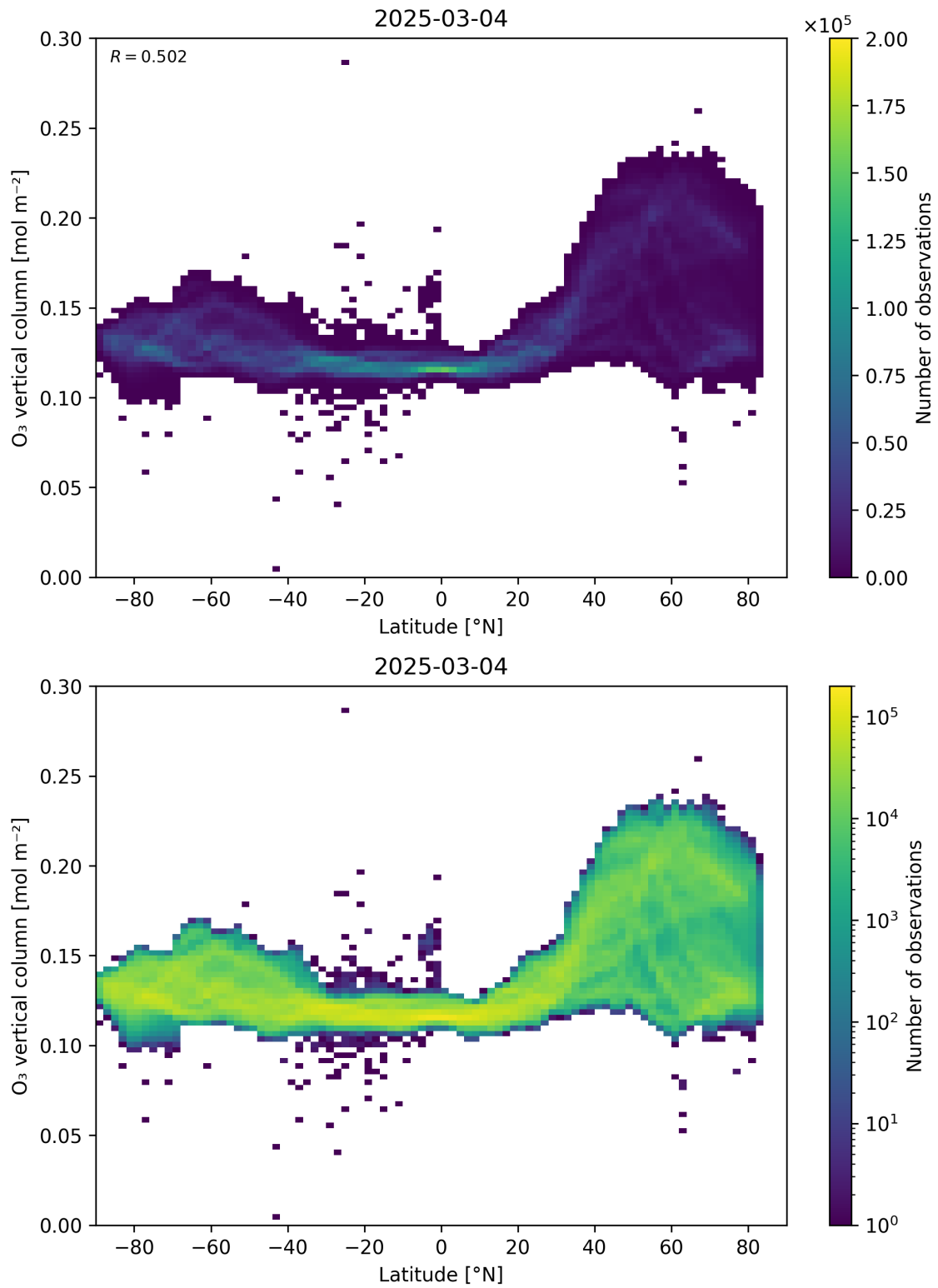
Figure 36: Scatter density plot of “Latitude” against “O 3 vertical column” for 2025-03-03 to 2025-03-05.
