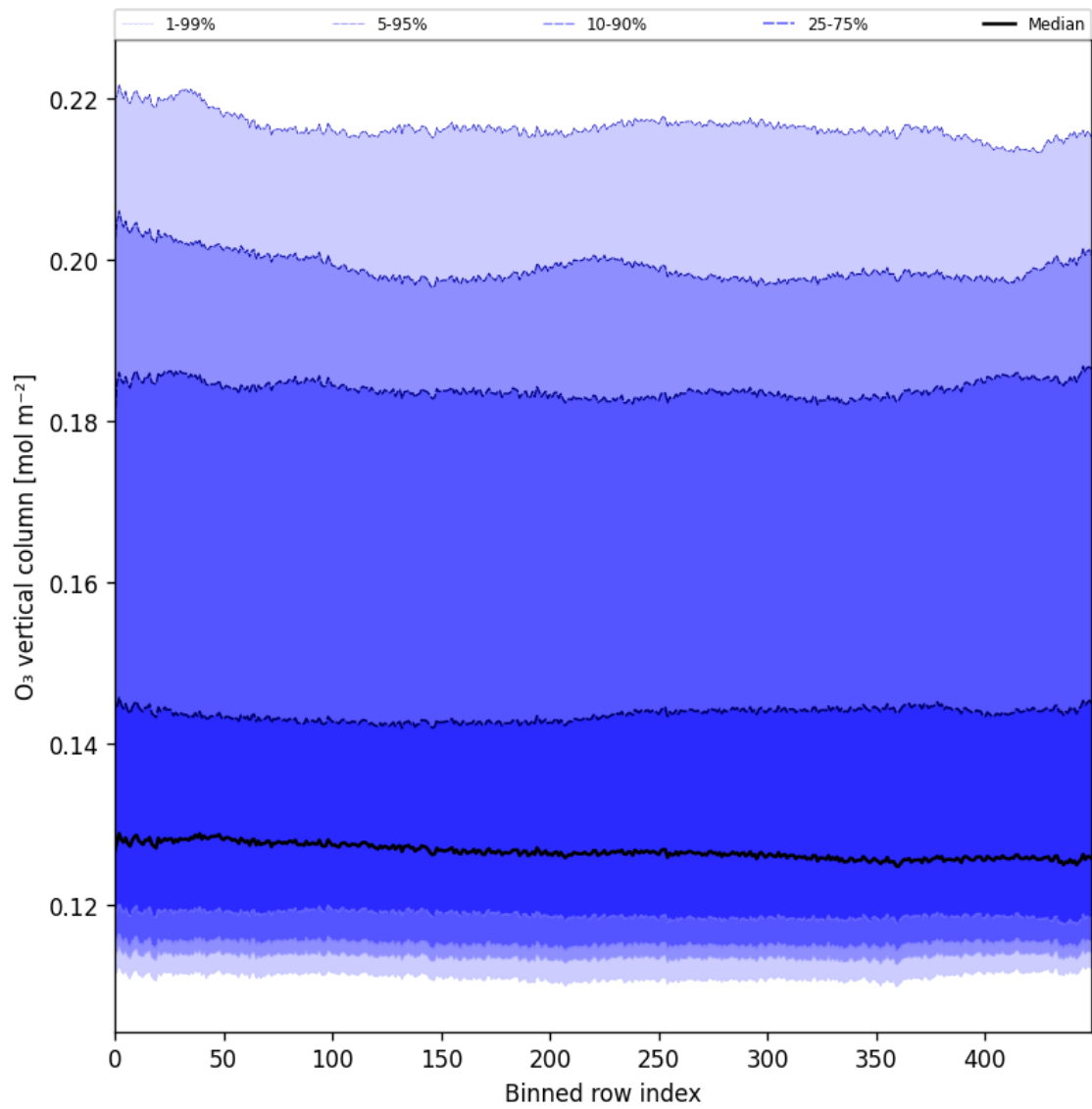
Figure 28: Along track statistics of “O 3 vertical column” for 2025-03-03 to 2025-03-05
