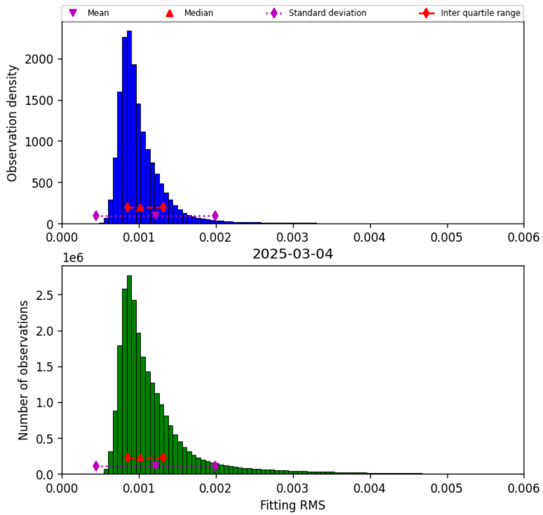
Figure 23: Histogram of “Fitting RMS” for 2025-03-03 to 2025-03-05
