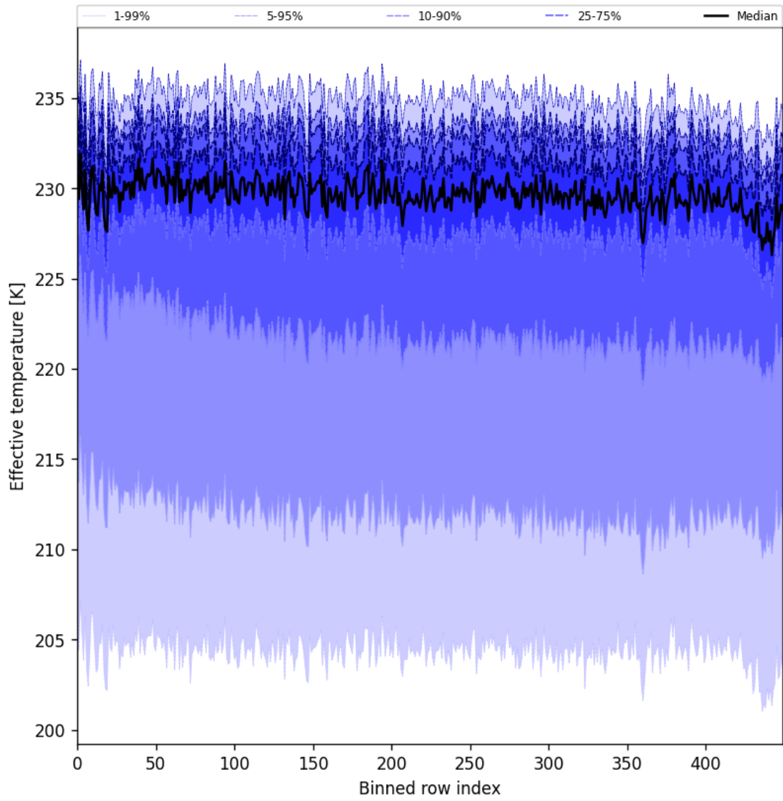
Figure 31: Along track statistics of “Effective temperature” for 2025-03-03 to 2025-03-05
