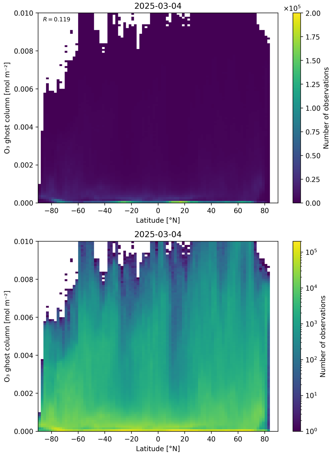
Figure 35: Scatter density plot of “Latitude” against “O 3 ghost column” for 2025-03-03 to 2025-03-05.
