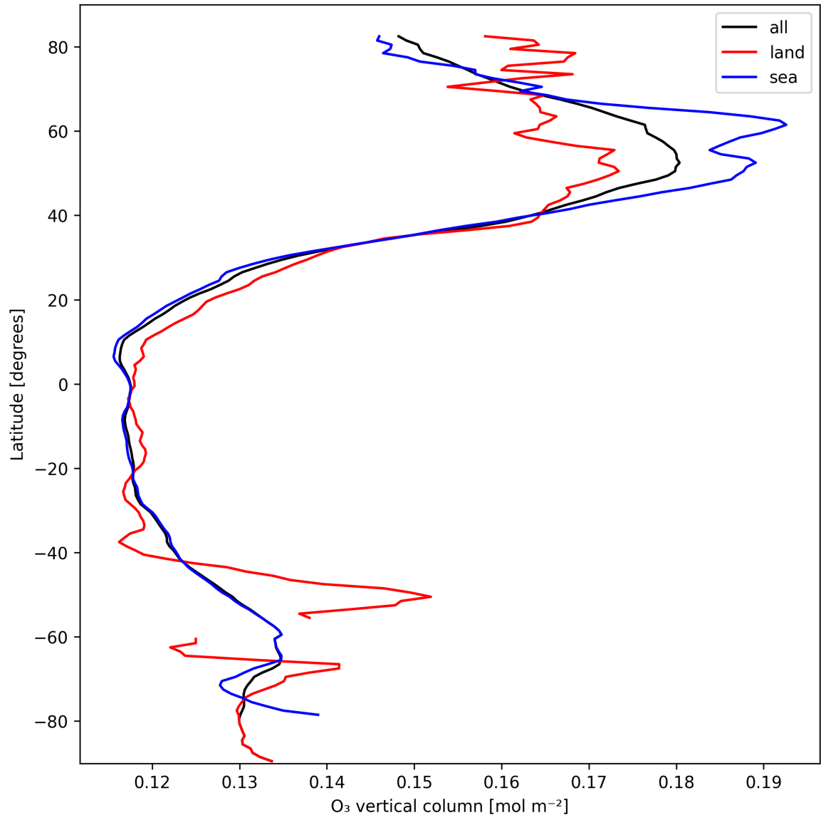
Figure 14: Zonal average of “O 3 vertical column” for 2025-03-03 to 2025-03-05.
