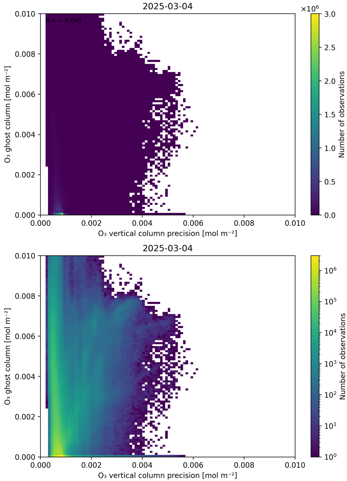
Figure 43: Scatter density plot of “O 3 vertical column precision” against “O 3 ghost column” for 2025-03-03 to 2025-03-05.
