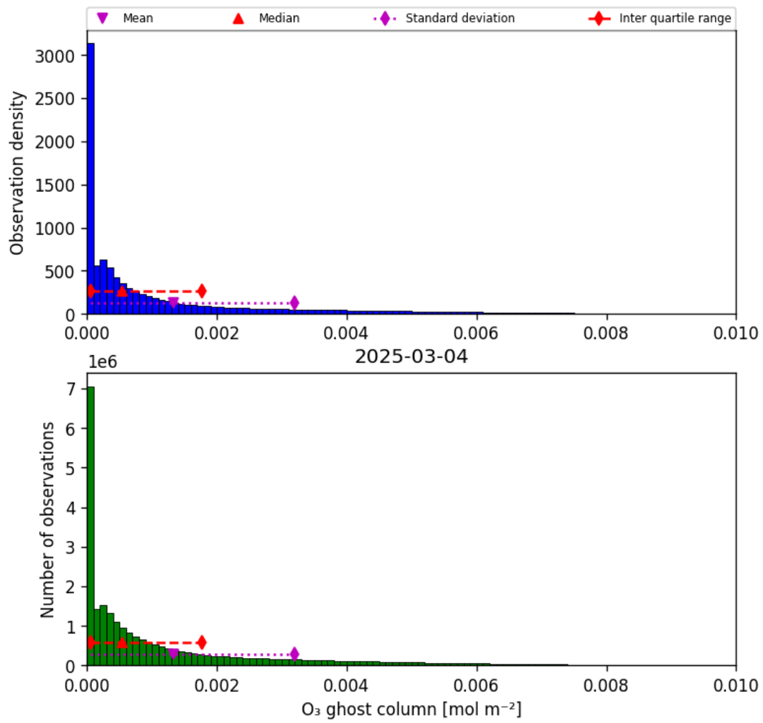
Figure 25: Histogram of “O 3 ghost column” for 2025-03-03 to 2025-03-05
