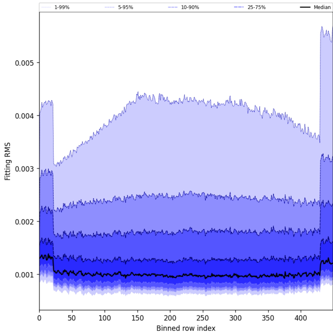
Figure 30: Along track statistics of “Fitting RMS” for 2025-03-03 to 2025-03-05
