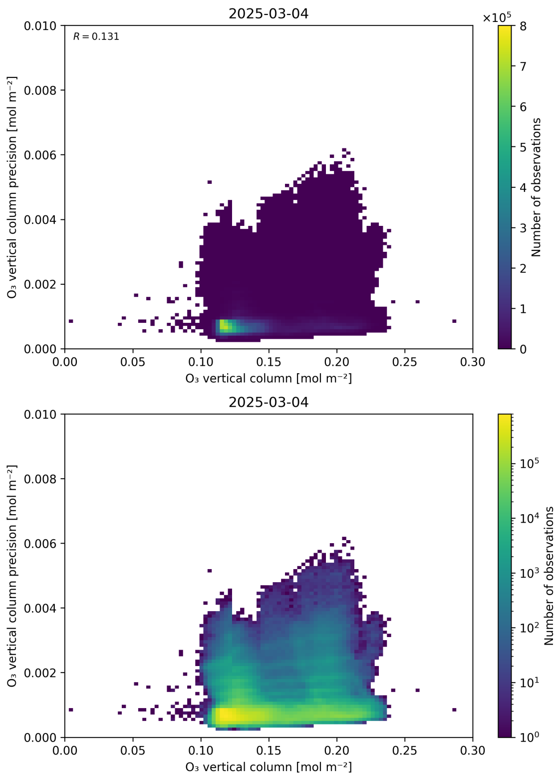
Figure 41: Scatter density plot of “O 3 vertical column” against “O 3 vertical column precision” for 2025-03-03 to 2025-03-05.
