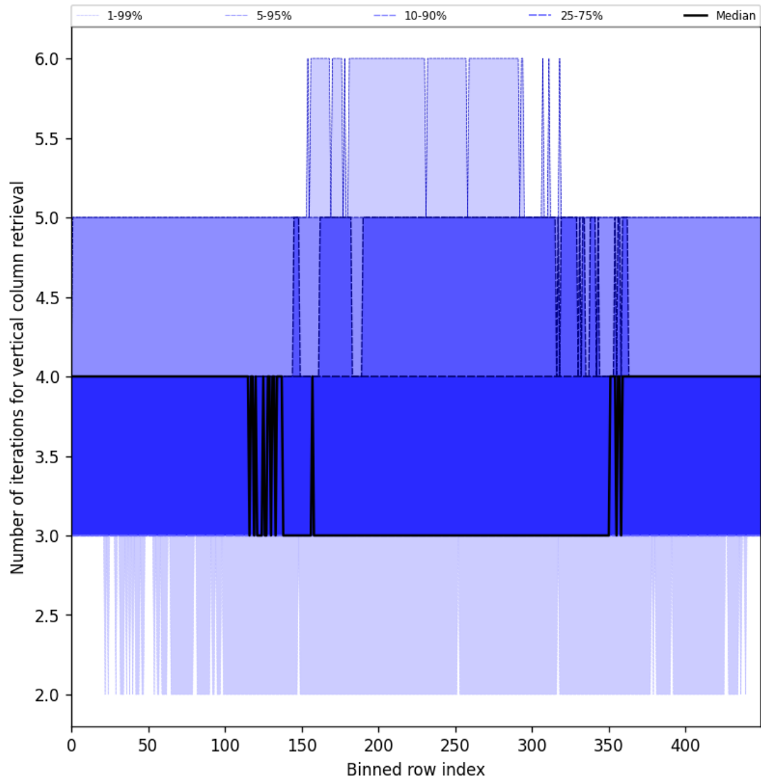
Figure 33: Along track statistics of “Number of iterations for vertical column retrieval” for 2025-03-03 to 2025-03-05
