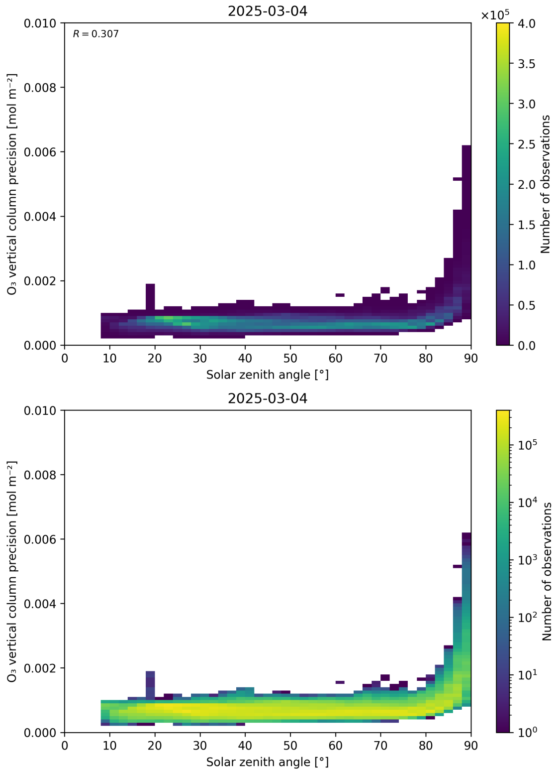
Figure 48: Scatter density plot of “Solar zenith angle” against “O 3 vertical column precision” for 2025-03-03 to 2025-03-05.
