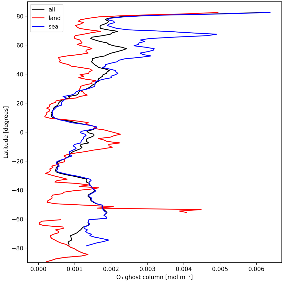
Figure 18: Zonal average of “O 3 ghost column” for 2025-03-03 to 2025-03-05.
