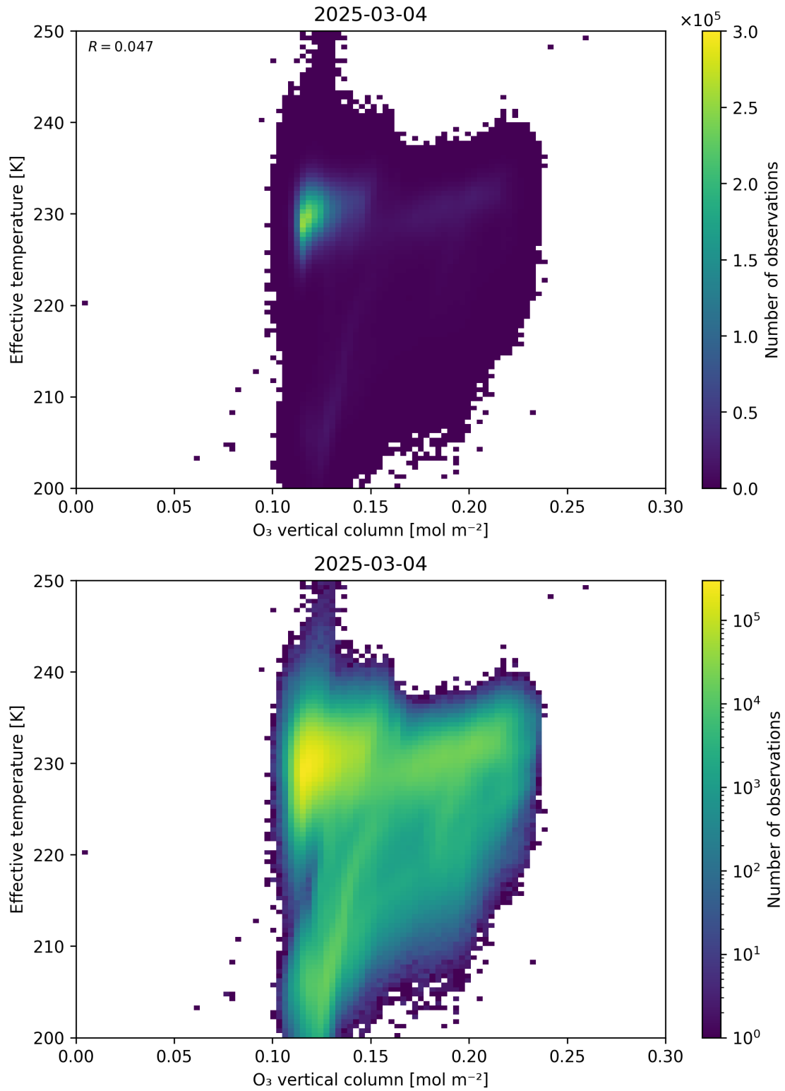
Figure 39: Scatter density plot of “O 3 vertical column” against “Effective temperature” for 2025-03-03 to 2025-03-05.
