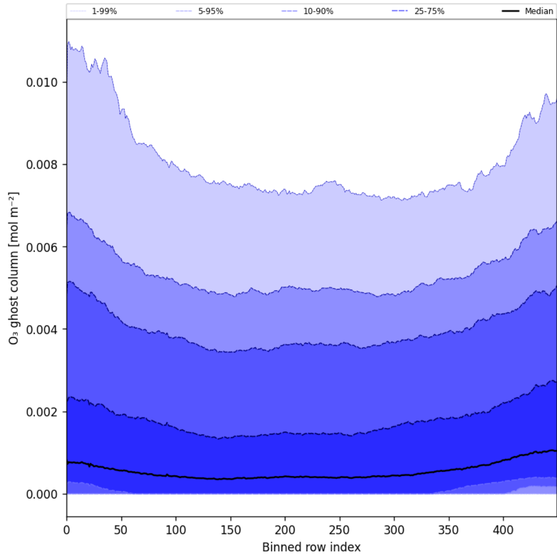
Figure 32: Along track statistics of “O 3 ghost column” for 2025-03-03 to 2025-03-05
