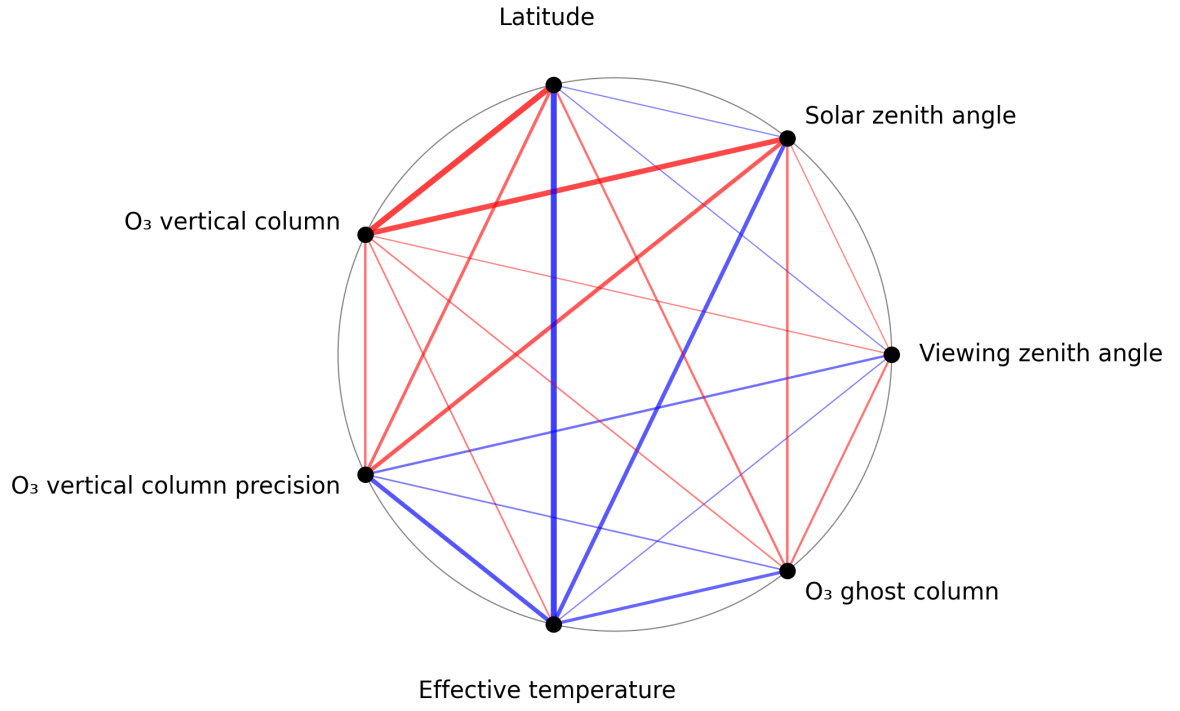
Figure 1: Map of correlation graph for 2025-03-03 to 2025-03-05.
