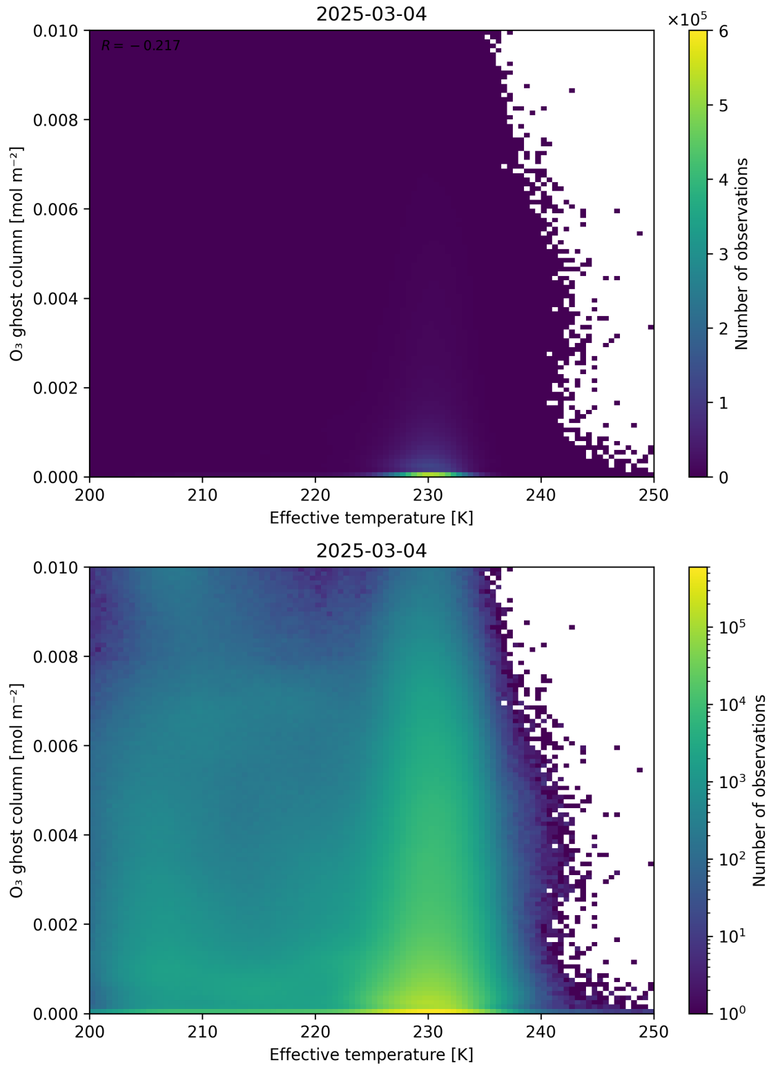
Figure 38: Scatter density plot of “Effective temperature” against “O 3 ghost column” for 2025-03-03 to 2025-03-05.
