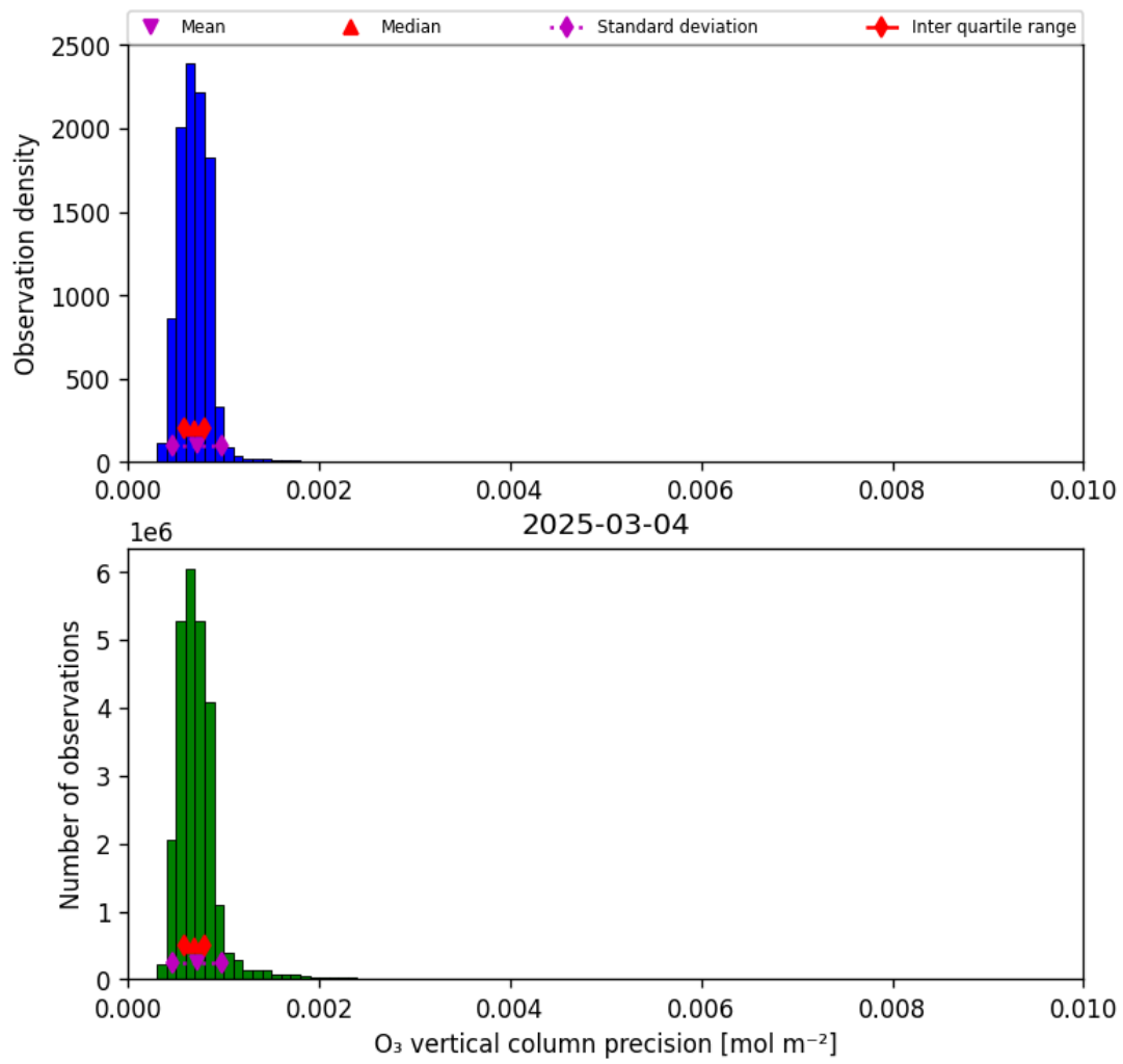
Figure 22: Histogram of "O 3 vertical column precision" for 2025-03-03 to 2025-03-05
