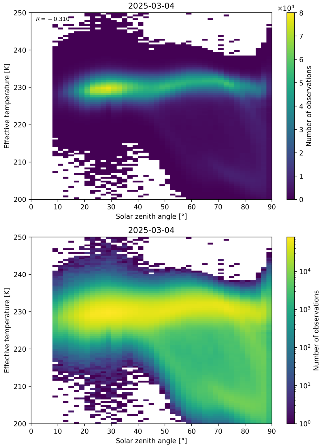
Figure 45: Scatter density plot of “Solar zenith angle” against “Effective temperature” for 2025-03-03 to 2025-03-05.
