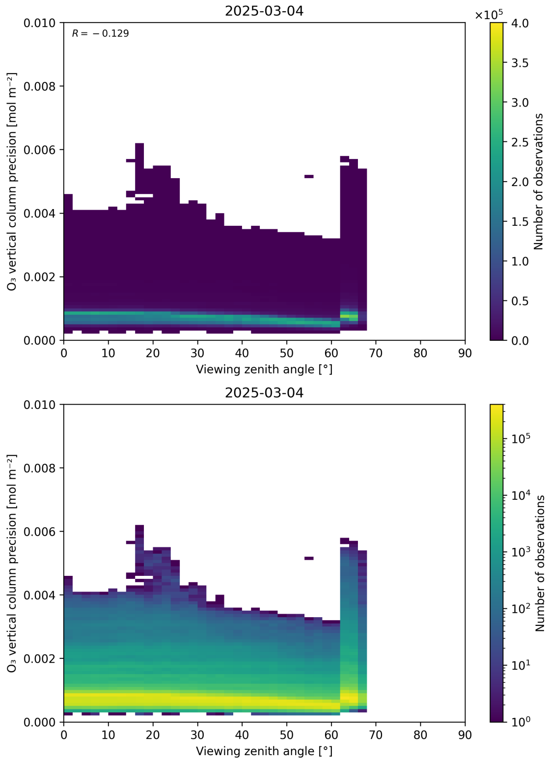
Figure 53: Scatter density plot of “Viewing zenith angle” against “O 3 vertical column precision” for 2025-03-03 to 2025-03-05.
