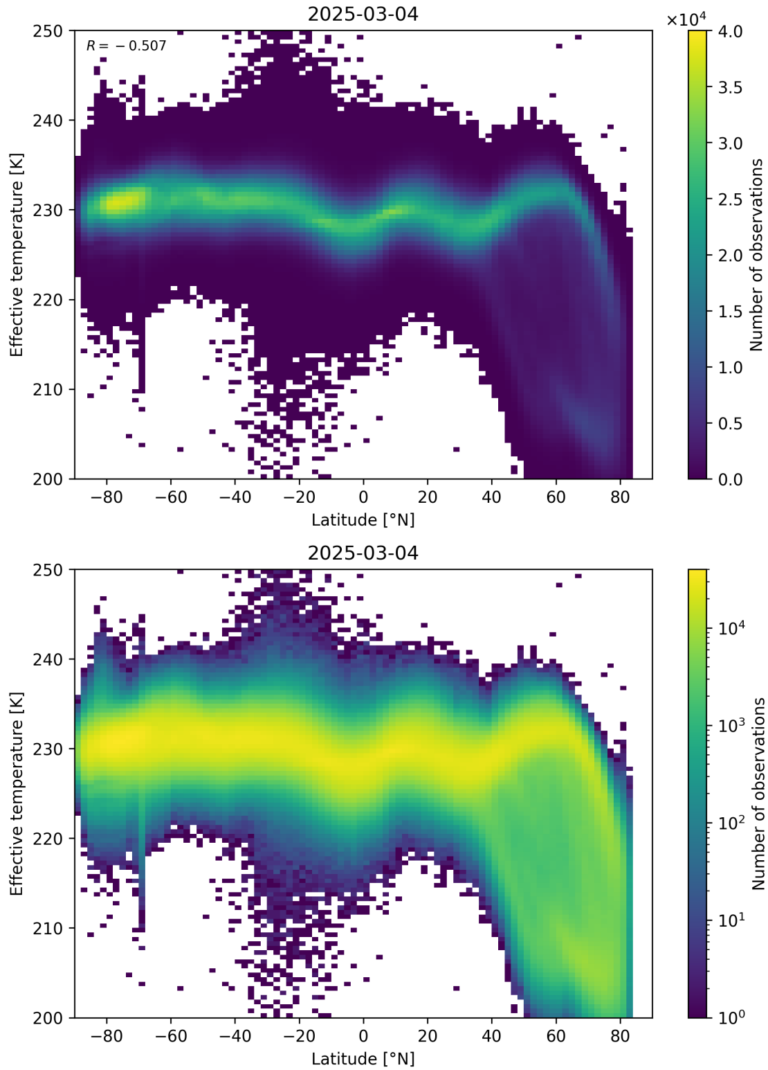
Figure 34: Scatter density plot of “Latitude” against “Effective temperature” for 2025-03-03 to 2025-03-05.
