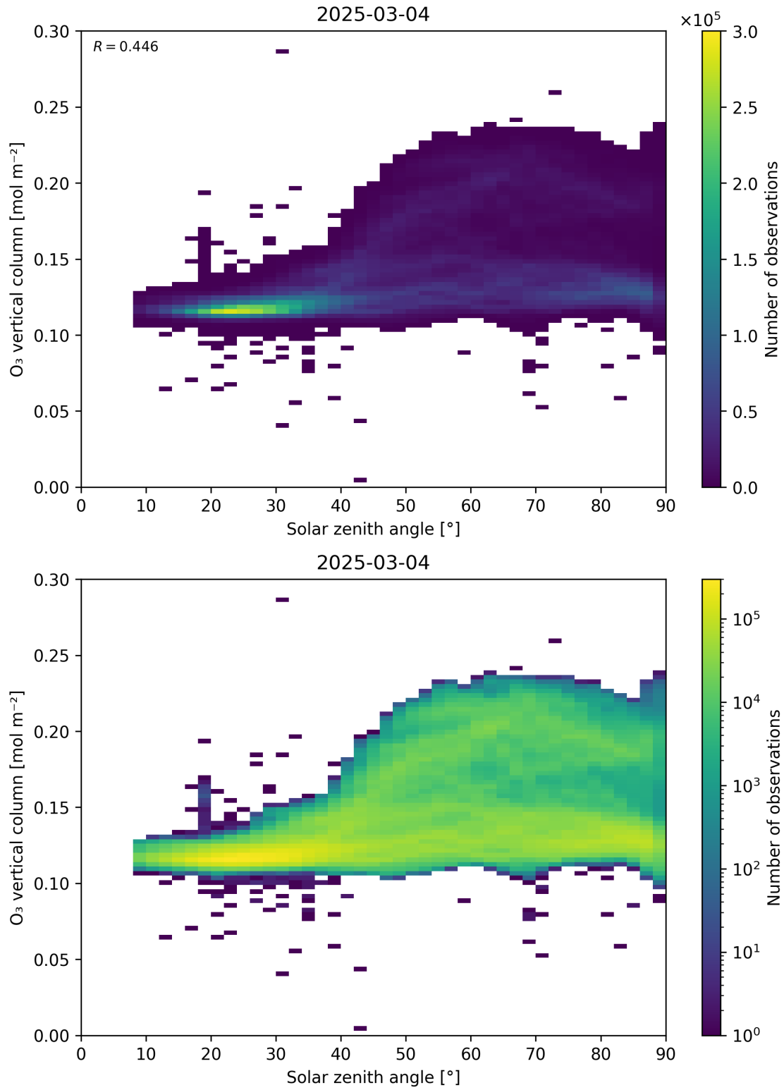
Figure 47: Scatter density plot of “Solar zenith angle” against “O 3 vertical column” for 2025-03-03 to 2025-03-05.
