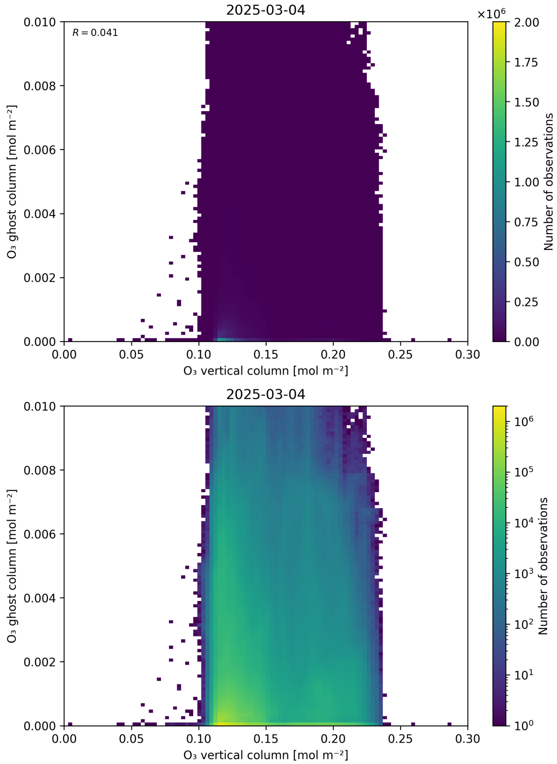
Figure 40: Scatter density plot of “O 3 vertical column” against “O 3 ghost column” for 2025-03-03 to 2025-03-05.
