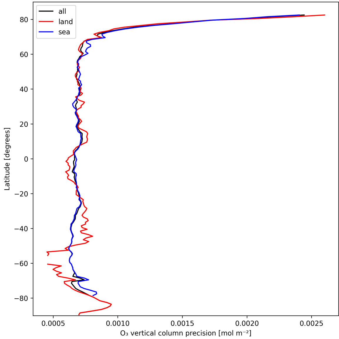
Figure 15: Zonal average of “O 3 vertical column precision” for 2025-03-03 to 2025-03-05.
