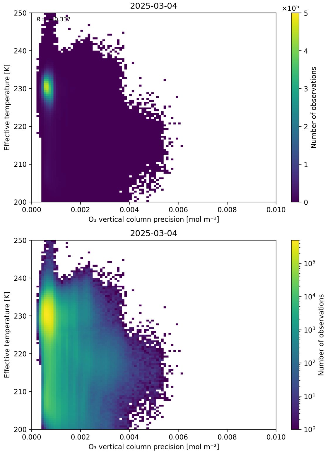
Figure 42: Scatter density plot of “O 3 vertical column precision” against “Effective temperature” for 2025-03-03 to 2025-03-05.
