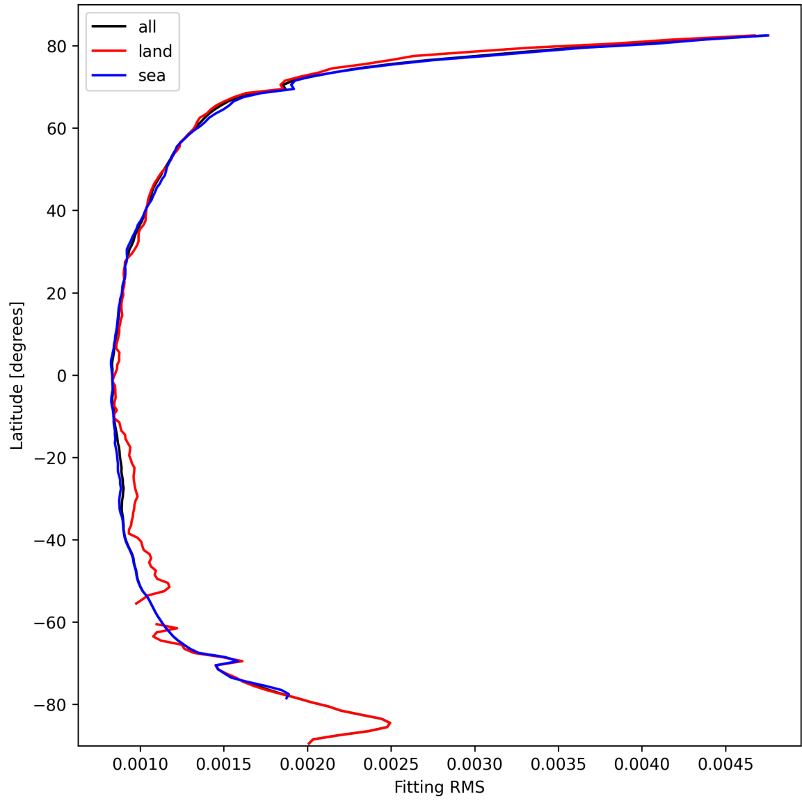
Figure 16: Zonal average of “Fitting RMS” for 2025-03-03 to 2025-03-05.
