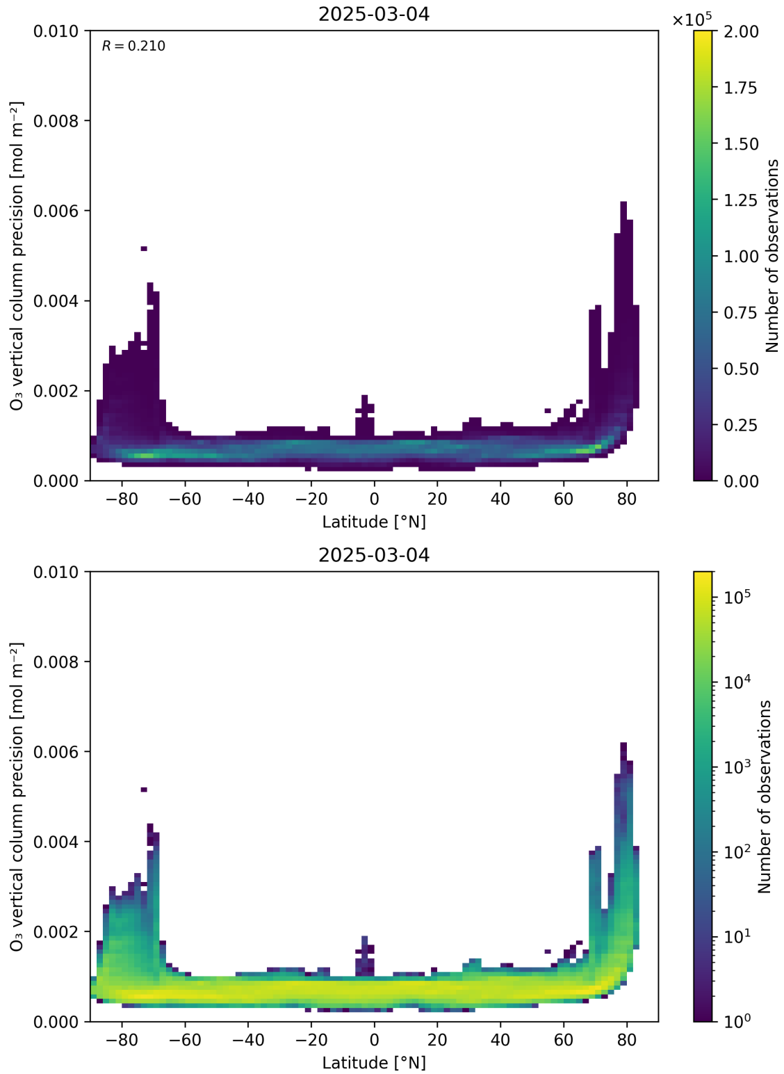
Figure 37: Scatter density plot of “Latitude” against “O 3 vertical column precision” for 2025-03-03 to 2025-03-05.
