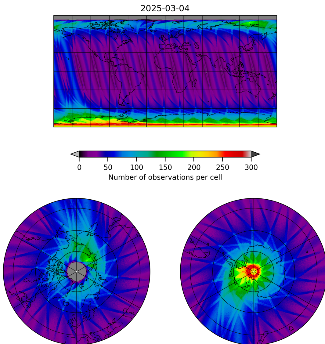
Figure 12: Map of the number of observations for 2025-03-03 to 2025-03-05
