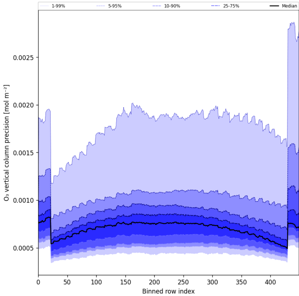
Figure 29: Along track statistics of “O 3 vertical column precision” for 2025-03-03 to 2025-03-05
