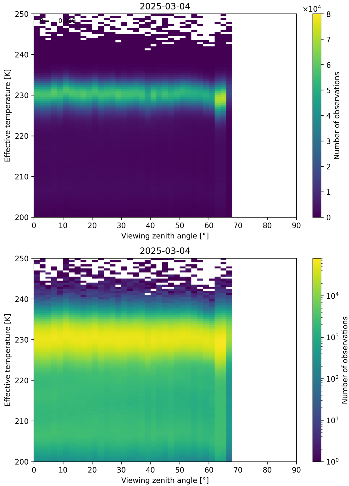
Figure 50: Scatter density plot of “Viewing zenith angle” against “Effective temperature” for 2025-03-03 to 2025-03-05.
