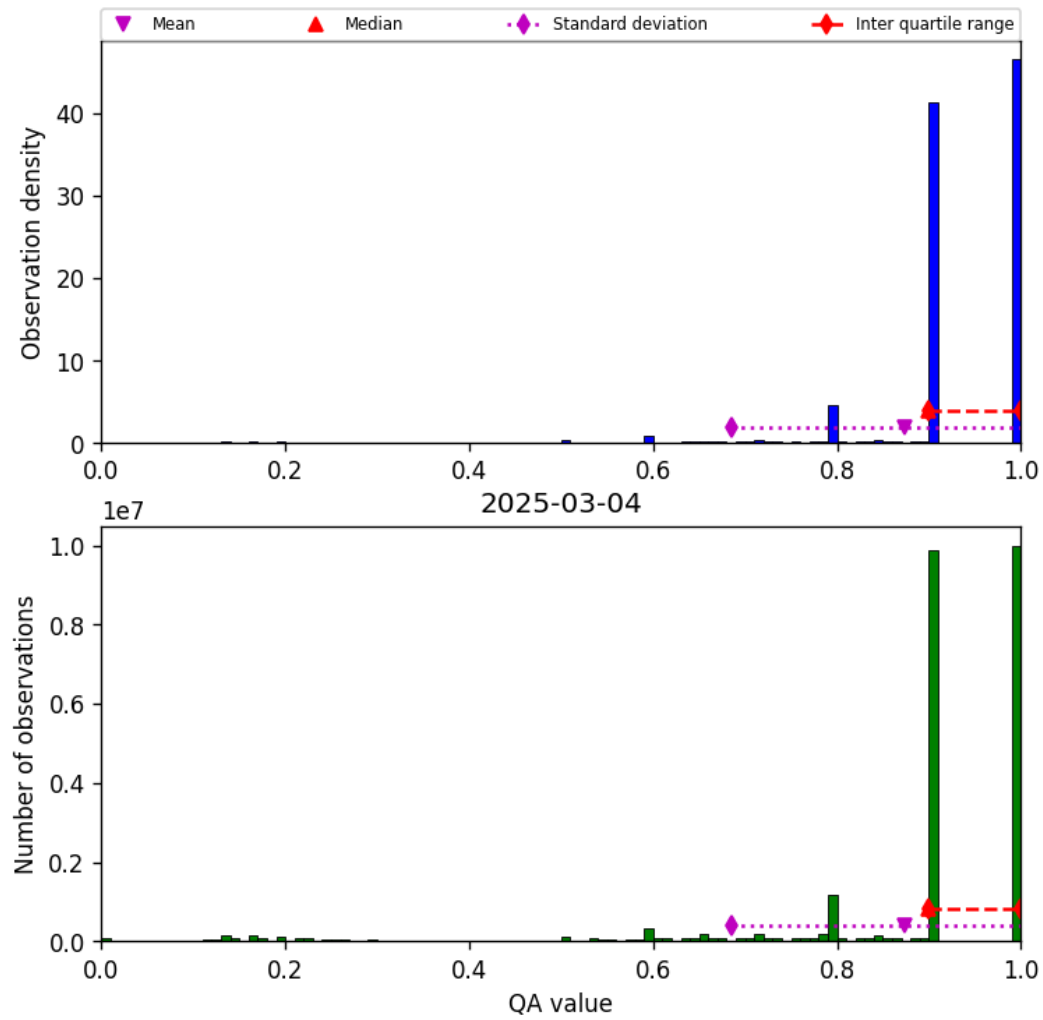
Figure 20: Histogram of “QA value” for 2025-03-03 to 2025-03-05
