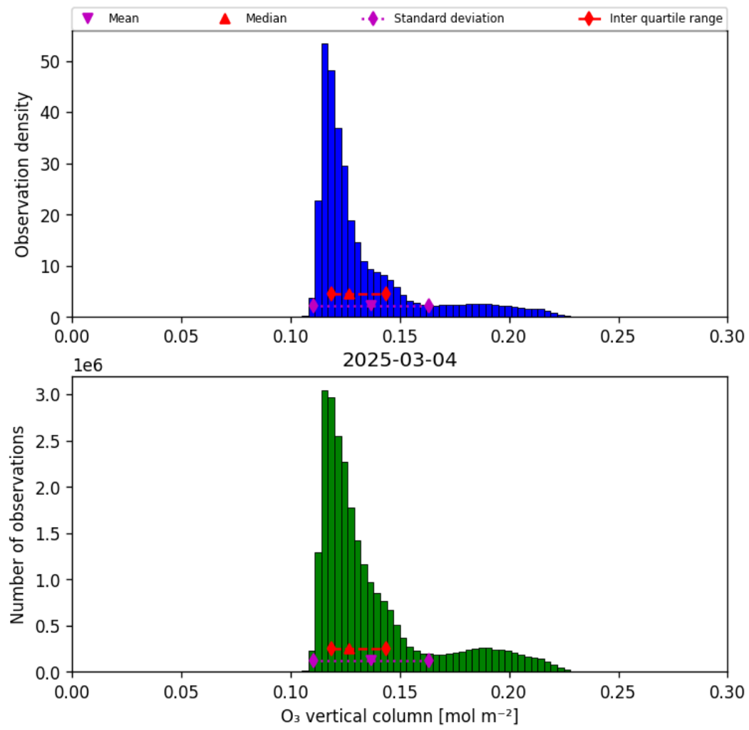
Figure 21: Histogram of “O 3 vertical column” for 2025-03-03 to 2025-03-05
