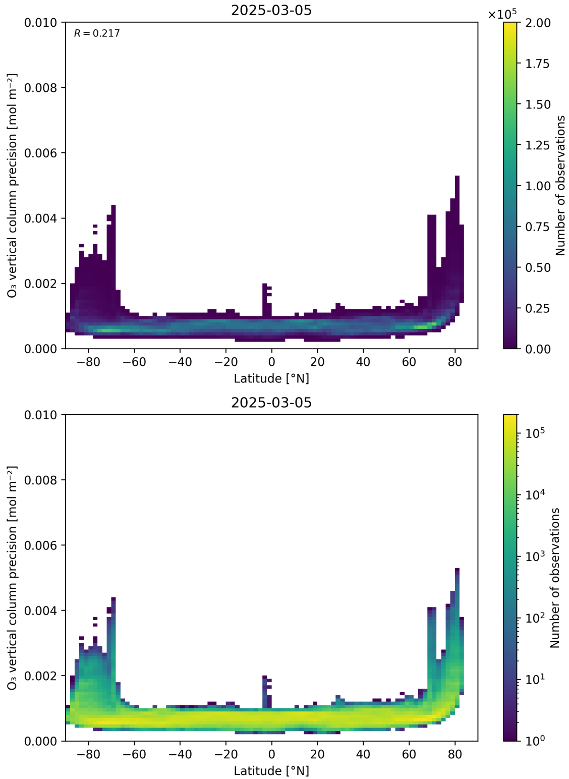
Figure 37: Scatter density plot of “Latitude” against “O 3 vertical column precision” for 2025-03-04 to 2025-03-06.
