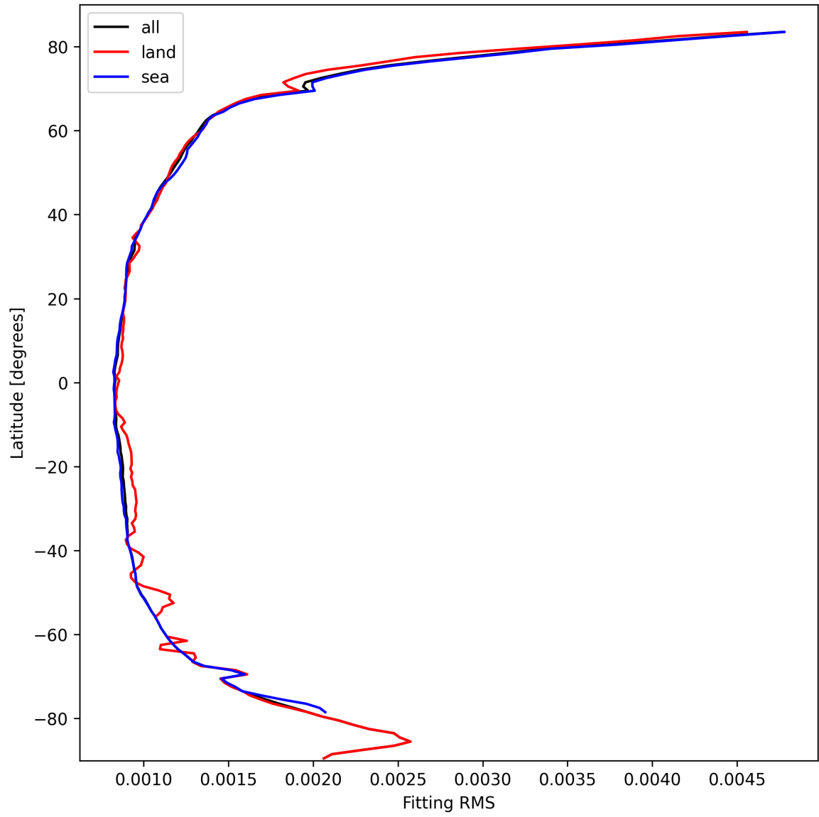
Figure 16: Zonal average of “Fitting RMS” for 2025-03-04 to 2025-03-06.
