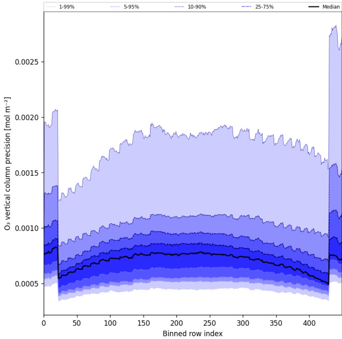
Figure 29: Along track statistics of “O 3 vertical column precision” for 2025-03-04 to 2025-03-06
