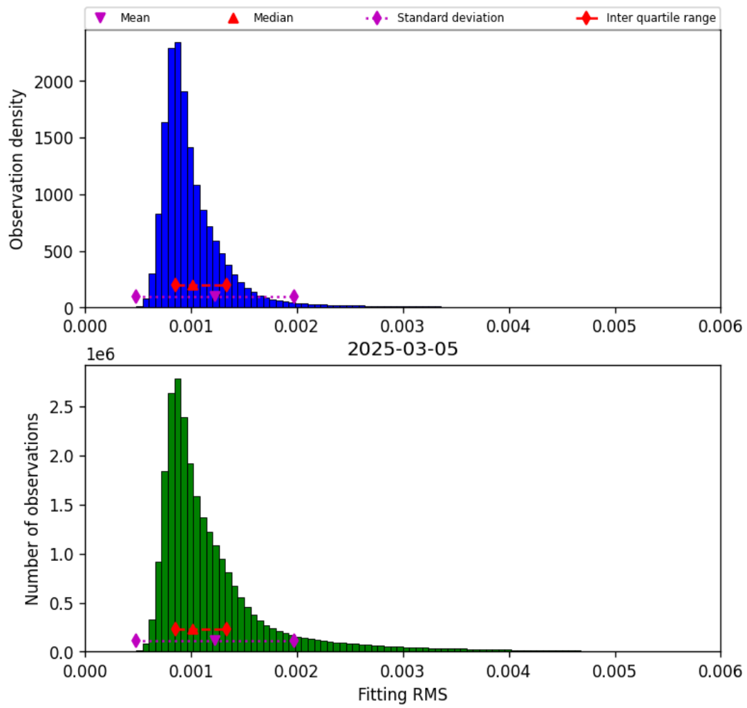
Figure 23: Histogram of “Fitting RMS” for 2025-03-04 to 2025-03-06
