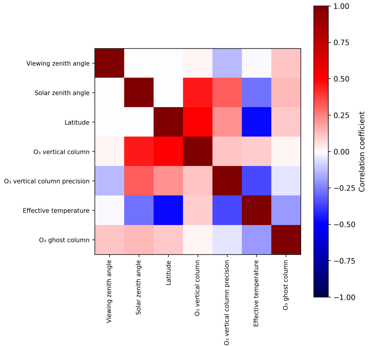
Figure 2: Map of correlation matrix for 2025-03-04 to 2025-03-06.
