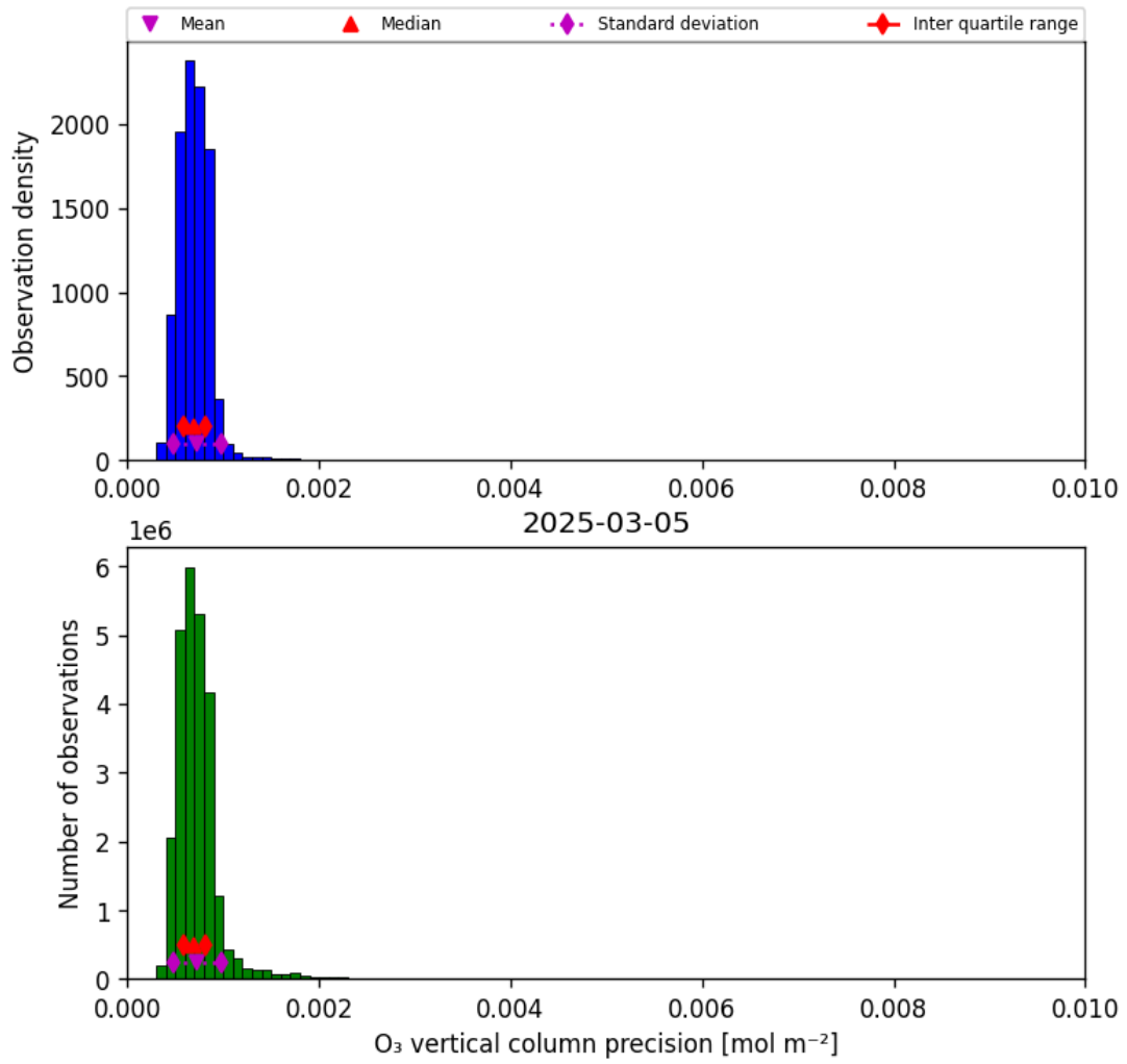
Figure 22: Histogram of “O 3 vertical column precision” for 2025-03-04 to 2025-03-06
