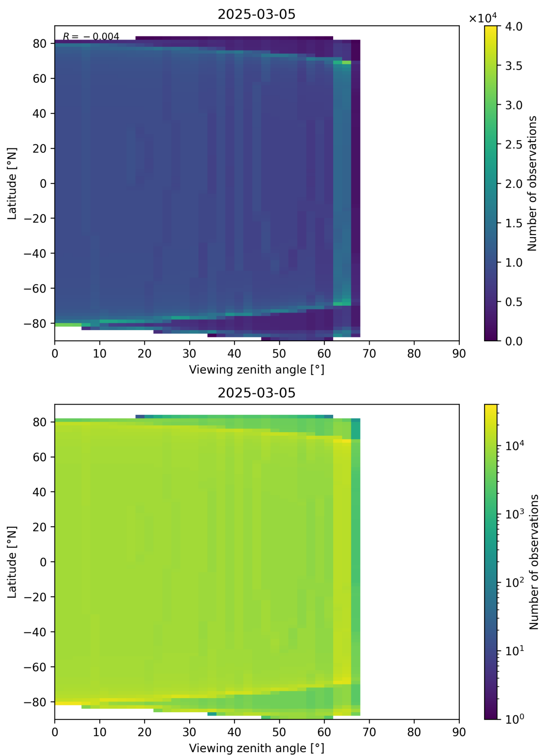
Figure 49: Scatter density plot of “Viewing zenith angle” against “Latitude” for 2025-03-04 to 2025-03-06.
