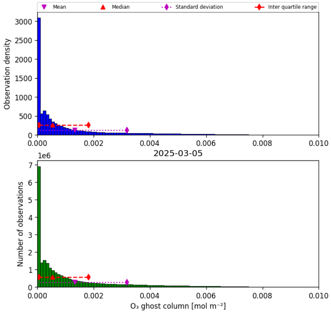
Figure 25: Histogram of “O 3 ghost column” for 2025-03-04 to 2025-03-06
