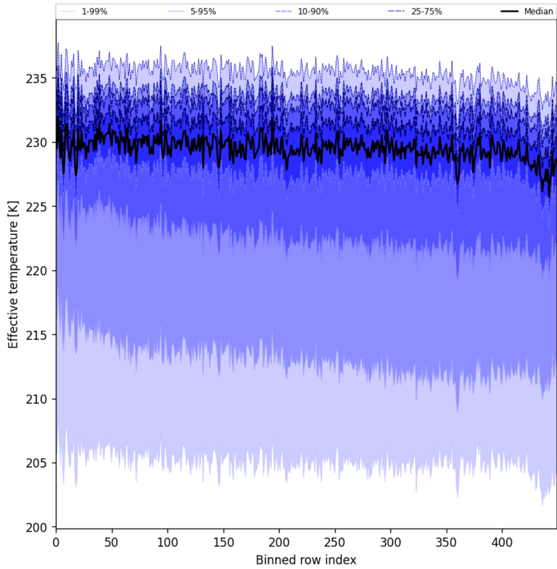
Figure 31: Along track statistics of “Effective temperature” for 2025-03-04 to 2025-03-06
