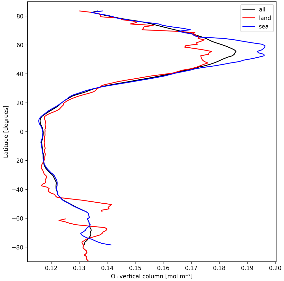
Figure 14: Zonal average of “O 3 vertical column” for 2025-03-04 to 2025-03-06.
