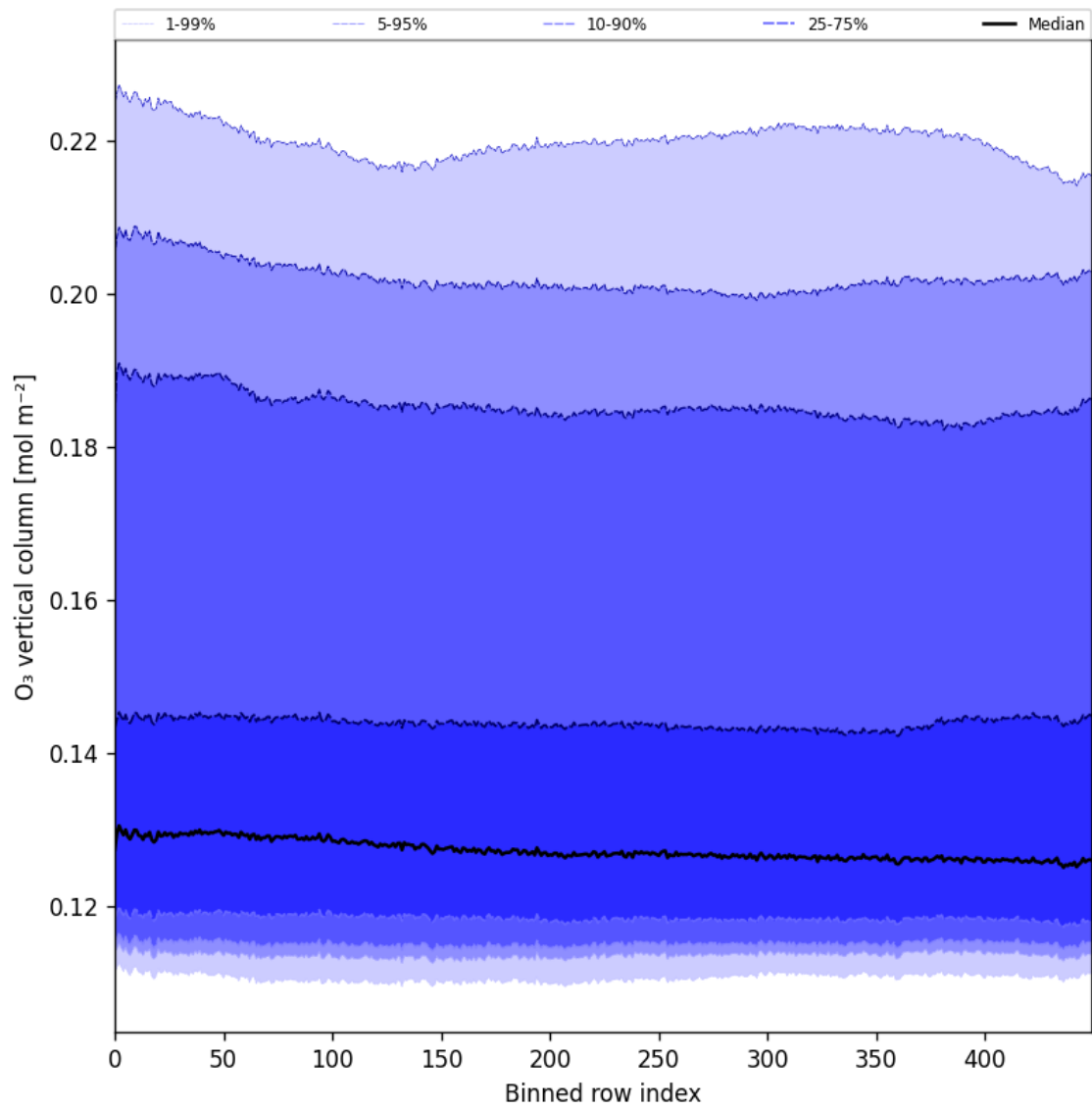
Figure 28: Along track statistics of “O 3 vertical column” for 2025-03-04 to 2025-03-06
