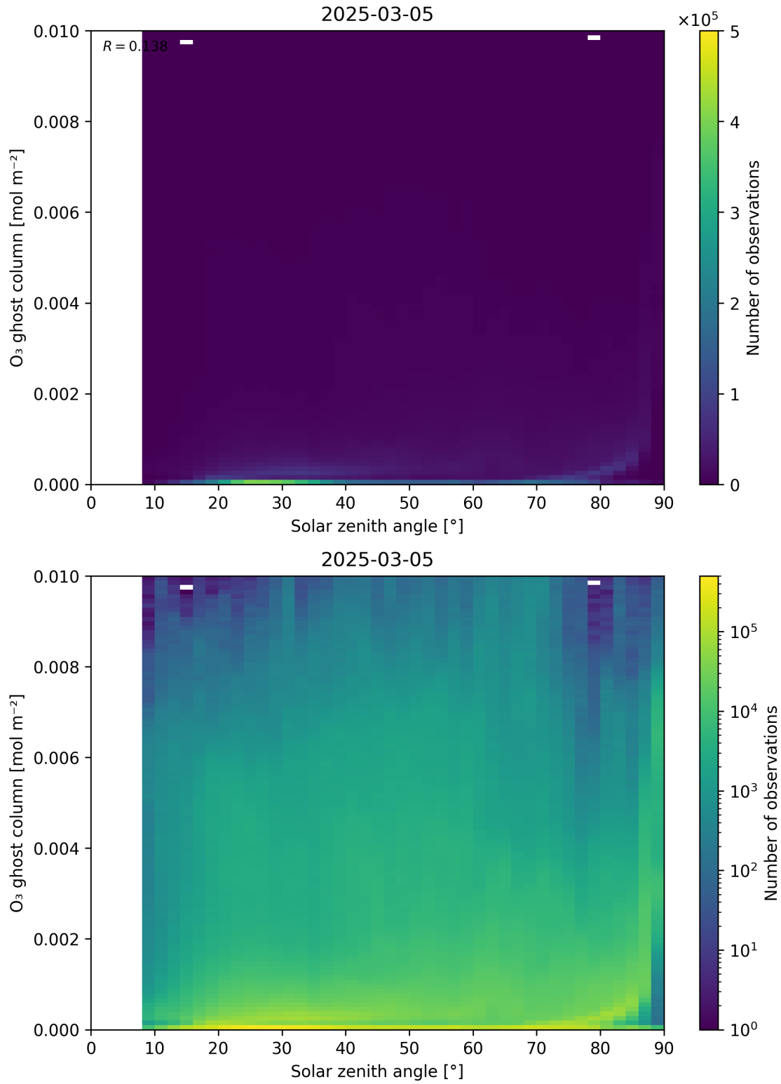
Figure 46: Scatter density plot of “Solar zenith angle” against “O 3 ghost column” for 2025-03-04 to 2025-03-06.
