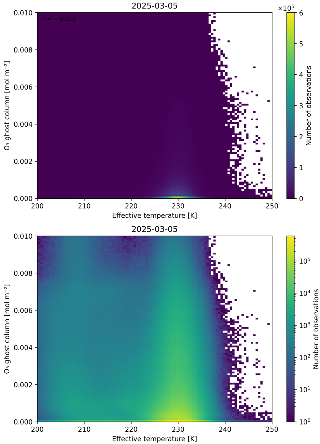
Figure 38: Scatter density plot of “Effective temperature” against “O 3 ghost column” for 2025-03-04 to 2025-03-06.
