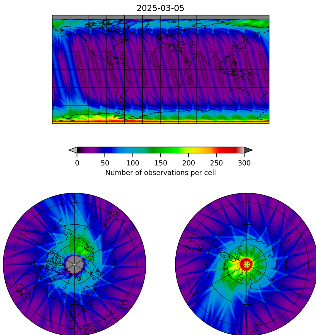
Figure 12: Map of the number of observations for 2025-03-04 to 2025-03-06
