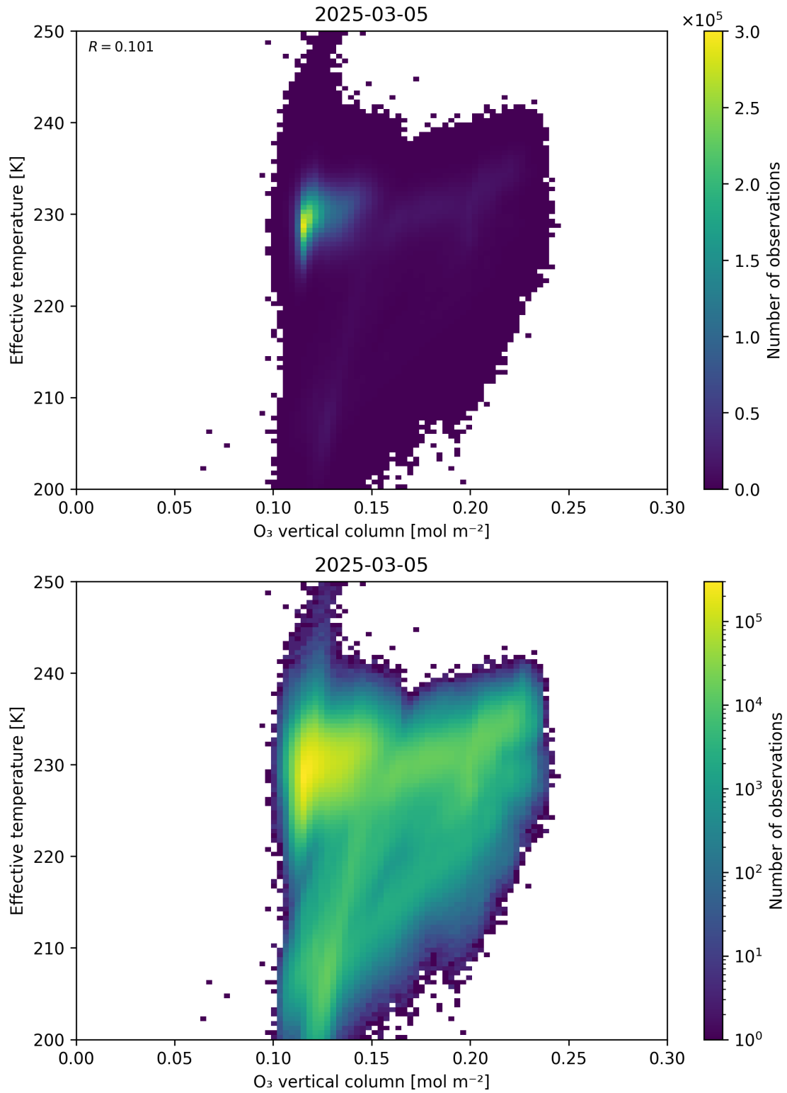
Figure 39: Scatter density plot of “O 3 vertical column” against “Effective temperature” for 2025-03-04 to 2025-03-06.
