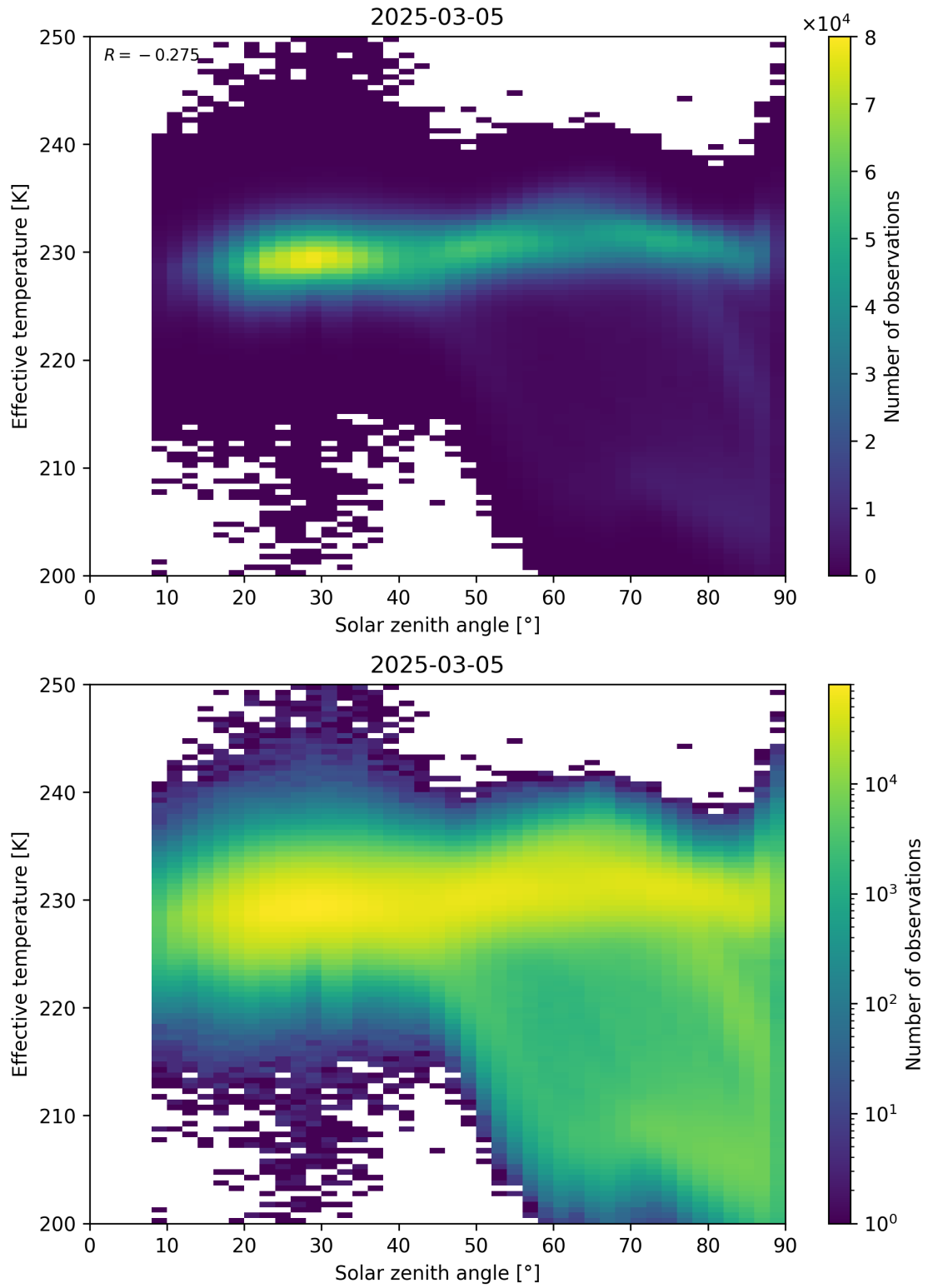
Figure 45: Scatter density plot of “Solar zenith angle” against “Effective temperature” for 2025-03-04 to 2025-03-06.
