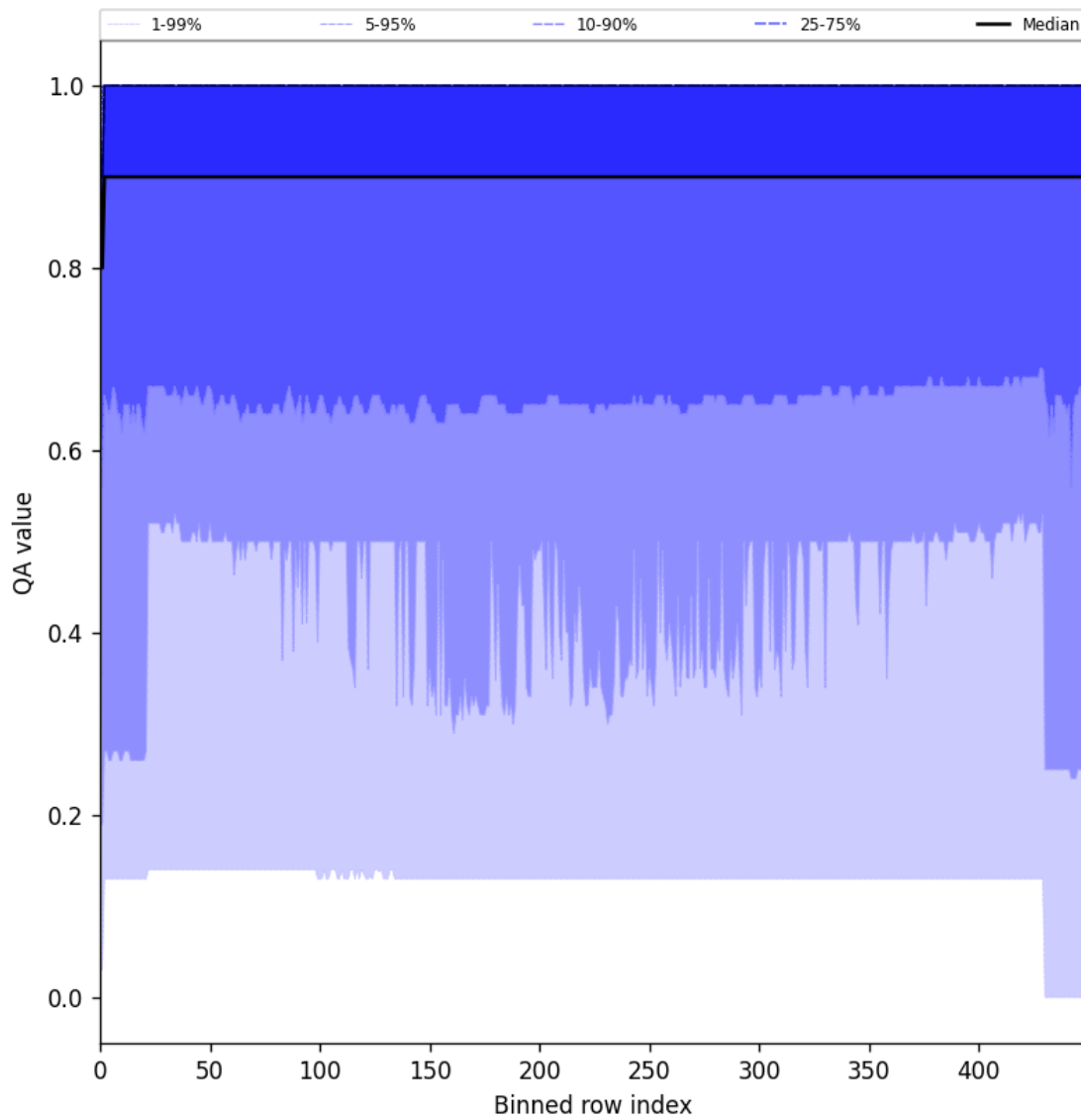
Figure 27: Along track statistics of “QA value” for 2025-03-04 to 2025-03-06
