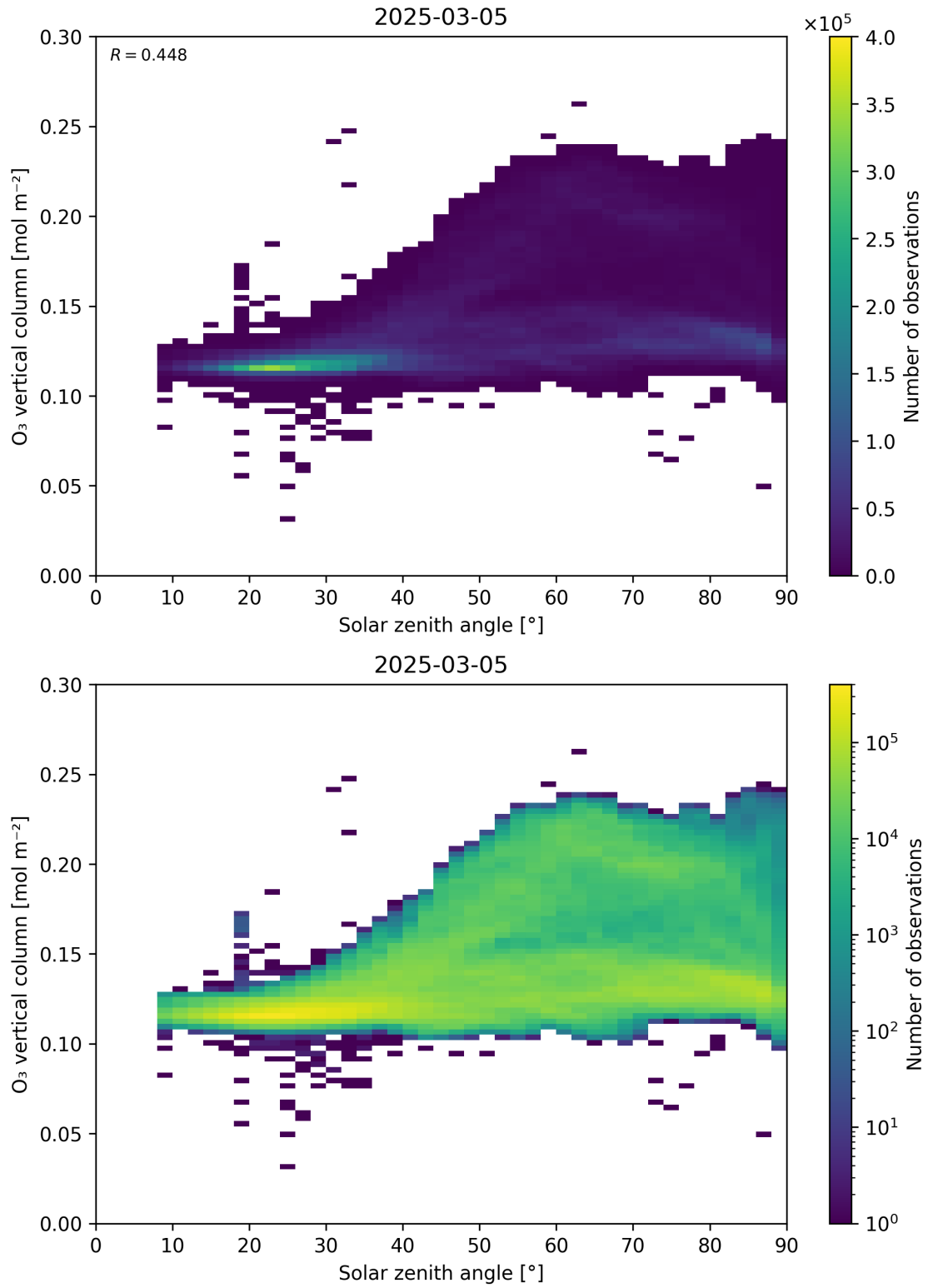
Figure 47: Scatter density plot of “Solar zenith angle” against “O 3 vertical column” for 2025-03-04 to 2025-03-06.
