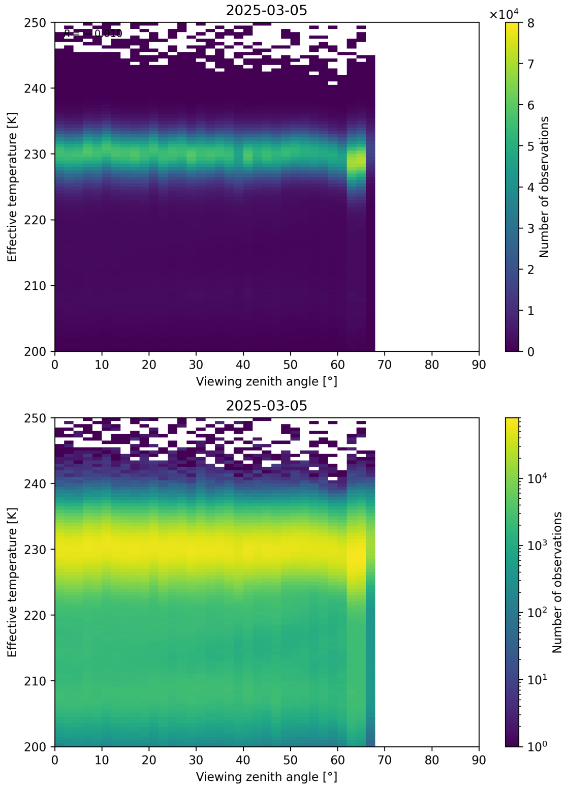
Figure 50: Scatter density plot of “Viewing zenith angle” against “Effective temperature” for 2025-03-04 to 2025-03-06.
