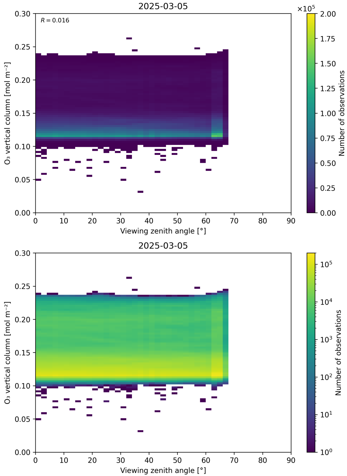
Figure 52: Scatter density plot of “Viewing zenith angle” against “O 3 vertical column” for 2025-03-04 to 2025-03-06.
