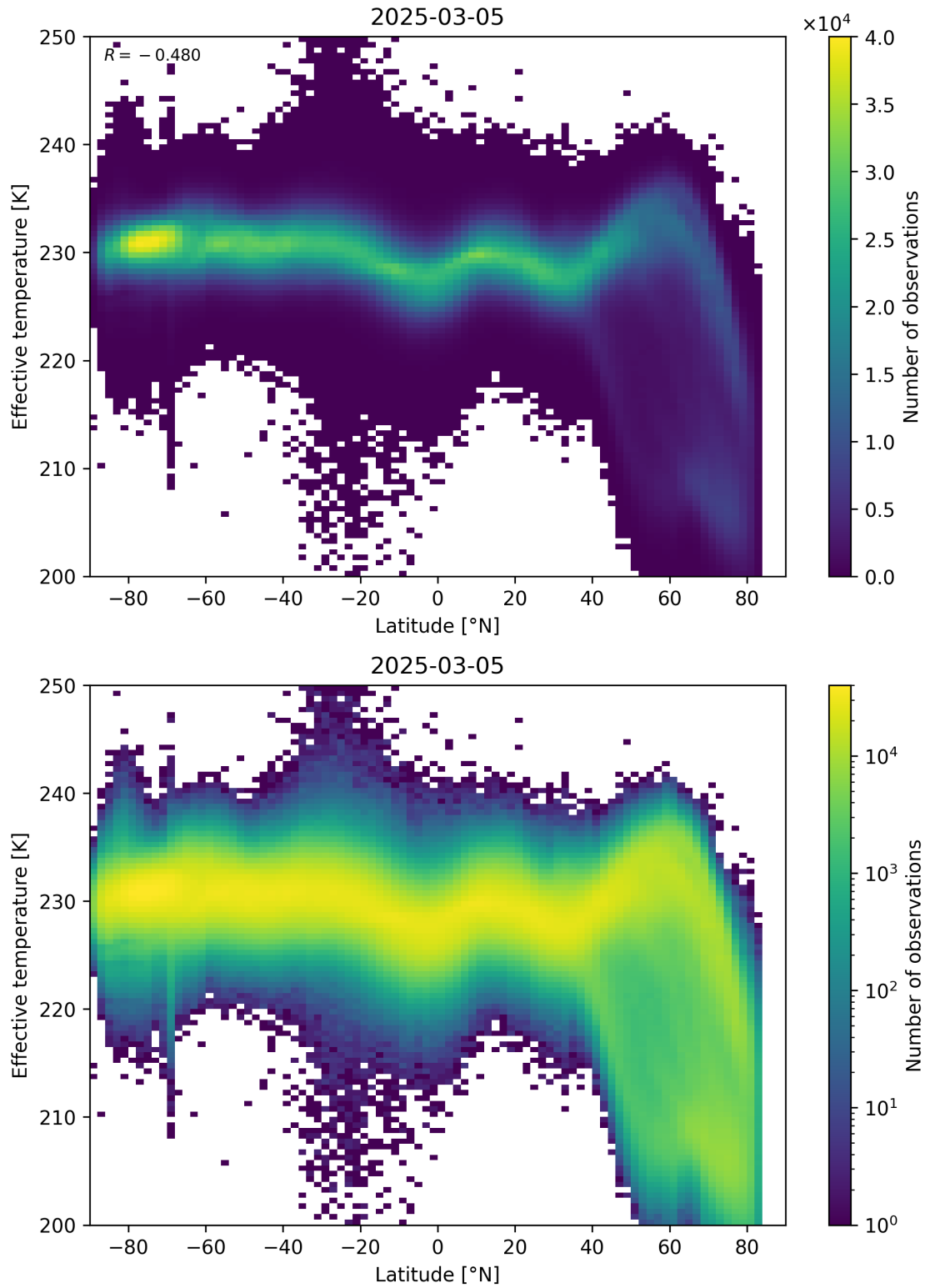
Figure 34: Scatter density plot of “Latitude” against “Effective temperature” for 2025-03-04 to 2025-03-06.
