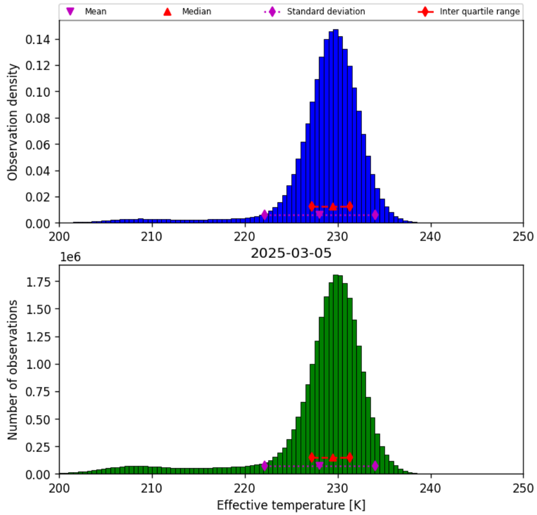
Figure 24: Histogram of “Effective temperature” for 2025-03-04 to 2025-03-06
