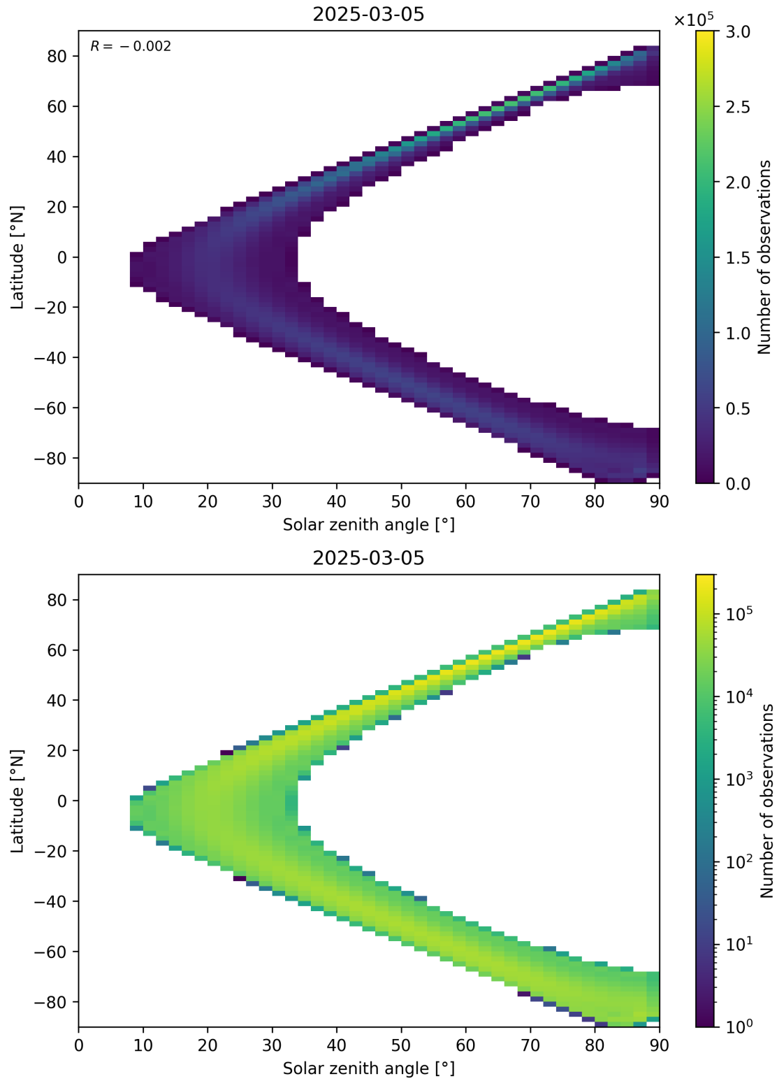
Figure 44: Scatter density plot of “Solar zenith angle” against “Latitude” for 2025-03-04 to 2025-03-06.
