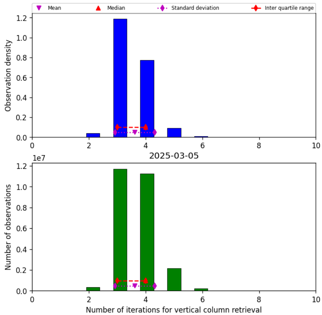
Figure 26: Histogram of “Number of iterations for vertical column retrieval” for 2025-03-04 to 2025-03-06
