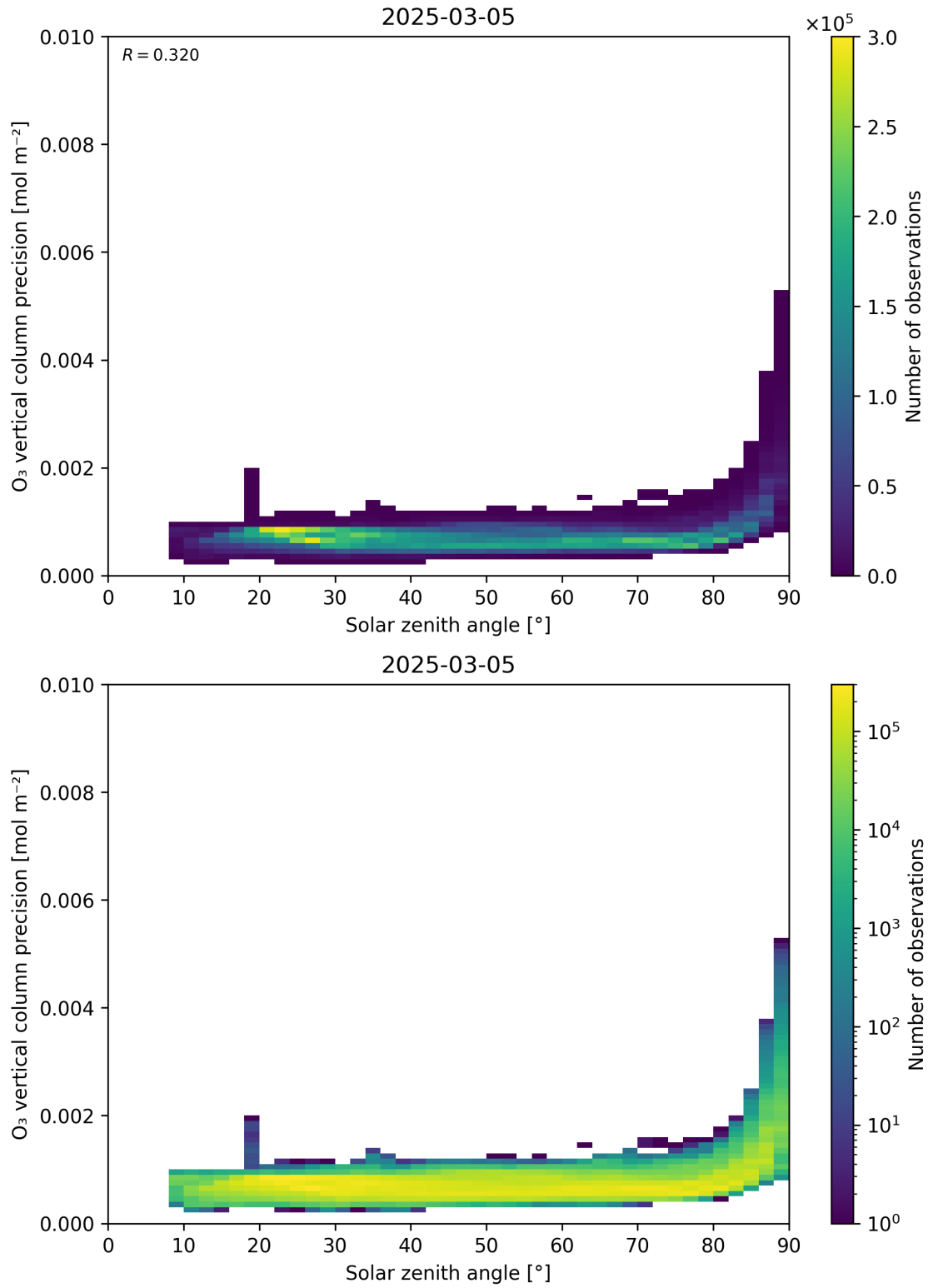
Figure 48: Scatter density plot of “Solar zenith angle” against “O 3 vertical column precision” for 2025-03-04 to 2025-03-06.
