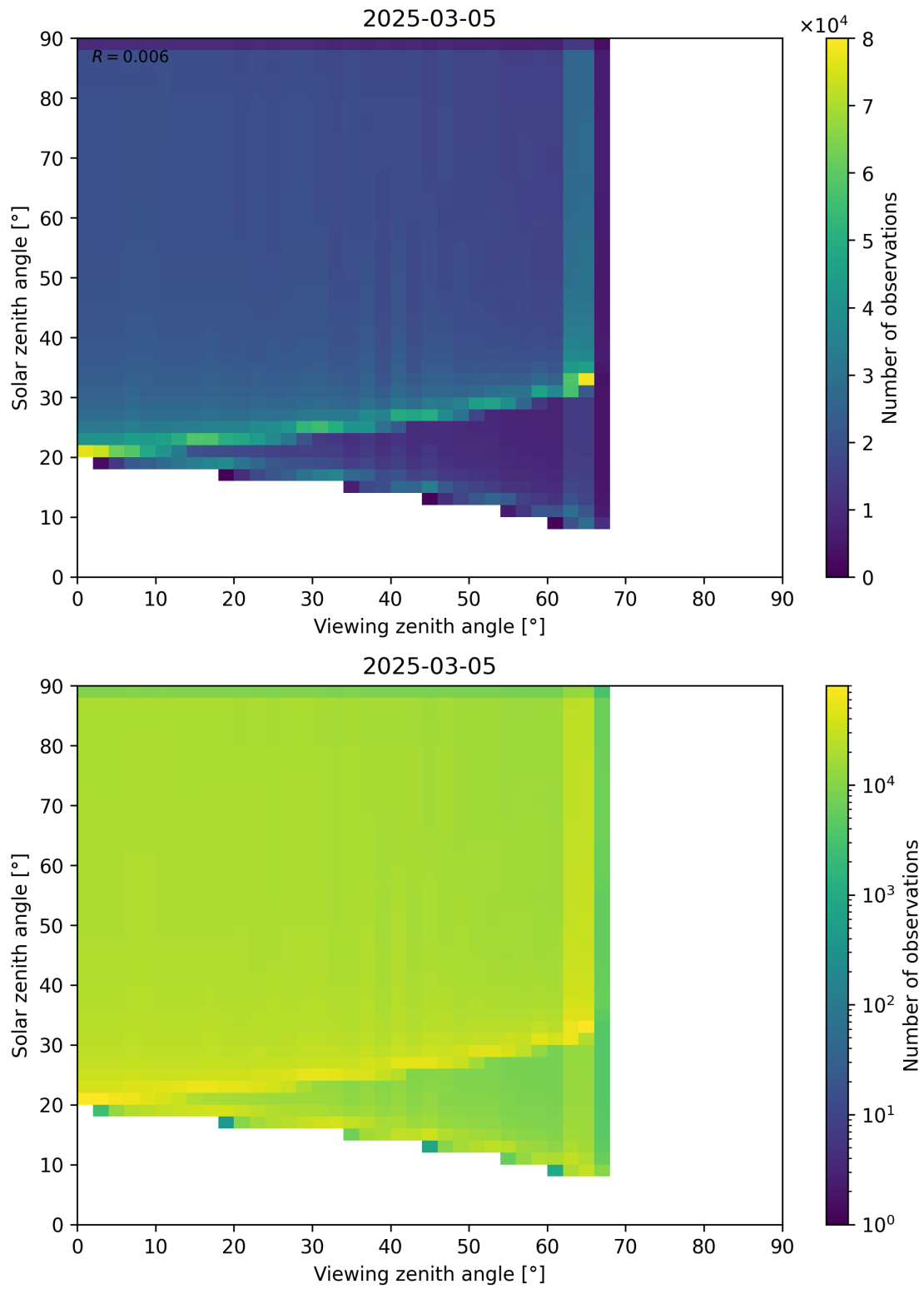
Figure 54: Scatter density plot of “Viewing zenith angle” against “Solar zenith angle” for 2025-03-04 to 2025-03-06.
