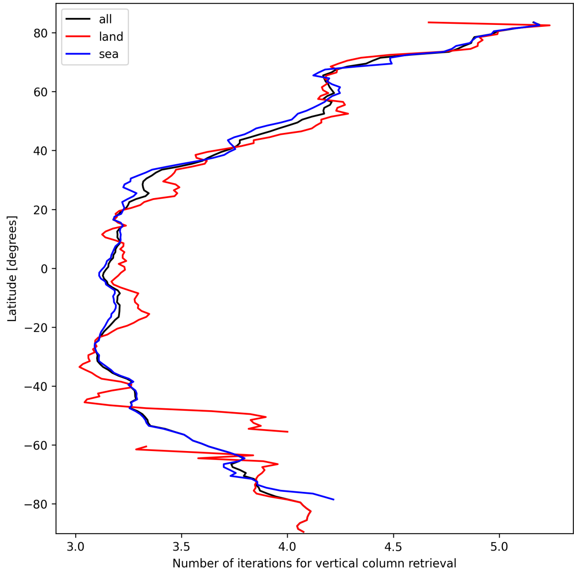
Figure 19: Zonal average of “Number of iterations for vertical column retrieval” for 2025-03-04 to 2025-03-06.
