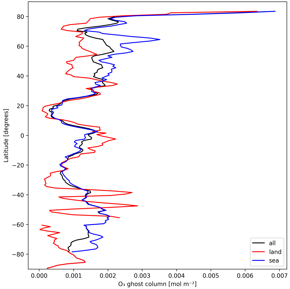
Figure 18: Zonal average of “O 3 ghost column” for 2025-03-04 to 2025-03-06.
