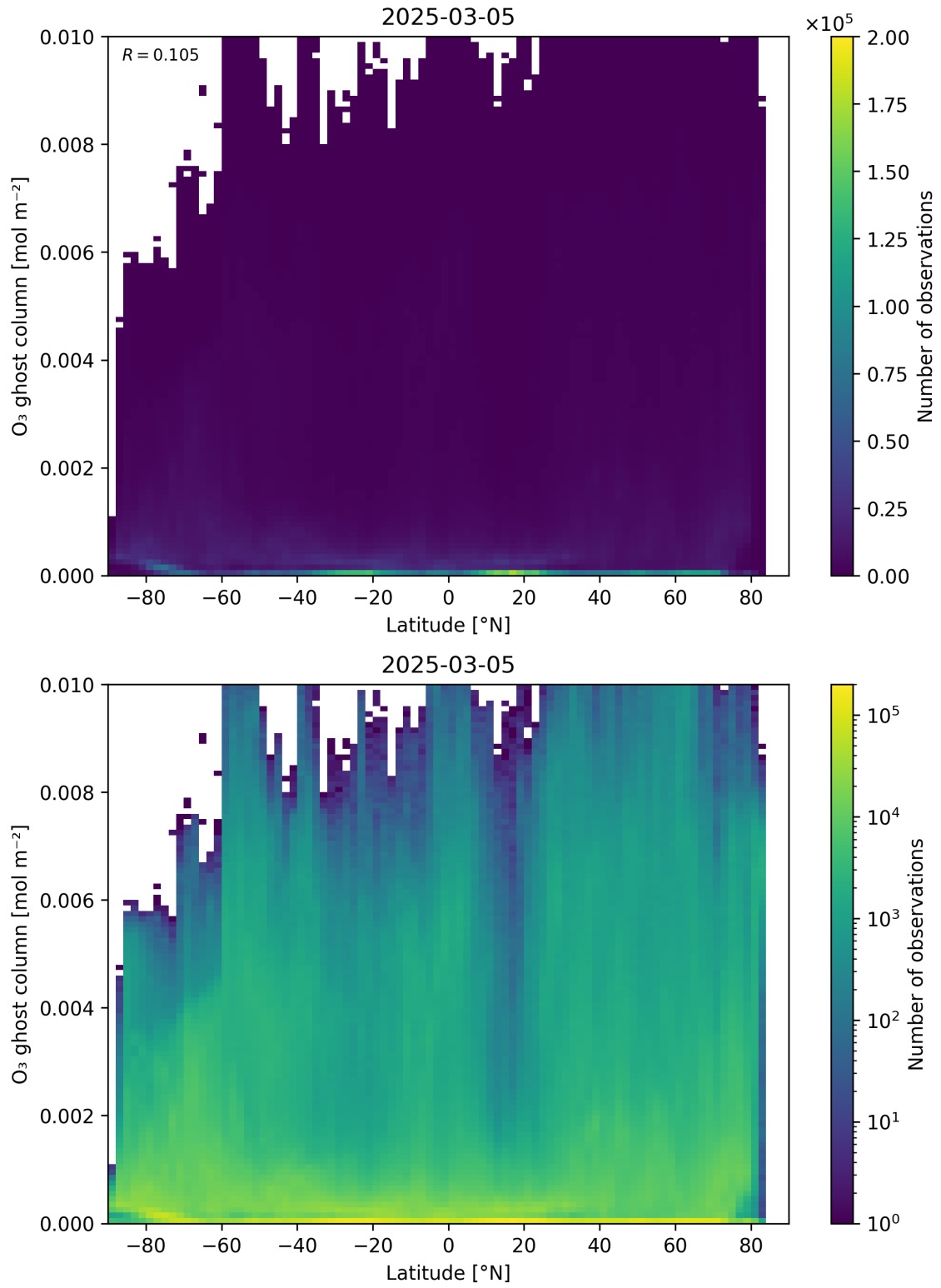
Figure 35: Scatter density plot of “Latitude” against “O 3 ghost column” for 2025-03-04 to 2025-03-06.
