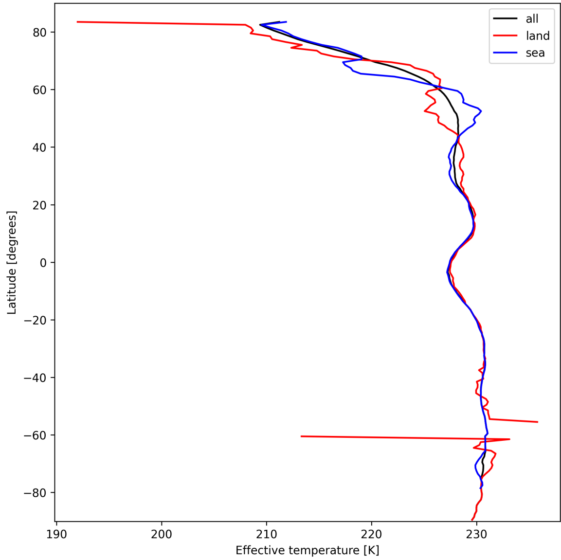
Figure 17: Zonal average of "Effective temperature" for 2025-03-04 to 2025-03-06.
