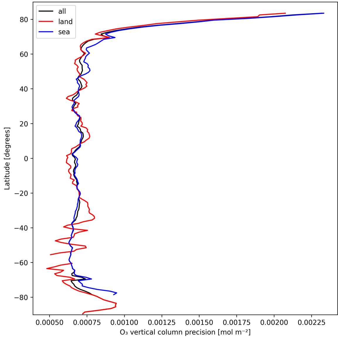
Figure 15: Zonal average of “O 3 vertical column precision” for 2025-03-04 to 2025-03-06.
