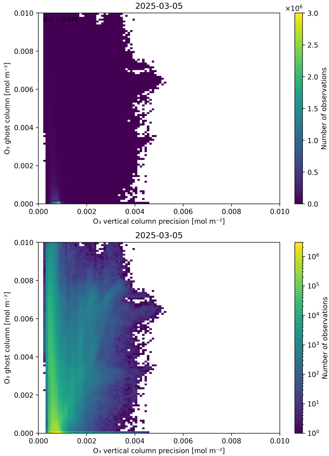
Figure 43: Scatter density plot of “O 3 vertical column precision” against “O 3 ghost column” for 2025-03-04 to 2025-03-06.
