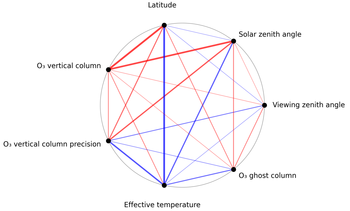
Figure 1: Map of correlation graph for 2025-03-04 to 2025-03-06.
