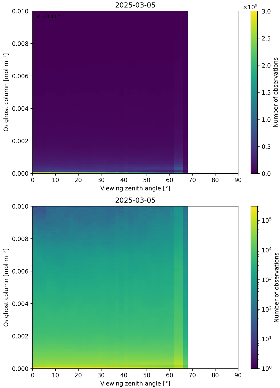
Figure 51: Scatter density plot of “Viewing zenith angle” against “O 3 ghost column” for 2025-03-04 to 2025-03-06.
