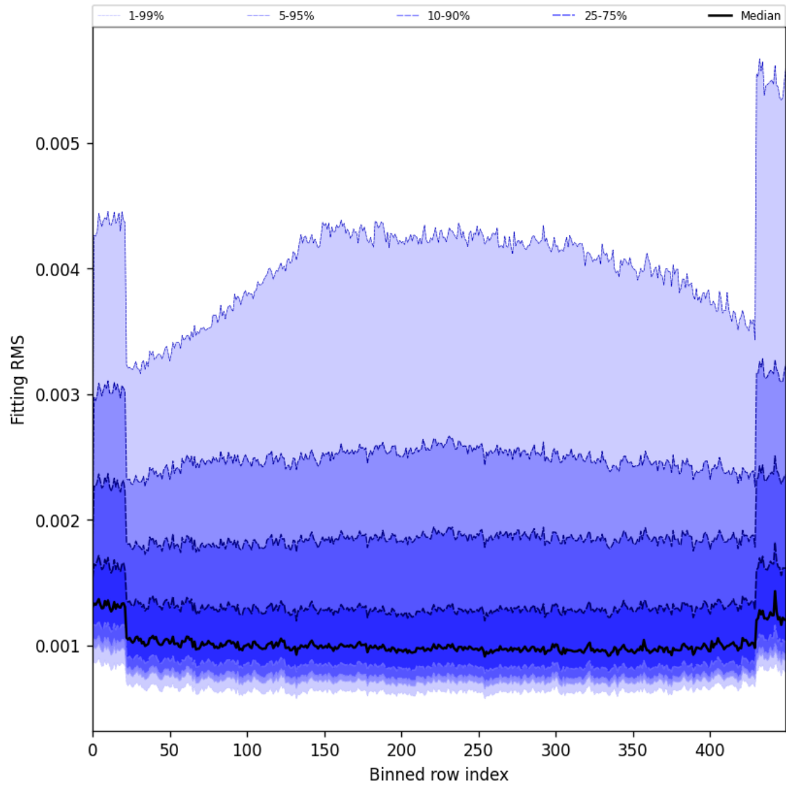
Figure 30: Along track statistics of “Fitting RMS” for 2025-03-04 to 2025-03-06
