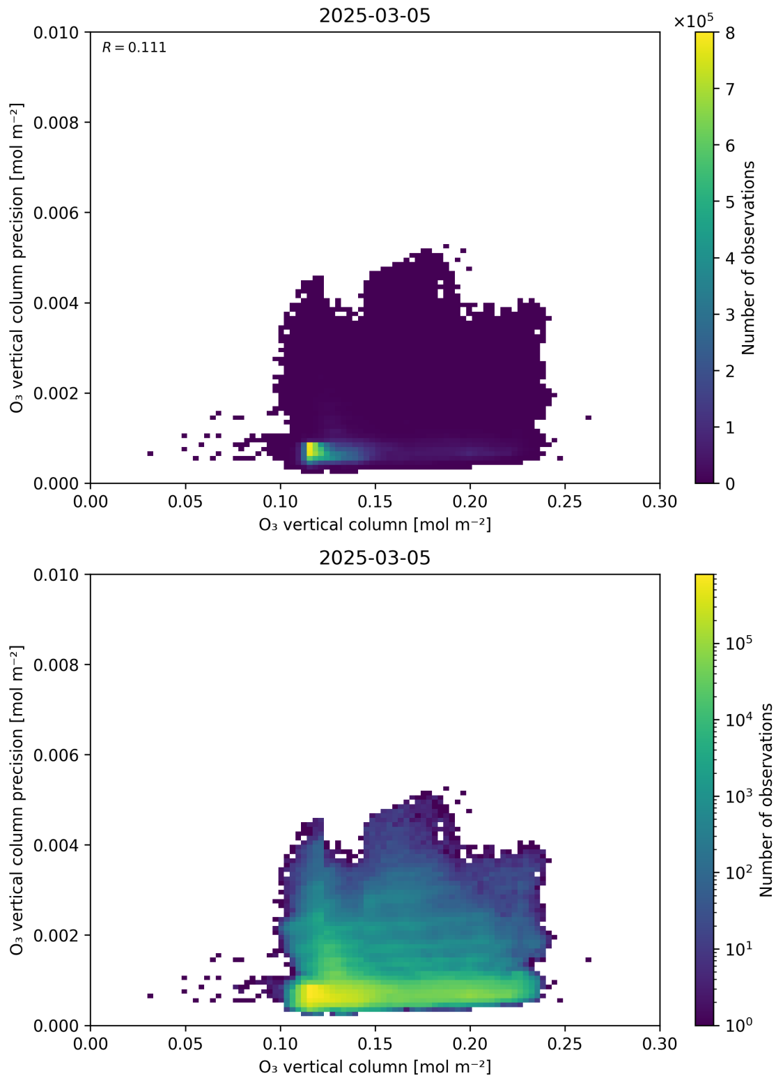
Figure 41: Scatter density plot of “O 3 vertical column” against “O 3 vertical column precision” for 2025-03-04 to 2025-03-06.
