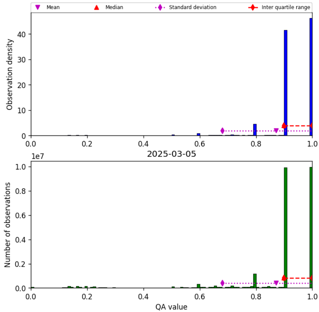
Figure 20: Histogram of “QA value” for 2025-03-04 to 2025-03-06
