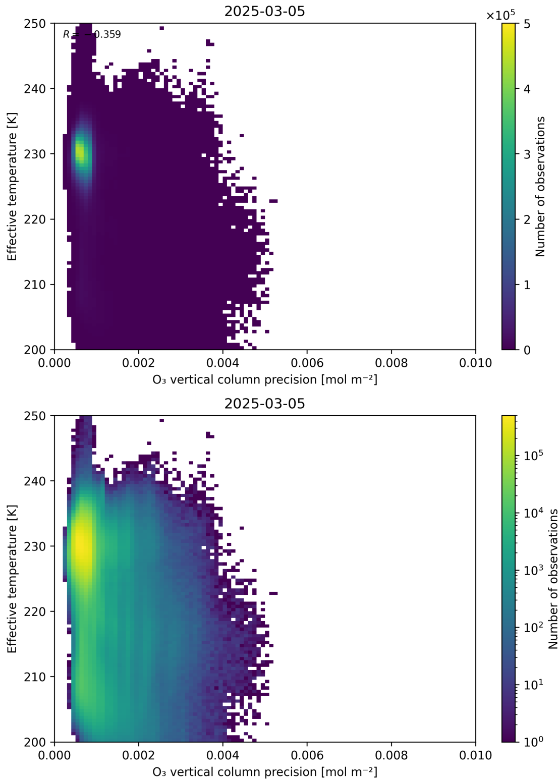
Figure 42: Scatter density plot of “O 3 vertical column precision” against “Effective temperature” for 2025-03-04 to 2025-03-06.
