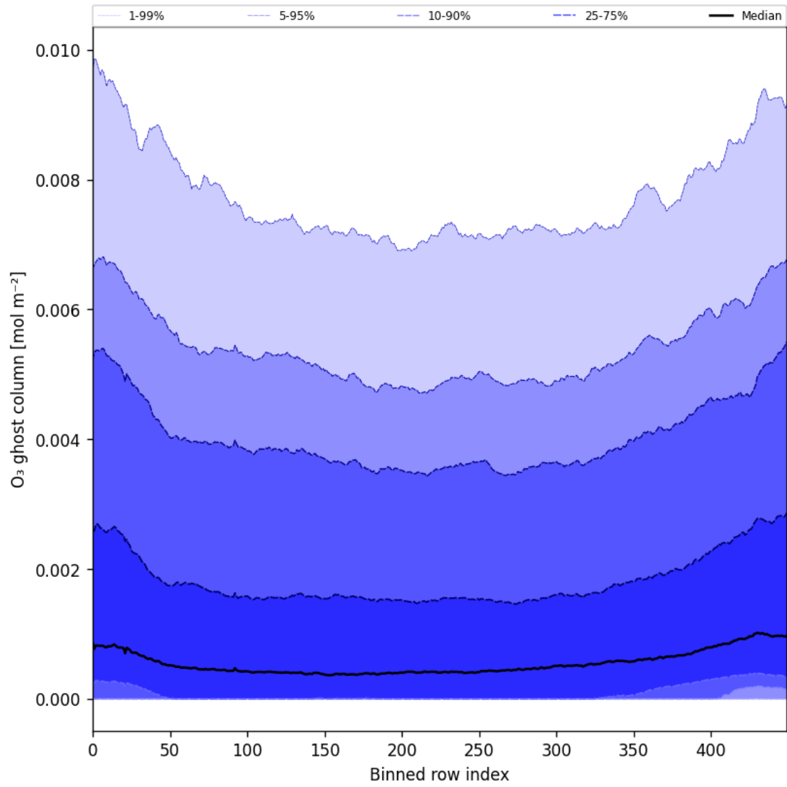
Figure 32: Along track statistics of “O 3 ghost column” for 2025-03-04 to 2025-03-06
