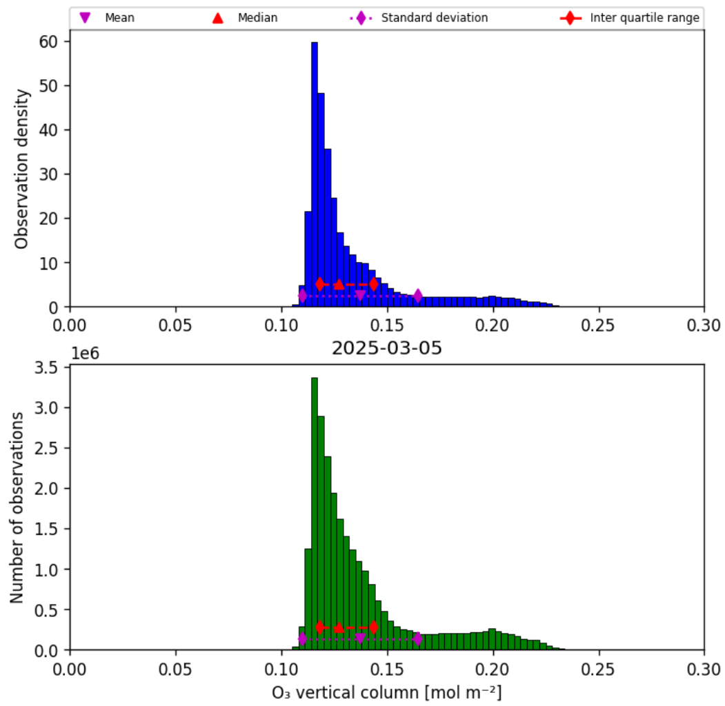
Figure 21: Histogram of “O 3 vertical column” for 2025-03-04 to 2025-03-06
