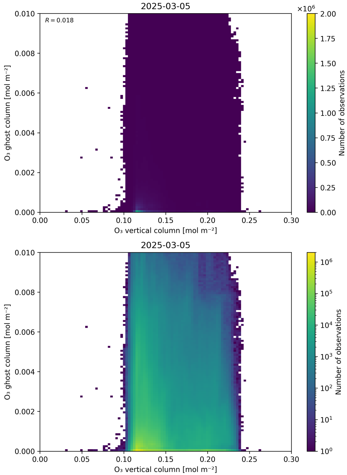
Figure 40: Scatter density plot of “O 3 vertical column” against “O 3 ghost column” for 2025-03-04 to 2025-03-06.
