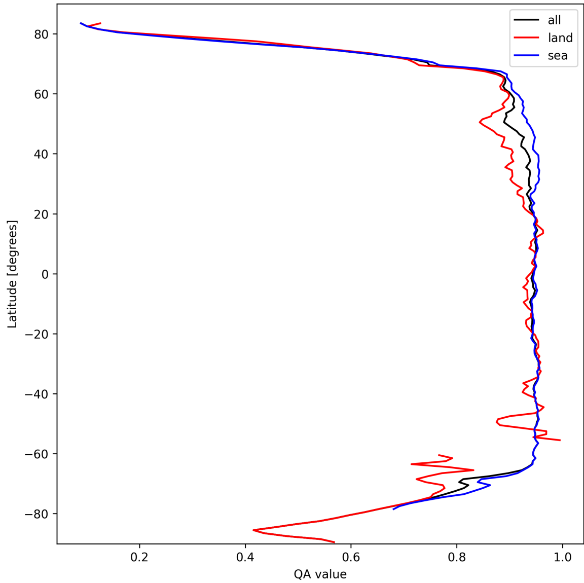
Figure 13: Zonal average of “QA value” for 2025-03-04 to 2025-03-06.
