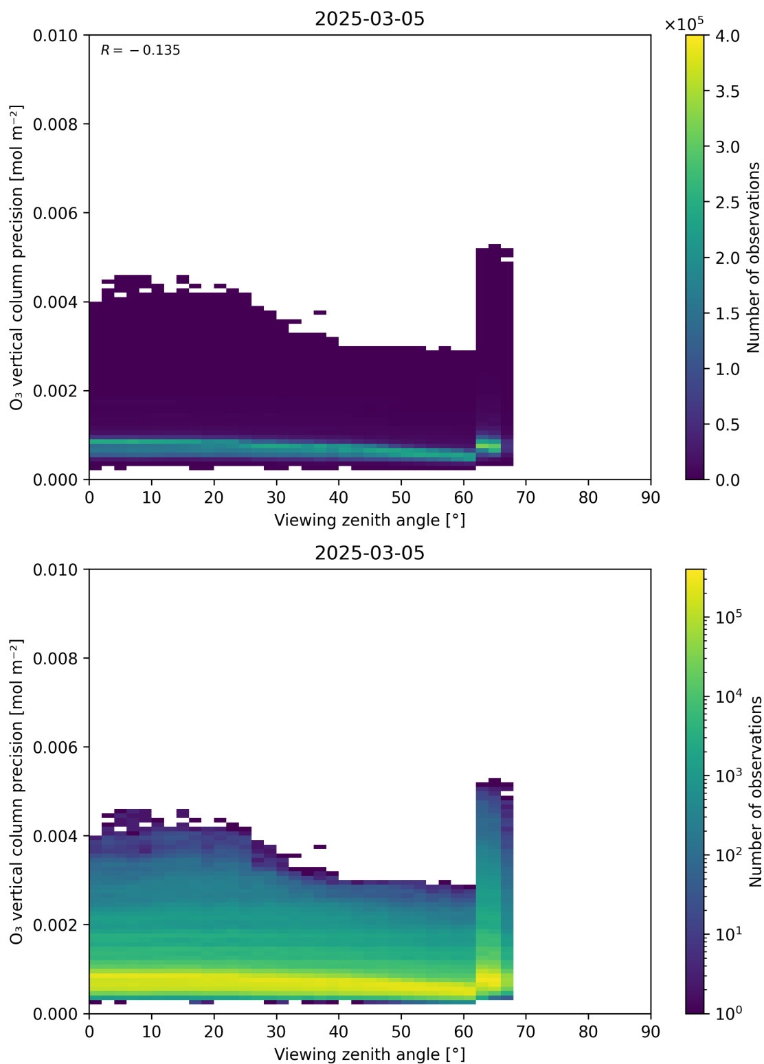
Figure 53: Scatter density plot of “Viewing zenith angle” against “O 3 vertical column precision” for 2025-03-04 to 2025-03-06.
