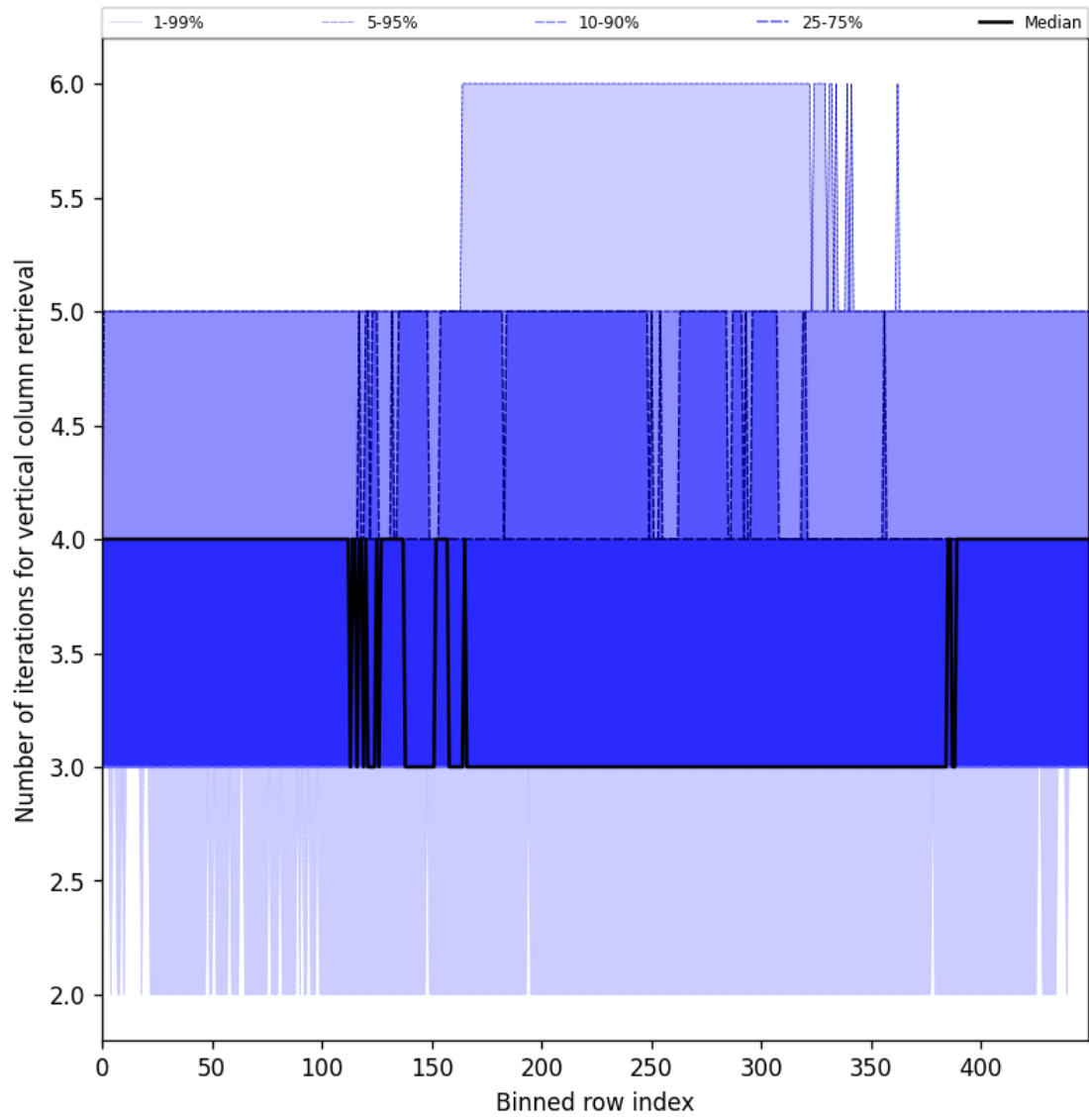
Figure 33: Along track statistics of “Number of iterations for vertical column retrieval” for 2025-03-04 to 2025-03-06
