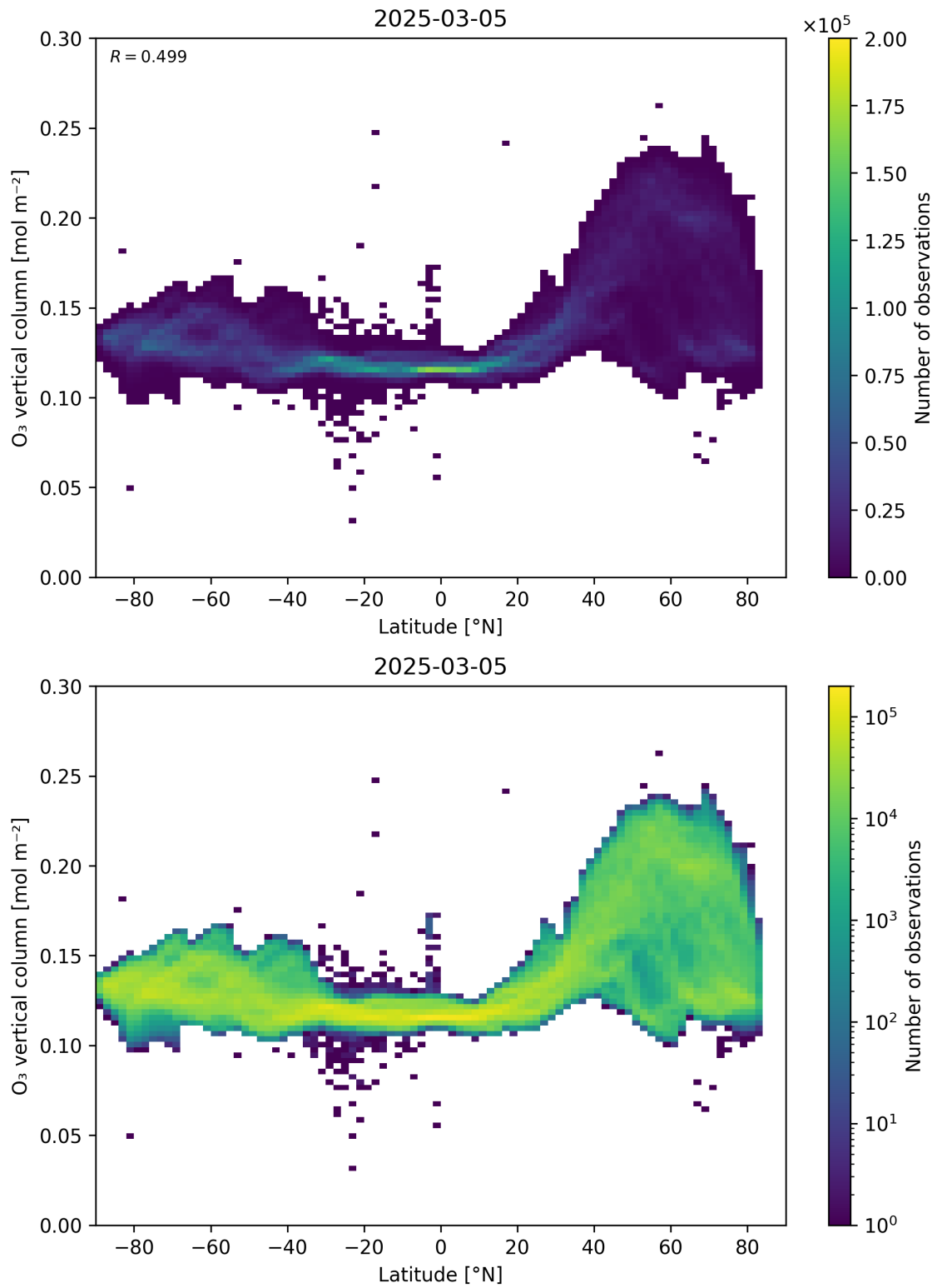
Figure 36: Scatter density plot of “Latitude” against “O 3 vertical column” for 2025-03-04 to 2025-03-06.
