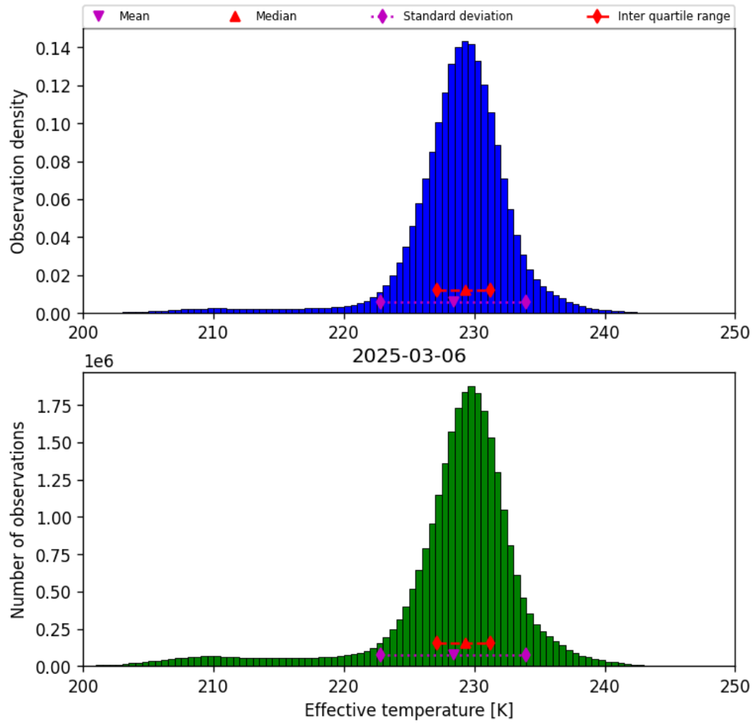
Figure 24: Histogram of “Effective temperature” for 2025-03-05 to 2025-03-07
