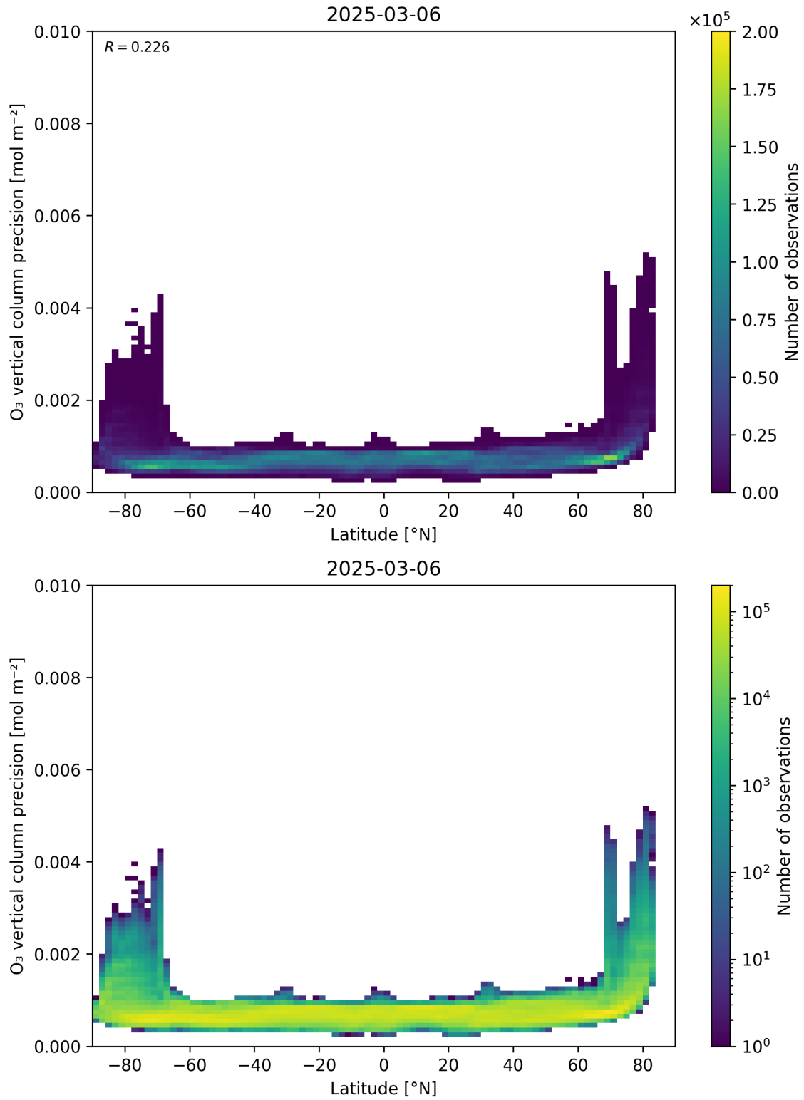
Figure 37: Scatter density plot of “Latitude” against “O 3 vertical column precision” for 2025-03-05 to 2025-03-07.
