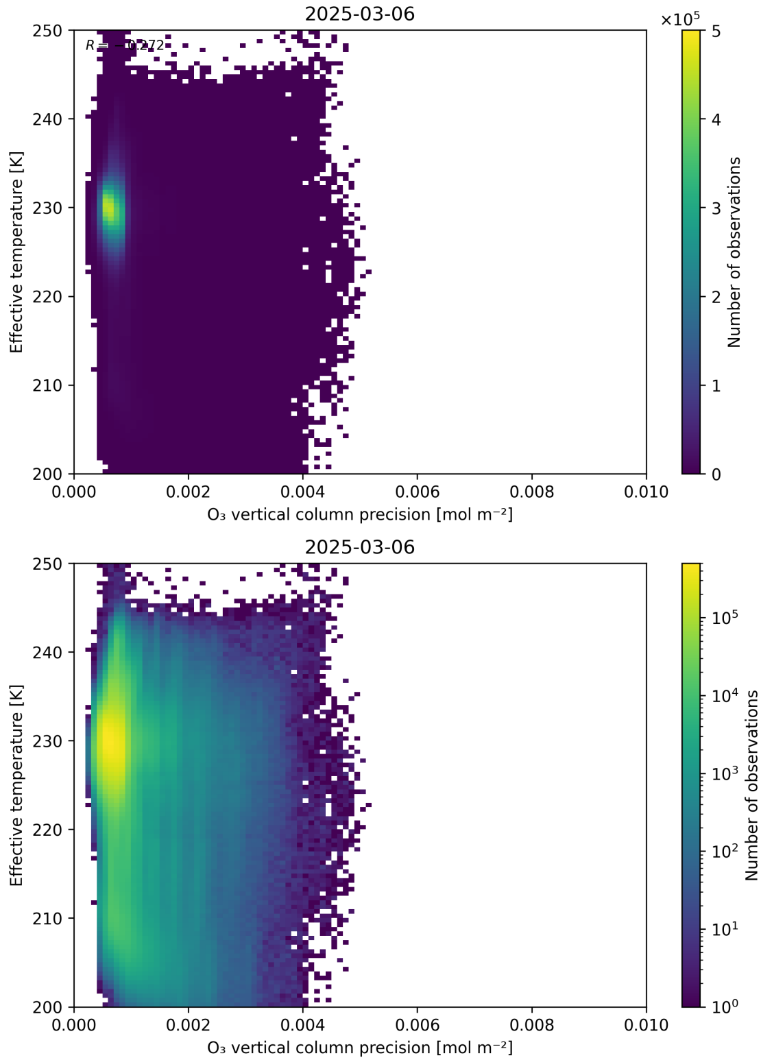
Figure 42: Scatter density plot of “O 3 vertical column precision” against “Effective temperature” for 2025-03-05 to 2025-03-07.
