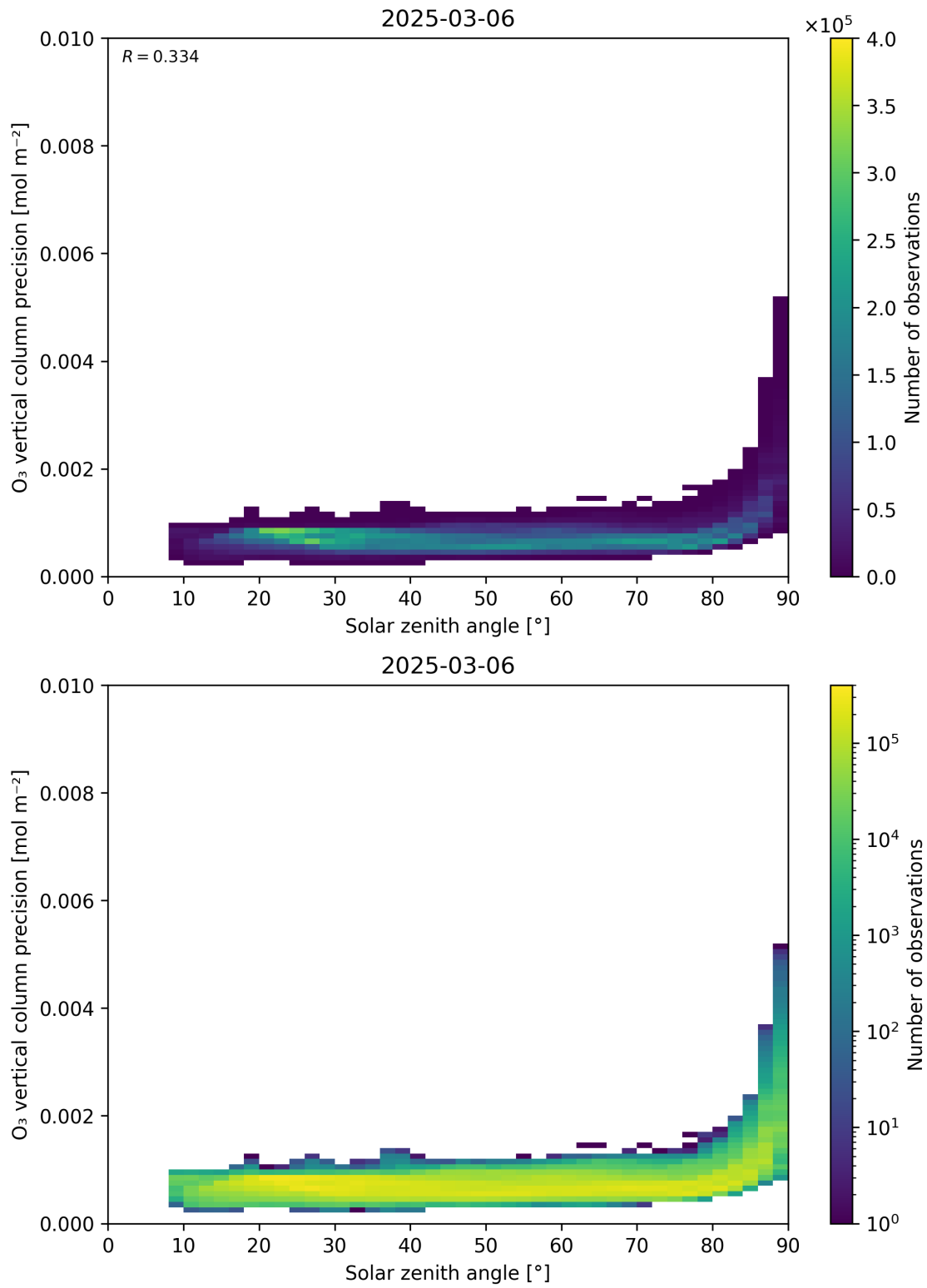
Figure 48: Scatter density plot of “Solar zenith angle” against “O 3 vertical column precision” for 2025-03-05 to 2025-03-07.
