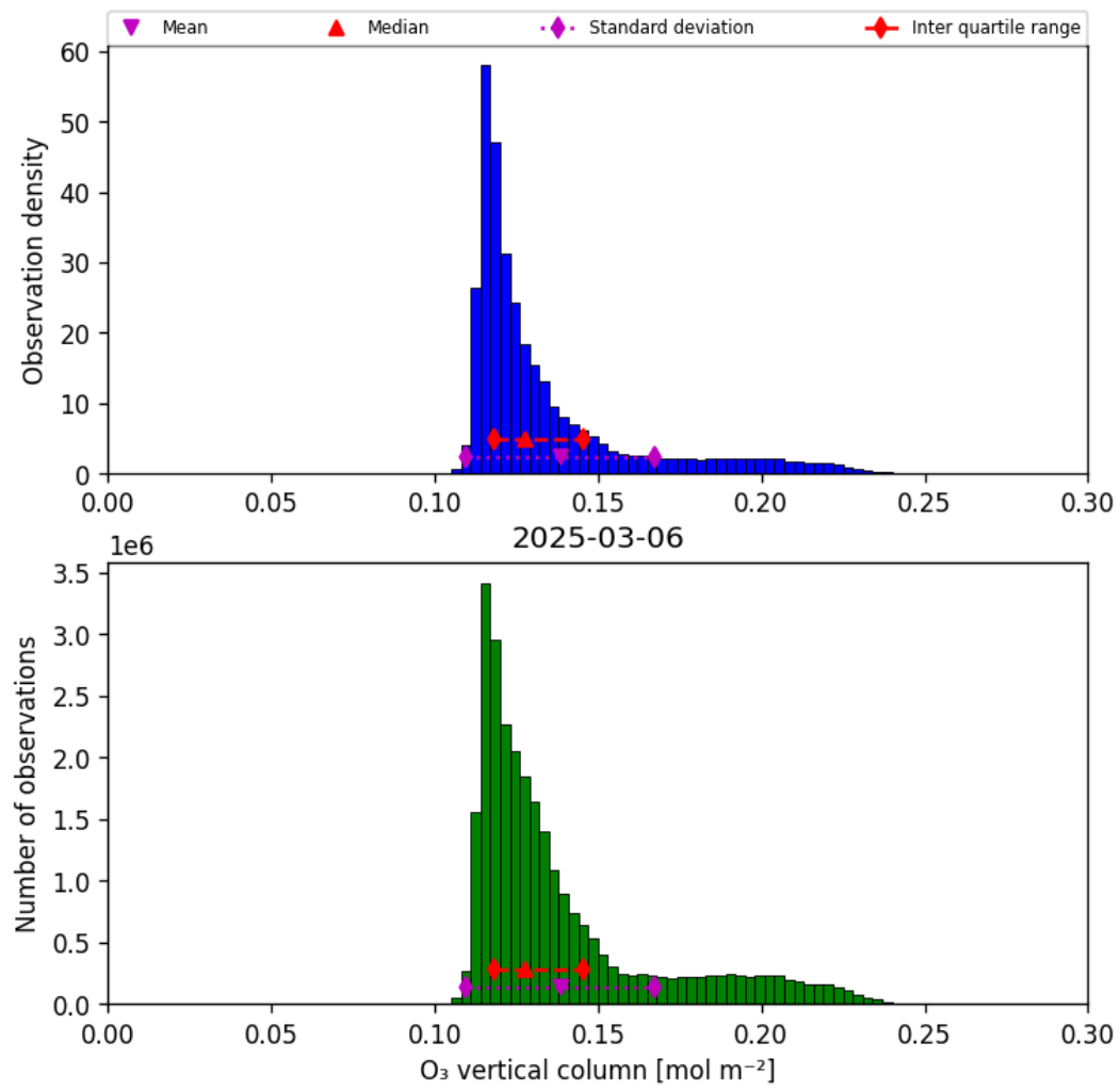
Figure 21: Histogram of “O 3 vertical column” for 2025-03-05 to 2025-03-07
