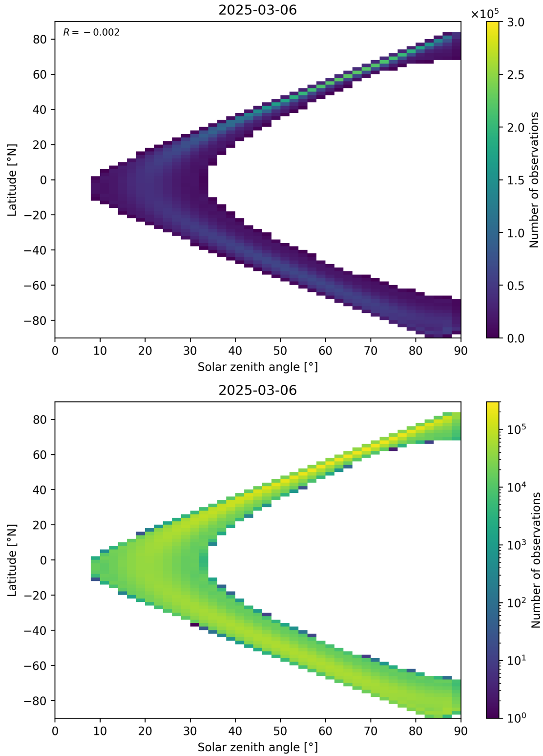
Figure 44: Scatter density plot of “Solar zenith angle” against “Latitude” for 2025-03-05 to 2025-03-07.
