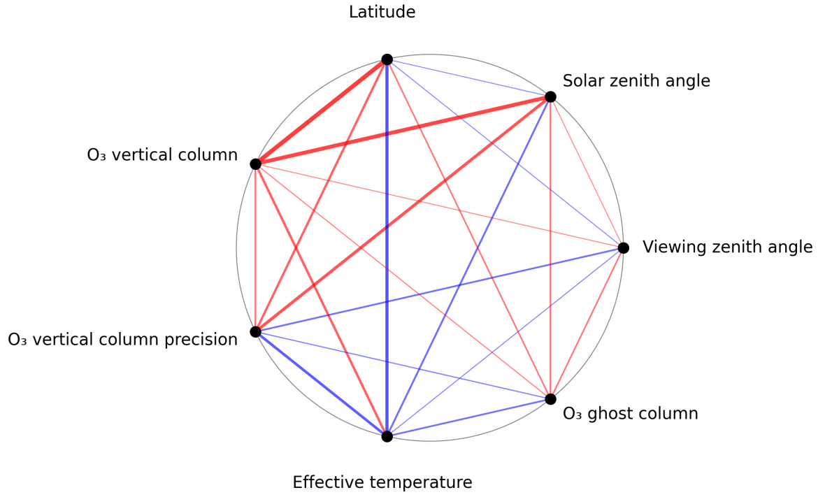
Figure 1: Map of correlation graph for 2025-03-05 to 2025-03-07.
