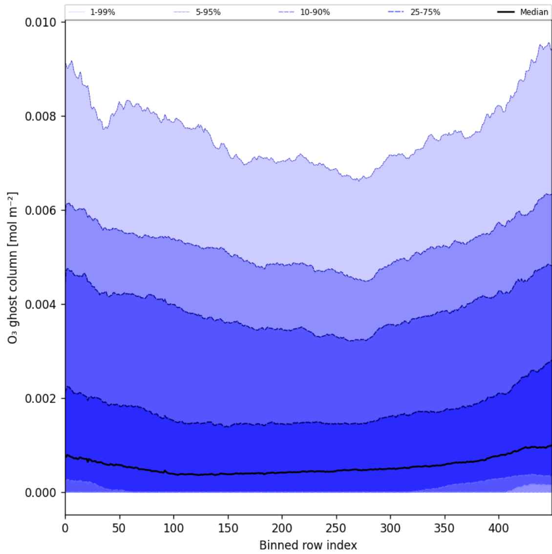
Figure 32: Along track statistics of “O 3 ghost column” for 2025-03-05 to 2025-03-07
