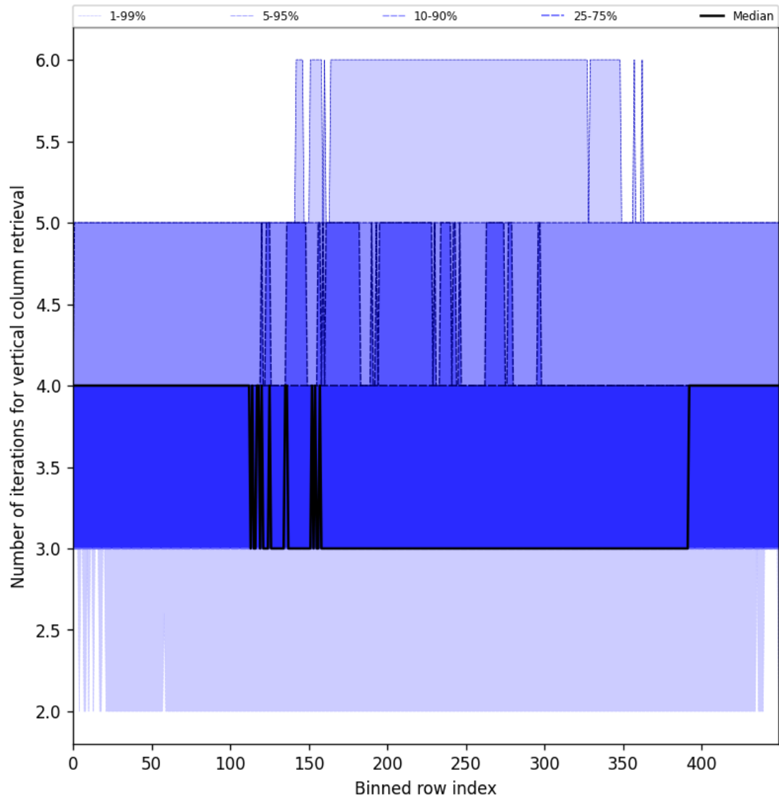
Figure 33: Along track statistics of “Number of iterations for vertical column retrieval” for 2025-03-05 to 2025-03-07
