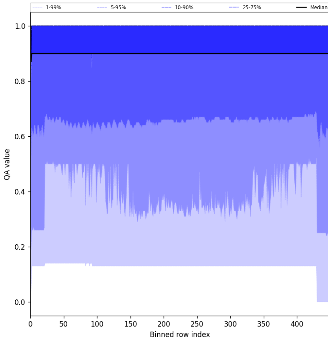
Figure 27: Along track statistics of “QA value” for 2025-03-05 to 2025-03-07
