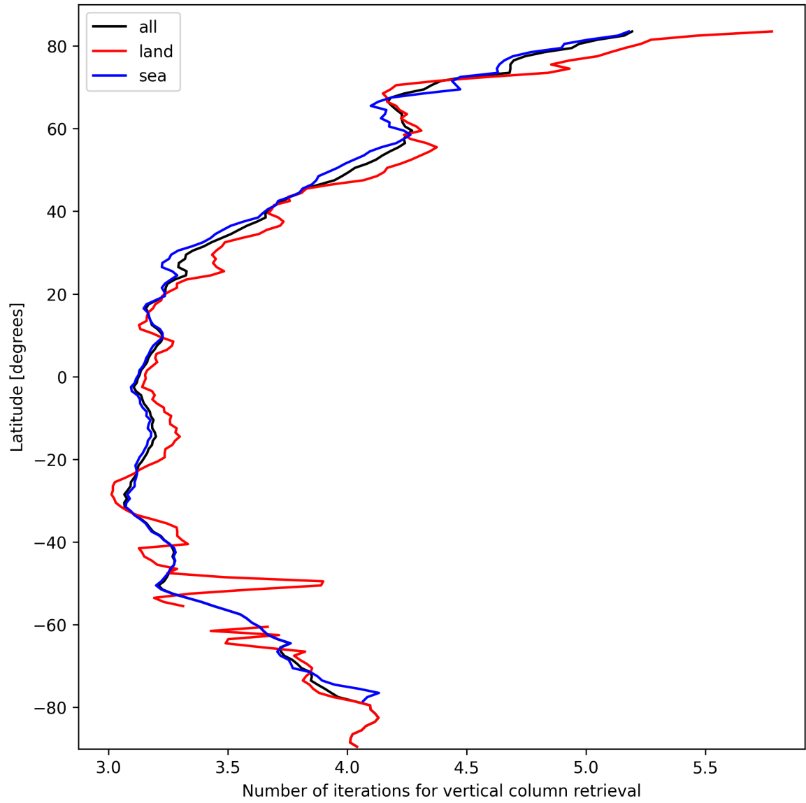
Figure 19: Zonal average of “Number of iterations for vertical column retrieval” for 2025-03-05 to 2025-03-07.
