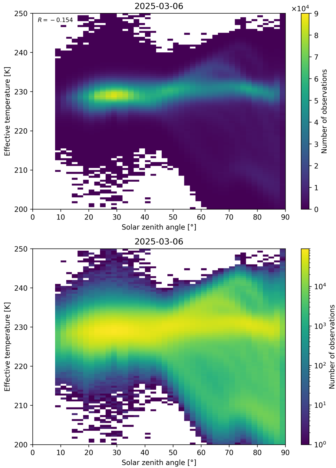
Figure 45: Scatter density plot of “Solar zenith angle” against “Effective temperature” for 2025-03-05 to 2025-03-07.
