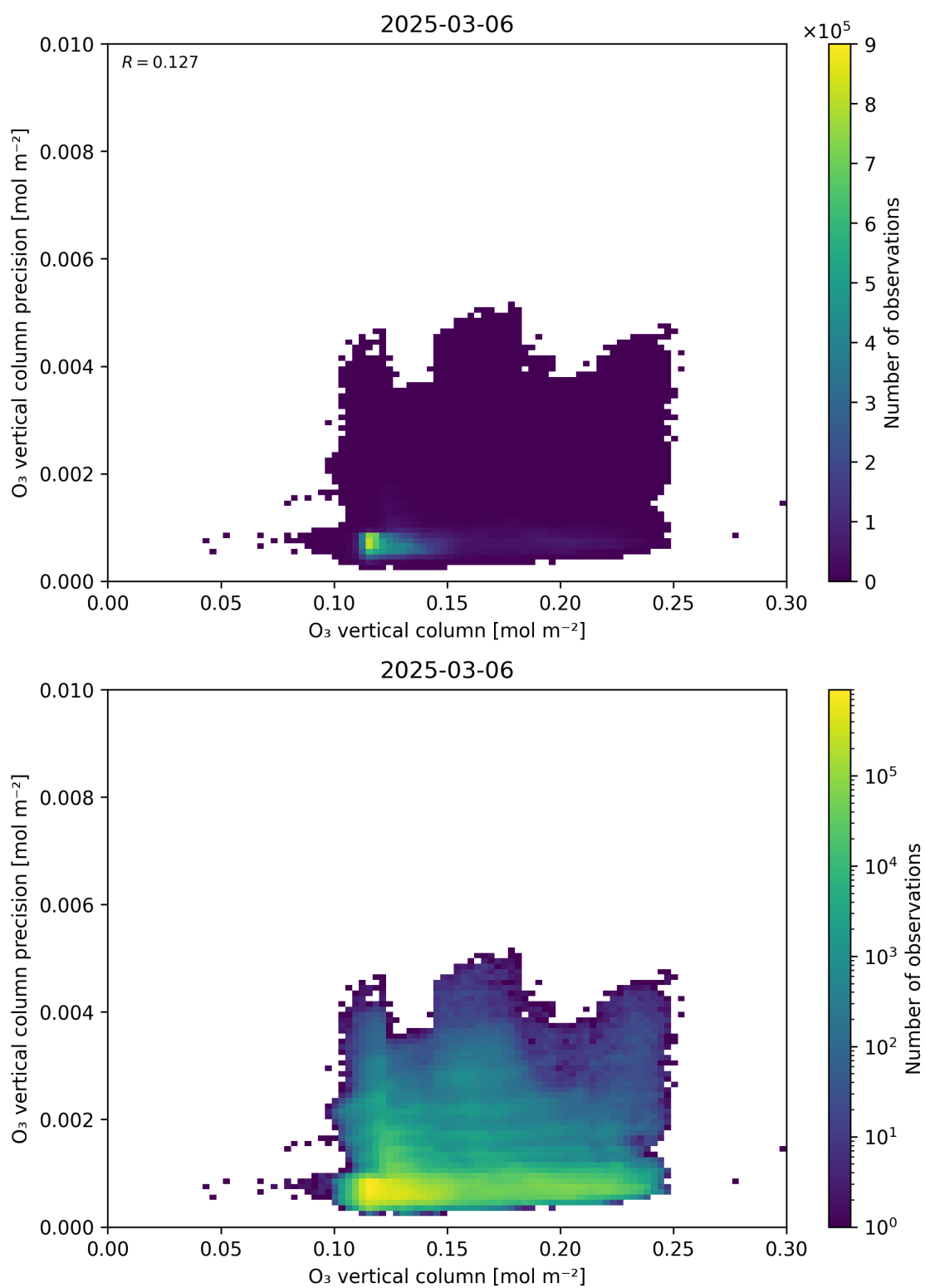
Figure 41: Scatter density plot of “O 3 vertical column” against “O 3 vertical column precision” for 2025-03-05 to 2025-03-07.
