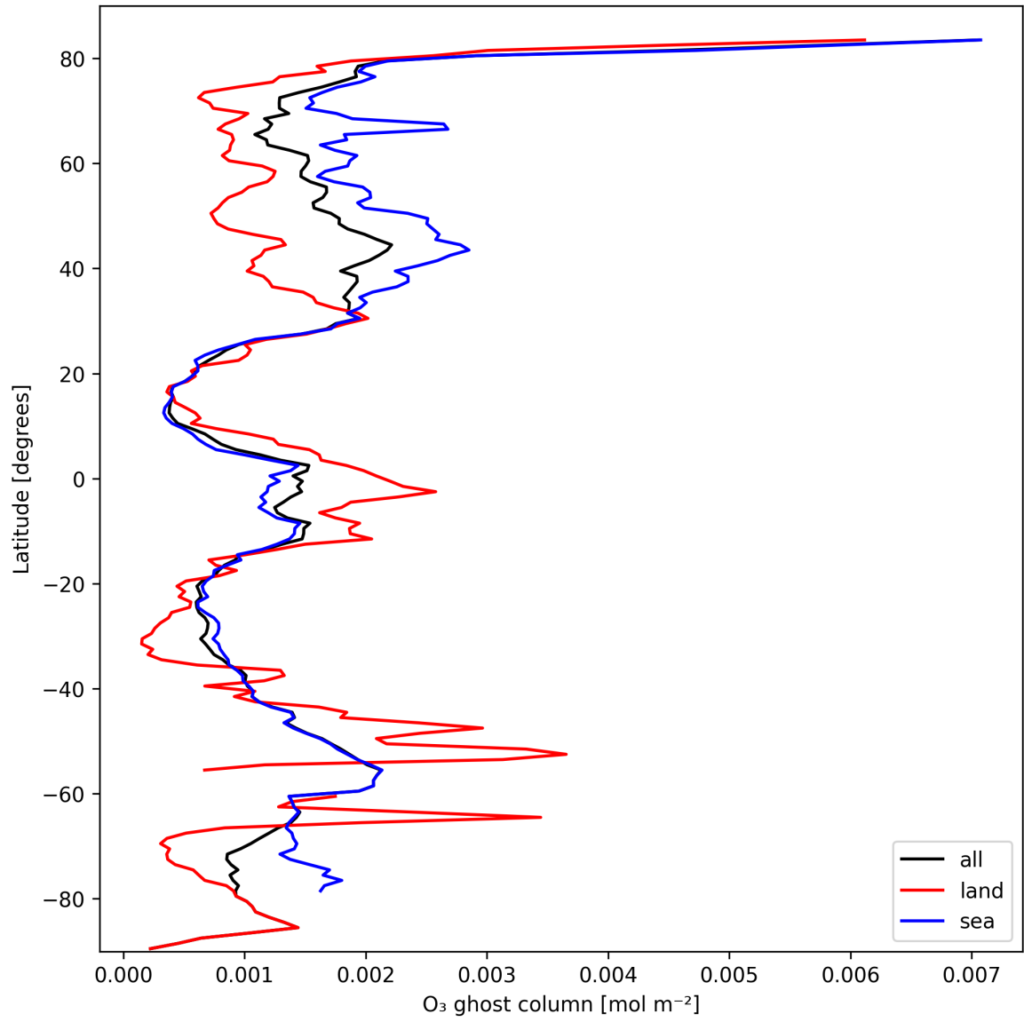
Figure 18: Zonal average of “O 3 ghost column” for 2025-03-05 to 2025-03-07.
