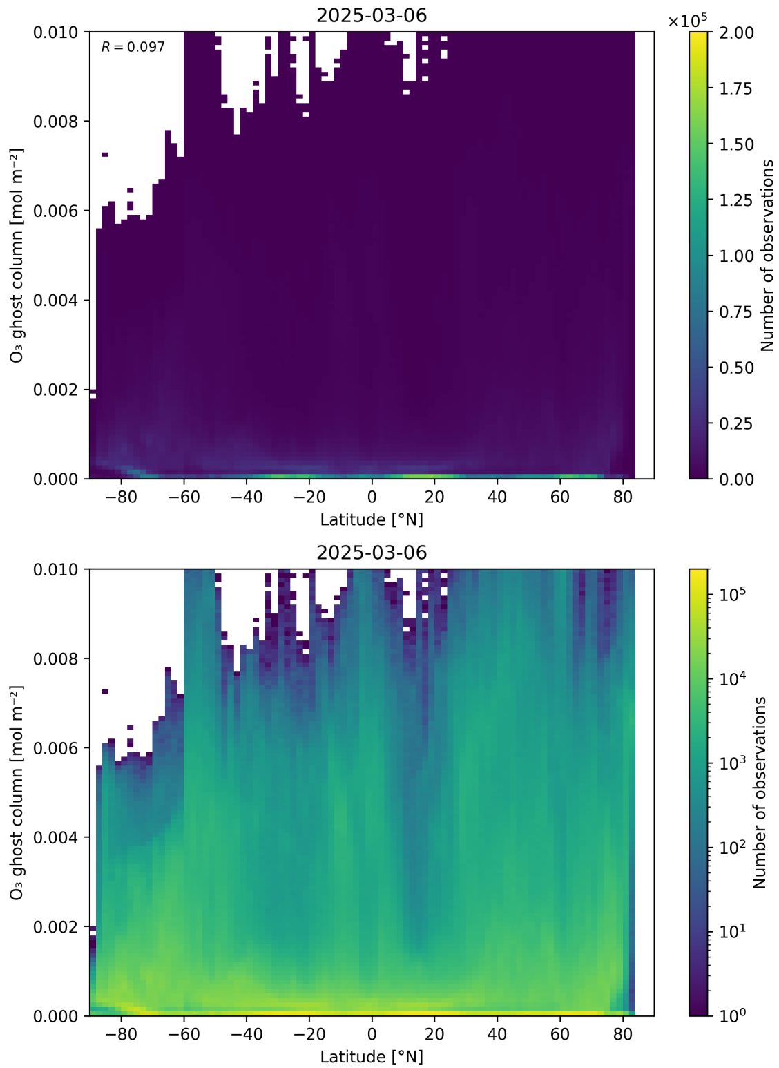
Figure 35: Scatter density plot of “Latitude” against “O 3 ghost column” for 2025-03-05 to 2025-03-07.
