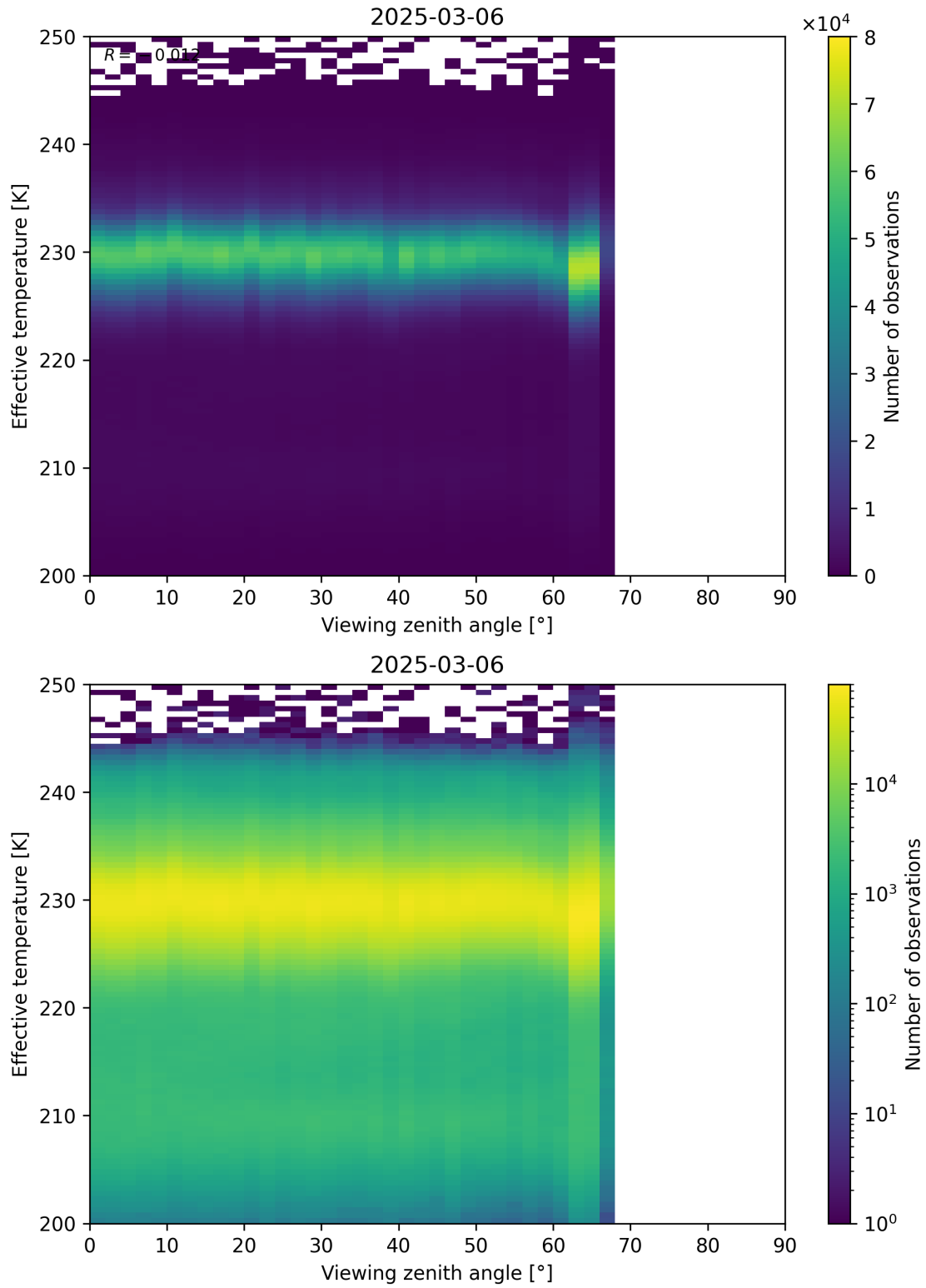
Figure 50: Scatter density plot of “Viewing zenith angle” against “Effective temperature” for 2025-03-05 to 2025-03-07.
