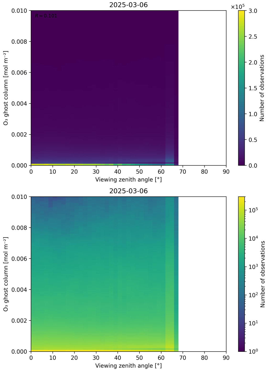
Figure 51: Scatter density plot of “Viewing zenith angle” against “O 3 ghost column” for 2025-03-05 to 2025-03-07.
