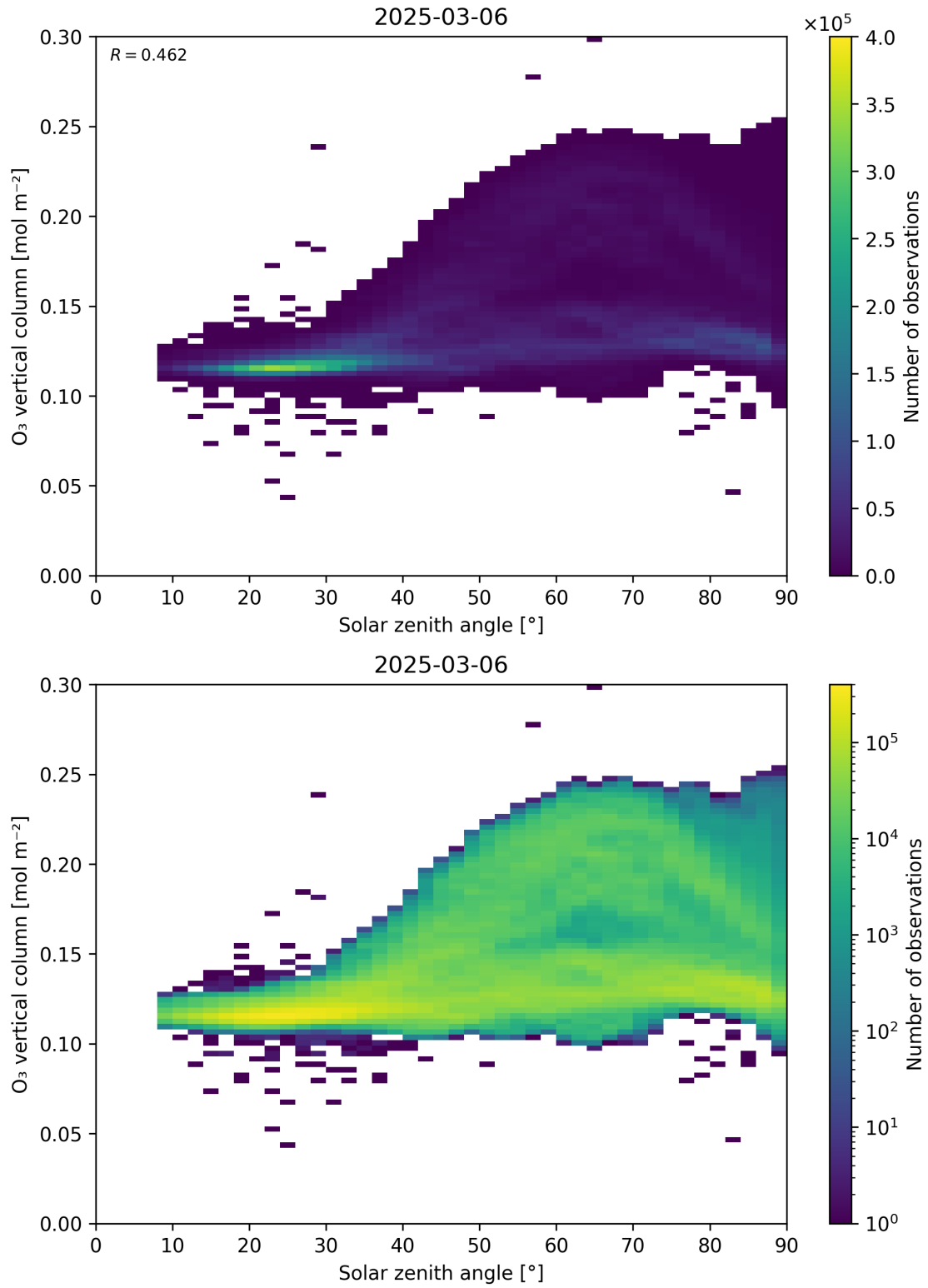
Figure 47: Scatter density plot of “Solar zenith angle” against “O 3 vertical column” for 2025-03-05 to 2025-03-07.
