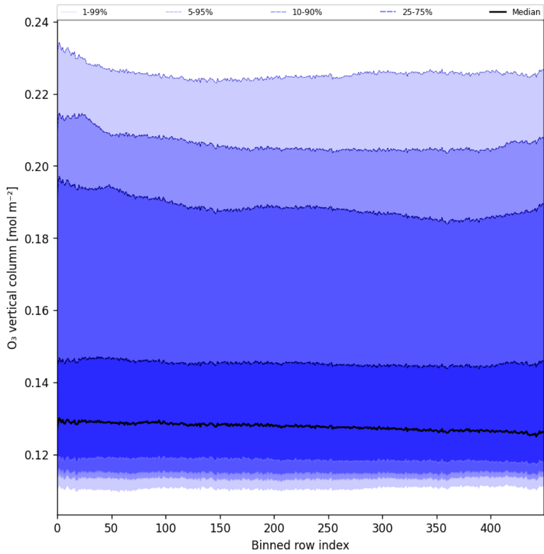
Figure 28: Along track statistics of “O 3 vertical column” for 2025-03-05 to 2025-03-07
