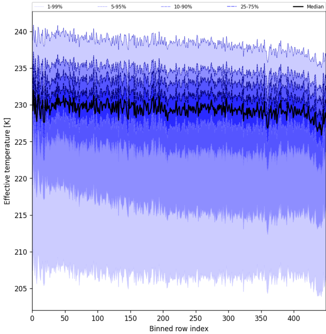
Figure 31: Along track statistics of “Effective temperature” for 2025-03-05 to 2025-03-07
