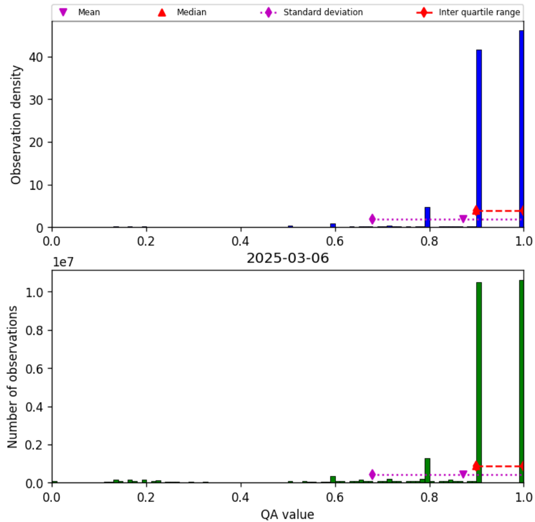
Figure 20: Histogram of “QA value” for 2025-03-05 to 2025-03-07
