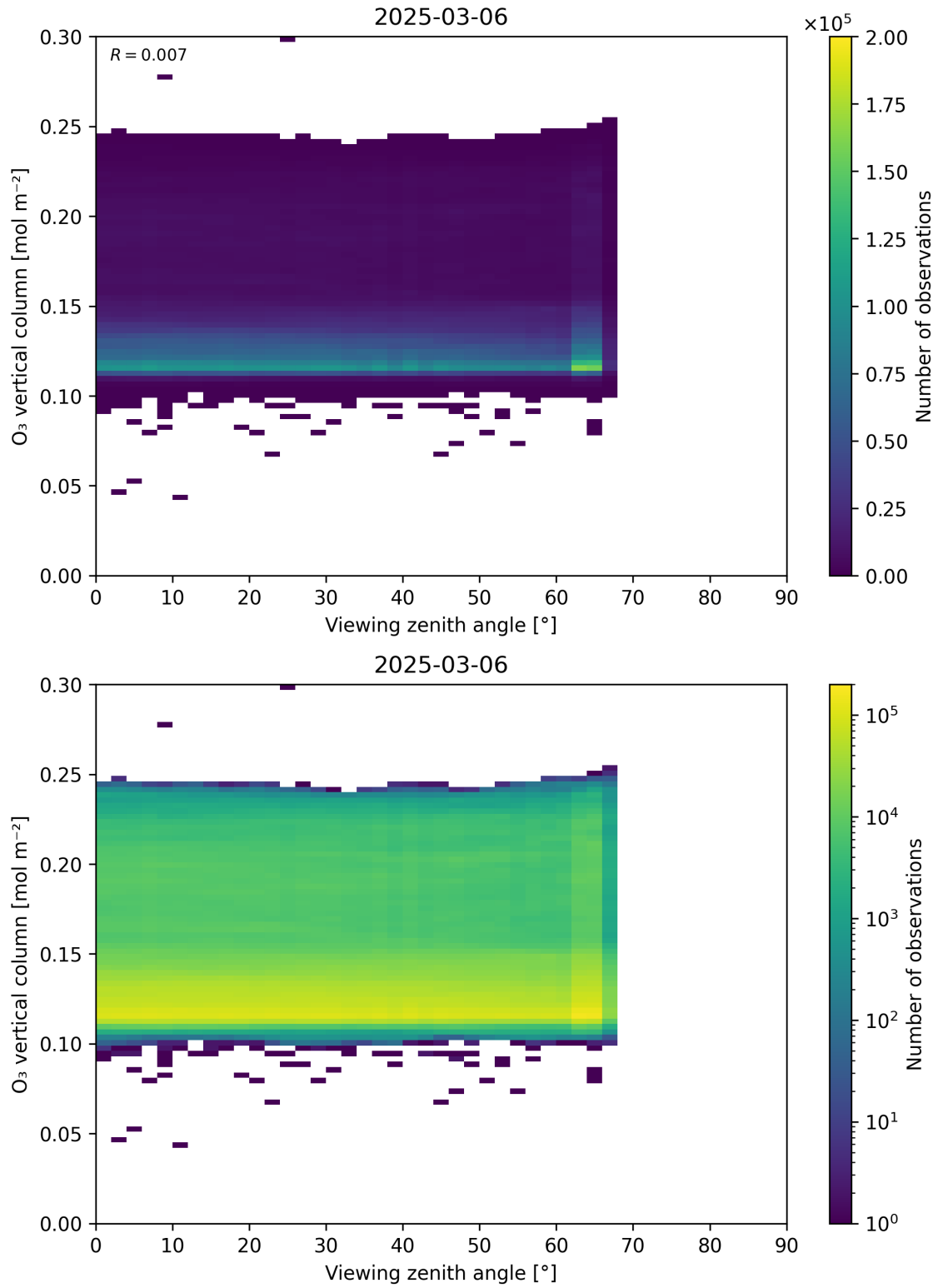
Figure 52: Scatter density plot of “Viewing zenith angle” against “O 3 vertical column” for 2025-03-05 to 2025-03-07.
