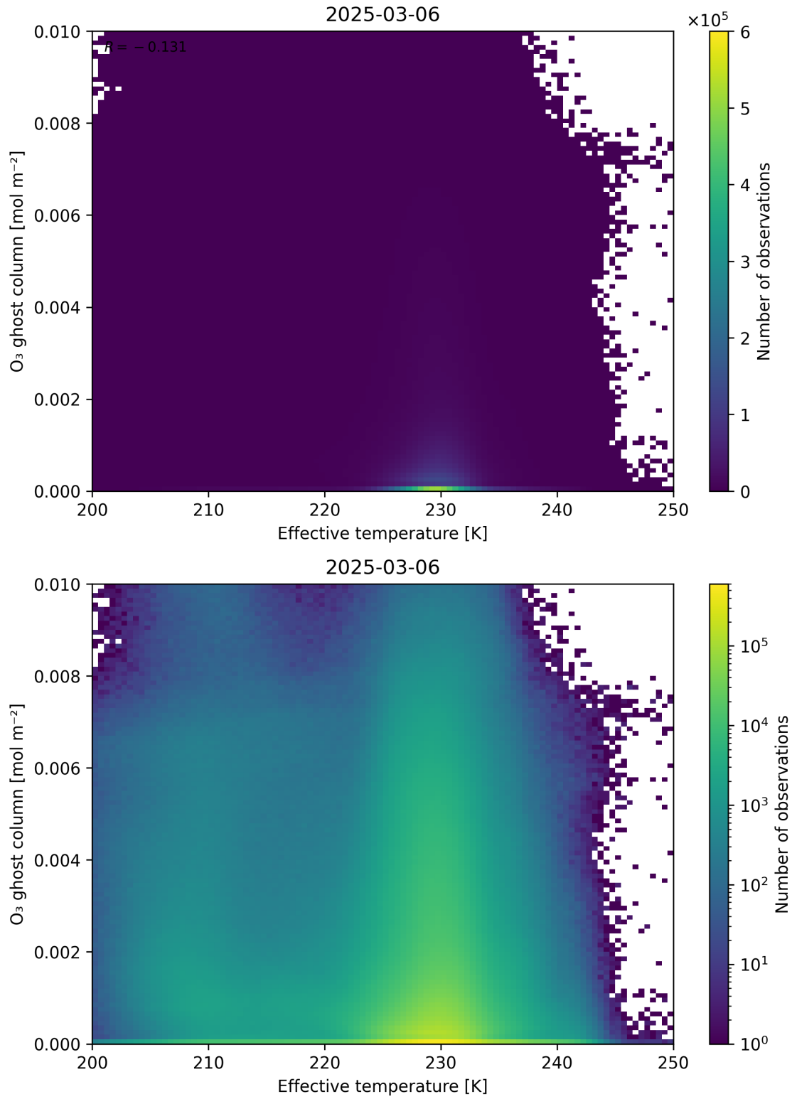
Figure 38: Scatter density plot of “Effective temperature” against “O 3 ghost column” for 2025-03-05 to 2025-03-07.
