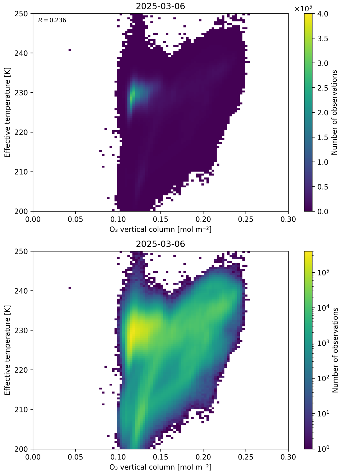
Figure 39: Scatter density plot of “O 3 vertical column” against “Effective temperature” for 2025-03-05 to 2025-03-07.
