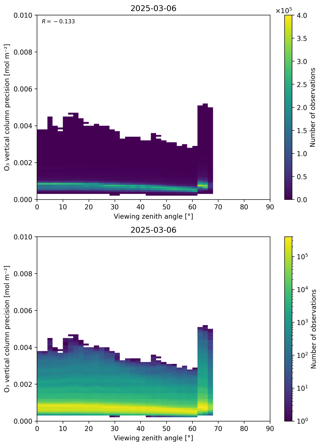
Figure 53: Scatter density plot of “Viewing zenith angle” against “O 3 vertical column precision” for 2025-03-05 to 2025-03-07.
