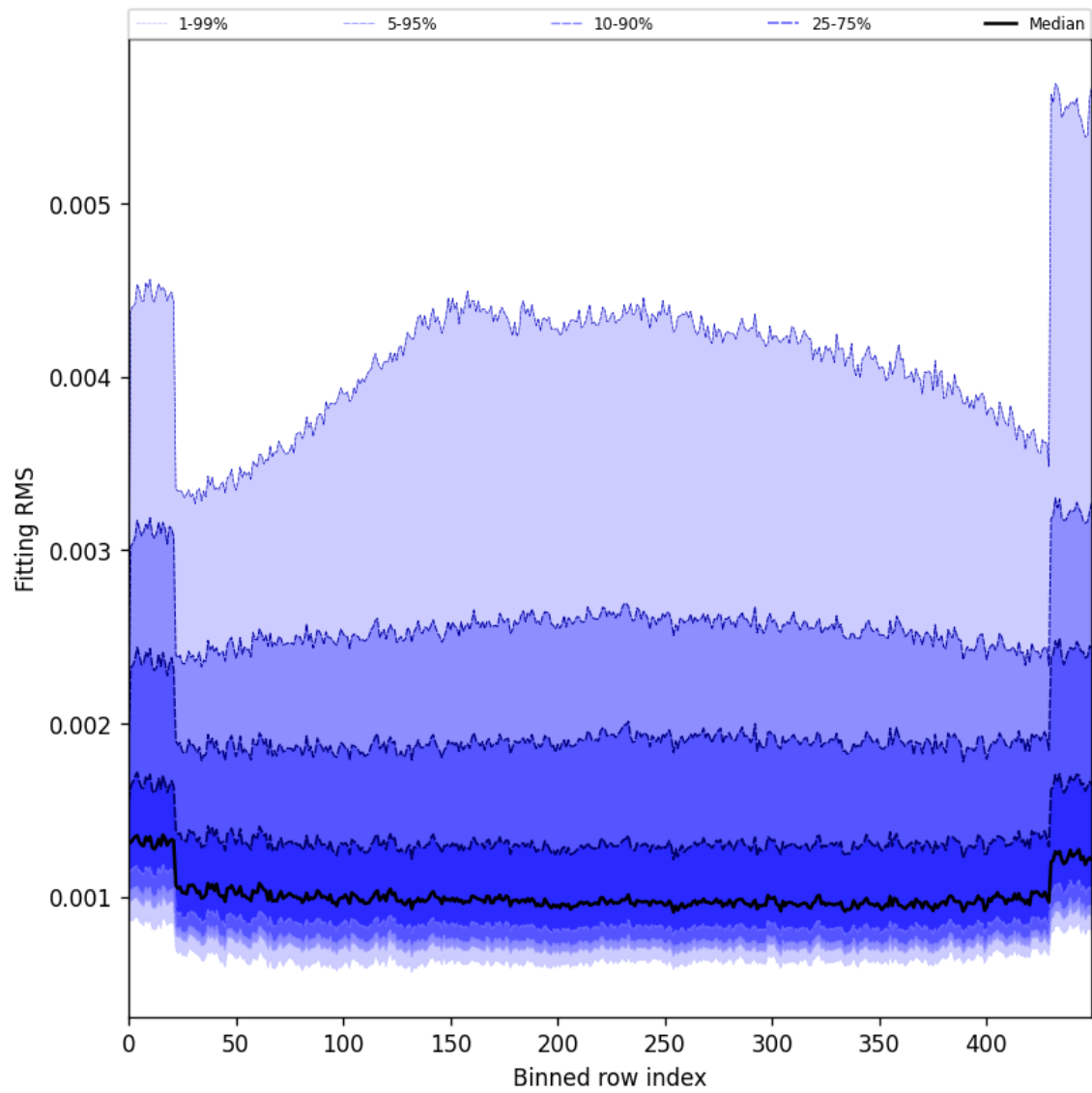
Figure 30: Along track statistics of “Fitting RMS” for 2025-03-05 to 2025-03-07
