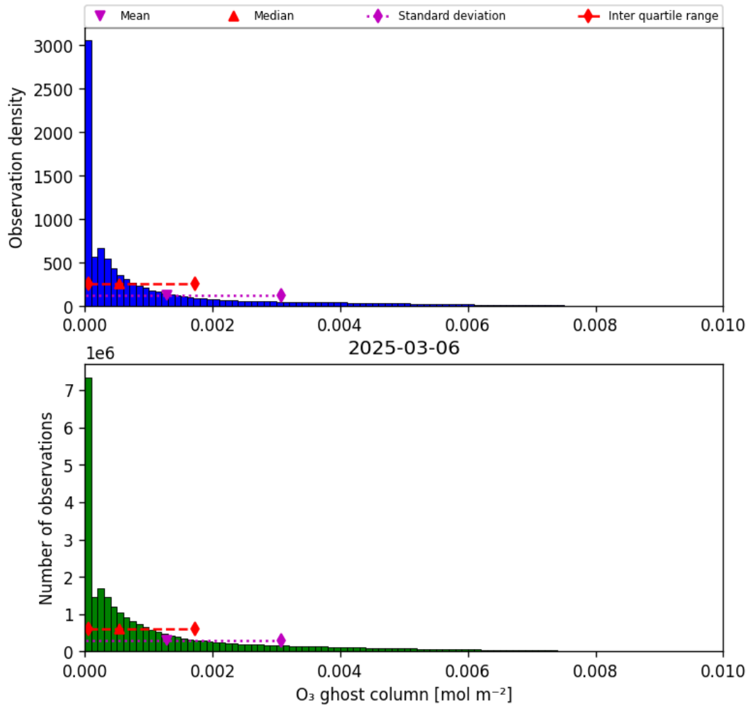
Figure 25: Histogram of “O 3 ghost column” for 2025-03-05 to 2025-03-07
