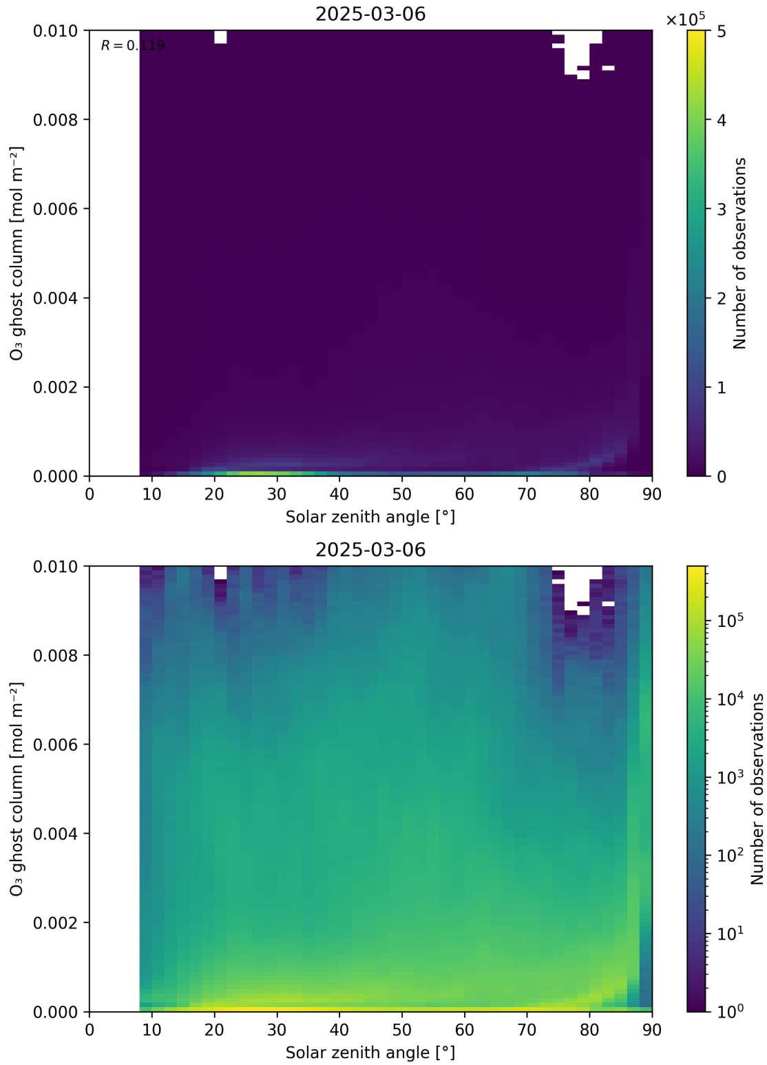
Figure 46: Scatter density plot of “Solar zenith angle” against “O 3 ghost column” for 2025-03-05 to 2025-03-07.
