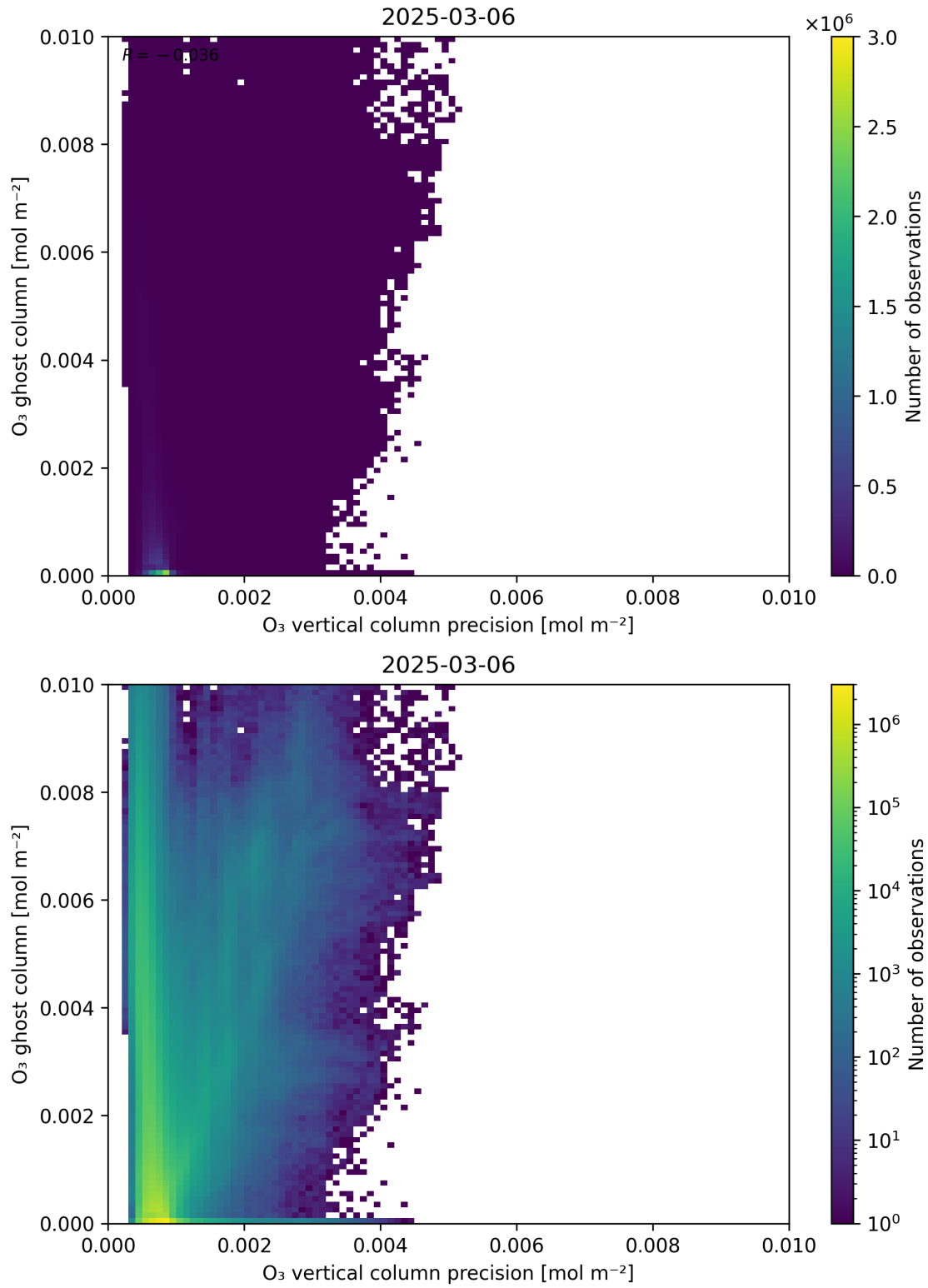
Figure 43: Scatter density plot of “ \text{O}_3 vertical column precision” against “ \text{O}_3 ghost column” for 2025-03-05 to 2025-03-07.
