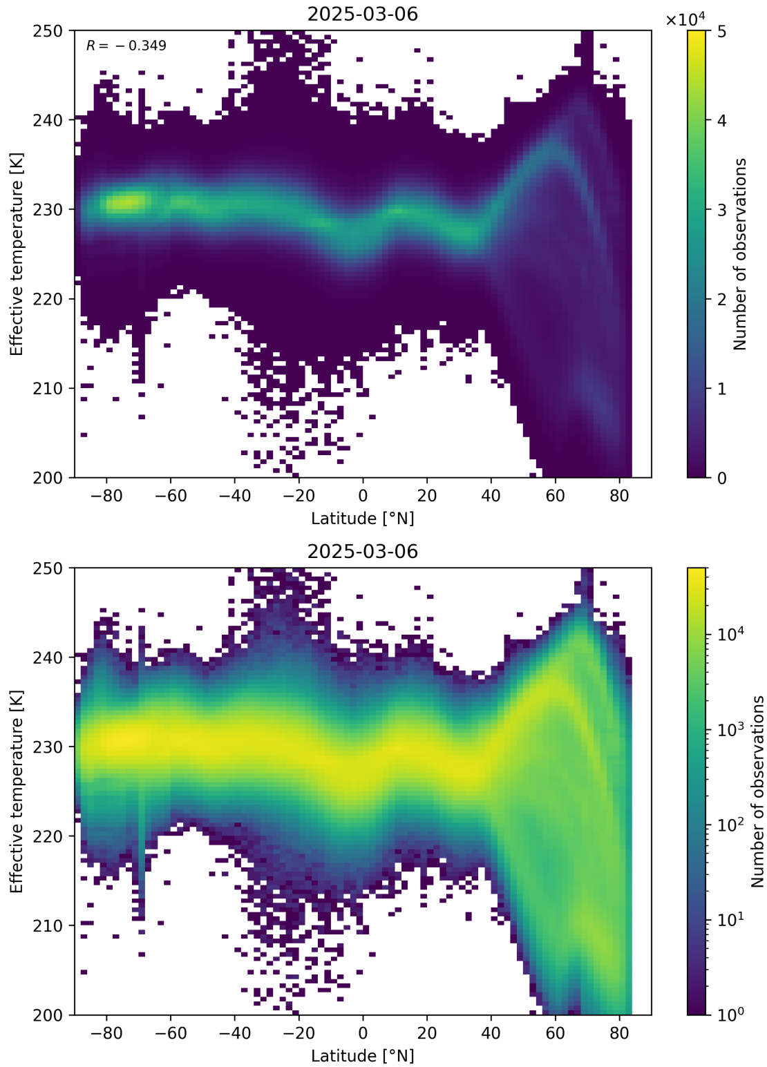
Figure 34: Scatter density plot of “Latitude” against “Effective temperature” for 2025-03-05 to 2025-03-07.
