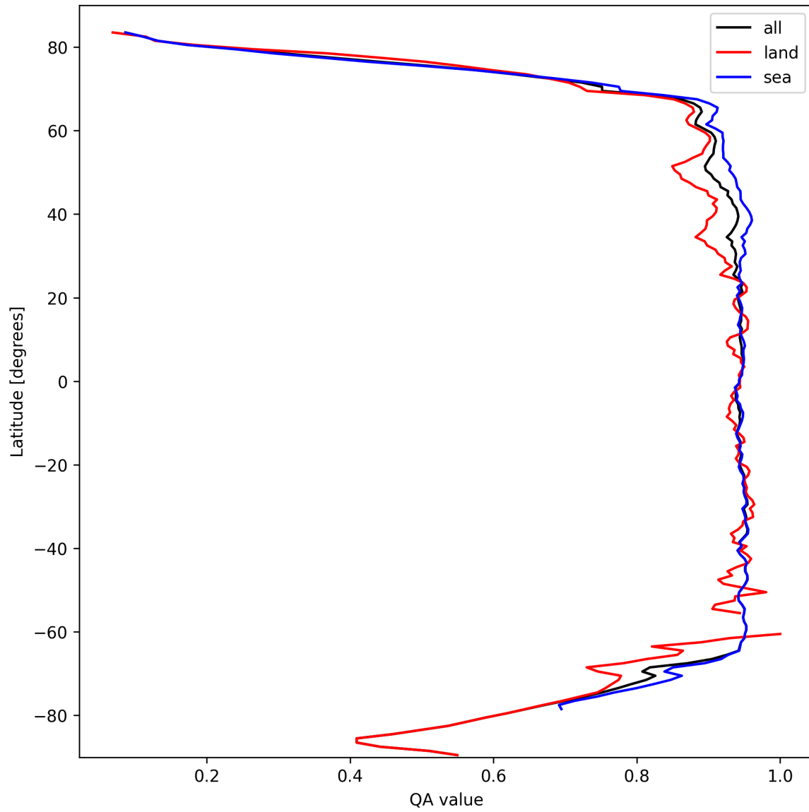
Figure 13: Zonal average of “QA value” for 2025-03-05 to 2025-03-07.
