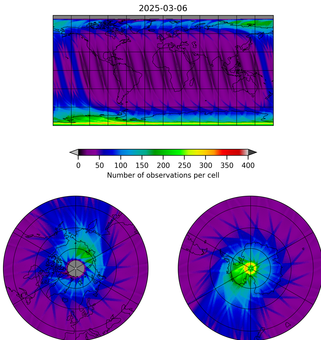
Figure 12: Map of the number of observations for 2025-03-05 to 2025-03-07
