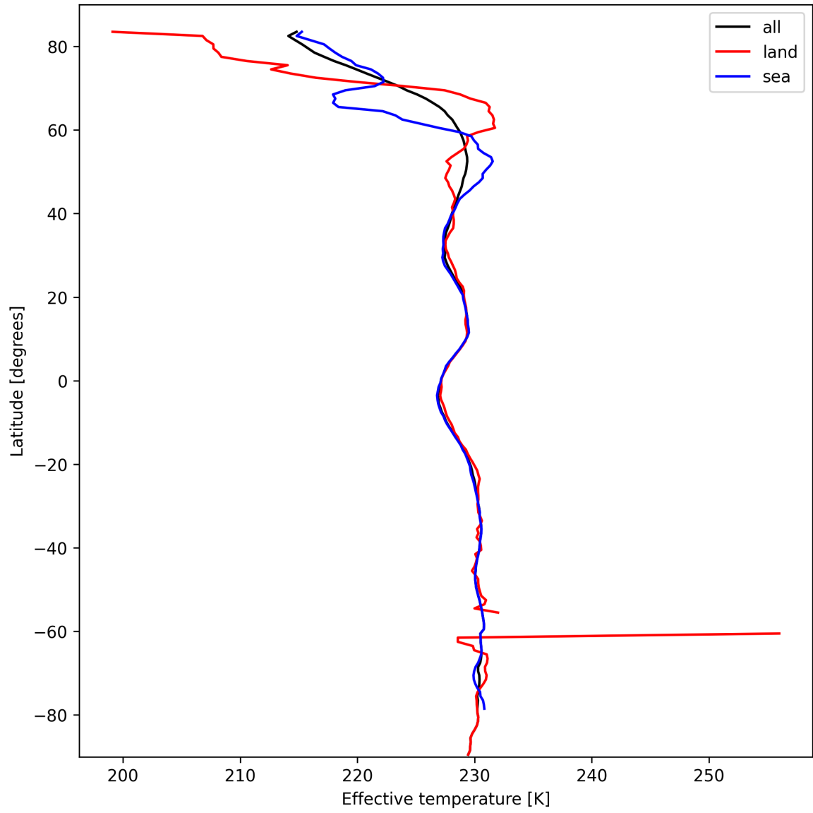
Figure 17: Zonal average of “Effective temperature” for 2025-03-05 to 2025-03-07.
