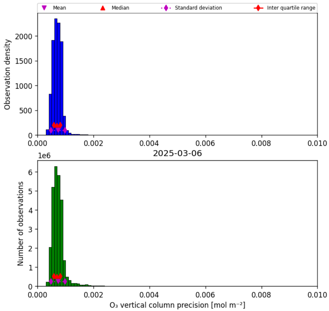
Figure 22: Histogram of "O 3 vertical column precision" for 2025-03-05 to 2025-03-07
