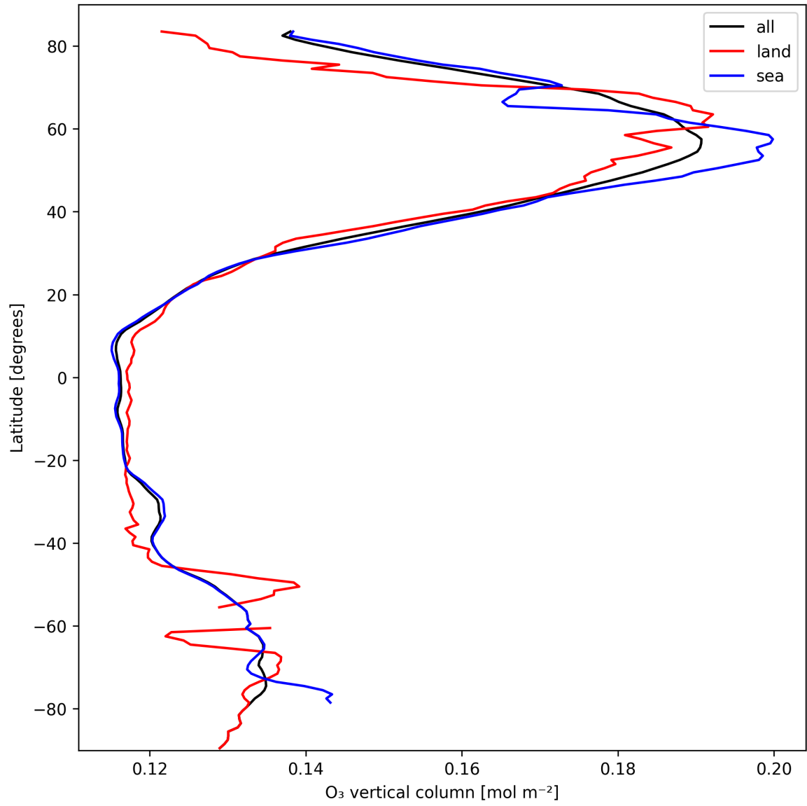
Figure 14: Zonal average of “O 3 vertical column” for 2025-03-05 to 2025-03-07.
