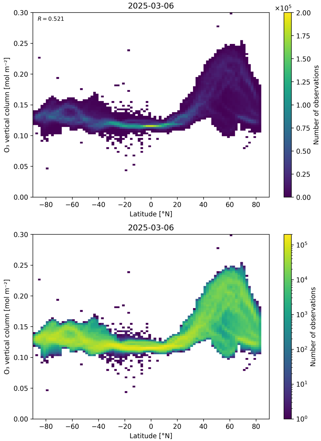
Figure 36: Scatter density plot of “Latitude” against “O 3 vertical column” for 2025-03-05 to 2025-03-07.
