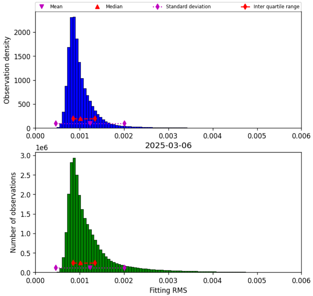
Figure 23: Histogram of “Fitting RMS” for 2025-03-05 to 2025-03-07
