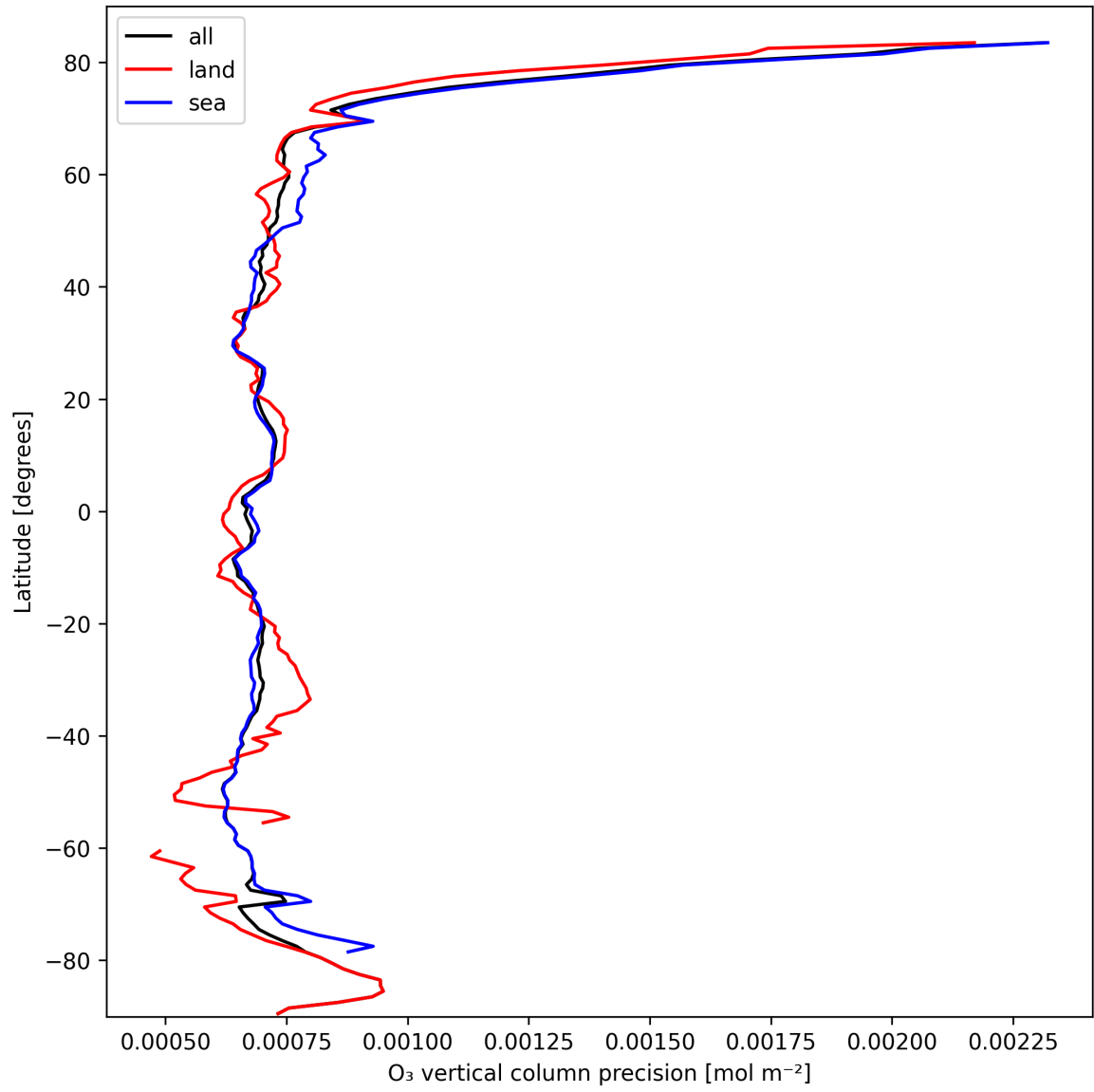
Figure 15: Zonal average of “O 3 vertical column precision” for 2025-03-05 to 2025-03-07.
