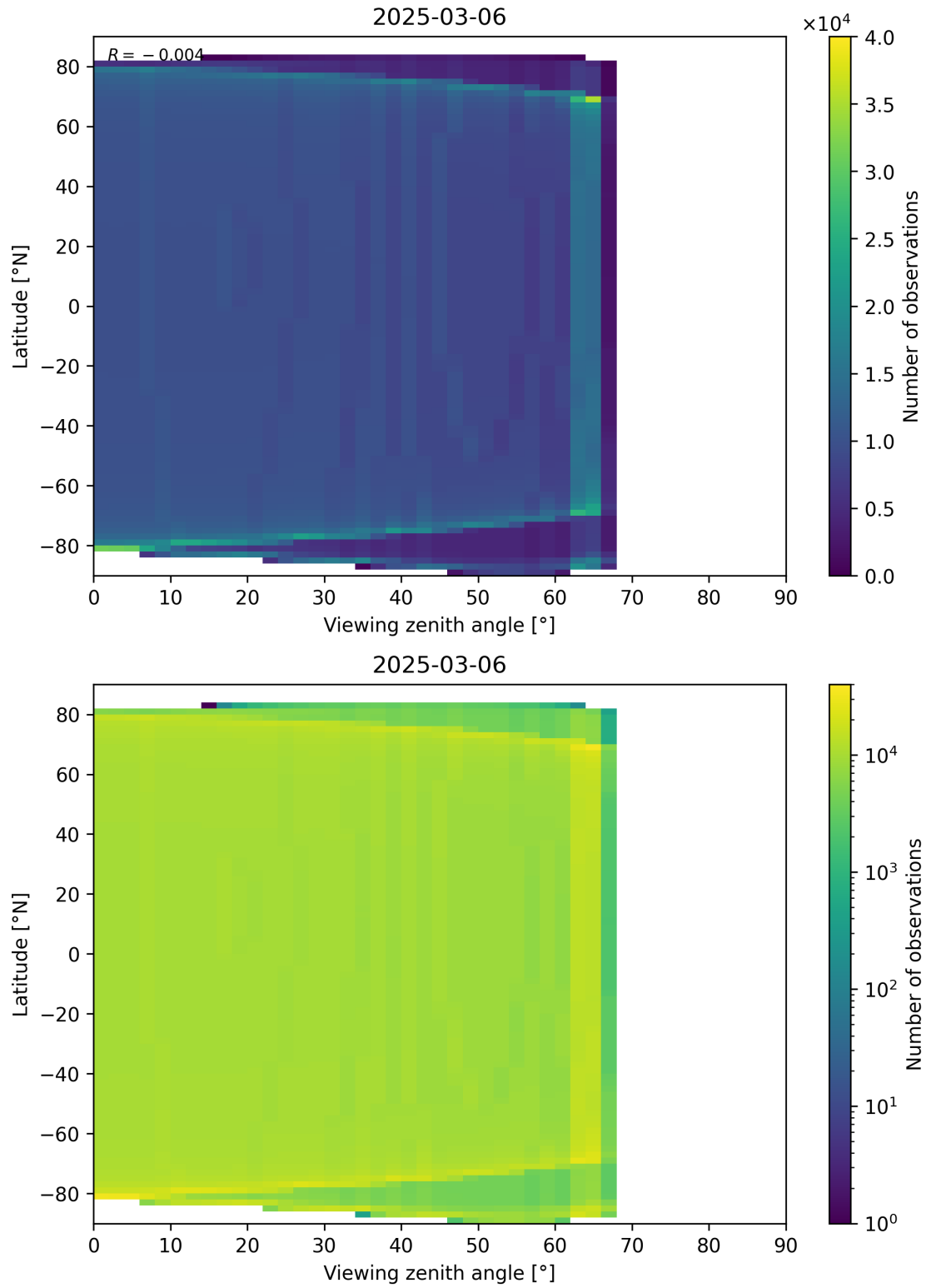
Figure 49: Scatter density plot of “Viewing zenith angle” against “Latitude” for 2025-03-05 to 2025-03-07.
