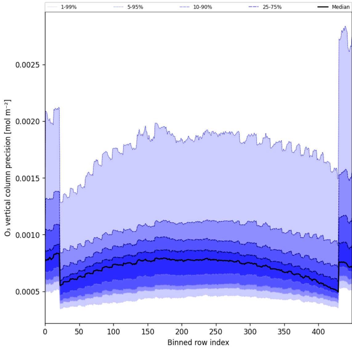
Figure 29: Along track statistics of “O 3 vertical column precision” for 2025-03-05 to 2025-03-07
