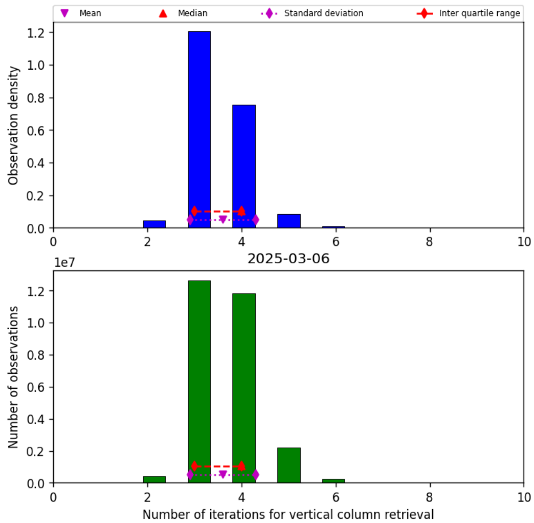
Figure 26: Histogram of “Number of iterations for vertical column retrieval” for 2025-03-05 to 2025-03-07
