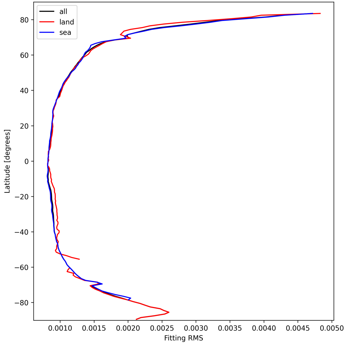
Figure 16: Zonal average of “Fitting RMS” for 2025-03-05 to 2025-03-07.
