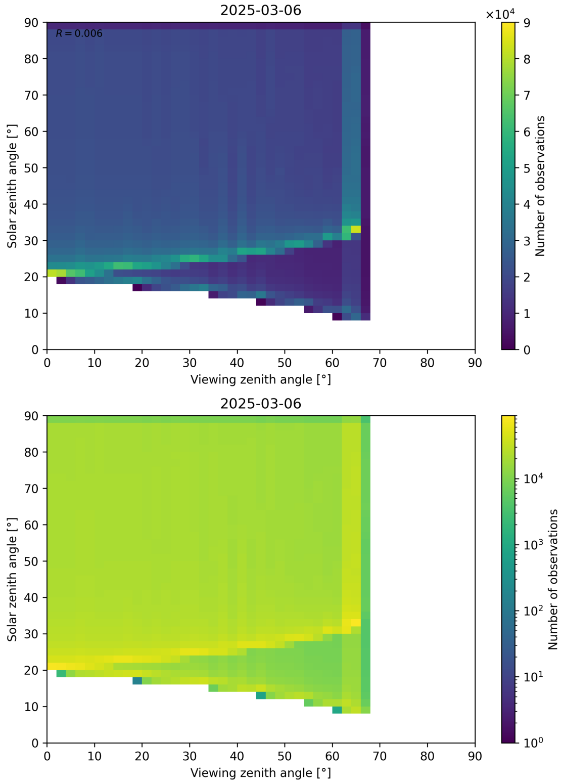
Figure 54: Scatter density plot of “Viewing zenith angle” against “Solar zenith angle” for 2025-03-05 to 2025-03-07.
