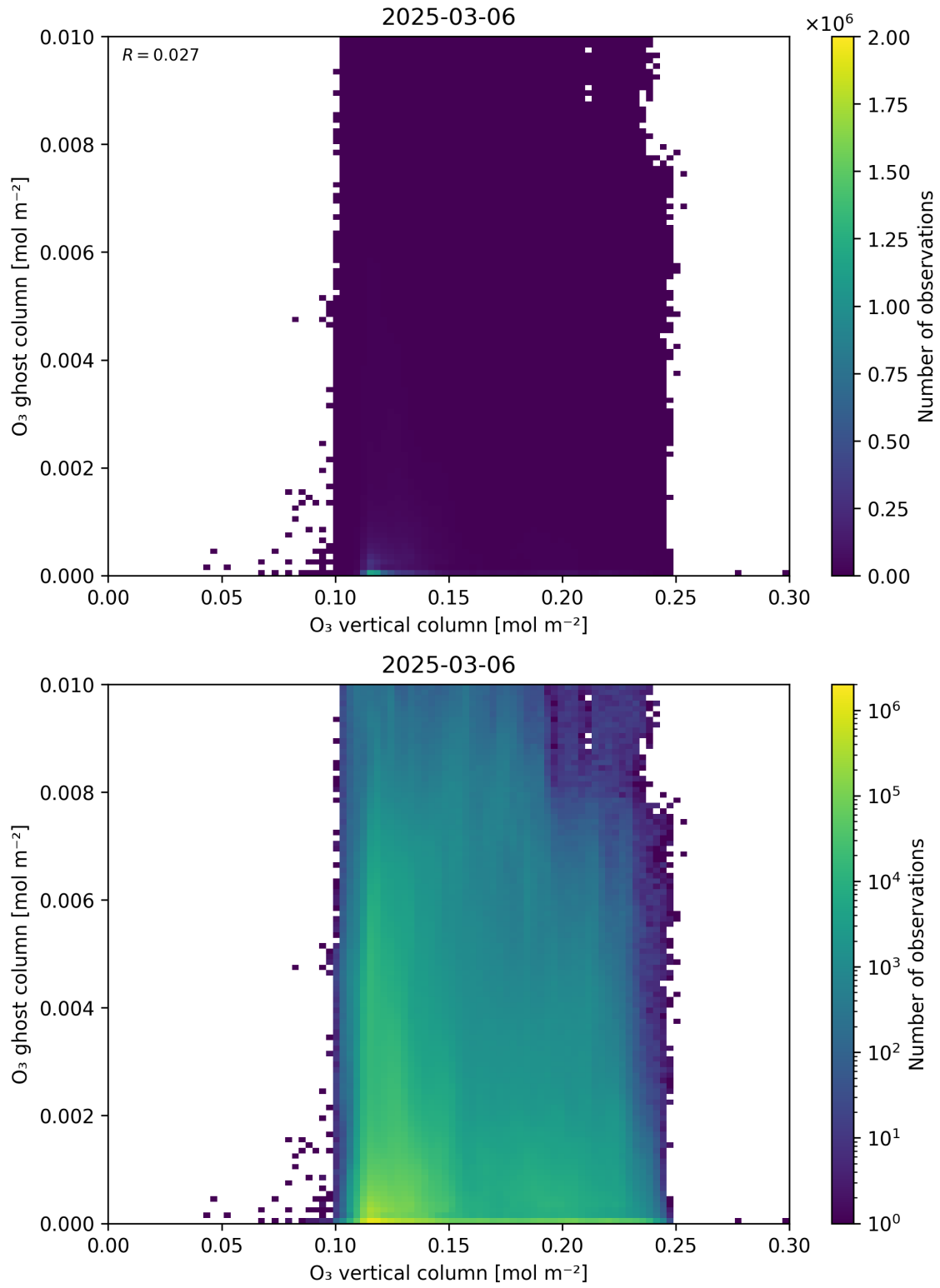
Figure 40: Scatter density plot of “O 3 vertical column” against “O 3 ghost column” for 2025-03-05 to 2025-03-07.
