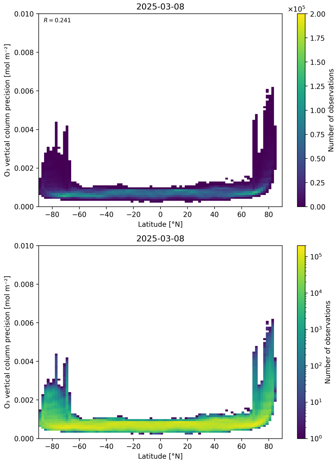
Figure 37: Scatter density plot of “Latitude” against “O 3 vertical column precision” for 2025-03-07 to 2025-03-09.
