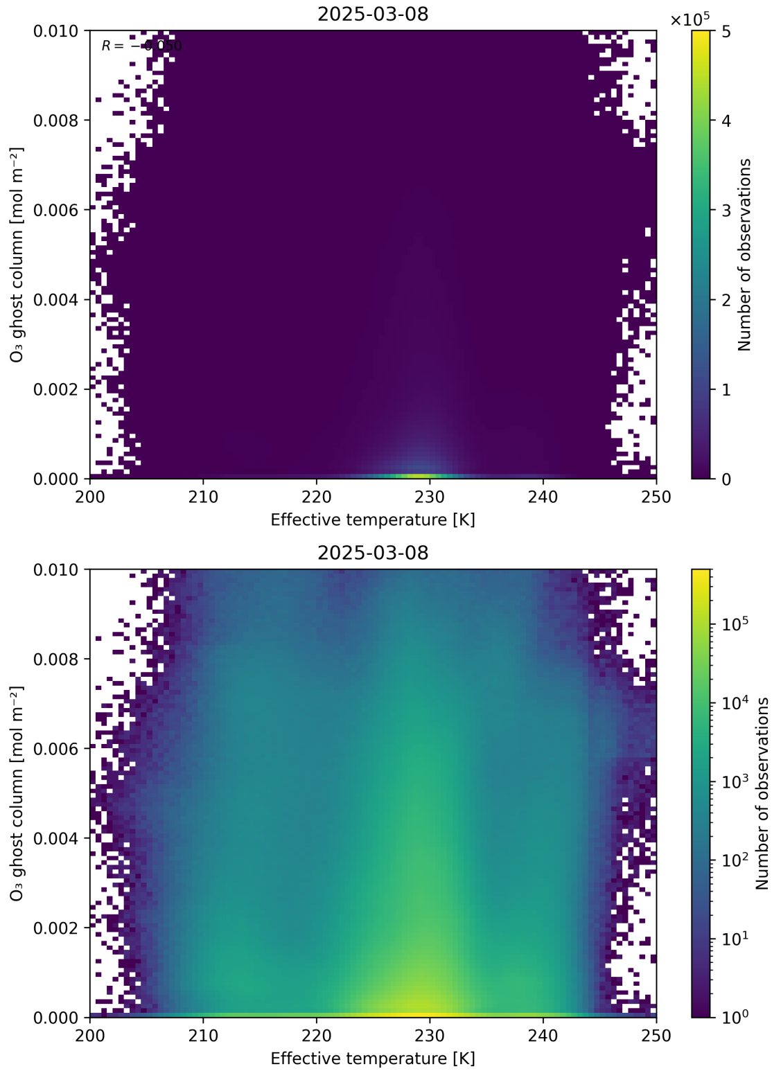
Figure 38: Scatter density plot of “Effective temperature” against “O 3 ghost column” for 2025-03-07 to 2025-03-09.
