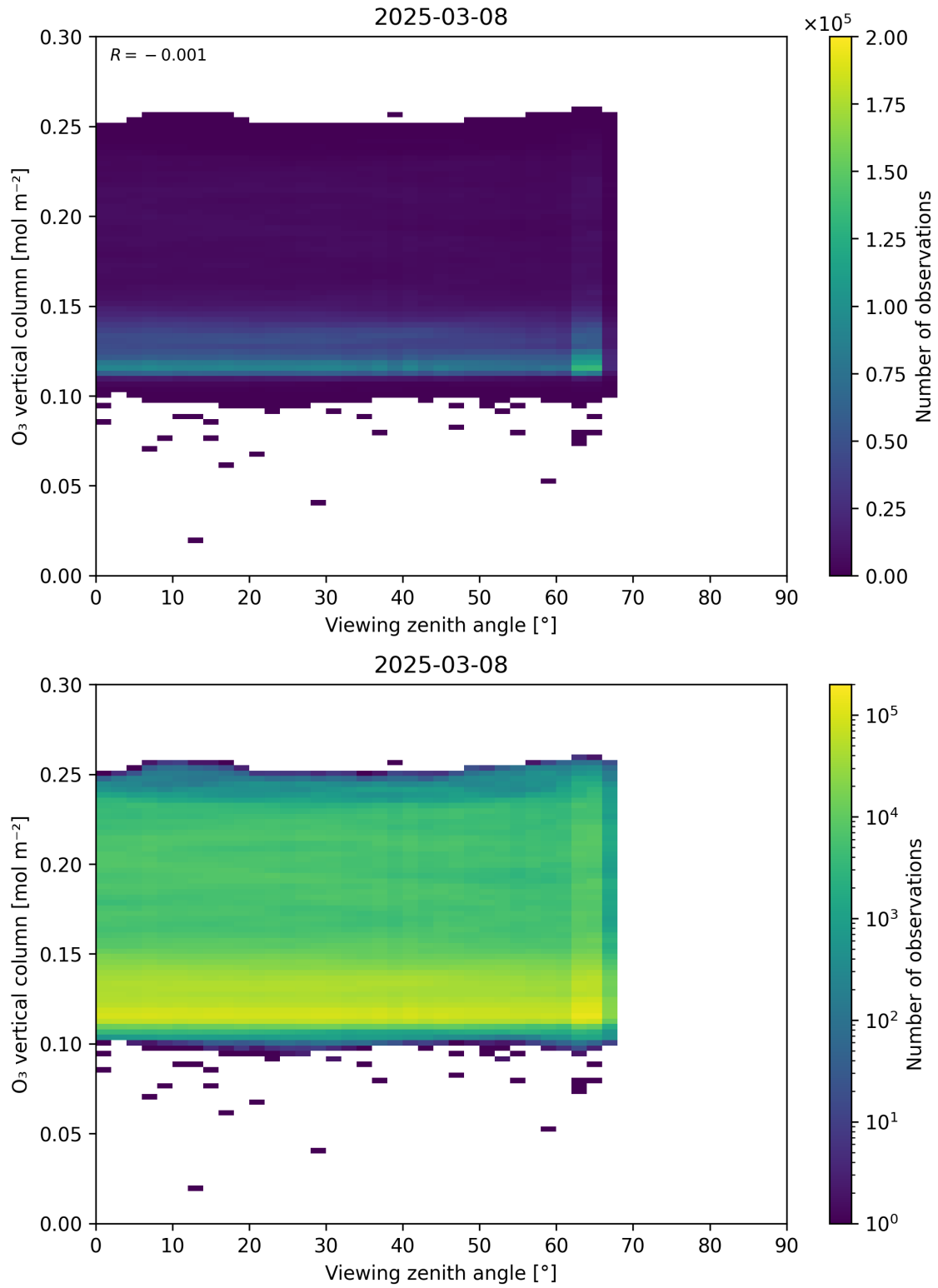
Figure 52: Scatter density plot of “Viewing zenith angle” against “O 3 vertical column” for 2025-03-07 to 2025-03-09.
