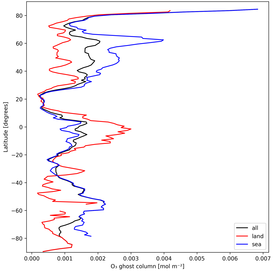
Figure 18: Zonal average of “O 3 ghost column” for 2025-03-07 to 2025-03-09.
