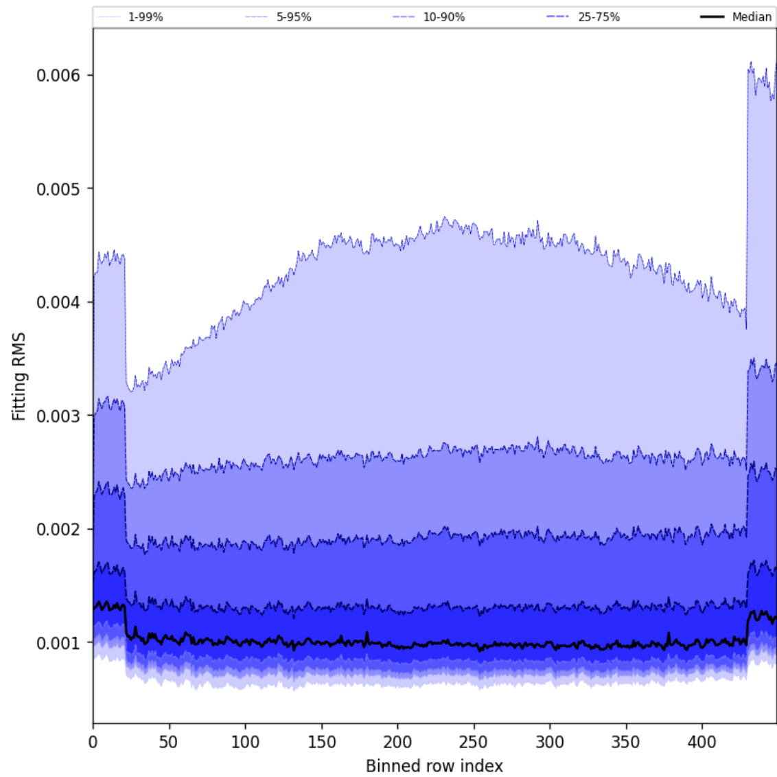
Figure 30: Along track statistics of “Fitting RMS” for 2025-03-07 to 2025-03-09
