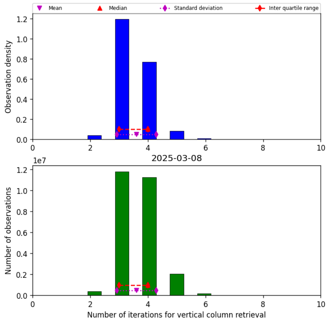
Figure 26: Histogram of “Number of iterations for vertical column retrieval” for 2025-03-07 to 2025-03-09
