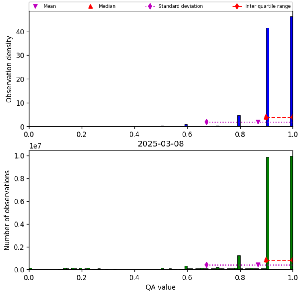
Figure 20: Histogram of “QA value” for 2025-03-07 to 2025-03-09
