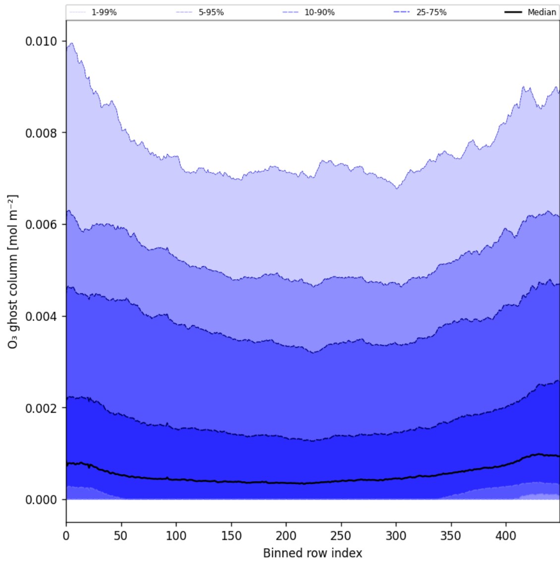
Figure 32: Along track statistics of “O 3 ghost column” for 2025-03-07 to 2025-03-09
