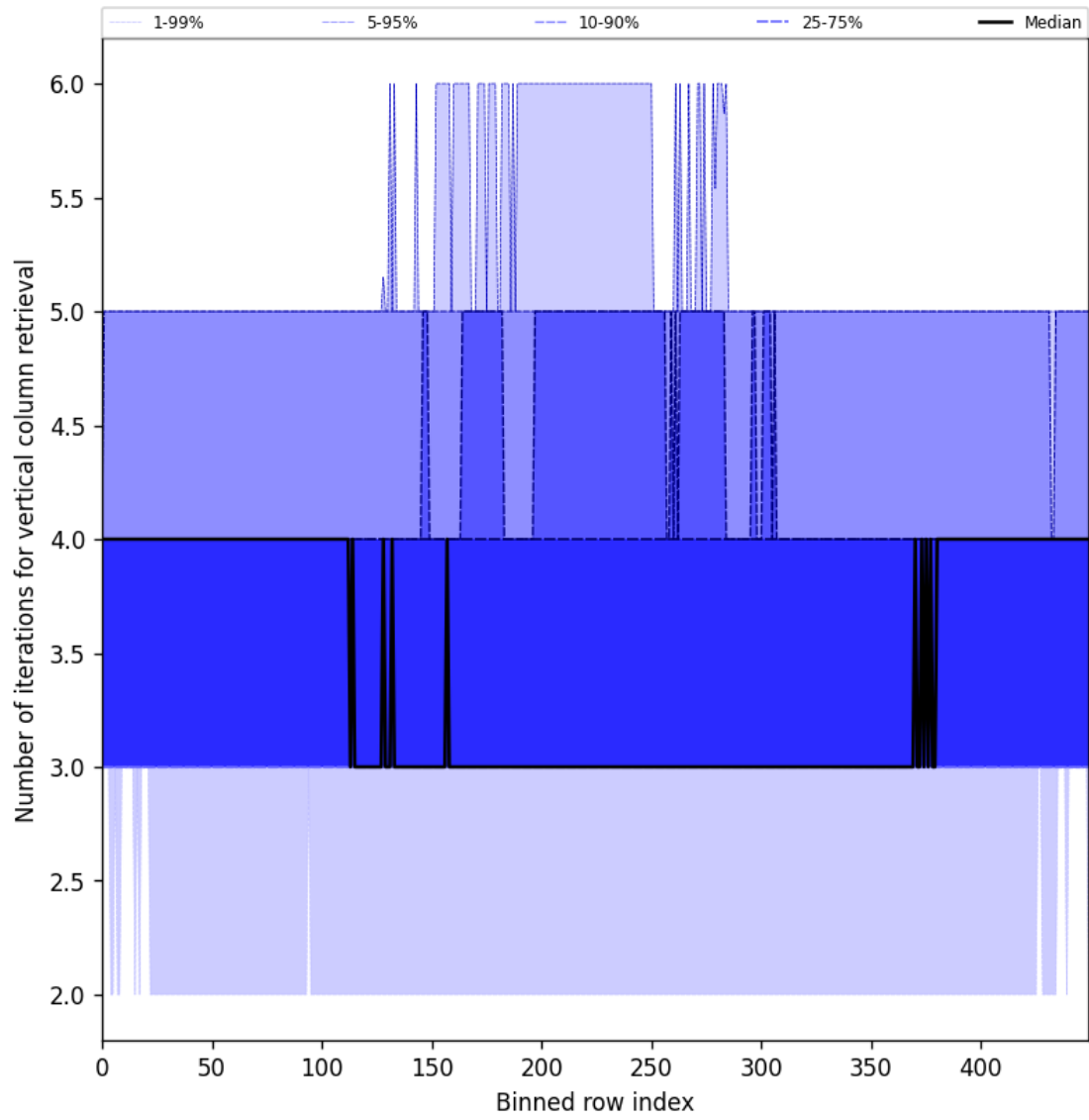
Figure 33: Along track statistics of “Number of iterations for vertical column retrieval” for 2025-03-07 to 2025-03-09
