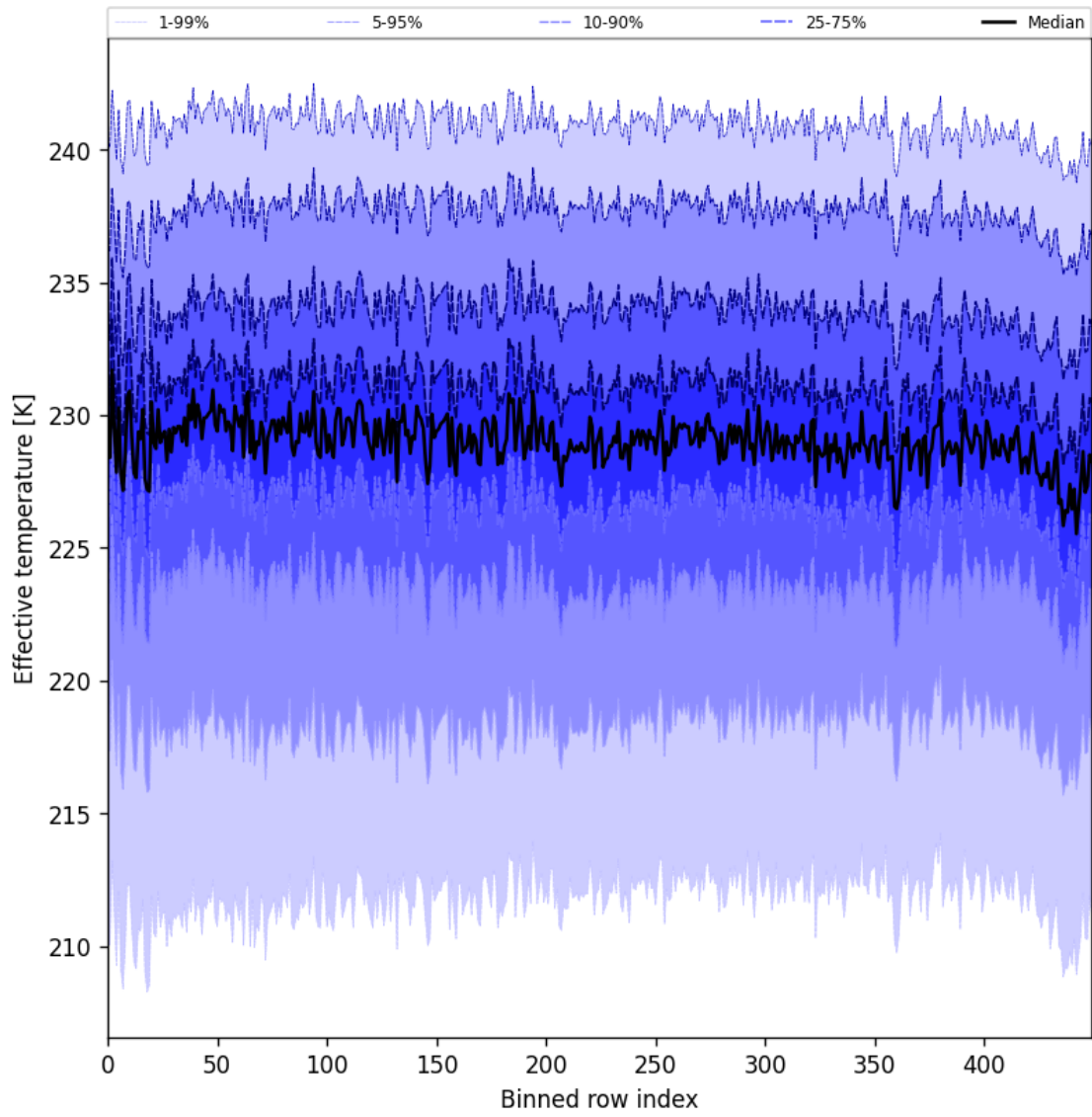
Figure 31: Along track statistics of “Effective temperature” for 2025-03-07 to 2025-03-09
