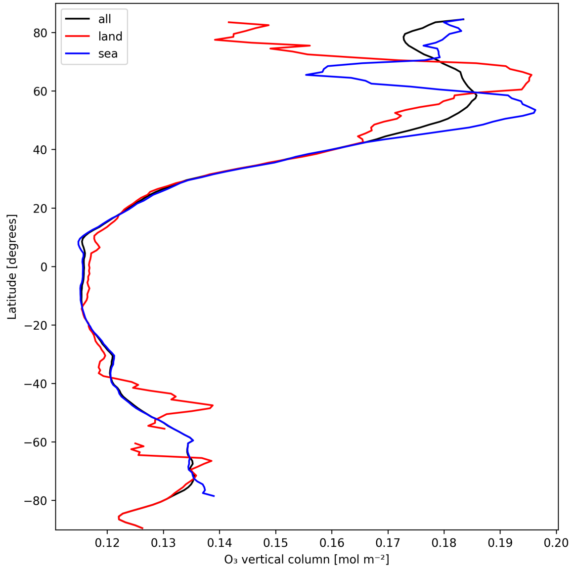
Figure 14: Zonal average of “O 3 vertical column” for 2025-03-07 to 2025-03-09.
