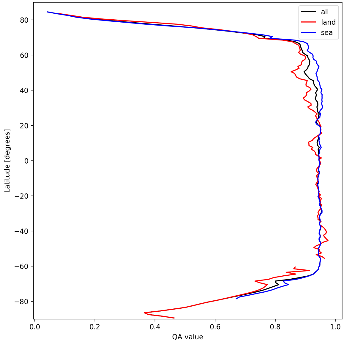
Figure 13: Zonal average of “QA value” for 2025-03-07 to 2025-03-09.
