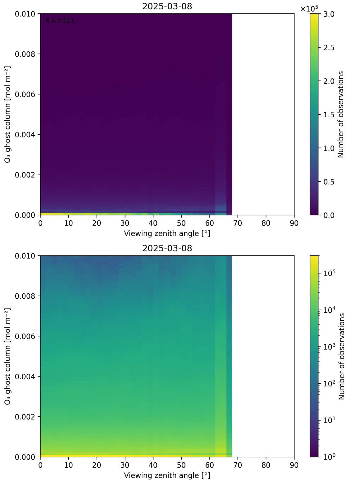
Figure 51: Scatter density plot of “Viewing zenith angle” against “O 3 ghost column” for 2025-03-07 to 2025-03-09.
