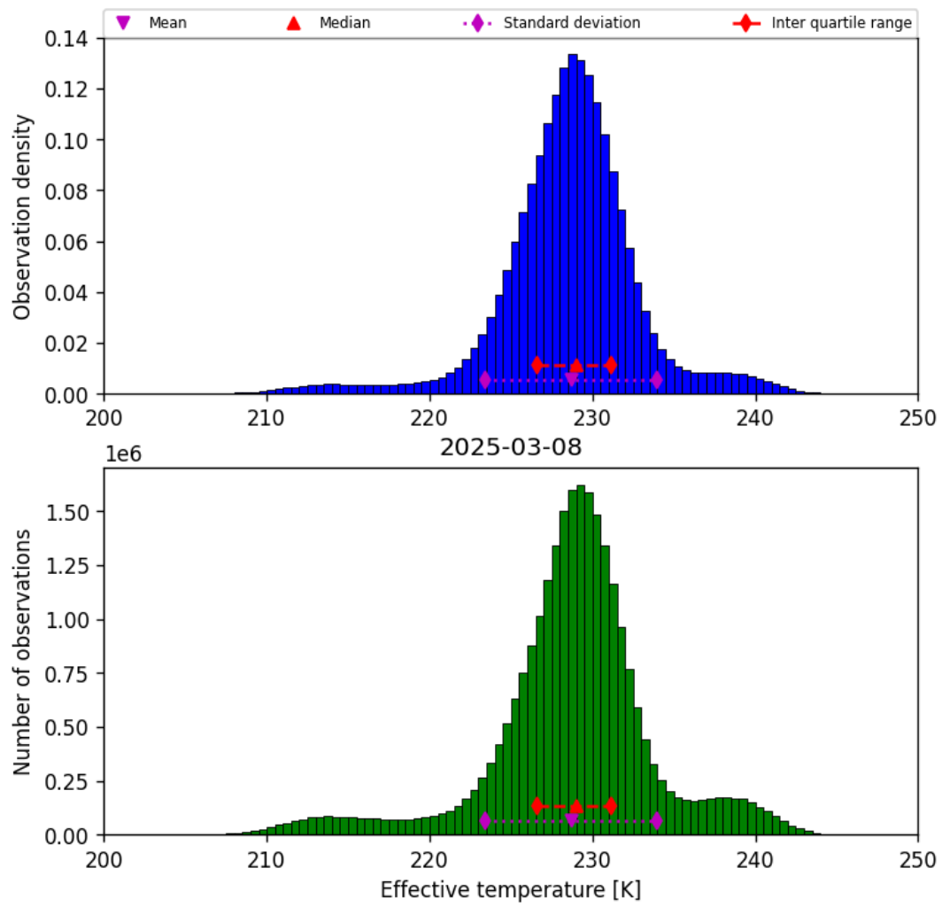
Figure 24: Histogram of “Effective temperature” for 2025-03-07 to 2025-03-09
