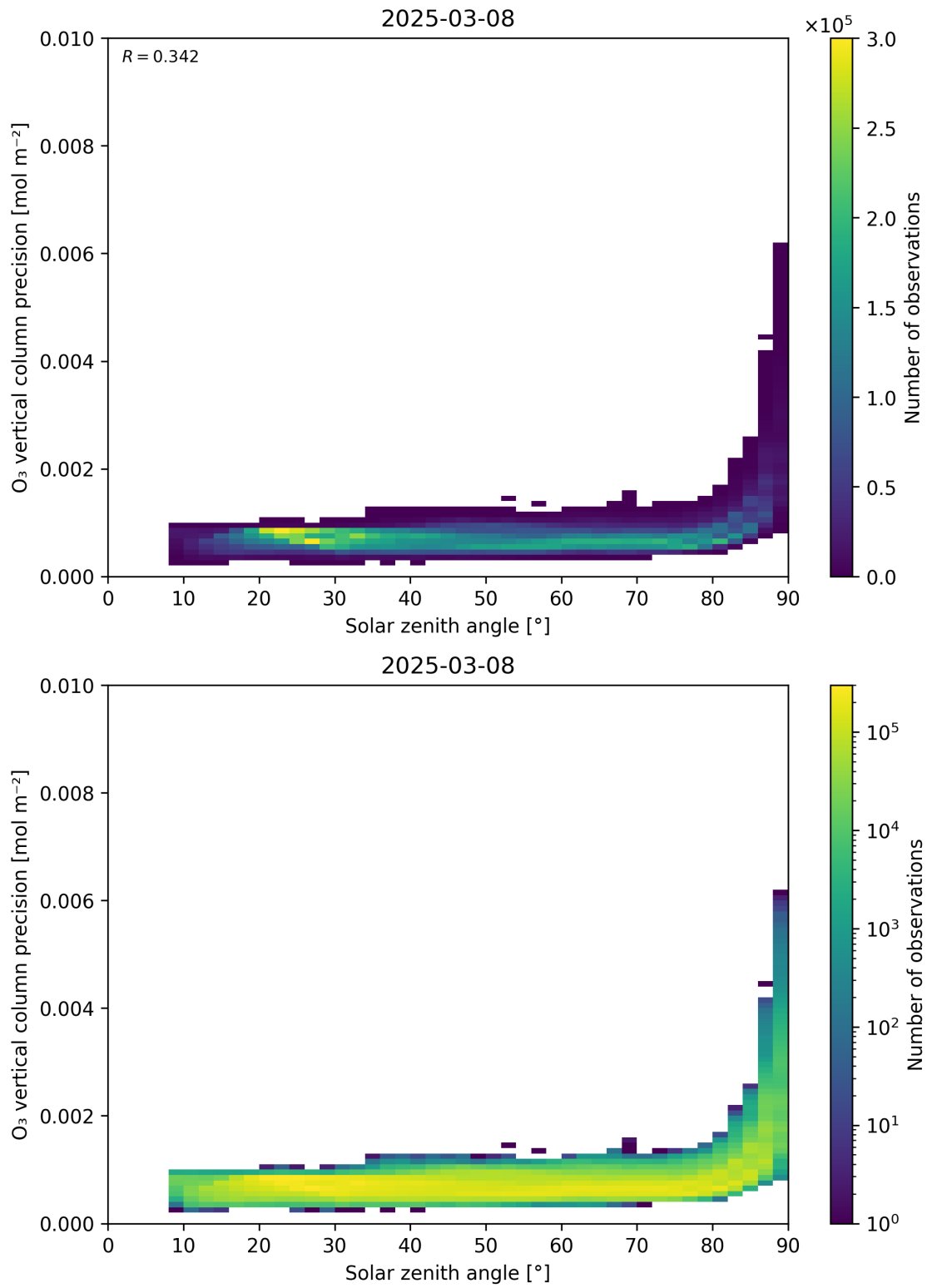
Figure 48: Scatter density plot of “Solar zenith angle” against “O 3 vertical column precision” for 2025-03-07 to 2025-03-09.
