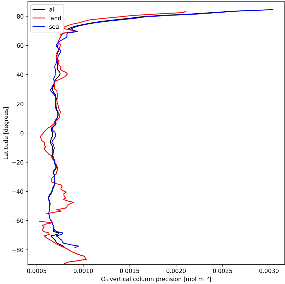
Figure 15: Zonal average of “O 3 vertical column precision” for 2025-03-07 to 2025-03-09.
