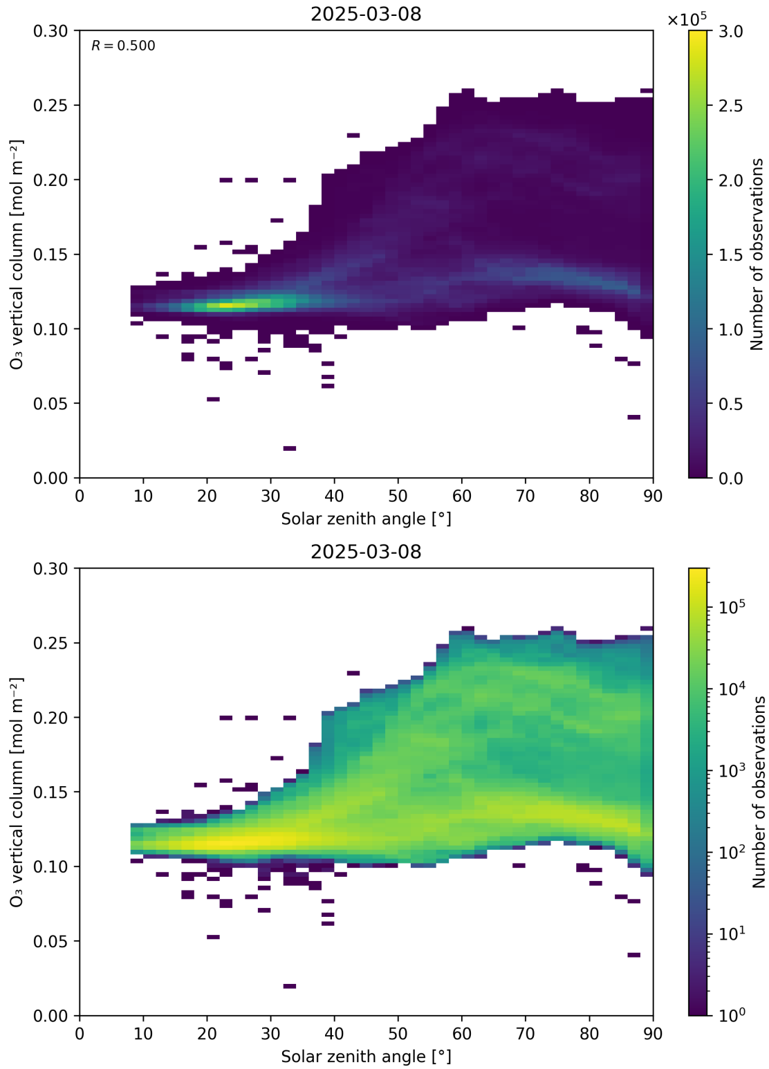
Figure 47: Scatter density plot of “Solar zenith angle” against “O 3 vertical column” for 2025-03-07 to 2025-03-09.
