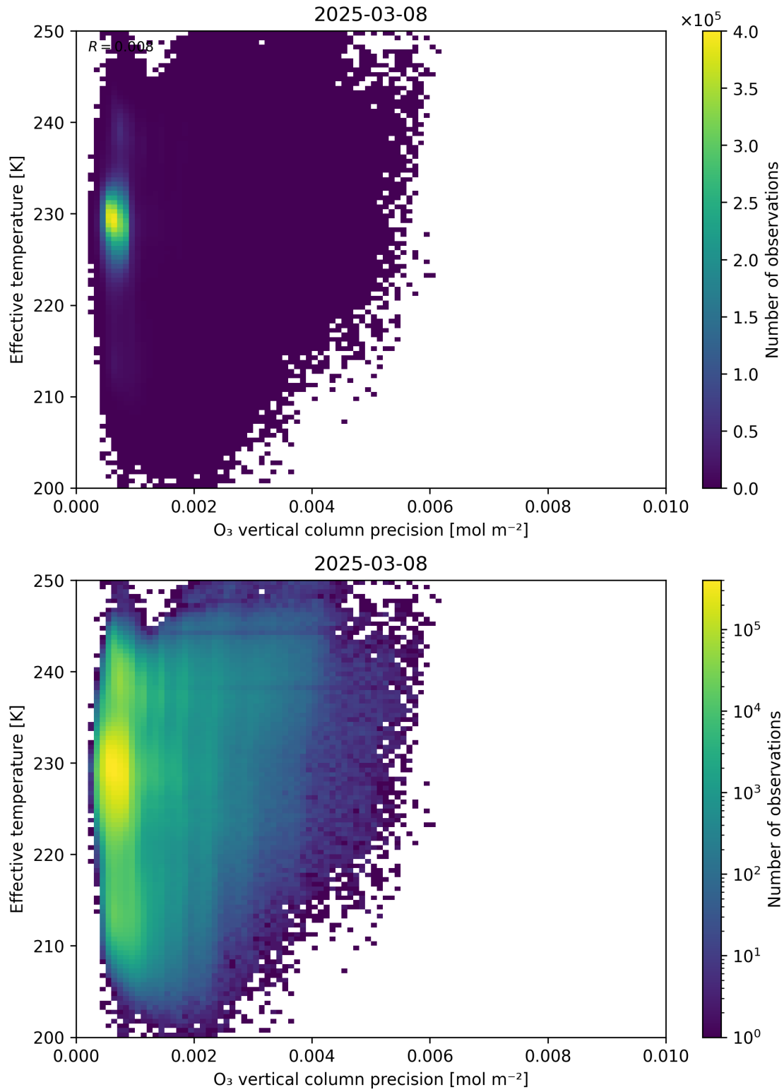
Figure 42: Scatter density plot of “O 3 vertical column precision” against “Effective temperature” for 2025-03-07 to 2025-03-09.
