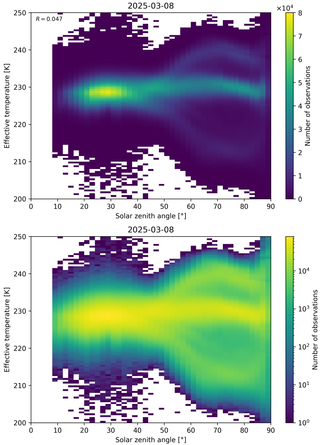
Figure 45: Scatter density plot of “Solar zenith angle” against “Effective temperature” for 2025-03-07 to 2025-03-09.
