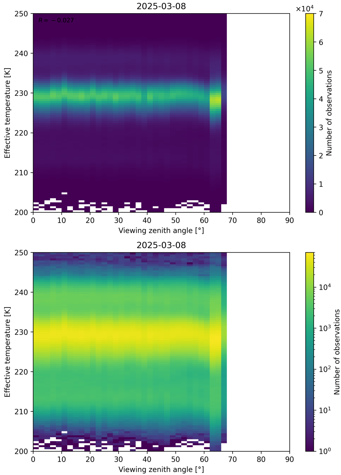
Figure 50: Scatter density plot of “Viewing zenith angle” against “Effective temperature” for 2025-03-07 to 2025-03-09.
