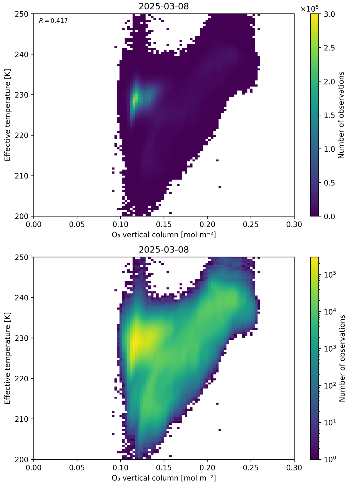
Figure 39: Scatter density plot of “O 3 vertical column” against “Effective temperature” for 2025-03-07 to 2025-03-09.
