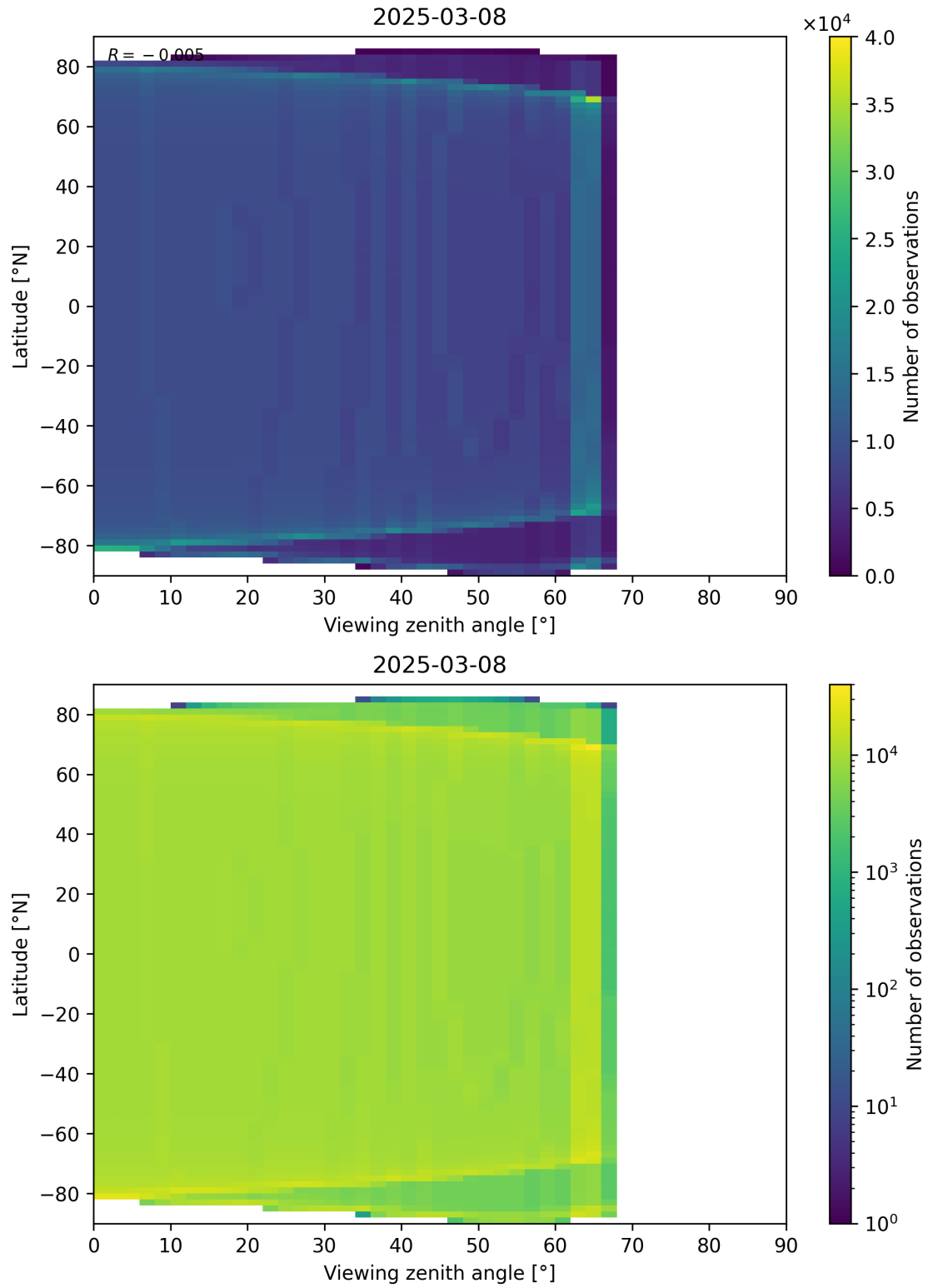
Figure 49: Scatter density plot of “Viewing zenith angle” against “Latitude” for 2025-03-07 to 2025-03-09.
