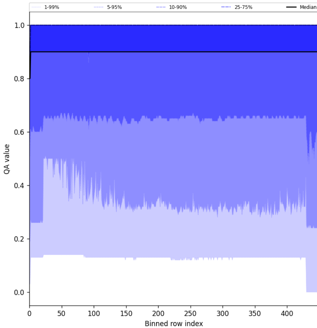
Figure 27: Along track statistics of “QA value” for 2025-03-07 to 2025-03-09
