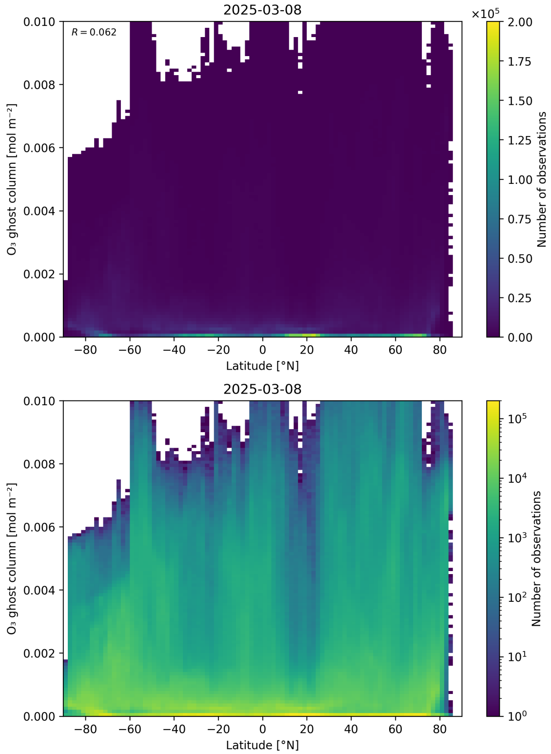
Figure 35: Scatter density plot of “Latitude” against “O 3 ghost column” for 2025-03-07 to 2025-03-09.
