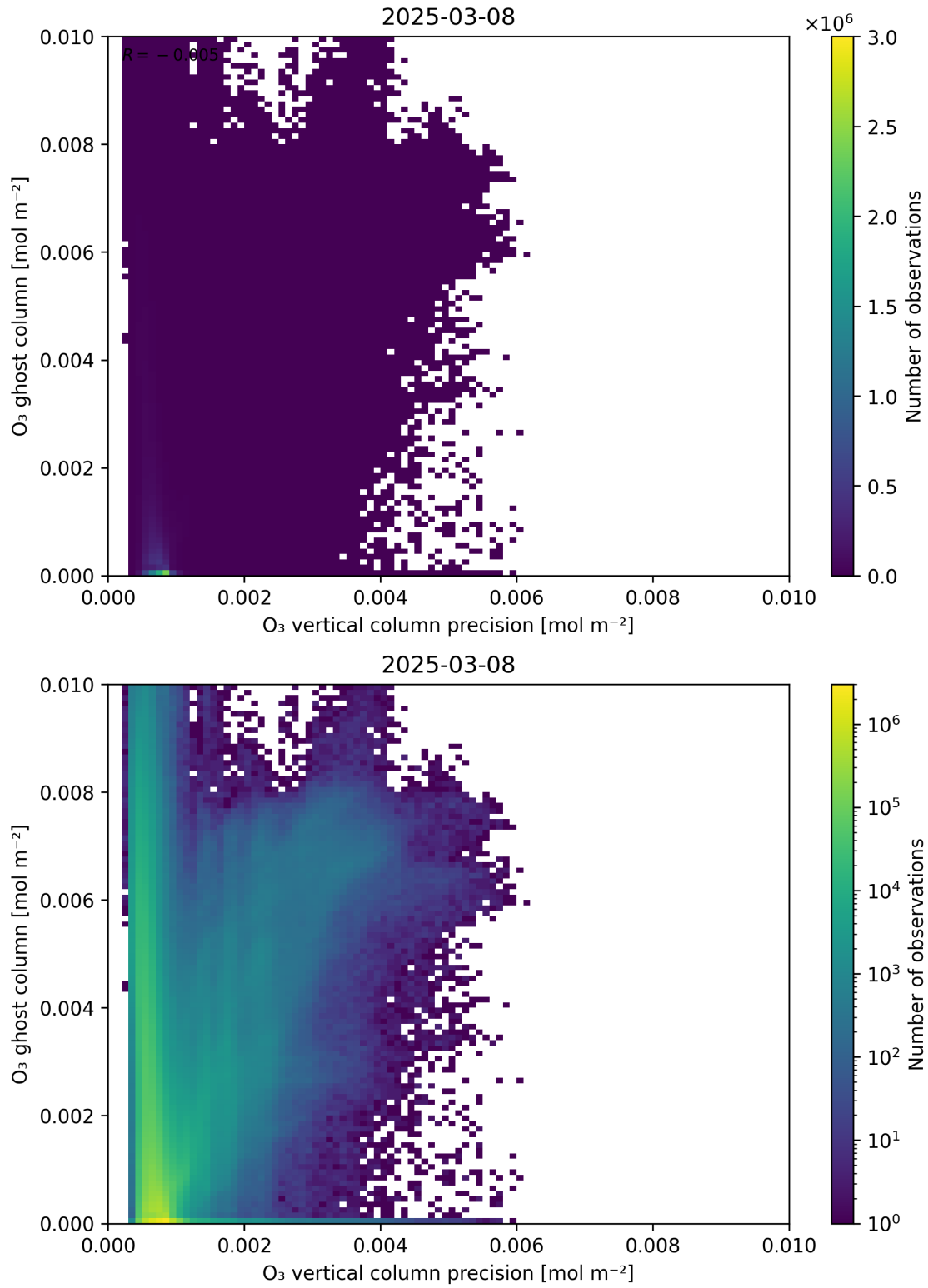
Figure 43: Scatter density plot of “ \text{O}_3 vertical column precision” against “ \text{O}_3 ghost column” for 2025-03-07 to 2025-03-09.
