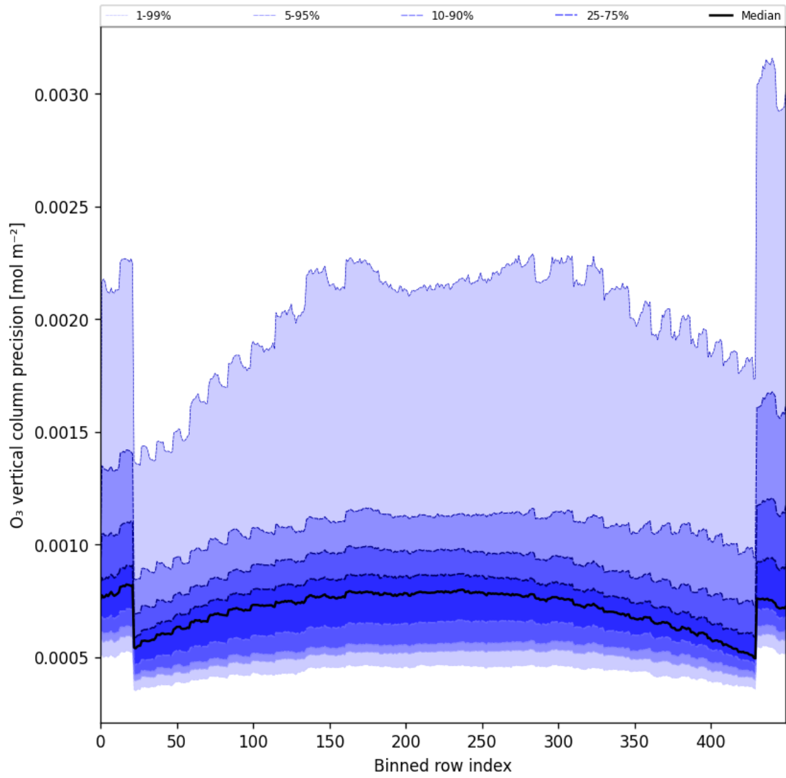
Figure 29: Along track statistics of “O 3 vertical column precision” for 2025-03-07 to 2025-03-09
