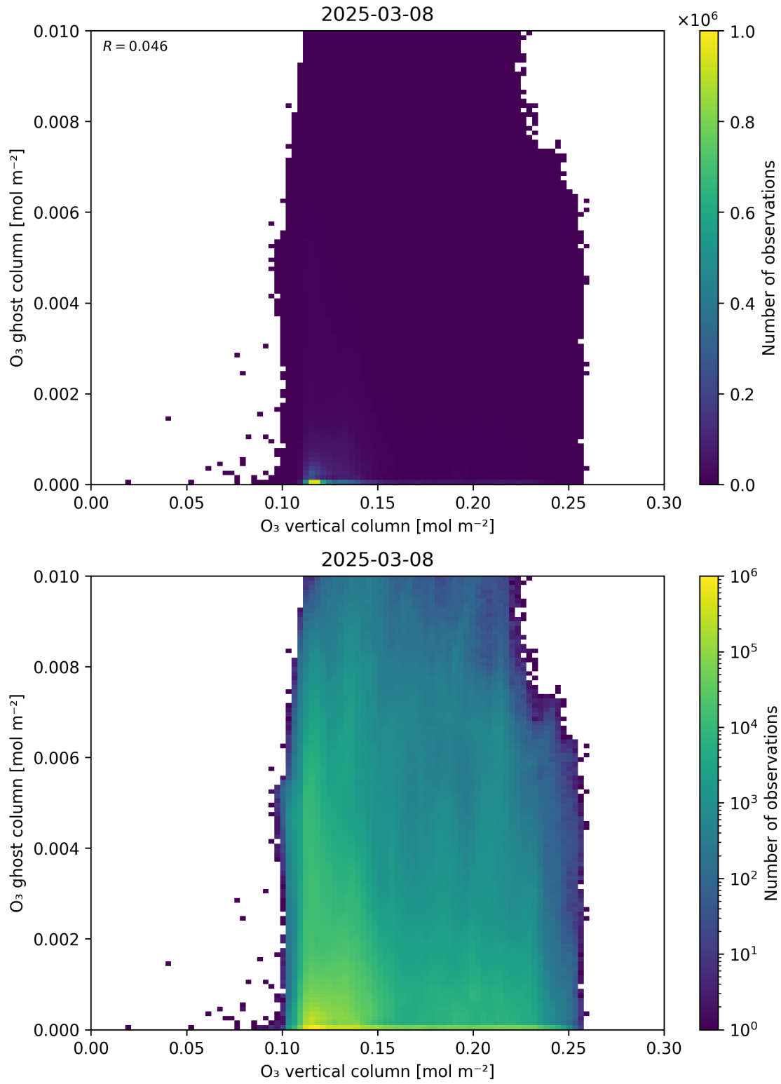
Figure 40: Scatter density plot of “O 3 vertical column” against “O 3 ghost column” for 2025-03-07 to 2025-03-09.
