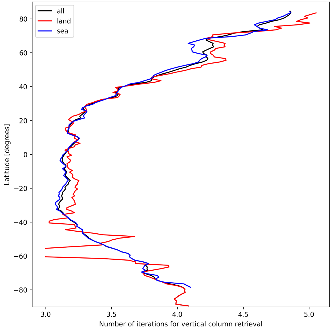
Figure 19: Zonal average of “Number of iterations for vertical column retrieval” for 2025-03-07 to 2025-03-09.
