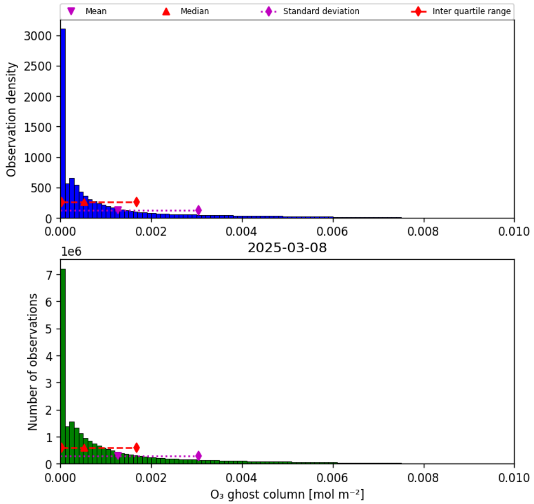
Figure 25: Histogram of “O 3 ghost column” for 2025-03-07 to 2025-03-09
