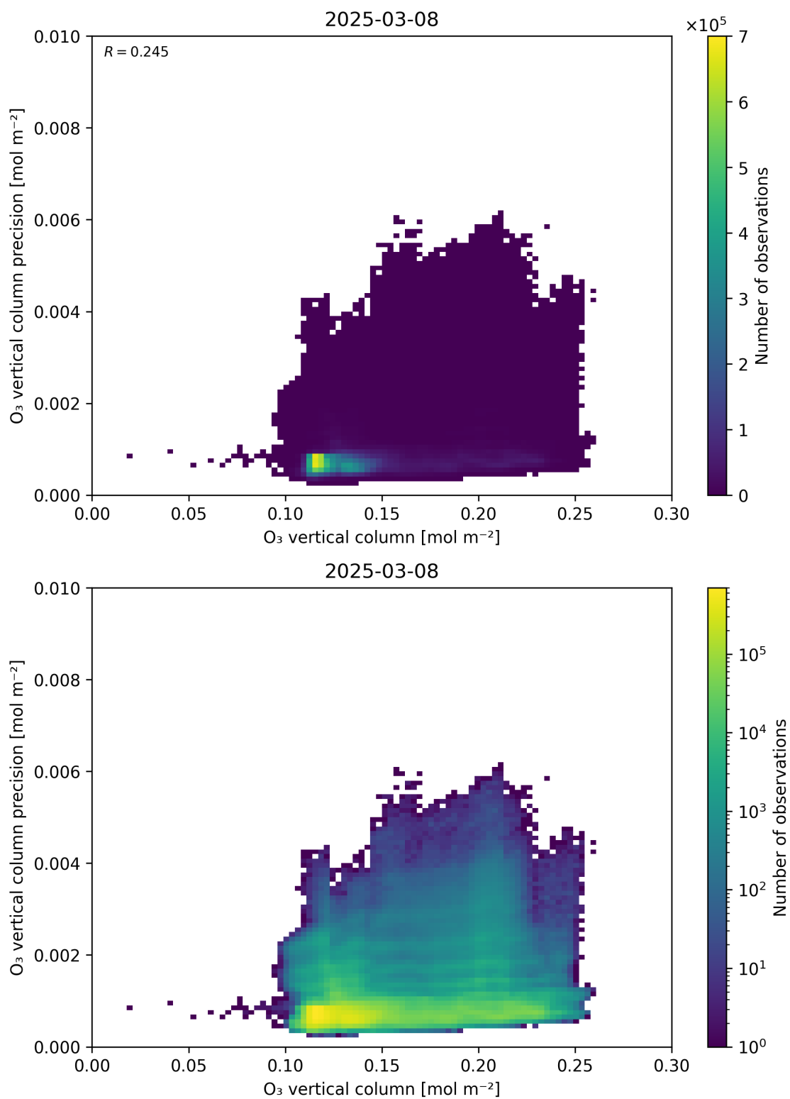
Figure 41: Scatter density plot of “O 3 vertical column” against “O 3 vertical column precision” for 2025-03-07 to 2025-03-09.
