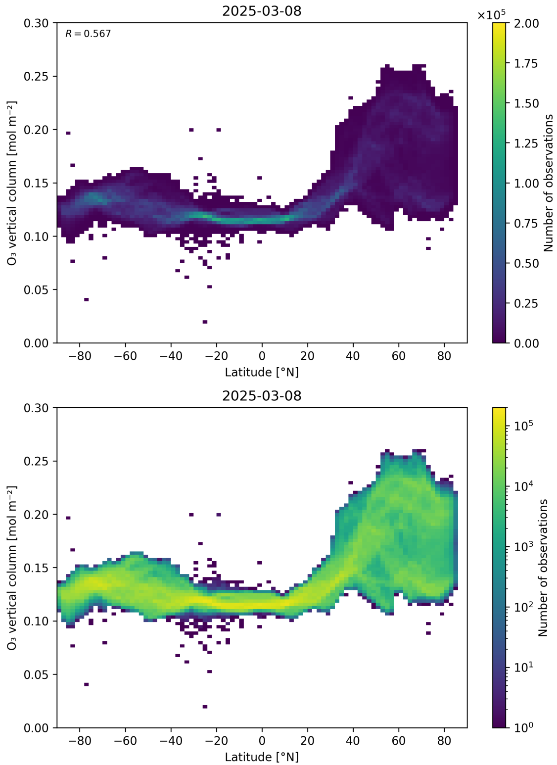
Figure 36: Scatter density plot of “Latitude” against “O 3 vertical column” for 2025-03-07 to 2025-03-09.
