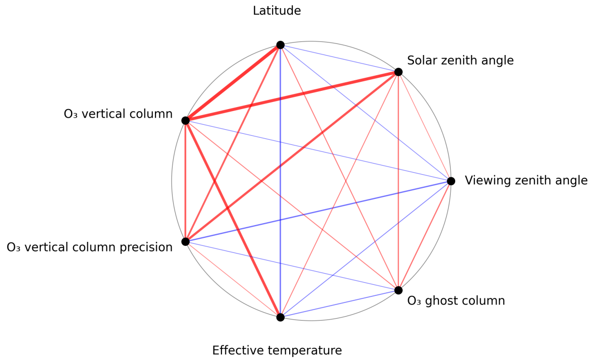
Figure 1: Map of correlation graph for 2025-03-07 to 2025-03-09.
