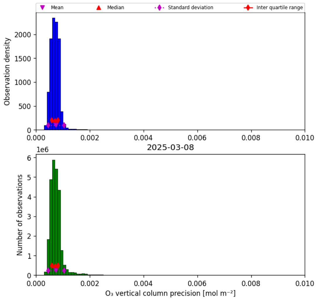
Figure 22: Histogram of “O 3 vertical column precision” for 2025-03-07 to 2025-03-09
