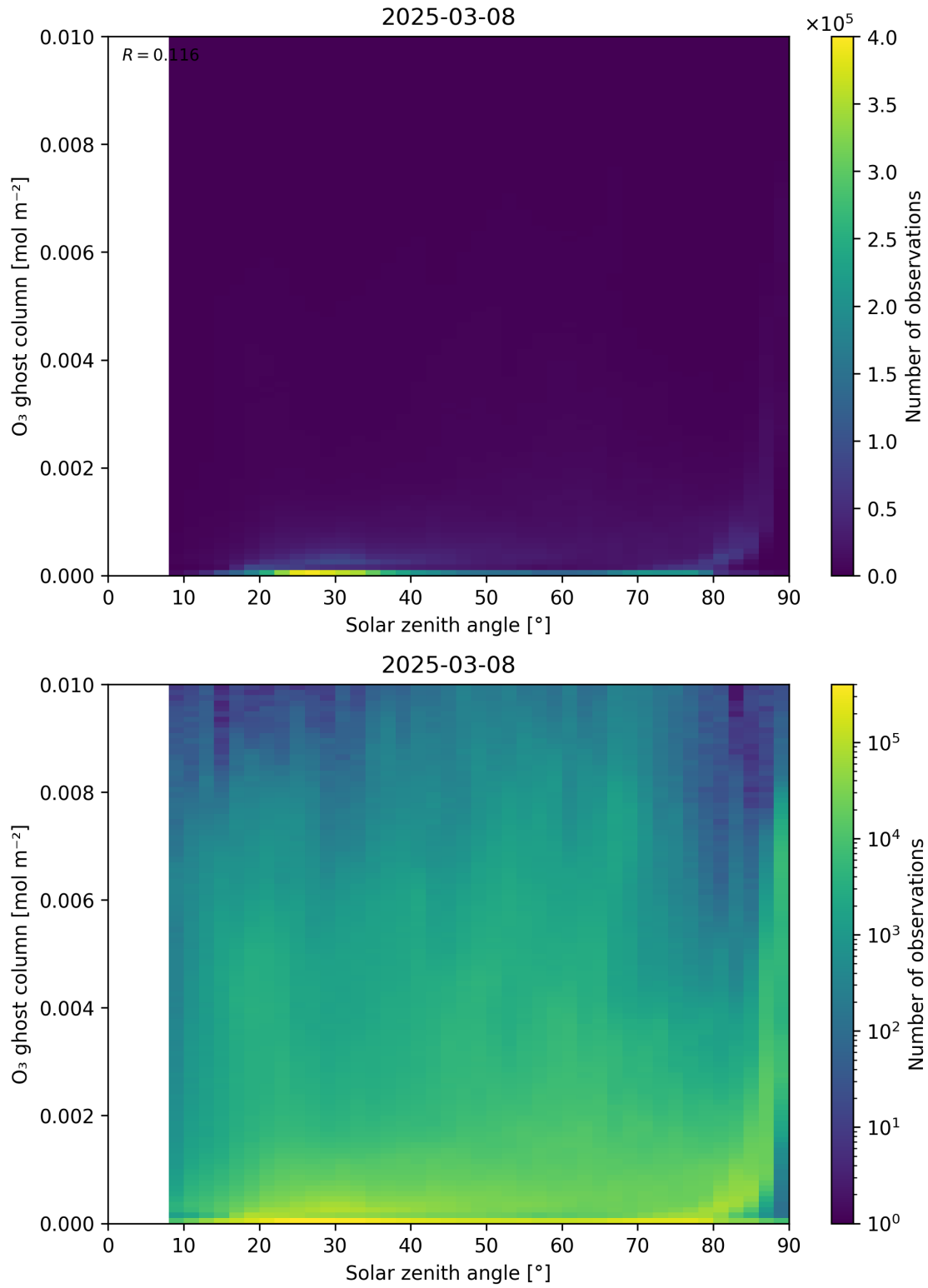
Figure 46: Scatter density plot of “Solar zenith angle” against “O 3 ghost column” for 2025-03-07 to 2025-03-09.
