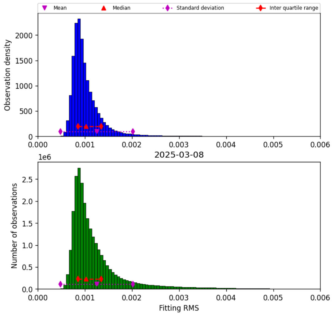
Figure 23: Histogram of “Fitting RMS” for 2025-03-07 to 2025-03-09
