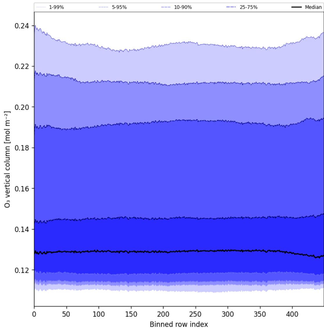
Figure 28: Along track statistics of “O 3 vertical column” for 2025-03-07 to 2025-03-09
