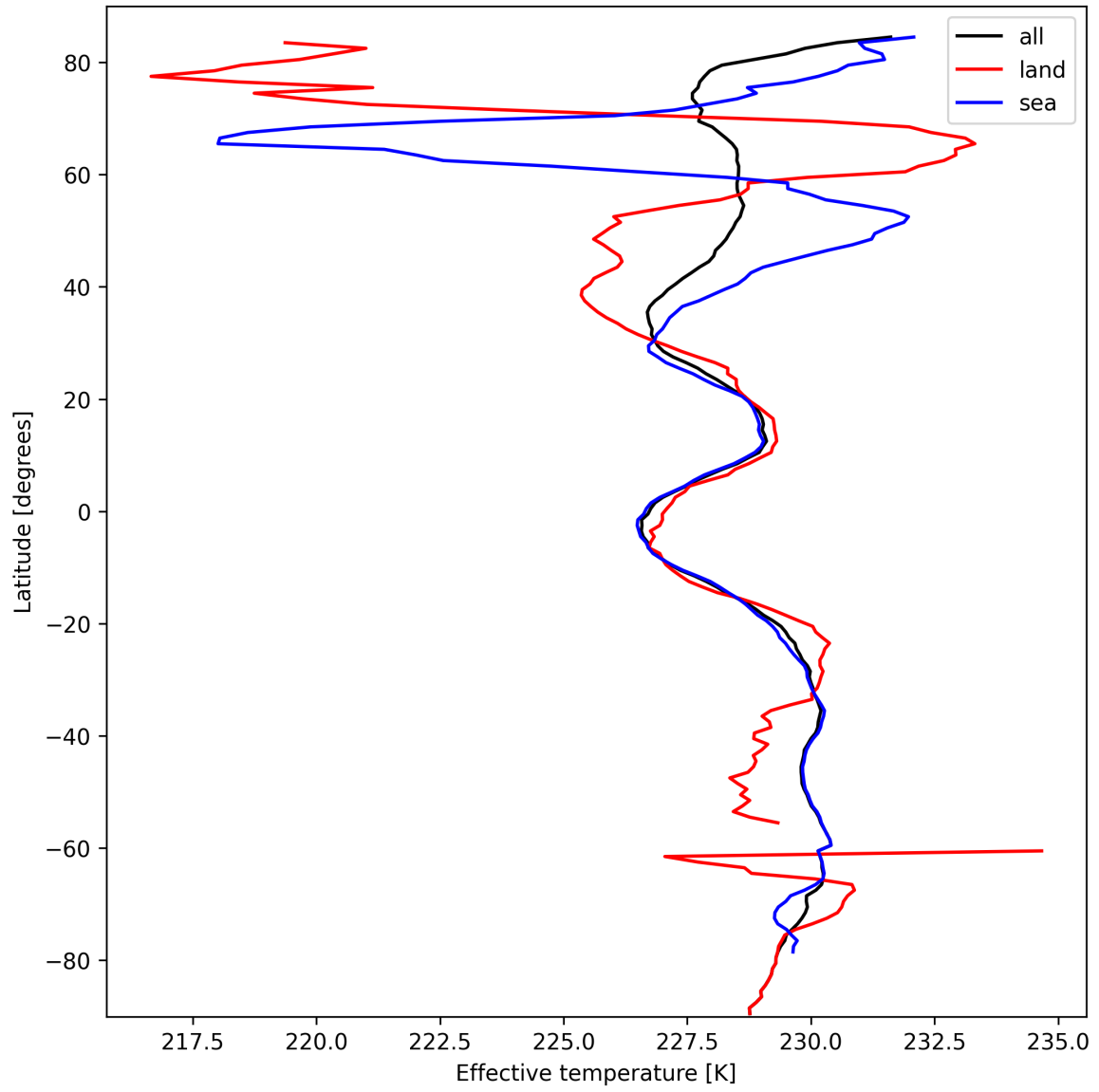
Figure 17: Zonal average of “Effective temperature” for 2025-03-07 to 2025-03-09.
