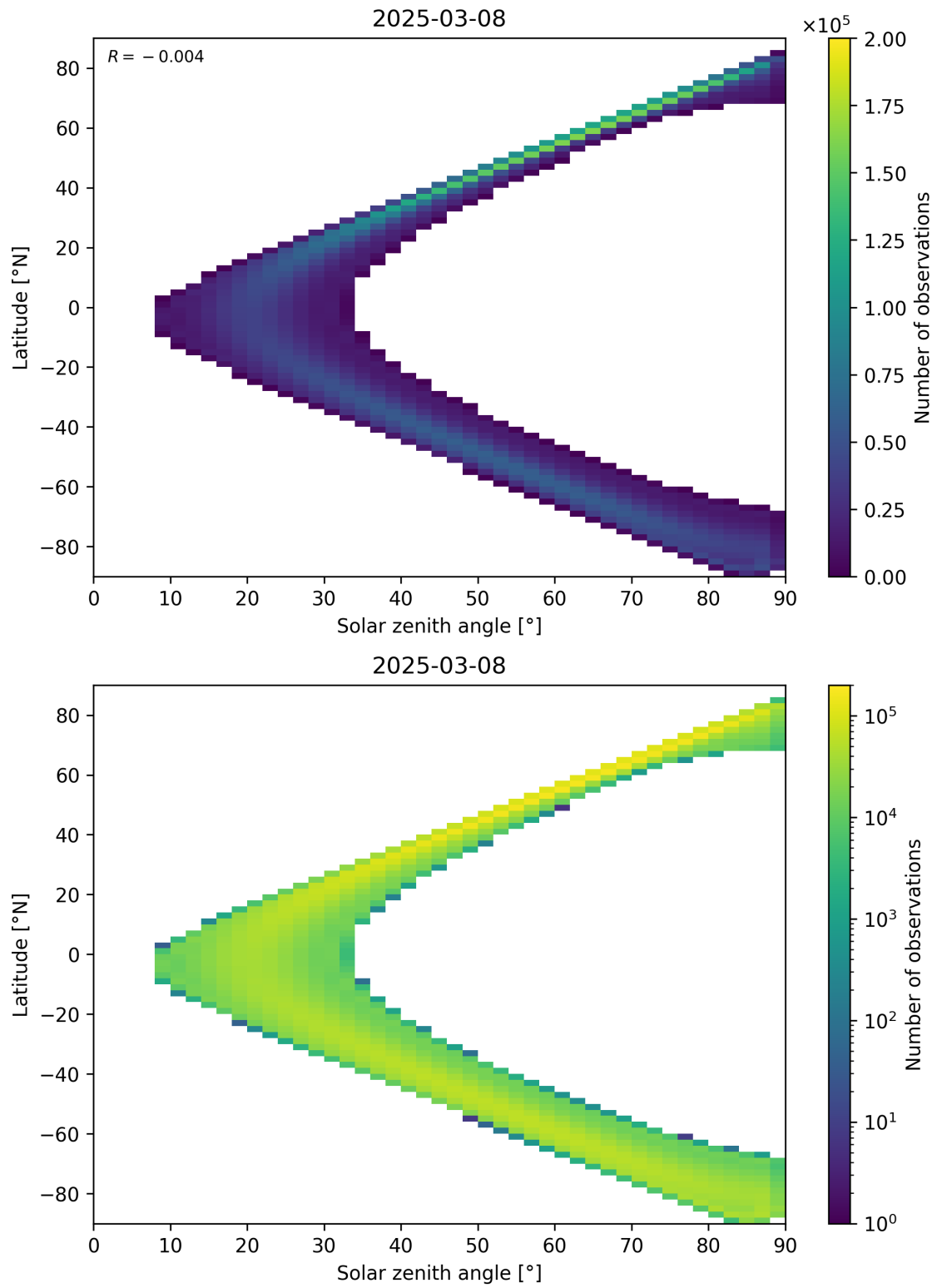
Figure 44: Scatter density plot of “Solar zenith angle” against “Latitude” for 2025-03-07 to 2025-03-09.
