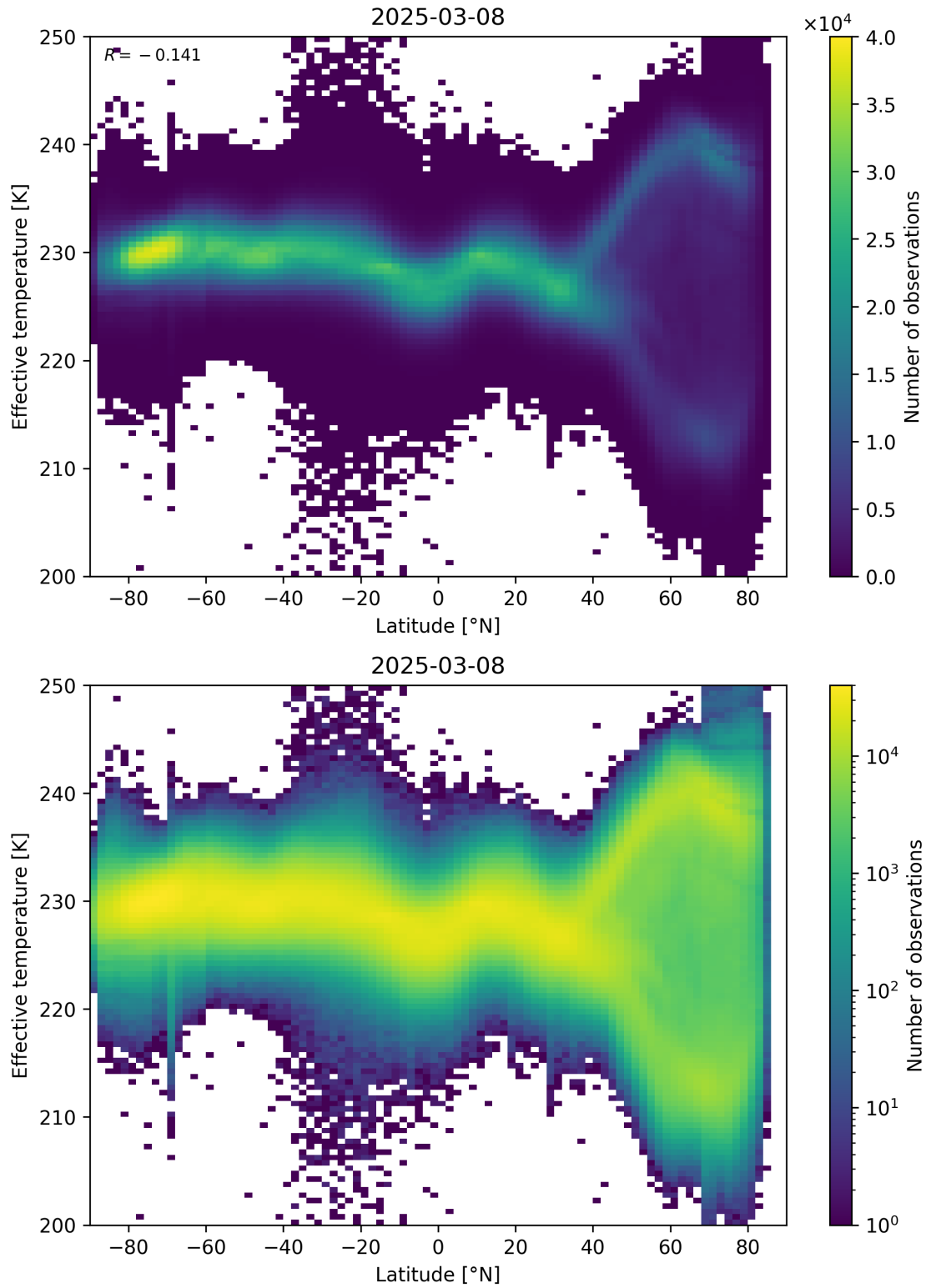
Figure 34: Scatter density plot of “Latitude” against “Effective temperature” for 2025-03-07 to 2025-03-09.
