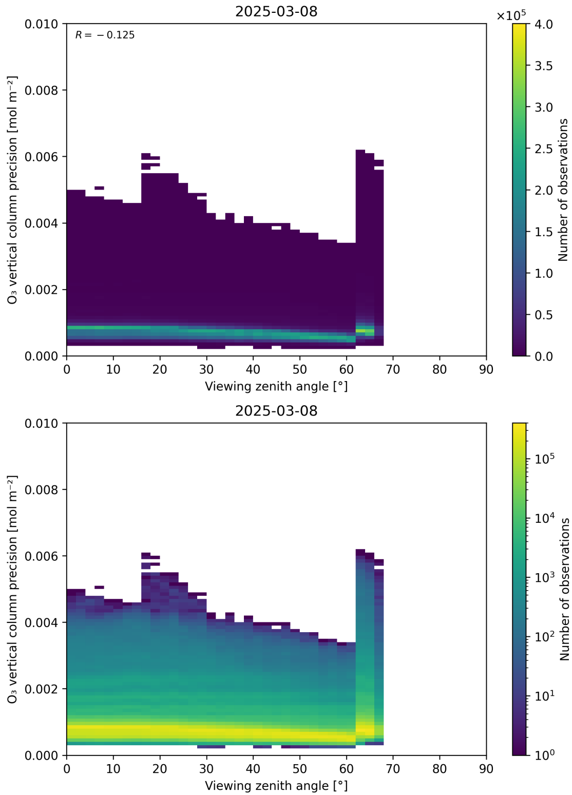
Figure 53: Scatter density plot of “Viewing zenith angle” against “O 3 vertical column precision” for 2025-03-07 to 2025-03-09.
