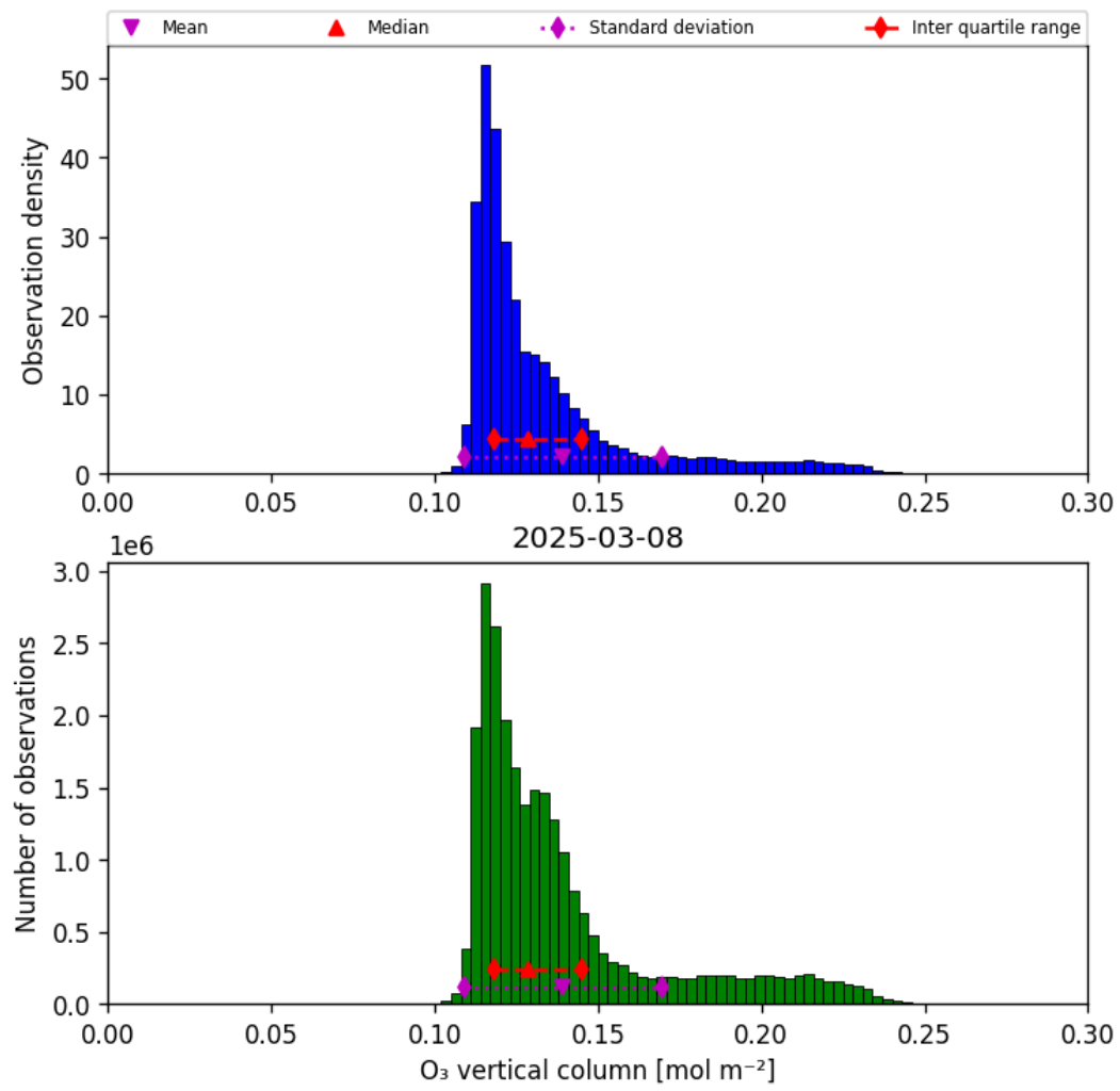
Figure 21: Histogram of “O 3 vertical column” for 2025-03-07 to 2025-03-09
