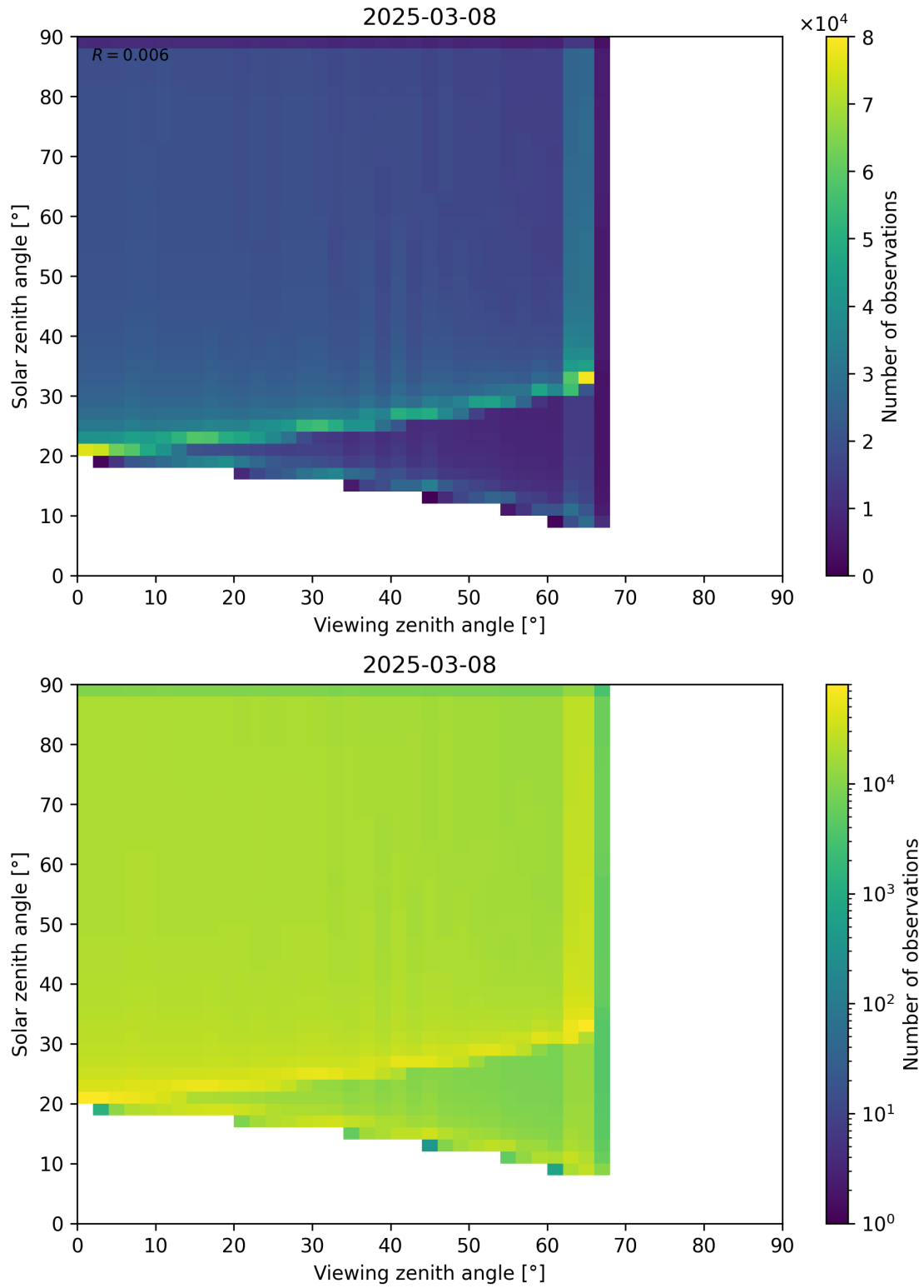
Figure 54: Scatter density plot of “Viewing zenith angle” against “Solar zenith angle” for 2025-03-07 to 2025-03-09.
