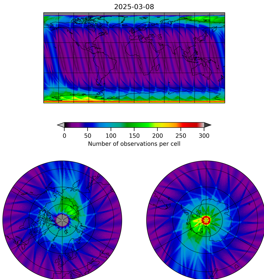
Figure 12: Map of the number of observations for 2025-03-07 to 2025-03-09
