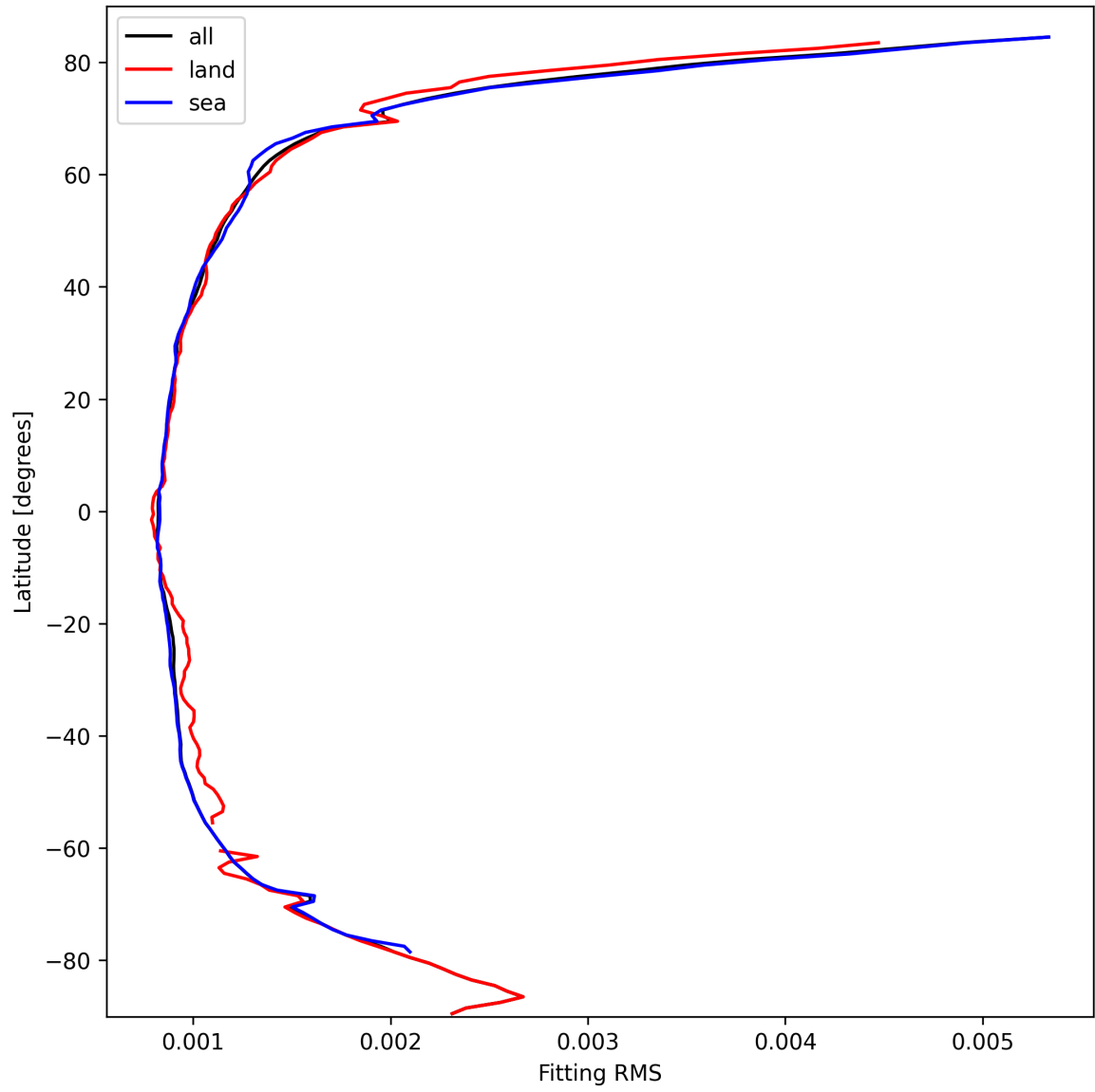
Figure 16: Zonal average of “Fitting RMS” for 2025-03-07 to 2025-03-09.
