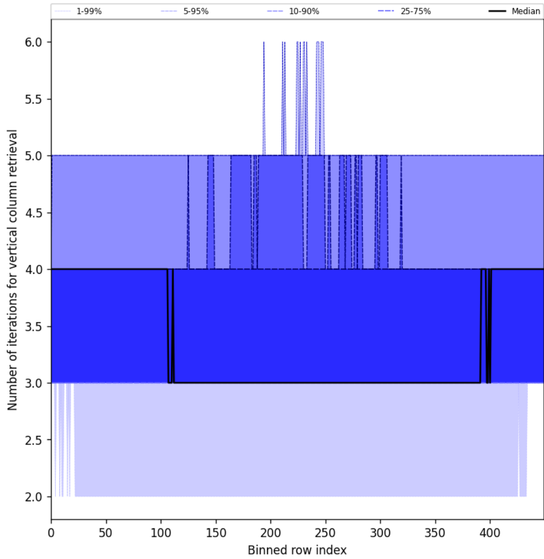
Figure 33: Along track statistics of “Number of iterations for vertical column retrieval” for 2025-03-08 to 2025-03-10
