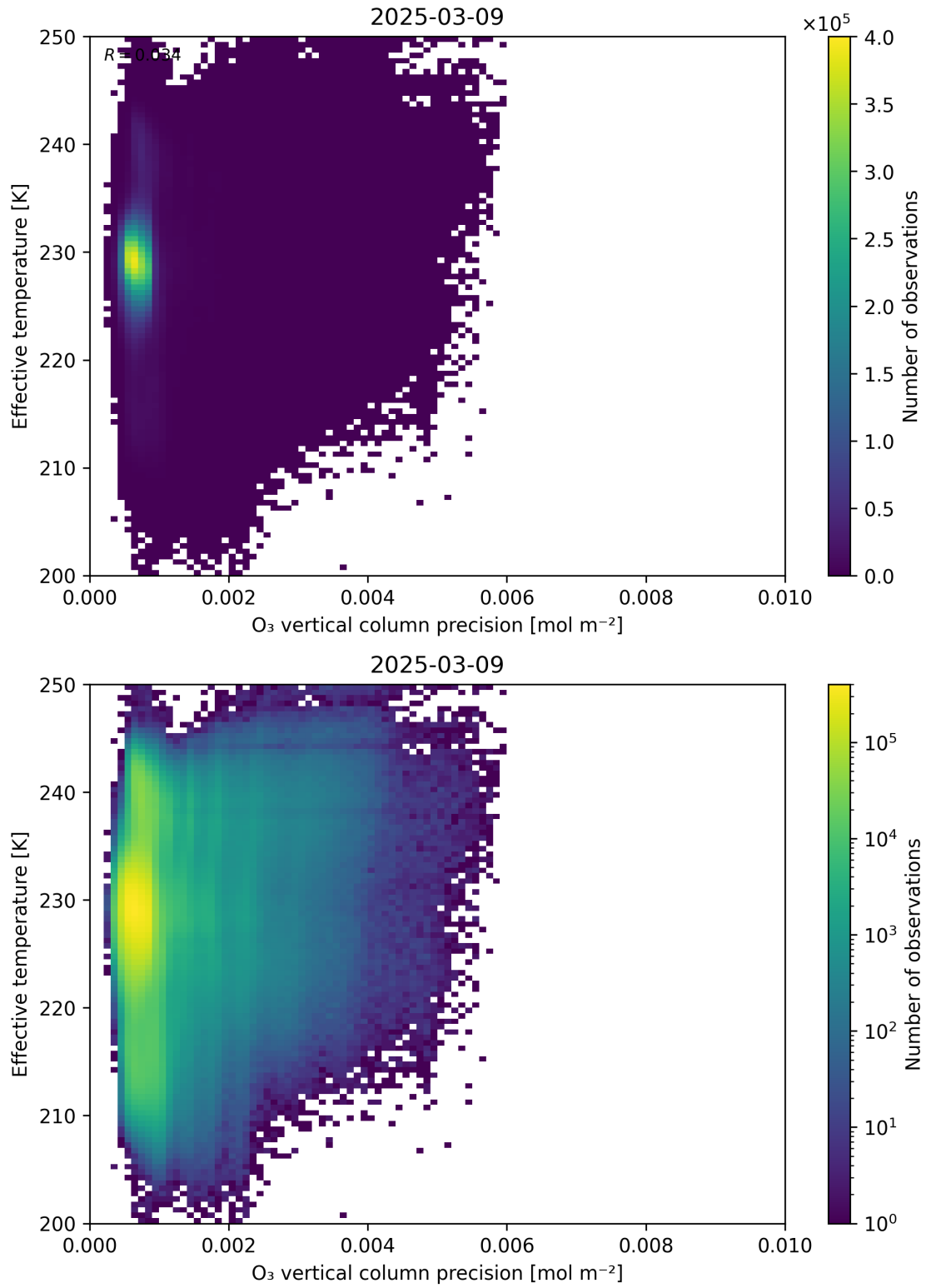
Figure 42: Scatter density plot of “O 3 vertical column precision” against “Effective temperature” for 2025-03-08 to 2025-03-10.
