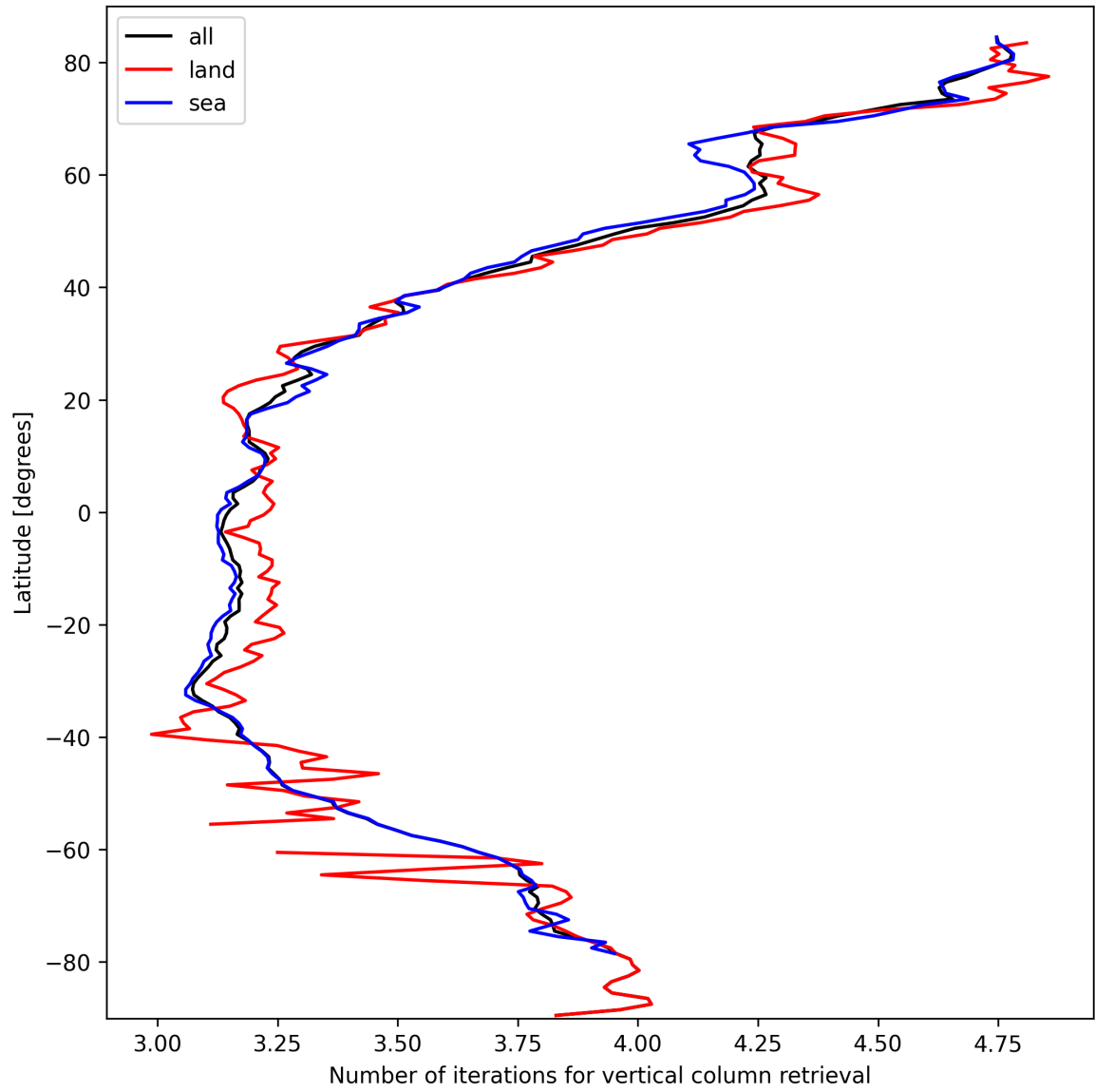
Figure 19: Zonal average of “Number of iterations for vertical column retrieval” for 2025-03-08 to 2025-03-10.
