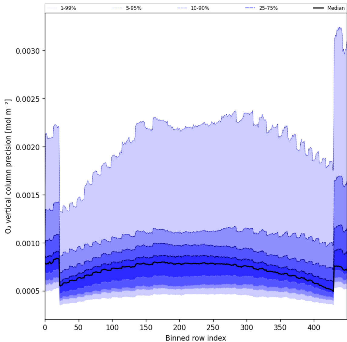
Figure 29: Along track statistics of “O 3 vertical column precision” for 2025-03-08 to 2025-03-10
