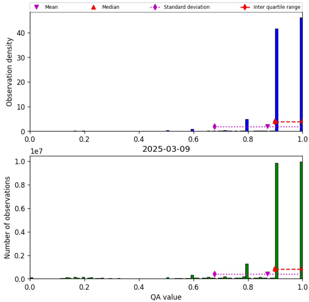
Figure 20: Histogram of “QA value” for 2025-03-08 to 2025-03-10
