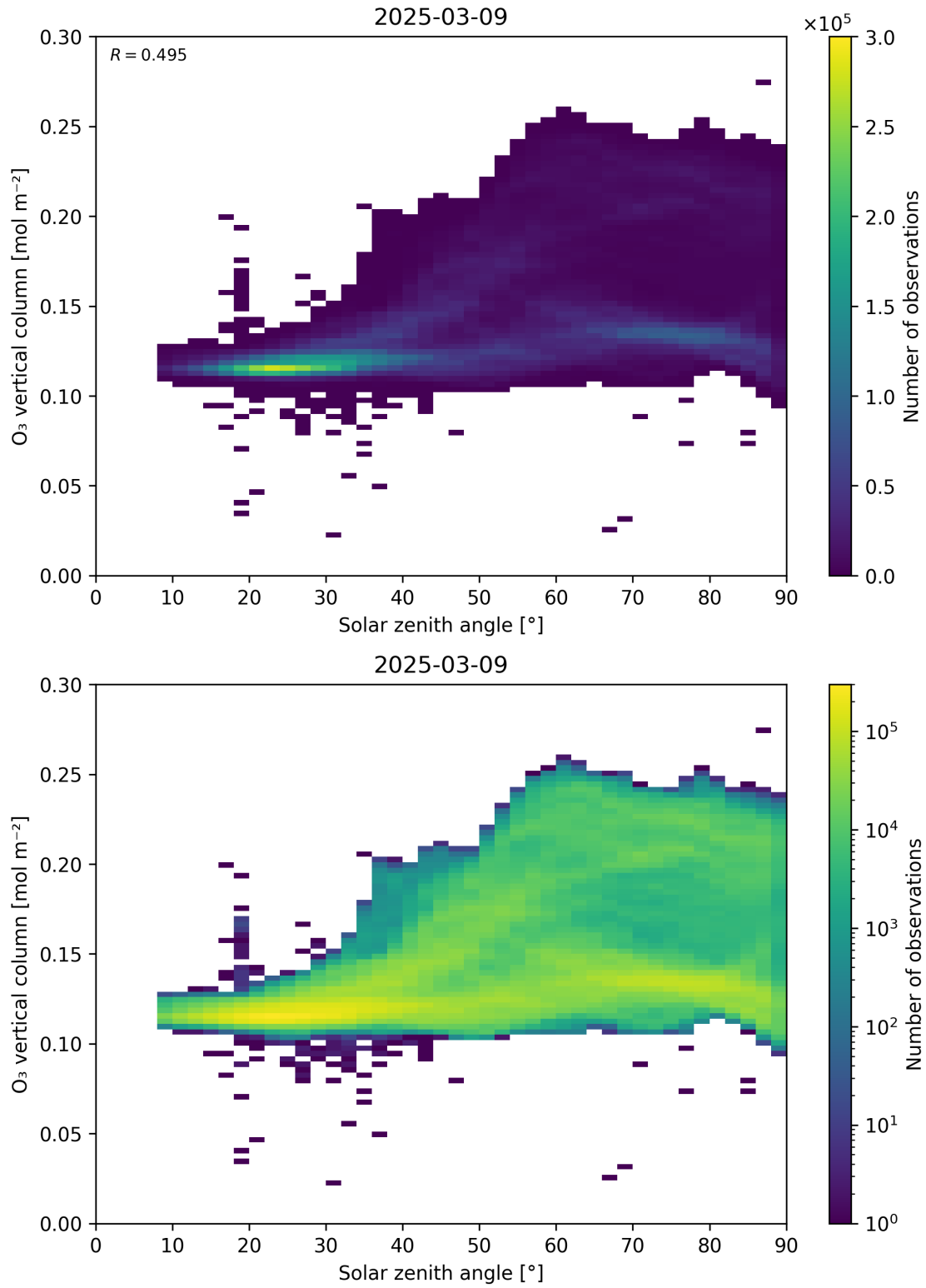
Figure 47: Scatter density plot of “Solar zenith angle” against “O 3 vertical column” for 2025-03-08 to 2025-03-10.
