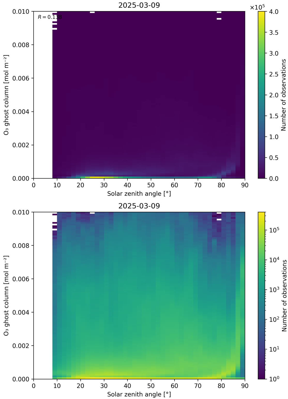
Figure 46: Scatter density plot of “Solar zenith angle” against “O 3 ghost column” for 2025-03-08 to 2025-03-10.
