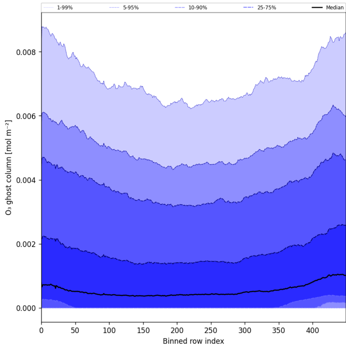
Figure 32: Along track statistics of “O 3 ghost column” for 2025-03-08 to 2025-03-10
