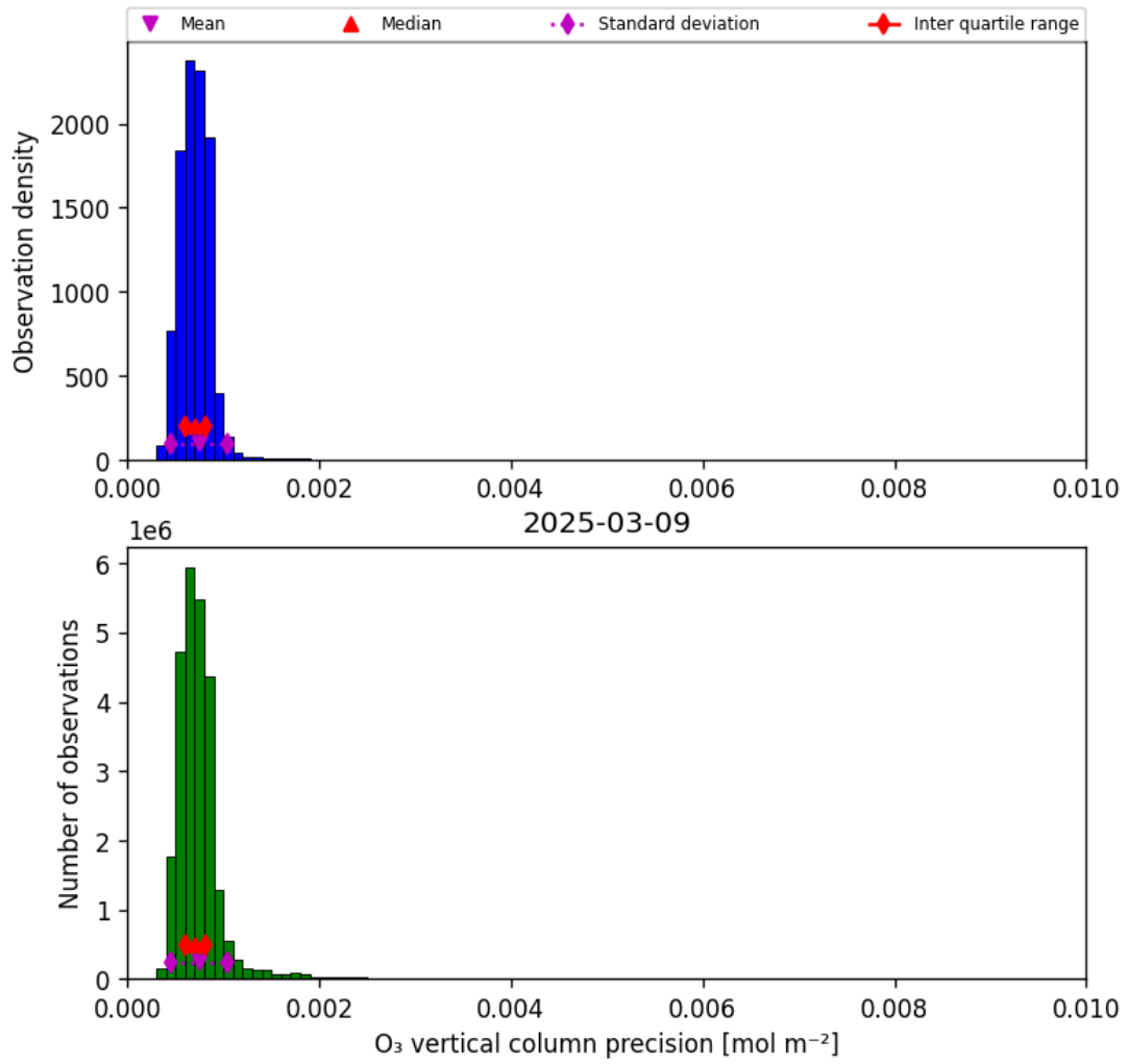
Figure 22: Histogram of “O 3 vertical column precision” for 2025-03-08 to 2025-03-10
