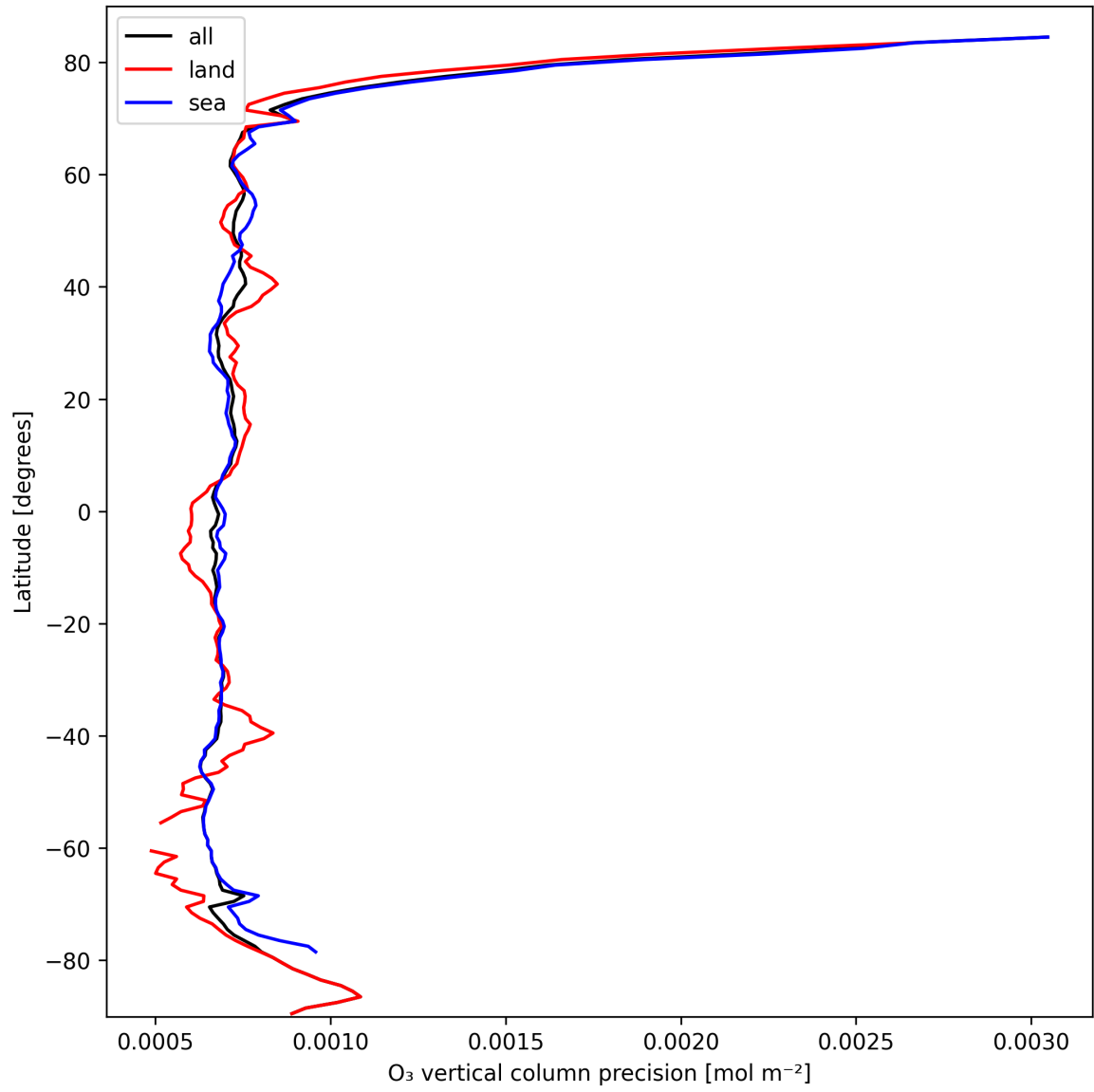
Figure 15: Zonal average of “O 3 vertical column precision” for 2025-03-08 to 2025-03-10.
