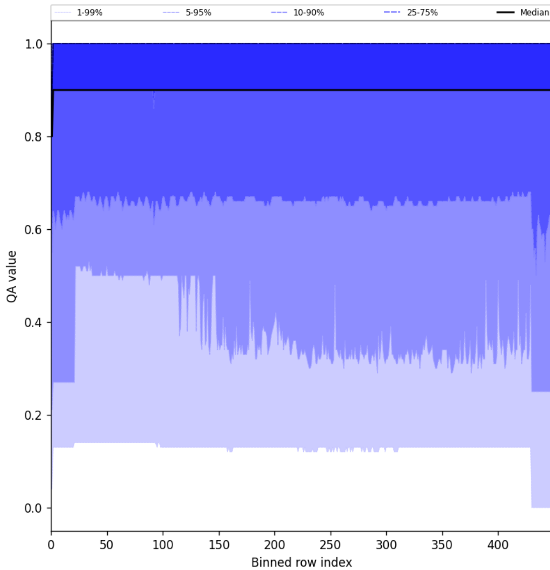
Figure 27: Along track statistics of “QA value” for 2025-03-08 to 2025-03-10
