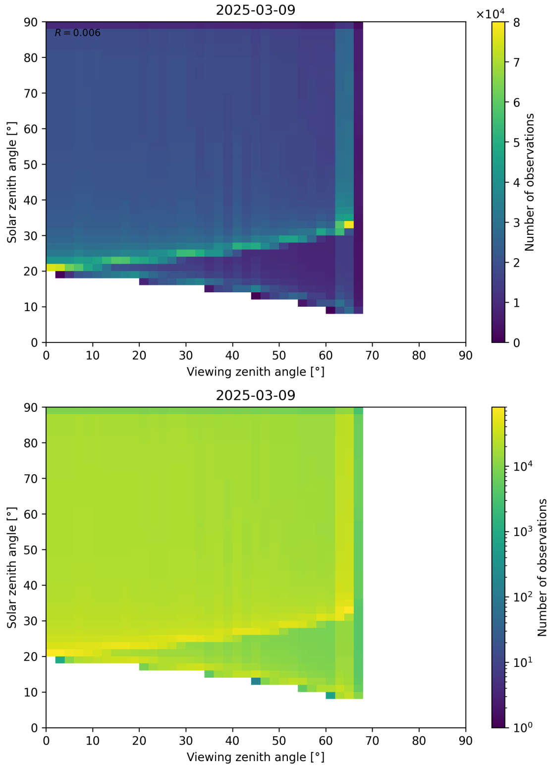
Figure 54: Scatter density plot of “Viewing zenith angle” against “Solar zenith angle” for 2025-03-08 to 2025-03-10.
