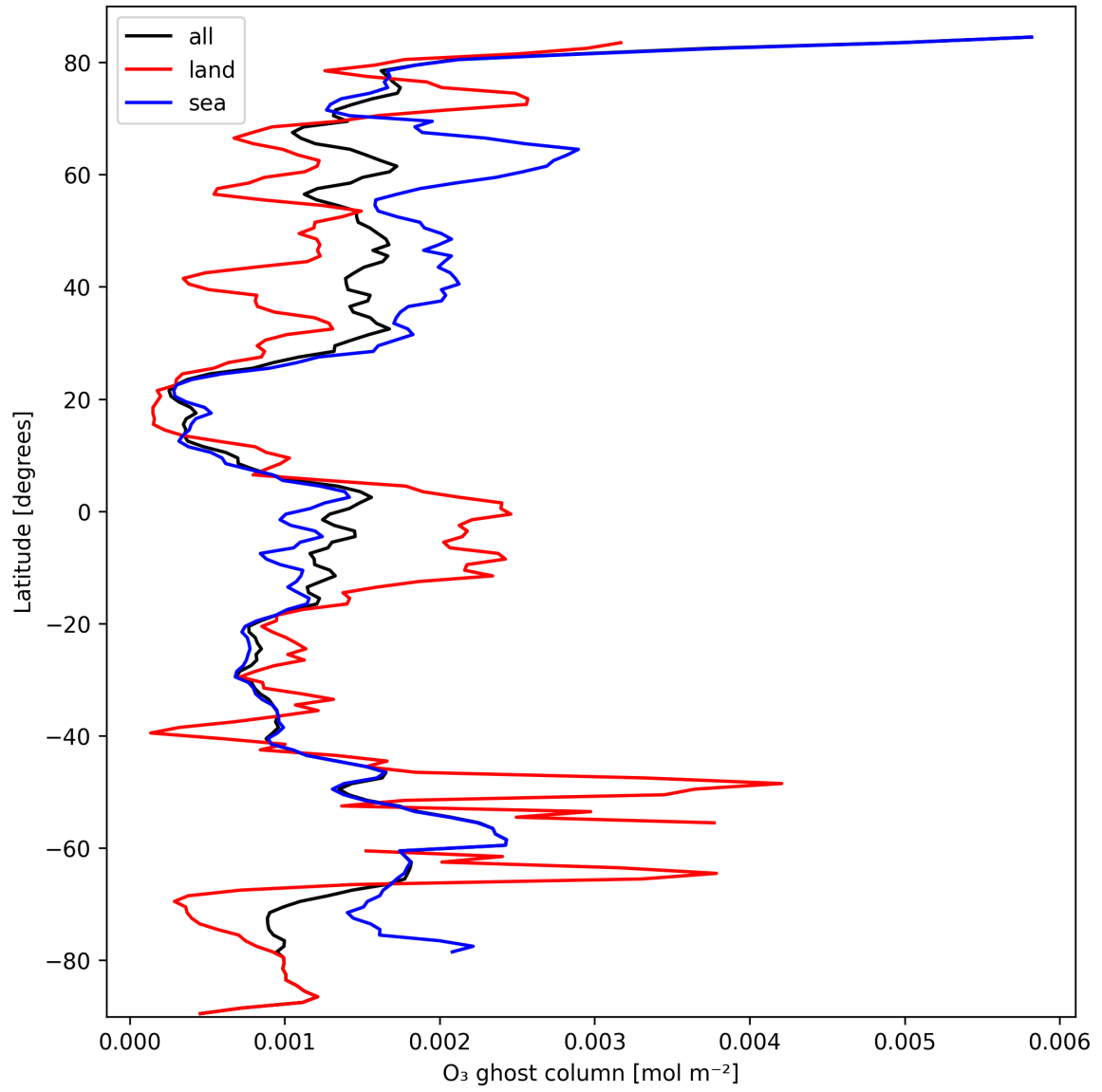
Figure 18: Zonal average of “O 3 ghost column” for 2025-03-08 to 2025-03-10.
