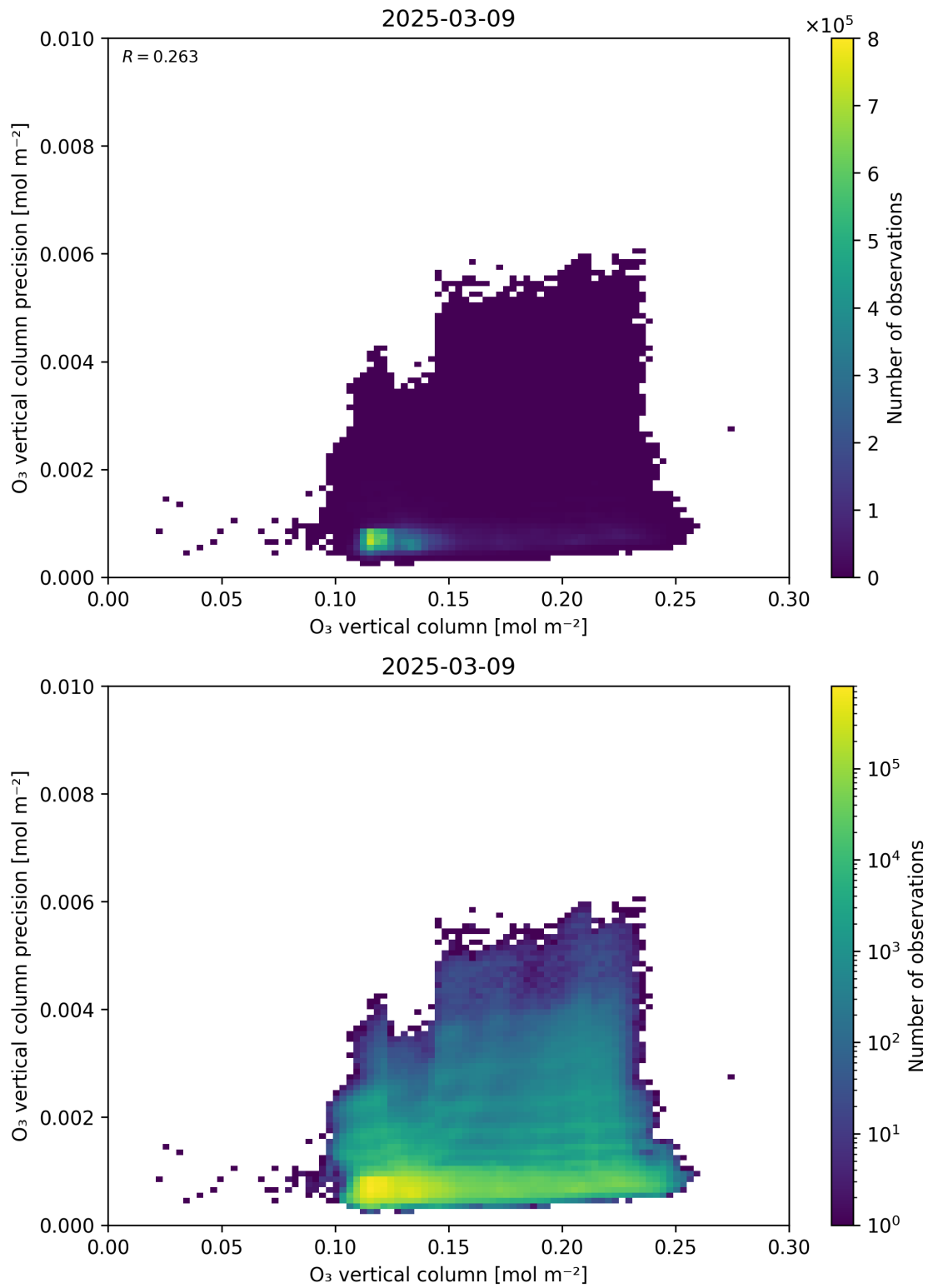
Figure 41: Scatter density plot of “O 3 vertical column” against “O 3 vertical column precision” for 2025-03-08 to 2025-03-10.
