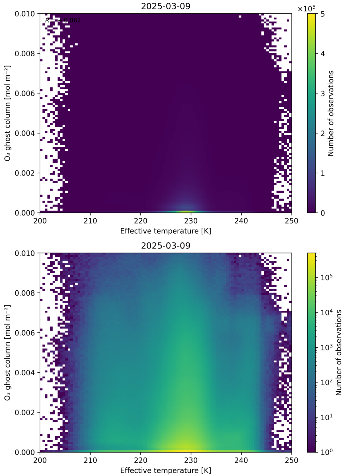
Figure 38: Scatter density plot of “Effective temperature” against “O 3 ghost column” for 2025-03-08 to 2025-03-10.
