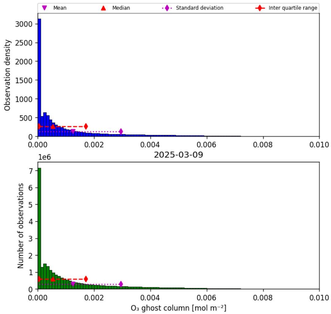
Figure 25: Histogram of “O 3 ghost column” for 2025-03-08 to 2025-03-10
