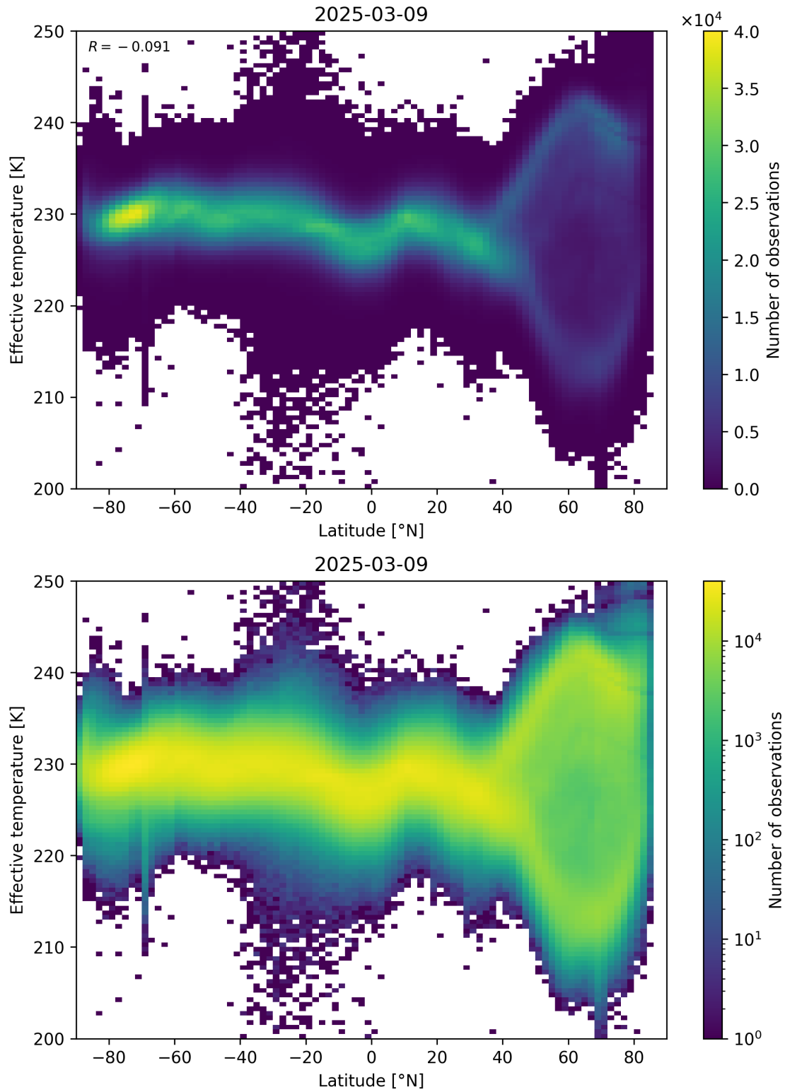
Figure 34: Scatter density plot of “Latitude” against “Effective temperature” for 2025-03-08 to 2025-03-10.
