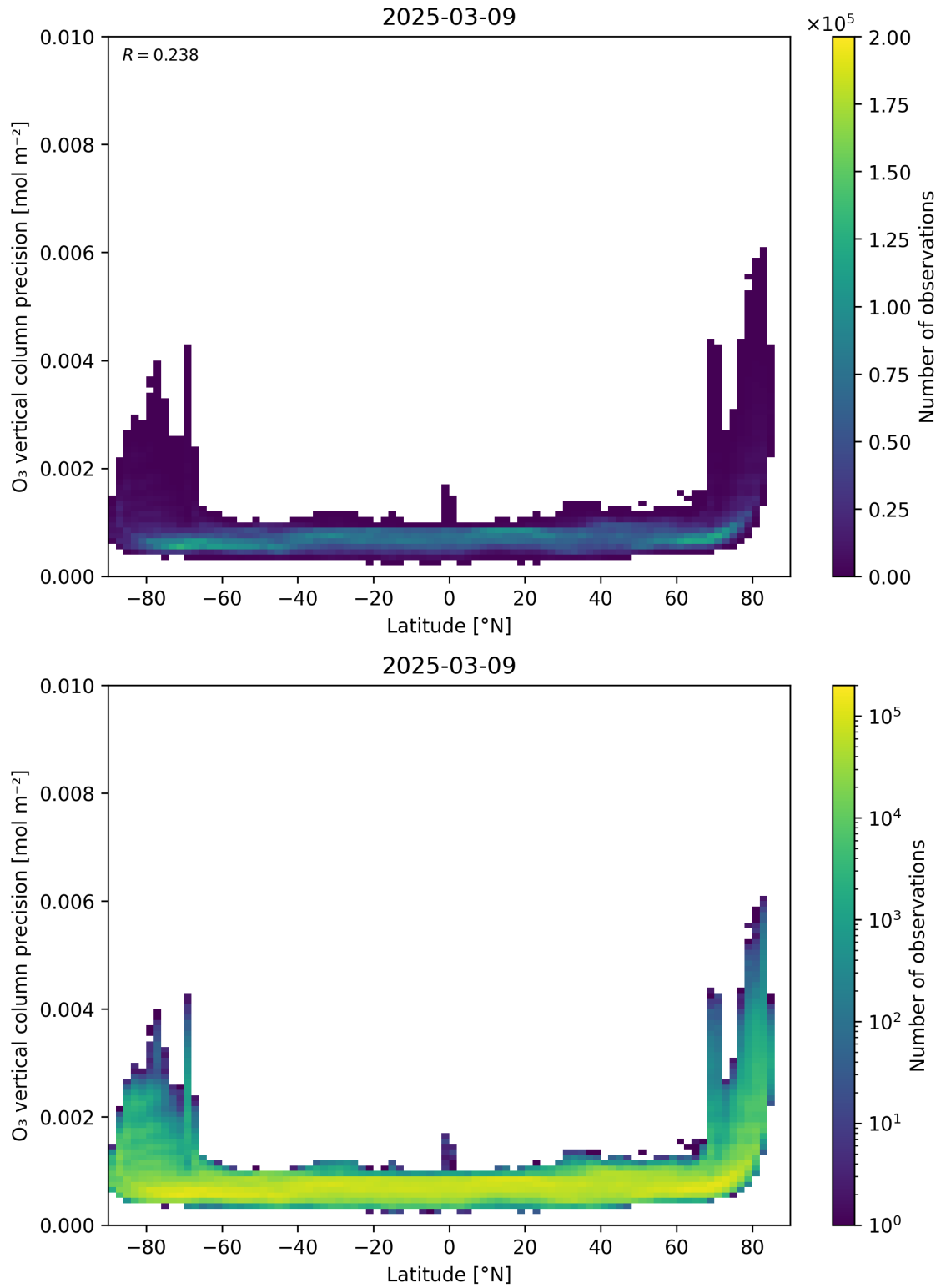
Figure 37: Scatter density plot of “Latitude” against “O 3 vertical column precision” for 2025-03-08 to 2025-03-10.
