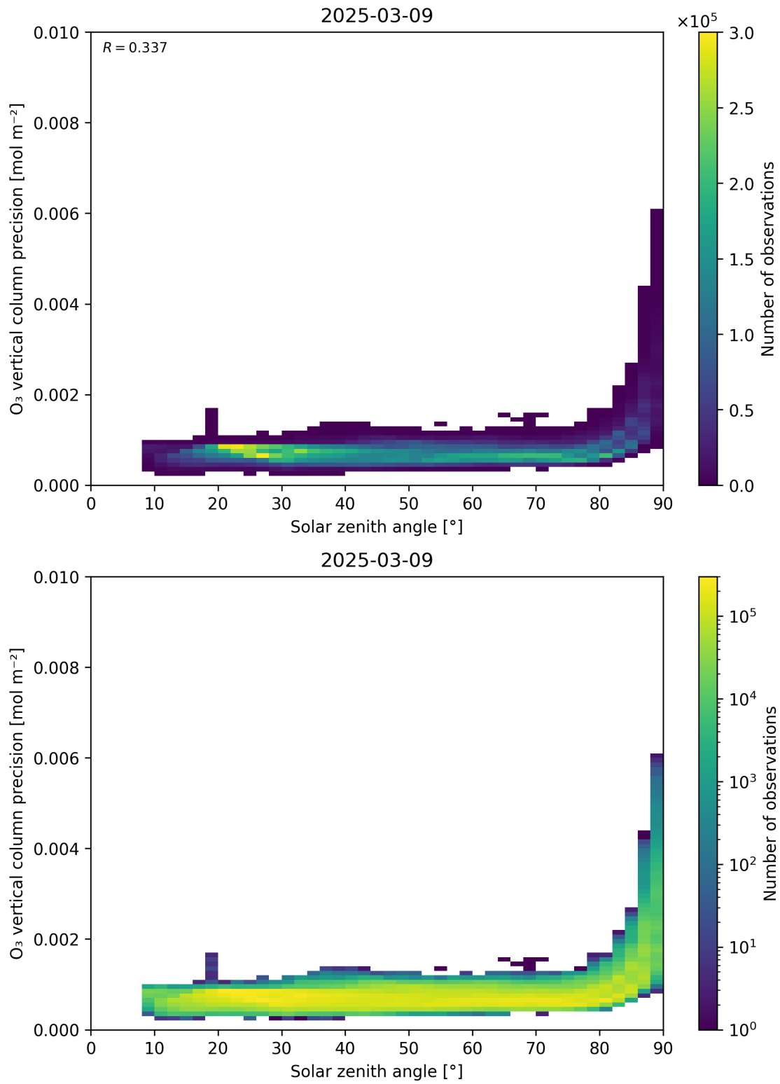
Figure 48: Scatter density plot of “Solar zenith angle” against “O 3 vertical column precision” for 2025-03-08 to 2025-03-10.
