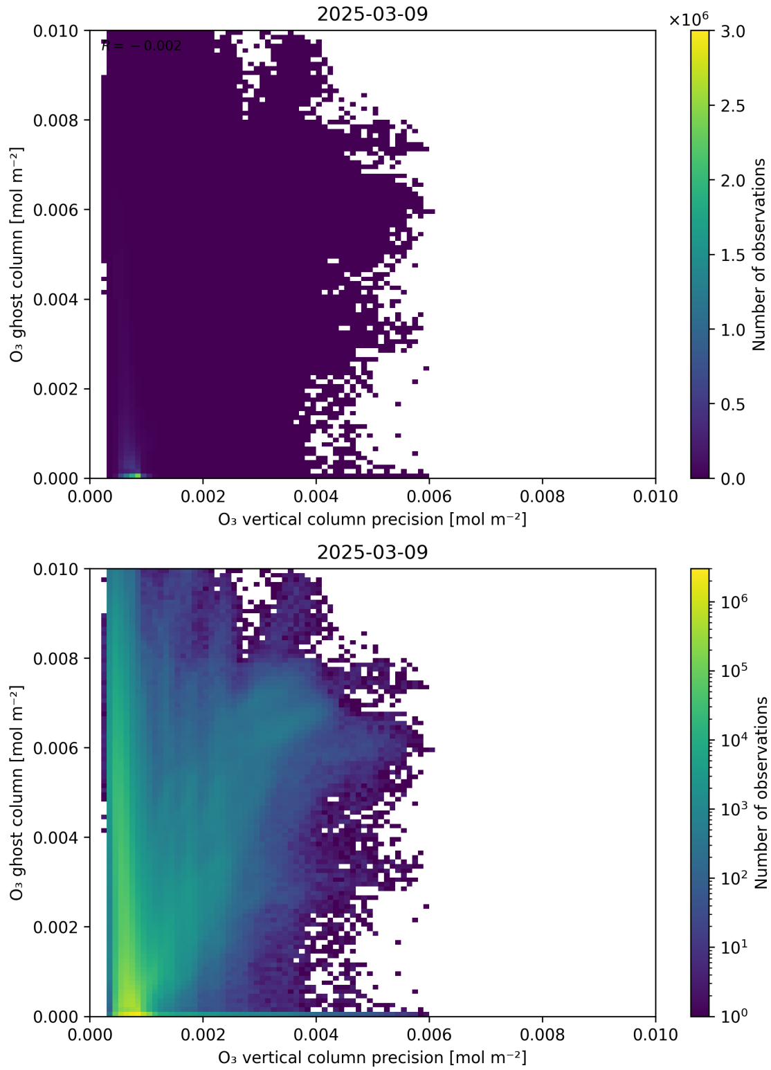
Figure 43: Scatter density plot of “O 3 vertical column precision” against “O 3 ghost column” for 2025-03-08 to 2025-03-10.
