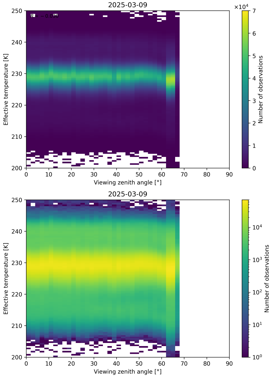
Figure 50: Scatter density plot of “Viewing zenith angle” against “Effective temperature” for 2025-03-08 to 2025-03-10.
