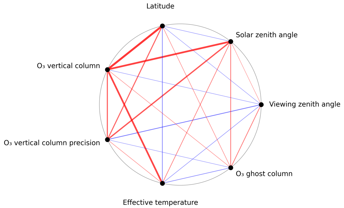
Figure 1: Map of correlation graph for 2025-03-08 to 2025-03-10.
