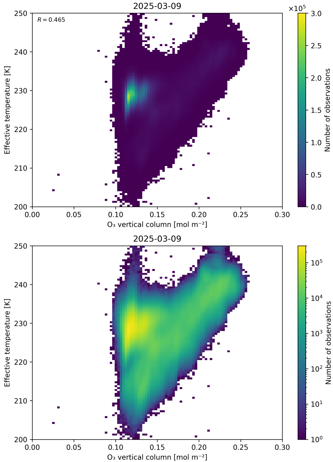
Figure 39: Scatter density plot of “O 3 vertical column” against “Effective temperature” for 2025-03-08 to 2025-03-10.
