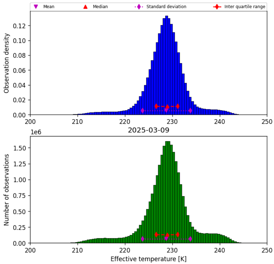
Figure 24: Histogram of “Effective temperature” for 2025-03-08 to 2025-03-10
