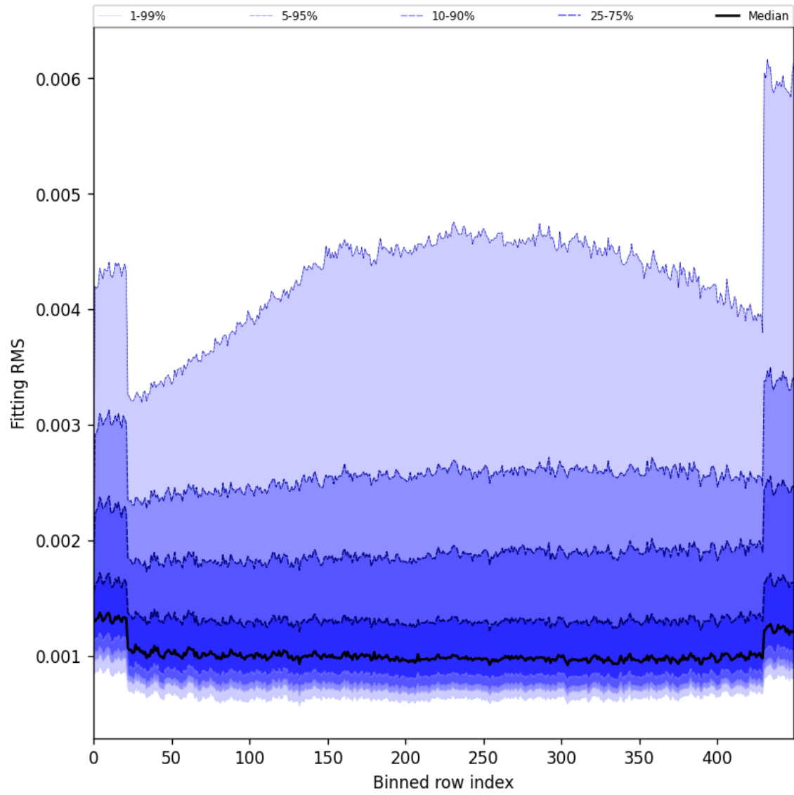
Figure 30: Along track statistics of “Fitting RMS” for 2025-03-08 to 2025-03-10
