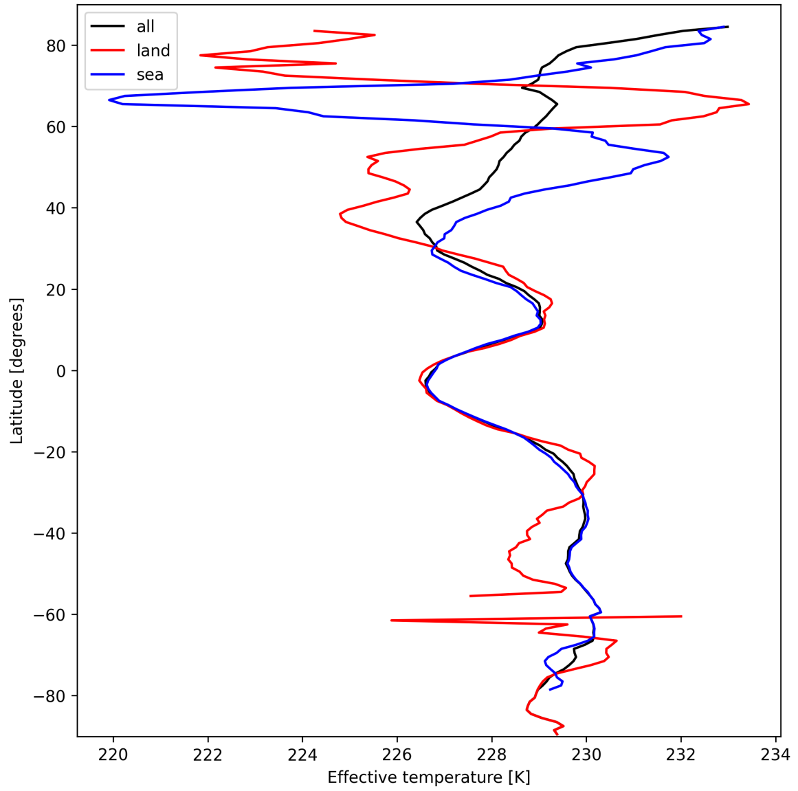
Figure 17: Zonal average of "Effective temperature" for 2025-03-08 to 2025-03-10.
