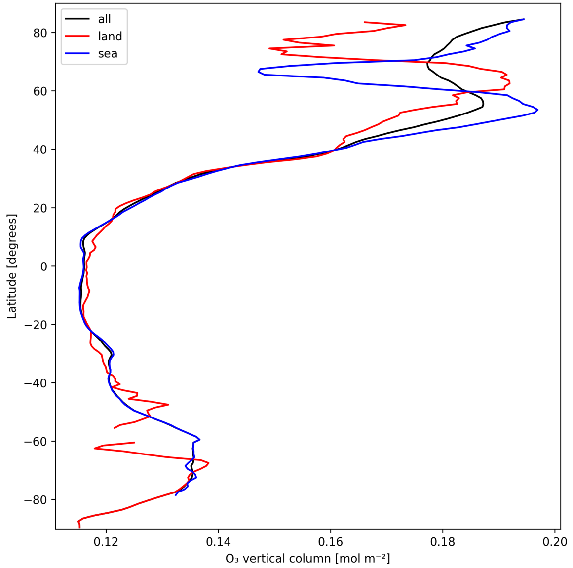
Figure 14: Zonal average of “O 3 vertical column” for 2025-03-08 to 2025-03-10.
