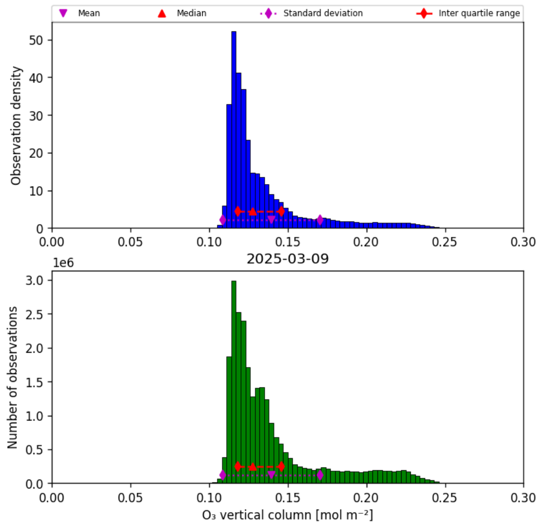
Figure 21: Histogram of “O 3 vertical column” for 2025-03-08 to 2025-03-10
