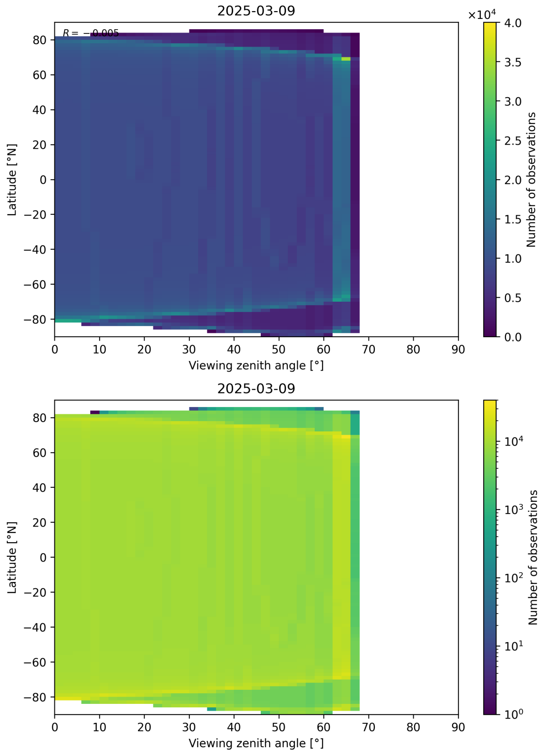
Figure 49: Scatter density plot of “Viewing zenith angle” against “Latitude” for 2025-03-08 to 2025-03-10.
