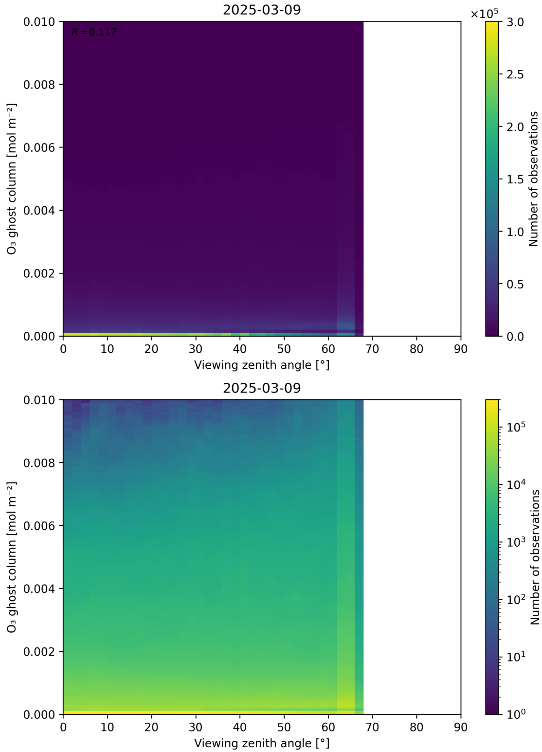
Figure 51: Scatter density plot of “Viewing zenith angle” against “O 3 ghost column” for 2025-03-08 to 2025-03-10.
