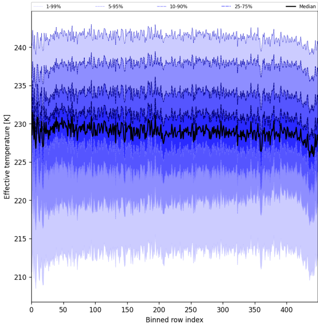
Figure 31: Along track statistics of “Effective temperature” for 2025-03-08 to 2025-03-10
