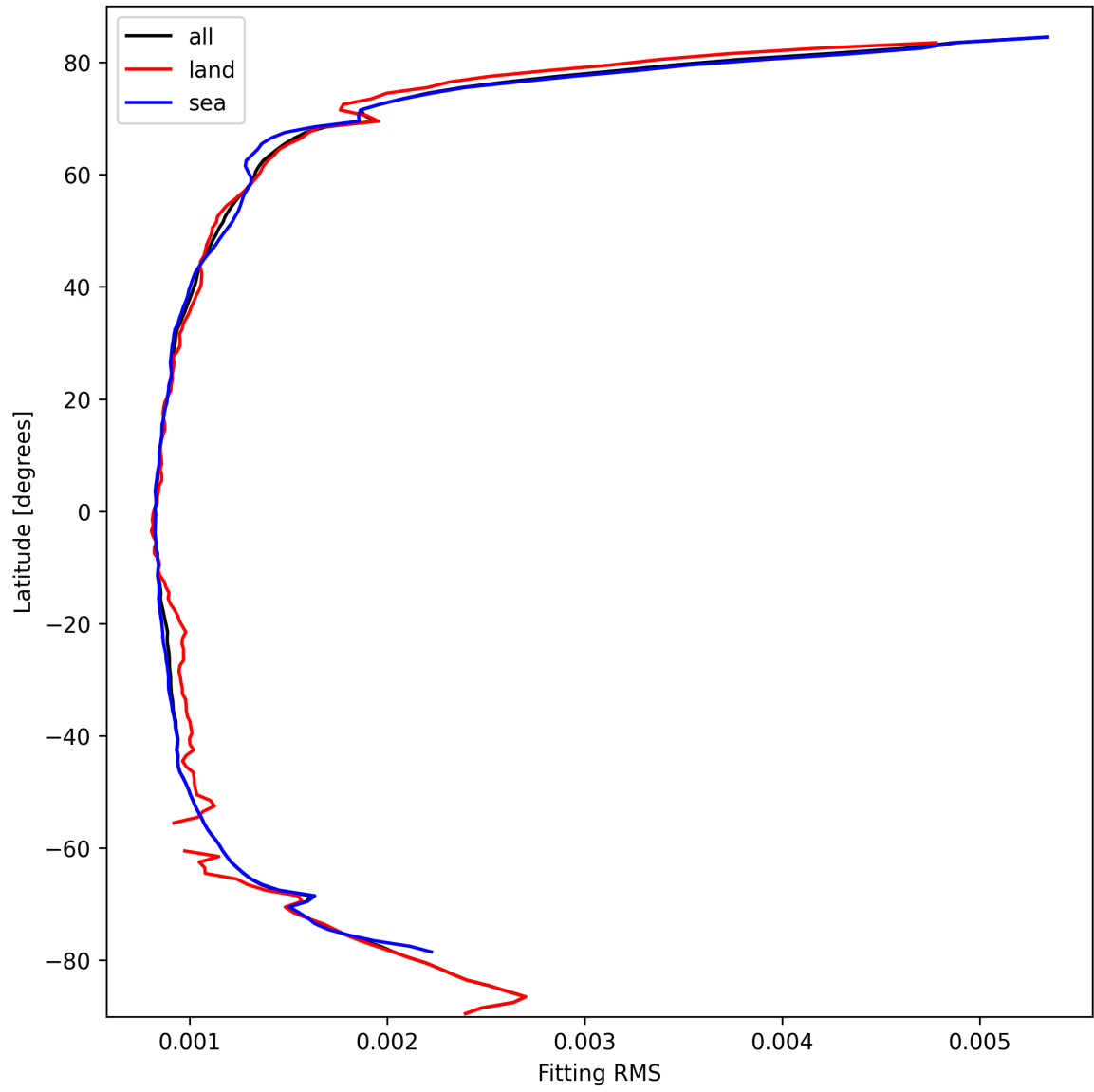
Figure 16: Zonal average of “Fitting RMS” for 2025-03-08 to 2025-03-10.
