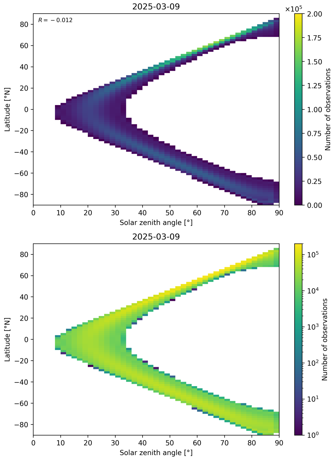
Figure 44: Scatter density plot of “Solar zenith angle” against “Latitude” for 2025-03-08 to 2025-03-10.
