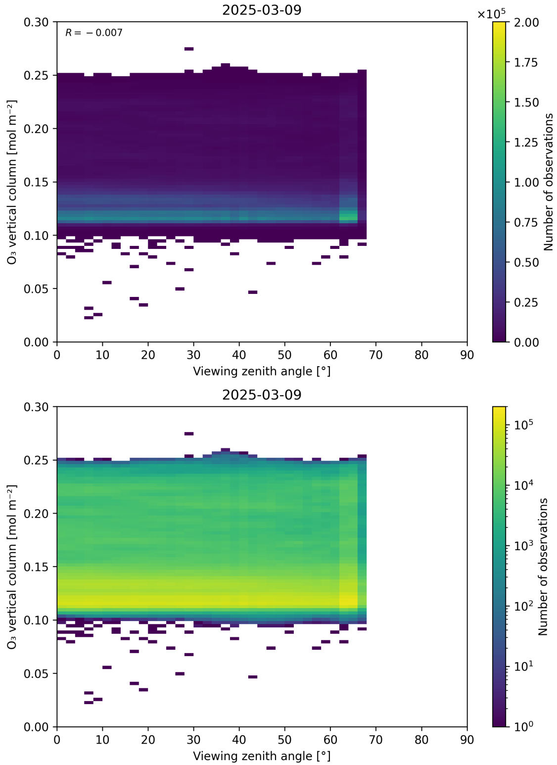
Figure 52: Scatter density plot of “Viewing zenith angle” against “O 3 vertical column” for 2025-03-08 to 2025-03-10.
