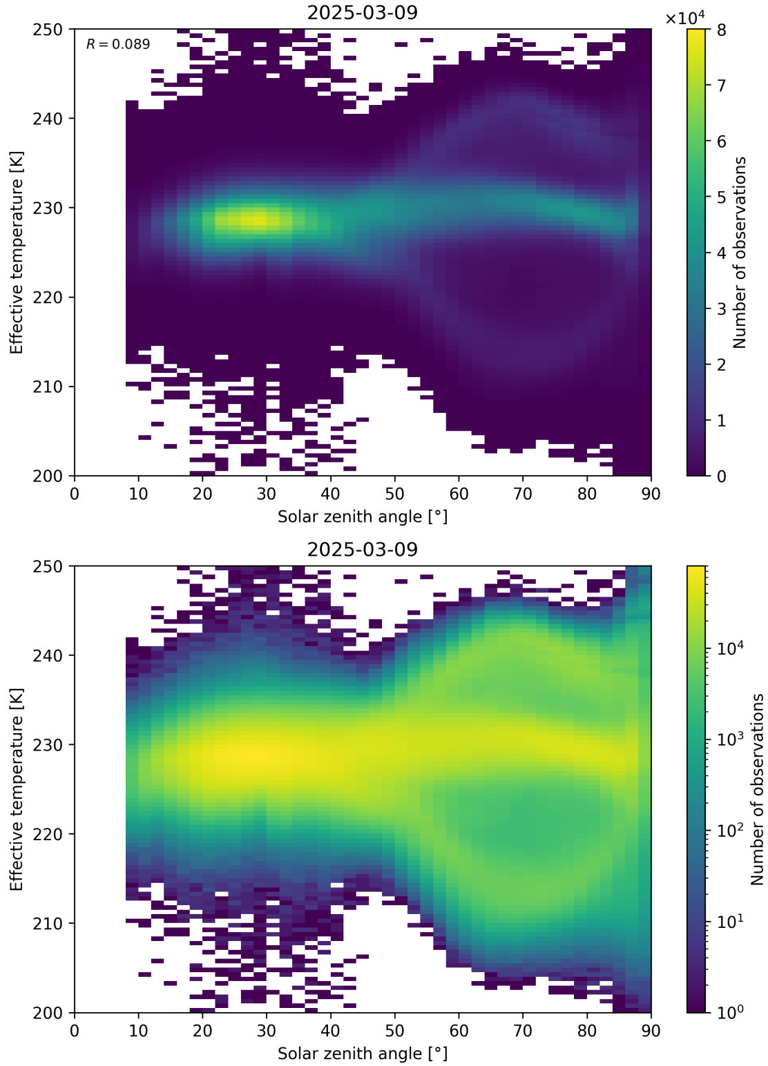
Figure 45: Scatter density plot of “Solar zenith angle” against “Effective temperature” for 2025-03-08 to 2025-03-10.
