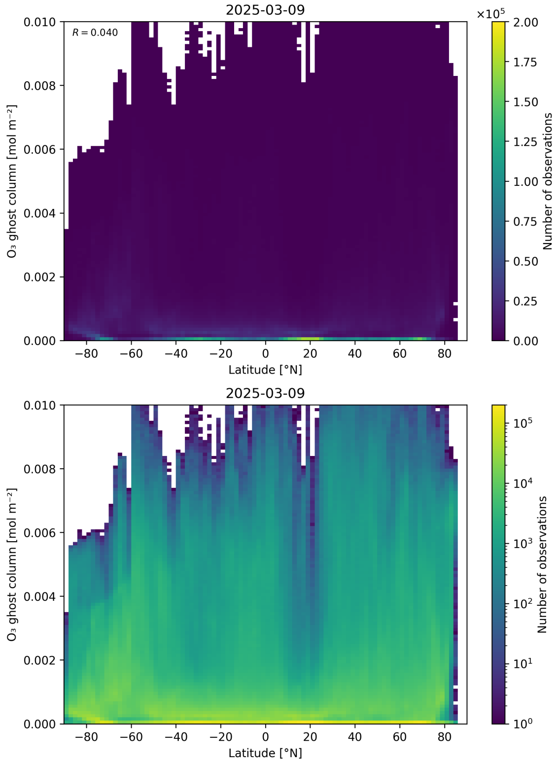
Figure 35: Scatter density plot of “Latitude” against “O 3 ghost column” for 2025-03-08 to 2025-03-10.
