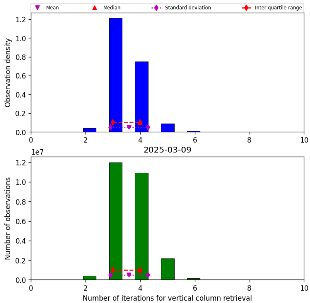
Figure 26: Histogram of “Number of iterations for vertical column retrieval” for 2025-03-08 to 2025-03-10
