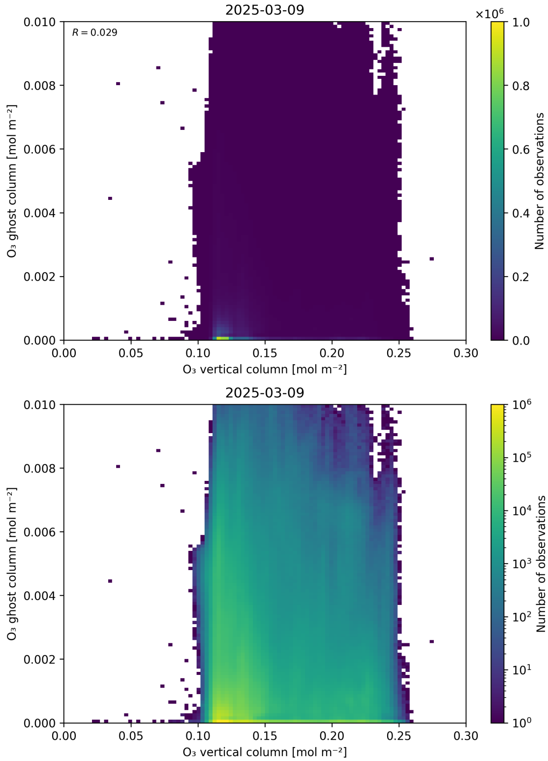
Figure 40: Scatter density plot of “O 3 vertical column” against “O 3 ghost column” for 2025-03-08 to 2025-03-10.
