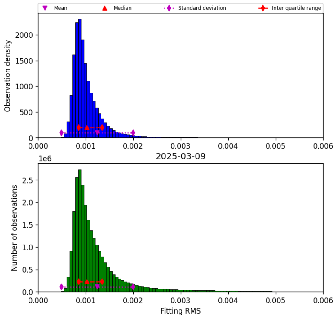
Figure 23: Histogram of “Fitting RMS” for 2025-03-08 to 2025-03-10
