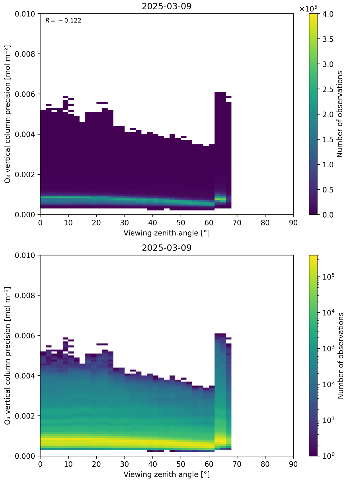
Figure 53: Scatter density plot of “Viewing zenith angle” against “O 3 vertical column precision” for 2025-03-08 to 2025-03-10.
