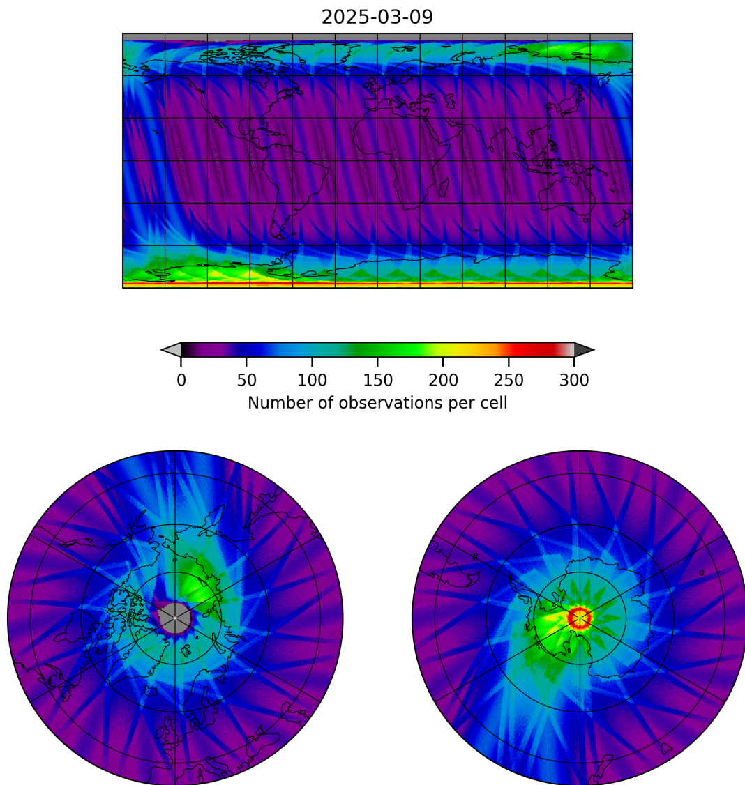
Figure 12: Map of the number of observations for 2025-03-08 to 2025-03-10
