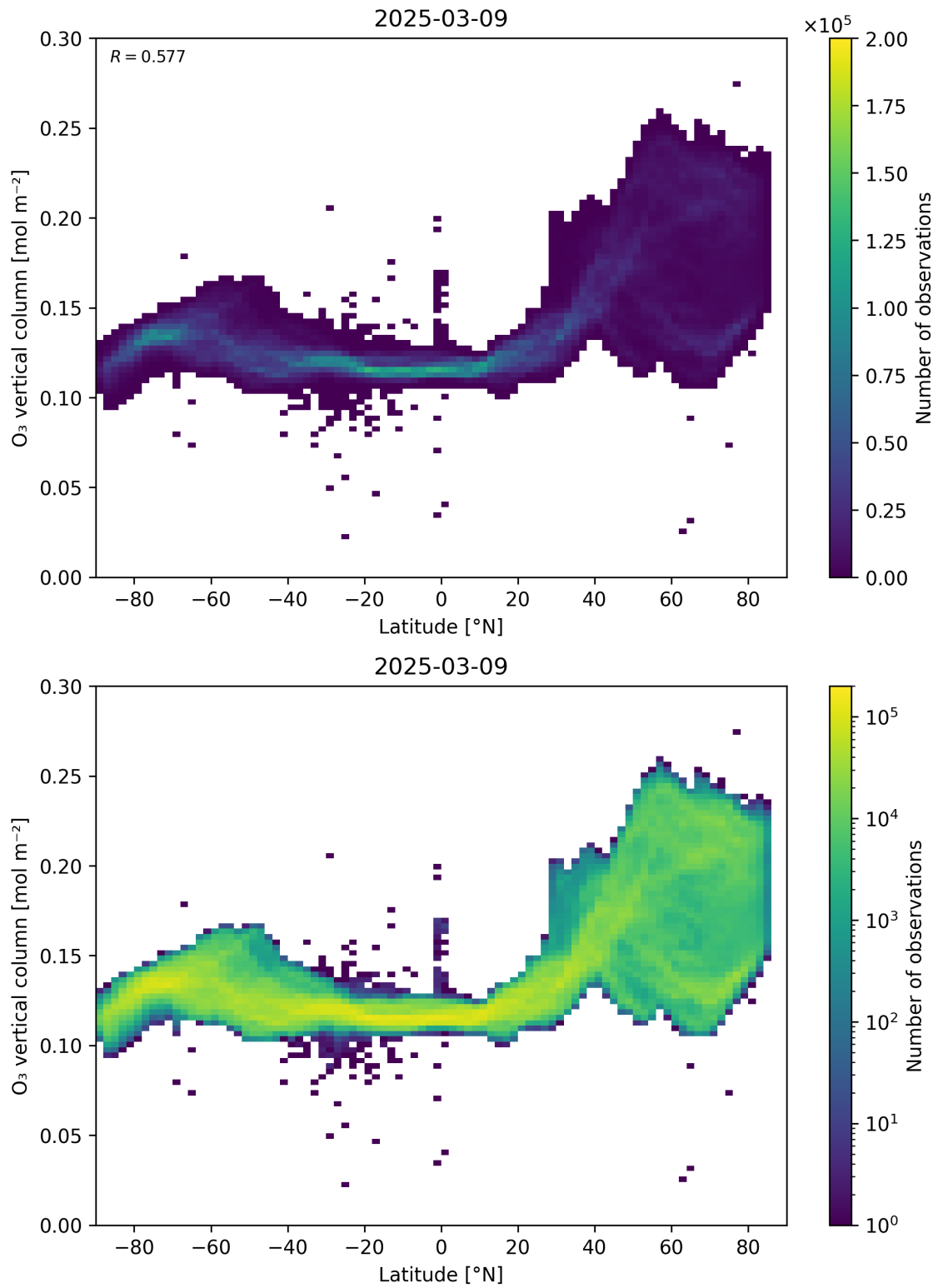
Figure 36: Scatter density plot of “Latitude” against “O 3 vertical column” for 2025-03-08 to 2025-03-10.
