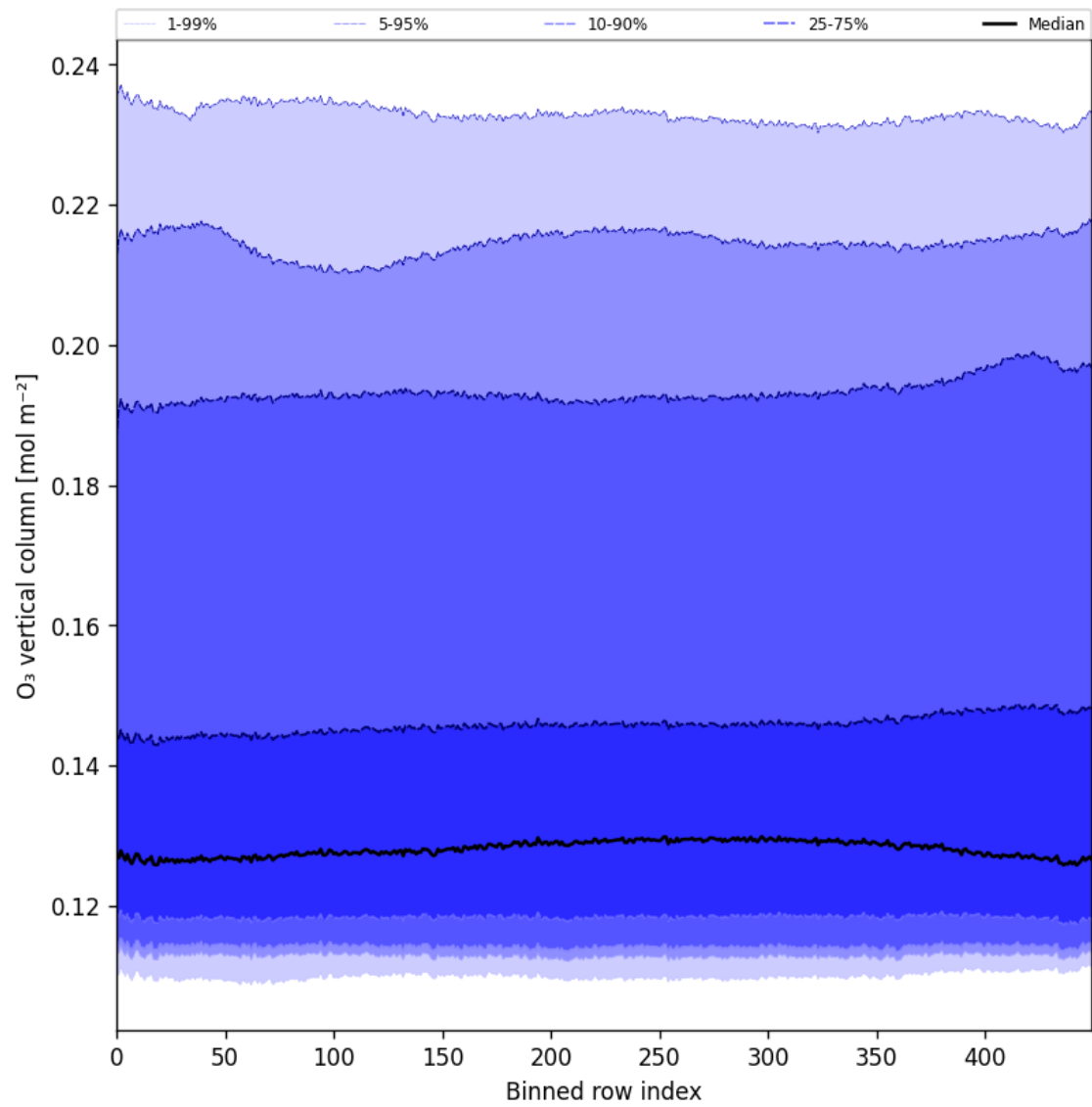
Figure 28: Along track statistics of “O 3 vertical column” for 2025-03-08 to 2025-03-10
