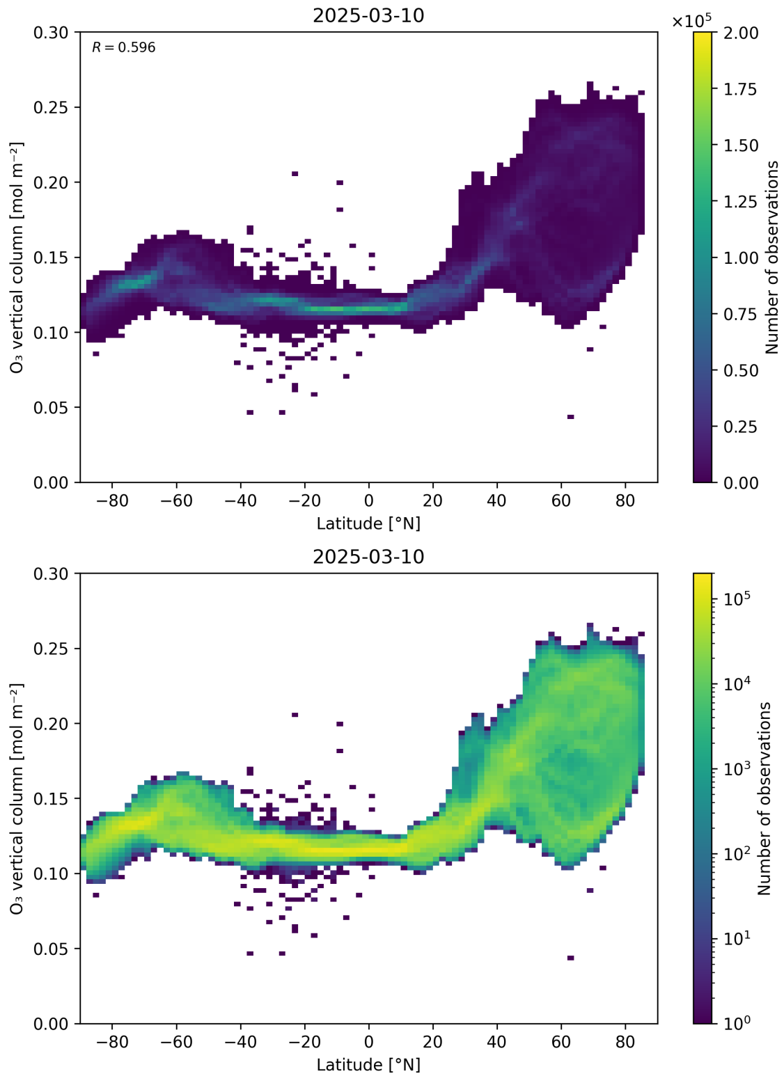
Figure 36: Scatter density plot of “Latitude” against “O 3 vertical column” for 2025-03-09 to 2025-03-11.
