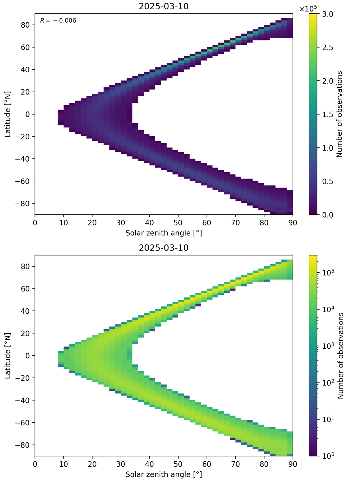
Figure 44: Scatter density plot of “Solar zenith angle” against “Latitude” for 2025-03-09 to 2025-03-11.
