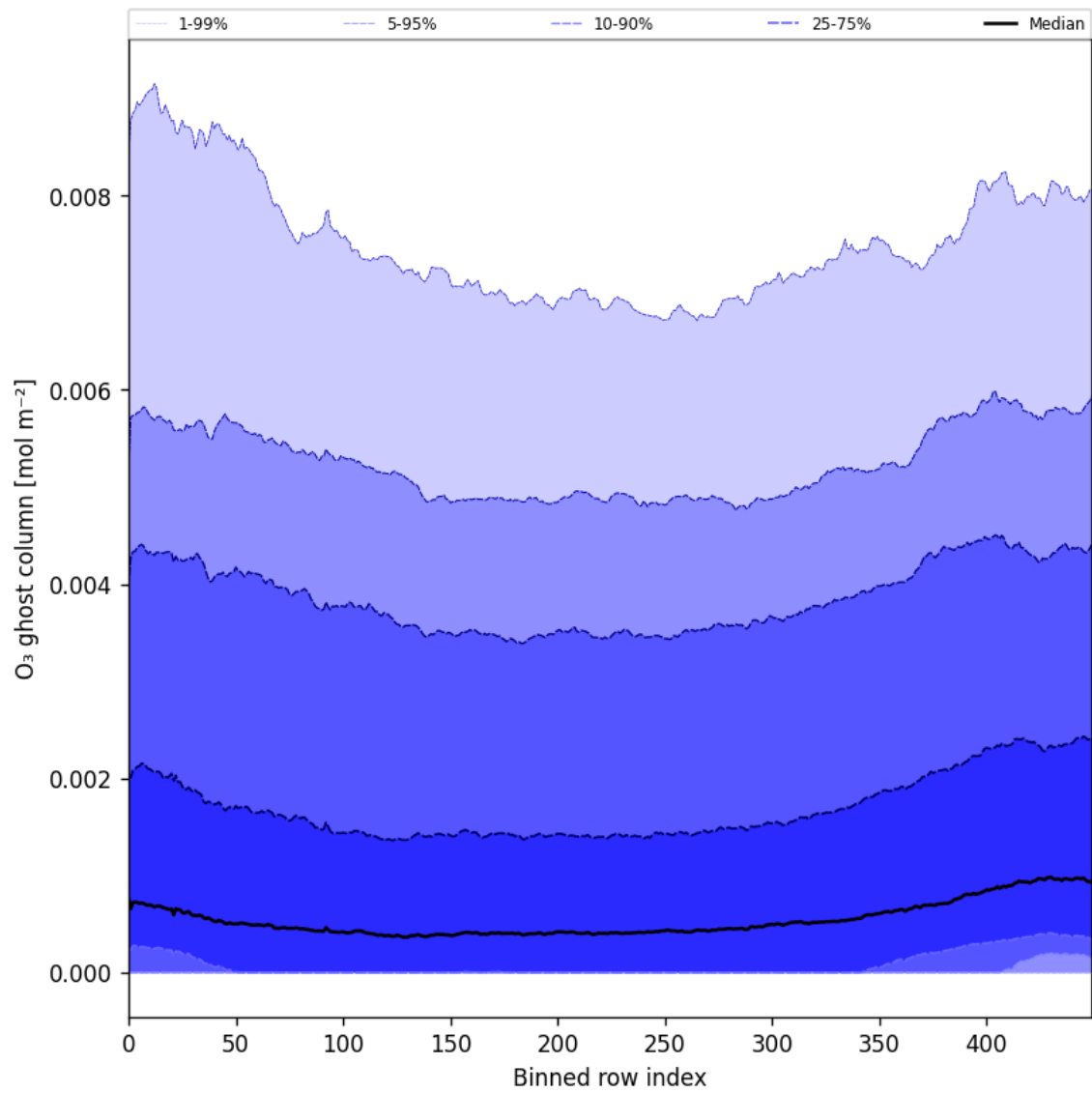
Figure 32: Along track statistics of “O 3 ghost column” for 2025-03-09 to 2025-03-11
