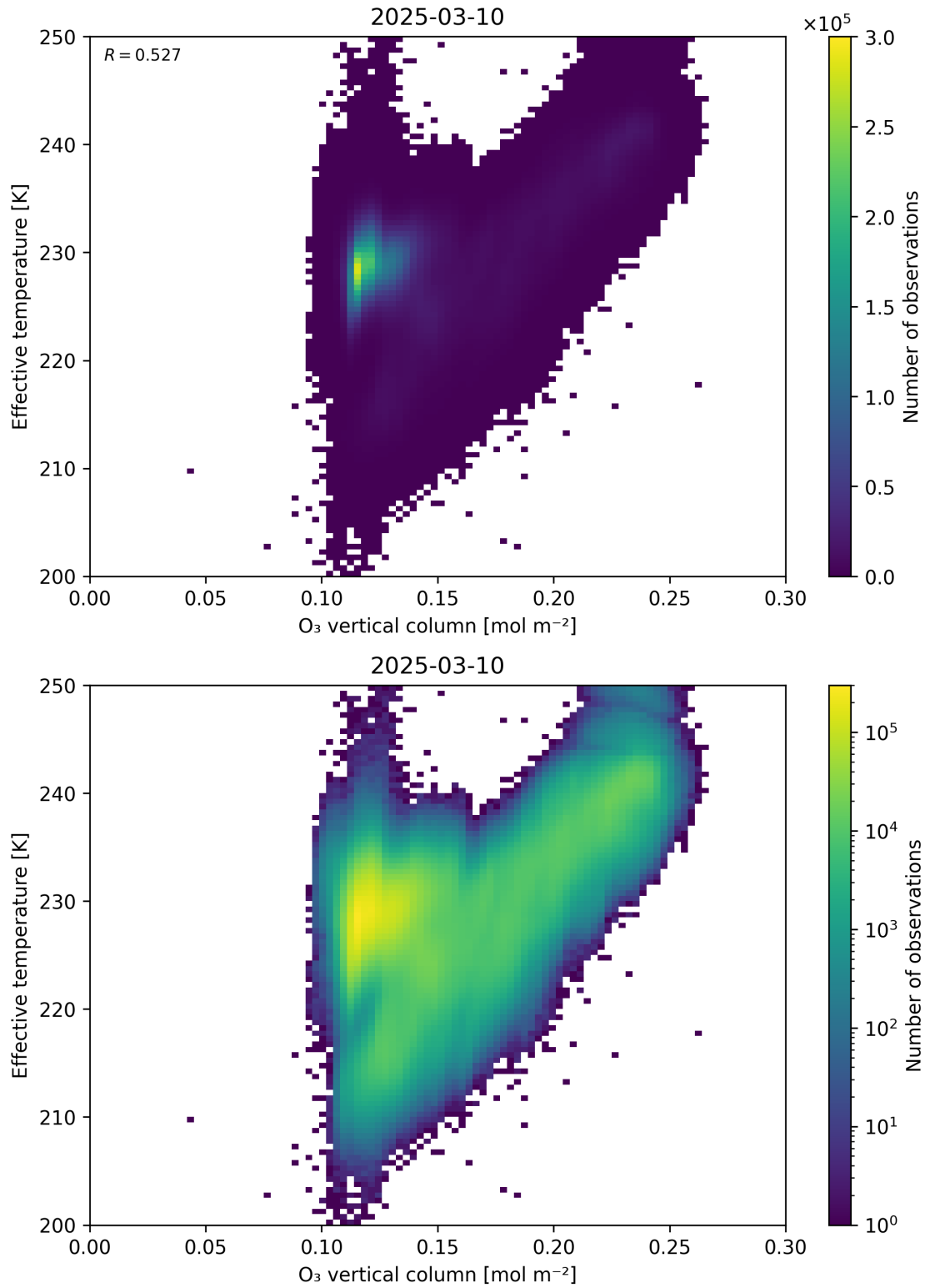
Figure 39: Scatter density plot of “O 3 vertical column” against “Effective temperature” for 2025-03-09 to 2025-03-11.
