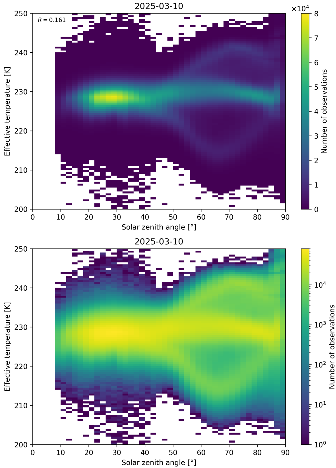
Figure 45: Scatter density plot of “Solar zenith angle” against “Effective temperature” for 2025-03-09 to 2025-03-11.
