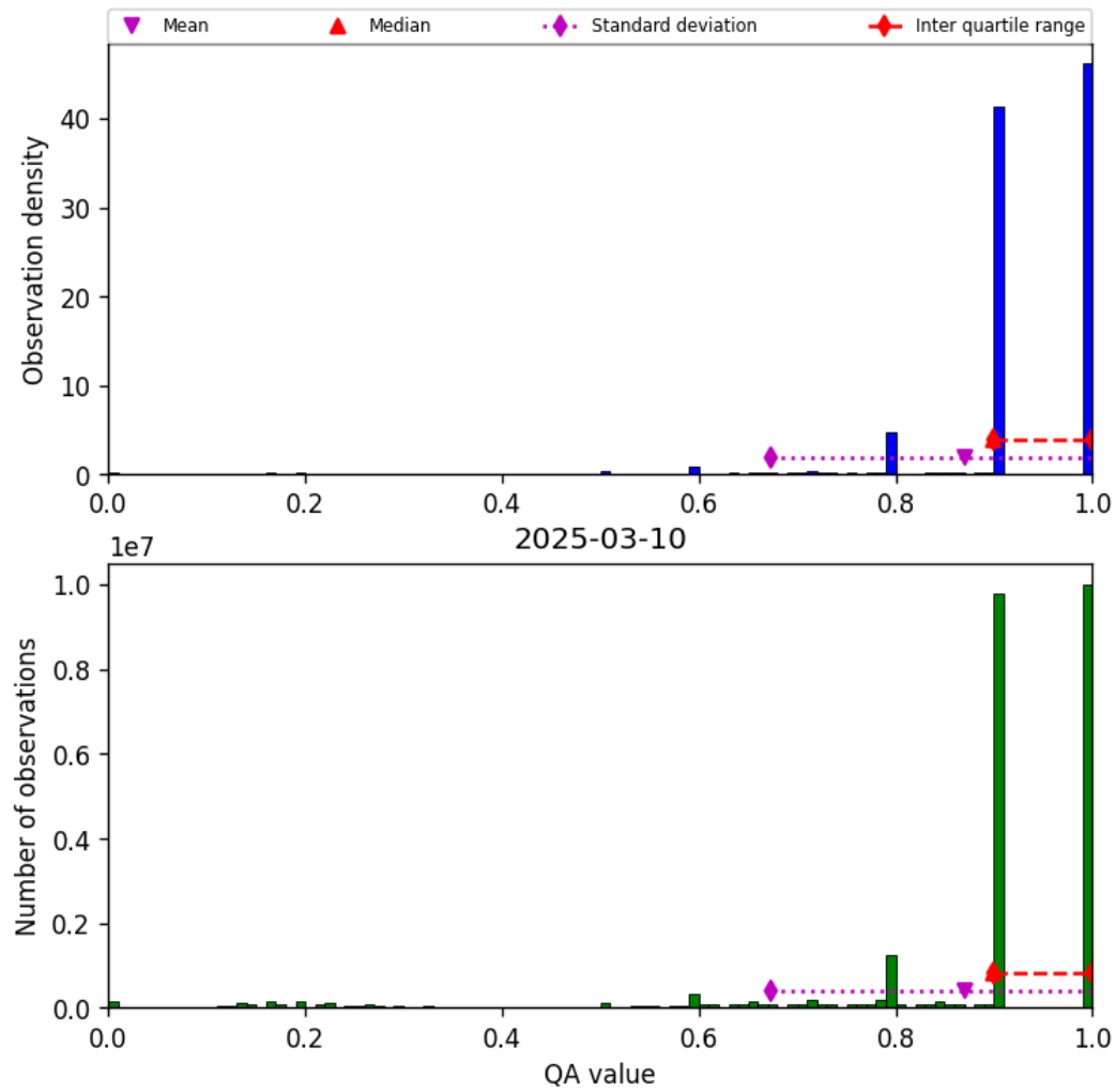
Figure 20: Histogram of “QA value” for 2025-03-09 to 2025-03-11
