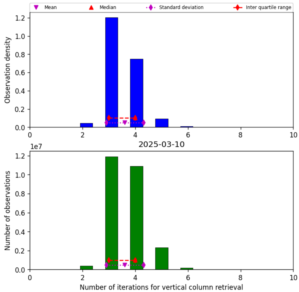
Figure 26: Histogram of “Number of iterations for vertical column retrieval” for 2025-03-09 to 2025-03-11
