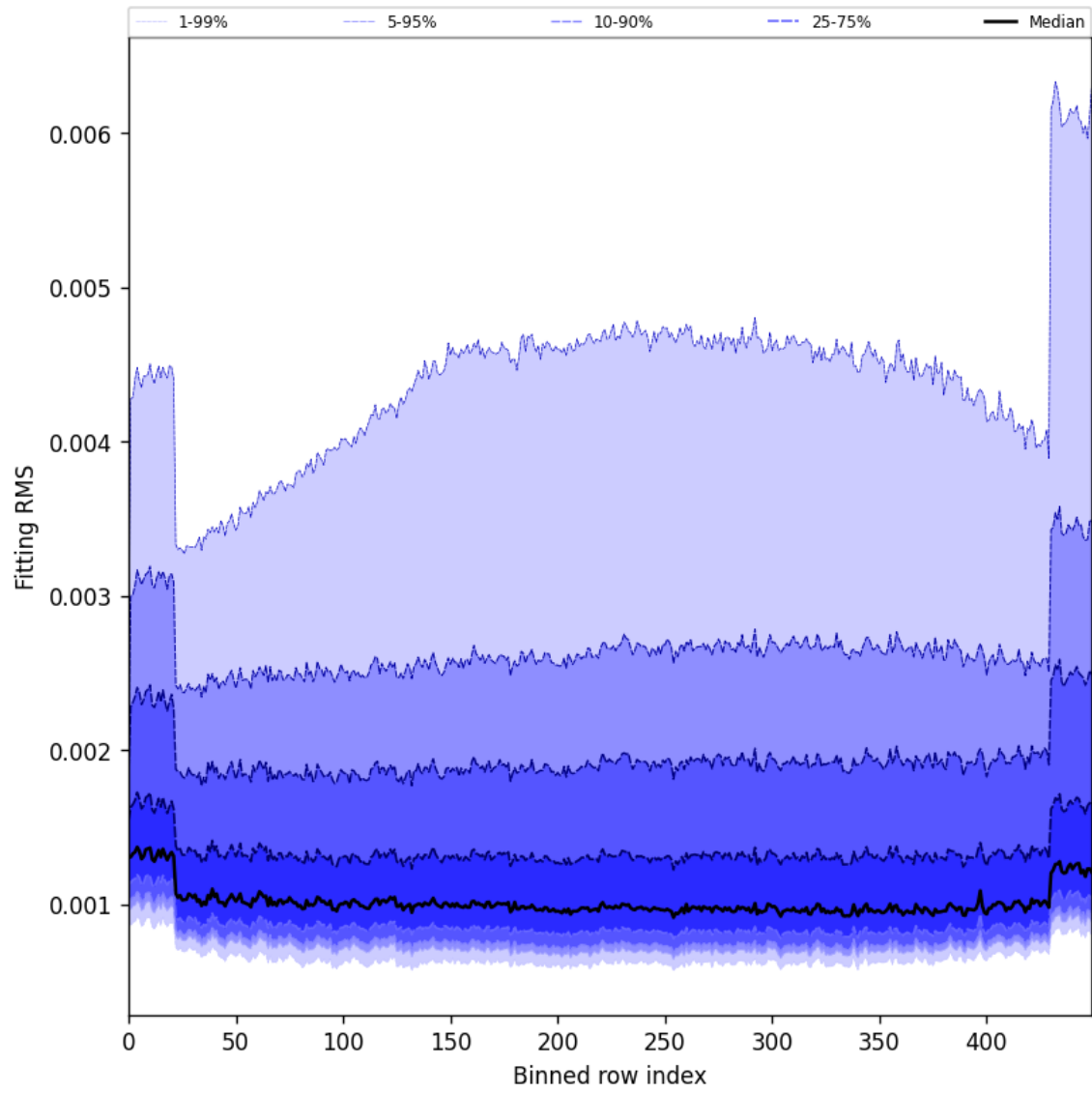
Figure 30: Along track statistics of “Fitting RMS” for 2025-03-09 to 2025-03-11
