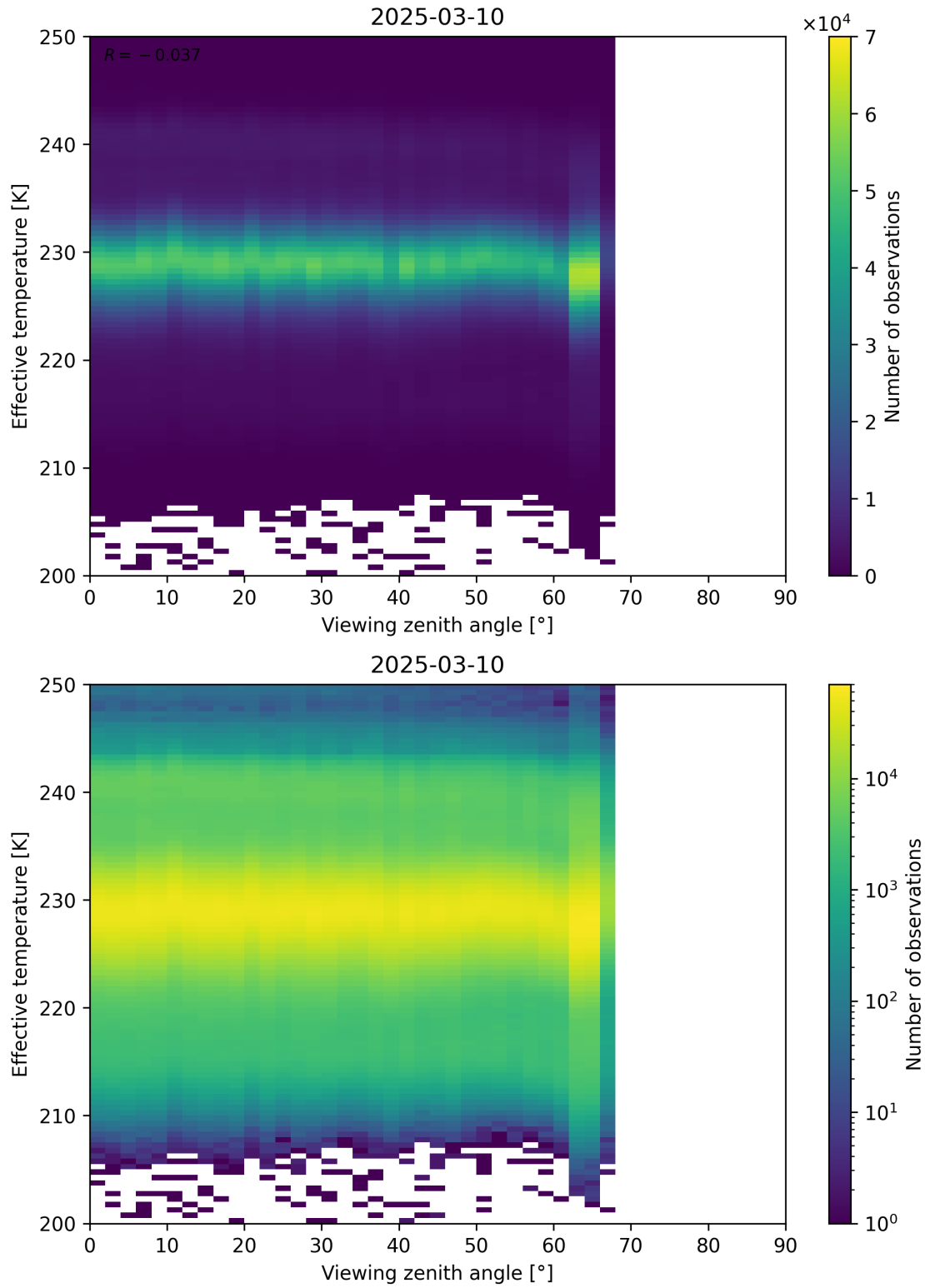
Figure 50: Scatter density plot of “Viewing zenith angle” against “Effective temperature” for 2025-03-09 to 2025-03-11.
