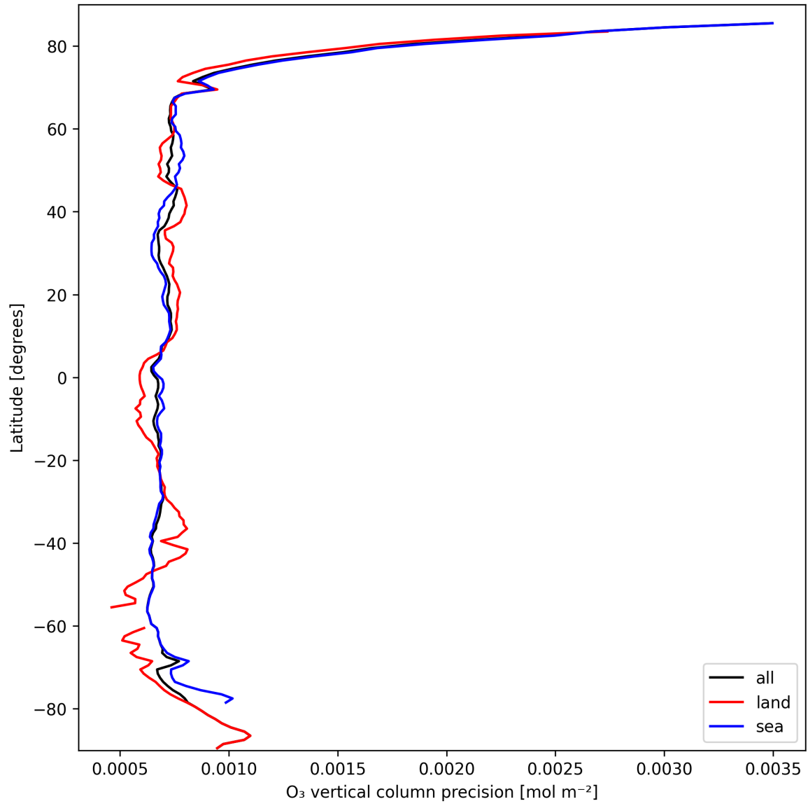
Figure 15: Zonal average of "O 3 vertical column precision" for 2025-03-09 to 2025-03-11.
