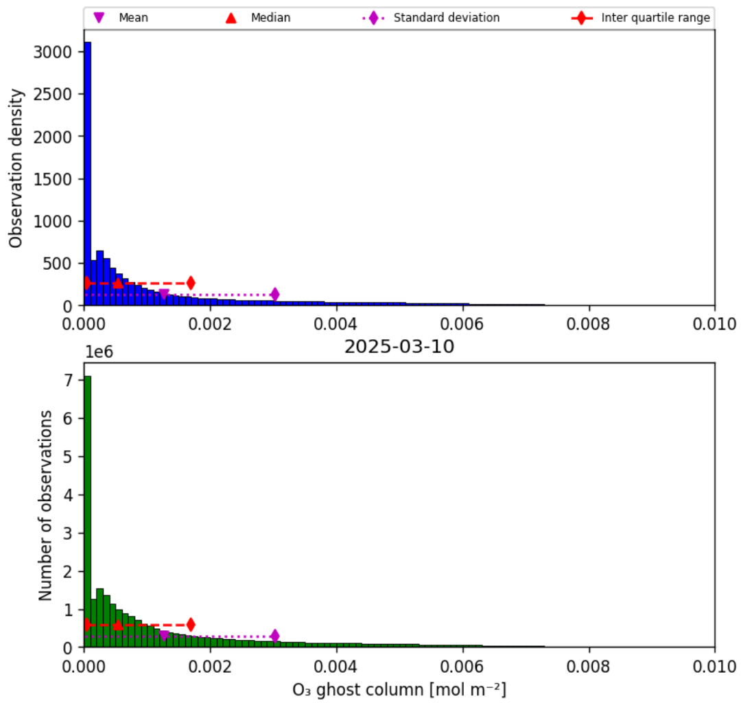
Figure 25: Histogram of “O 3 ghost column” for 2025-03-09 to 2025-03-11
