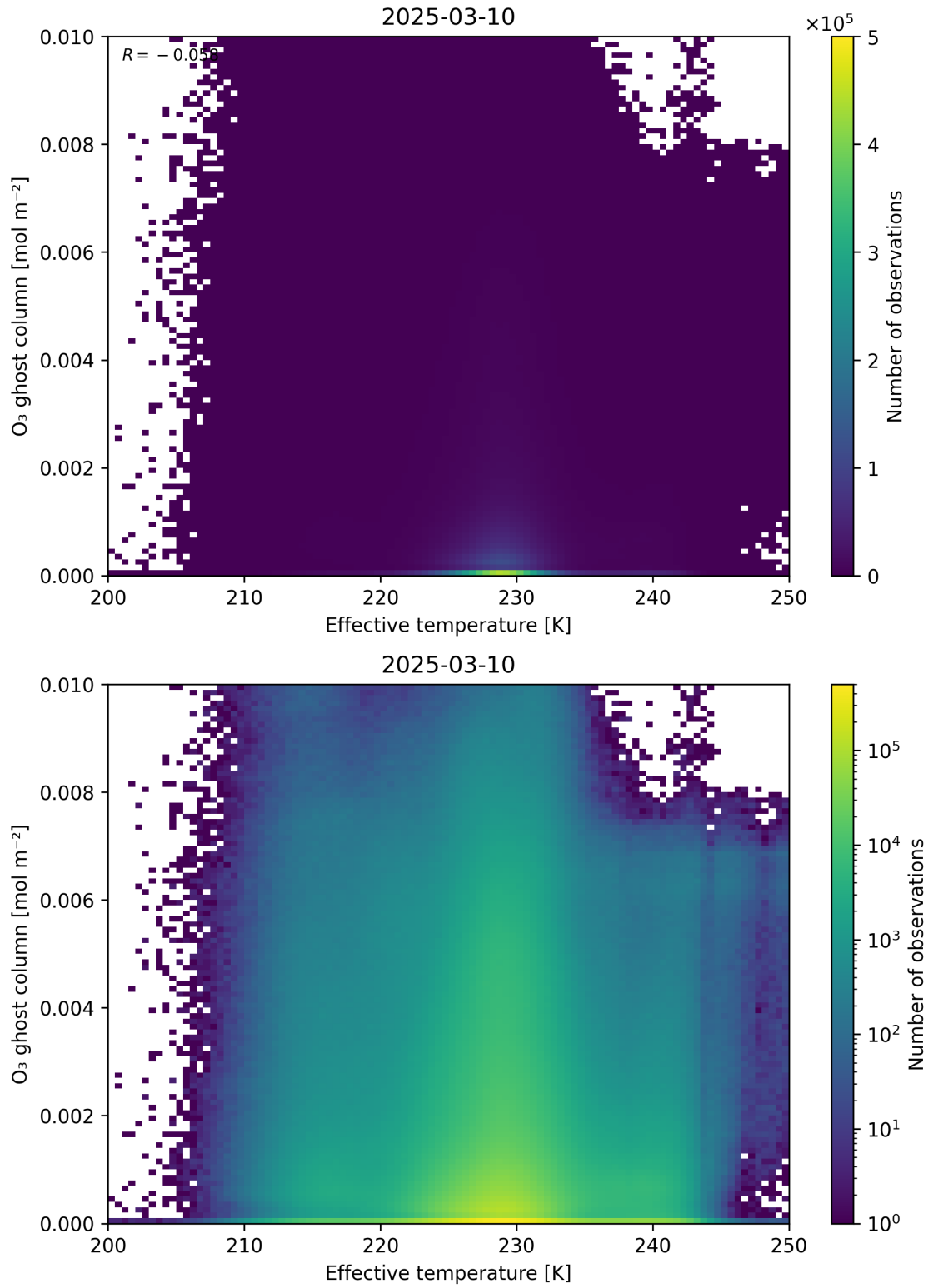
Figure 38: Scatter density plot of “Effective temperature” against “O 3 ghost column” for 2025-03-09 to 2025-03-11.
