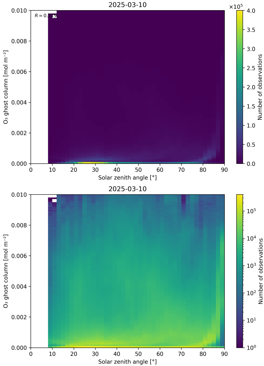
Figure 46: Scatter density plot of “Solar zenith angle” against “O 3 ghost column” for 2025-03-09 to 2025-03-11.
