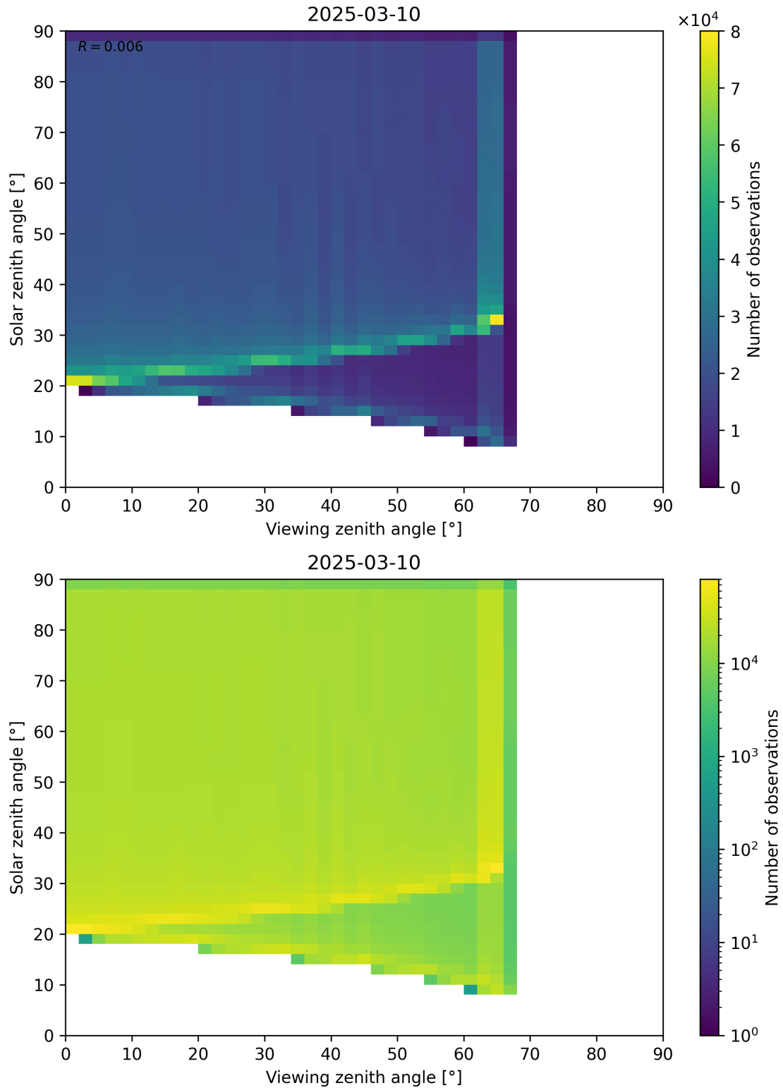
Figure 54: Scatter density plot of “Viewing zenith angle” against “Solar zenith angle” for 2025-03-09 to 2025-03-11.
