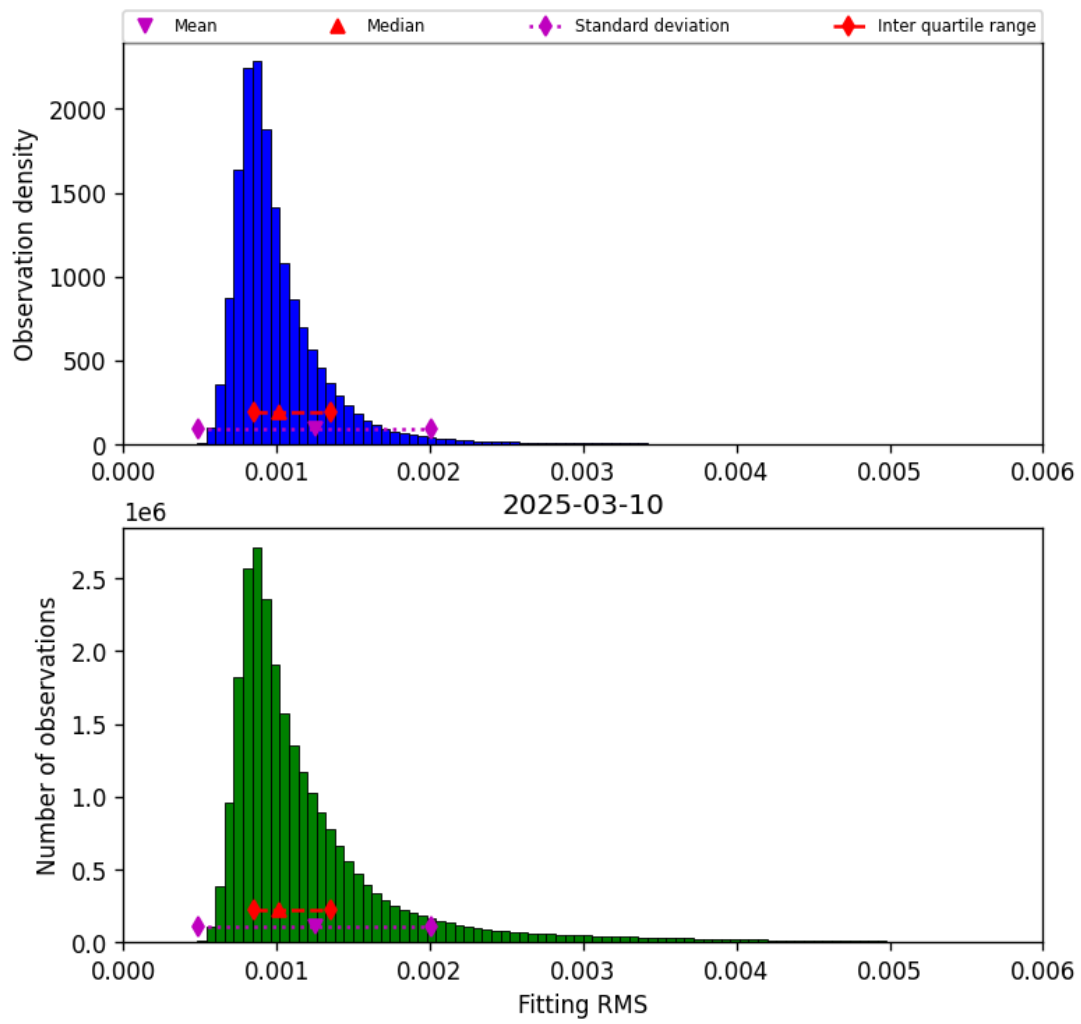
Figure 23: Histogram of “Fitting RMS” for 2025-03-09 to 2025-03-11
