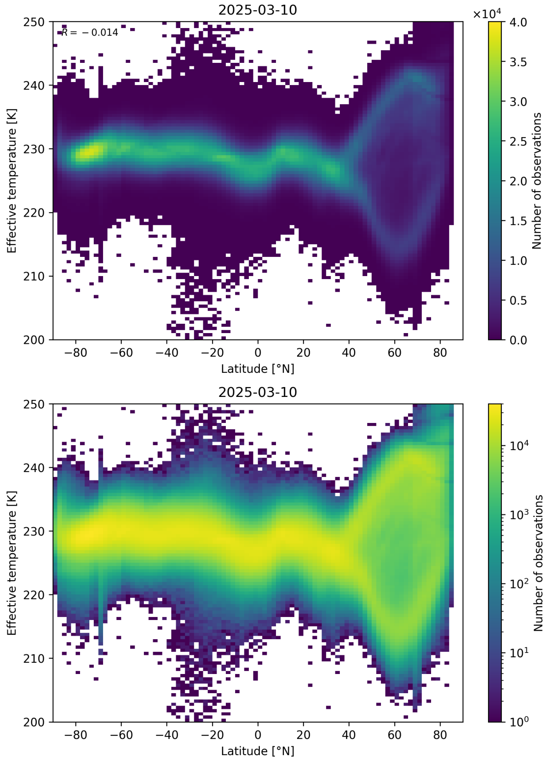
Figure 34: Scatter density plot of “Latitude” against “Effective temperature” for 2025-03-09 to 2025-03-11.
