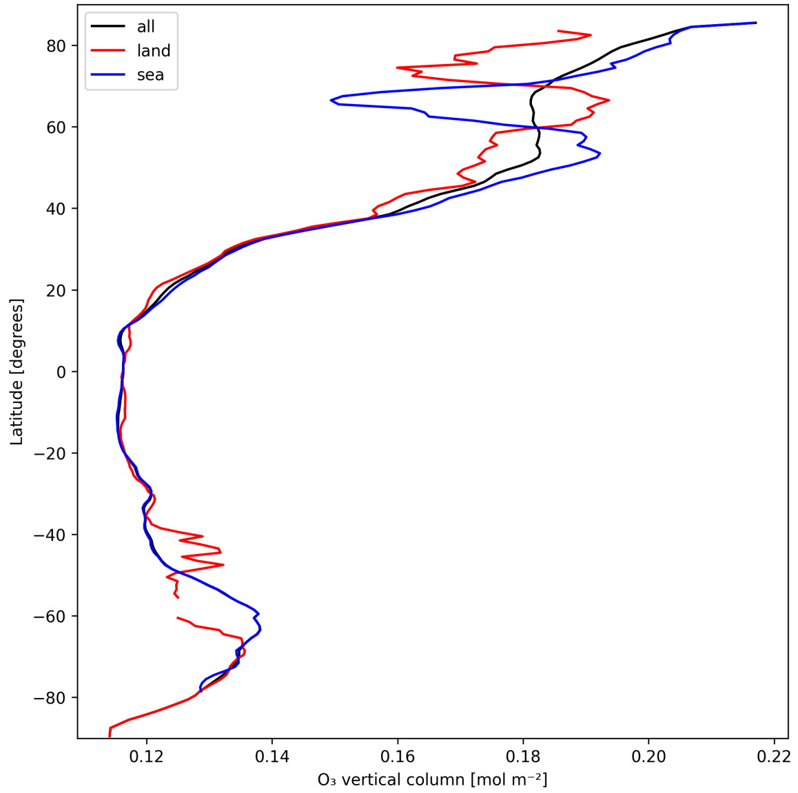
Figure 14: Zonal average of “O 3 vertical column” for 2025-03-09 to 2025-03-11.
