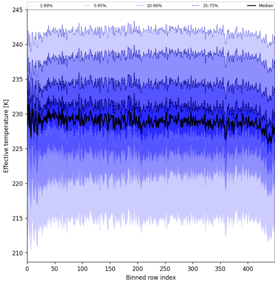
Figure 31: Along track statistics of “Effective temperature” for 2025-03-09 to 2025-03-11
