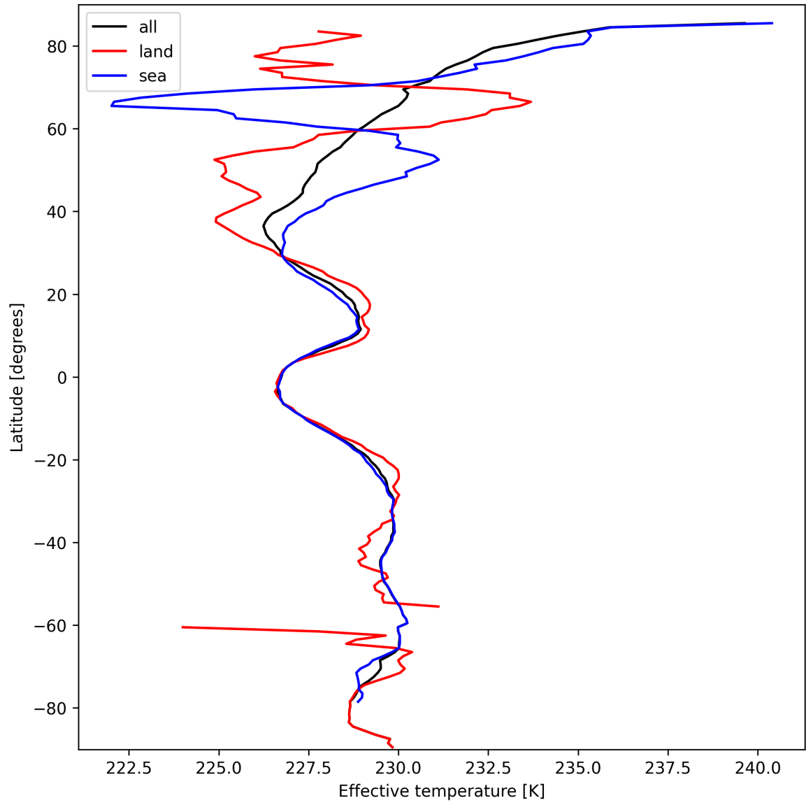
Figure 17: Zonal average of “Effective temperature” for 2025-03-09 to 2025-03-11.
