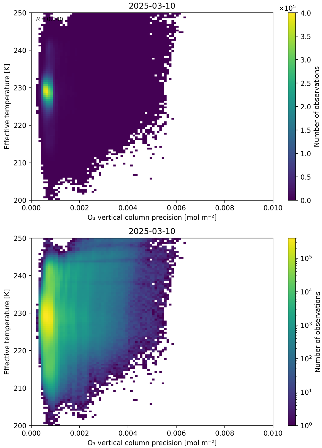
Figure 42: Scatter density plot of “O 3 vertical column precision” against “Effective temperature” for 2025-03-09 to 2025-03-11.
