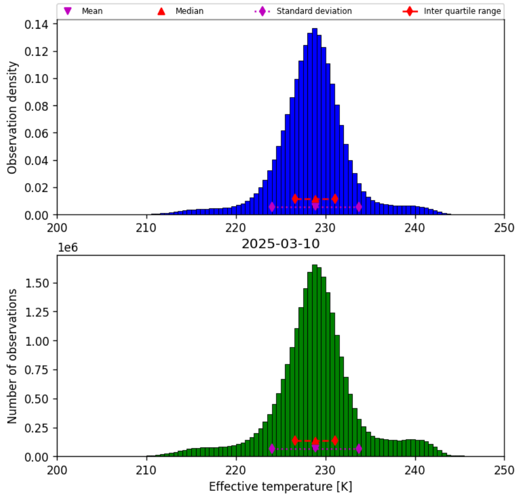
Figure 24: Histogram of “Effective temperature” for 2025-03-09 to 2025-03-11
