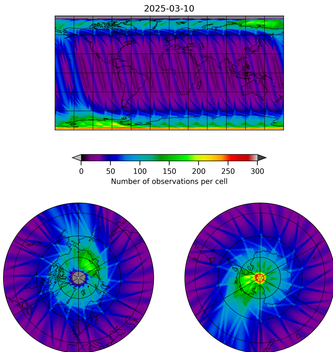
Figure 12: Map of the number of observations for 2025-03-09 to 2025-03-11
