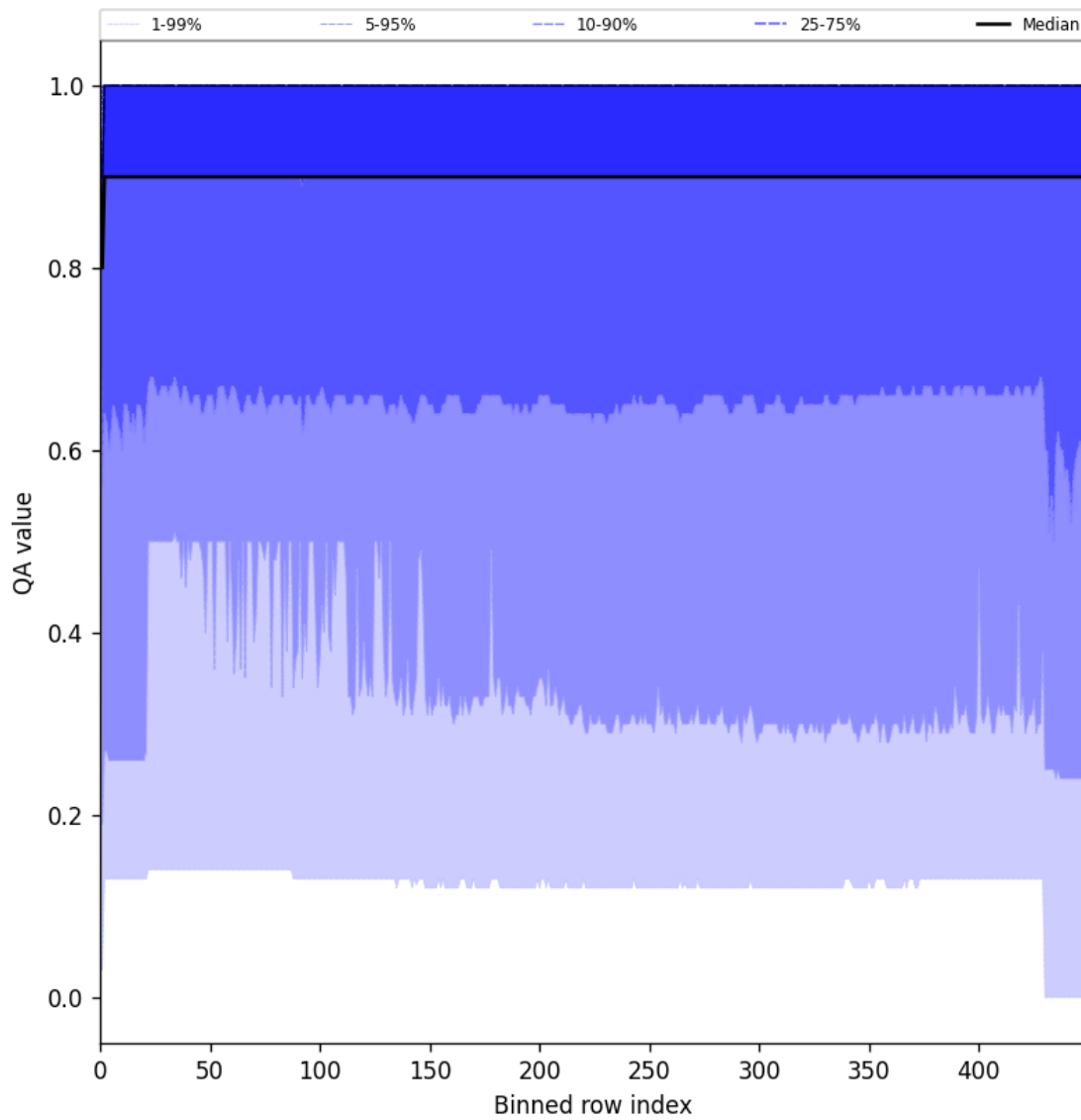
Figure 27: Along track statistics of “QA value” for 2025-03-09 to 2025-03-11
