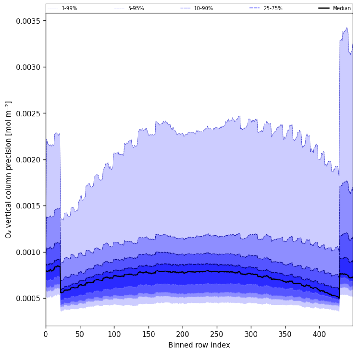
Figure 29: Along track statistics of “O 3 vertical column precision” for 2025-03-09 to 2025-03-11
