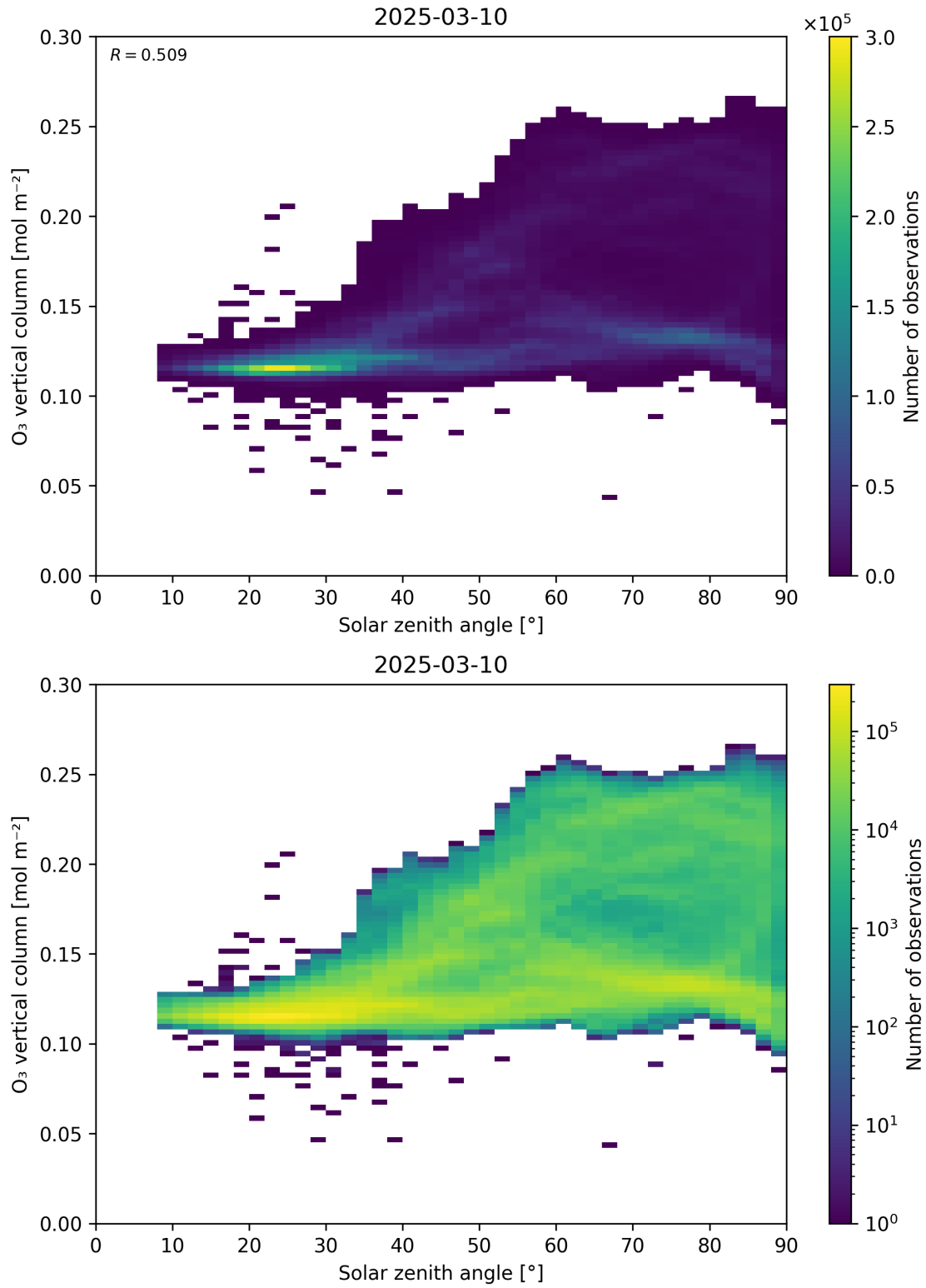
Figure 47: Scatter density plot of “Solar zenith angle” against “O 3 vertical column” for 2025-03-09 to 2025-03-11.
