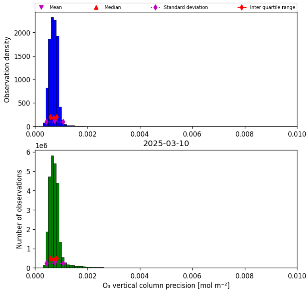
Figure 22: Histogram of “O 3 vertical column precision” for 2025-03-09 to 2025-03-11
