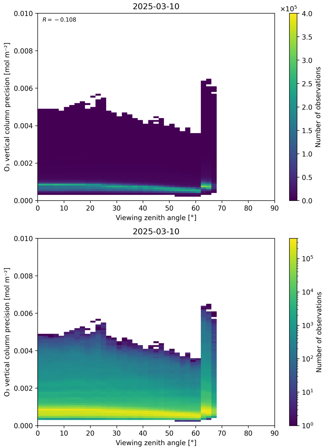
Figure 53: Scatter density plot of “Viewing zenith angle” against “O 3 vertical column precision” for 2025-03-09 to 2025-03-11.
