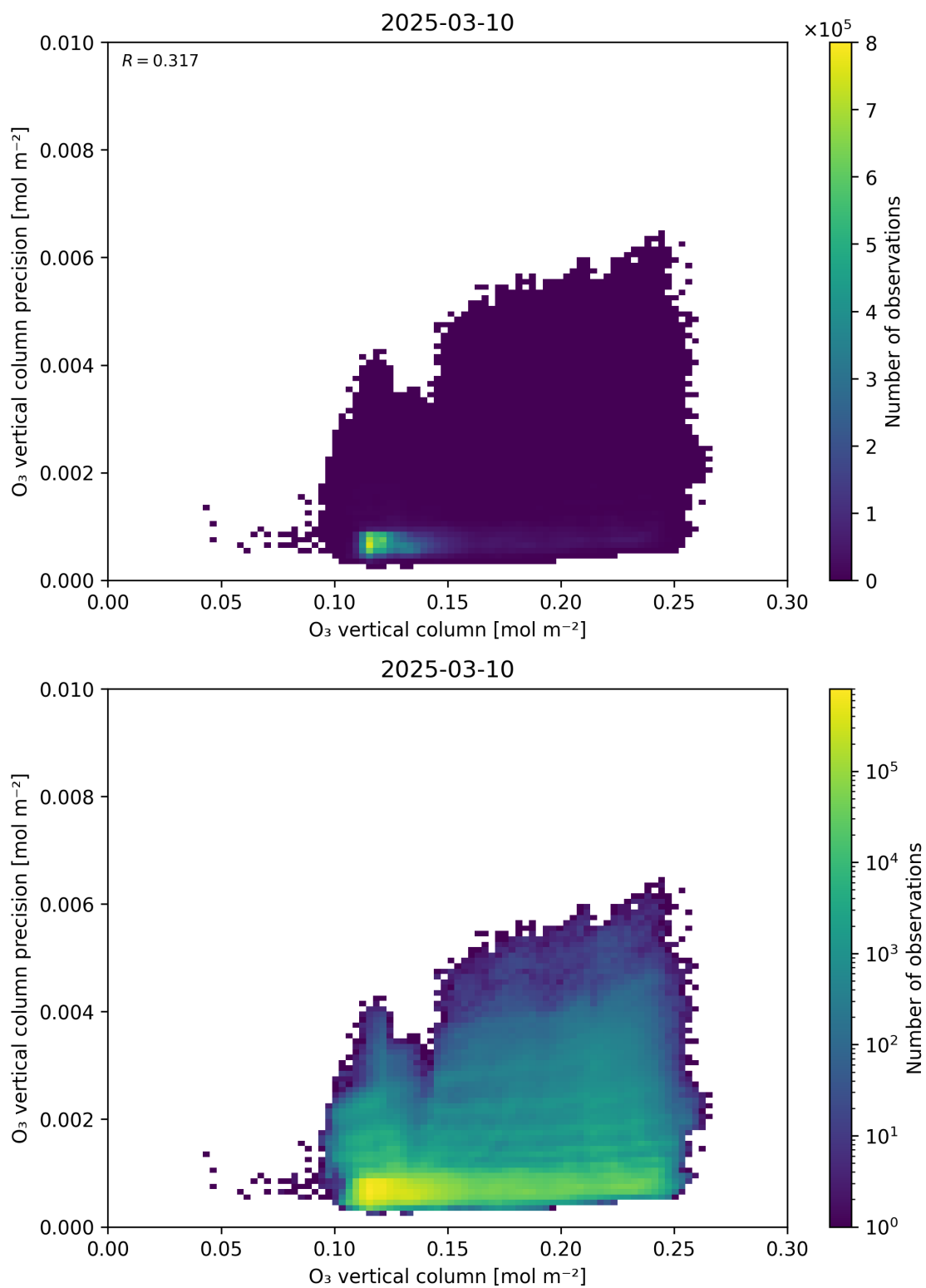
Figure 41: Scatter density plot of “O 3 vertical column” against “O 3 vertical column precision” for 2025-03-09 to 2025-03-11.
