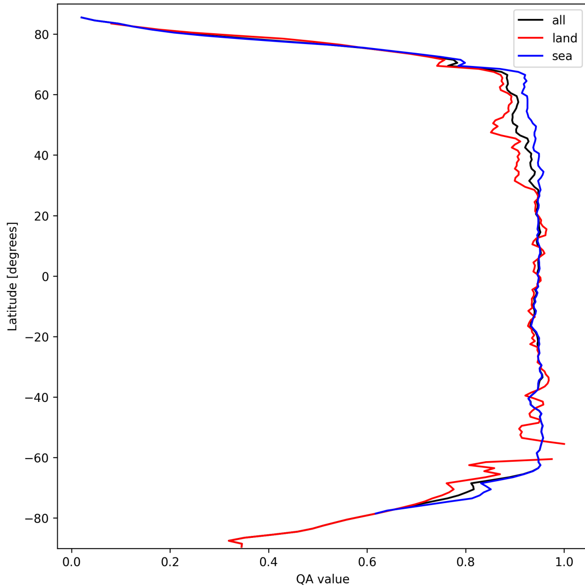
Figure 13: Zonal average of “QA value” for 2025-03-09 to 2025-03-11.
