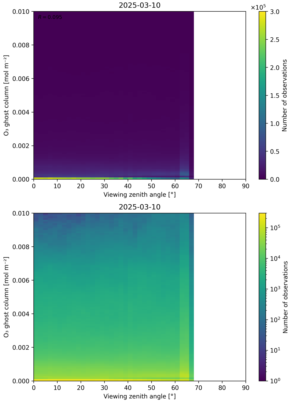
Figure 51: Scatter density plot of “Viewing zenith angle” against “O 3 ghost column” for 2025-03-09 to 2025-03-11.
