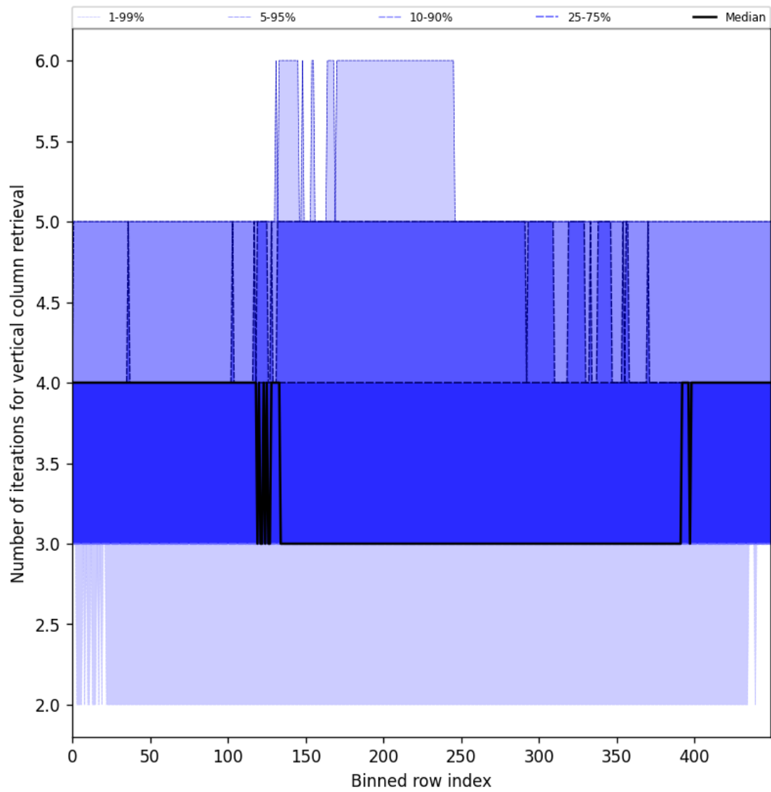
Figure 33: Along track statistics of “Number of iterations for vertical column retrieval” for 2025-03-09 to 2025-03-11
