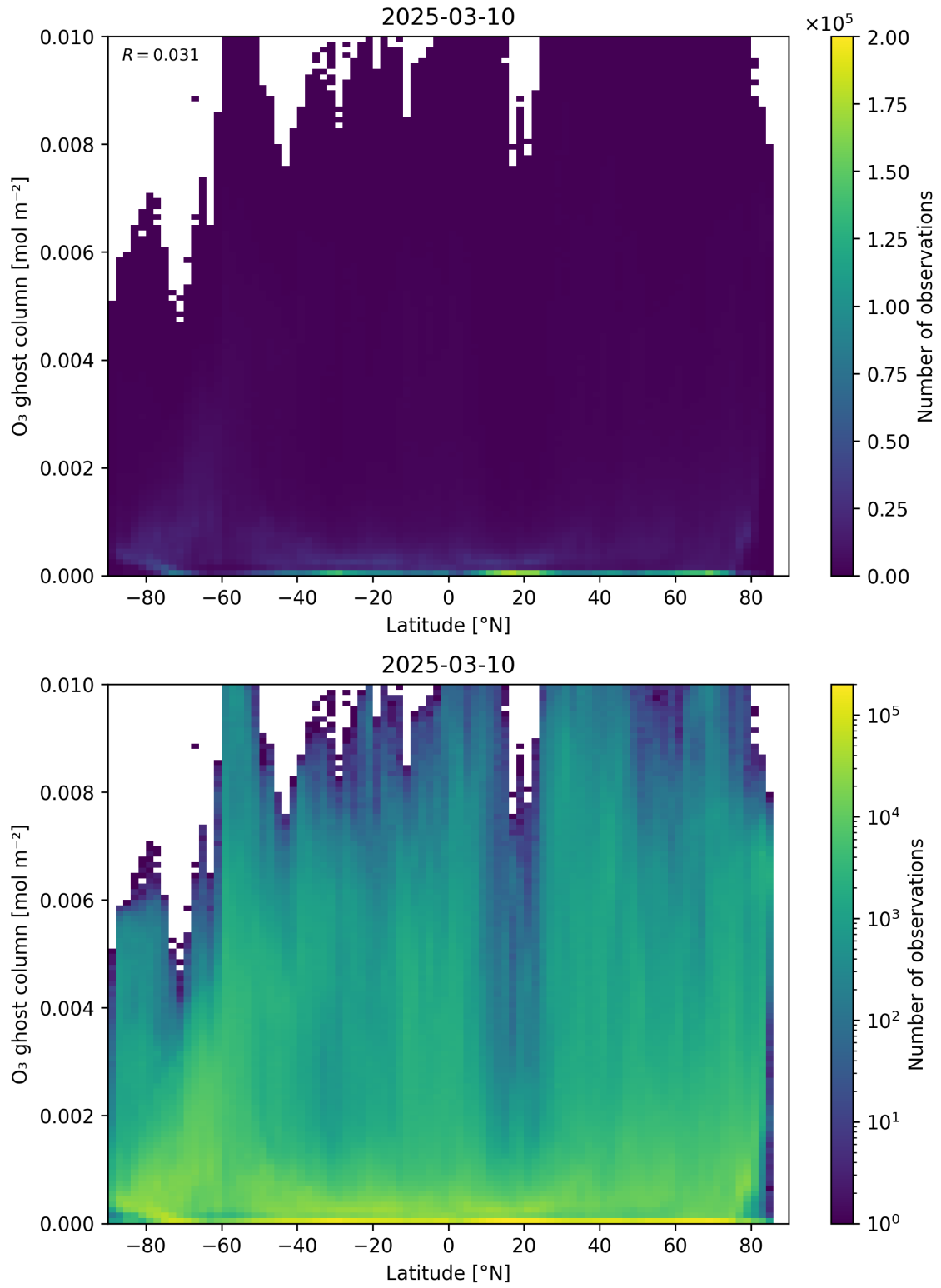
Figure 35: Scatter density plot of “Latitude” against “O 3 ghost column” for 2025-03-09 to 2025-03-11.
