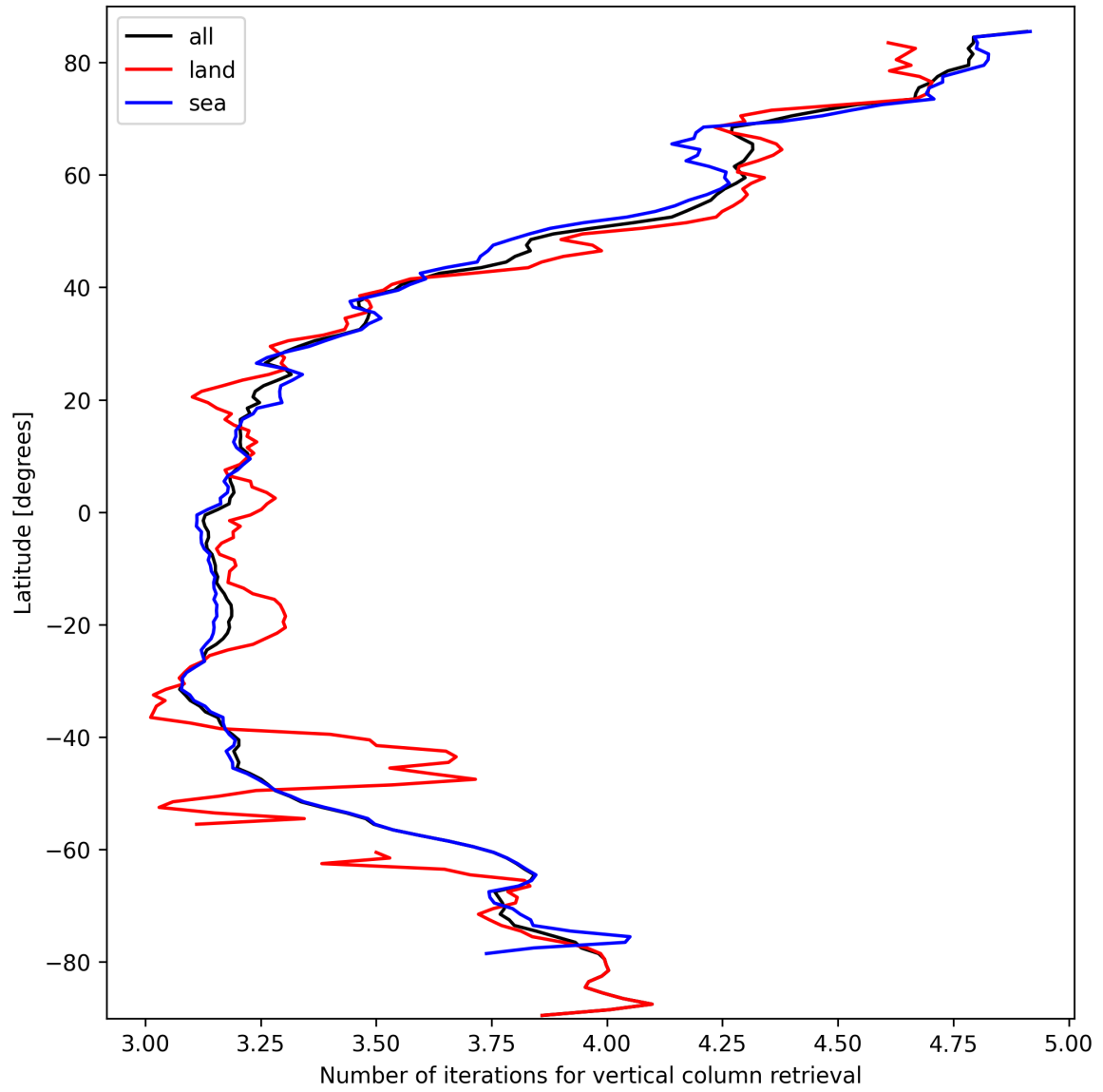
Figure 19: Zonal average of “Number of iterations for vertical column retrieval” for 2025-03-09 to 2025-03-11.
