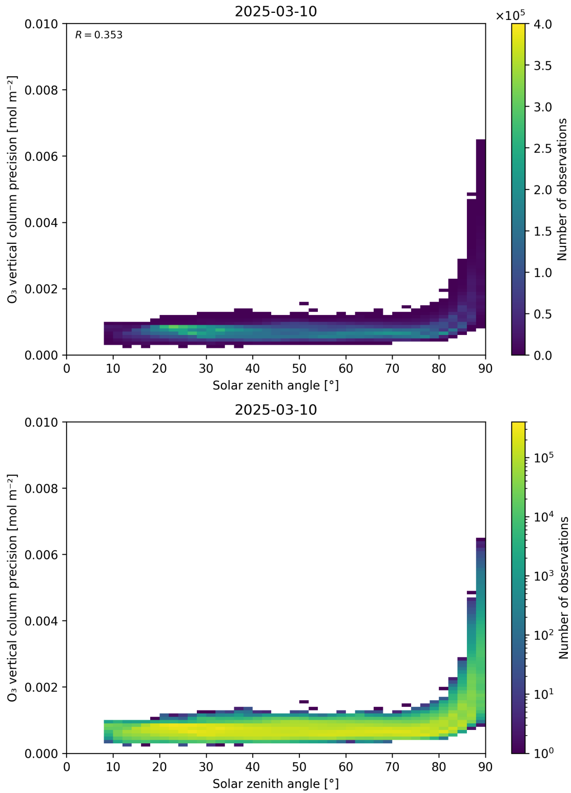
Figure 48: Scatter density plot of “Solar zenith angle” against “O 3 vertical column precision” for 2025-03-09 to 2025-03-11.
