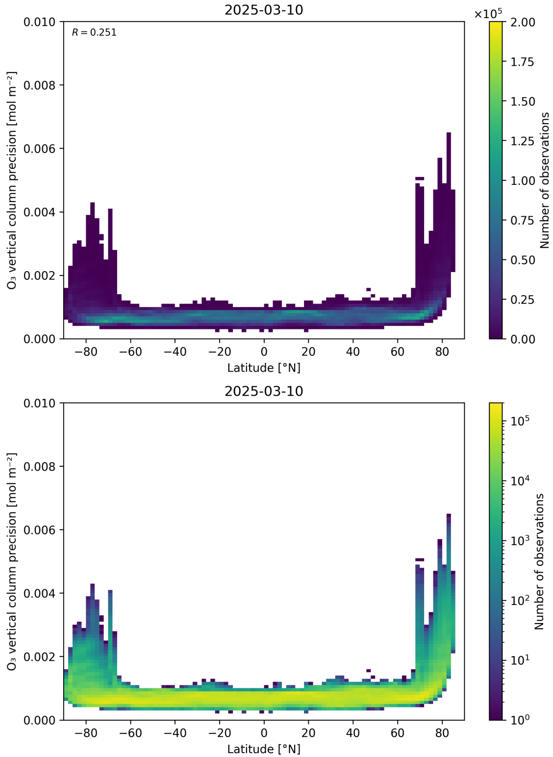
Figure 37: Scatter density plot of “Latitude” against “O 3 vertical column precision” for 2025-03-09 to 2025-03-11.
