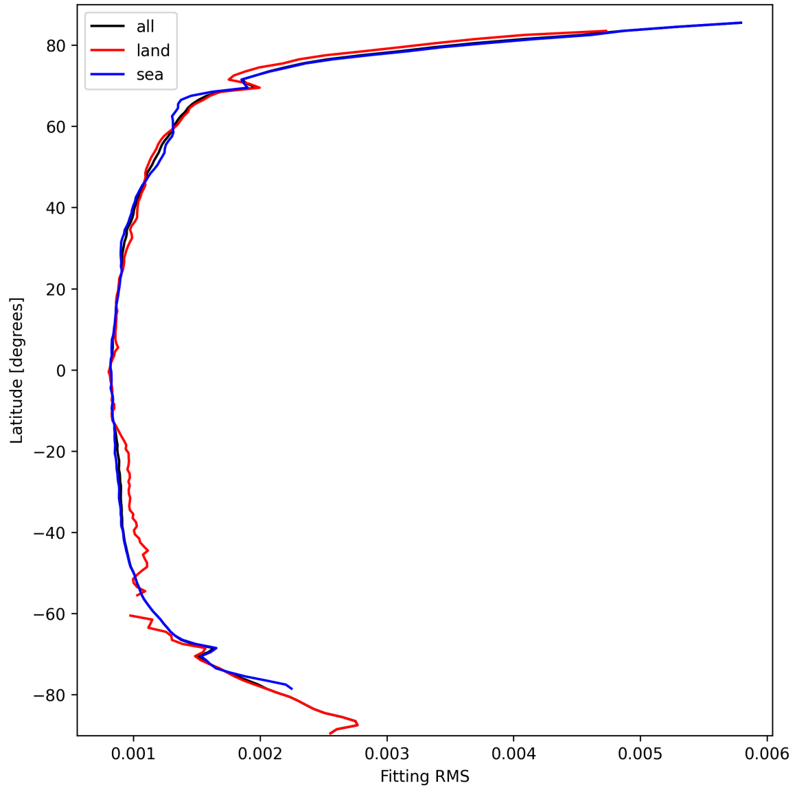
Figure 16: Zonal average of “Fitting RMS” for 2025-03-09 to 2025-03-11.
