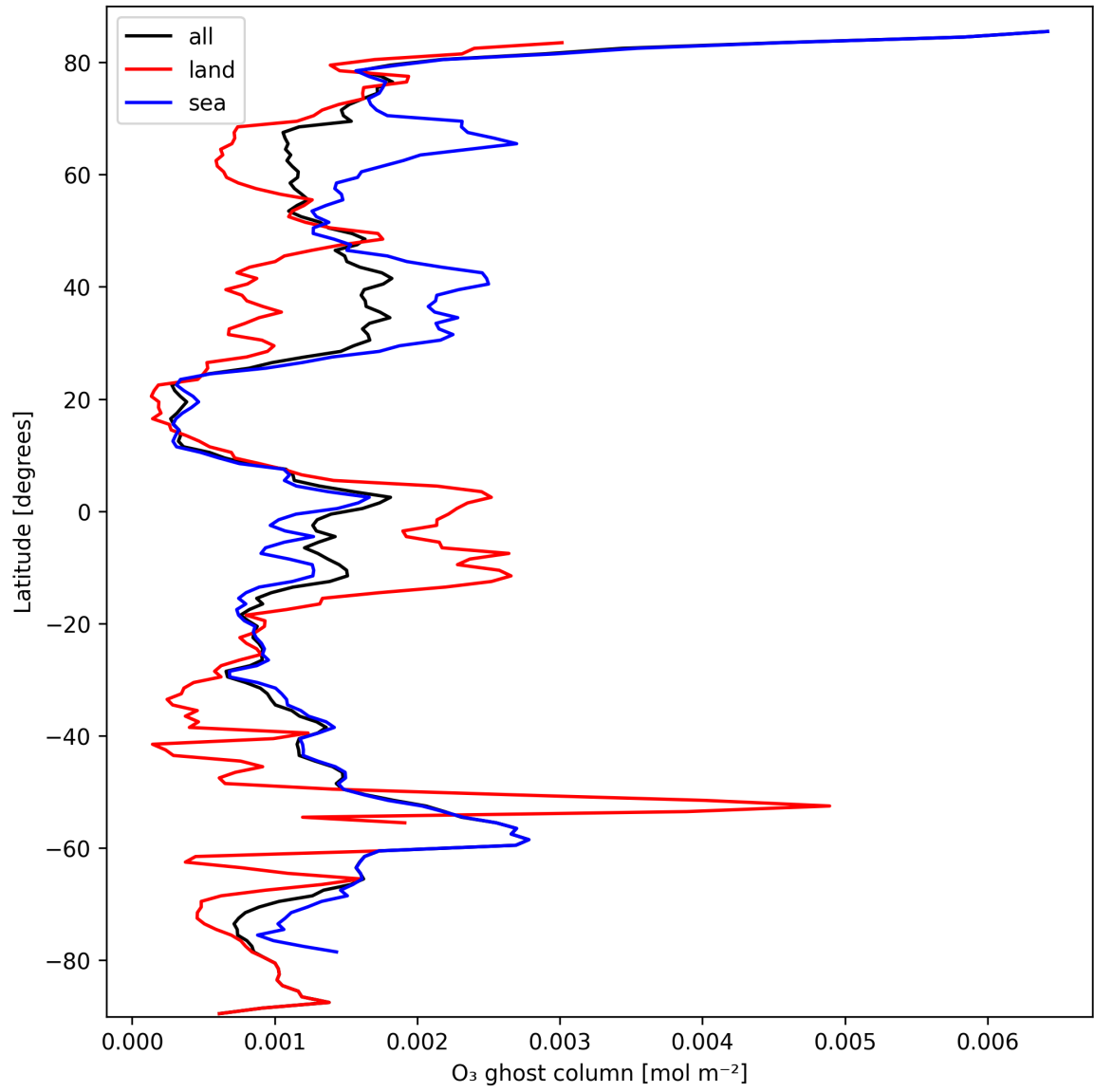
Figure 18: Zonal average of “O 3 ghost column” for 2025-03-09 to 2025-03-11.
