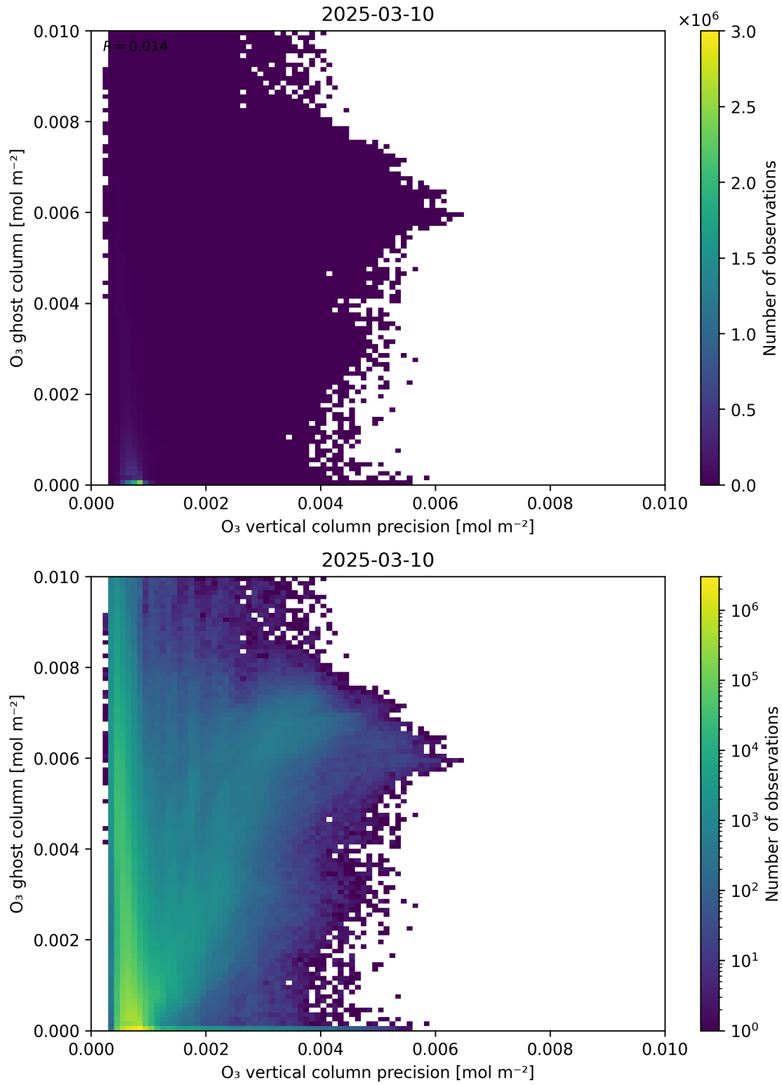
Figure 43: Scatter density plot of “O 3 vertical column precision” against “O 3 ghost column” for 2025-03-09 to 2025-03-11.
