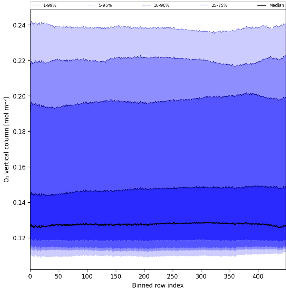
Figure 28: Along track statistics of “ O_3 vertical column” for 2025-03-09 to 2025-03-11
