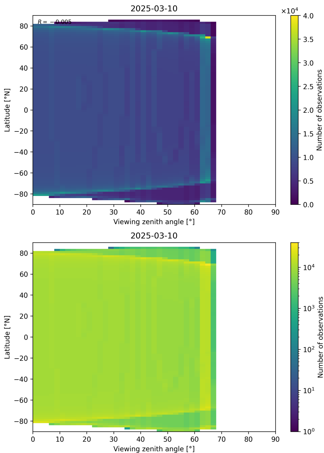
Figure 49: Scatter density plot of “Viewing zenith angle” against “Latitude” for 2025-03-09 to 2025-03-11.
