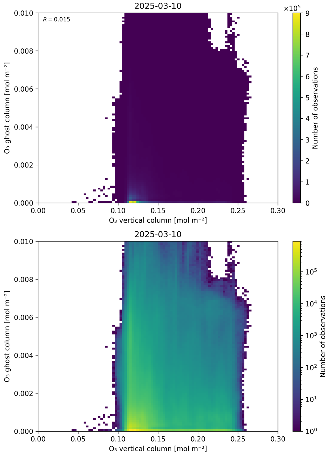
Figure 40: Scatter density plot of “O 3 vertical column” against “O 3 ghost column” for 2025-03-09 to 2025-03-11.
