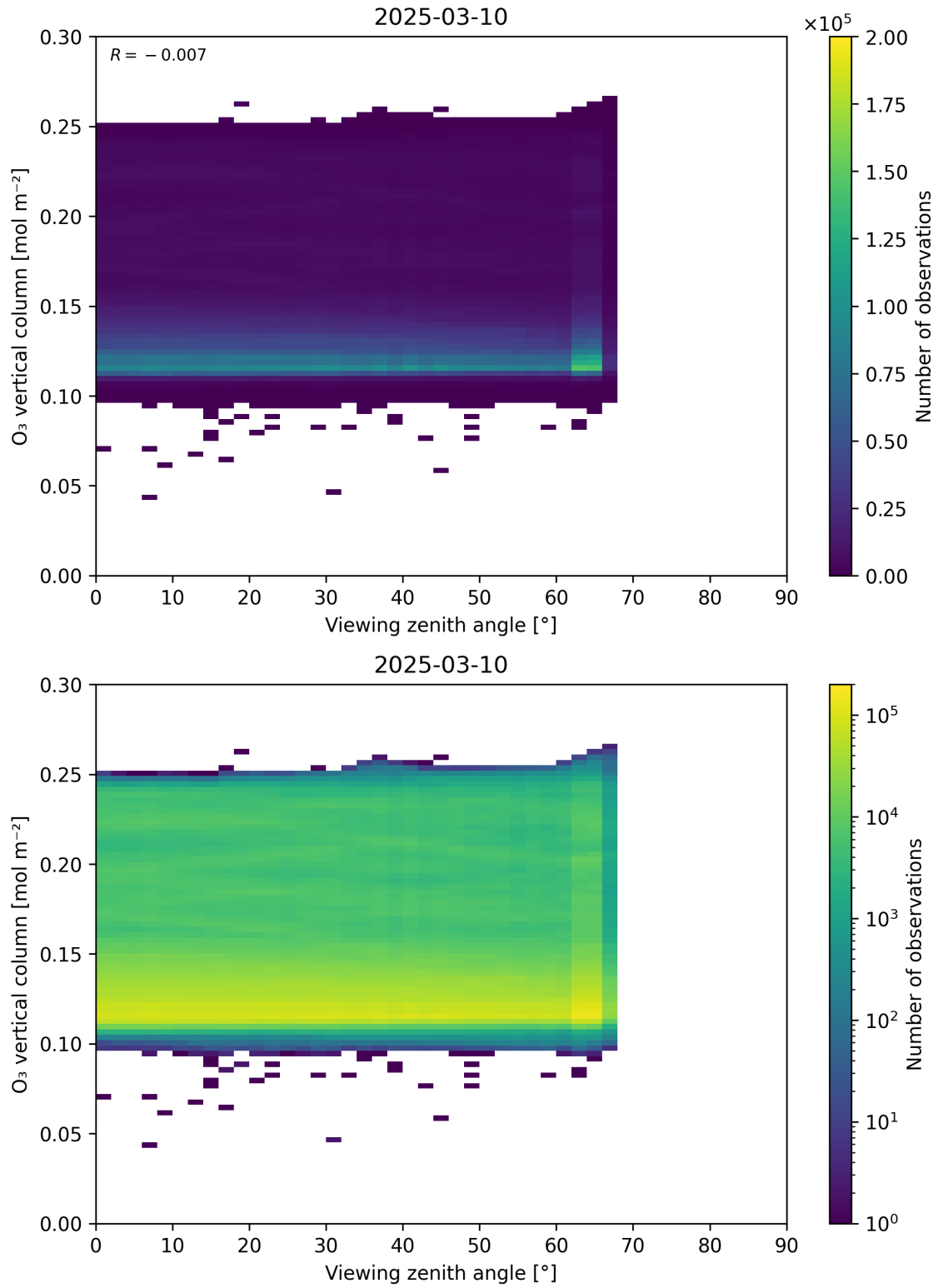
Figure 52: Scatter density plot of “Viewing zenith angle” against “O 3 vertical column” for 2025-03-09 to 2025-03-11.
