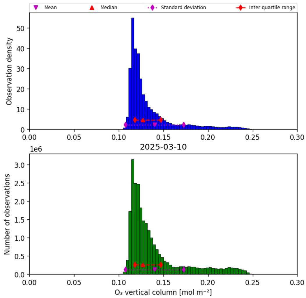
Figure 21: Histogram of “O 3 vertical column” for 2025-03-09 to 2025-03-11
