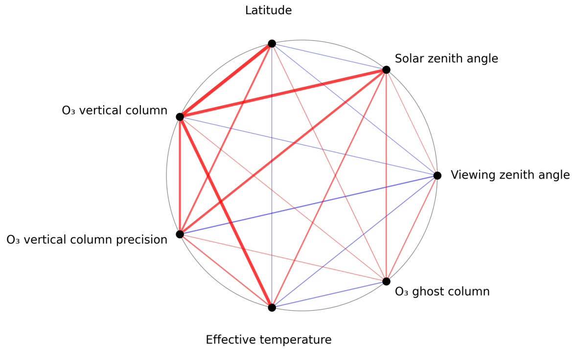
Figure 1: Map of correlation graph for 2025-03-09 to 2025-03-11.
