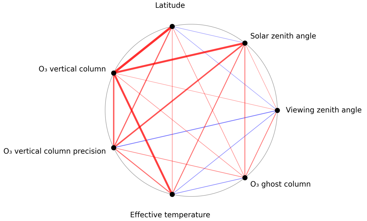
Figure 1: Map of correlation graph for 2025-03-12 to 2025-03-13.
