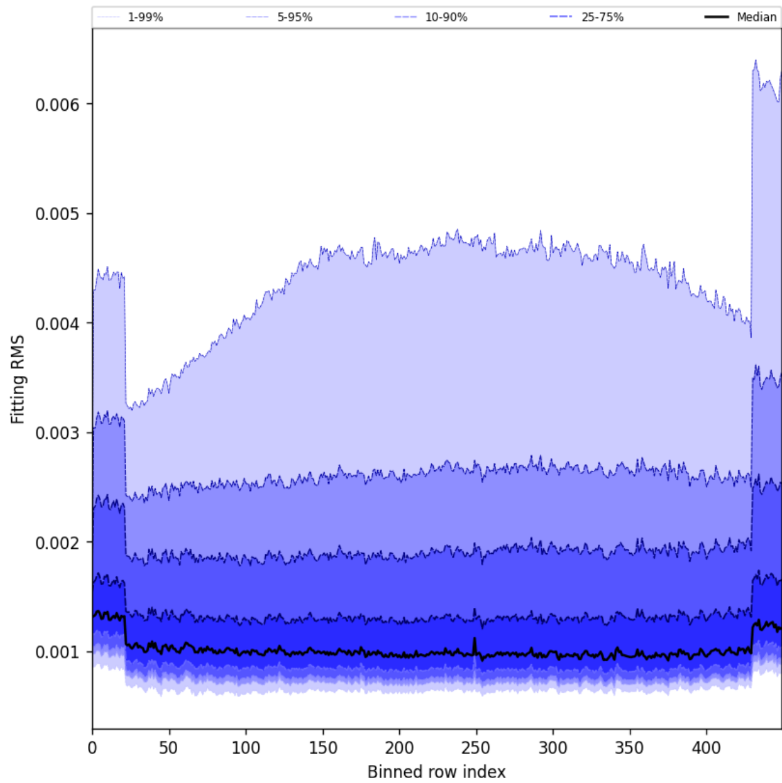
Figure 30: Along track statistics of “Fitting RMS” for 2025-03-12 to 2025-03-13
