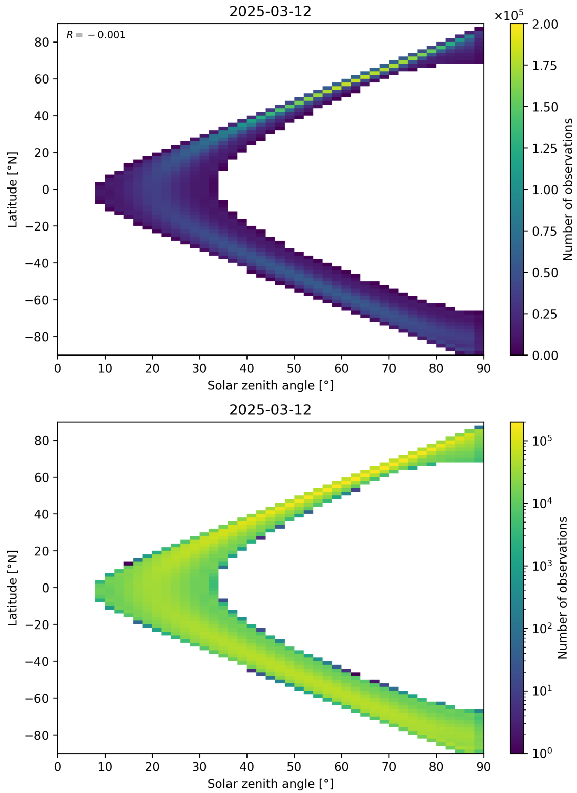
Figure 44: Scatter density plot of “Solar zenith angle” against “Latitude” for 2025-03-12 to 2025-03-13.
