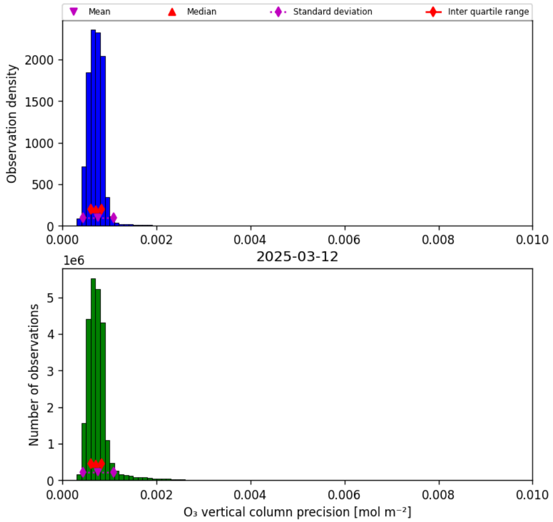
Figure 22: Histogram of “O 3 vertical column precision” for 2025-03-12 to 2025-03-13
