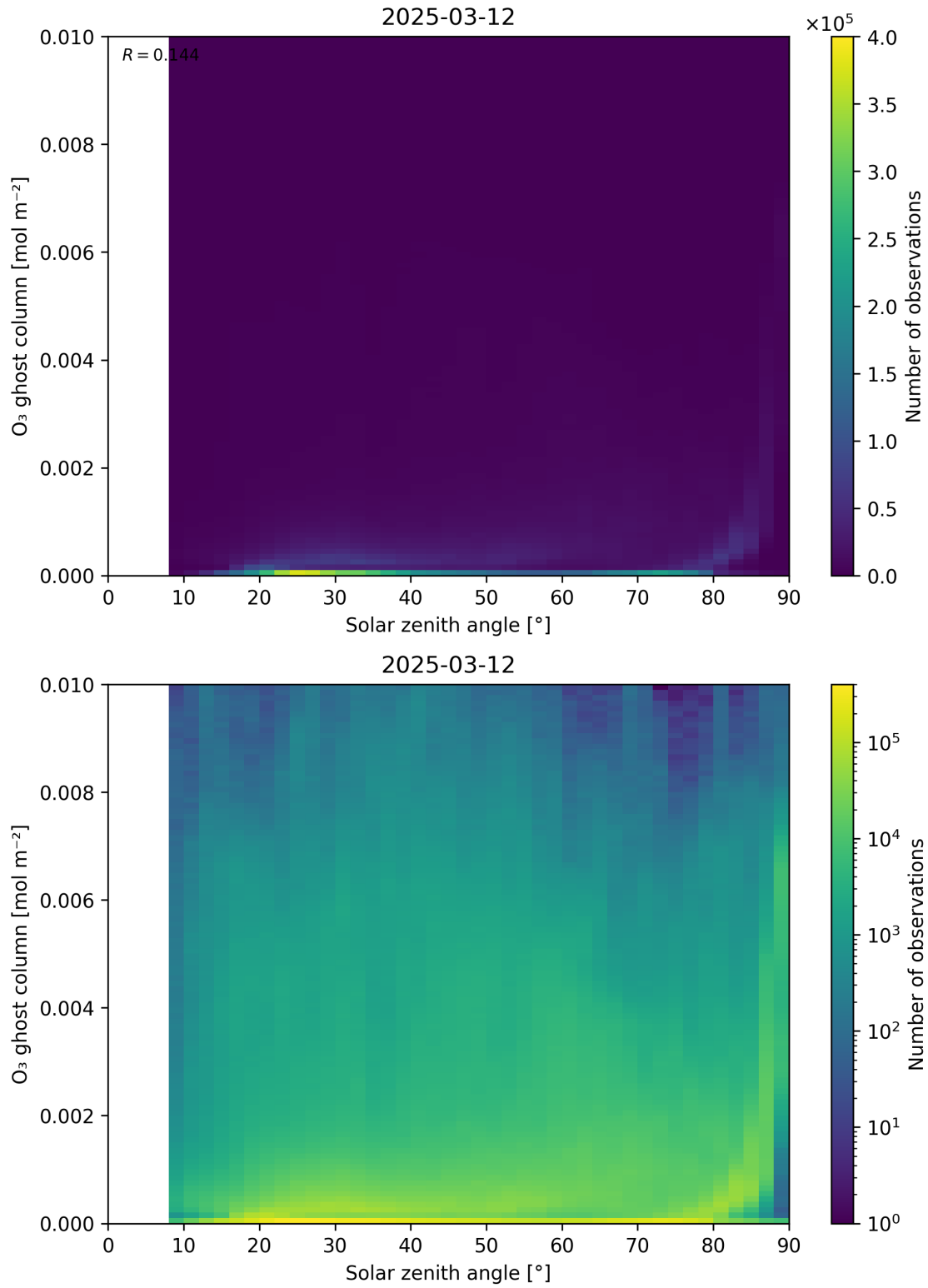
Figure 46: Scatter density plot of “Solar zenith angle” against “O 3 ghost column” for 2025-03-12 to 2025-03-13.
