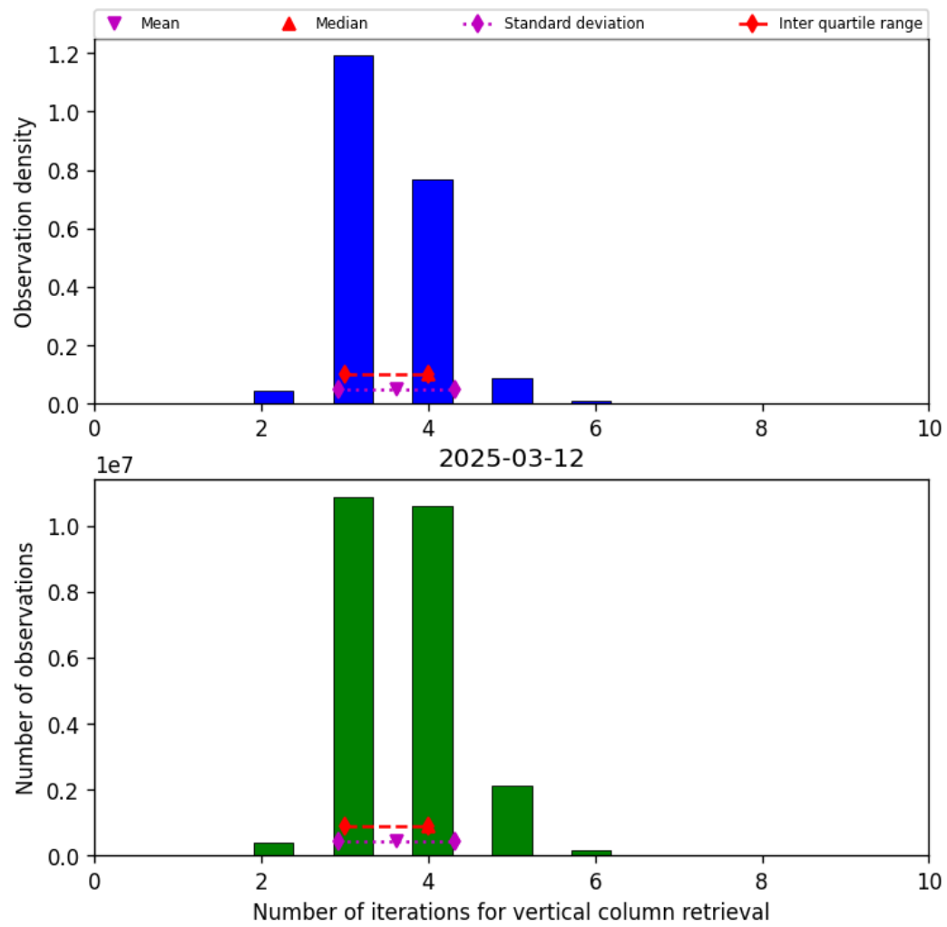
Figure 26: Histogram of “Number of iterations for vertical column retrieval” for 2025-03-12 to 2025-03-13
