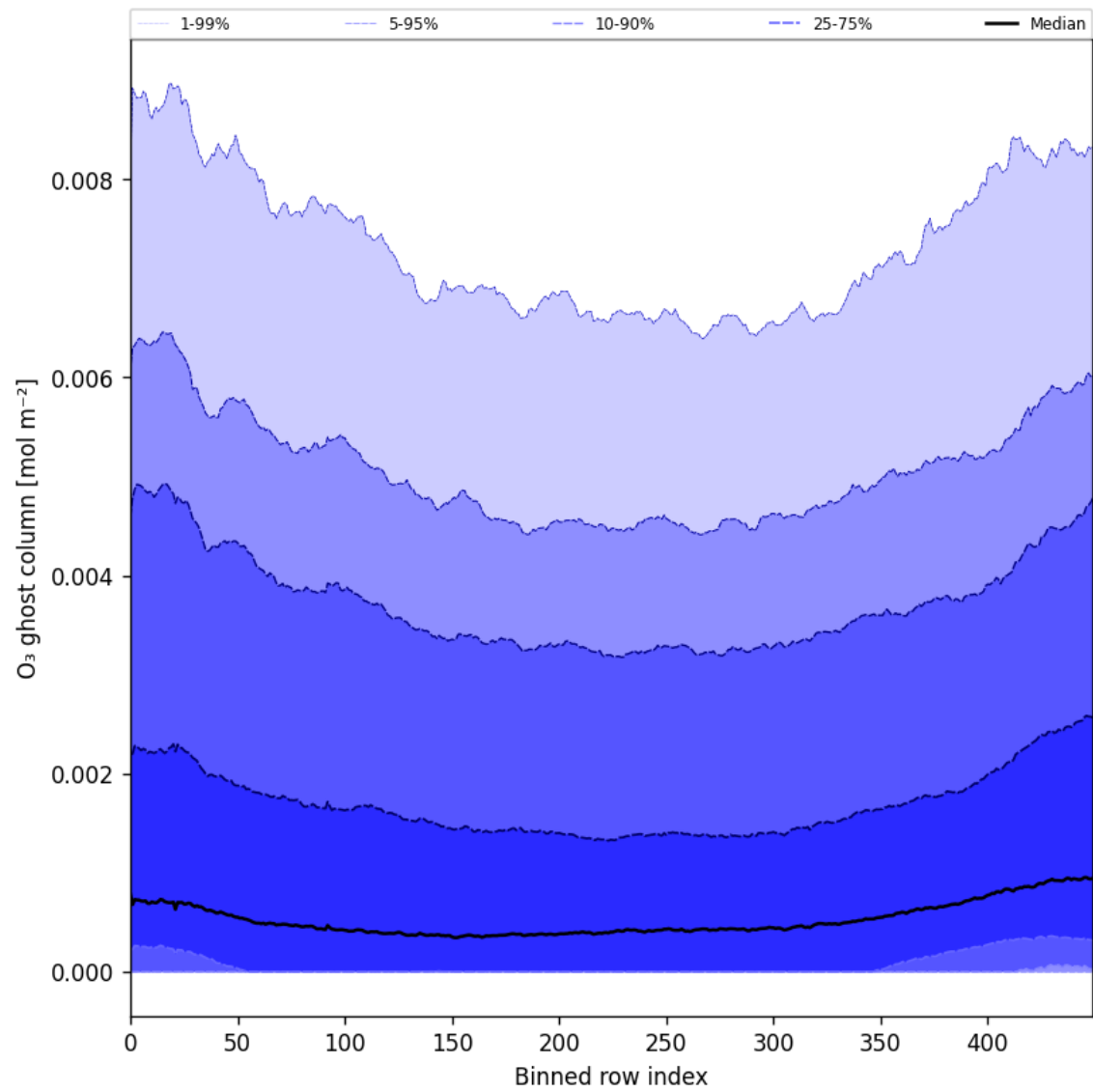
Figure 32: Along track statistics of “O 3 ghost column” for 2025-03-12 to 2025-03-13
