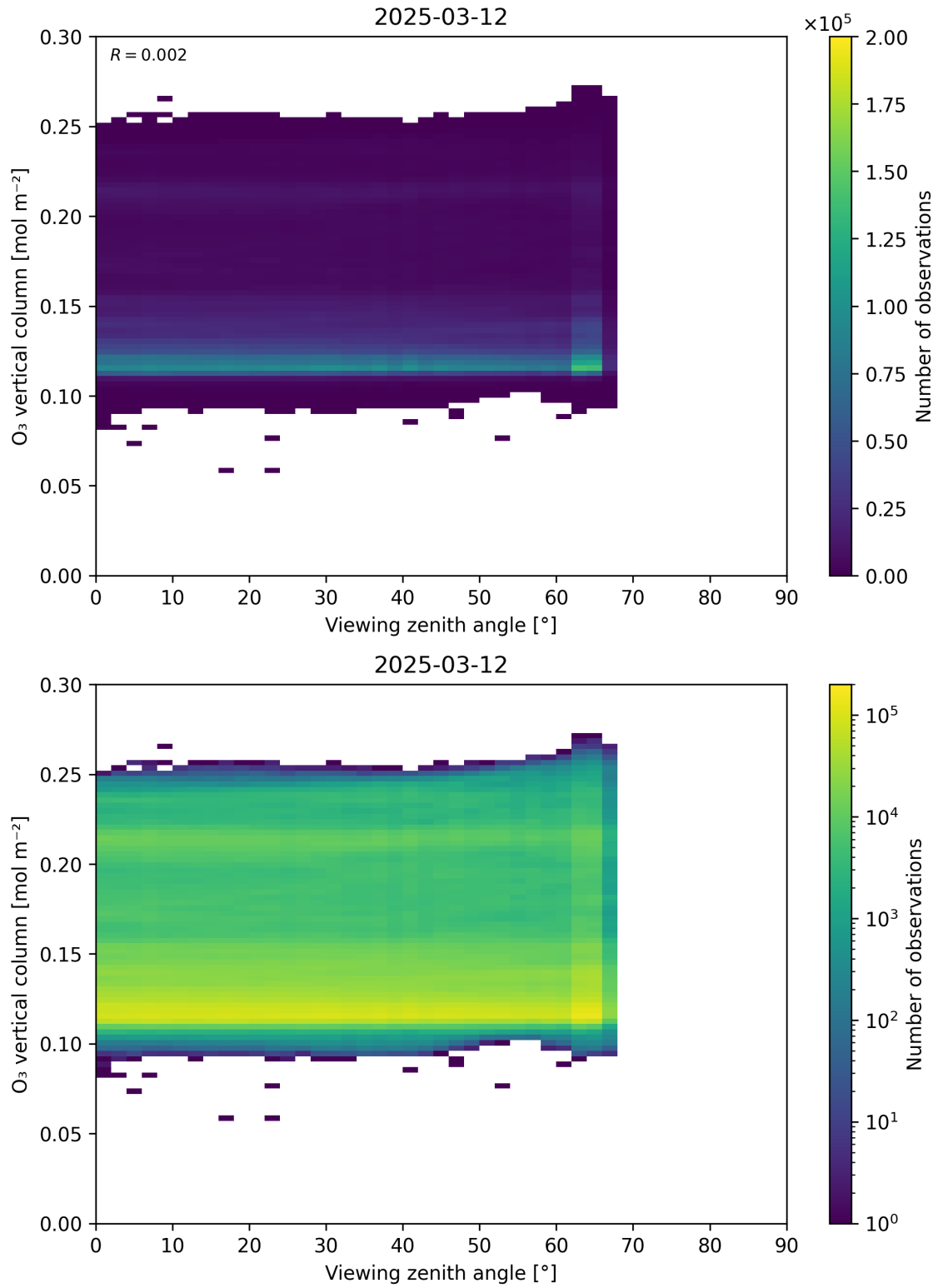
Figure 52: Scatter density plot of “Viewing zenith angle” against “O 3 vertical column” for 2025-03-12 to 2025-03-13.
