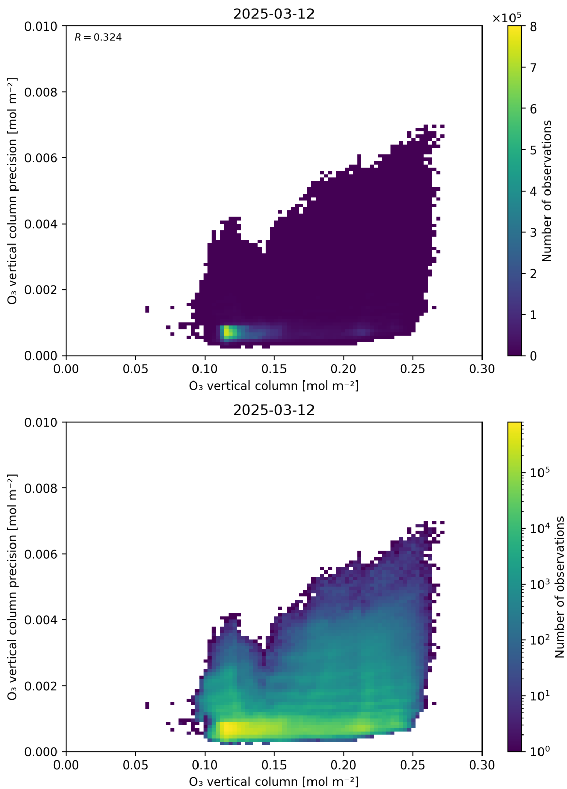
Figure 41: Scatter density plot of “O 3 vertical column” against “O 3 vertical column precision” for 2025-03-12 to 2025-03-13.
