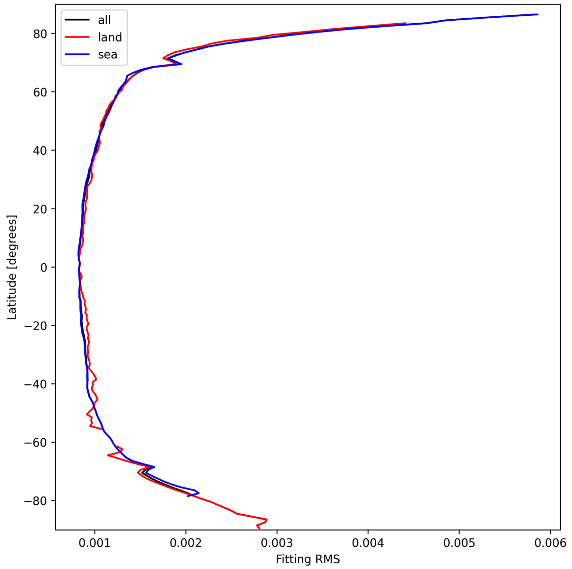
Figure 16: Zonal average of “Fitting RMS” for 2025-03-12 to 2025-03-13.
