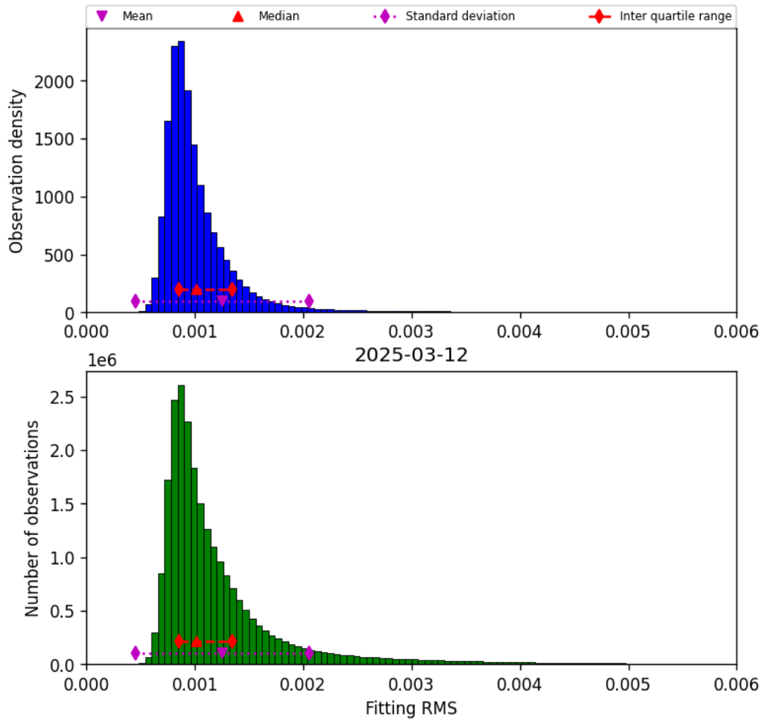
Figure 23: Histogram of “Fitting RMS” for 2025-03-12 to 2025-03-13
