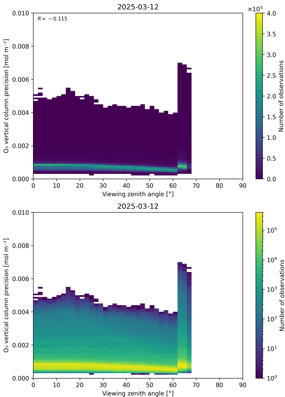
Figure 53: Scatter density plot of “Viewing zenith angle” against “O 3 vertical column precision” for 2025-03-12 to 2025-03-13.
