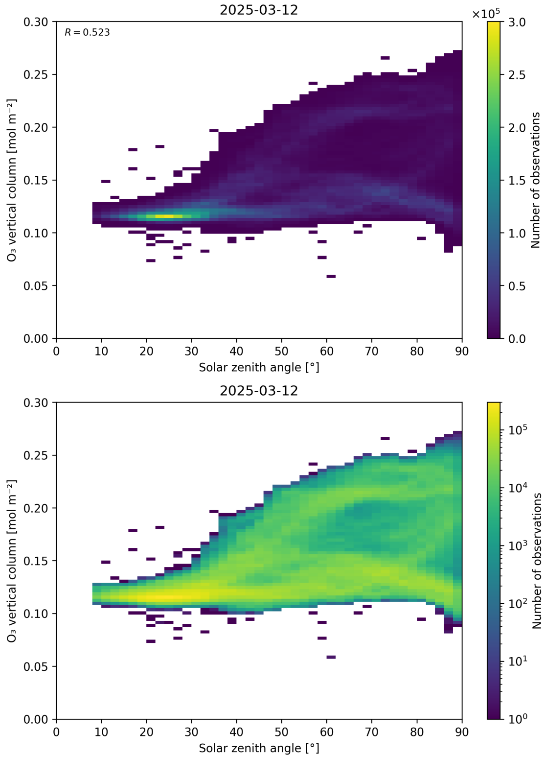
Figure 47: Scatter density plot of “Solar zenith angle” against “O 3 vertical column” for 2025-03-12 to 2025-03-13.
