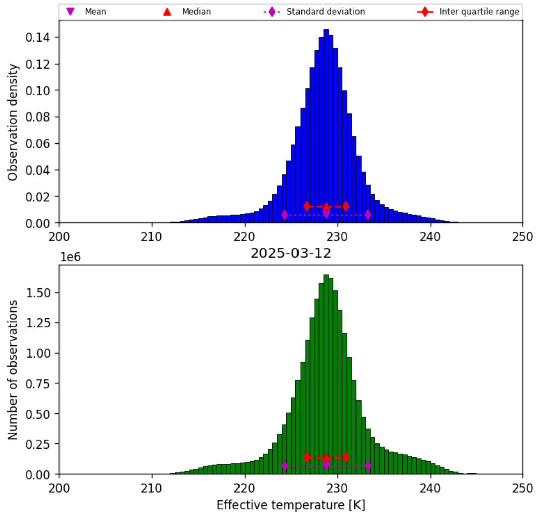
Figure 24: Histogram of “Effective temperature” for 2025-03-12 to 2025-03-13
