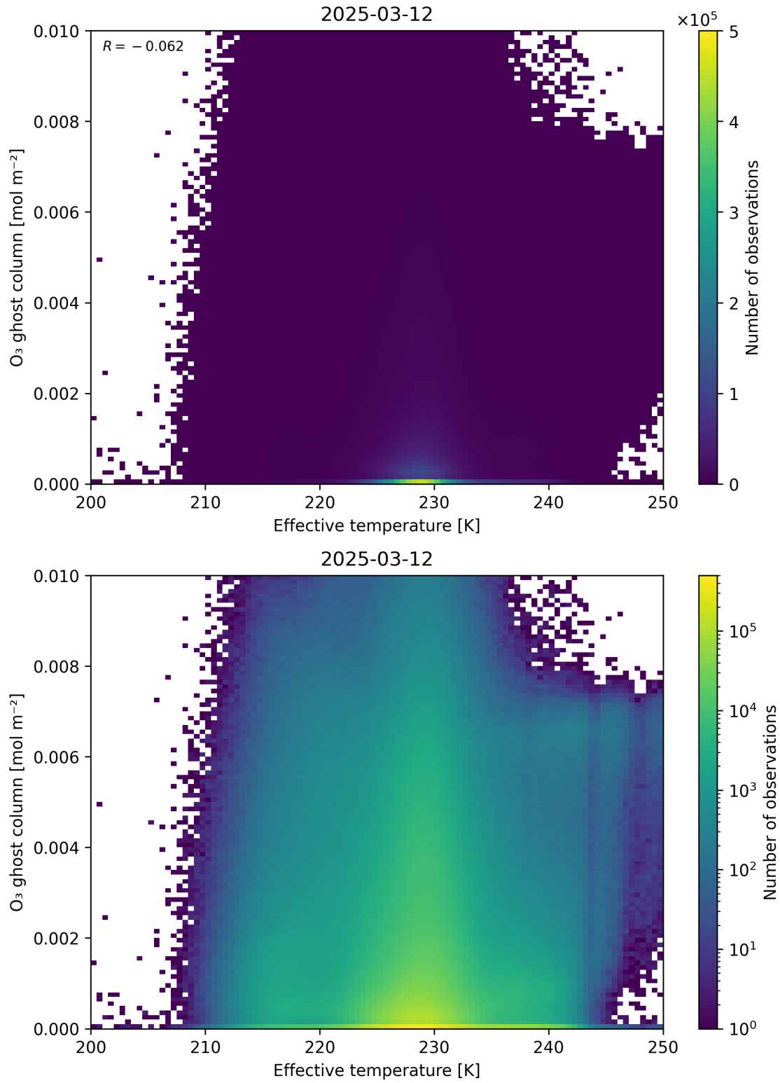
Figure 38: Scatter density plot of “Effective temperature” against “O 3 ghost column” for 2025-03-12 to 2025-03-13.
