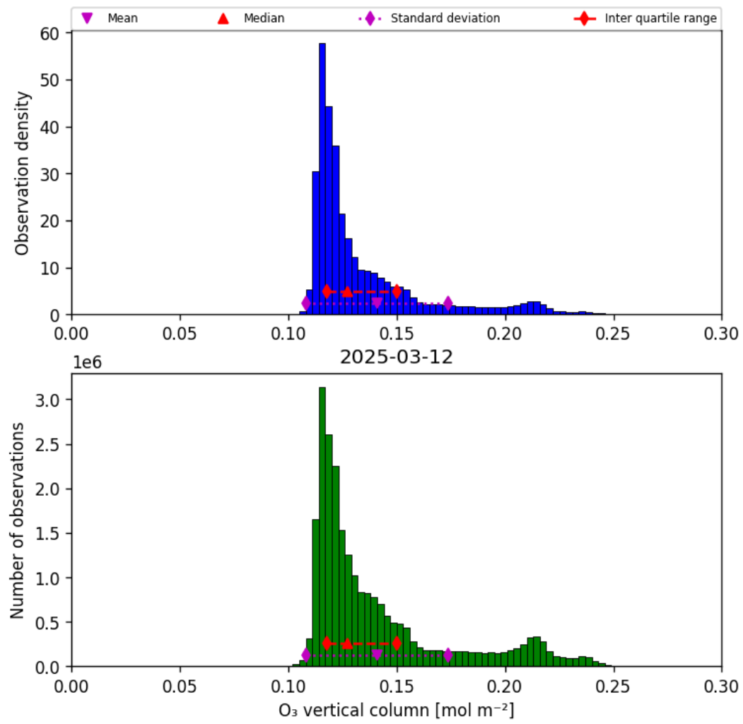
Figure 21: Histogram of “O 3 vertical column” for 2025-03-12 to 2025-03-13
