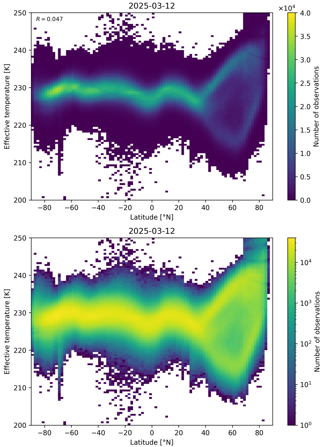
Figure 34: Scatter density plot of “Latitude” against “Effective temperature” for 2025-03-12 to 2025-03-13.
