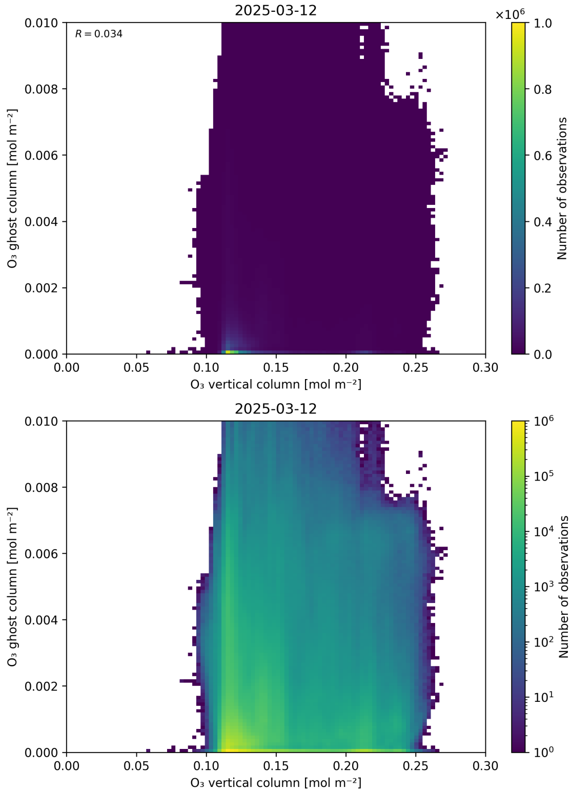
Figure 40: Scatter density plot of “O 3 vertical column” against “O 3 ghost column” for 2025-03-12 to 2025-03-13.
