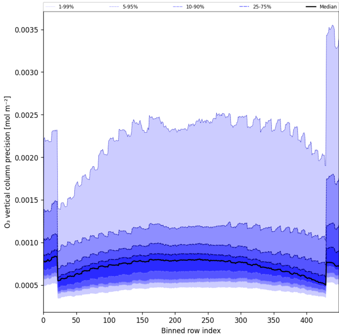
Figure 29: Along track statistics of “O 3 vertical column precision” for 2025-03-12 to 2025-03-13
