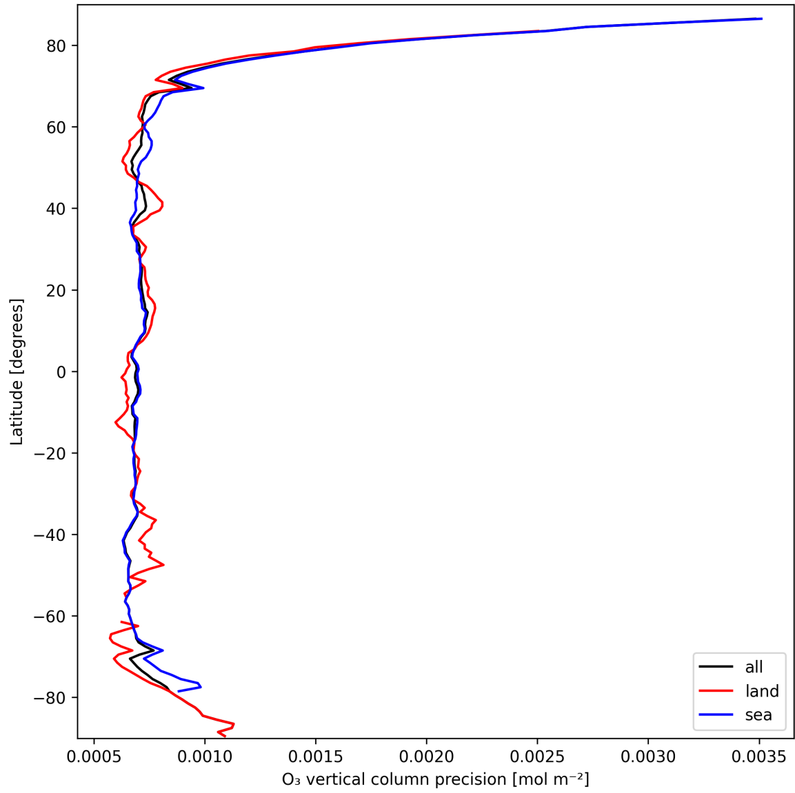
Figure 15: Zonal average of “O 3 vertical column precision” for 2025-03-12 to 2025-03-13.
