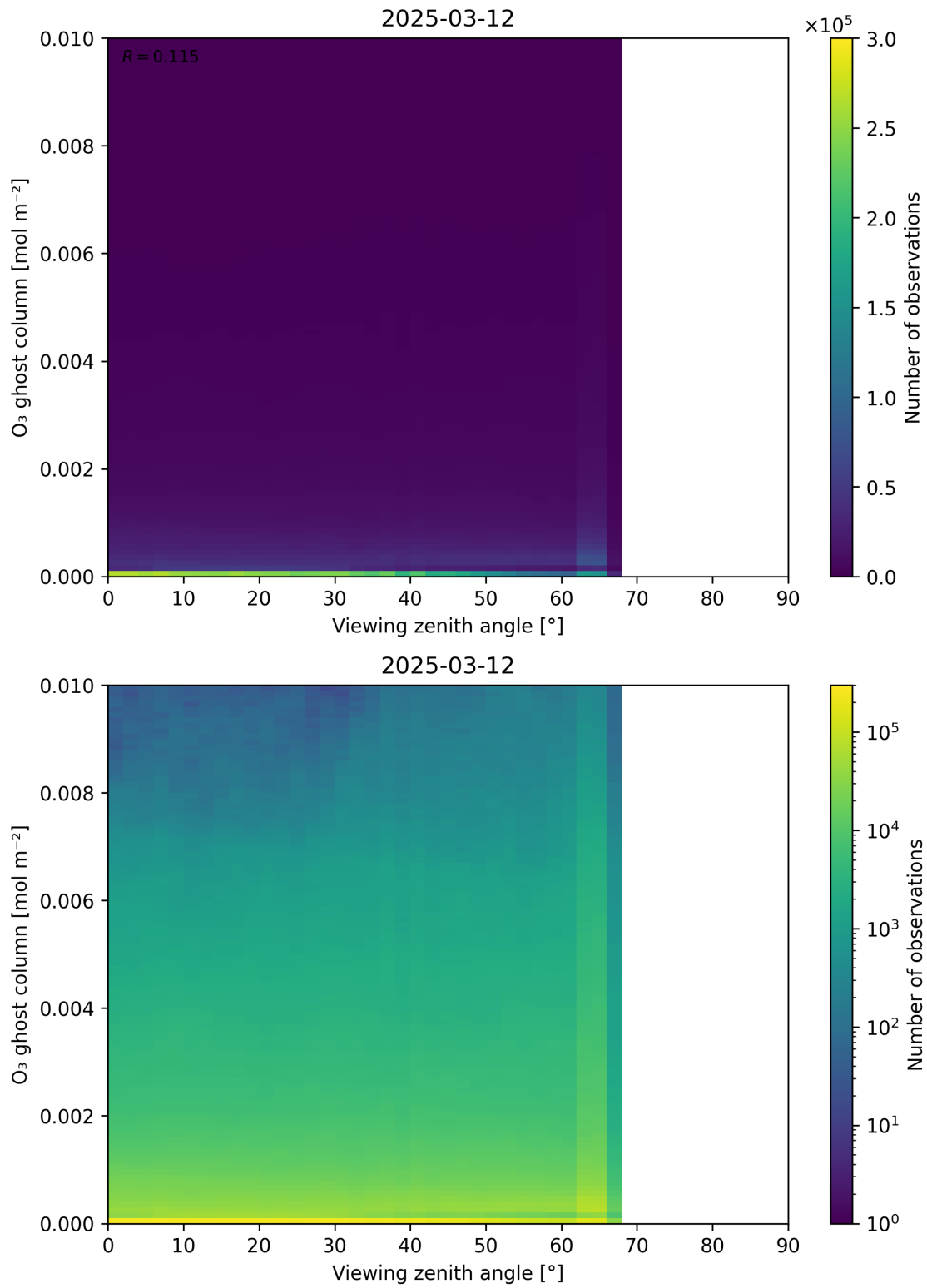
Figure 51: Scatter density plot of “Viewing zenith angle” against “O 3 ghost column” for 2025-03-12 to 2025-03-13.
