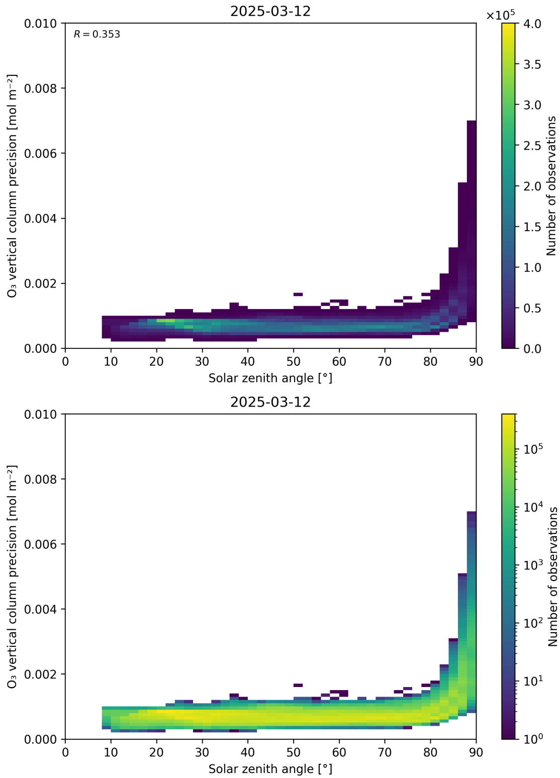
Figure 48: Scatter density plot of “Solar zenith angle” against “O 3 vertical column precision” for 2025-03-12 to 2025-03-13.
