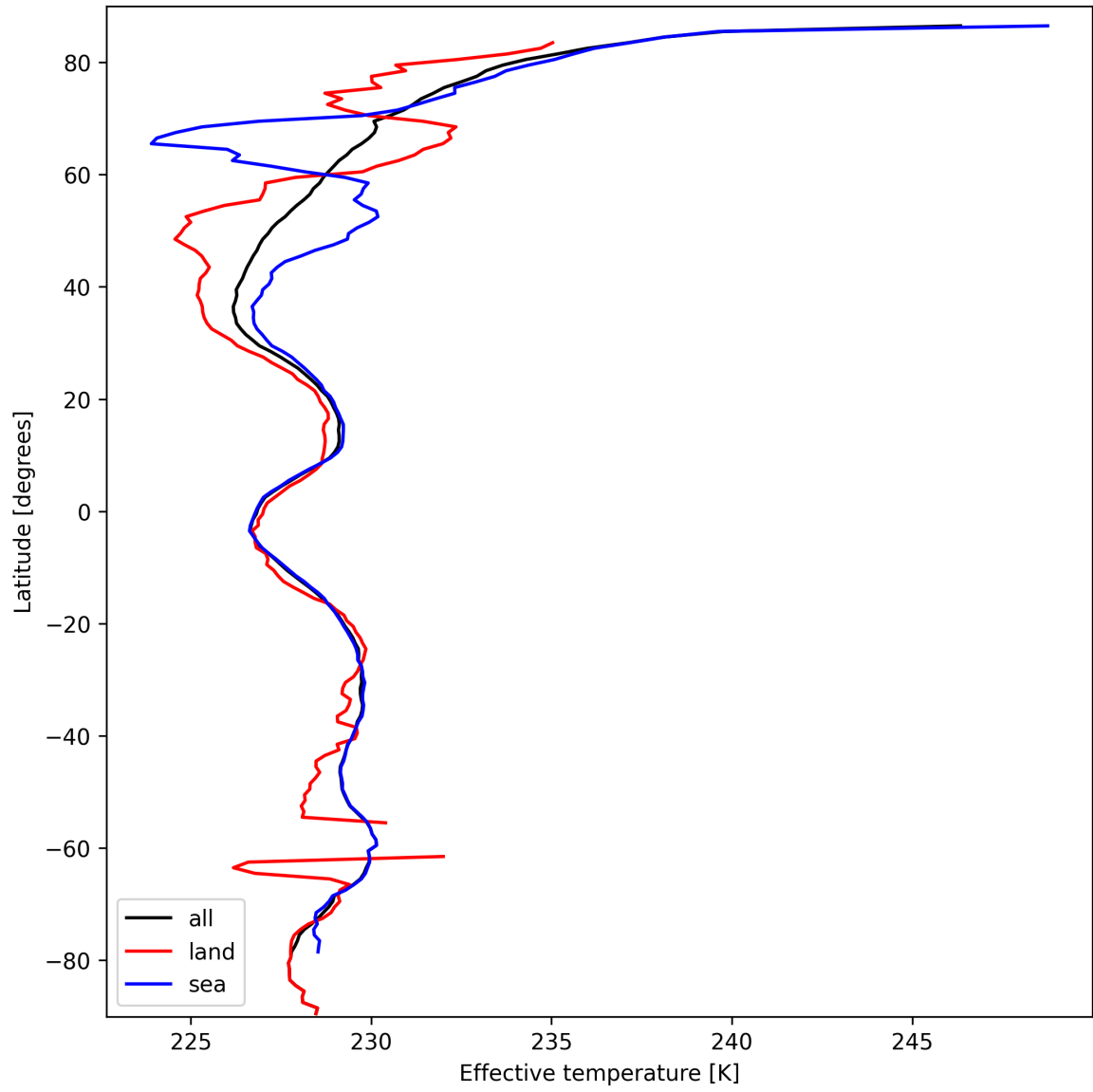
Figure 17: Zonal average of “Effective temperature” for 2025-03-12 to 2025-03-13.
