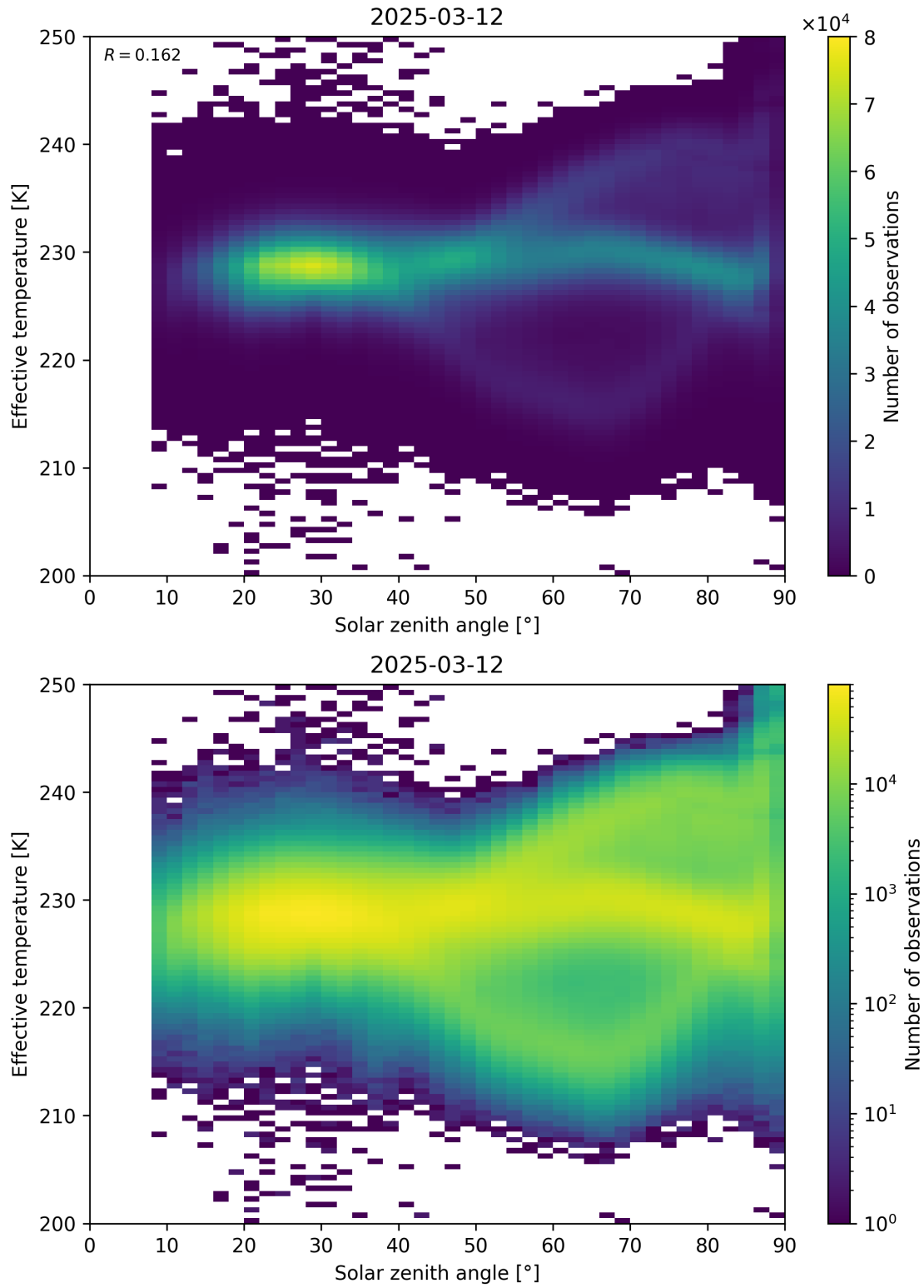
Figure 45: Scatter density plot of “Solar zenith angle” against “Effective temperature” for 2025-03-12 to 2025-03-13.
