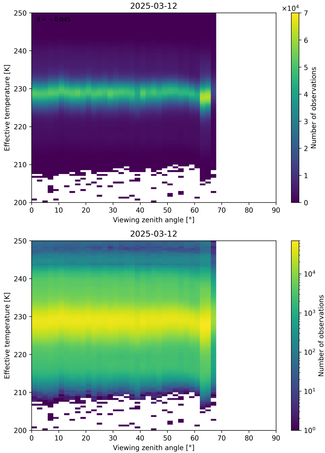
Figure 50: Scatter density plot of “Viewing zenith angle” against “Effective temperature” for 2025-03-12 to 2025-03-13.
