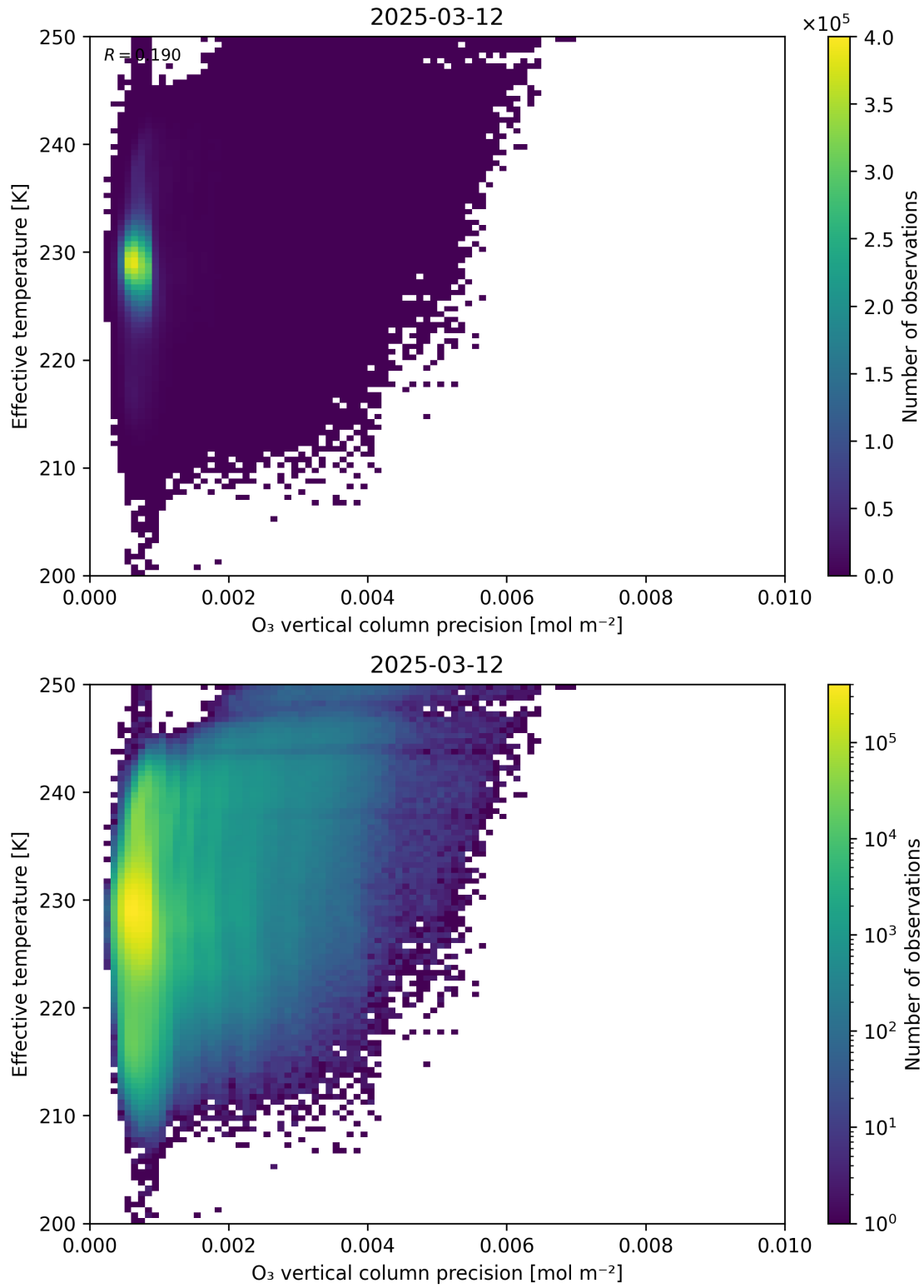
Figure 42: Scatter density plot of “O 3 vertical column precision” against “Effective temperature” for 2025-03-12 to 2025-03-13.
