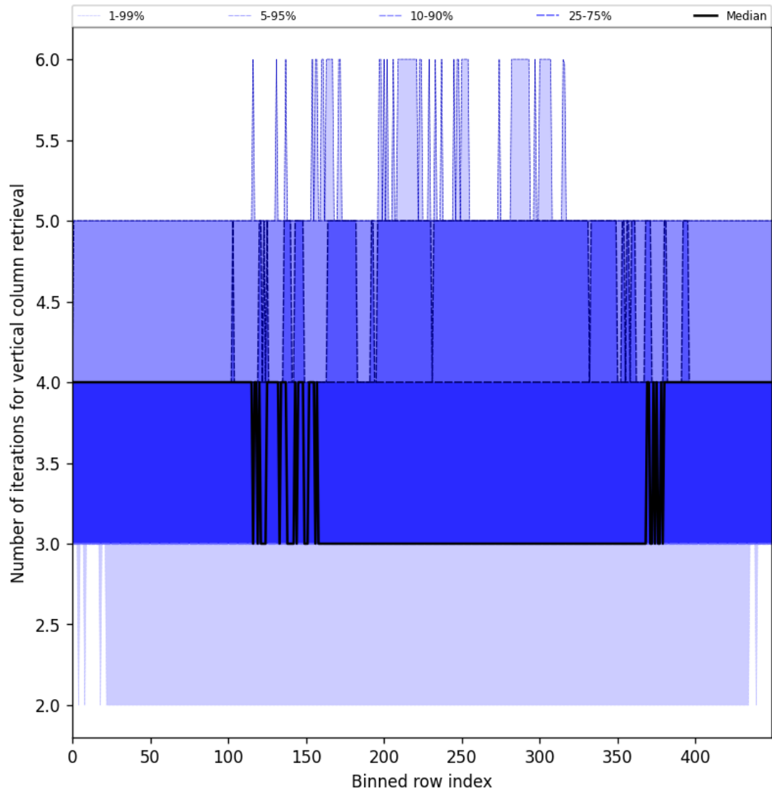
Figure 33: Along track statistics of “Number of iterations for vertical column retrieval” for 2025-03-12 to 2025-03-13
