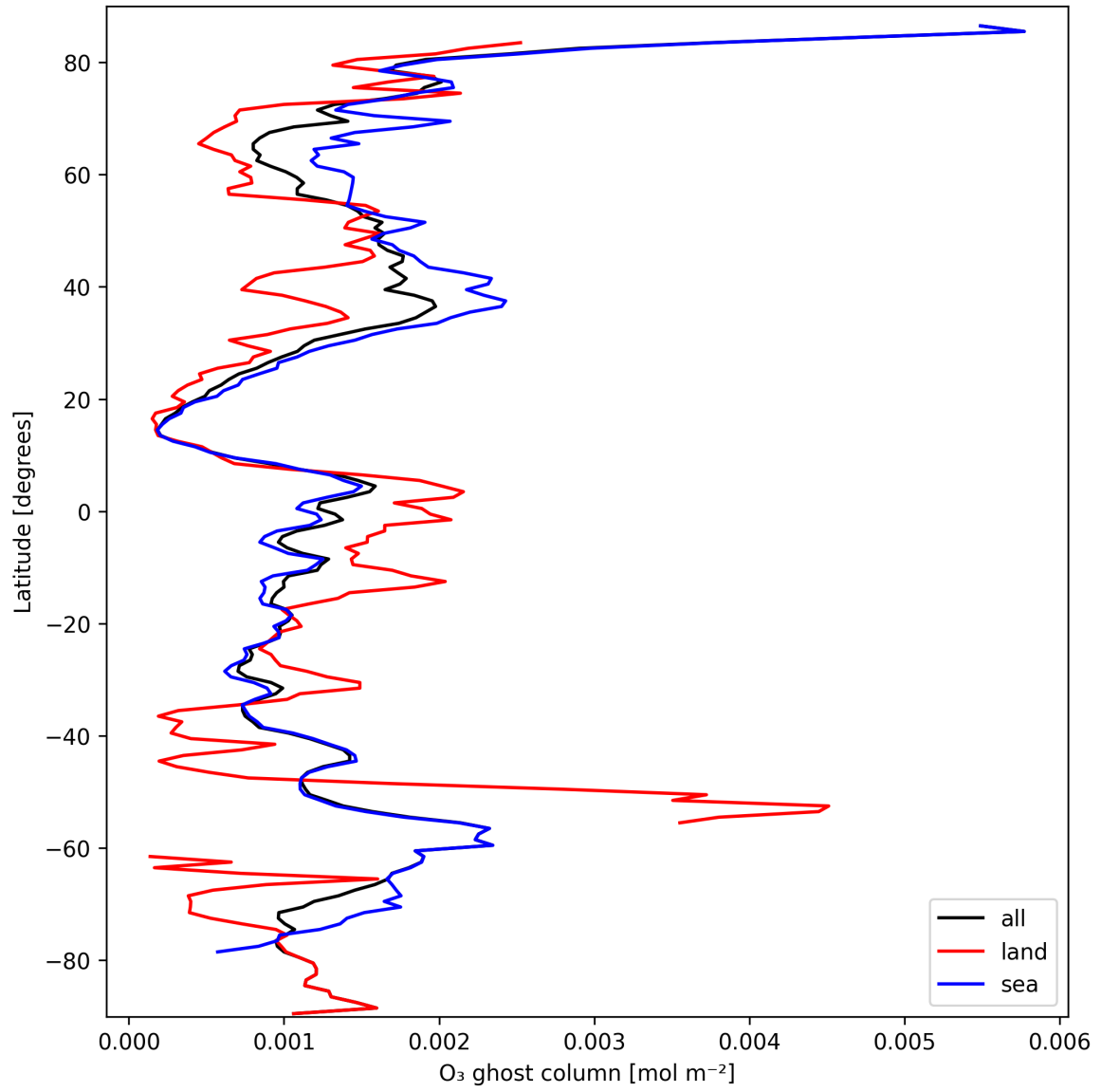
Figure 18: Zonal average of "O 3 ghost column" for 2025-03-12 to 2025-03-13.
