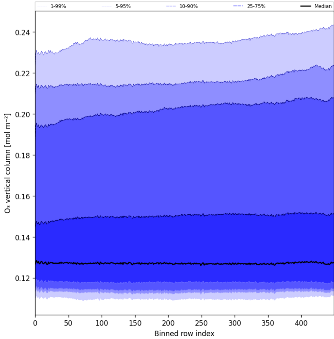
Figure 28: Along track statistics of "O 3 vertical column" for 2025-03-12 to 2025-03-13
