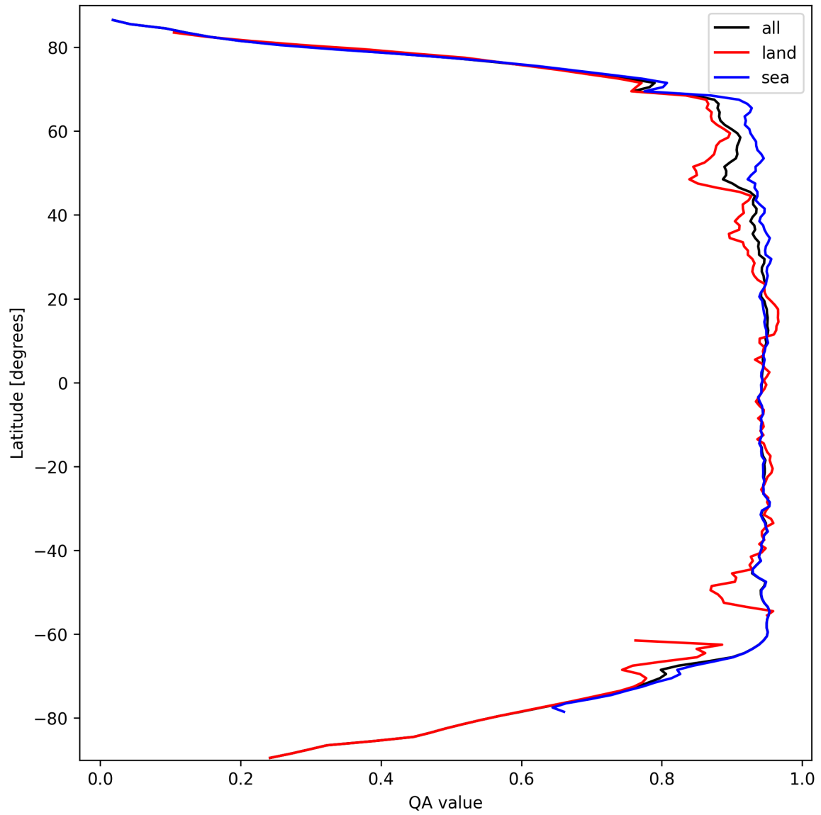
Figure 13: Zonal average of “QA value” for 2025-03-12 to 2025-03-13.
