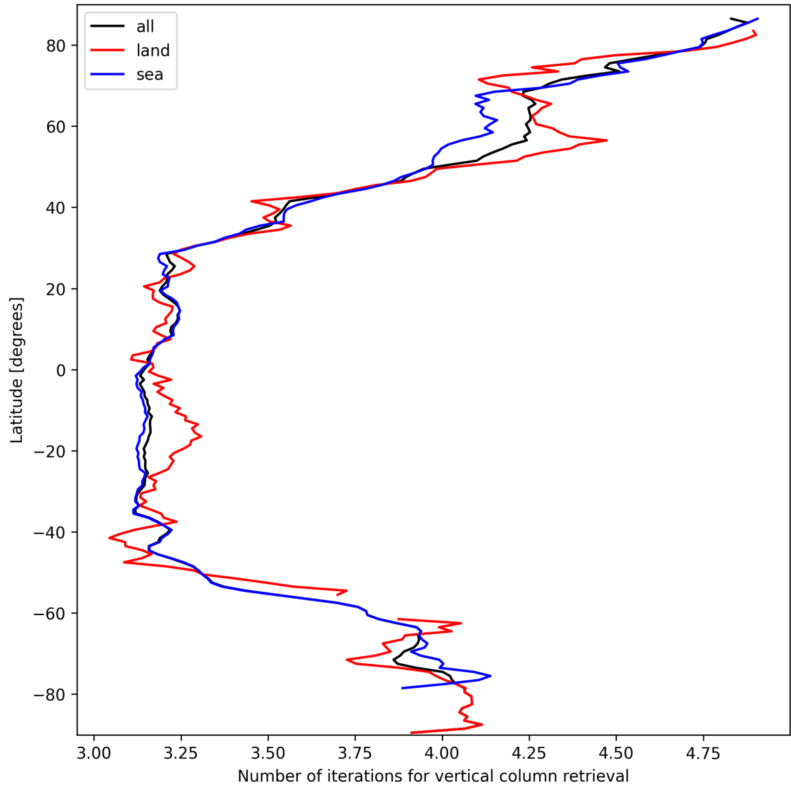
Figure 19: Zonal average of “Number of iterations for vertical column retrieval” for 2025-03-12 to 2025-03-13.
