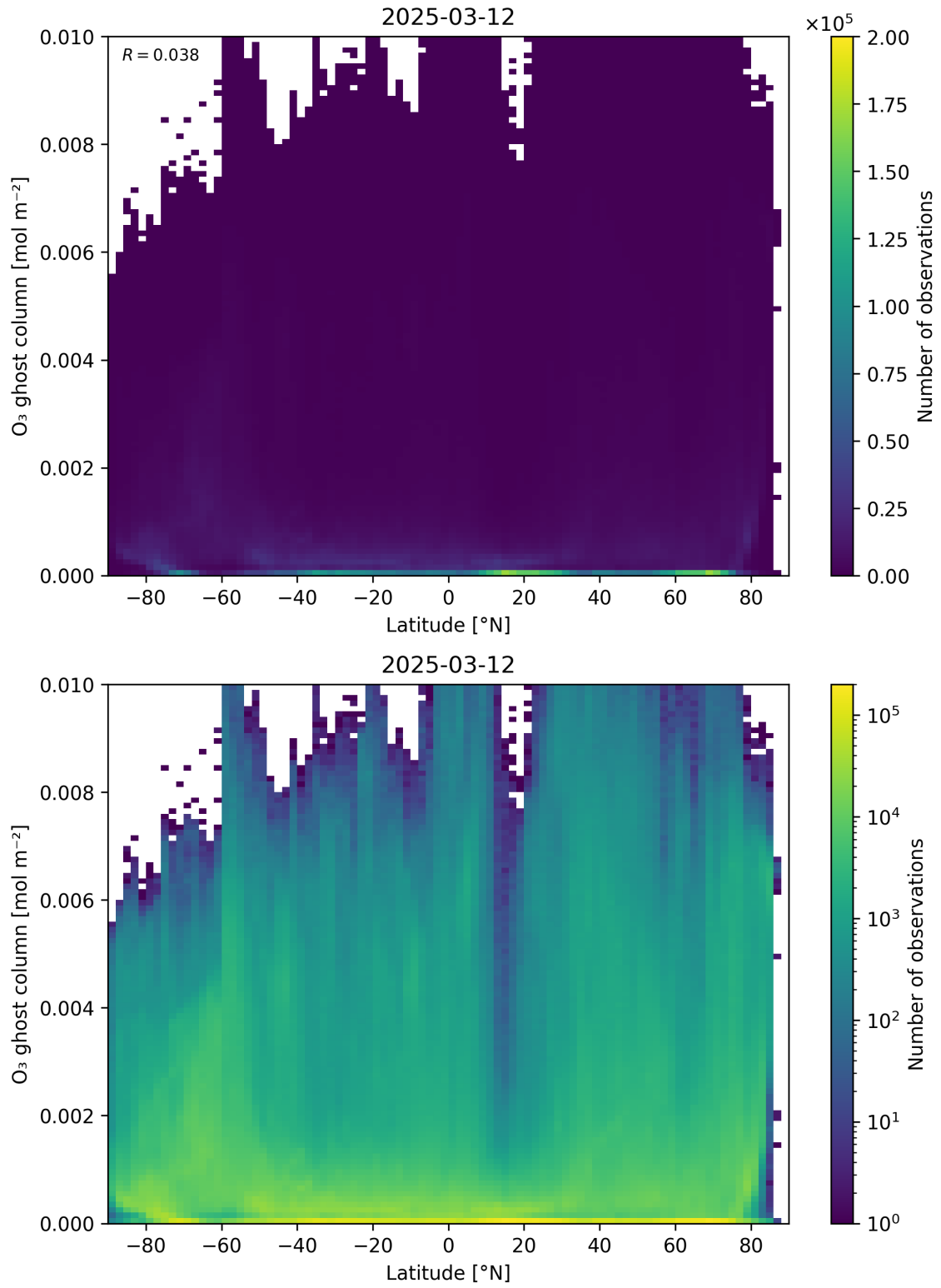
Figure 35: Scatter density plot of “Latitude” against “O 3 ghost column” for 2025-03-12 to 2025-03-13.
