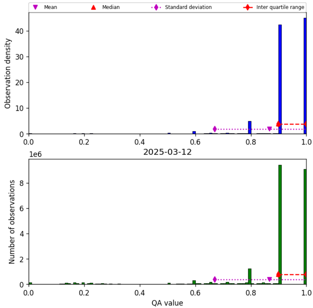
Figure 20: Histogram of “QA value” for 2025-03-12 to 2025-03-13
