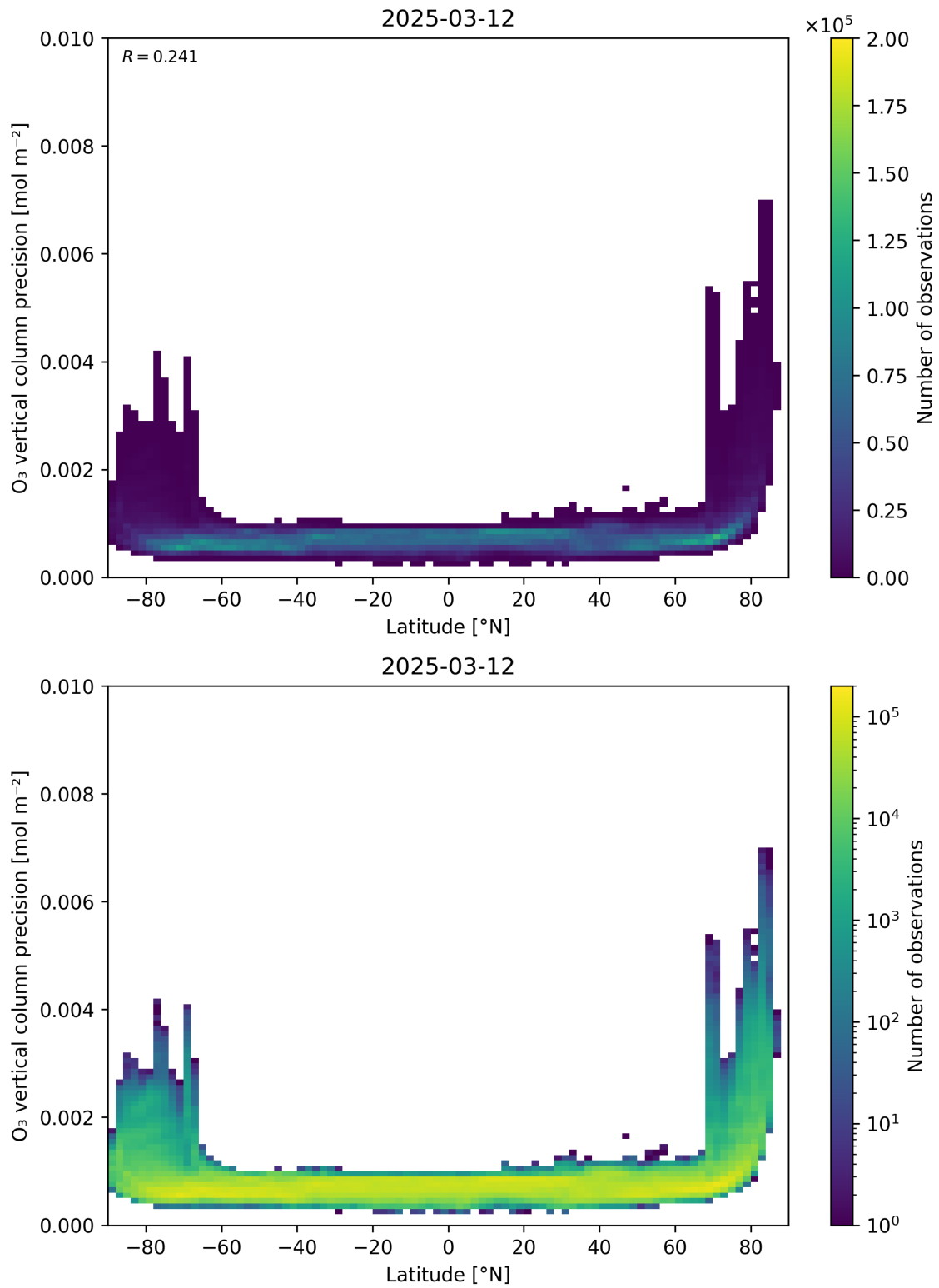
Figure 37: Scatter density plot of “Latitude” against “O 3 vertical column precision” for 2025-03-12 to 2025-03-13.
