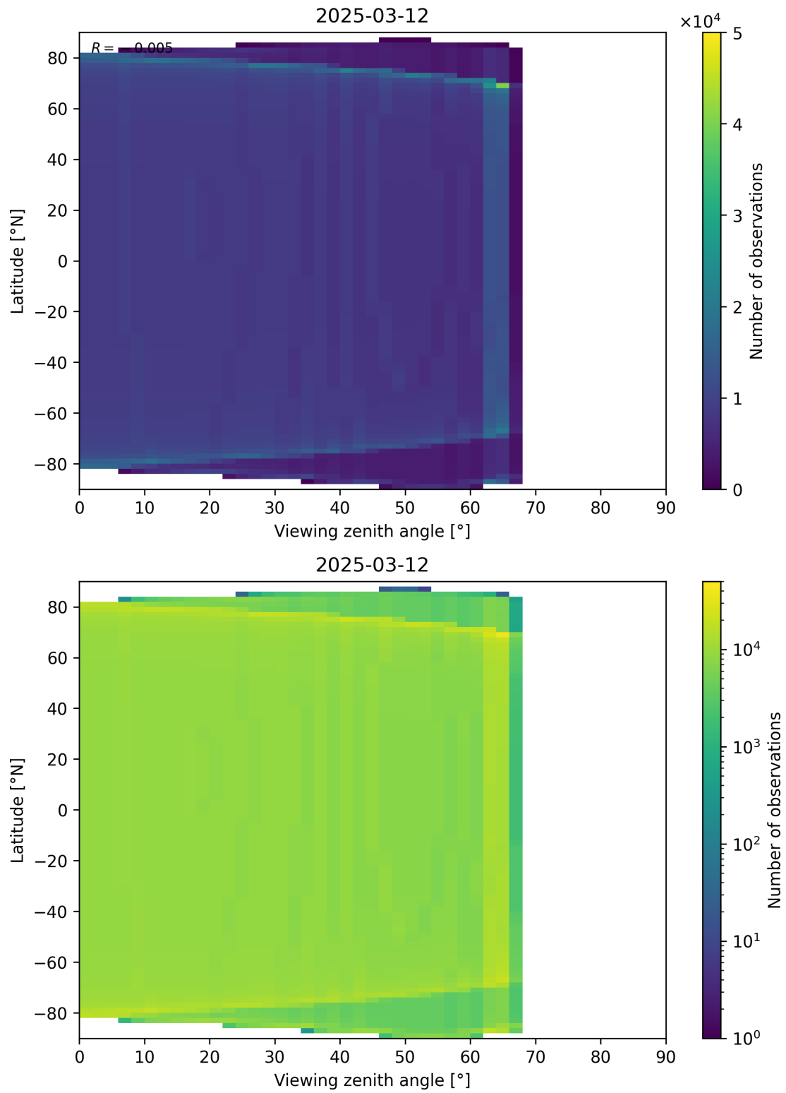
Figure 49: Scatter density plot of “Viewing zenith angle” against “Latitude” for 2025-03-12 to 2025-03-13.
