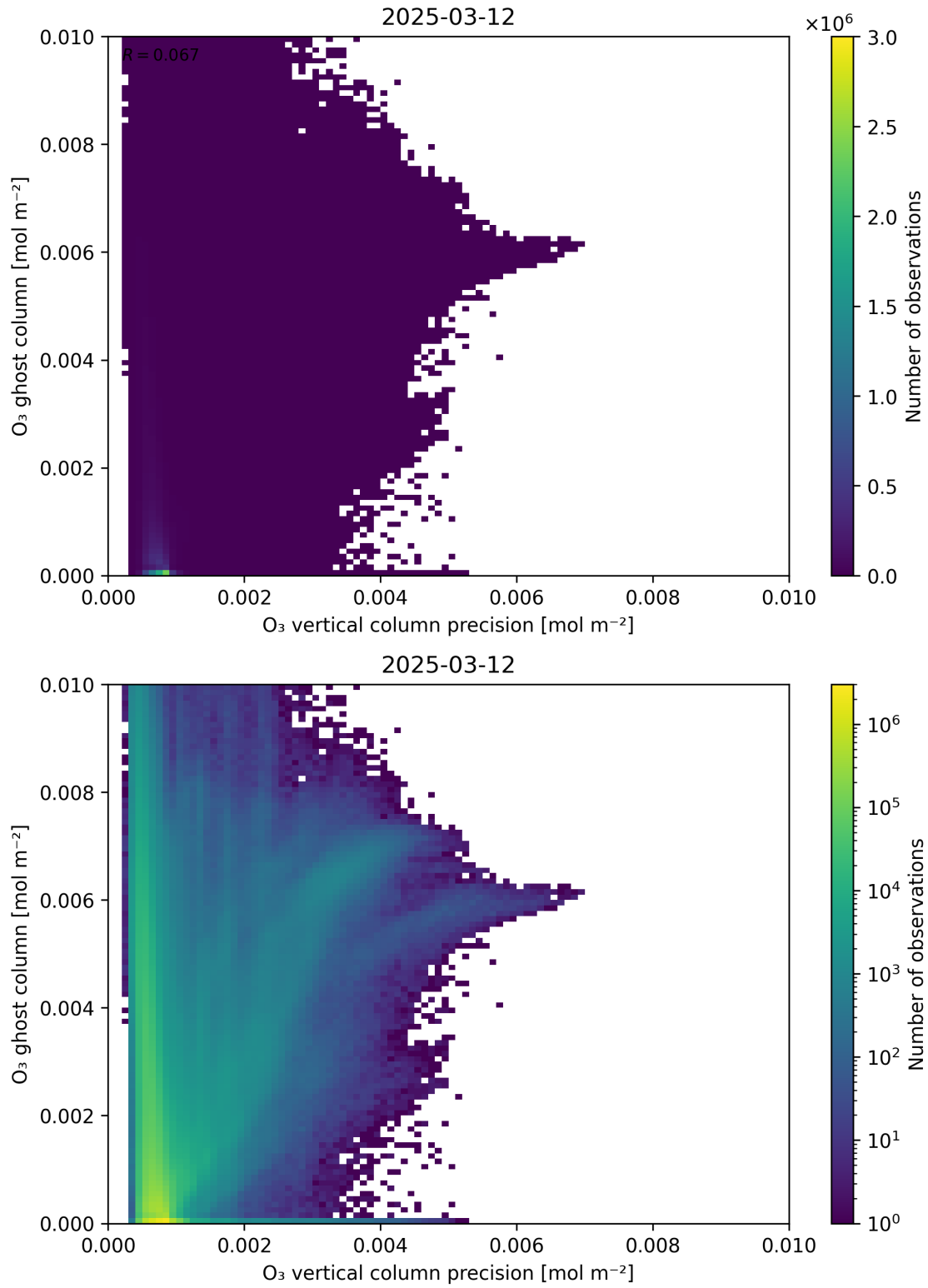
Figure 43: Scatter density plot of “O 3 vertical column precision” against “O 3 ghost column” for 2025-03-12 to 2025-03-13.
