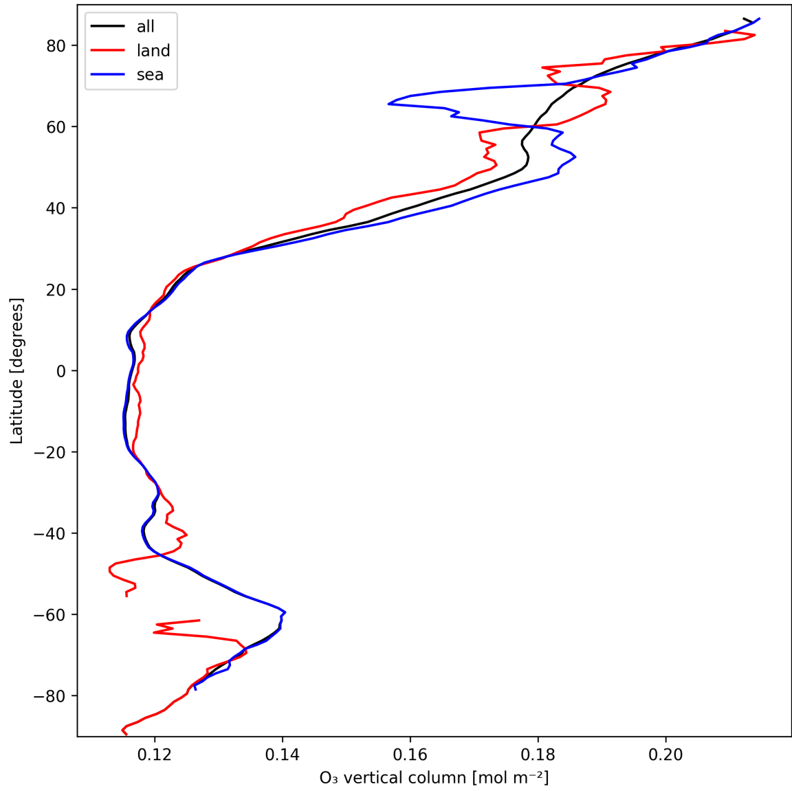
Figure 14: Zonal average of “O 3 vertical column” for 2025-03-12 to 2025-03-13.
