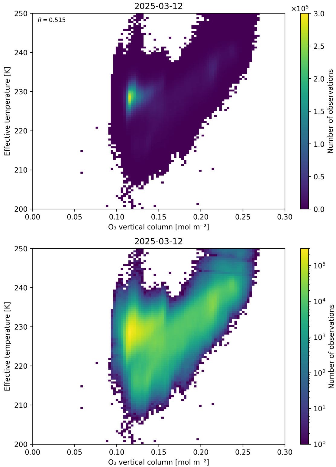
Figure 39: Scatter density plot of “O 3 vertical column” against “Effective temperature” for 2025-03-12 to 2025-03-13.
