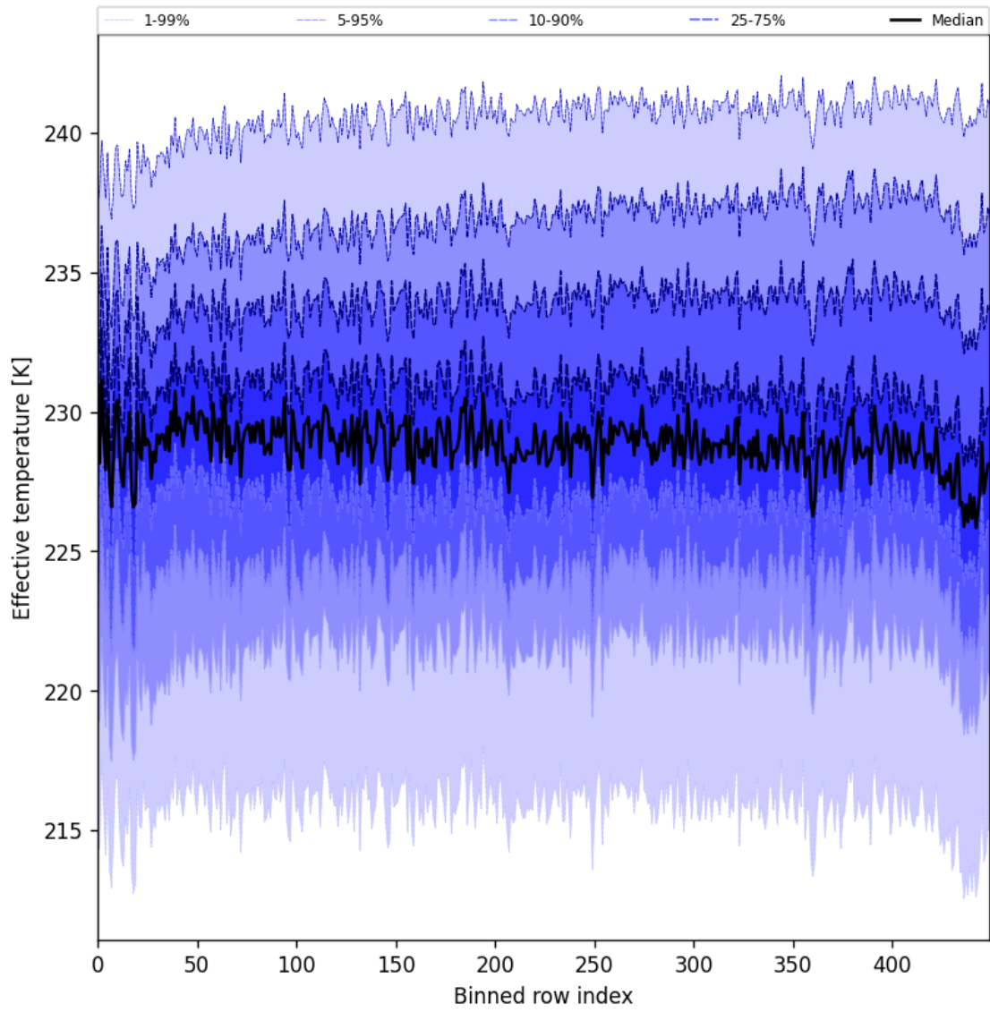
Figure 31: Along track statistics of “Effective temperature” for 2025-03-12 to 2025-03-13
