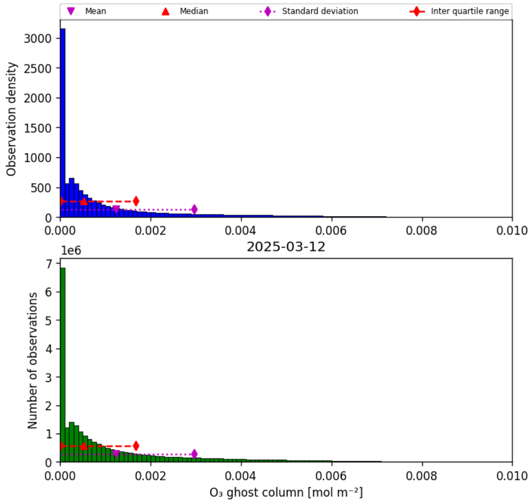
Figure 25: Histogram of “O 3 ghost column” for 2025-03-12 to 2025-03-13
