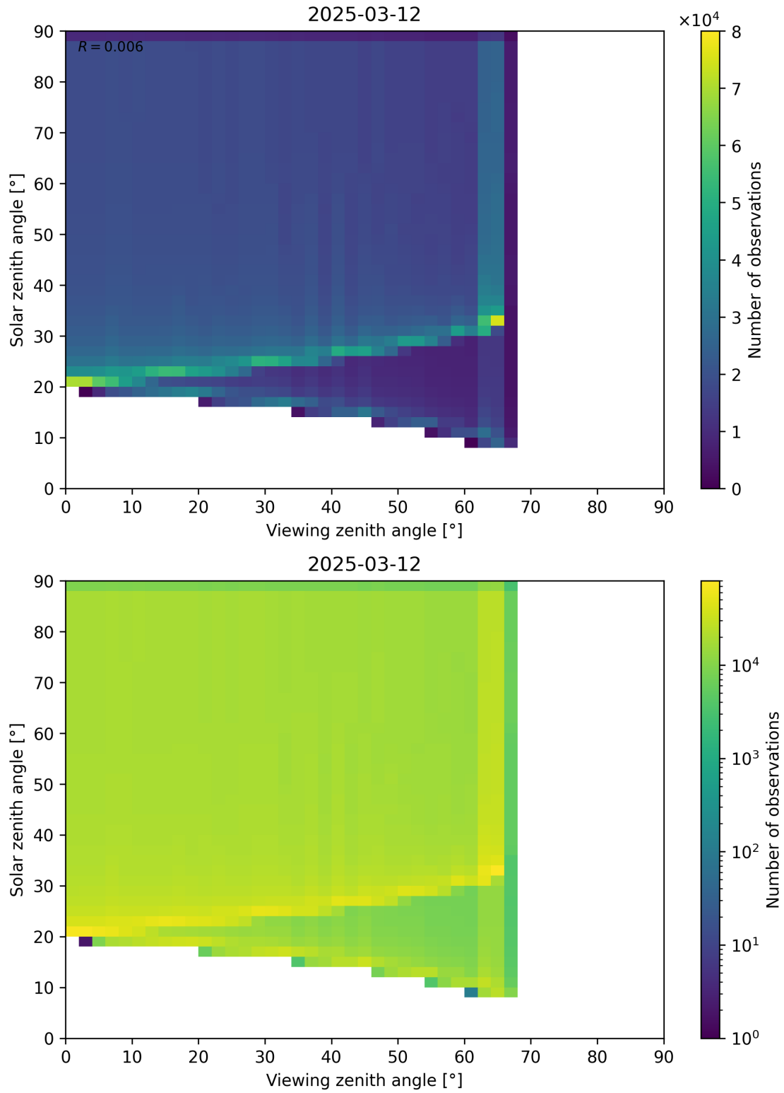
Figure 54: Scatter density plot of “Viewing zenith angle” against “Solar zenith angle” for 2025-03-12 to 2025-03-13.
