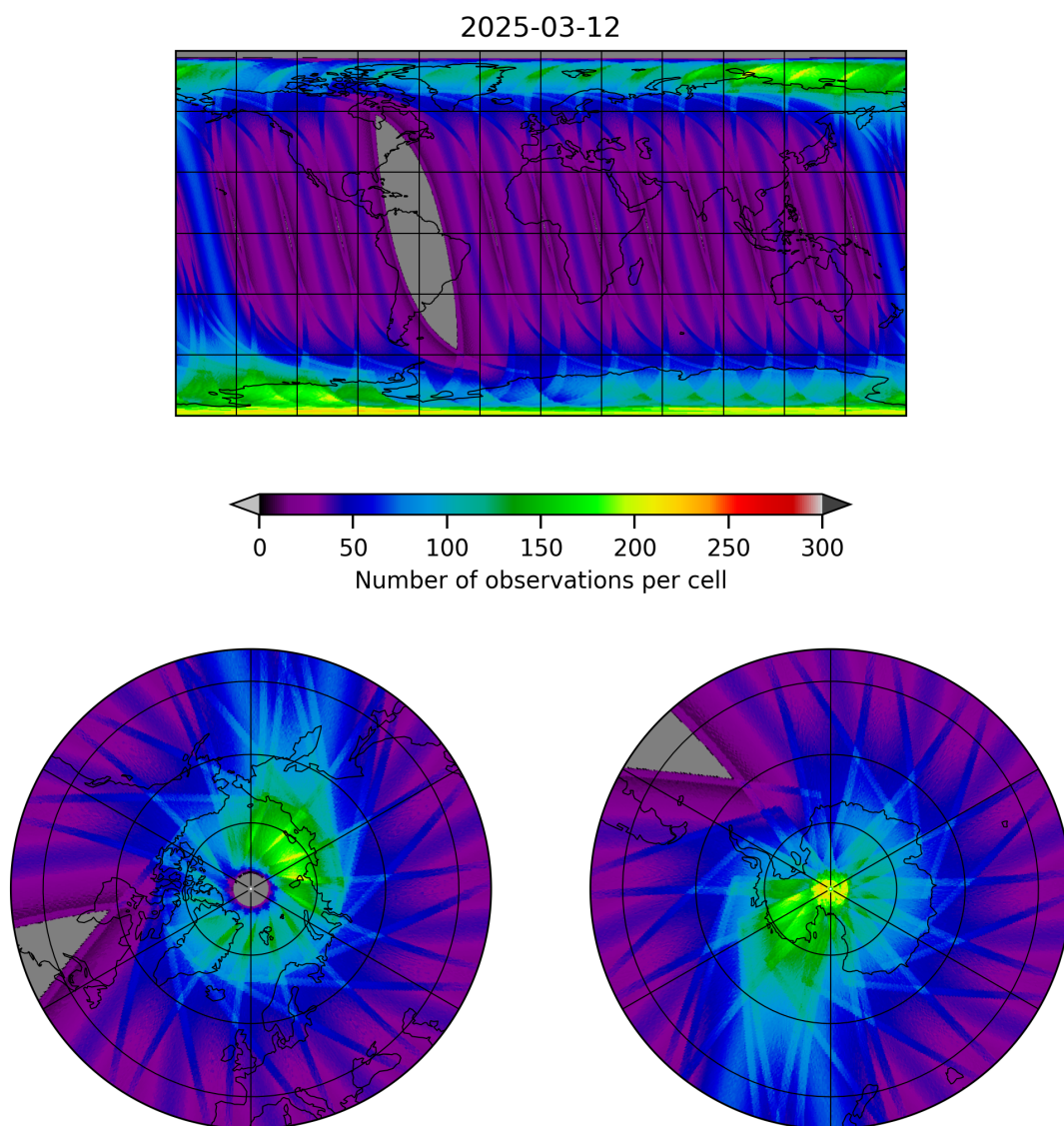
Figure 12: Map of the number of observations for 2025-03-12 to 2025-03-13
