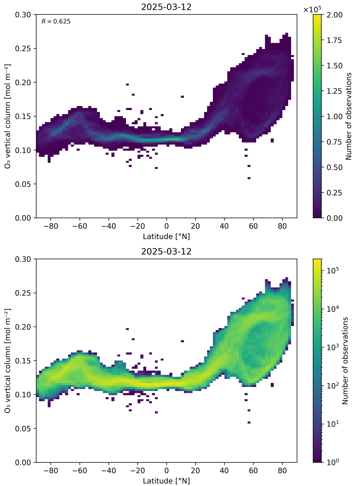
Figure 36: Scatter density plot of “Latitude” against “O 3 vertical column” for 2025-03-12 to 2025-03-13.
