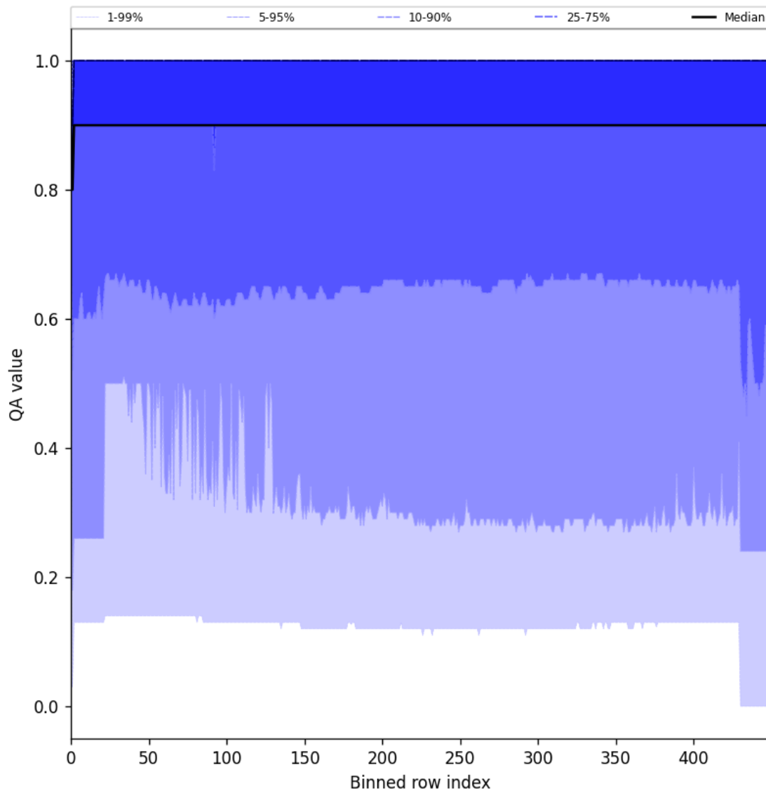
Figure 27: Along track statistics of “QA value” for 2025-03-12 to 2025-03-13
