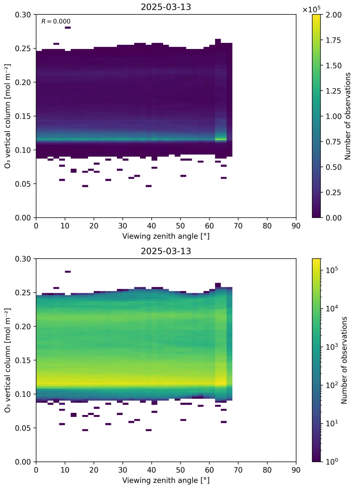
Figure 52: Scatter density plot of “Viewing zenith angle” against “O 3 vertical column” for 2025-03-12 to 2025-03-14.
