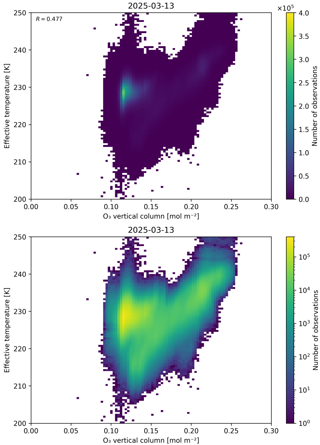
Figure 39: Scatter density plot of “O 3 vertical column” against “Effective temperature” for 2025-03-12 to 2025-03-14.
