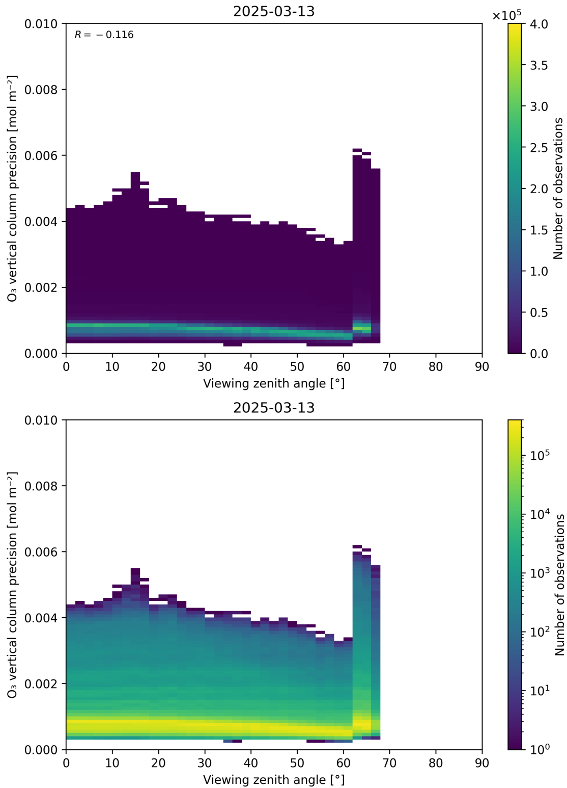
Figure 53: Scatter density plot of “Viewing zenith angle” against “O 3 vertical column precision” for 2025-03-12 to 2025-03-14.
