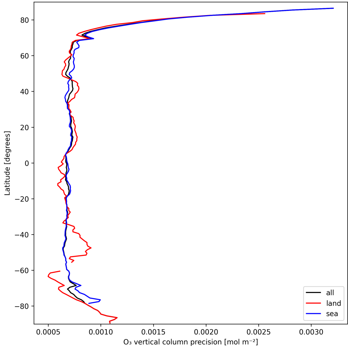
Figure 15: Zonal average of “O 3 vertical column precision” for 2025-03-12 to 2025-03-14.
