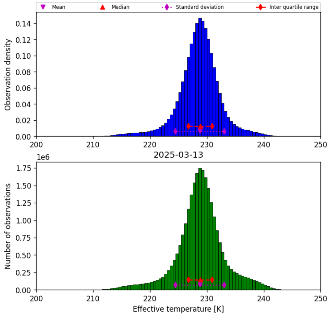
Figure 24: Histogram of “Effective temperature” for 2025-03-12 to 2025-03-14
