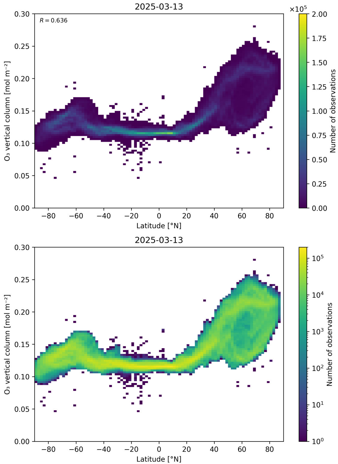
Figure 36: Scatter density plot of “Latitude” against “O 3 vertical column” for 2025-03-12 to 2025-03-14.
