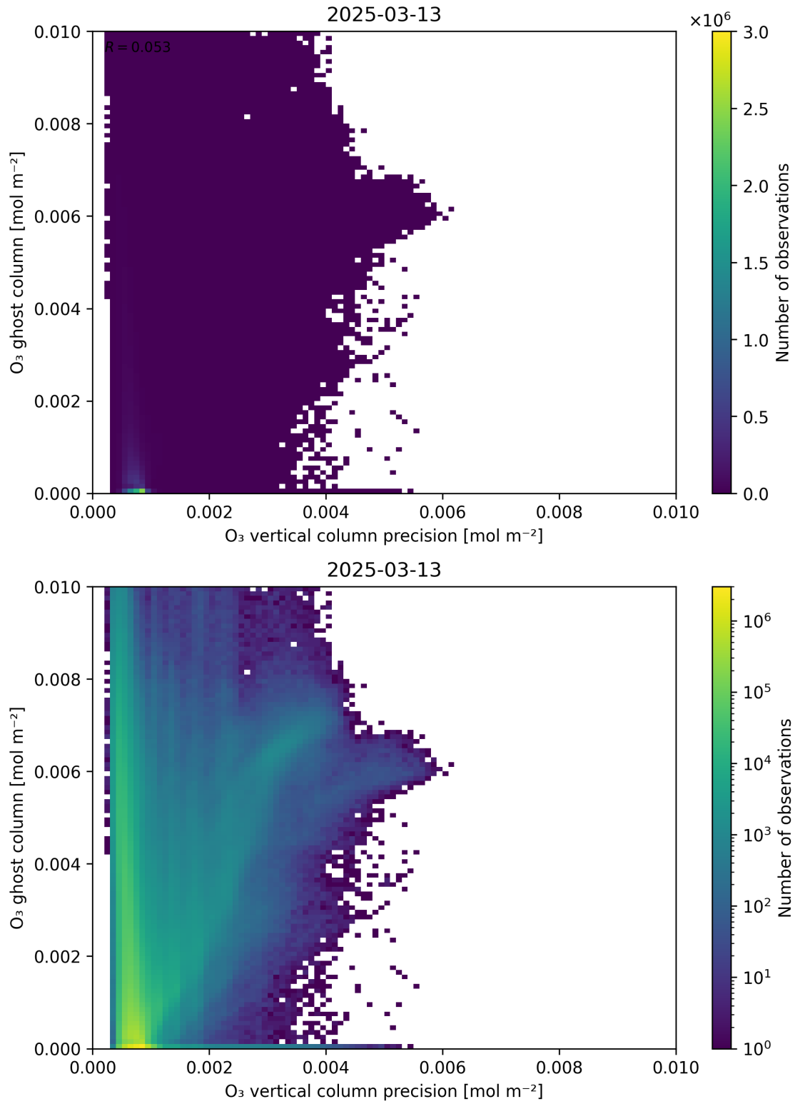
Figure 43: Scatter density plot of “ \text{O}_3 vertical column precision” against “ \text{O}_3 ghost column” for 2025-03-12 to 2025-03-14.
