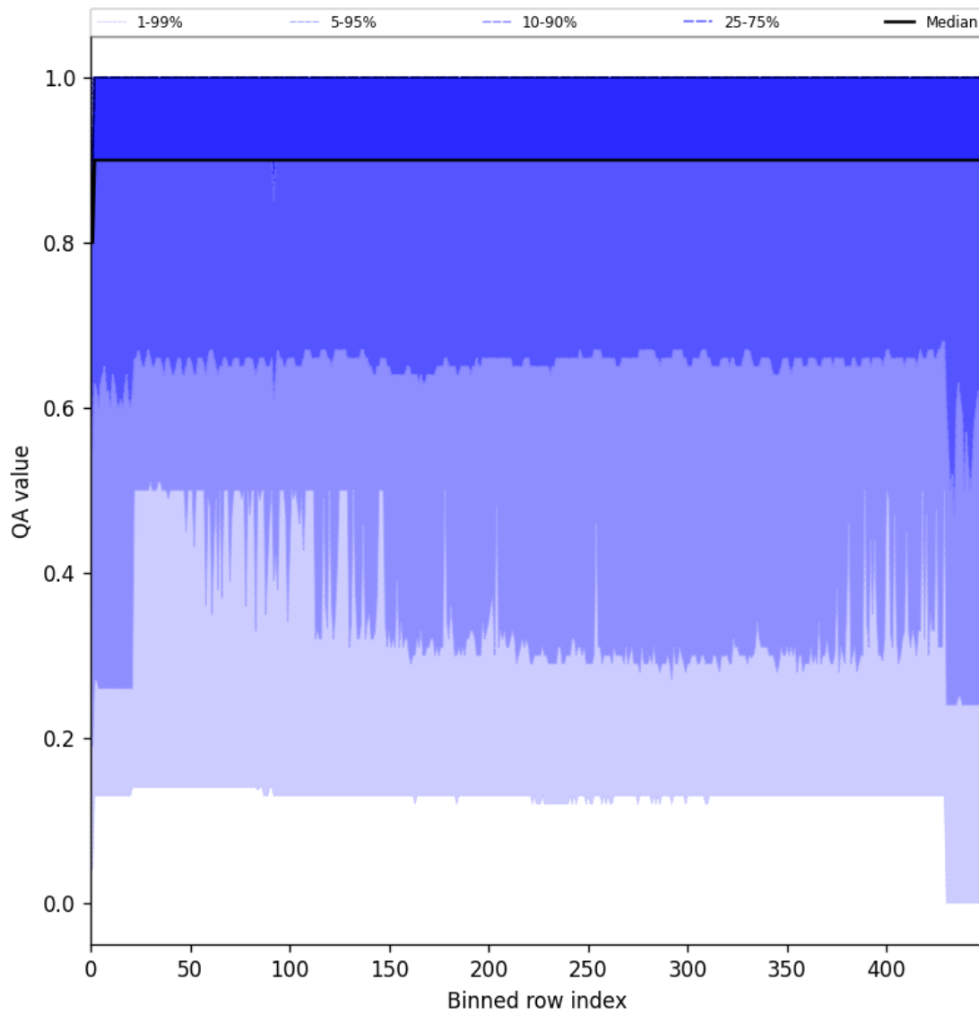
Figure 27: Along track statistics of “QA value” for 2025-03-12 to 2025-03-14
