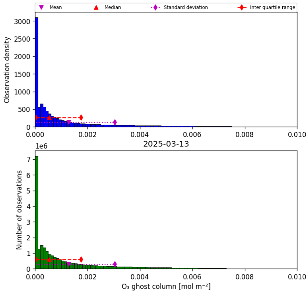
Figure 25: Histogram of “O 3 ghost column” for 2025-03-12 to 2025-03-14
