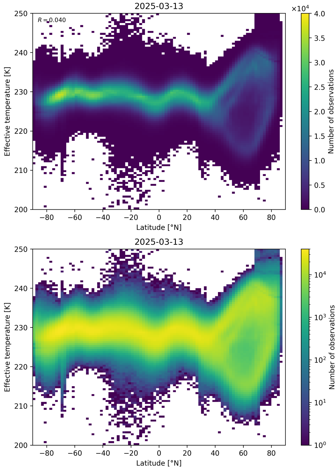
Figure 34: Scatter density plot of “Latitude” against “Effective temperature” for 2025-03-12 to 2025-03-14.
