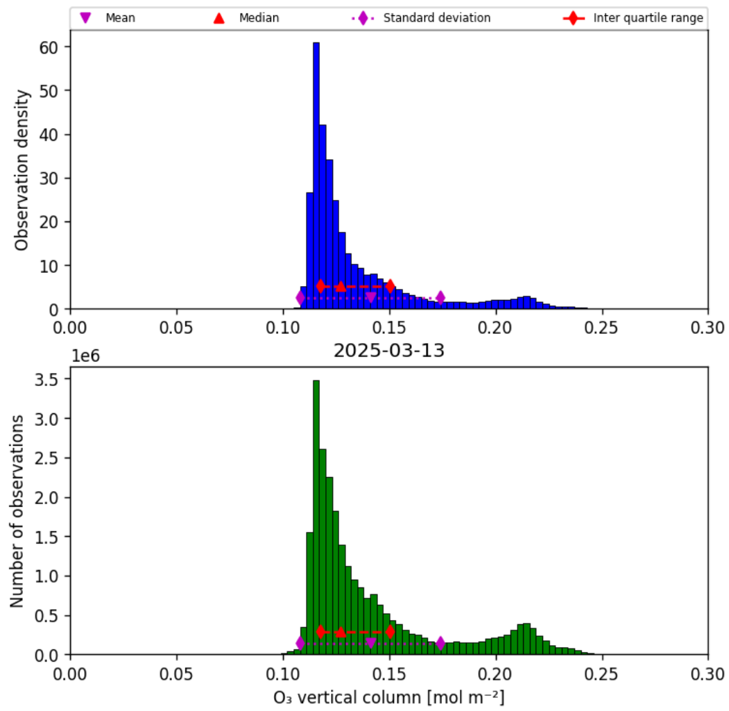
Figure 21: Histogram of “O 3 vertical column” for 2025-03-12 to 2025-03-14
