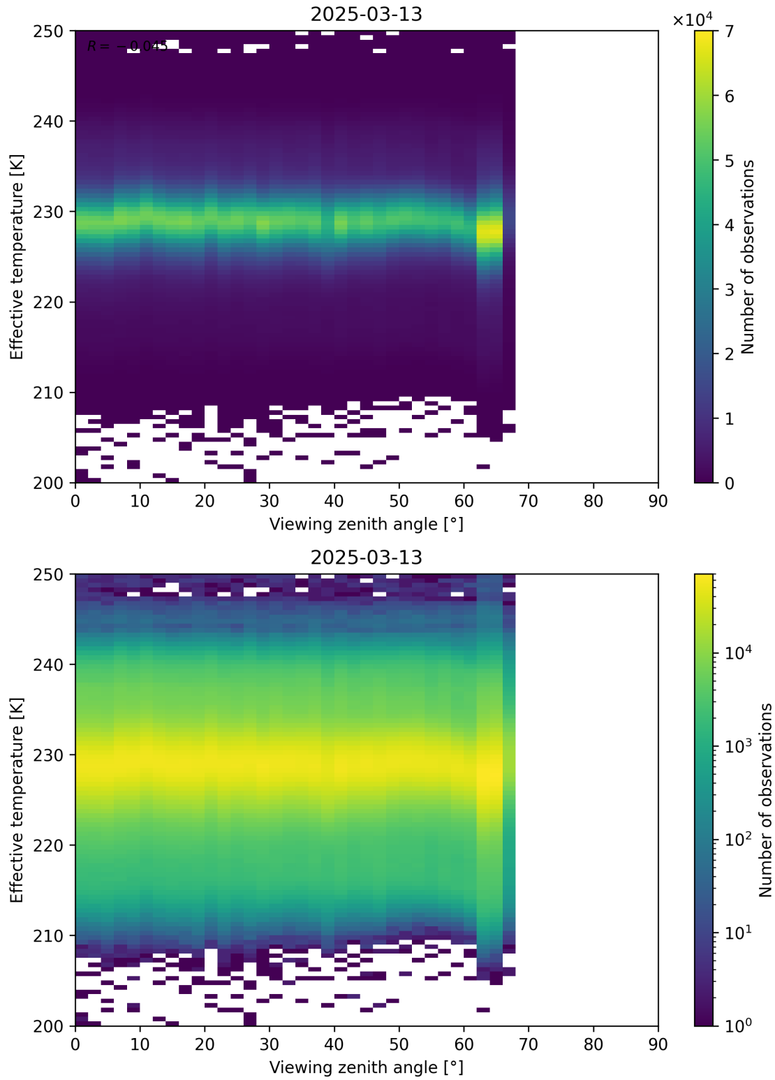
Figure 50: Scatter density plot of “Viewing zenith angle” against “Effective temperature” for 2025-03-12 to 2025-03-14.
