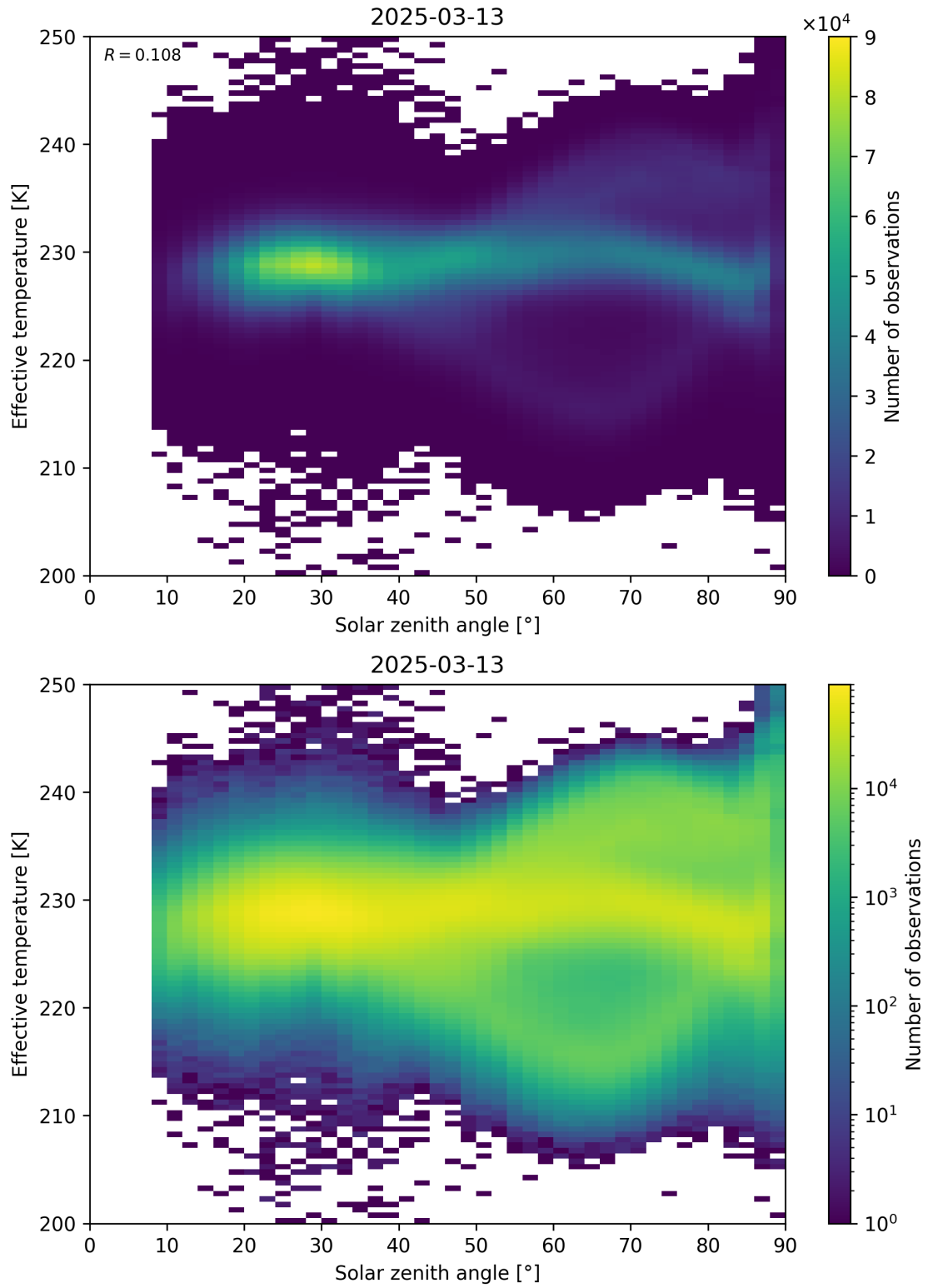
Figure 45: Scatter density plot of “Solar zenith angle” against “Effective temperature” for 2025-03-12 to 2025-03-14.
