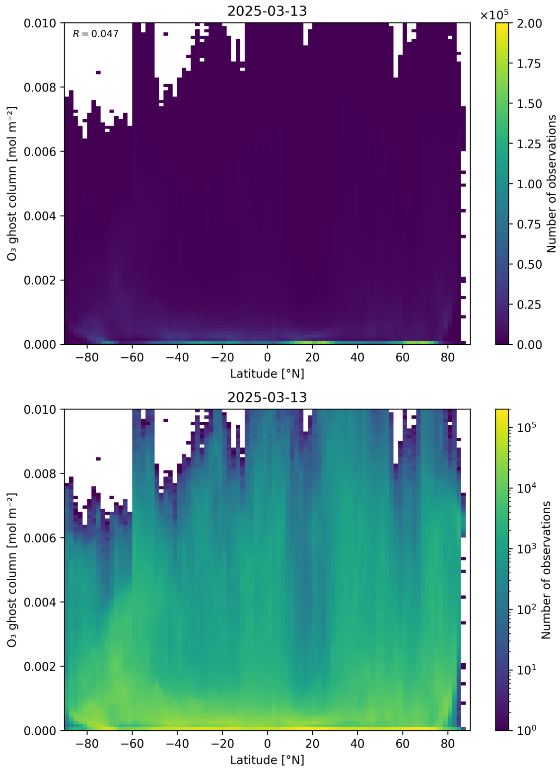
Figure 35: Scatter density plot of “Latitude” against “O 3 ghost column” for 2025-03-12 to 2025-03-14.
