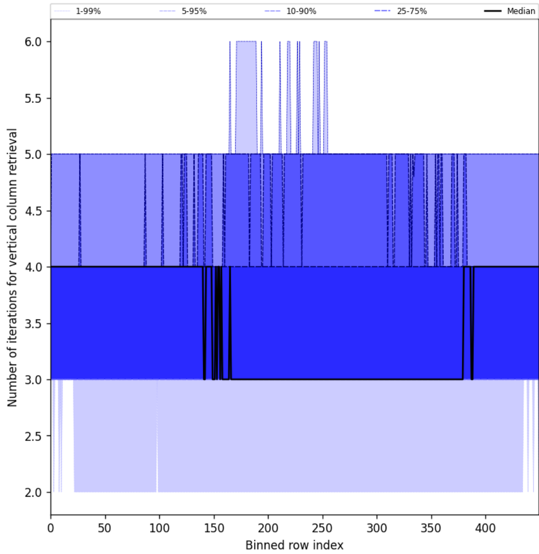
Figure 33: Along track statistics of “Number of iterations for vertical column retrieval” for 2025-03-12 to 2025-03-14
