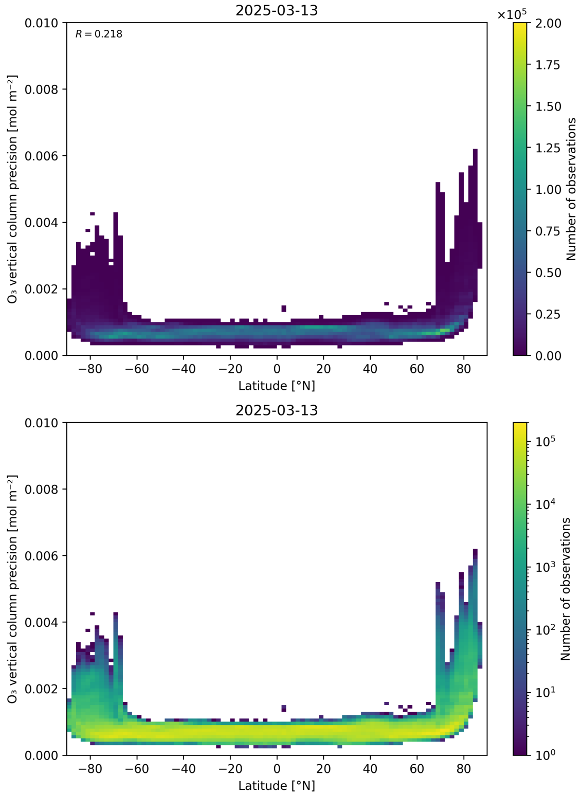
Figure 37: Scatter density plot of “Latitude” against “O 3 vertical column precision” for 2025-03-12 to 2025-03-14.
