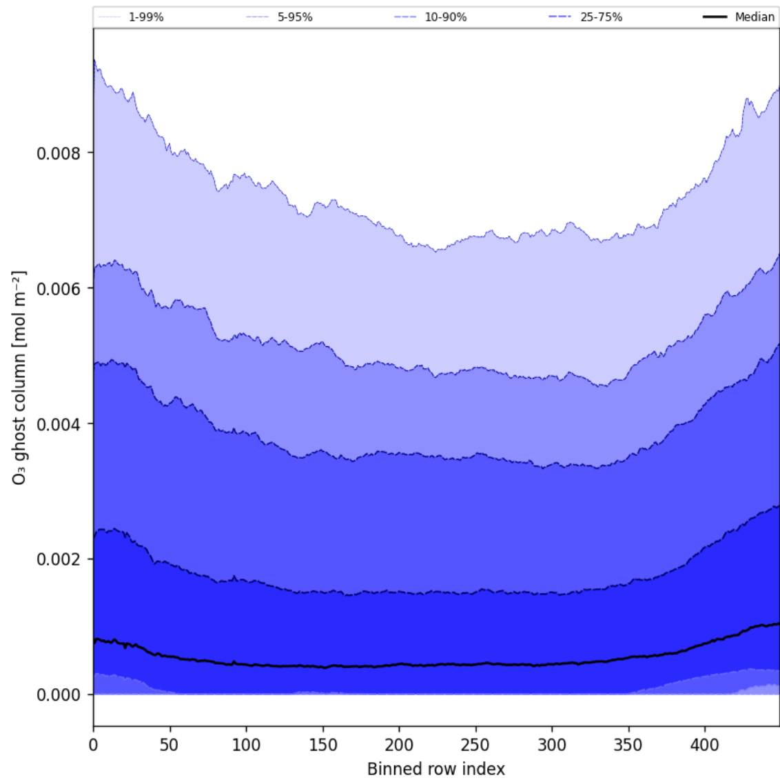
Figure 32: Along track statistics of “O 3 ghost column” for 2025-03-12 to 2025-03-14
