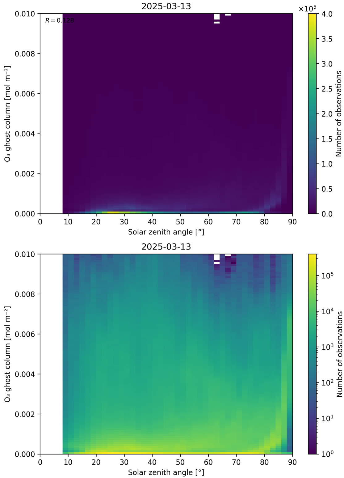
Figure 46: Scatter density plot of “Solar zenith angle” against “O 3 ghost column” for 2025-03-12 to 2025-03-14.
