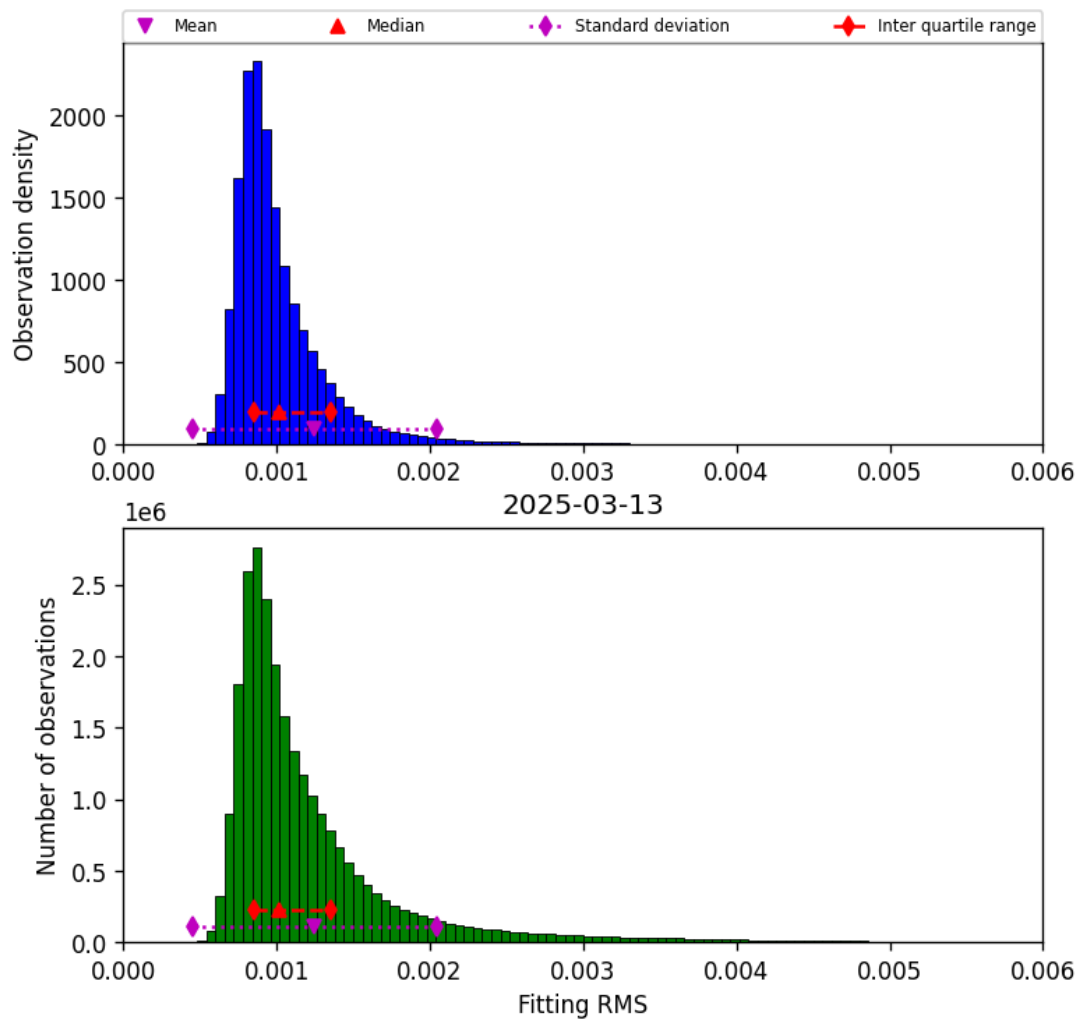
Figure 23: Histogram of “Fitting RMS” for 2025-03-12 to 2025-03-14
