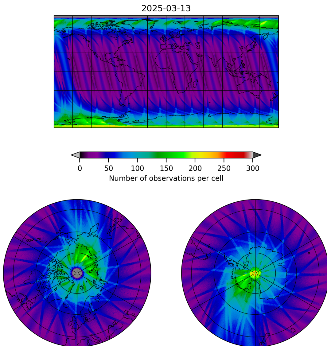
Figure 12: Map of the number of observations for 2025-03-12 to 2025-03-14
