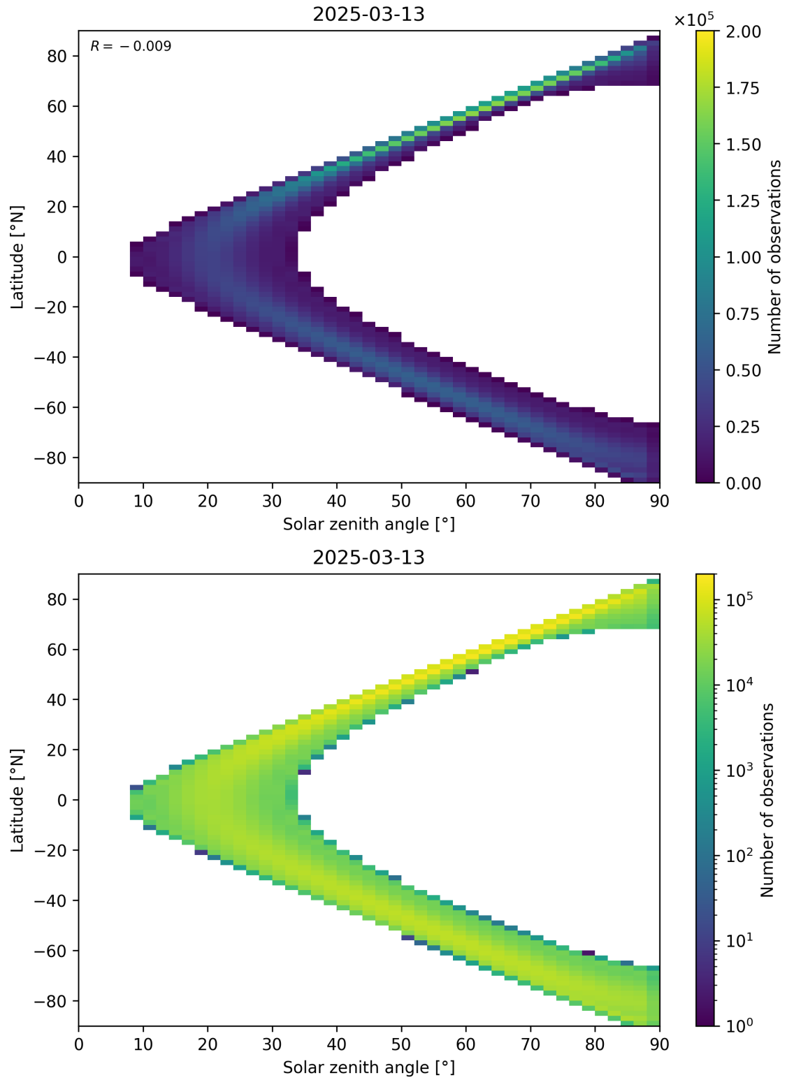
Figure 44: Scatter density plot of “Solar zenith angle” against “Latitude” for 2025-03-12 to 2025-03-14.
