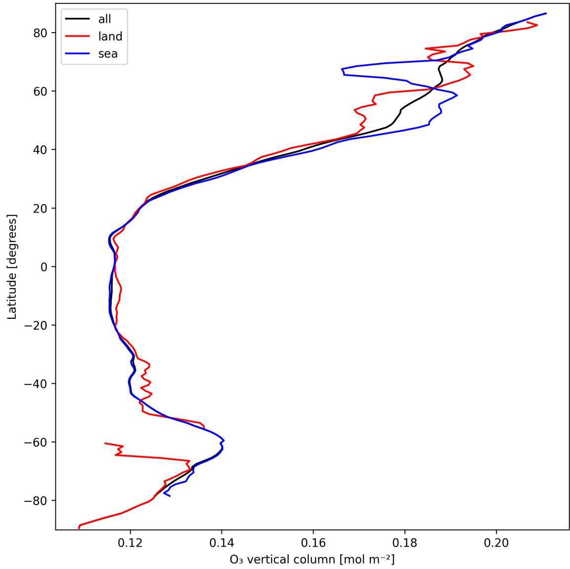
Figure 14: Zonal average of “O 3 vertical column” for 2025-03-12 to 2025-03-14.
