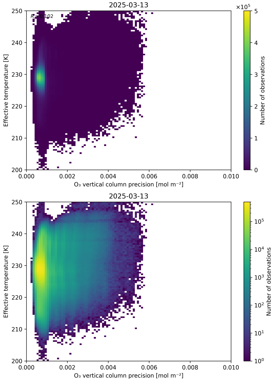
Figure 42: Scatter density plot of “O 3 vertical column precision” against “Effective temperature” for 2025-03-12 to 2025-03-14.
