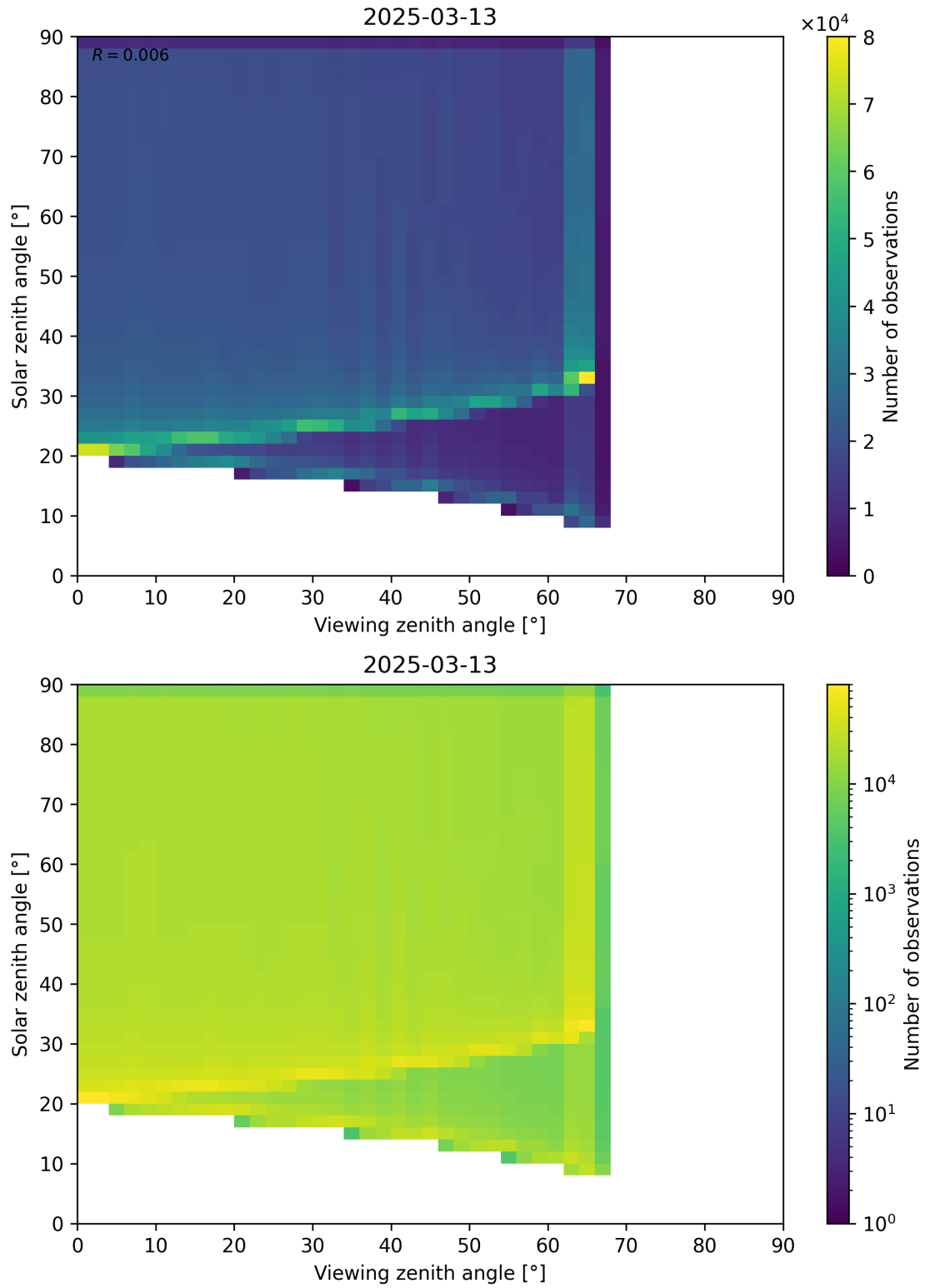
Figure 54: Scatter density plot of “Viewing zenith angle” against “Solar zenith angle” for 2025-03-12 to 2025-03-14.
