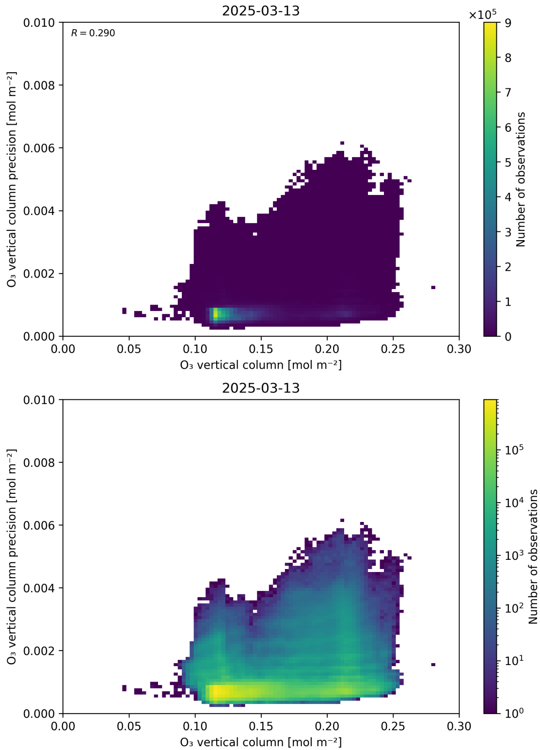
Figure 41: Scatter density plot of “O 3 vertical column” against “O 3 vertical column precision” for 2025-03-12 to 2025-03-14.
