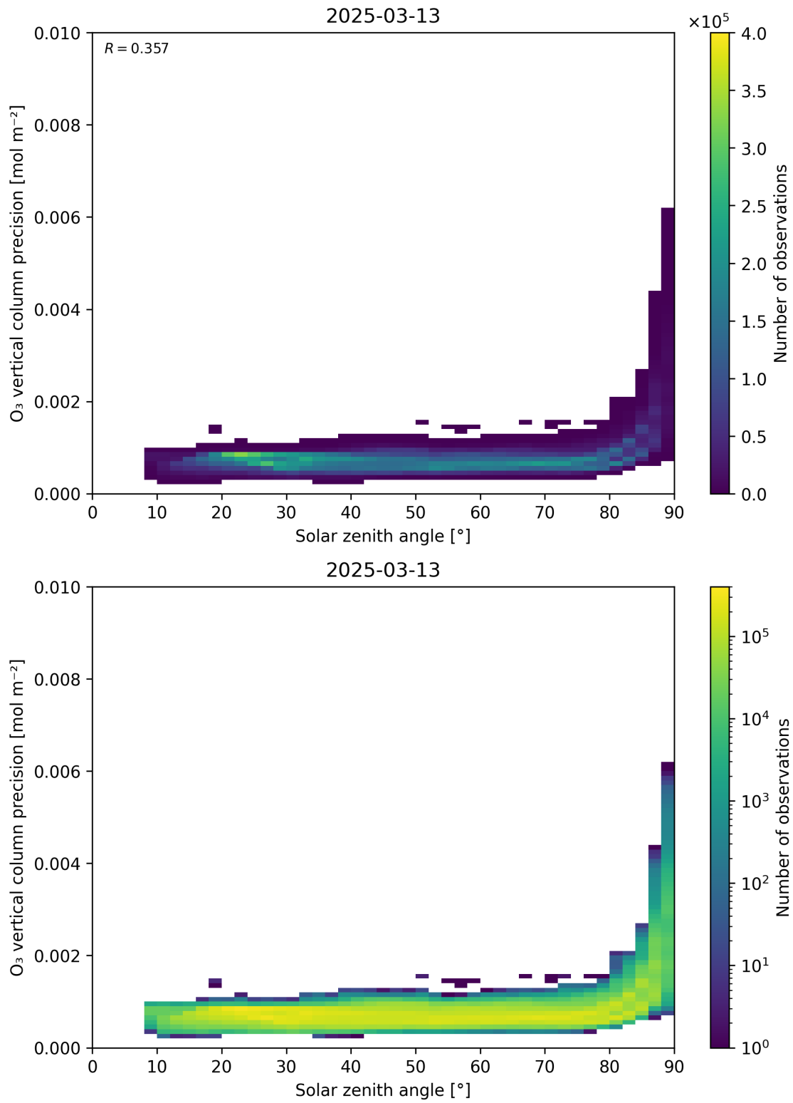
Figure 48: Scatter density plot of “Solar zenith angle” against “O 3 vertical column precision” for 2025-03-12 to 2025-03-14.
