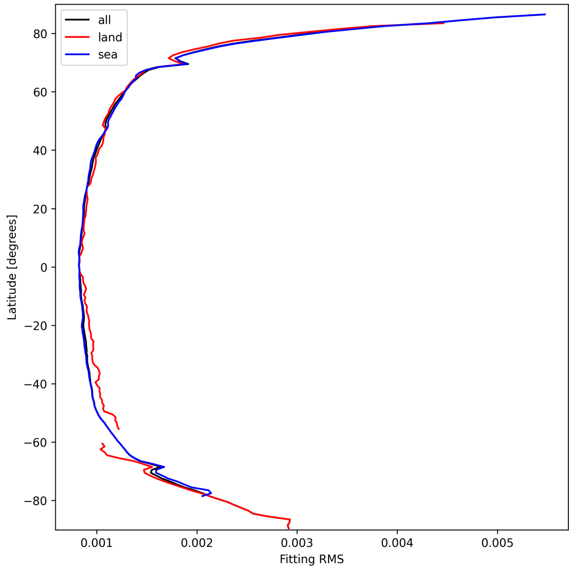
Figure 16: Zonal average of “Fitting RMS” for 2025-03-12 to 2025-03-14.
