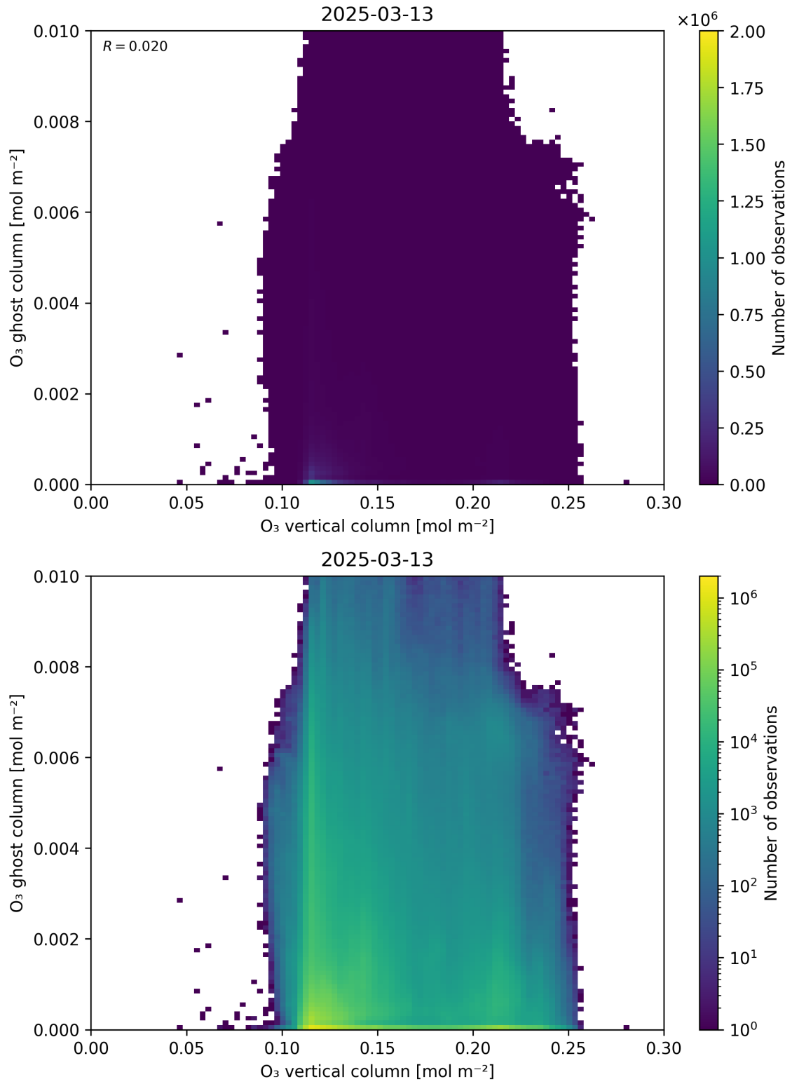
Figure 40: Scatter density plot of “O 3 vertical column” against “O 3 ghost column” for 2025-03-12 to 2025-03-14.
