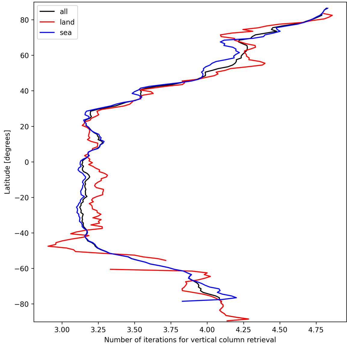
Figure 19: Zonal average of “Number of iterations for vertical column retrieval” for 2025-03-12 to 2025-03-14.
