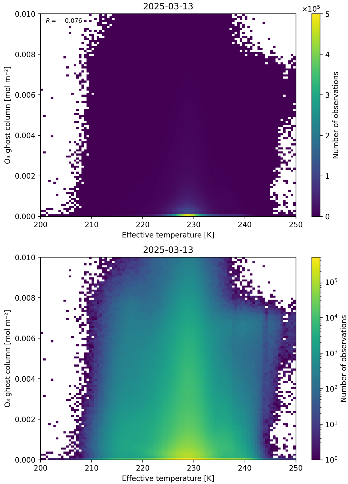
Figure 38: Scatter density plot of “Effective temperature” against “O 3 ghost column” for 2025-03-12 to 2025-03-14.
