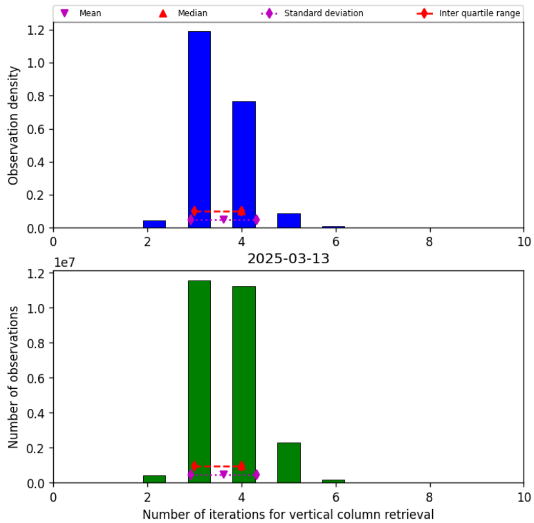
Figure 26: Histogram of “Number of iterations for vertical column retrieval” for 2025-03-12 to 2025-03-14
