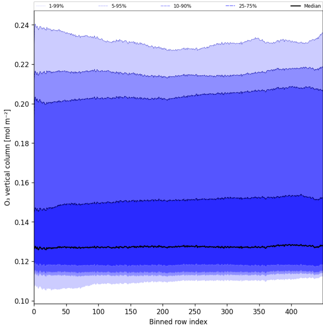
Figure 28: Along track statistics of “O 3 vertical column” for 2025-03-12 to 2025-03-14
