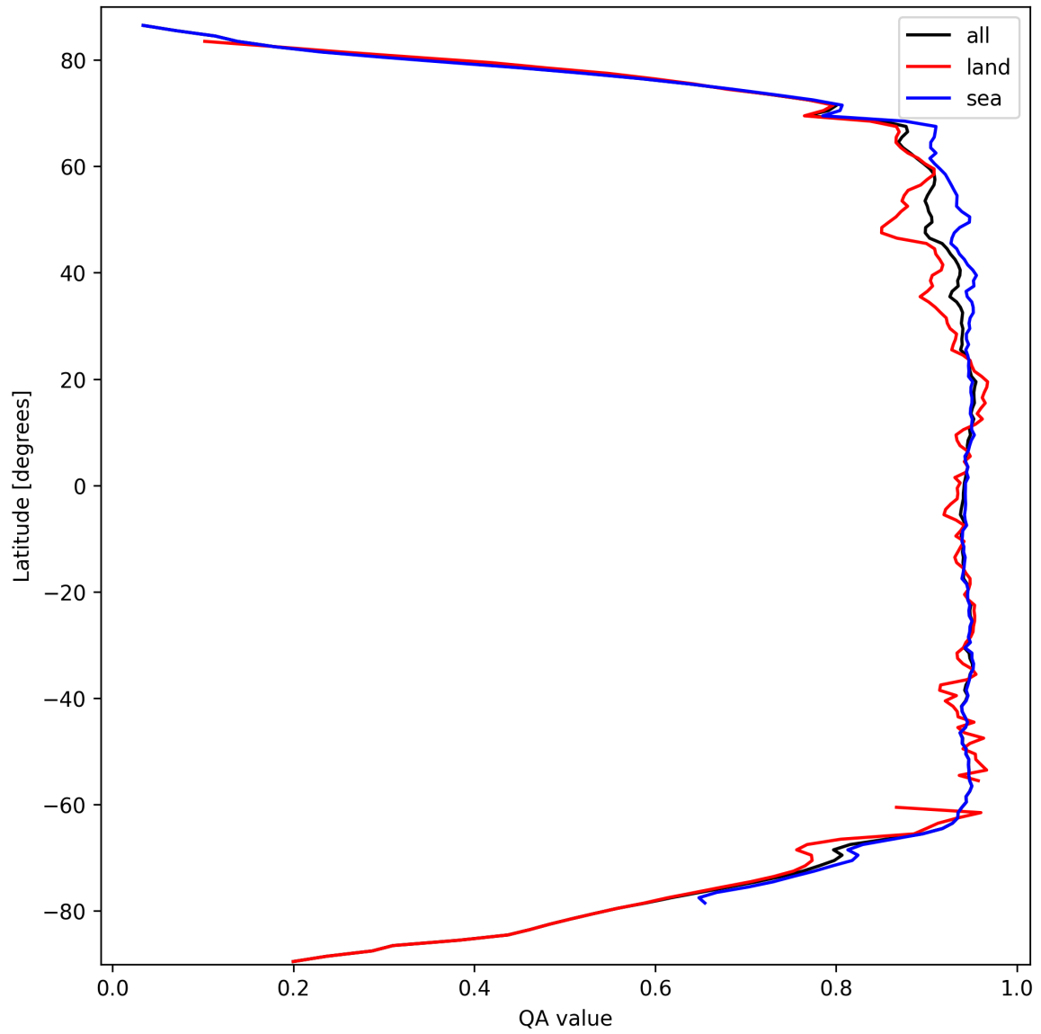
Figure 13: Zonal average of “QA value” for 2025-03-12 to 2025-03-14.
