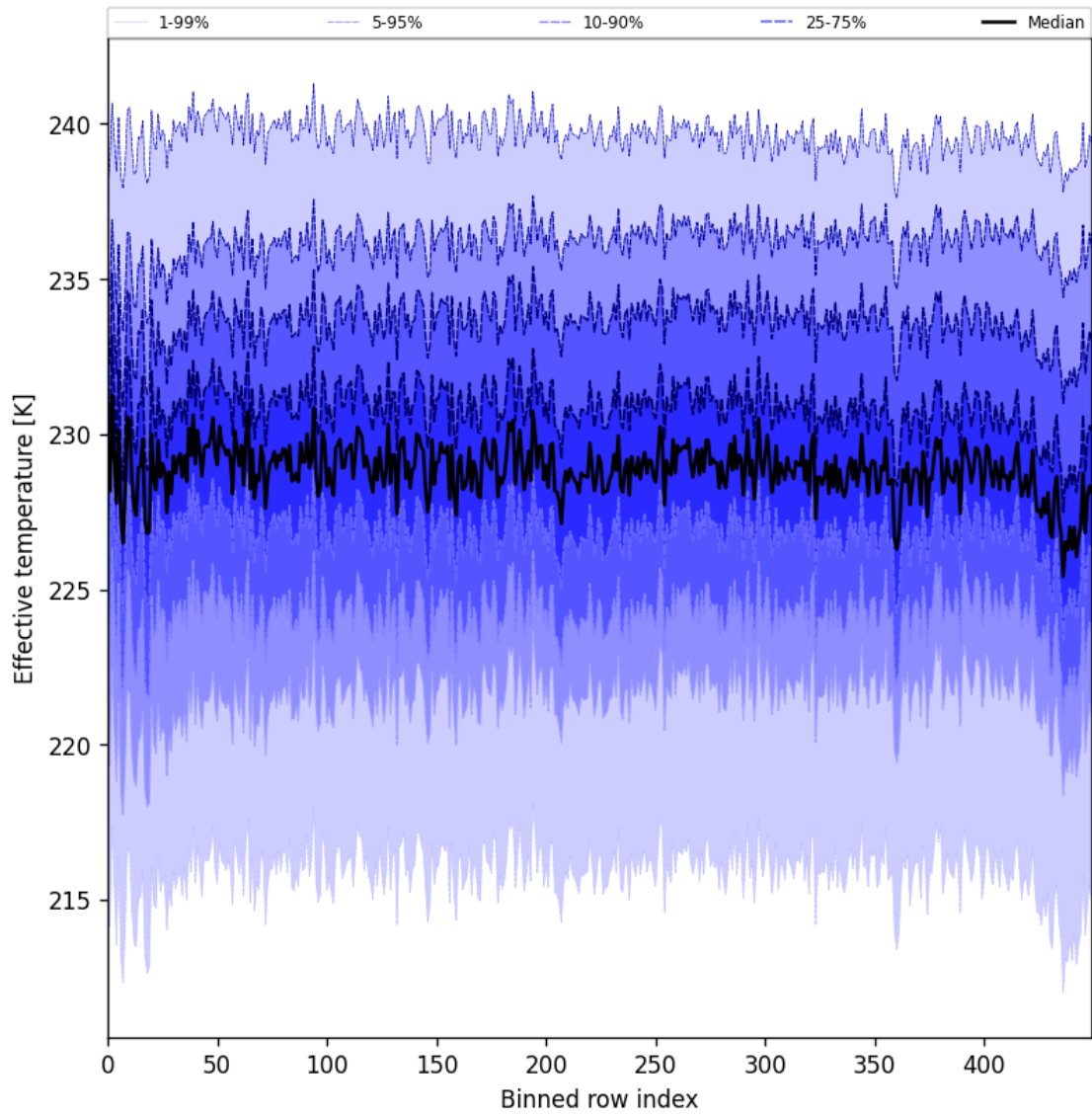
Figure 31: Along track statistics of "Effective temperature" for 2025-03-12 to 2025-03-14
