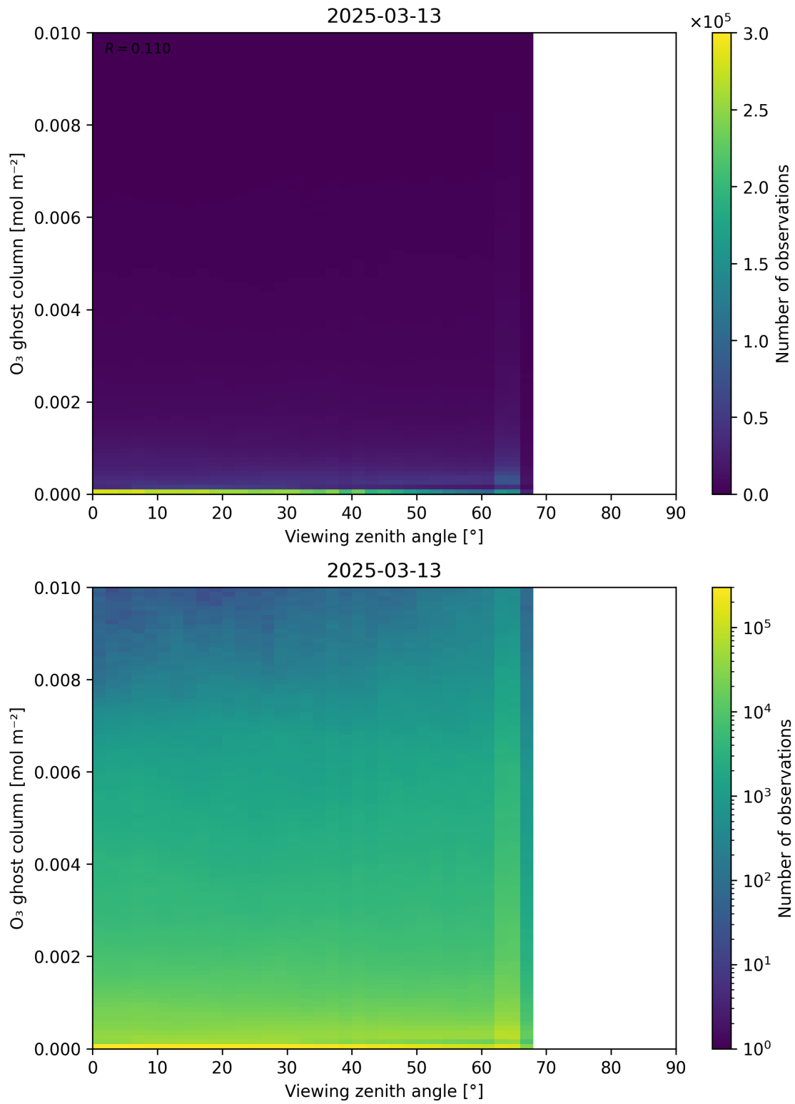
Figure 51: Scatter density plot of “Viewing zenith angle” against “O 3 ghost column” for 2025-03-12 to 2025-03-14.
