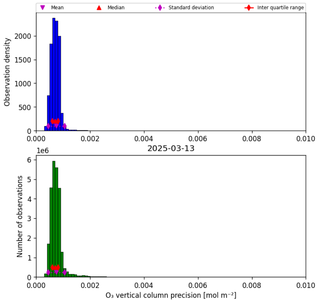
Figure 22: Histogram of “O 3 vertical column precision” for 2025-03-12 to 2025-03-14
