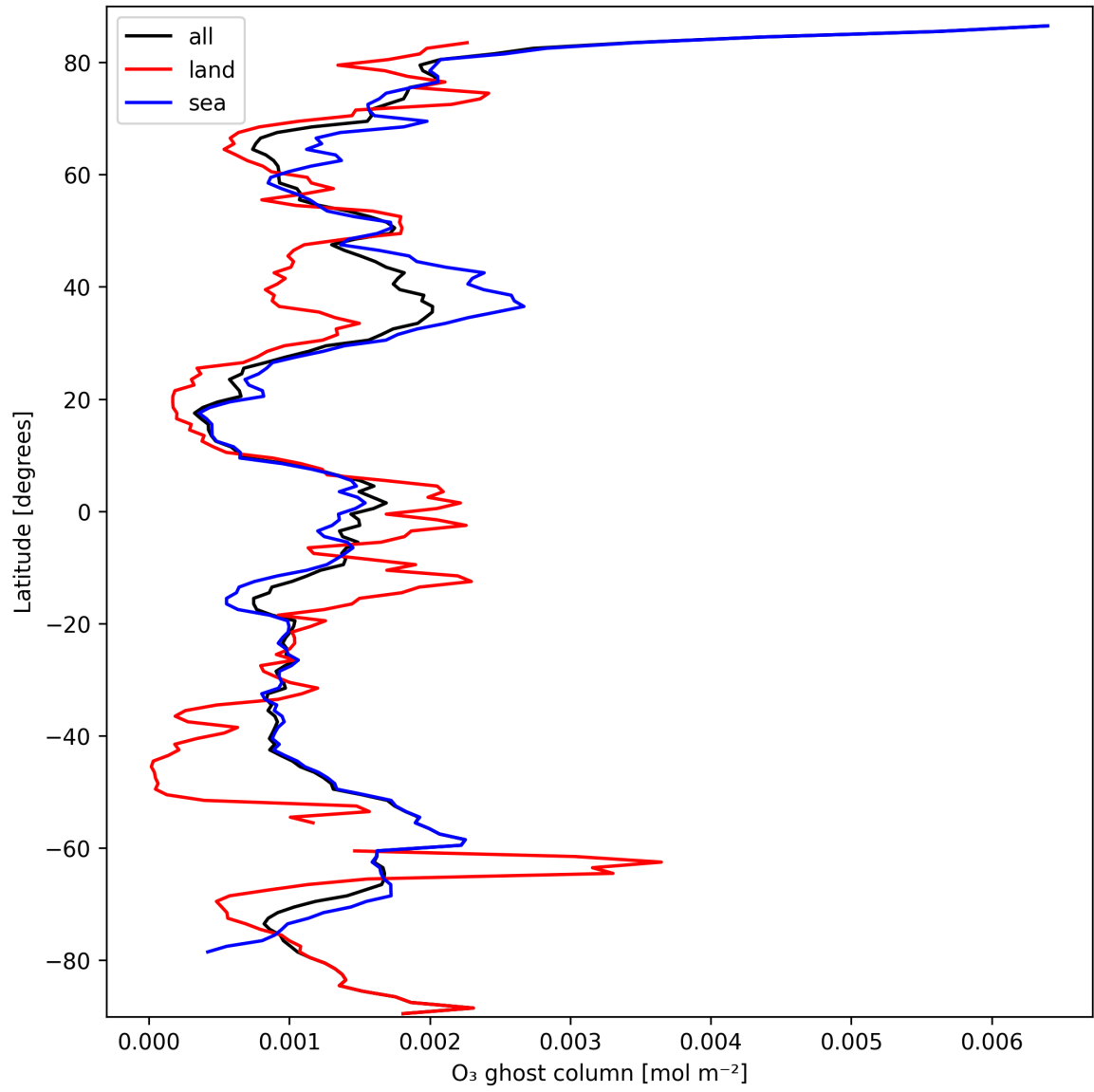
Figure 18: Zonal average of “O 3 ghost column” for 2025-03-12 to 2025-03-14.
