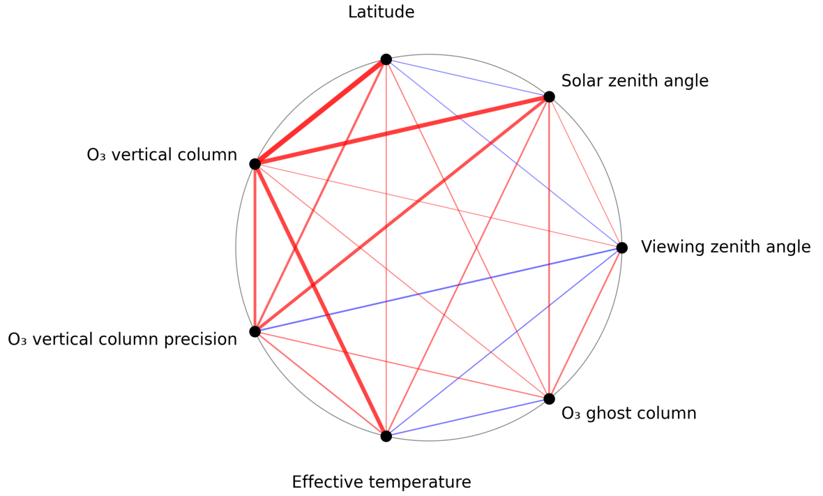
Figure 1: Map of correlation graph for 2025-03-12 to 2025-03-14.
