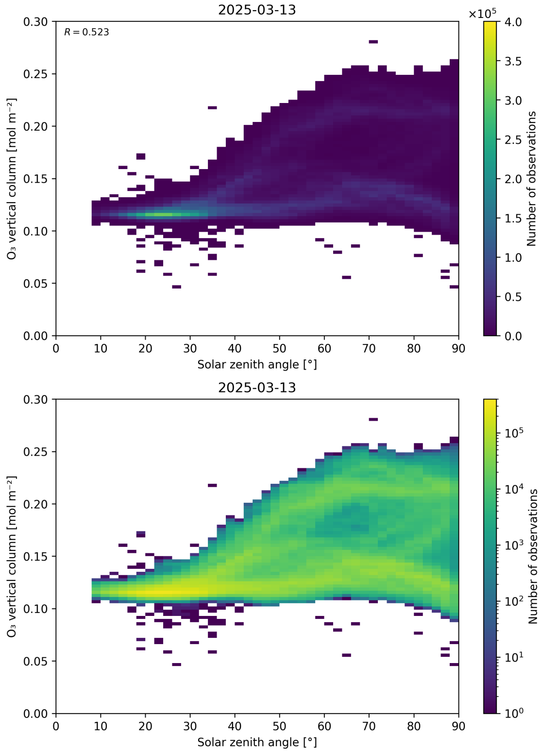
Figure 47: Scatter density plot of “Solar zenith angle” against “O 3 vertical column” for 2025-03-12 to 2025-03-14.
