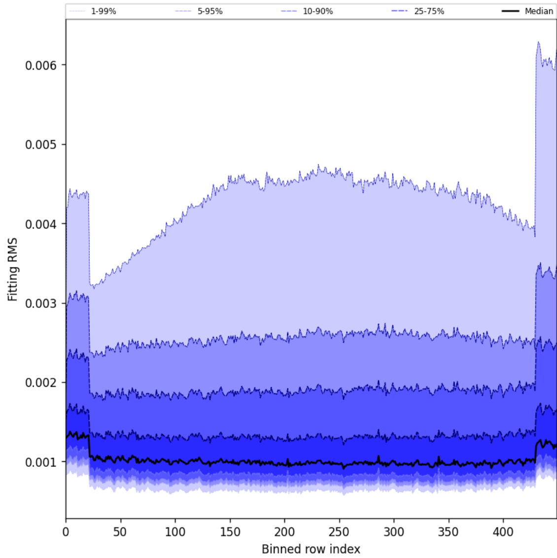
Figure 30: Along track statistics of “Fitting RMS” for 2025-03-12 to 2025-03-14
