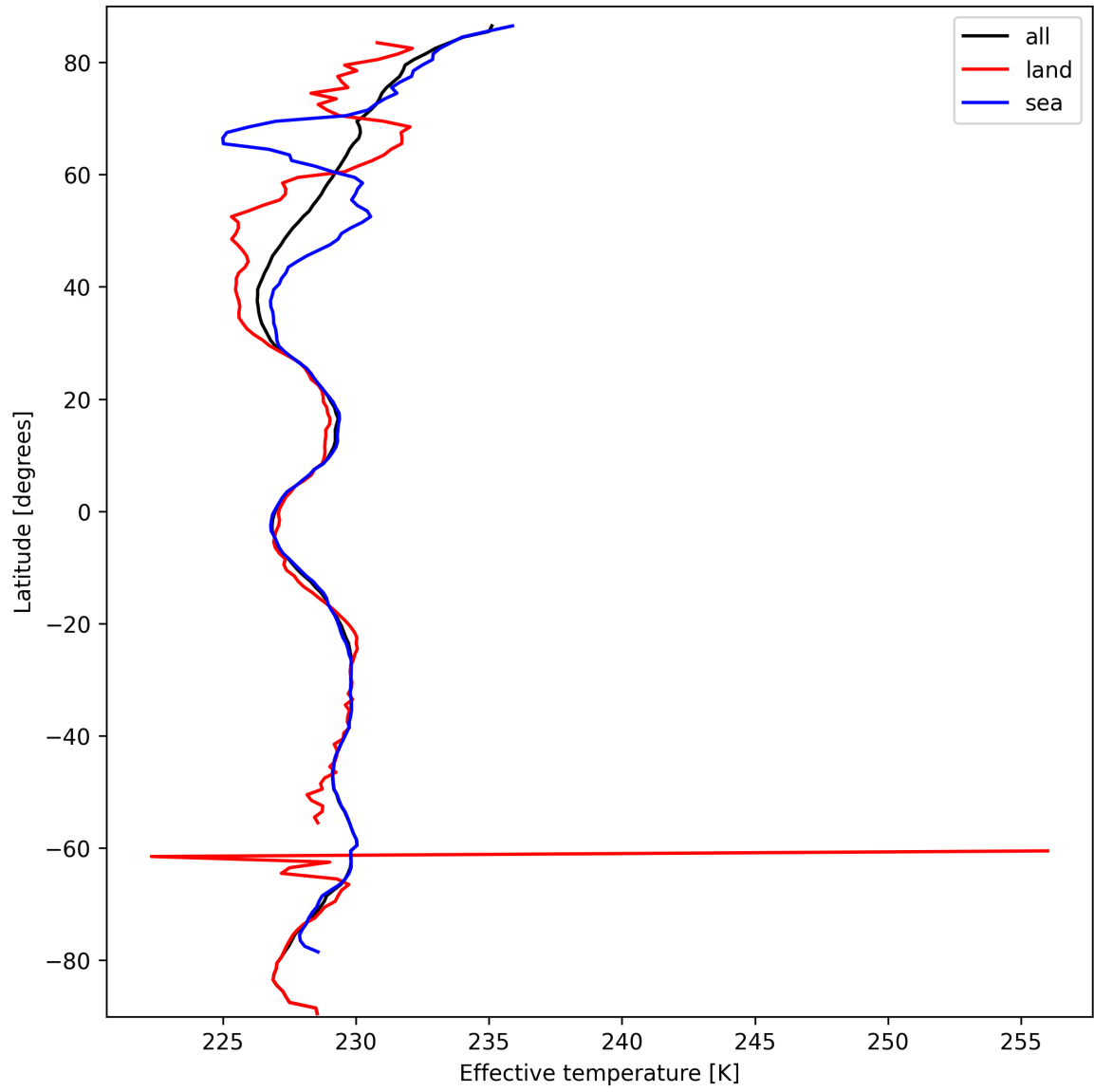
Figure 17: Zonal average of "Effective temperature" for 2025-03-12 to 2025-03-14.
