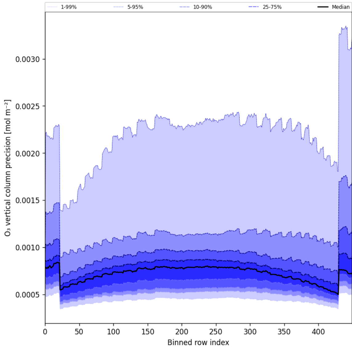
Figure 29: Along track statistics of “O 3 vertical column precision” for 2025-03-12 to 2025-03-14
