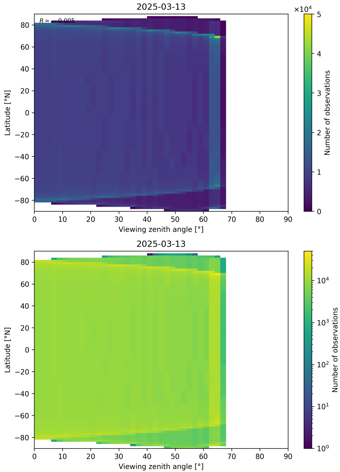
Figure 49: Scatter density plot of “Viewing zenith angle” against “Latitude” for 2025-03-12 to 2025-03-14.
