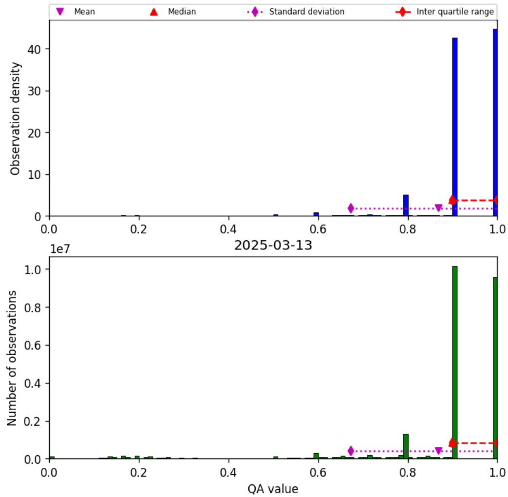
Figure 20: Histogram of “QA value” for 2025-03-12 to 2025-03-14
