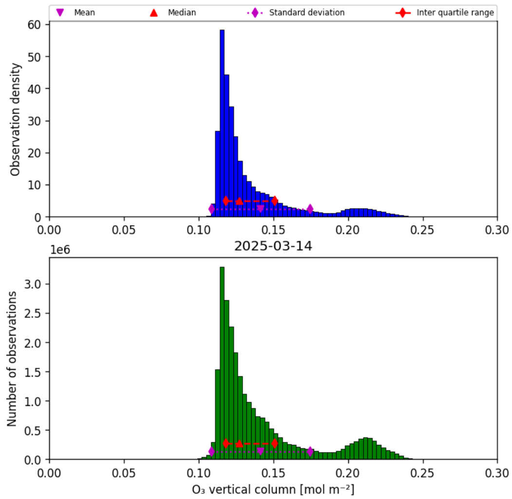
Figure 21: Histogram of “O 3 vertical column” for 2025-03-13 to 2025-03-15
