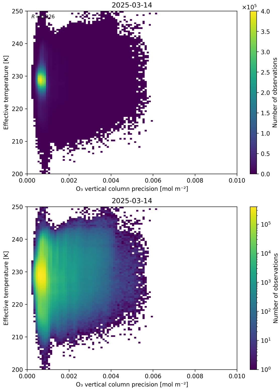
Figure 42: Scatter density plot of “O 3 vertical column precision” against “Effective temperature” for 2025-03-13 to 2025-03-15.
