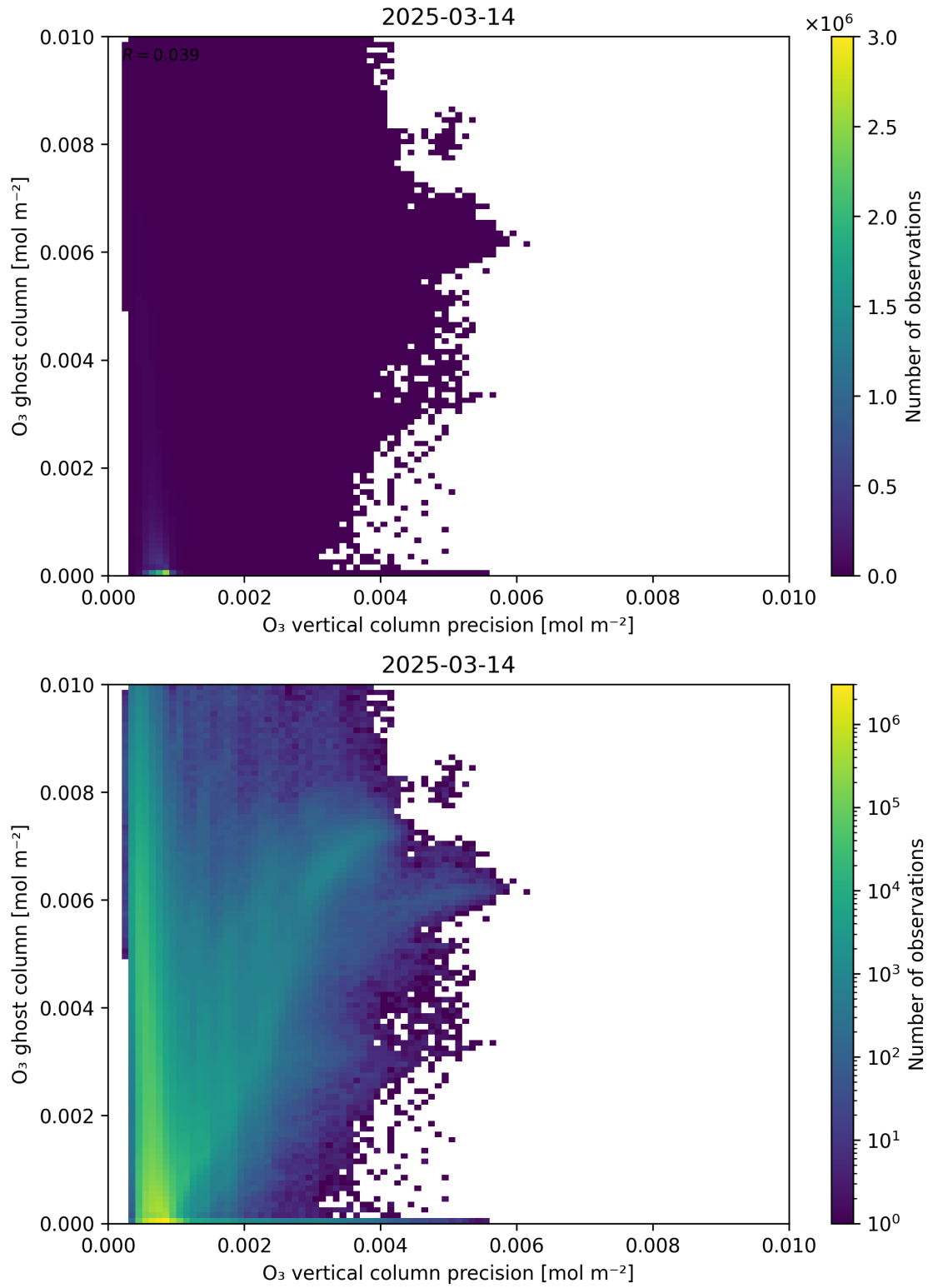
Figure 43: Scatter density plot of “O 3 vertical column precision” against “O 3 ghost column” for 2025-03-13 to 2025-03-15.
