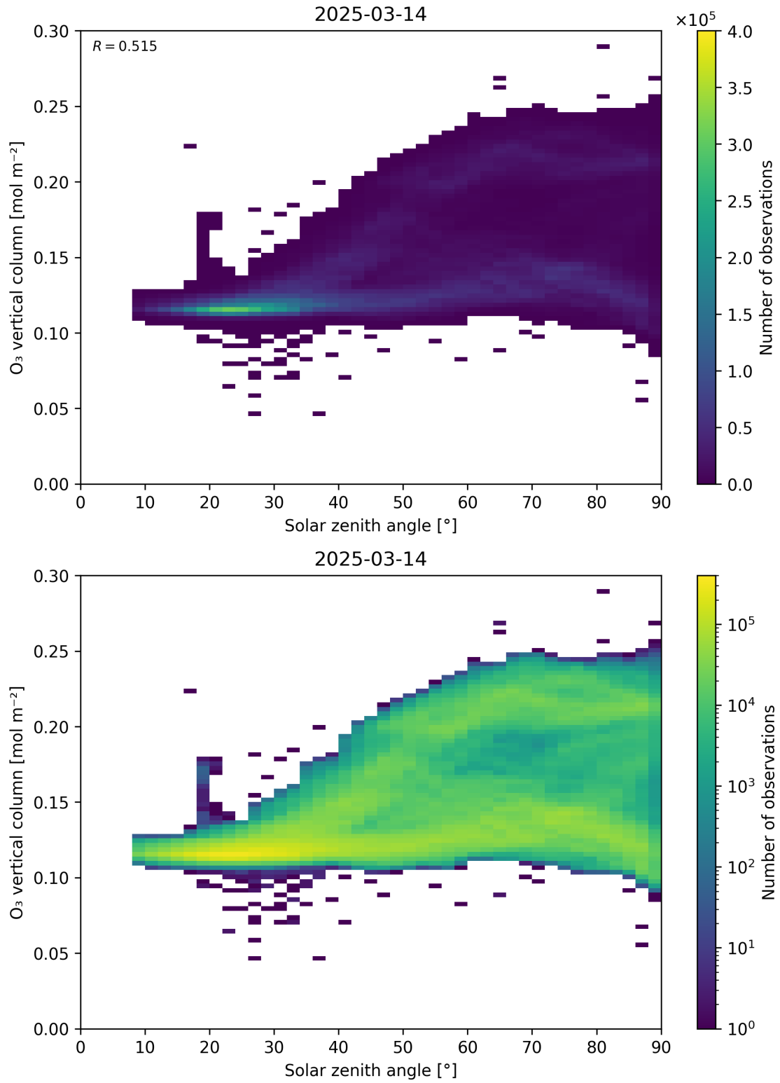
Figure 47: Scatter density plot of “Solar zenith angle” against “O 3 vertical column” for 2025-03-13 to 2025-03-15.
