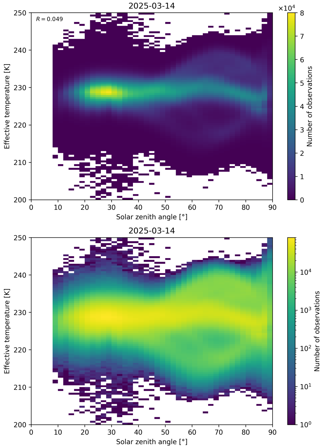
Figure 45: Scatter density plot of “Solar zenith angle” against “Effective temperature” for 2025-03-13 to 2025-03-15.
