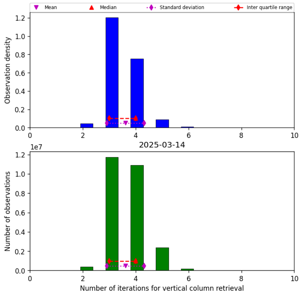
Figure 26: Histogram of “Number of iterations for vertical column retrieval” for 2025-03-13 to 2025-03-15
