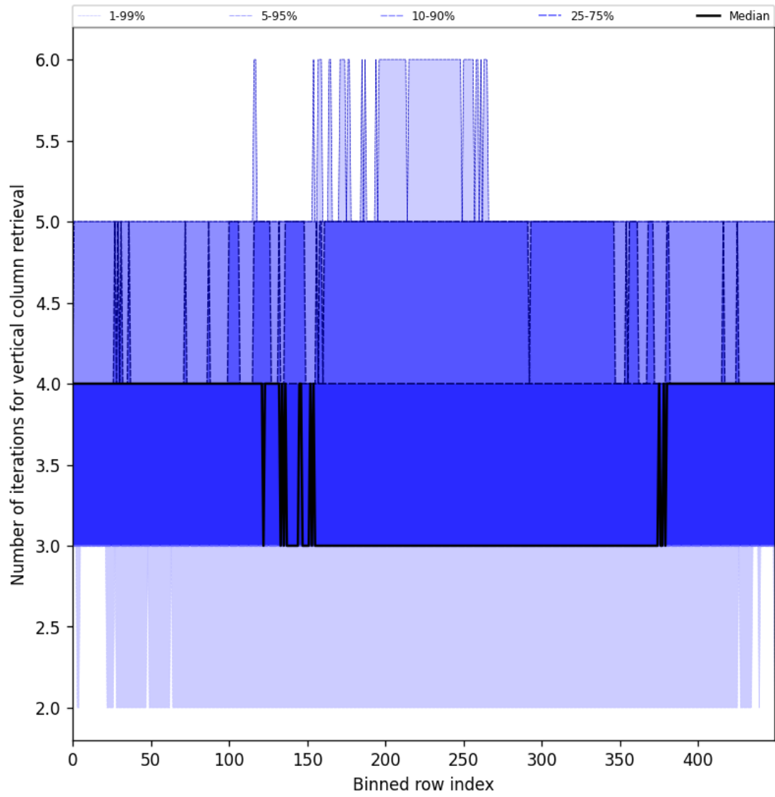
Figure 33: Along track statistics of “Number of iterations for vertical column retrieval” for 2025-03-13 to 2025-03-15
