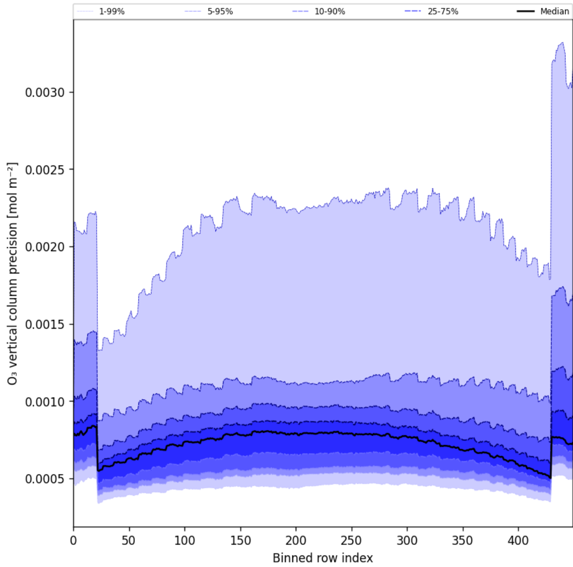
Figure 29: Along track statistics of “O 3 vertical column precision” for 2025-03-13 to 2025-03-15
