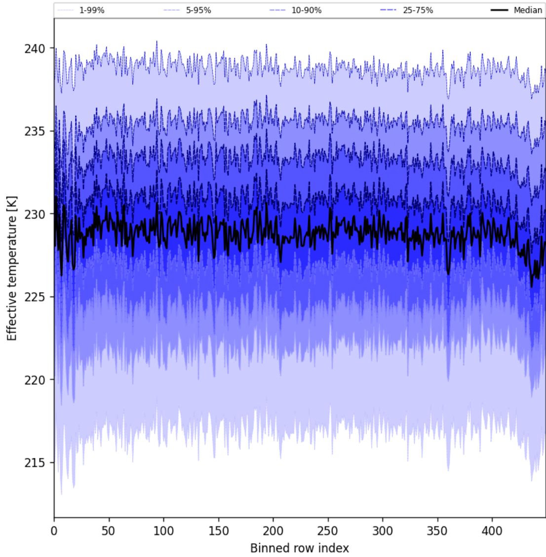
Figure 31: Along track statistics of “Effective temperature” for 2025-03-13 to 2025-03-15
