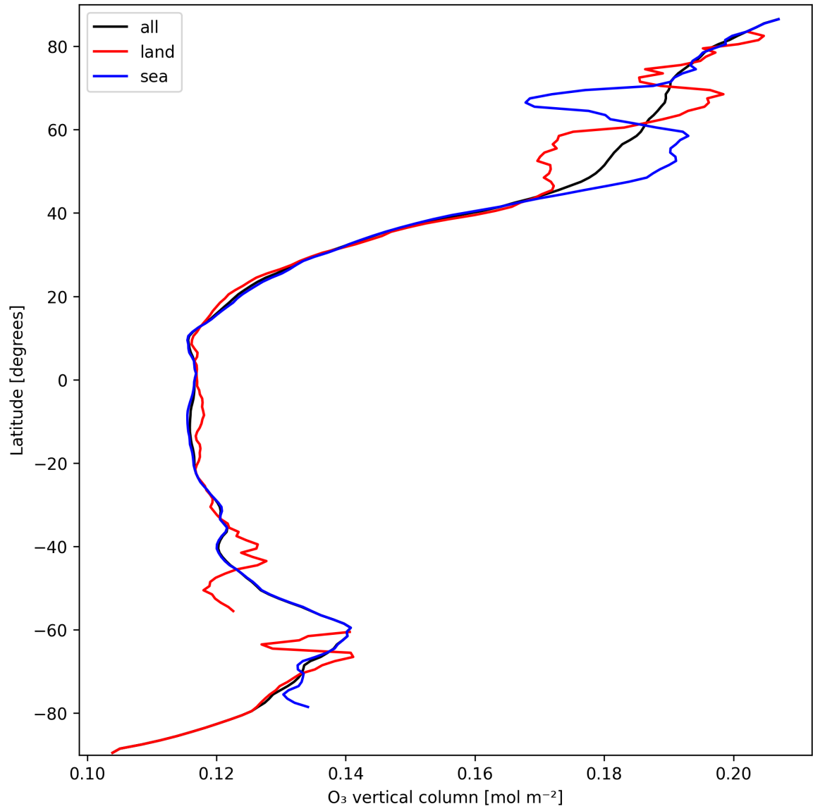
Figure 14: Zonal average of “O 3 vertical column” for 2025-03-13 to 2025-03-15.
