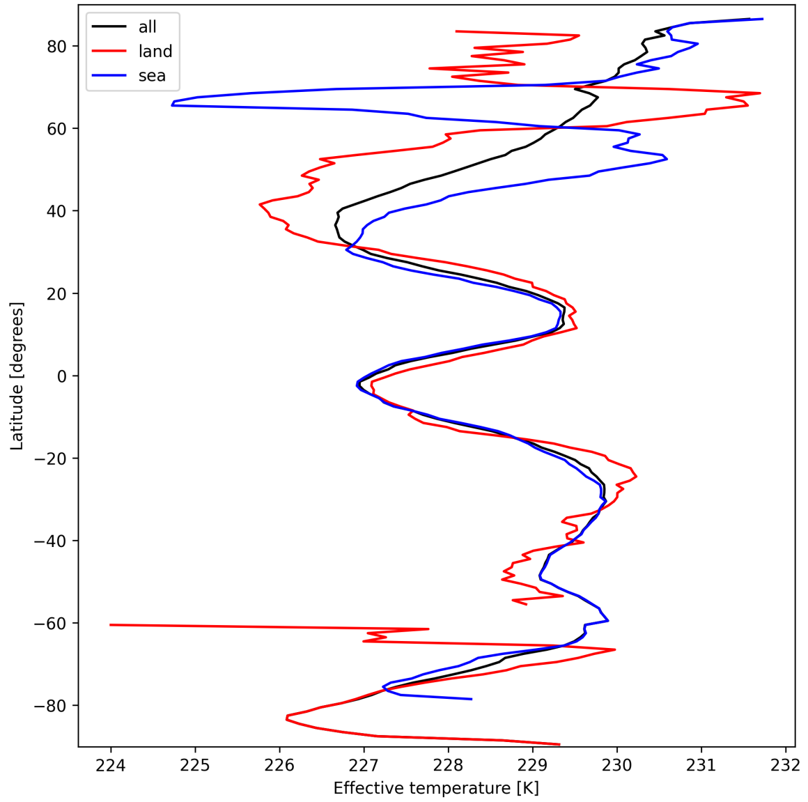
Figure 17: Zonal average of “Effective temperature” for 2025-03-13 to 2025-03-15.
