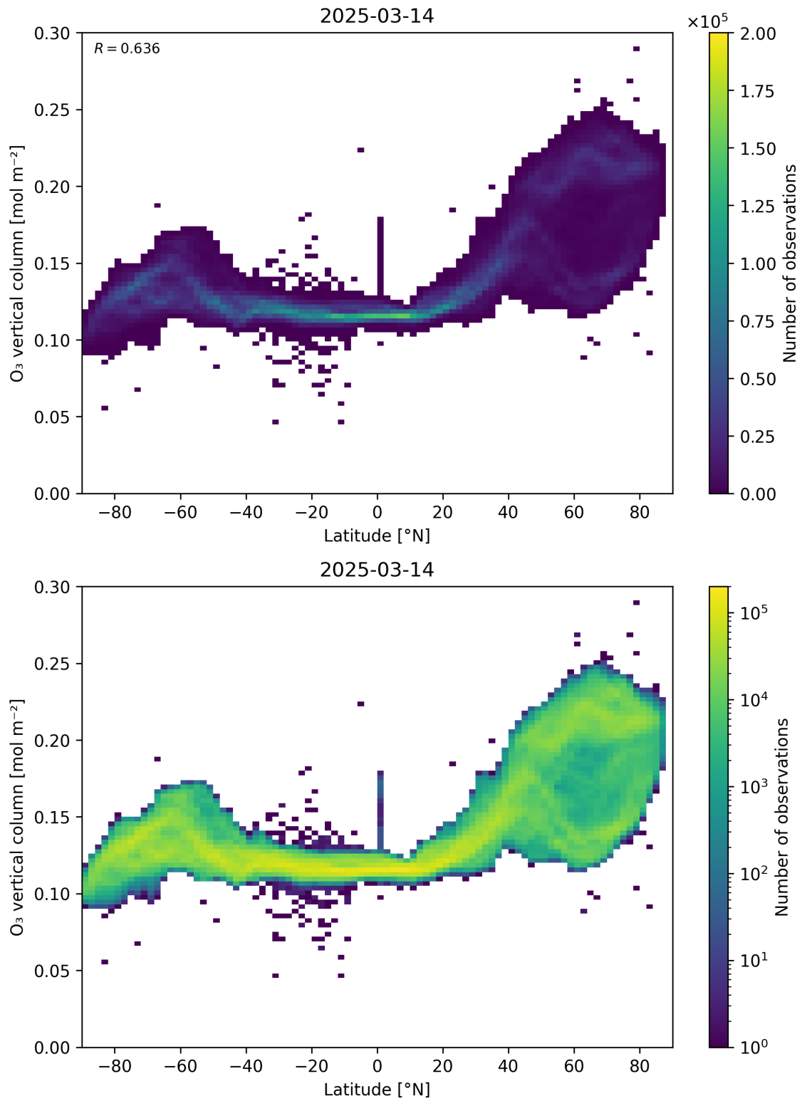
Figure 36: Scatter density plot of “Latitude” against “O 3 vertical column” for 2025-03-13 to 2025-03-15.
