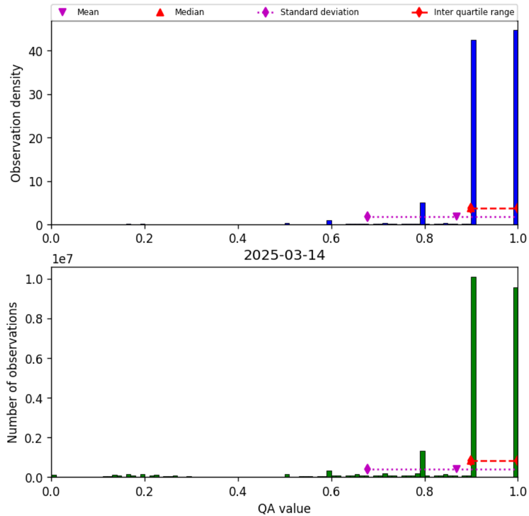
Figure 20: Histogram of “QA value” for 2025-03-13 to 2025-03-15
