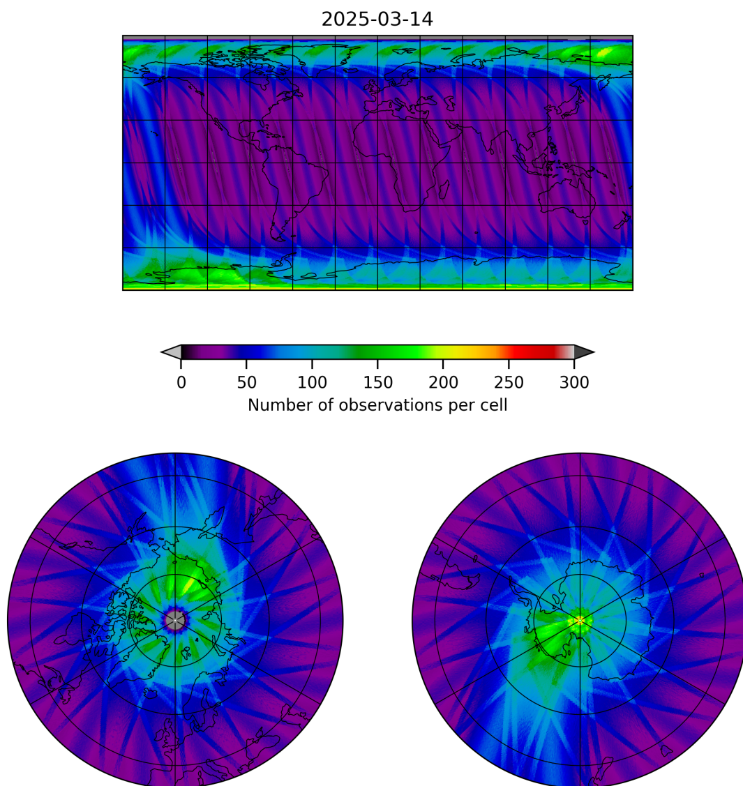
Figure 12: Map of the number of observations for 2025-03-13 to 2025-03-15
