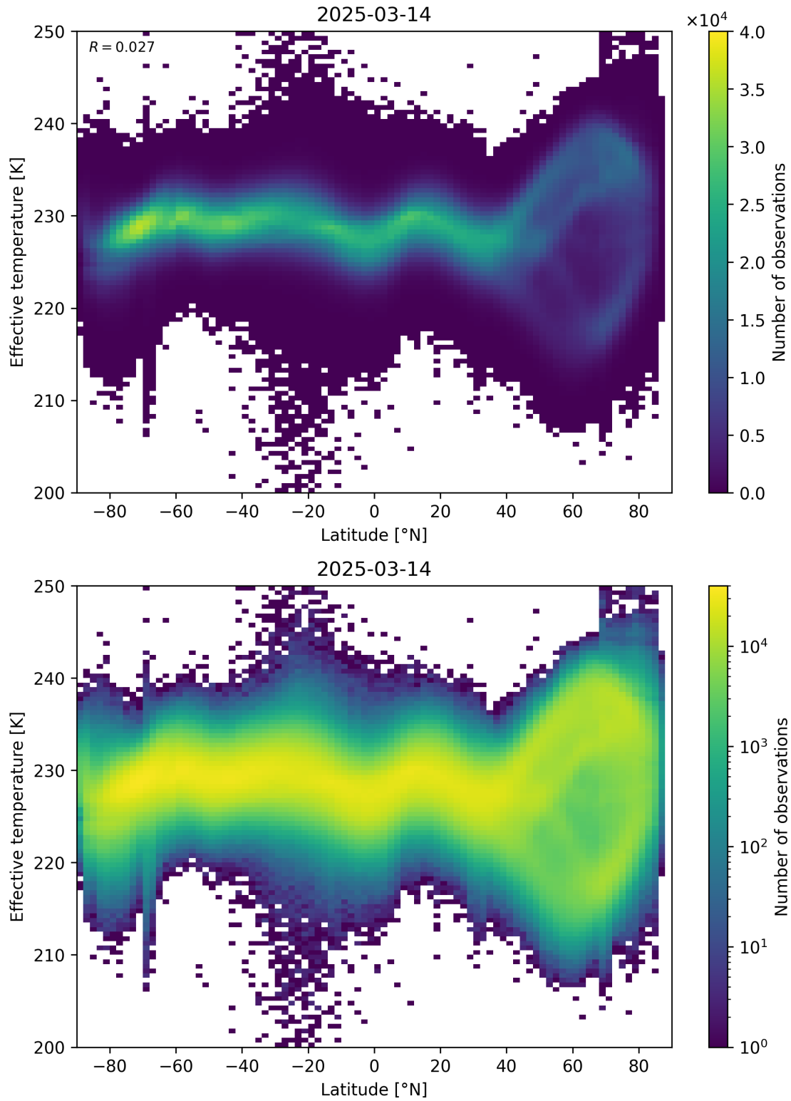
Figure 34: Scatter density plot of “Latitude” against “Effective temperature” for 2025-03-13 to 2025-03-15.
