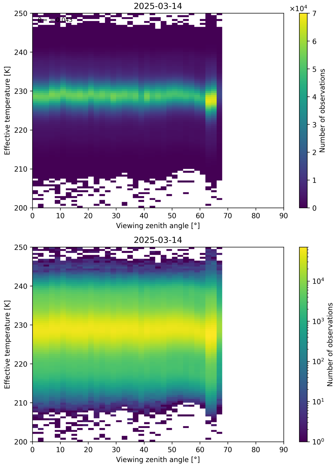
Figure 50: Scatter density plot of “Viewing zenith angle” against “Effective temperature” for 2025-03-13 to 2025-03-15.
