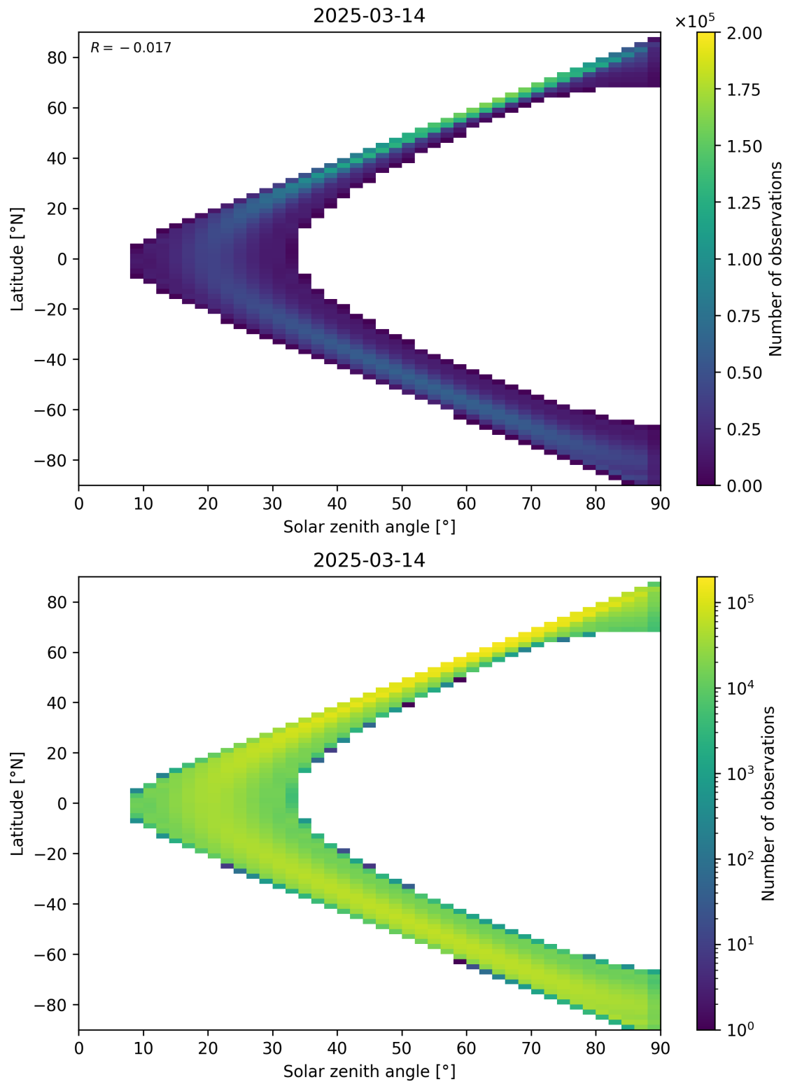
Figure 44: Scatter density plot of “Solar zenith angle” against “Latitude” for 2025-03-13 to 2025-03-15.
