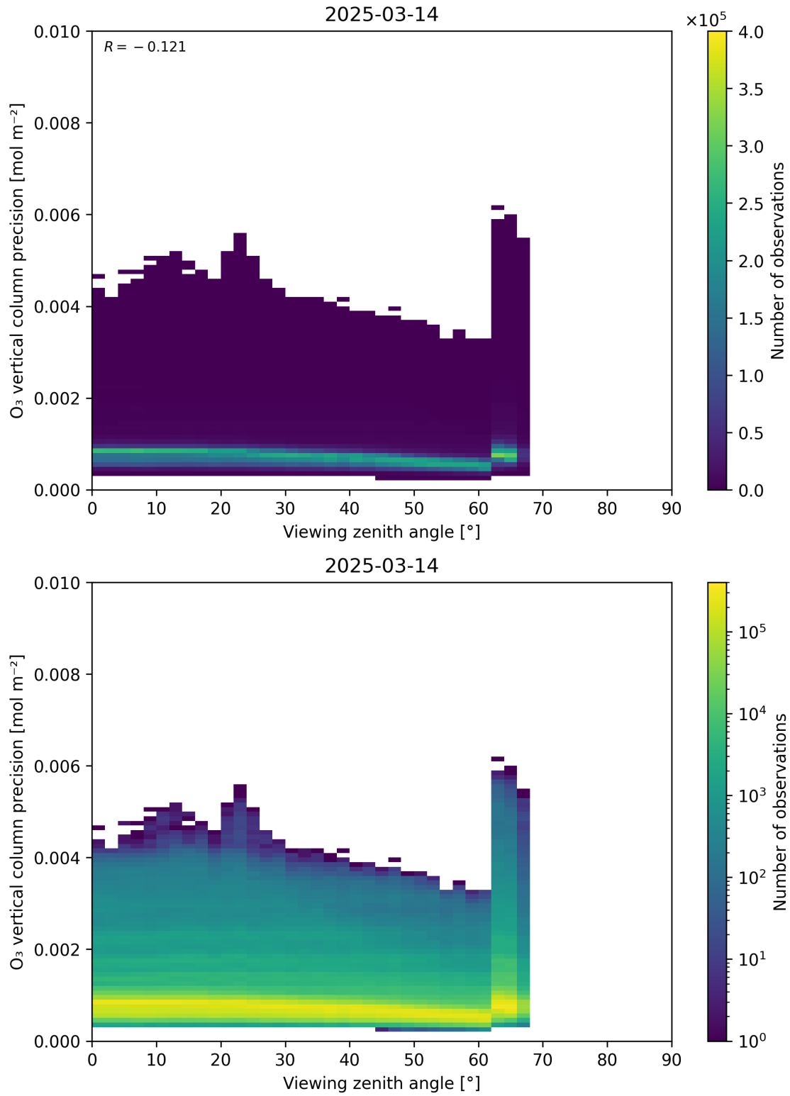
Figure 53: Scatter density plot of “Viewing zenith angle” against “O 3 vertical column precision” for 2025-03-13 to 2025-03-15.
