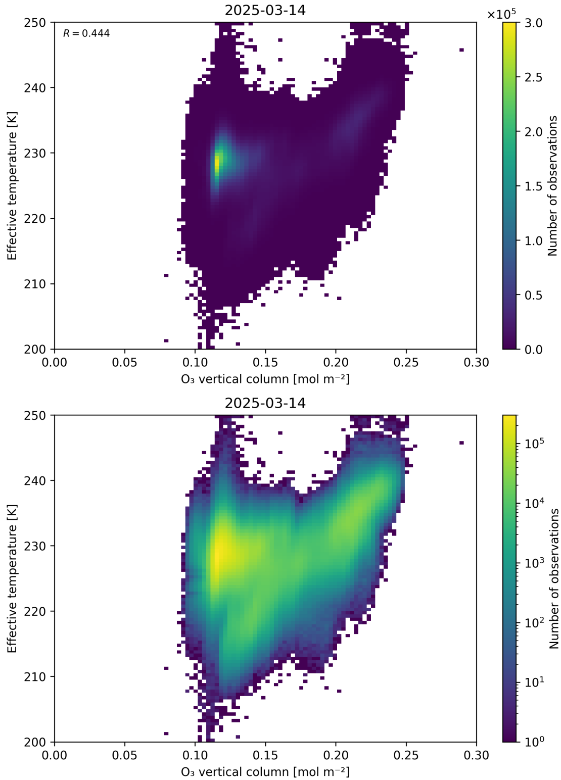
Figure 39: Scatter density plot of “O 3 vertical column” against “Effective temperature” for 2025-03-13 to 2025-03-15.
