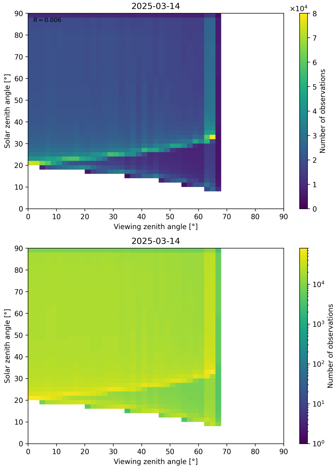
Figure 54: Scatter density plot of “Viewing zenith angle” against “Solar zenith angle” for 2025-03-13 to 2025-03-15.
