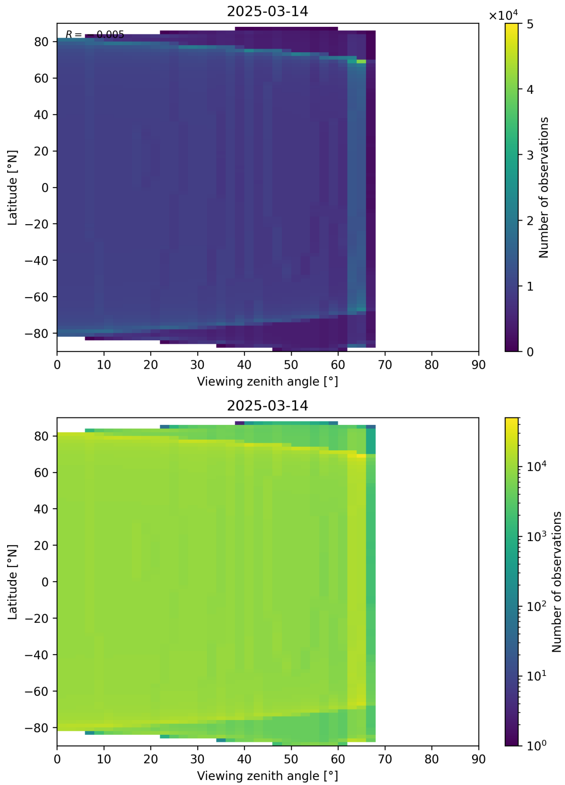
Figure 49: Scatter density plot of “Viewing zenith angle” against “Latitude” for 2025-03-13 to 2025-03-15.
