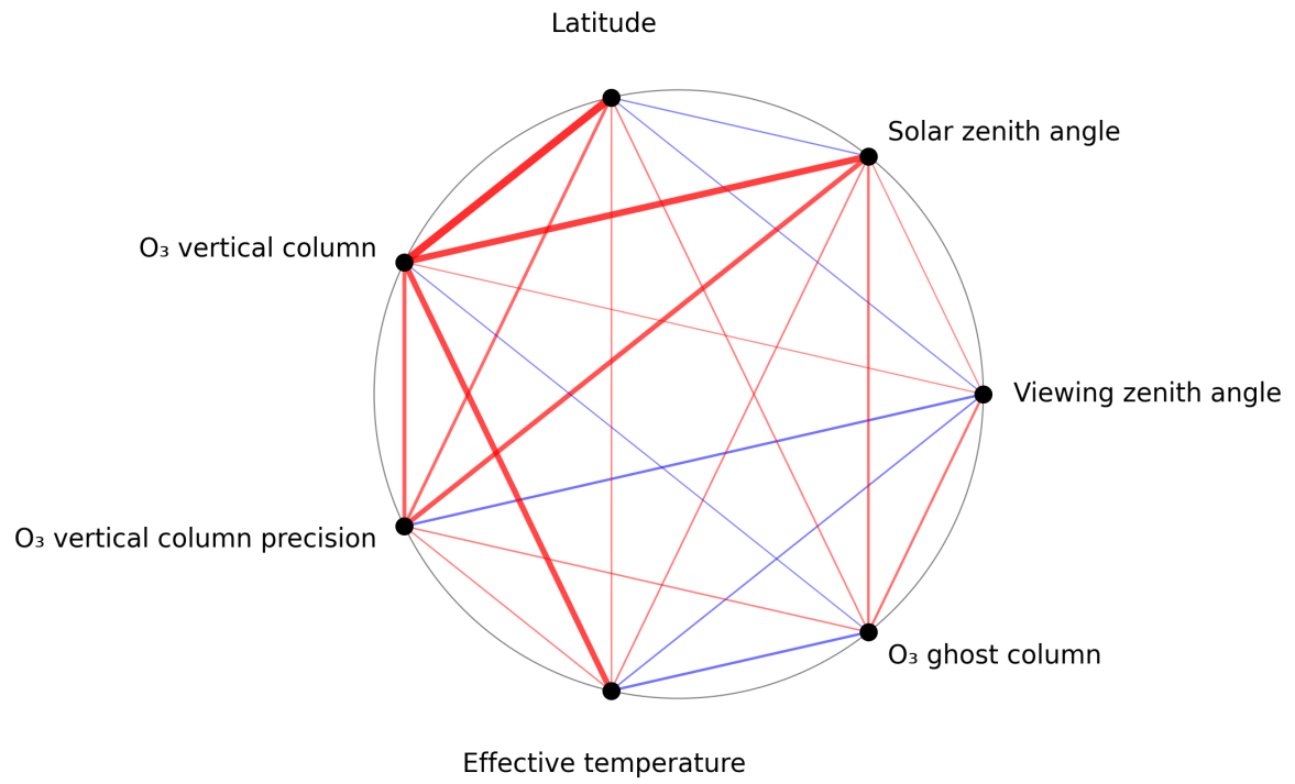
Figure 1: Map of correlation graph for 2025-03-13 to 2025-03-15.
