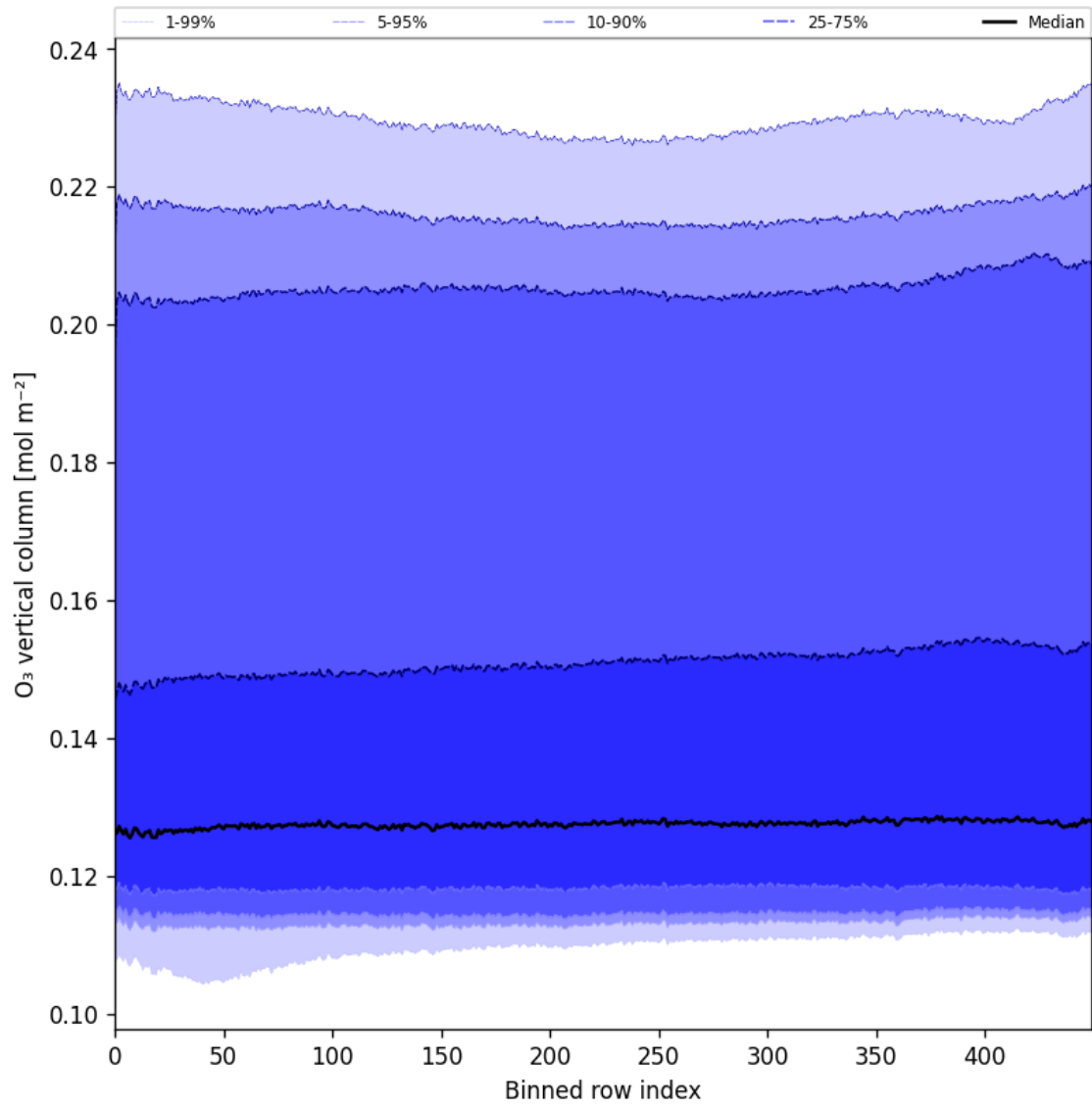
Figure 28: Along track statistics of “O 3 vertical column” for 2025-03-13 to 2025-03-15
