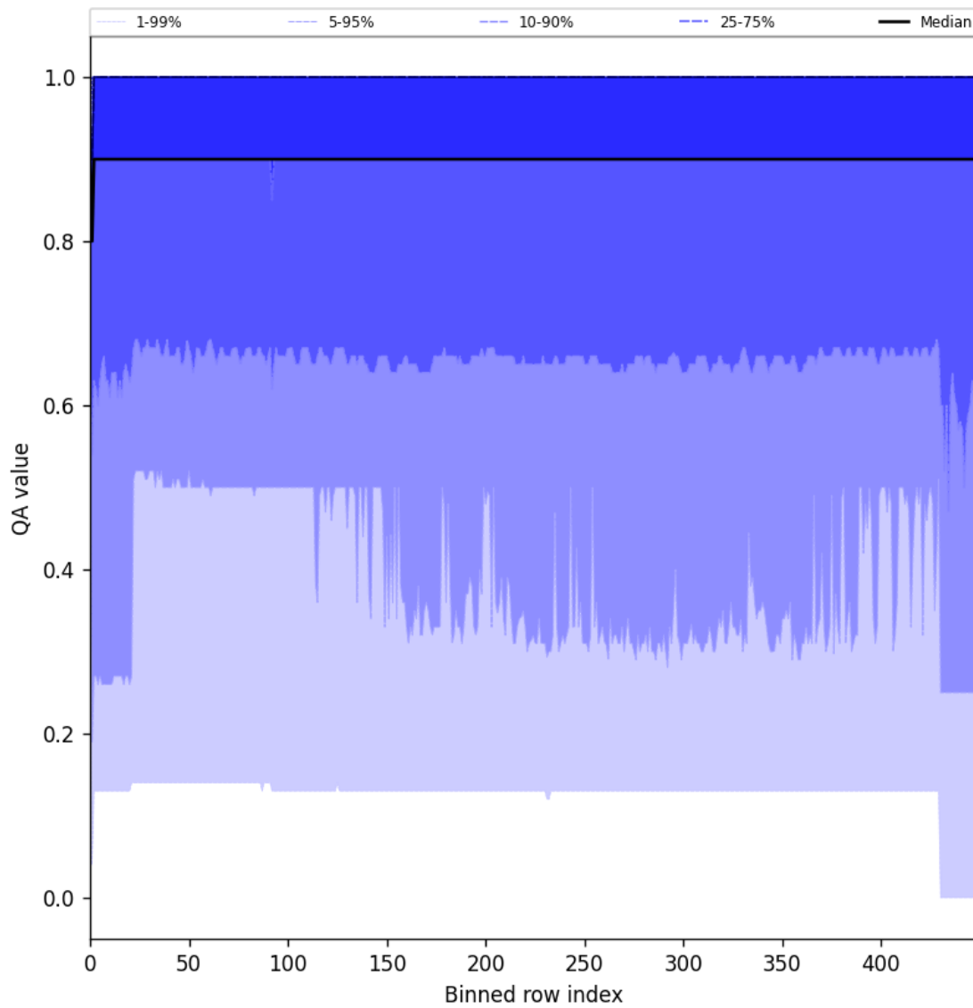
Figure 27: Along track statistics of “QA value” for 2025-03-13 to 2025-03-15
