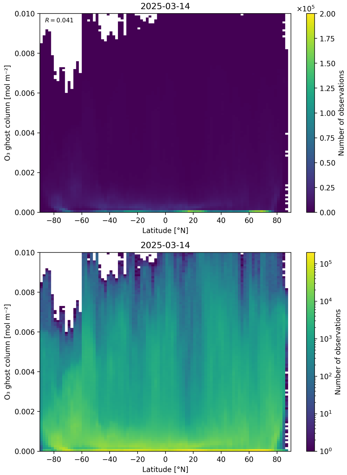
Figure 35: Scatter density plot of “Latitude” against “O 3 ghost column” for 2025-03-13 to 2025-03-15.
