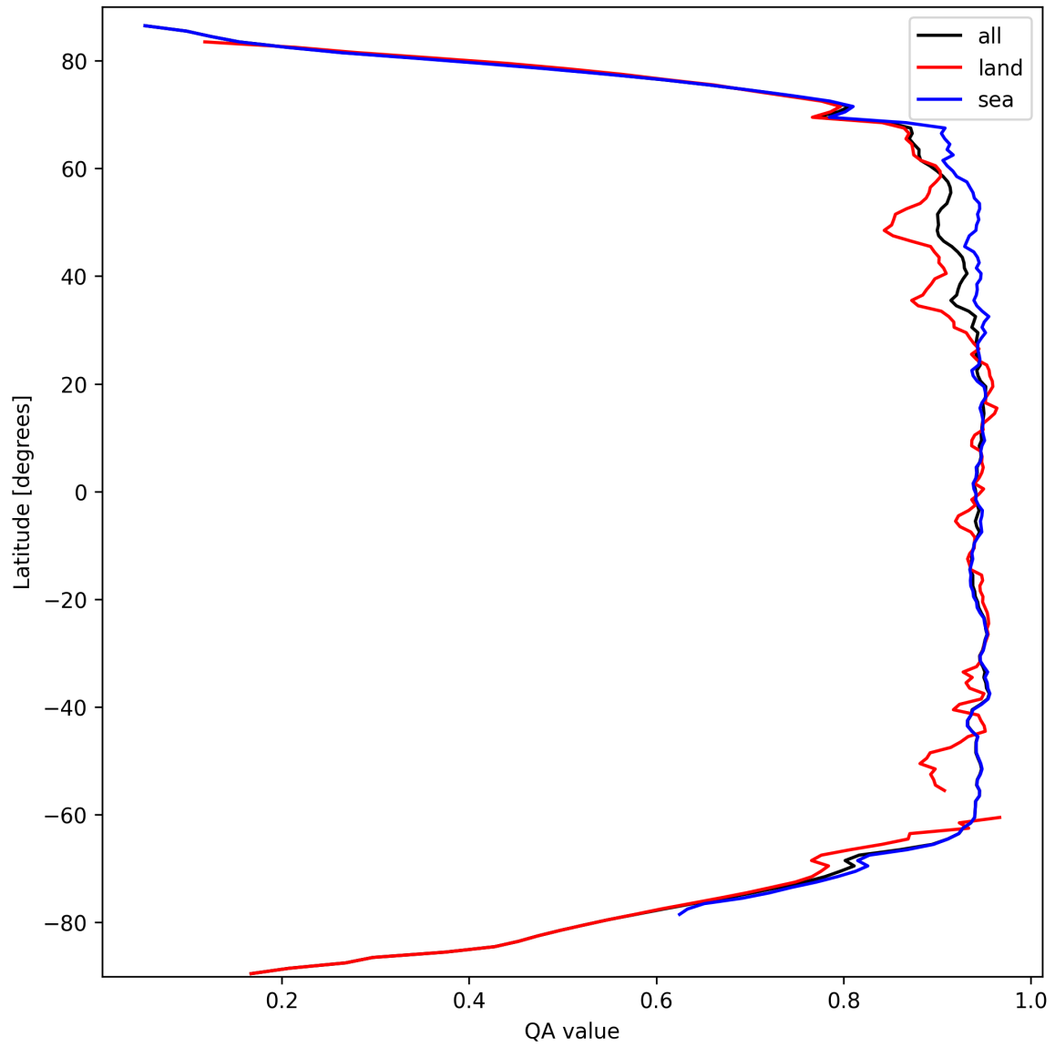
Figure 13: Zonal average of “QA value” for 2025-03-13 to 2025-03-15.
