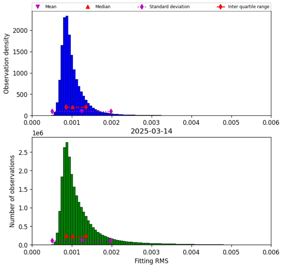
Figure 23: Histogram of “Fitting RMS” for 2025-03-13 to 2025-03-15
