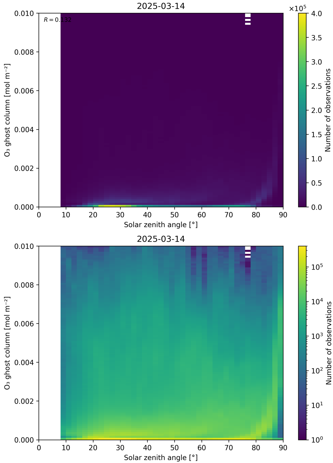
Figure 46: Scatter density plot of “Solar zenith angle” against “O 3 ghost column” for 2025-03-13 to 2025-03-15.
