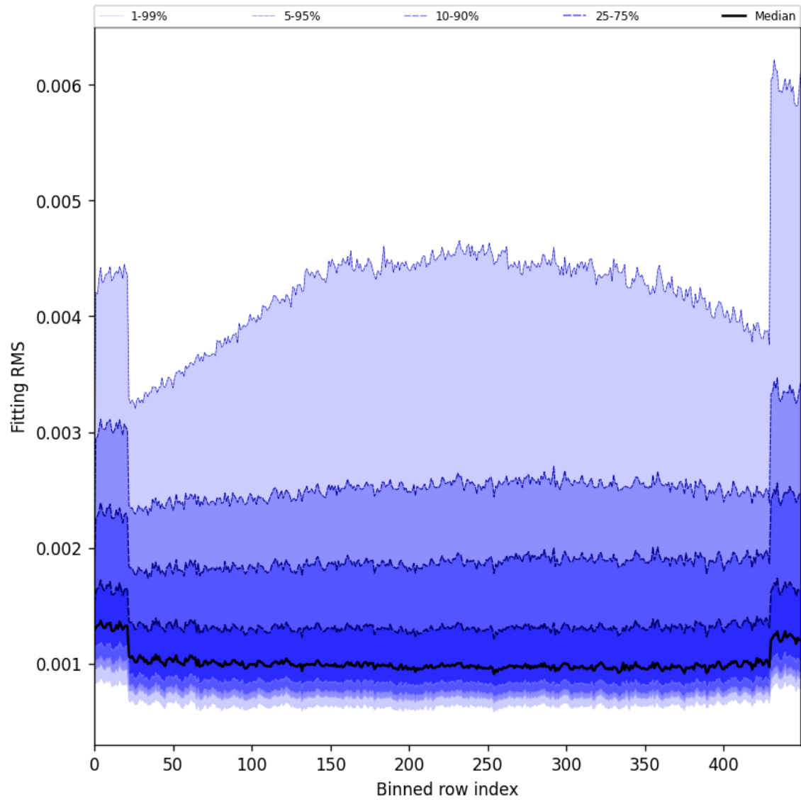
Figure 30: Along track statistics of “Fitting RMS” for 2025-03-13 to 2025-03-15
