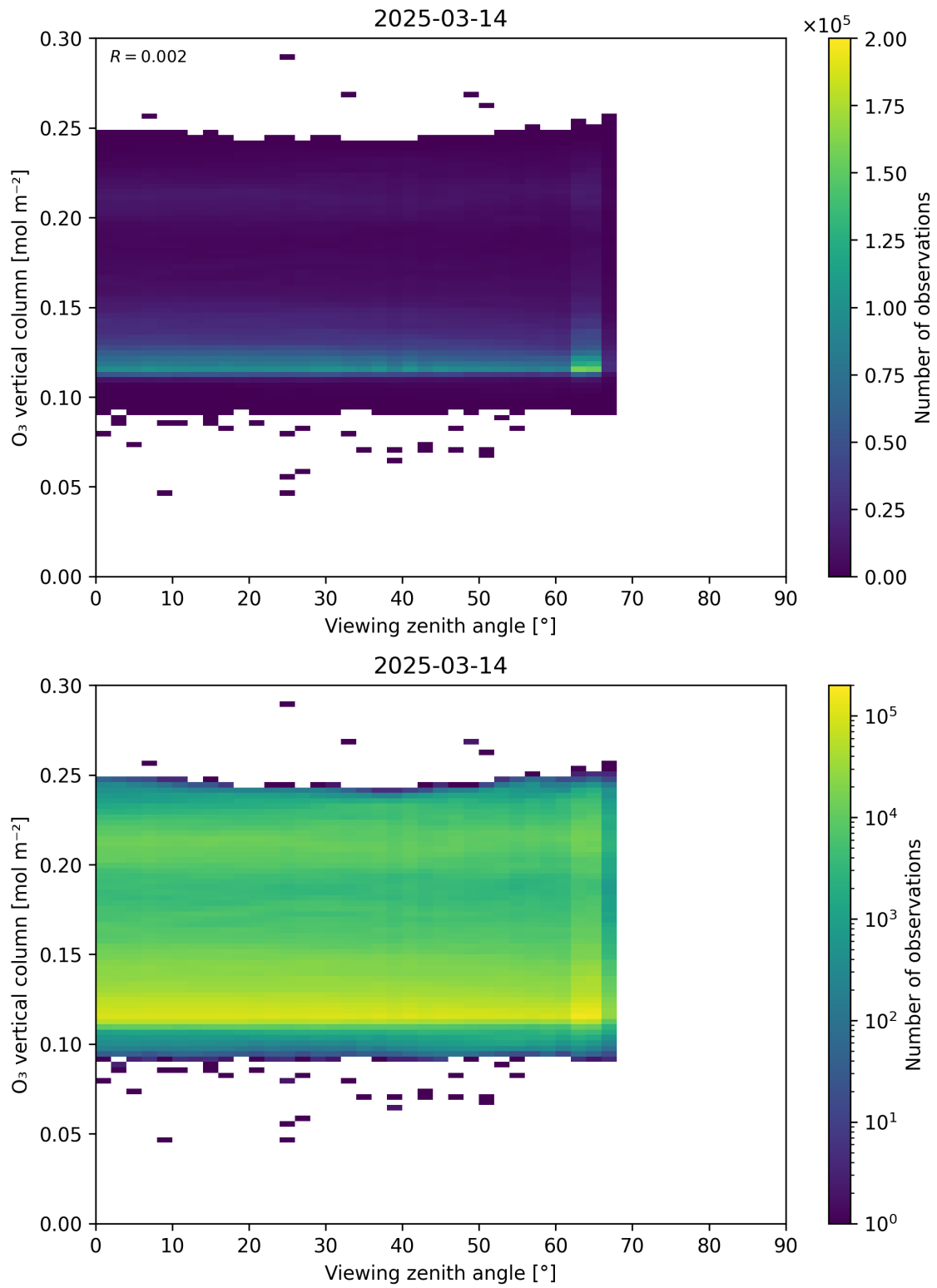
Figure 52: Scatter density plot of “Viewing zenith angle” against “O 3 vertical column” for 2025-03-13 to 2025-03-15.
