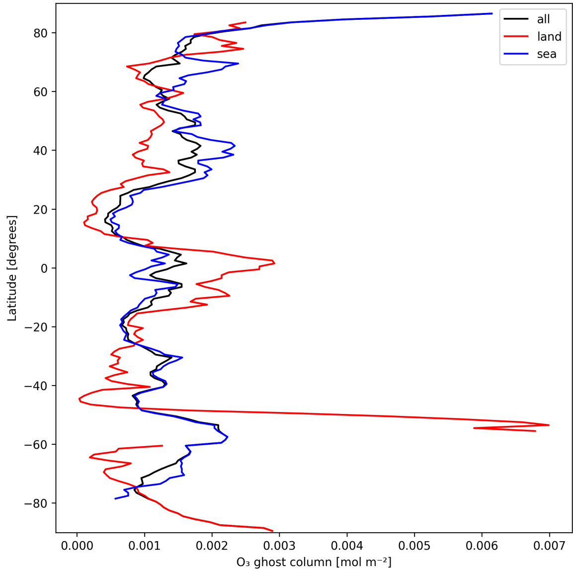
Figure 18: Zonal average of "O 3 ghost column" for 2025-03-13 to 2025-03-15.
