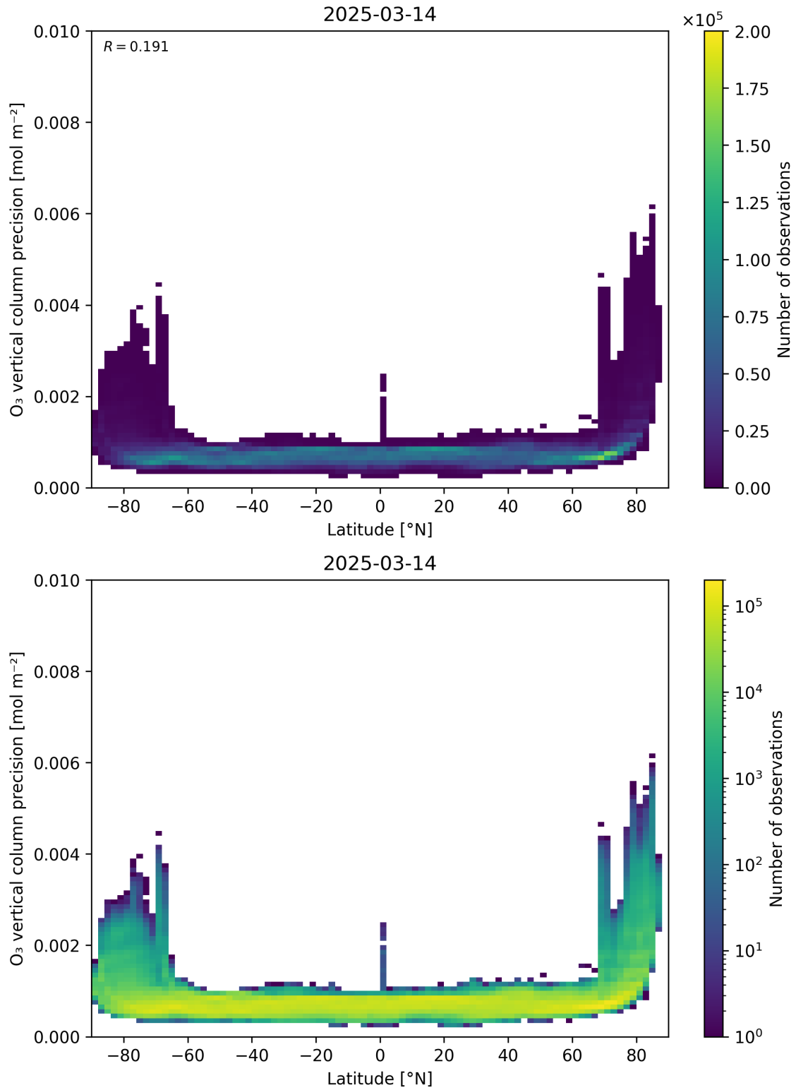
Figure 37: Scatter density plot of “Latitude” against “O 3 vertical column precision” for 2025-03-13 to 2025-03-15.
