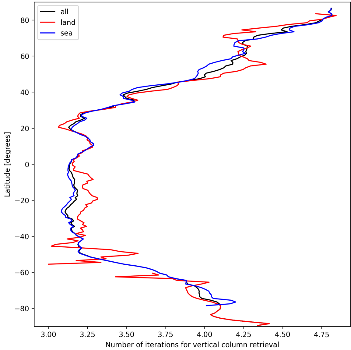
Figure 19: Zonal average of “Number of iterations for vertical column retrieval” for 2025-03-13 to 2025-03-15.
