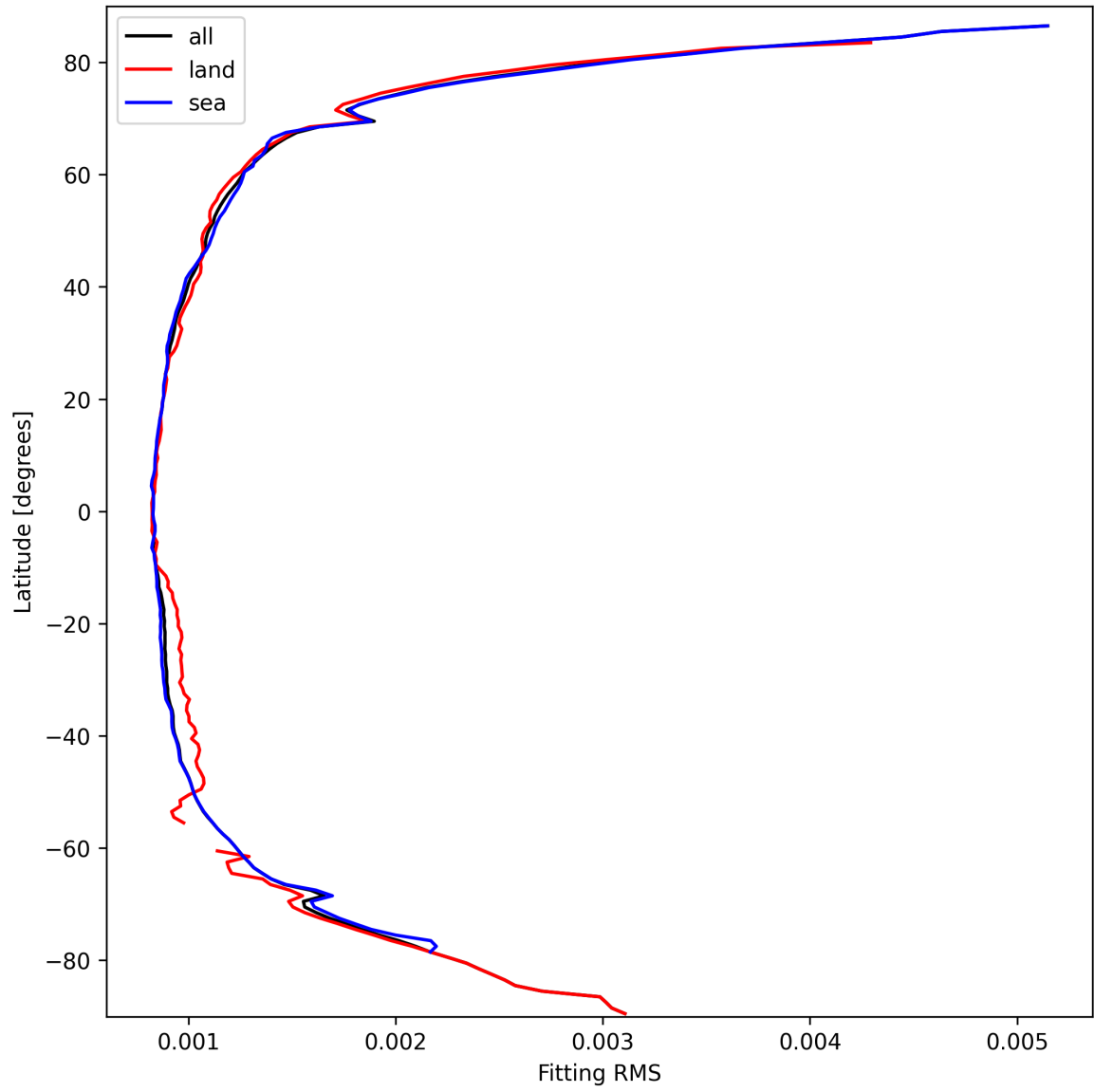
Figure 16: Zonal average of “Fitting RMS” for 2025-03-13 to 2025-03-15.
