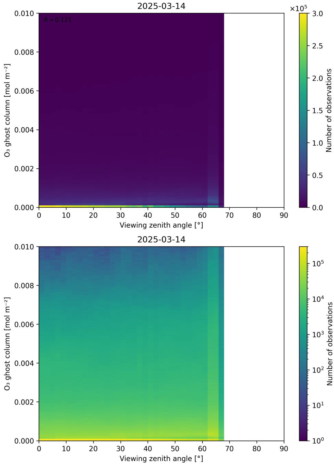
Figure 51: Scatter density plot of “Viewing zenith angle” against “O 3 ghost column” for 2025-03-13 to 2025-03-15.
