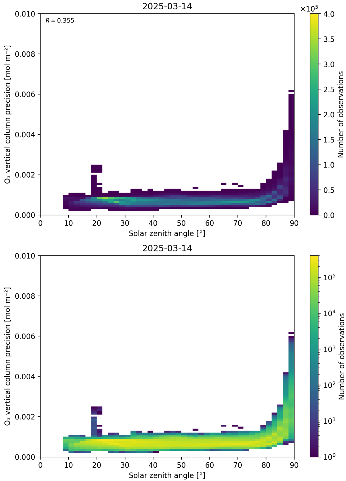
Figure 48: Scatter density plot of “Solar zenith angle” against “O 3 vertical column precision” for 2025-03-13 to 2025-03-15.
