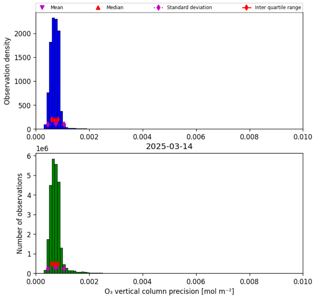
Figure 22: Histogram of “O 3 vertical column precision” for 2025-03-13 to 2025-03-15
