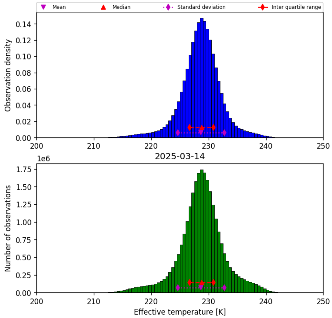
Figure 24: Histogram of “Effective temperature” for 2025-03-13 to 2025-03-15
