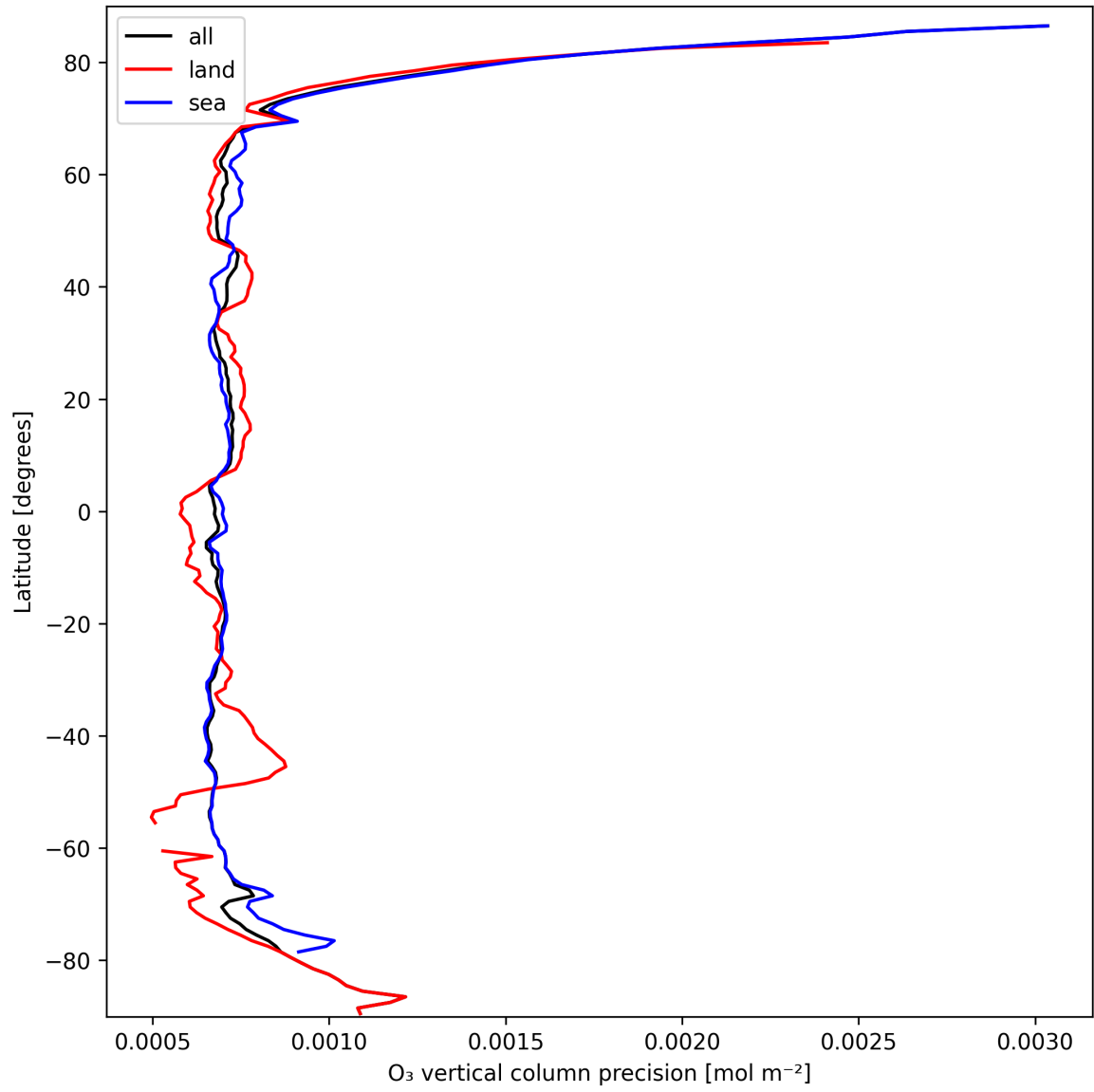
Figure 15: Zonal average of “O 3 vertical column precision” for 2025-03-13 to 2025-03-15.
