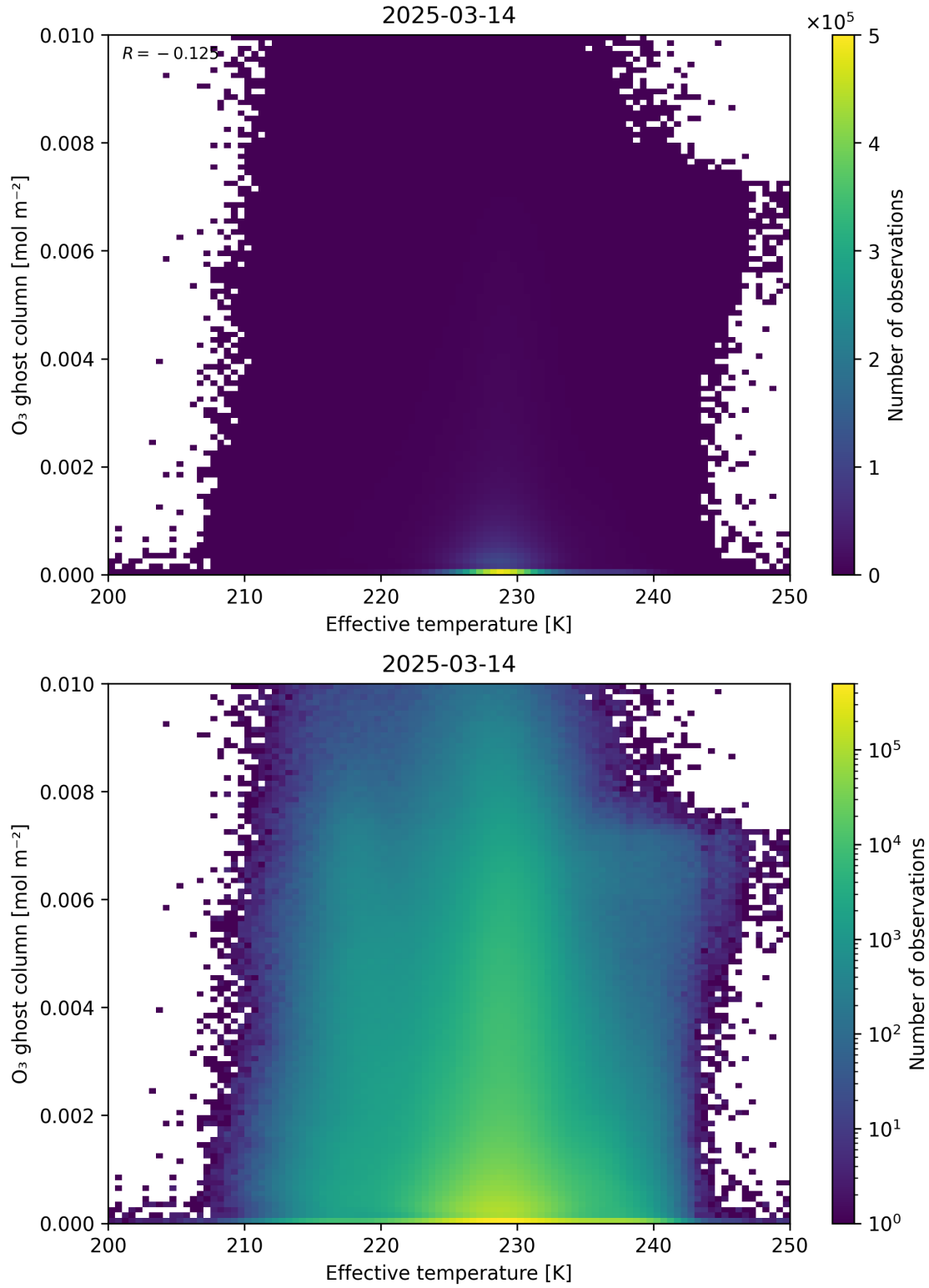
Figure 38: Scatter density plot of “Effective temperature” against “O 3 ghost column” for 2025-03-13 to 2025-03-15.
