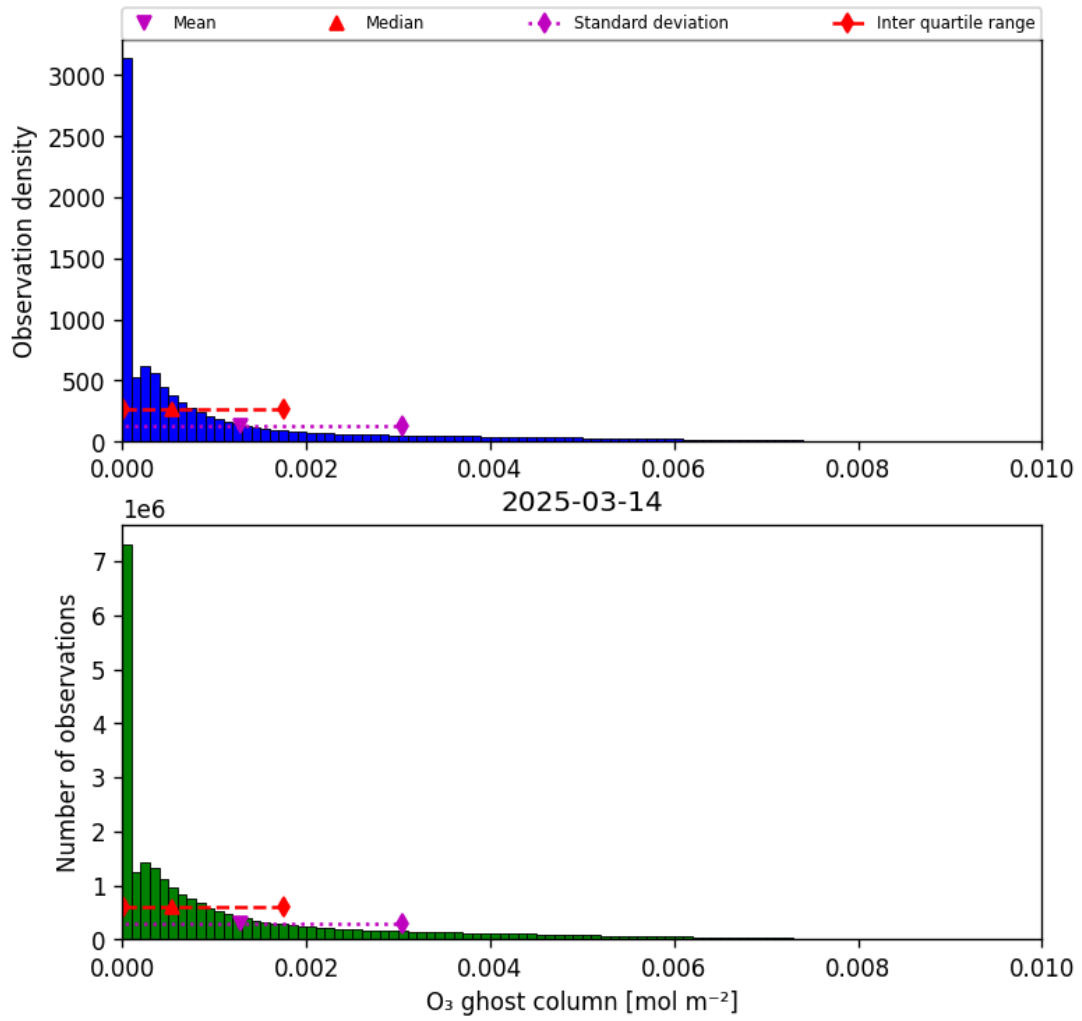
Figure 25: Histogram of "O 3 ghost column" for 2025-03-13 to 2025-03-15
