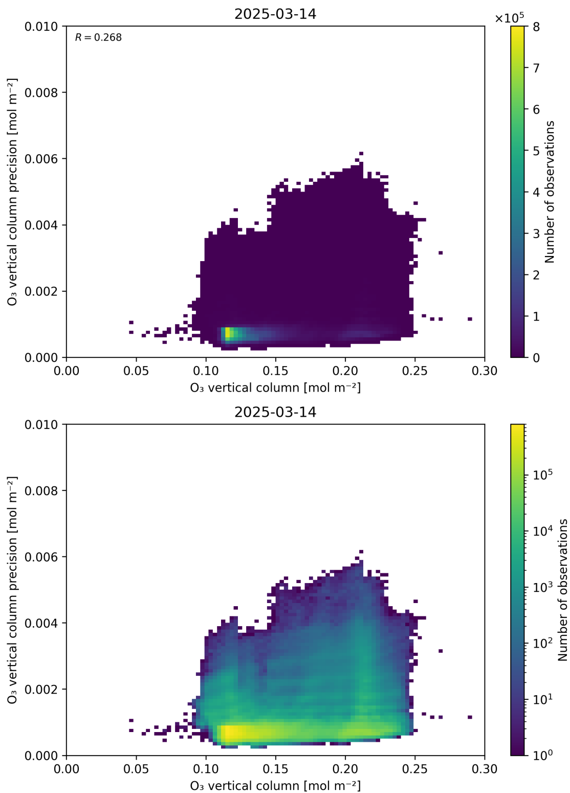
Figure 41: Scatter density plot of “O 3 vertical column” against “O 3 vertical column precision” for 2025-03-13 to 2025-03-15.
