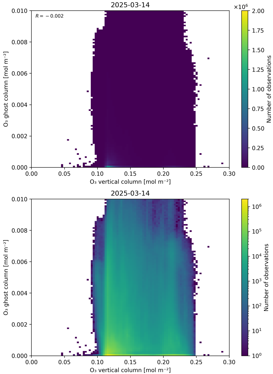
Figure 40: Scatter density plot of “O 3 vertical column” against “O 3 ghost column” for 2025-03-13 to 2025-03-15.
