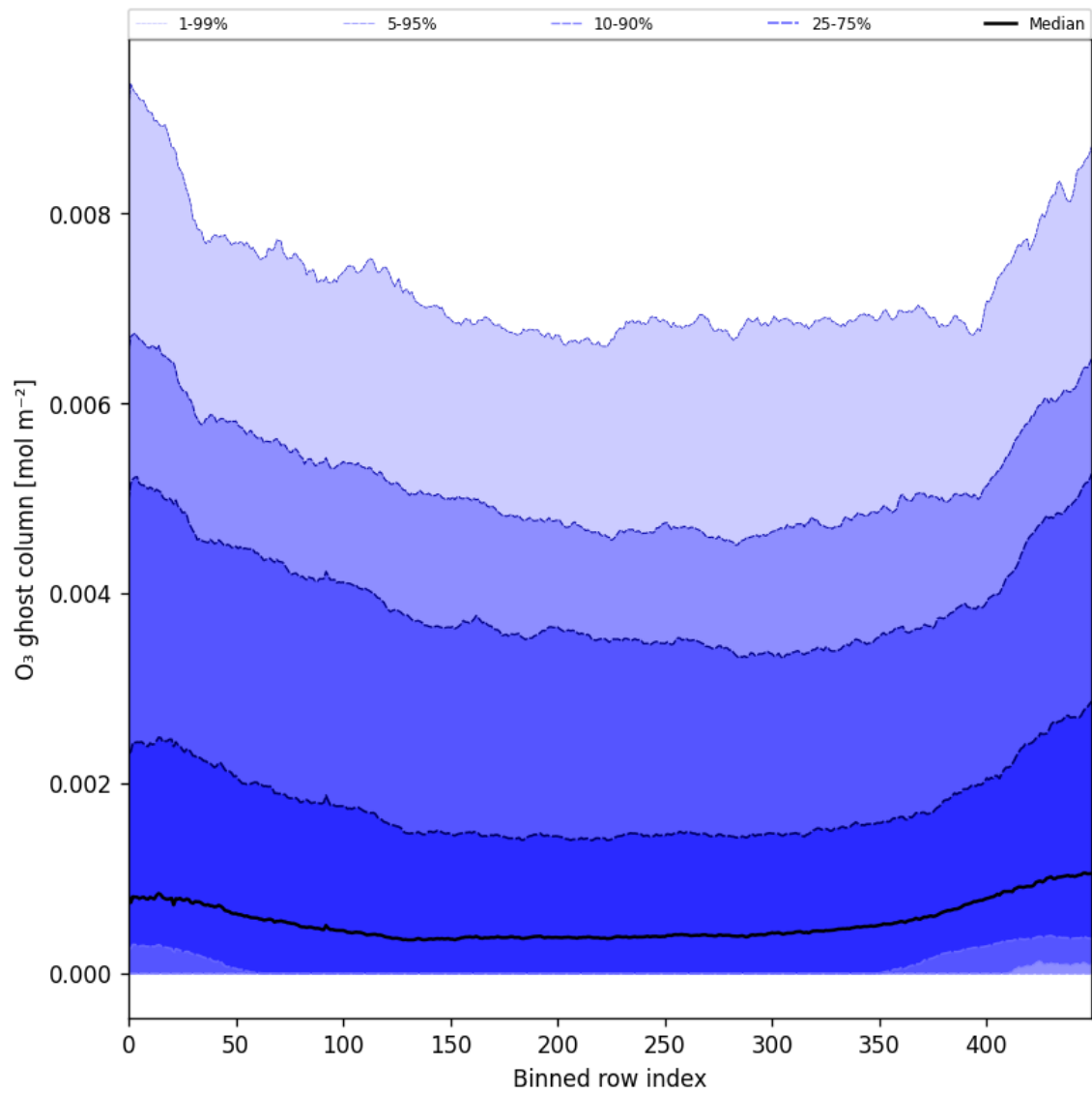
Figure 32: Along track statistics of “O 3 ghost column” for 2025-03-13 to 2025-03-15
