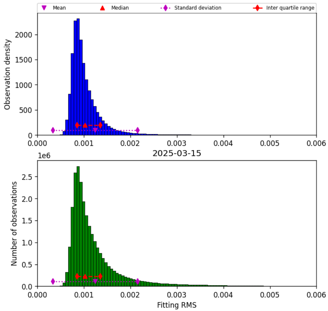
Figure 23: Histogram of “Fitting RMS” for 2025-03-14 to 2025-03-16
