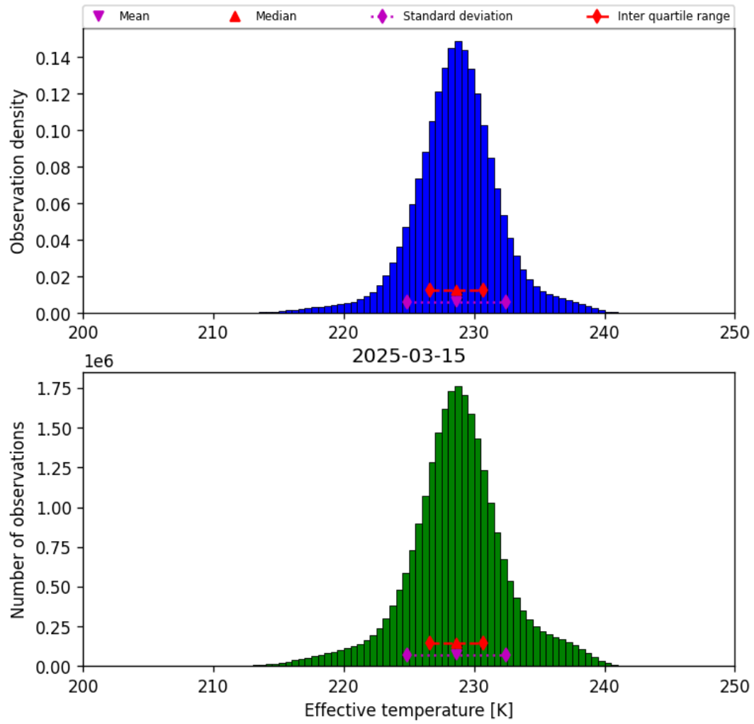
Figure 24: Histogram of “Effective temperature” for 2025-03-14 to 2025-03-16
