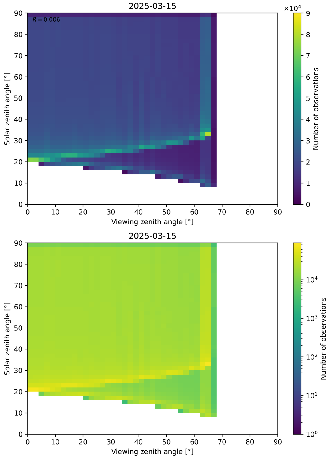
Figure 54: Scatter density plot of “Viewing zenith angle” against “Solar zenith angle” for 2025-03-14 to 2025-03-16.
