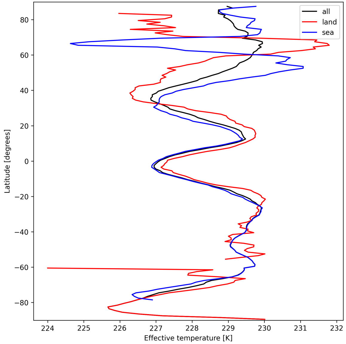
Figure 17: Zonal average of “Effective temperature” for 2025-03-14 to 2025-03-16.
