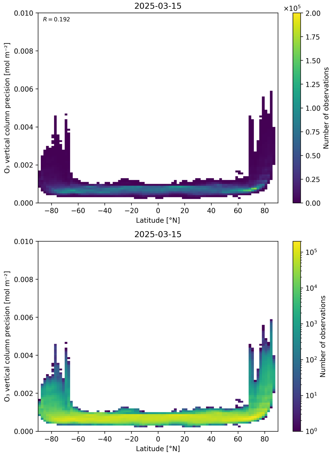
Figure 37: Scatter density plot of “Latitude” against “O 3 vertical column precision” for 2025-03-14 to 2025-03-16.
