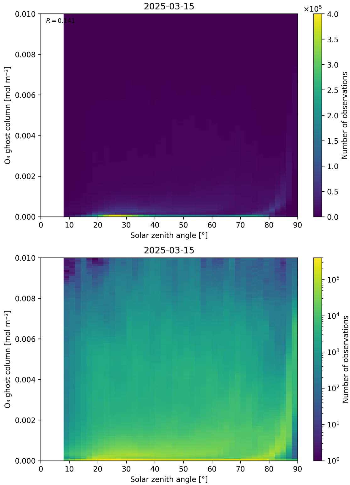
Figure 46: Scatter density plot of “Solar zenith angle” against “O 3 ghost column” for 2025-03-14 to 2025-03-16.
