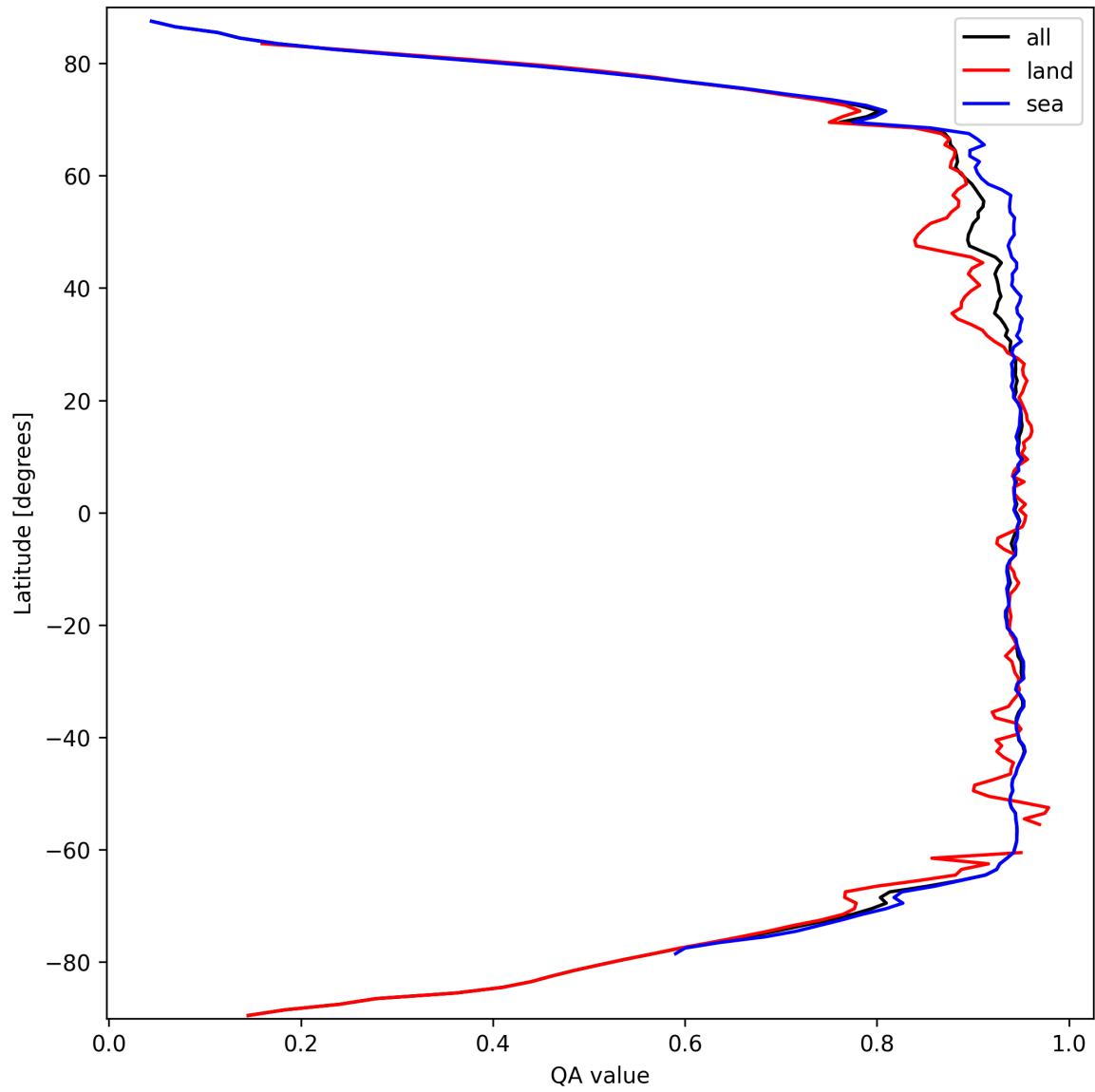
Figure 13: Zonal average of “QA value” for 2025-03-14 to 2025-03-16.
