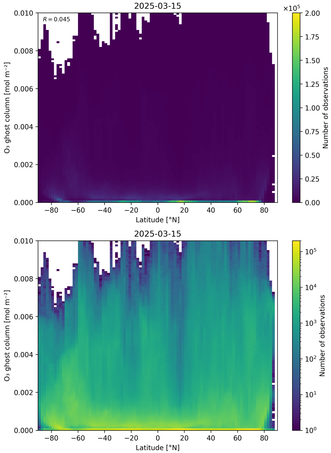
Figure 35: Scatter density plot of “Latitude” against “O 3 ghost column” for 2025-03-14 to 2025-03-16.
