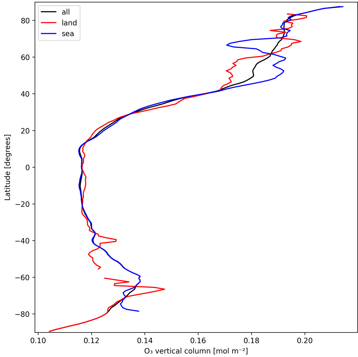
Figure 14: Zonal average of “O 3 vertical column” for 2025-03-14 to 2025-03-16.
