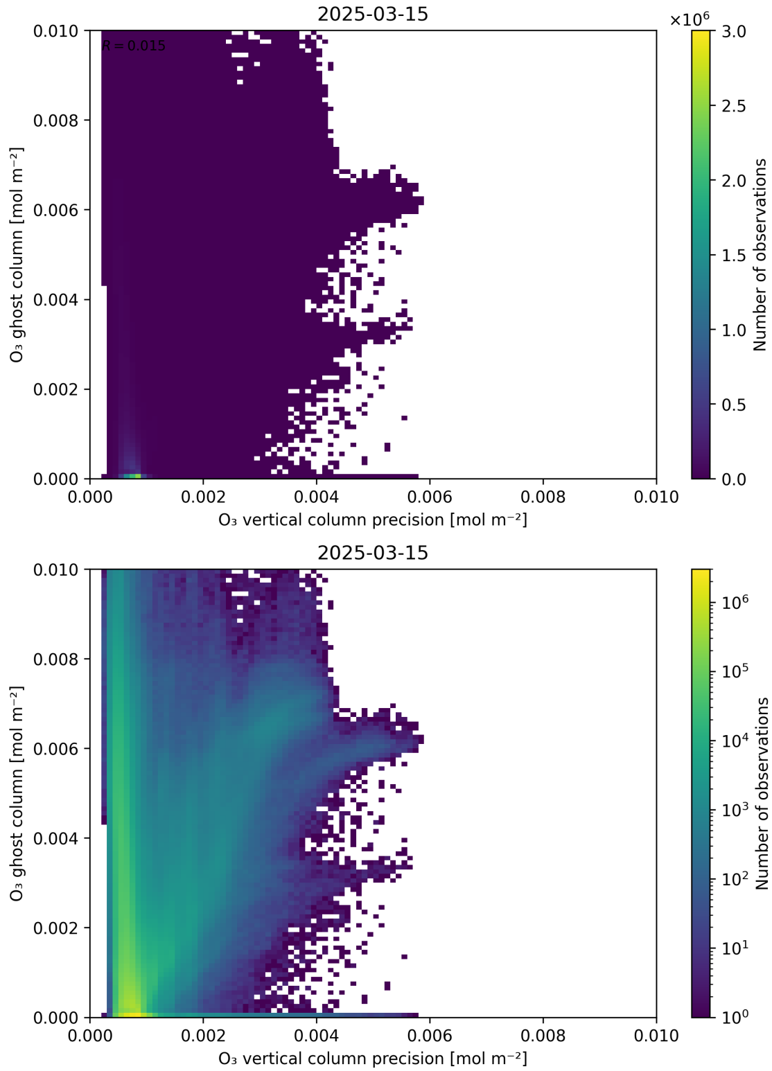
Figure 43: Scatter density plot of “O 3 vertical column precision” against “O 3 ghost column” for 2025-03-14 to 2025-03-16.
