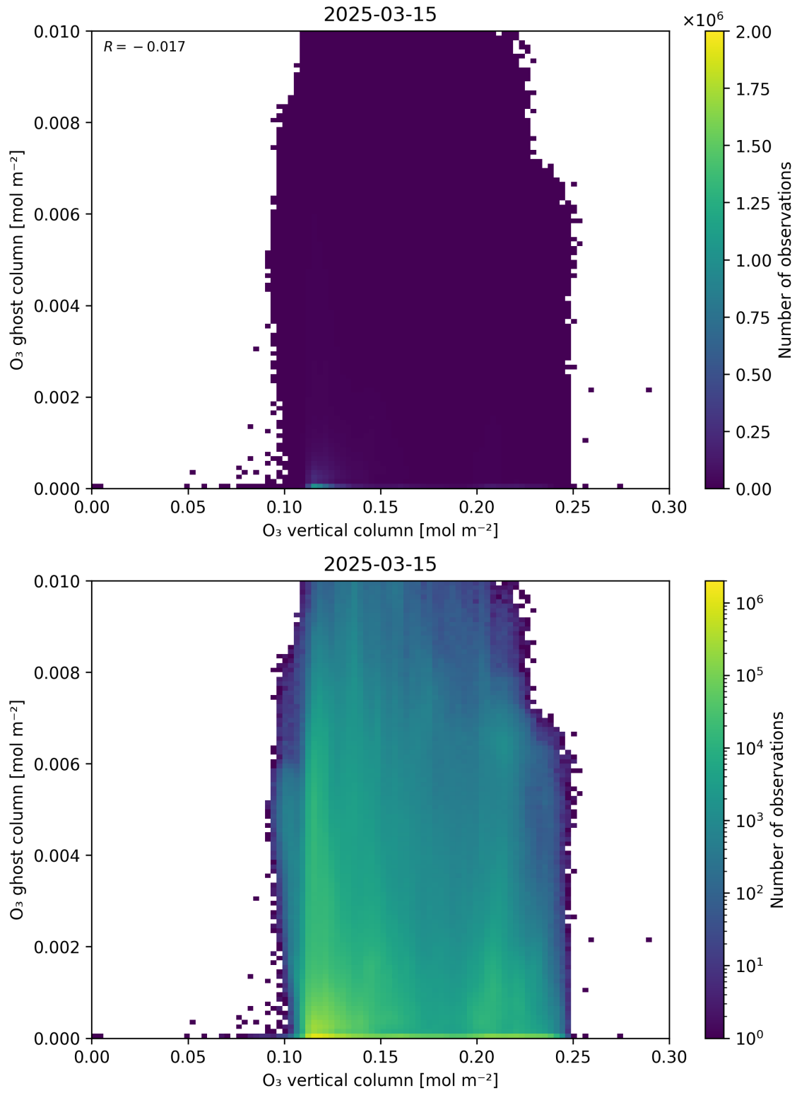
Figure 40: Scatter density plot of “O 3 vertical column” against “O 3 ghost column” for 2025-03-14 to 2025-03-16.
