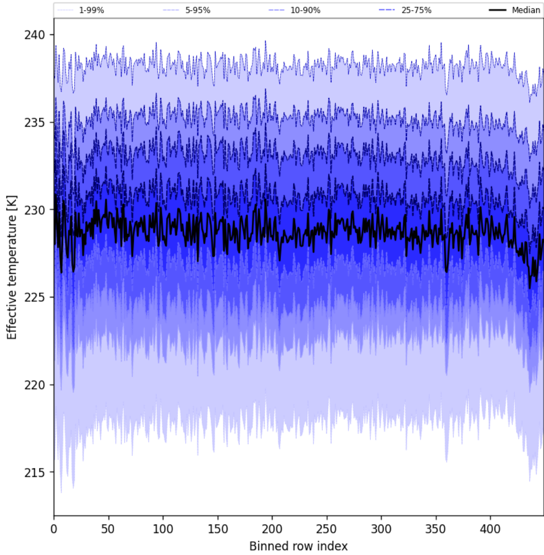
Figure 31: Along track statistics of “Effective temperature” for 2025-03-14 to 2025-03-16
