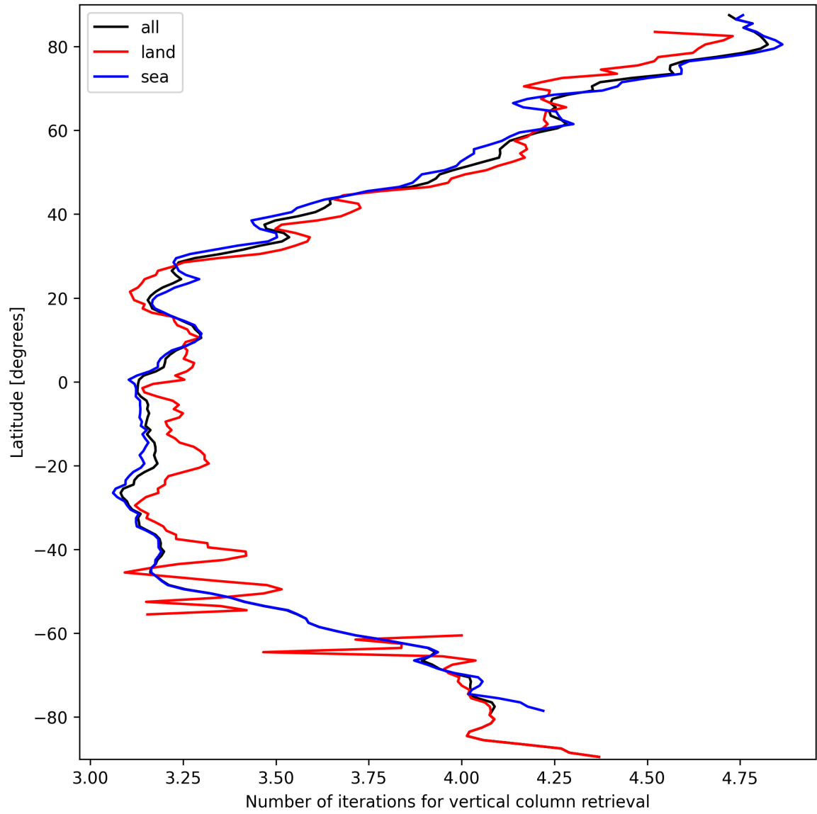
Figure 19: Zonal average of “Number of iterations for vertical column retrieval” for 2025-03-14 to 2025-03-16.
