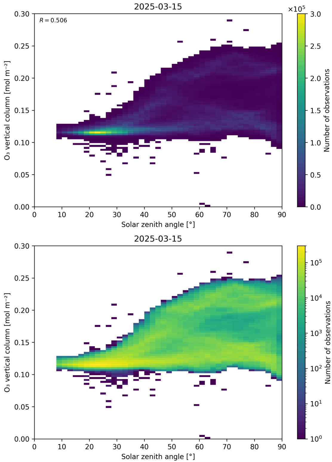
Figure 47: Scatter density plot of “Solar zenith angle” against “O 3 vertical column” for 2025-03-14 to 2025-03-16.
