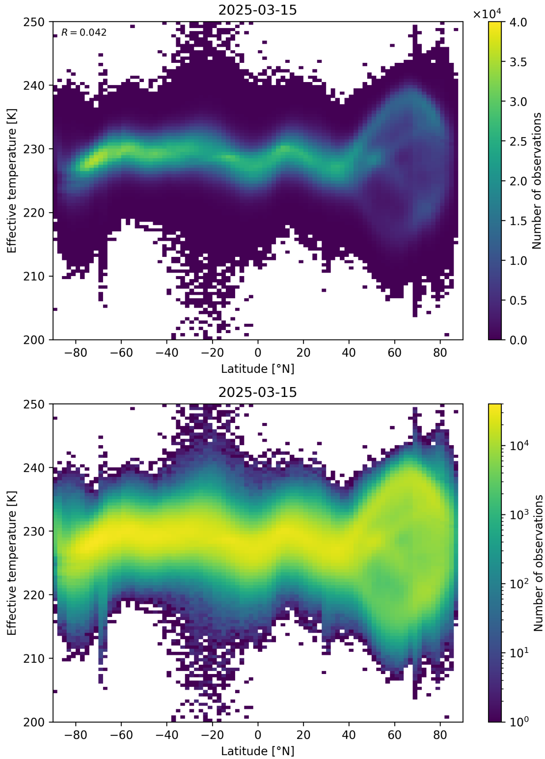
Figure 34: Scatter density plot of “Latitude” against “Effective temperature” for 2025-03-14 to 2025-03-16.
