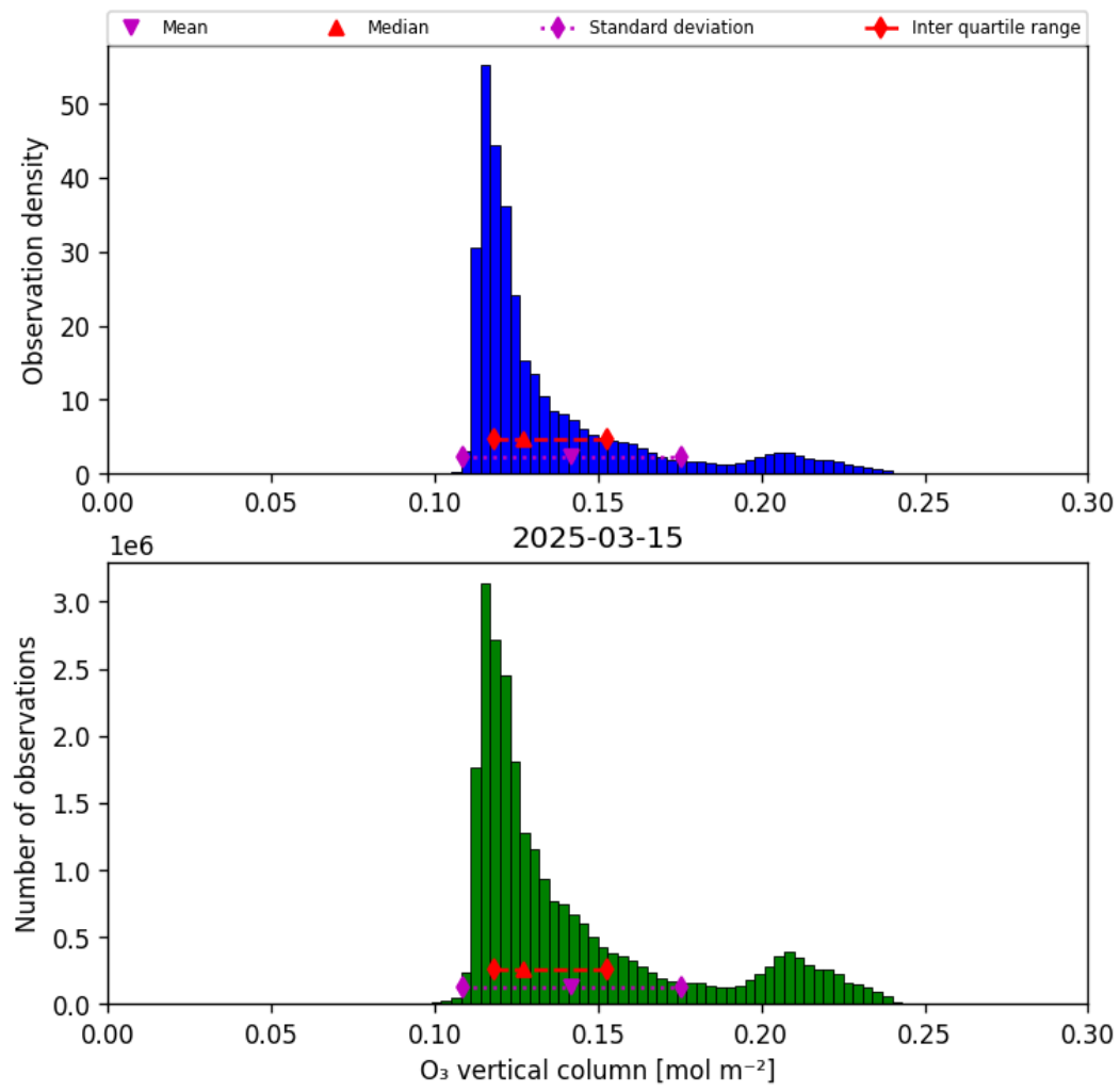
Figure 21: Histogram of “O 3 vertical column” for 2025-03-14 to 2025-03-16
