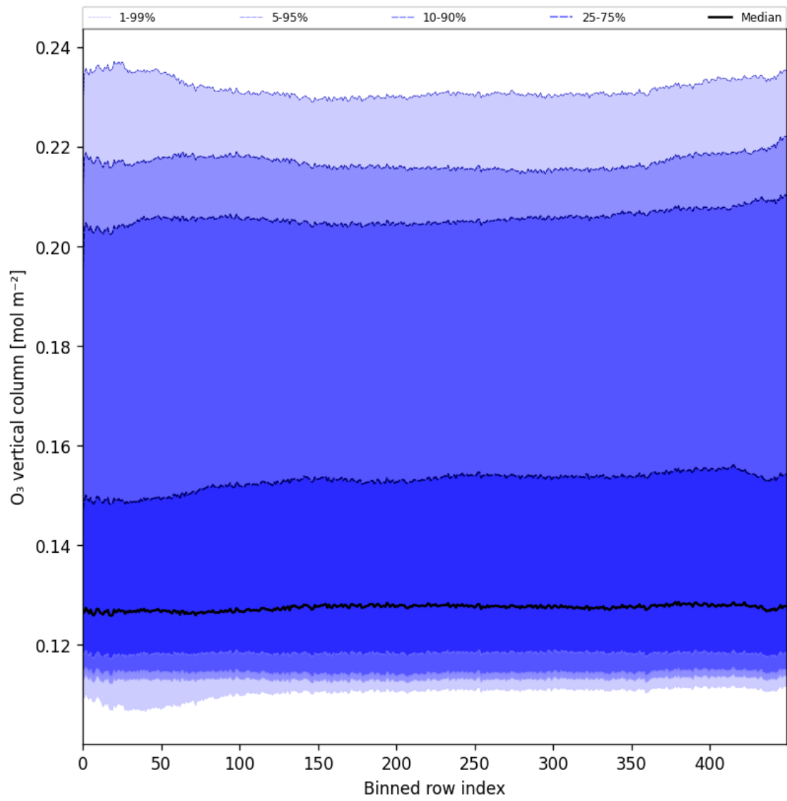
Figure 28: Along track statistics of “O 3 vertical column” for 2025-03-14 to 2025-03-16
