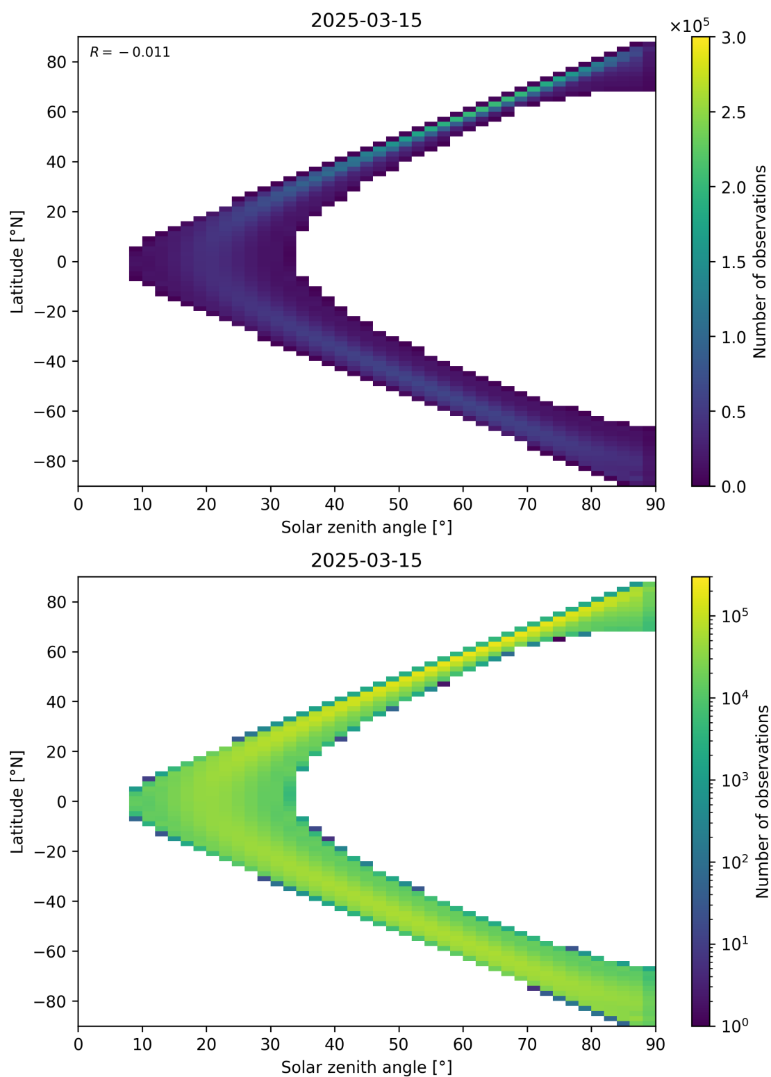
Figure 44: Scatter density plot of “Solar zenith angle” against “Latitude” for 2025-03-14 to 2025-03-16.
