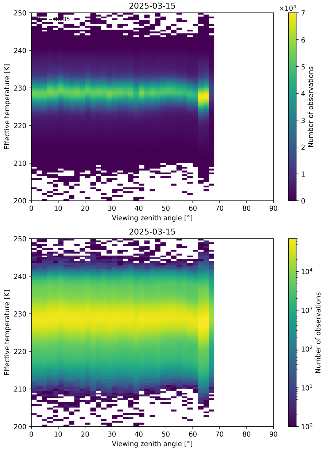
Figure 50: Scatter density plot of “Viewing zenith angle” against “Effective temperature” for 2025-03-14 to 2025-03-16.
