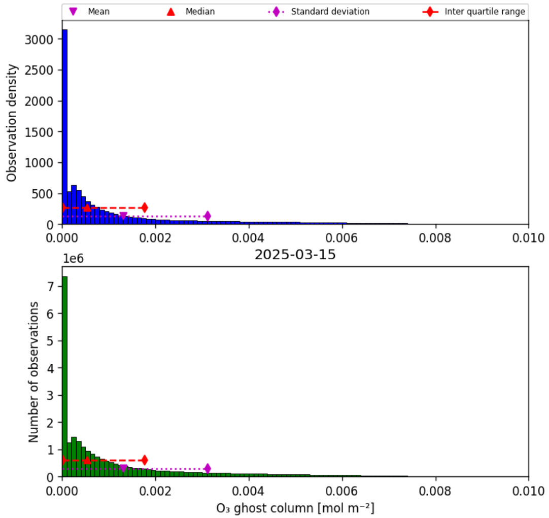
Figure 25: Histogram of “O 3 ghost column” for 2025-03-14 to 2025-03-16
