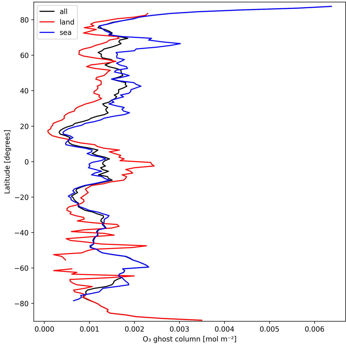
Figure 18: Zonal average of “O 3 ghost column” for 2025-03-14 to 2025-03-16.
