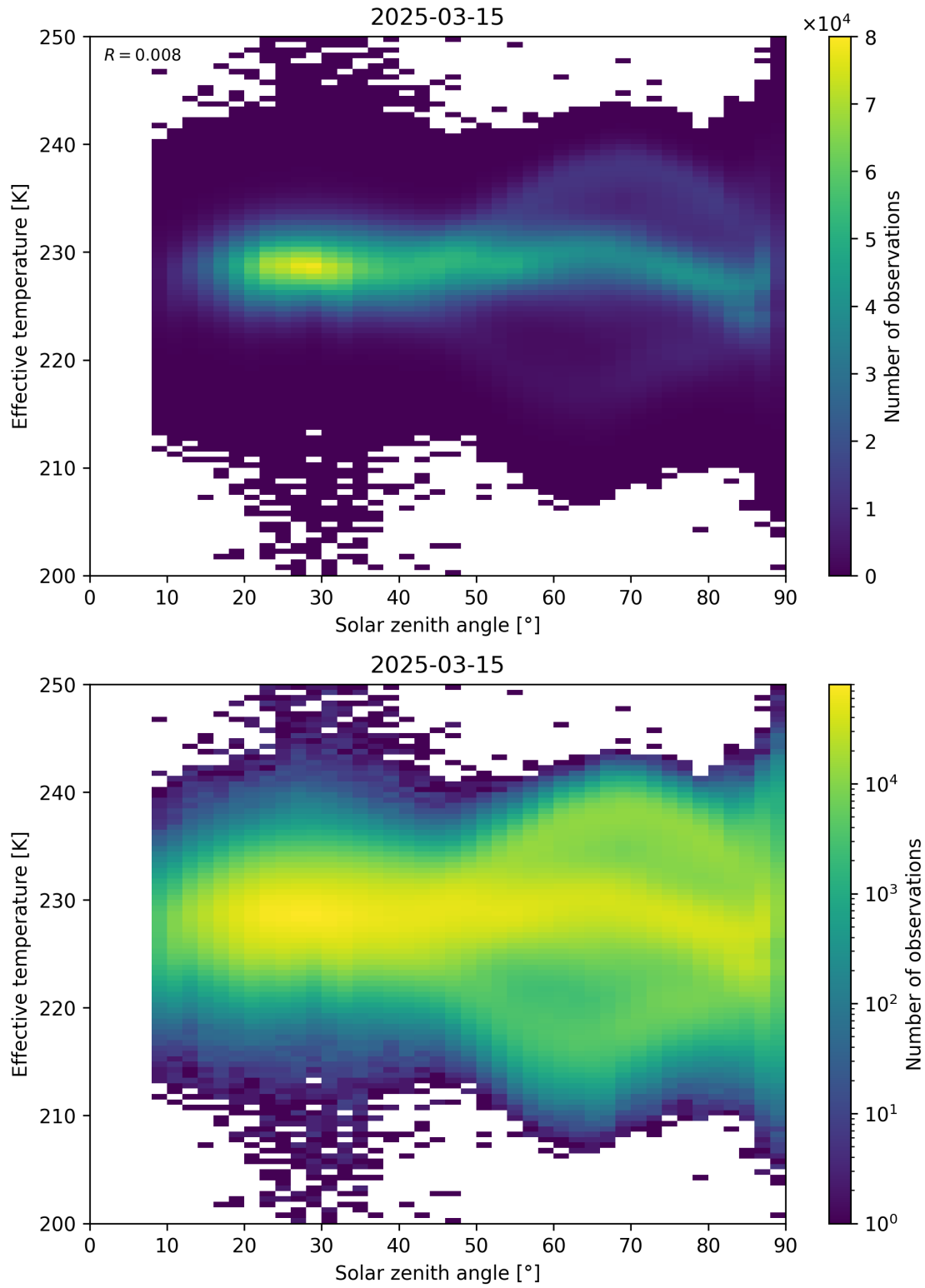
Figure 45: Scatter density plot of “Solar zenith angle” against “Effective temperature” for 2025-03-14 to 2025-03-16.
