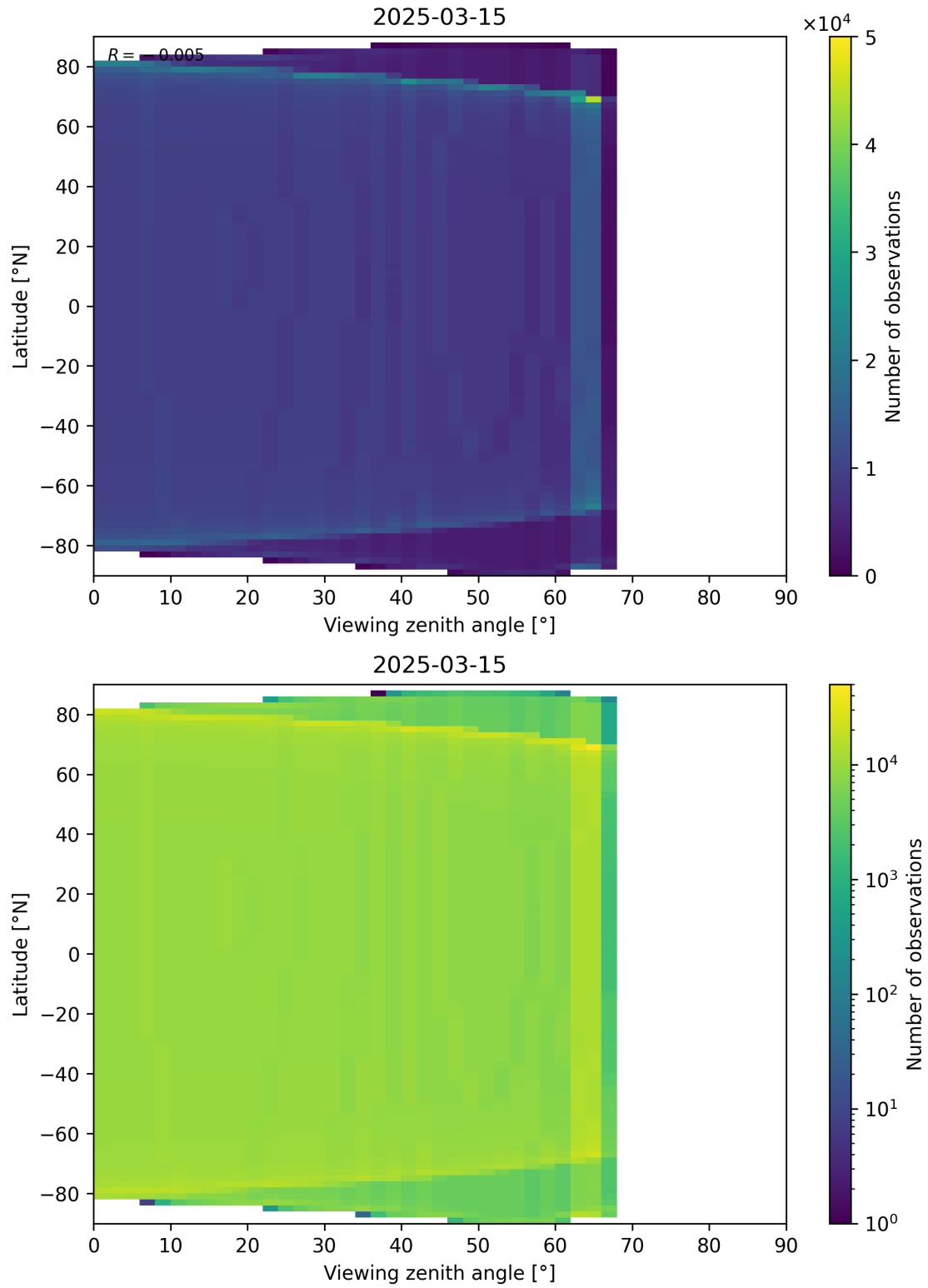
Figure 49: Scatter density plot of “Viewing zenith angle” against “Latitude” for 2025-03-14 to 2025-03-16.
