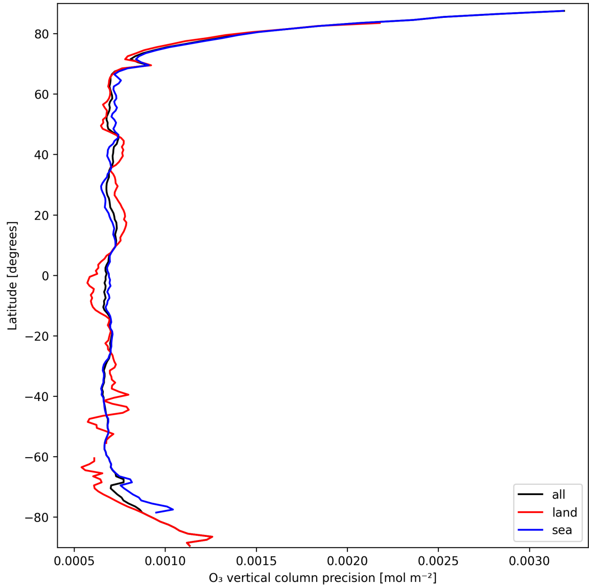
Figure 15: Zonal average of “O 3 vertical column precision” for 2025-03-14 to 2025-03-16.
