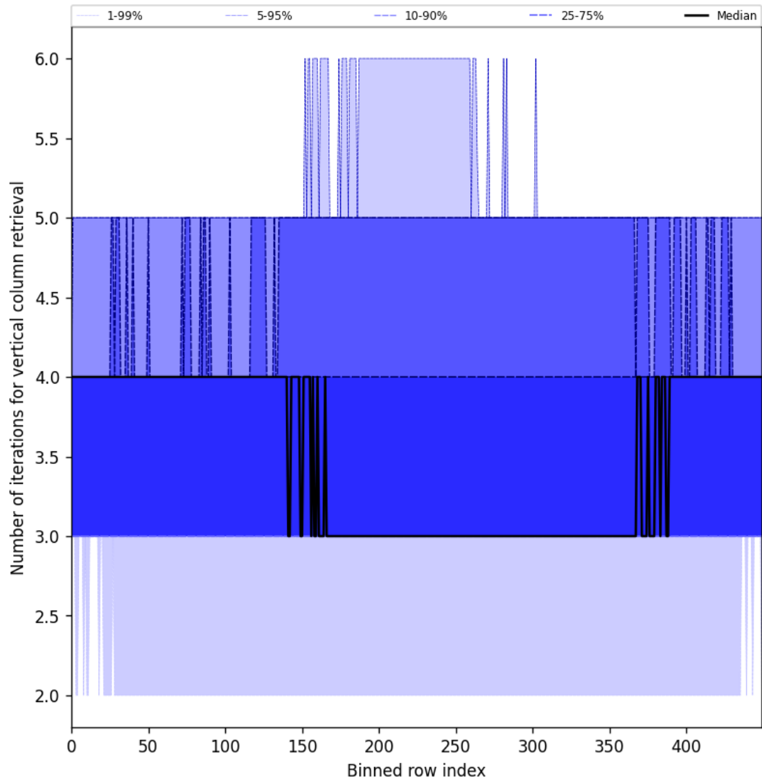
Figure 33: Along track statistics of “Number of iterations for vertical column retrieval” for 2025-03-14 to 2025-03-16
