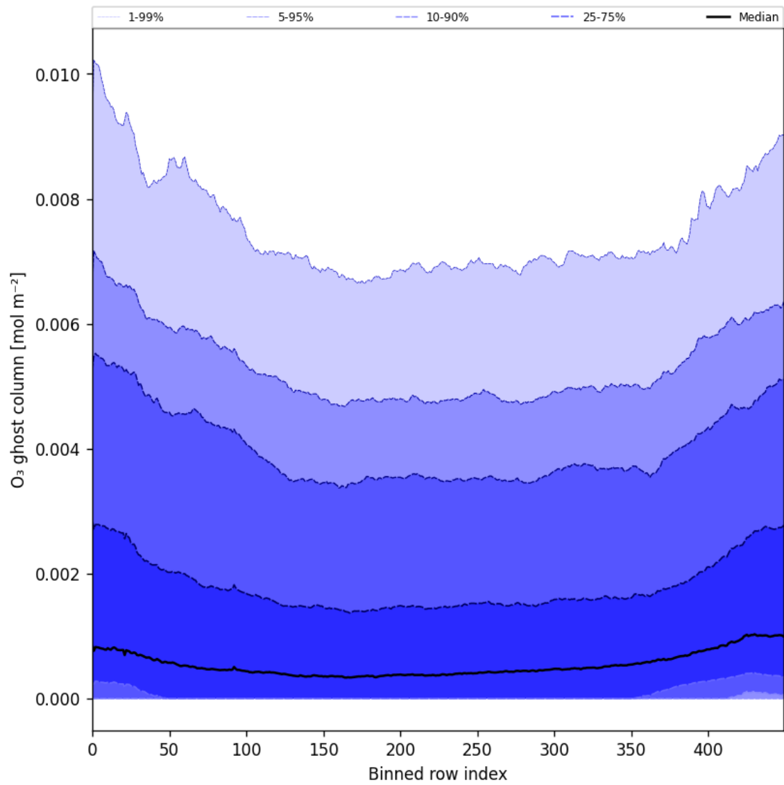
Figure 32: Along track statistics of “O 3 ghost column” for 2025-03-14 to 2025-03-16
