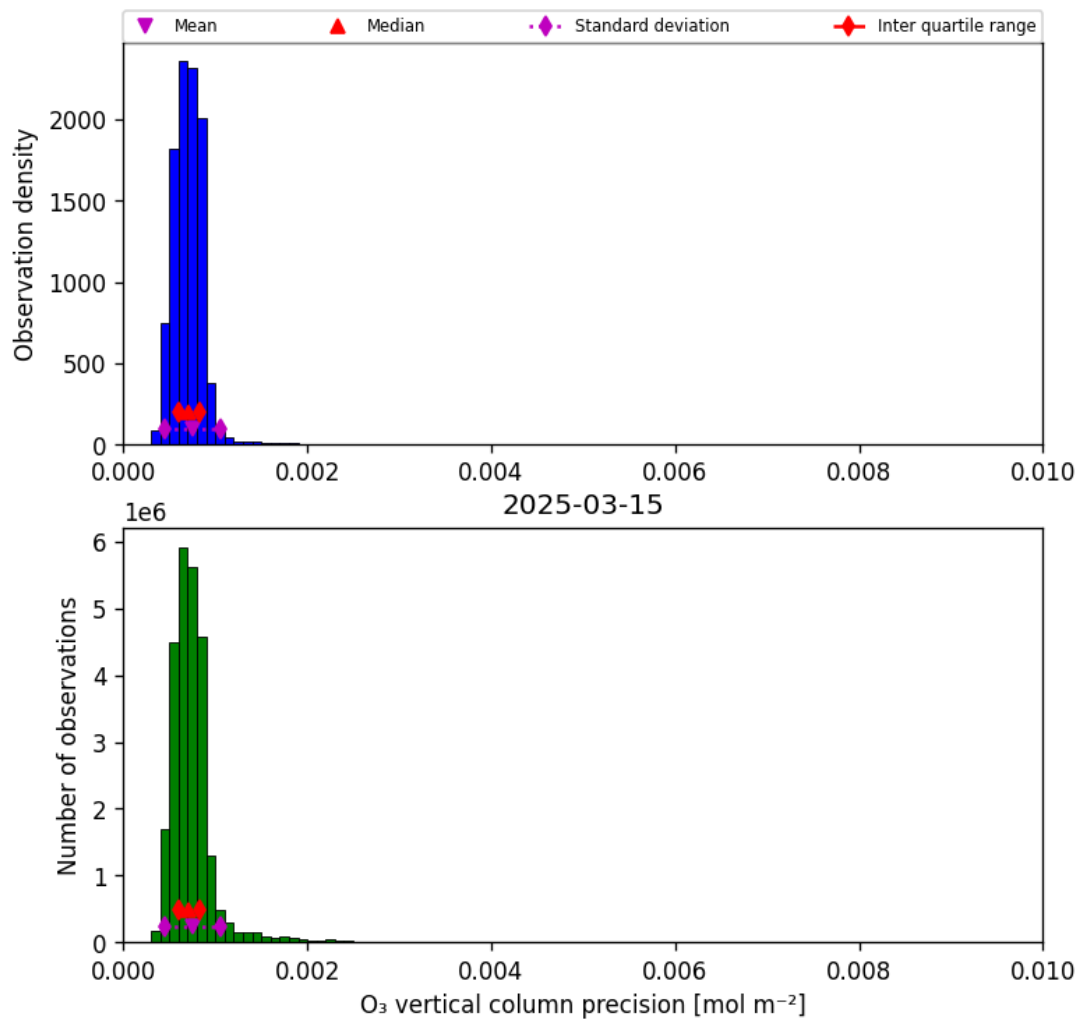
Figure 22: Histogram of “O 3 vertical column precision” for 2025-03-14 to 2025-03-16
