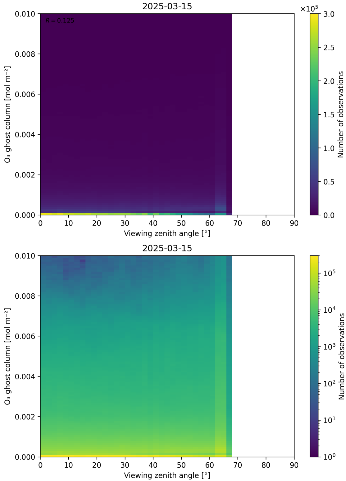
Figure 51: Scatter density plot of “Viewing zenith angle” against “O 3 ghost column” for 2025-03-14 to 2025-03-16.
