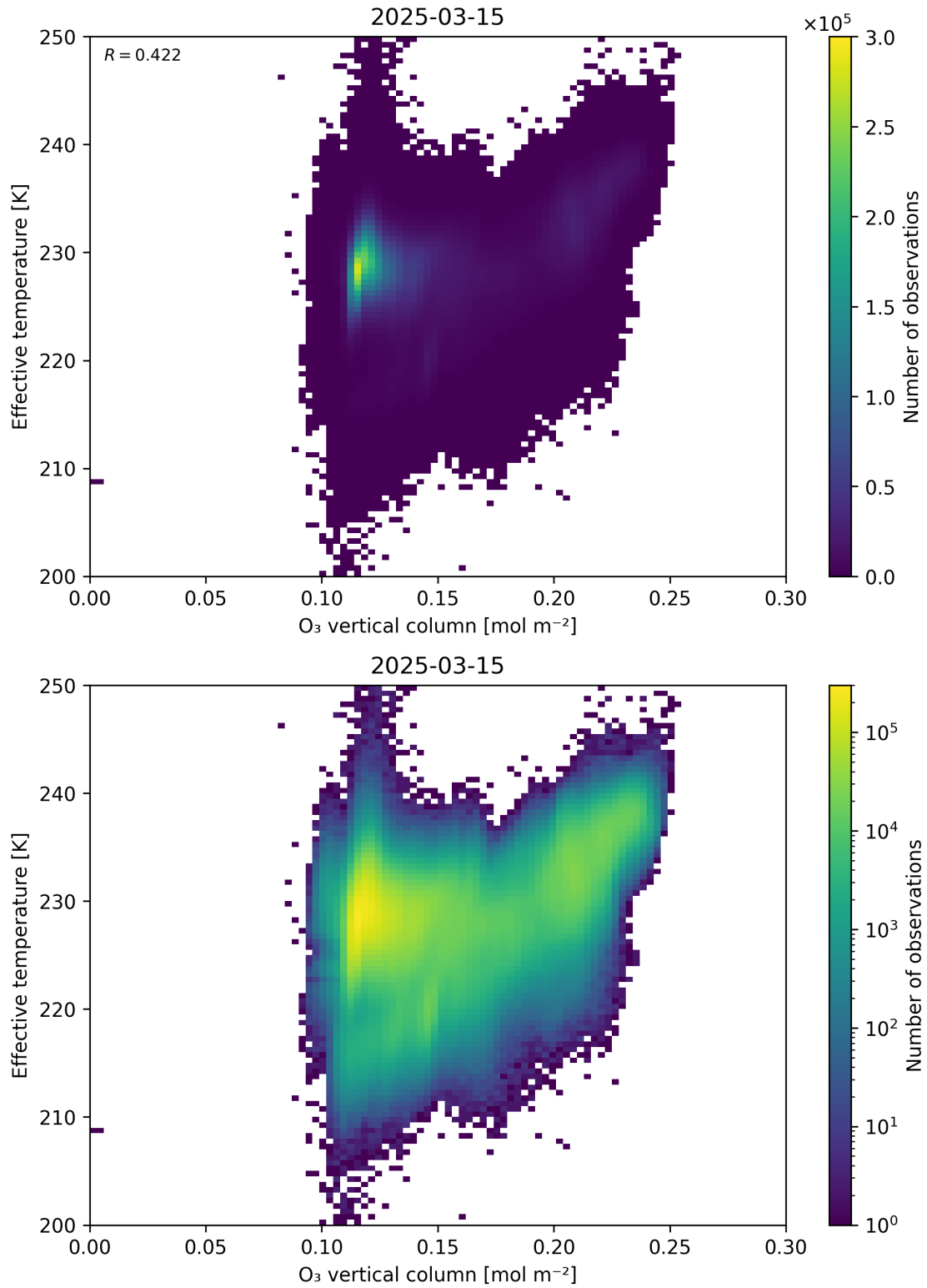
Figure 39: Scatter density plot of “O 3 vertical column” against “Effective temperature” for 2025-03-14 to 2025-03-16.
