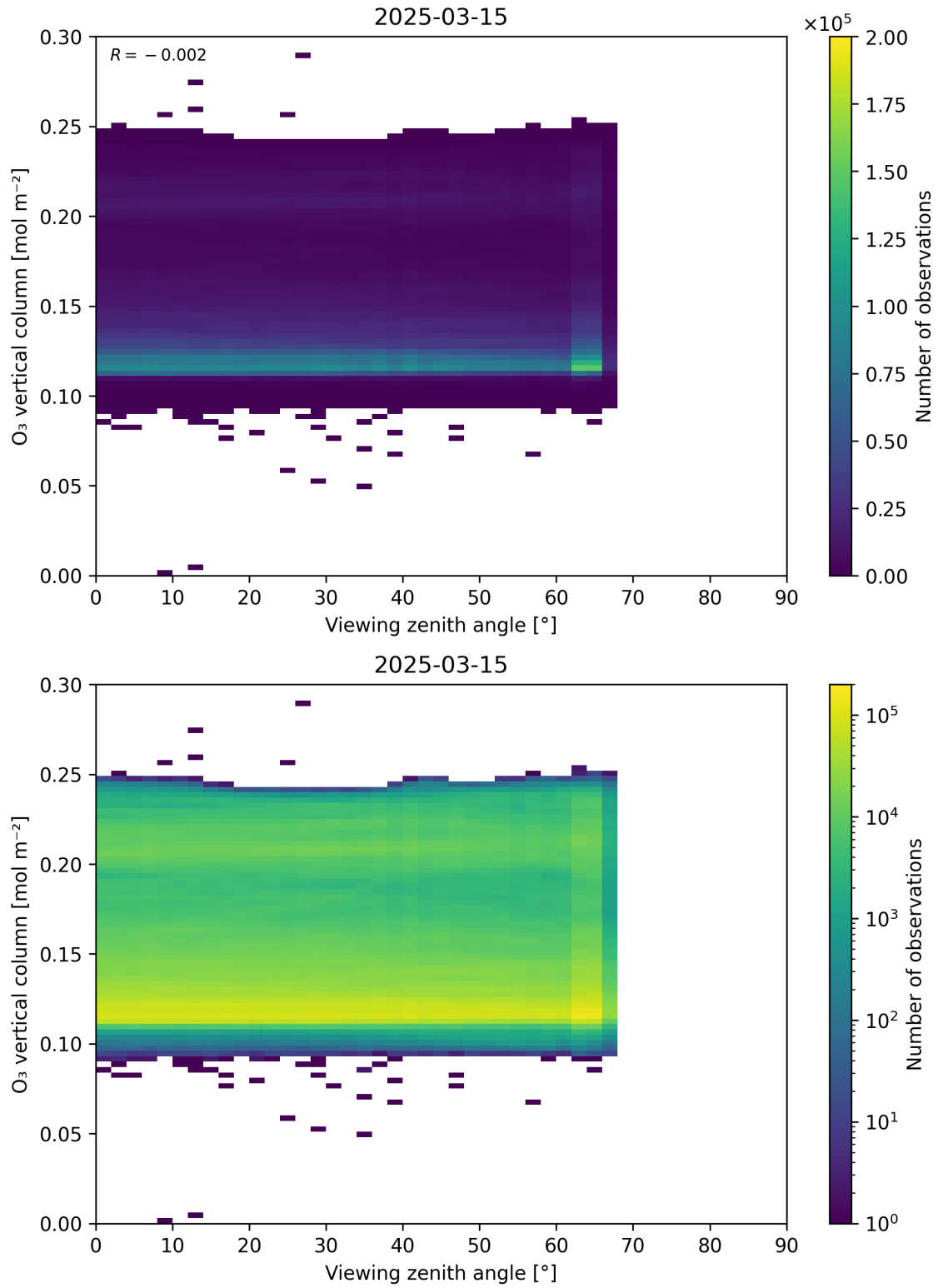
Figure 52: Scatter density plot of “Viewing zenith angle” against “O 3 vertical column” for 2025-03-14 to 2025-03-16.
