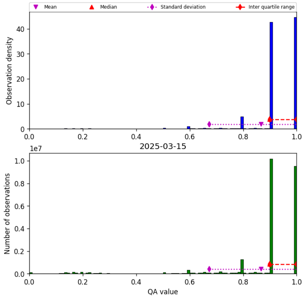
Figure 20: Histogram of “QA value” for 2025-03-14 to 2025-03-16
