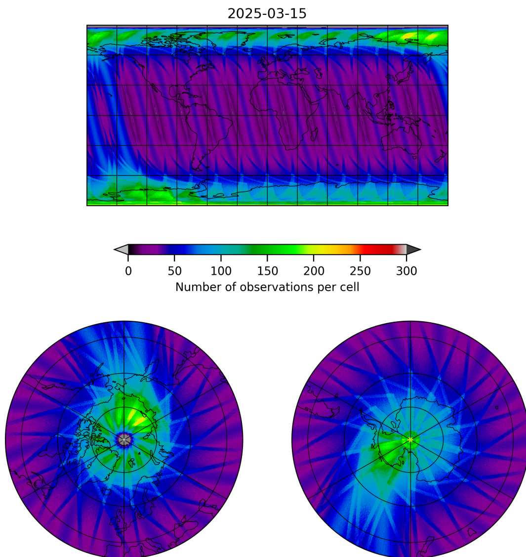
Figure 12: Map of the number of observations for 2025-03-14 to 2025-03-16
