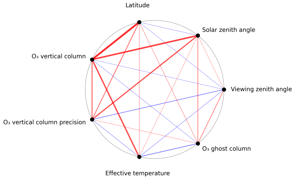
Figure 1: Map of correlation graph for 2025-03-14 to 2025-03-16.
