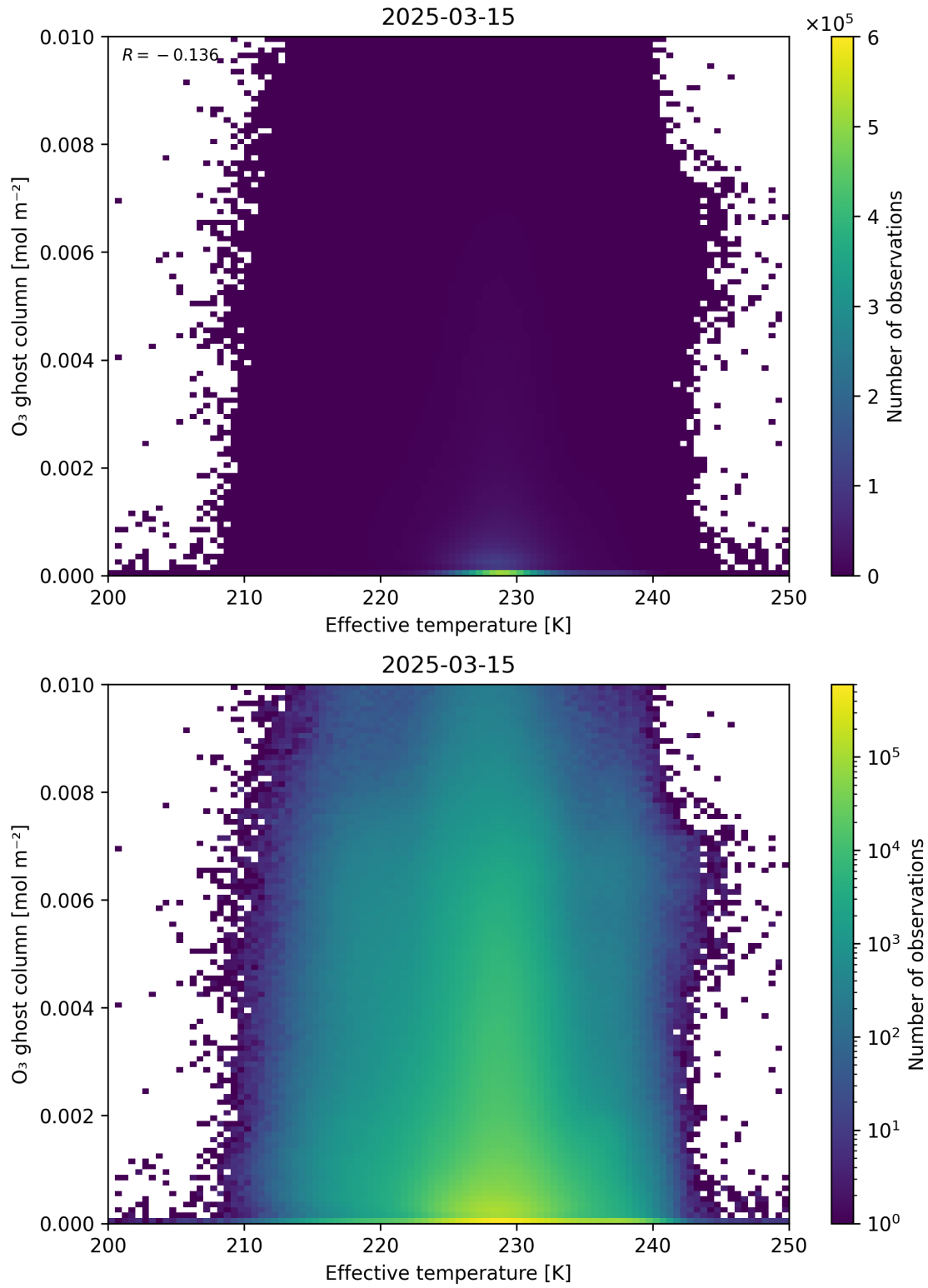
Figure 38: Scatter density plot of “Effective temperature” against “O 3 ghost column” for 2025-03-14 to 2025-03-16.
