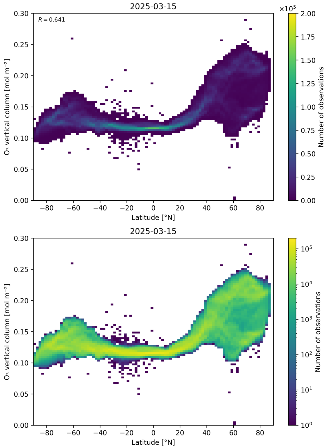
Figure 36: Scatter density plot of “Latitude” against “O 3 vertical column” for 2025-03-14 to 2025-03-16.
