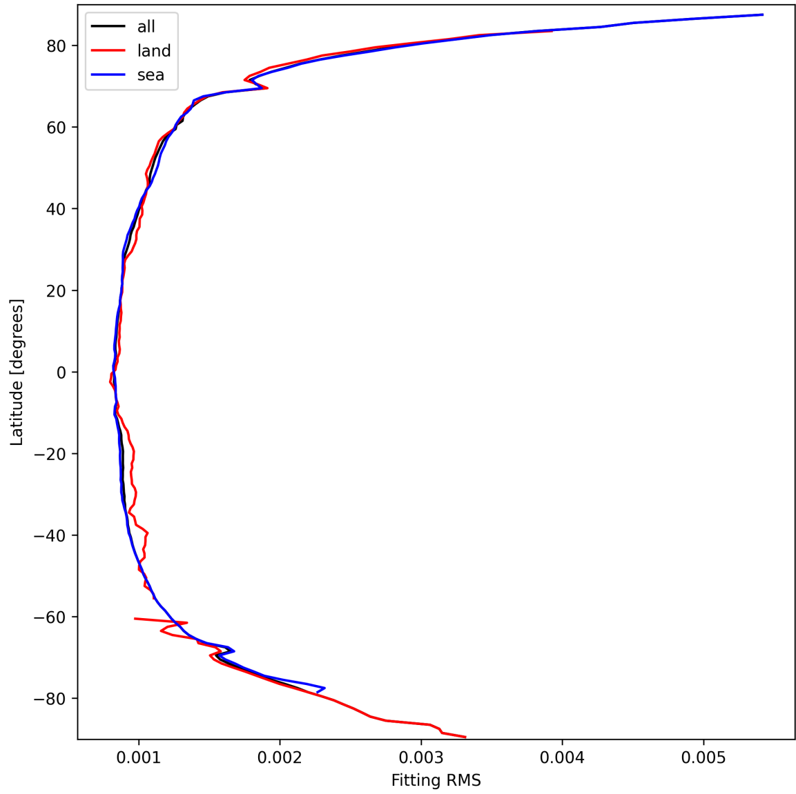
Figure 16: Zonal average of “Fitting RMS” for 2025-03-14 to 2025-03-16.
