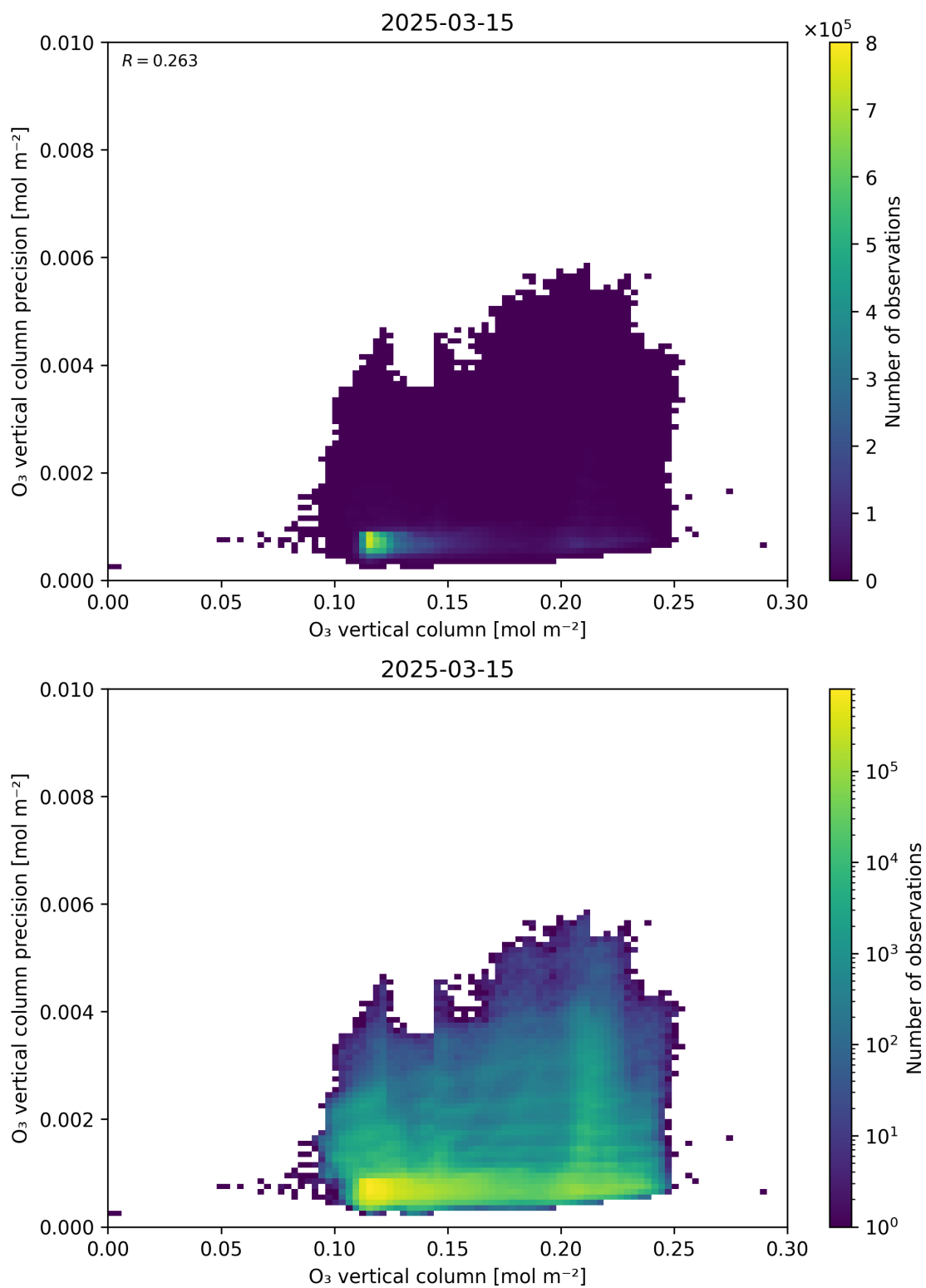
Figure 41: Scatter density plot of “O 3 vertical column” against “O 3 vertical column precision” for 2025-03-14 to 2025-03-16.
