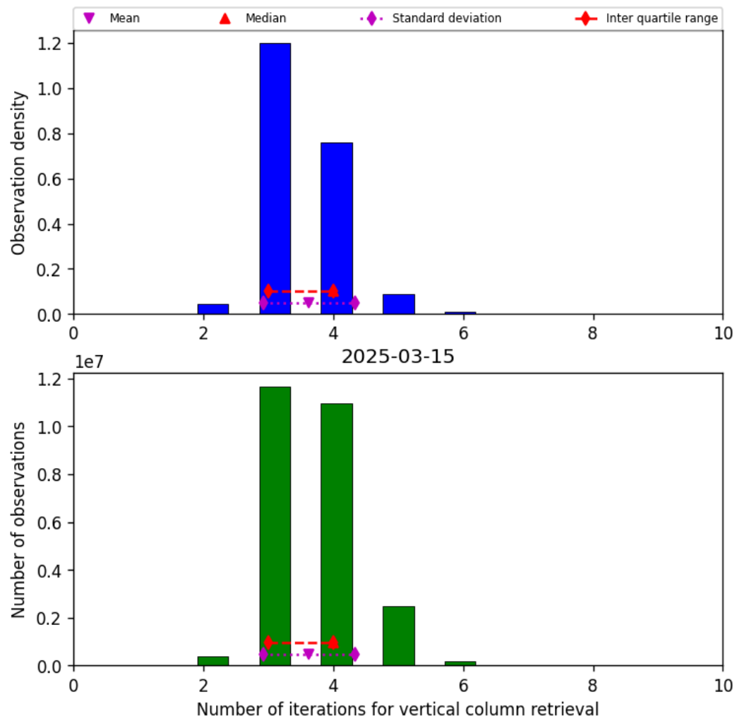
Figure 26: Histogram of “Number of iterations for vertical column retrieval” for 2025-03-14 to 2025-03-16
