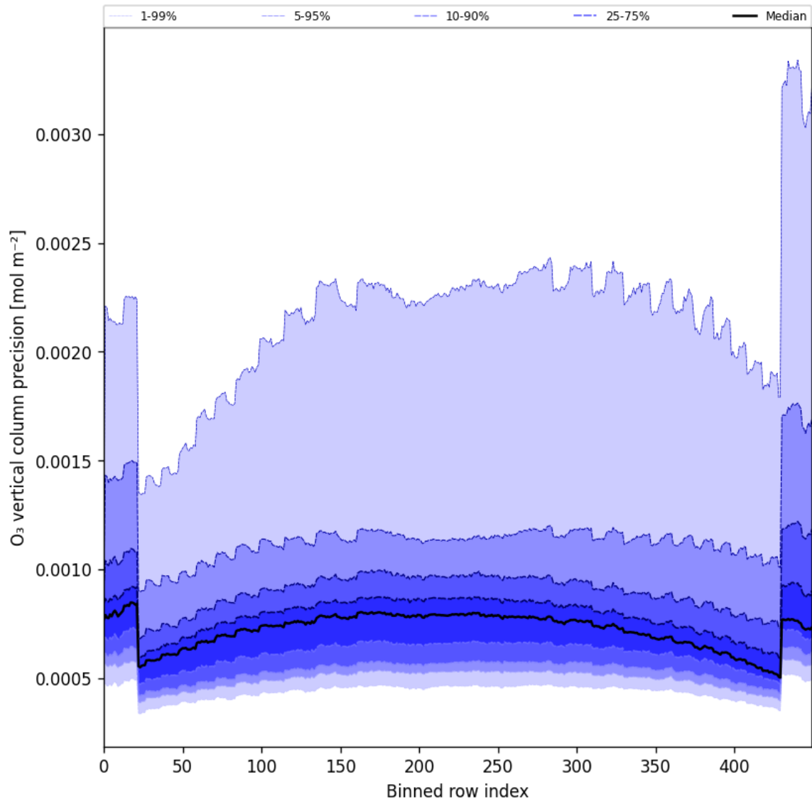
Figure 29: Along track statistics of “O 3 vertical column precision” for 2025-03-14 to 2025-03-16
