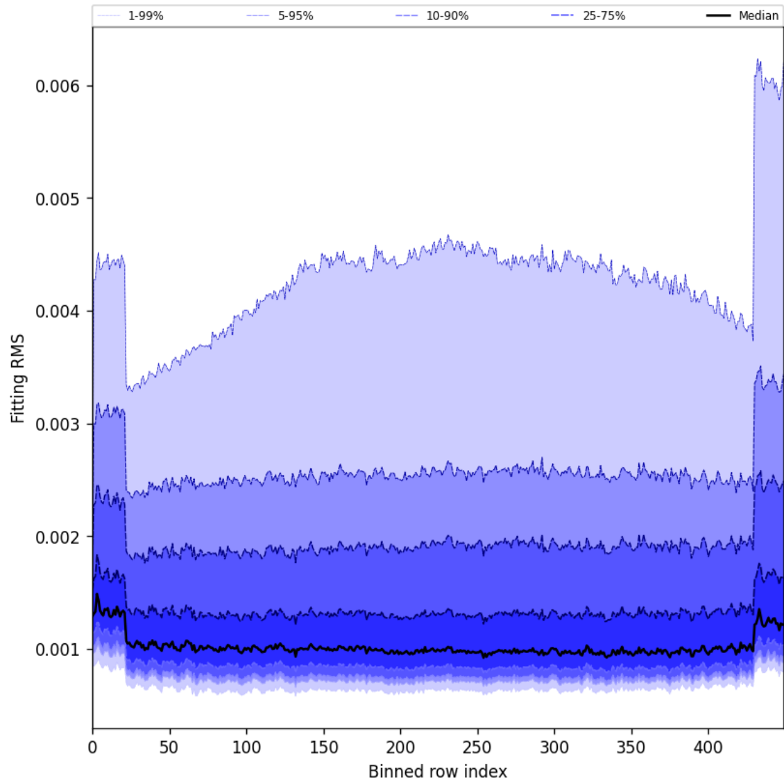
Figure 30: Along track statistics of “Fitting RMS” for 2025-03-14 to 2025-03-16
