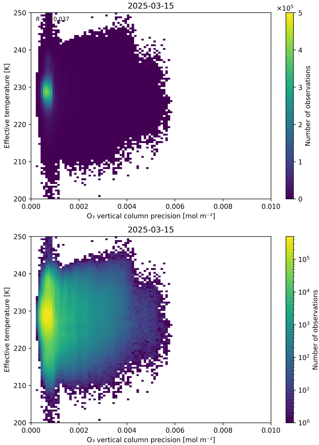
Figure 42: Scatter density plot of “O 3 vertical column precision” against “Effective temperature” for 2025-03-14 to 2025-03-16.
