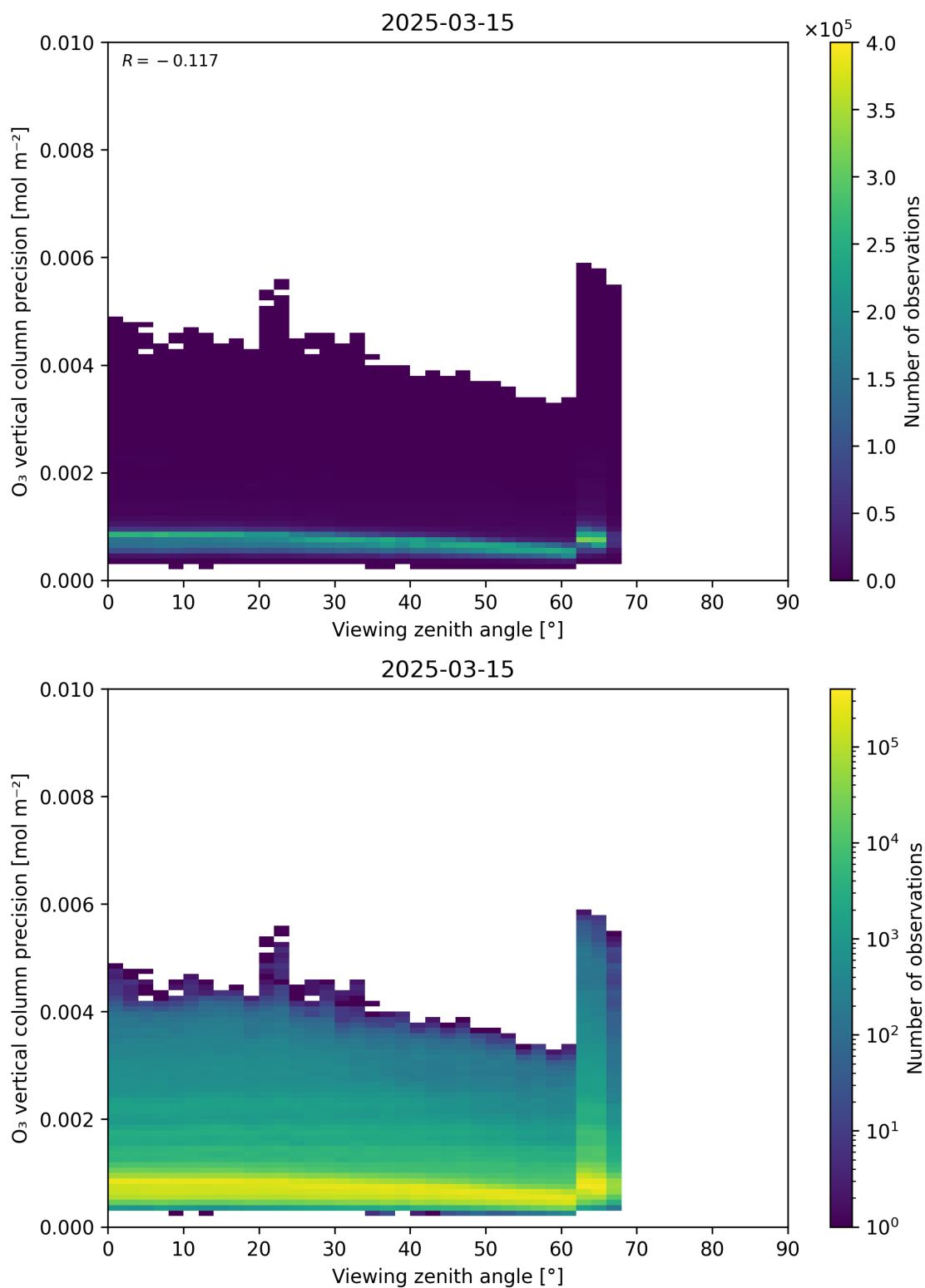
Figure 53: Scatter density plot of “Viewing zenith angle” against “O 3 vertical column precision” for 2025-03-14 to 2025-03-16.
