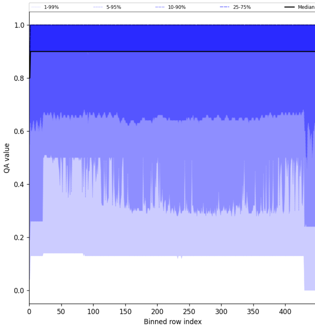
Figure 27: Along track statistics of “QA value” for 2025-03-14 to 2025-03-16
