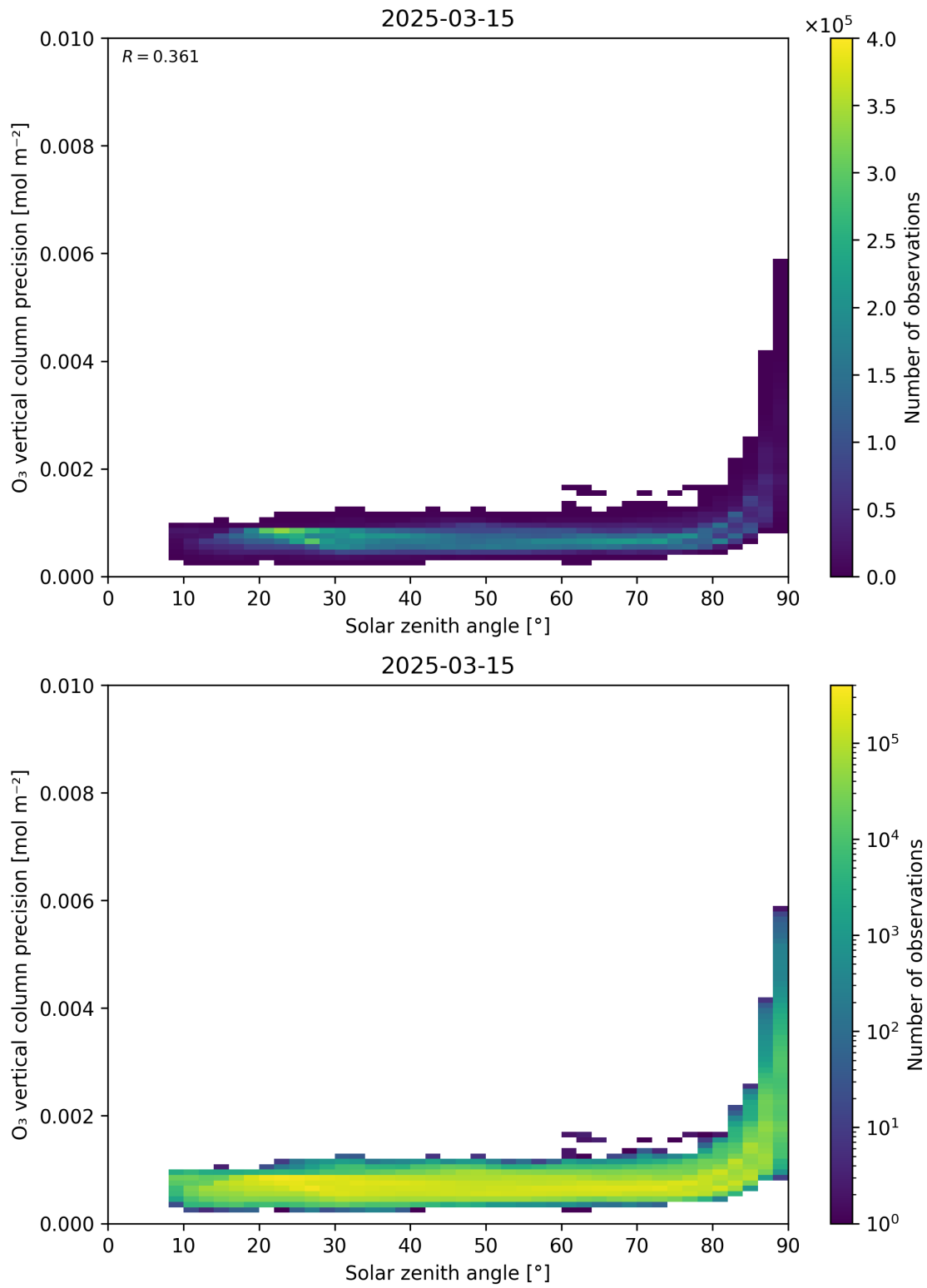
Figure 48: Scatter density plot of “Solar zenith angle” against “O 3 vertical column precision” for 2025-03-14 to 2025-03-16.
