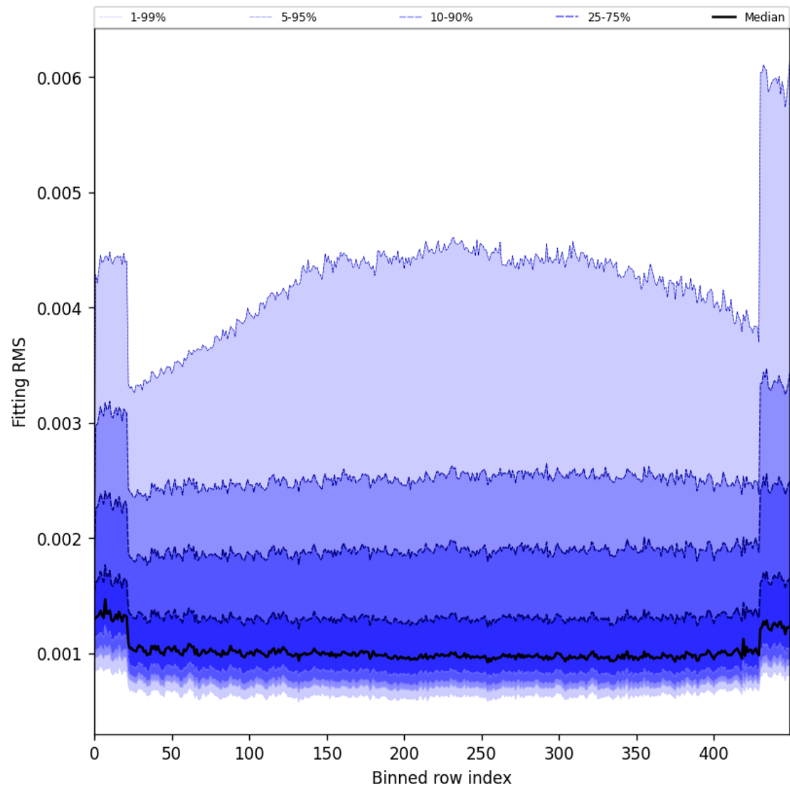
Figure 30: Along track statistics of “Fitting RMS” for 2025-03-15 to 2025-03-17
