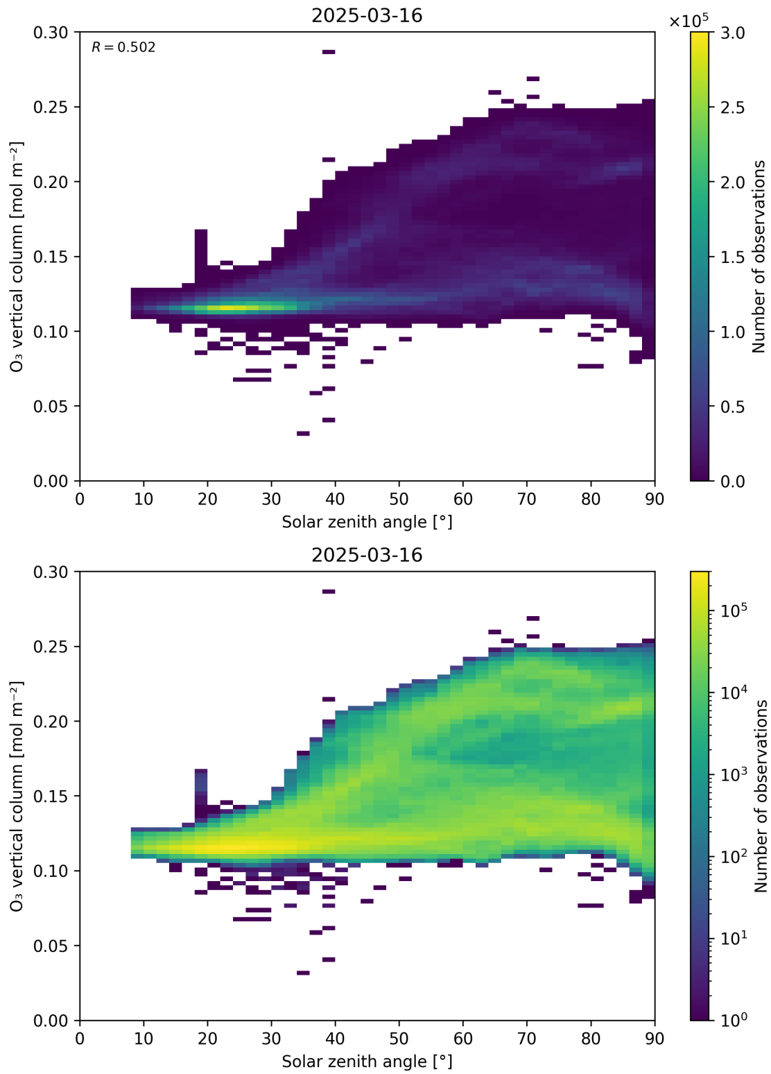
Figure 47: Scatter density plot of “Solar zenith angle” against “O 3 vertical column” for 2025-03-15 to 2025-03-17.
