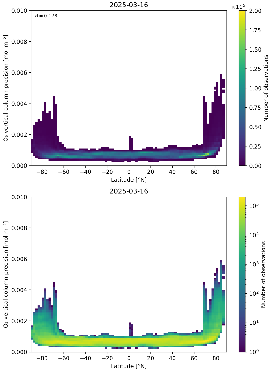
Figure 37: Scatter density plot of “Latitude” against “O 3 vertical column precision” for 2025-03-15 to 2025-03-17.
