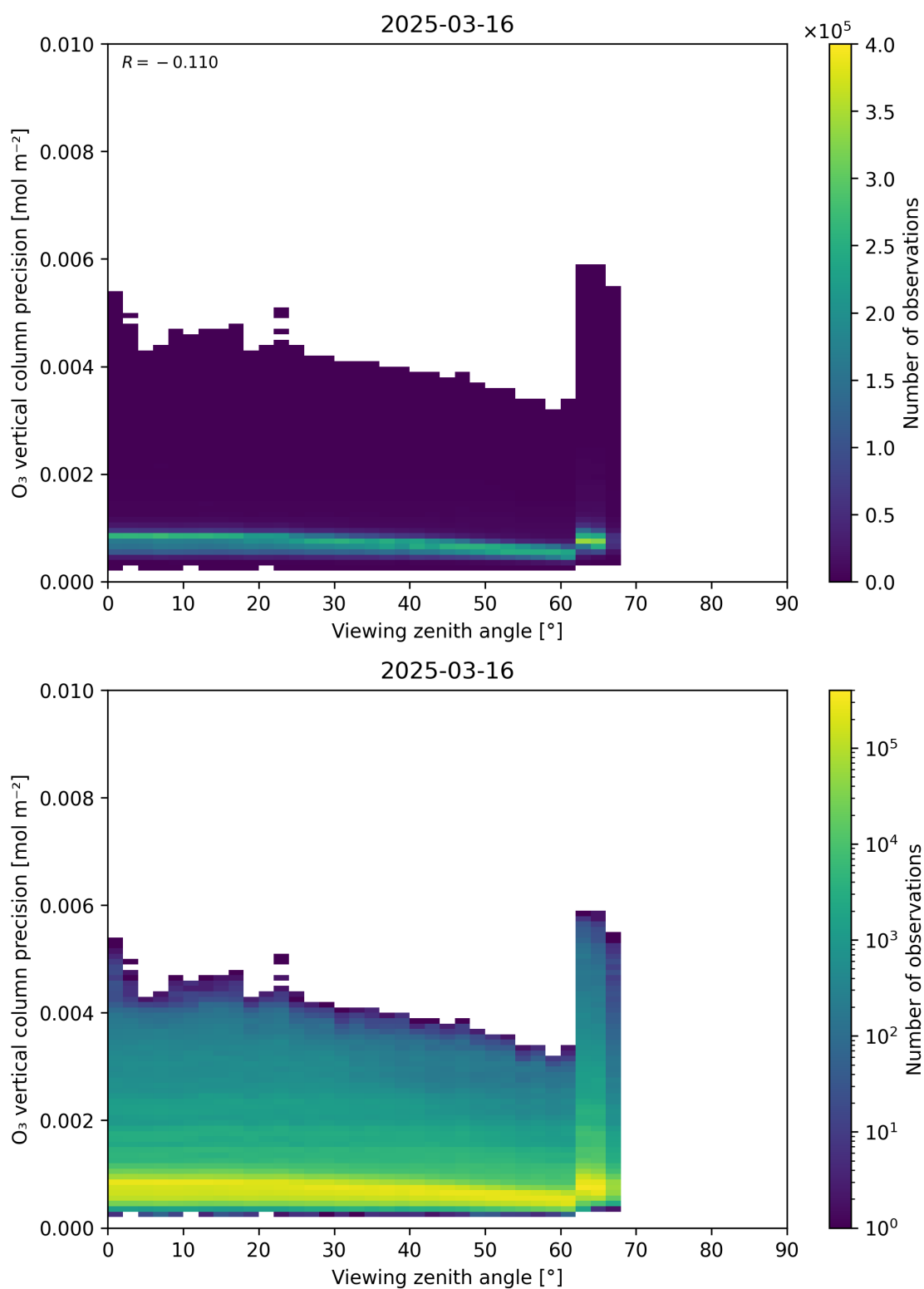
Figure 53: Scatter density plot of “Viewing zenith angle” against “O 3 vertical column precision” for 2025-03-15 to 2025-03-17.
