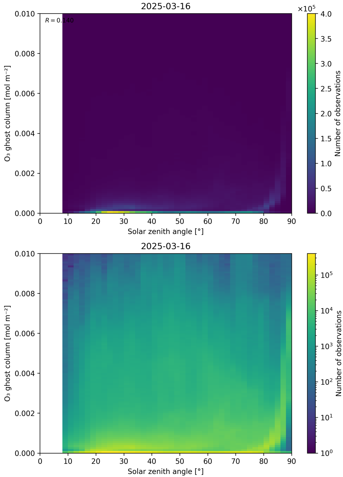
Figure 46: Scatter density plot of “Solar zenith angle” against “O 3 ghost column” for 2025-03-15 to 2025-03-17.
