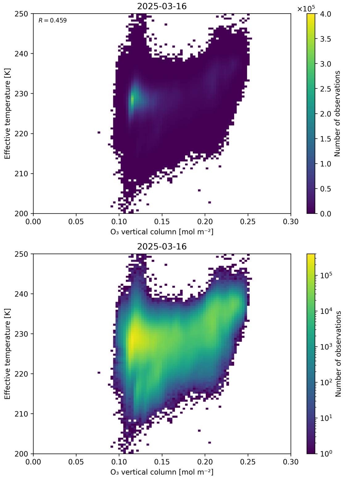
Figure 39: Scatter density plot of “O 3 vertical column” against “Effective temperature” for 2025-03-15 to 2025-03-17.
