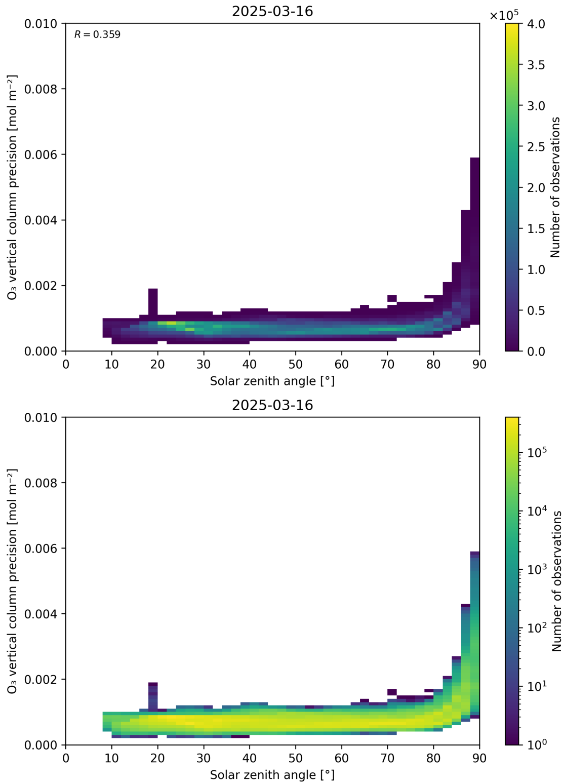
Figure 48: Scatter density plot of “Solar zenith angle” against “O 3 vertical column precision” for 2025-03-15 to 2025-03-17.
