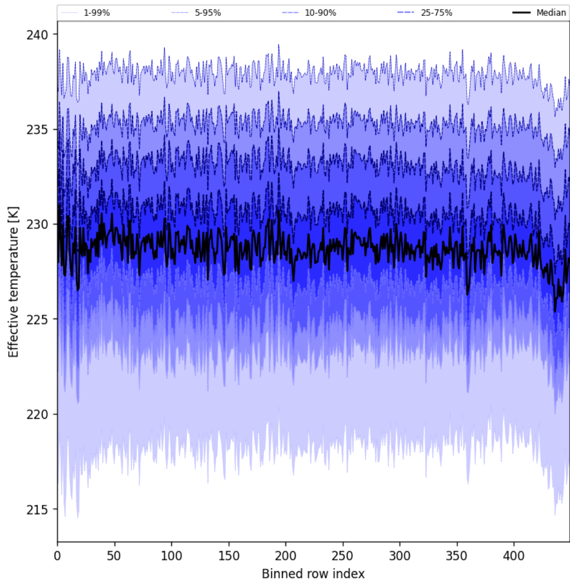
Figure 31: Along track statistics of “Effective temperature” for 2025-03-15 to 2025-03-17
