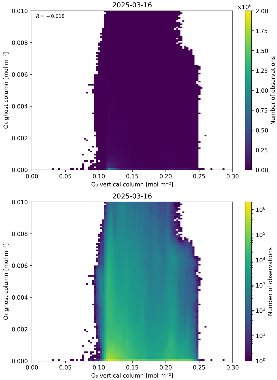
Figure 40: Scatter density plot of “O 3 vertical column” against “O 3 ghost column” for 2025-03-15 to 2025-03-17.
