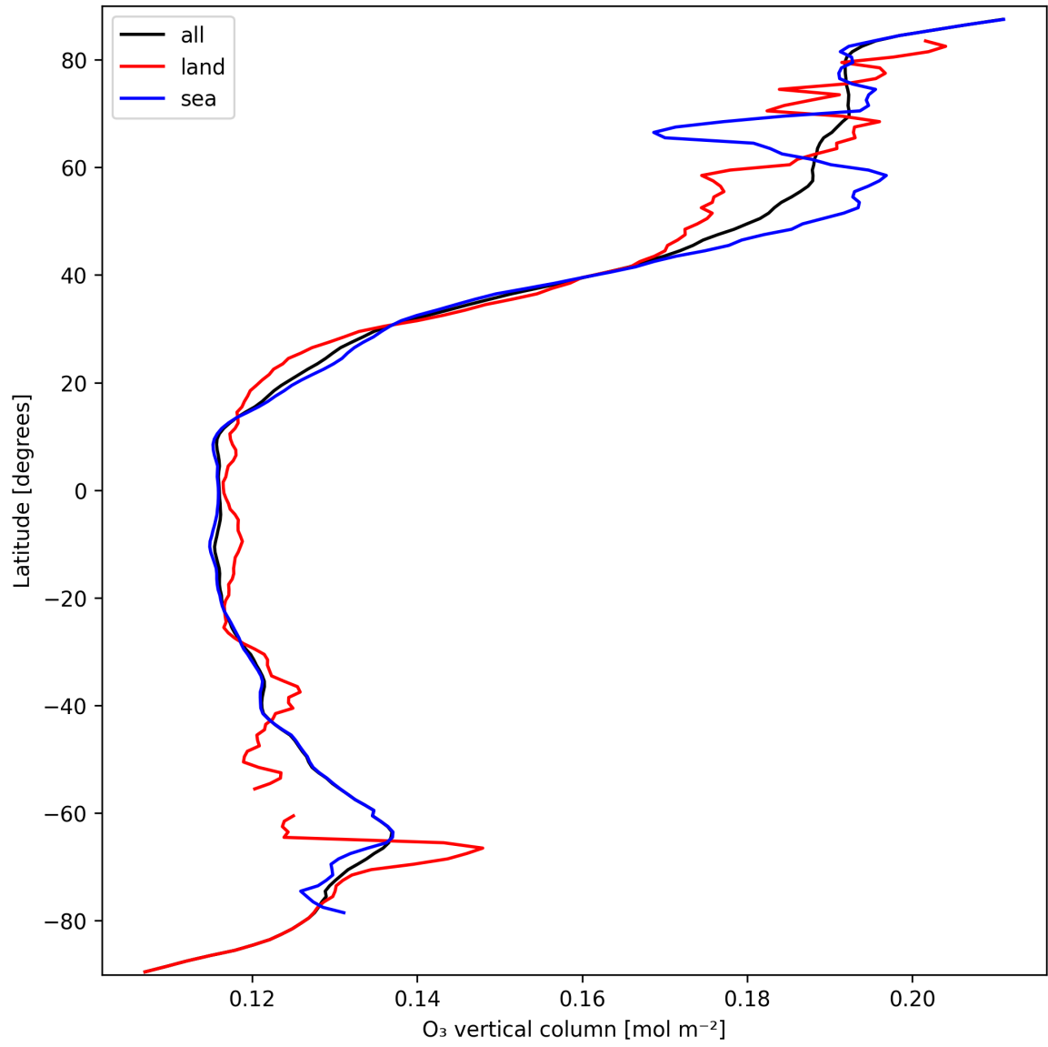
Figure 14: Zonal average of “O 3 vertical column” for 2025-03-15 to 2025-03-17.
