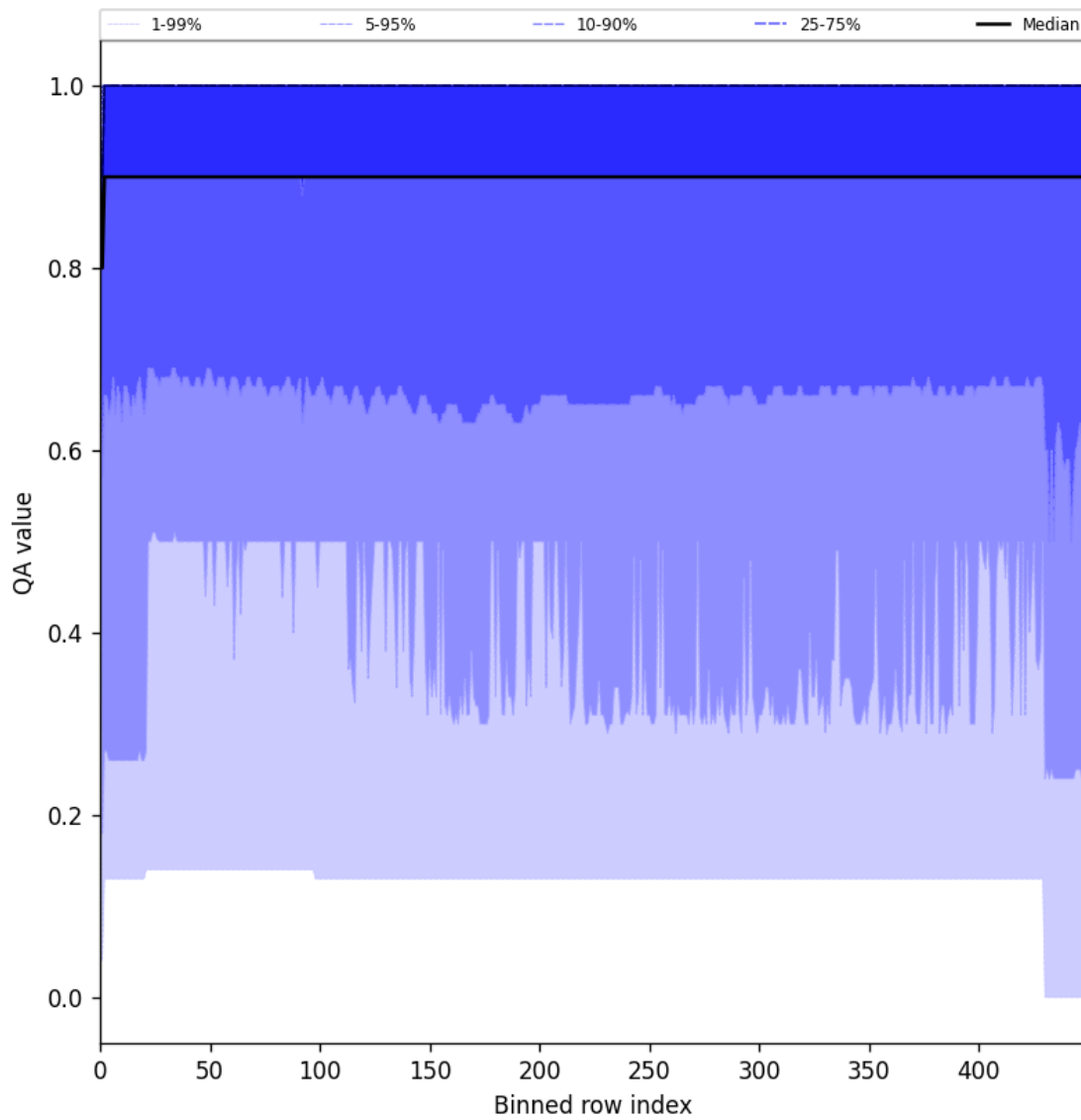
Figure 27: Along track statistics of “QA value” for 2025-03-15 to 2025-03-17
