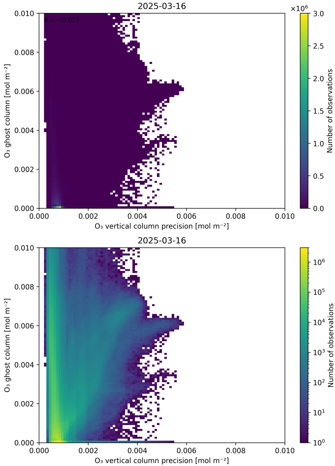
Figure 43: Scatter density plot of “O 3 vertical column precision” against “O 3 ghost column” for 2025-03-15 to 2025-03-17.
