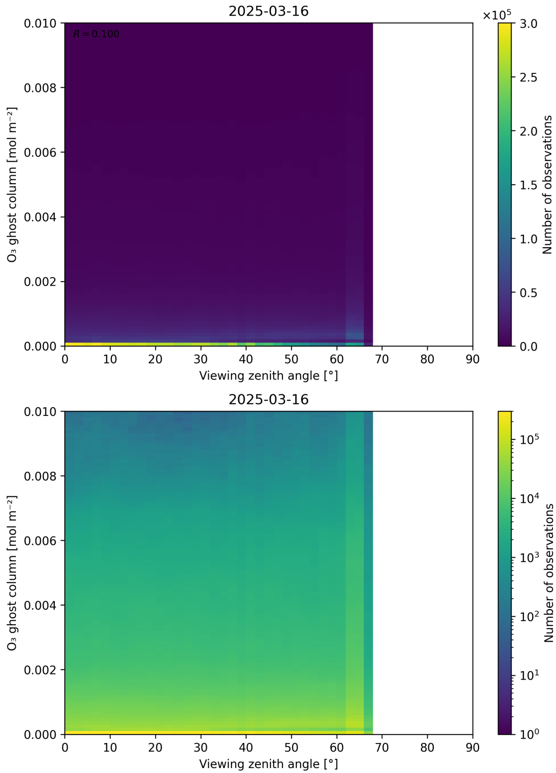
Figure 51: Scatter density plot of “Viewing zenith angle” against “O 3 ghost column” for 2025-03-15 to 2025-03-17.
