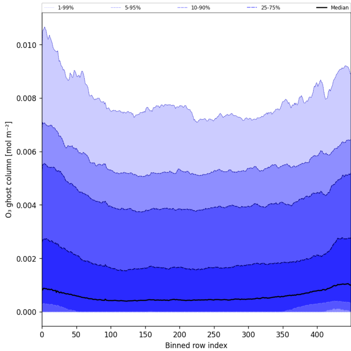
Figure 32: Along track statistics of “O 3 ghost column” for 2025-03-15 to 2025-03-17
