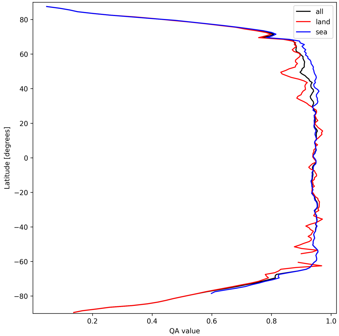
Figure 13: Zonal average of “QA value” for 2025-03-15 to 2025-03-17.
