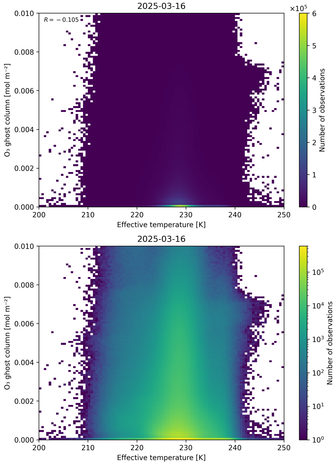
Figure 38: Scatter density plot of “Effective temperature” against “O 3 ghost column” for 2025-03-15 to 2025-03-17.
