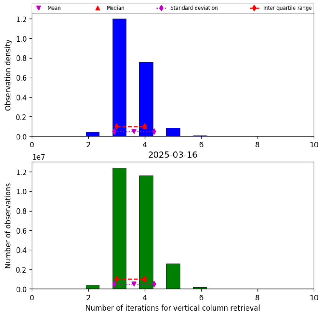
Figure 26: Histogram of “Number of iterations for vertical column retrieval” for 2025-03-15 to 2025-03-17
