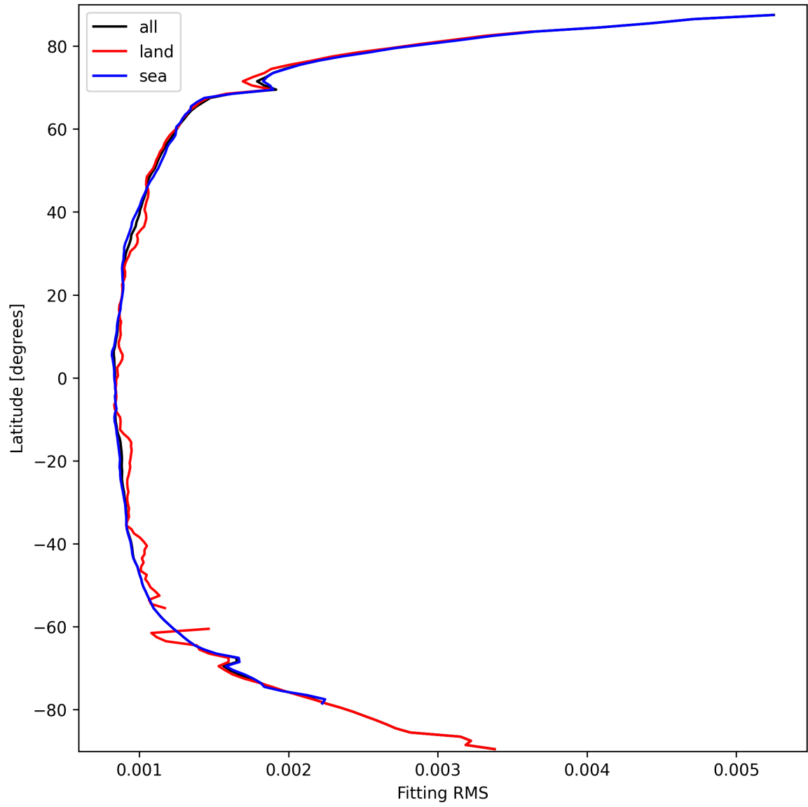
Figure 16: Zonal average of “Fitting RMS” for 2025-03-15 to 2025-03-17.
