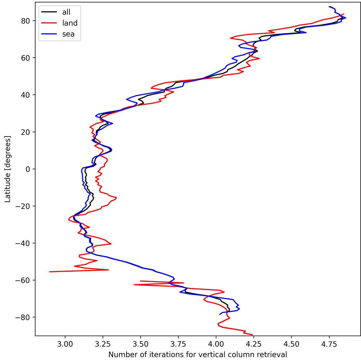
Figure 19: Zonal average of “Number of iterations for vertical column retrieval” for 2025-03-15 to 2025-03-17.
