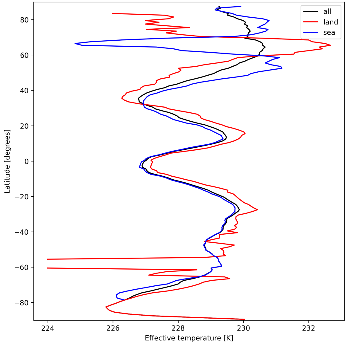
Figure 17: Zonal average of “Effective temperature” for 2025-03-15 to 2025-03-17.
