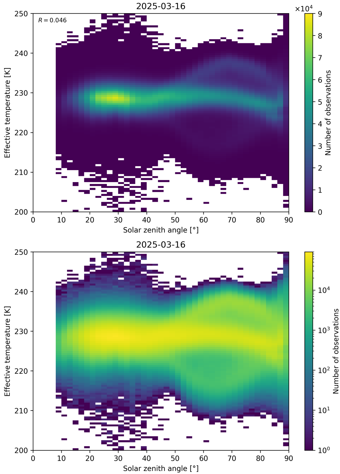
Figure 45: Scatter density plot of “Solar zenith angle” against “Effective temperature” for 2025-03-15 to 2025-03-17.
