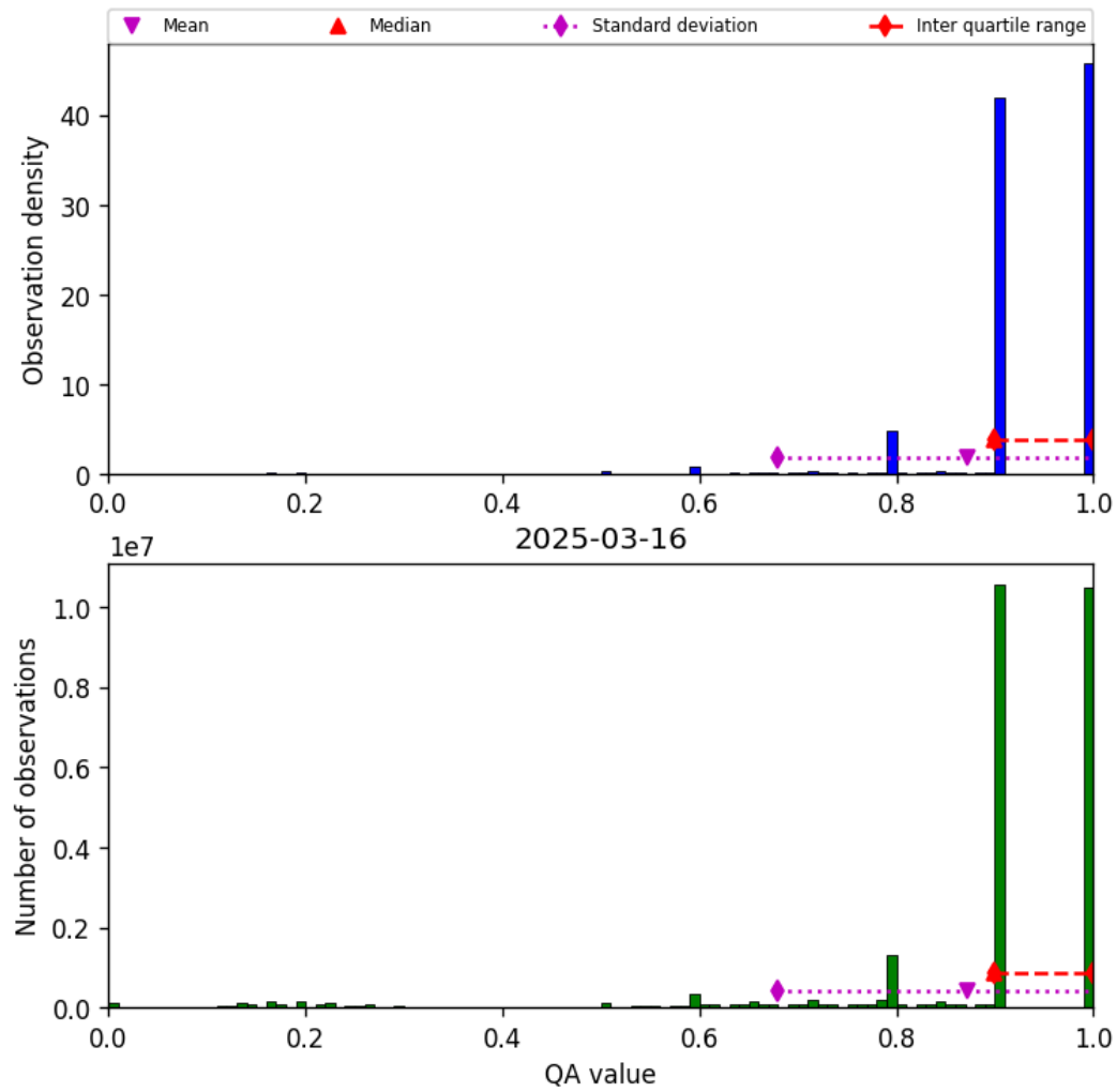
Figure 20: Histogram of “QA value” for 2025-03-15 to 2025-03-17
