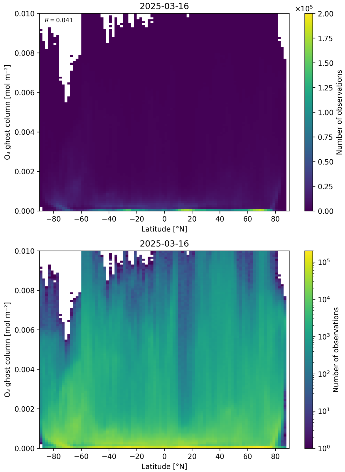
Figure 35: Scatter density plot of “Latitude” against “O 3 ghost column” for 2025-03-15 to 2025-03-17.
