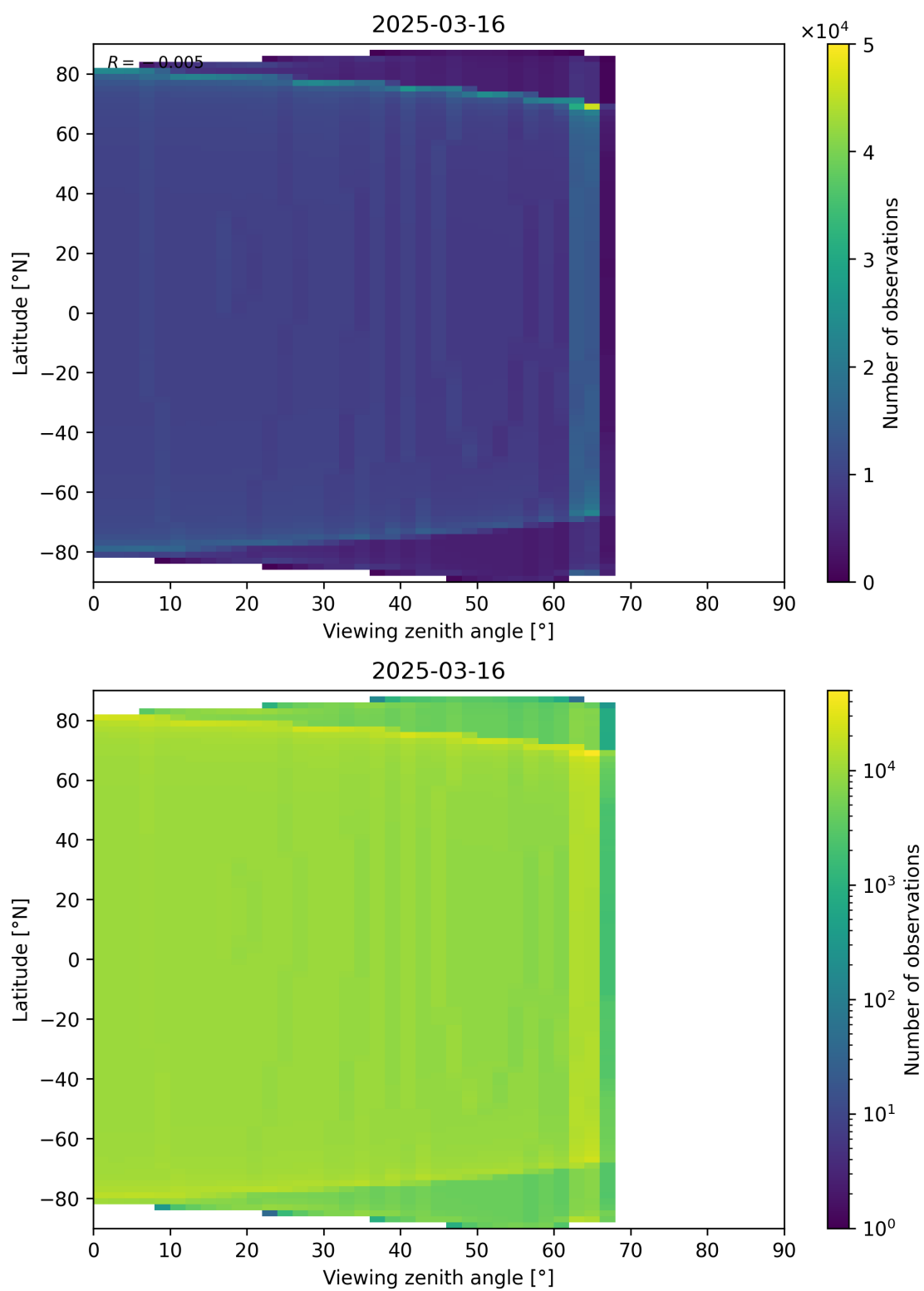
Figure 49: Scatter density plot of “Viewing zenith angle” against “Latitude” for 2025-03-15 to 2025-03-17.
