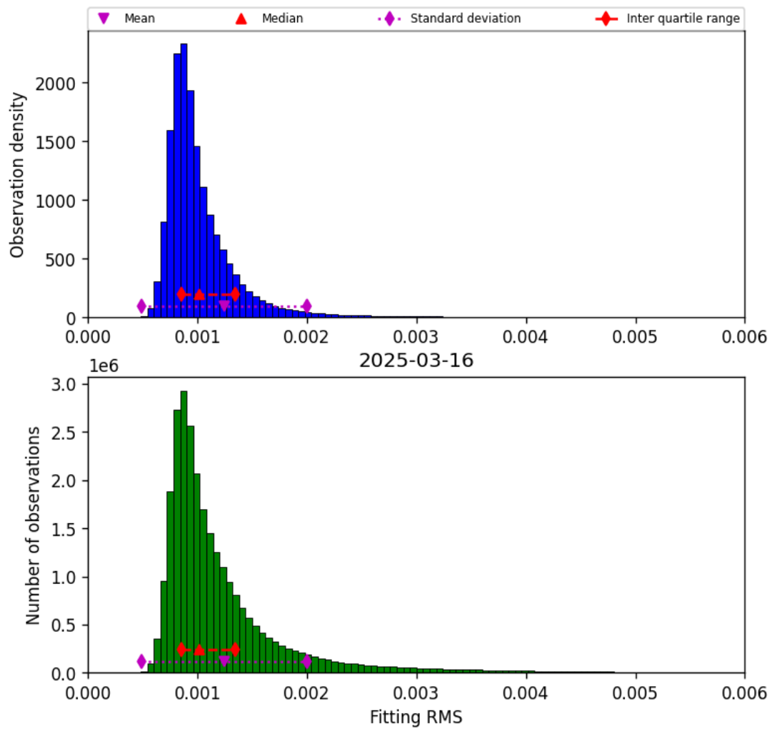
Figure 23: Histogram of “Fitting RMS” for 2025-03-15 to 2025-03-17
