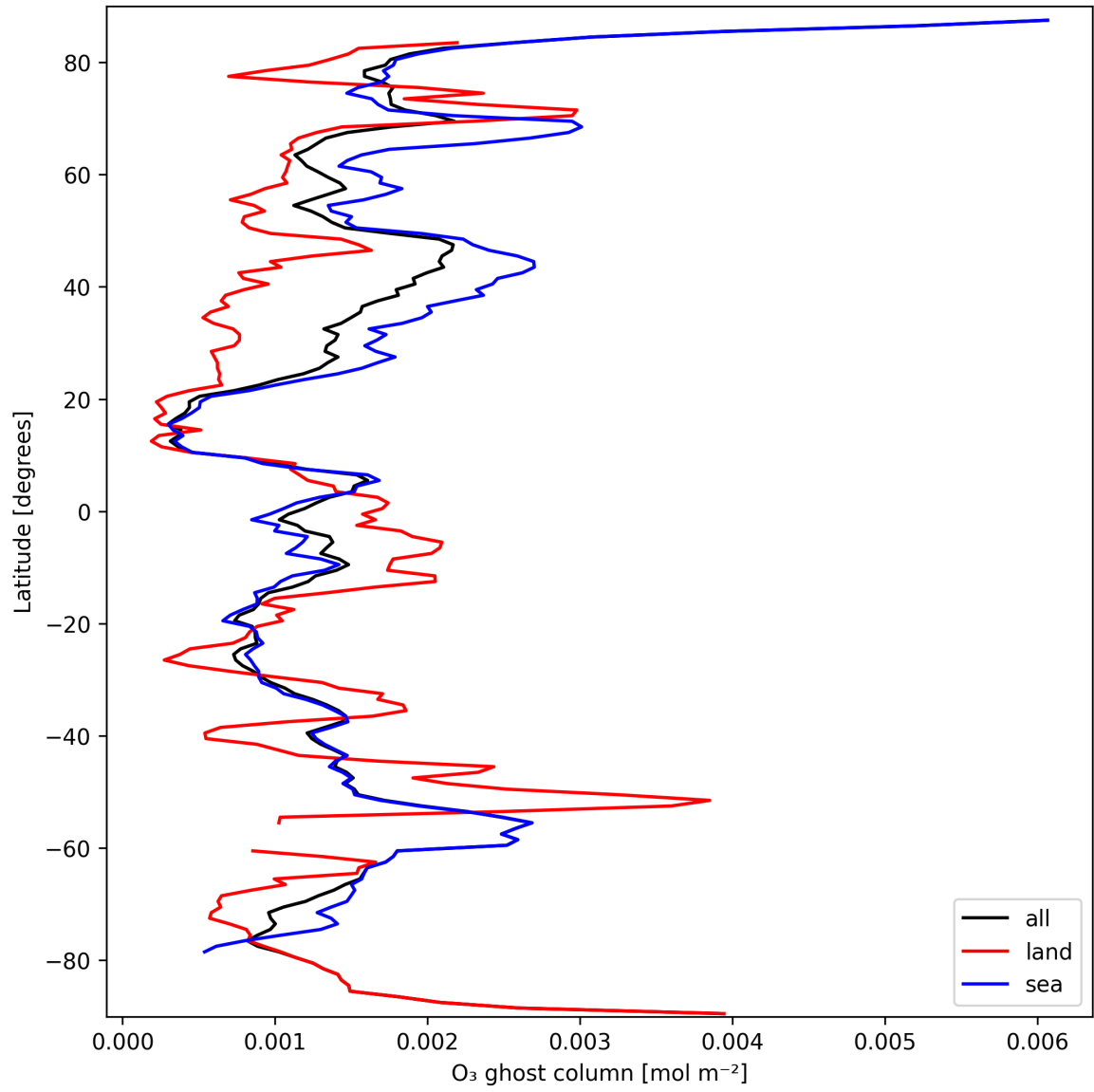
Figure 18: Zonal average of “O 3 ghost column” for 2025-03-15 to 2025-03-17.
