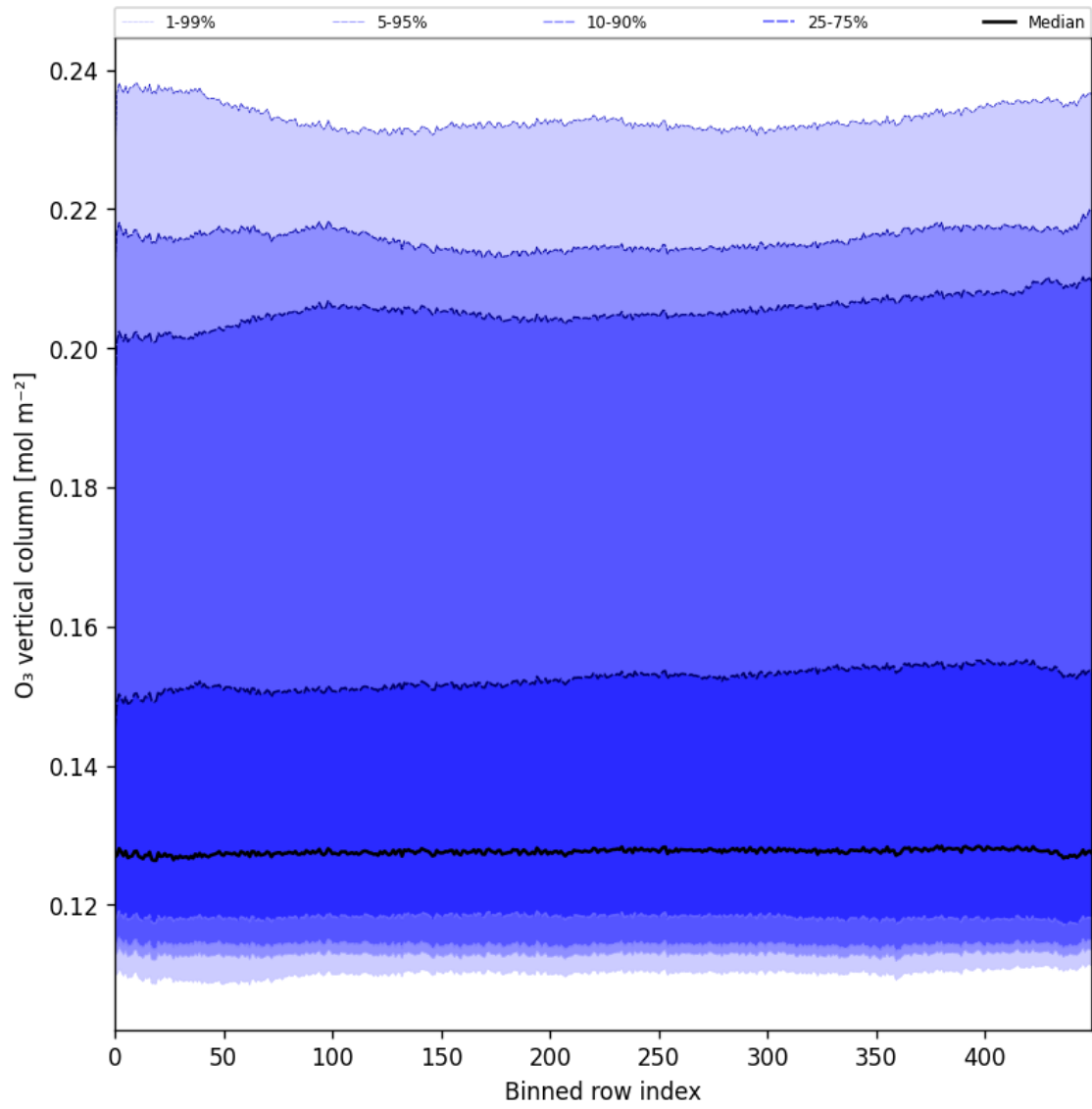
Figure 28: Along track statistics of “O 3 vertical column” for 2025-03-15 to 2025-03-17
