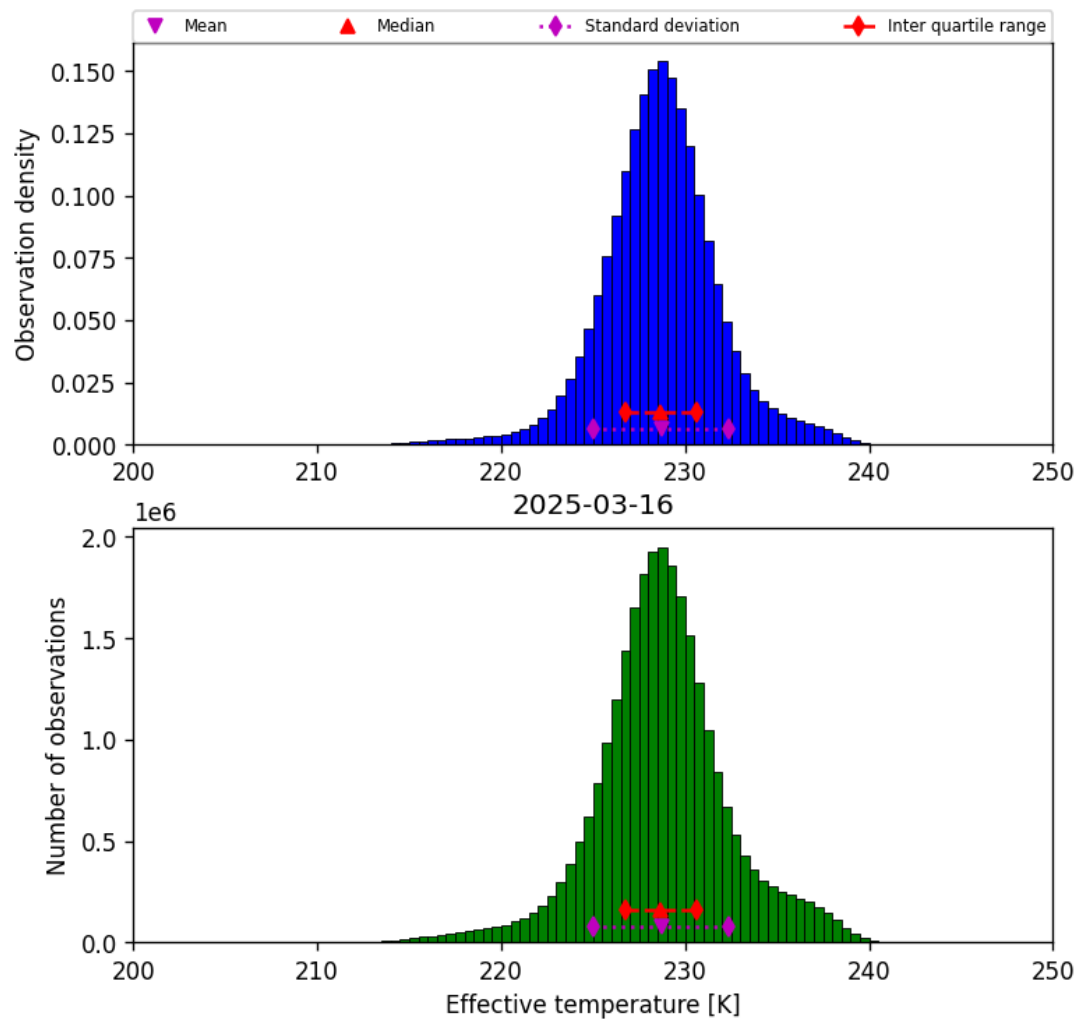
Figure 24: Histogram of “Effective temperature” for 2025-03-15 to 2025-03-17
