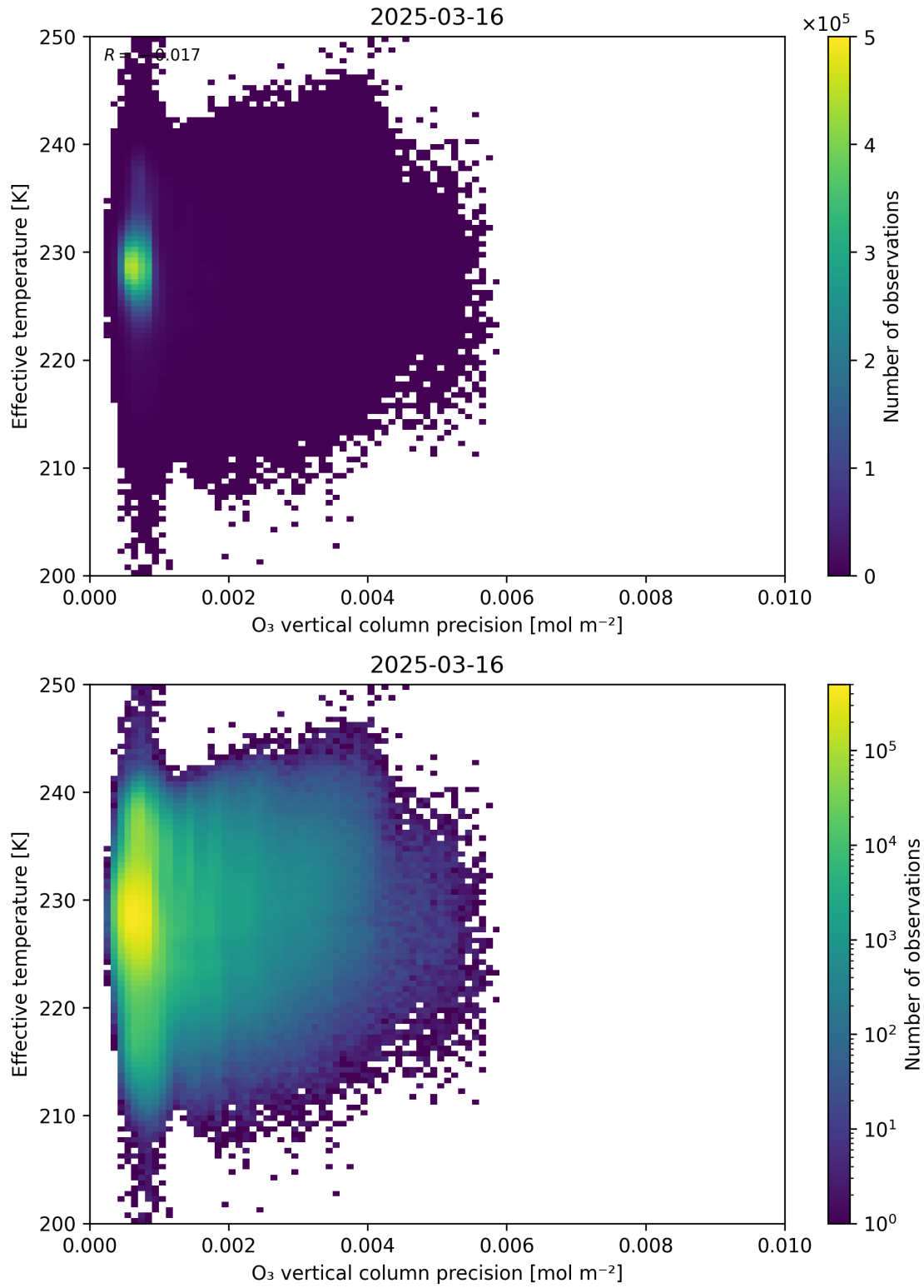
Figure 42: Scatter density plot of “O 3 vertical column precision” against “Effective temperature” for 2025-03-15 to 2025-03-17.
