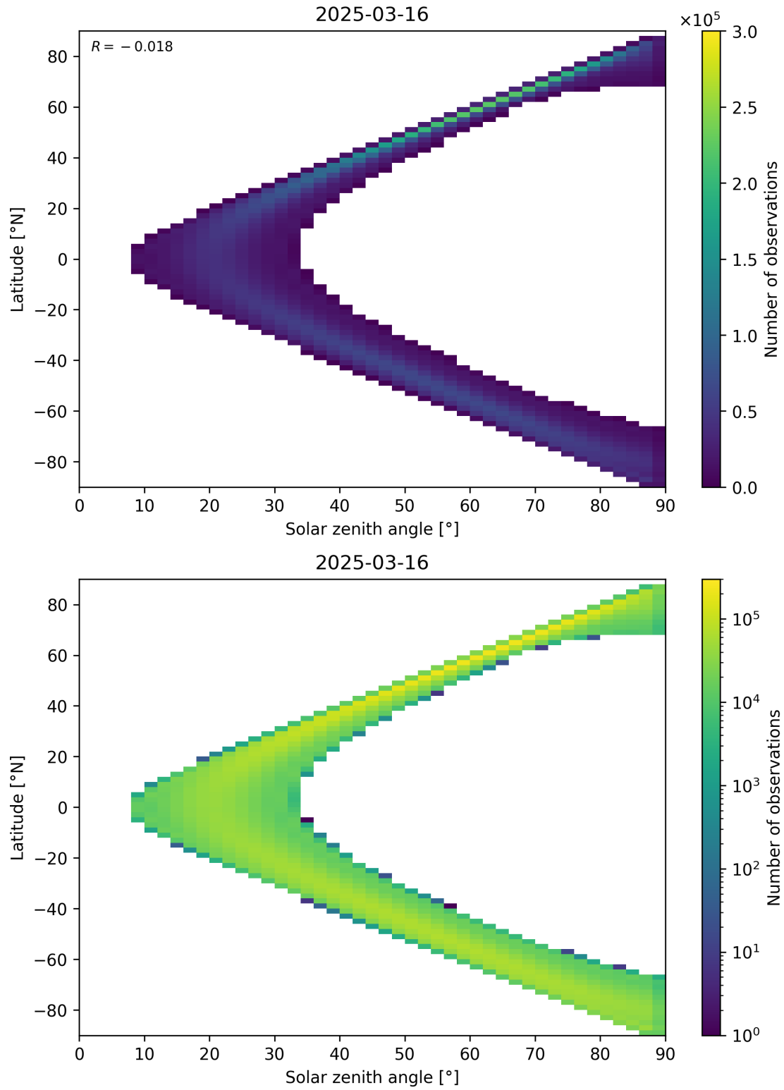
Figure 44: Scatter density plot of “Solar zenith angle” against “Latitude” for 2025-03-15 to 2025-03-17.
