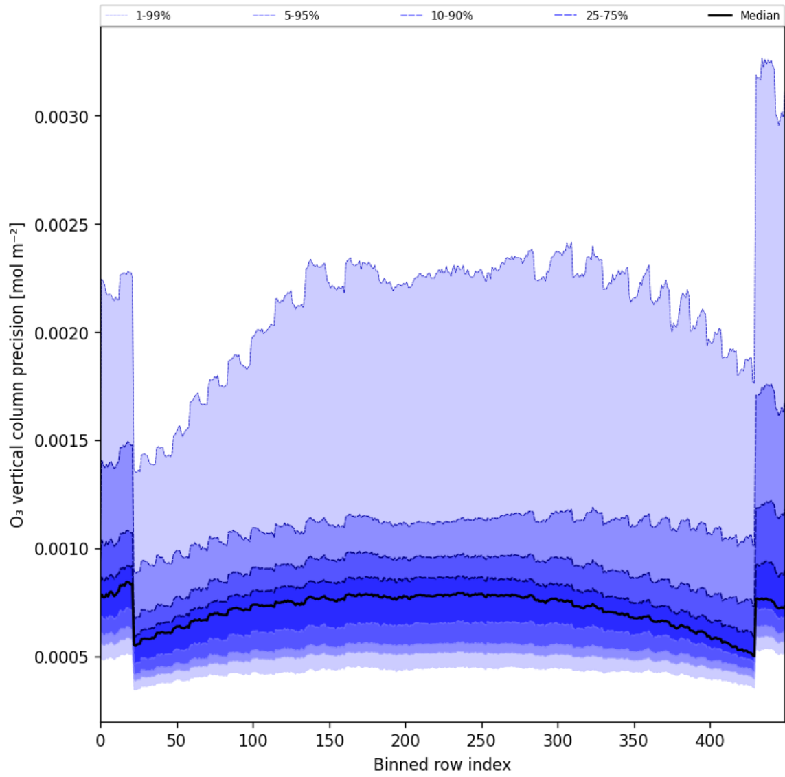
Figure 29: Along track statistics of “O 3 vertical column precision” for 2025-03-15 to 2025-03-17
