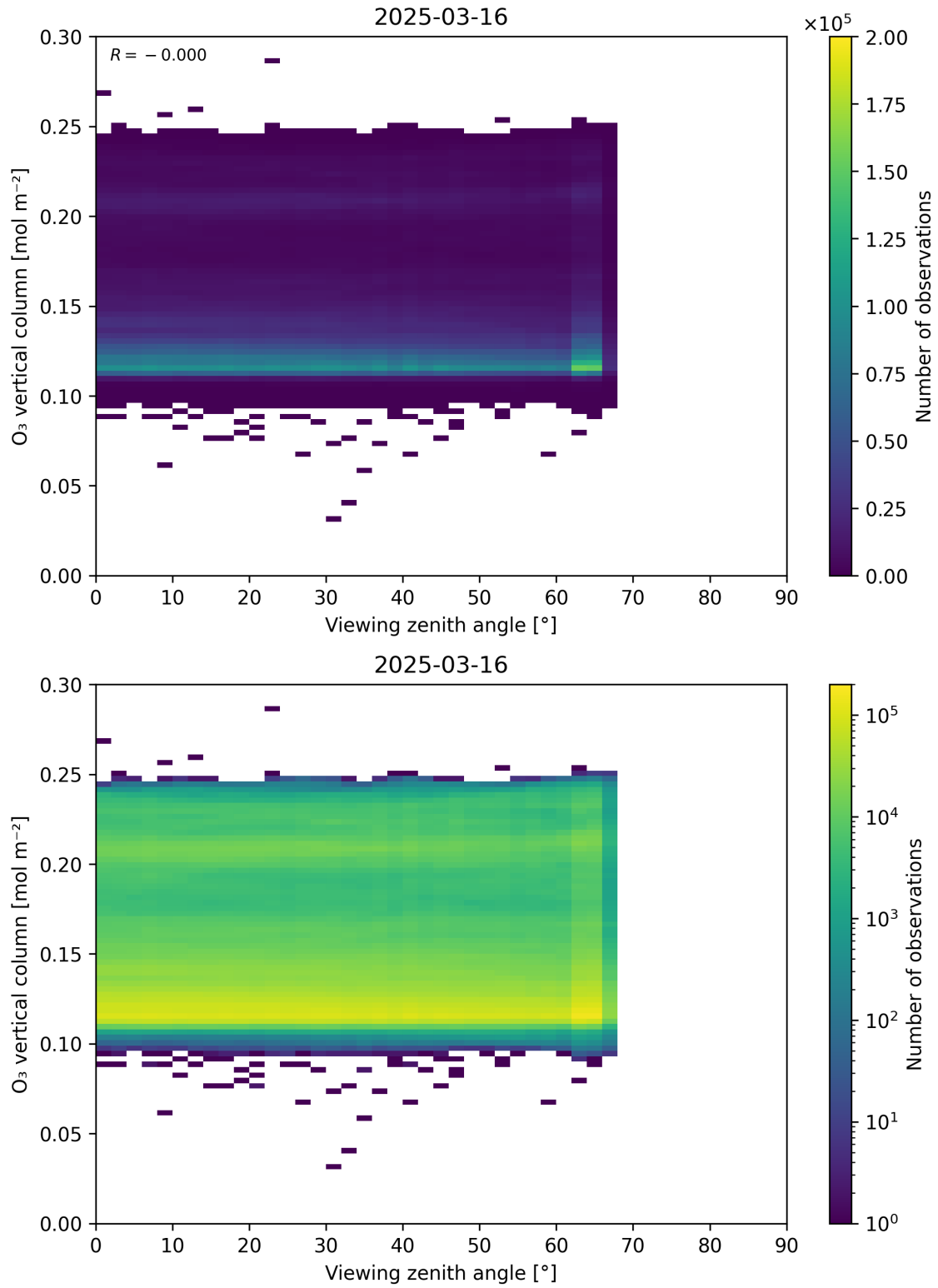
Figure 52: Scatter density plot of “Viewing zenith angle” against “O 3 vertical column” for 2025-03-15 to 2025-03-17.
