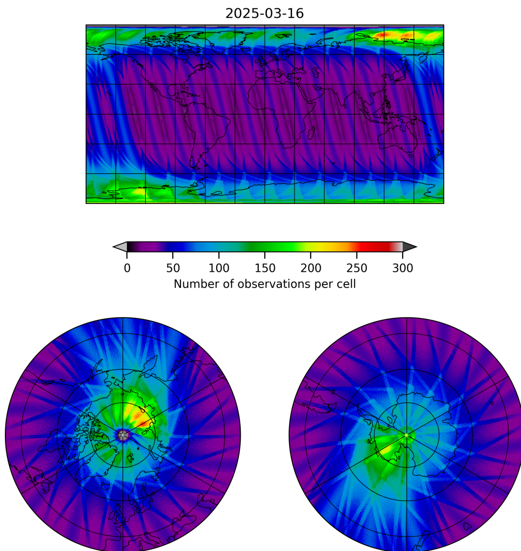
Figure 12: Map of the number of observations for 2025-03-15 to 2025-03-17
