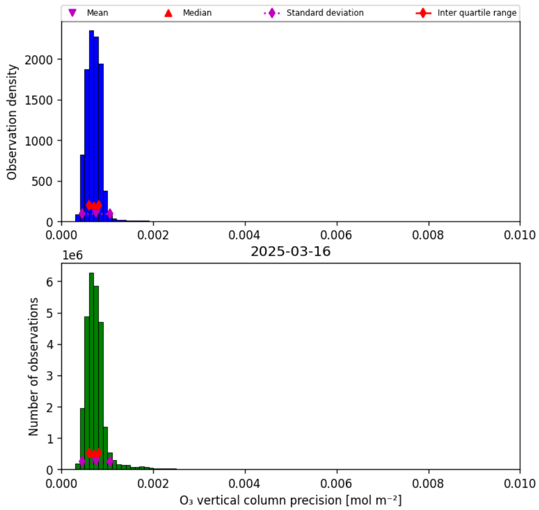
Figure 22: Histogram of “O 3 vertical column precision” for 2025-03-15 to 2025-03-17
