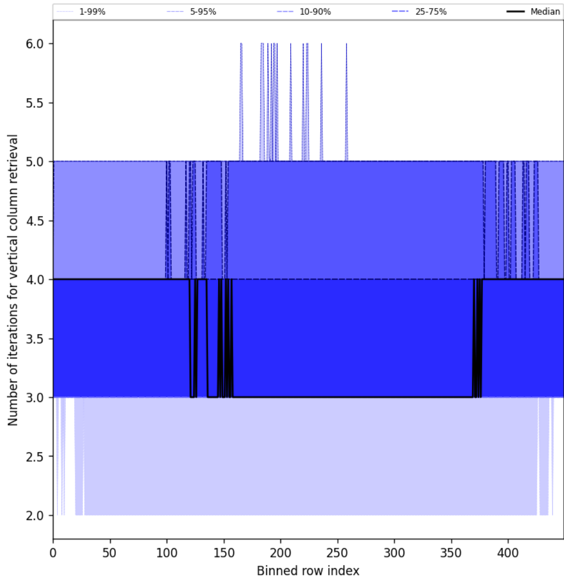
Figure 33: Along track statistics of “Number of iterations for vertical column retrieval” for 2025-03-15 to 2025-03-17
