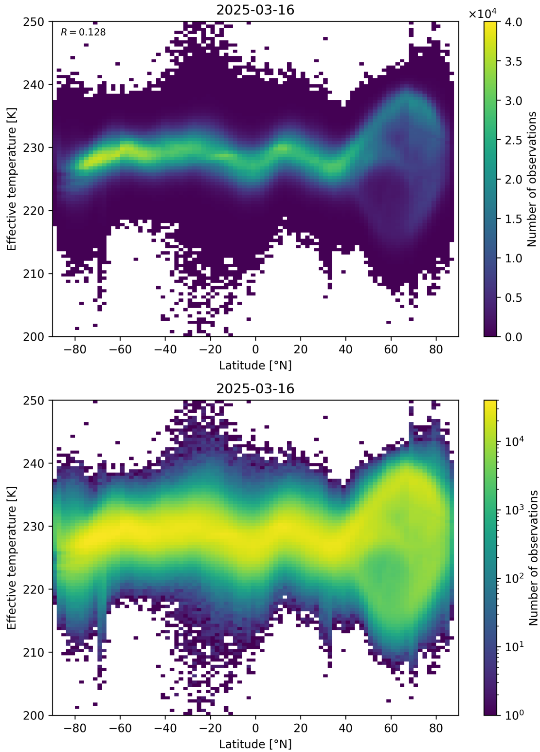
Figure 34: Scatter density plot of “Latitude” against “Effective temperature” for 2025-03-15 to 2025-03-17.
