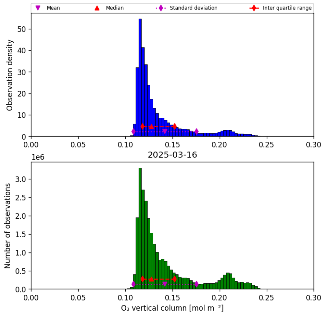
Figure 21: Histogram of “O 3 vertical column” for 2025-03-15 to 2025-03-17
