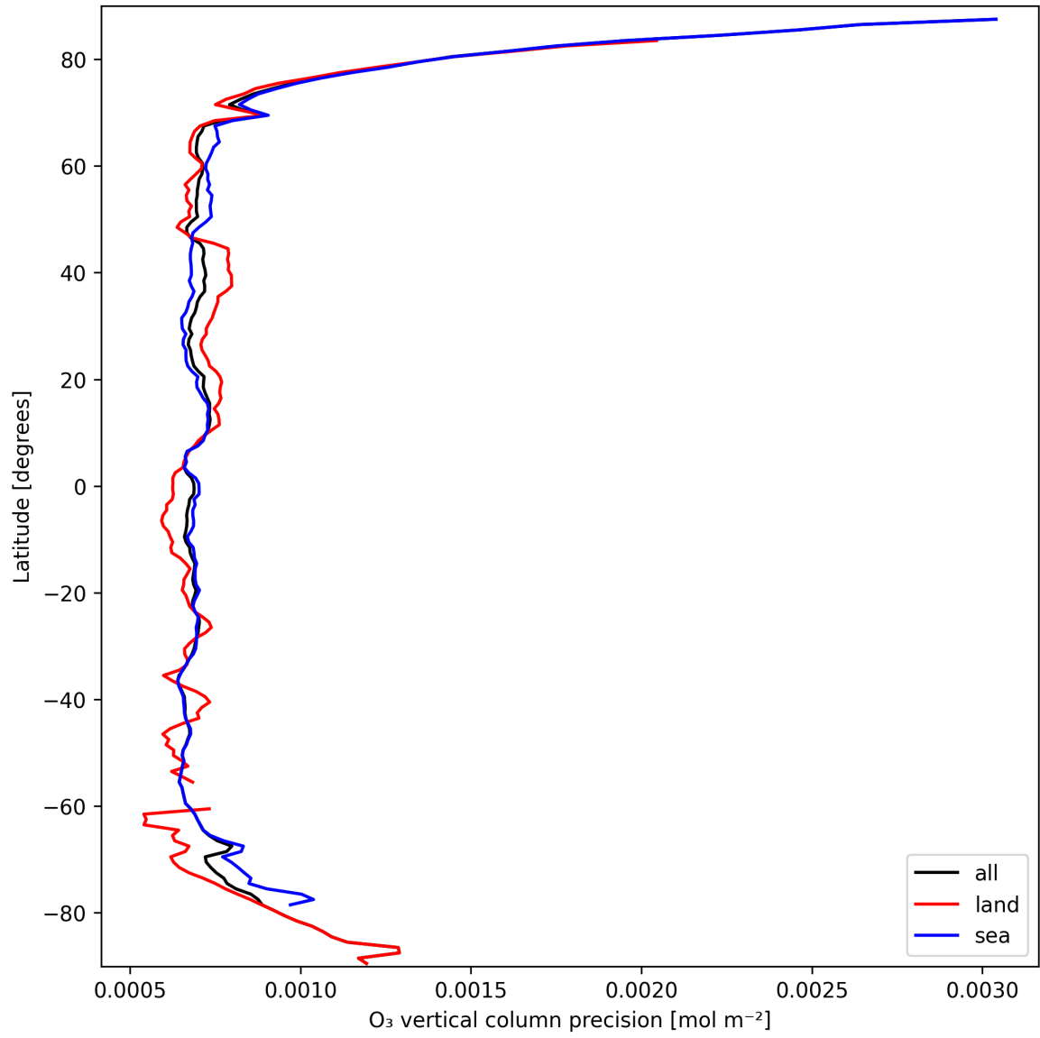
Figure 15: Zonal average of “O 3 vertical column precision” for 2025-03-15 to 2025-03-17.
