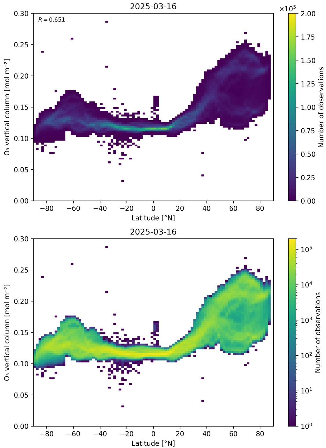
Figure 36: Scatter density plot of “Latitude” against “O 3 vertical column” for 2025-03-15 to 2025-03-17.
