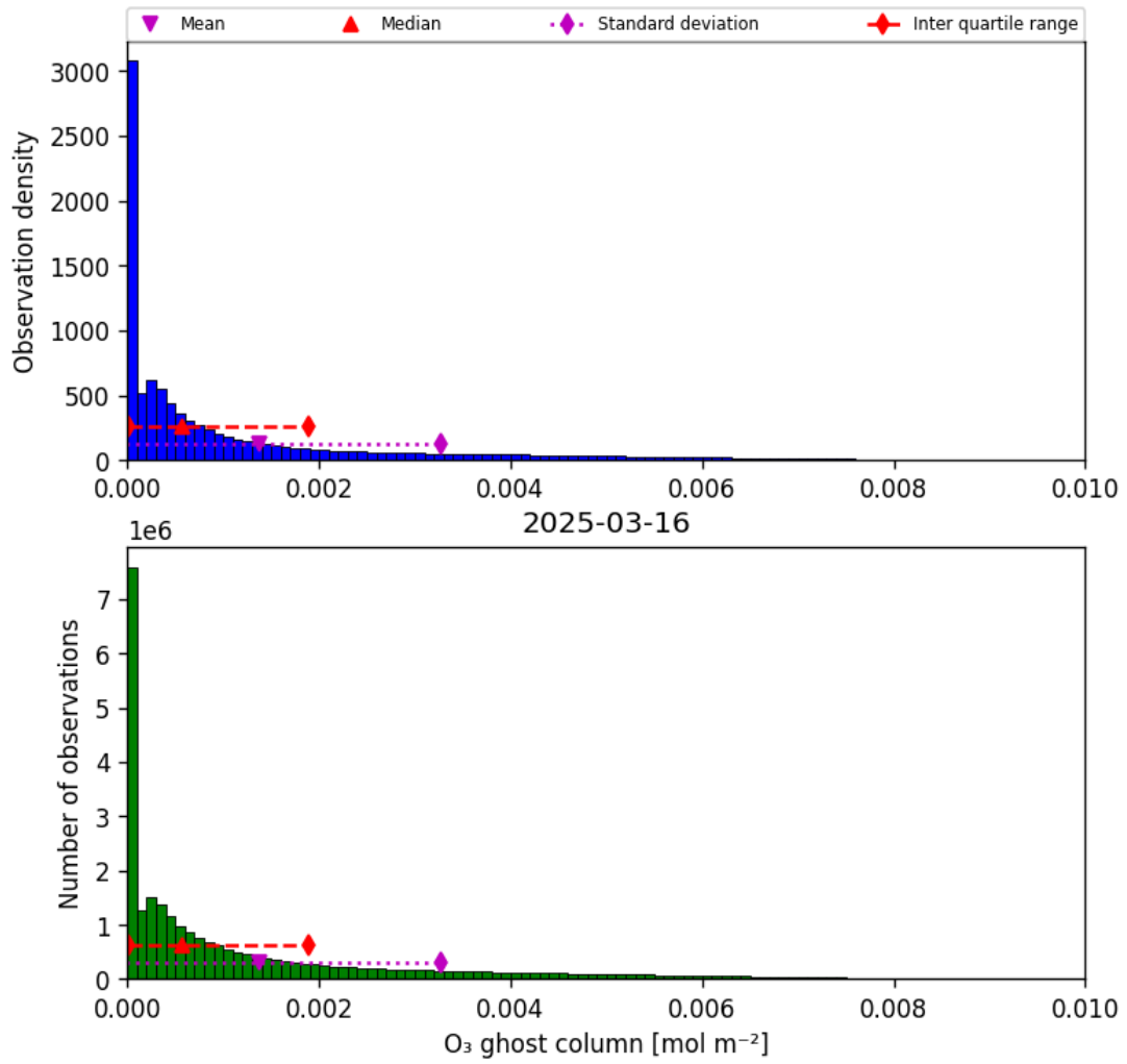
Figure 25: Histogram of “O 3 ghost column” for 2025-03-15 to 2025-03-17
