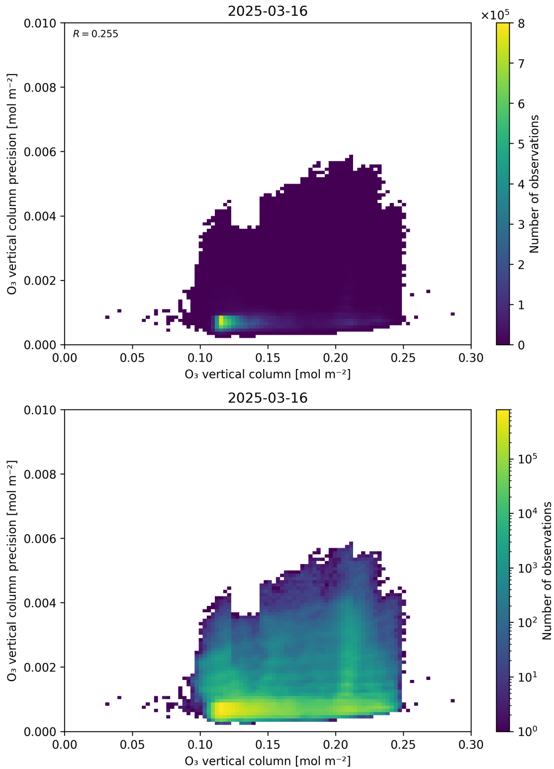
Figure 41: Scatter density plot of “O 3 vertical column” against “O 3 vertical column precision” for 2025-03-15 to 2025-03-17.
