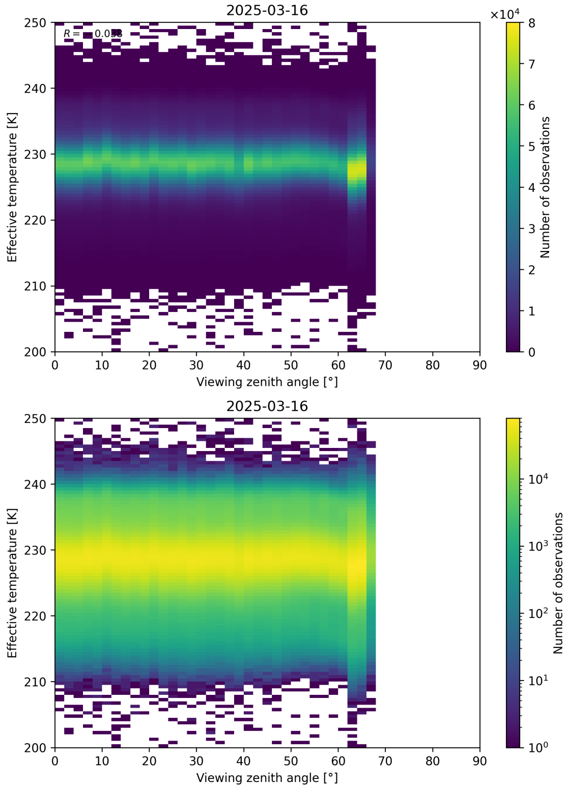
Figure 50: Scatter density plot of “Viewing zenith angle” against “Effective temperature” for 2025-03-15 to 2025-03-17.
