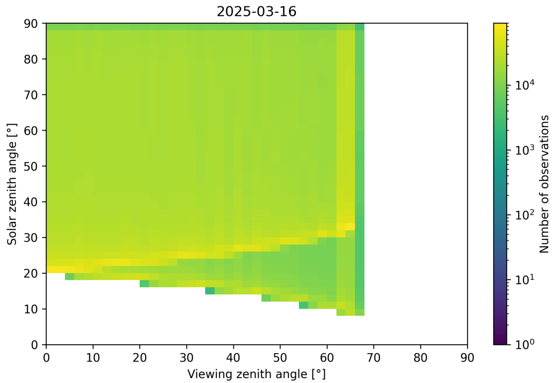
Figure 54: Scatter density plot of “Viewing zenith angle” against “Solar zenith angle” for 2025-03-15 to 2025-03-17.
