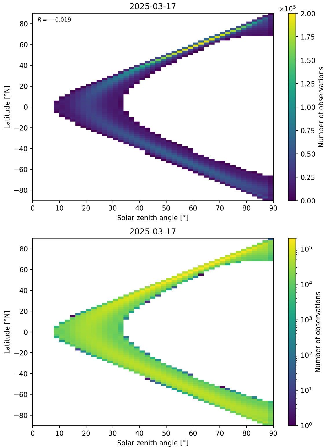
Figure 44: Scatter density plot of “Solar zenith angle” against “Latitude” for 2025-03-17 to 2025-03-18.
