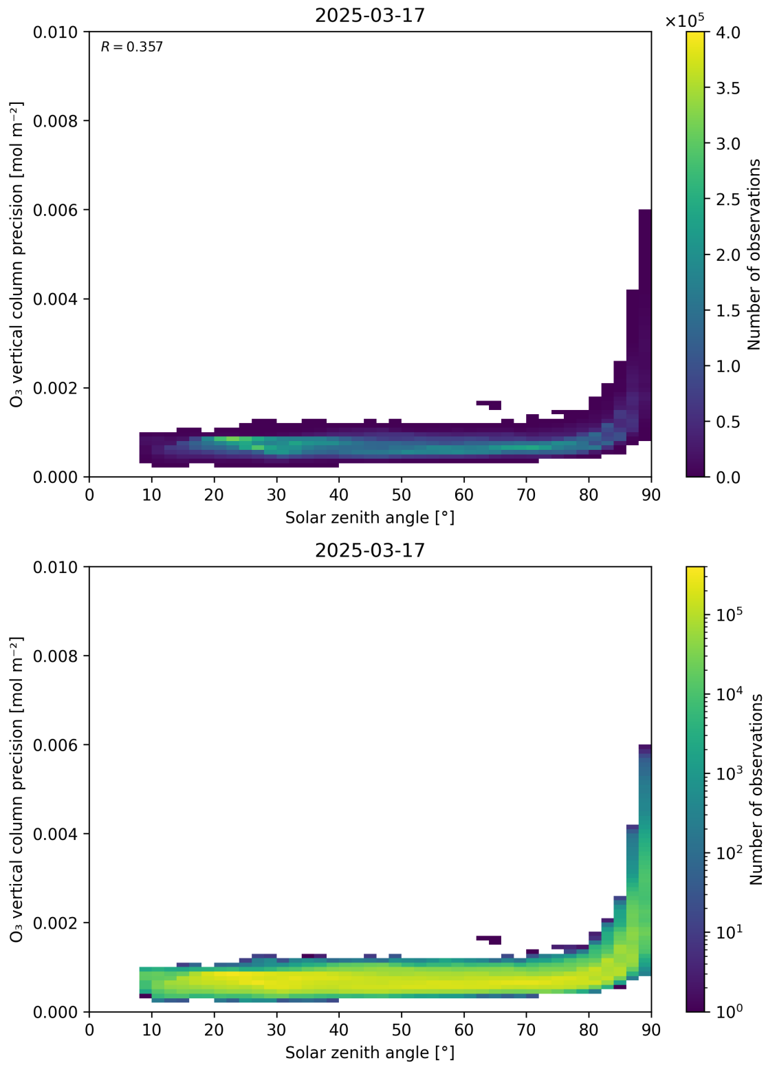
Figure 48: Scatter density plot of “Solar zenith angle” against “O 3 vertical column precision” for 2025-03-17 to 2025-03-18.
