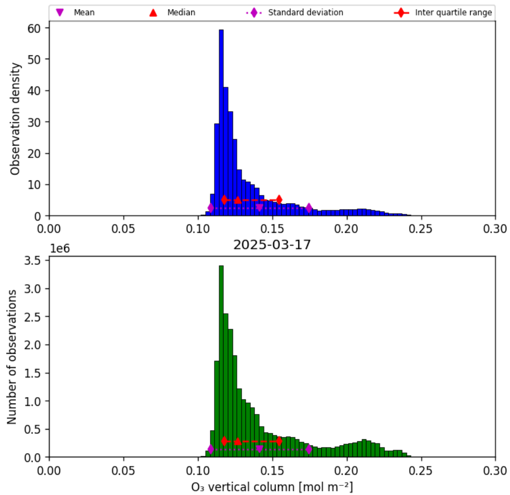
Figure 21: Histogram of “O 3 vertical column” for 2025-03-17 to 2025-03-18
