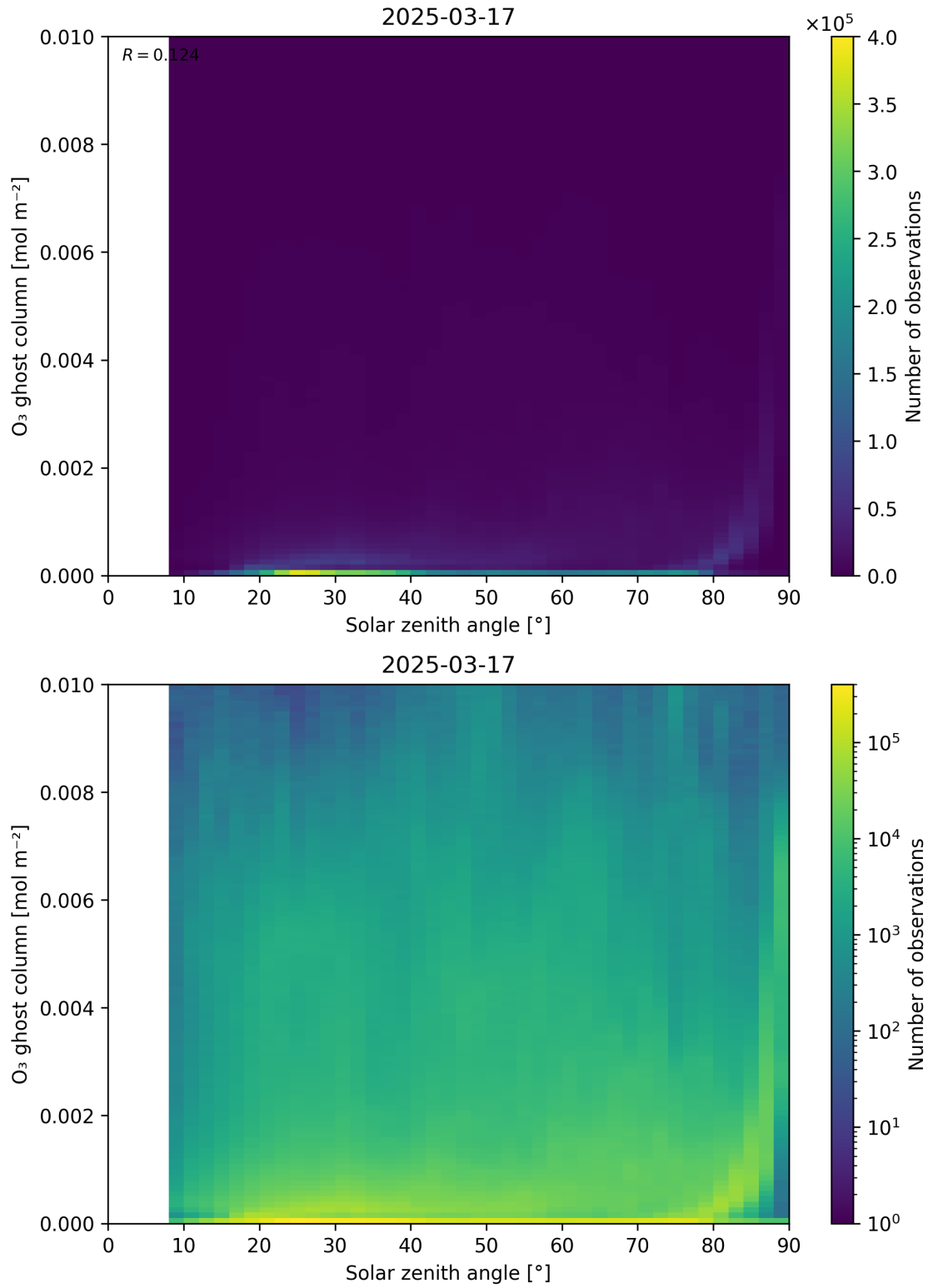
Figure 46: Scatter density plot of “Solar zenith angle” against “O 3 ghost column” for 2025-03-17 to 2025-03-18.
