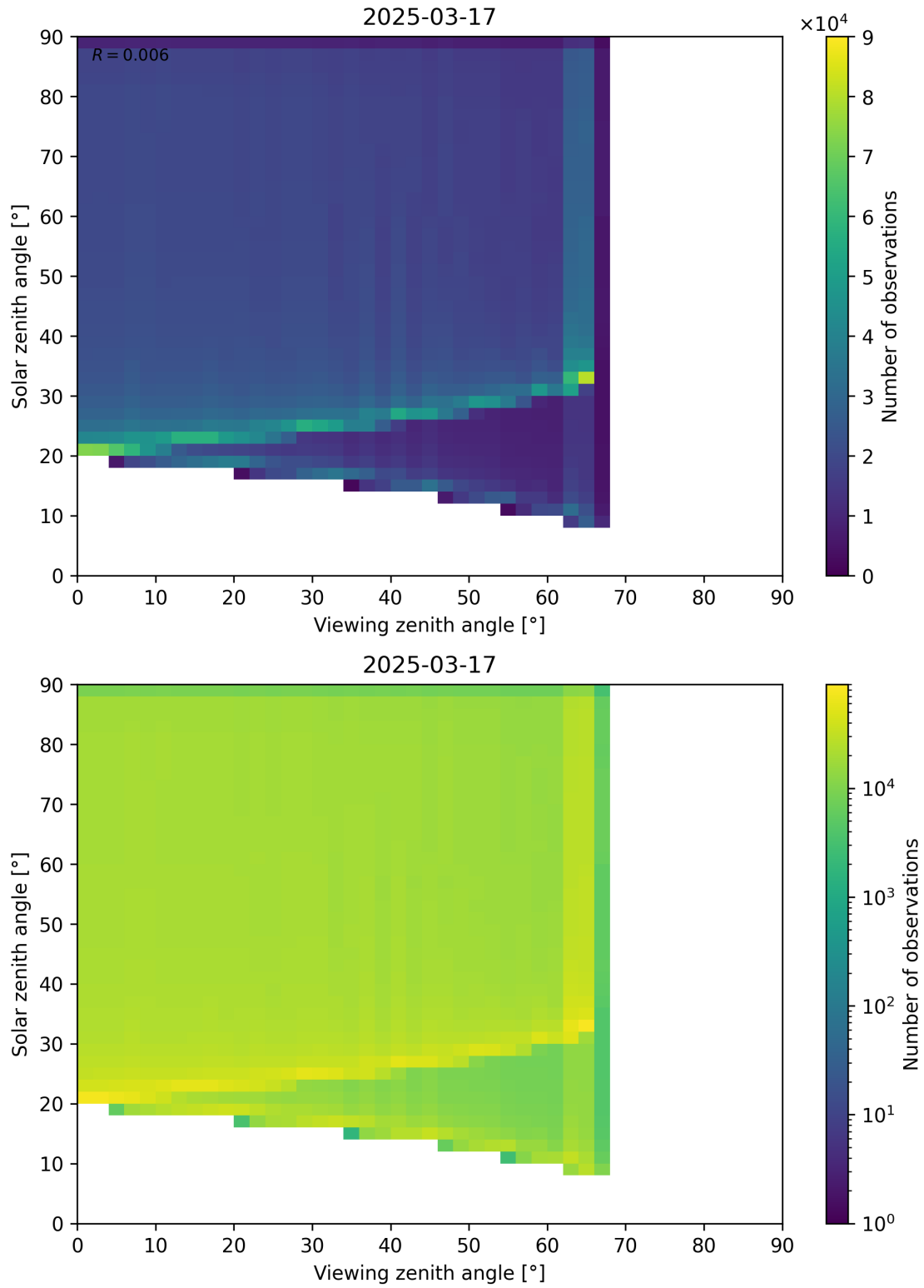
Figure 54: Scatter density plot of “Viewing zenith angle” against “Solar zenith angle” for 2025-03-17 to 2025-03-18.
