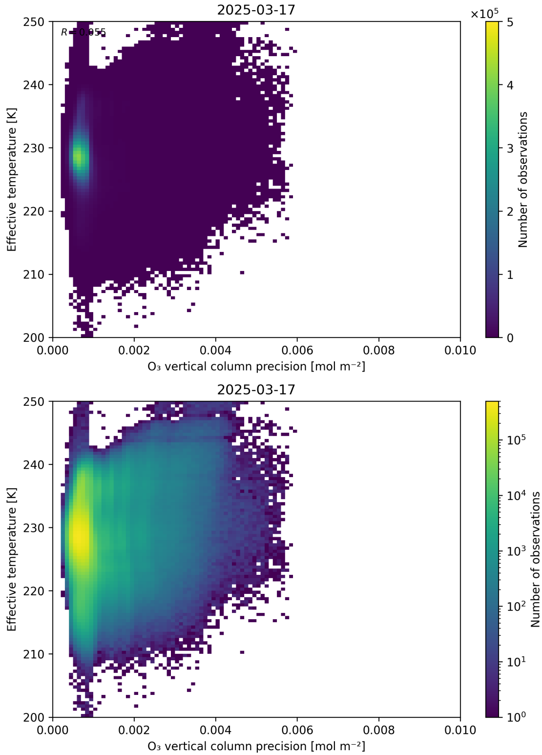
Figure 42: Scatter density plot of “O 3 vertical column precision” against “Effective temperature” for 2025-03-17 to 2025-03-18.
