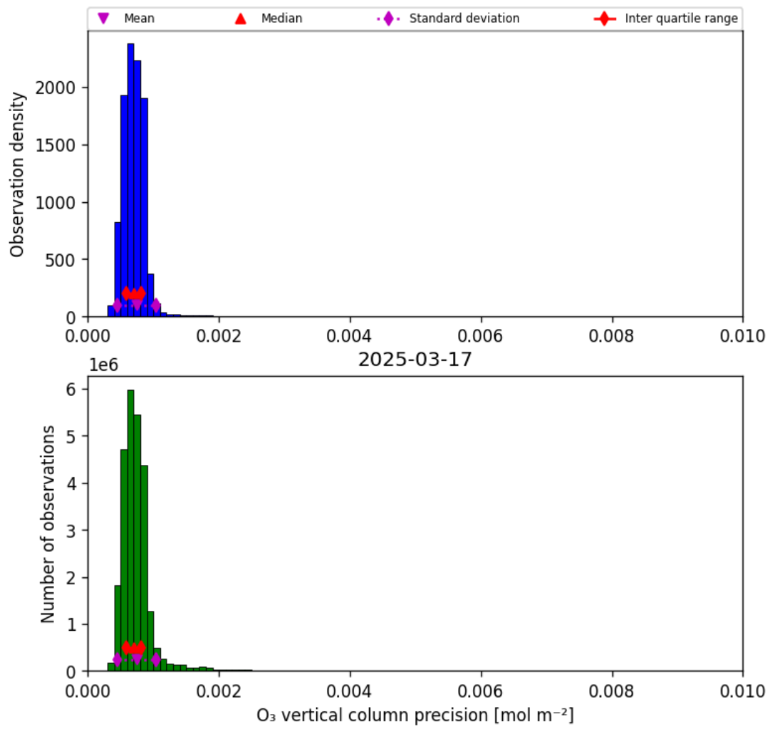
Figure 22: Histogram of “O 3 vertical column precision” for 2025-03-17 to 2025-03-18
