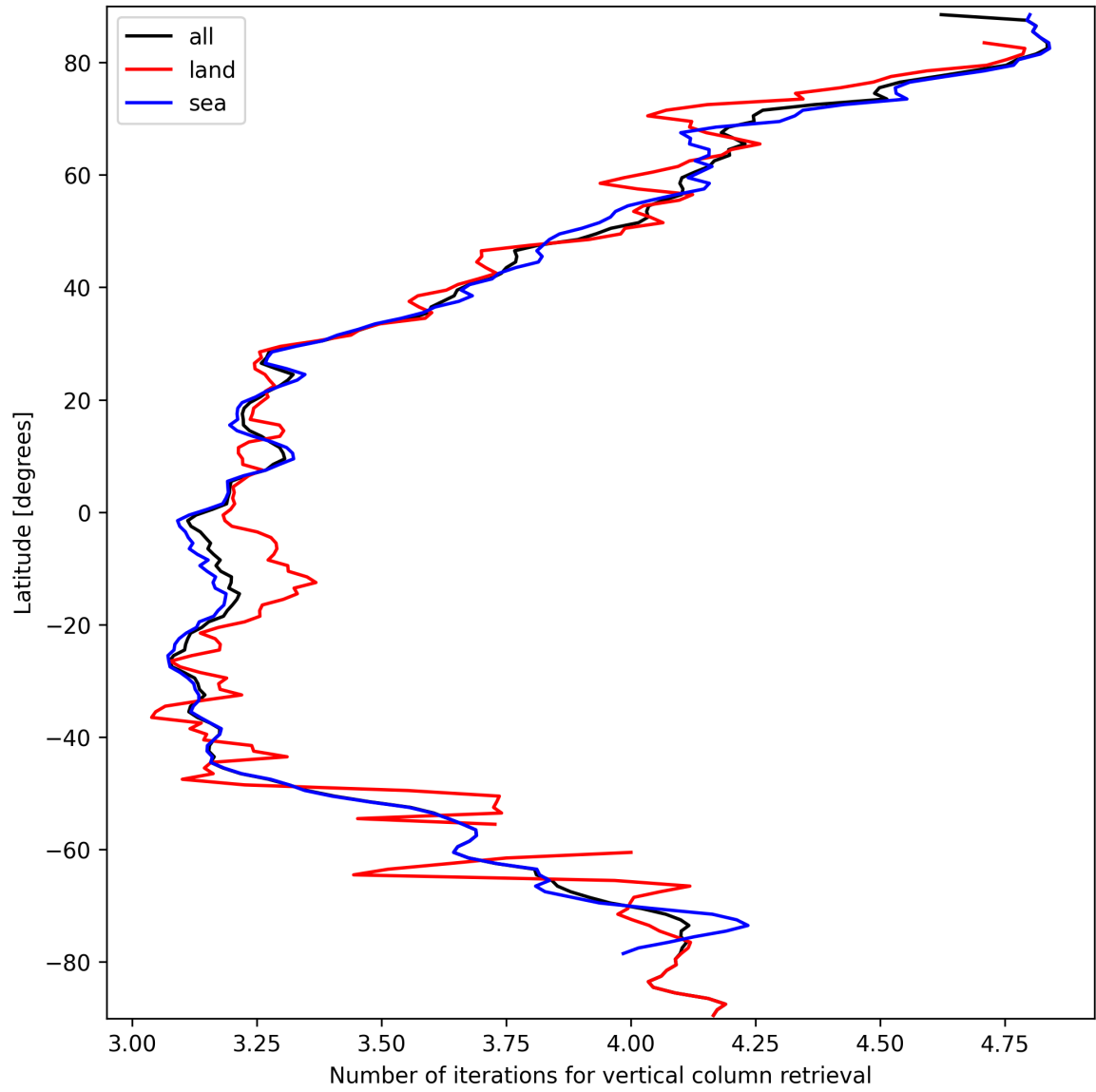
Figure 19: Zonal average of “Number of iterations for vertical column retrieval” for 2025-03-17 to 2025-03-18.
