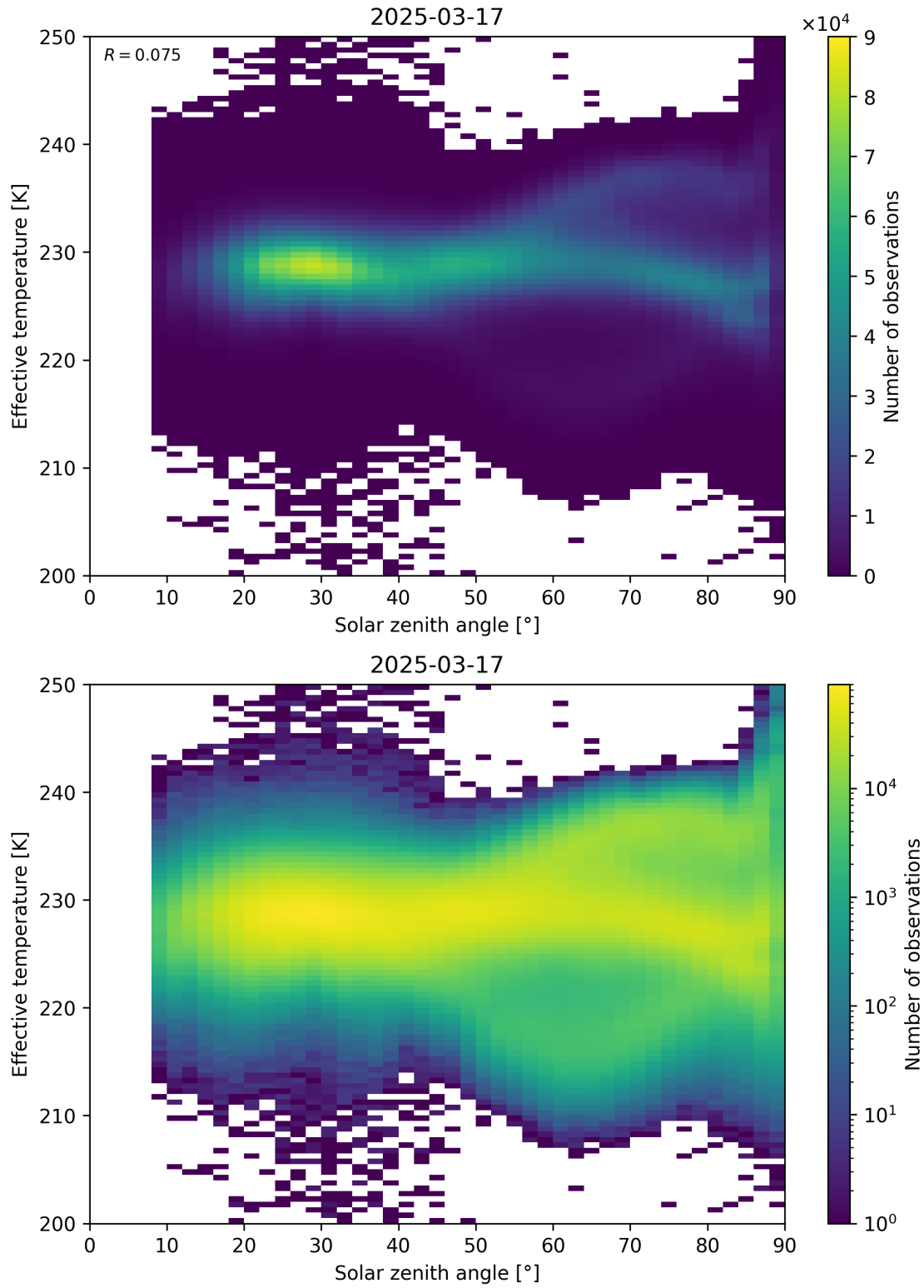
Figure 45: Scatter density plot of “Solar zenith angle” against “Effective temperature” for 2025-03-17 to 2025-03-18.
