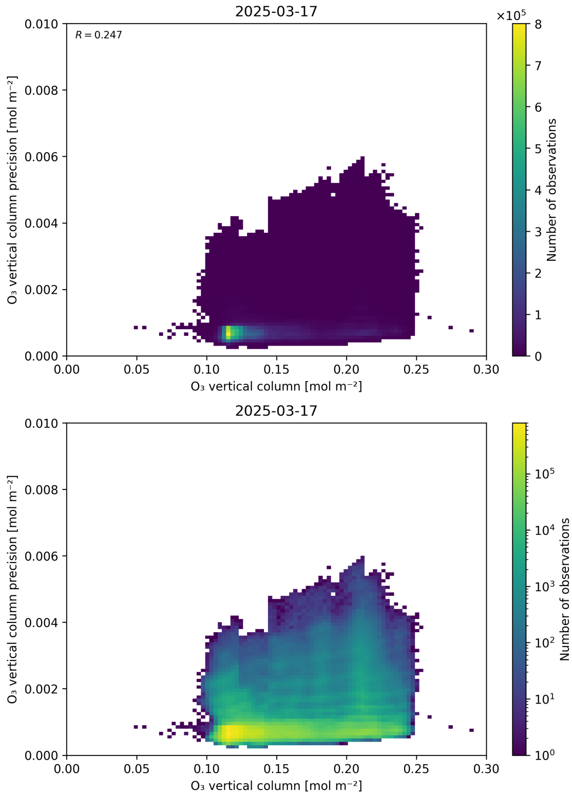
Figure 41: Scatter density plot of “O 3 vertical column” against “O 3 vertical column precision” for 2025-03-17 to 2025-03-18.
