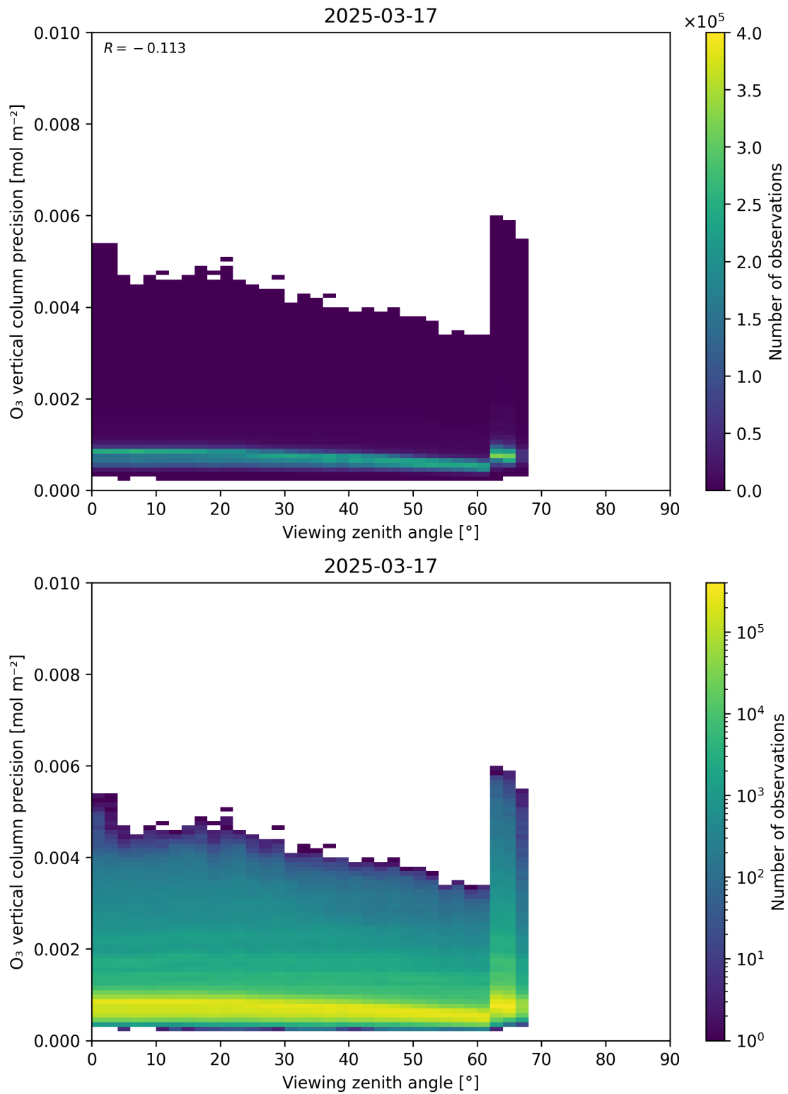
Figure 53: Scatter density plot of “Viewing zenith angle” against “O 3 vertical column precision” for 2025-03-17 to 2025-03-18.
