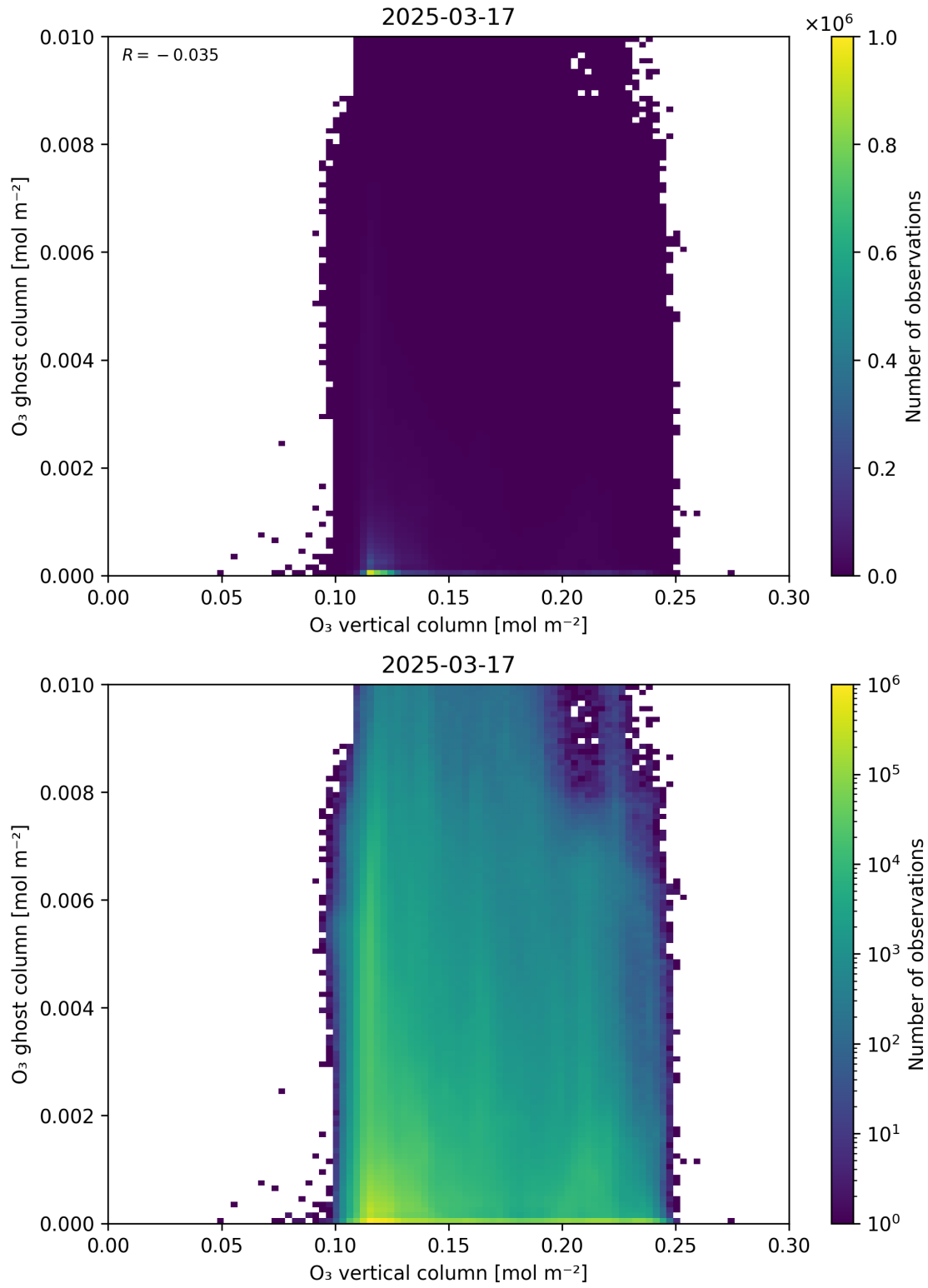
Figure 40: Scatter density plot of “O 3 vertical column” against “O 3 ghost column” for 2025-03-17 to 2025-03-18.
