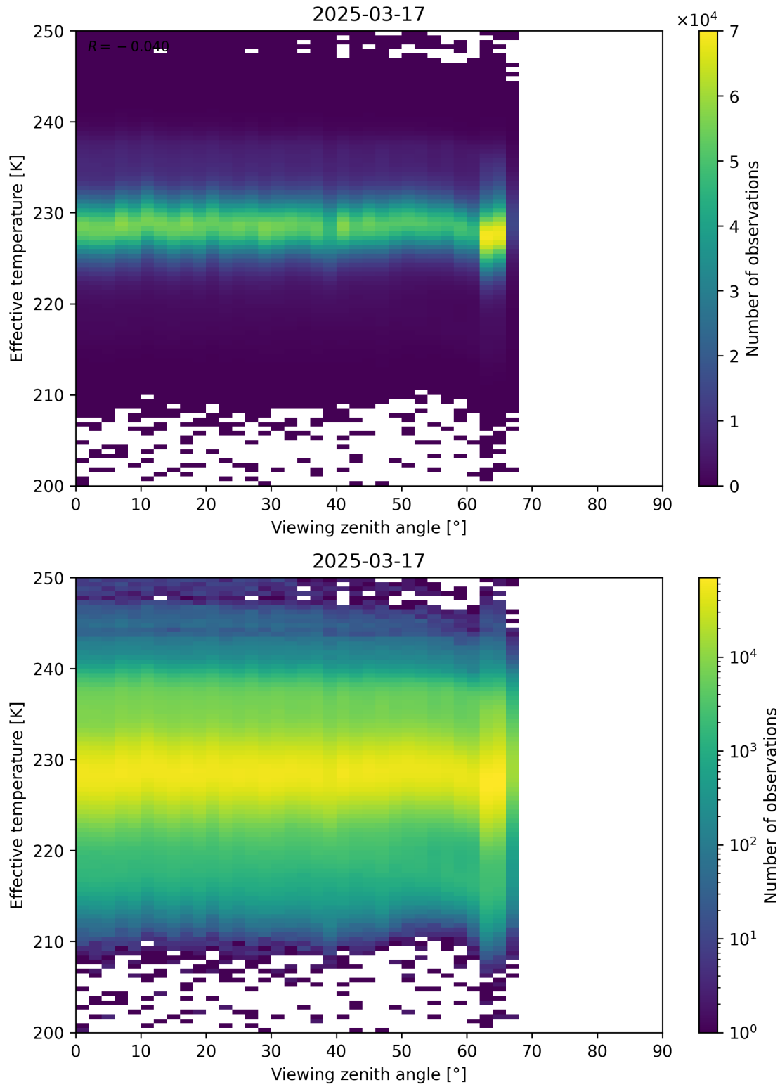
Figure 50: Scatter density plot of “Viewing zenith angle” against “Effective temperature” for 2025-03-17 to 2025-03-18.
