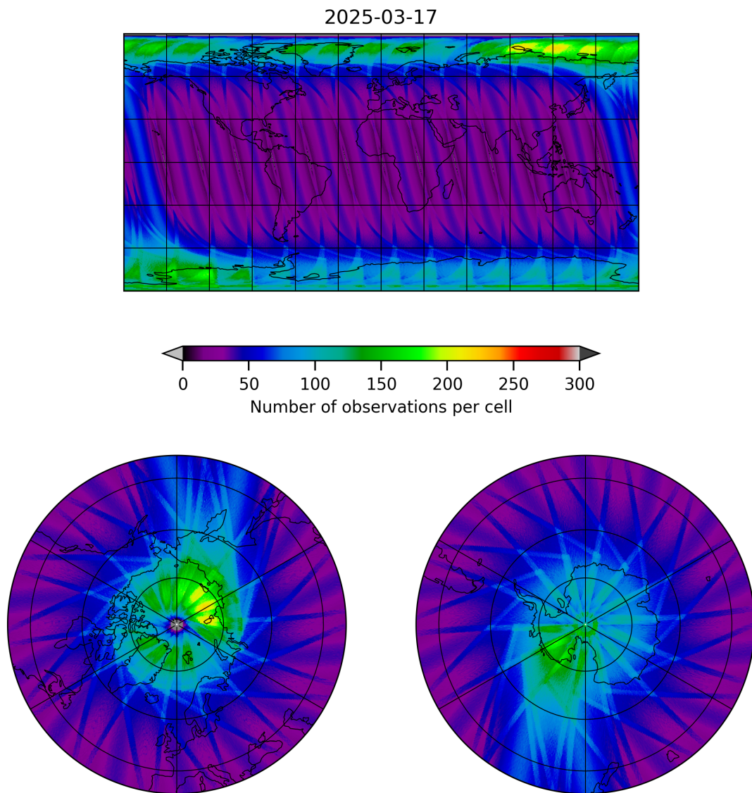
Figure 12: Map of the number of observations for 2025-03-17 to 2025-03-18
