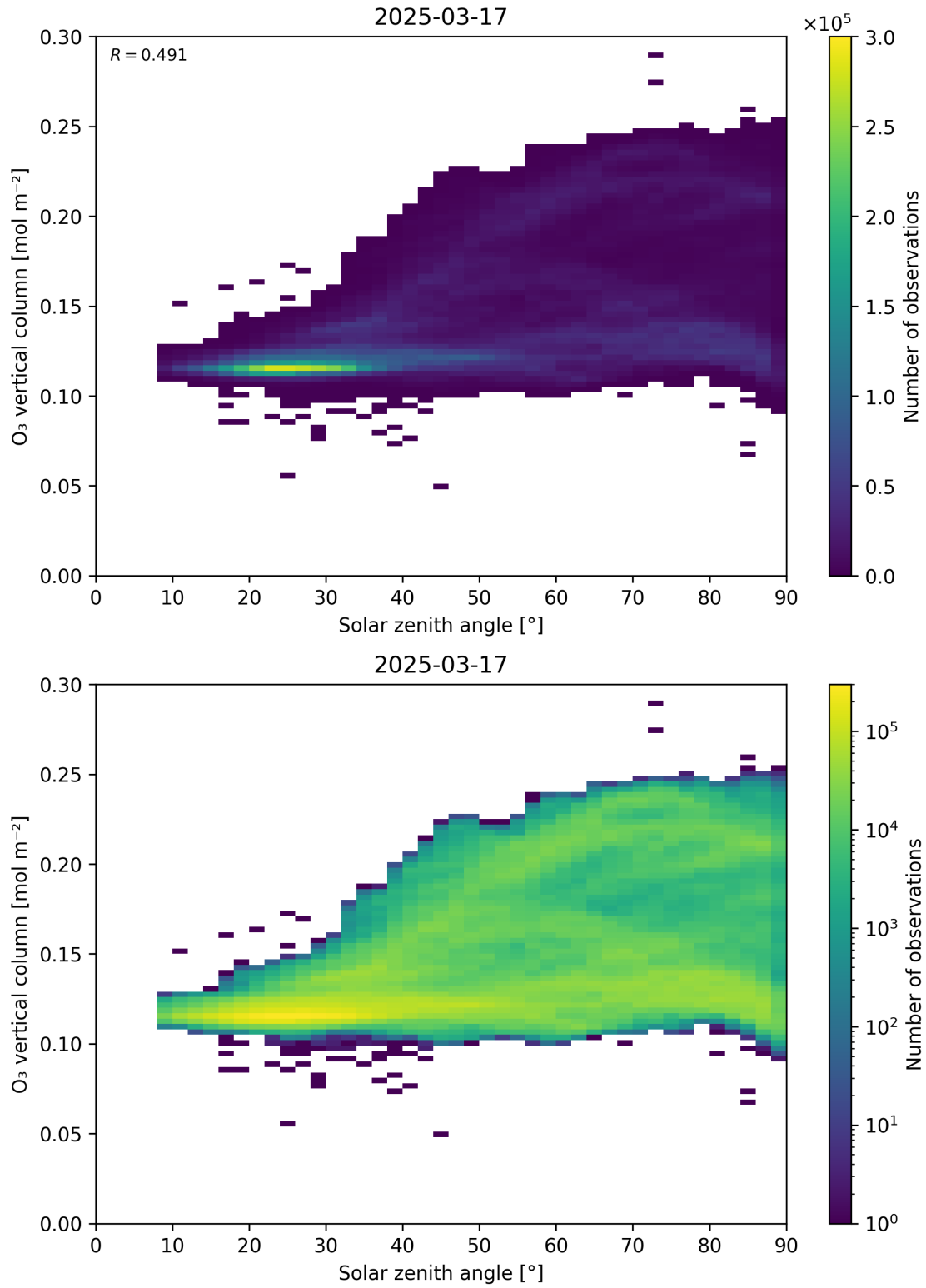
Figure 47: Scatter density plot of “Solar zenith angle” against “O 3 vertical column” for 2025-03-17 to 2025-03-18.
