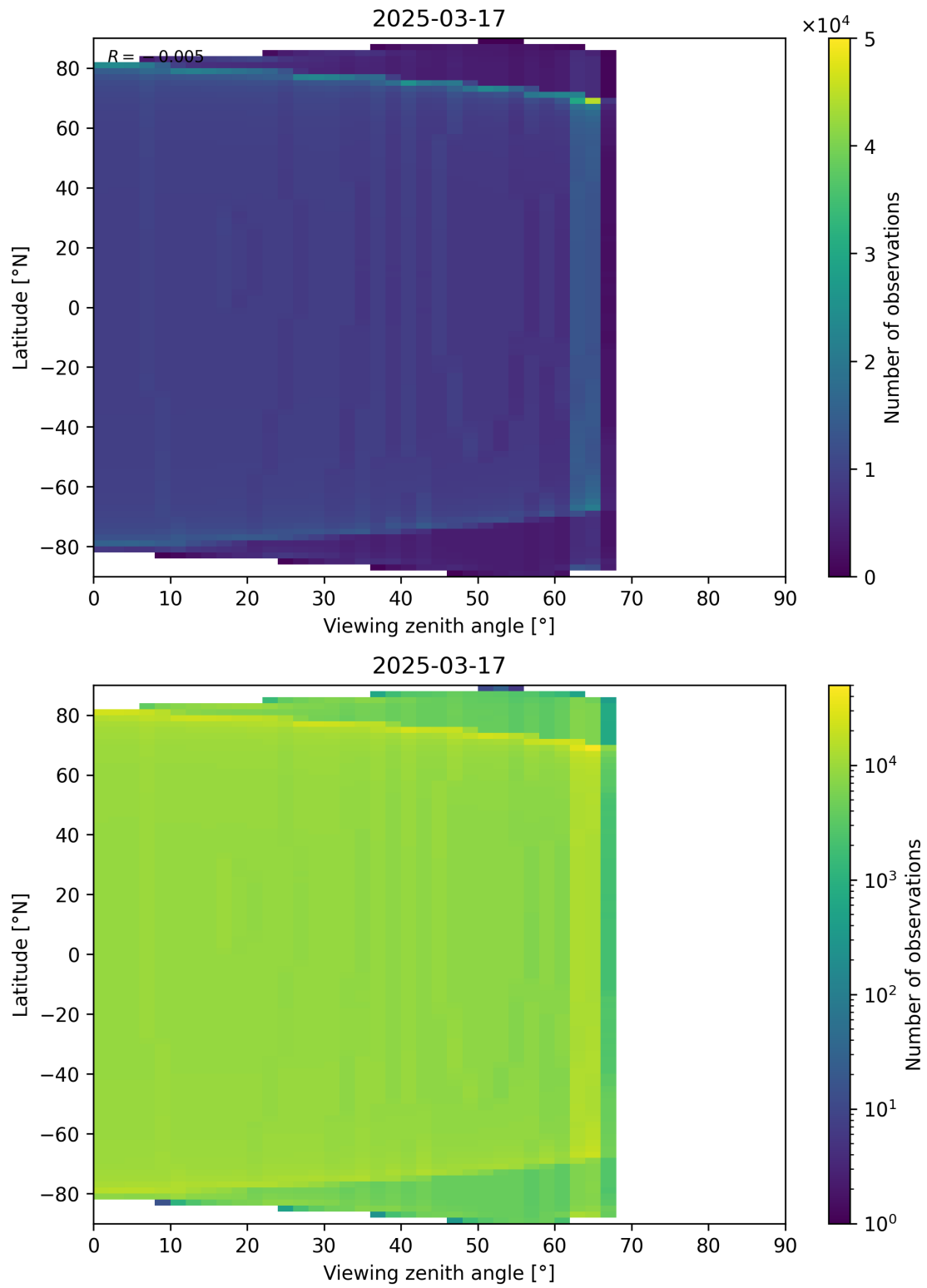
Figure 49: Scatter density plot of “Viewing zenith angle” against “Latitude” for 2025-03-17 to 2025-03-18.
