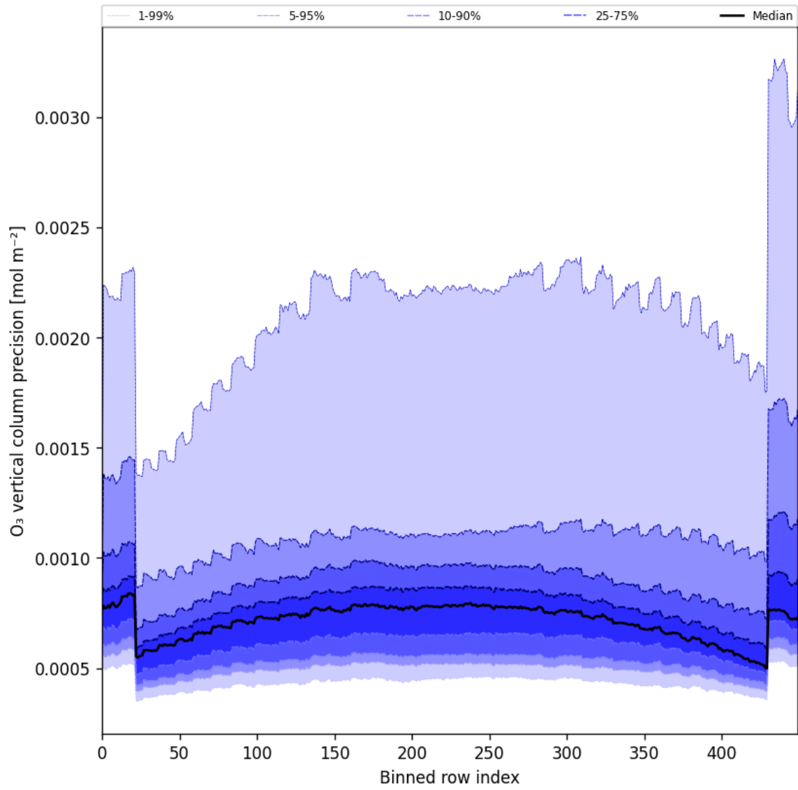
Figure 29: Along track statistics of “O 3 vertical column precision” for 2025-03-17 to 2025-03-18
