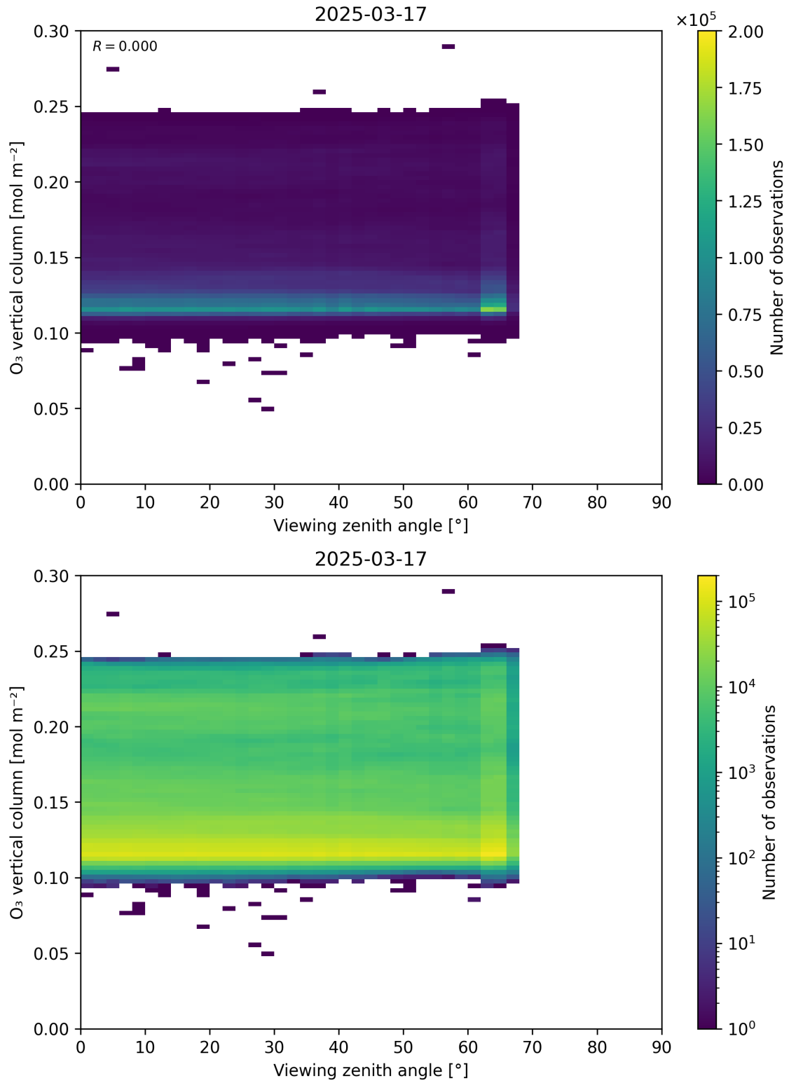
Figure 52: Scatter density plot of “Viewing zenith angle” against “O 3 vertical column” for 2025-03-17 to 2025-03-18.
