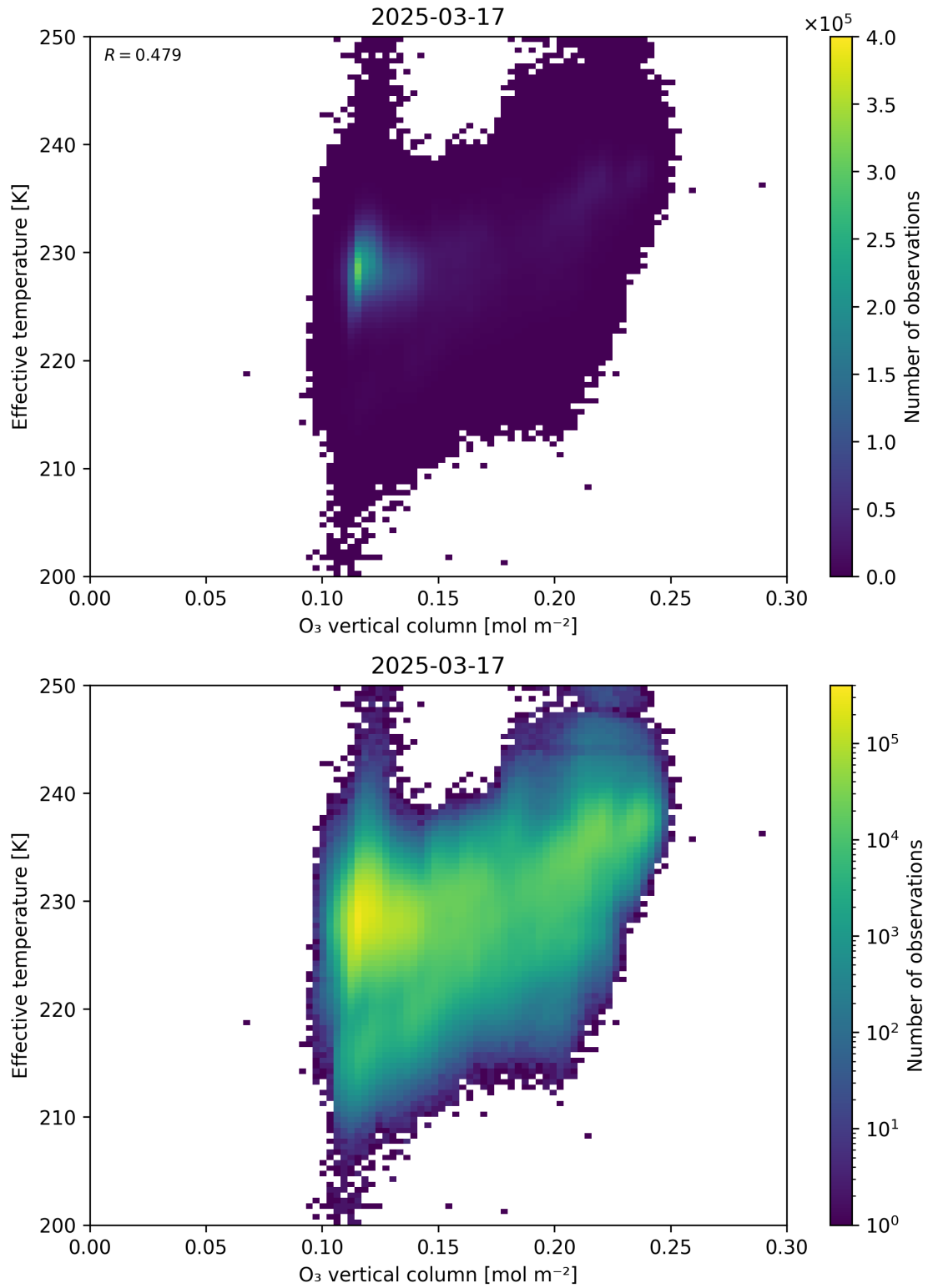
Figure 39: Scatter density plot of “O 3 vertical column” against “Effective temperature” for 2025-03-17 to 2025-03-18.
