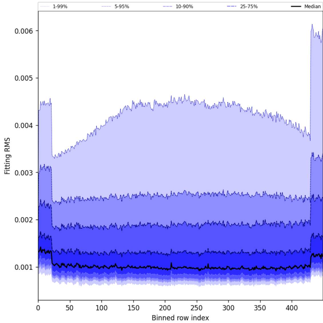
Figure 30: Along track statistics of “Fitting RMS” for 2025-03-17 to 2025-03-18
