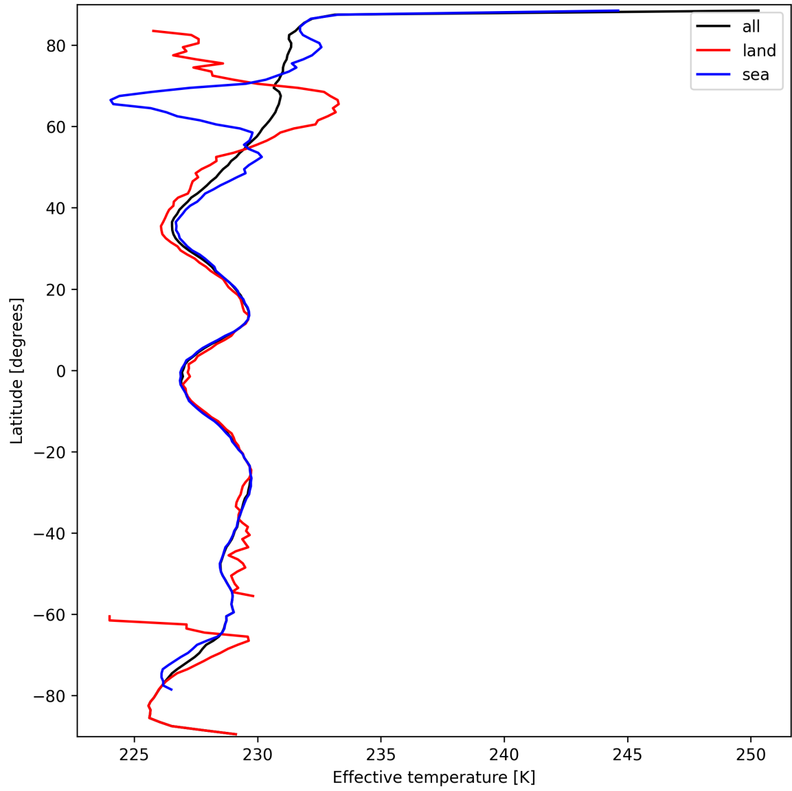
Figure 17: Zonal average of “Effective temperature” for 2025-03-17 to 2025-03-18.
