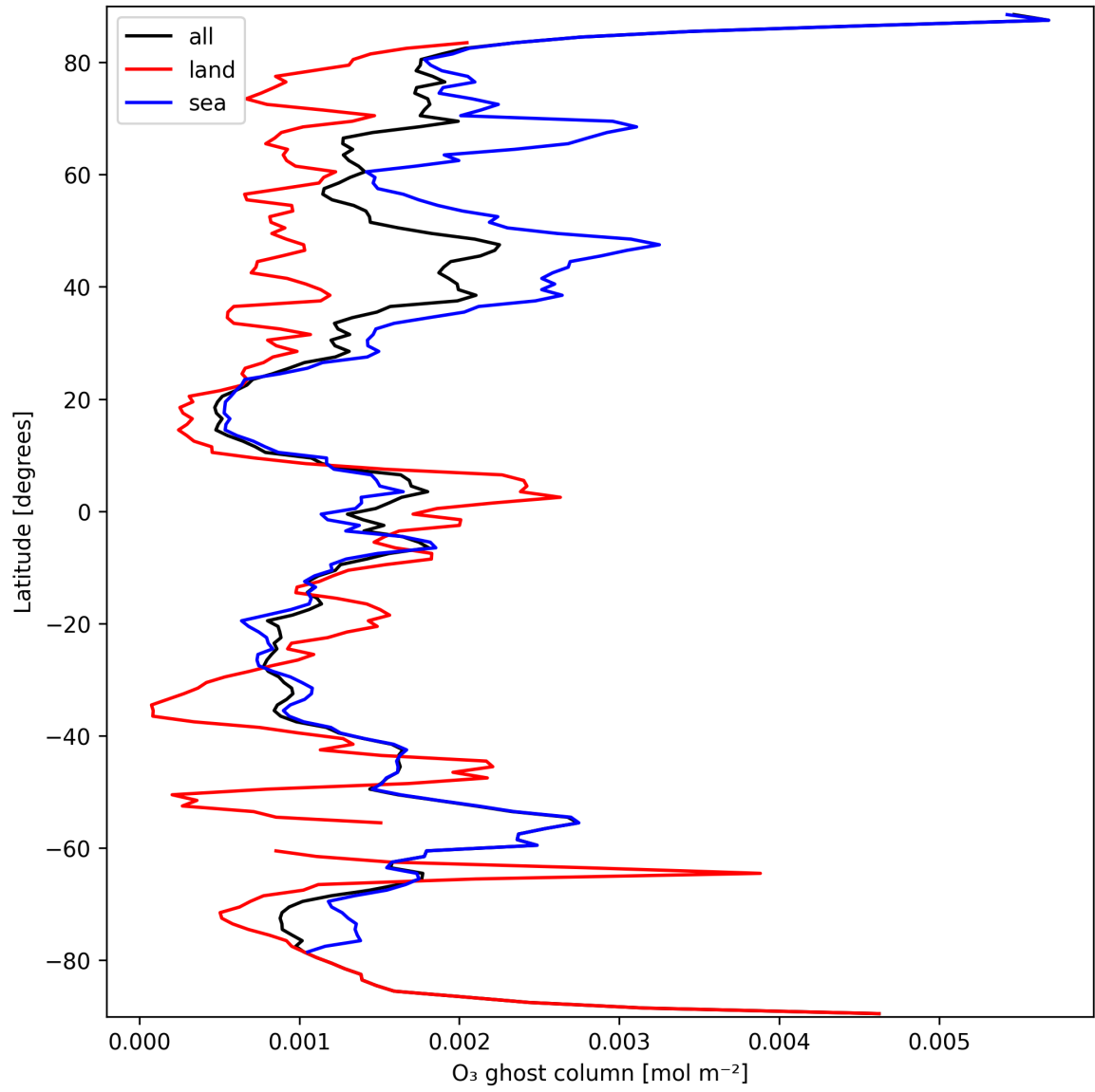
Figure 18: Zonal average of “O 3 ghost column” for 2025-03-17 to 2025-03-18.
