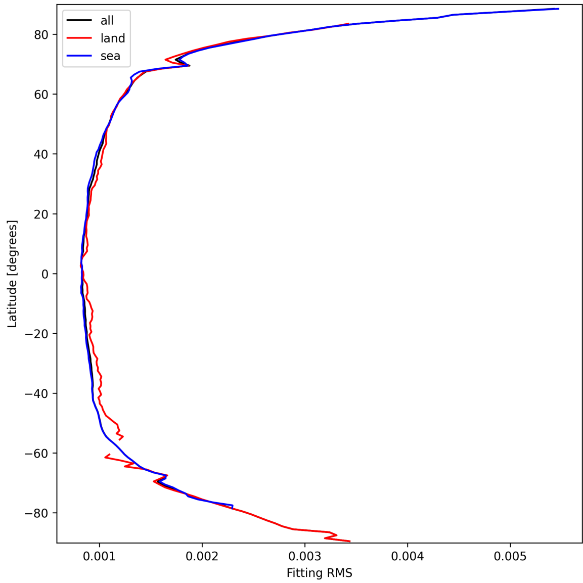
Figure 16: Zonal average of “Fitting RMS” for 2025-03-17 to 2025-03-18.
