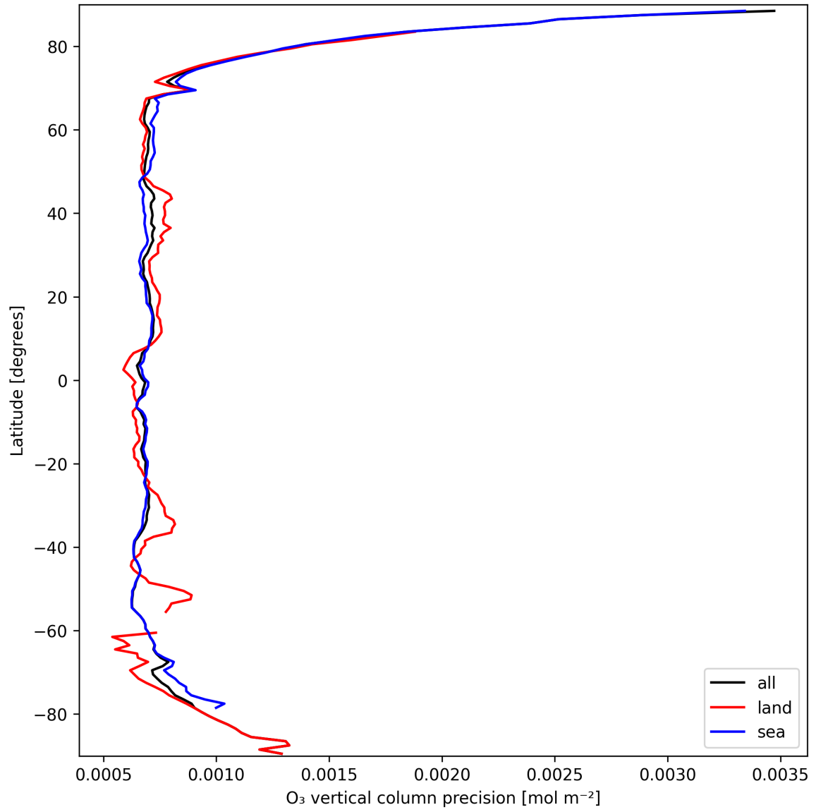
Figure 15: Zonal average of "O 3 vertical column precision" for 2025-03-17 to 2025-03-18.
