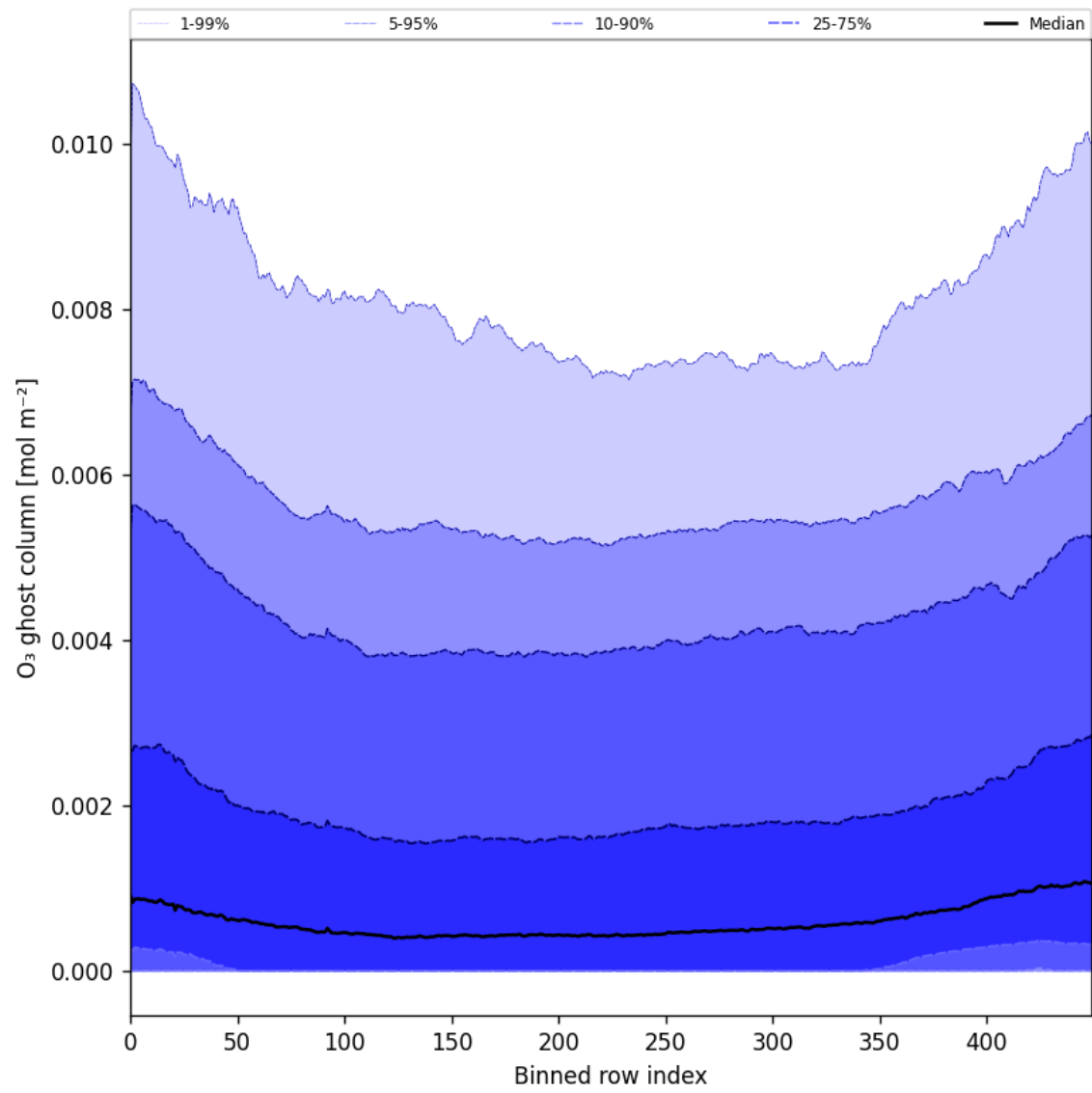
Figure 32: Along track statistics of “O 3 ghost column” for 2025-03-17 to 2025-03-18
