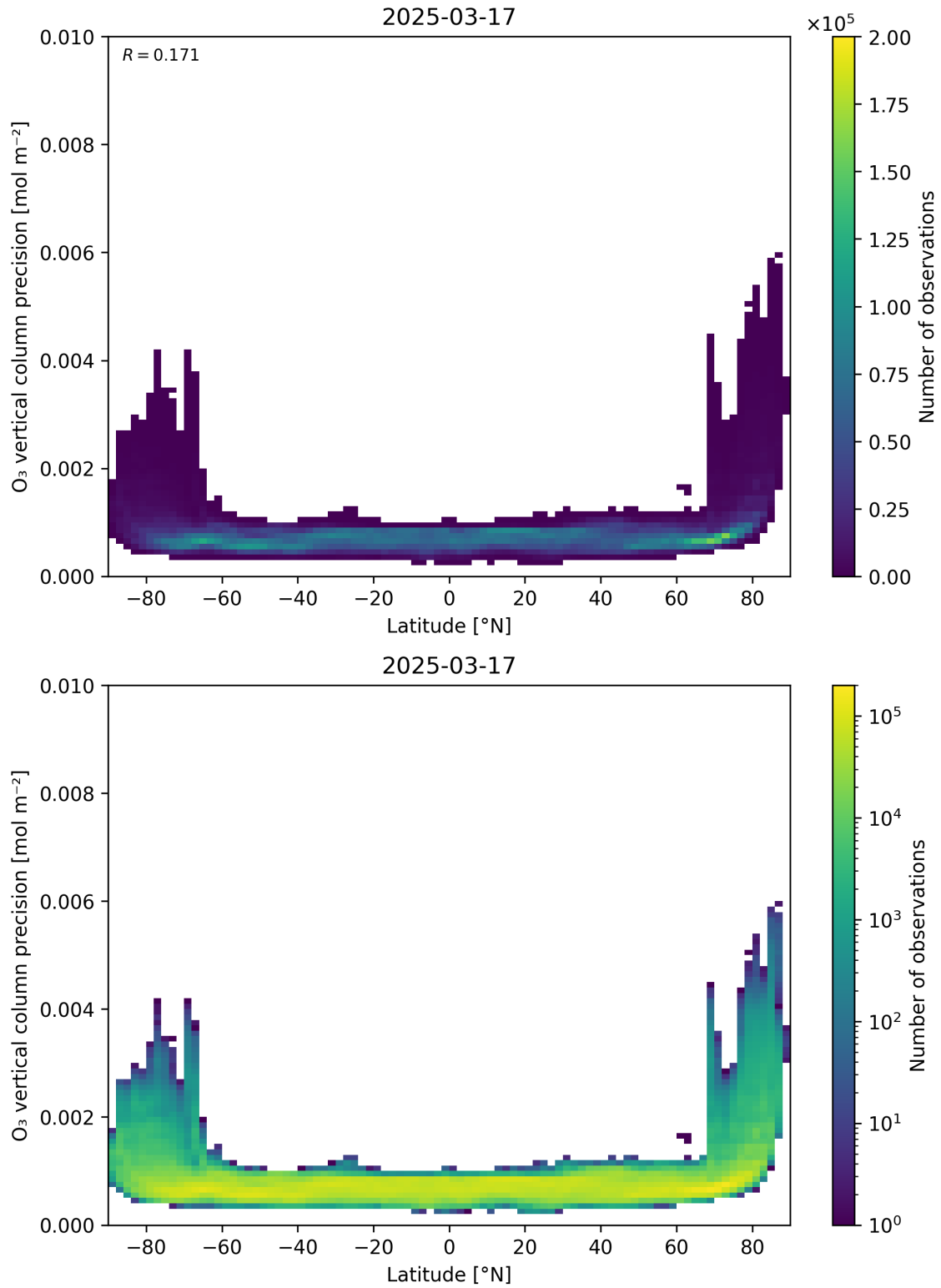
Figure 37: Scatter density plot of “Latitude” against “O 3 vertical column precision” for 2025-03-17 to 2025-03-18.
