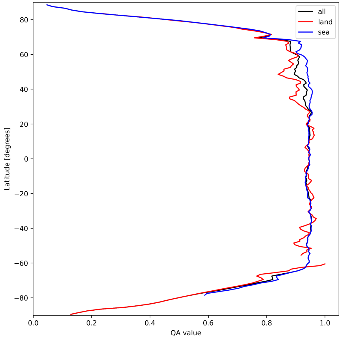
Figure 13: Zonal average of “QA value” for 2025-03-17 to 2025-03-18.
