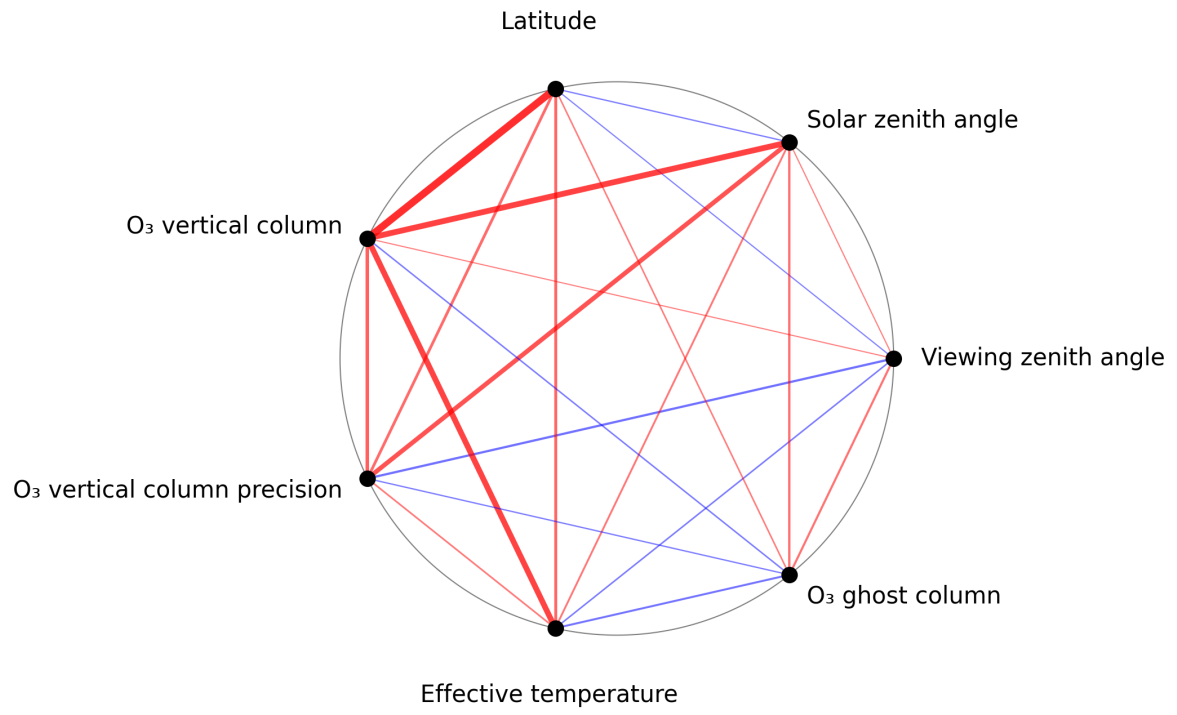
Figure 1: Map of correlation graph for 2025-03-17 to 2025-03-18.
