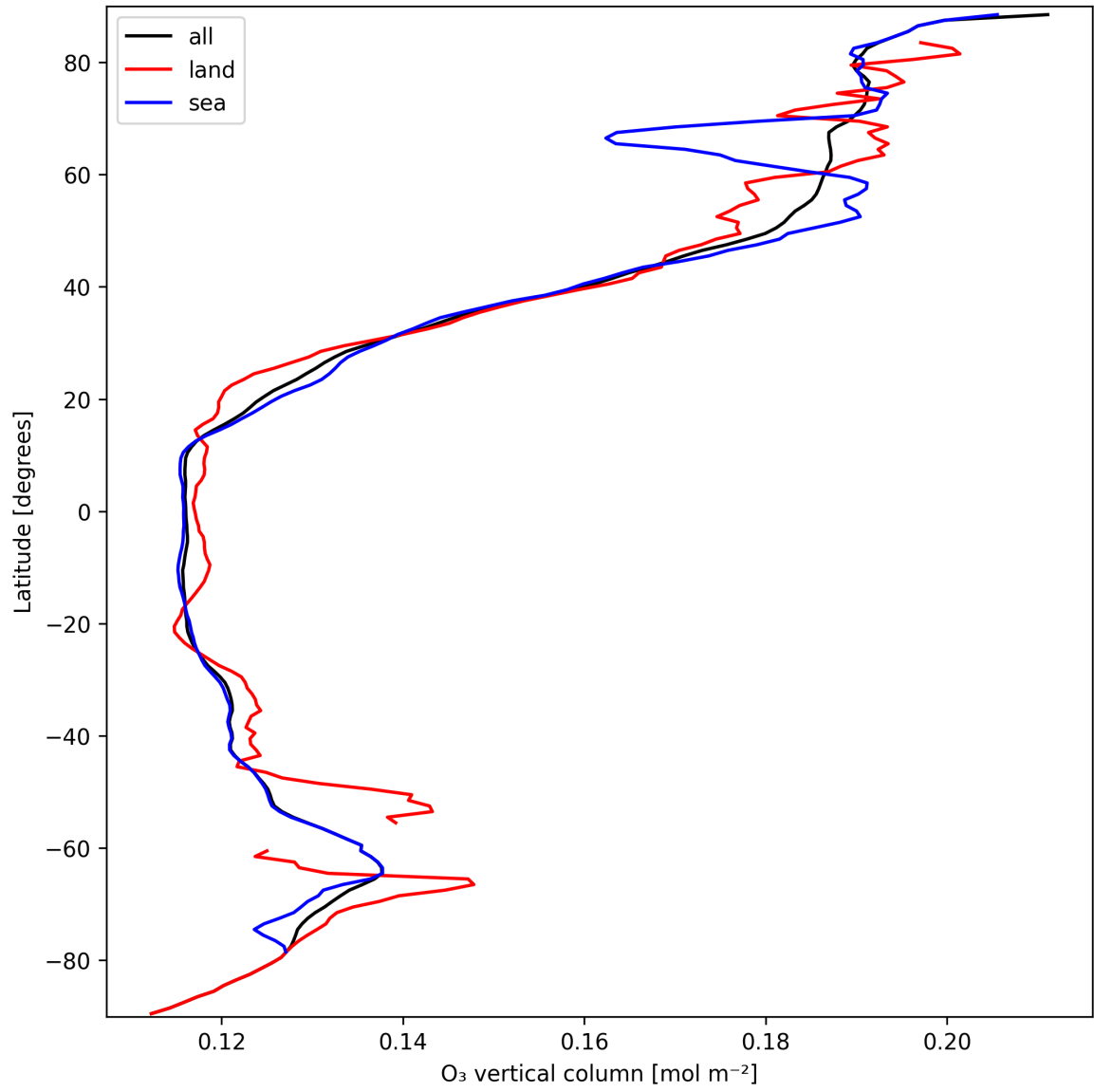
Figure 14: Zonal average of “O 3 vertical column” for 2025-03-17 to 2025-03-18.
