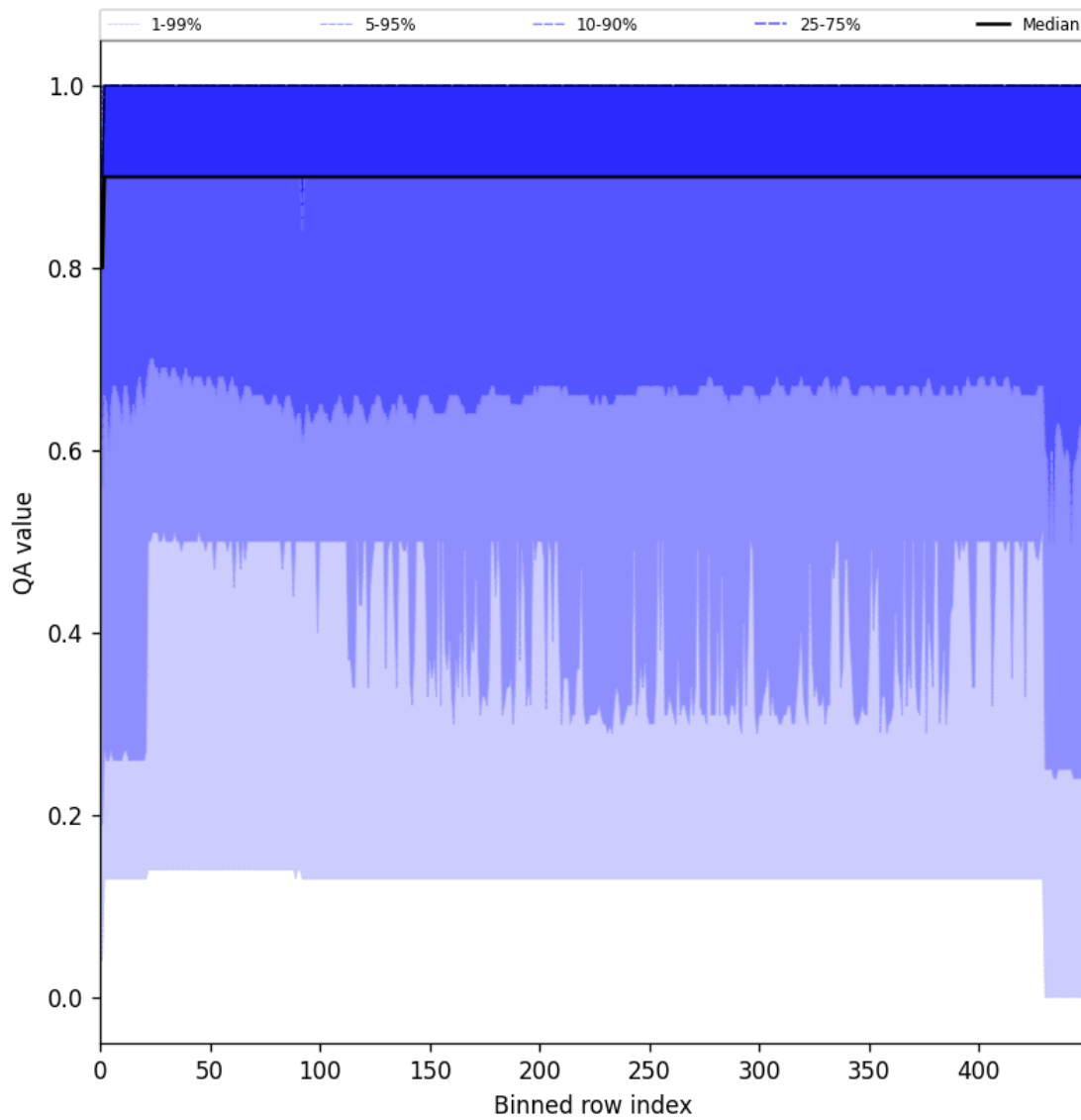
Figure 27: Along track statistics of “QA value” for 2025-03-17 to 2025-03-18
