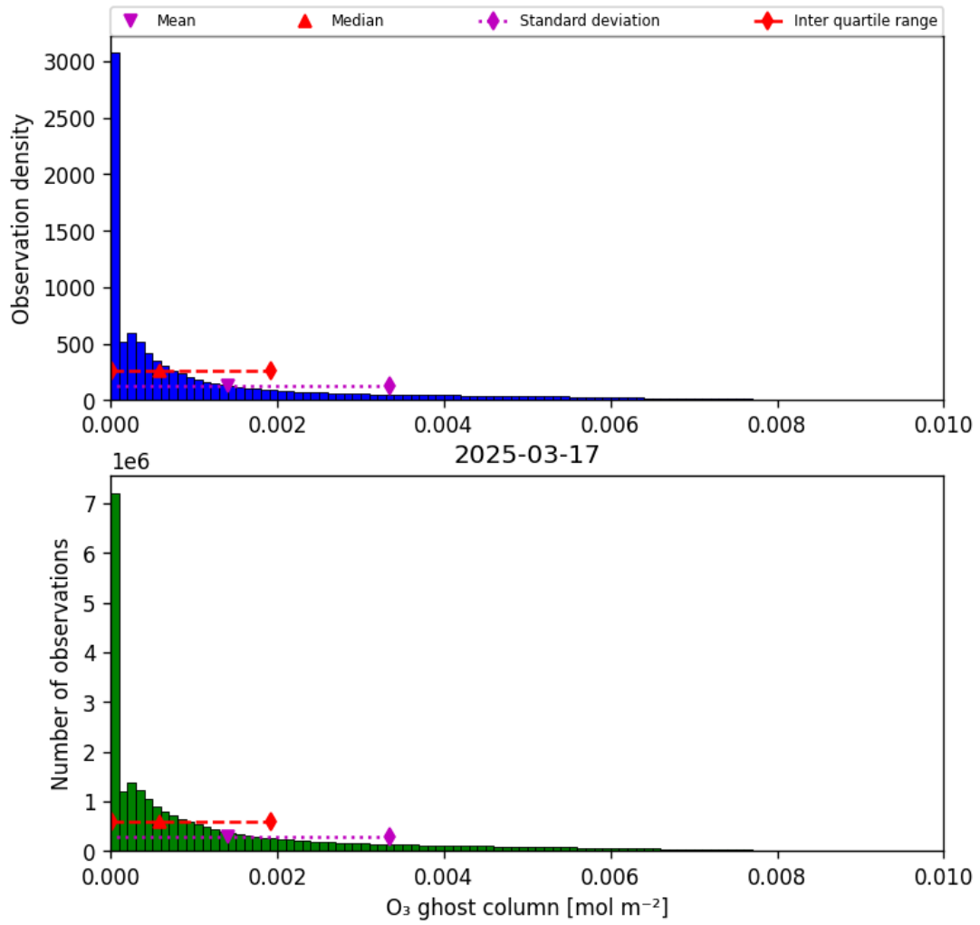
Figure 25: Histogram of “O 3 ghost column” for 2025-03-17 to 2025-03-18
