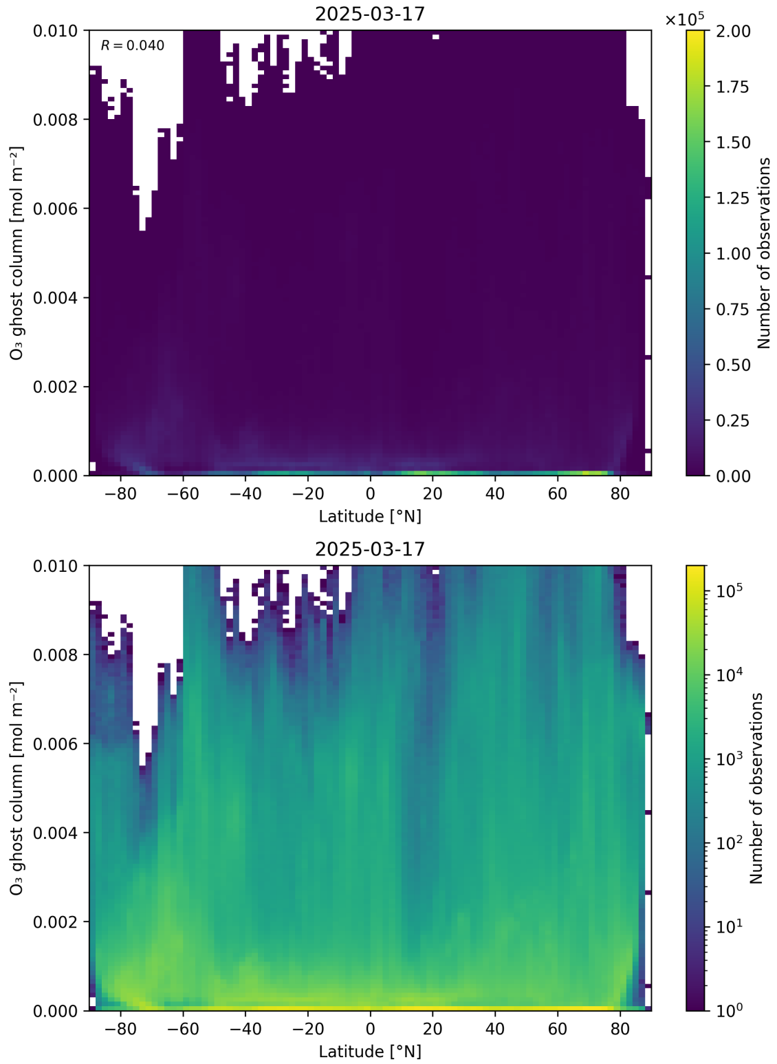
Figure 35: Scatter density plot of “Latitude” against “O 3 ghost column” for 2025-03-17 to 2025-03-18.
