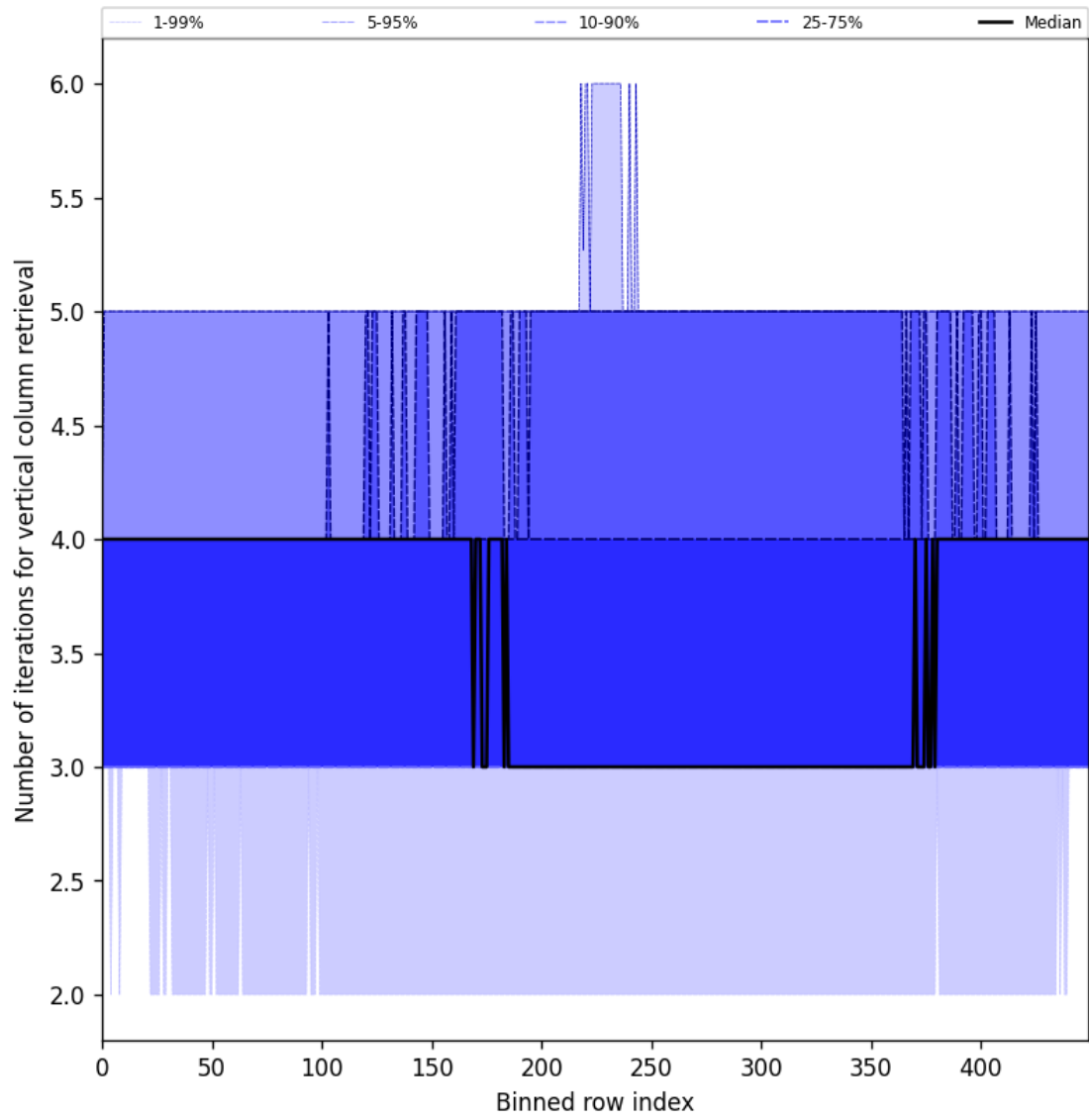
Figure 33: Along track statistics of “Number of iterations for vertical column retrieval” for 2025-03-17 to 2025-03-18
