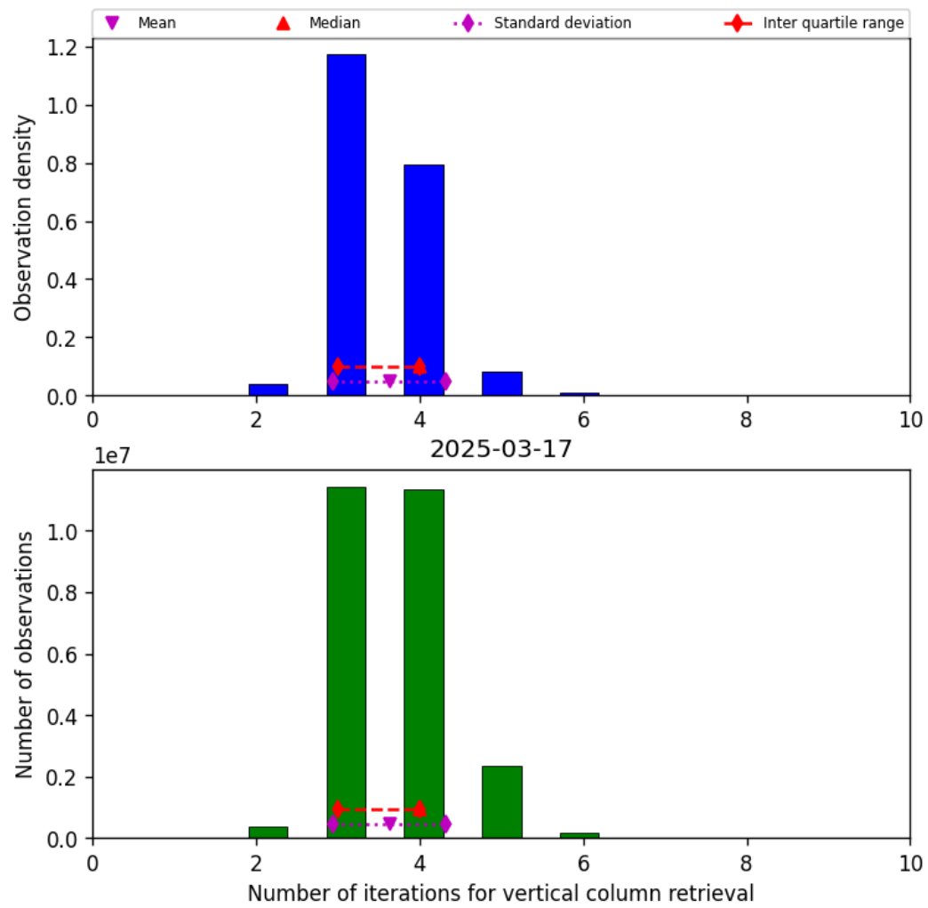
Figure 26: Histogram of “Number of iterations for vertical column retrieval” for 2025-03-17 to 2025-03-18
