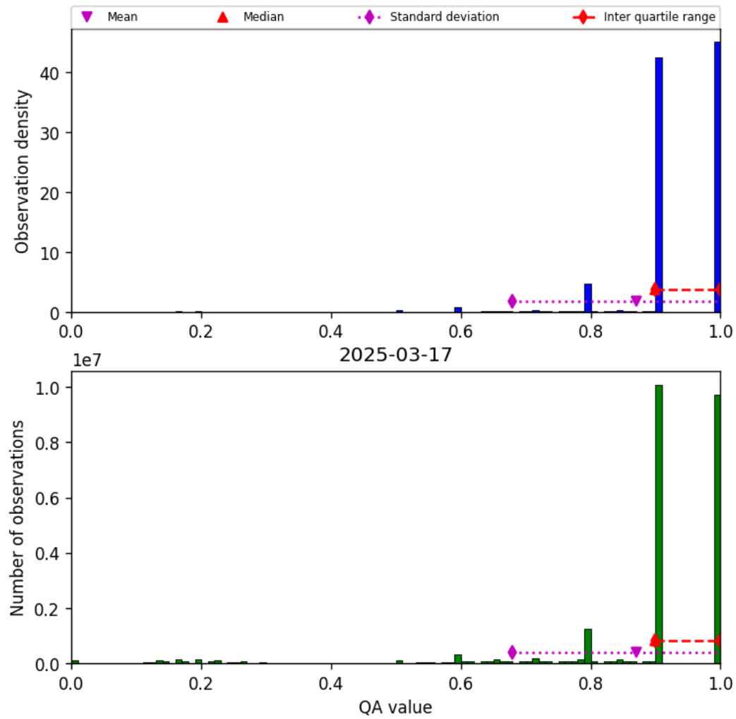
Figure 20: Histogram of “QA value” for 2025-03-17 to 2025-03-18
