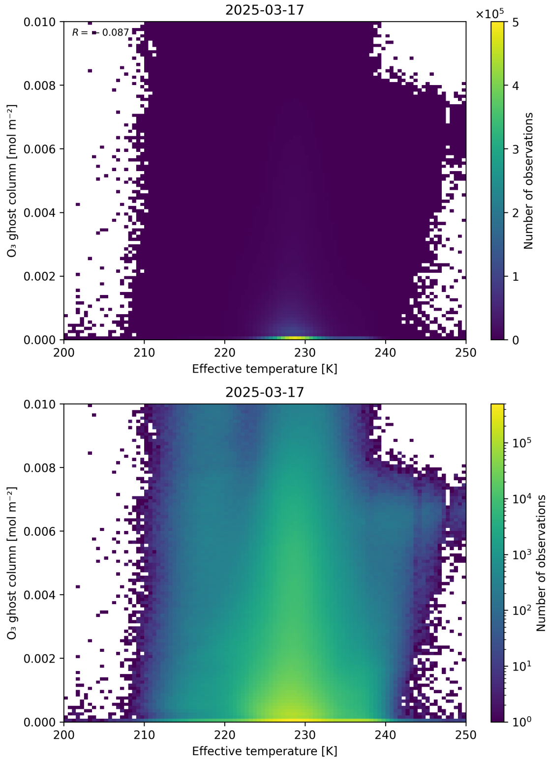
Figure 38: Scatter density plot of “Effective temperature” against “O 3 ghost column” for 2025-03-17 to 2025-03-18.
