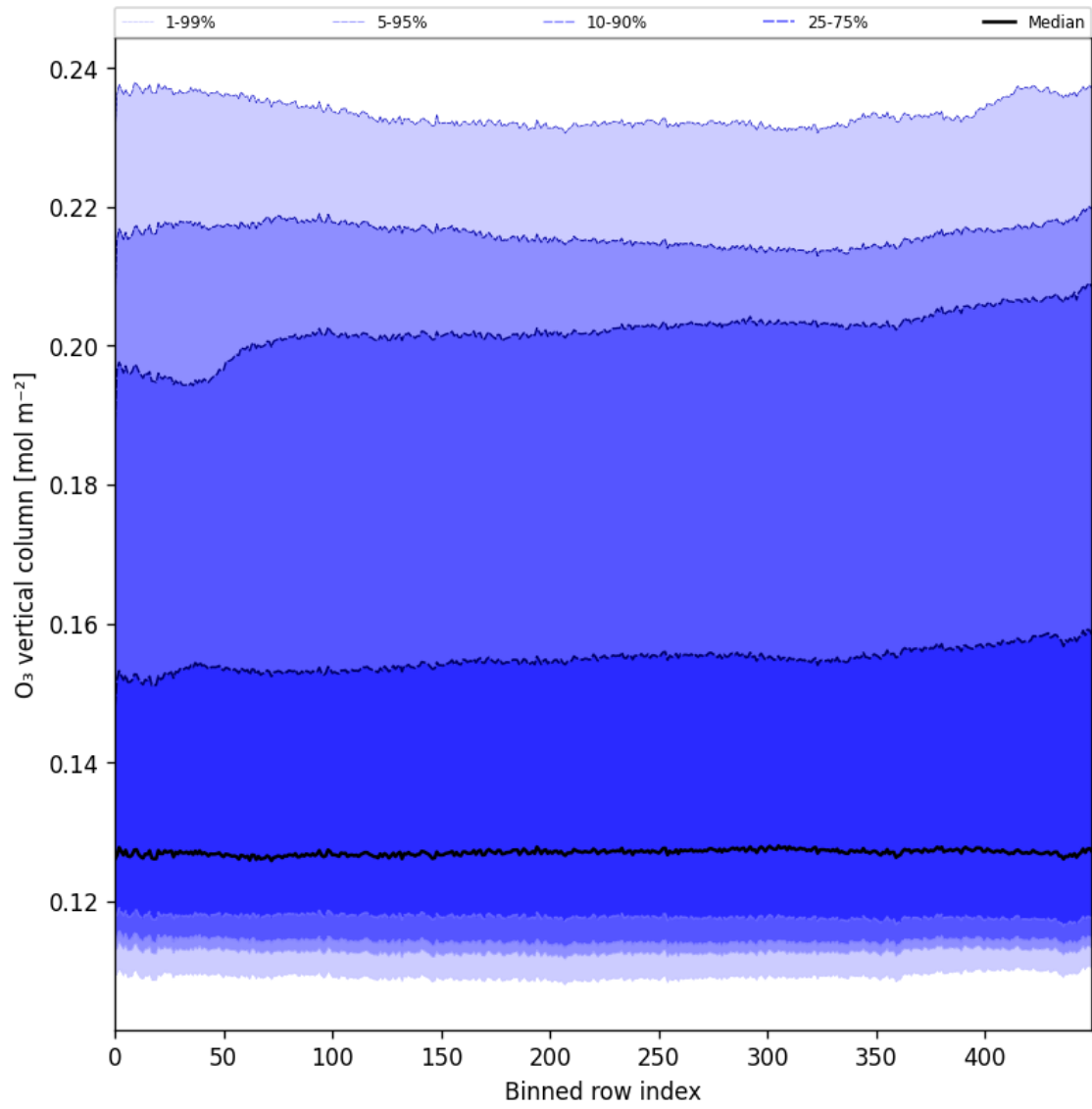
Figure 28: Along track statistics of “O 3 vertical column” for 2025-03-17 to 2025-03-18
