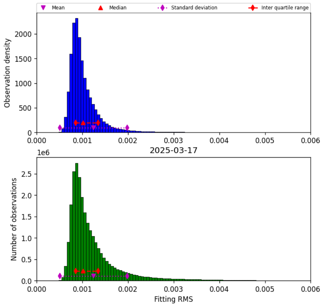
Figure 23: Histogram of “Fitting RMS” for 2025-03-17 to 2025-03-18
