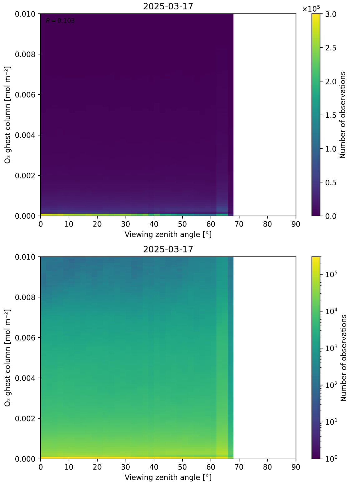
Figure 51: Scatter density plot of “Viewing zenith angle” against “O 3 ghost column” for 2025-03-17 to 2025-03-18.
