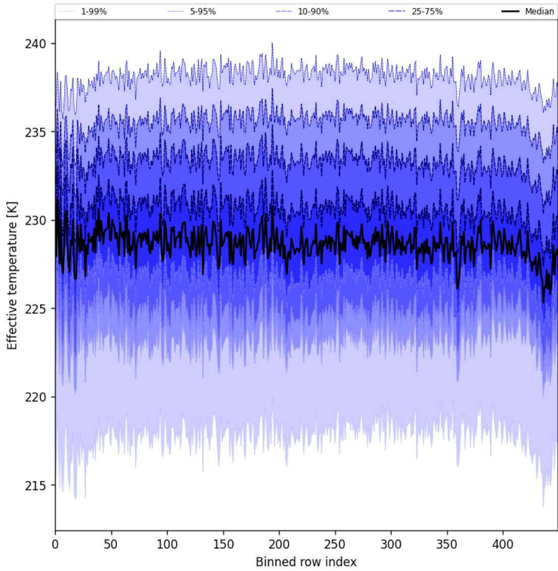
Figure 31: Along track statistics of “Effective temperature” for 2025-03-17 to 2025-03-18
