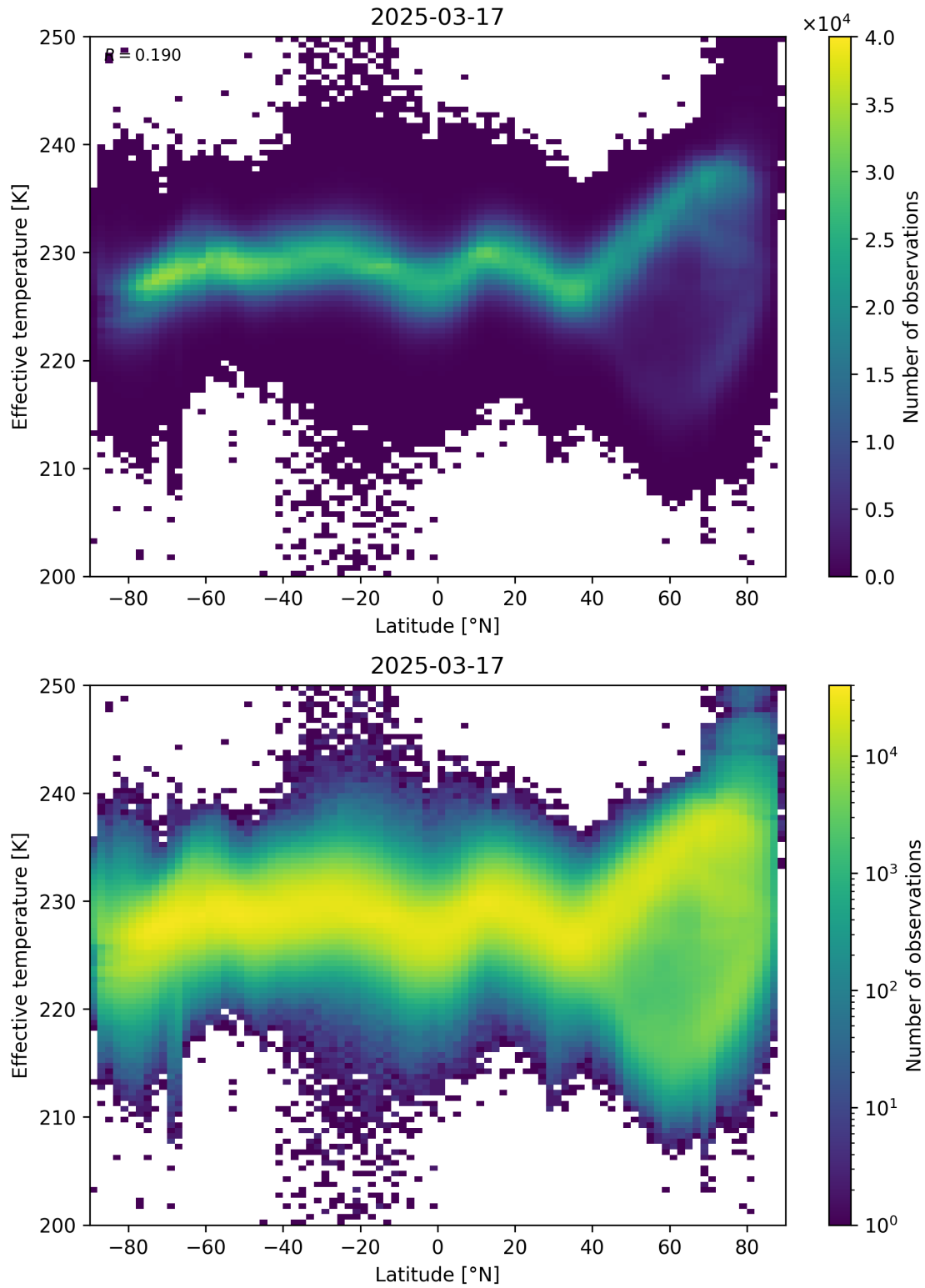
Figure 34: Scatter density plot of “Latitude” against “Effective temperature” for 2025-03-17 to 2025-03-18.
