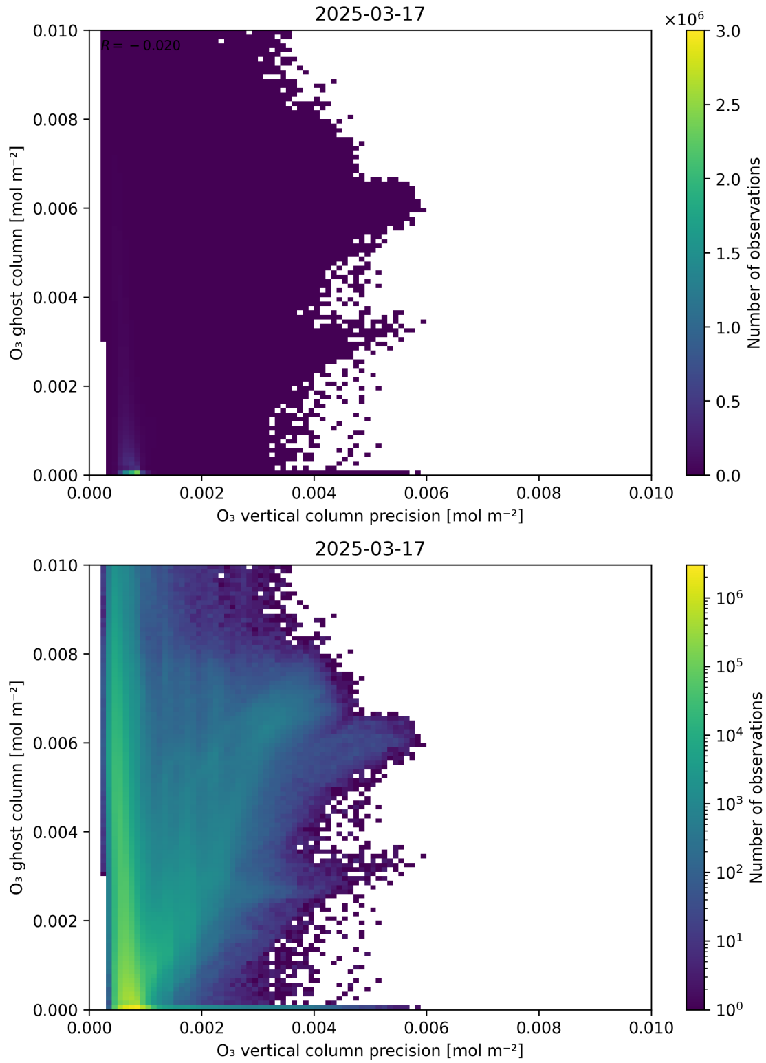
Figure 43: Scatter density plot of “ O_3 vertical column precision” against “ O_3 ghost column” for 2025-03-17 to 2025-03-18.
