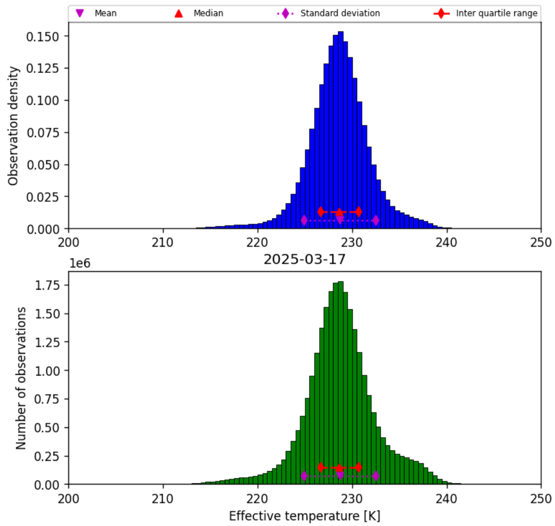
Figure 24: Histogram of “Effective temperature” for 2025-03-17 to 2025-03-18
