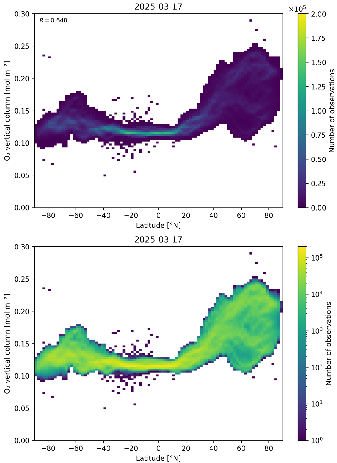
Figure 36: Scatter density plot of “Latitude” against “O 3 vertical column” for 2025-03-17 to 2025-03-18.
