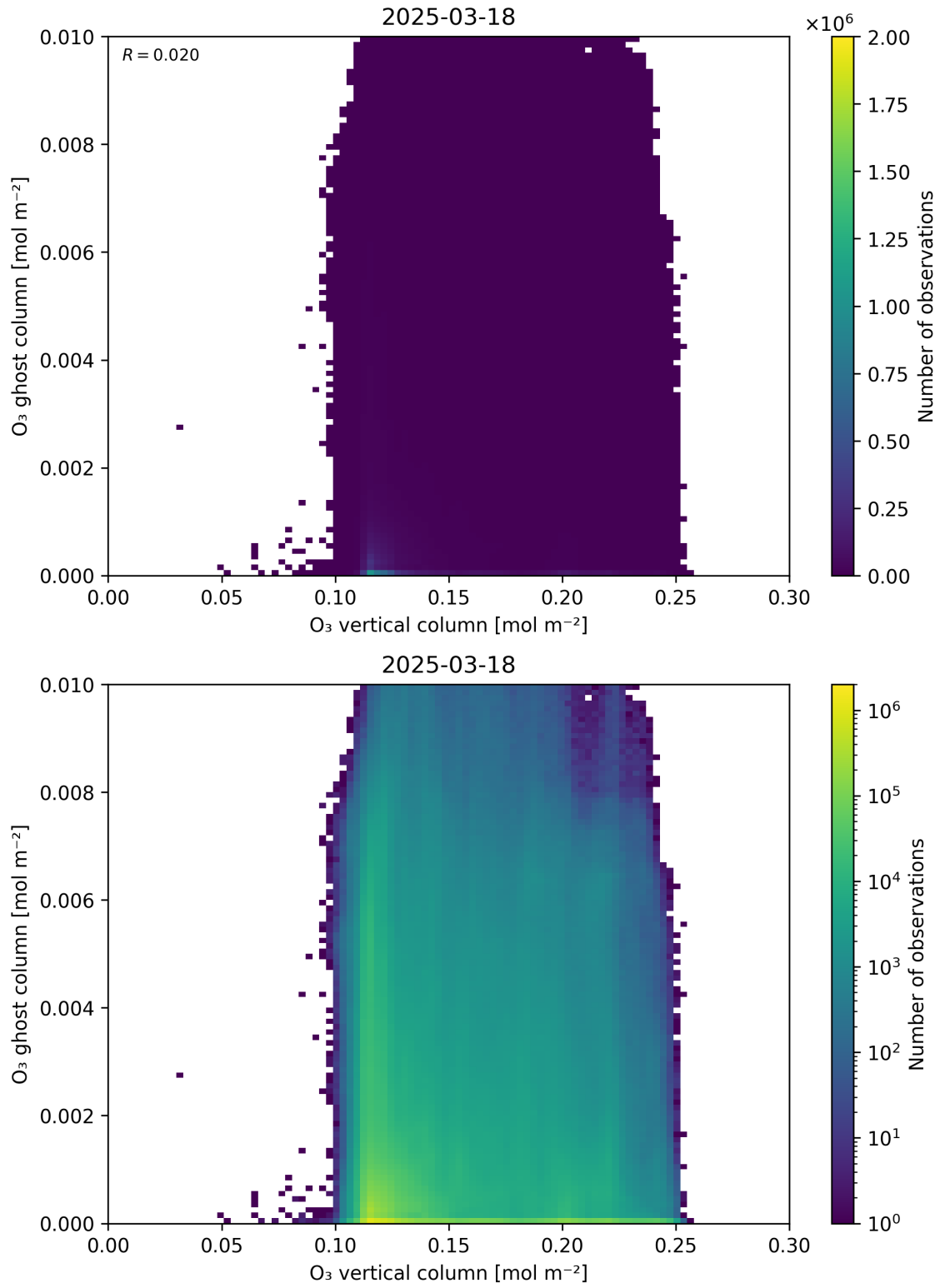
Figure 40: Scatter density plot of “O 3 vertical column” against “O 3 ghost column” for 2025-03-17 to 2025-03-19.
