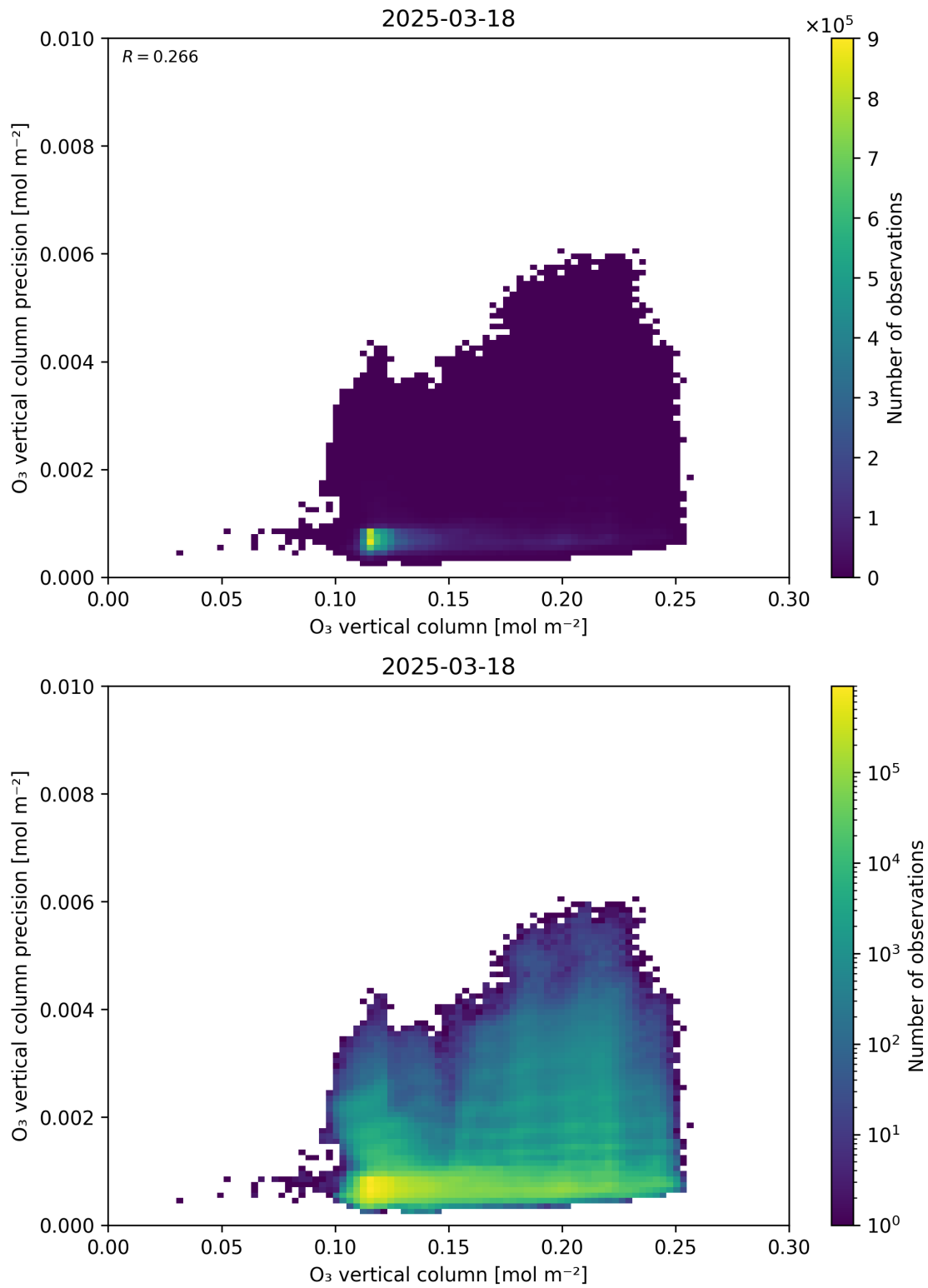
Figure 41: Scatter density plot of “O 3 vertical column” against “O 3 vertical column precision” for 2025-03-17 to 2025-03-19.
