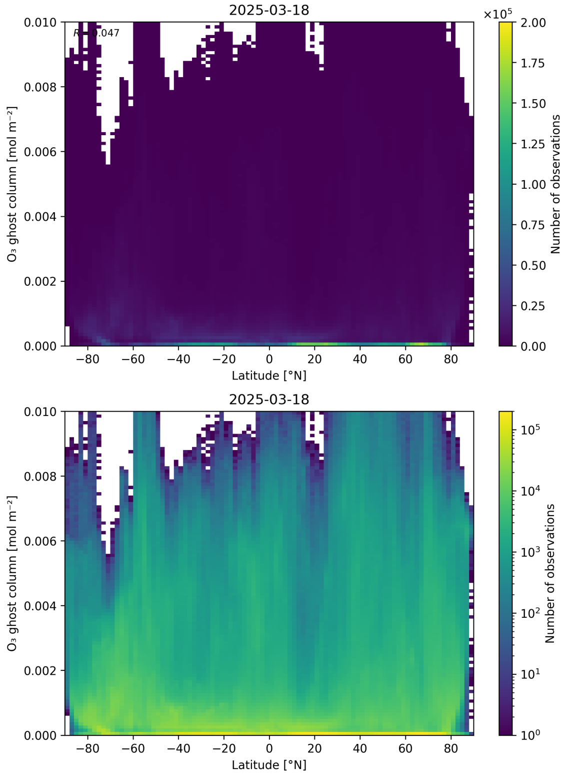
Figure 35: Scatter density plot of “Latitude” against “O 3 ghost column” for 2025-03-17 to 2025-03-19.
