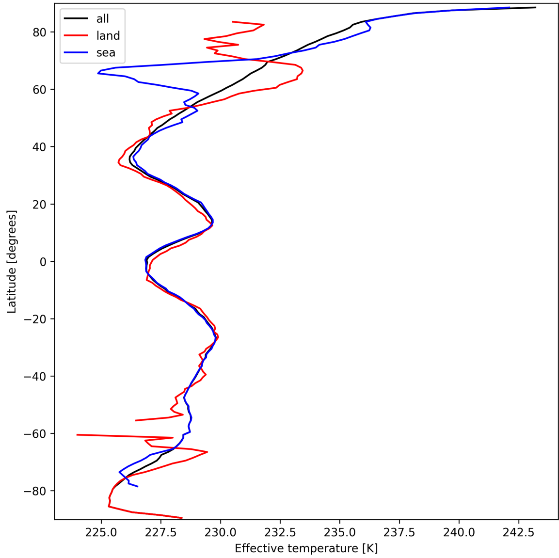
Figure 17: Zonal average of “Effective temperature” for 2025-03-17 to 2025-03-19.
