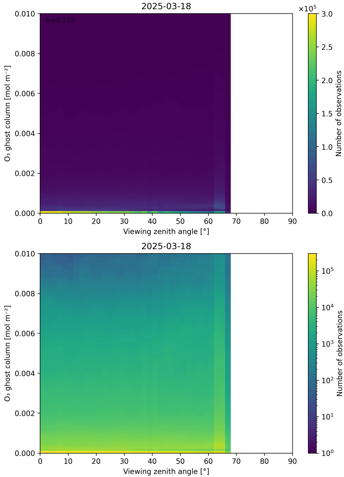
Figure 51: Scatter density plot of “Viewing zenith angle” against “O 3 ghost column” for 2025-03-17 to 2025-03-19.
