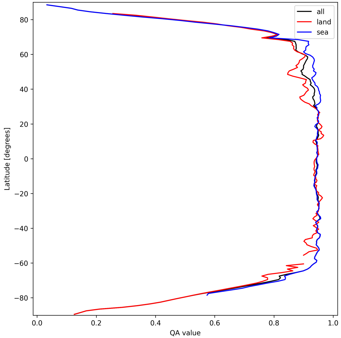
Figure 13: Zonal average of “QA value” for 2025-03-17 to 2025-03-19.
