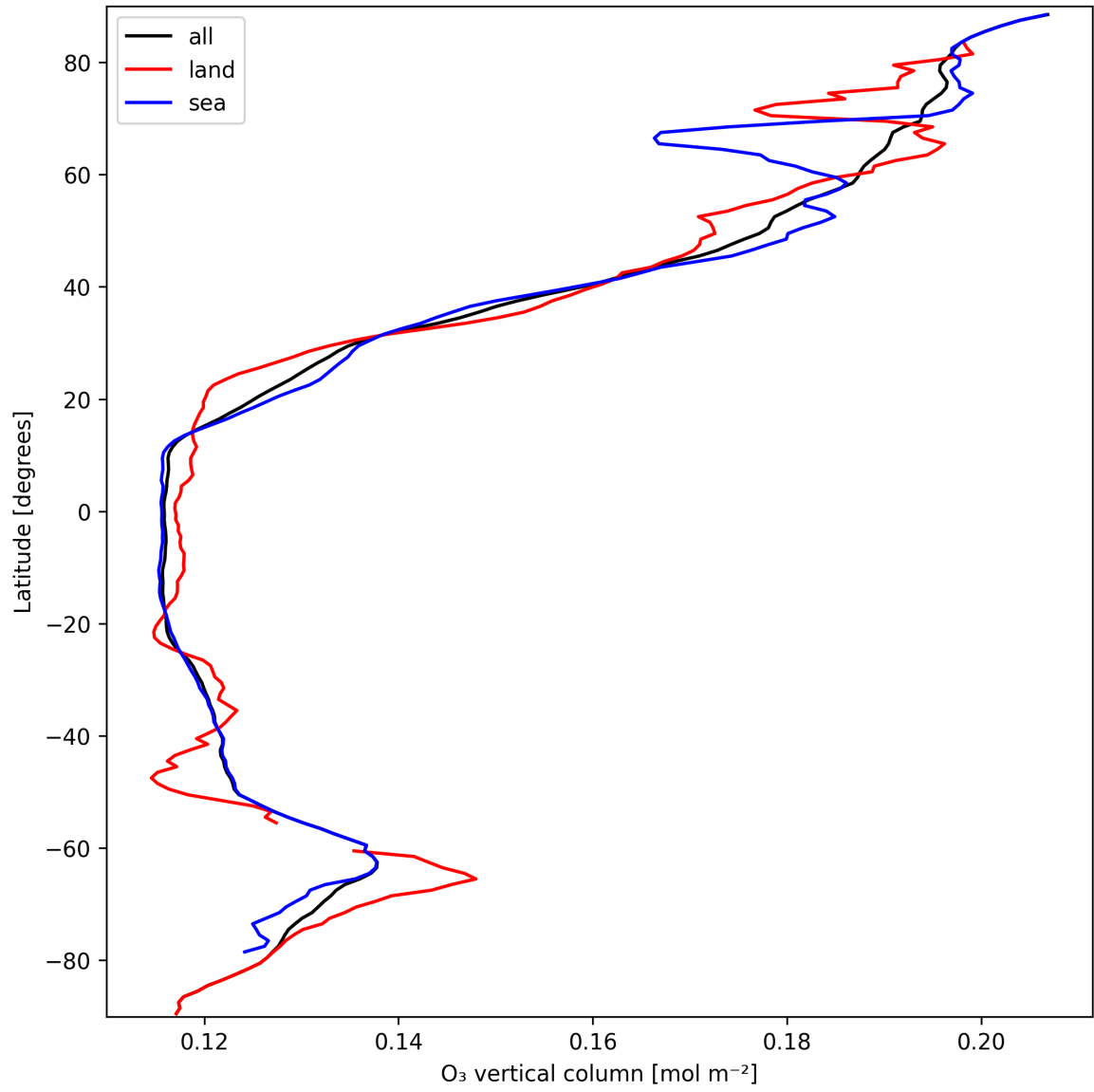
Figure 14: Zonal average of “O 3 vertical column” for 2025-03-17 to 2025-03-19.
