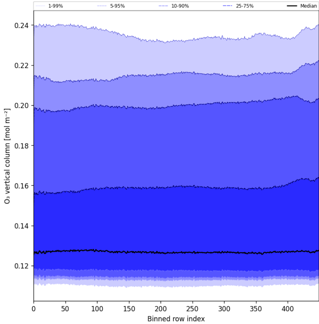
Figure 28: Along track statistics of “O 3 vertical column” for 2025-03-17 to 2025-03-19
