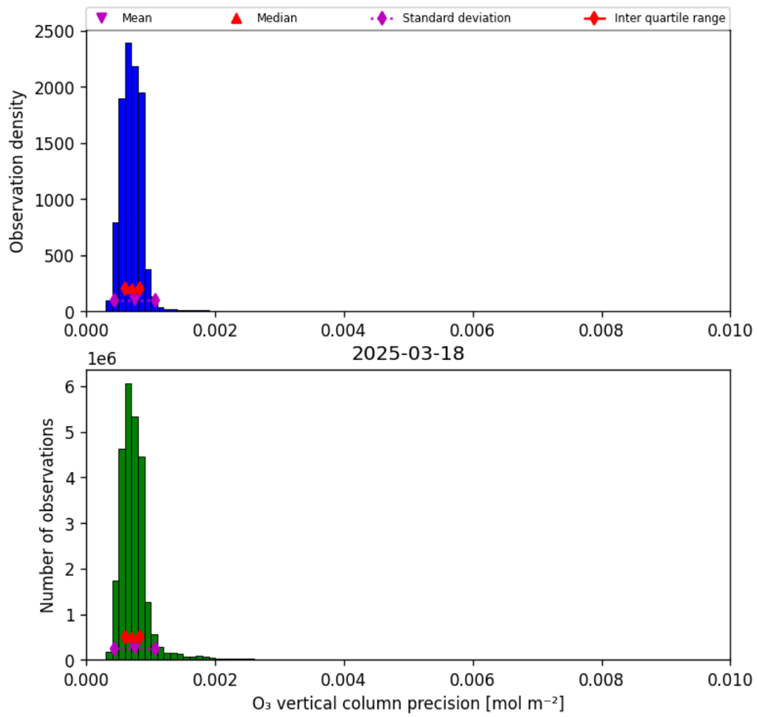
Figure 22: Histogram of “O 3 vertical column precision” for 2025-03-17 to 2025-03-19
