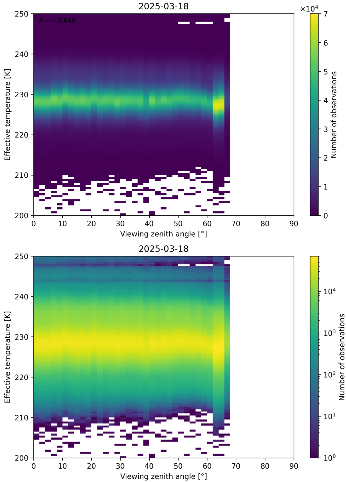
Figure 50: Scatter density plot of “Viewing zenith angle” against “Effective temperature” for 2025-03-17 to 2025-03-19.
