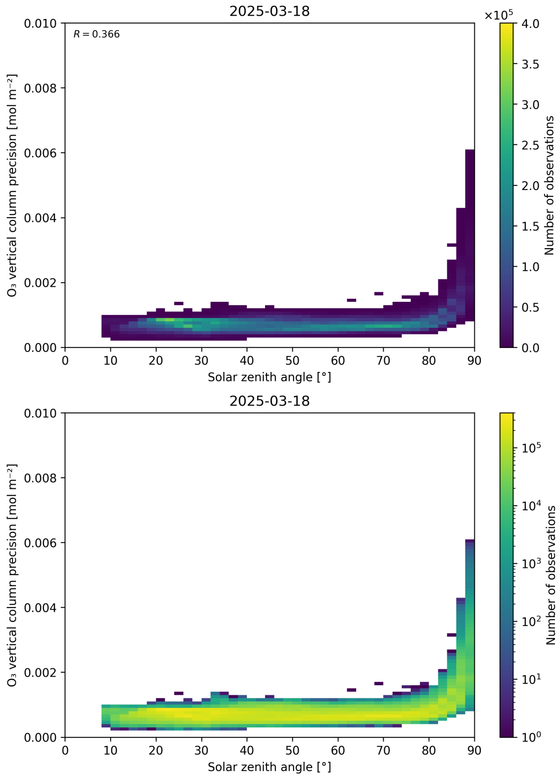
Figure 48: Scatter density plot of “Solar zenith angle” against “O 3 vertical column precision” for 2025-03-17 to 2025-03-19.
