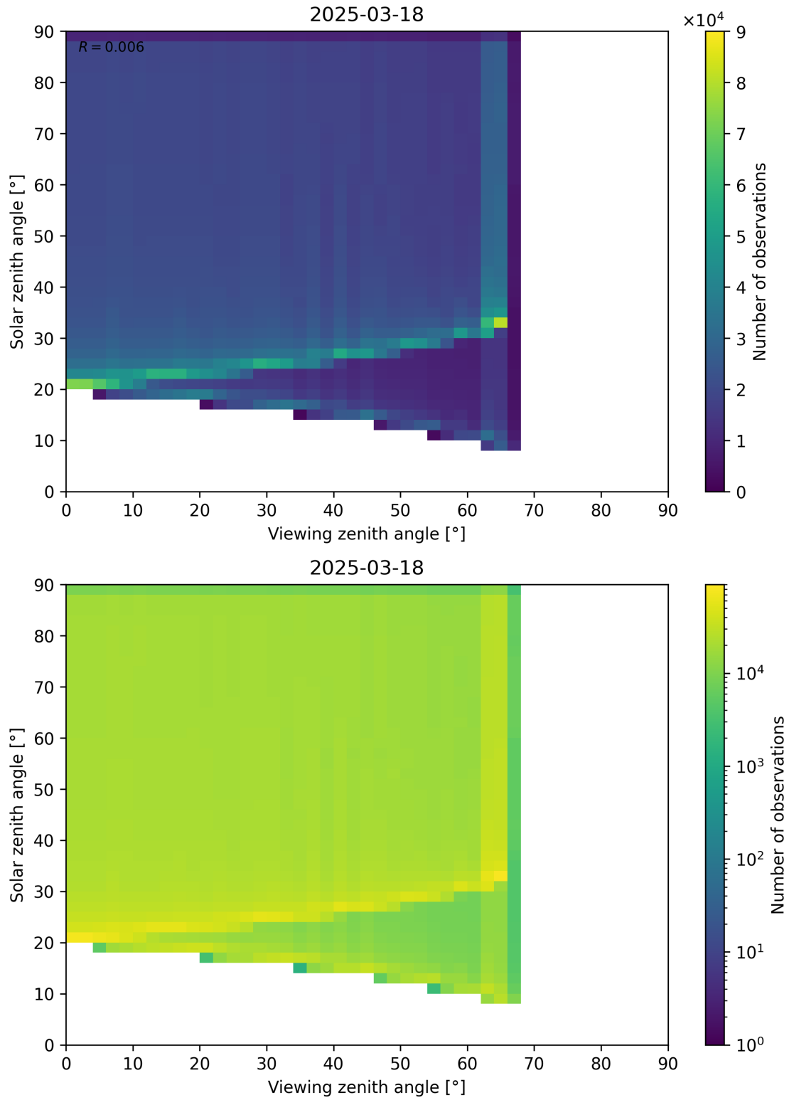
Figure 54: Scatter density plot of “Viewing zenith angle” against “Solar zenith angle” for 2025-03-17 to 2025-03-19.
