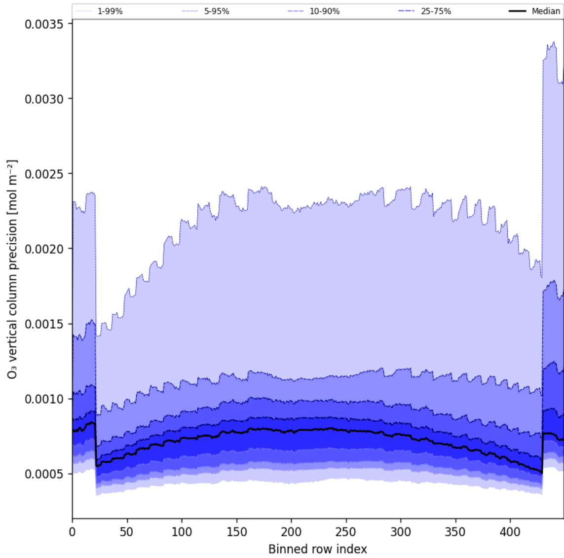
Figure 29: Along track statistics of “O 3 vertical column precision” for 2025-03-17 to 2025-03-19
