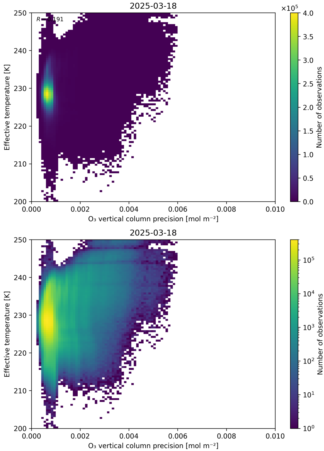
Figure 42: Scatter density plot of “O 3 vertical column precision” against “Effective temperature” for 2025-03-17 to 2025-03-19.
