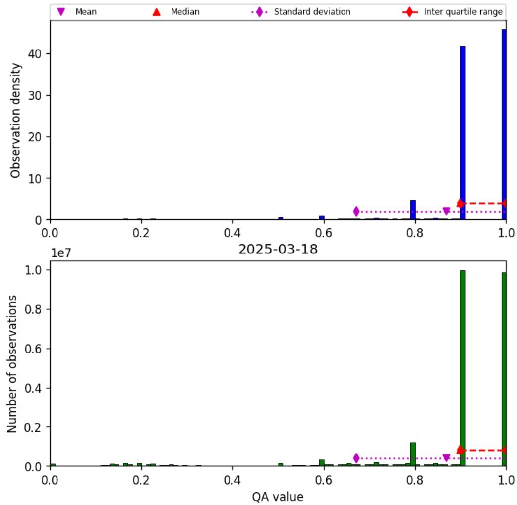
Figure 20: Histogram of “QA value” for 2025-03-17 to 2025-03-19
