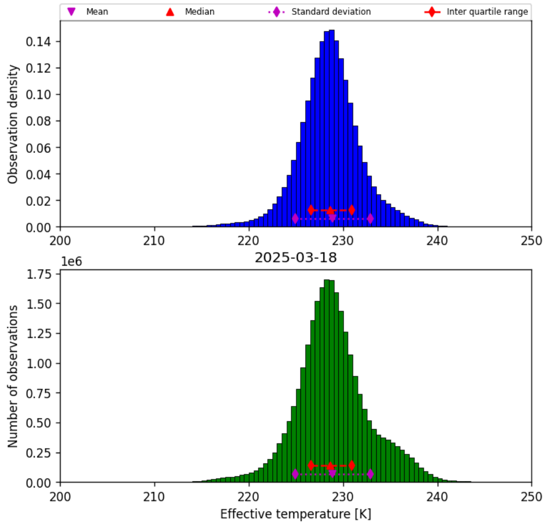
Figure 24: Histogram of “Effective temperature” for 2025-03-17 to 2025-03-19
