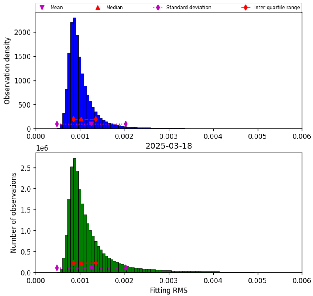
Figure 23: Histogram of “Fitting RMS” for 2025-03-17 to 2025-03-19
