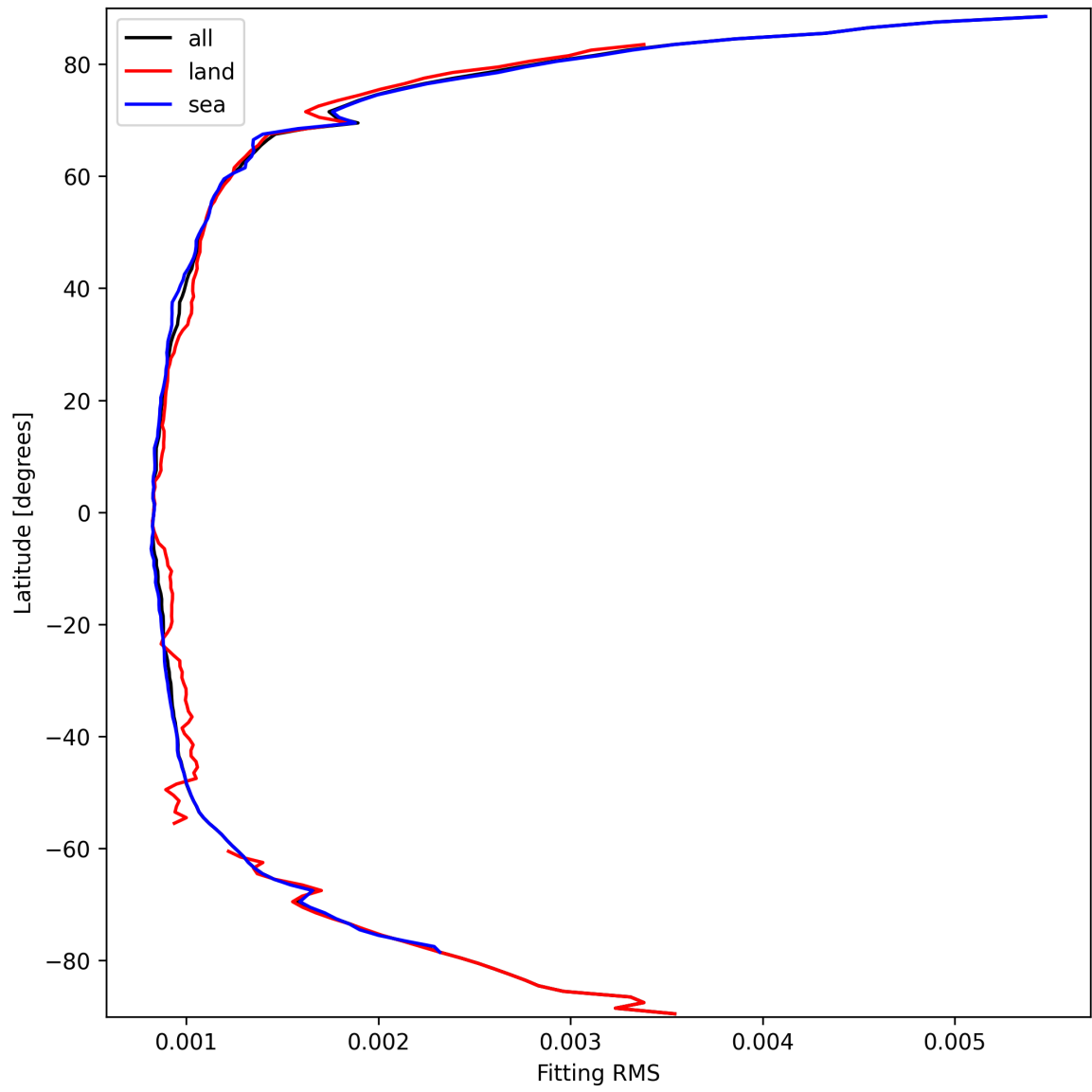
Figure 16: Zonal average of “Fitting RMS” for 2025-03-17 to 2025-03-19.
