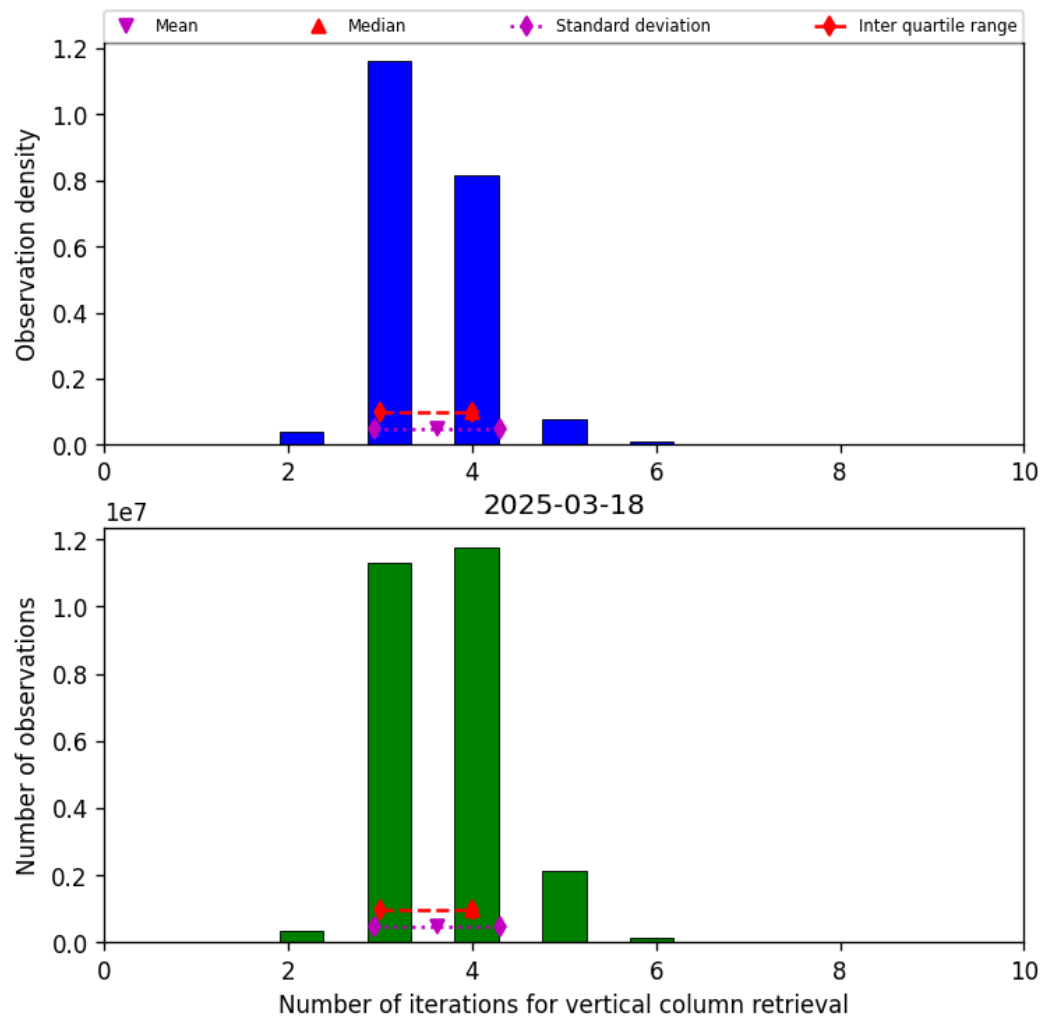
Figure 26: Histogram of “Number of iterations for vertical column retrieval” for 2025-03-17 to 2025-03-19
