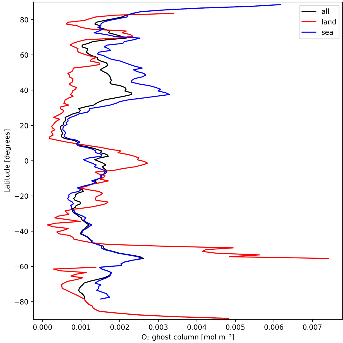
Figure 18: Zonal average of “O 3 ghost column” for 2025-03-17 to 2025-03-19.
