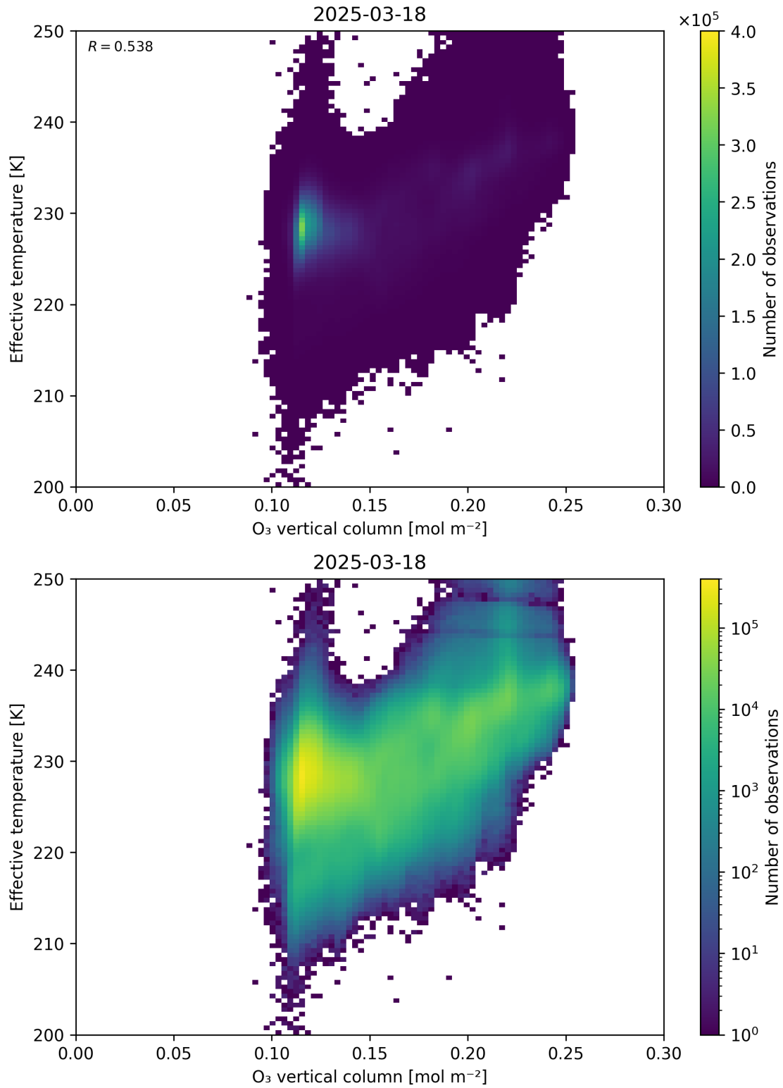
Figure 39: Scatter density plot of “O 3 vertical column” against “Effective temperature” for 2025-03-17 to 2025-03-19.
