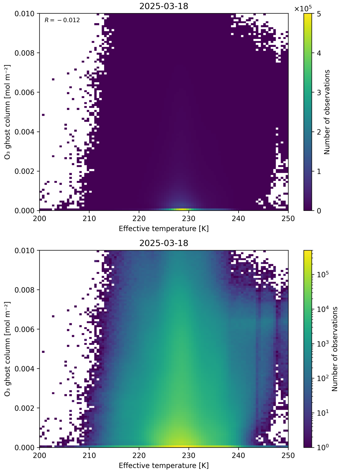
Figure 38: Scatter density plot of “Effective temperature” against “O 3 ghost column” for 2025-03-17 to 2025-03-19.
