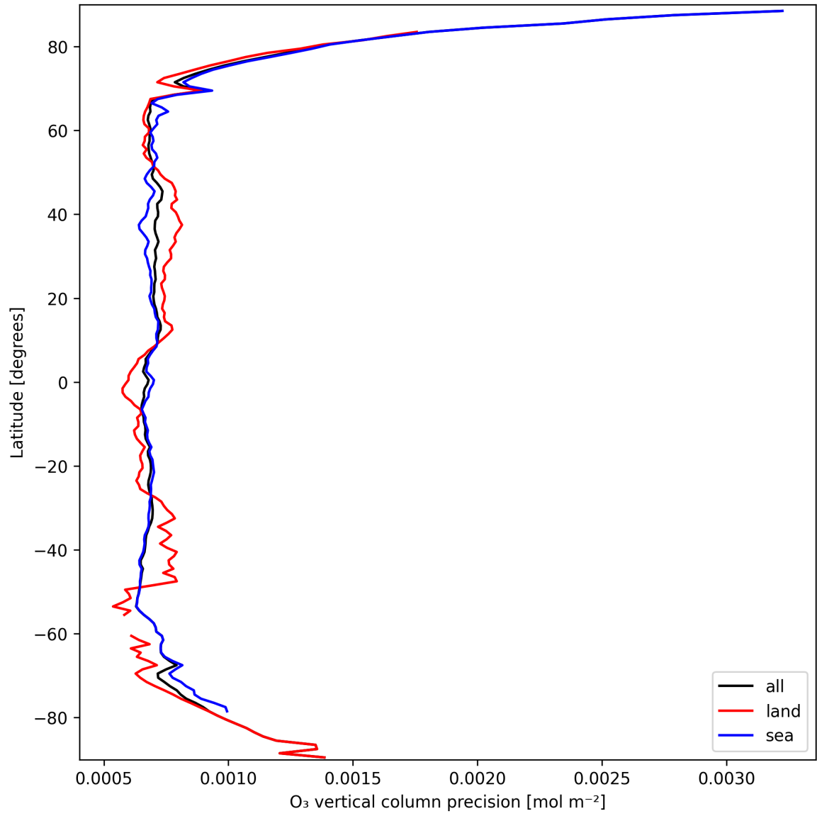
Figure 15: Zonal average of “O 3 vertical column precision” for 2025-03-17 to 2025-03-19.
