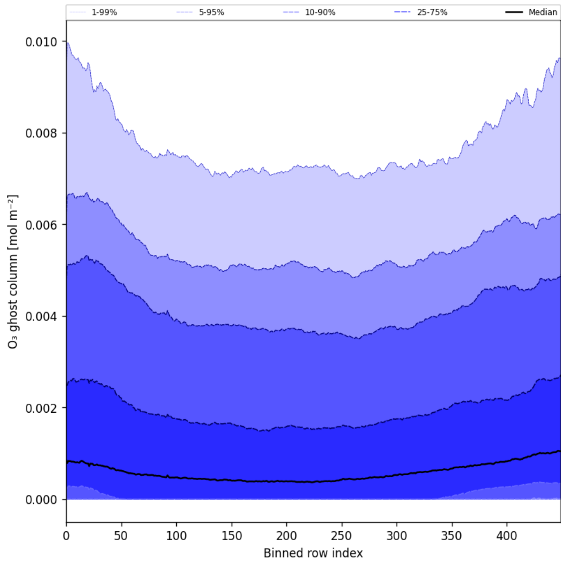
Figure 32: Along track statistics of “O 3 ghost column” for 2025-03-17 to 2025-03-19
