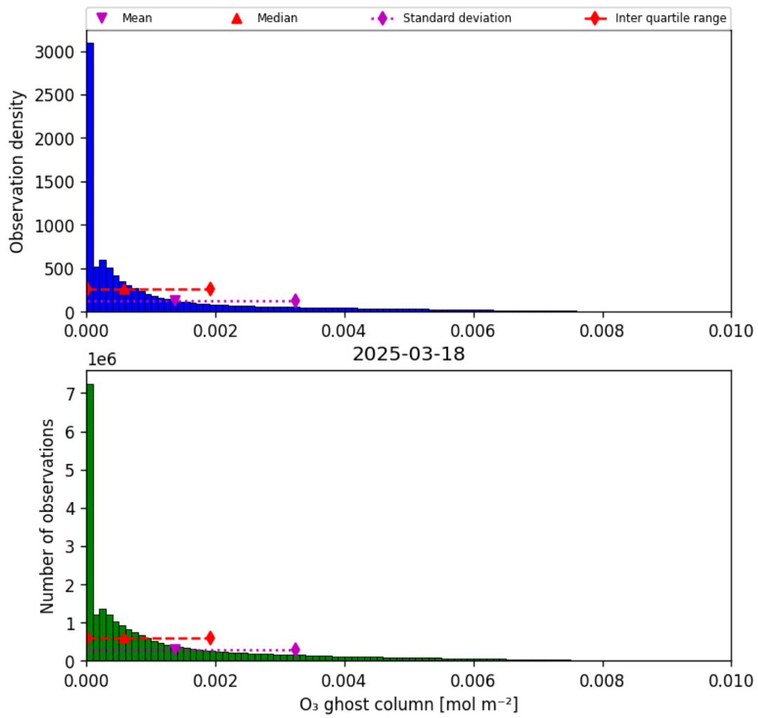
Figure 25: Histogram of "O 3 ghost column" for 2025-03-17 to 2025-03-19
