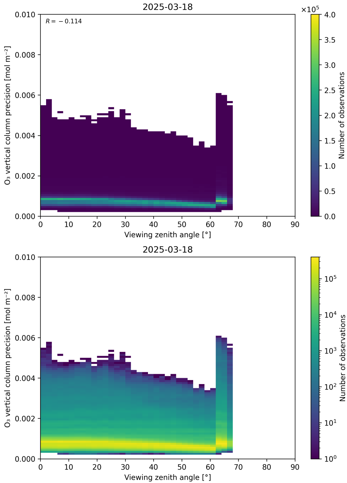
Figure 53: Scatter density plot of “Viewing zenith angle” against “O 3 vertical column precision” for 2025-03-17 to 2025-03-19.
