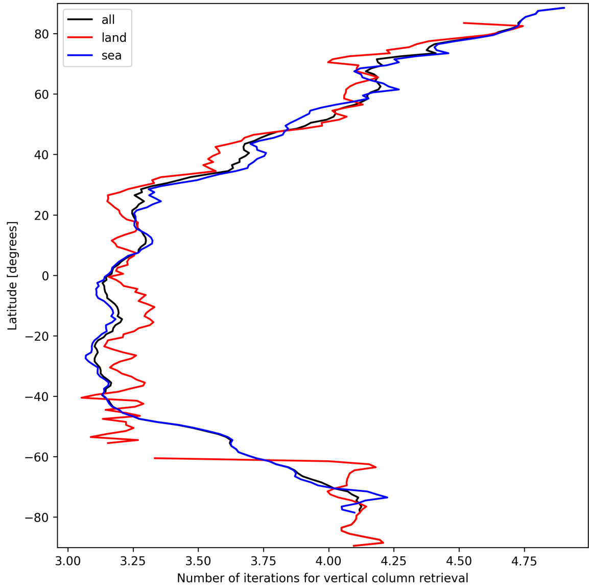
Figure 19: Zonal average of “Number of iterations for vertical column retrieval” for 2025-03-17 to 2025-03-19.
