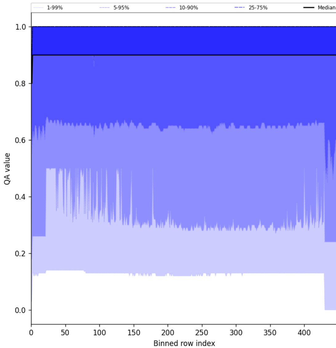
Figure 27: Along track statistics of “QA value” for 2025-03-17 to 2025-03-19
