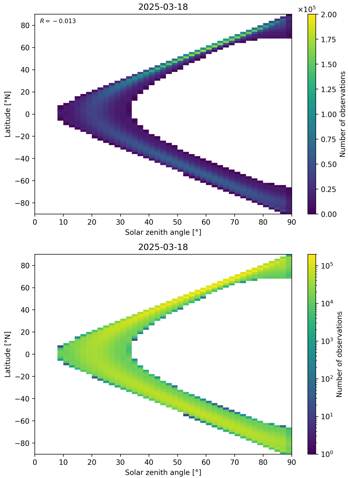
Figure 44: Scatter density plot of “Solar zenith angle” against “Latitude” for 2025-03-17 to 2025-03-19.
