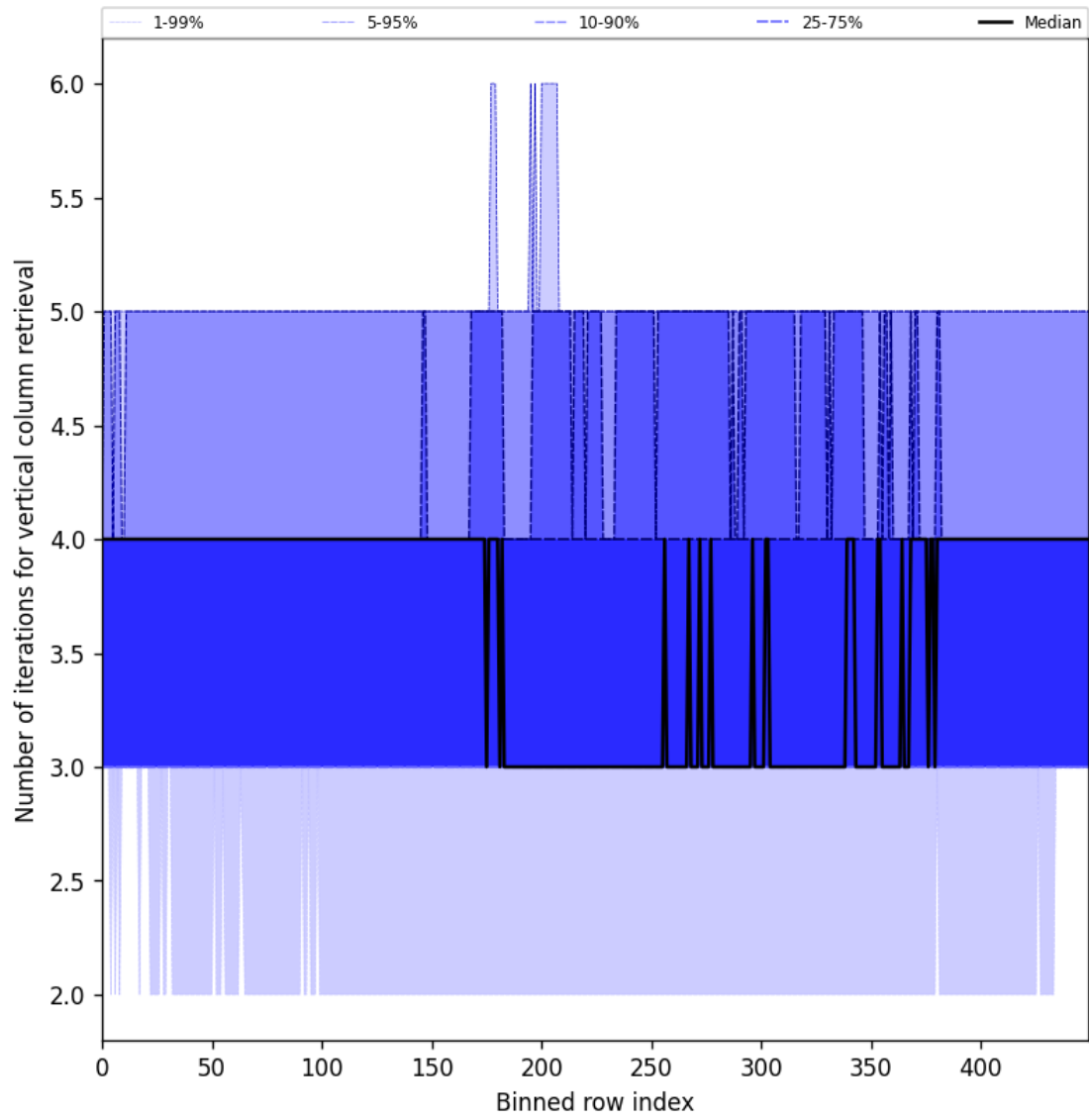
Figure 33: Along track statistics of “Number of iterations for vertical column retrieval” for 2025-03-17 to 2025-03-19
