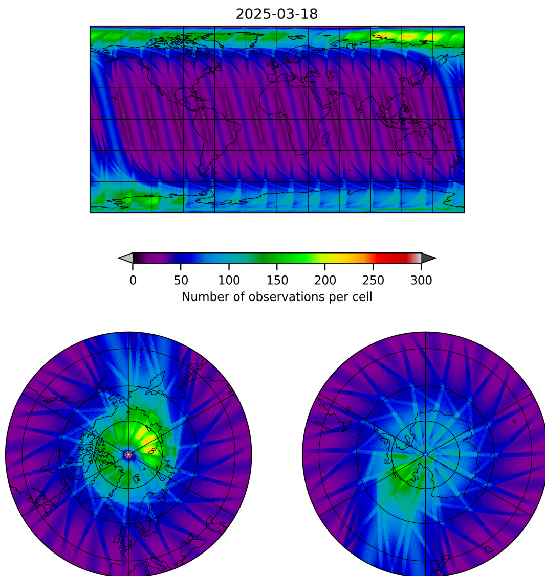
Figure 12: Map of the number of observations for 2025-03-17 to 2025-03-19
