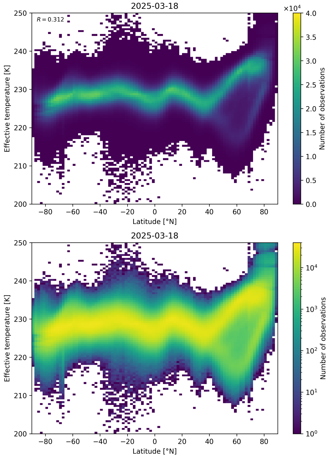
Figure 34: Scatter density plot of “Latitude” against “Effective temperature” for 2025-03-17 to 2025-03-19.
