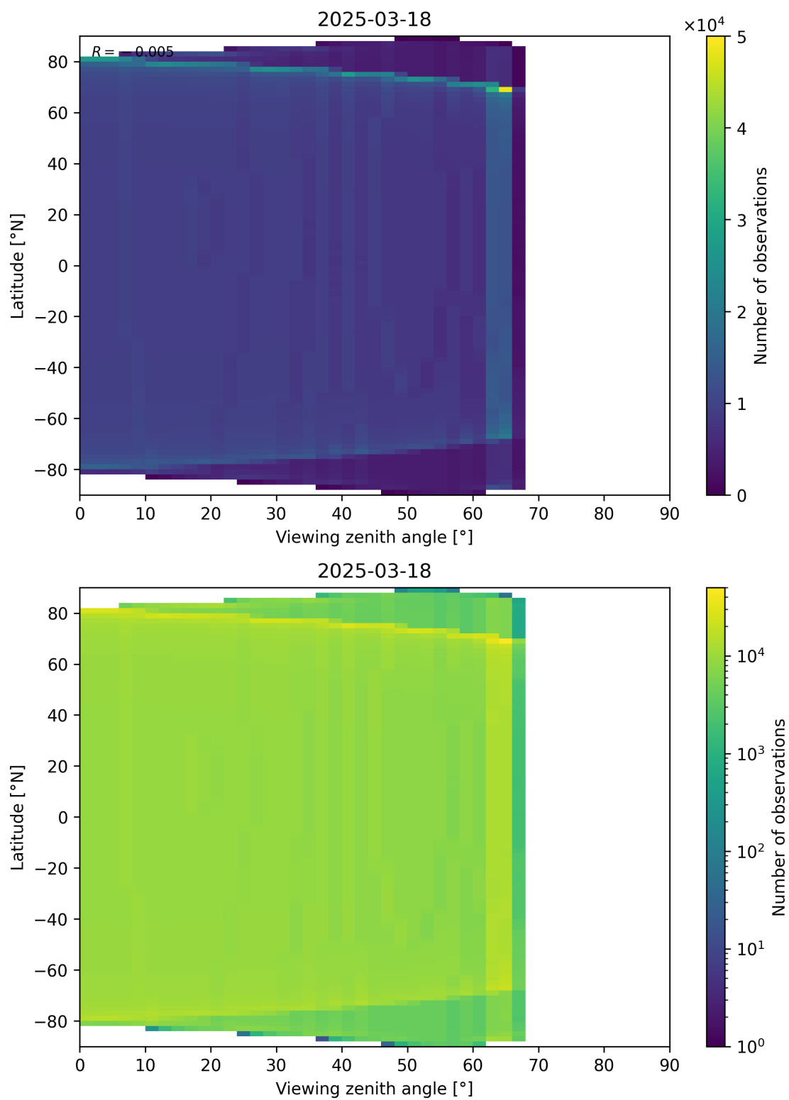
Figure 49: Scatter density plot of “Viewing zenith angle” against “Latitude” for 2025-03-17 to 2025-03-19.
