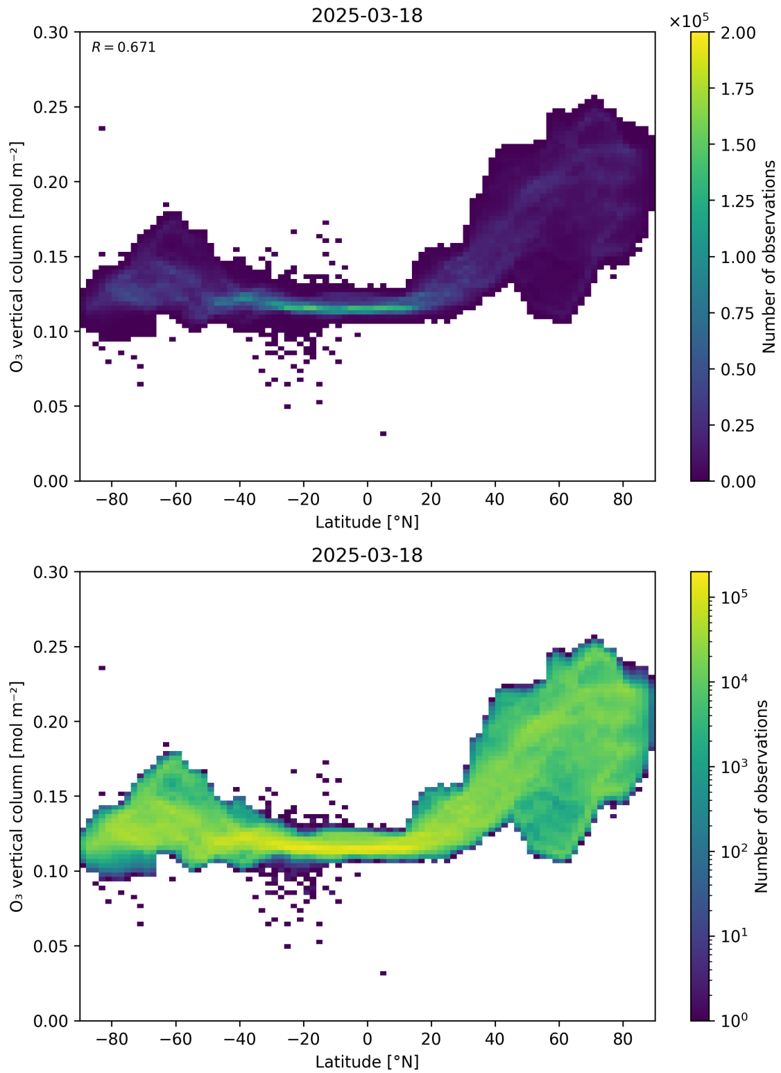
Figure 36: Scatter density plot of “Latitude” against “O 3 vertical column” for 2025-03-17 to 2025-03-19.
