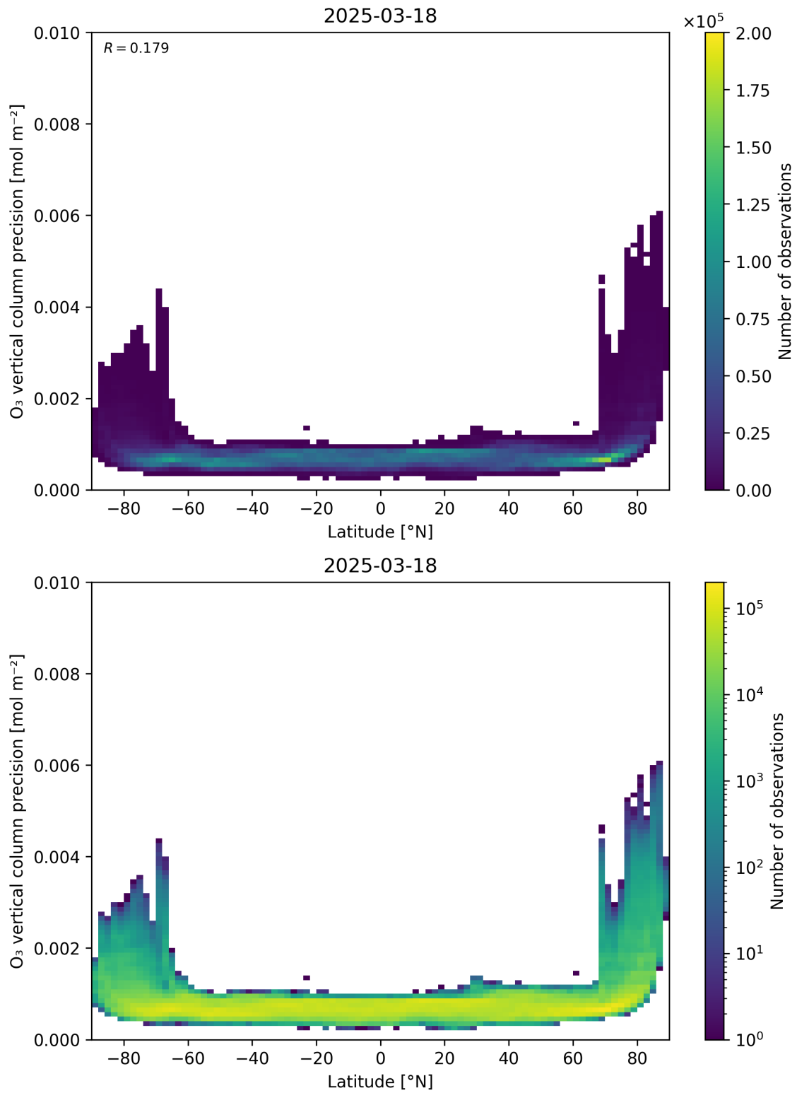
Figure 37: Scatter density plot of “Latitude” against “O 3 vertical column precision” for 2025-03-17 to 2025-03-19.
