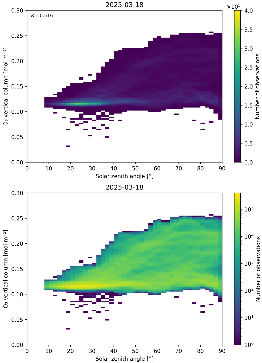
Figure 47: Scatter density plot of “Solar zenith angle” against “O 3 vertical column” for 2025-03-17 to 2025-03-19.
