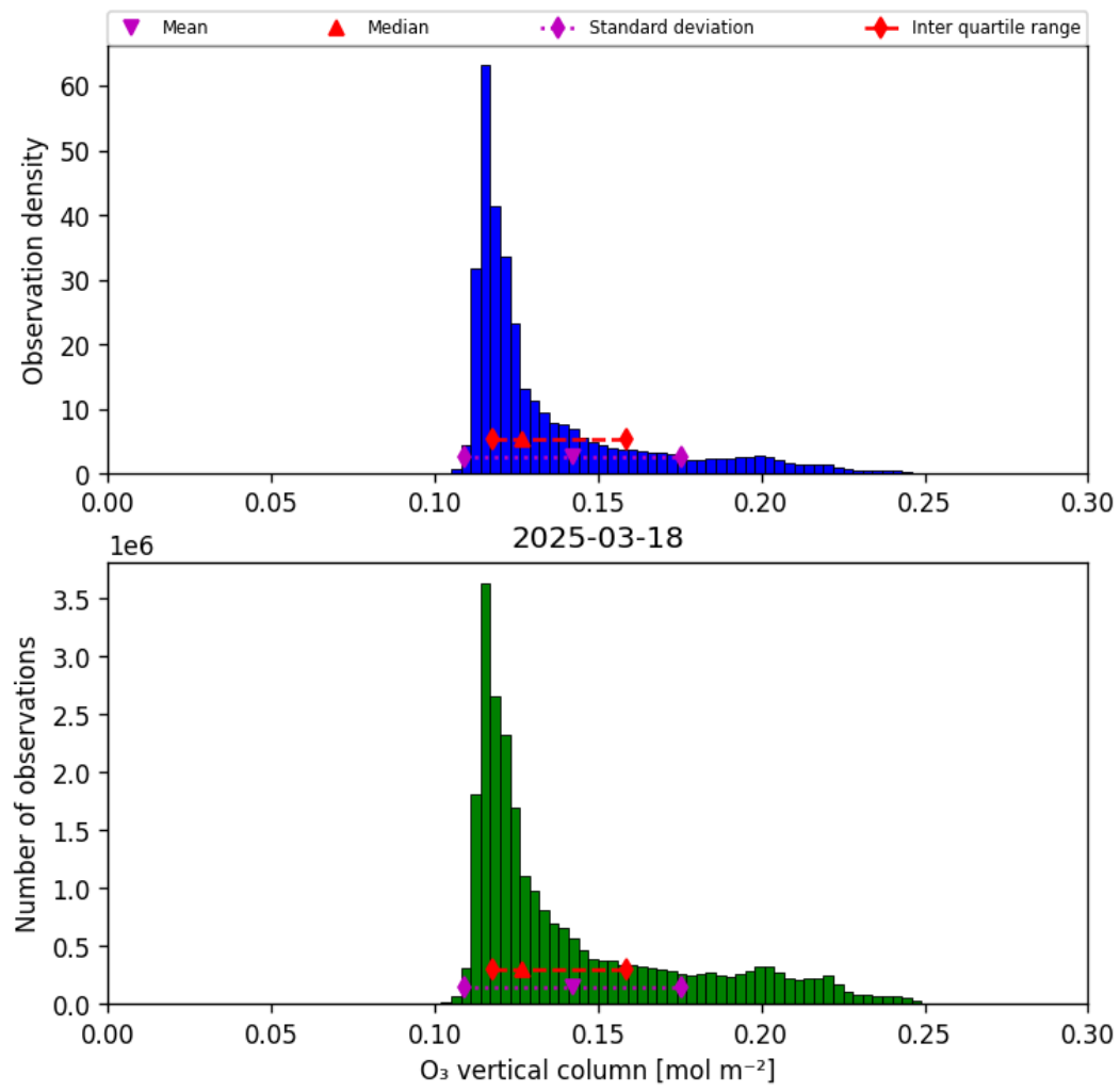
Figure 21: Histogram of “O 3 vertical column” for 2025-03-17 to 2025-03-19
