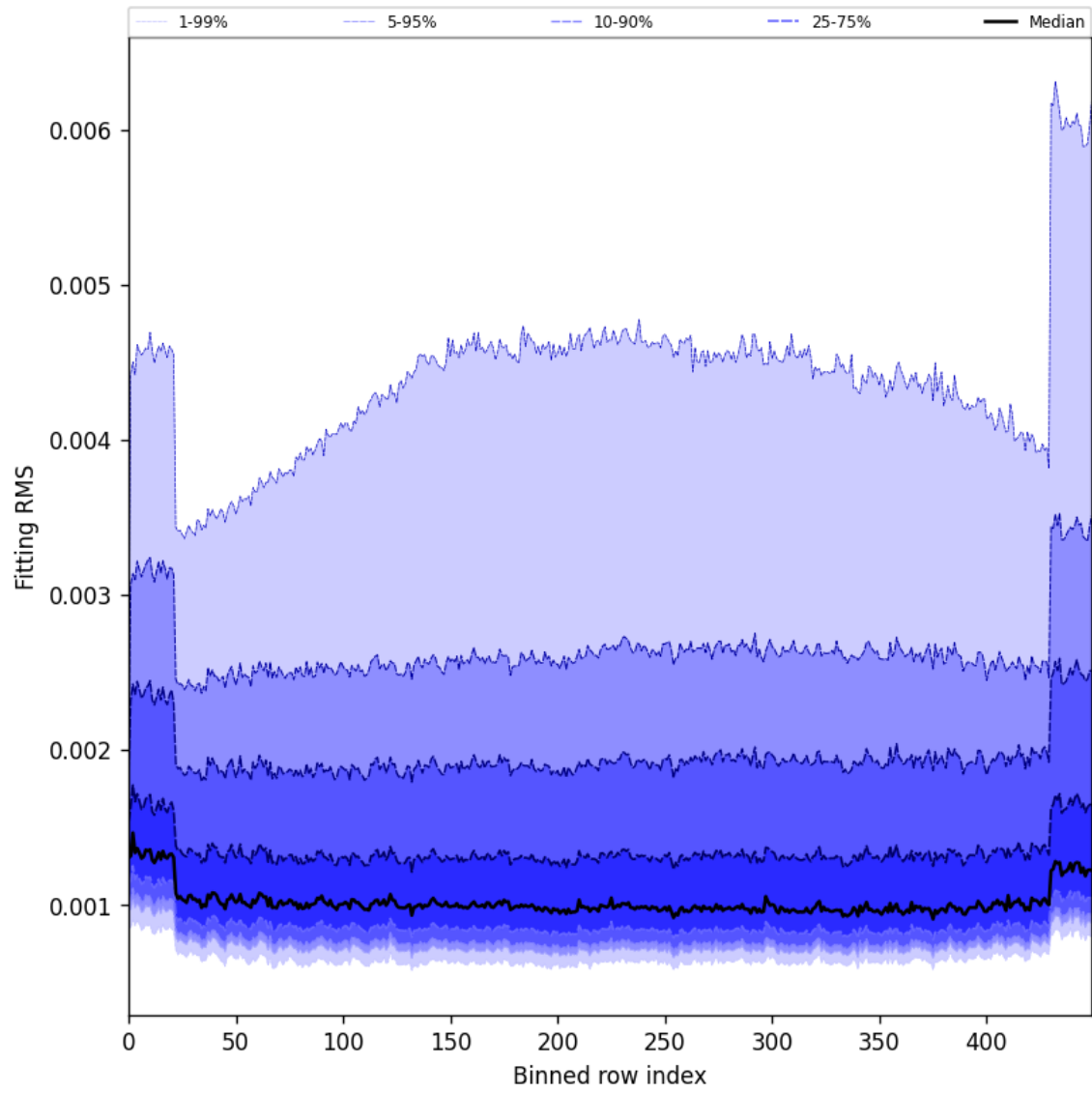
Figure 30: Along track statistics of “Fitting RMS” for 2025-03-17 to 2025-03-19
