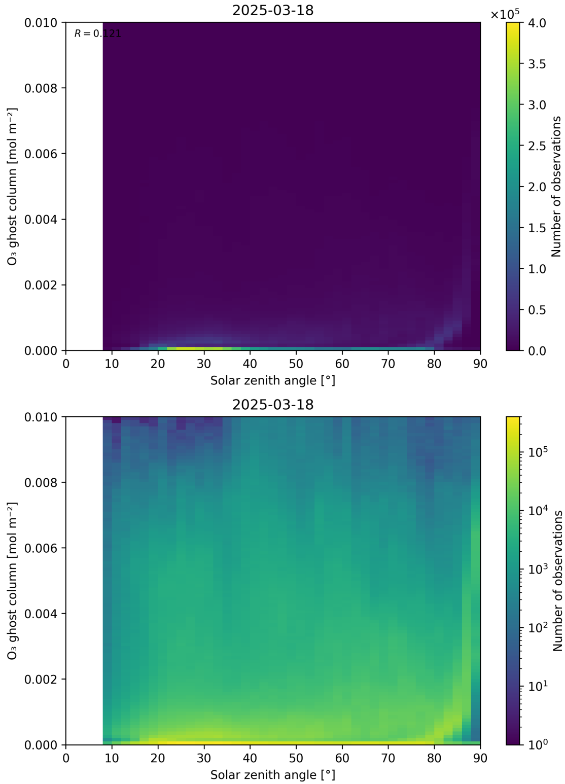
Figure 46: Scatter density plot of “Solar zenith angle” against “O 3 ghost column” for 2025-03-17 to 2025-03-19.
