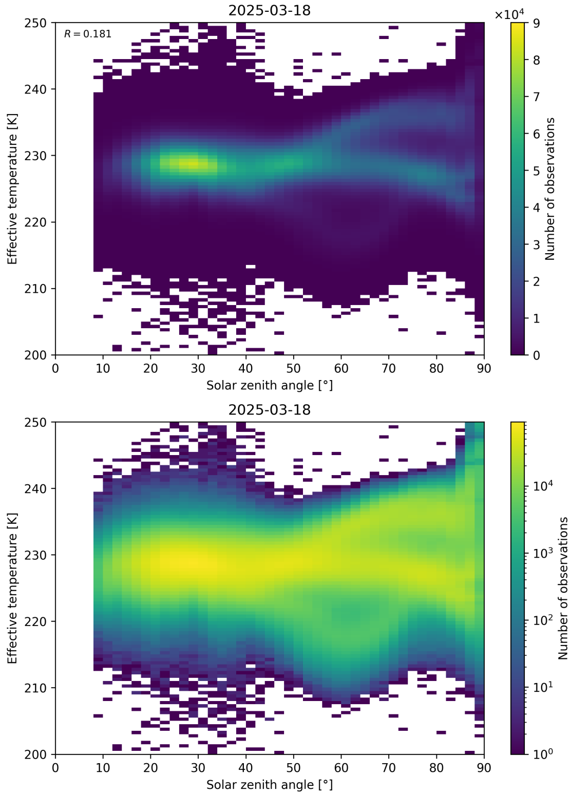
Figure 45: Scatter density plot of “Solar zenith angle” against “Effective temperature” for 2025-03-17 to 2025-03-19.
