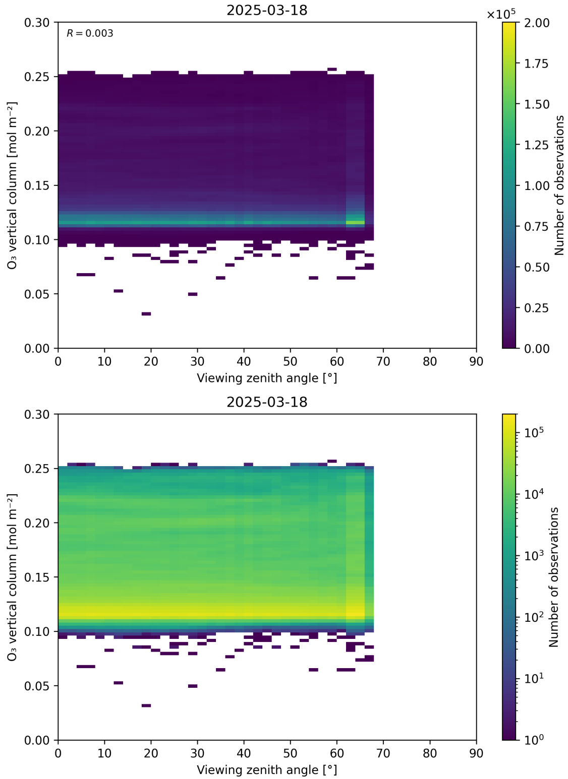
Figure 52: Scatter density plot of “Viewing zenith angle” against “O 3 vertical column” for 2025-03-17 to 2025-03-19.
