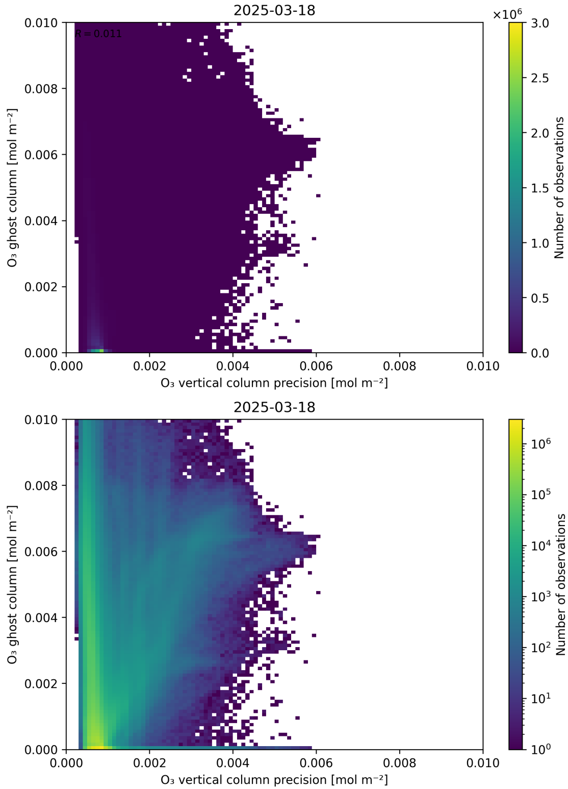
Figure 43: Scatter density plot of “ \text{O}_3 vertical column precision” against “ \text{O}_3 ghost column” for 2025-03-17 to 2025-03-19.
