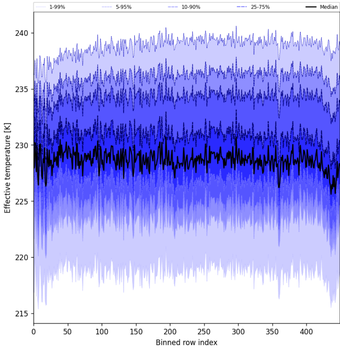
Figure 31: Along track statistics of “Effective temperature” for 2025-03-17 to 2025-03-19
