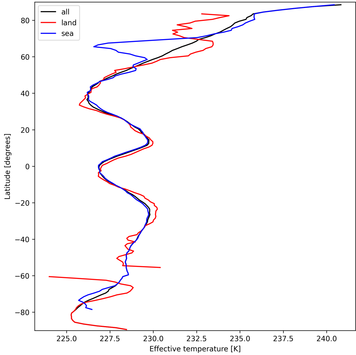
Figure 17: Zonal average of “Effective temperature” for 2025-03-18 to 2025-03-20.
