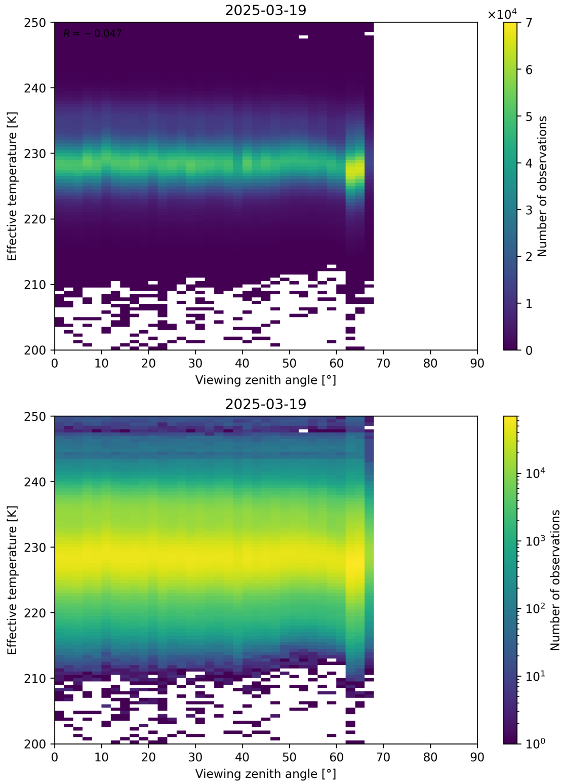
Figure 50: Scatter density plot of “Viewing zenith angle” against “Effective temperature” for 2025-03-18 to 2025-03-20.
