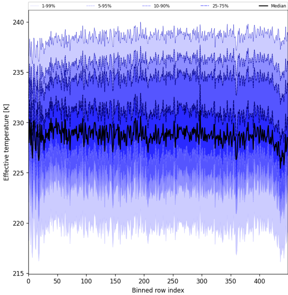
Figure 31: Along track statistics of “Effective temperature” for 2025-03-18 to 2025-03-20
