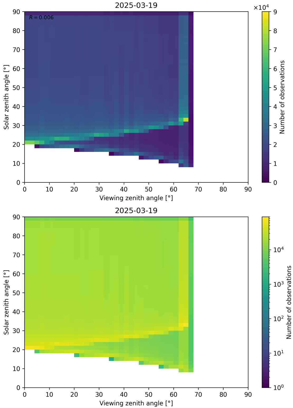
Figure 54: Scatter density plot of “Viewing zenith angle” against “Solar zenith angle” for 2025-03-18 to 2025-03-20.
