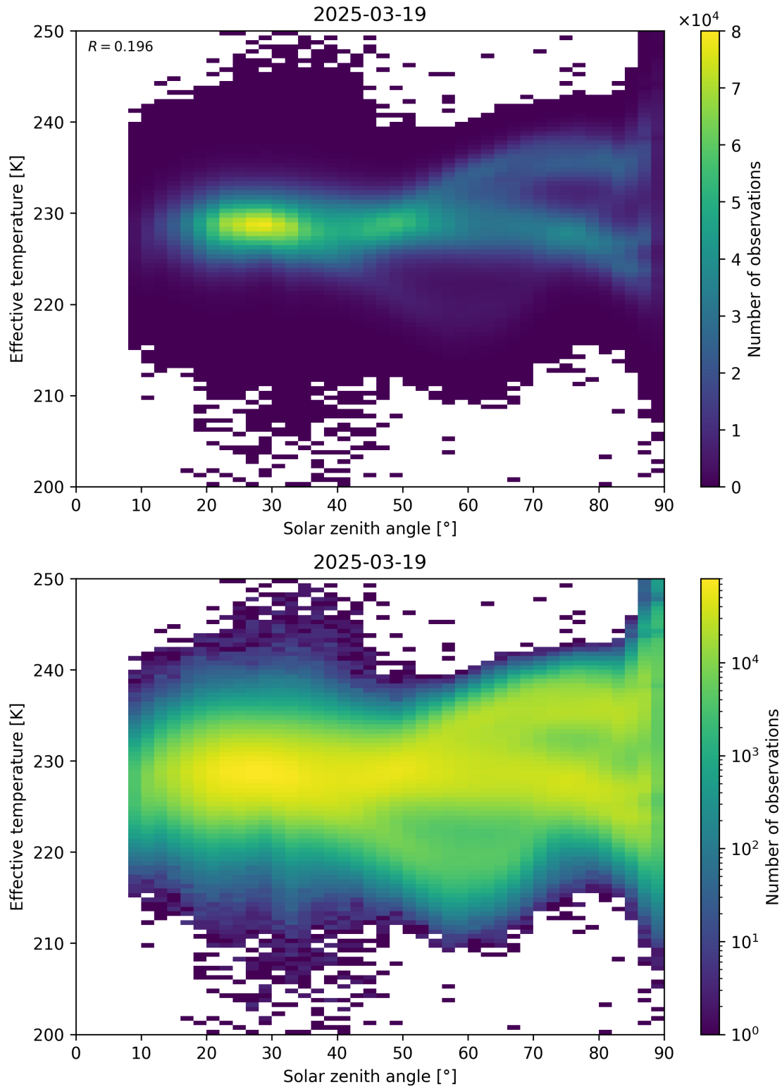
Figure 45: Scatter density plot of “Solar zenith angle” against “Effective temperature” for 2025-03-18 to 2025-03-20.
