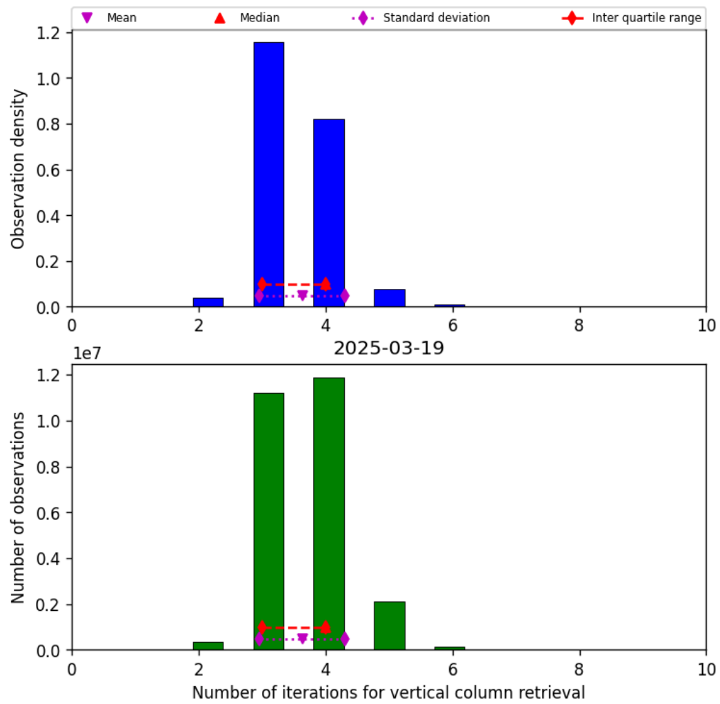
Figure 26: Histogram of “Number of iterations for vertical column retrieval” for 2025-03-18 to 2025-03-20
