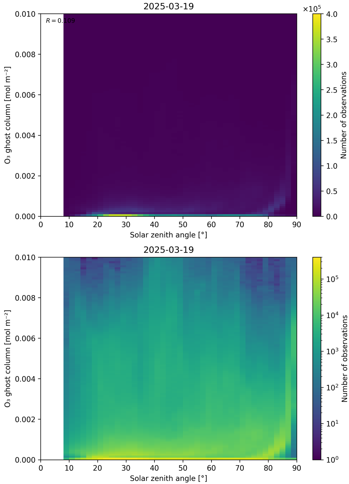
Figure 46: Scatter density plot of “Solar zenith angle” against “O 3 ghost column” for 2025-03-18 to 2025-03-20.
