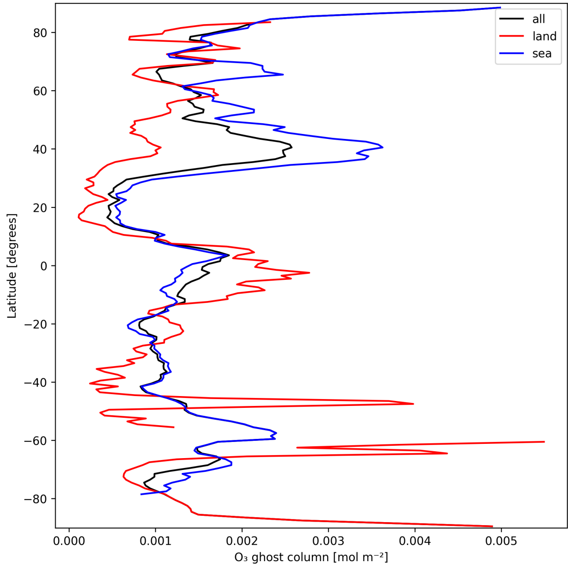
Figure 18: Zonal average of “O 3 ghost column” for 2025-03-18 to 2025-03-20.
