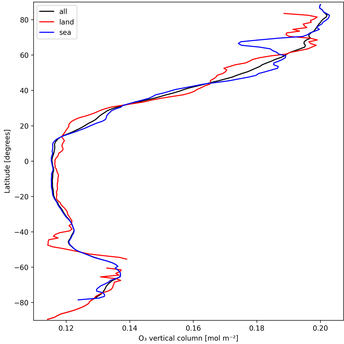
Figure 14: Zonal average of “O 3 vertical column” for 2025-03-18 to 2025-03-20.
