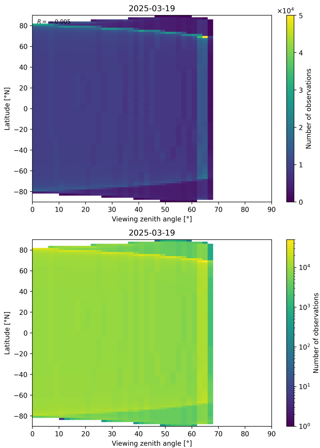
Figure 49: Scatter density plot of “Viewing zenith angle” against “Latitude” for 2025-03-18 to 2025-03-20.
