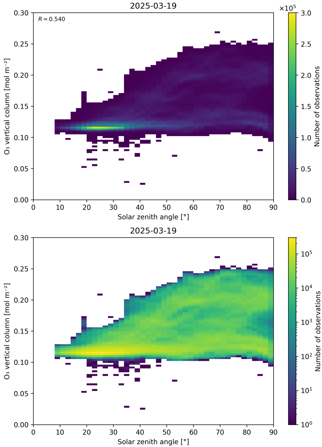
Figure 47: Scatter density plot of “Solar zenith angle” against “O 3 vertical column” for 2025-03-18 to 2025-03-20.
