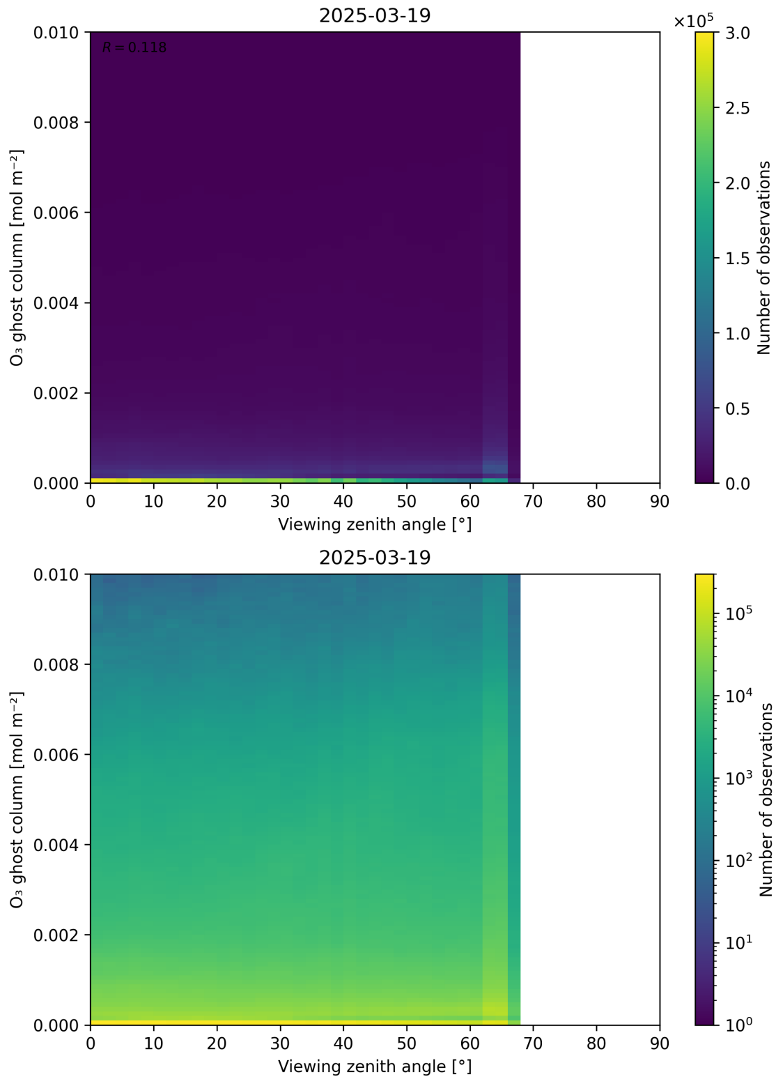
Figure 51: Scatter density plot of “Viewing zenith angle” against “O 3 ghost column” for 2025-03-18 to 2025-03-20.
