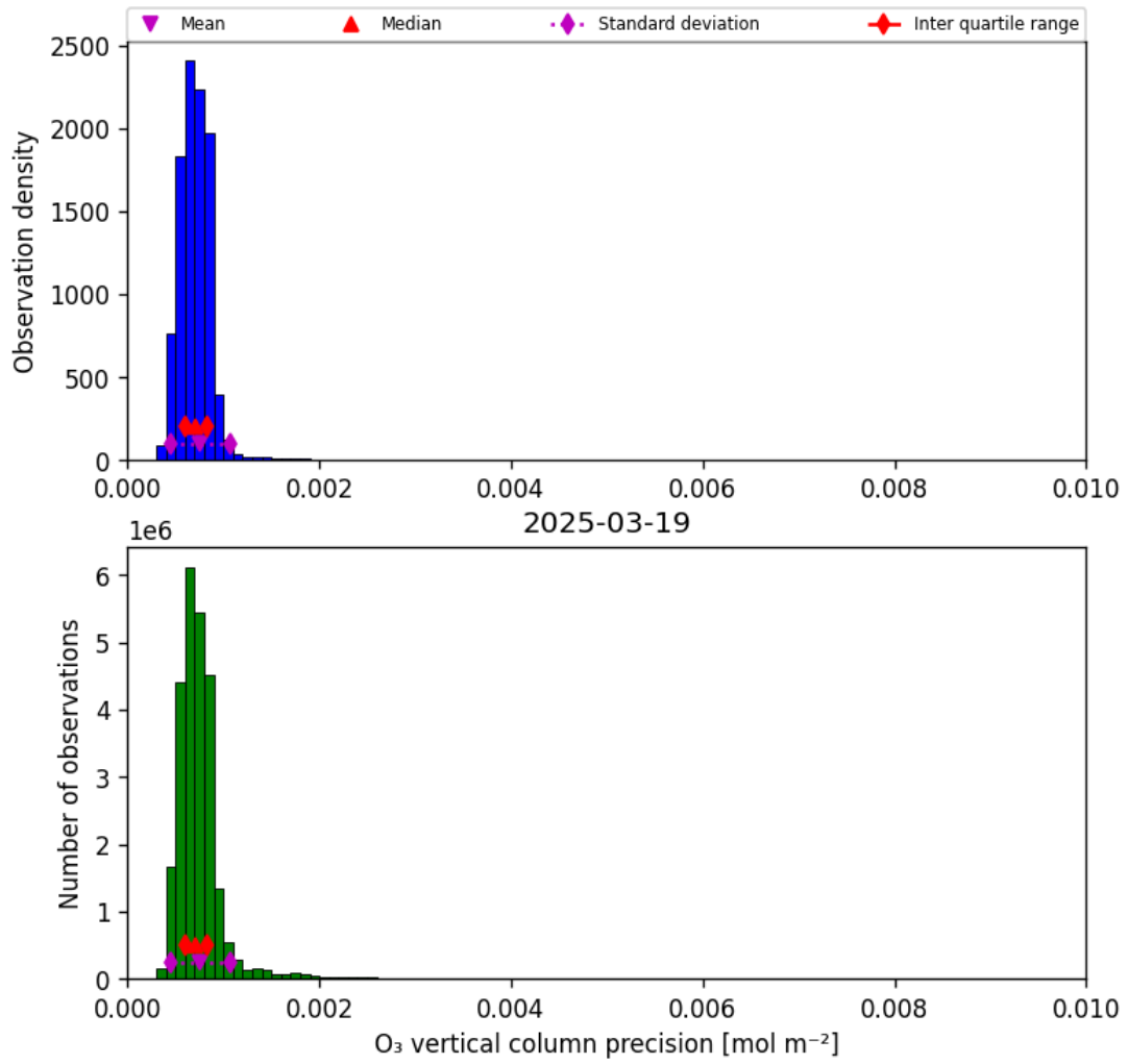
Figure 22: Histogram of “O 3 vertical column precision” for 2025-03-18 to 2025-03-20
