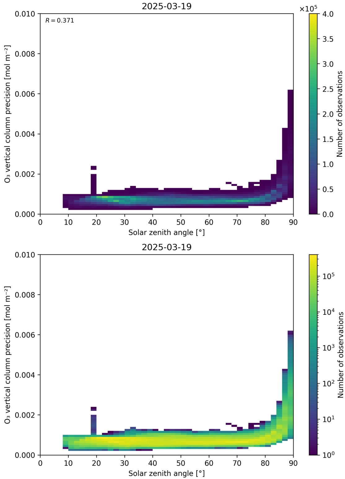
Figure 48: Scatter density plot of “Solar zenith angle” against “O 3 vertical column precision” for 2025-03-18 to 2025-03-20.
