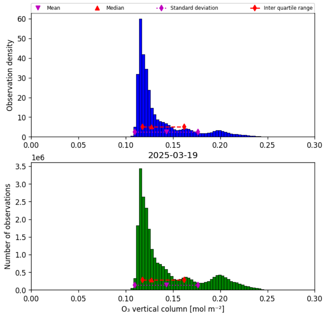
Figure 21: Histogram of “O 3 vertical column” for 2025-03-18 to 2025-03-20
