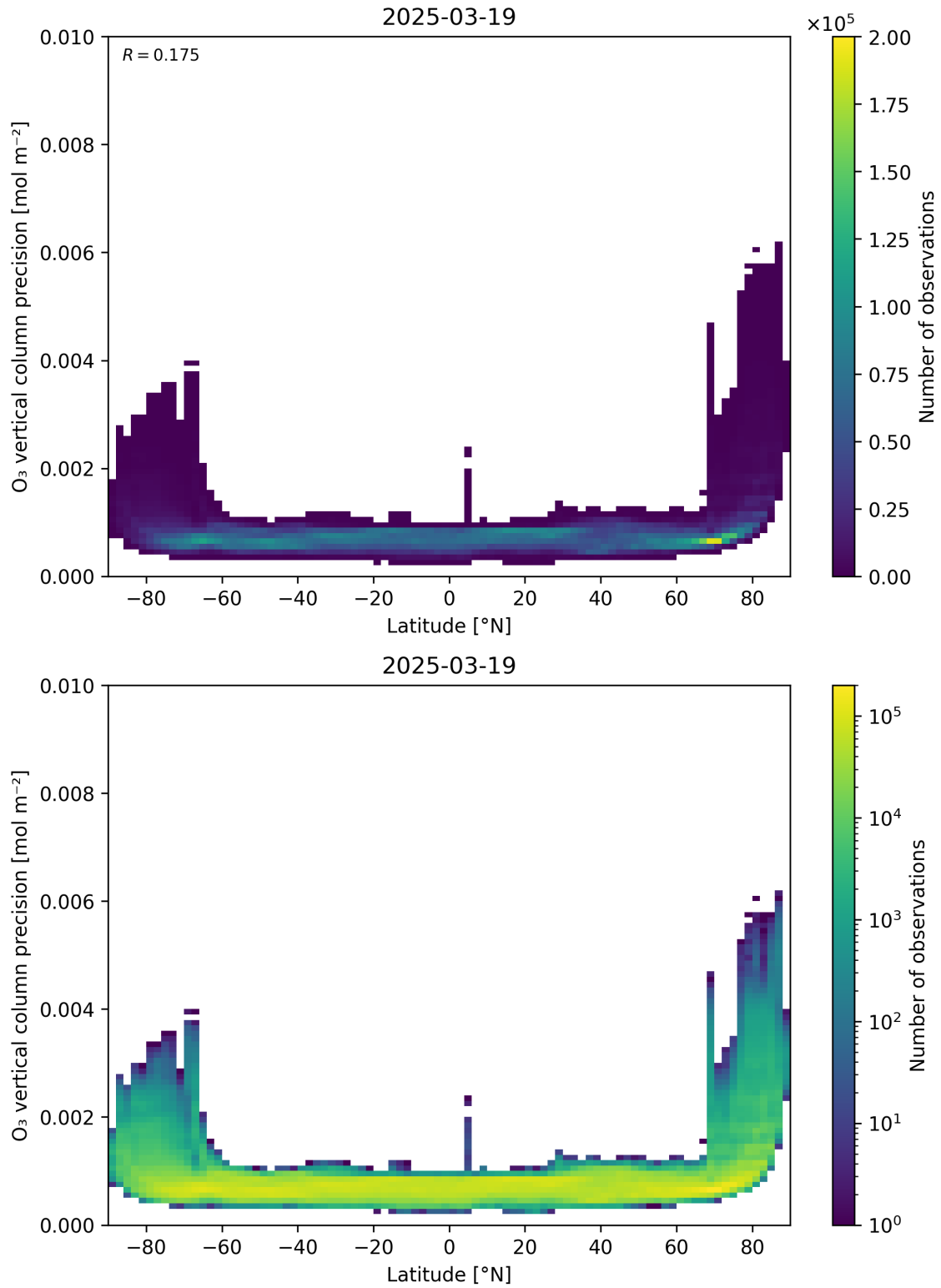
Figure 37: Scatter density plot of “Latitude” against “O 3 vertical column precision” for 2025-03-18 to 2025-03-20.
