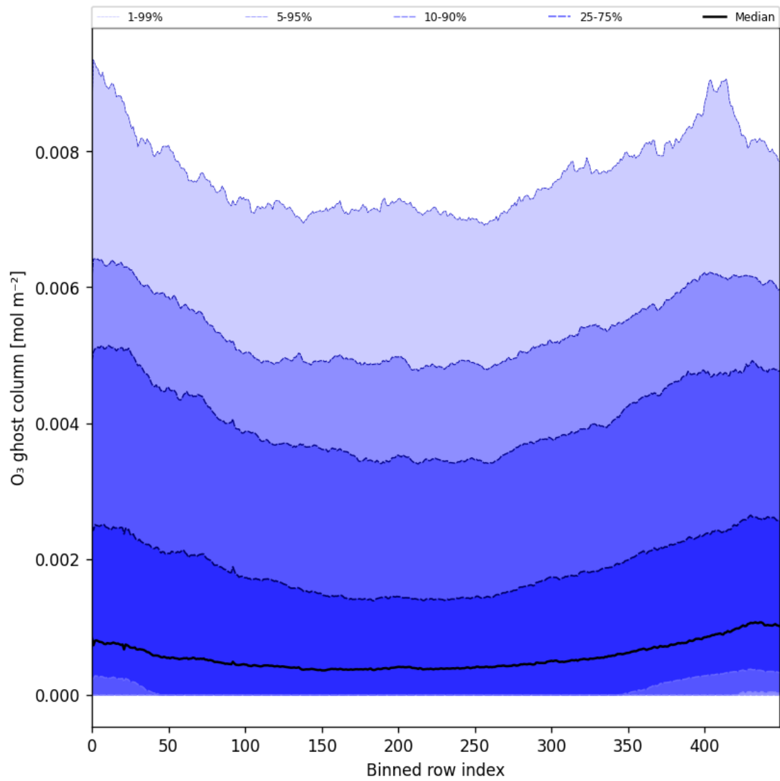
Figure 32: Along track statistics of “O 3 ghost column” for 2025-03-18 to 2025-03-20
