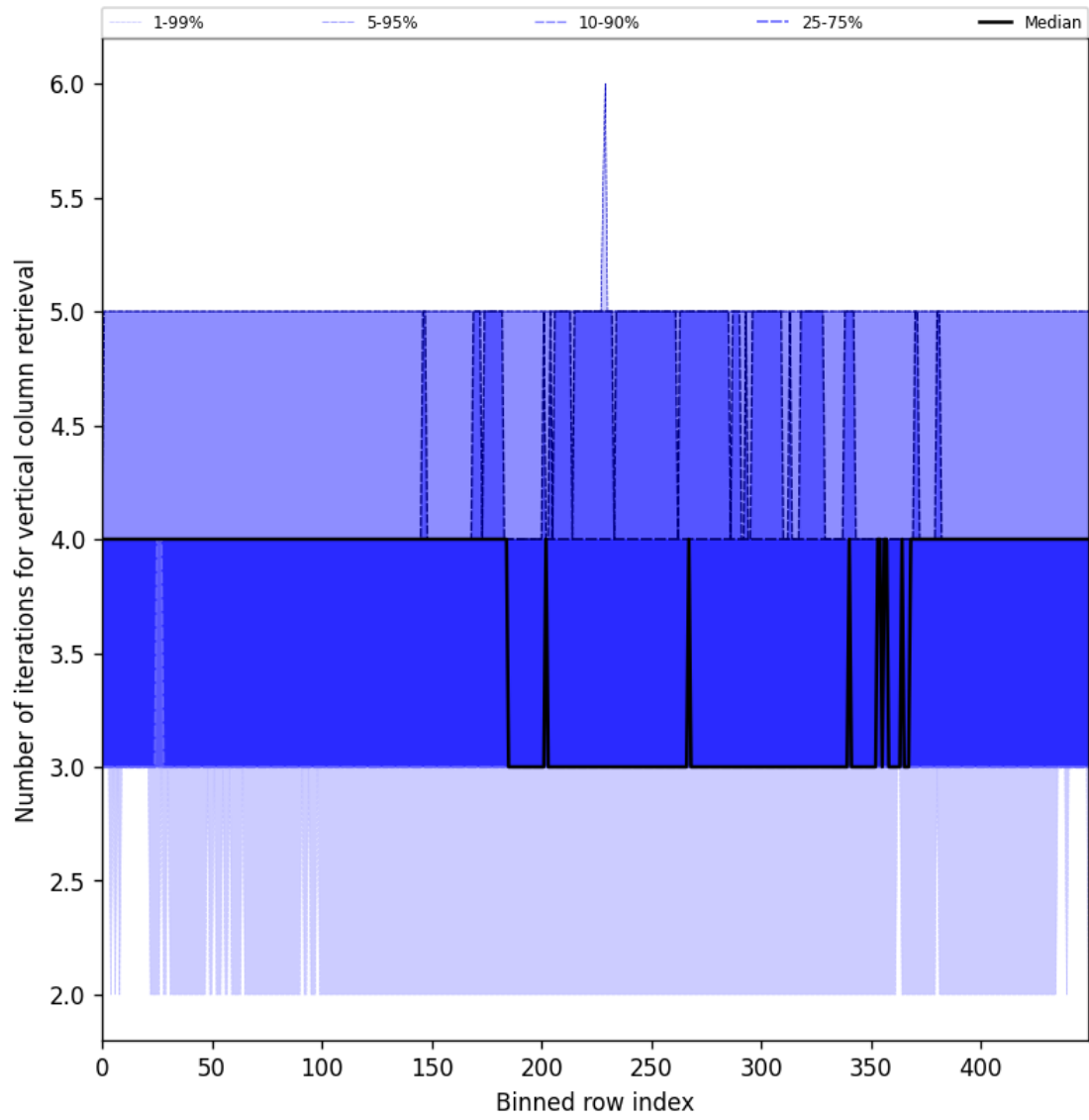
Figure 33: Along track statistics of “Number of iterations for vertical column retrieval” for 2025-03-18 to 2025-03-20
