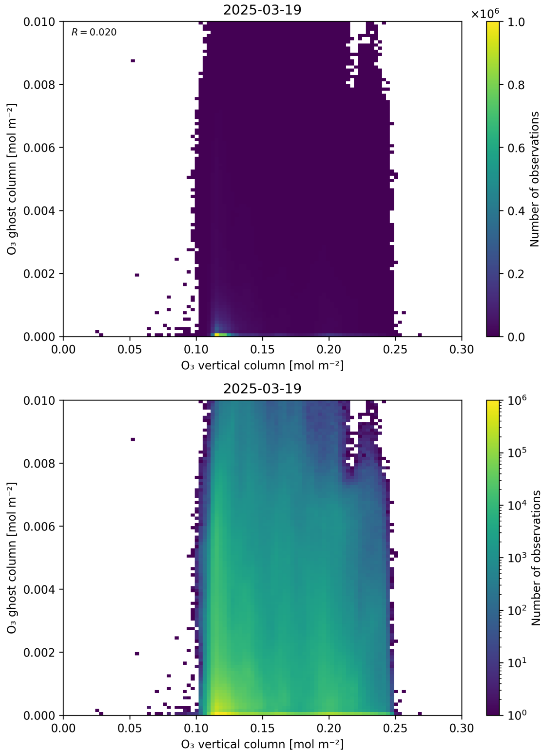
Figure 40: Scatter density plot of “O 3 vertical column” against “O 3 ghost column” for 2025-03-18 to 2025-03-20.
