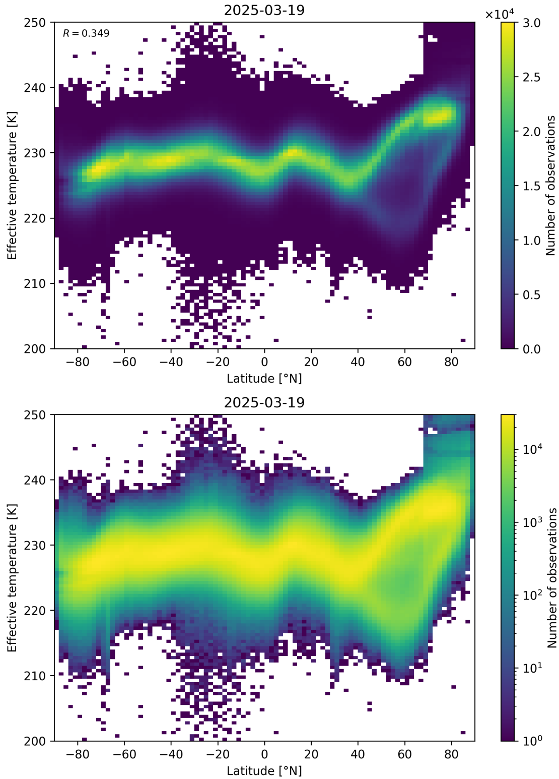
Figure 34: Scatter density plot of “Latitude” against “Effective temperature” for 2025-03-18 to 2025-03-20.
