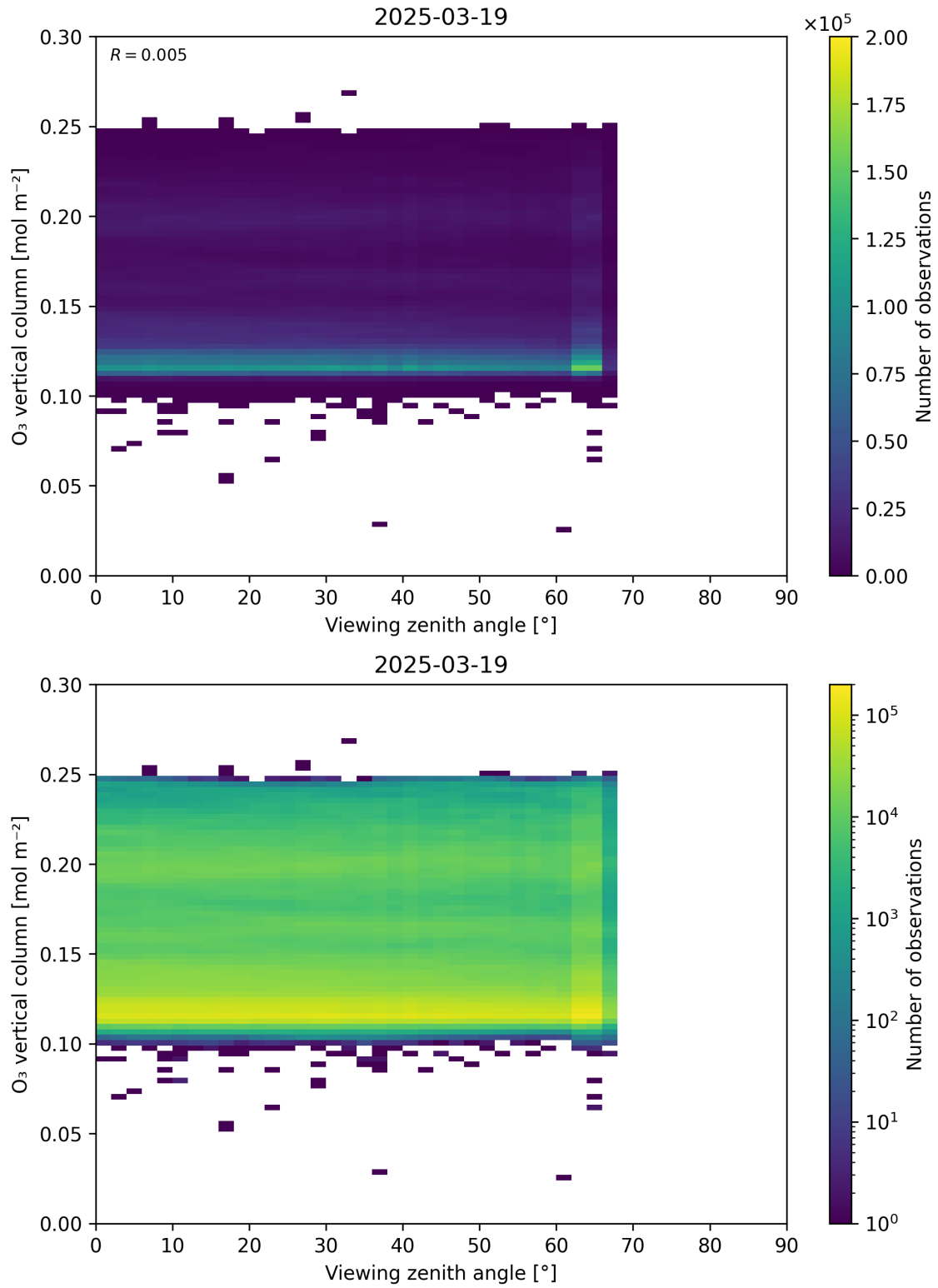
Figure 52: Scatter density plot of “Viewing zenith angle” against “O 3 vertical column” for 2025-03-18 to 2025-03-20.
