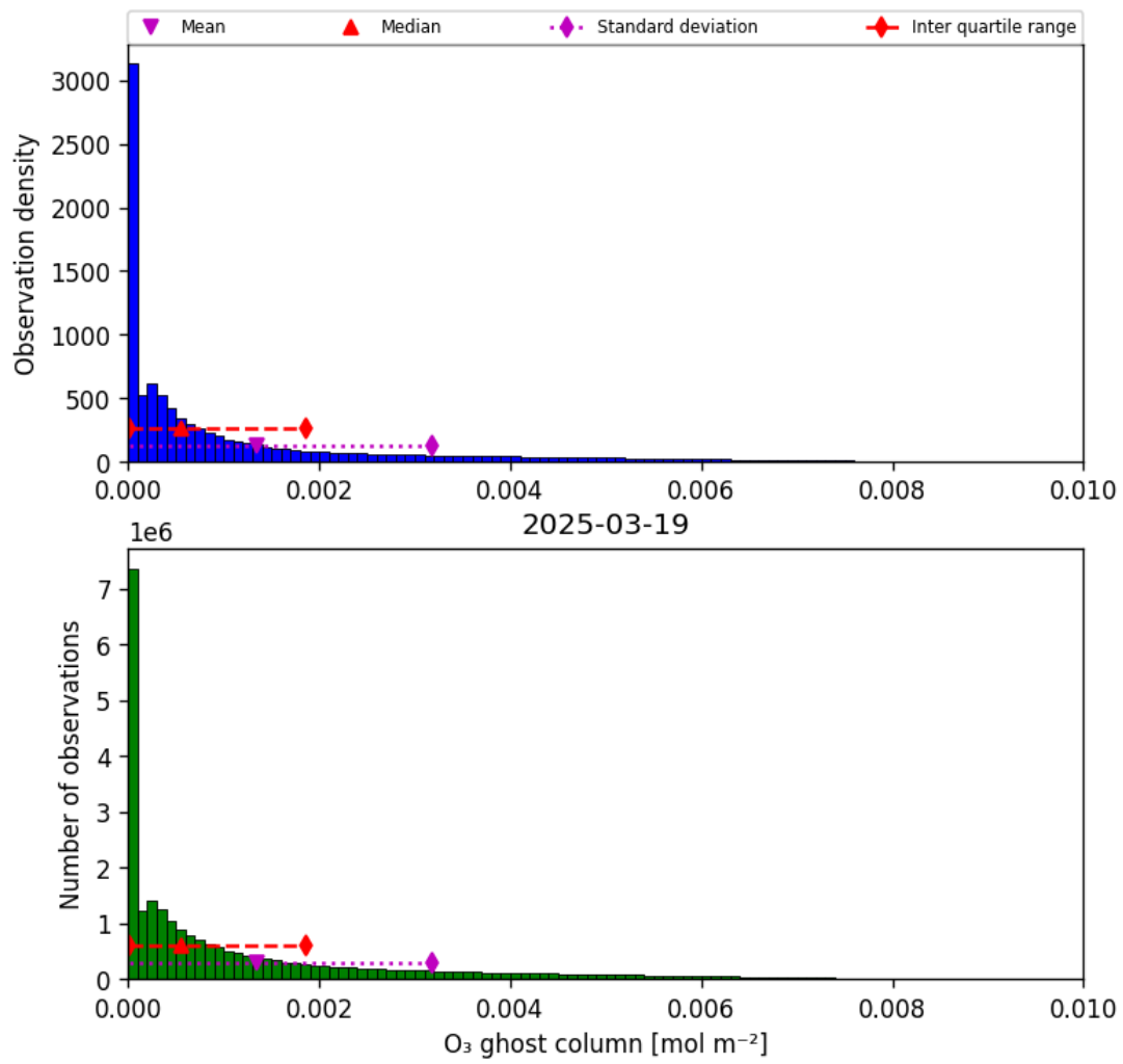
Figure 25: Histogram of “O 3 ghost column” for 2025-03-18 to 2025-03-20
