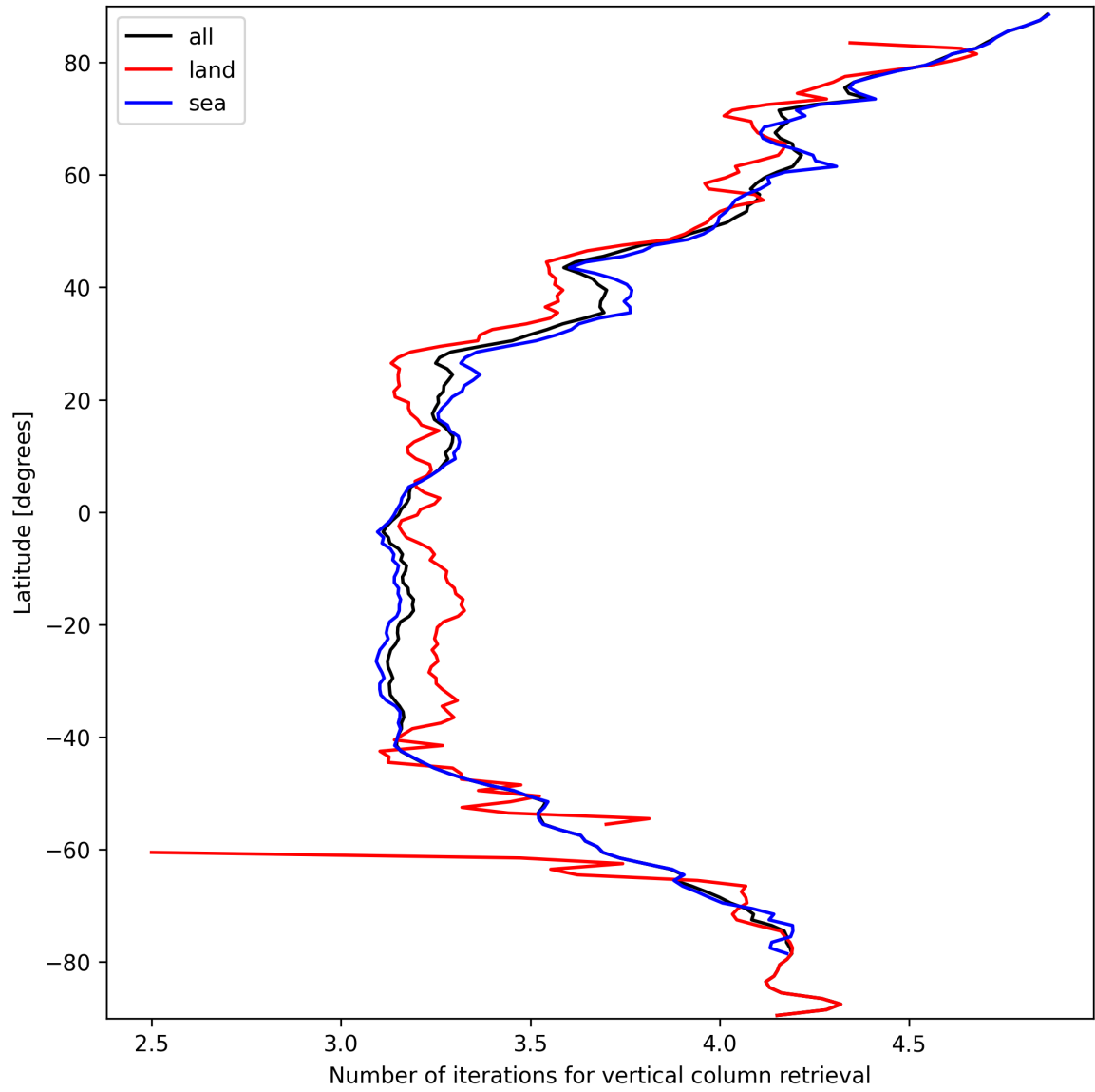
Figure 19: Zonal average of “Number of iterations for vertical column retrieval” for 2025-03-18 to 2025-03-20.
