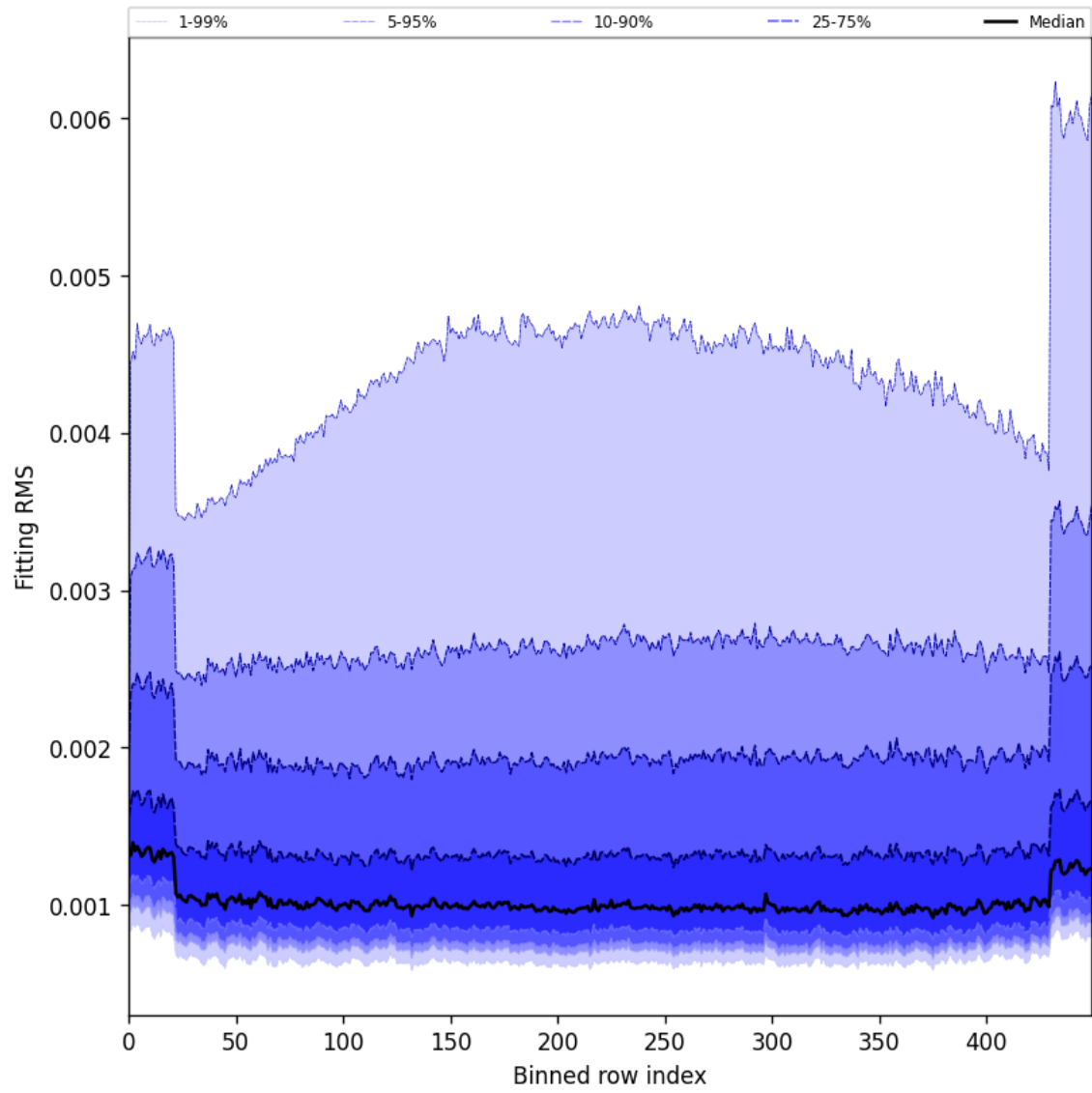
Figure 30: Along track statistics of “Fitting RMS” for 2025-03-18 to 2025-03-20
