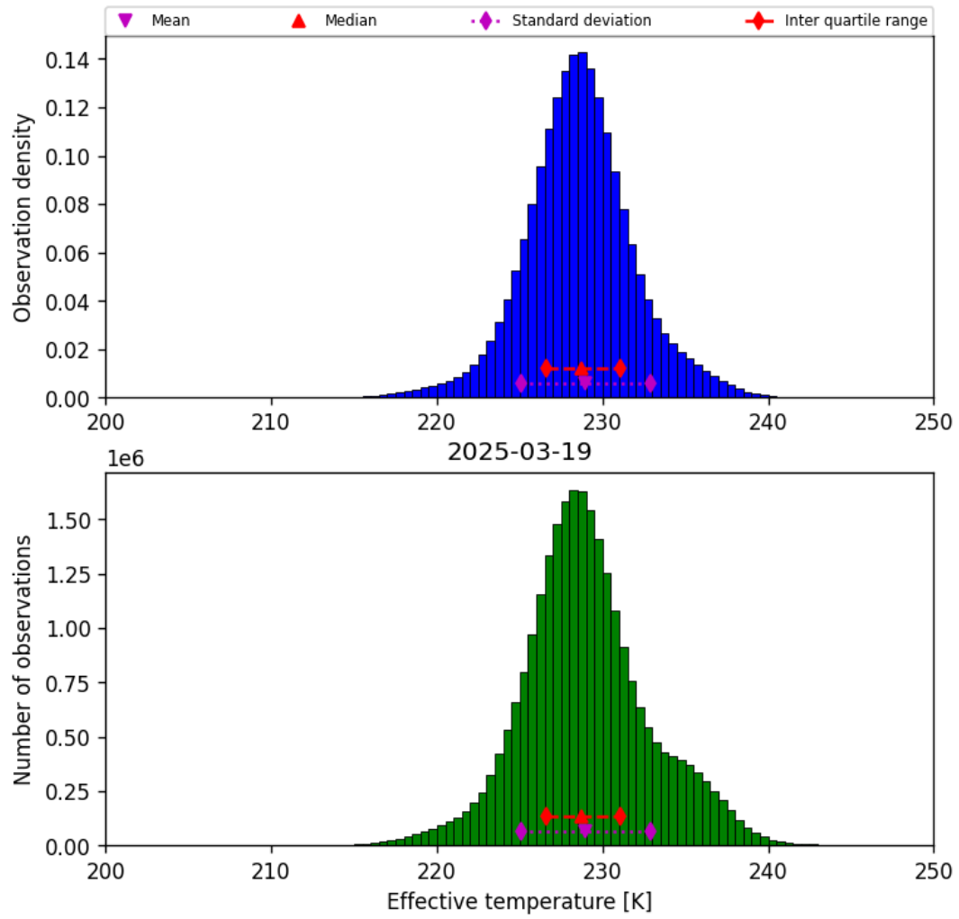
Figure 24: Histogram of “Effective temperature” for 2025-03-18 to 2025-03-20
