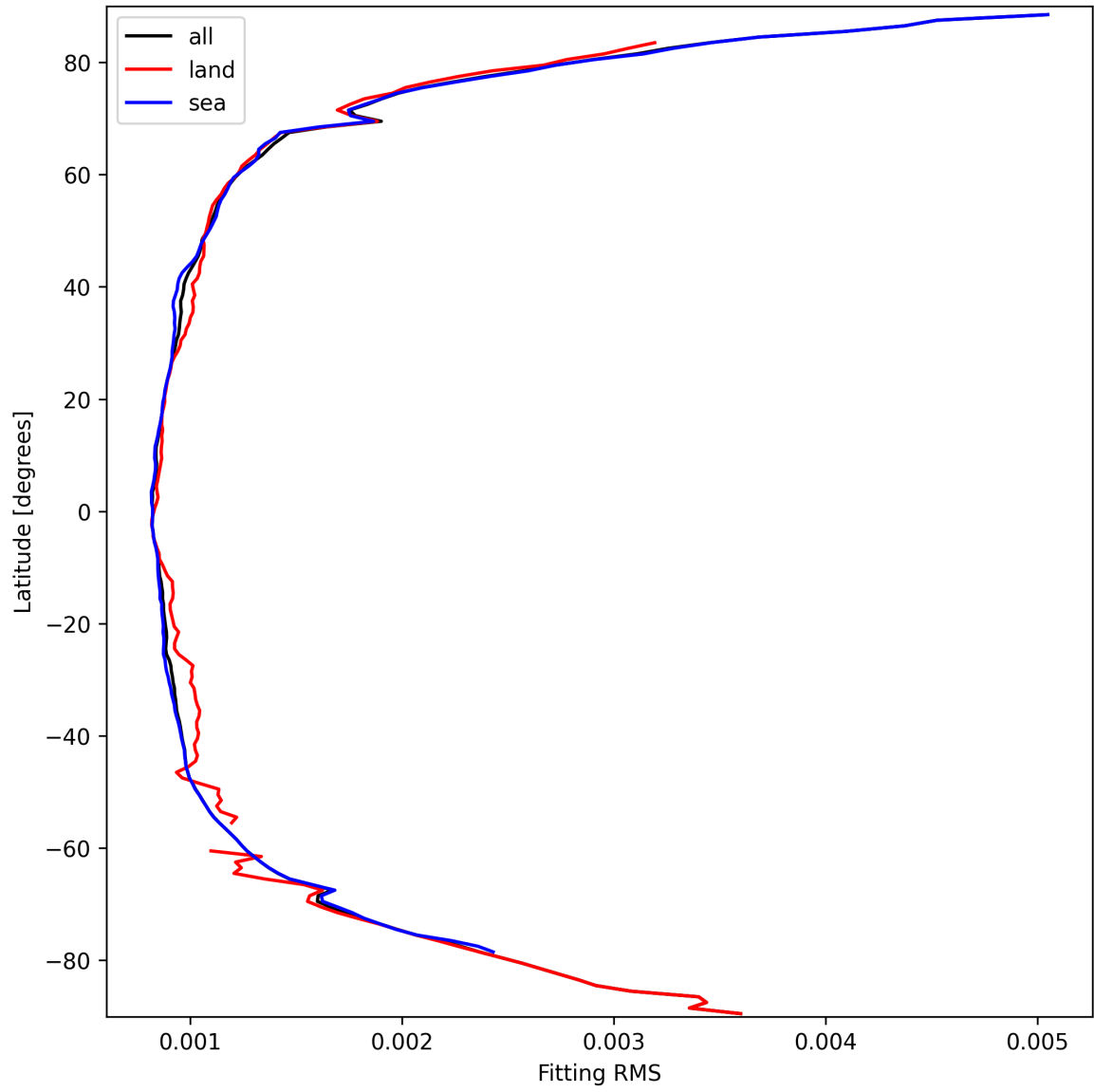
Figure 16: Zonal average of “Fitting RMS” for 2025-03-18 to 2025-03-20.
