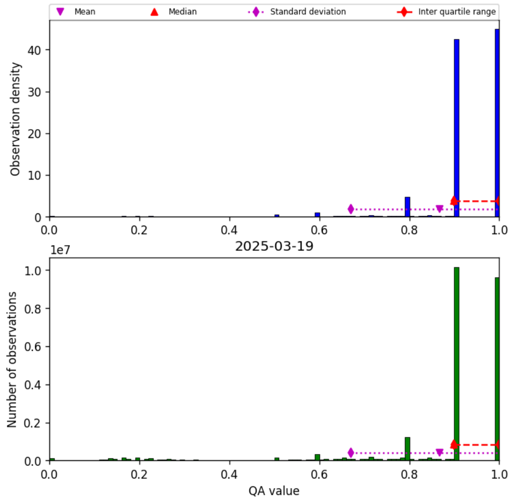
Figure 20: Histogram of “QA value” for 2025-03-18 to 2025-03-20
