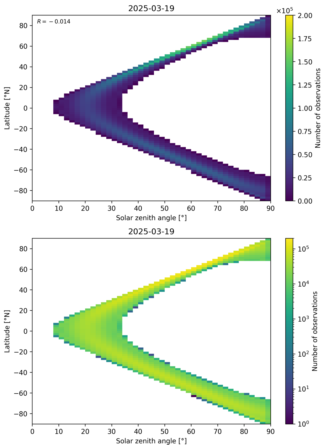
Figure 44: Scatter density plot of “Solar zenith angle” against “Latitude” for 2025-03-18 to 2025-03-20.
