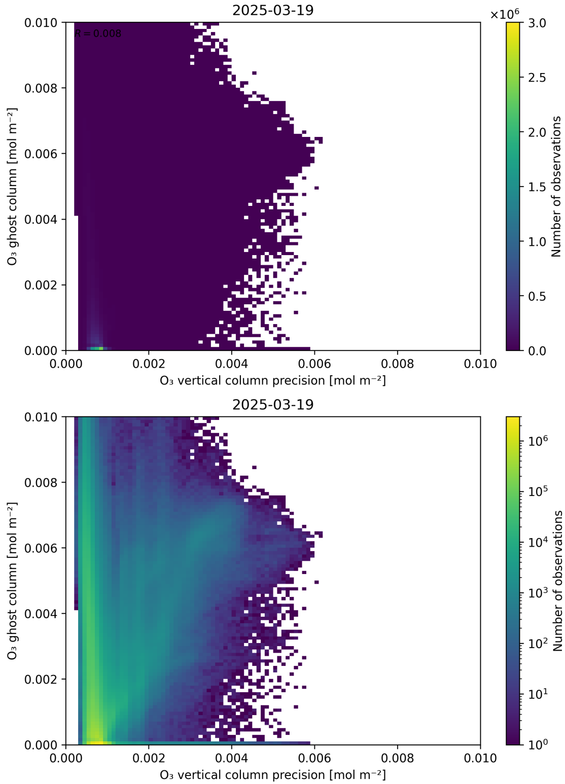
Figure 43: Scatter density plot of “ O_3 vertical column precision” against “ O_3 ghost column” for 2025-03-18 to 2025-03-20.
