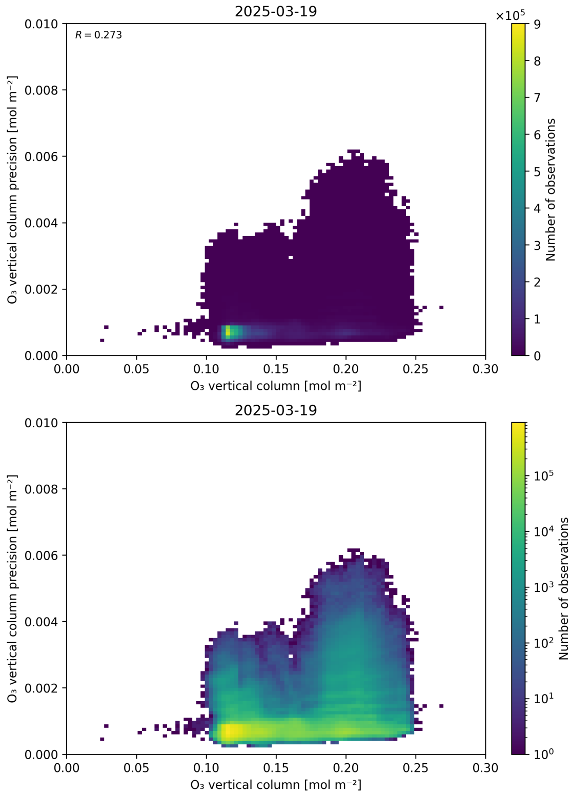
Figure 41: Scatter density plot of “O 3 vertical column” against “O 3 vertical column precision” for 2025-03-18 to 2025-03-20.
