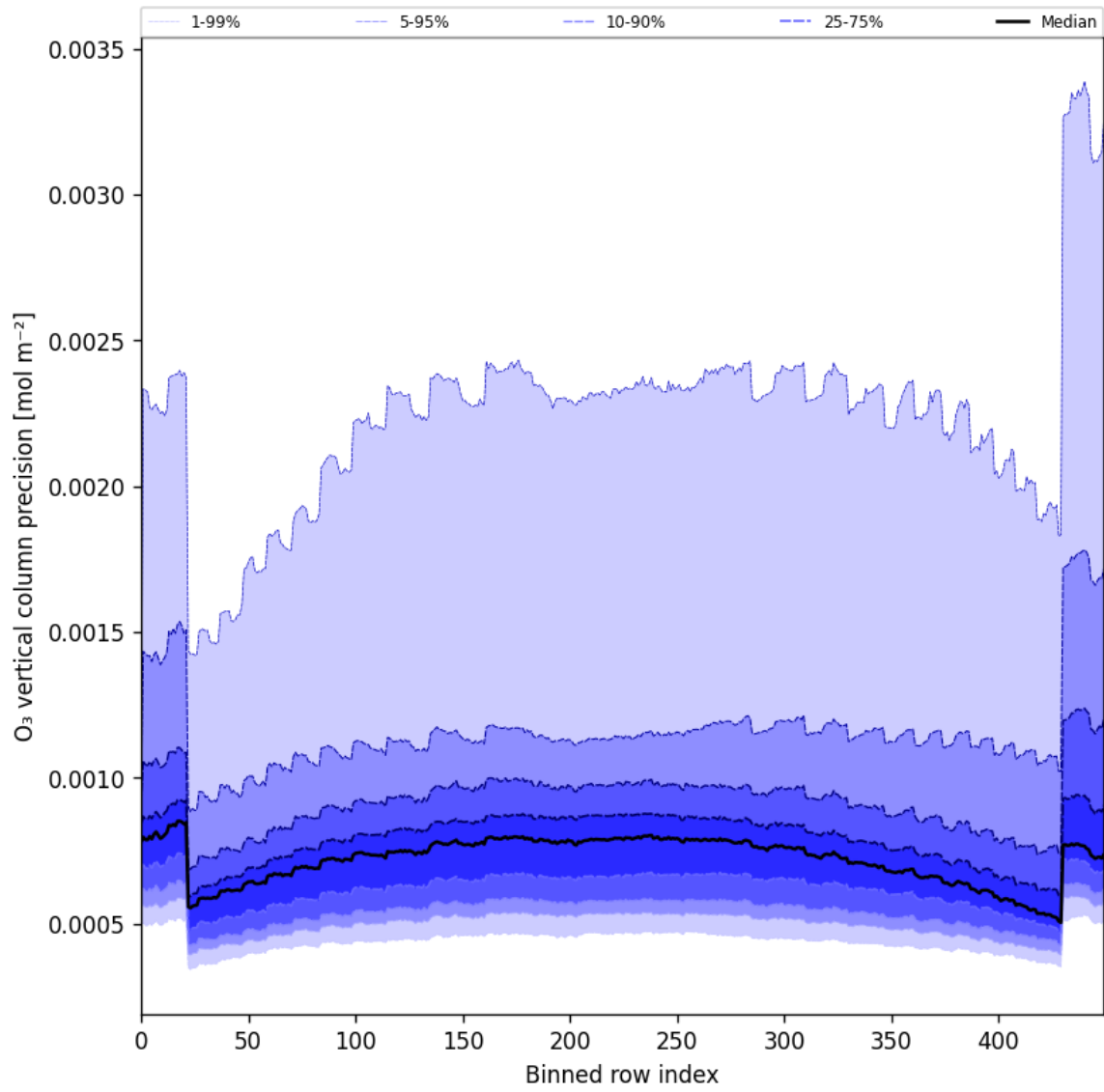
Figure 29: Along track statistics of “O 3 vertical column precision” for 2025-03-18 to 2025-03-20
