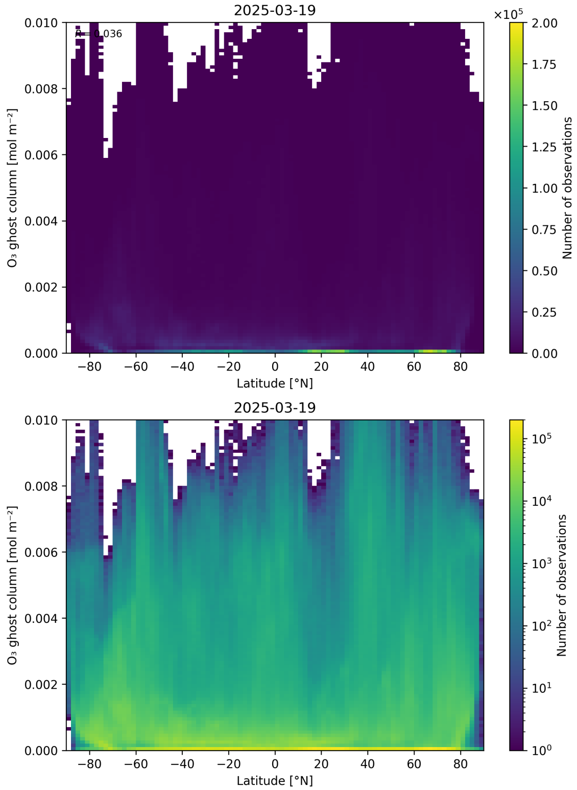
Figure 35: Scatter density plot of “Latitude” against “O 3 ghost column” for 2025-03-18 to 2025-03-20.
