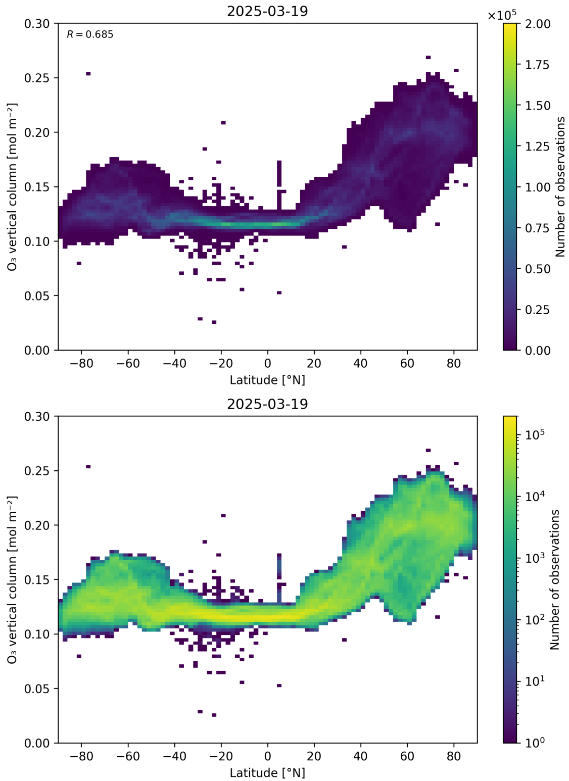
Figure 36: Scatter density plot of “Latitude” against “O 3 vertical column” for 2025-03-18 to 2025-03-20.
