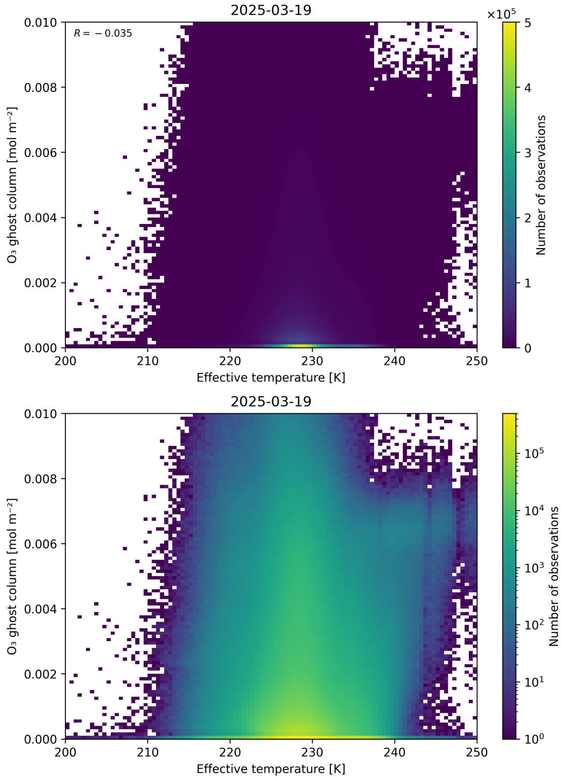
Figure 38: Scatter density plot of “Effective temperature” against “O 3 ghost column” for 2025-03-18 to 2025-03-20.
