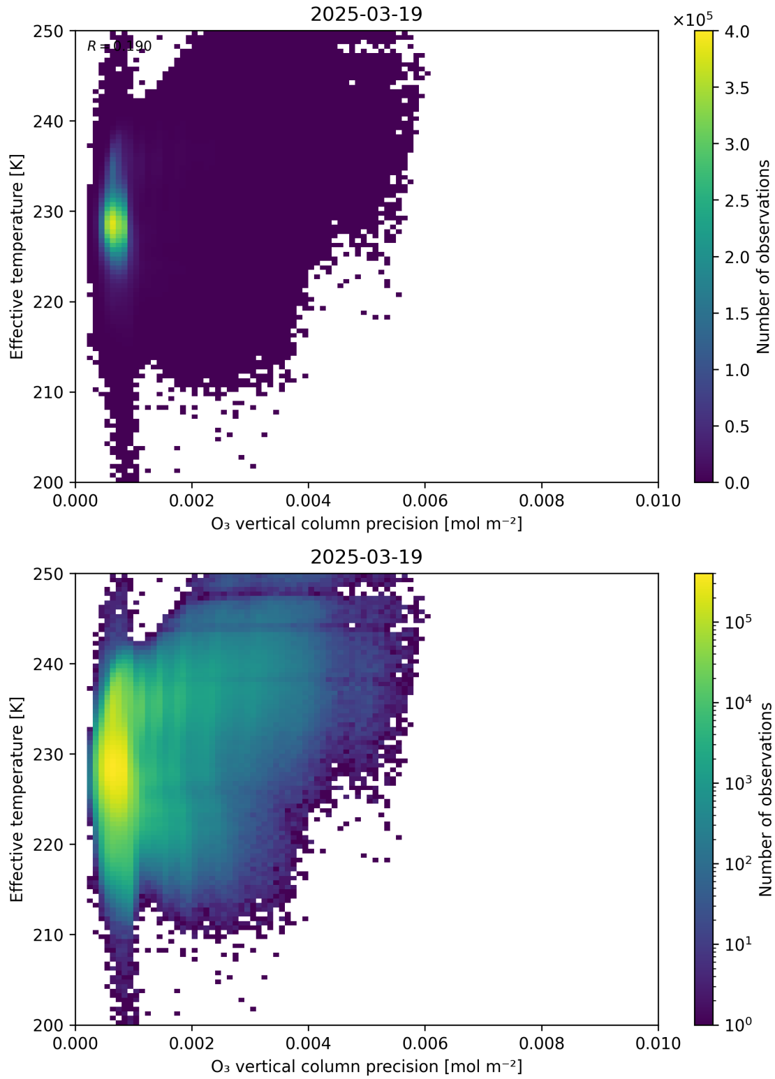
Figure 42: Scatter density plot of “O 3 vertical column precision” against “Effective temperature” for 2025-03-18 to 2025-03-20.
