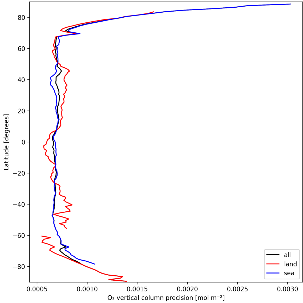
Figure 15: Zonal average of “O 3 vertical column precision” for 2025-03-18 to 2025-03-20.
