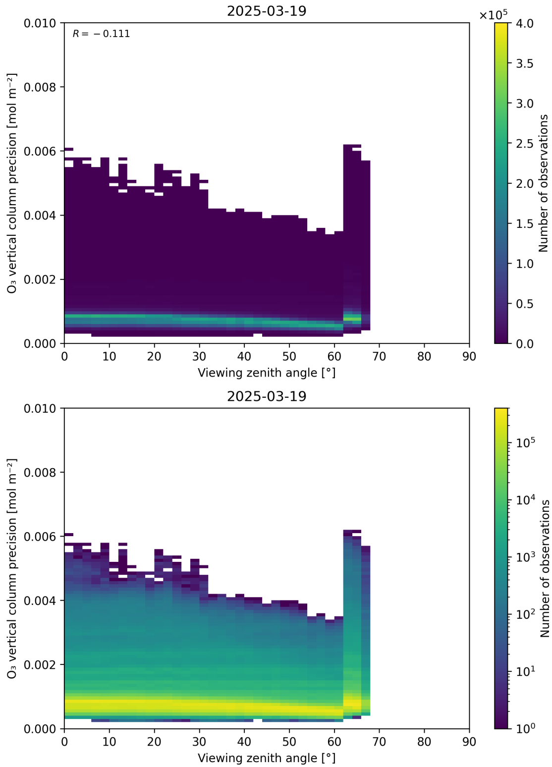
Figure 53: Scatter density plot of “Viewing zenith angle” against “O 3 vertical column precision” for 2025-03-18 to 2025-03-20.
