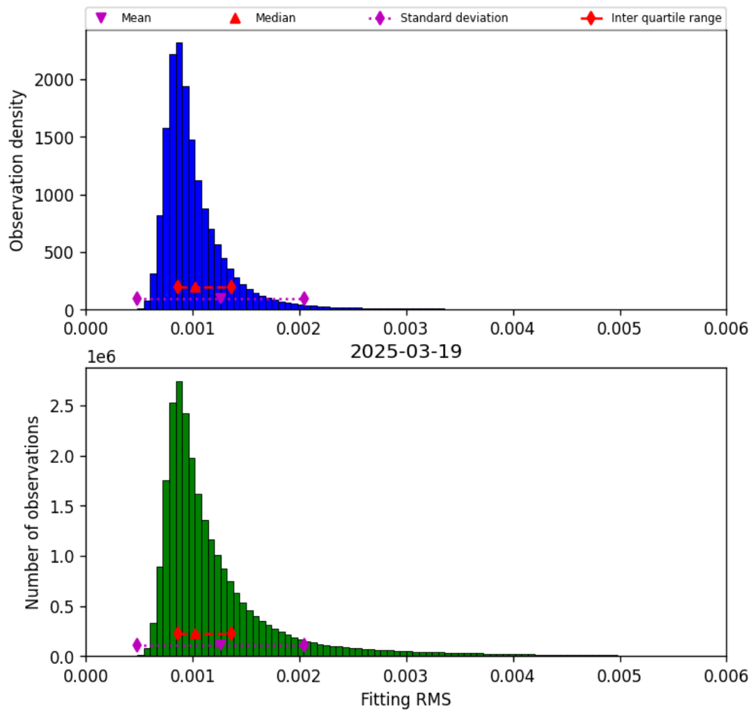
Figure 23: Histogram of “Fitting RMS” for 2025-03-18 to 2025-03-20
