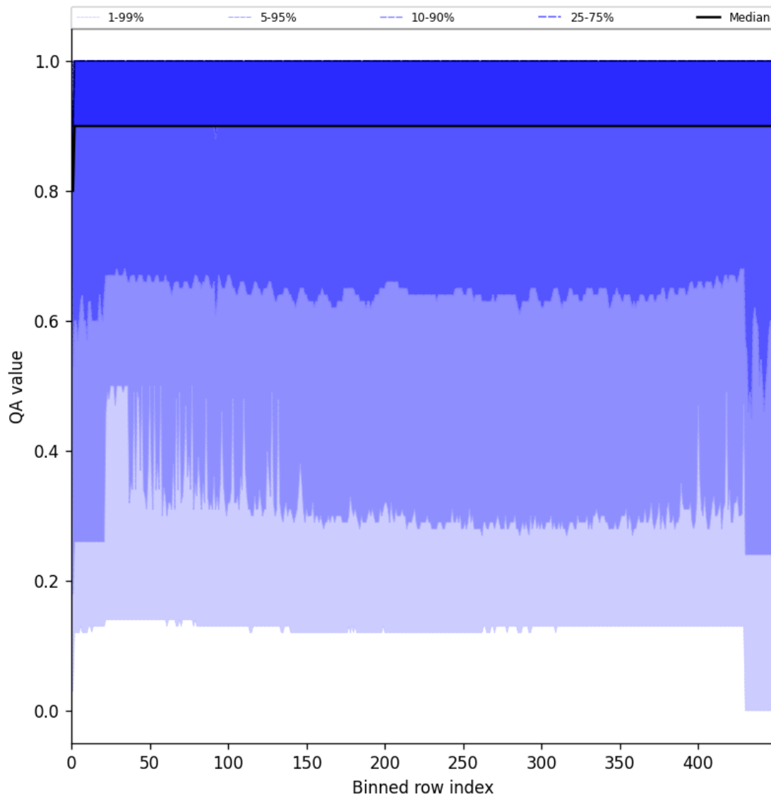
Figure 27: Along track statistics of “QA value” for 2025-03-18 to 2025-03-20
