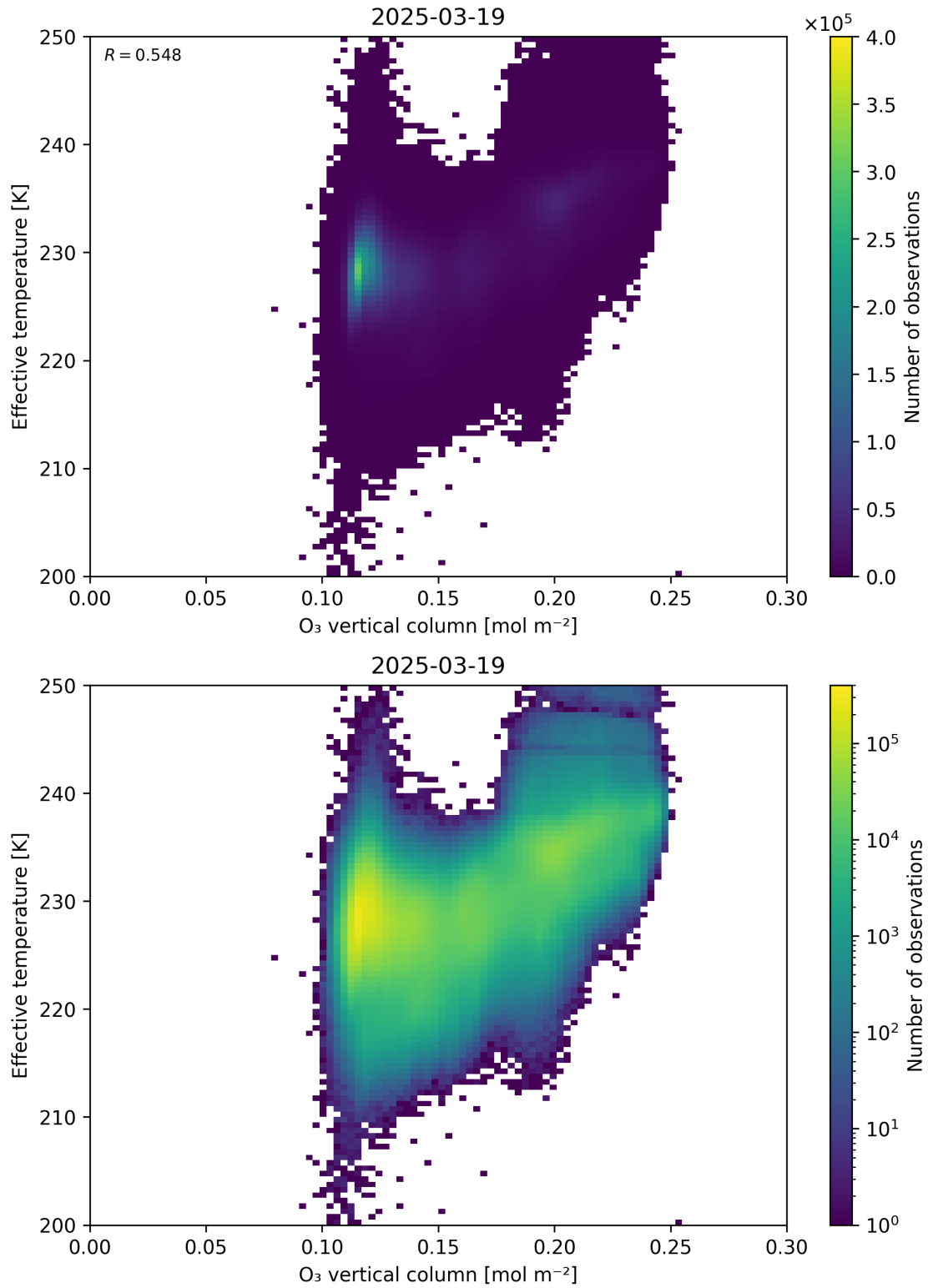
Figure 39: Scatter density plot of “O 3 vertical column” against “Effective temperature” for 2025-03-18 to 2025-03-20.
