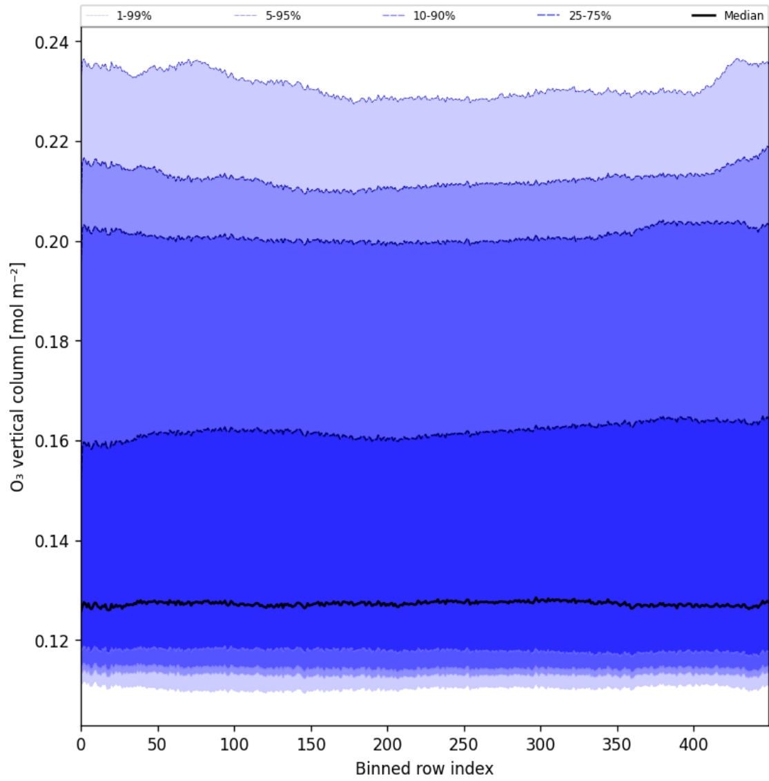
Figure 28: Along track statistics of “O 3 vertical column” for 2025-03-18 to 2025-03-20
