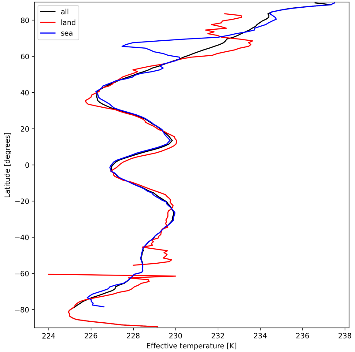
Figure 17: Zonal average of “Effective temperature” for 2025-03-19 to 2025-03-21.
