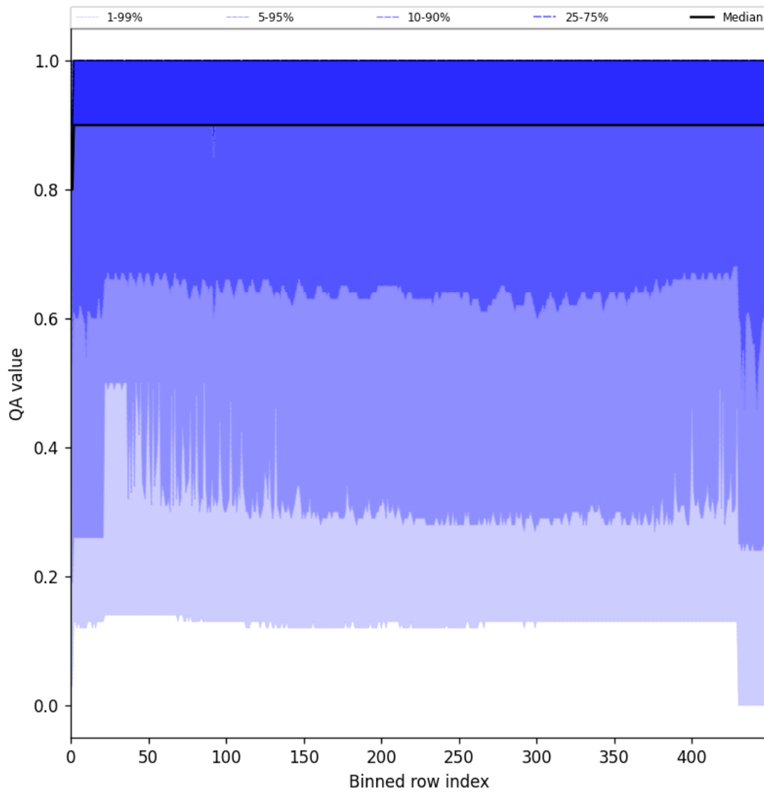
Figure 27: Along track statistics of “QA value” for 2025-03-19 to 2025-03-21
