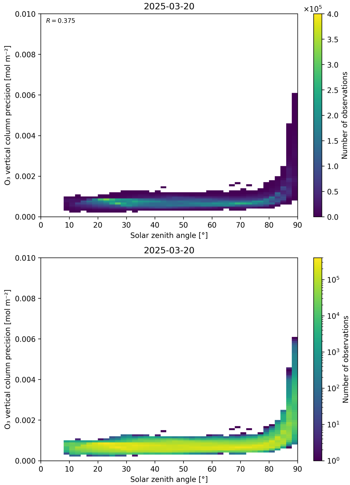
Figure 48: Scatter density plot of “Solar zenith angle” against “O 3 vertical column precision” for 2025-03-19 to 2025-03-21.
