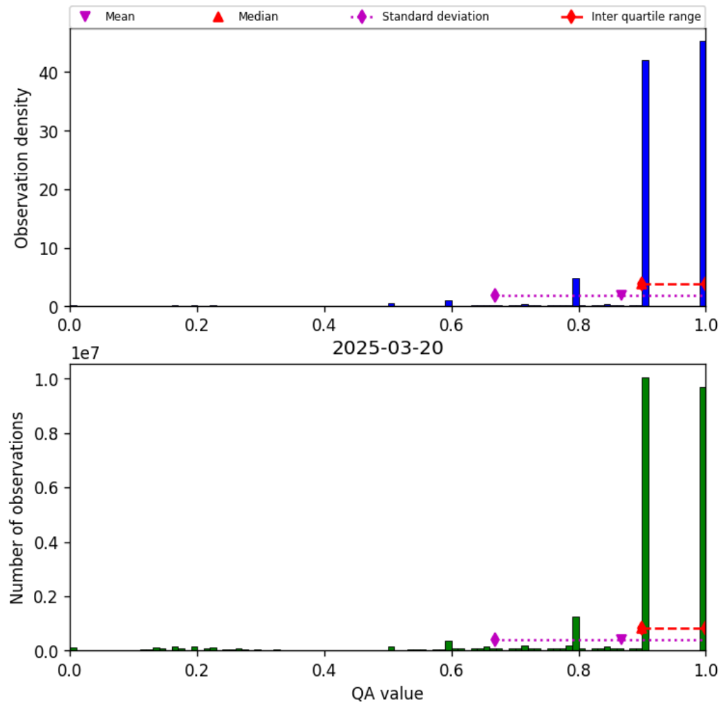
Figure 20: Histogram of “QA value” for 2025-03-19 to 2025-03-21
