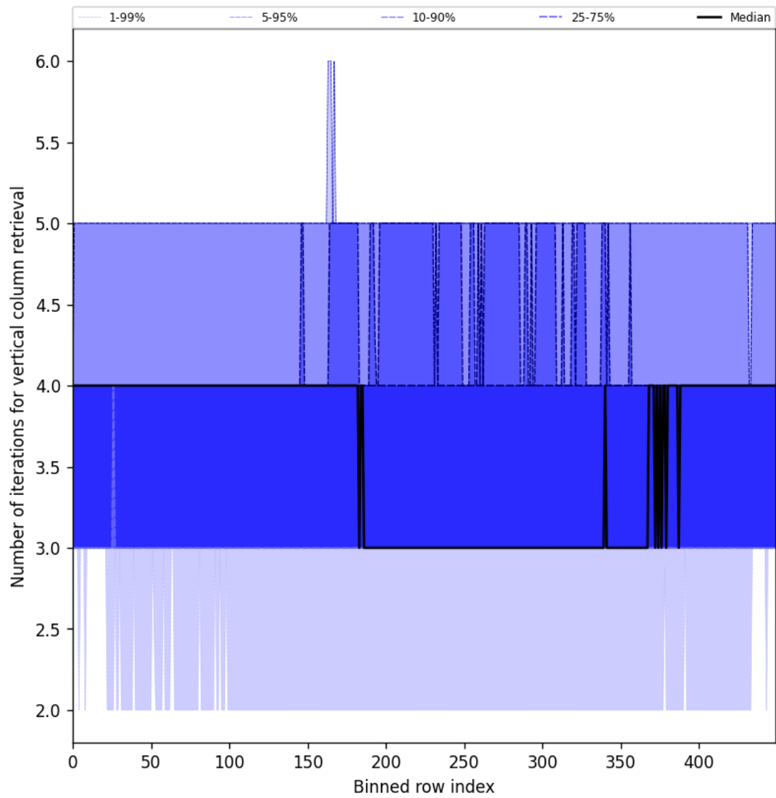
Figure 33: Along track statistics of “Number of iterations for vertical column retrieval” for 2025-03-19 to 2025-03-21
