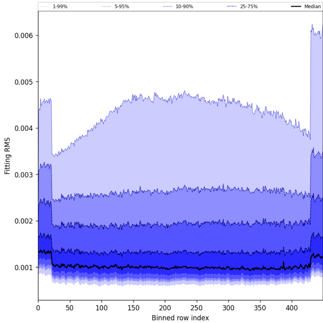
Figure 30: Along track statistics of “Fitting RMS” for 2025-03-19 to 2025-03-21
