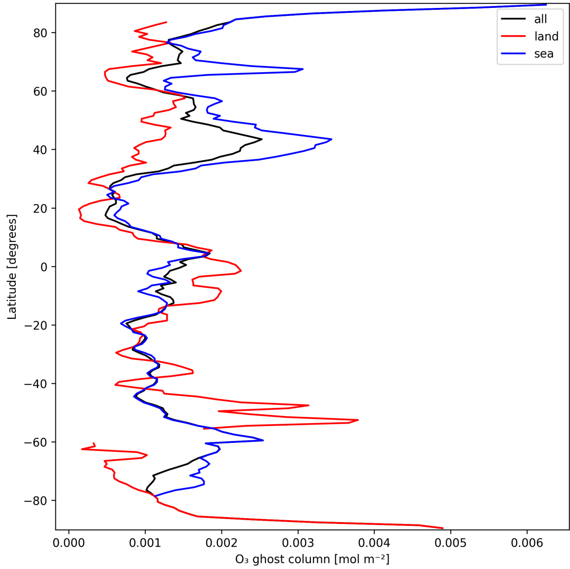
Figure 18: Zonal average of “O 3 ghost column” for 2025-03-19 to 2025-03-21.
