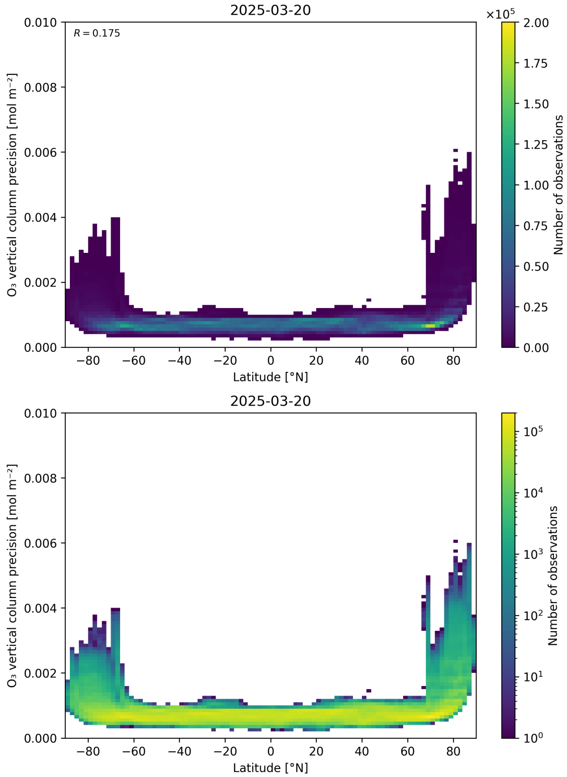
Figure 37: Scatter density plot of “Latitude” against “O 3 vertical column precision” for 2025-03-19 to 2025-03-21.
