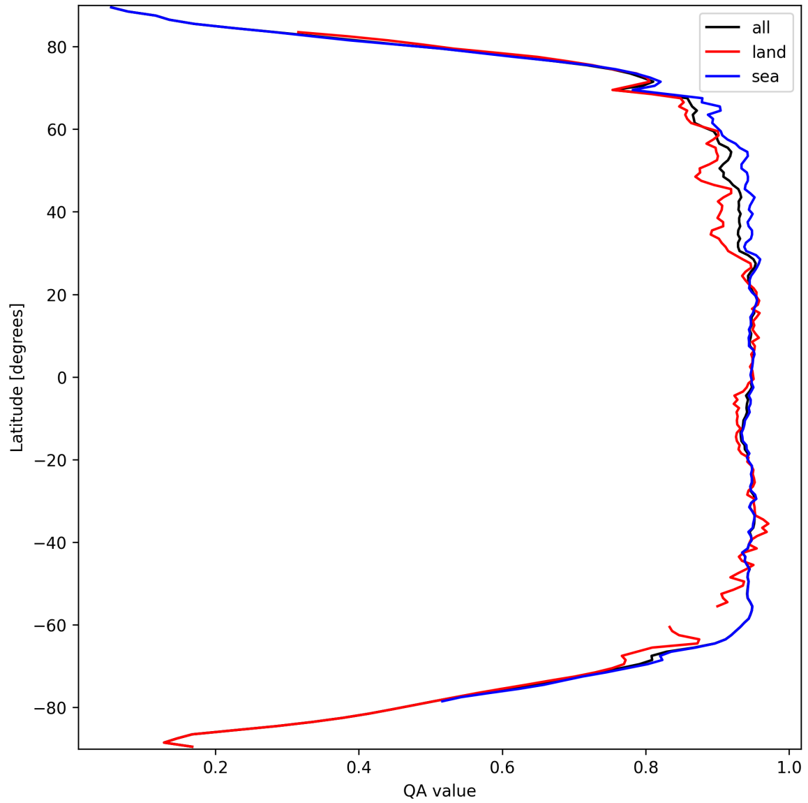
Figure 13: Zonal average of “QA value” for 2025-03-19 to 2025-03-21.
