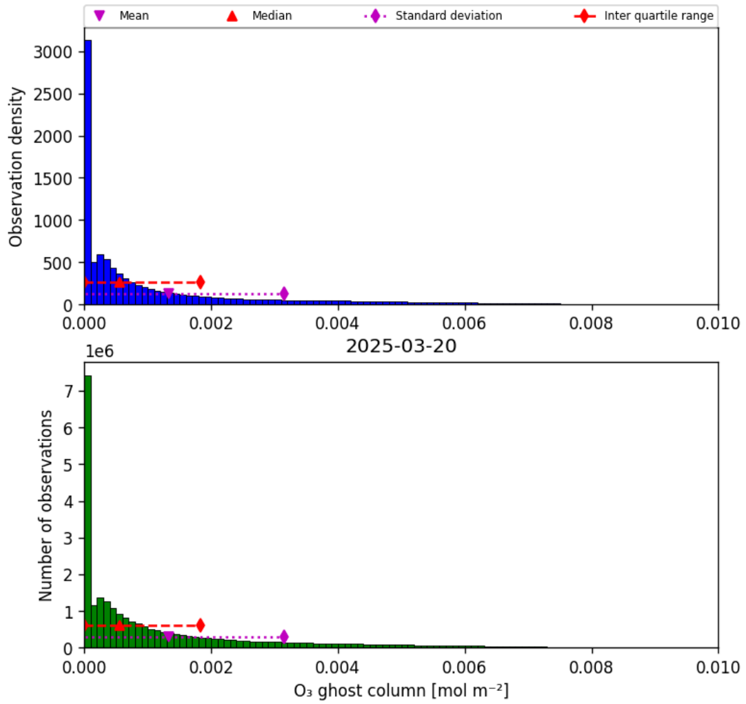
Figure 25: Histogram of “O 3 ghost column” for 2025-03-19 to 2025-03-21
