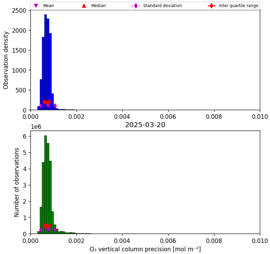
Figure 22: Histogram of "O 3 vertical column precision" for 2025-03-19 to 2025-03-21
