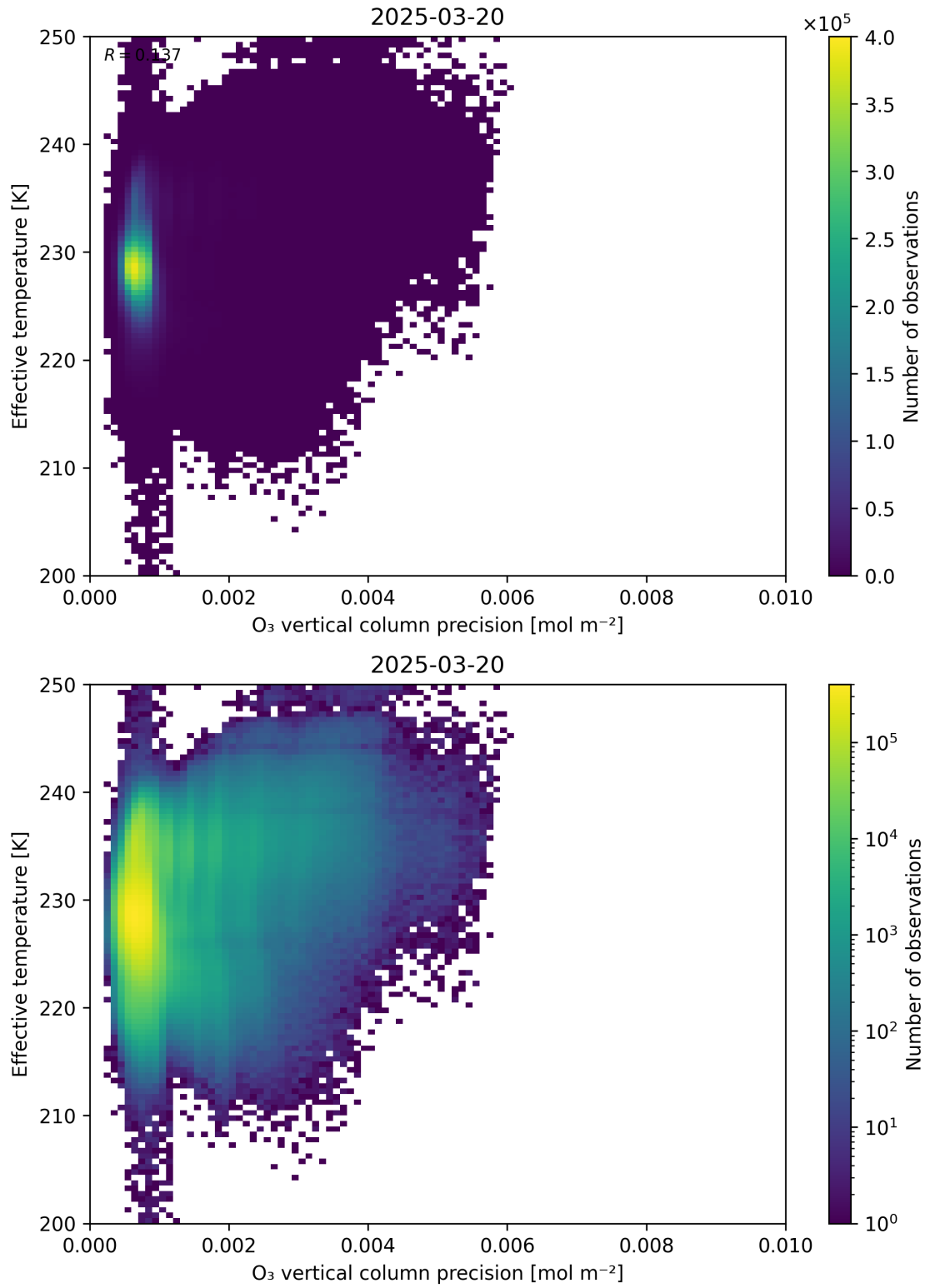
Figure 42: Scatter density plot of “O 3 vertical column precision” against “Effective temperature” for 2025-03-19 to 2025-03-21.
