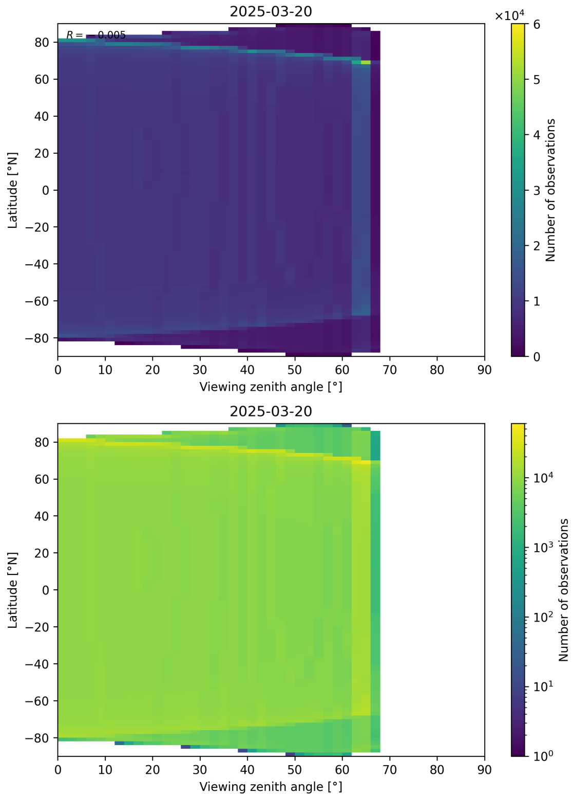
Figure 49: Scatter density plot of “Viewing zenith angle” against “Latitude” for 2025-03-19 to 2025-03-21.
