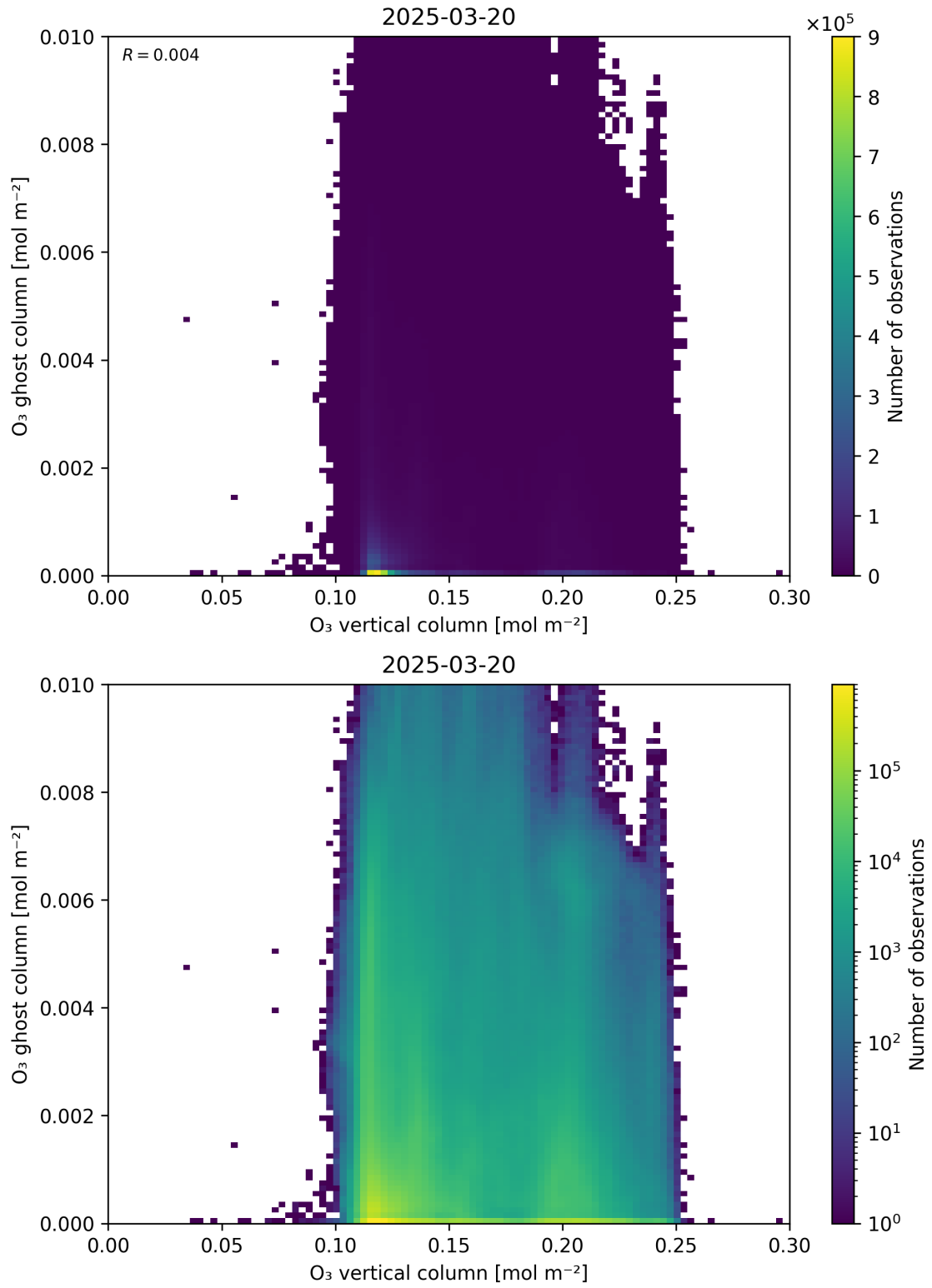
Figure 40: Scatter density plot of “O 3 vertical column” against “O 3 ghost column” for 2025-03-19 to 2025-03-21.
