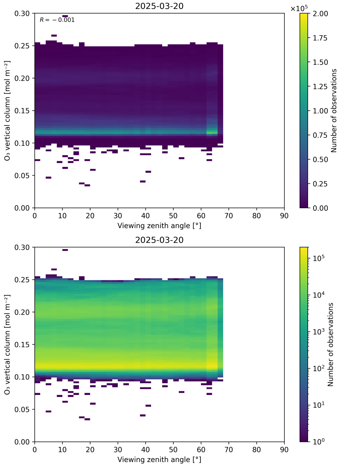
Figure 52: Scatter density plot of “Viewing zenith angle” against “O 3 vertical column” for 2025-03-19 to 2025-03-21.
