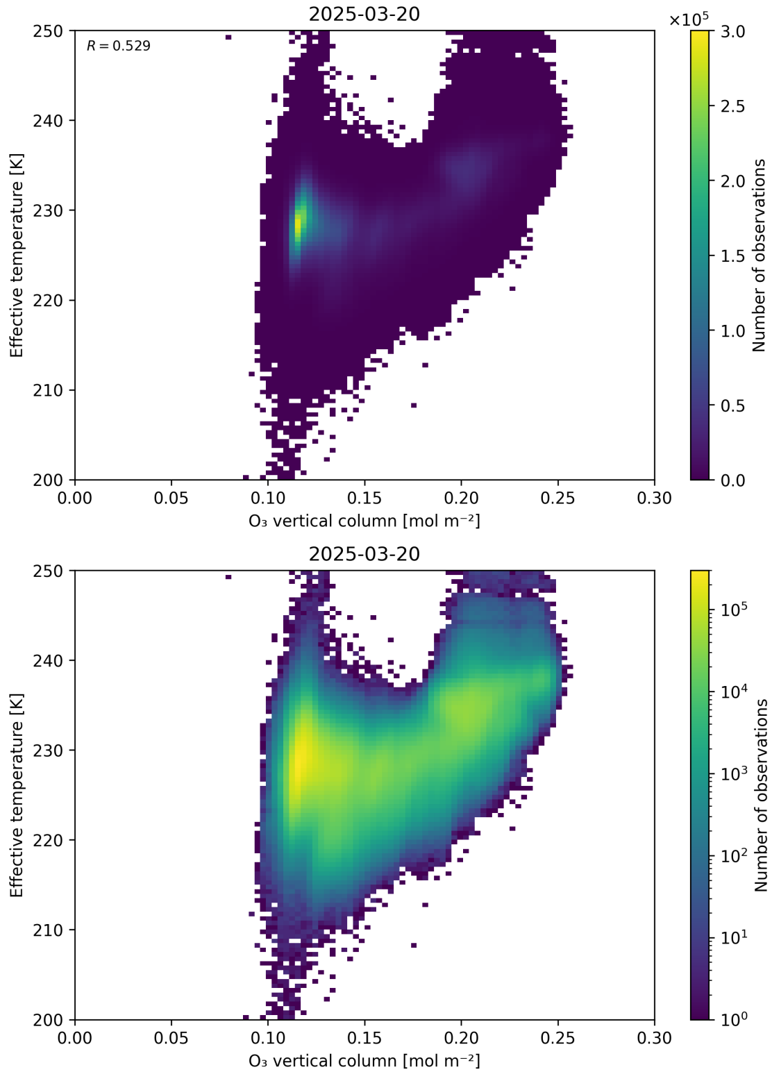
Figure 39: Scatter density plot of “O 3 vertical column” against “Effective temperature” for 2025-03-19 to 2025-03-21.
