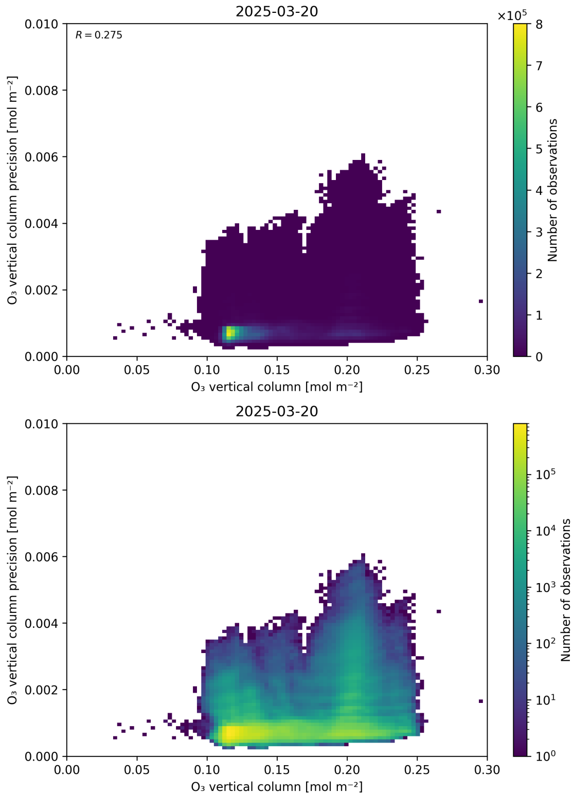
Figure 41: Scatter density plot of “O 3 vertical column” against “O 3 vertical column precision” for 2025-03-19 to 2025-03-21.
