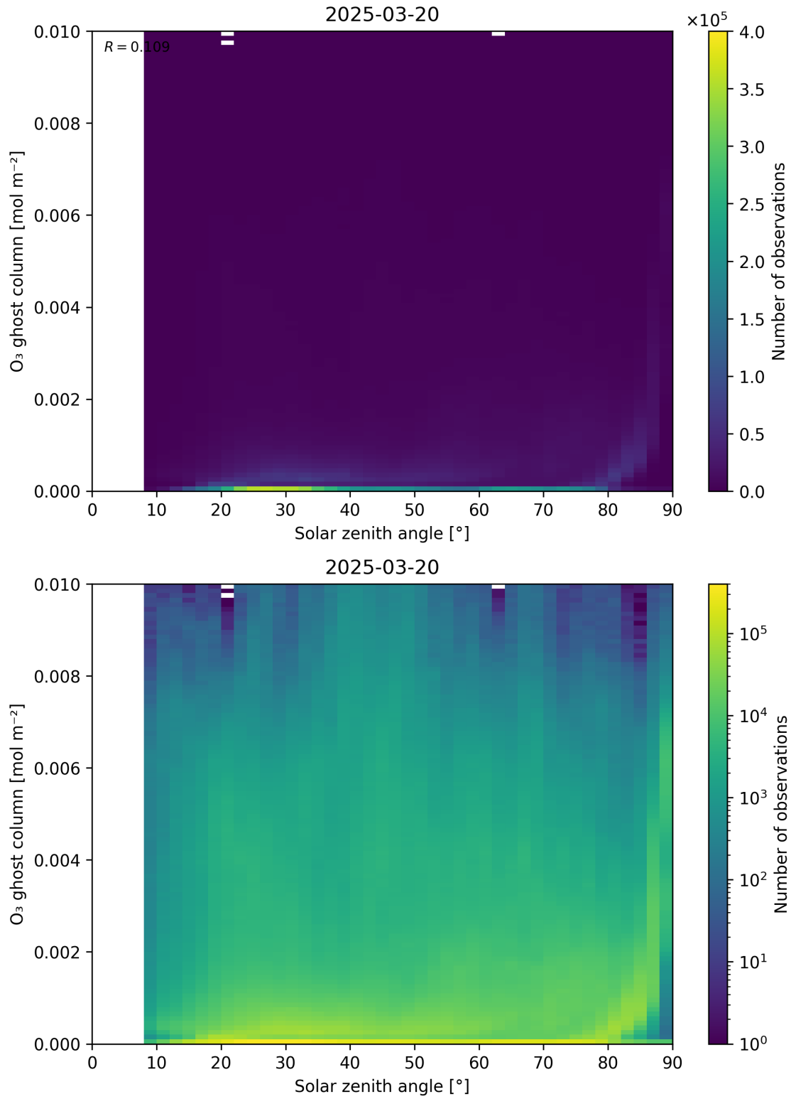
Figure 46: Scatter density plot of “Solar zenith angle” against “O 3 ghost column” for 2025-03-19 to 2025-03-21.
