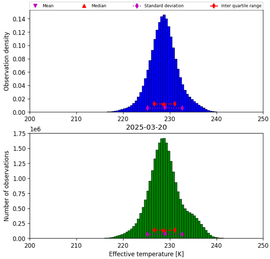
Figure 24: Histogram of “Effective temperature” for 2025-03-19 to 2025-03-21
