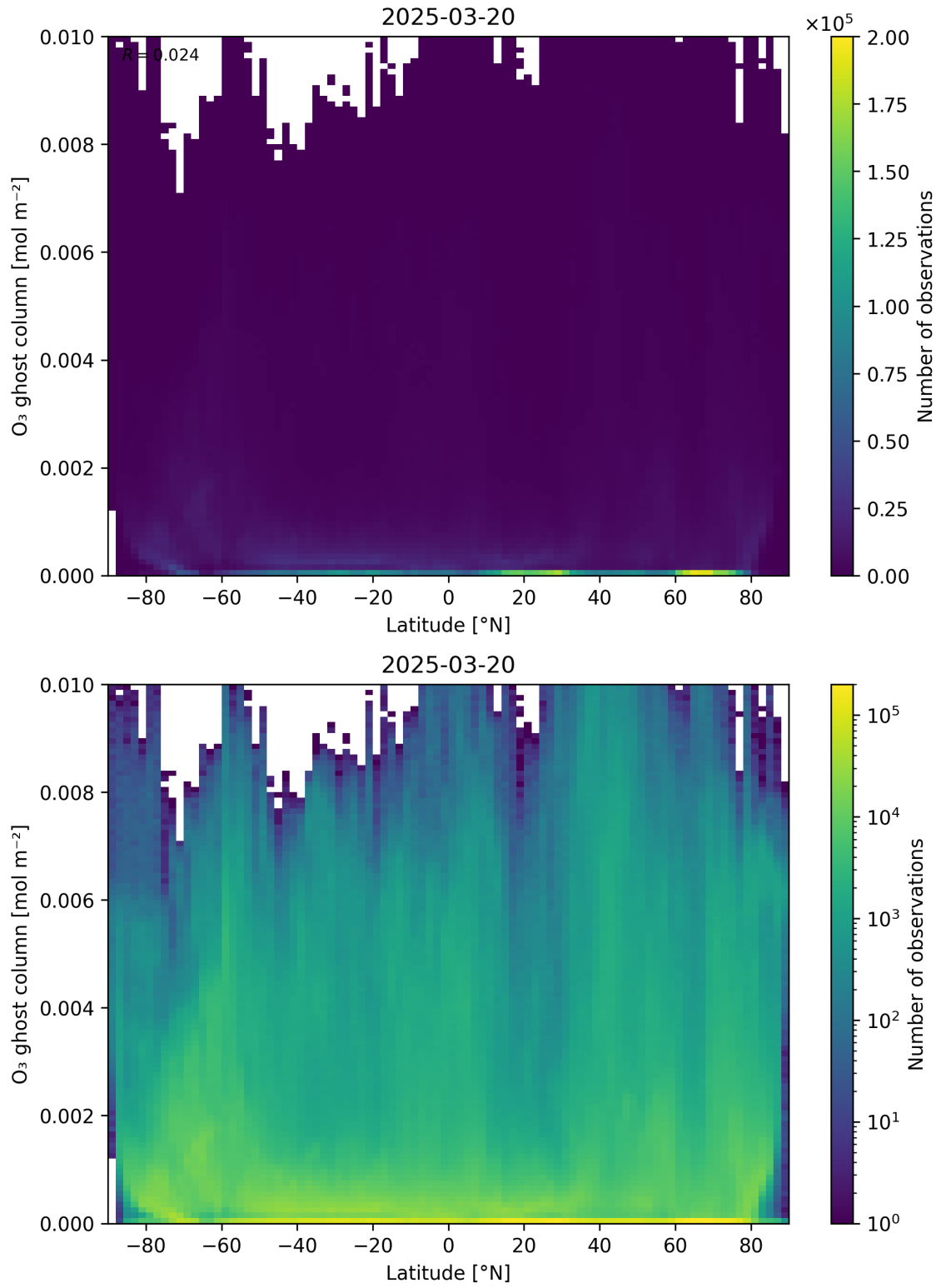
Figure 35: Scatter density plot of “Latitude” against “O 3 ghost column” for 2025-03-19 to 2025-03-21.
