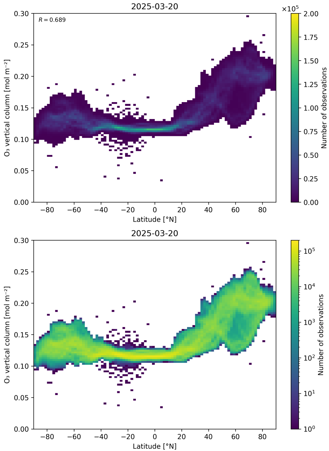
Figure 36: Scatter density plot of “Latitude” against “O 3 vertical column” for 2025-03-19 to 2025-03-21.
