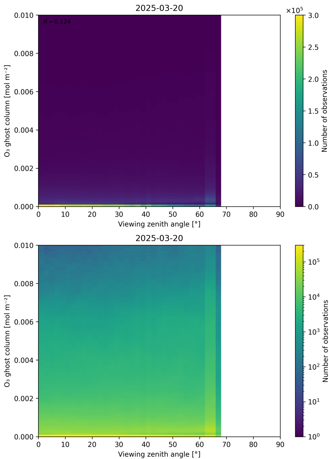
Figure 51: Scatter density plot of “Viewing zenith angle” against “O 3 ghost column” for 2025-03-19 to 2025-03-21.
