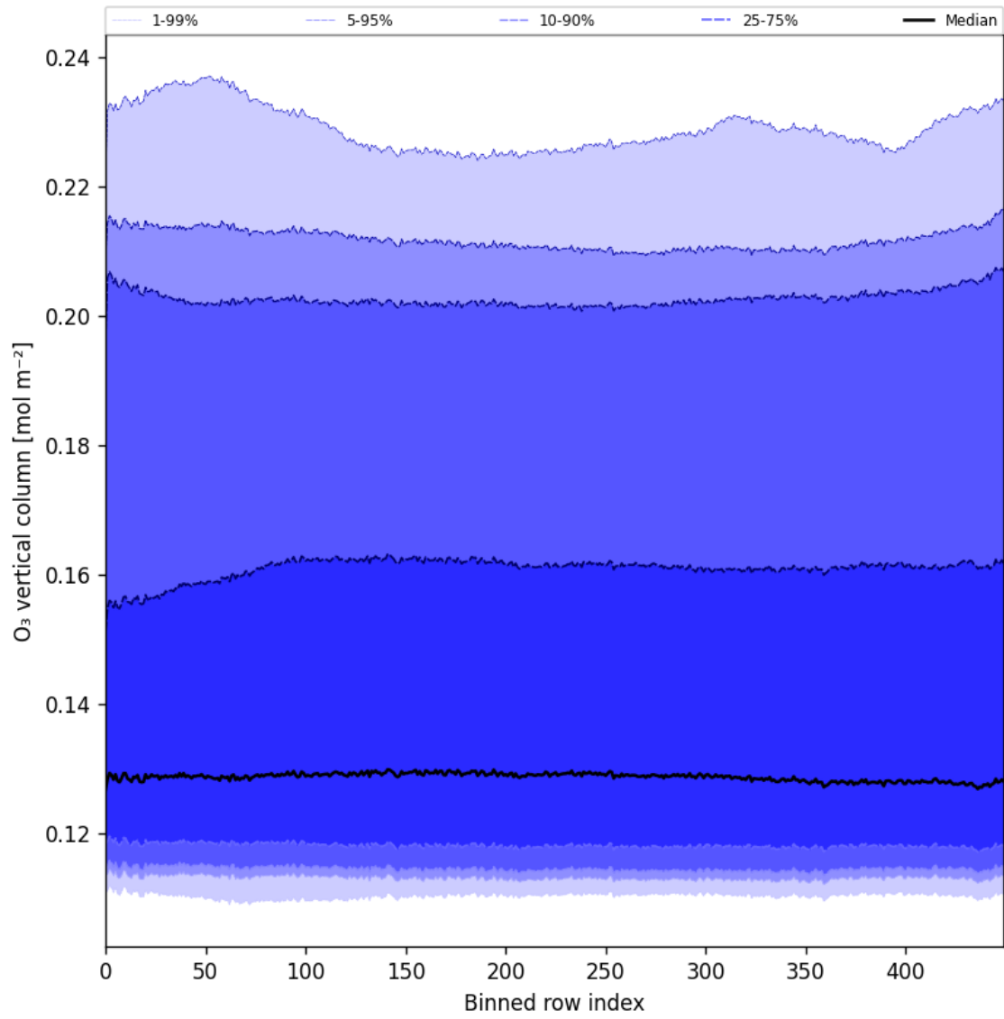
Figure 28: Along track statistics of “O 3 vertical column” for 2025-03-19 to 2025-03-21
