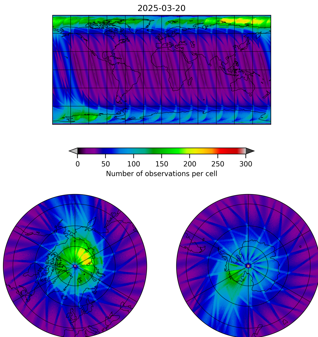
Figure 12: Map of the number of observations for 2025-03-19 to 2025-03-21
