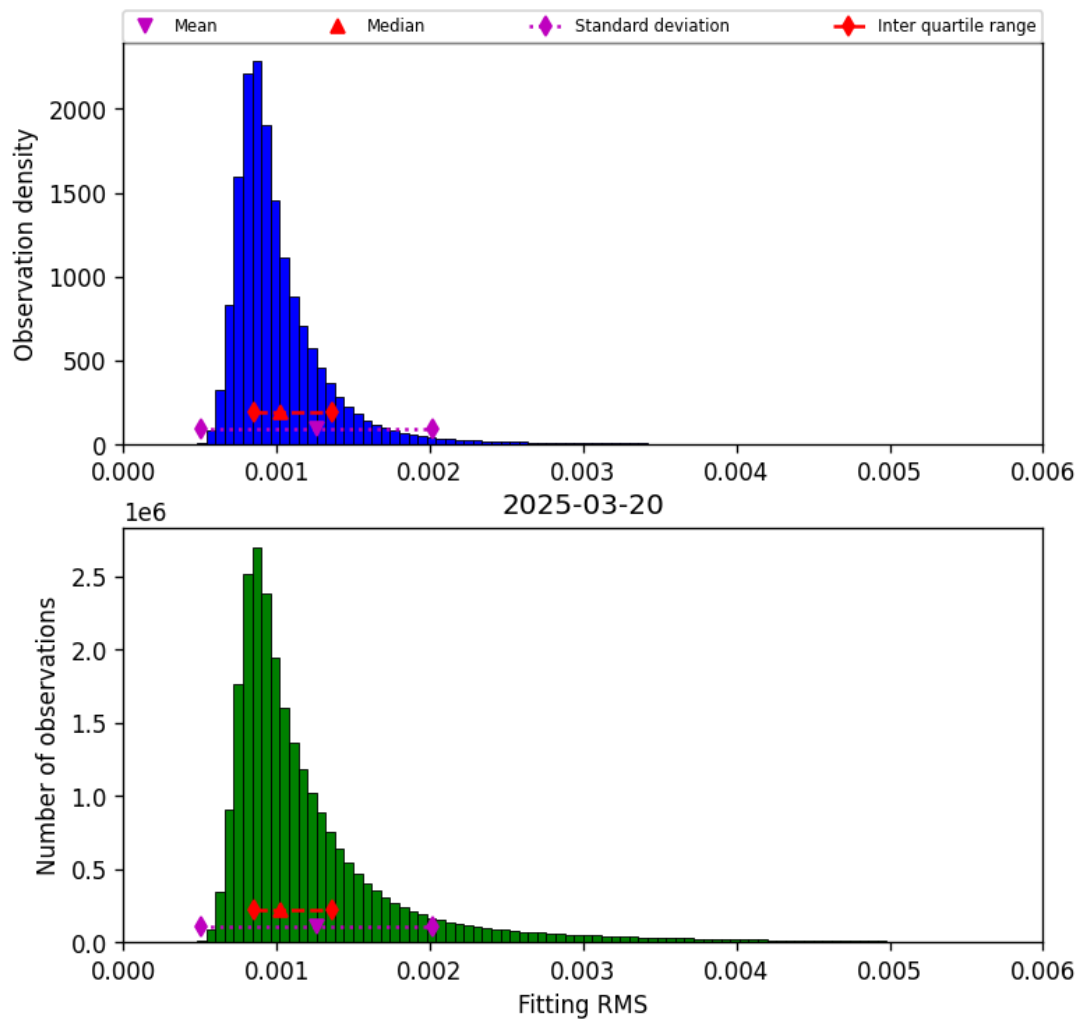
Figure 23: Histogram of “Fitting RMS” for 2025-03-19 to 2025-03-21
