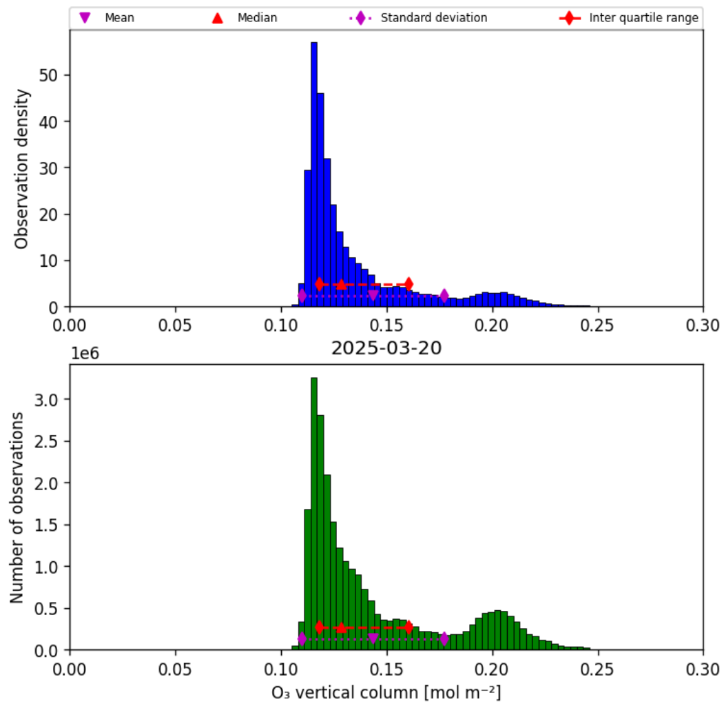
Figure 21: Histogram of “O 3 vertical column” for 2025-03-19 to 2025-03-21
