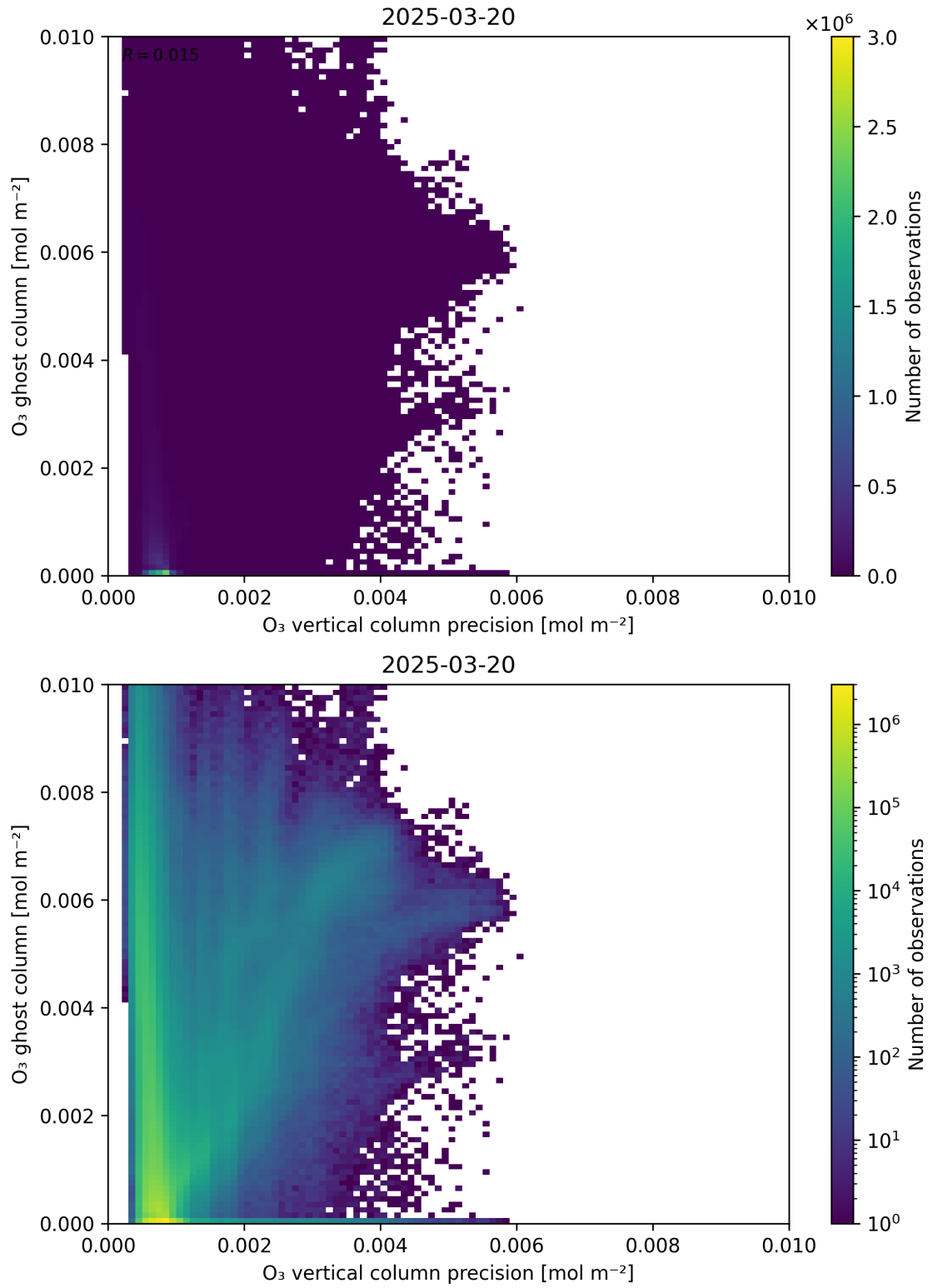
Figure 43: Scatter density plot of “O 3 vertical column precision” against “O 3 ghost column” for 2025-03-19 to 2025-03-21.
