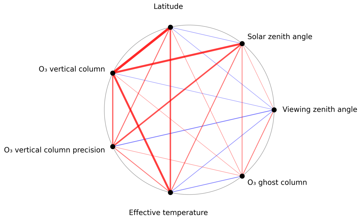
Figure 1: Map of correlation graph for 2025-03-19 to 2025-03-21.
