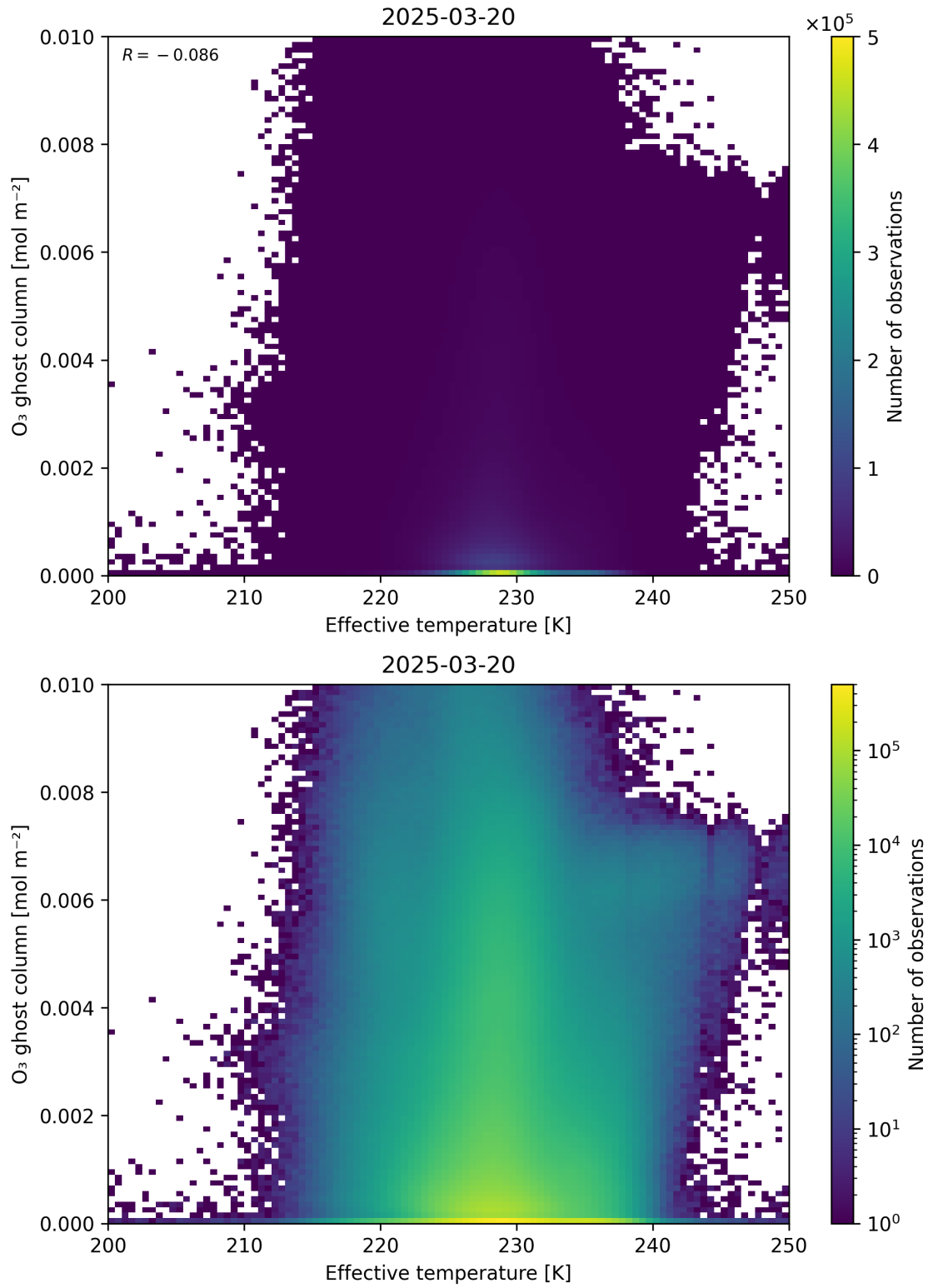
Figure 38: Scatter density plot of “Effective temperature” against “O 3 ghost column” for 2025-03-19 to 2025-03-21.
