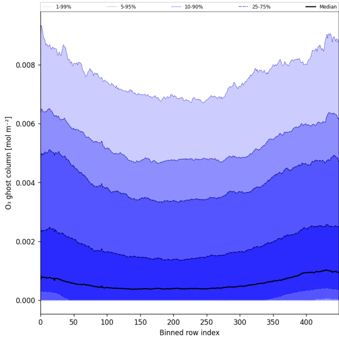
Figure 32: Along track statistics of “O 3 ghost column” for 2025-03-19 to 2025-03-21
