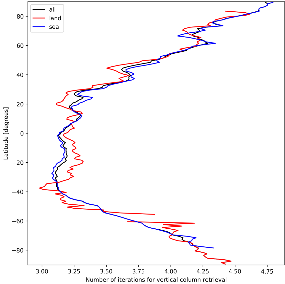
Figure 19: Zonal average of “Number of iterations for vertical column retrieval” for 2025-03-19 to 2025-03-21.
