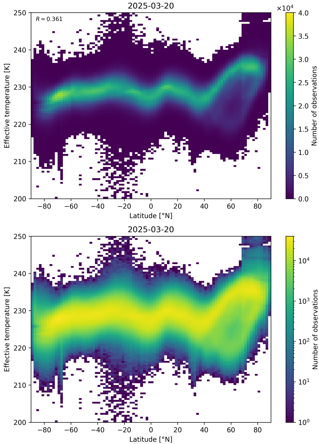
Figure 34: Scatter density plot of “Latitude” against “Effective temperature” for 2025-03-19 to 2025-03-21.
