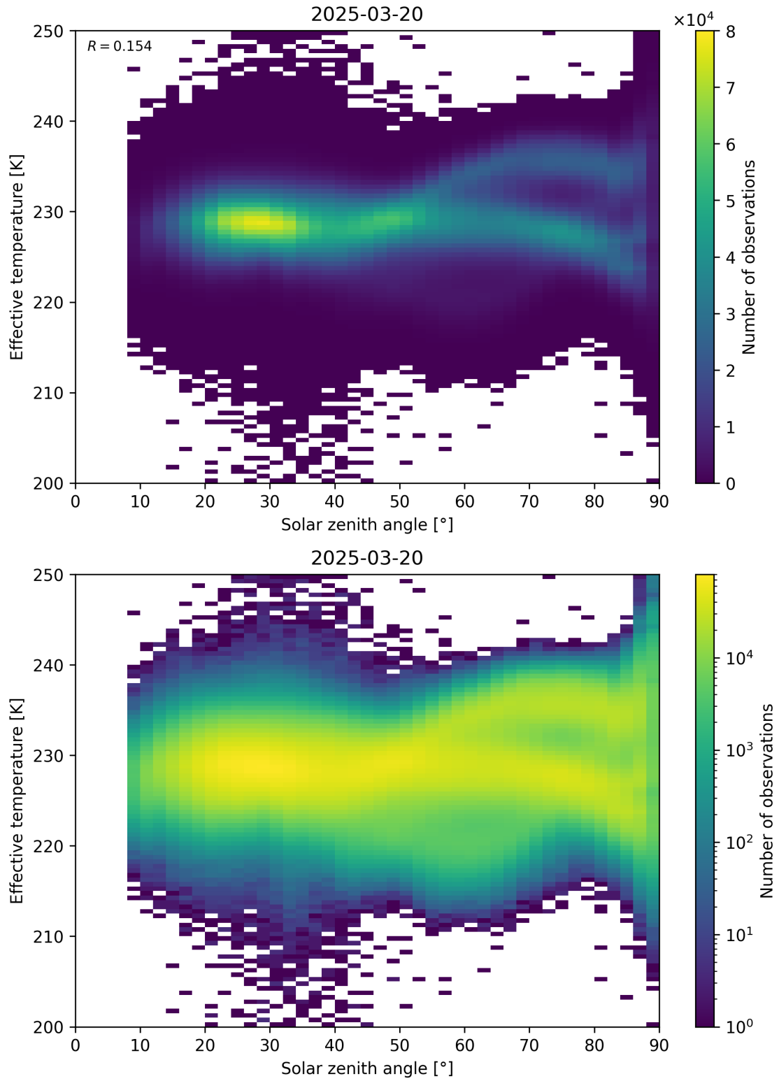
Figure 45: Scatter density plot of “Solar zenith angle” against “Effective temperature” for 2025-03-19 to 2025-03-21.
