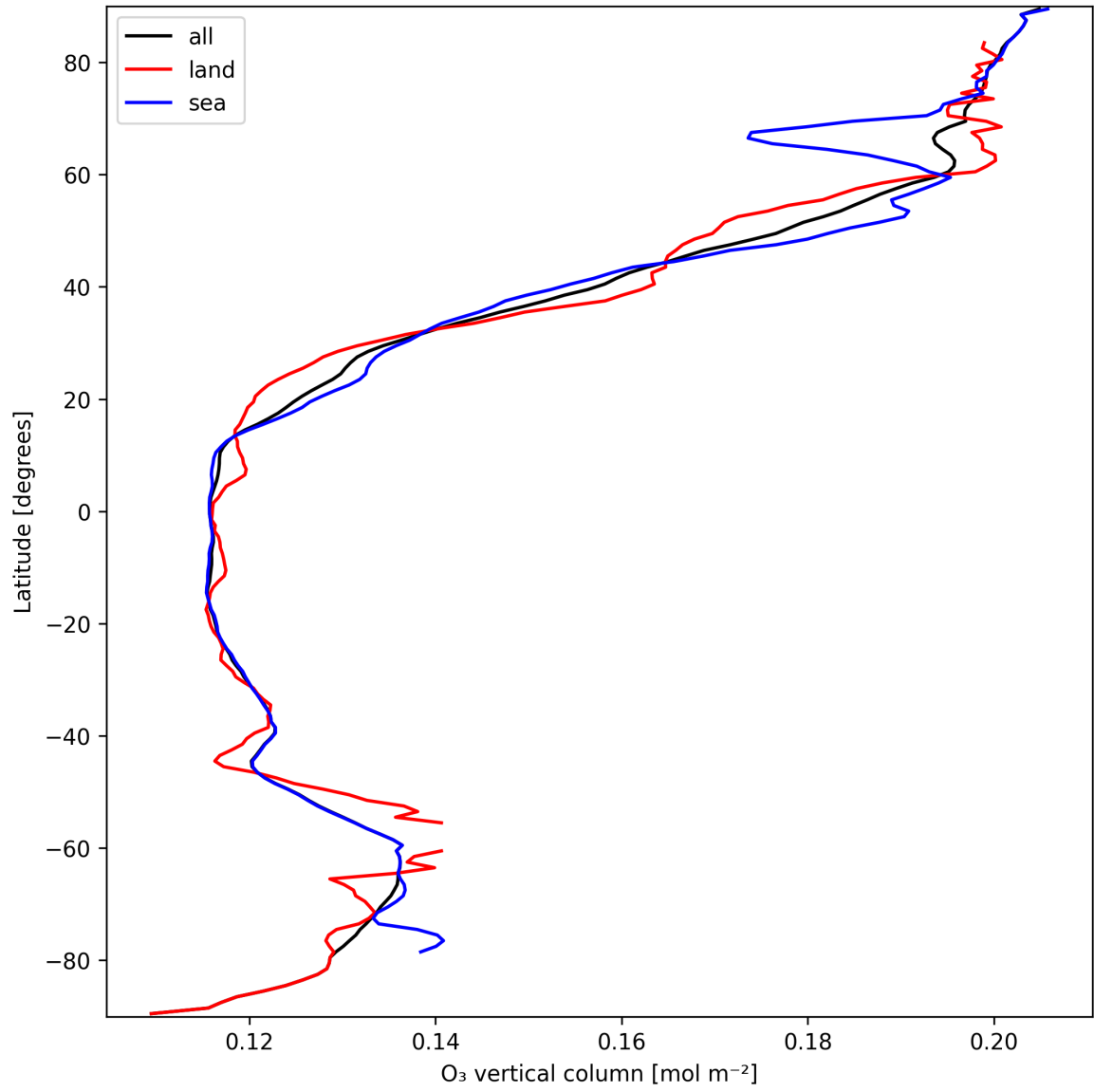
Figure 14: Zonal average of “O 3 vertical column” for 2025-03-19 to 2025-03-21.
