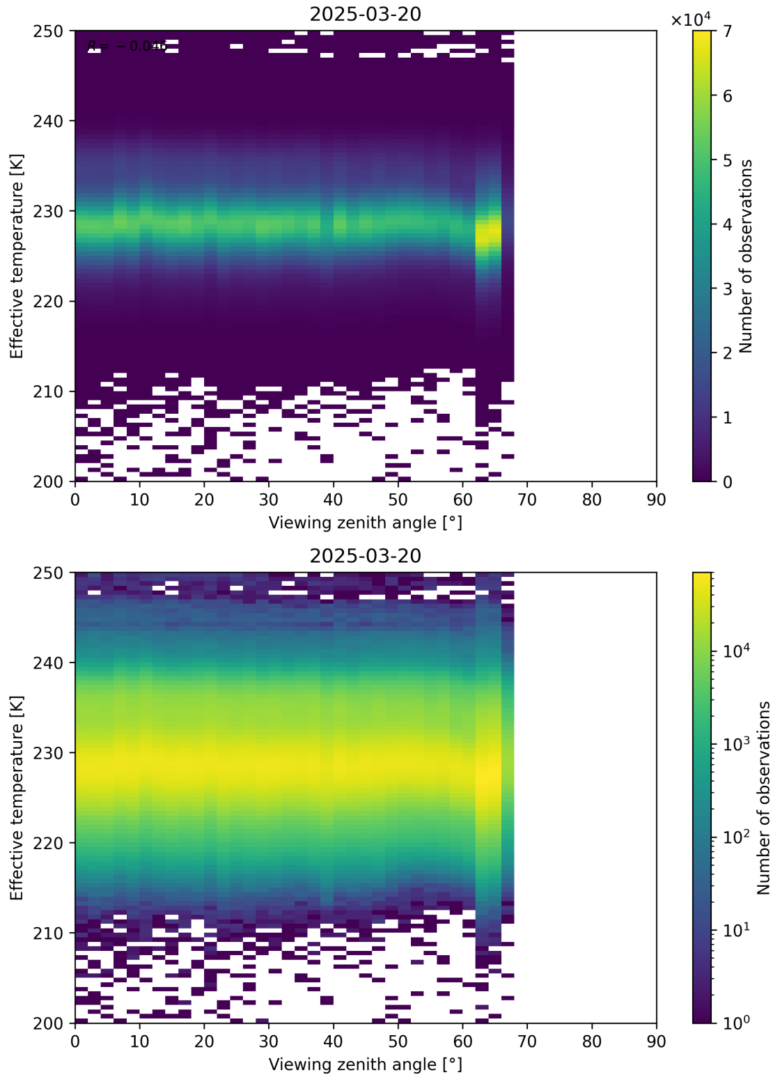
Figure 50: Scatter density plot of “Viewing zenith angle” against “Effective temperature” for 2025-03-19 to 2025-03-21.
