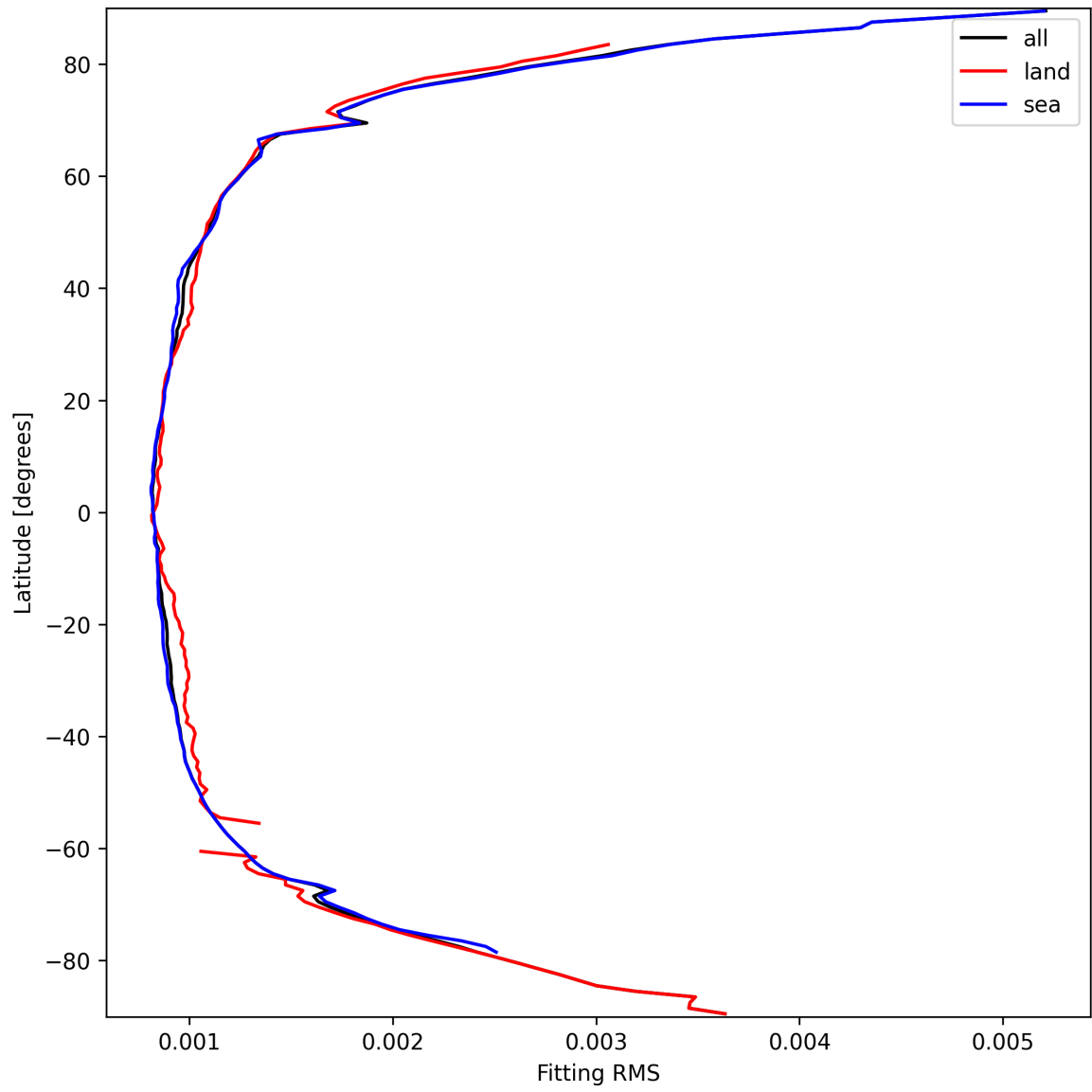
Figure 16: Zonal average of “Fitting RMS” for 2025-03-19 to 2025-03-21.
