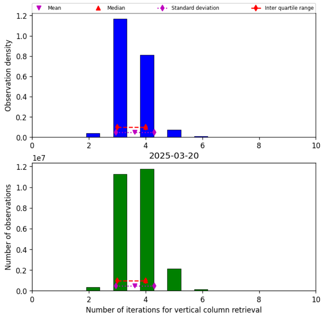
Figure 26: Histogram of “Number of iterations for vertical column retrieval” for 2025-03-19 to 2025-03-21
