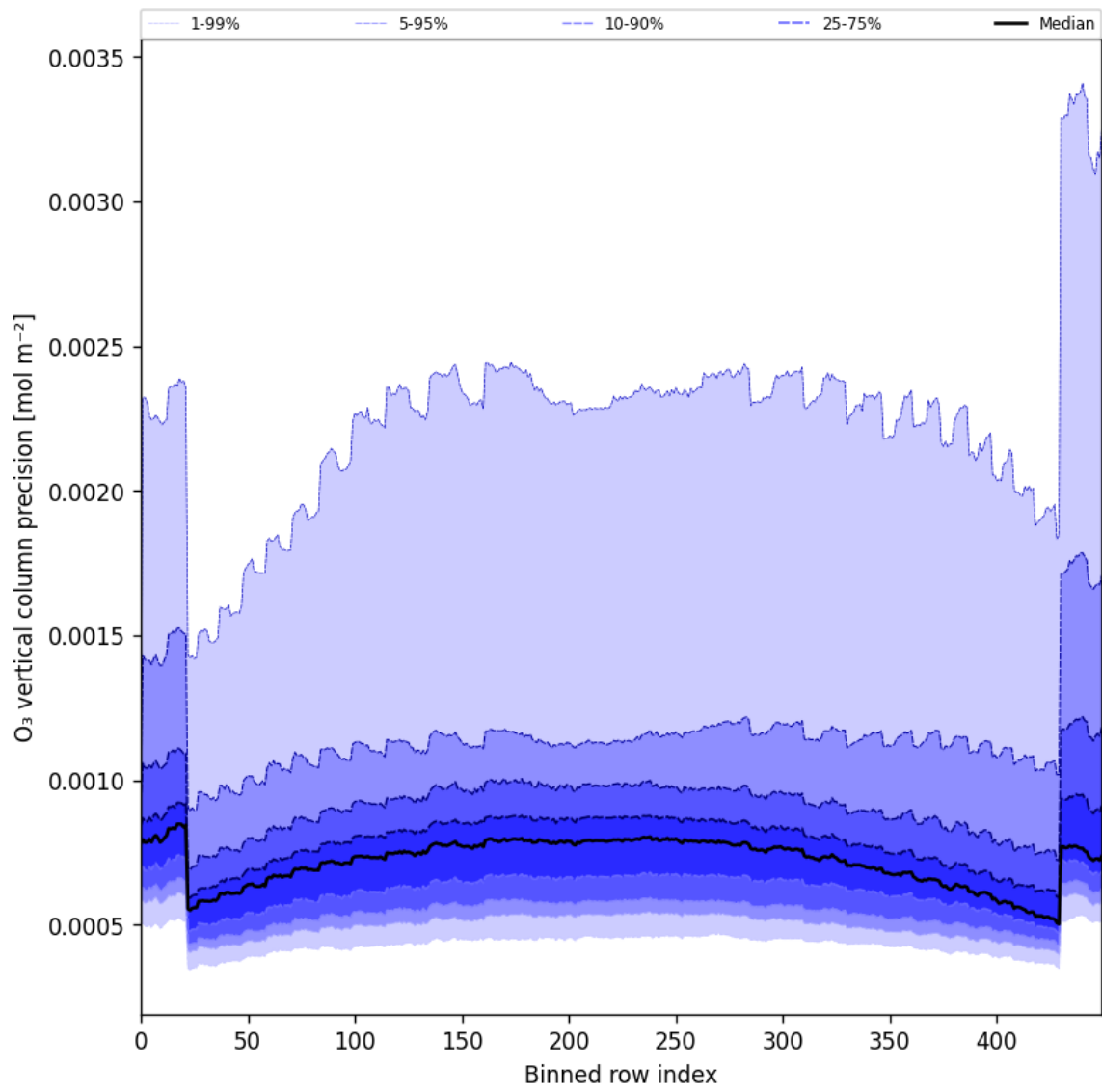
Figure 29: Along track statistics of “O 3 vertical column precision” for 2025-03-19 to 2025-03-21
