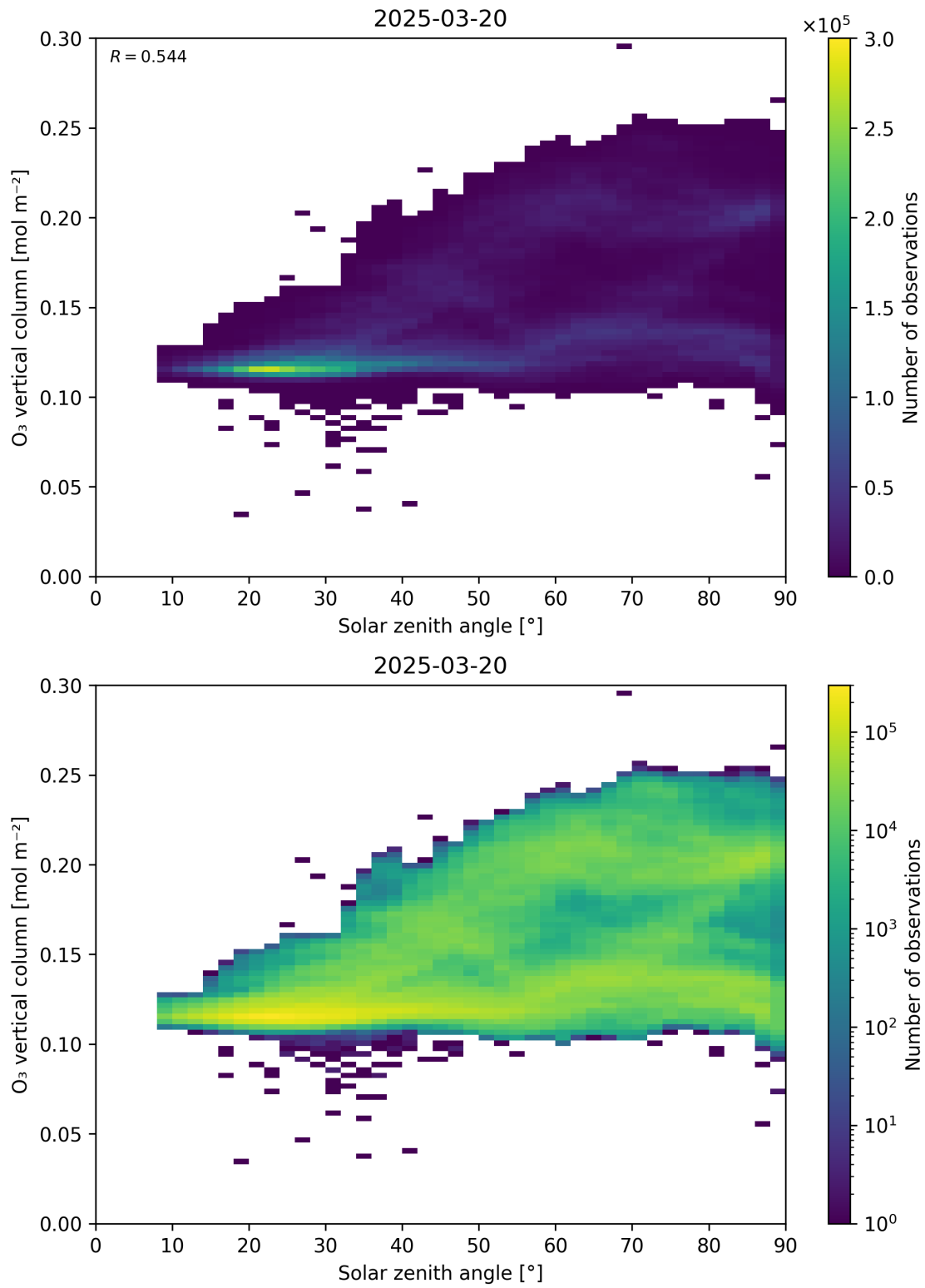
Figure 47: Scatter density plot of “Solar zenith angle” against “O 3 vertical column” for 2025-03-19 to 2025-03-21.
