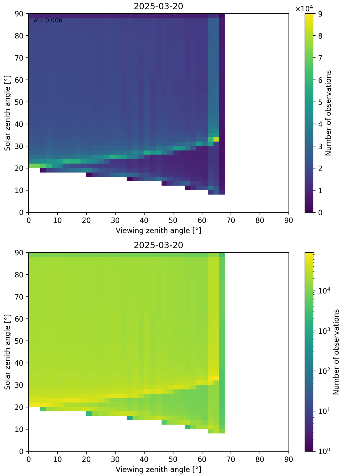
Figure 54: Scatter density plot of “Viewing zenith angle” against “Solar zenith angle” for 2025-03-19 to 2025-03-21.
