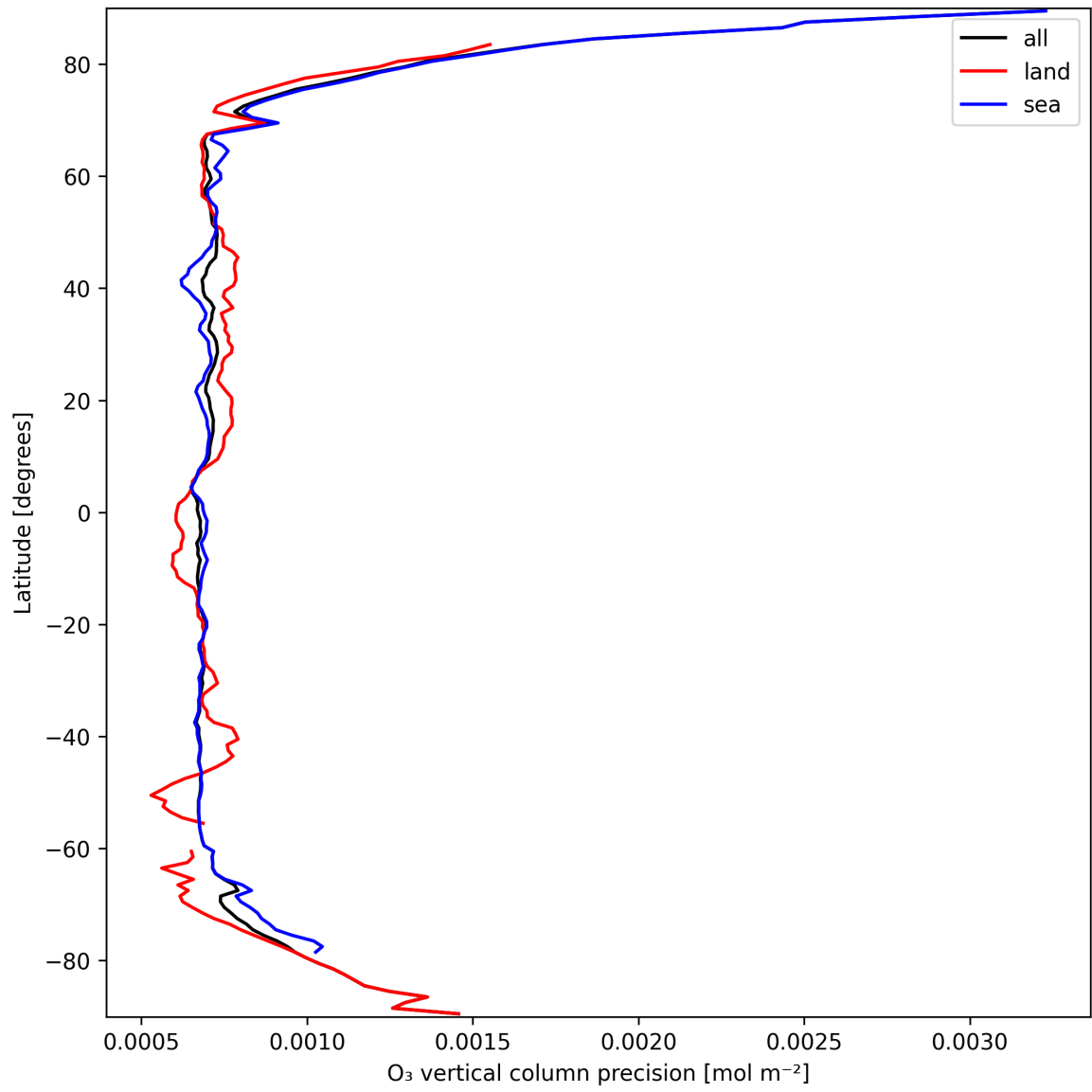
Figure 15: Zonal average of “O 3 vertical column precision” for 2025-03-19 to 2025-03-21.
