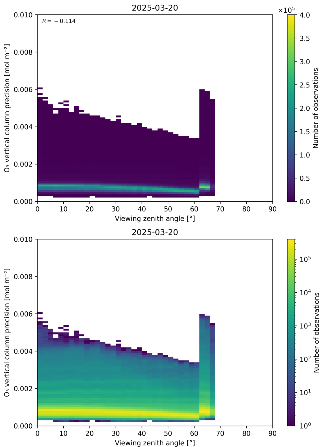
Figure 53: Scatter density plot of “Viewing zenith angle” against “O 3 vertical column precision” for 2025-03-19 to 2025-03-21.
