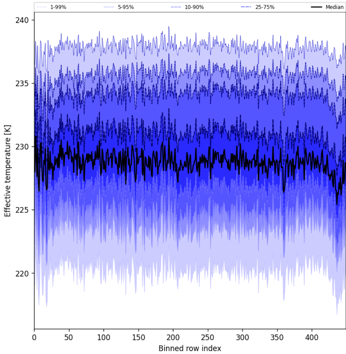
Figure 31: Along track statistics of “Effective temperature” for 2025-03-19 to 2025-03-21
