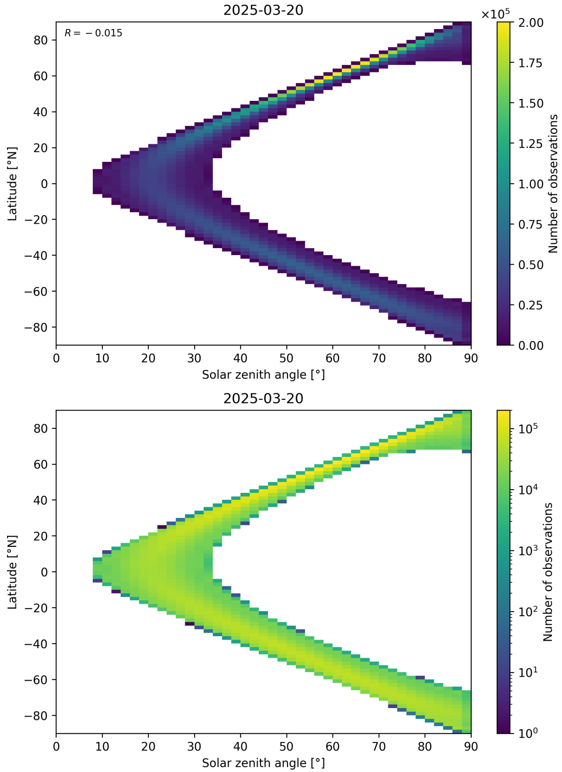
Figure 44: Scatter density plot of “Solar zenith angle” against “Latitude” for 2025-03-19 to 2025-03-21.
