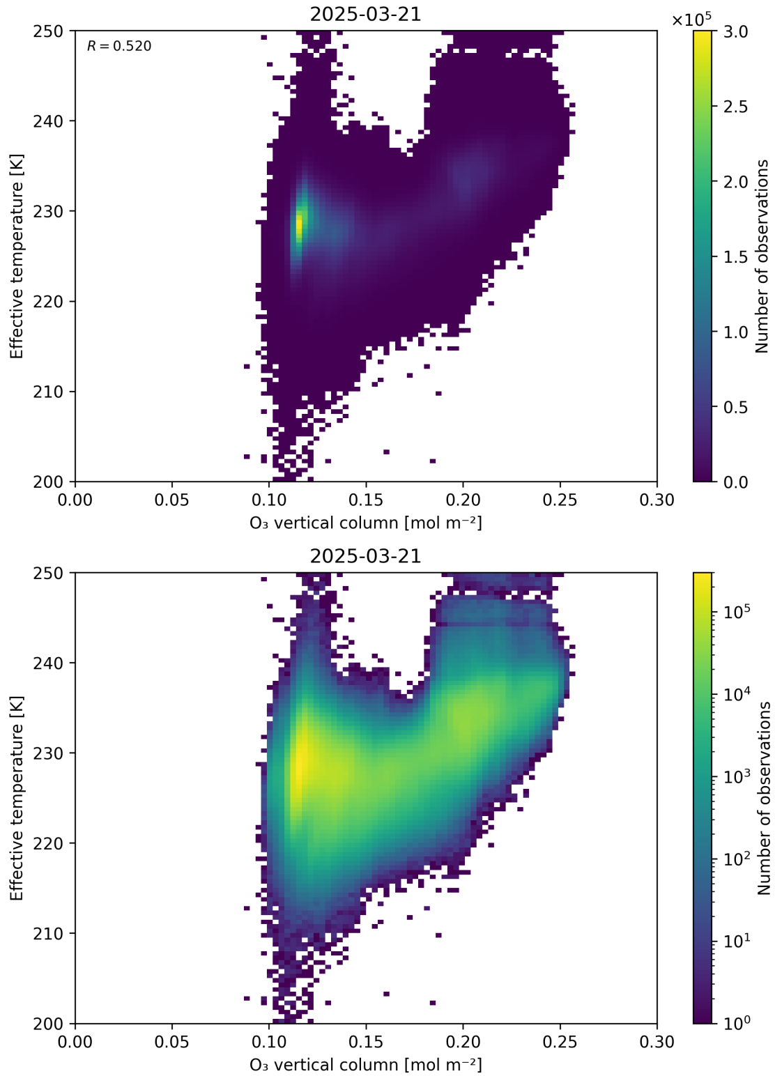
Figure 39: Scatter density plot of “O 3 vertical column” against “Effective temperature” for 2025-03-20 to 2025-03-22.
