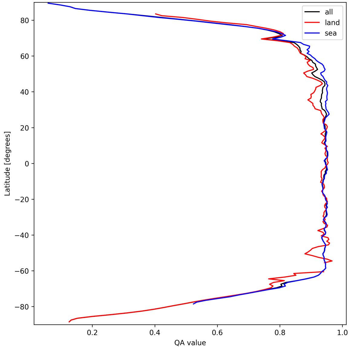
Figure 13: Zonal average of “QA value” for 2025-03-20 to 2025-03-22.
