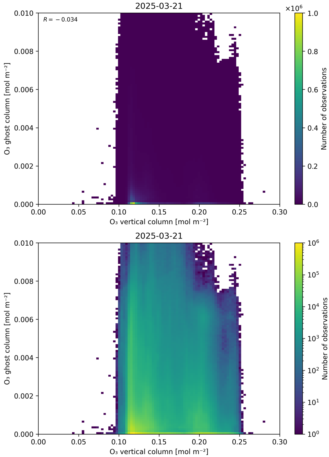
Figure 40: Scatter density plot of “O 3 vertical column” against “O 3 ghost column” for 2025-03-20 to 2025-03-22.
