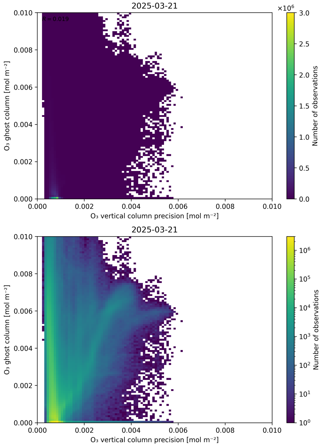
Figure 43: Scatter density plot of “ O_3 vertical column precision” against “ O_3 ghost column” for 2025-03-20 to 2025-03-22.
