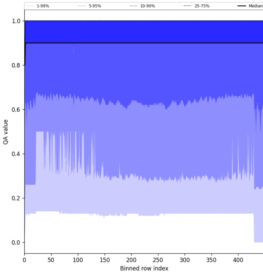
Figure 27: Along track statistics of “QA value” for 2025-03-20 to 2025-03-22
