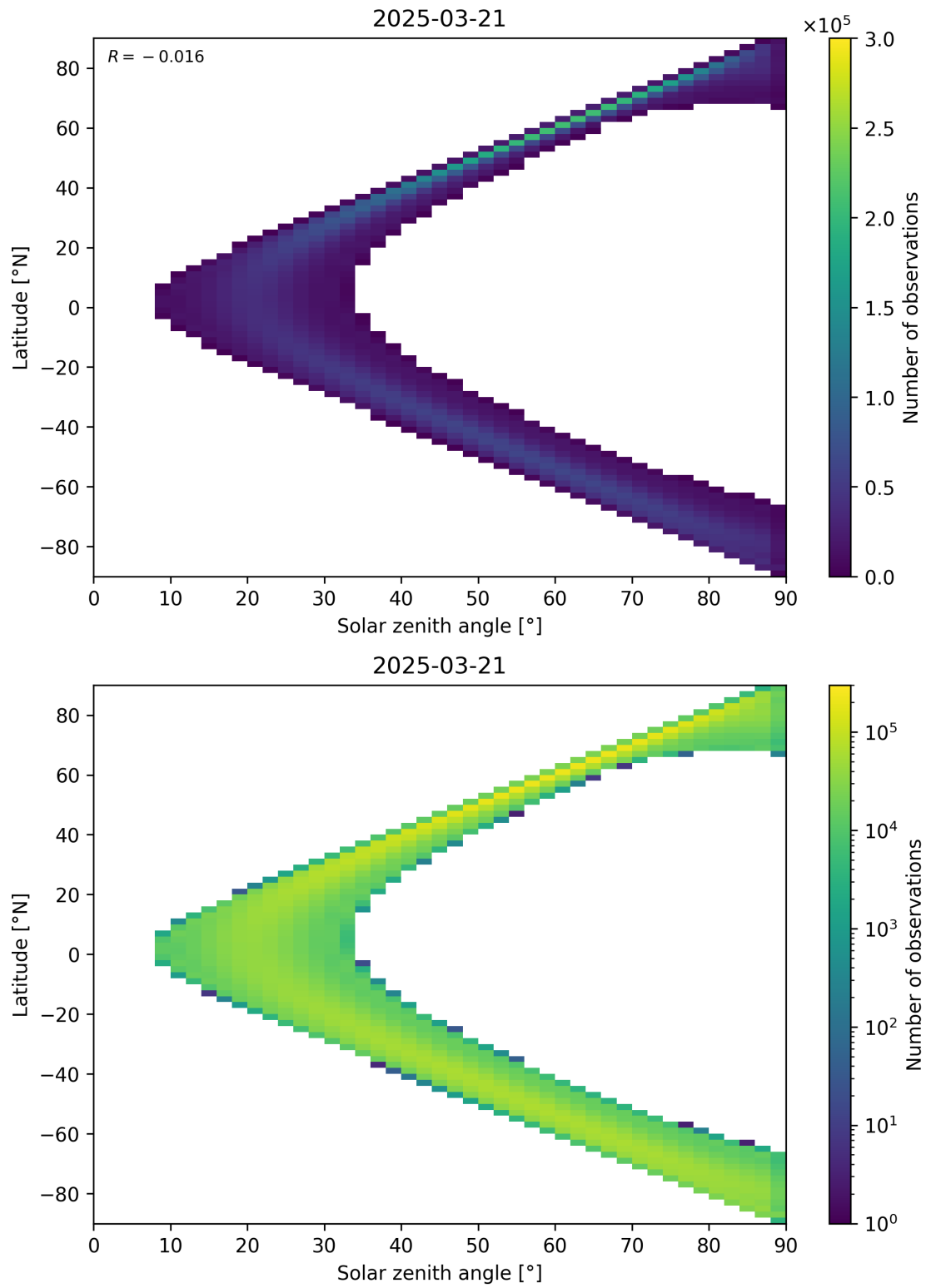
Figure 44: Scatter density plot of “Solar zenith angle” against “Latitude” for 2025-03-20 to 2025-03-22.
