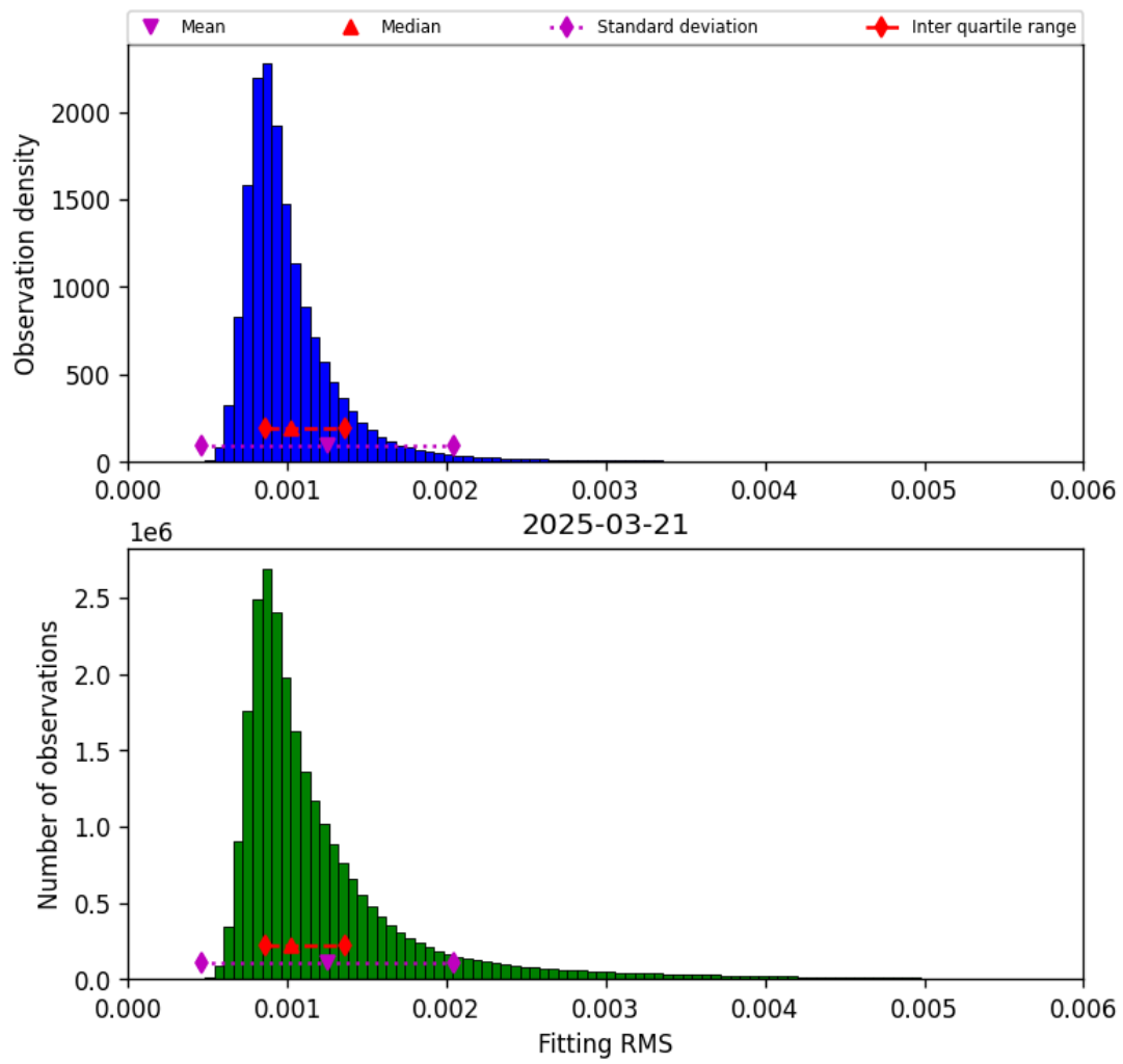
Figure 23: Histogram of “Fitting RMS” for 2025-03-20 to 2025-03-22
