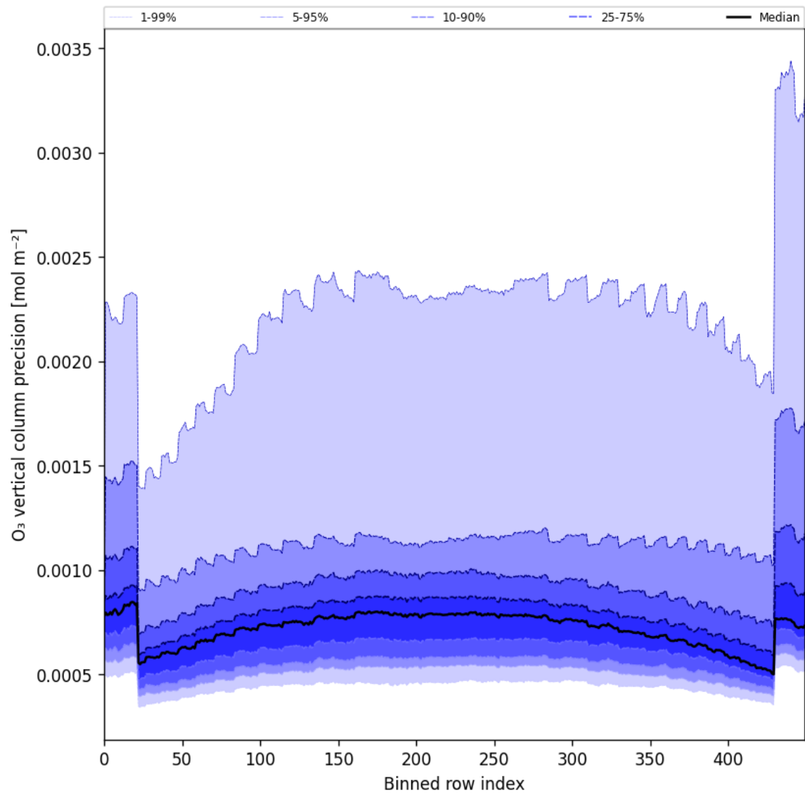
Figure 29: Along track statistics of “O 3 vertical column precision” for 2025-03-20 to 2025-03-22
