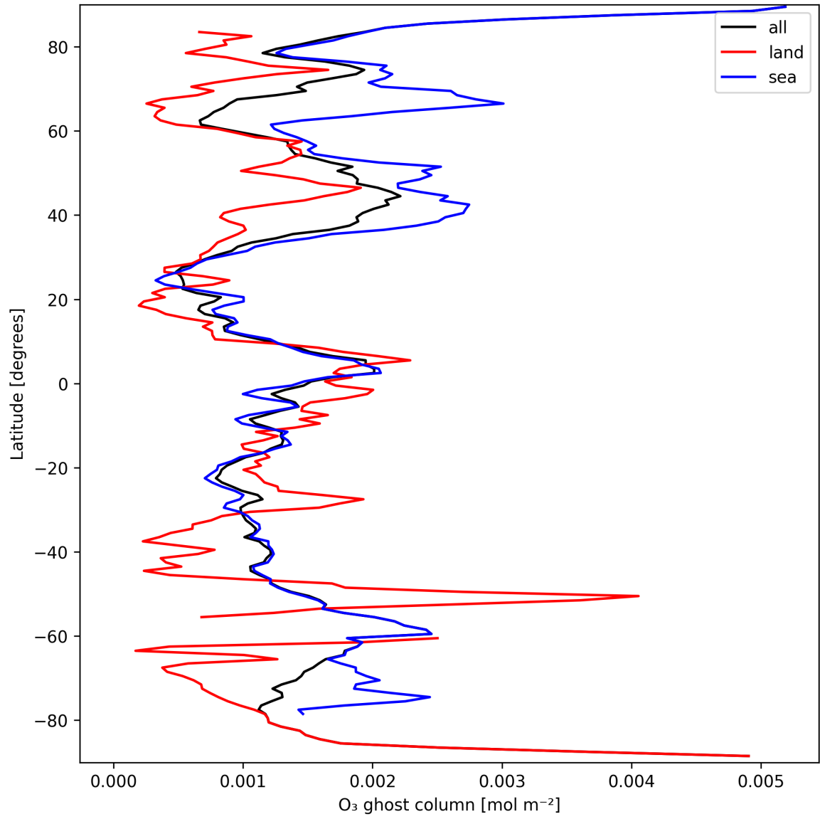
Figure 18: Zonal average of “O 3 ghost column” for 2025-03-20 to 2025-03-22.
