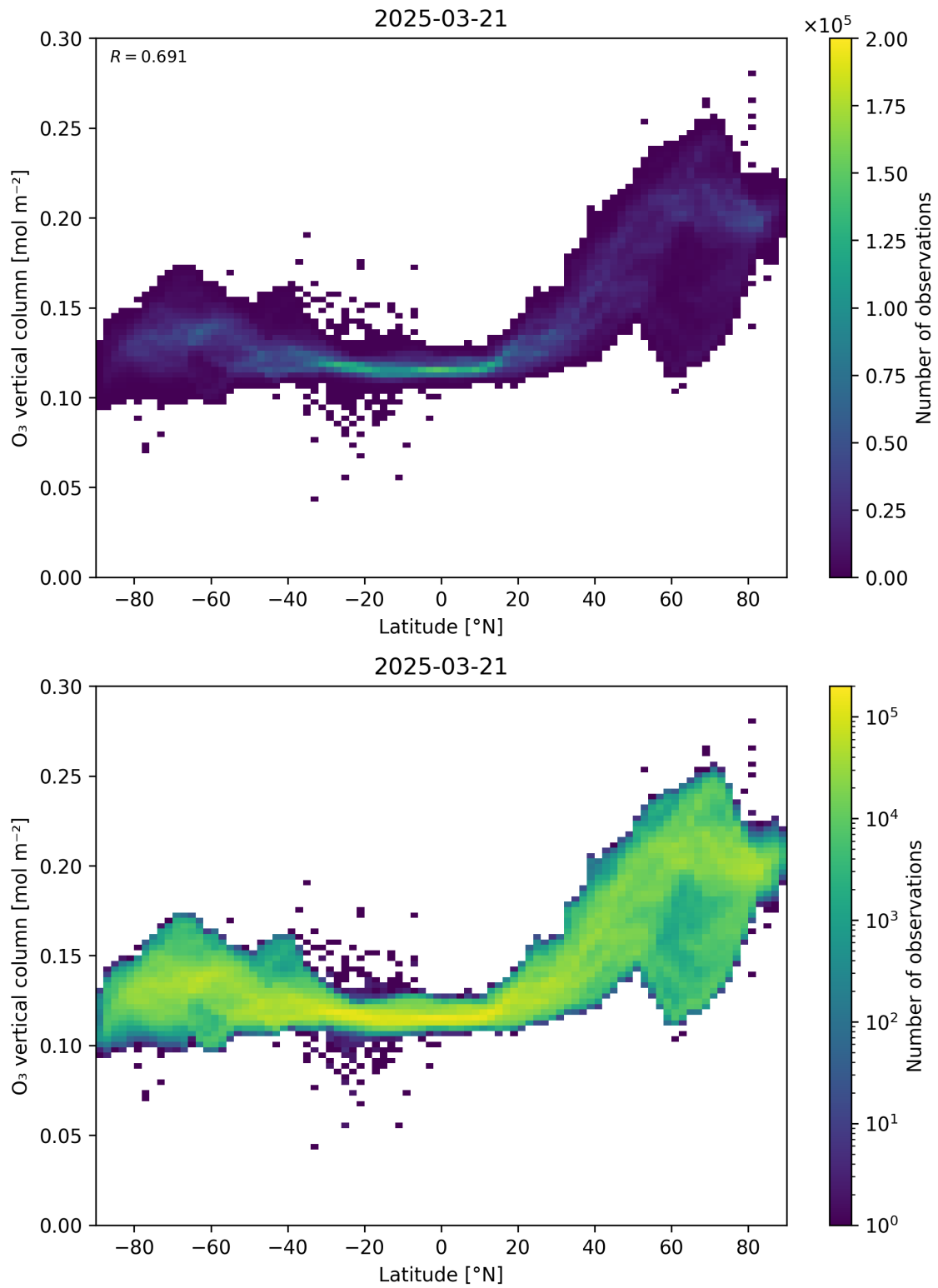
Figure 36: Scatter density plot of “Latitude” against “O 3 vertical column” for 2025-03-20 to 2025-03-22.
