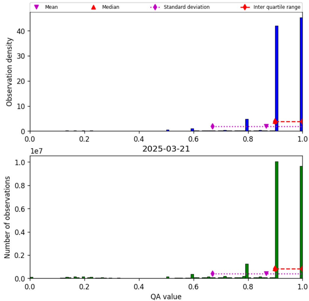
Figure 20: Histogram of “QA value” for 2025-03-20 to 2025-03-22
