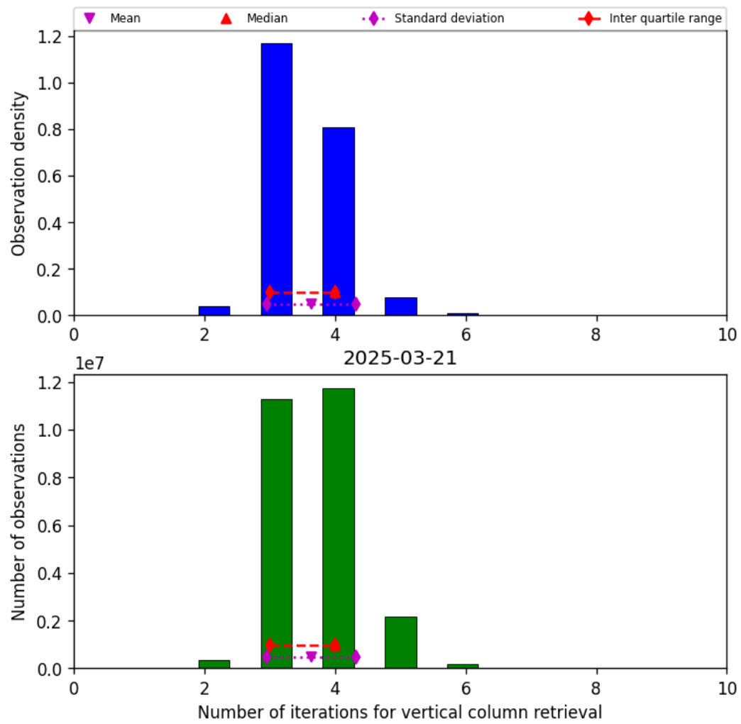
Figure 26: Histogram of “Number of iterations for vertical column retrieval” for 2025-03-20 to 2025-03-22
