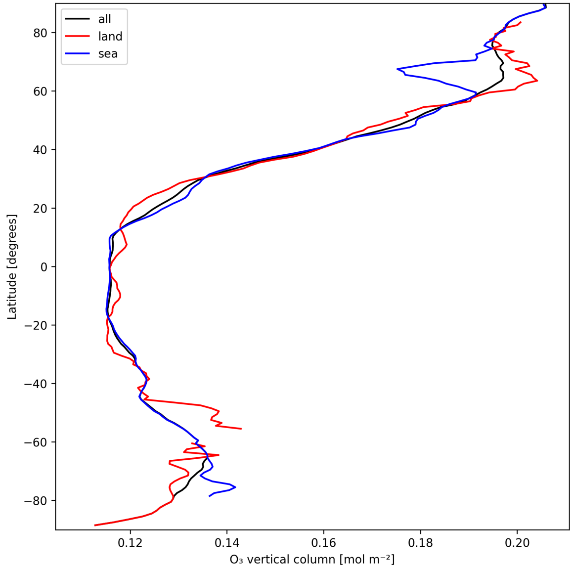
Figure 14: Zonal average of “O 3 vertical column” for 2025-03-20 to 2025-03-22.
