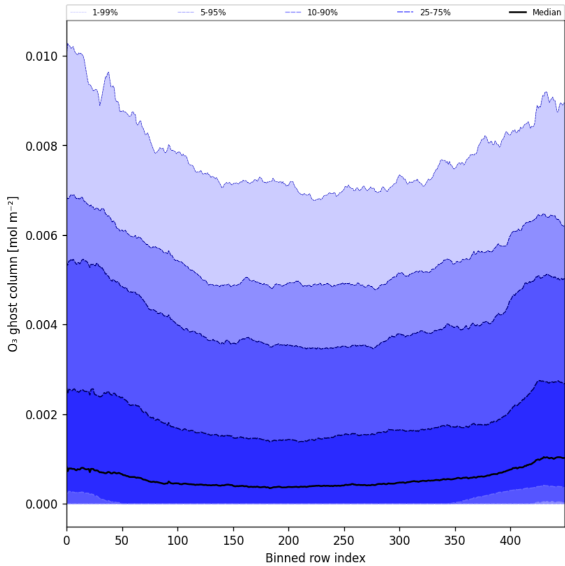
Figure 32: Along track statistics of “O 3 ghost column” for 2025-03-20 to 2025-03-22
