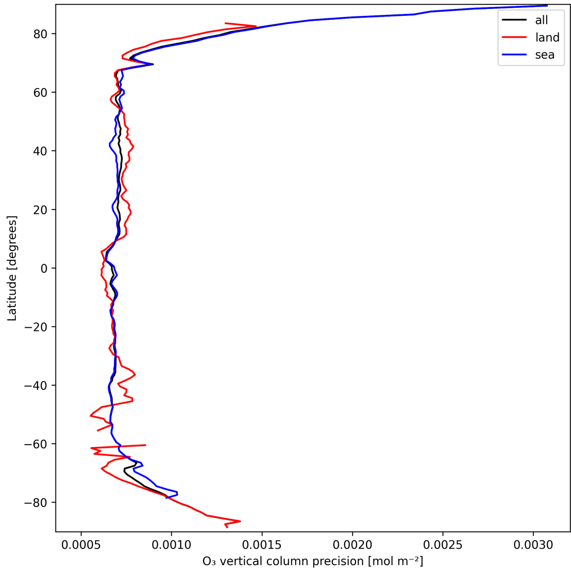
Figure 15: Zonal average of “O 3 vertical column precision” for 2025-03-20 to 2025-03-22.
