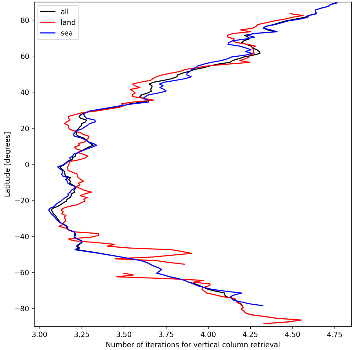
Figure 19: Zonal average of “Number of iterations for vertical column retrieval” for 2025-03-20 to 2025-03-22.
