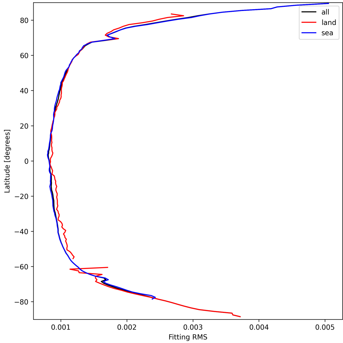
Figure 16: Zonal average of “Fitting RMS” for 2025-03-20 to 2025-03-22.
