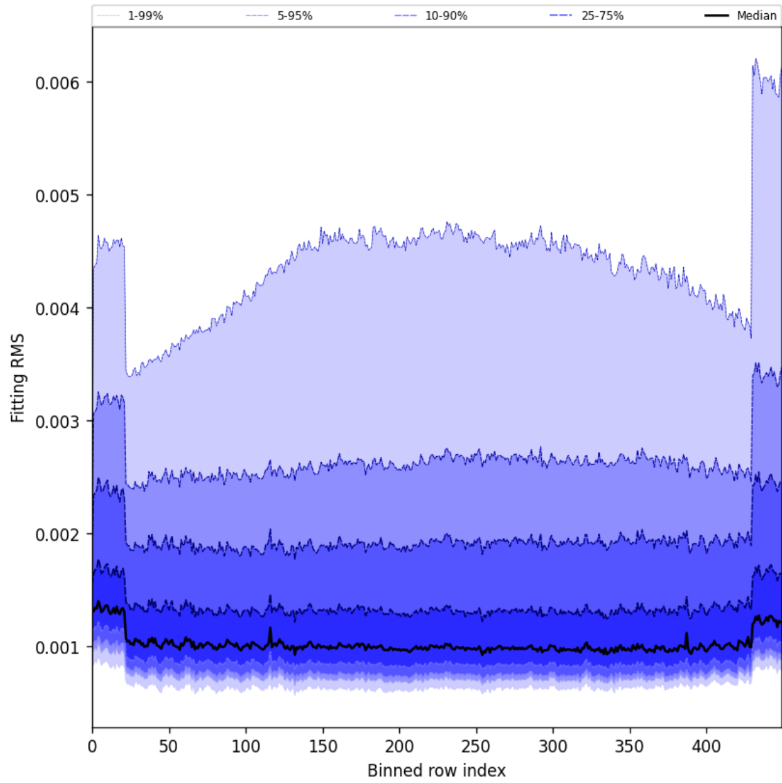
Figure 30: Along track statistics of “Fitting RMS” for 2025-03-20 to 2025-03-22
