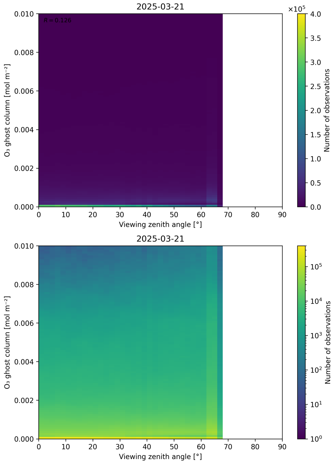
Figure 51: Scatter density plot of “Viewing zenith angle” against “O 3 ghost column” for 2025-03-20 to 2025-03-22.
