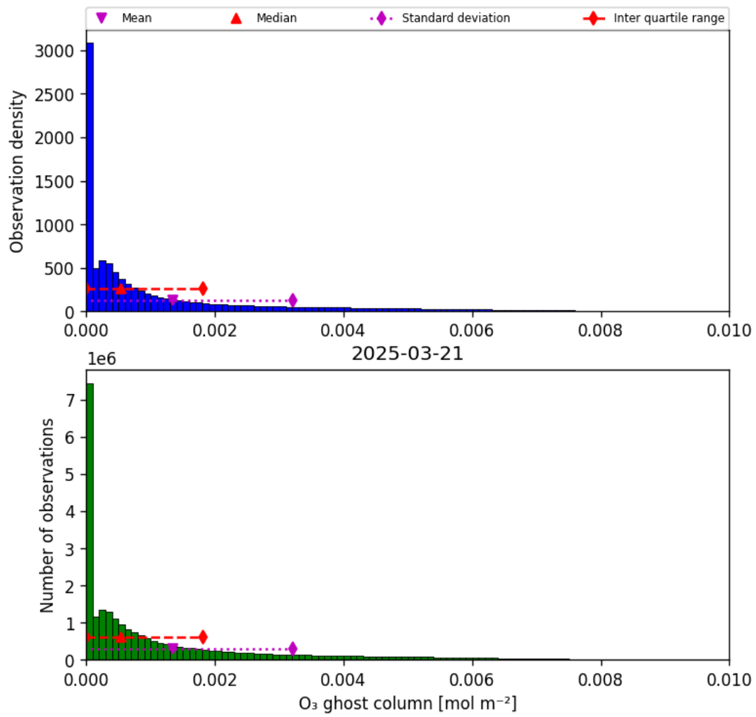
Figure 25: Histogram of “O 3 ghost column” for 2025-03-20 to 2025-03-22
