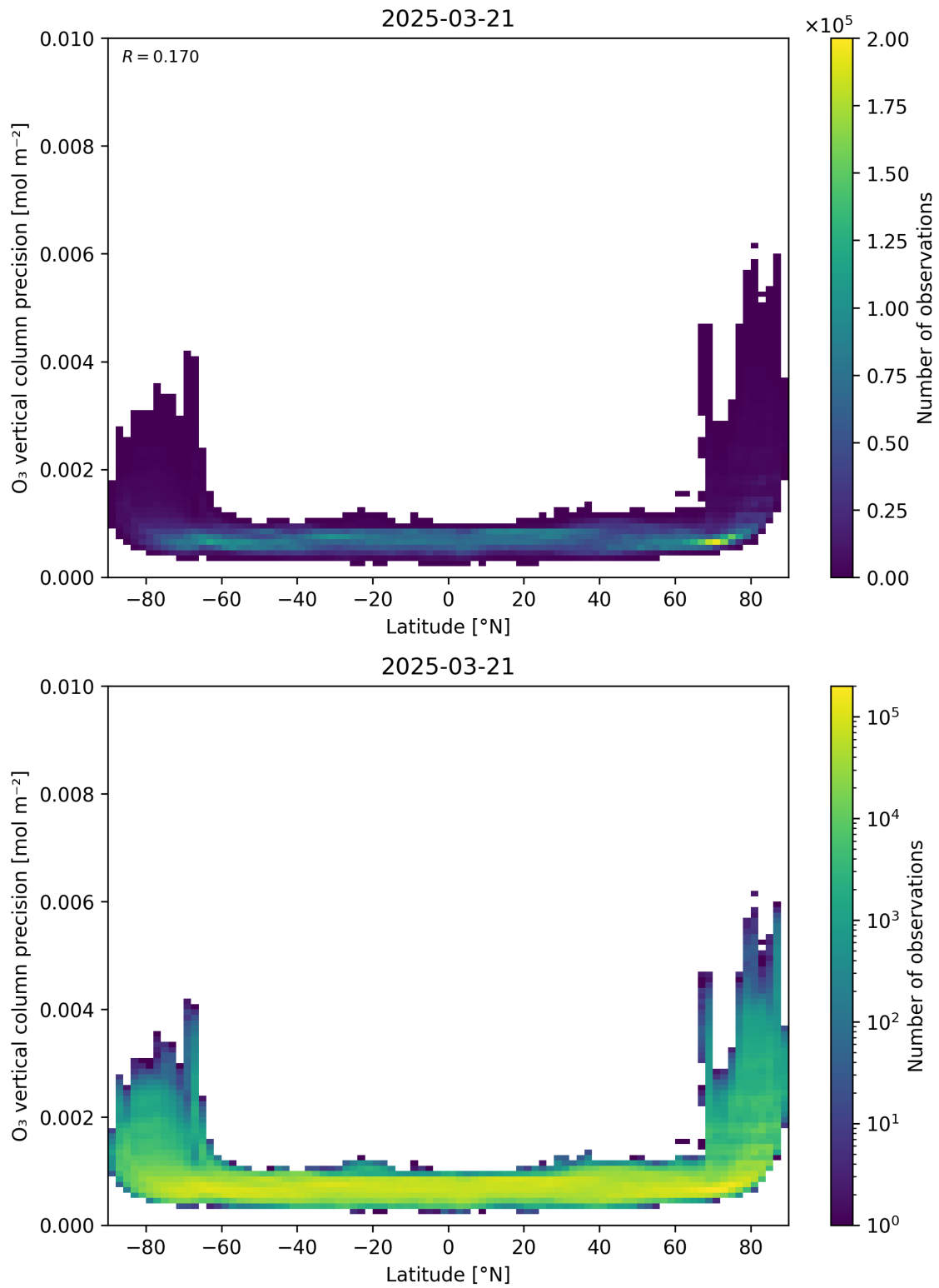
Figure 37: Scatter density plot of “Latitude” against “O 3 vertical column precision” for 2025-03-20 to 2025-03-22.
