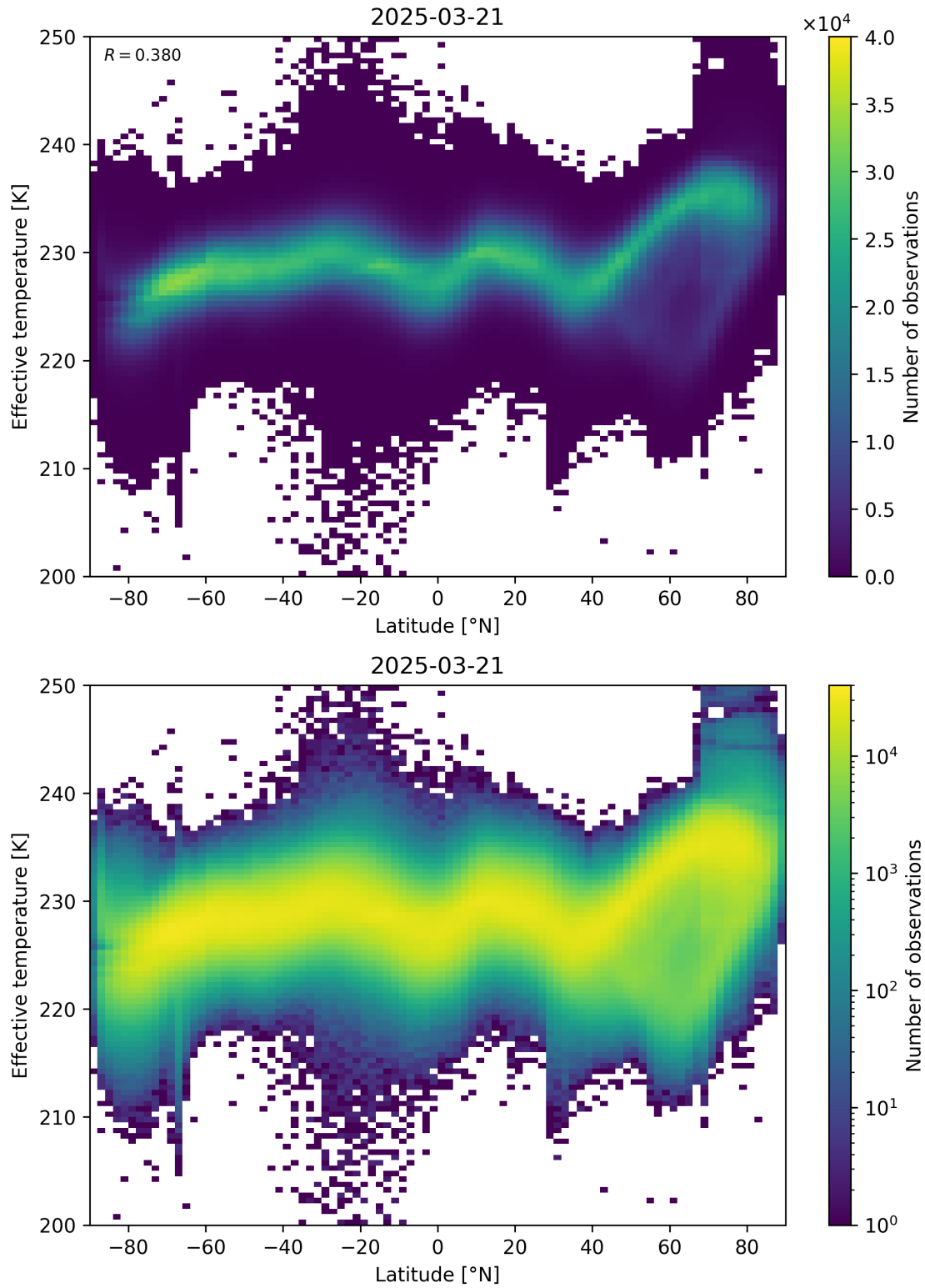
Figure 34: Scatter density plot of “Latitude” against “Effective temperature” for 2025-03-20 to 2025-03-22.
