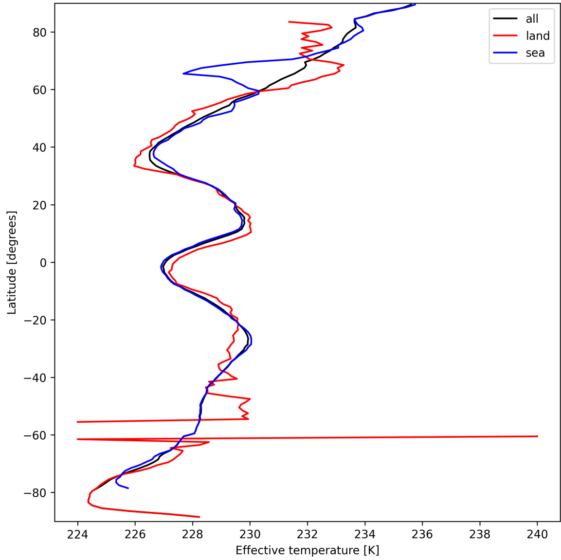
Figure 17: Zonal average of “Effective temperature” for 2025-03-20 to 2025-03-22.
