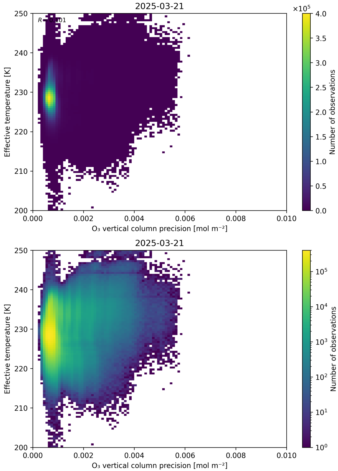
Figure 42: Scatter density plot of “O 3 vertical column precision” against “Effective temperature” for 2025-03-20 to 2025-03-22.
