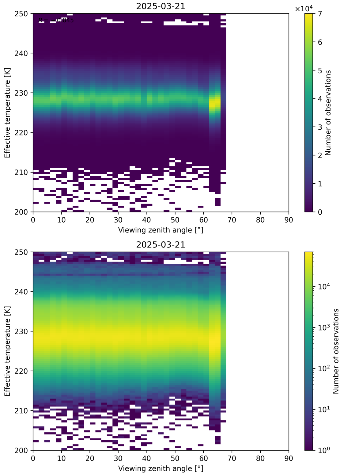
Figure 50: Scatter density plot of “Viewing zenith angle” against “Effective temperature” for 2025-03-20 to 2025-03-22.
