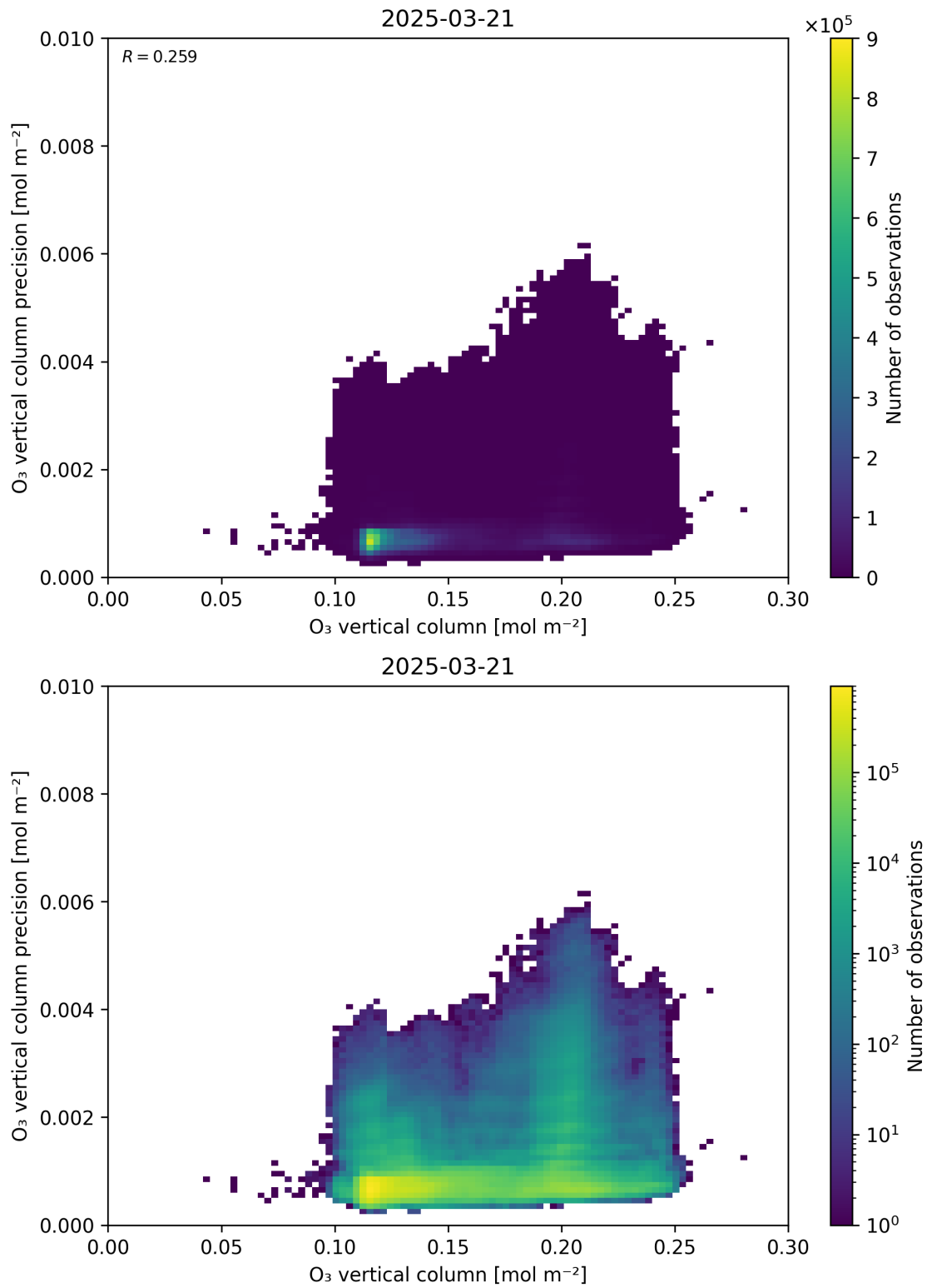
Figure 41: Scatter density plot of “O 3 vertical column” against “O 3 vertical column precision” for 2025-03-20 to 2025-03-22.
