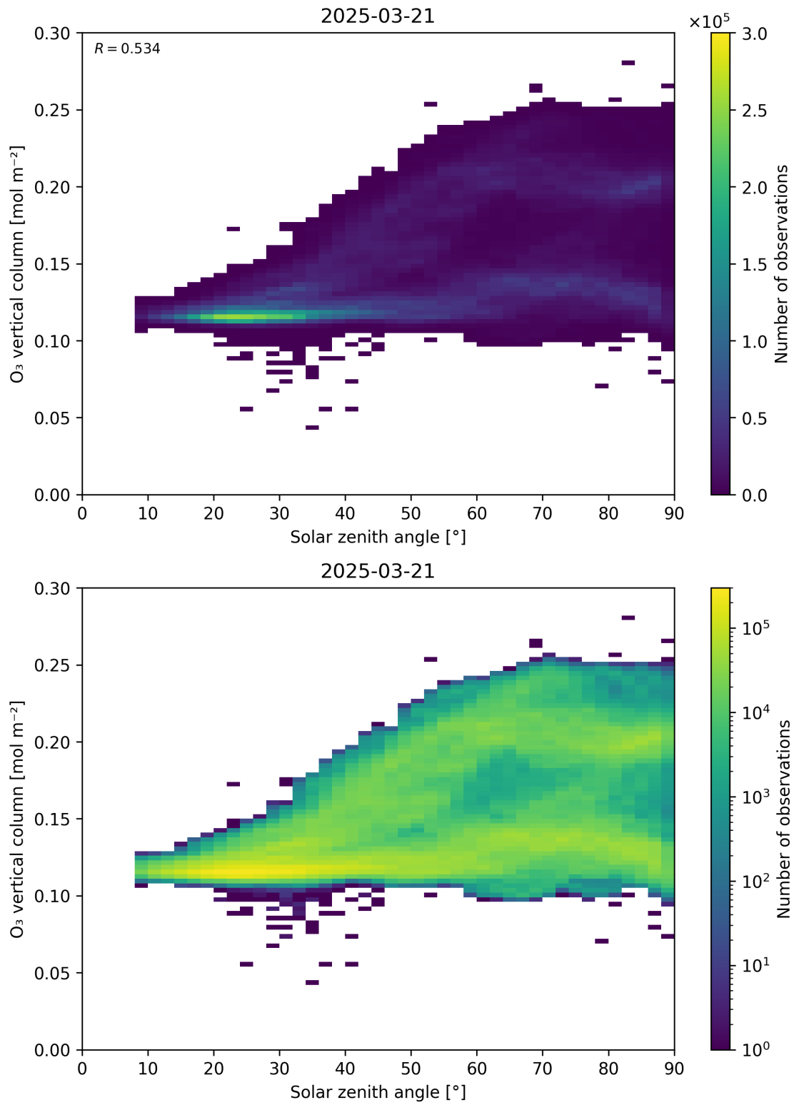
Figure 47: Scatter density plot of “Solar zenith angle” against “O 3 vertical column” for 2025-03-20 to 2025-03-22.
