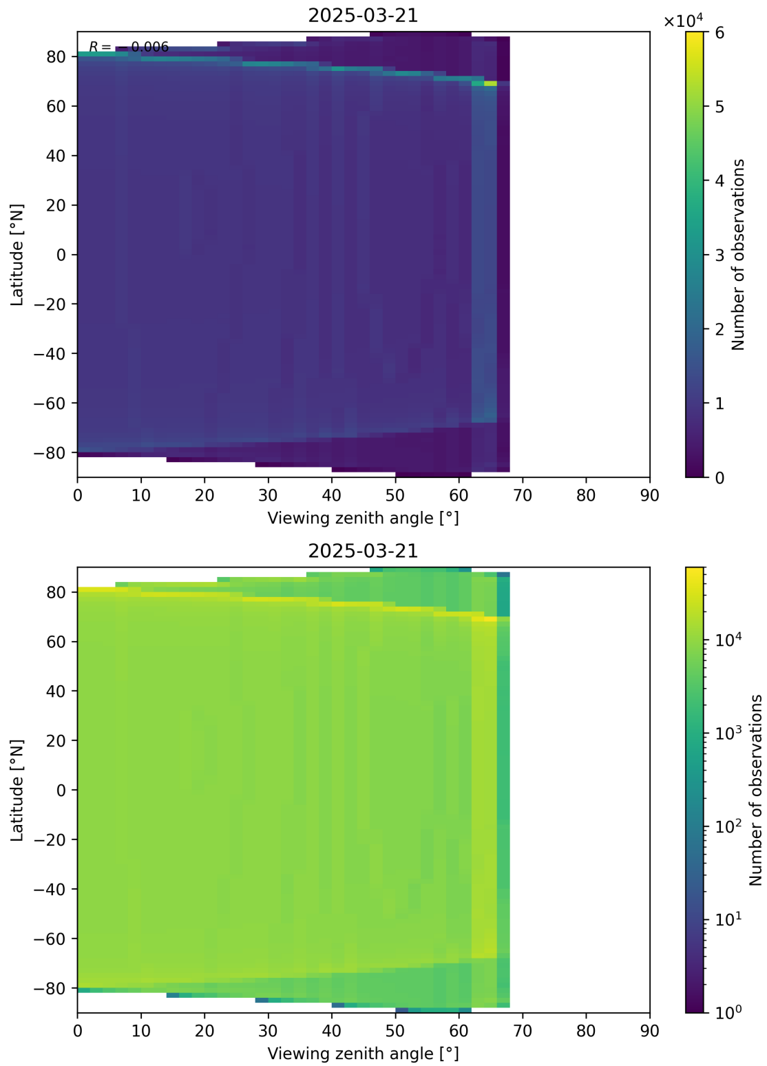
Figure 49: Scatter density plot of “Viewing zenith angle” against “Latitude” for 2025-03-20 to 2025-03-22.
