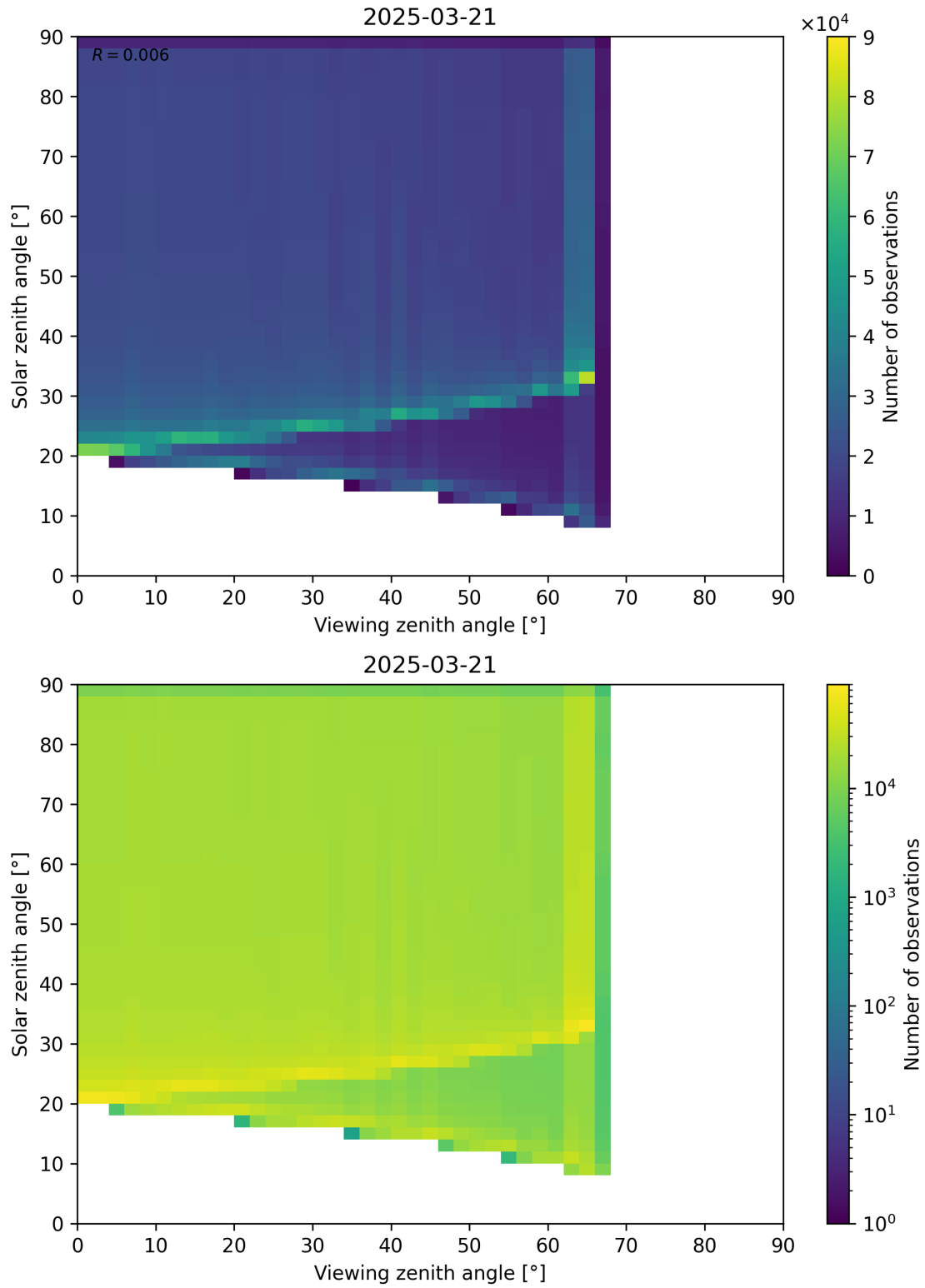
Figure 54: Scatter density plot of “Viewing zenith angle” against “Solar zenith angle” for 2025-03-20 to 2025-03-22.
