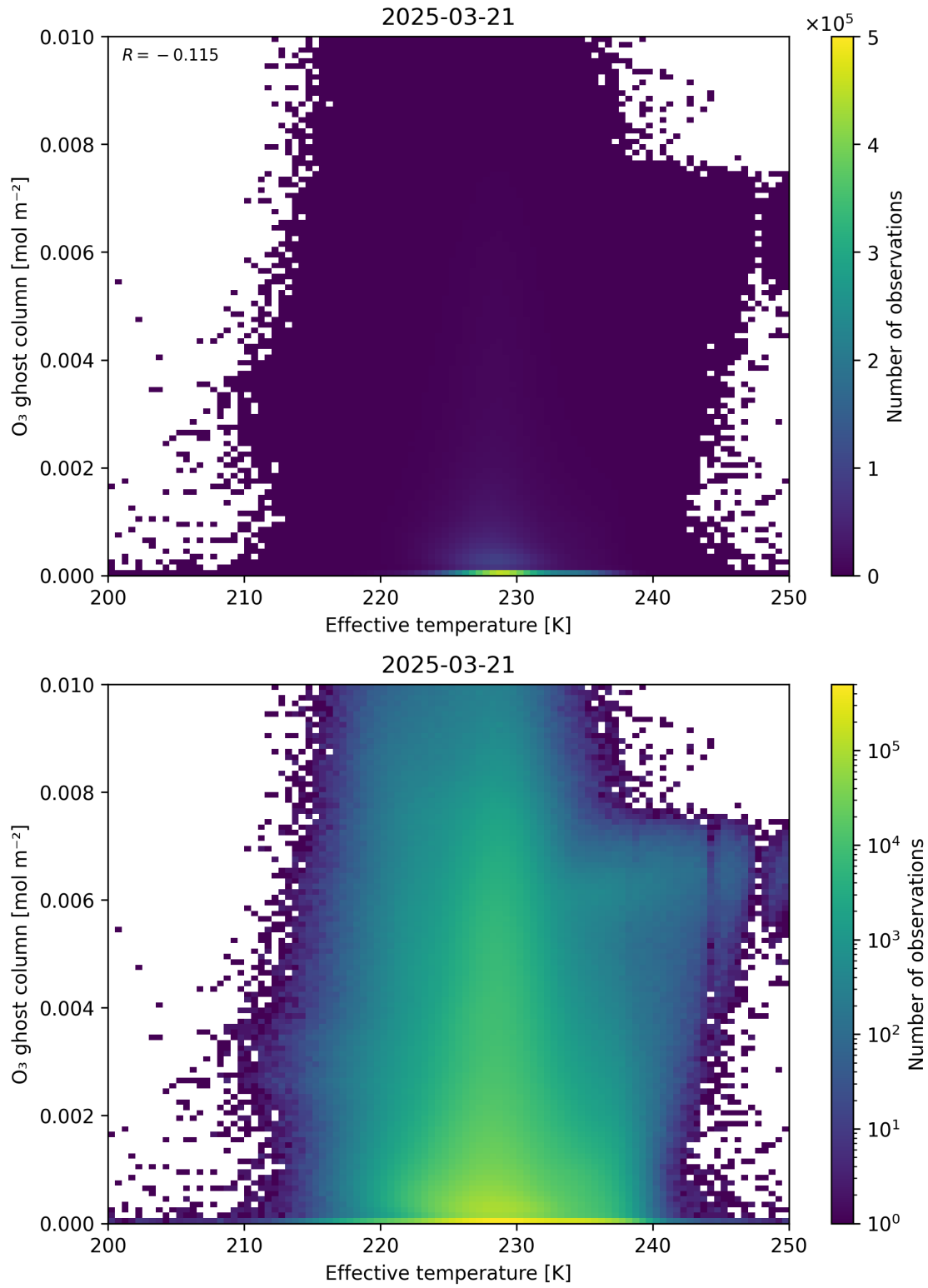
Figure 38: Scatter density plot of “Effective temperature” against “O 3 ghost column” for 2025-03-20 to 2025-03-22.
