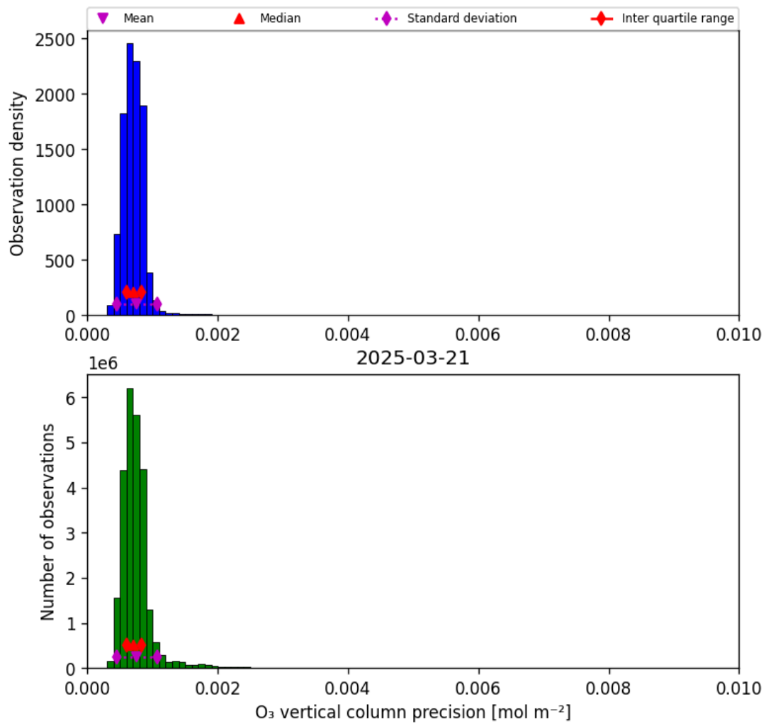
Figure 22: Histogram of "O 3 vertical column precision" for 2025-03-20 to 2025-03-22
