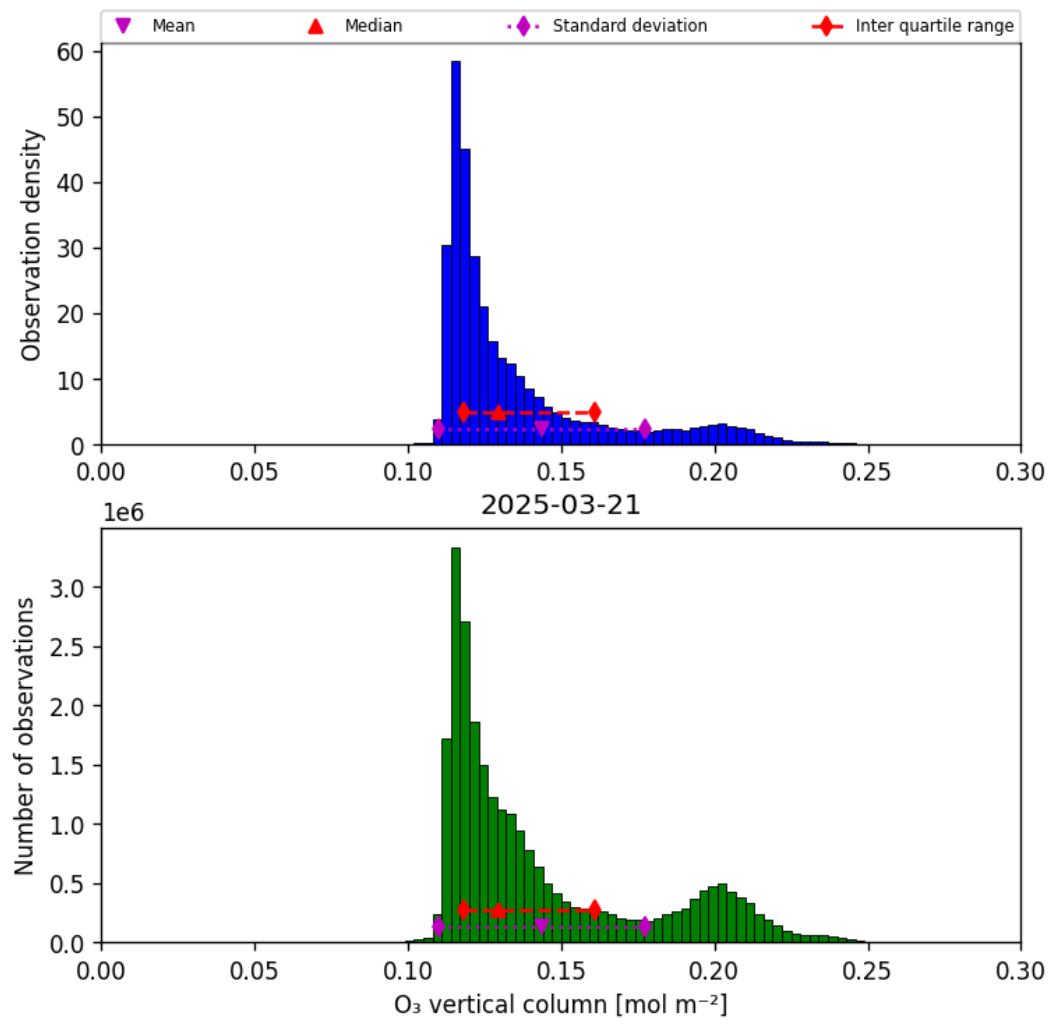
Figure 21: Histogram of “O 3 vertical column” for 2025-03-20 to 2025-03-22
