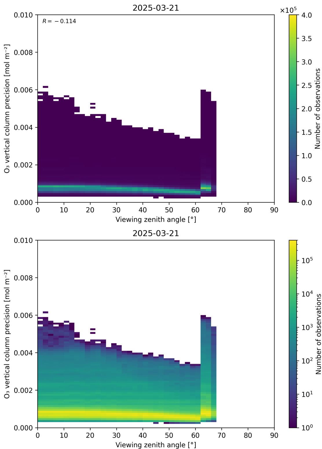
Figure 53: Scatter density plot of “Viewing zenith angle” against “O 3 vertical column precision” for 2025-03-20 to 2025-03-22.
