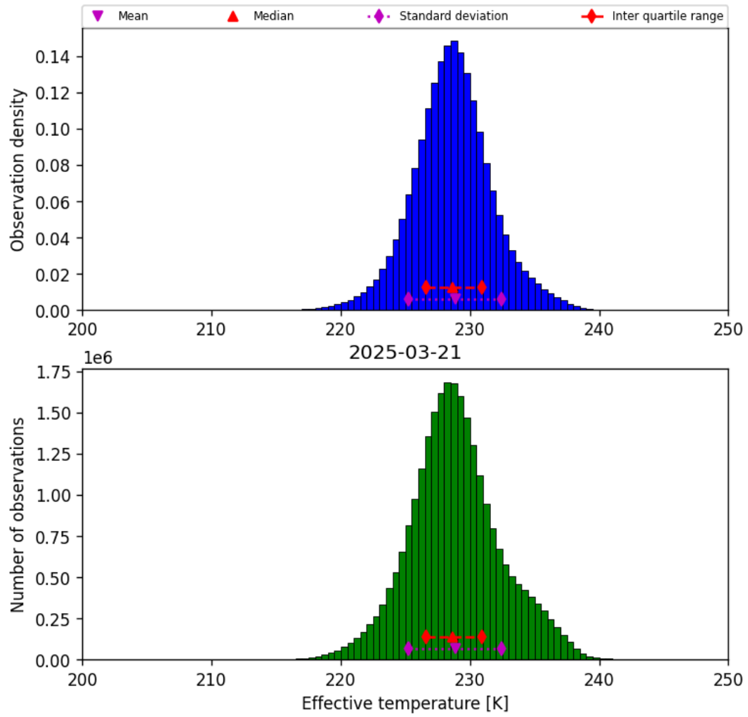
Figure 24: Histogram of “Effective temperature” for 2025-03-20 to 2025-03-22
