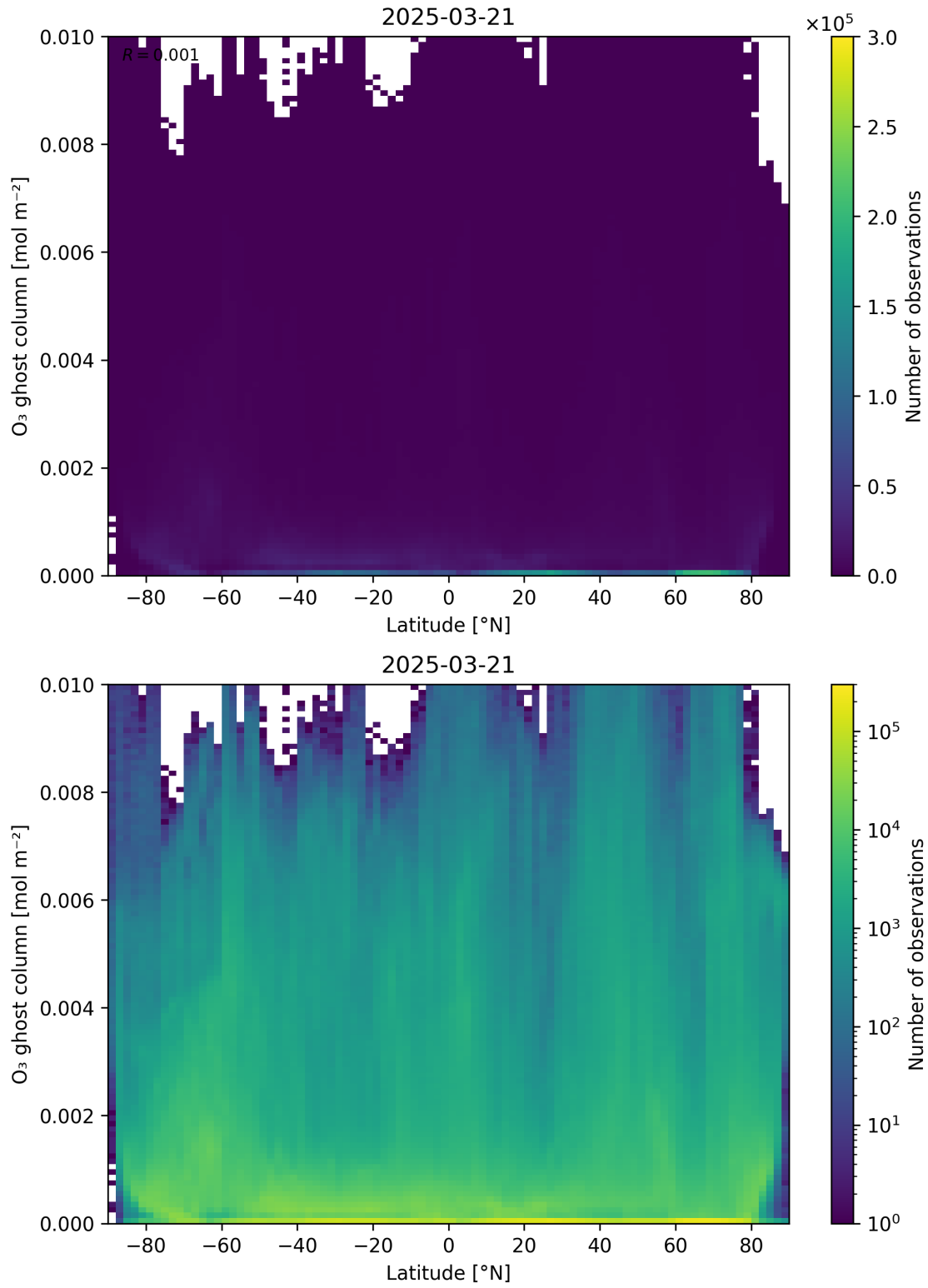
Figure 35: Scatter density plot of “Latitude” against “O 3 ghost column” for 2025-03-20 to 2025-03-22.
