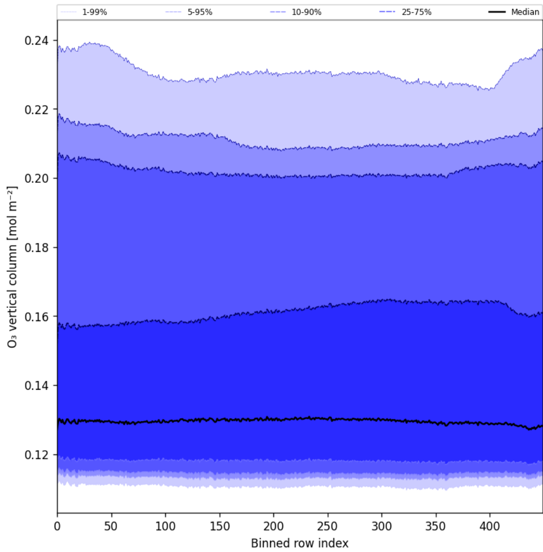
Figure 28: Along track statistics of “O 3 vertical column” for 2025-03-20 to 2025-03-22
