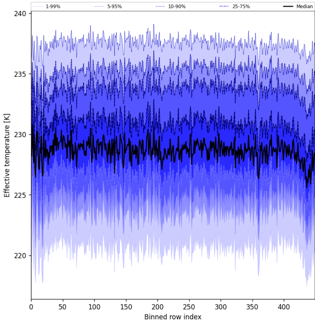
Figure 31: Along track statistics of “Effective temperature” for 2025-03-20 to 2025-03-22
