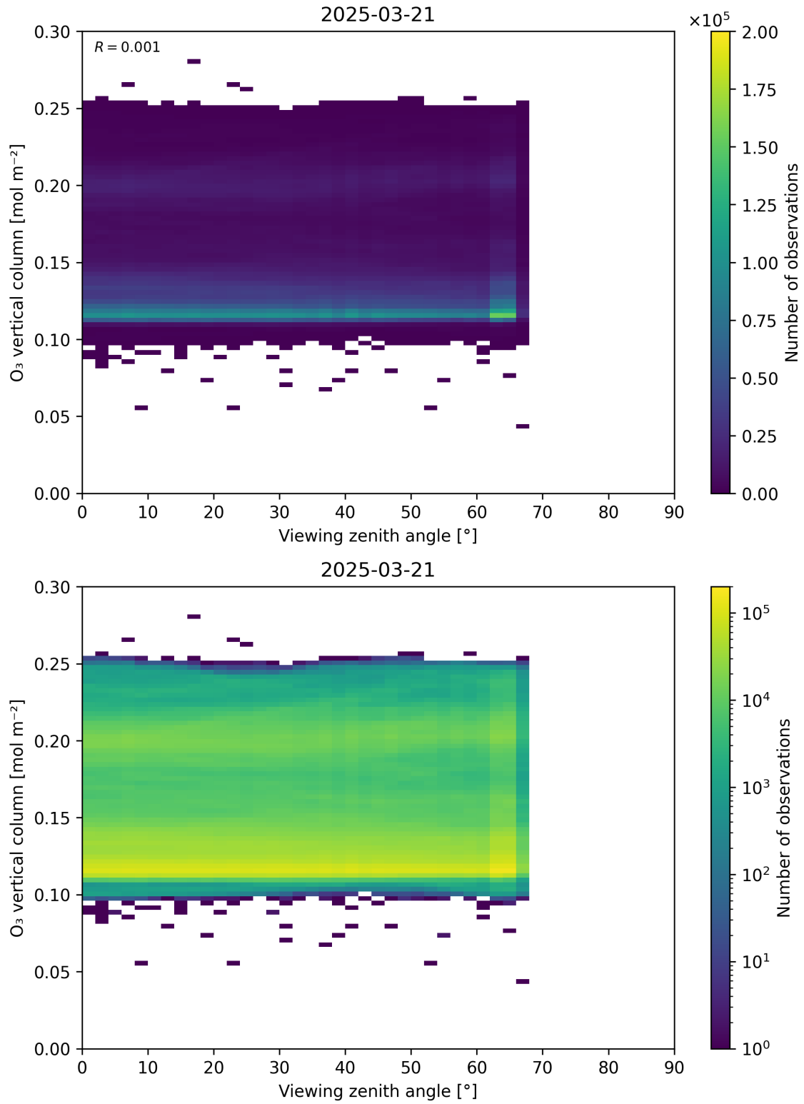
Figure 52: Scatter density plot of “Viewing zenith angle” against “O 3 vertical column” for 2025-03-20 to 2025-03-22.
