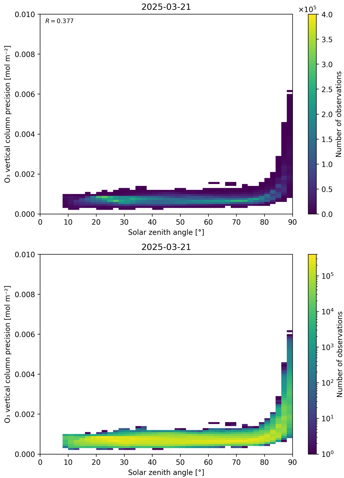
Figure 48: Scatter density plot of “Solar zenith angle” against “O 3 vertical column precision” for 2025-03-20 to 2025-03-22.
