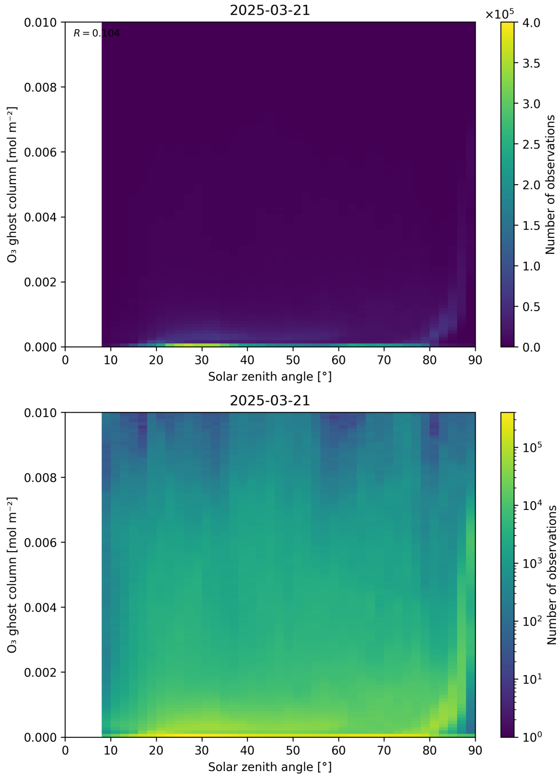
Figure 46: Scatter density plot of “Solar zenith angle” against “O 3 ghost column” for 2025-03-20 to 2025-03-22.
