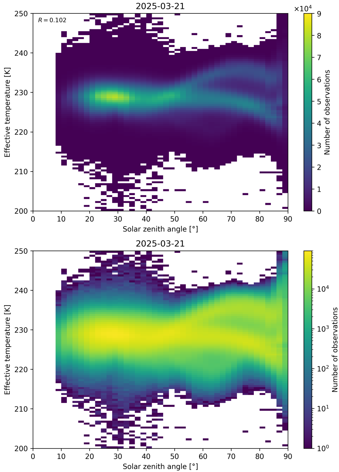
Figure 45: Scatter density plot of “Solar zenith angle” against “Effective temperature” for 2025-03-20 to 2025-03-22.
