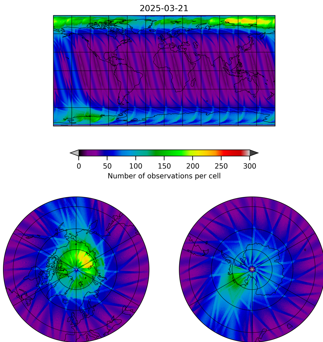
Figure 12: Map of the number of observations for 2025-03-20 to 2025-03-22
