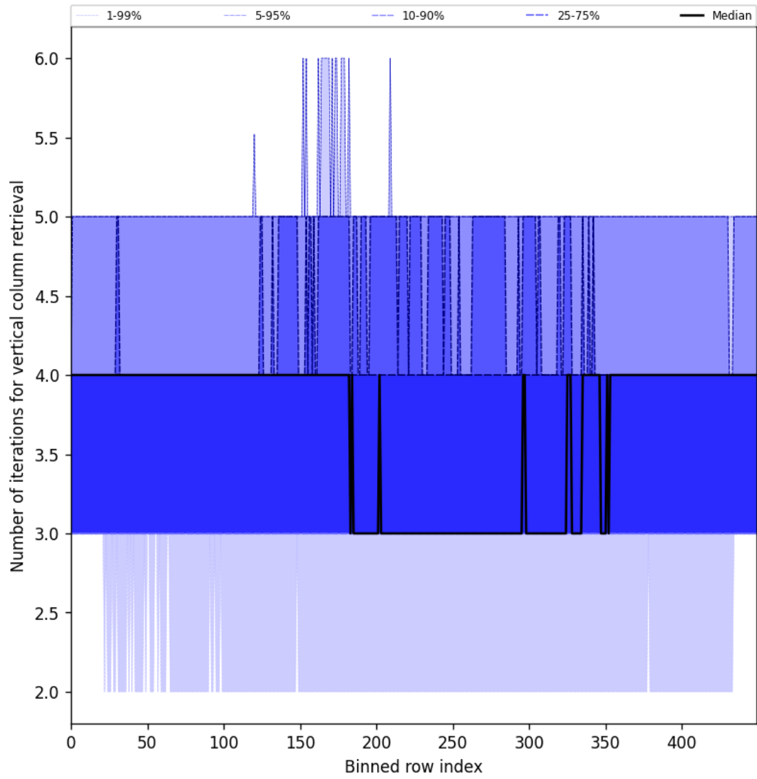
Figure 33: Along track statistics of “Number of iterations for vertical column retrieval” for 2025-03-20 to 2025-03-22
