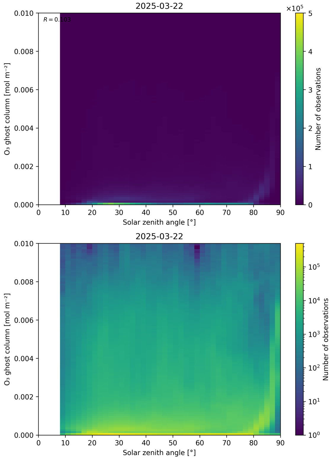
Figure 46: Scatter density plot of “Solar zenith angle” against “O 3 ghost column” for 2025-03-21 to 2025-03-23.
