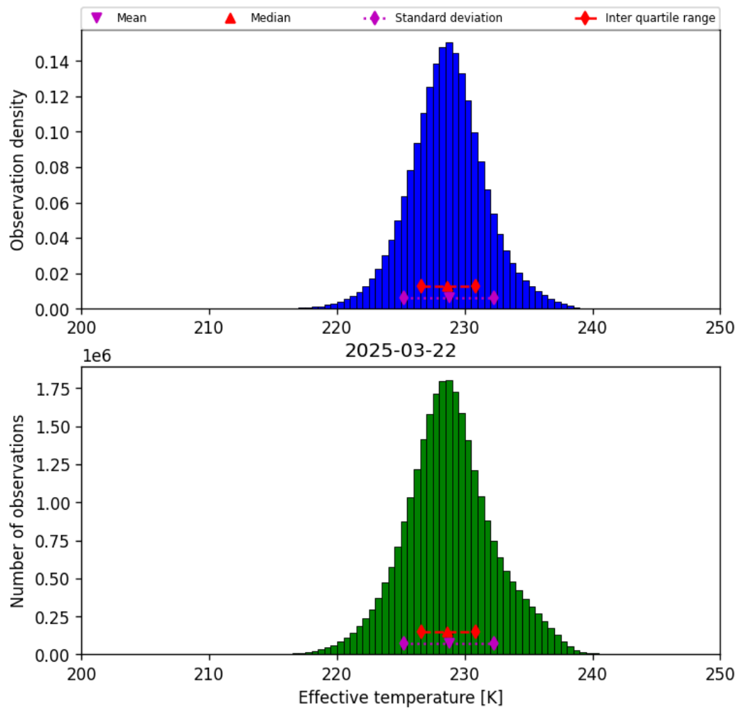
Figure 24: Histogram of “Effective temperature” for 2025-03-21 to 2025-03-23
