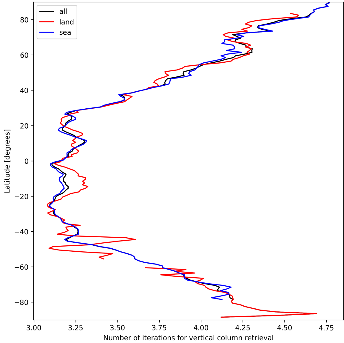
Figure 19: Zonal average of “Number of iterations for vertical column retrieval” for 2025-03-21 to 2025-03-23.
