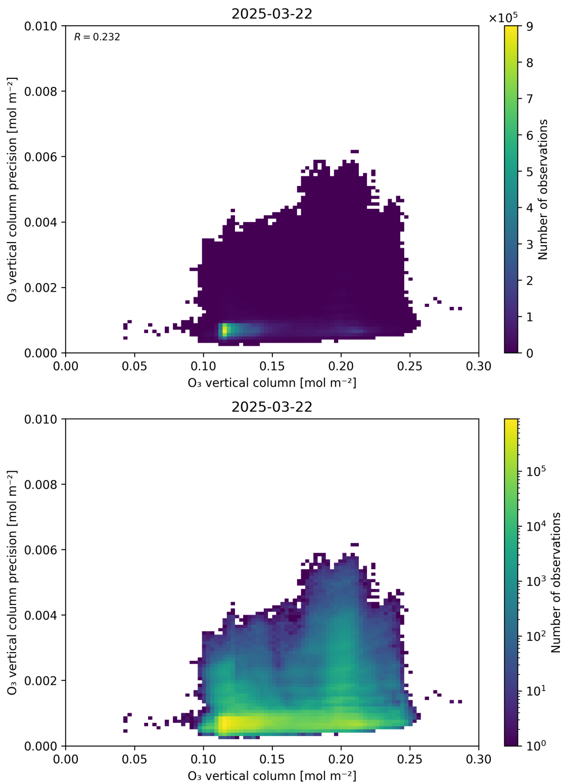
Figure 41: Scatter density plot of “O 3 vertical column” against “O 3 vertical column precision” for 2025-03-21 to 2025-03-23.
