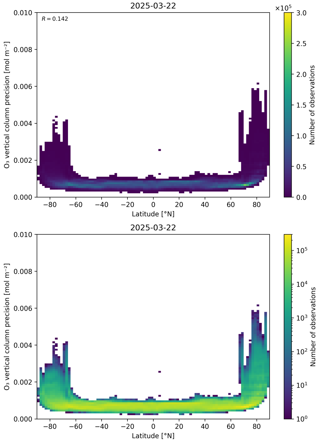
Figure 37: Scatter density plot of “Latitude” against “O 3 vertical column precision” for 2025-03-21 to 2025-03-23.
