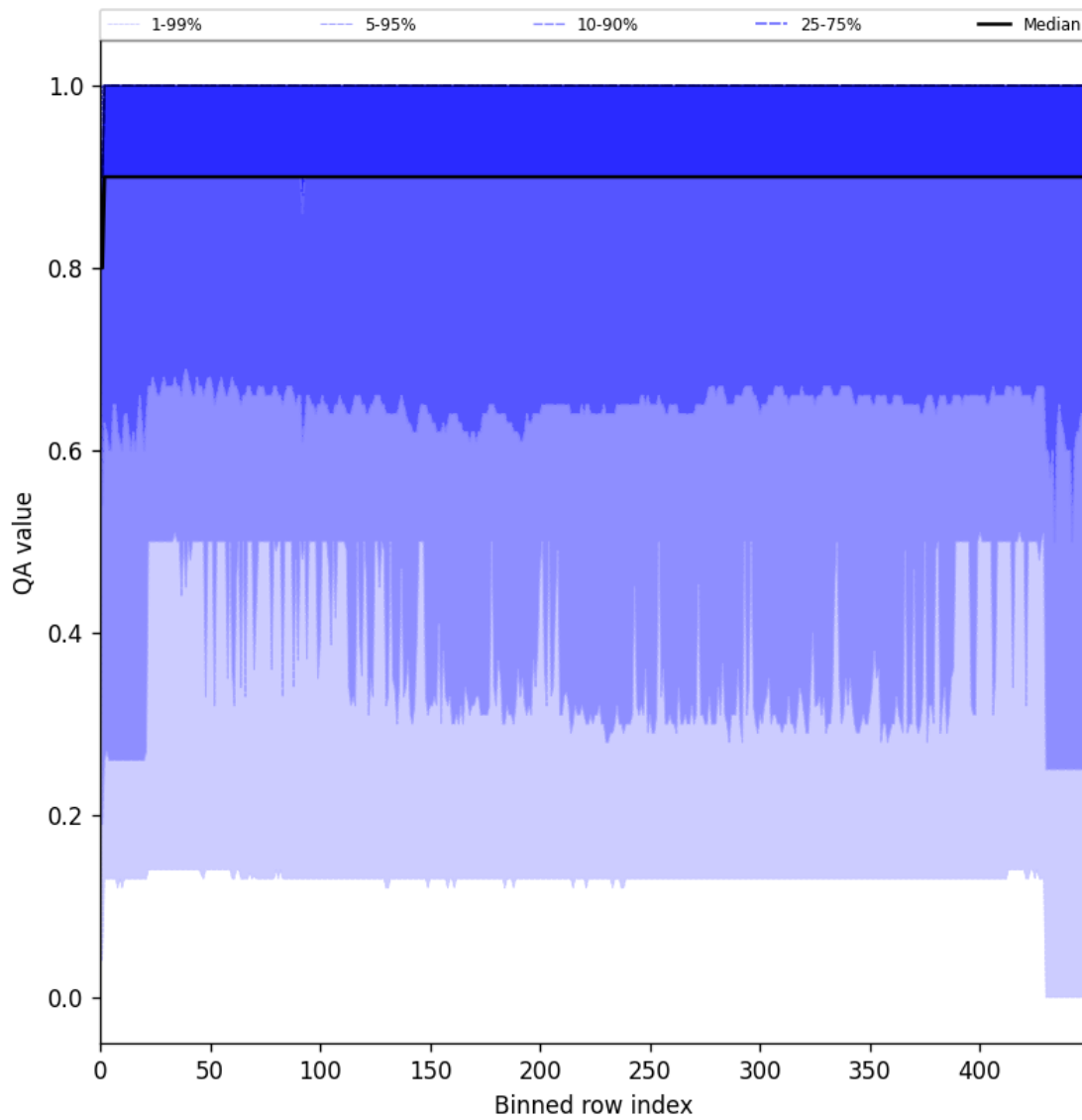
Figure 27: Along track statistics of “QA value” for 2025-03-21 to 2025-03-23
