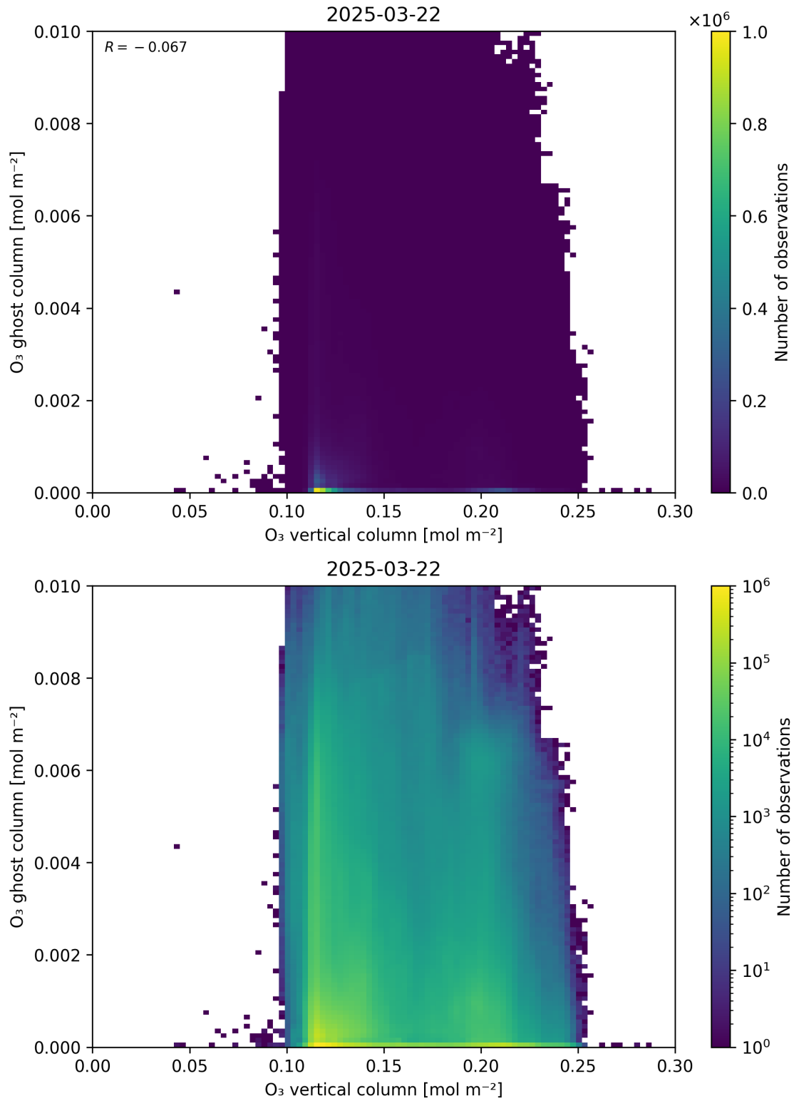
Figure 40: Scatter density plot of “O 3 vertical column” against “O 3 ghost column” for 2025-03-21 to 2025-03-23.
