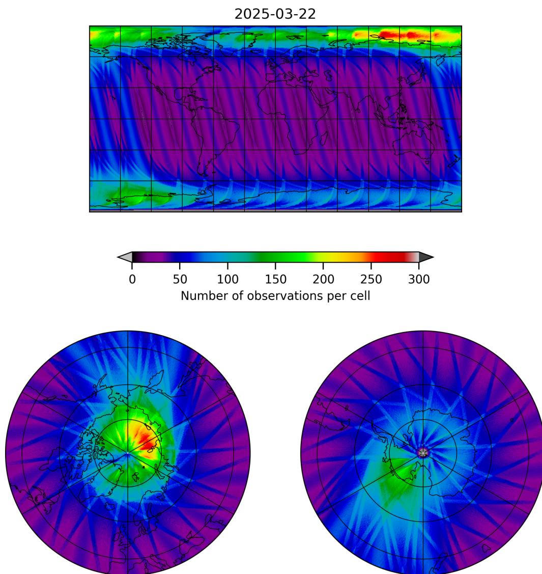
Figure 12: Map of the number of observations for 2025-03-21 to 2025-03-23
