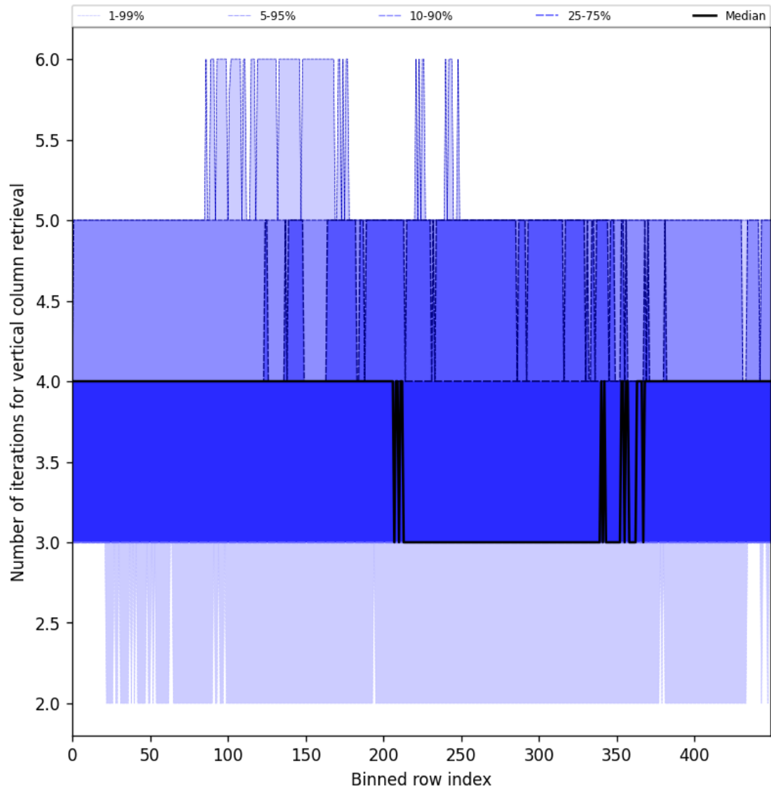
Figure 33: Along track statistics of “Number of iterations for vertical column retrieval” for 2025-03-21 to 2025-03-23
