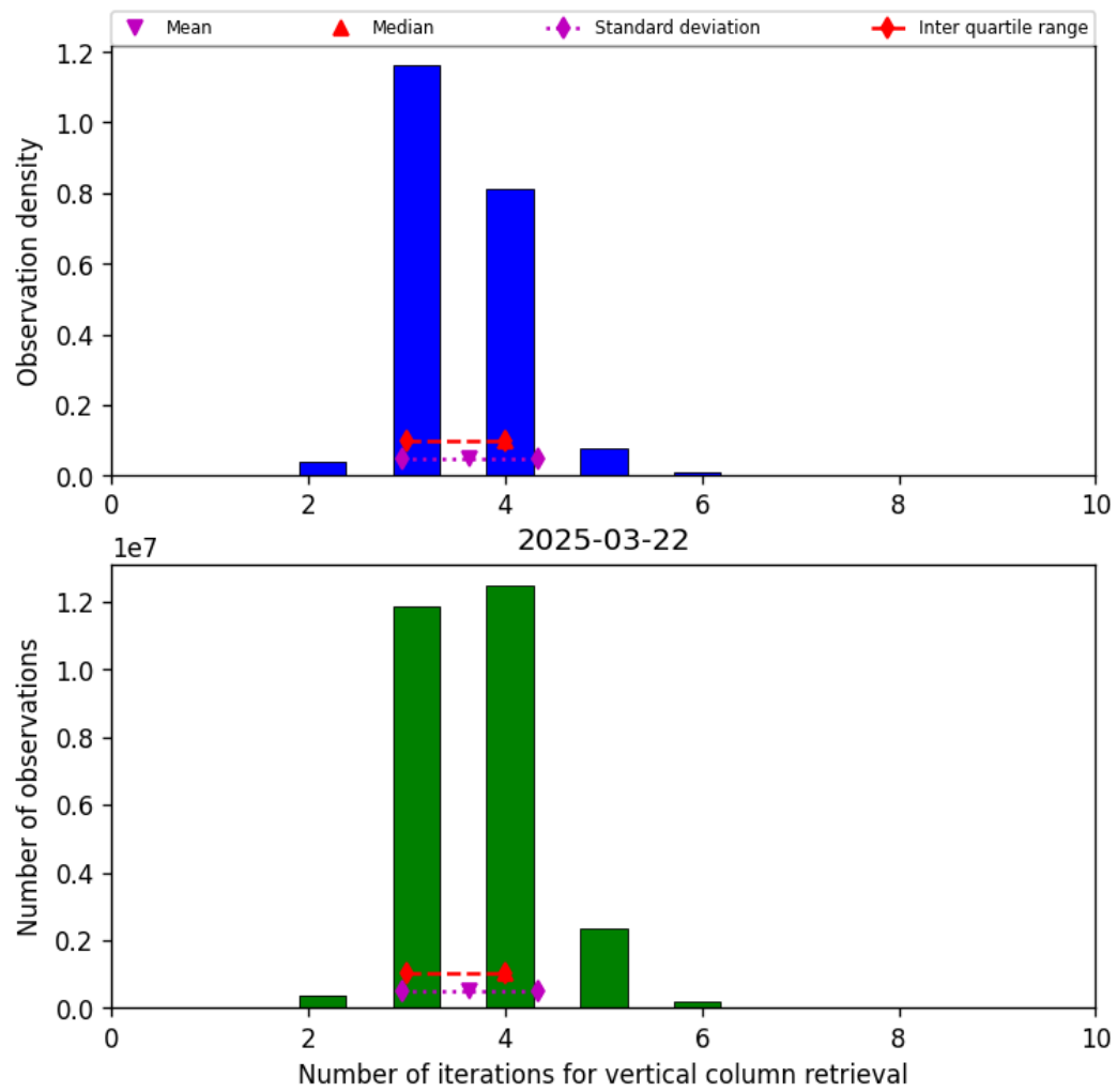
Figure 26: Histogram of “Number of iterations for vertical column retrieval” for 2025-03-21 to 2025-03-23
