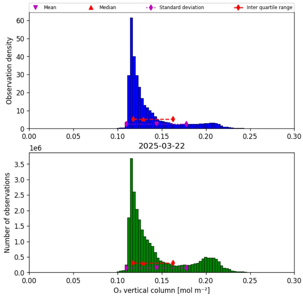
Figure 21: Histogram of “O 3 vertical column” for 2025-03-21 to 2025-03-23
