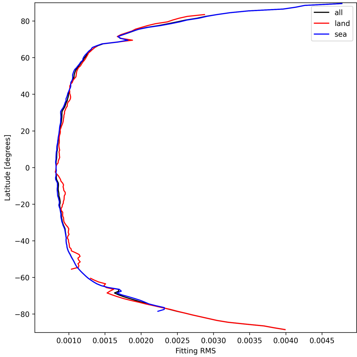
Figure 16: Zonal average of “Fitting RMS” for 2025-03-21 to 2025-03-23.
