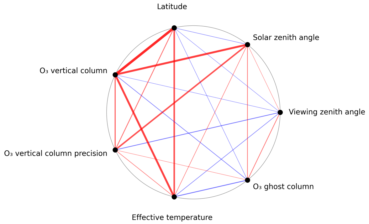
Figure 1: Map of correlation graph for 2025-03-21 to 2025-03-23.
