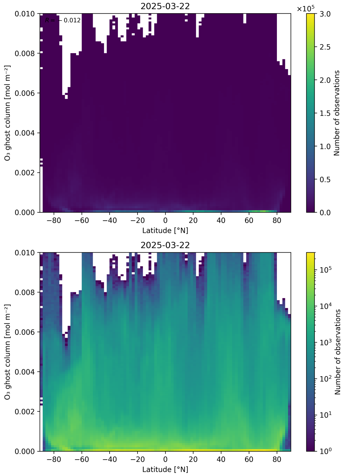
Figure 35: Scatter density plot of “Latitude” against “O 3 ghost column” for 2025-03-21 to 2025-03-23.
