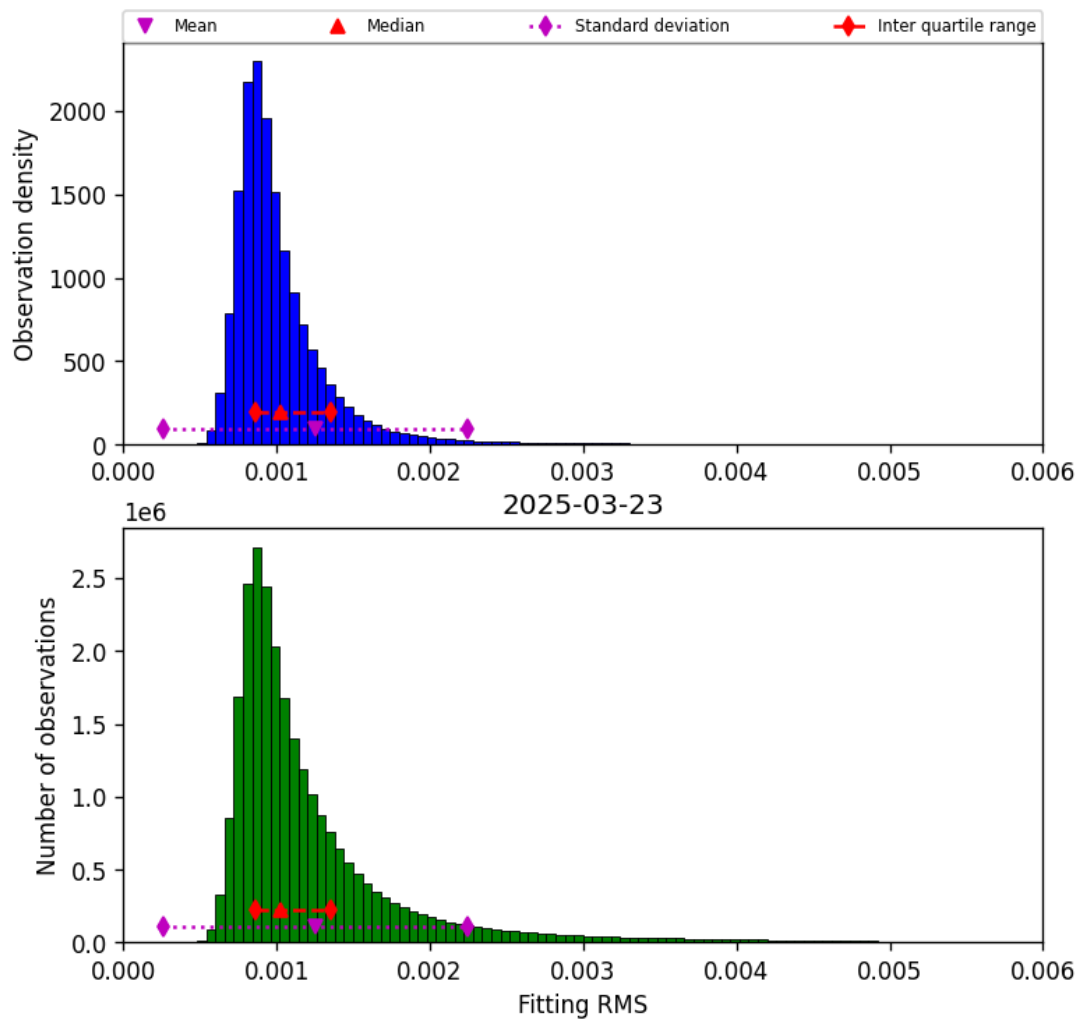
Figure 23: Histogram of “Fitting RMS” for 2025-03-23 to 2025-03-24
