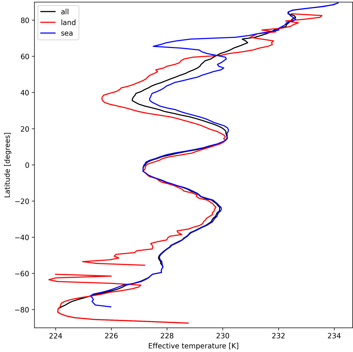
Figure 17: Zonal average of "Effective temperature" for 2025-03-23 to 2025-03-24.
