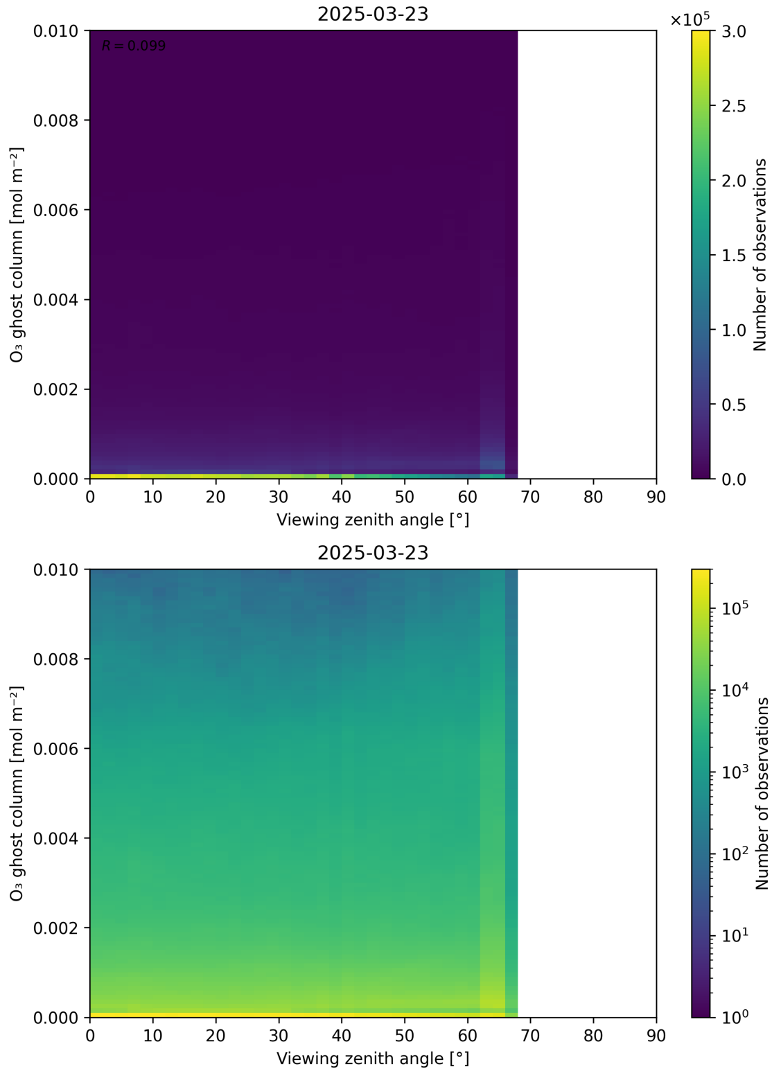
Figure 51: Scatter density plot of “Viewing zenith angle” against “O 3 ghost column” for 2025-03-23 to 2025-03-24.
