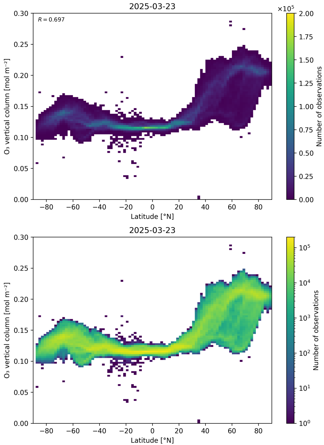
Figure 36: Scatter density plot of “Latitude” against “O 3 vertical column” for 2025-03-23 to 2025-03-24.
