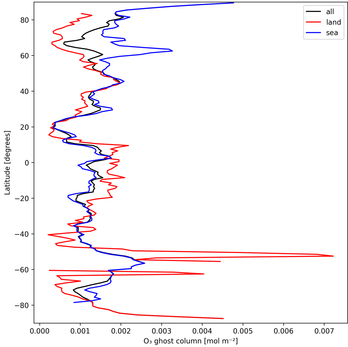
Figure 18: Zonal average of "O 3 ghost column" for 2025-03-23 to 2025-03-24.
