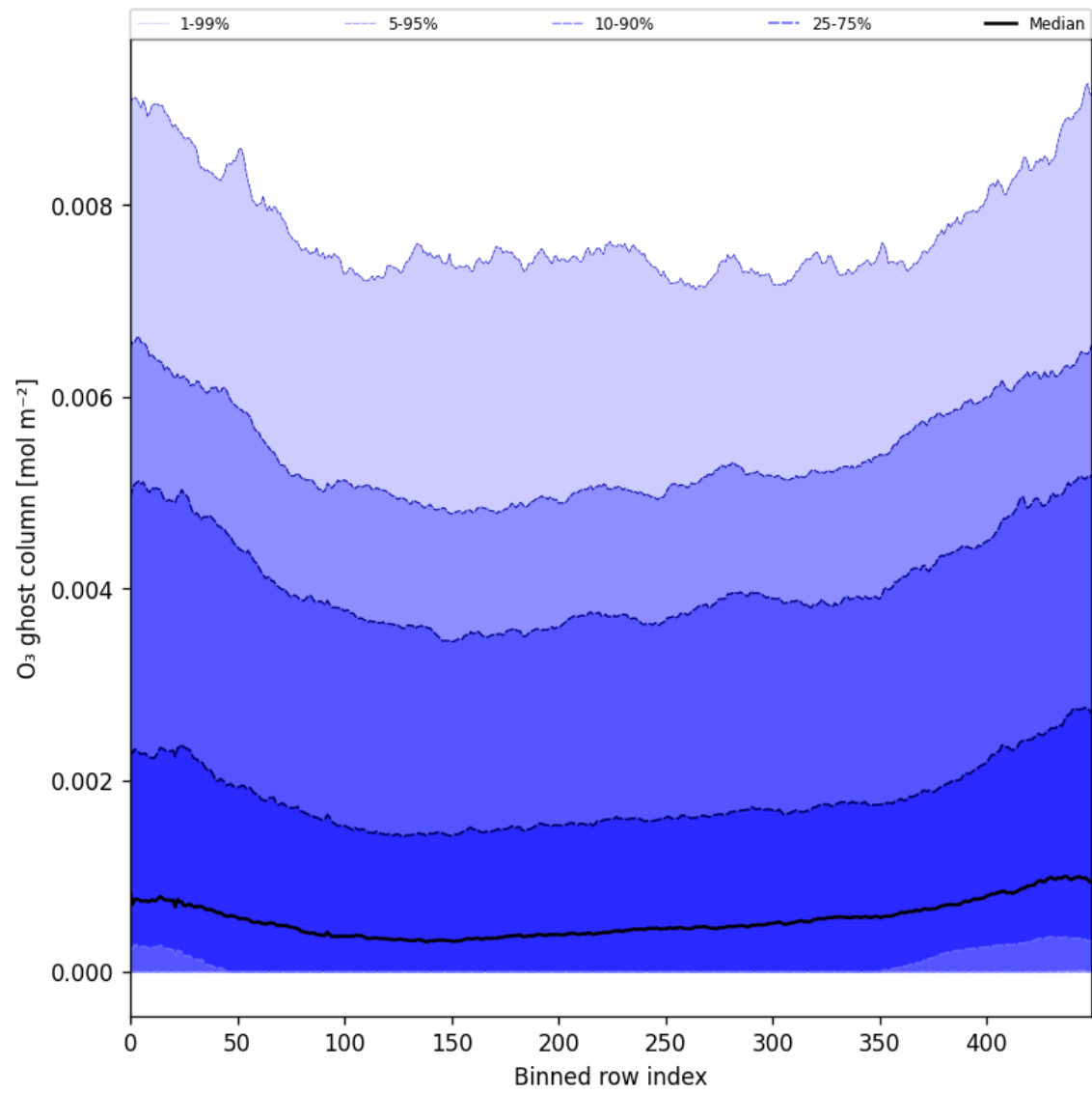
Figure 32: Along track statistics of “O 3 ghost column” for 2025-03-23 to 2025-03-24
