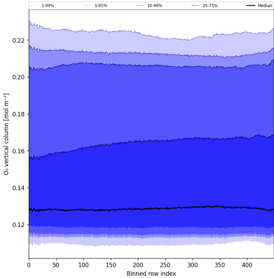
Figure 28: Along track statistics of “O 3 vertical column” for 2025-03-23 to 2025-03-24
