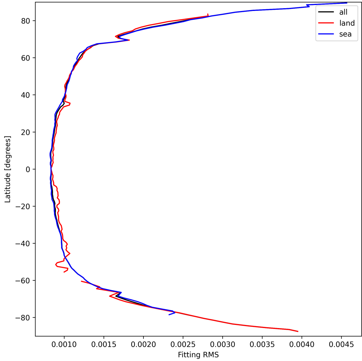
Figure 16: Zonal average of “Fitting RMS” for 2025-03-23 to 2025-03-24.
