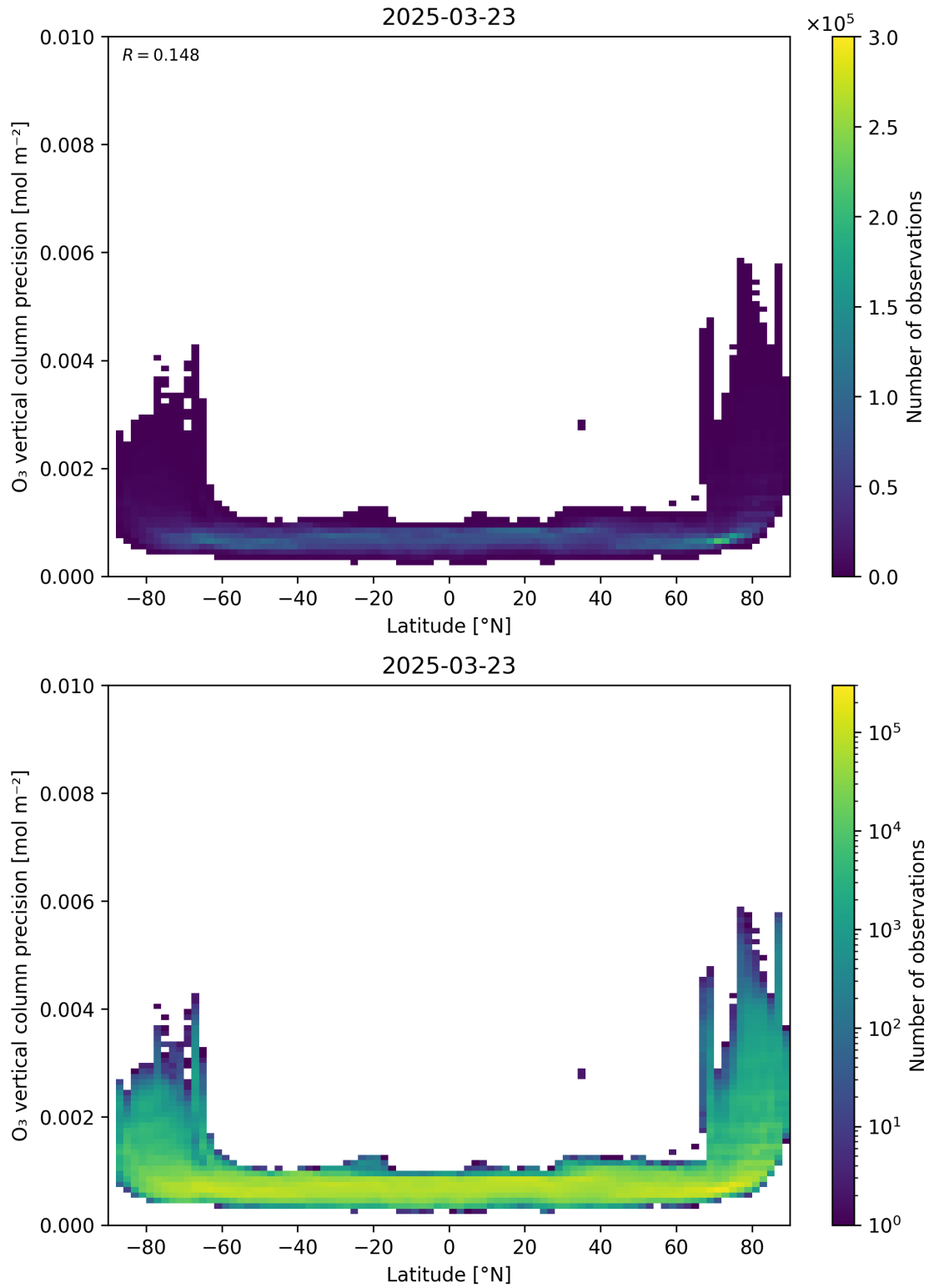
Figure 37: Scatter density plot of “Latitude” against “O 3 vertical column precision” for 2025-03-23 to 2025-03-24.
