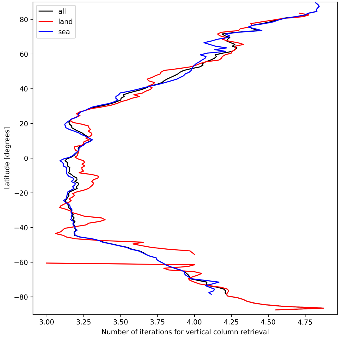
Figure 19: Zonal average of “Number of iterations for vertical column retrieval” for 2025-03-23 to 2025-03-24.
