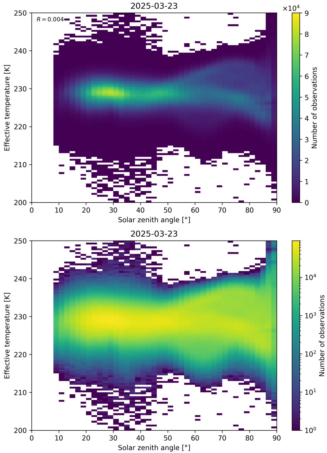
Figure 45: Scatter density plot of “Solar zenith angle” against “Effective temperature” for 2025-03-23 to 2025-03-24.
