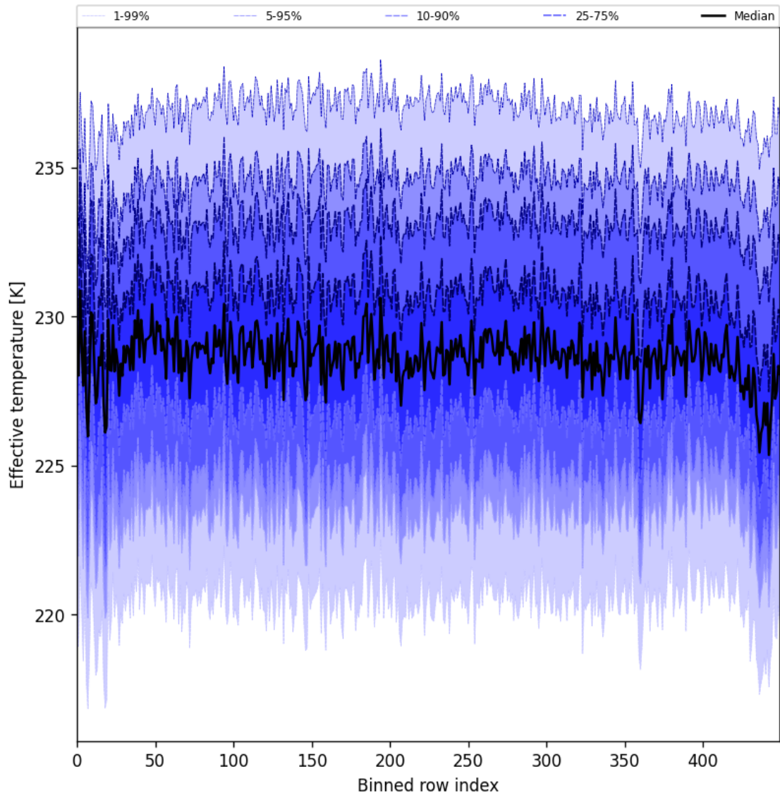
Figure 31: Along track statistics of “Effective temperature” for 2025-03-23 to 2025-03-24
