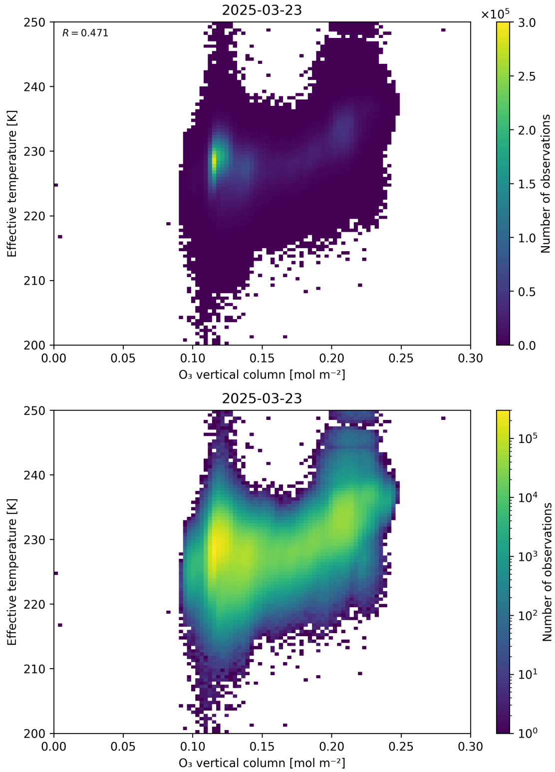
Figure 39: Scatter density plot of “O 3 vertical column” against “Effective temperature” for 2025-03-23 to 2025-03-24.
