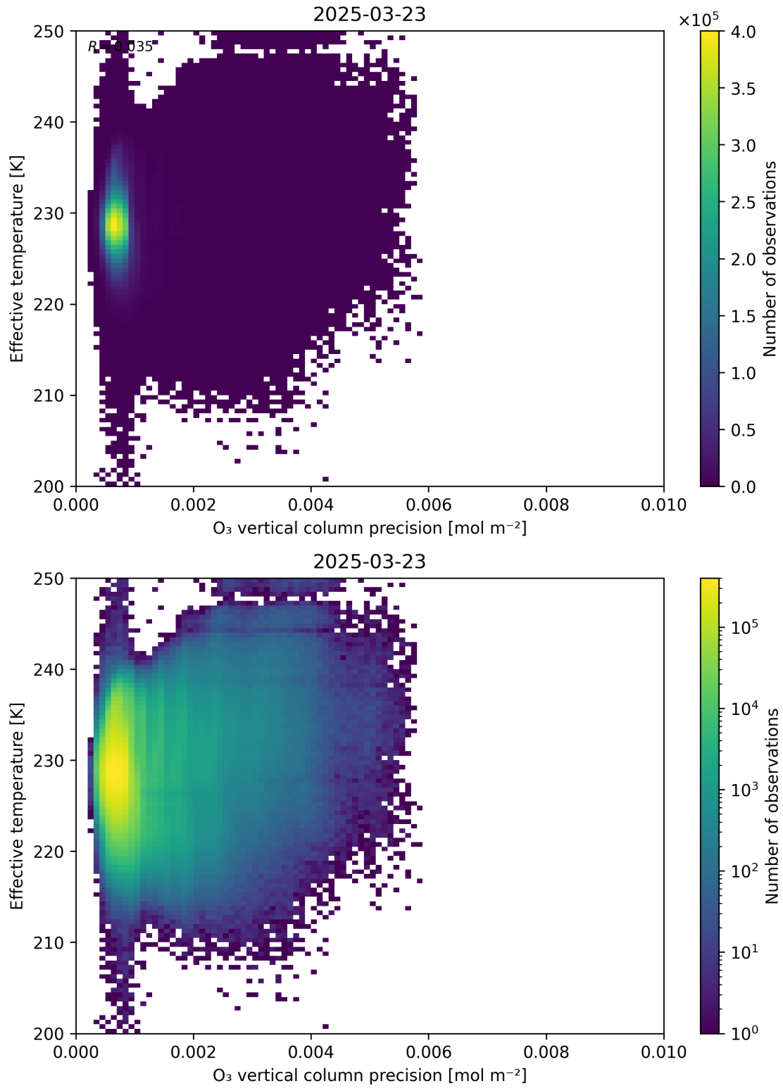
Figure 42: Scatter density plot of “O 3 vertical column precision” against “Effective temperature” for 2025-03-23 to 2025-03-24.
