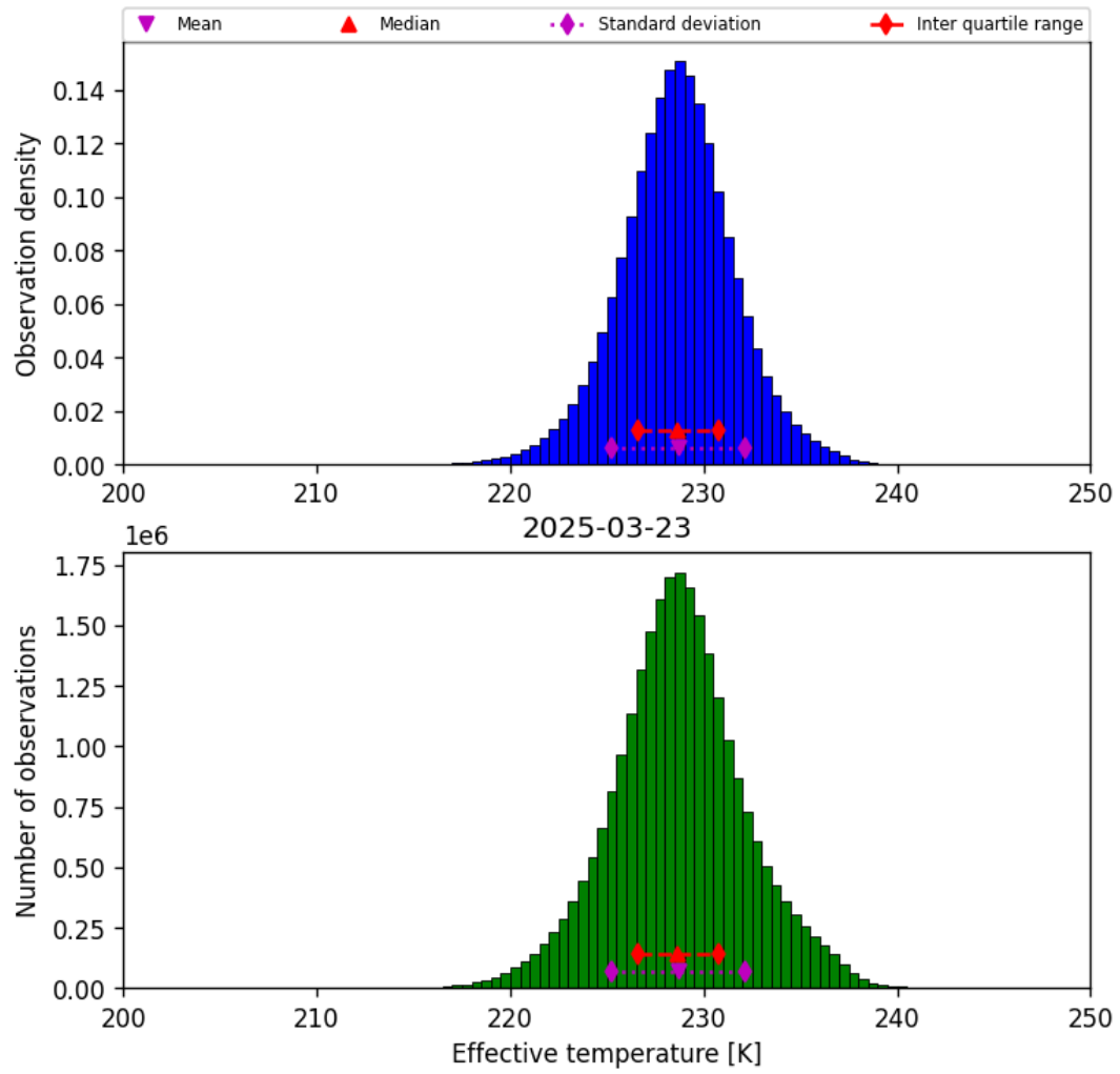
Figure 24: Histogram of “Effective temperature” for 2025-03-23 to 2025-03-24
