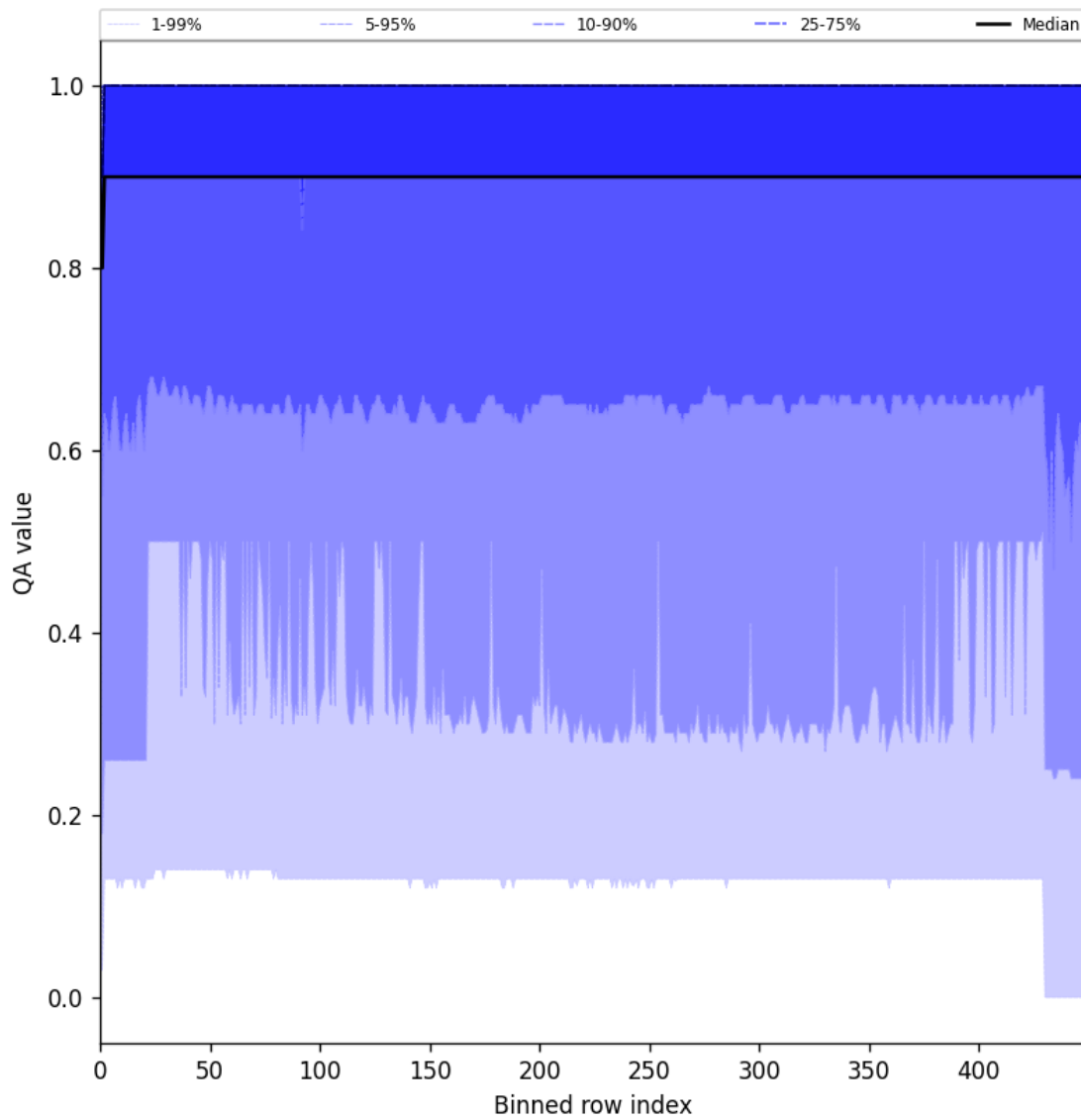
Figure 27: Along track statistics of “QA value” for 2025-03-23 to 2025-03-24
