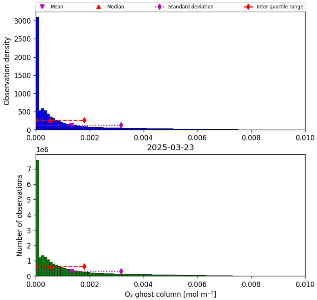
Figure 25: Histogram of “O 3 ghost column” for 2025-03-23 to 2025-03-24
