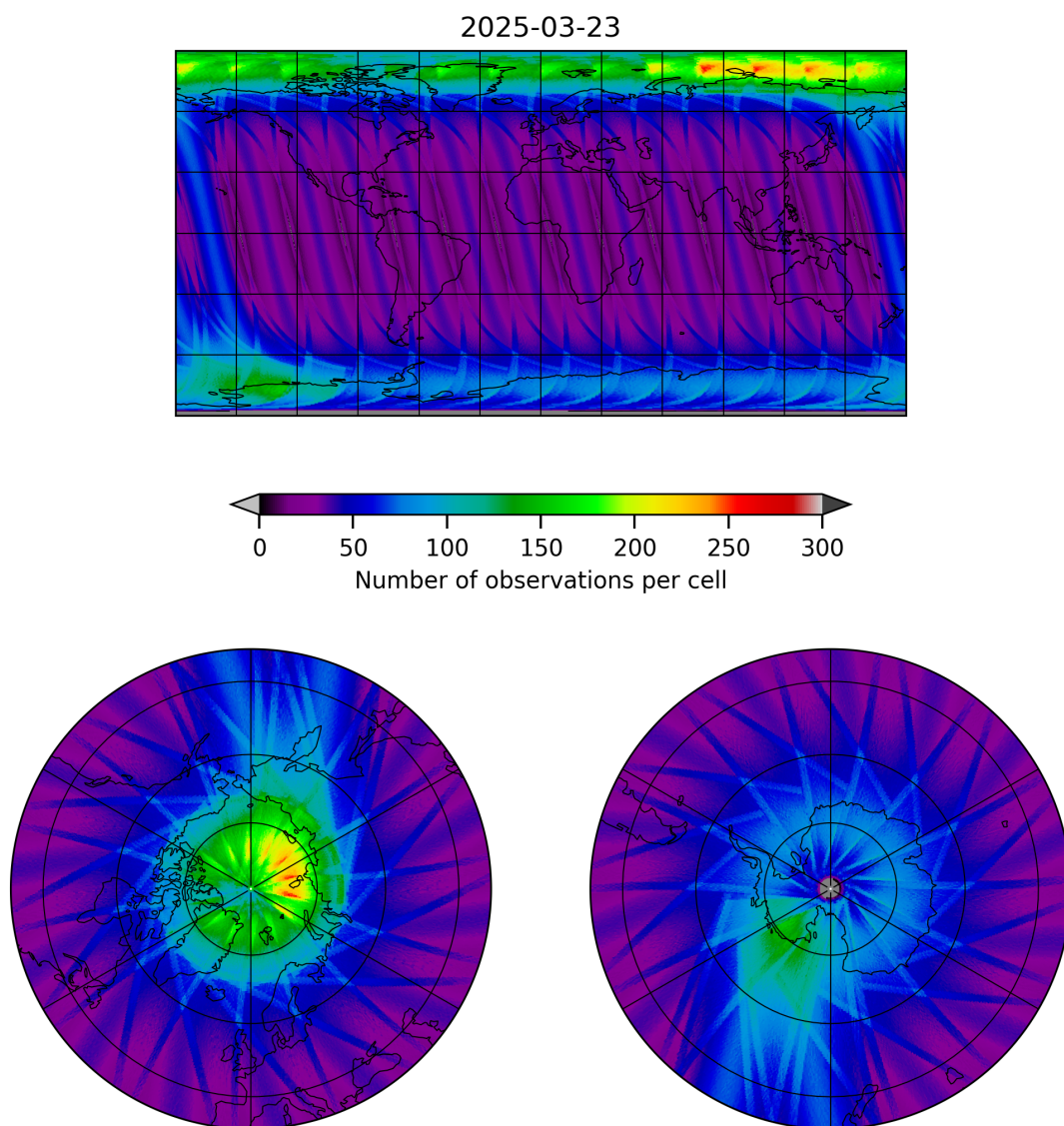
Figure 12: Map of the number of observations for 2025-03-23 to 2025-03-24
