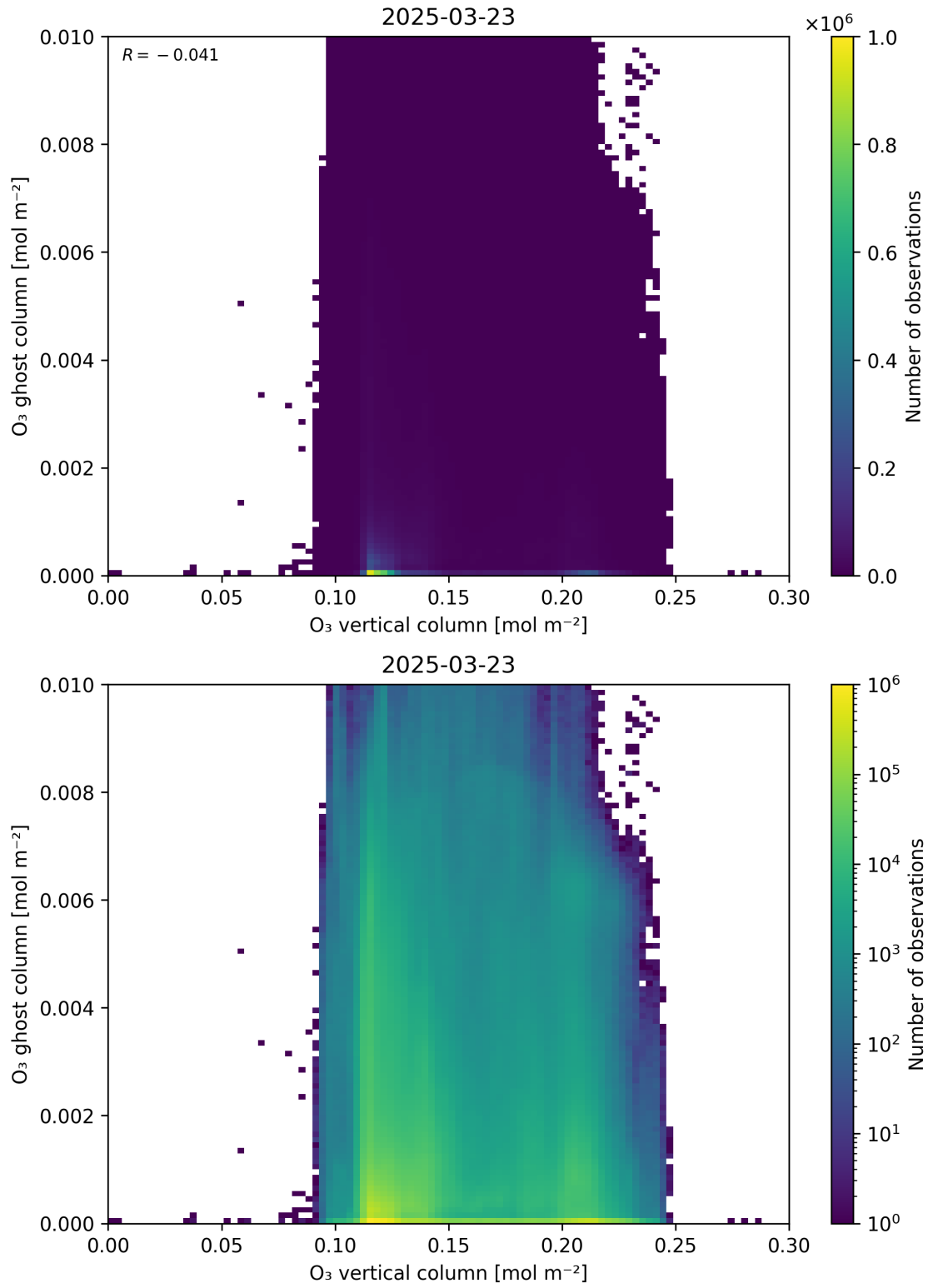
Figure 40: Scatter density plot of “O 3 vertical column” against “O 3 ghost column” for 2025-03-23 to 2025-03-24.
