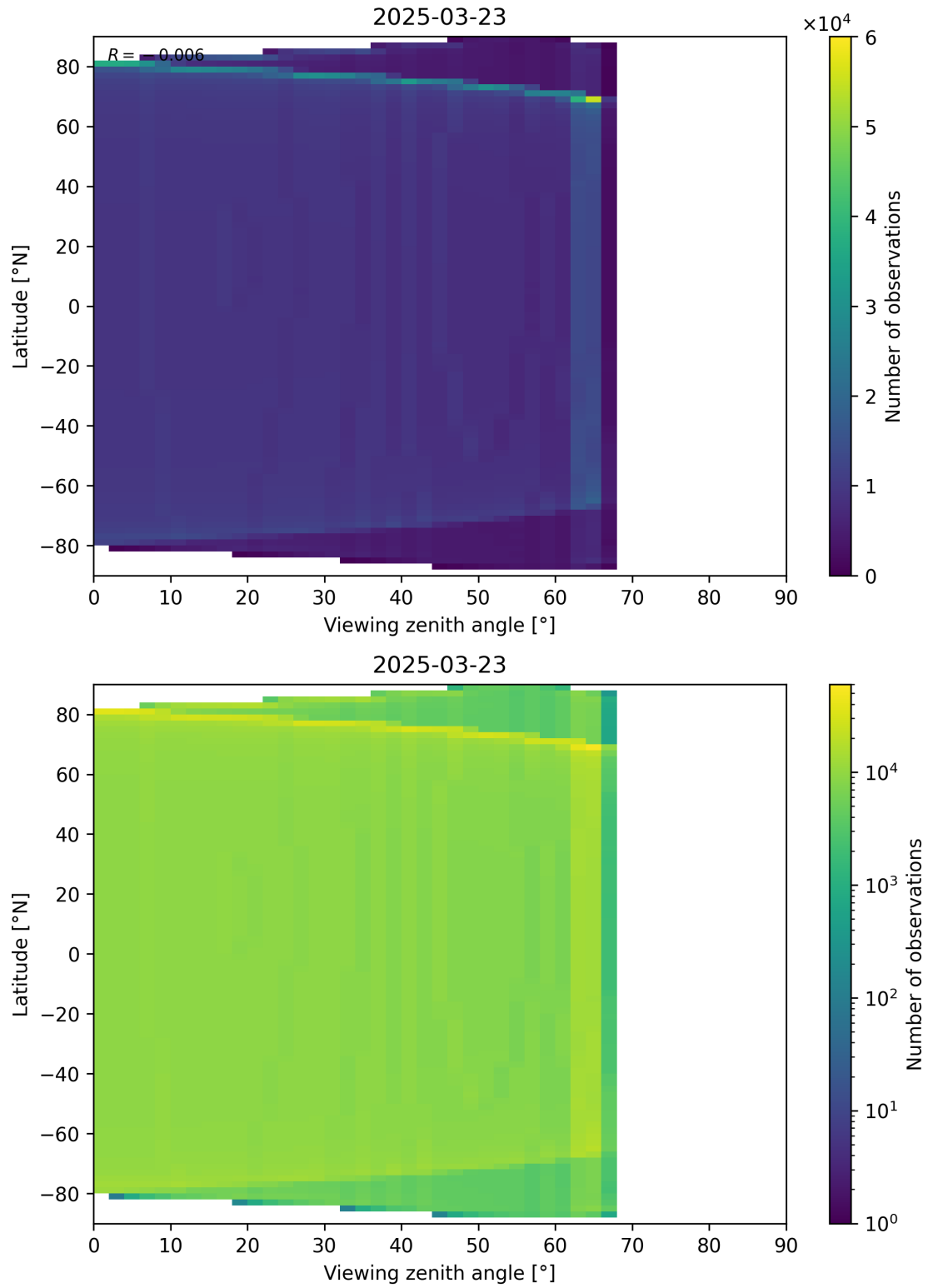
Figure 49: Scatter density plot of “Viewing zenith angle” against “Latitude” for 2025-03-23 to 2025-03-24.
