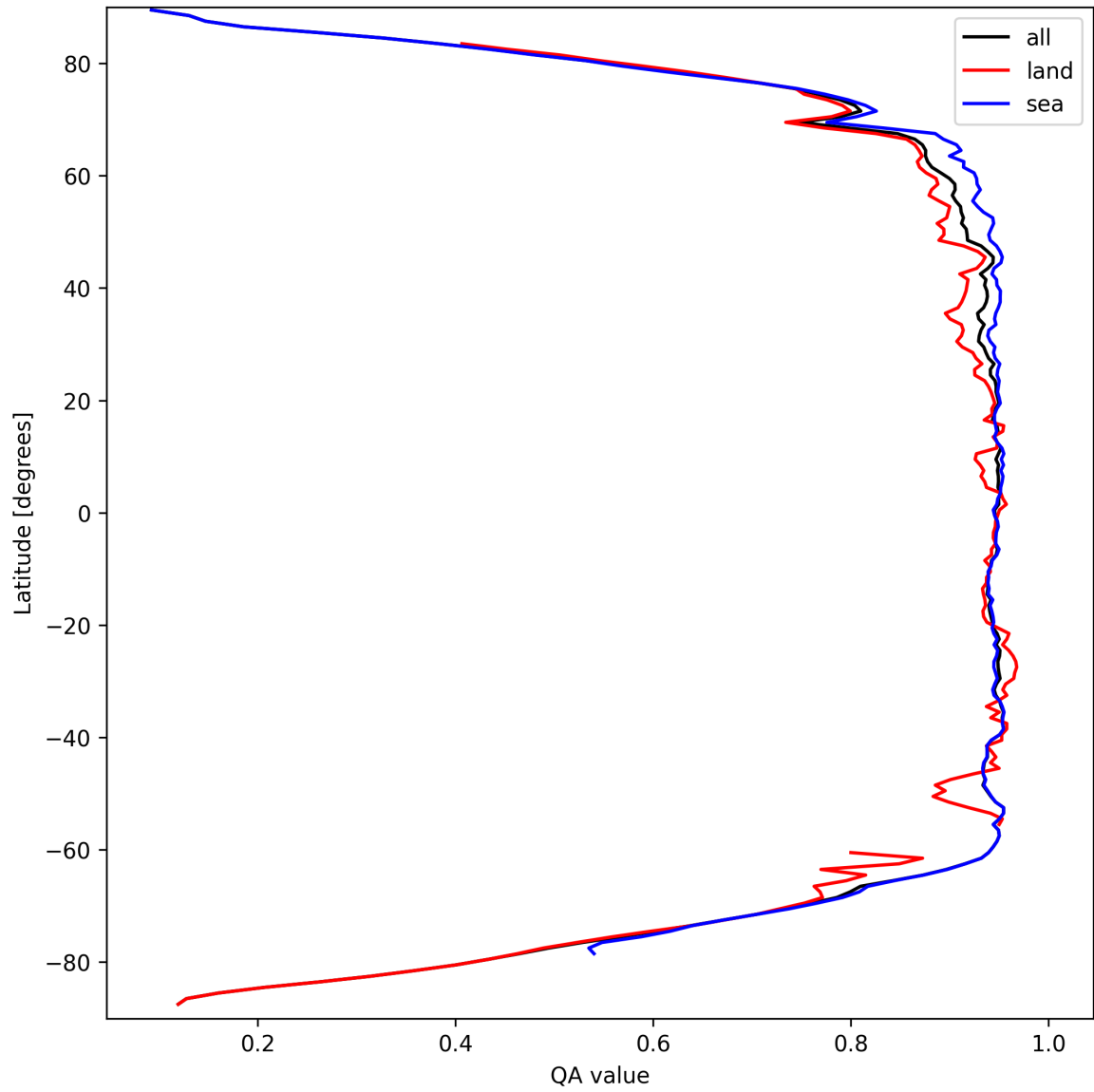
Figure 13: Zonal average of “QA value” for 2025-03-23 to 2025-03-24.
