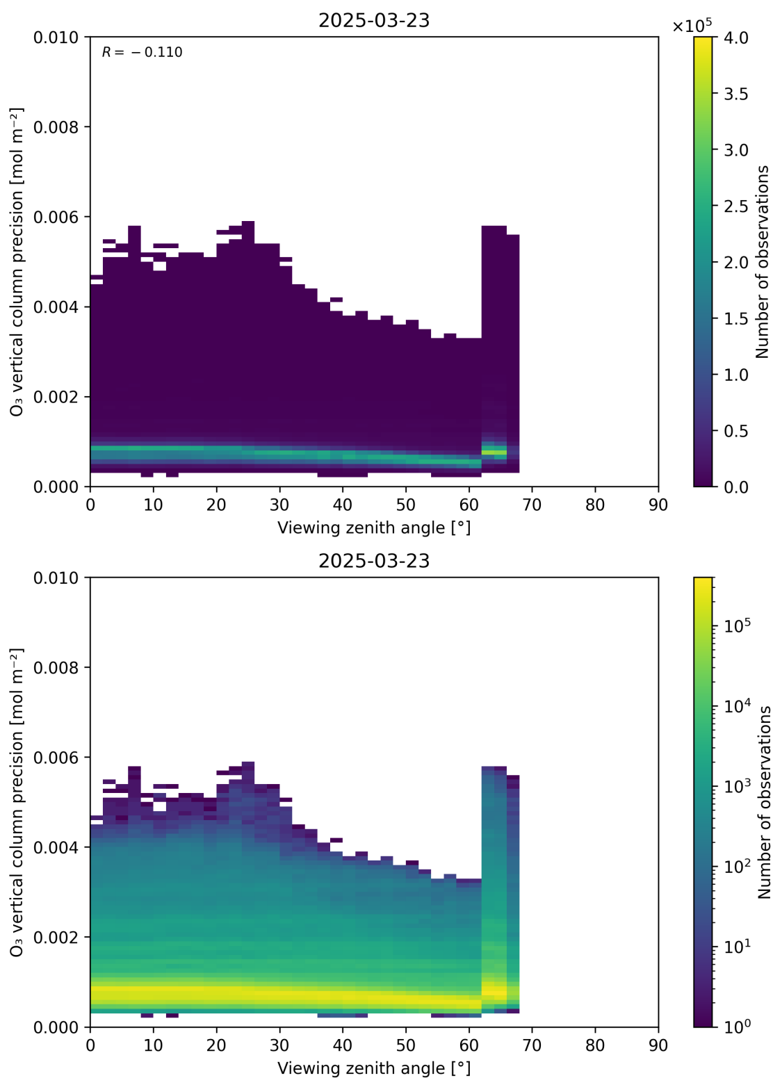
Figure 53: Scatter density plot of “Viewing zenith angle” against “O 3 vertical column precision” for 2025-03-23 to 2025-03-24.
