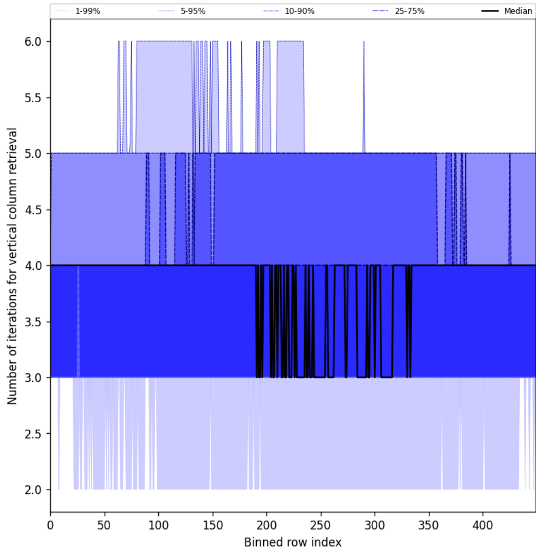
Figure 33: Along track statistics of “Number of iterations for vertical column retrieval” for 2025-03-23 to 2025-03-24
