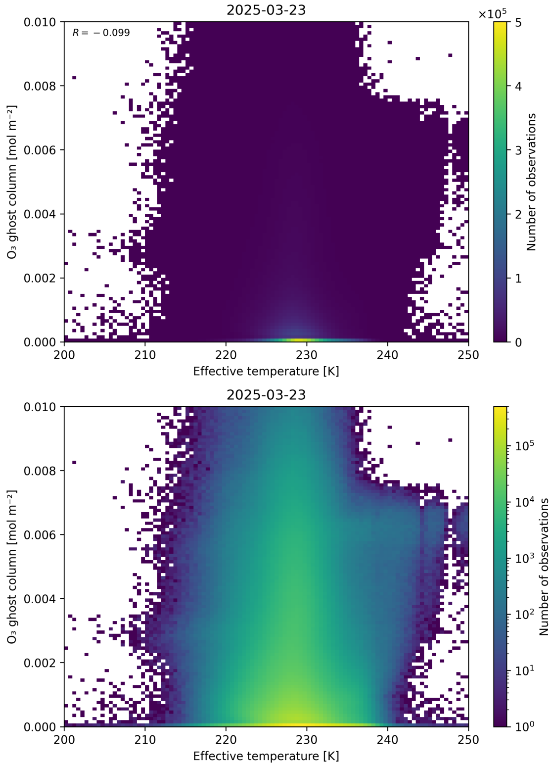
Figure 38: Scatter density plot of “Effective temperature” against “O 3 ghost column” for 2025-03-23 to 2025-03-24.
