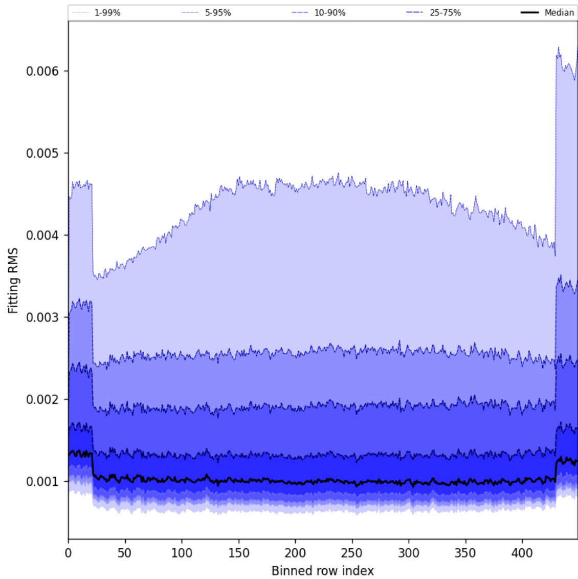
Figure 30: Along track statistics of “Fitting RMS” for 2025-03-23 to 2025-03-24
