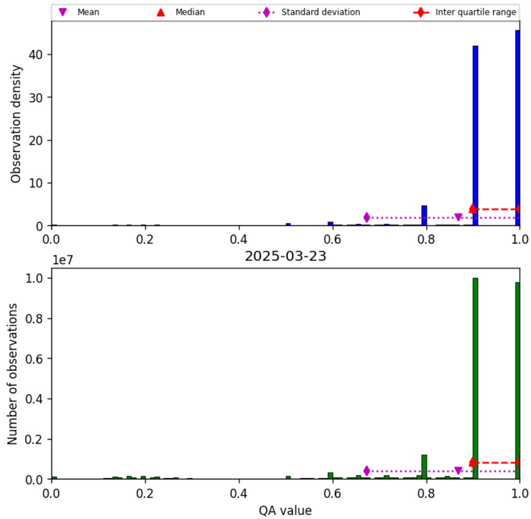
Figure 20: Histogram of “QA value” for 2025-03-23 to 2025-03-24
