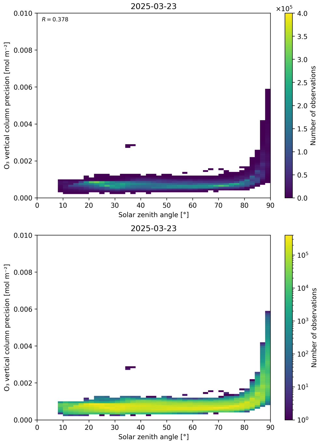
Figure 48: Scatter density plot of “Solar zenith angle” against “O 3 vertical column precision” for 2025-03-23 to 2025-03-24.
