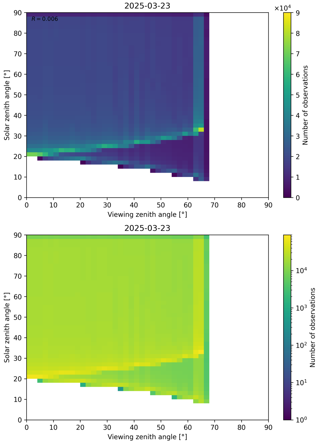
Figure 54: Scatter density plot of “Viewing zenith angle” against “Solar zenith angle” for 2025-03-23 to 2025-03-24.
