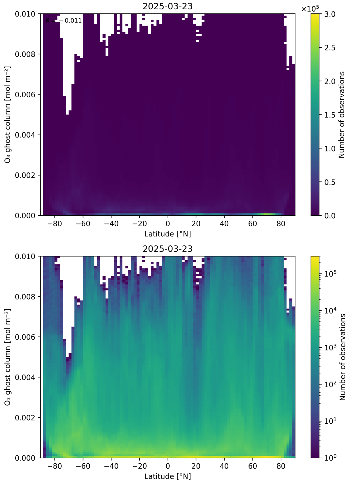
Figure 35: Scatter density plot of “Latitude” against “O 3 ghost column” for 2025-03-23 to 2025-03-24.
