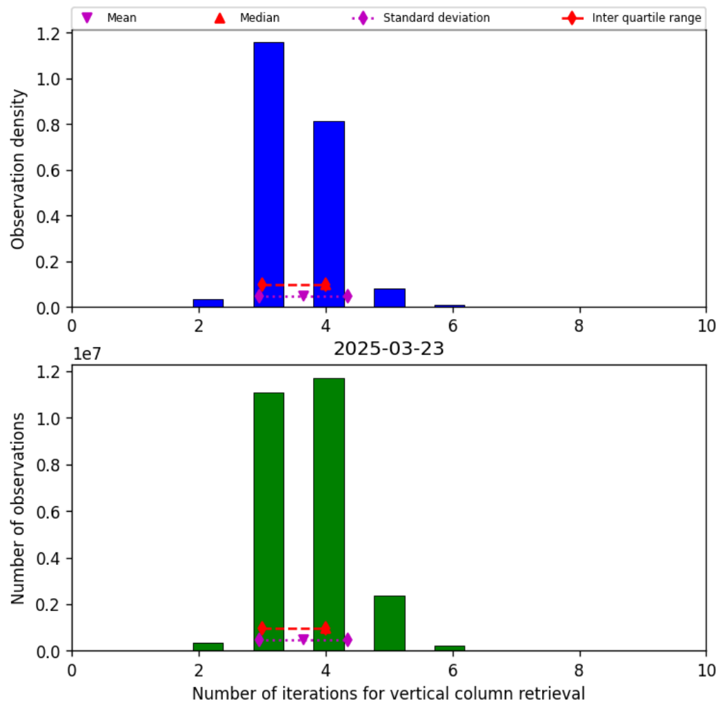
Figure 26: Histogram of “Number of iterations for vertical column retrieval” for 2025-03-23 to 2025-03-24
