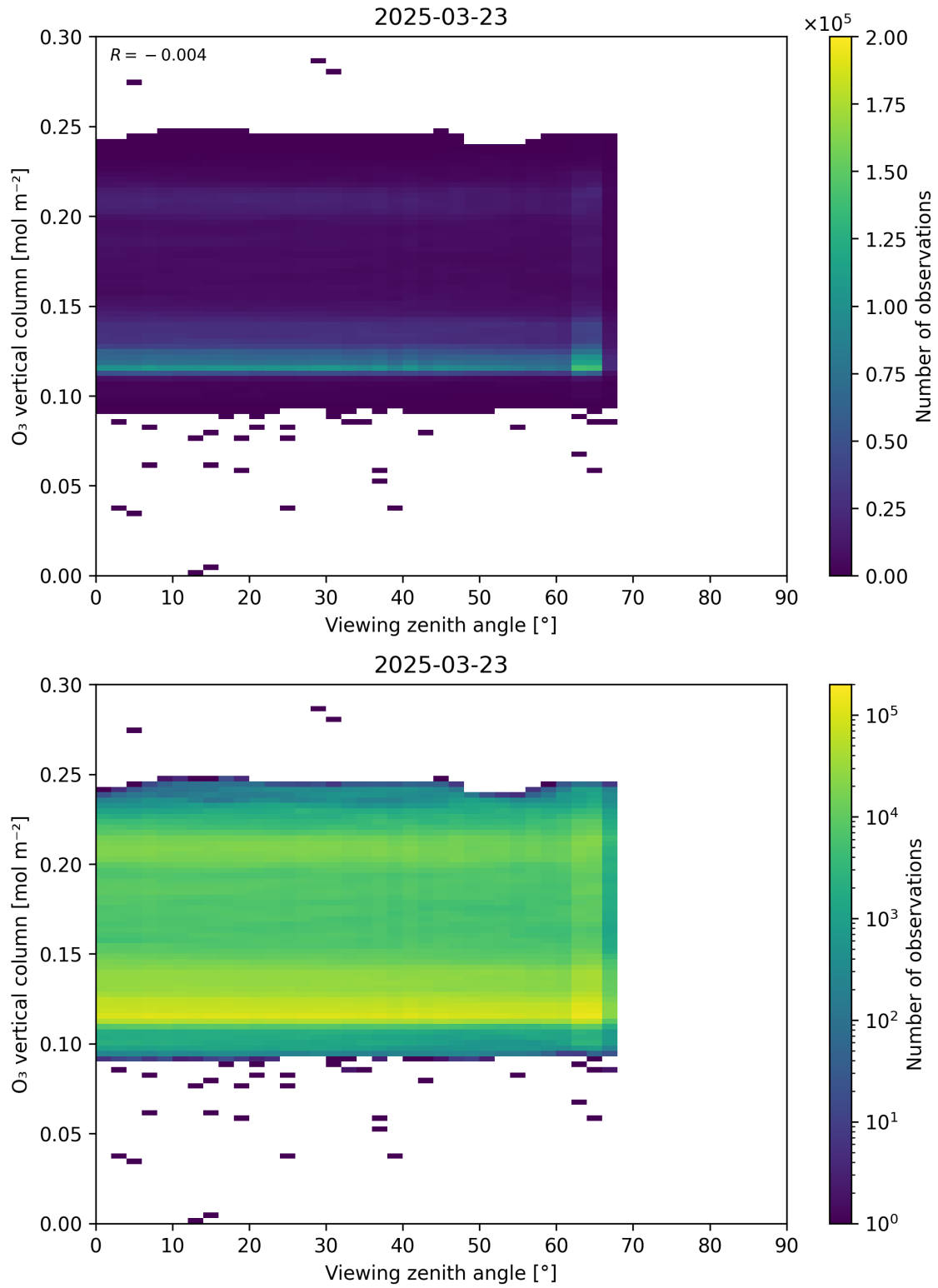
Figure 52: Scatter density plot of “Viewing zenith angle” against “O 3 vertical column” for 2025-03-23 to 2025-03-24.
