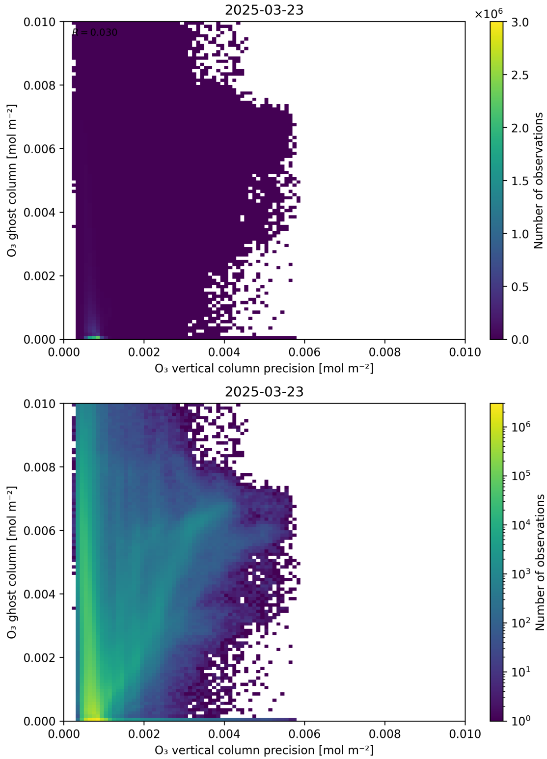
Figure 43: Scatter density plot of “O 3 vertical column precision” against “O 3 ghost column” for 2025-03-23 to 2025-03-24.
