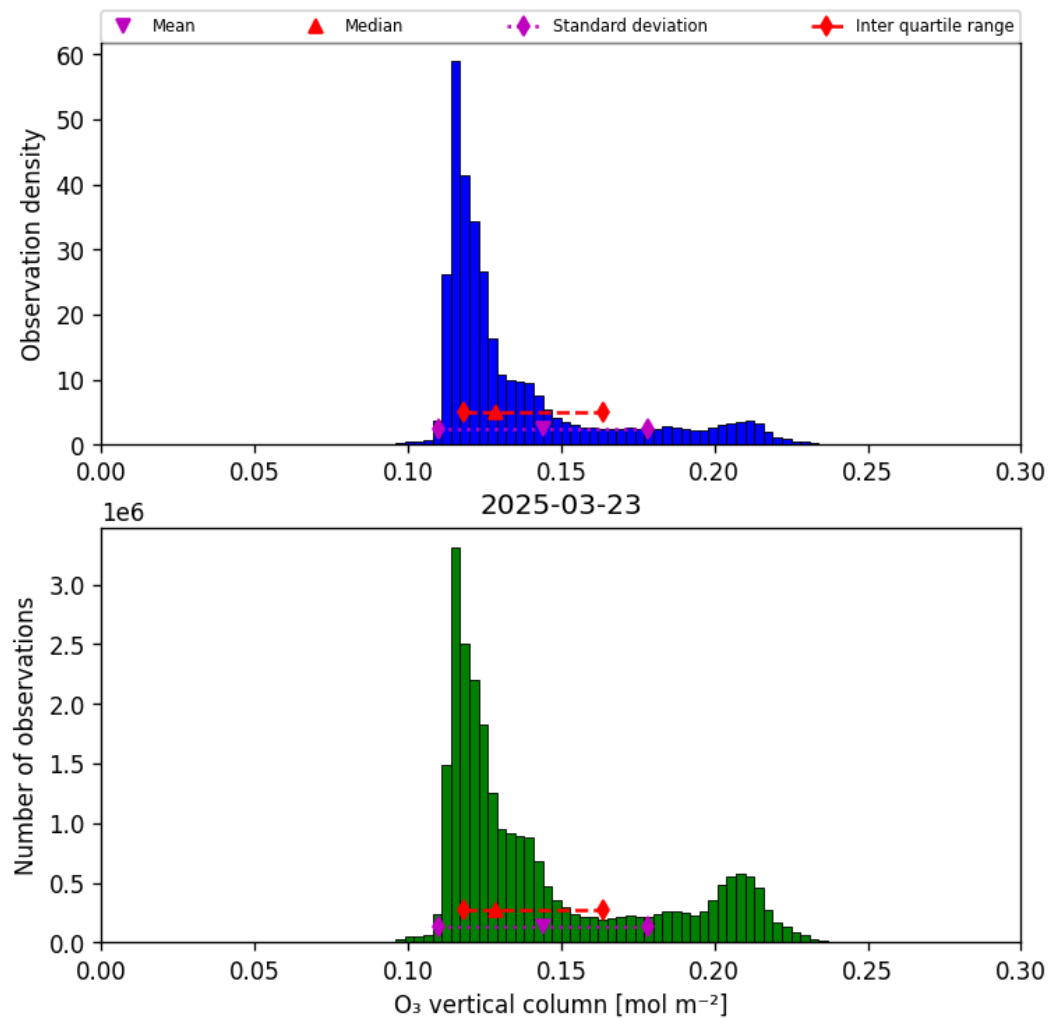
Figure 21: Histogram of “O 3 vertical column” for 2025-03-23 to 2025-03-24
