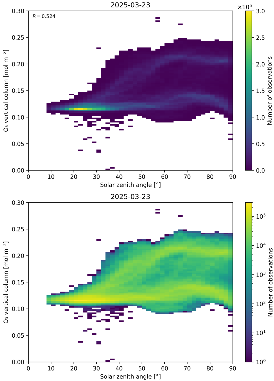
Figure 47: Scatter density plot of “Solar zenith angle” against “O 3 vertical column” for 2025-03-23 to 2025-03-24.
