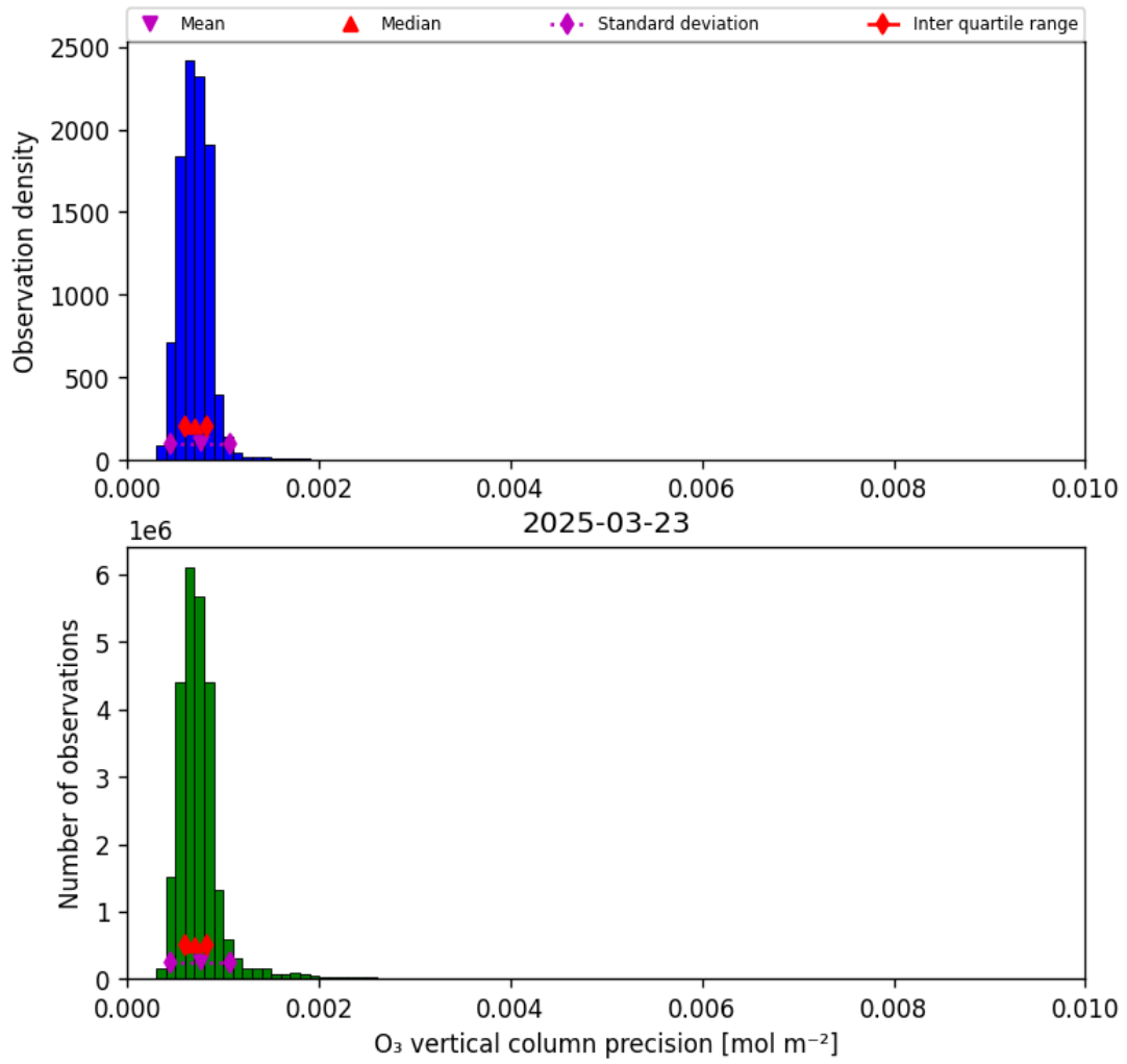
Figure 22: Histogram of “O 3 vertical column precision” for 2025-03-23 to 2025-03-24
