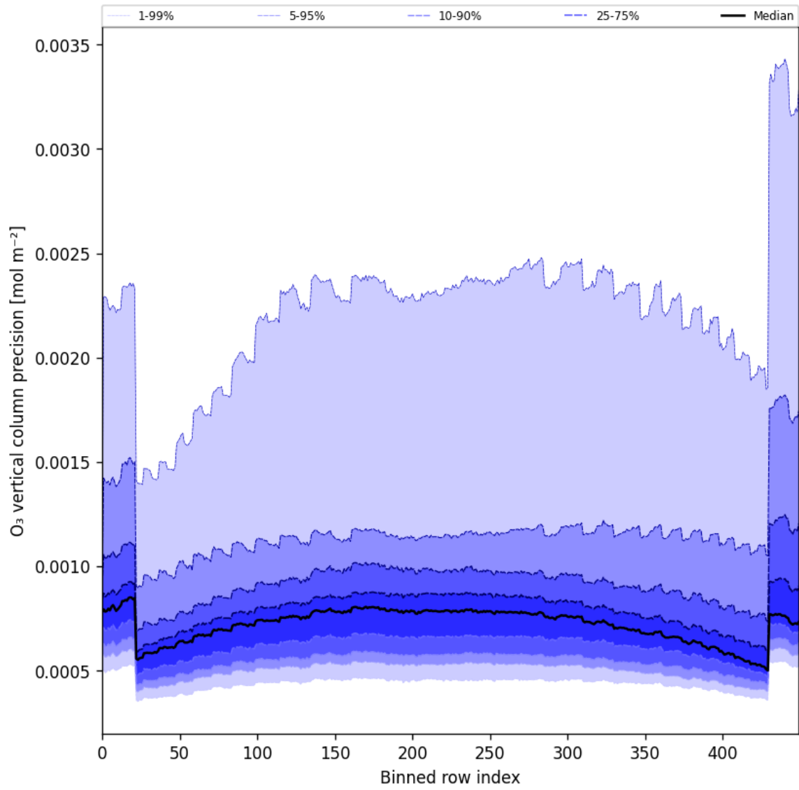
Figure 29: Along track statistics of “O 3 vertical column precision” for 2025-03-23 to 2025-03-24
