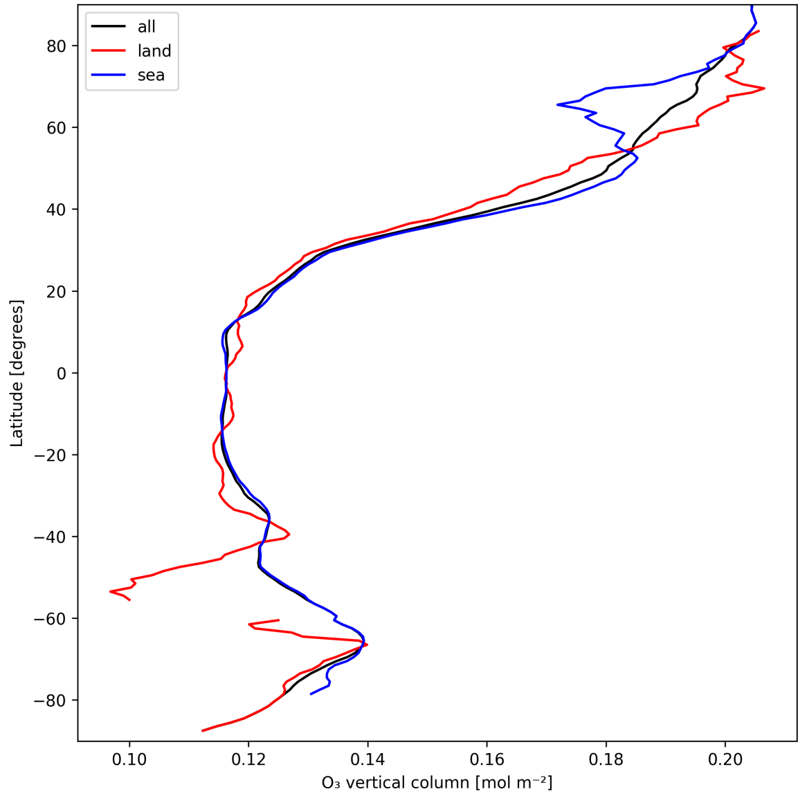
Figure 14: Zonal average of “O 3 vertical column” for 2025-03-23 to 2025-03-24.
