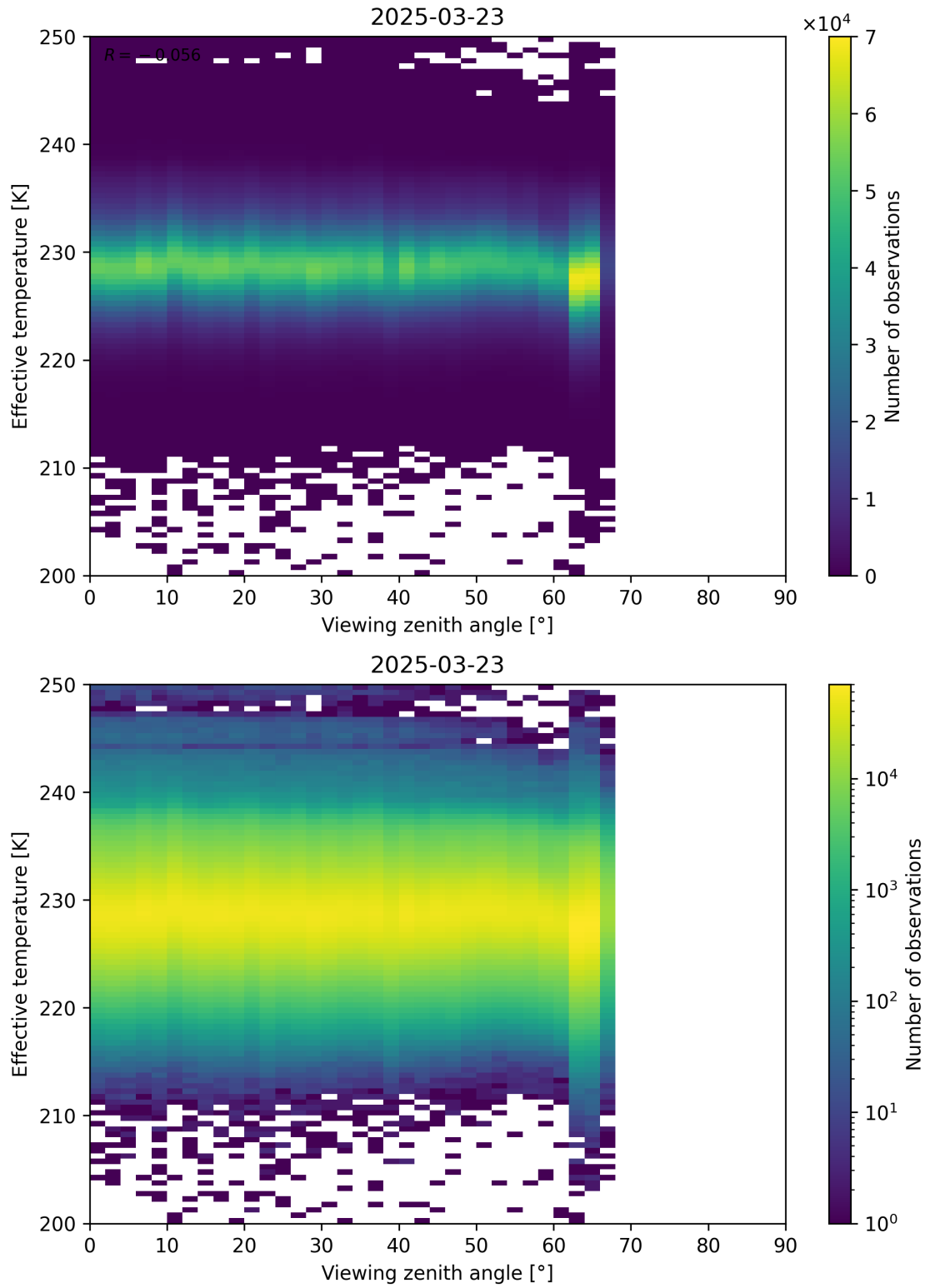
Figure 50: Scatter density plot of “Viewing zenith angle” against “Effective temperature” for 2025-03-23 to 2025-03-24.
