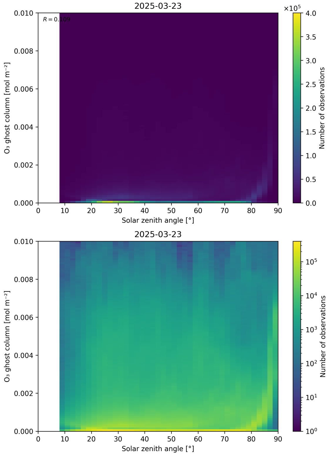
Figure 46: Scatter density plot of “Solar zenith angle” against “O 3 ghost column” for 2025-03-23 to 2025-03-24.
