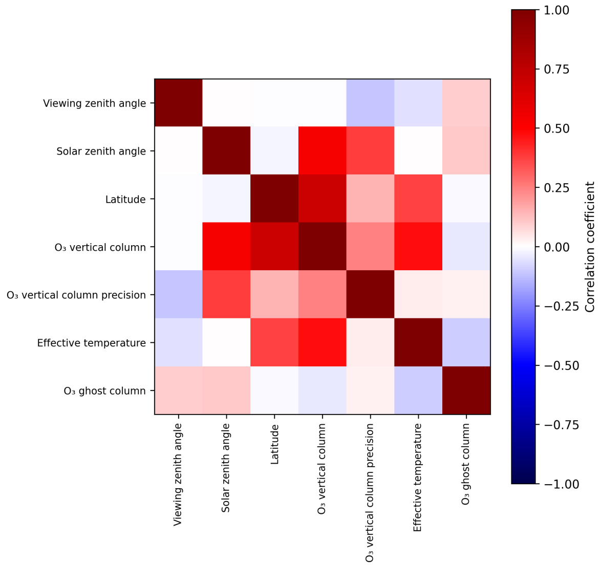
Figure 2: Map of correlation matrix for 2025-03-23 to 2025-03-24.
