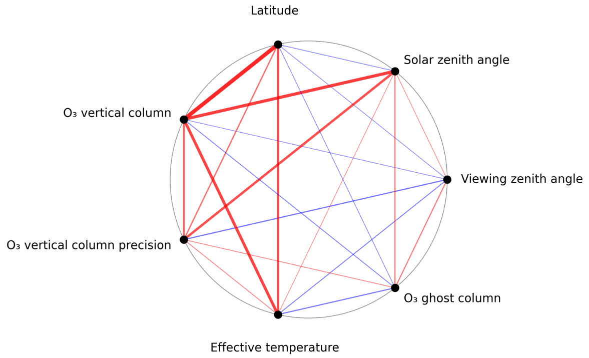
Figure 1: Map of correlation graph for 2025-03-23 to 2025-03-24.
