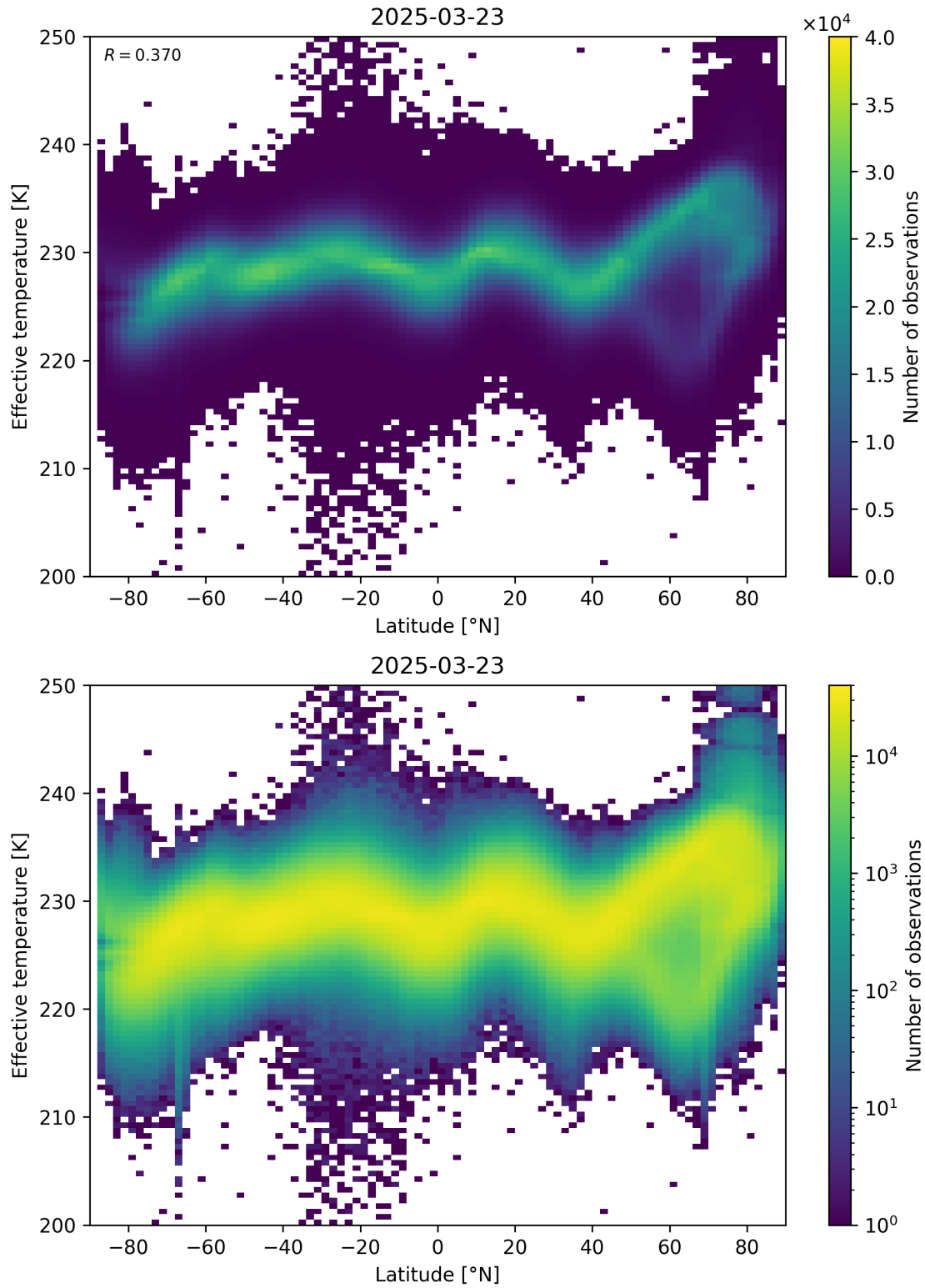
Figure 34: Scatter density plot of “Latitude” against “Effective temperature” for 2025-03-23 to 2025-03-24.
