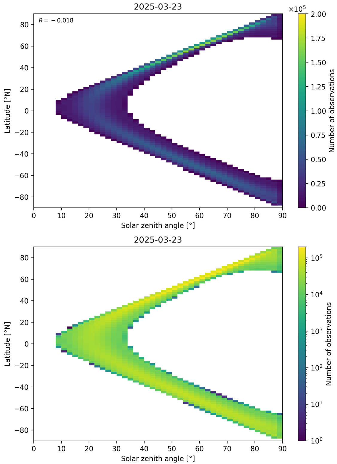
Figure 44: Scatter density plot of “Solar zenith angle” against “Latitude” for 2025-03-23 to 2025-03-24.
