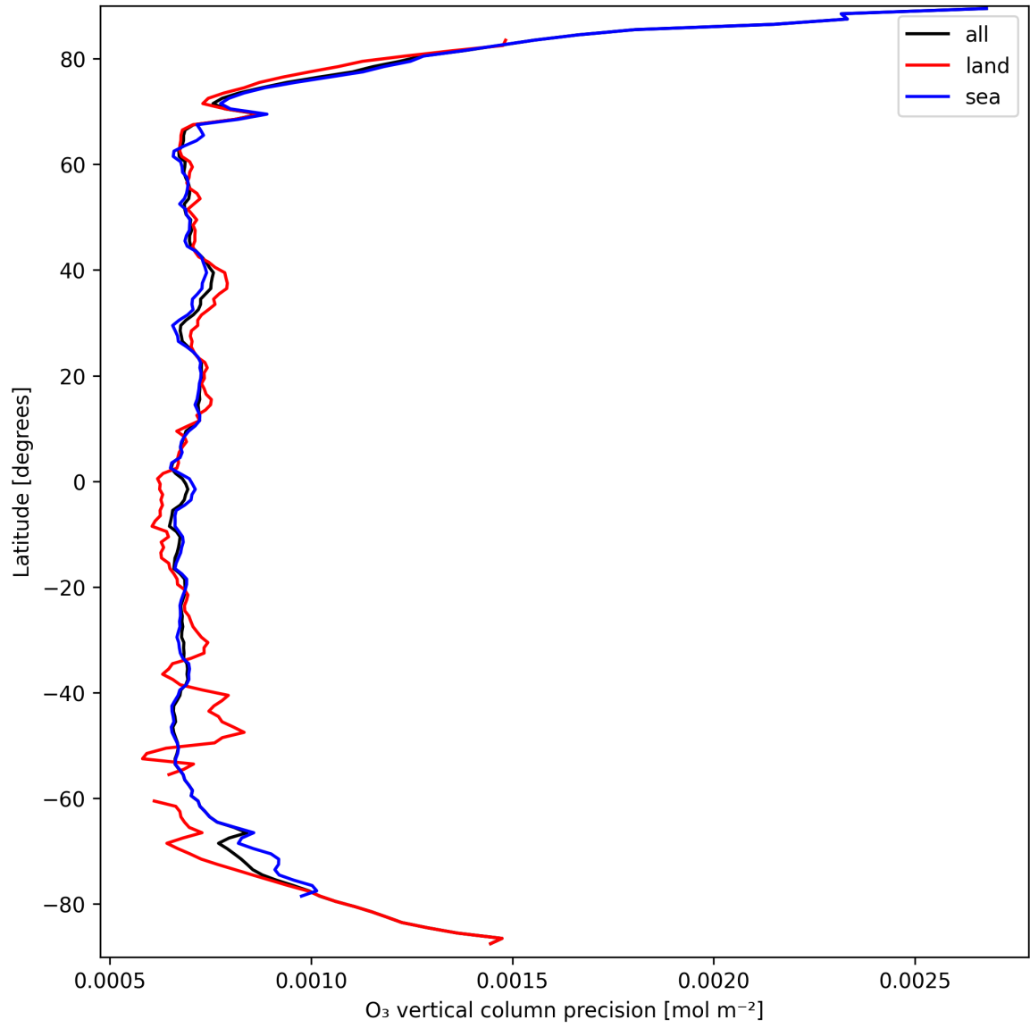
Figure 15: Zonal average of “O 3 vertical column precision” for 2025-03-23 to 2025-03-24.
