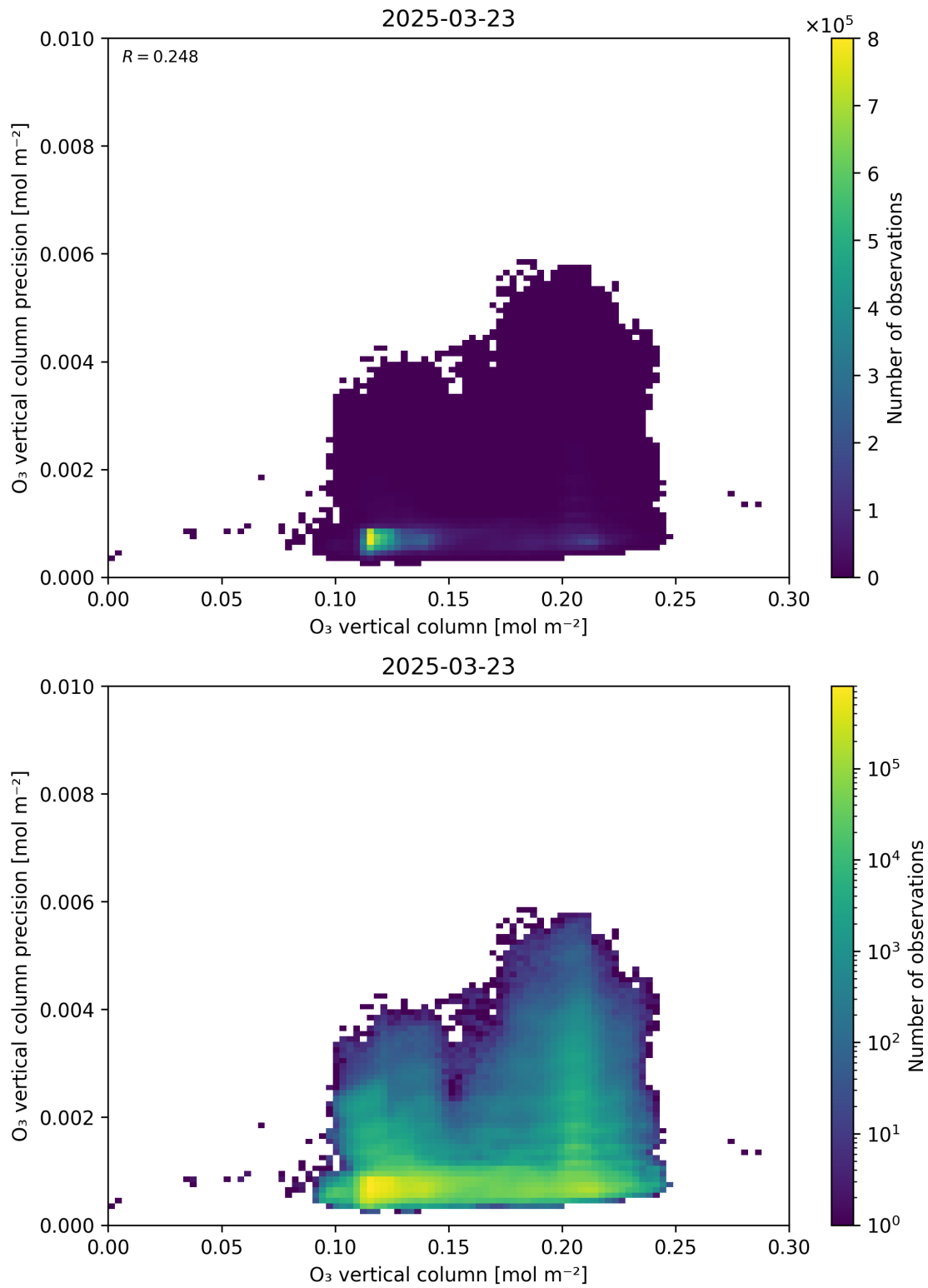
Figure 41: Scatter density plot of “O 3 vertical column” against “O 3 vertical column precision” for 2025-03-23 to 2025-03-24.
