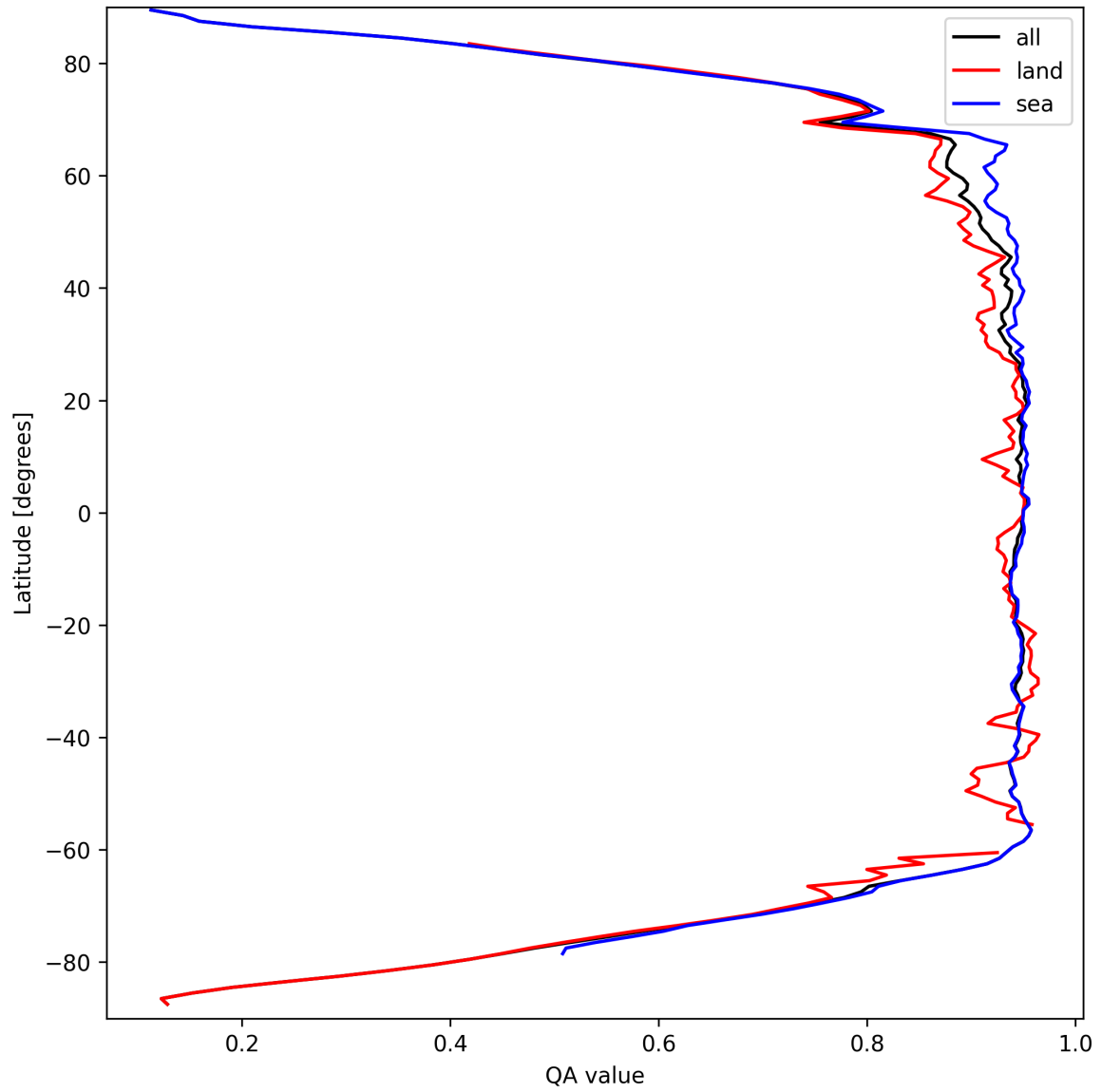
Figure 13: Zonal average of “QA value” for 2025-03-23 to 2025-03-25.
