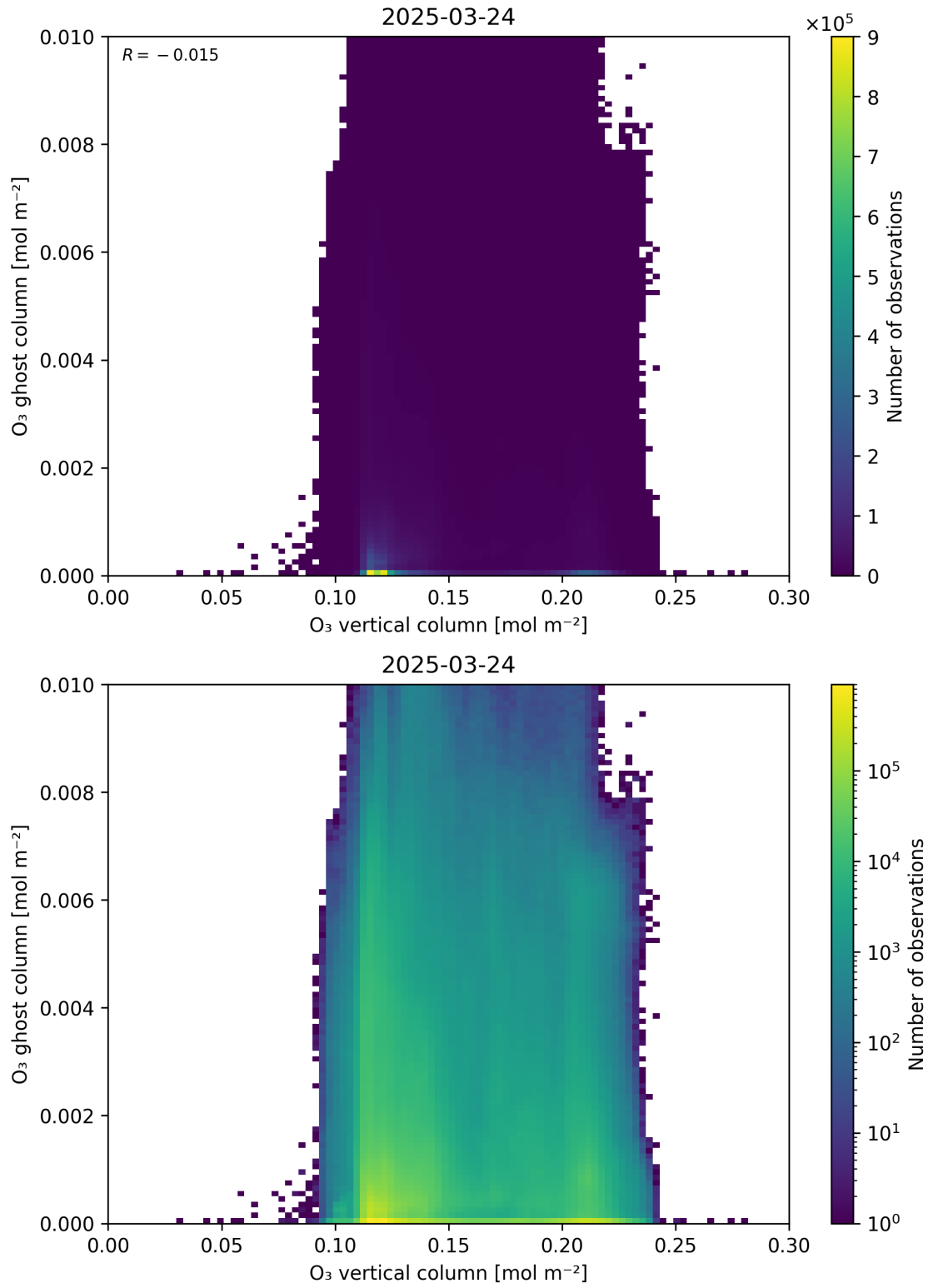
Figure 40: Scatter density plot of “ \text{O}_3 vertical column” against “ \text{O}_3 ghost column” for 2025-03-23 to 2025-03-25.
