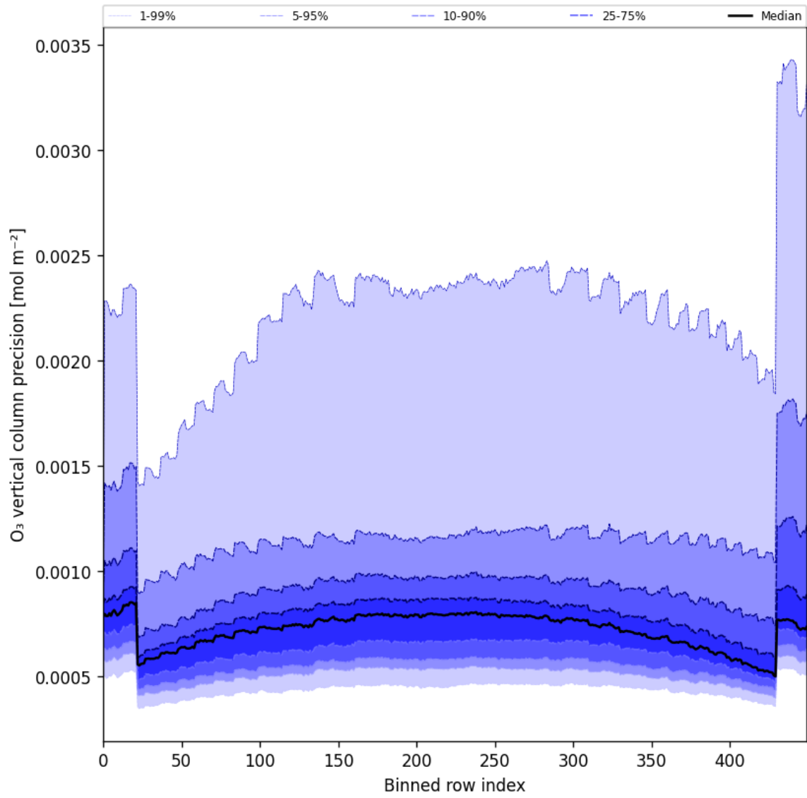
Figure 29: Along track statistics of “O 3 vertical column precision” for 2025-03-23 to 2025-03-25
