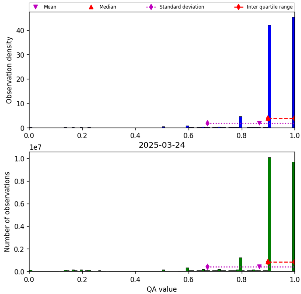
Figure 20: Histogram of “QA value” for 2025-03-23 to 2025-03-25
