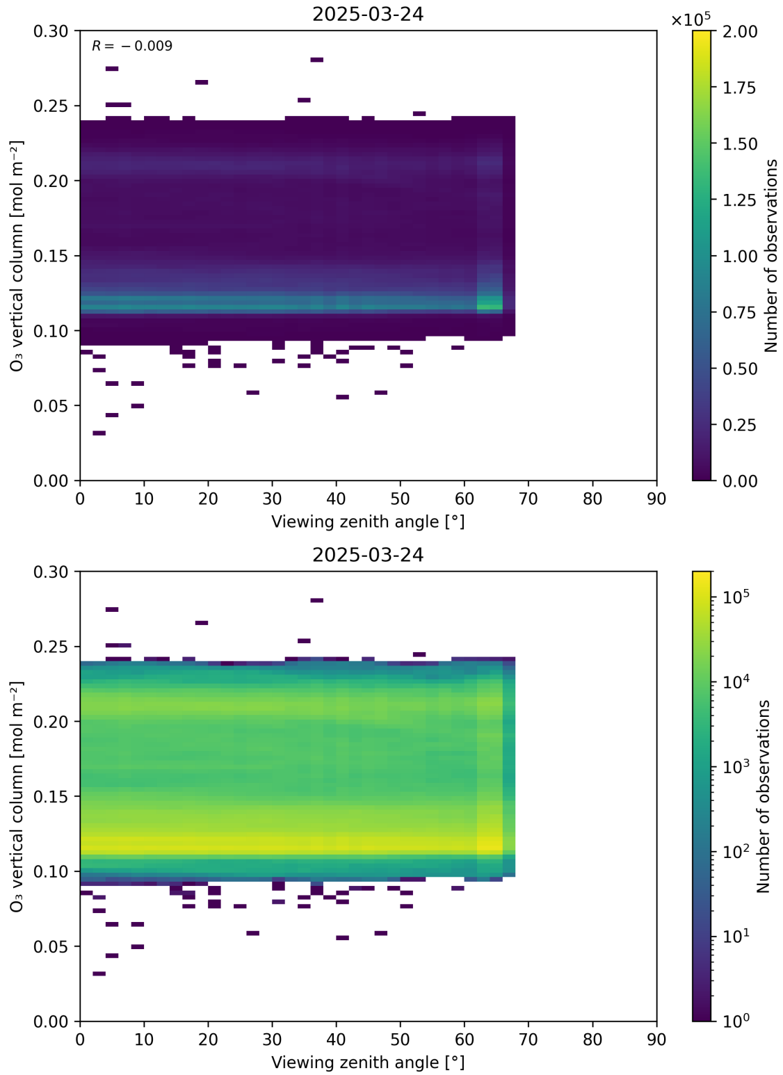
Figure 52: Scatter density plot of “Viewing zenith angle” against “O 3 vertical column” for 2025-03-23 to 2025-03-25.
