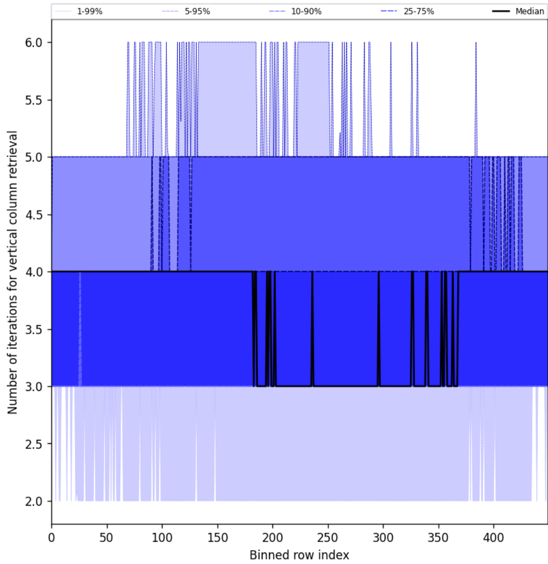
Figure 33: Along track statistics of “Number of iterations for vertical column retrieval” for 2025-03-23 to 2025-03-25
