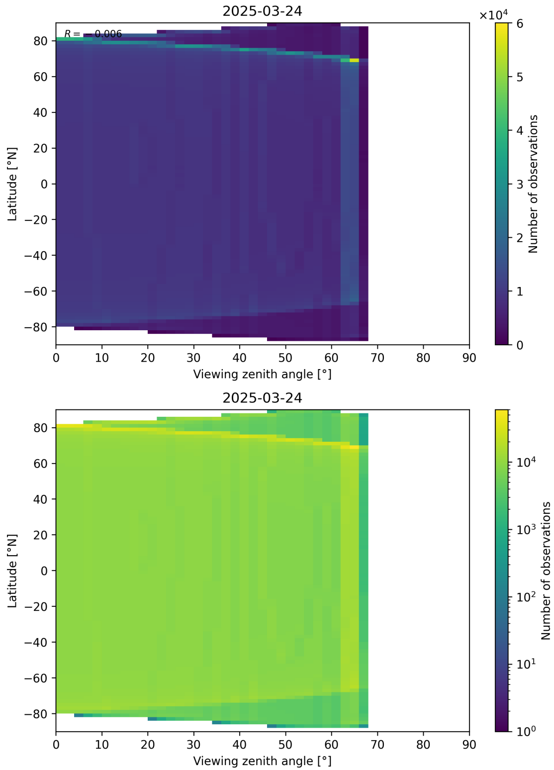
Figure 49: Scatter density plot of “Viewing zenith angle” against “Latitude” for 2025-03-23 to 2025-03-25.
