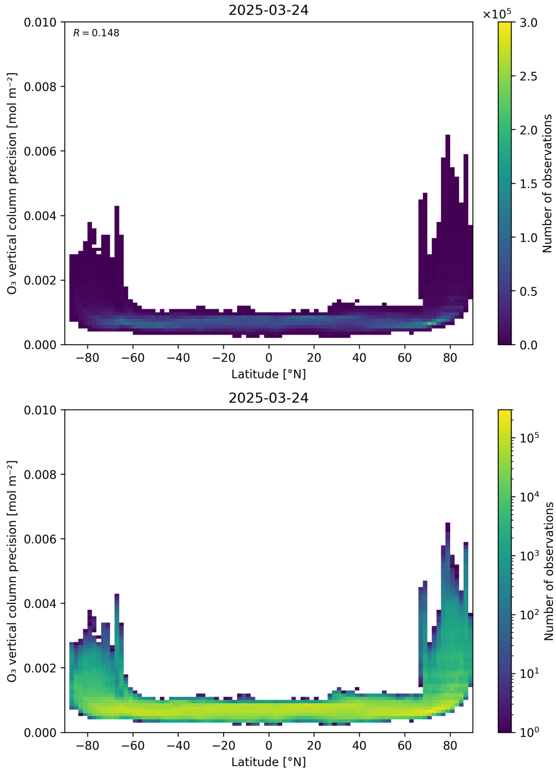
Figure 37: Scatter density plot of “Latitude” against “O 3 vertical column precision” for 2025-03-23 to 2025-03-25.
