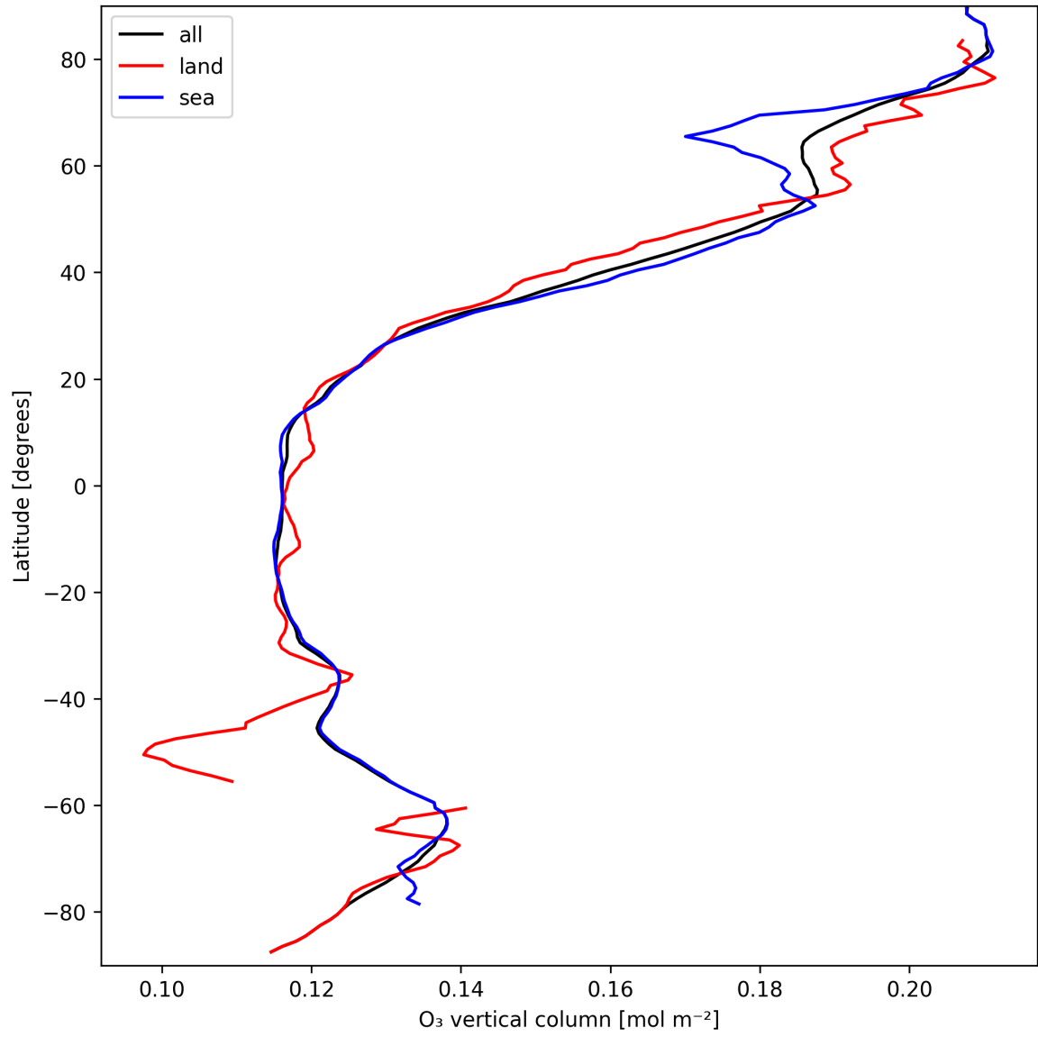
Figure 14: Zonal average of “O 3 vertical column” for 2025-03-23 to 2025-03-25.
