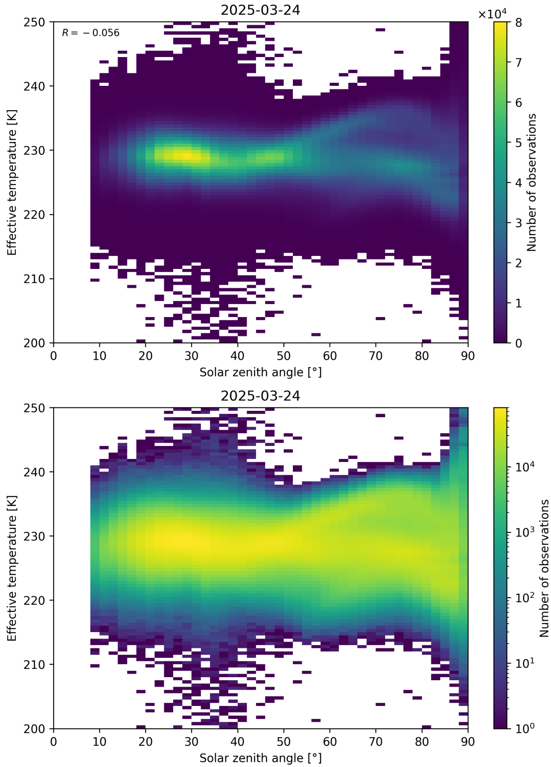
Figure 45: Scatter density plot of “Solar zenith angle” against “Effective temperature” for 2025-03-23 to 2025-03-25.
