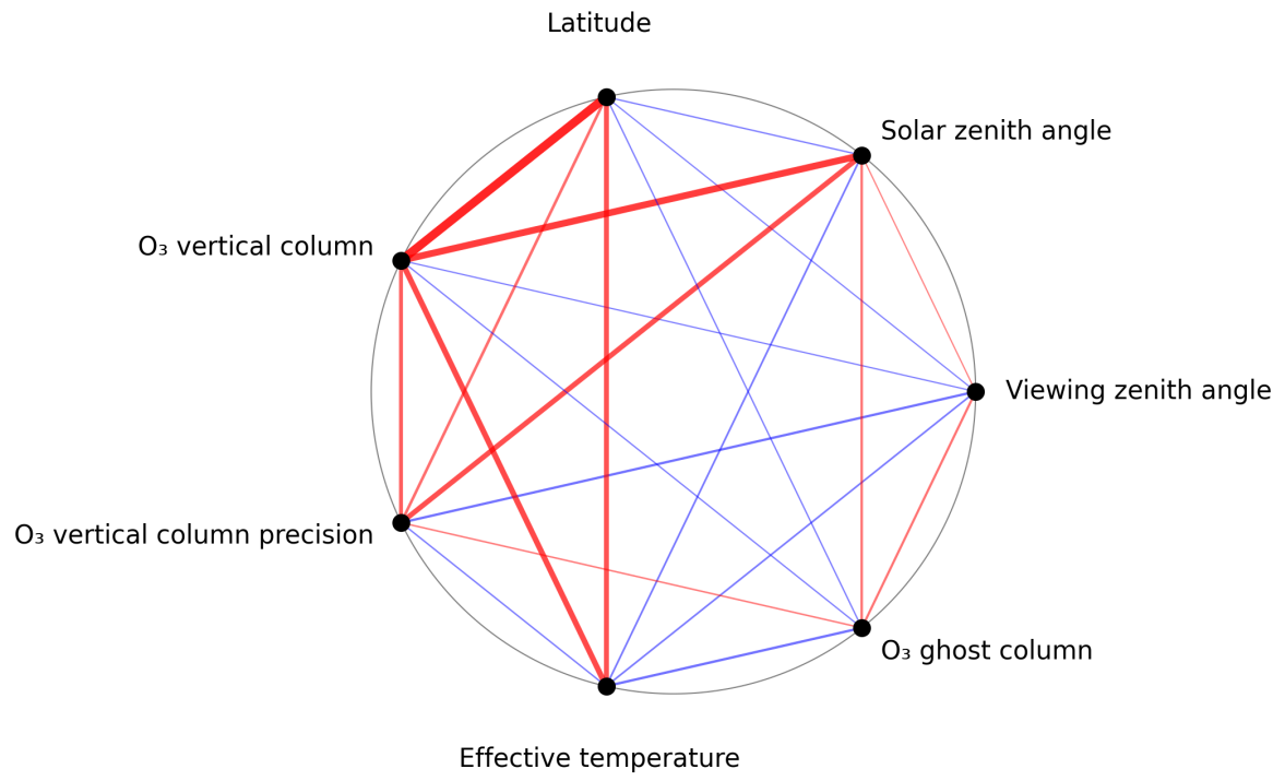
Figure 1: Map of correlation graph for 2025-03-23 to 2025-03-25.
