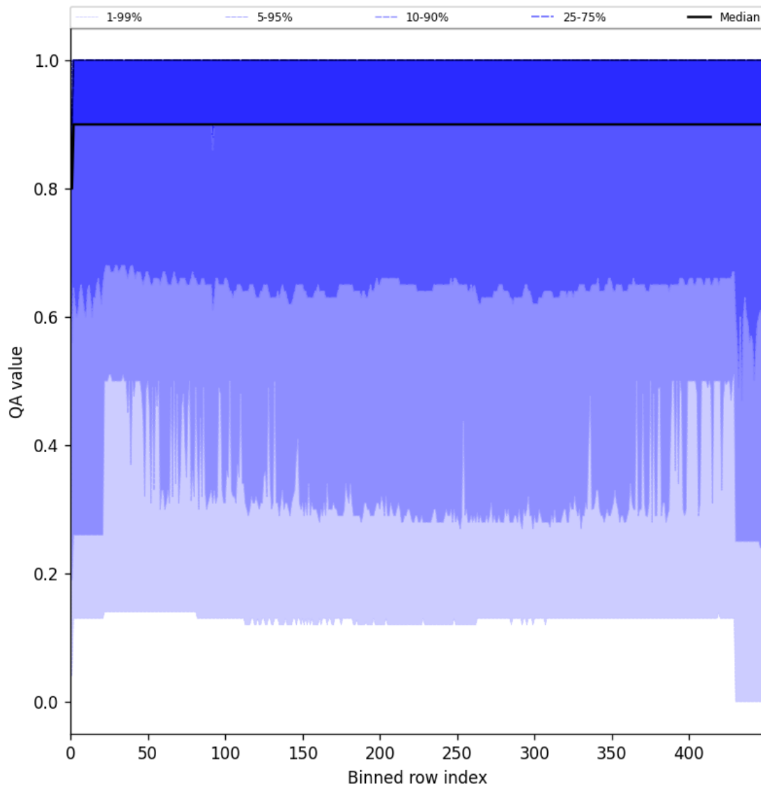
Figure 27: Along track statistics of “QA value” for 2025-03-23 to 2025-03-25
