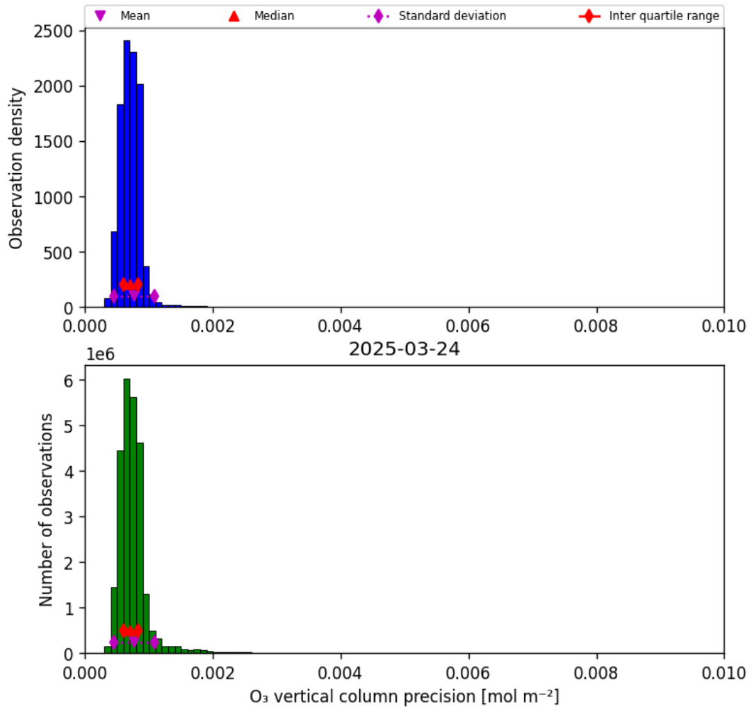
Figure 22: Histogram of “O 3 vertical column precision” for 2025-03-23 to 2025-03-25
