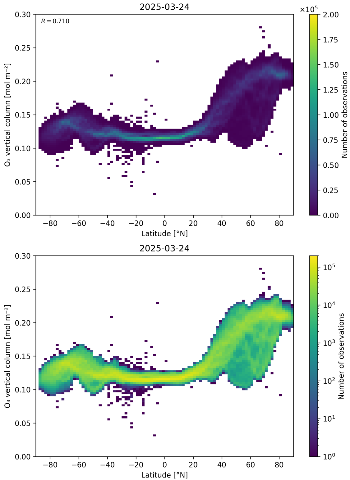
Figure 36: Scatter density plot of “Latitude” against “O 3 vertical column” for 2025-03-23 to 2025-03-25.
