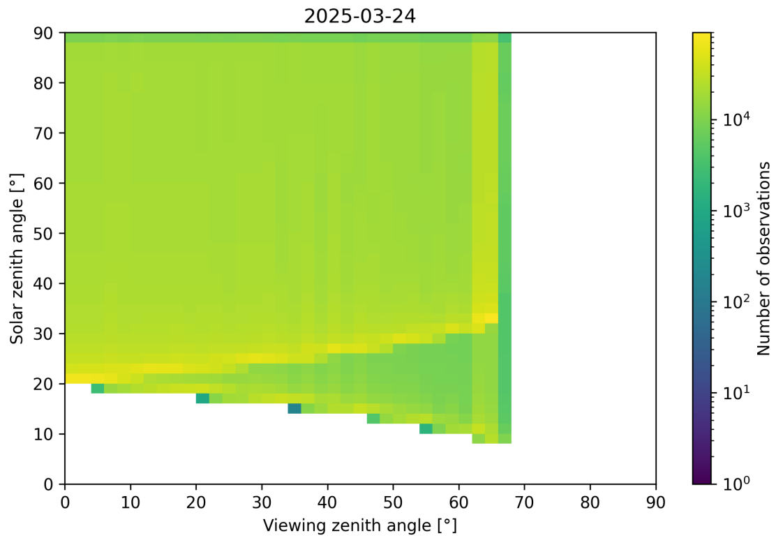
Figure 54: Scatter density plot of “Viewing zenith angle” against “Solar zenith angle” for 2025-03-23 to 2025-03-25.
