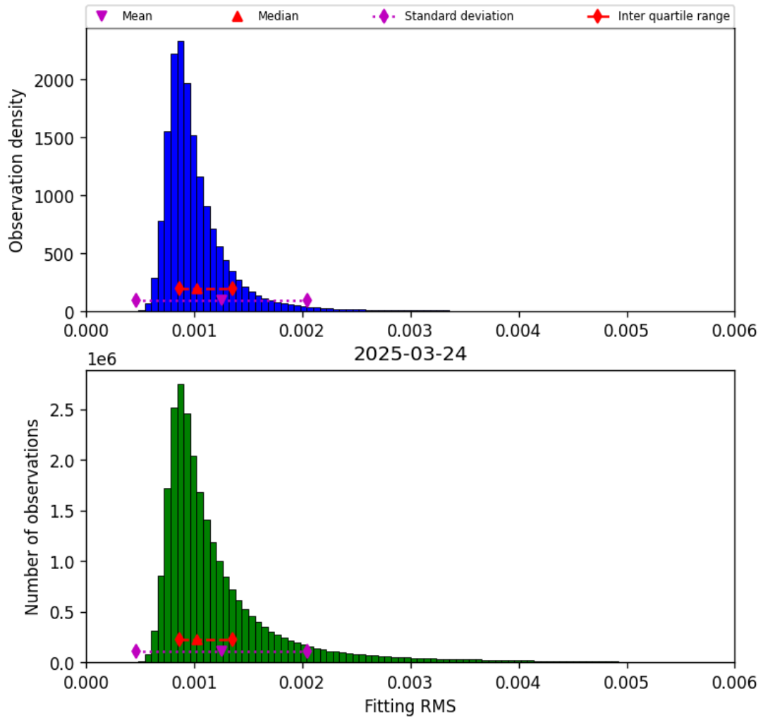
Figure 23: Histogram of “Fitting RMS” for 2025-03-23 to 2025-03-25
