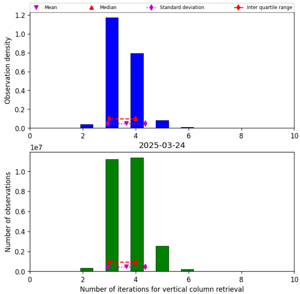
Figure 26: Histogram of “Number of iterations for vertical column retrieval” for 2025-03-23 to 2025-03-25
