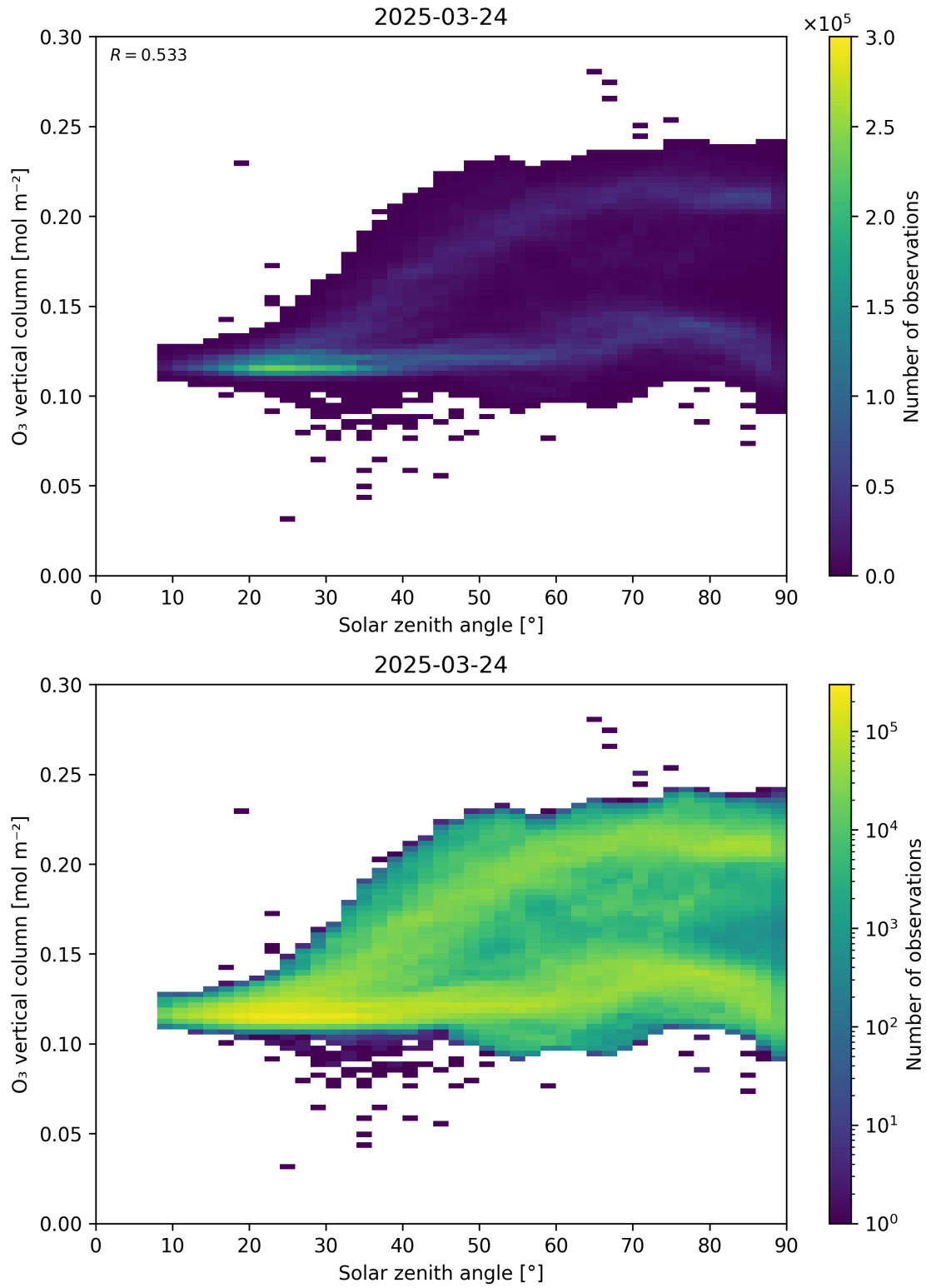
Figure 47: Scatter density plot of “Solar zenith angle” against “O 3 vertical column” for 2025-03-23 to 2025-03-25.
