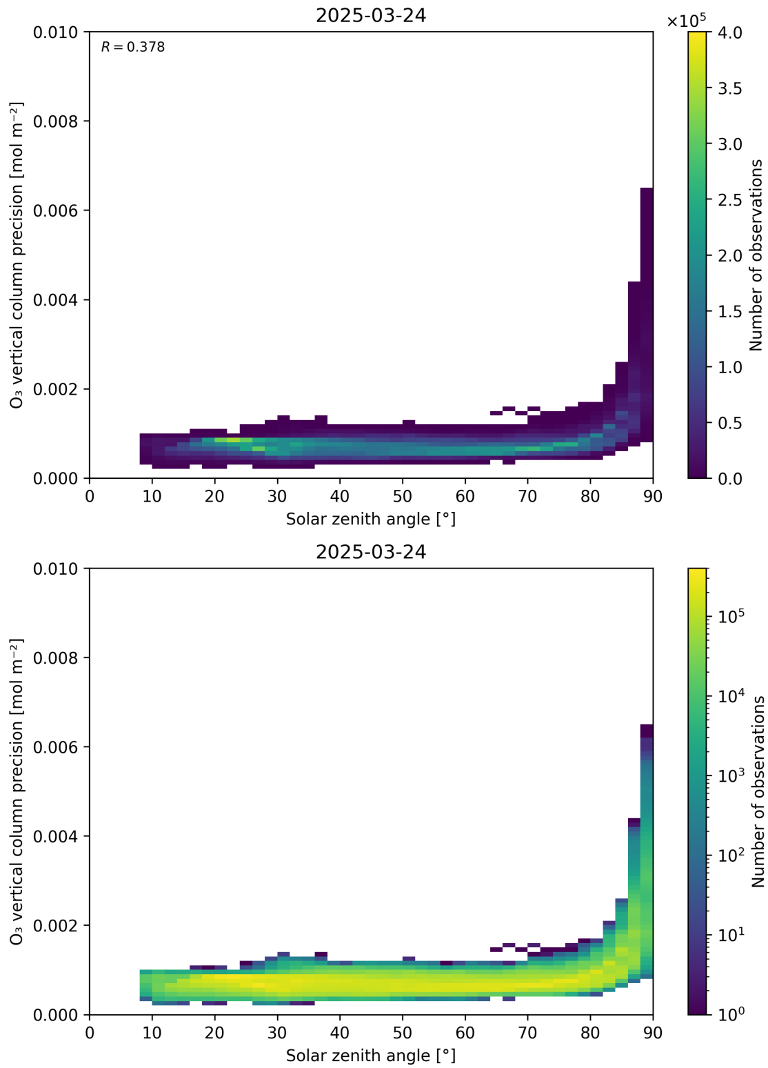
Figure 48: Scatter density plot of “Solar zenith angle” against “O 3 vertical column precision” for 2025-03-23 to 2025-03-25.
