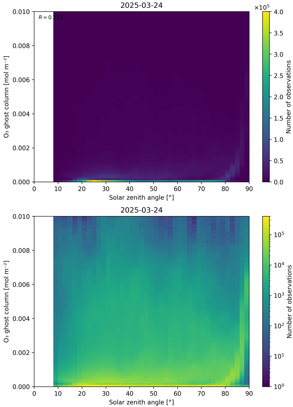
Figure 46: Scatter density plot of “Solar zenith angle” against “O 3 ghost column” for 2025-03-23 to 2025-03-25.
