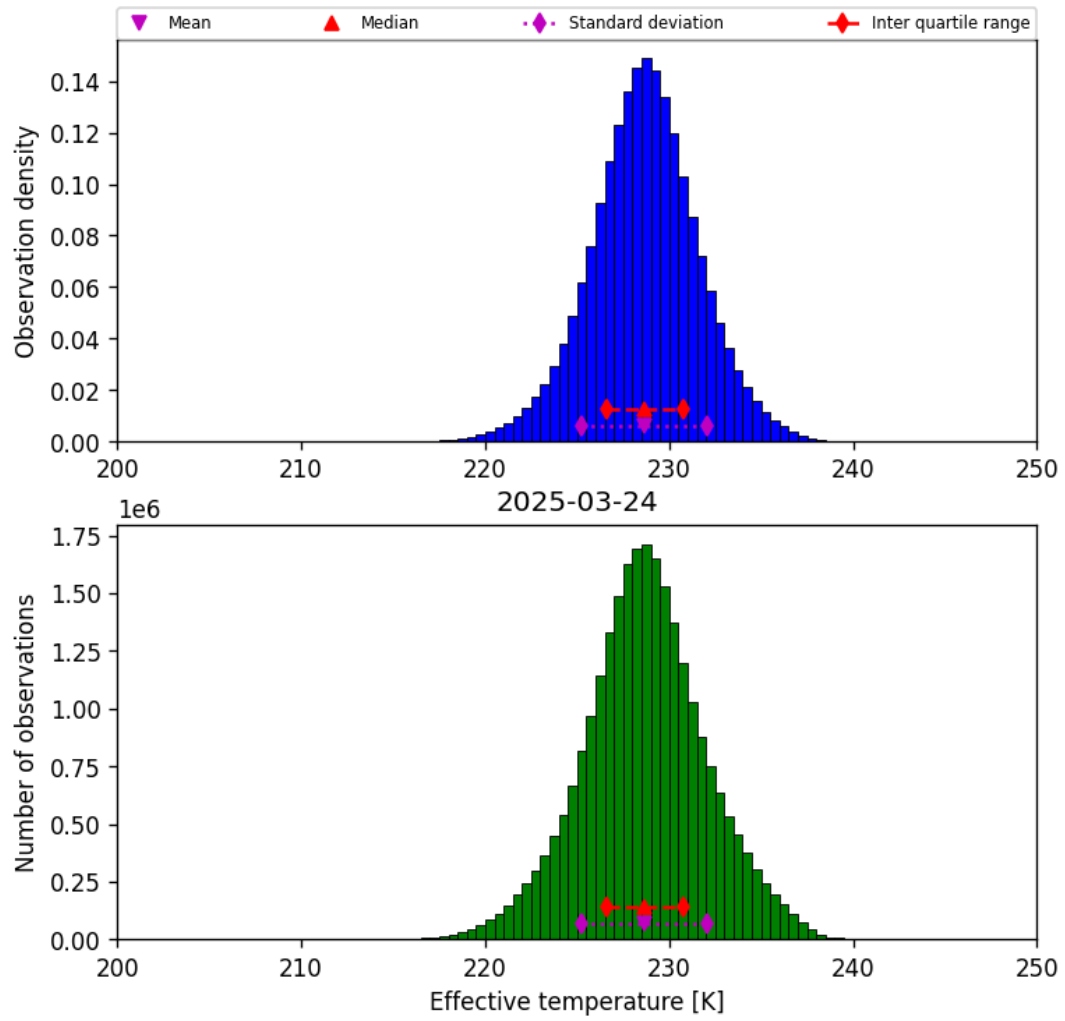
Figure 24: Histogram of “Effective temperature” for 2025-03-23 to 2025-03-25
