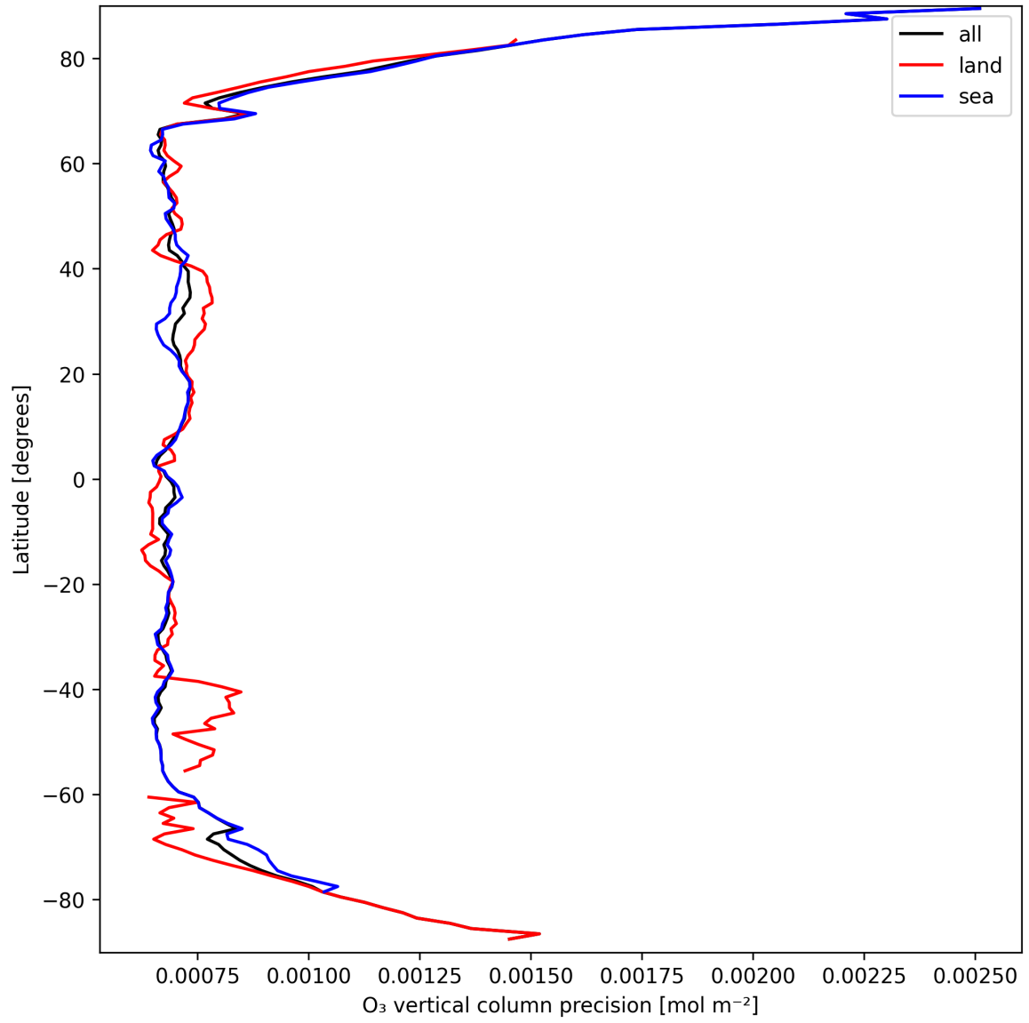
Figure 15: Zonal average of “O 3 vertical column precision” for 2025-03-23 to 2025-03-25.
