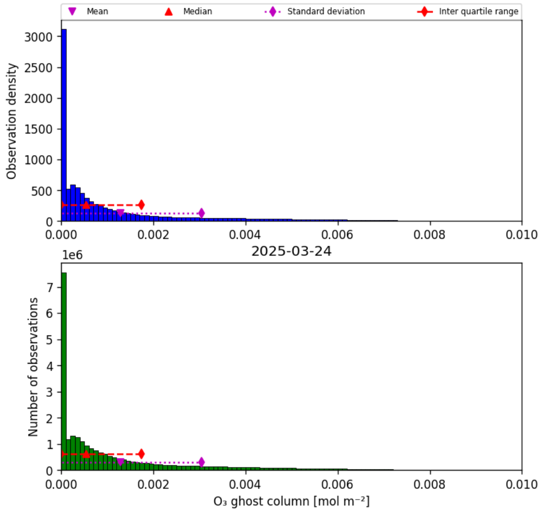
Figure 25: Histogram of “O 3 ghost column” for 2025-03-23 to 2025-03-25
