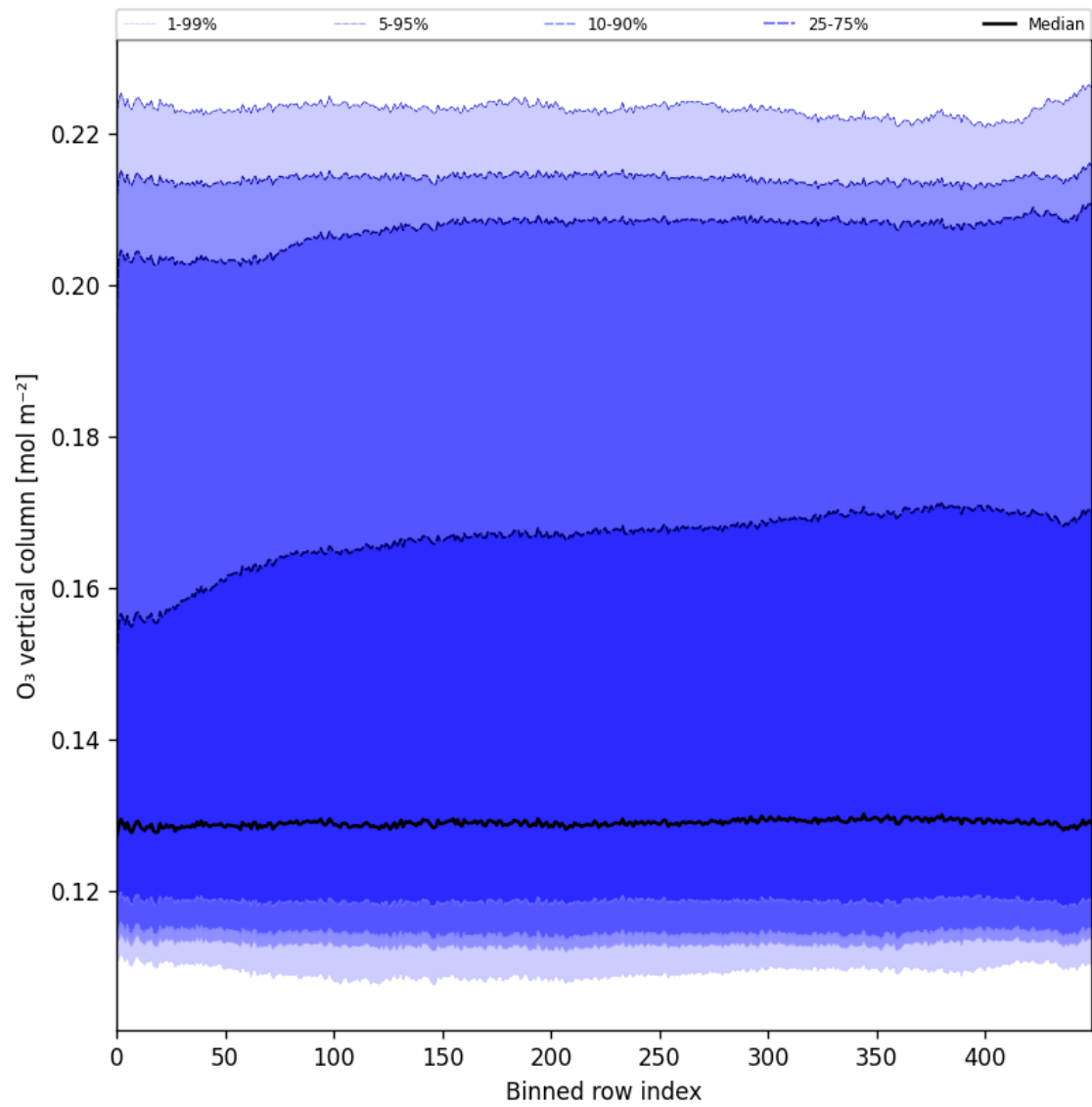
Figure 28: Along track statistics of “O 3 vertical column” for 2025-03-23 to 2025-03-25
