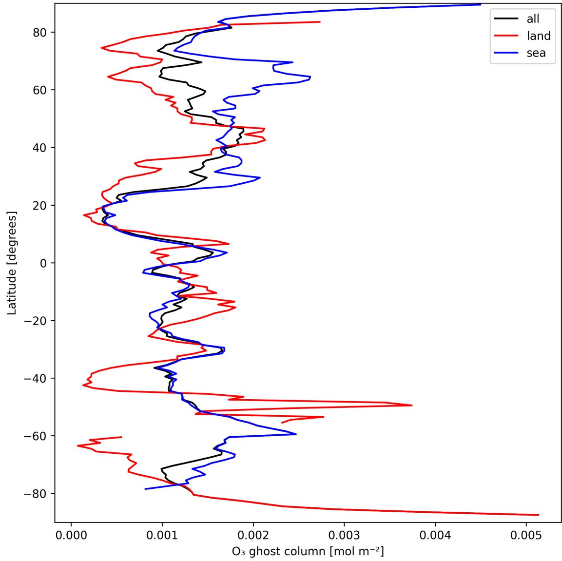
Figure 18: Zonal average of “O 3 ghost column” for 2025-03-23 to 2025-03-25.
