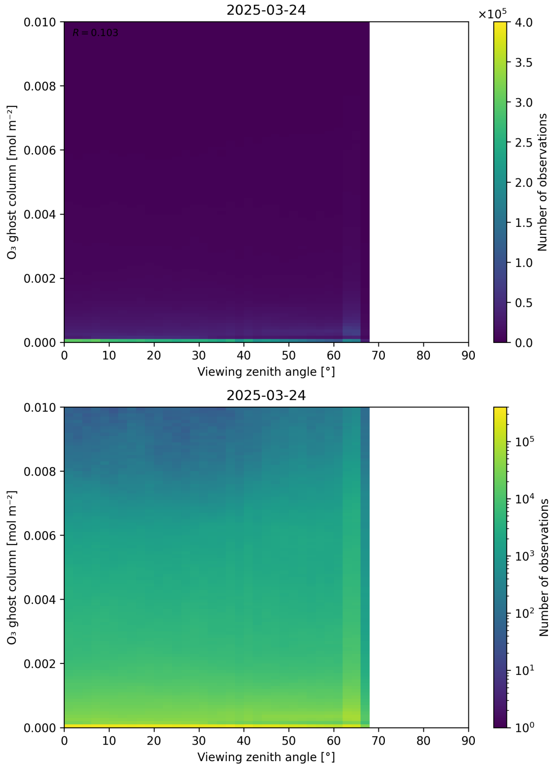
Figure 51: Scatter density plot of “Viewing zenith angle” against “O 3 ghost column” for 2025-03-23 to 2025-03-25.
