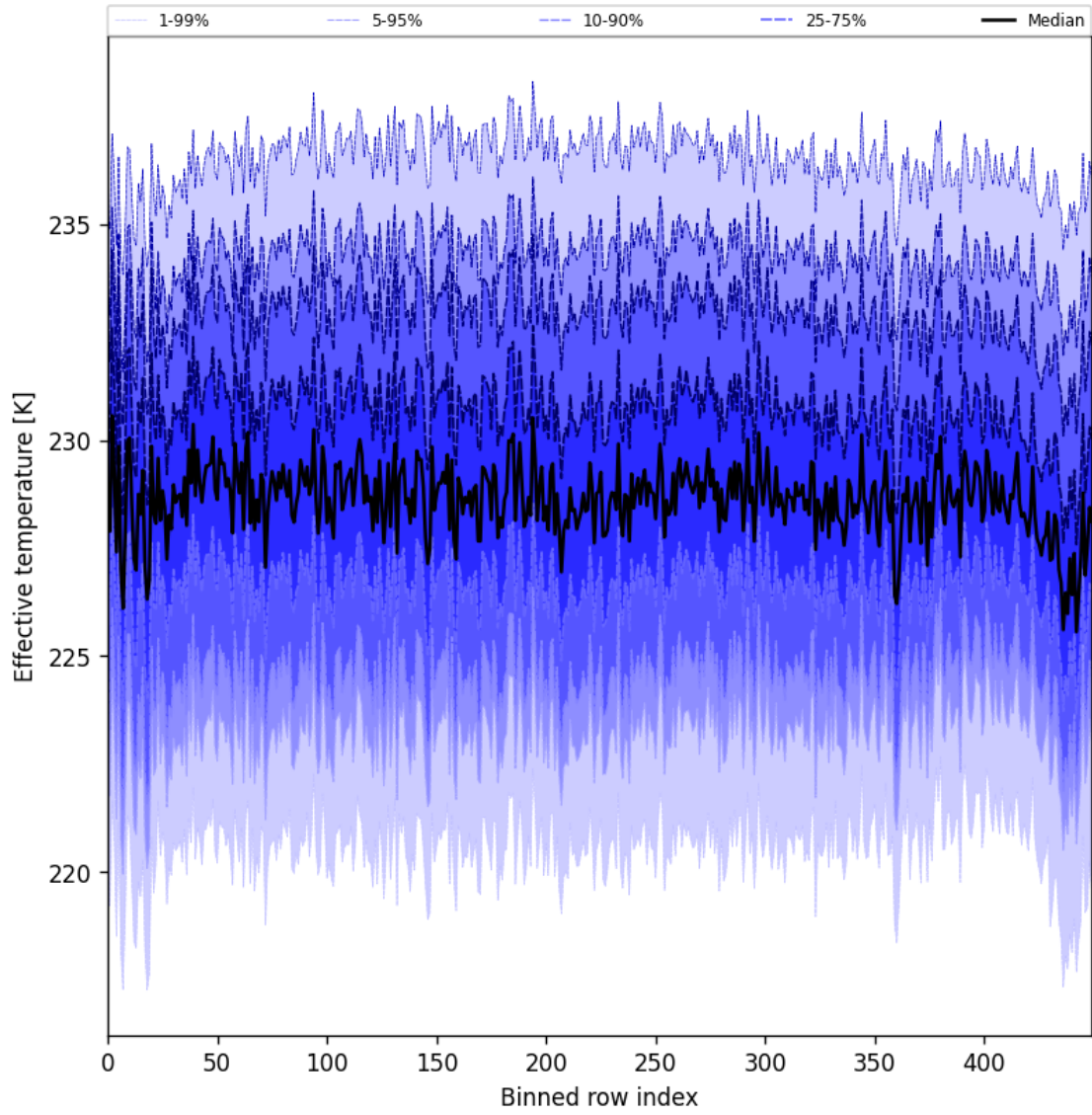
Figure 31: Along track statistics of “Effective temperature” for 2025-03-23 to 2025-03-25
