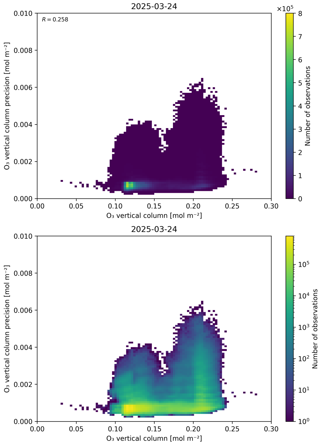
Figure 41: Scatter density plot of “O 3 vertical column” against “O 3 vertical column precision” for 2025-03-23 to 2025-03-25.
