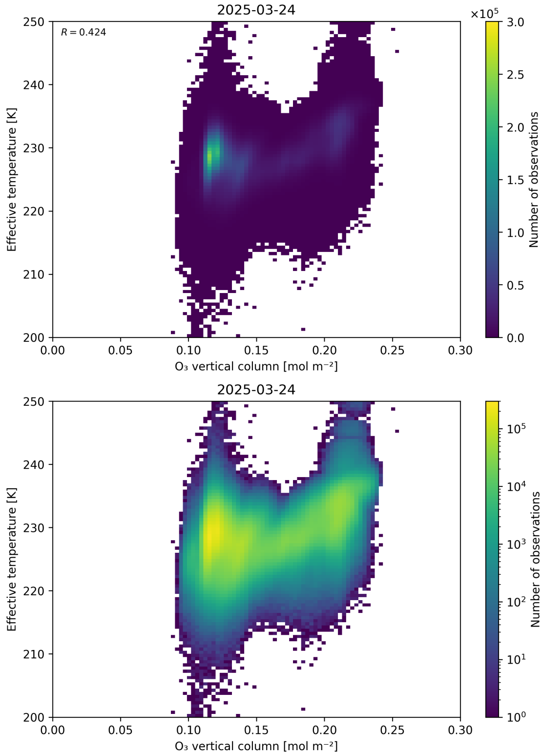
Figure 39: Scatter density plot of “O 3 vertical column” against “Effective temperature” for 2025-03-23 to 2025-03-25.
