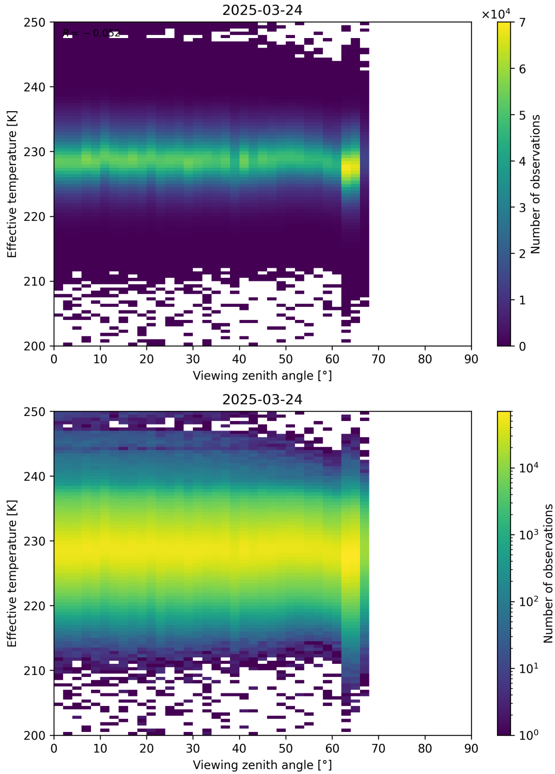
Figure 50: Scatter density plot of “Viewing zenith angle” against “Effective temperature” for 2025-03-23 to 2025-03-25.
