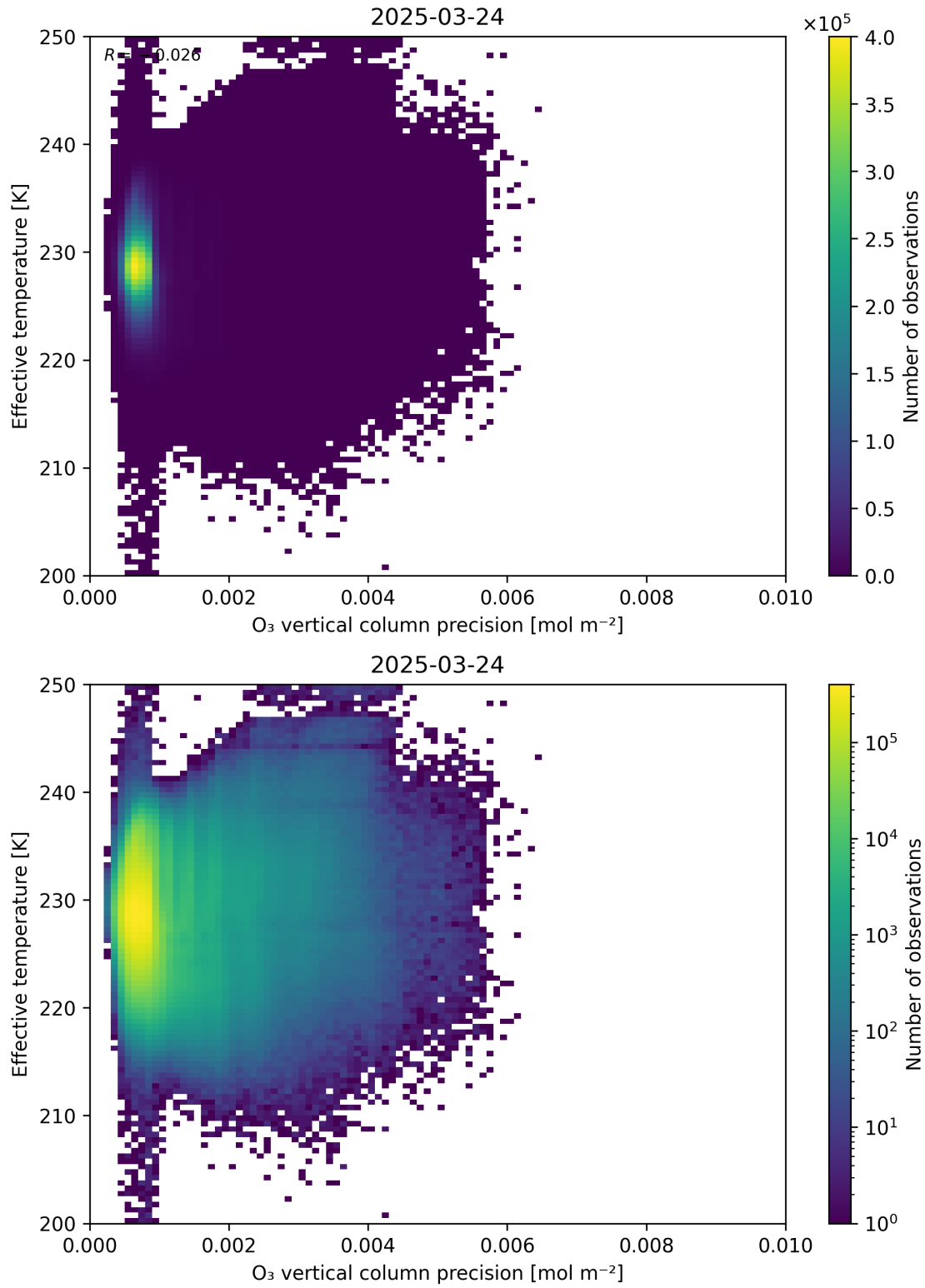
Figure 42: Scatter density plot of “O 3 vertical column precision” against “Effective temperature” for 2025-03-23 to 2025-03-25.
