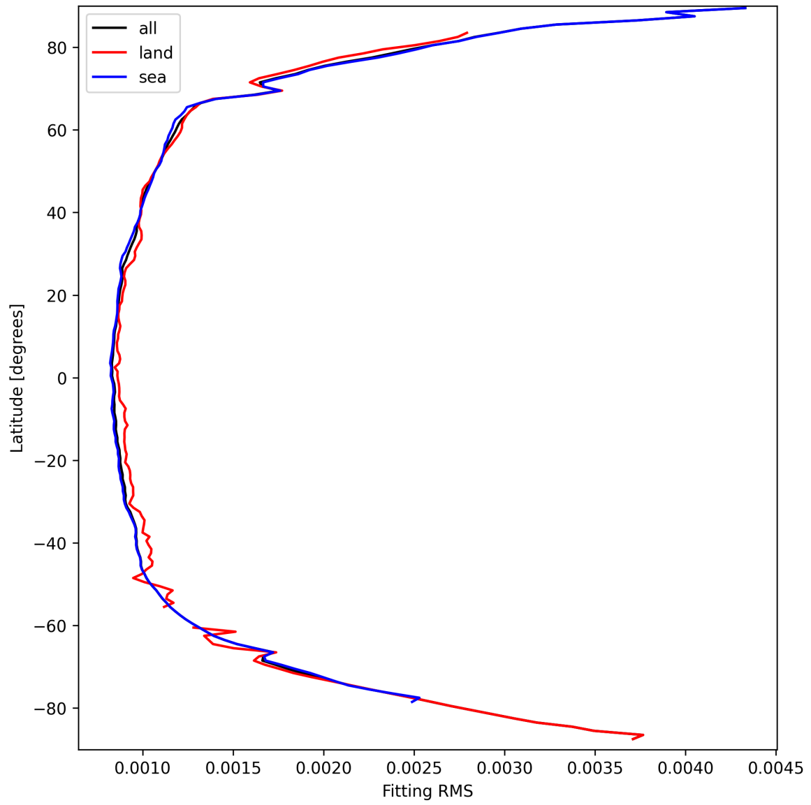
Figure 16: Zonal average of “Fitting RMS” for 2025-03-23 to 2025-03-25.
