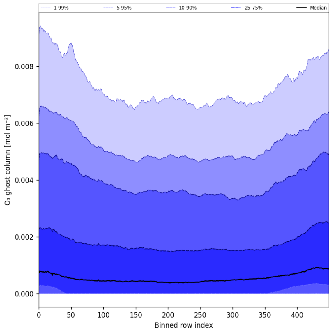
Figure 32: Along track statistics of “ \text{O}_3 ghost column” for 2025-03-23 to 2025-03-25
