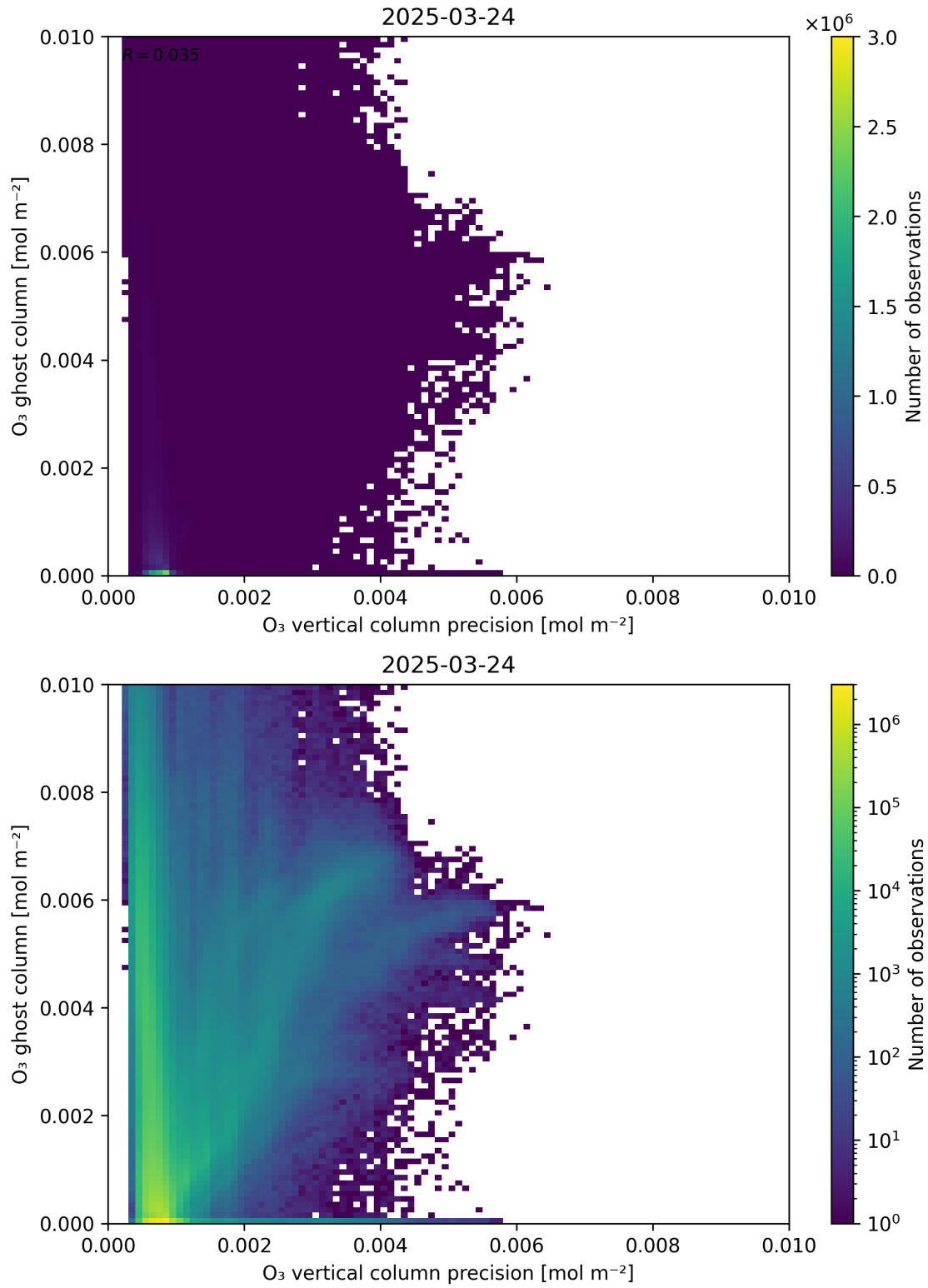
Figure 43: Scatter density plot of “ O_3 vertical column precision” against “ O_3 ghost column” for 2025-03-23 to 2025-03-25.
