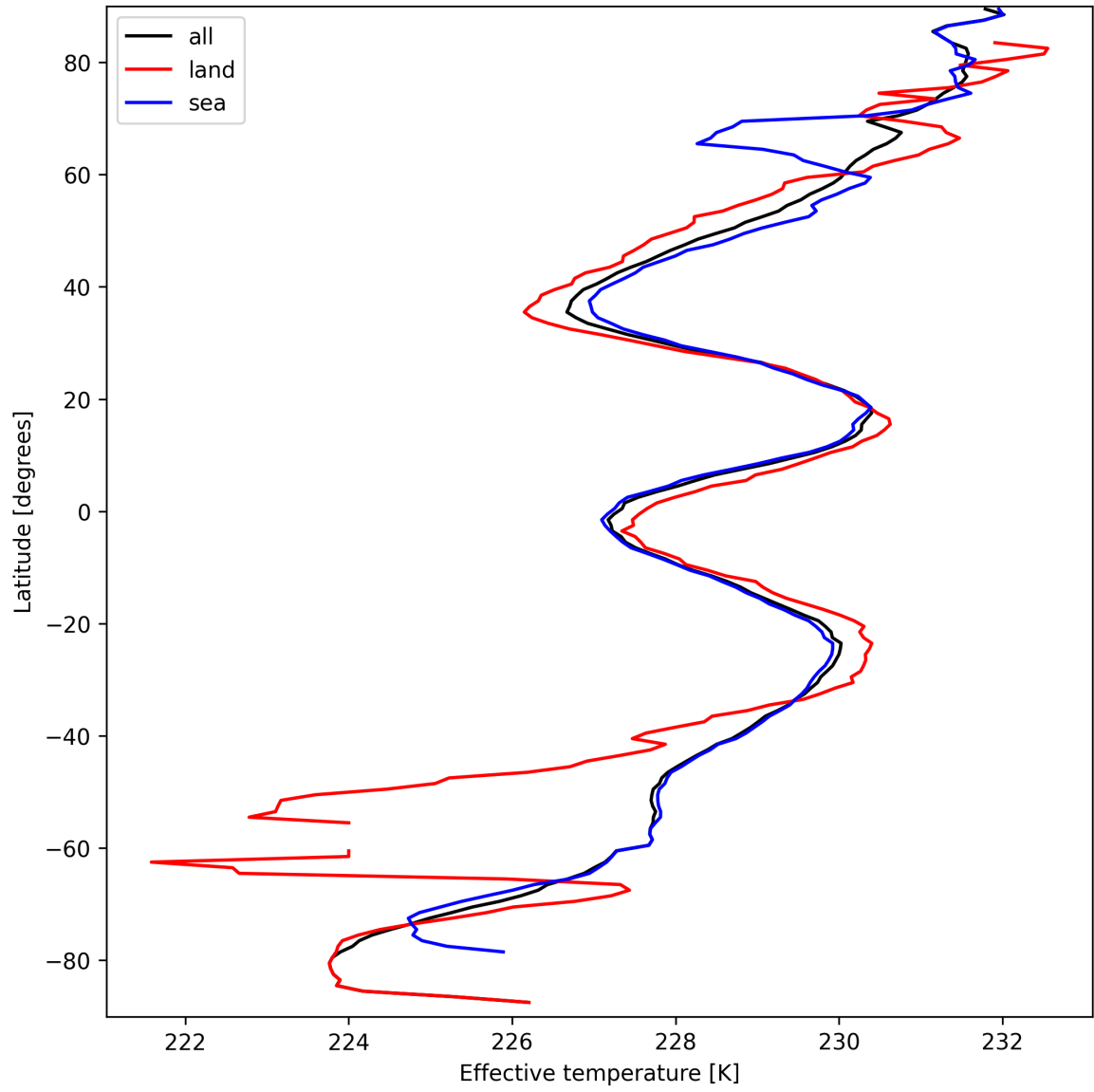
Figure 17: Zonal average of “Effective temperature” for 2025-03-23 to 2025-03-25.
