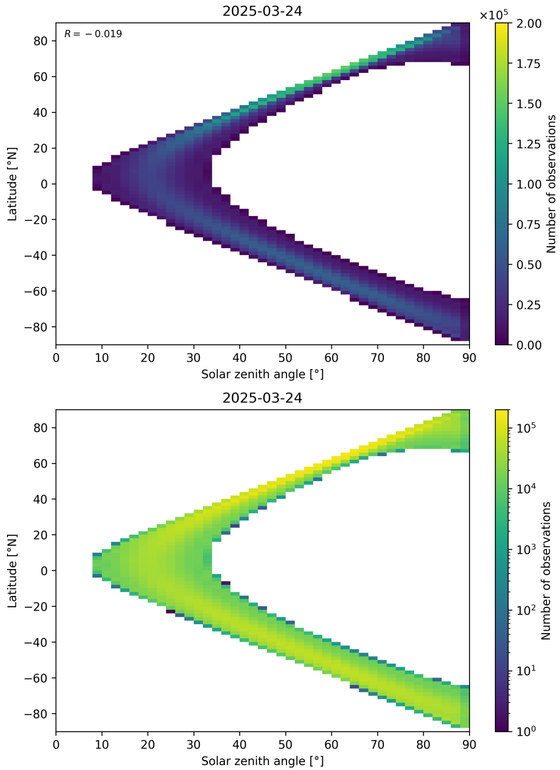
Figure 44: Scatter density plot of “Solar zenith angle” against “Latitude” for 2025-03-23 to 2025-03-25.
