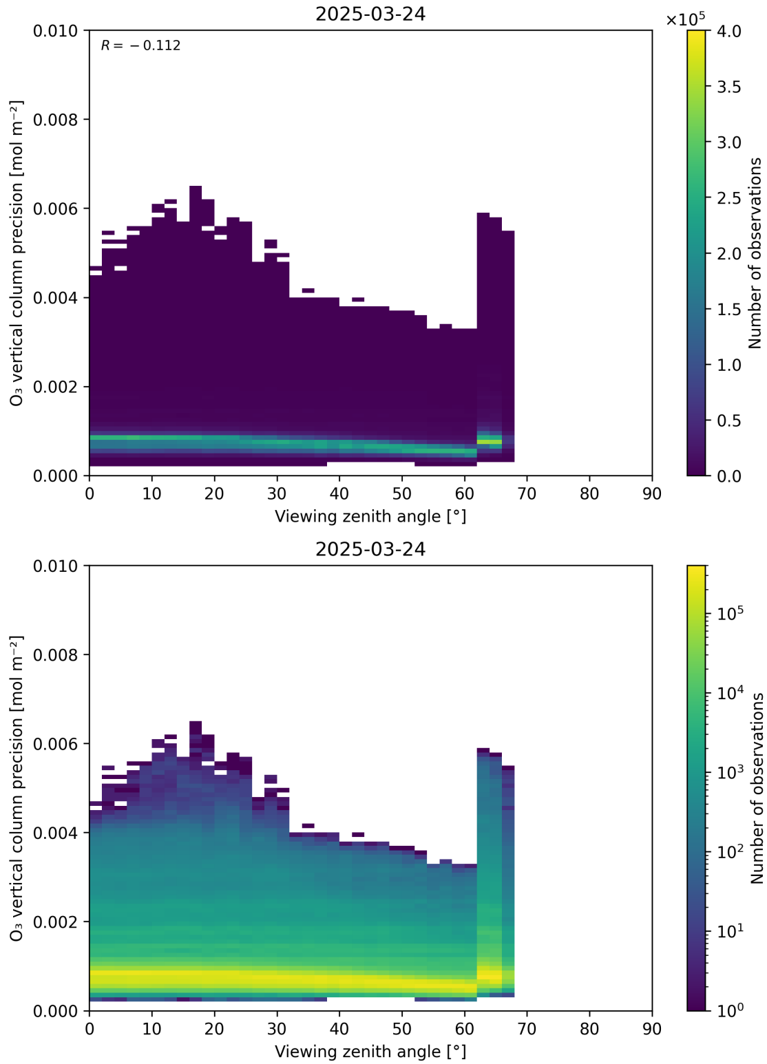
Figure 53: Scatter density plot of “Viewing zenith angle” against “O 3 vertical column precision” for 2025-03-23 to 2025-03-25.
