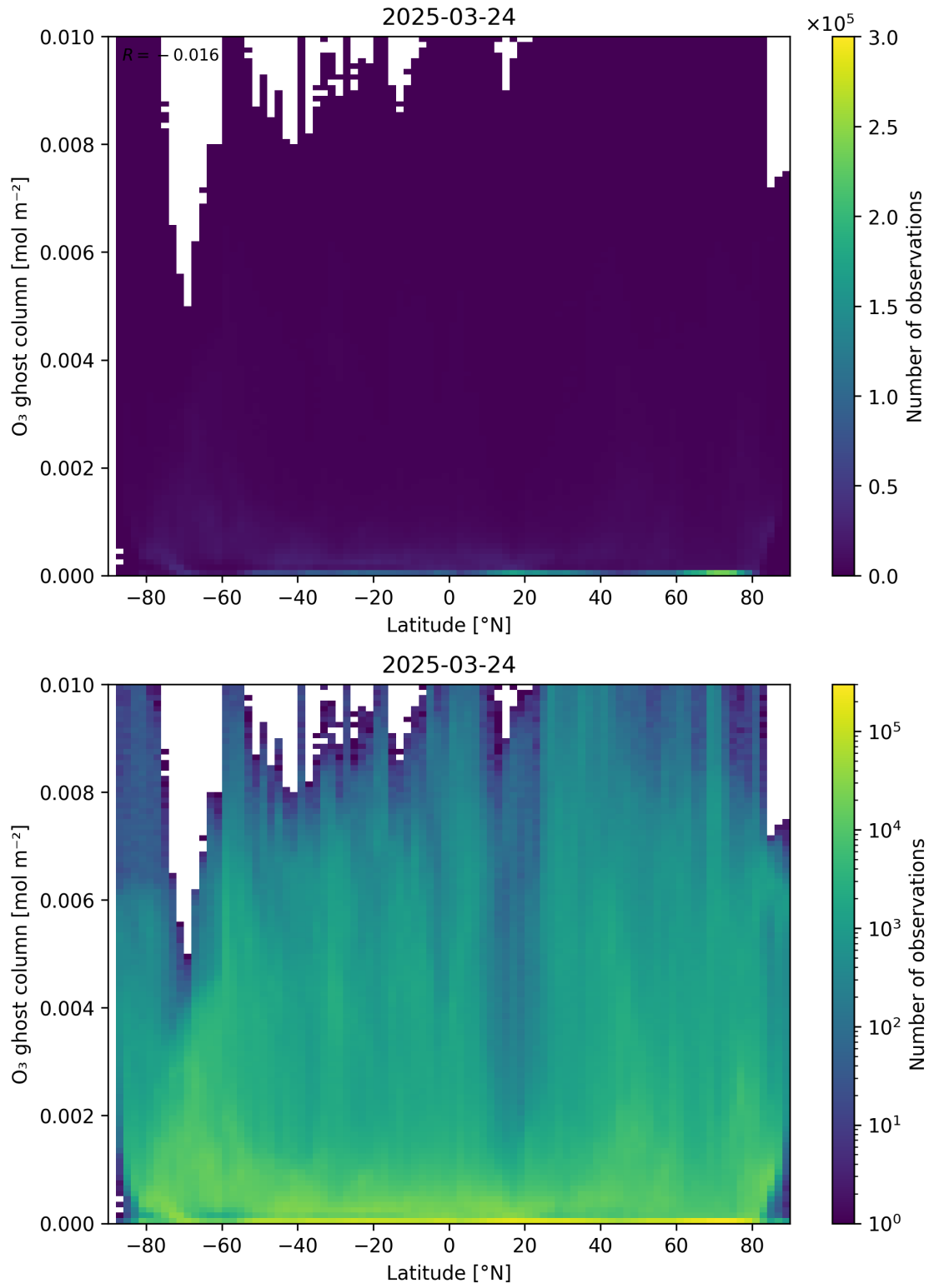
Figure 35: Scatter density plot of “Latitude” against “O 3 ghost column” for 2025-03-23 to 2025-03-25.
