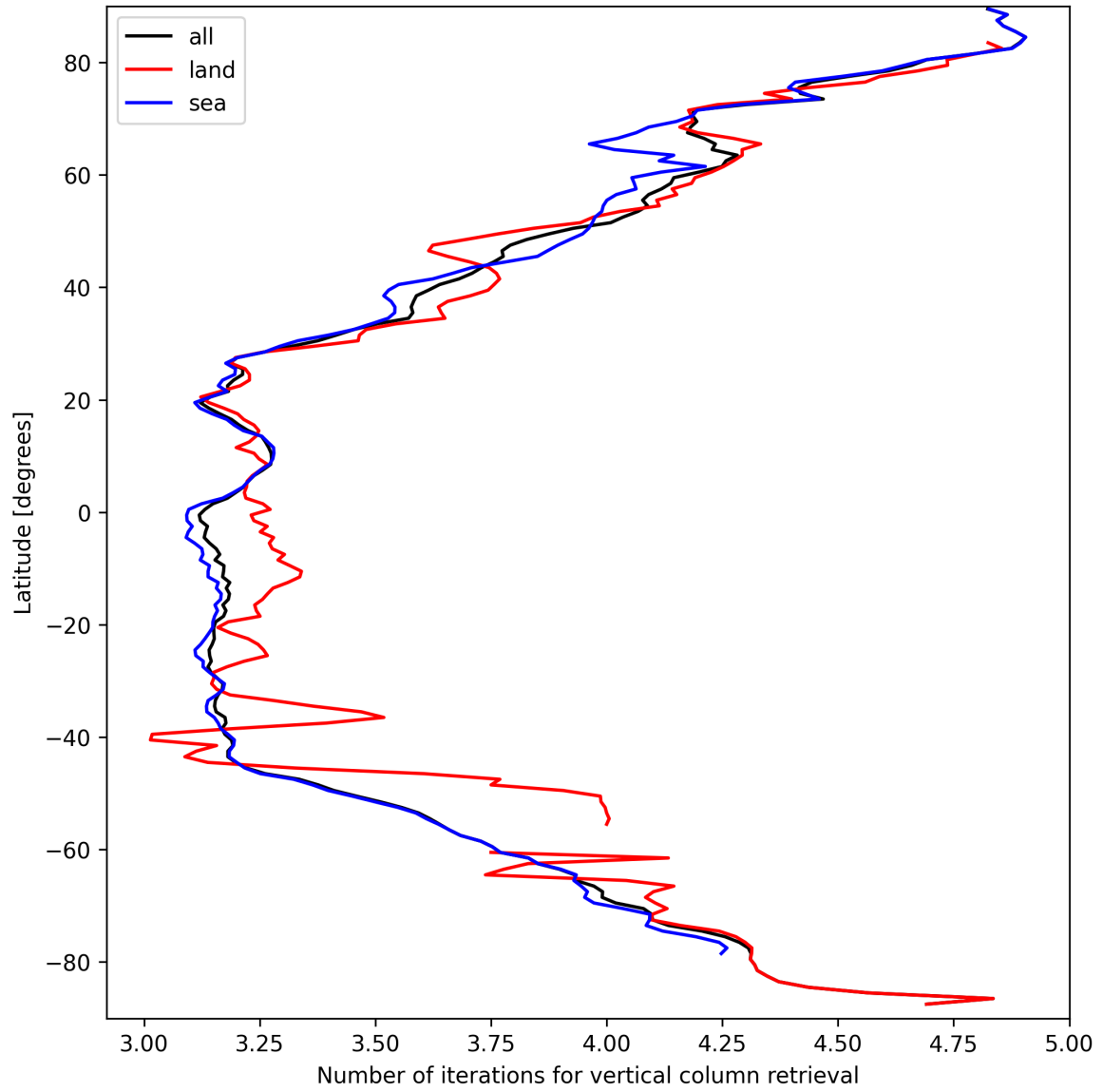
Figure 19: Zonal average of “Number of iterations for vertical column retrieval” for 2025-03-23 to 2025-03-25.
