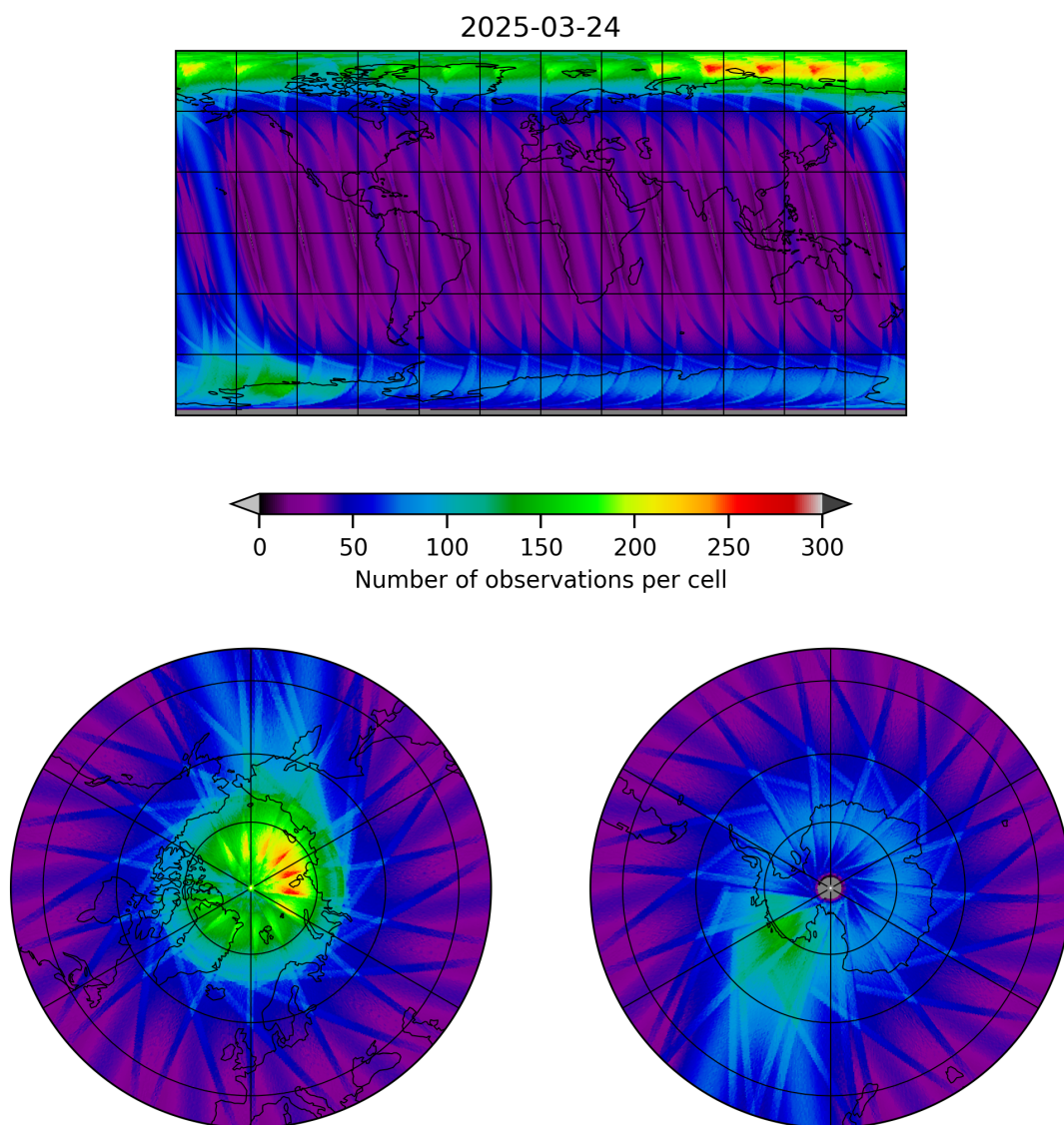
Figure 12: Map of the number of observations for 2025-03-23 to 2025-03-25
