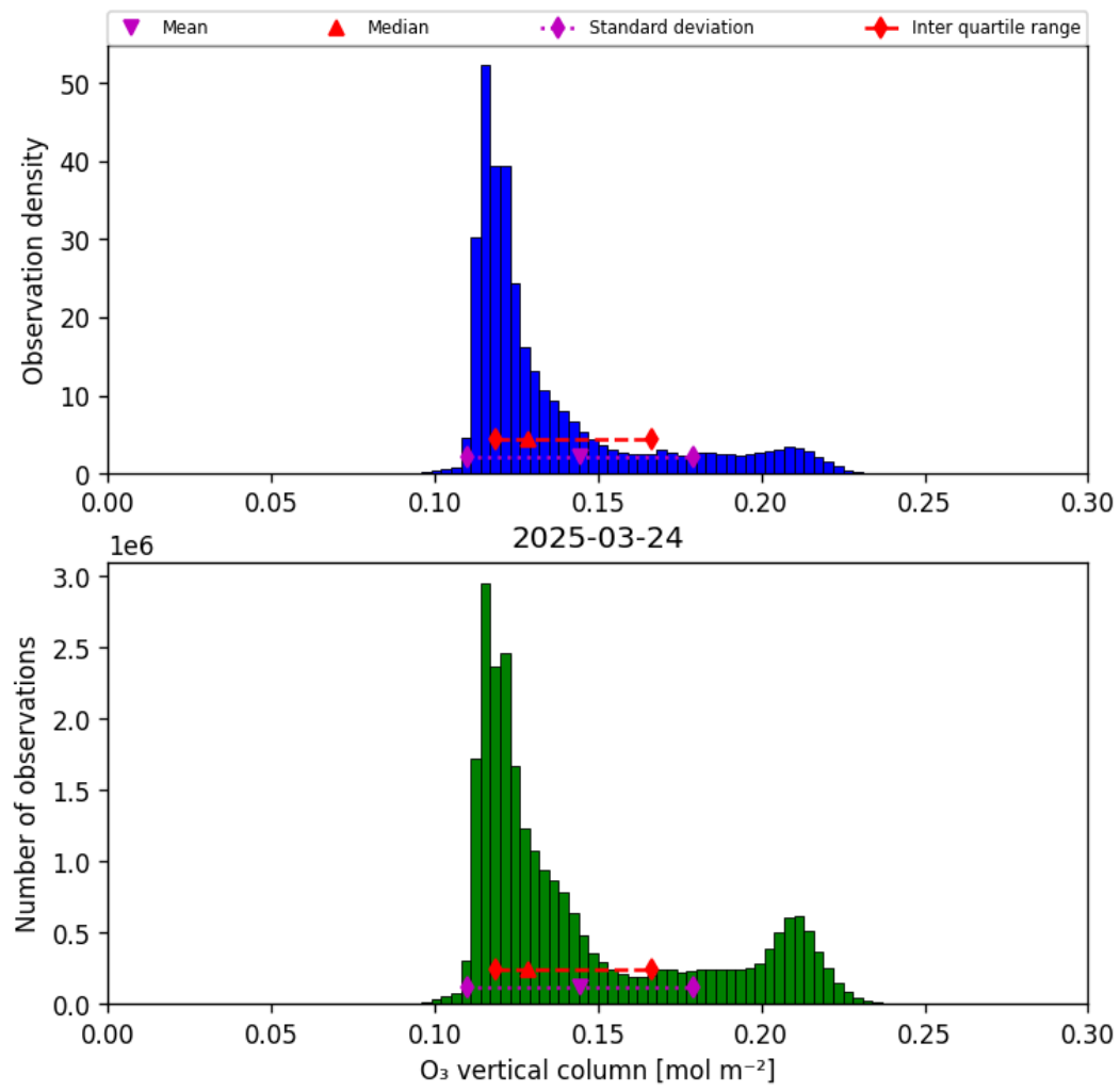
Figure 21: Histogram of “O 3 vertical column” for 2025-03-23 to 2025-03-25
