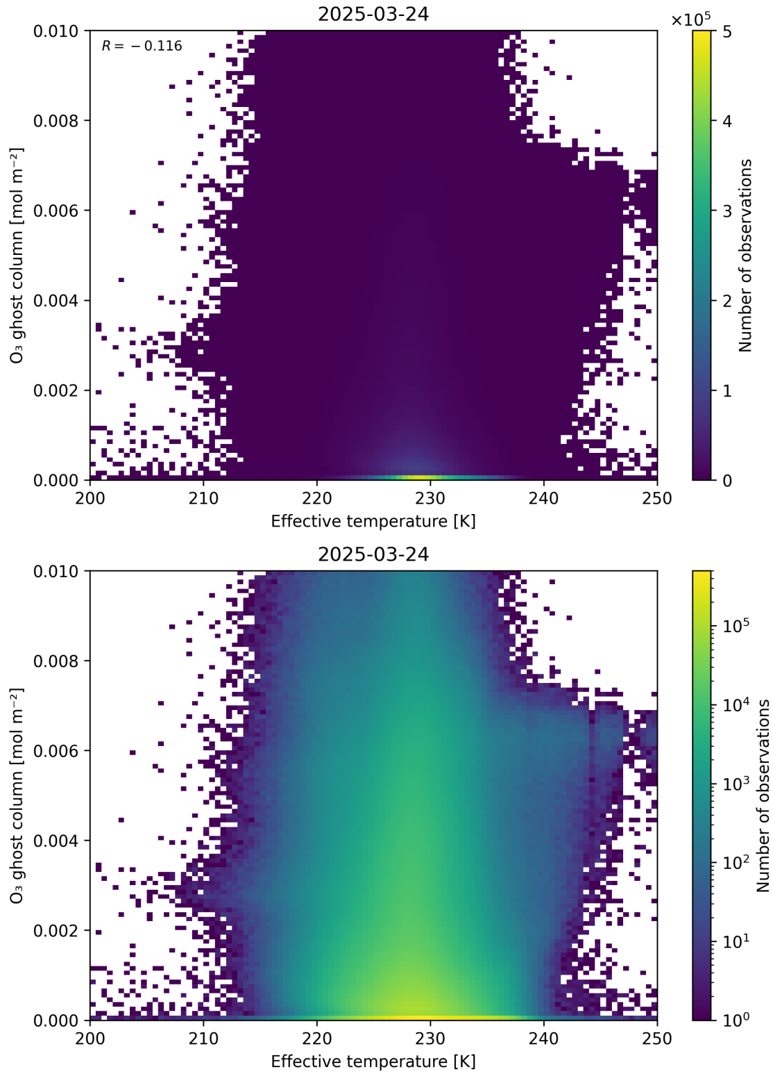
Figure 38: Scatter density plot of “Effective temperature” against “O 3 ghost column” for 2025-03-23 to 2025-03-25.
