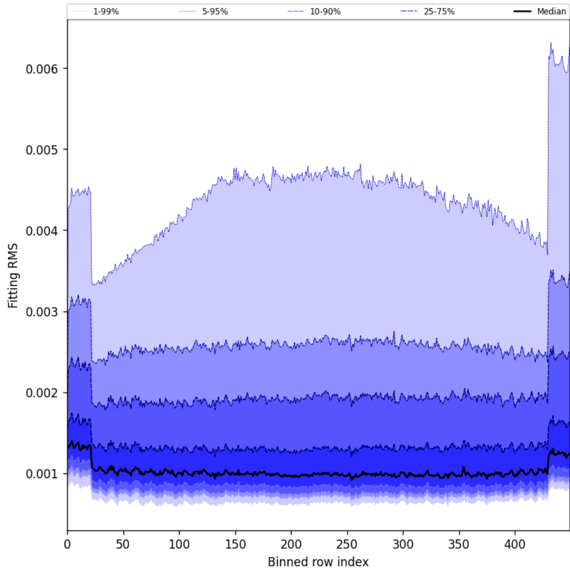
Figure 30: Along track statistics of “Fitting RMS” for 2025-03-23 to 2025-03-25
