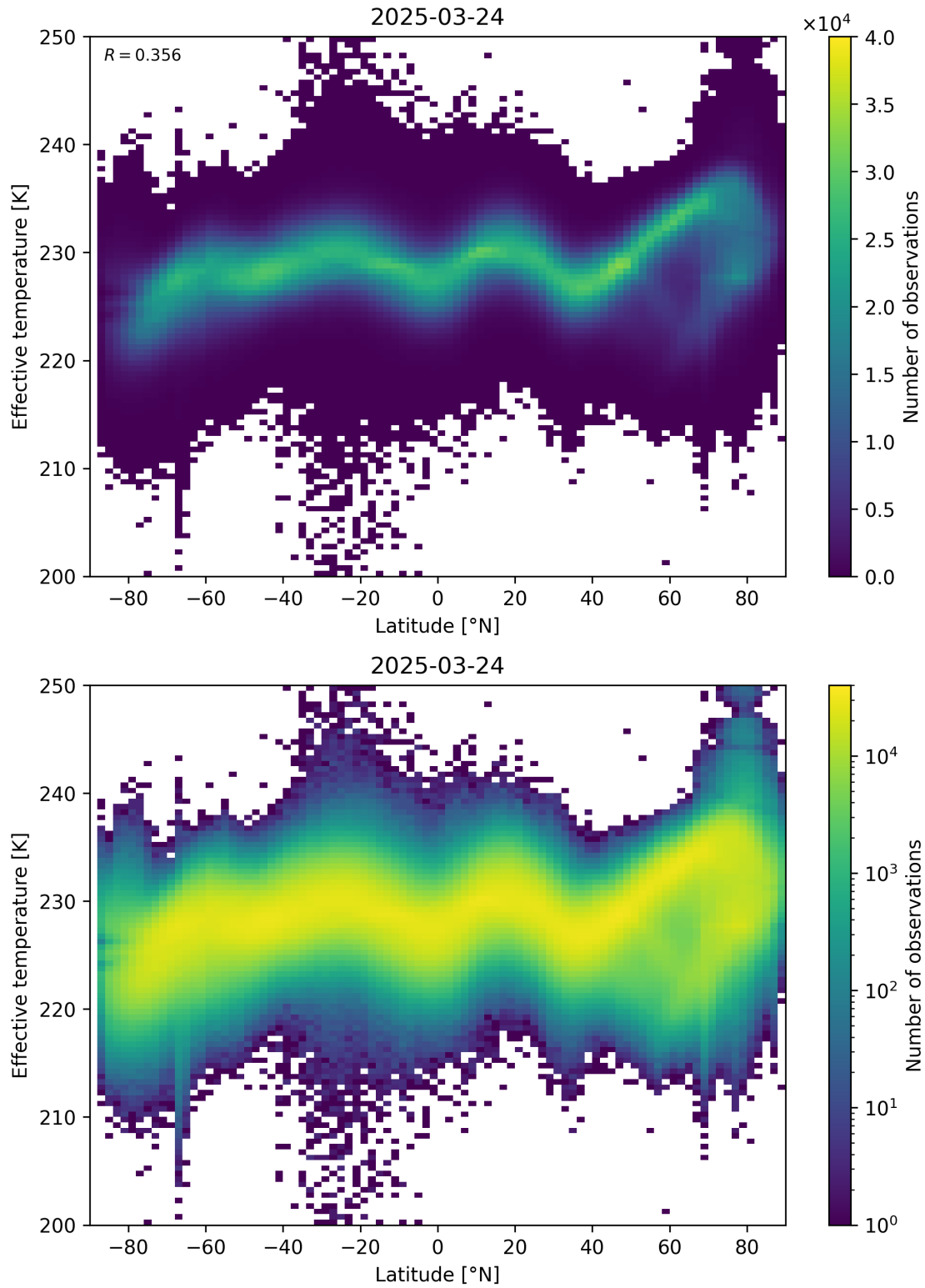
Figure 34: Scatter density plot of “Latitude” against “Effective temperature” for 2025-03-23 to 2025-03-25.
