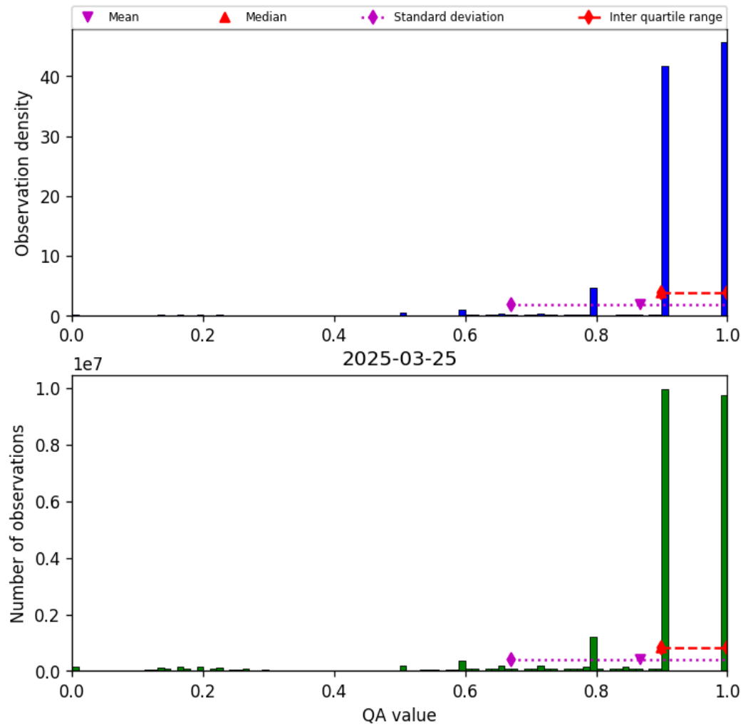
Figure 20: Histogram of “QA value” for 2025-03-24 to 2025-03-26
