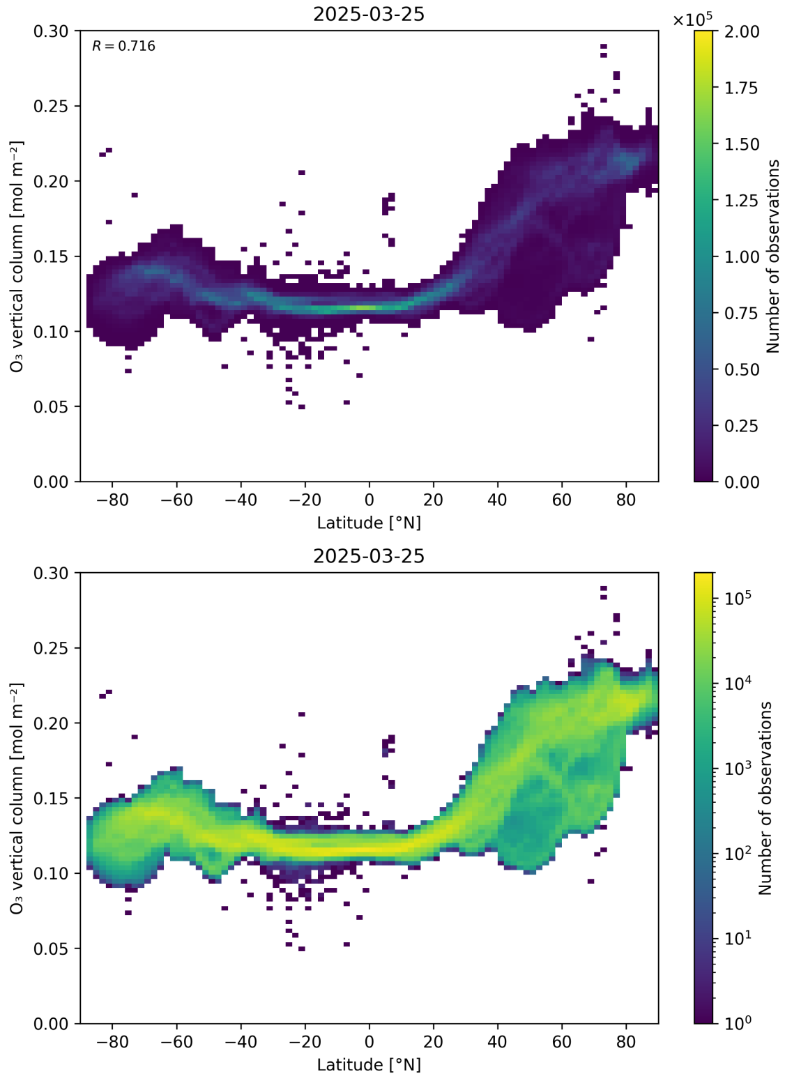
Figure 36: Scatter density plot of “Latitude” against “O 3 vertical column” for 2025-03-24 to 2025-03-26.
