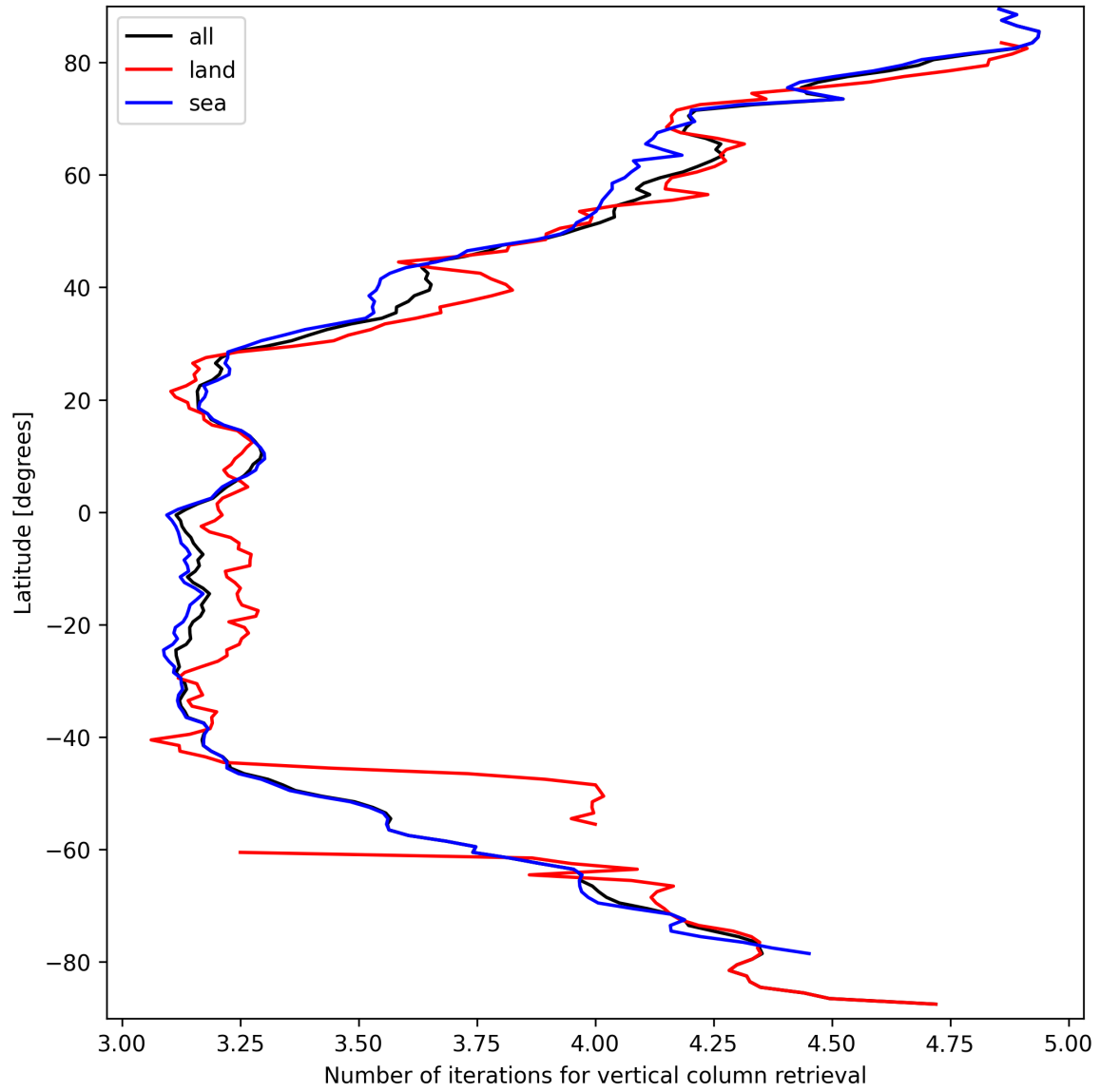
Figure 19: Zonal average of “Number of iterations for vertical column retrieval” for 2025-03-24 to 2025-03-26.
