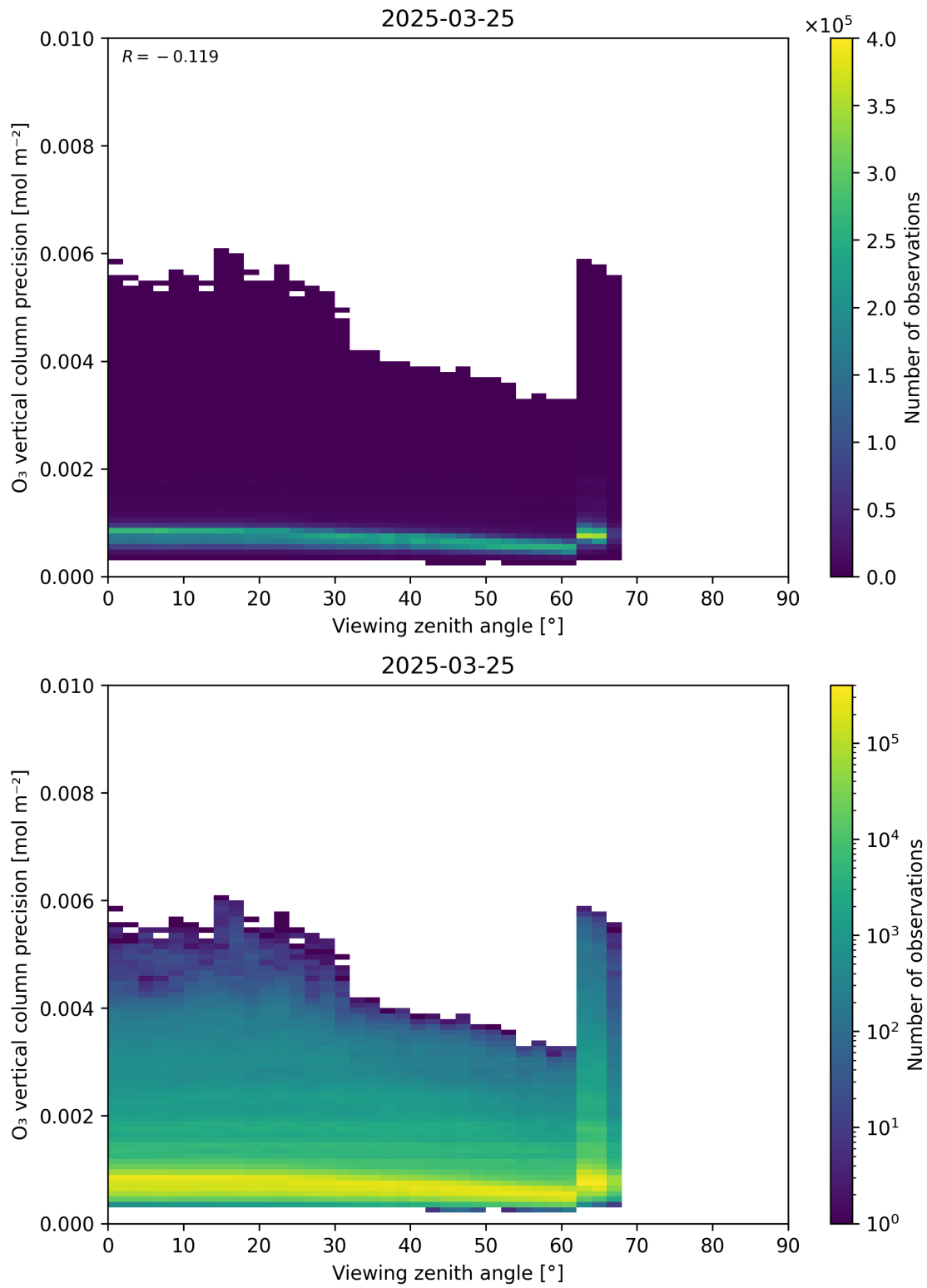
Figure 53: Scatter density plot of “Viewing zenith angle” against “O 3 vertical column precision” for 2025-03-24 to 2025-03-26.
