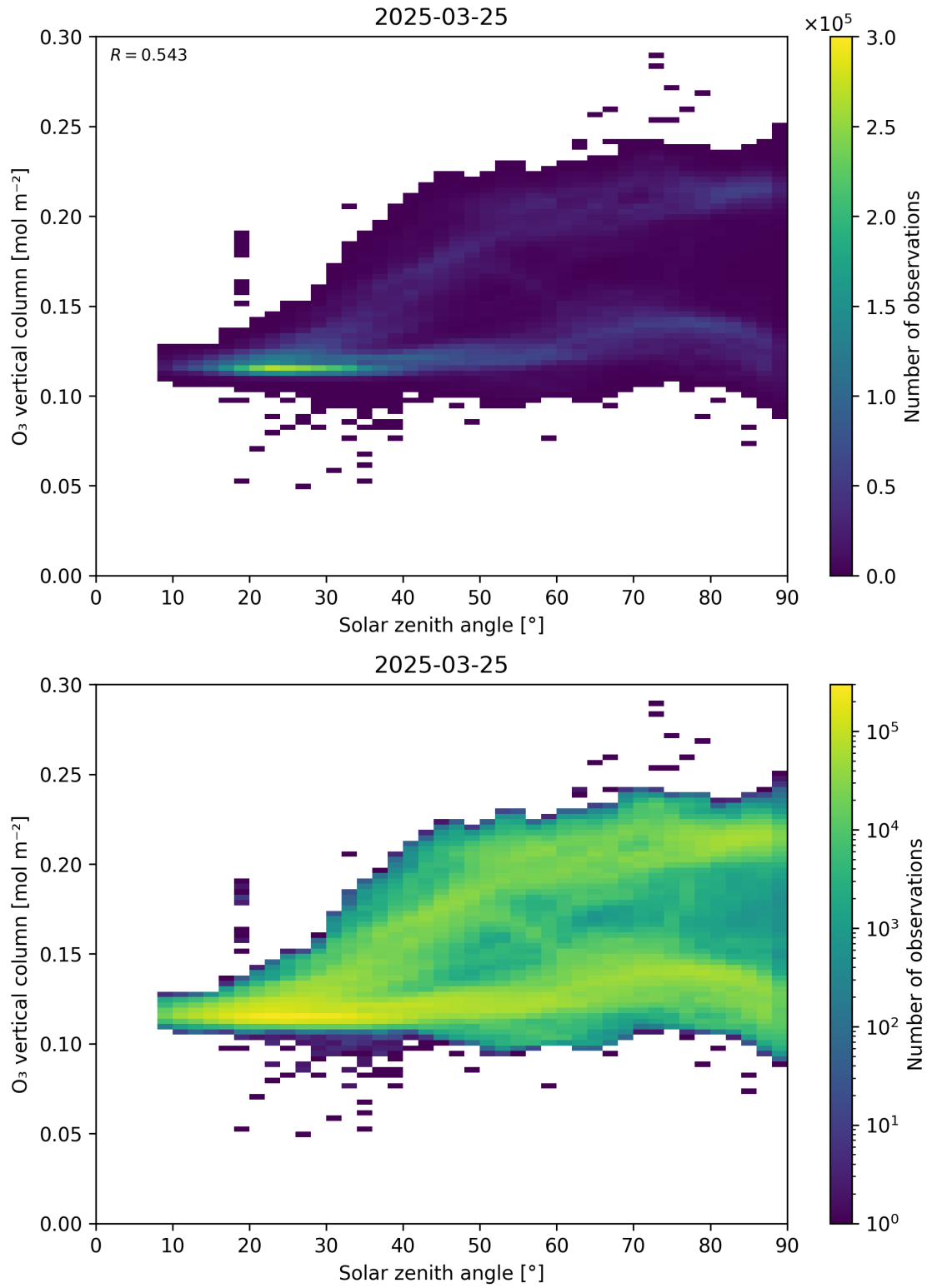
Figure 47: Scatter density plot of “Solar zenith angle” against “O 3 vertical column” for 2025-03-24 to 2025-03-26.
