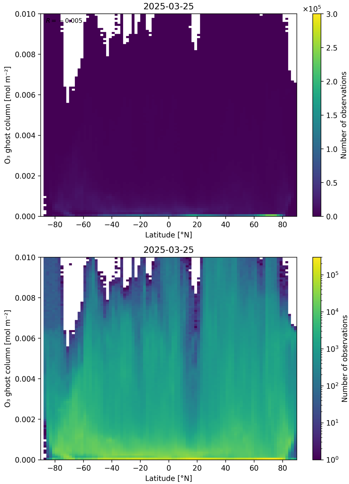
Figure 35: Scatter density plot of “Latitude” against “O 3 ghost column” for 2025-03-24 to 2025-03-26.
