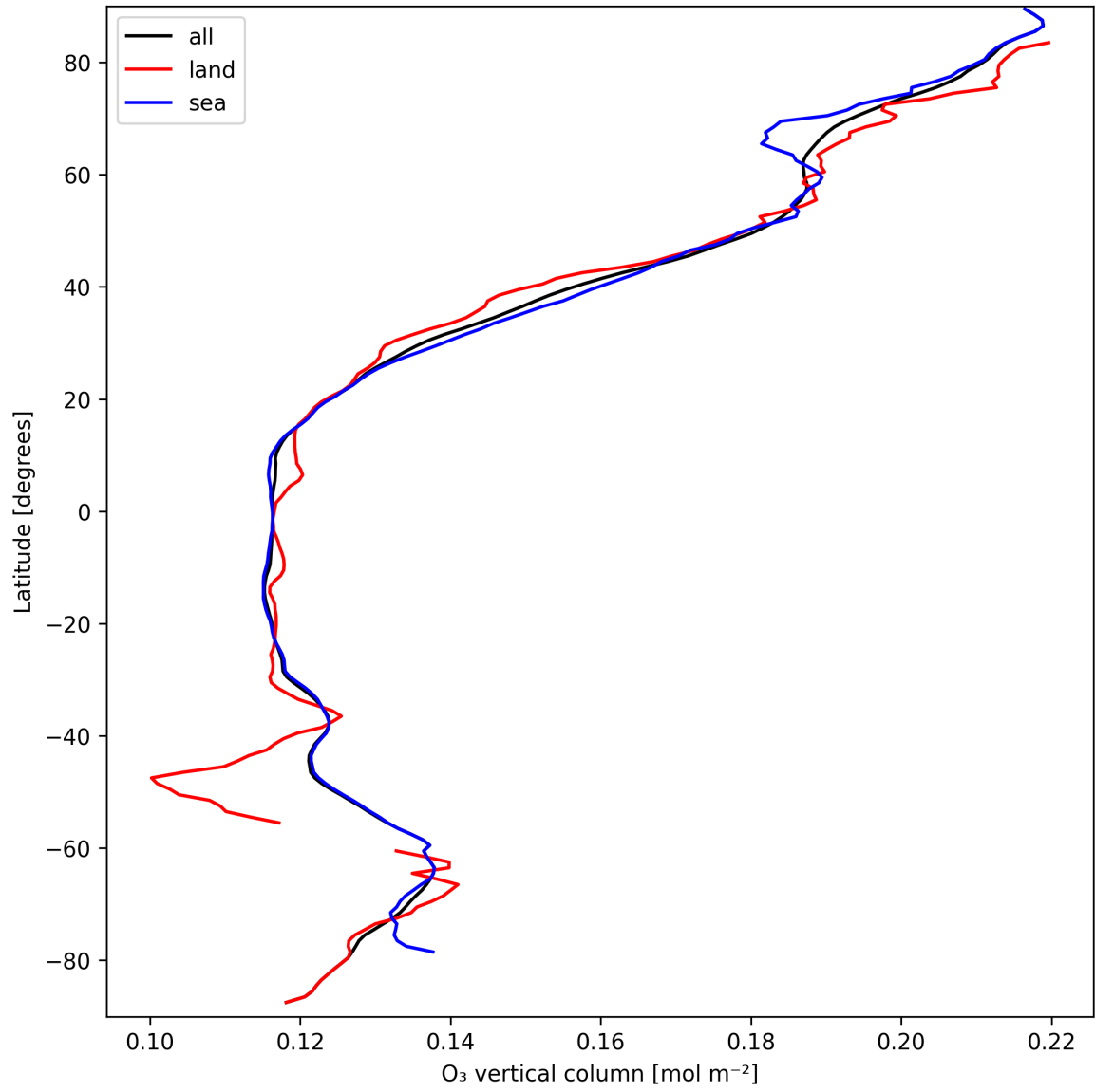
Figure 14: Zonal average of “O 3 vertical column” for 2025-03-24 to 2025-03-26.
