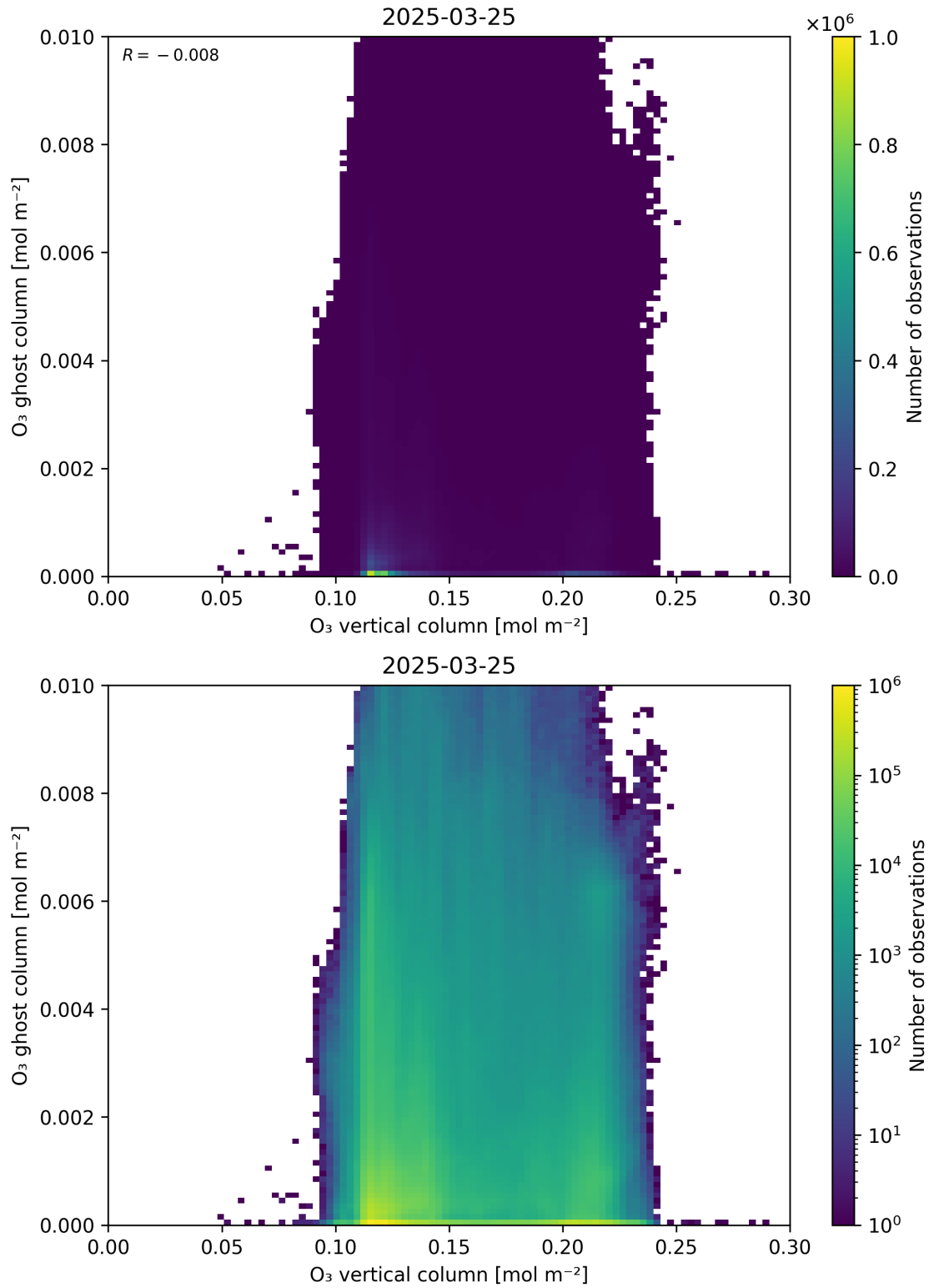
Figure 40: Scatter density plot of “O 3 vertical column” against “O 3 ghost column” for 2025-03-24 to 2025-03-26.
