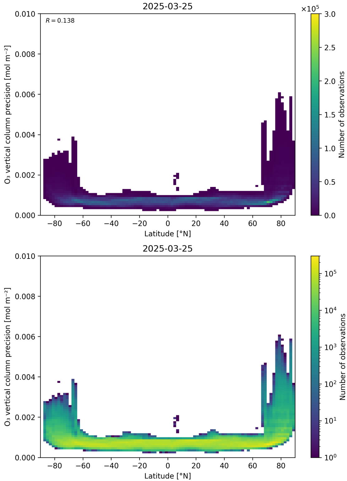
Figure 37: Scatter density plot of “Latitude” against “O 3 vertical column precision” for 2025-03-24 to 2025-03-26.
