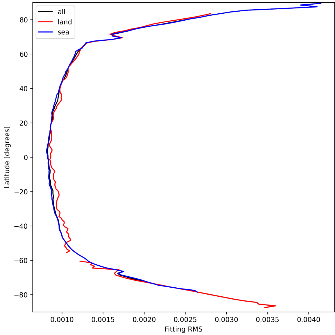
Figure 16: Zonal average of “Fitting RMS” for 2025-03-24 to 2025-03-26.
