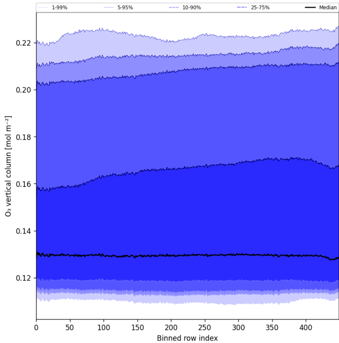
Figure 28: Along track statistics of “O 3 vertical column” for 2025-03-24 to 2025-03-26
