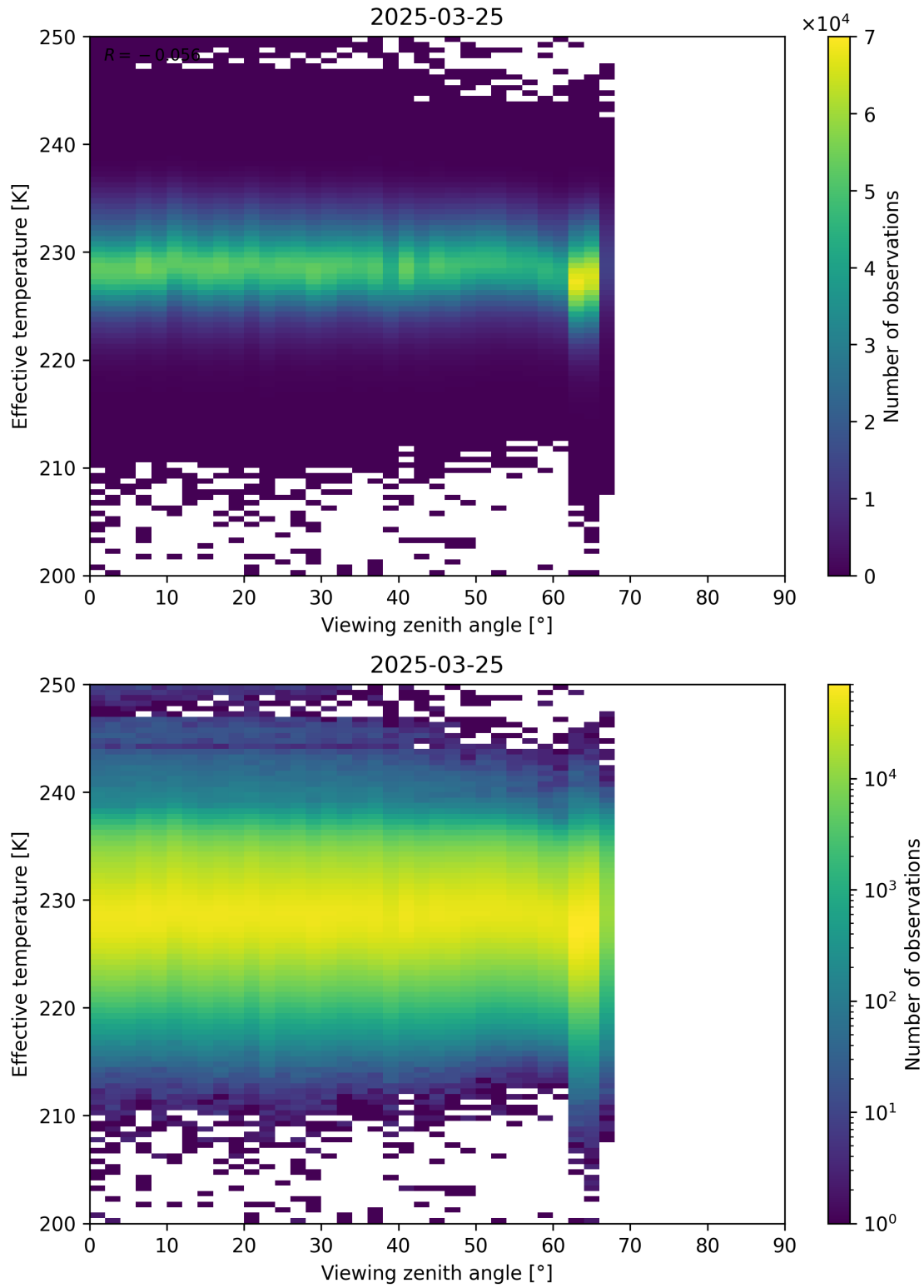
Figure 50: Scatter density plot of “Viewing zenith angle” against “Effective temperature” for 2025-03-24 to 2025-03-26.
