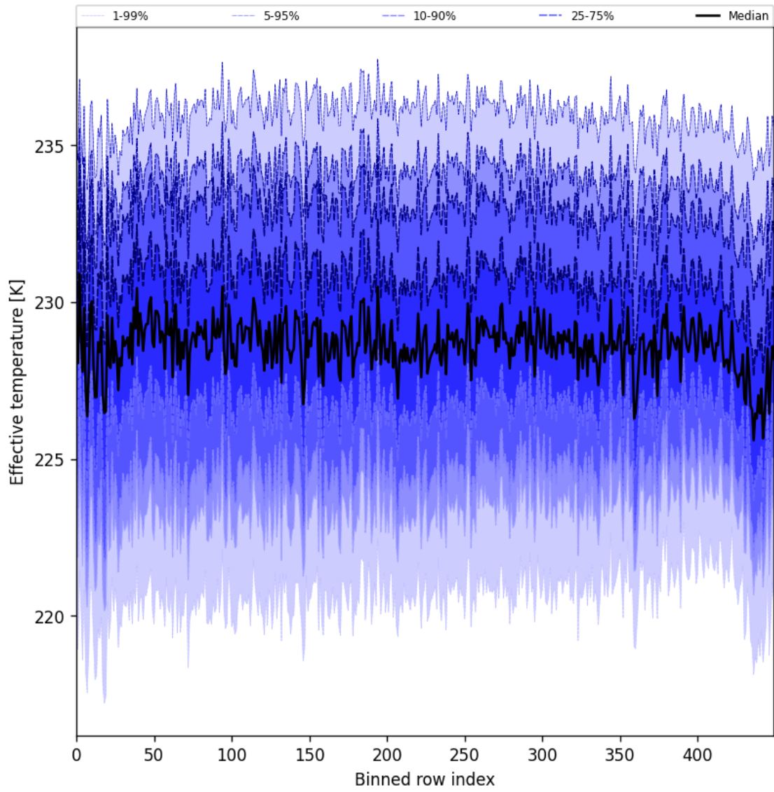
Figure 31: Along track statistics of “Effective temperature” for 2025-03-24 to 2025-03-26
