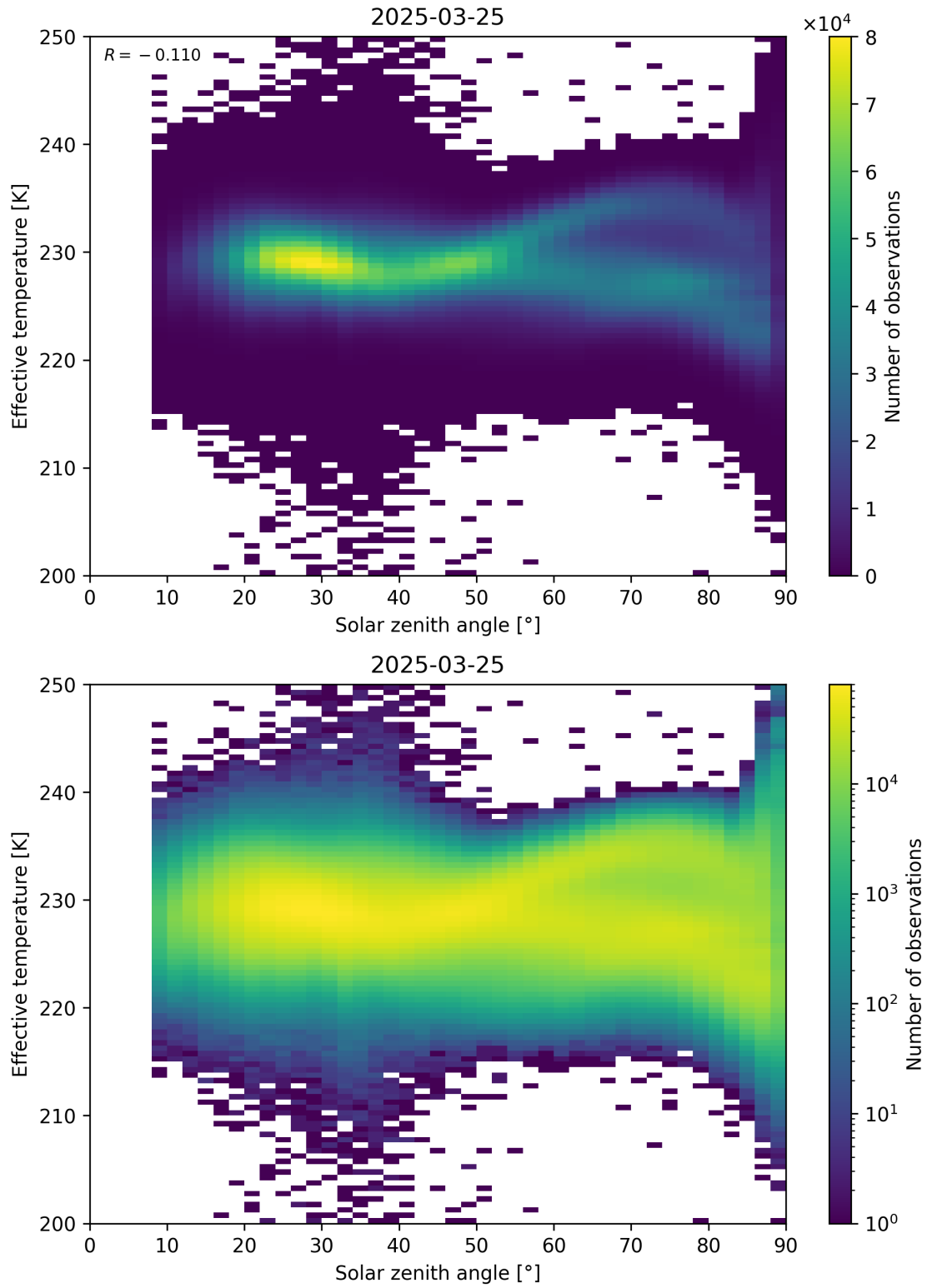
Figure 45: Scatter density plot of “Solar zenith angle” against “Effective temperature” for 2025-03-24 to 2025-03-26.
