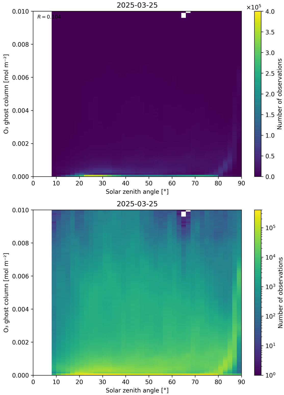
Figure 46: Scatter density plot of “Solar zenith angle” against “O 3 ghost column” for 2025-03-24 to 2025-03-26.
