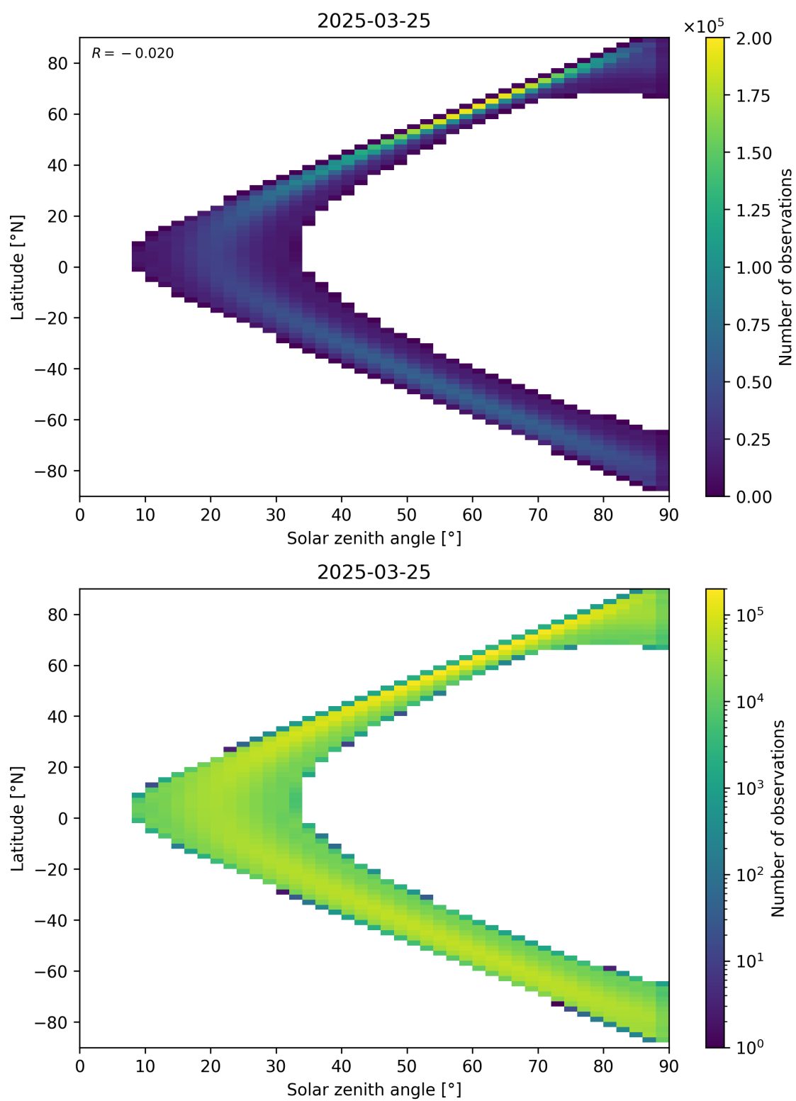
Figure 44: Scatter density plot of “Solar zenith angle” against “Latitude” for 2025-03-24 to 2025-03-26.
