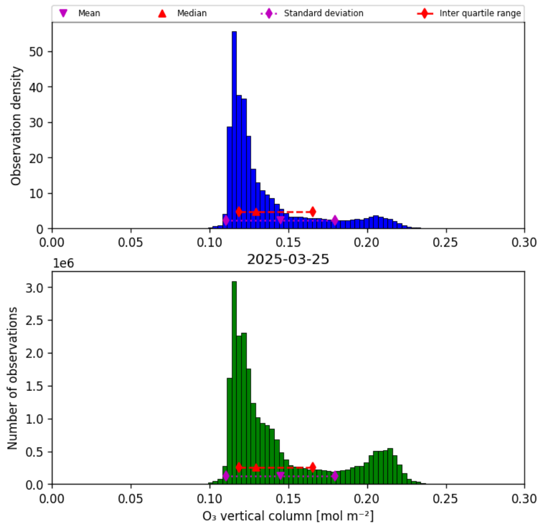
Figure 21: Histogram of “O 3 vertical column” for 2025-03-24 to 2025-03-26
