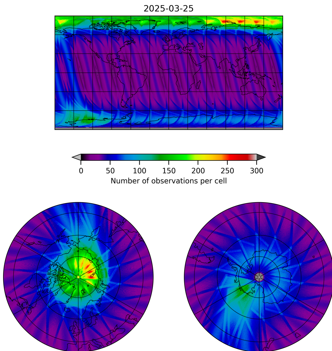
Figure 12: Map of the number of observations for 2025-03-24 to 2025-03-26
