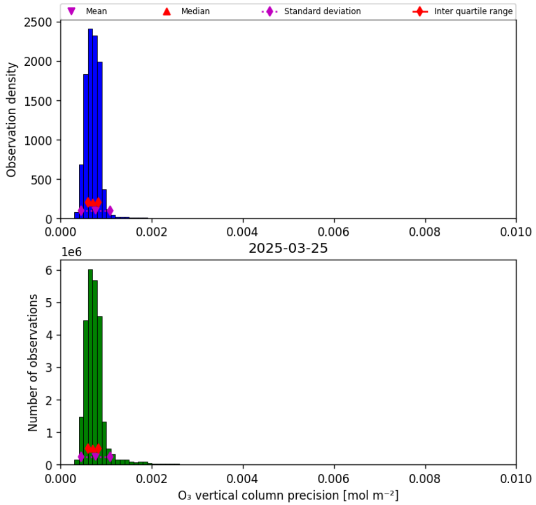
Figure 22: Histogram of “O 3 vertical column precision” for 2025-03-24 to 2025-03-26
