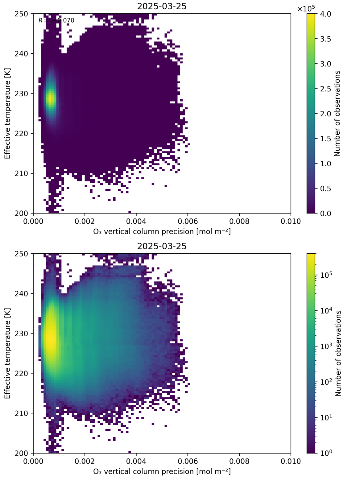
Figure 42: Scatter density plot of “O 3 vertical column precision” against “Effective temperature” for 2025-03-24 to 2025-03-26.
