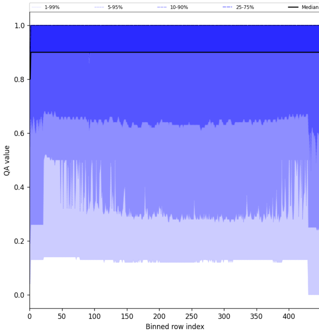
Figure 27: Along track statistics of “QA value” for 2025-03-24 to 2025-03-26
