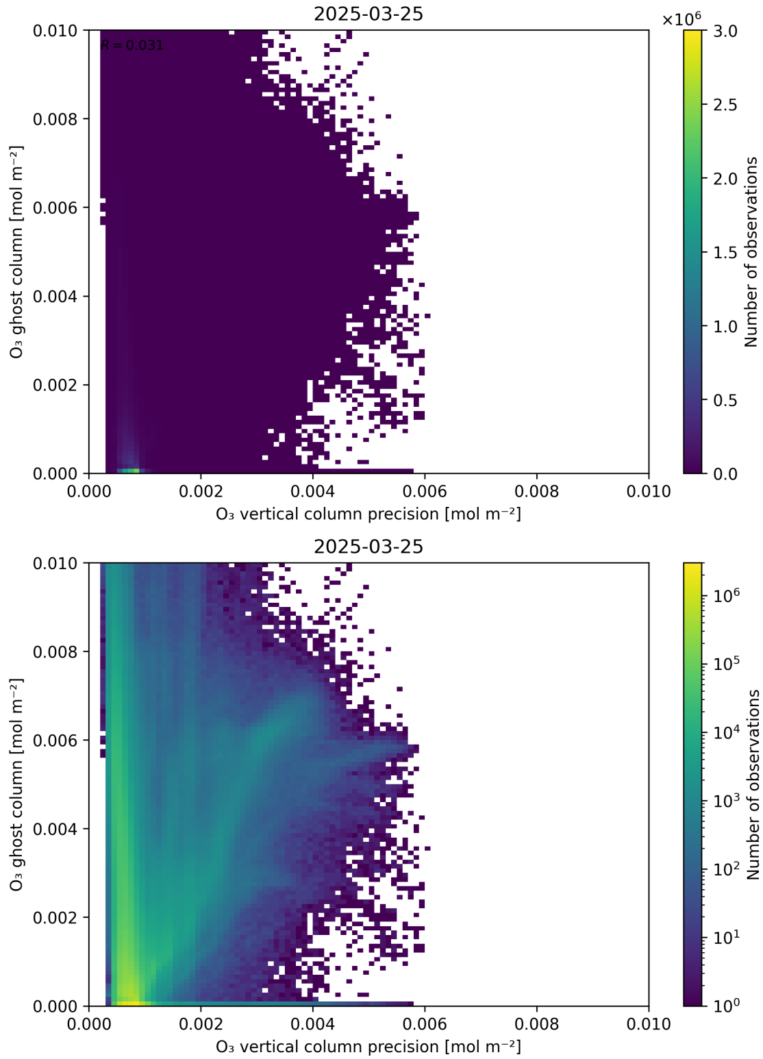
Figure 43: Scatter density plot of “ \text{O}_3 vertical column precision” against “ \text{O}_3 ghost column” for 2025-03-24 to 2025-03-26.
