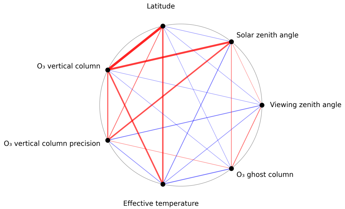
Figure 1: Map of correlation graph for 2025-03-24 to 2025-03-26.
