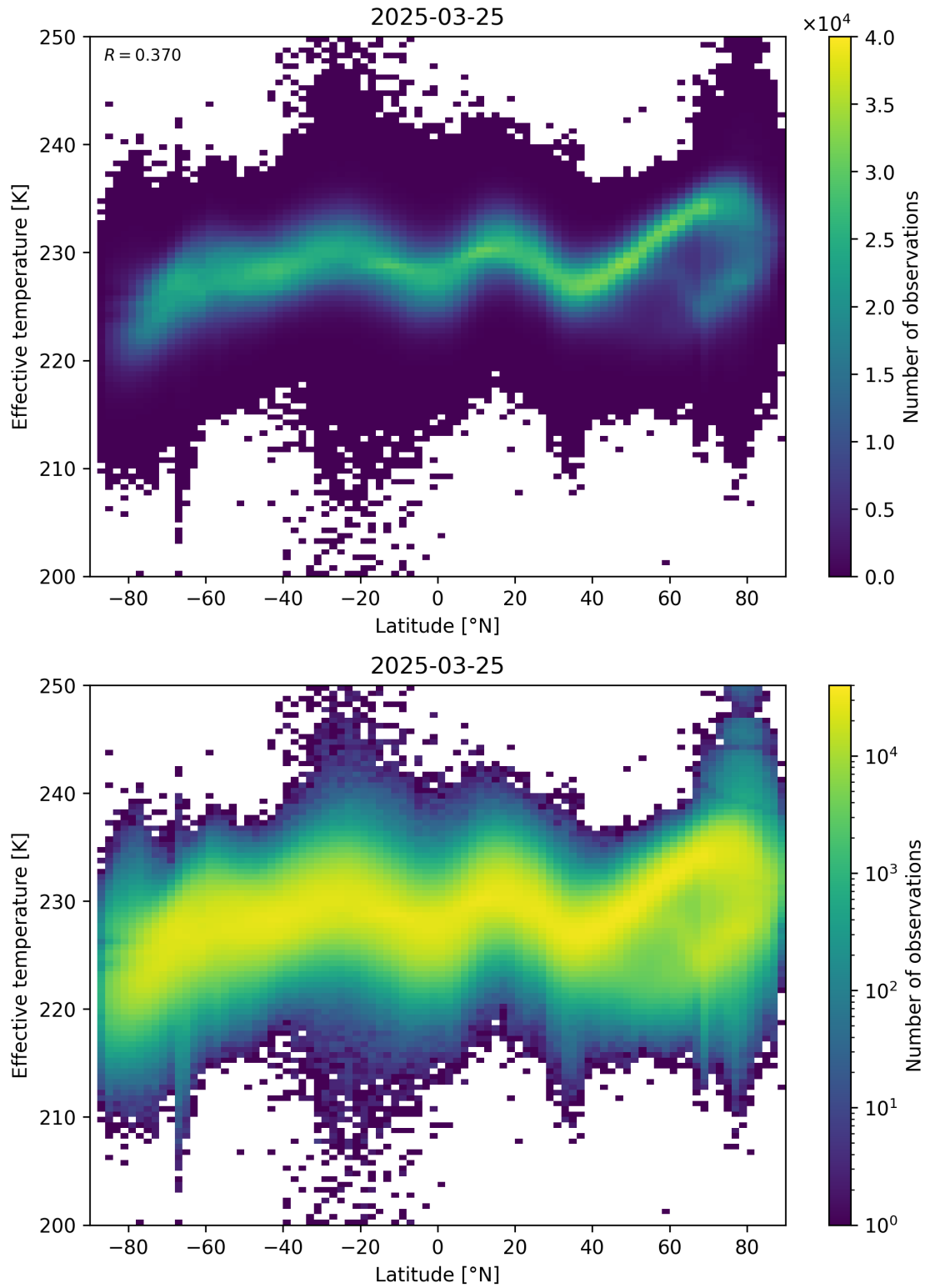
Figure 34: Scatter density plot of “Latitude” against “Effective temperature” for 2025-03-24 to 2025-03-26.
