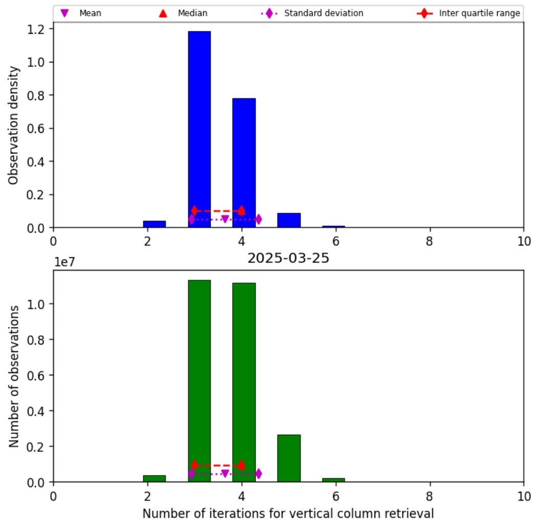
Figure 26: Histogram of “Number of iterations for vertical column retrieval” for 2025-03-24 to 2025-03-26
