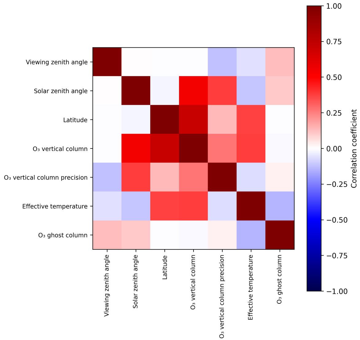
Figure 2: Map of correlation matrix for 2025-03-24 to 2025-03-26.
