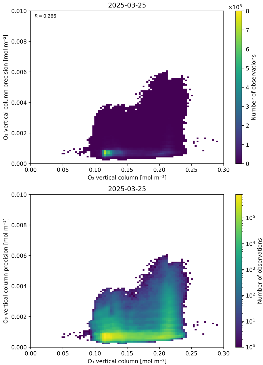
Figure 41: Scatter density plot of “O 3 vertical column” against “O 3 vertical column precision” for 2025-03-24 to 2025-03-26.
