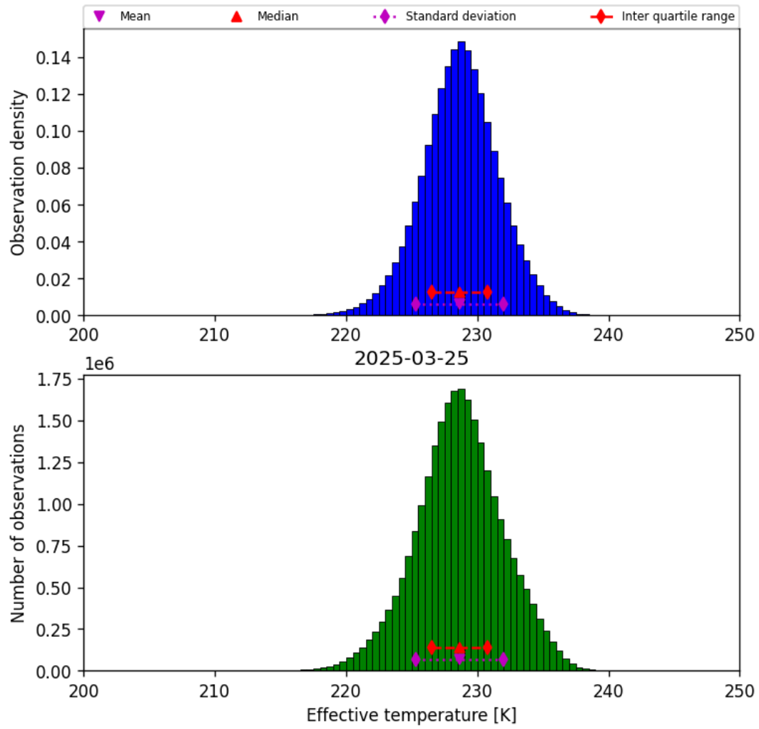
Figure 24: Histogram of “Effective temperature” for 2025-03-24 to 2025-03-26
