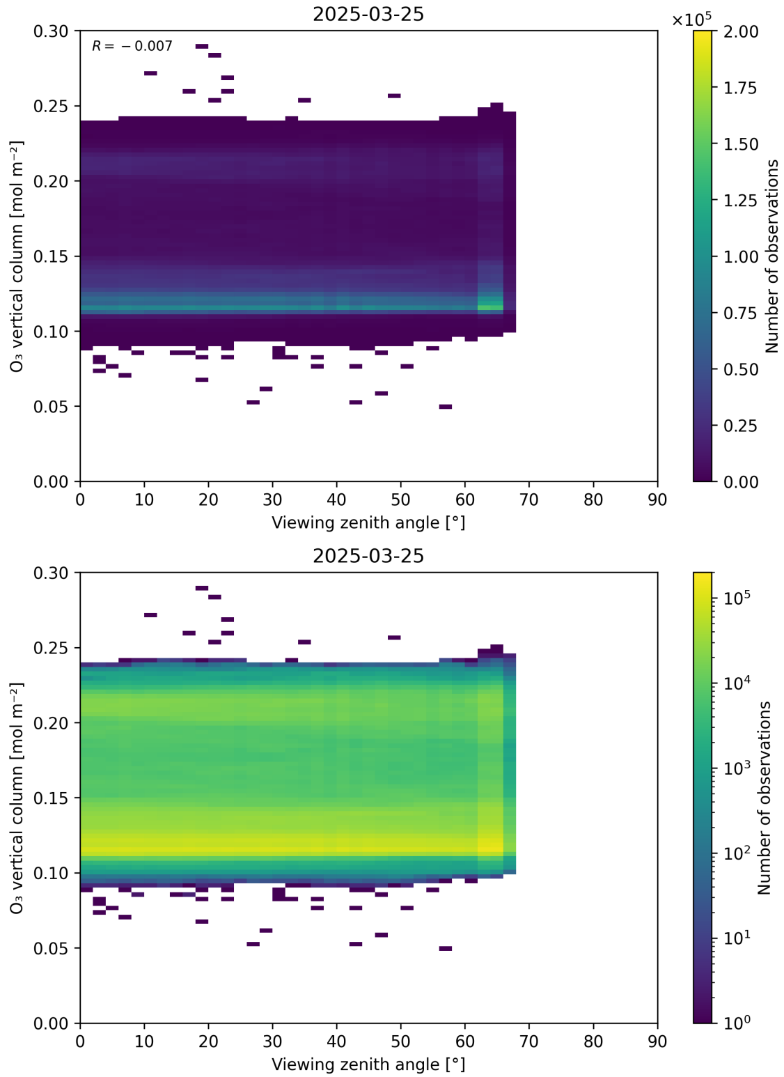
Figure 52: Scatter density plot of “Viewing zenith angle” against “O 3 vertical column” for 2025-03-24 to 2025-03-26.
