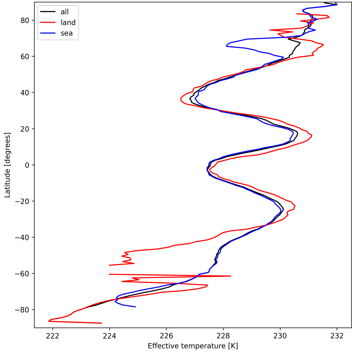
Figure 17: Zonal average of "Effective temperature" for 2025-03-24 to 2025-03-26.
