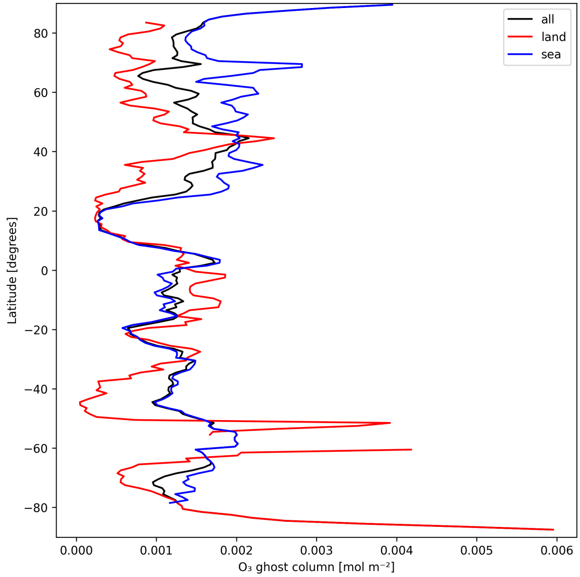
Figure 18: Zonal average of “O 3 ghost column” for 2025-03-24 to 2025-03-26.
