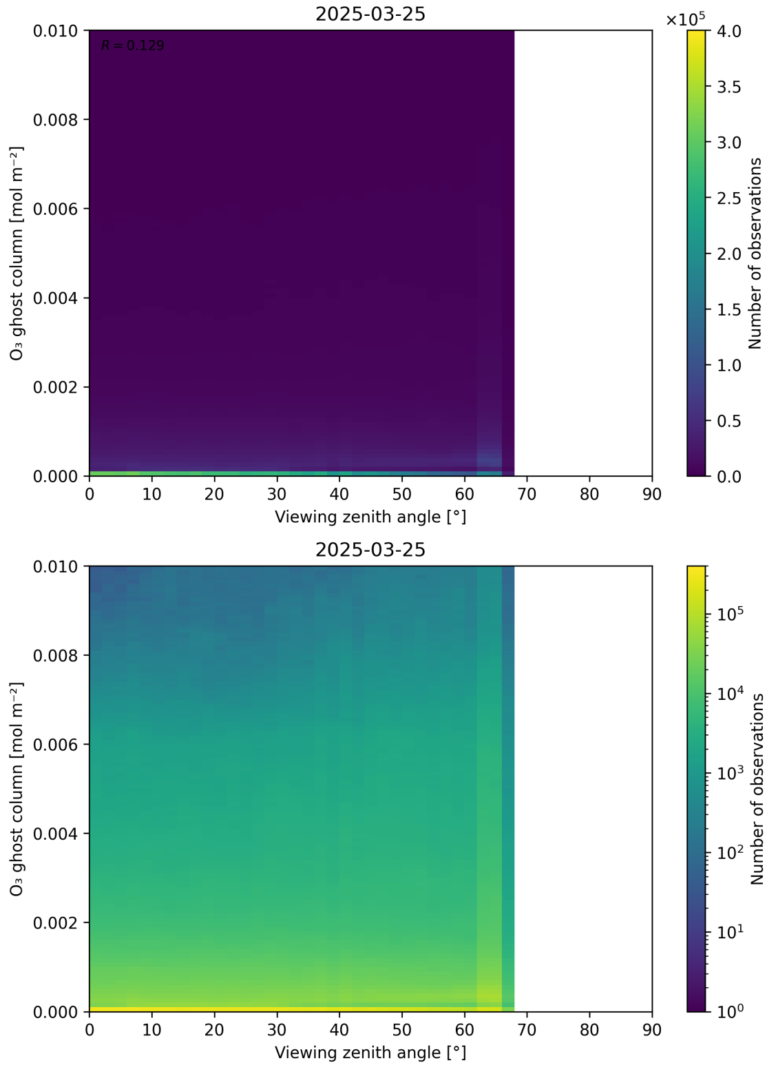
Figure 51: Scatter density plot of “Viewing zenith angle” against “O 3 ghost column” for 2025-03-24 to 2025-03-26.
