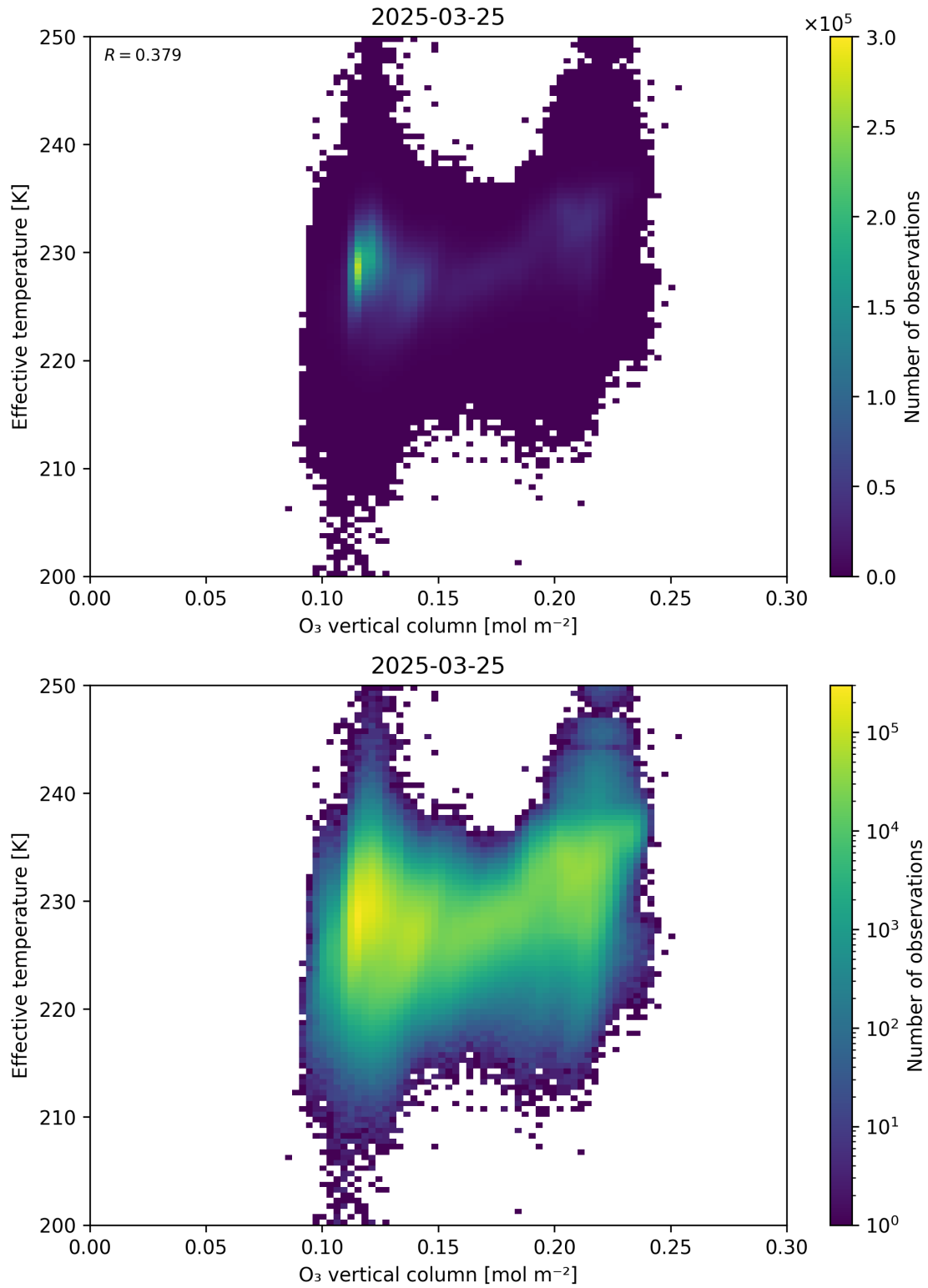
Figure 39: Scatter density plot of “O 3 vertical column” against “Effective temperature” for 2025-03-24 to 2025-03-26.
