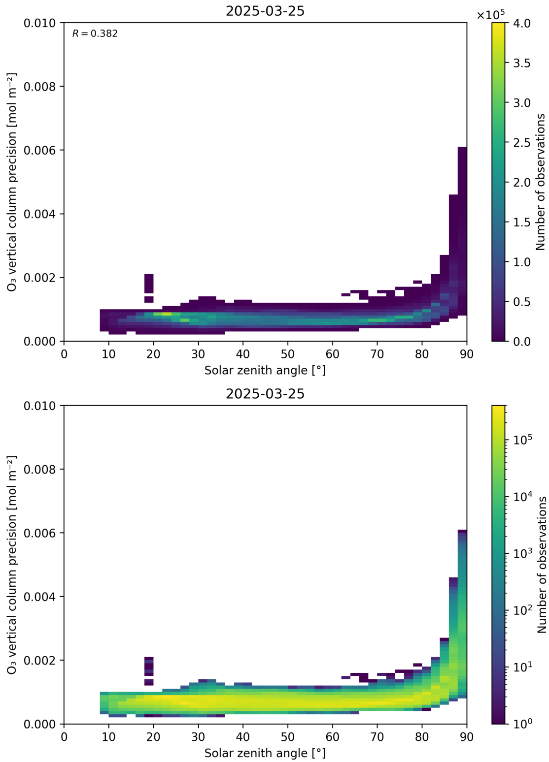
Figure 48: Scatter density plot of “Solar zenith angle” against “O 3 vertical column precision” for 2025-03-24 to 2025-03-26.
