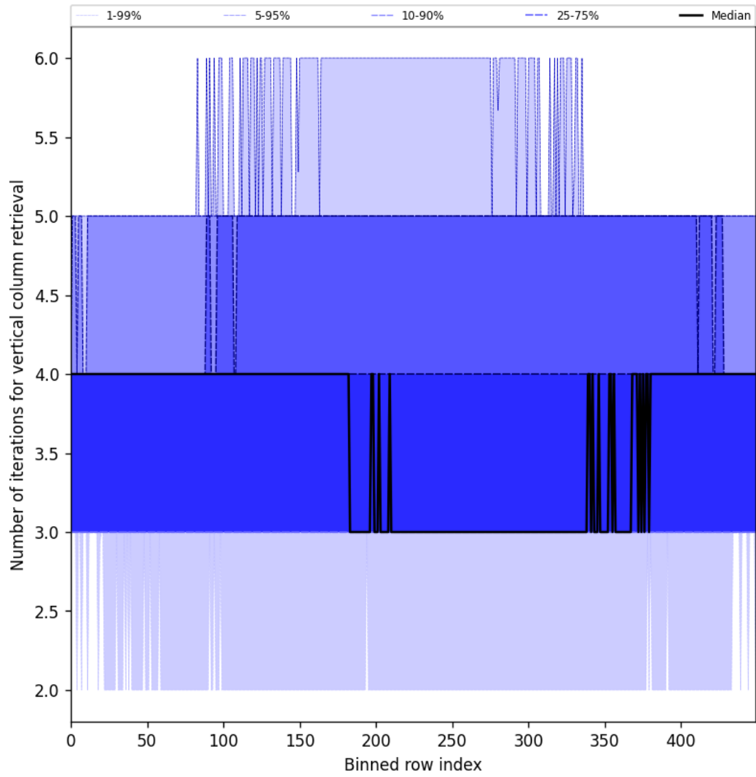
Figure 33: Along track statistics of “Number of iterations for vertical column retrieval” for 2025-03-24 to 2025-03-26
