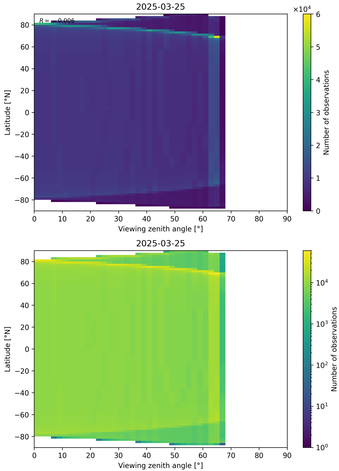
Figure 49: Scatter density plot of “Viewing zenith angle” against “Latitude” for 2025-03-24 to 2025-03-26.
