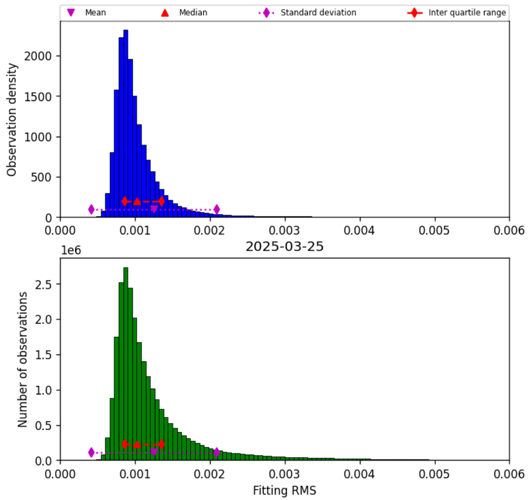
Figure 23: Histogram of “Fitting RMS” for 2025-03-24 to 2025-03-26
