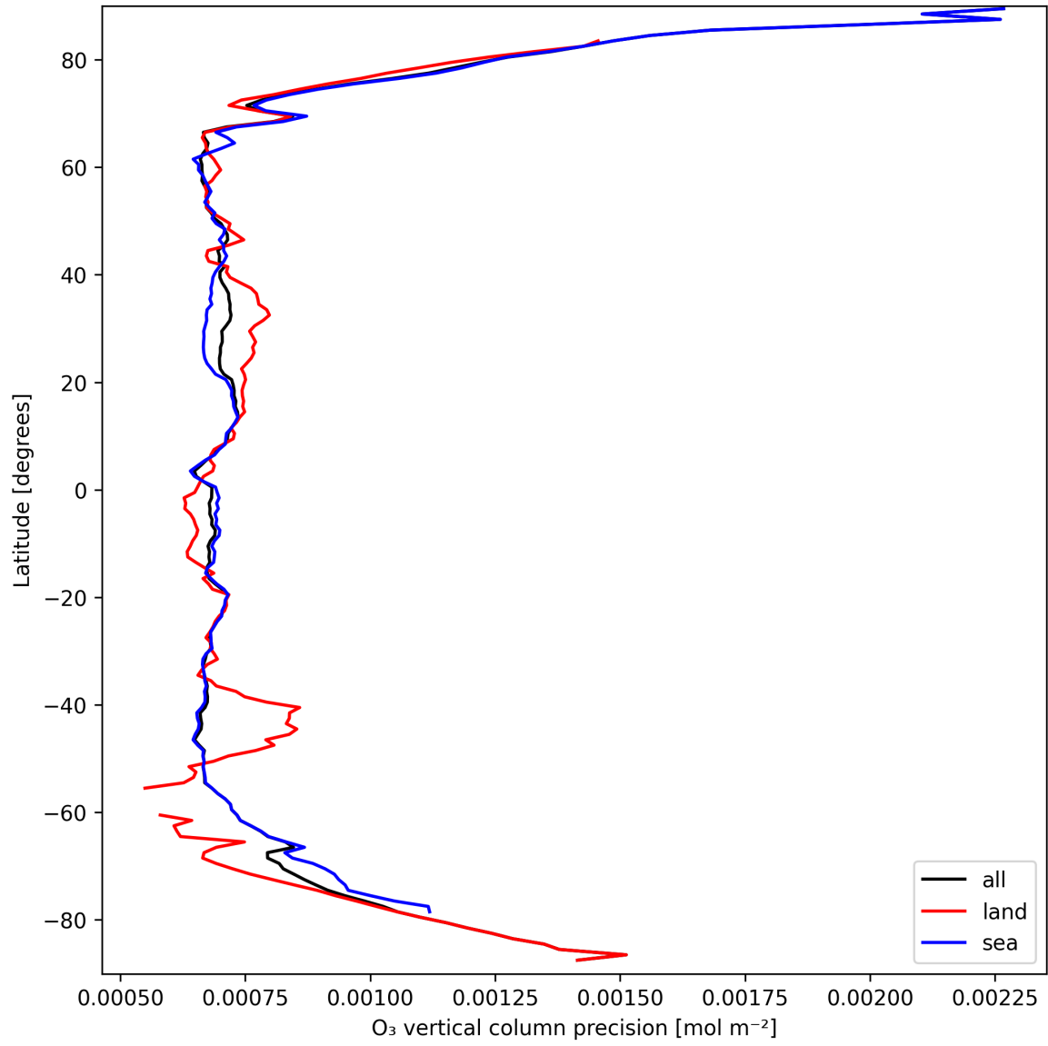
Figure 15: Zonal average of "O 3 vertical column precision" for 2025-03-24 to 2025-03-26.
