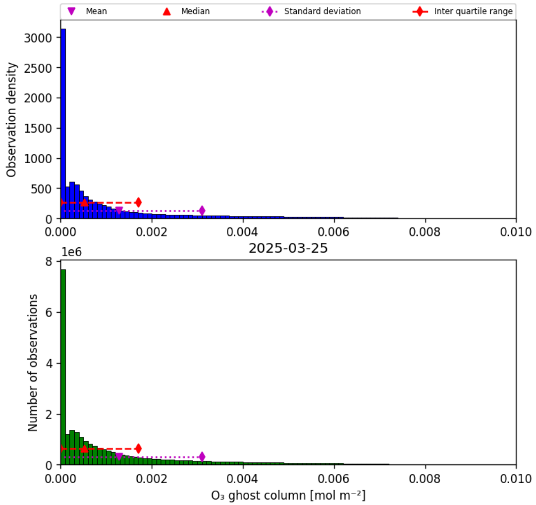
Figure 25: Histogram of “O 3 ghost column” for 2025-03-24 to 2025-03-26
