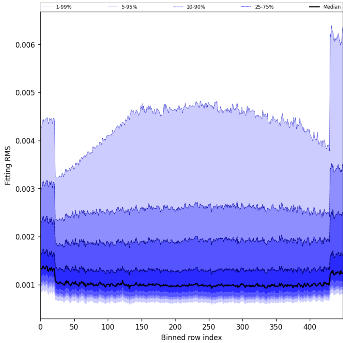
Figure 30: Along track statistics of “Fitting RMS” for 2025-03-24 to 2025-03-26
