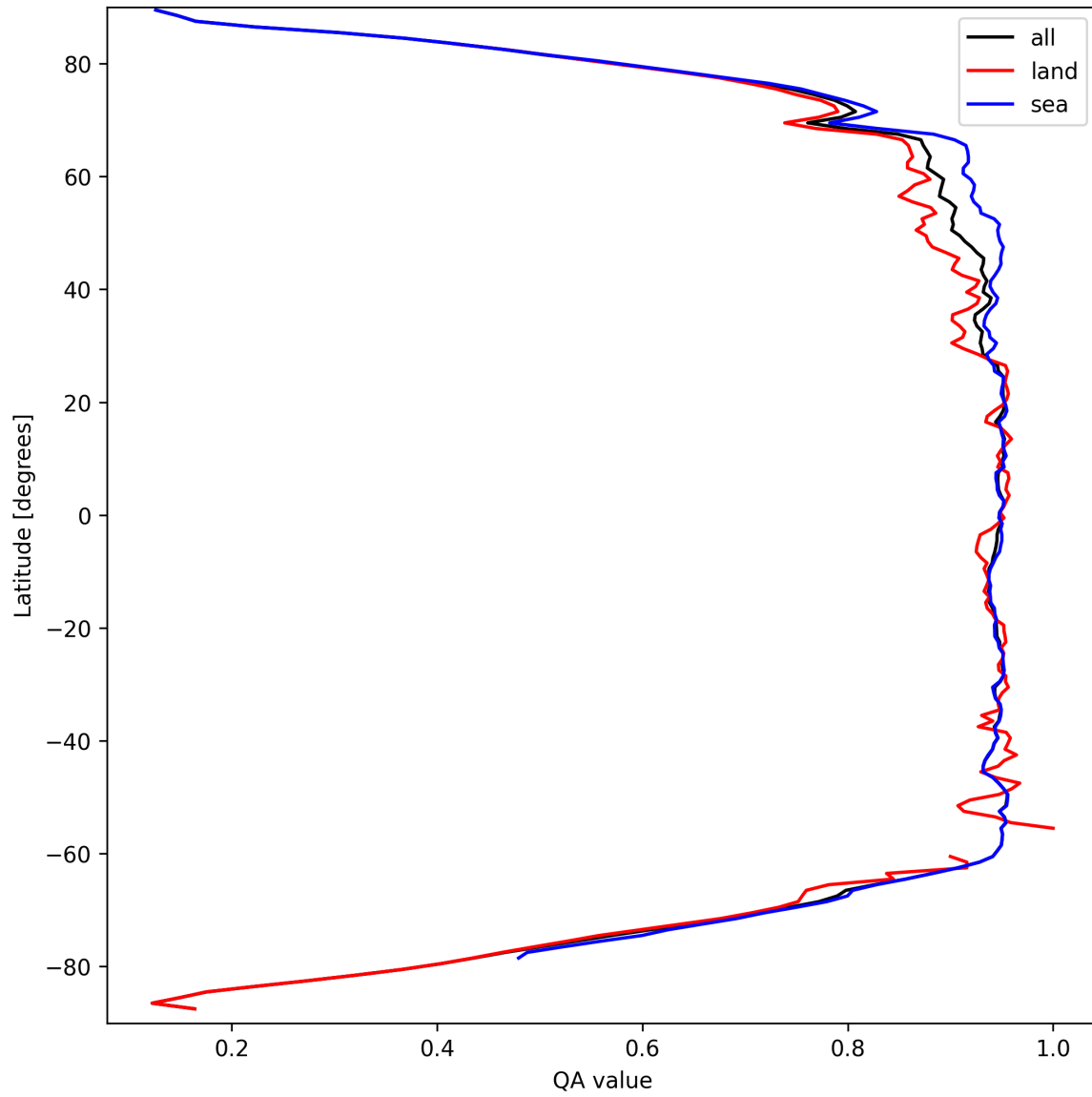
Figure 13: Zonal average of “QA value” for 2025-03-24 to 2025-03-26.
