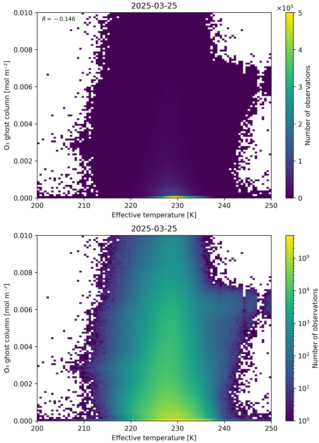
Figure 38: Scatter density plot of “Effective temperature” against “O 3 ghost column” for 2025-03-24 to 2025-03-26.
