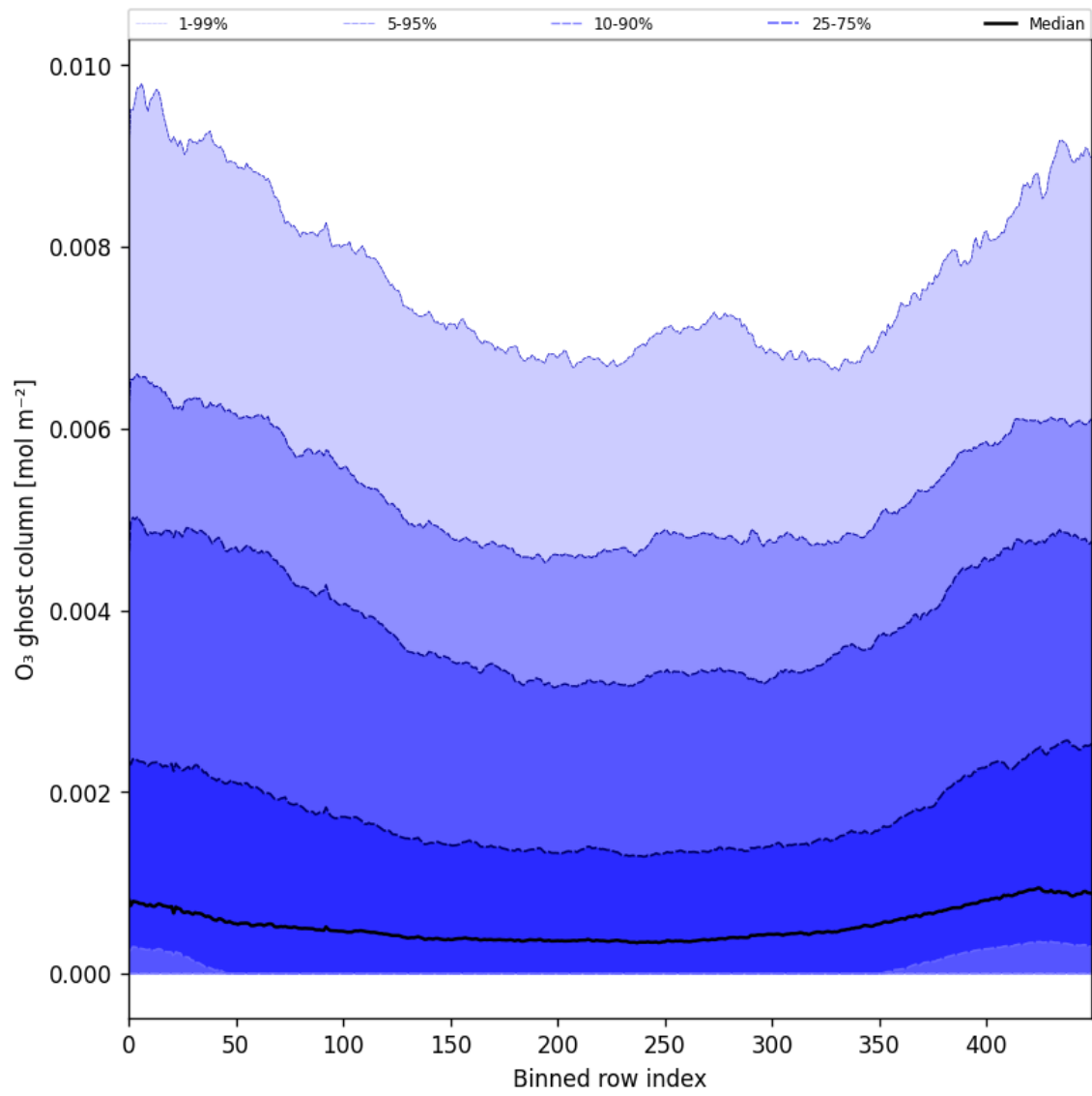
Figure 32: Along track statistics of “O 3 ghost column” for 2025-03-24 to 2025-03-26
