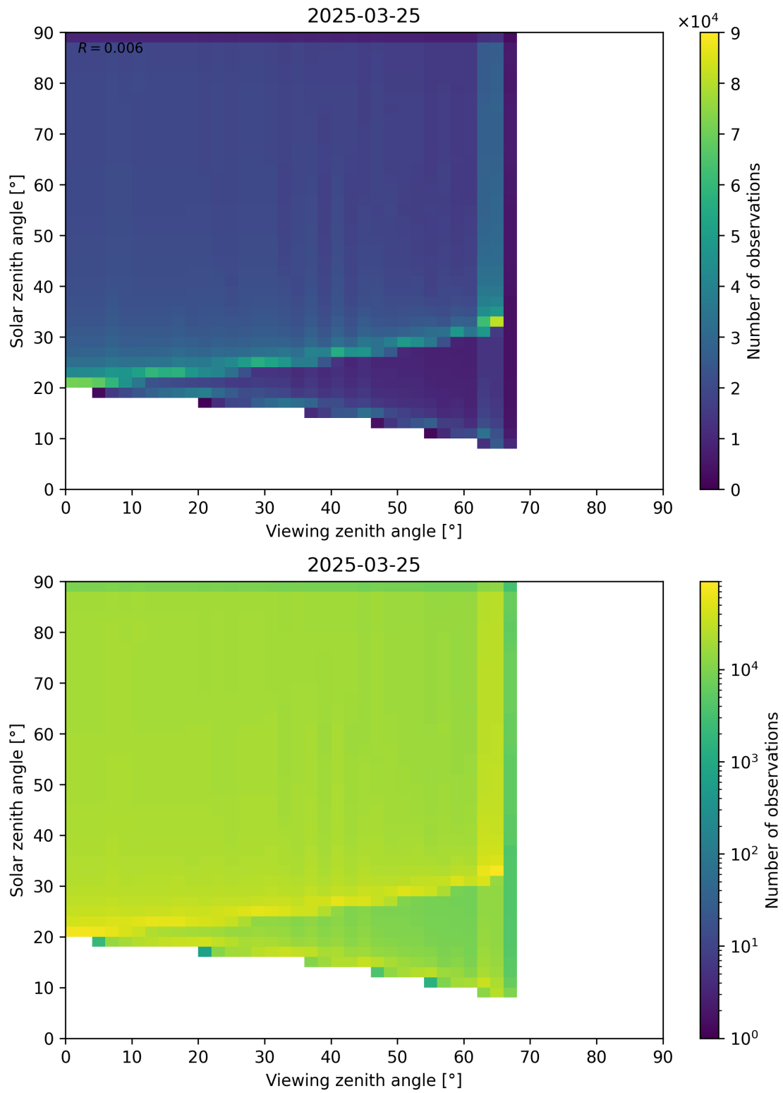
Figure 54: Scatter density plot of “Viewing zenith angle” against “Solar zenith angle” for 2025-03-24 to 2025-03-26.
