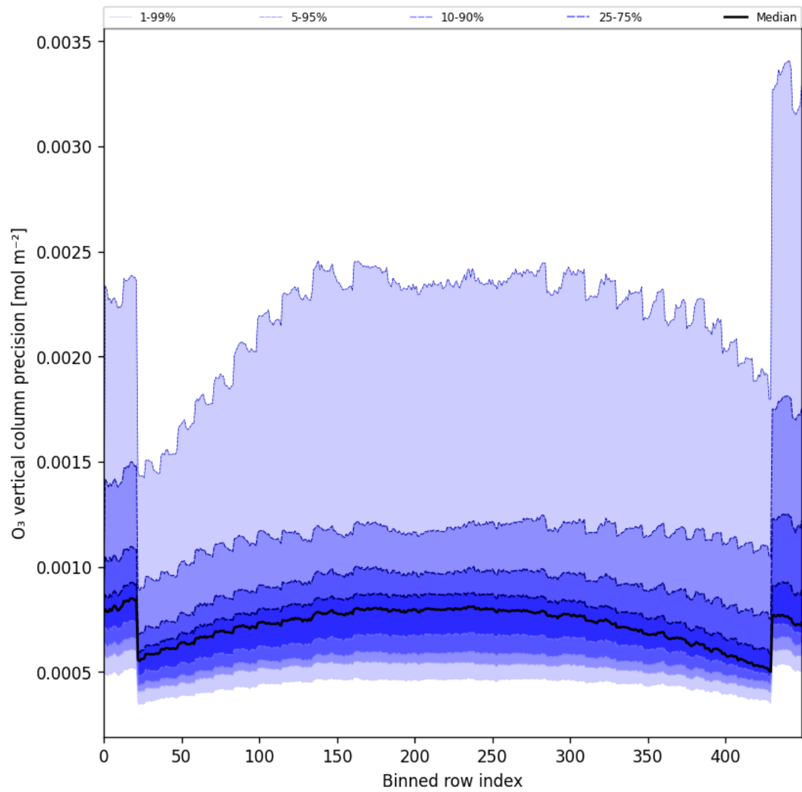
Figure 29: Along track statistics of “O 3 vertical column precision” for 2025-03-24 to 2025-03-26
