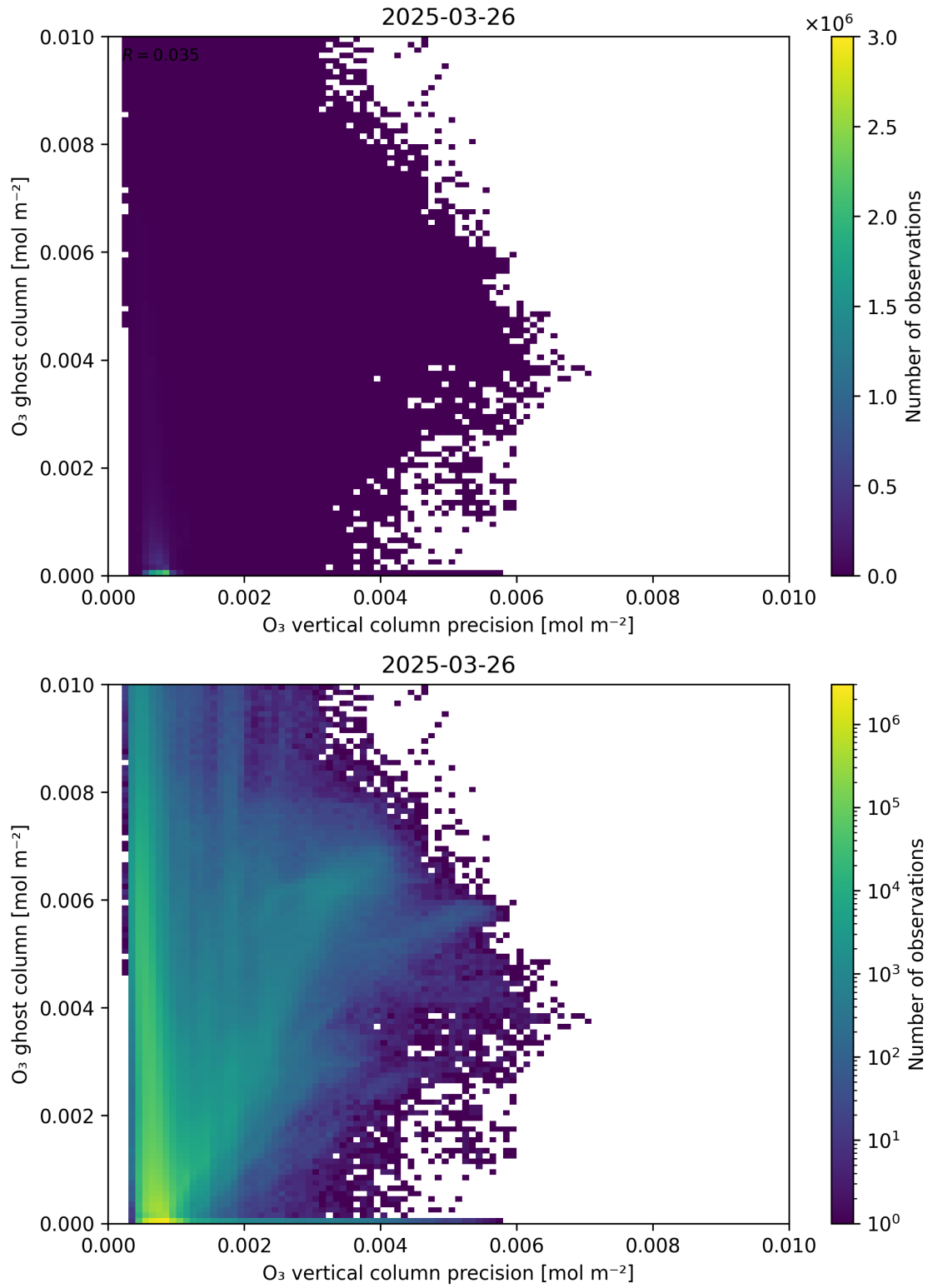
Figure 43: Scatter density plot of “ O_3 vertical column precision” against “ O_3 ghost column” for 2025-03-25 to 2025-03-27.
