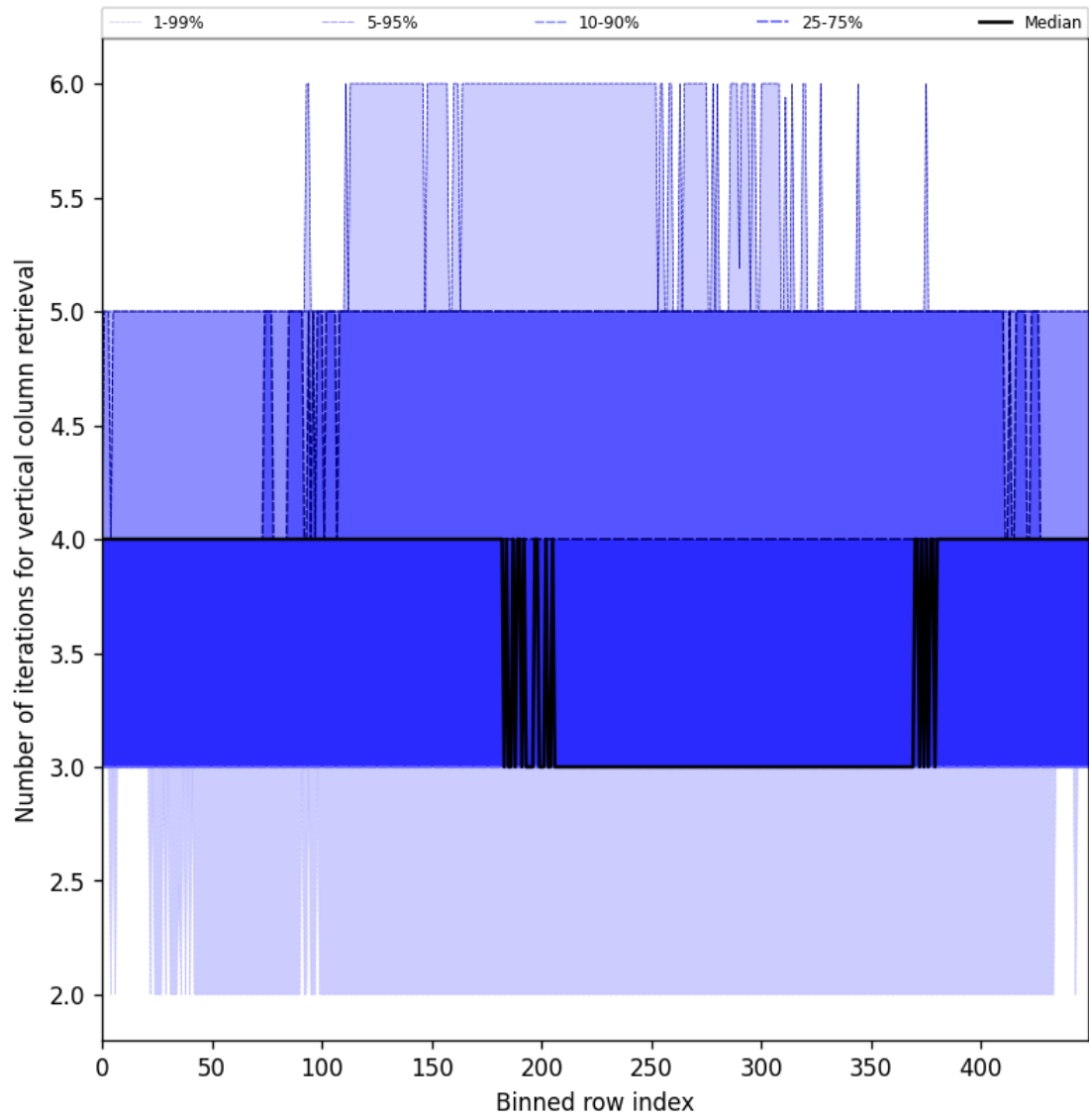
Figure 33: Along track statistics of “Number of iterations for vertical column retrieval” for 2025-03-25 to 2025-03-27
