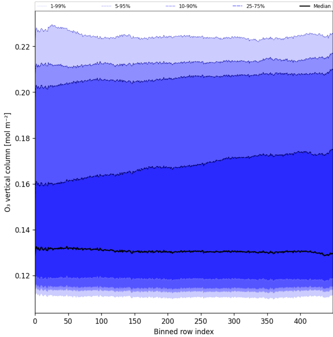
Figure 28: Along track statistics of “O 3 vertical column” for 2025-03-25 to 2025-03-27
