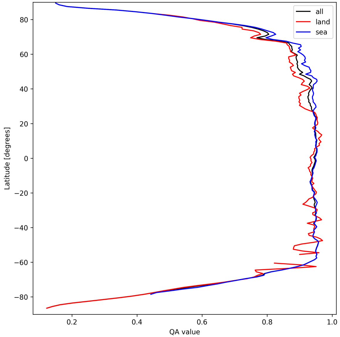
Figure 13: Zonal average of “QA value” for 2025-03-25 to 2025-03-27.
