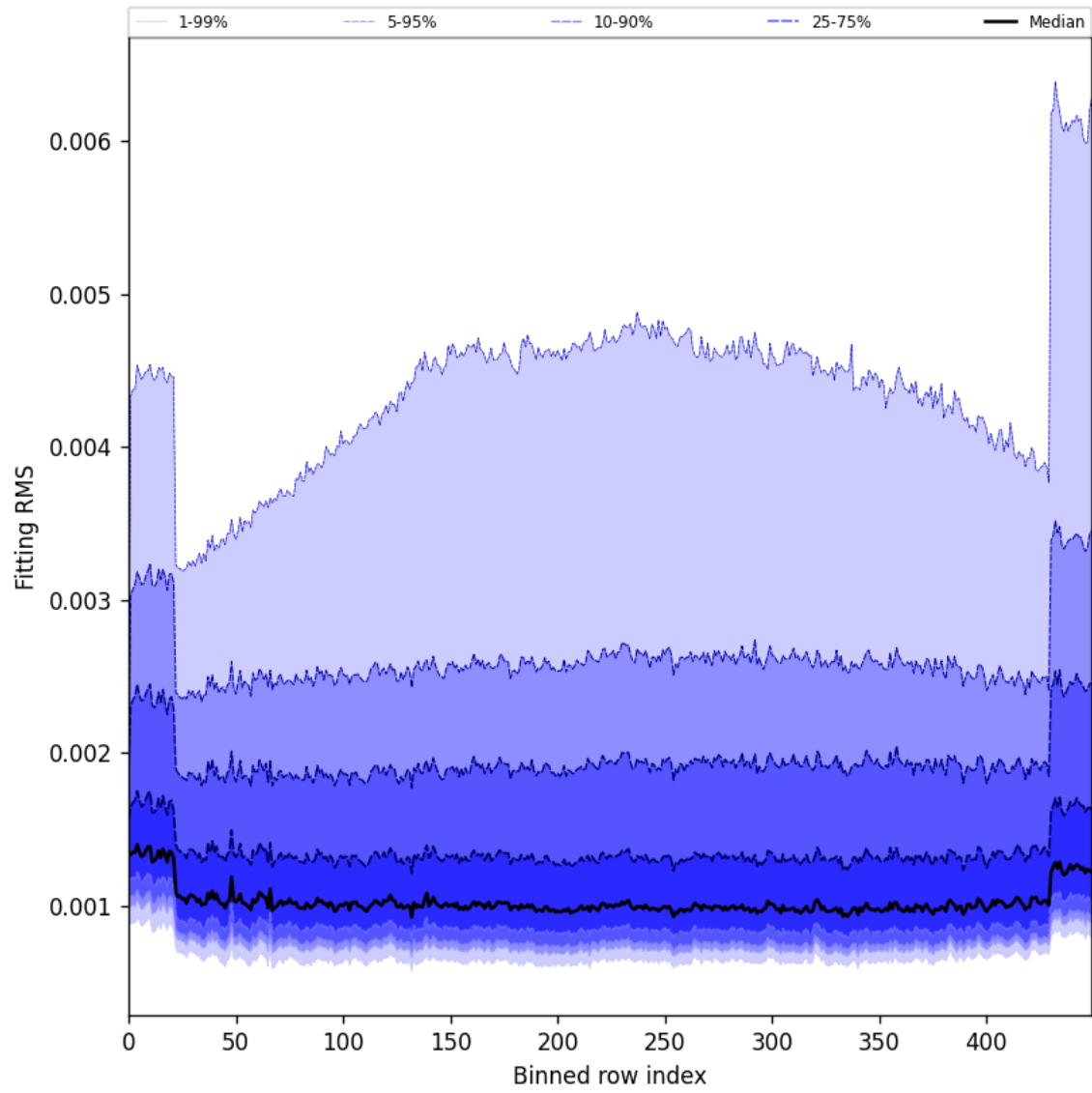
Figure 30: Along track statistics of “Fitting RMS” for 2025-03-25 to 2025-03-27
