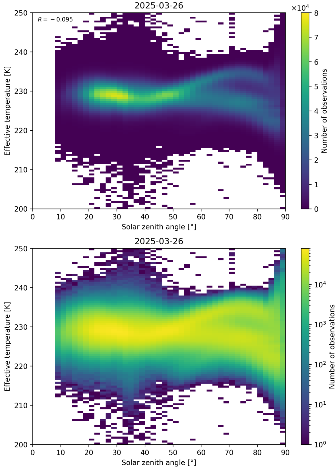
Figure 45: Scatter density plot of “Solar zenith angle” against “Effective temperature” for 2025-03-25 to 2025-03-27.
