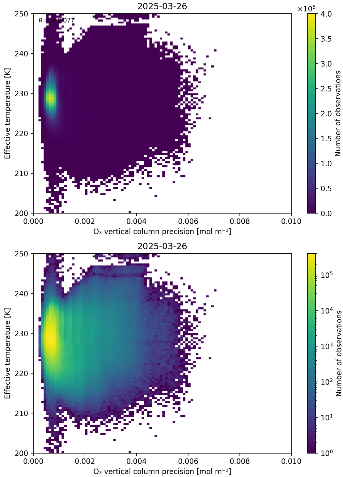
Figure 42: Scatter density plot of “O 3 vertical column precision” against “Effective temperature” for 2025-03-25 to 2025-03-27.
