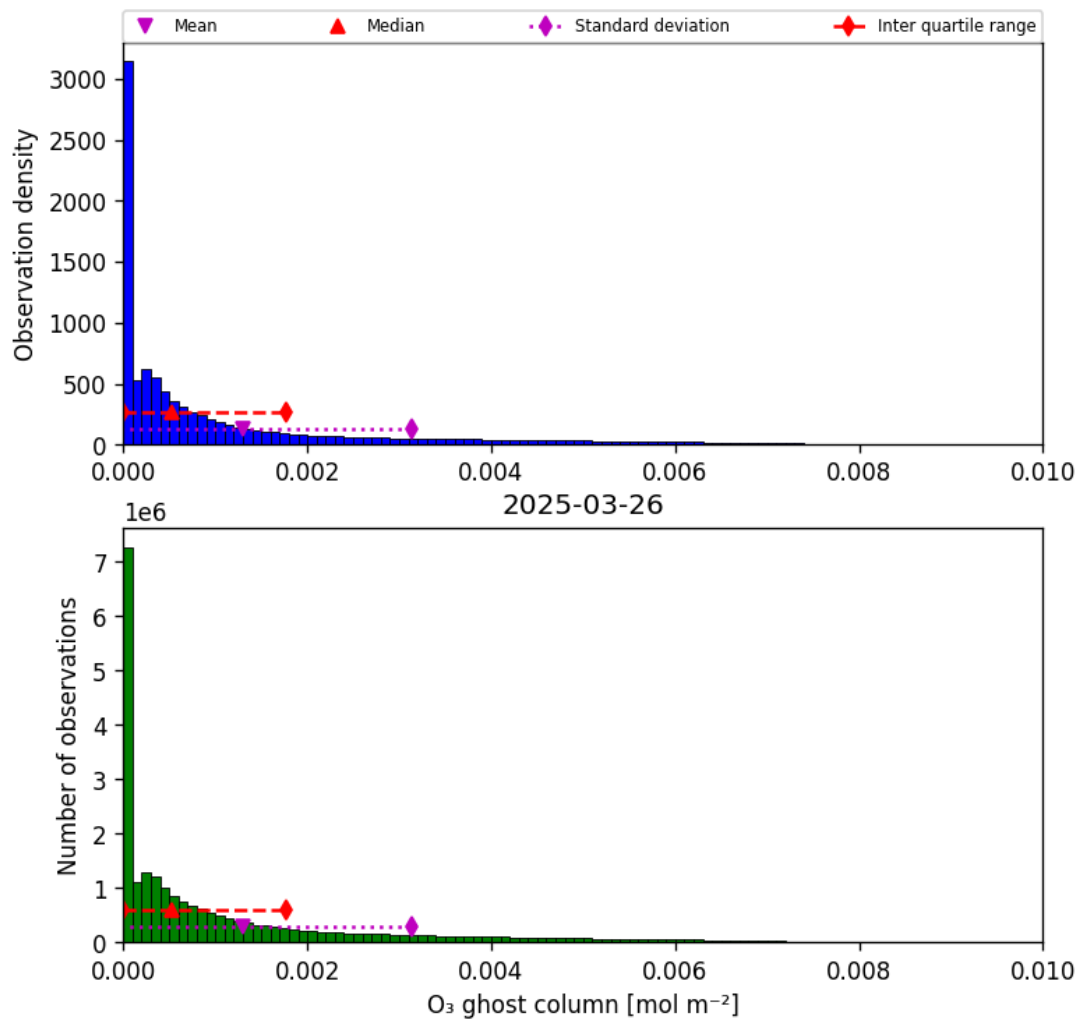
Figure 25: Histogram of “O 3 ghost column” for 2025-03-25 to 2025-03-27
