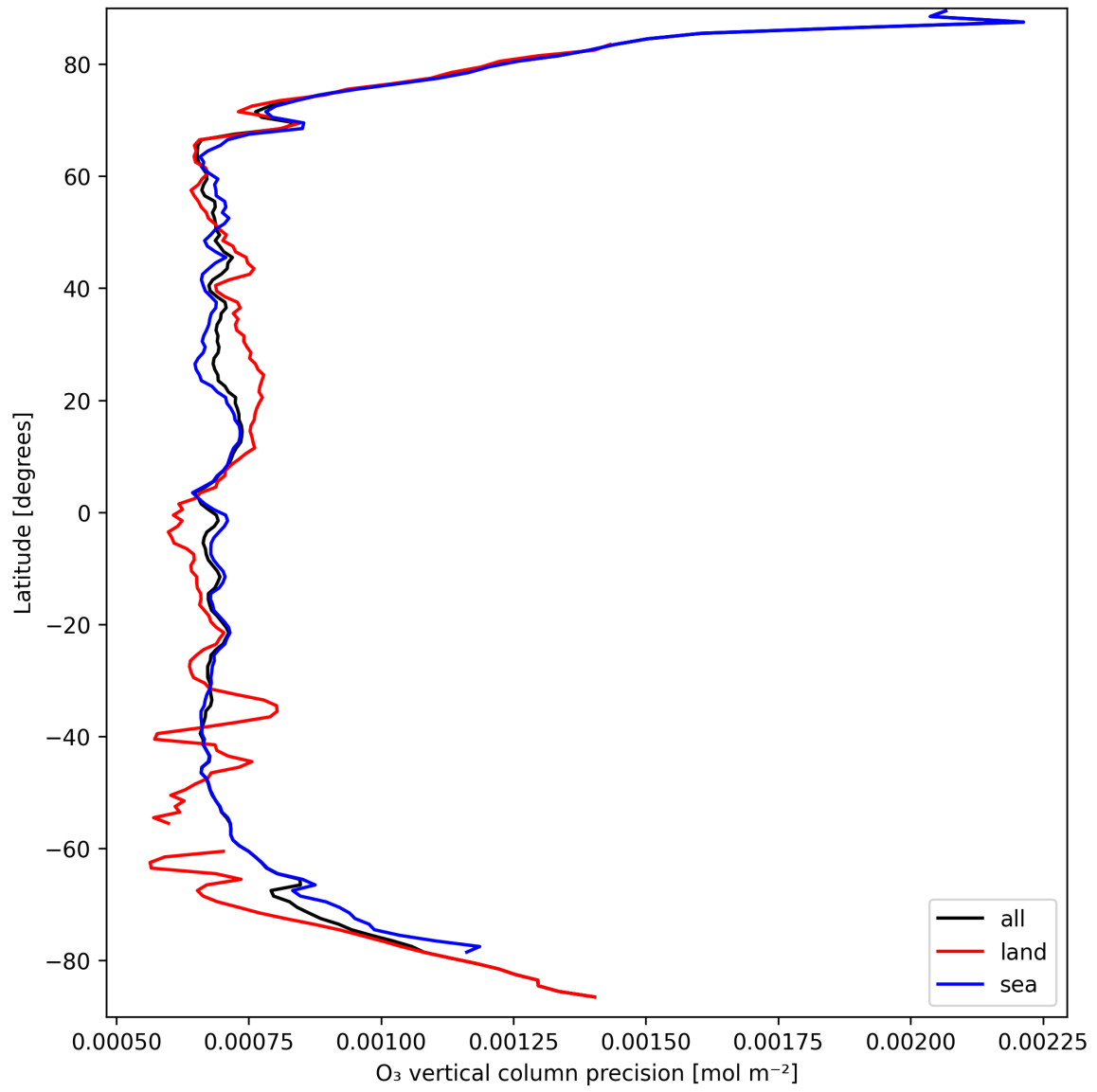
Figure 15: Zonal average of “O 3 vertical column precision” for 2025-03-25 to 2025-03-27.
