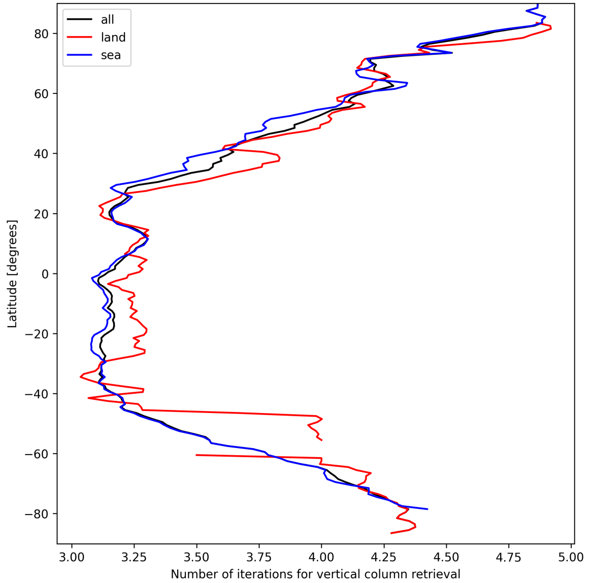
Figure 19: Zonal average of “Number of iterations for vertical column retrieval” for 2025-03-25 to 2025-03-27.
