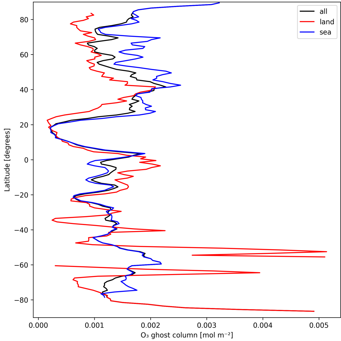
Figure 18: Zonal average of "O 3 ghost column" for 2025-03-25 to 2025-03-27.
