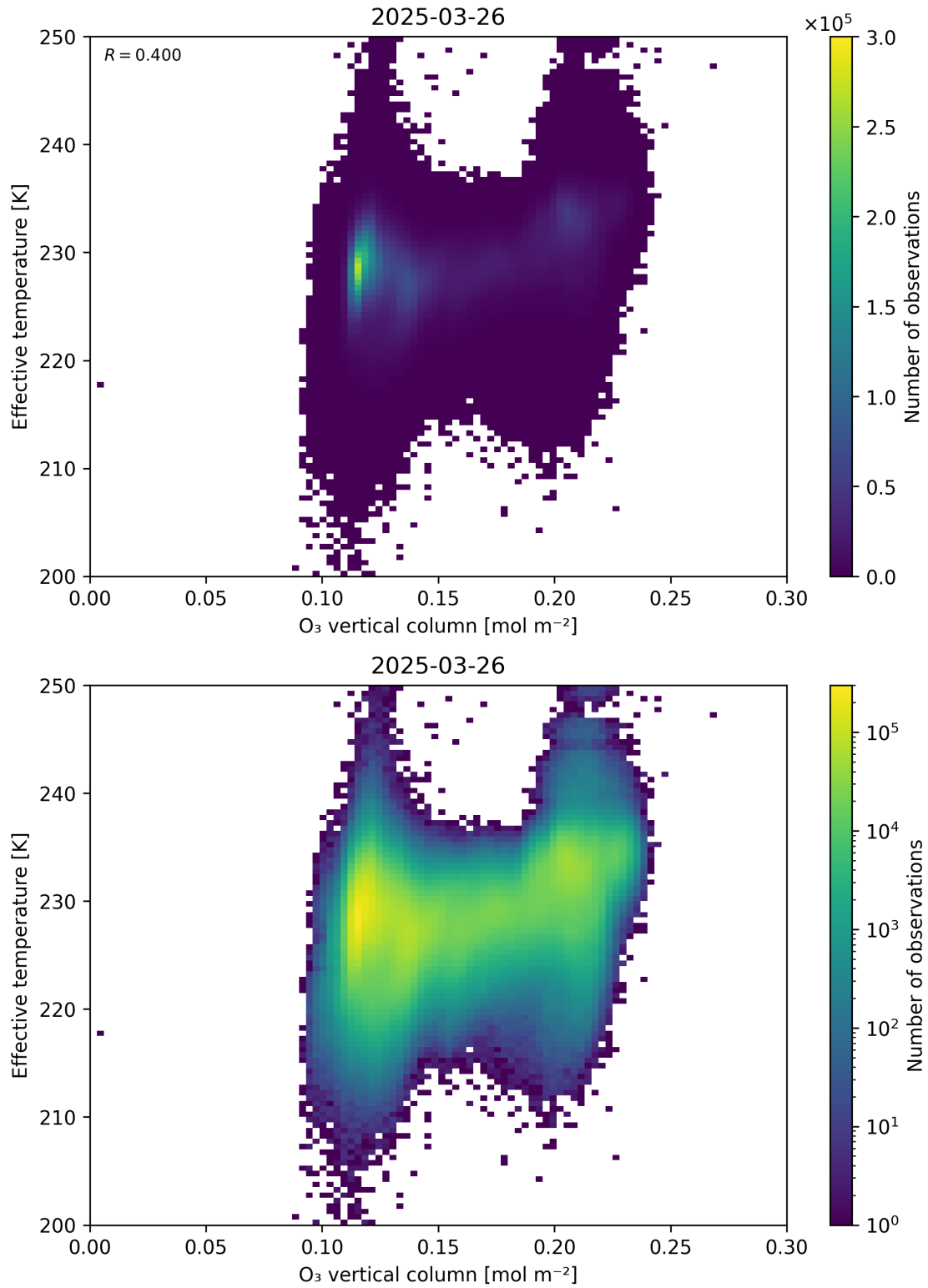
Figure 39: Scatter density plot of “O 3 vertical column” against “Effective temperature” for 2025-03-25 to 2025-03-27.
