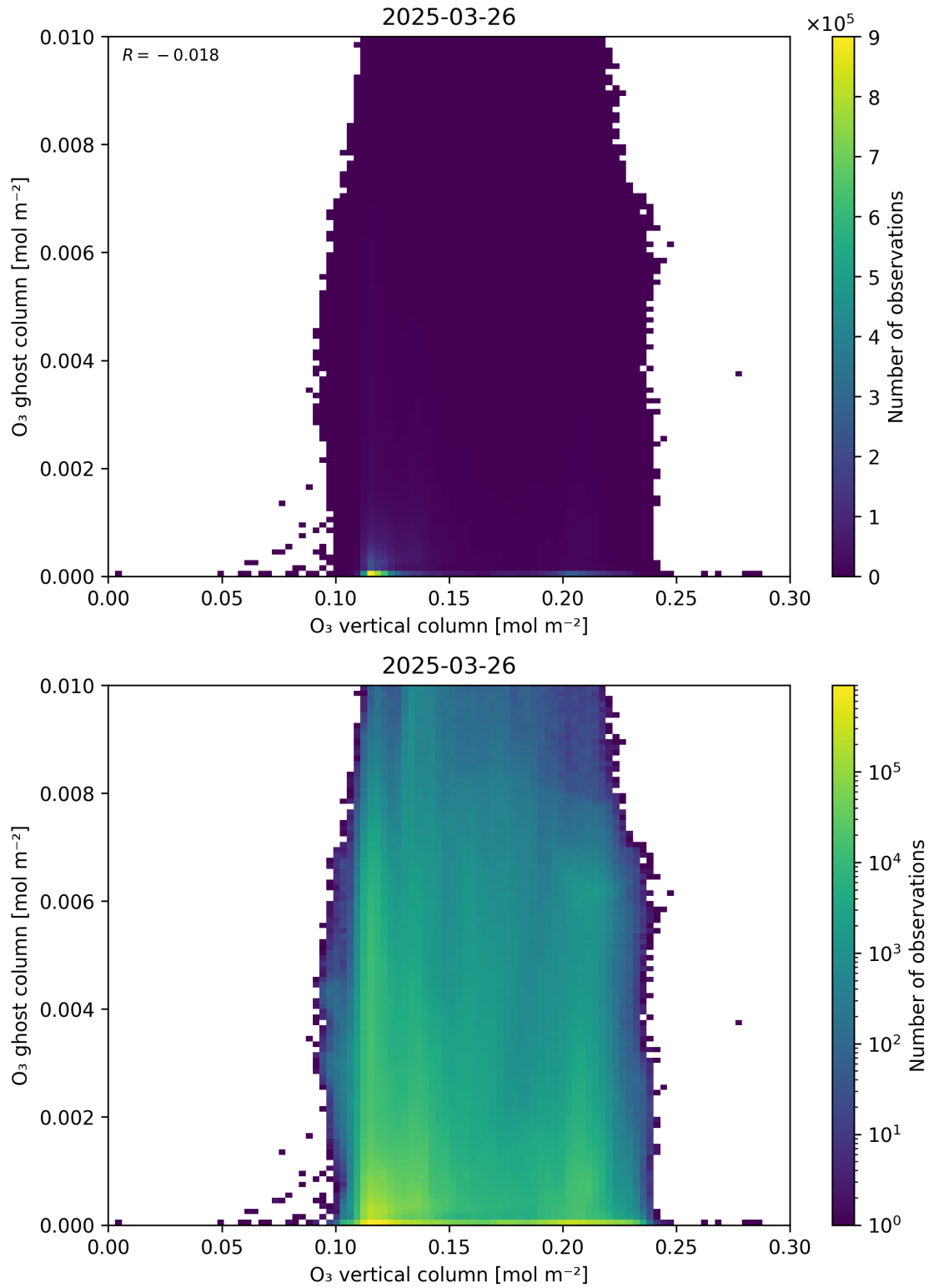
Figure 40: Scatter density plot of “O 3 vertical column” against “O 3 ghost column” for 2025-03-25 to 2025-03-27.
