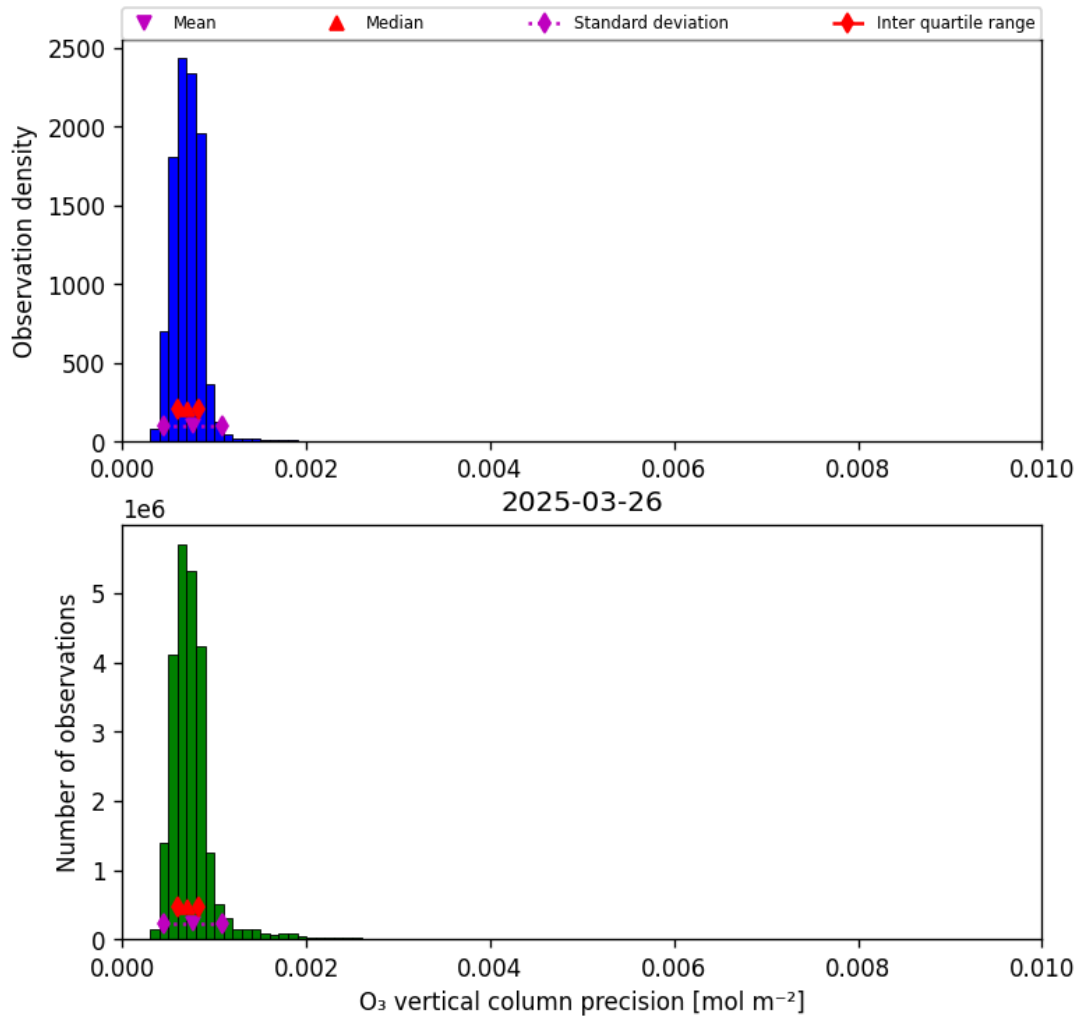
Figure 22: Histogram of “O 3 vertical column precision” for 2025-03-25 to 2025-03-27
