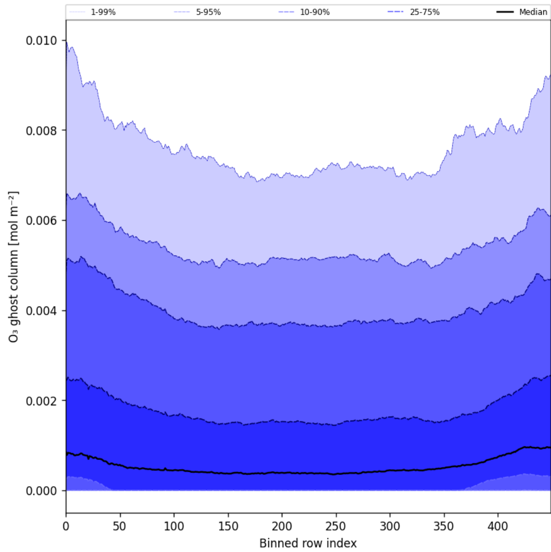
Figure 32: Along track statistics of “O 3 ghost column” for 2025-03-25 to 2025-03-27
