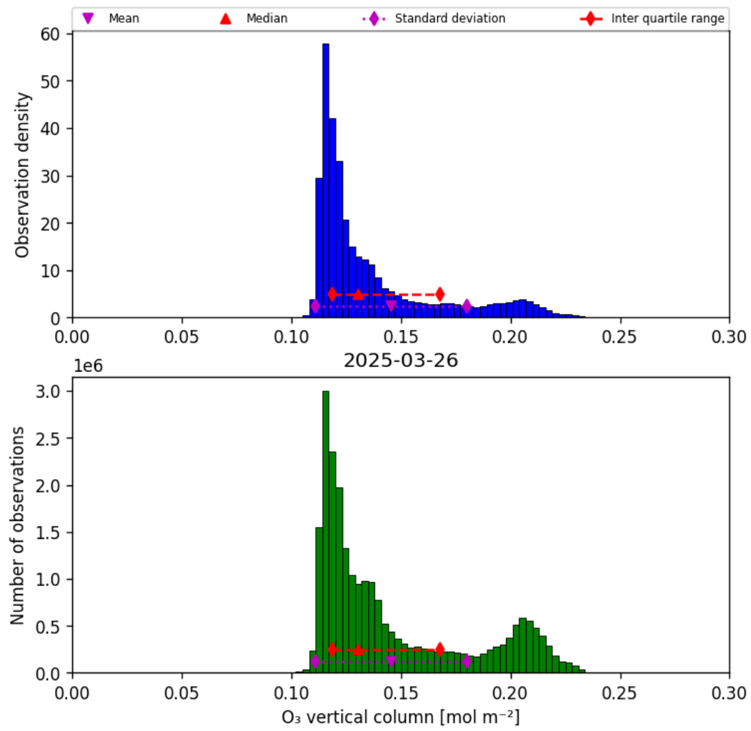
Figure 21: Histogram of “O 3 vertical column” for 2025-03-25 to 2025-03-27
