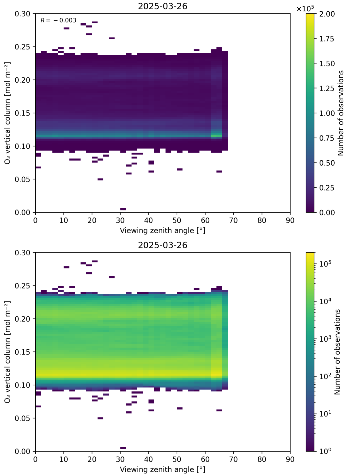
Figure 52: Scatter density plot of “Viewing zenith angle” against “O 3 vertical column” for 2025-03-25 to 2025-03-27.
