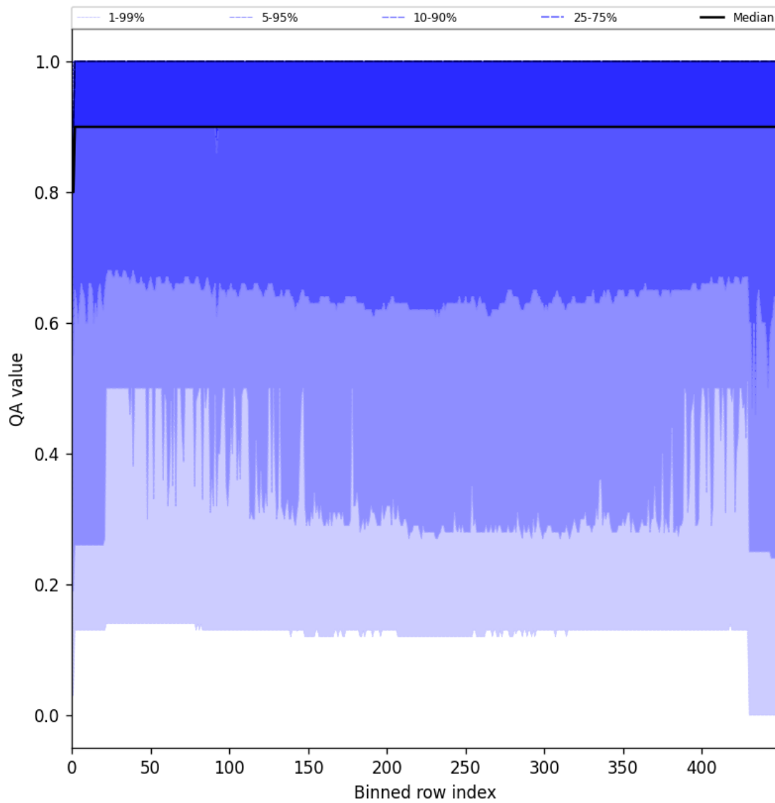
Figure 27: Along track statistics of “QA value” for 2025-03-25 to 2025-03-27
