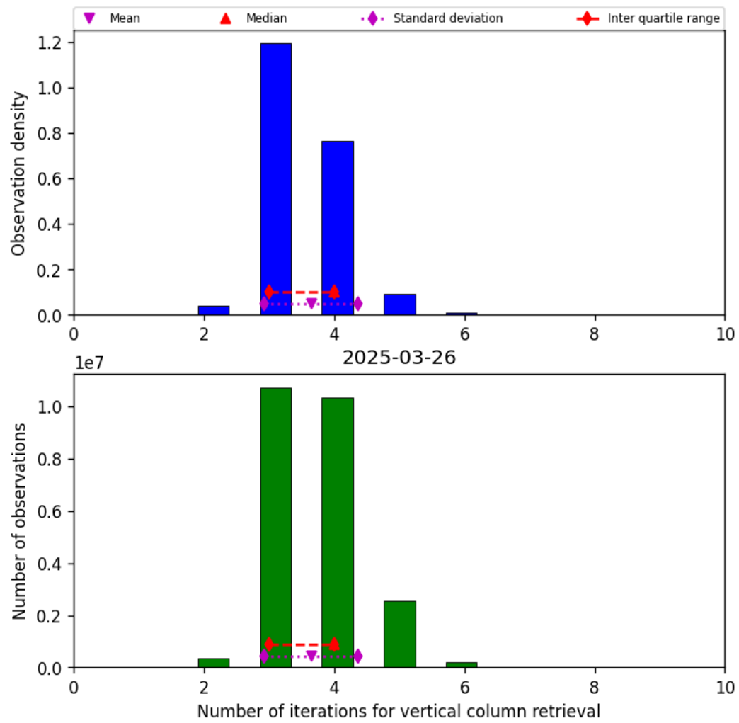
Figure 26: Histogram of “Number of iterations for vertical column retrieval” for 2025-03-25 to 2025-03-27
