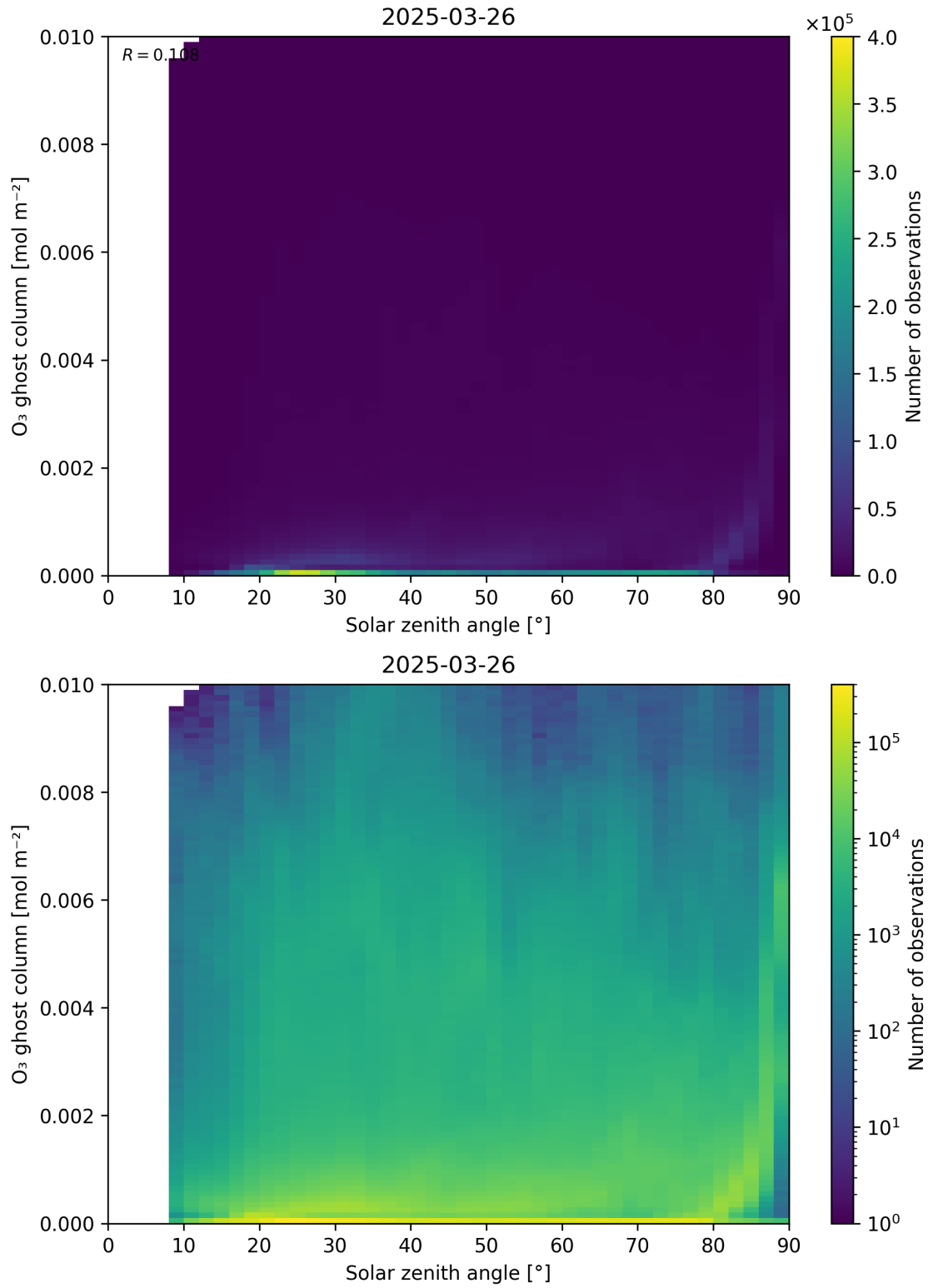
Figure 46: Scatter density plot of “Solar zenith angle” against “O 3 ghost column” for 2025-03-25 to 2025-03-27.
