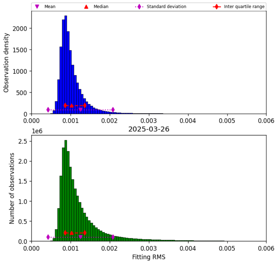
Figure 23: Histogram of “Fitting RMS” for 2025-03-25 to 2025-03-27
