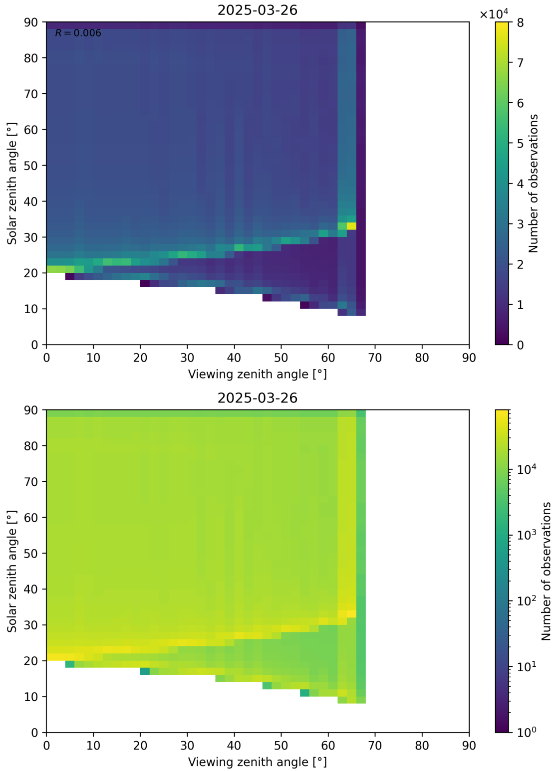
Figure 54: Scatter density plot of “Viewing zenith angle” against “Solar zenith angle” for 2025-03-25 to 2025-03-27.
