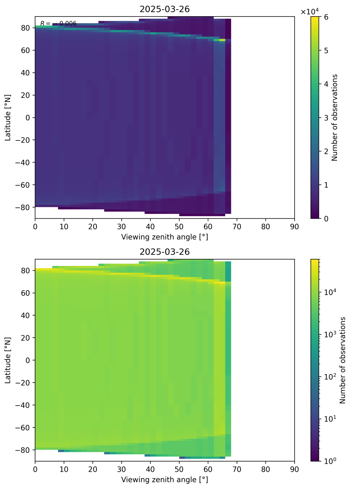
Figure 49: Scatter density plot of “Viewing zenith angle” against “Latitude” for 2025-03-25 to 2025-03-27.
