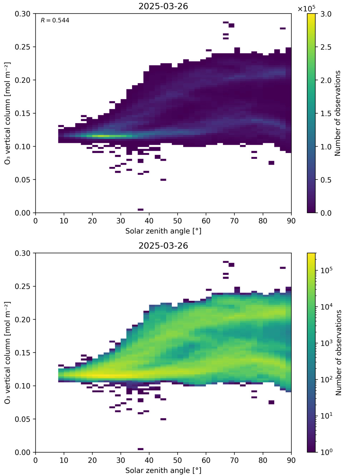
Figure 47: Scatter density plot of “Solar zenith angle” against “O 3 vertical column” for 2025-03-25 to 2025-03-27.
