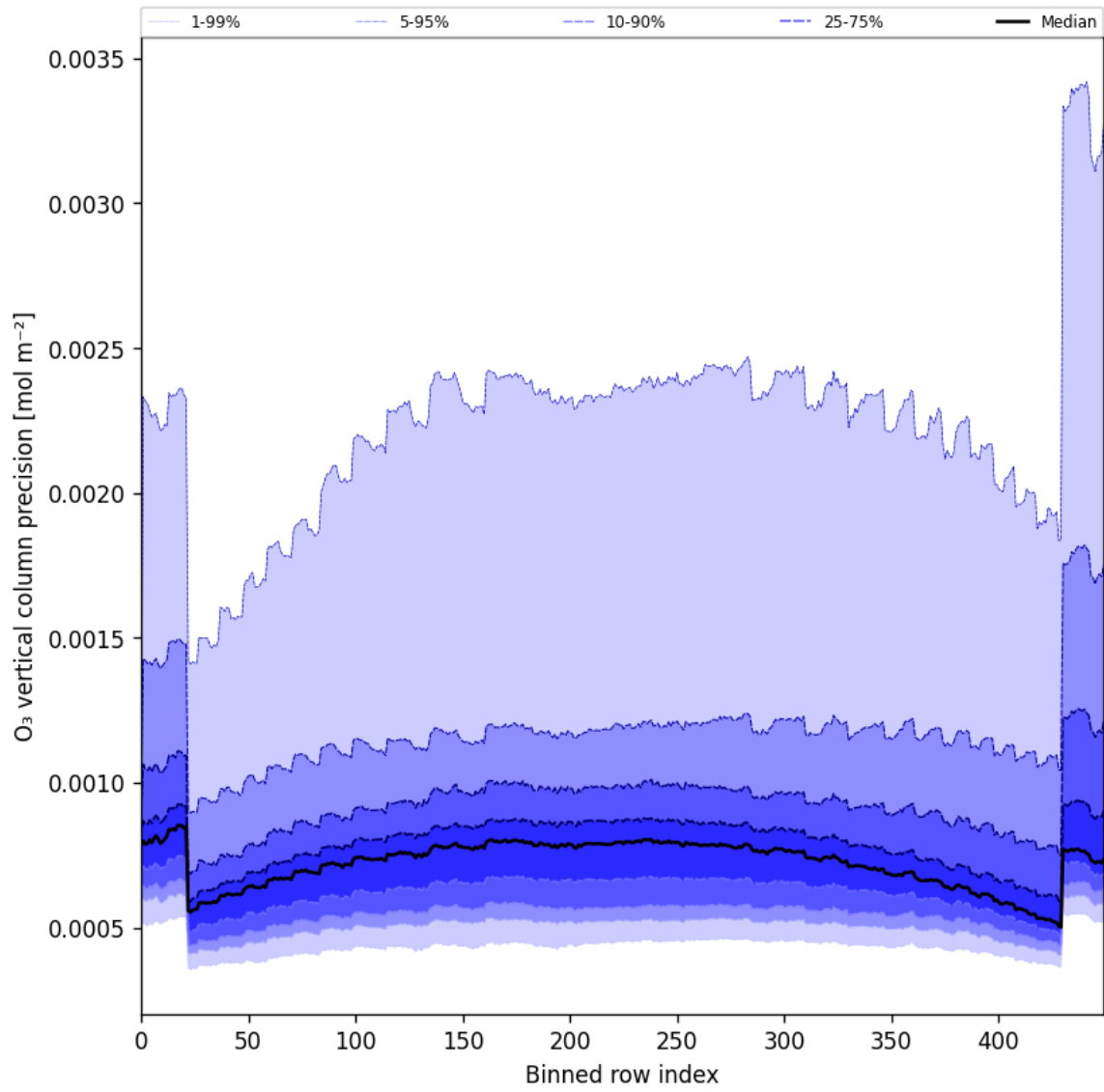
Figure 29: Along track statistics of “O 3 vertical column precision” for 2025-03-25 to 2025-03-27
