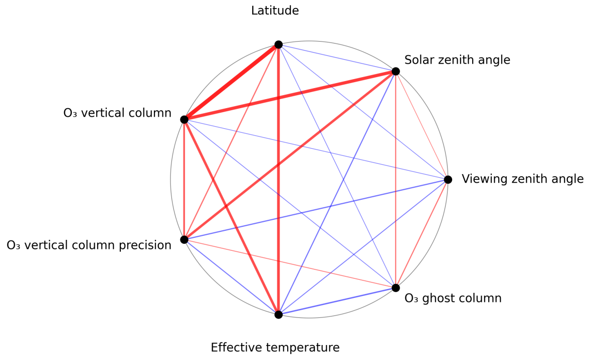
Figure 1: Map of correlation graph for 2025-03-25 to 2025-03-27.
