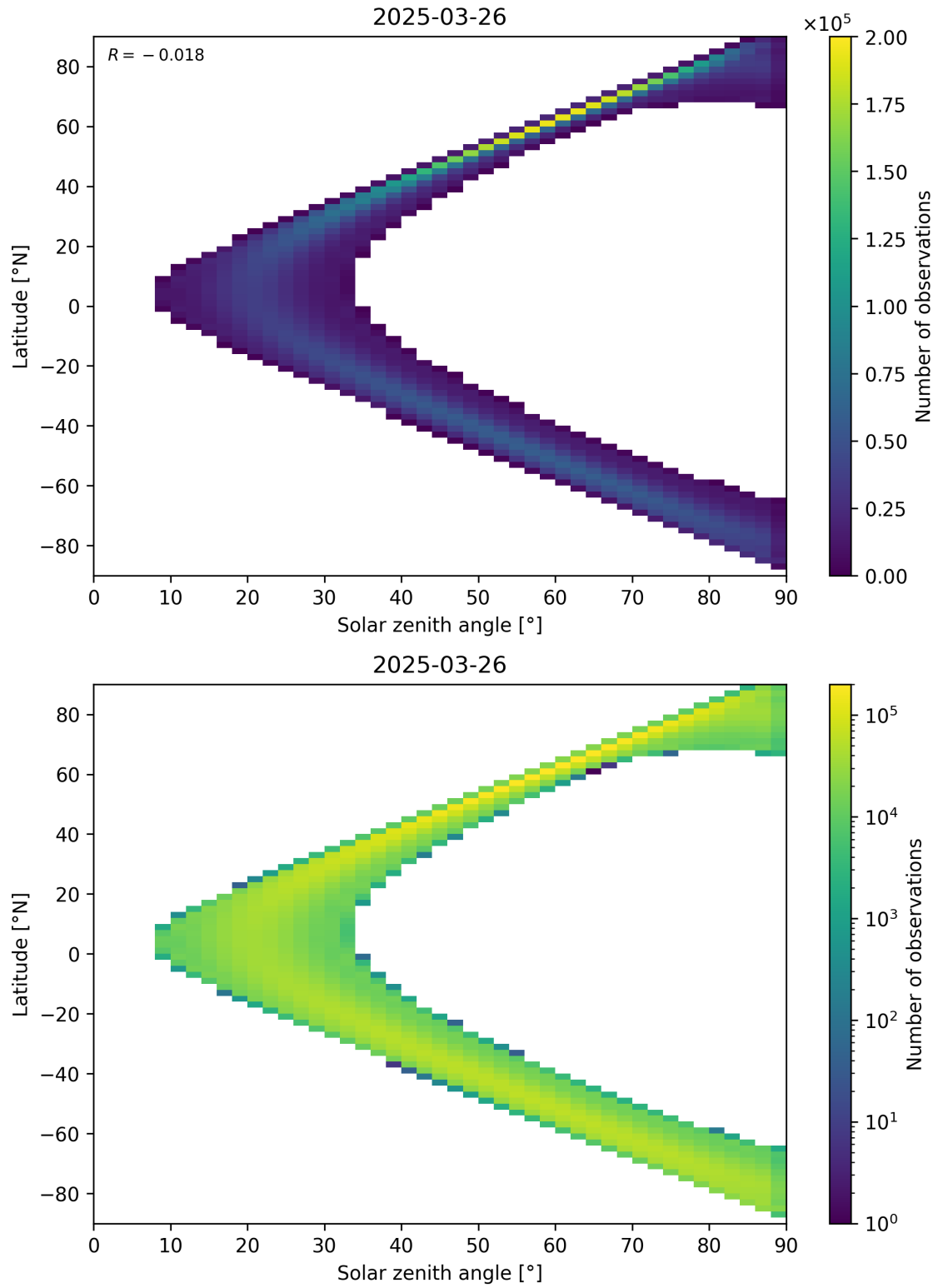
Figure 44: Scatter density plot of “Solar zenith angle” against “Latitude” for 2025-03-25 to 2025-03-27.
