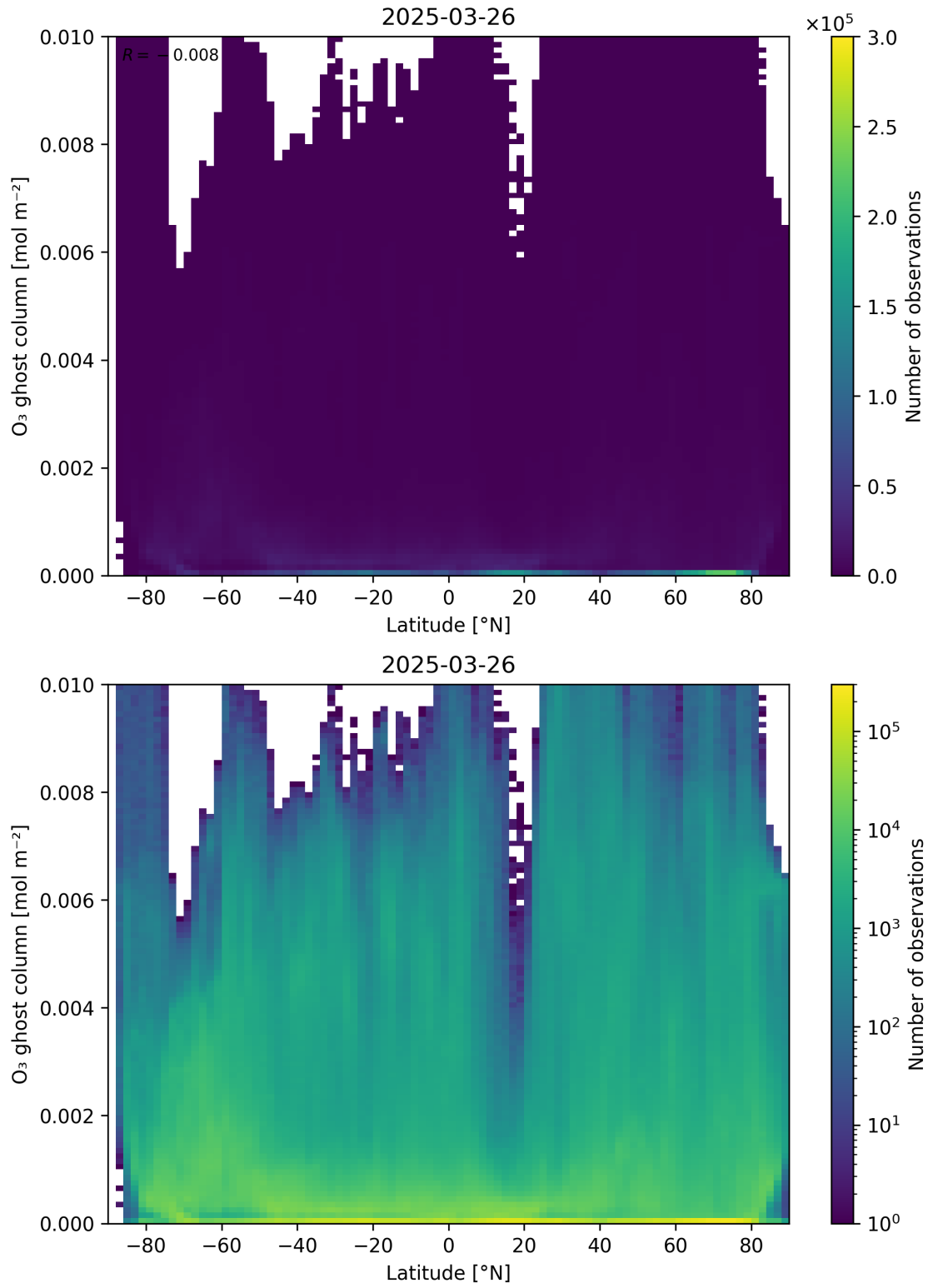
Figure 35: Scatter density plot of “Latitude” against “O 3 ghost column” for 2025-03-25 to 2025-03-27.
