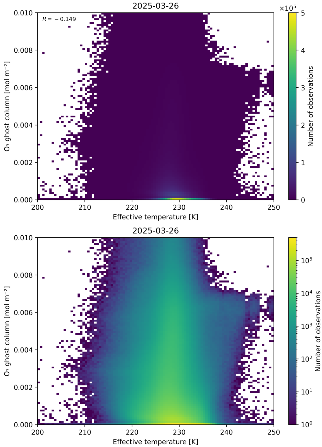
Figure 38: Scatter density plot of “Effective temperature” against “O 3 ghost column” for 2025-03-25 to 2025-03-27.
