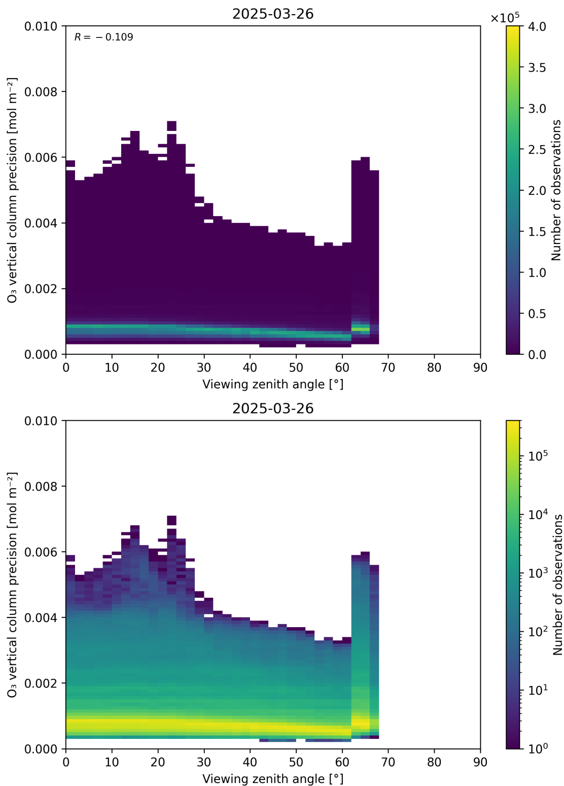
Figure 53: Scatter density plot of “Viewing zenith angle” against “O 3 vertical column precision” for 2025-03-25 to 2025-03-27.
