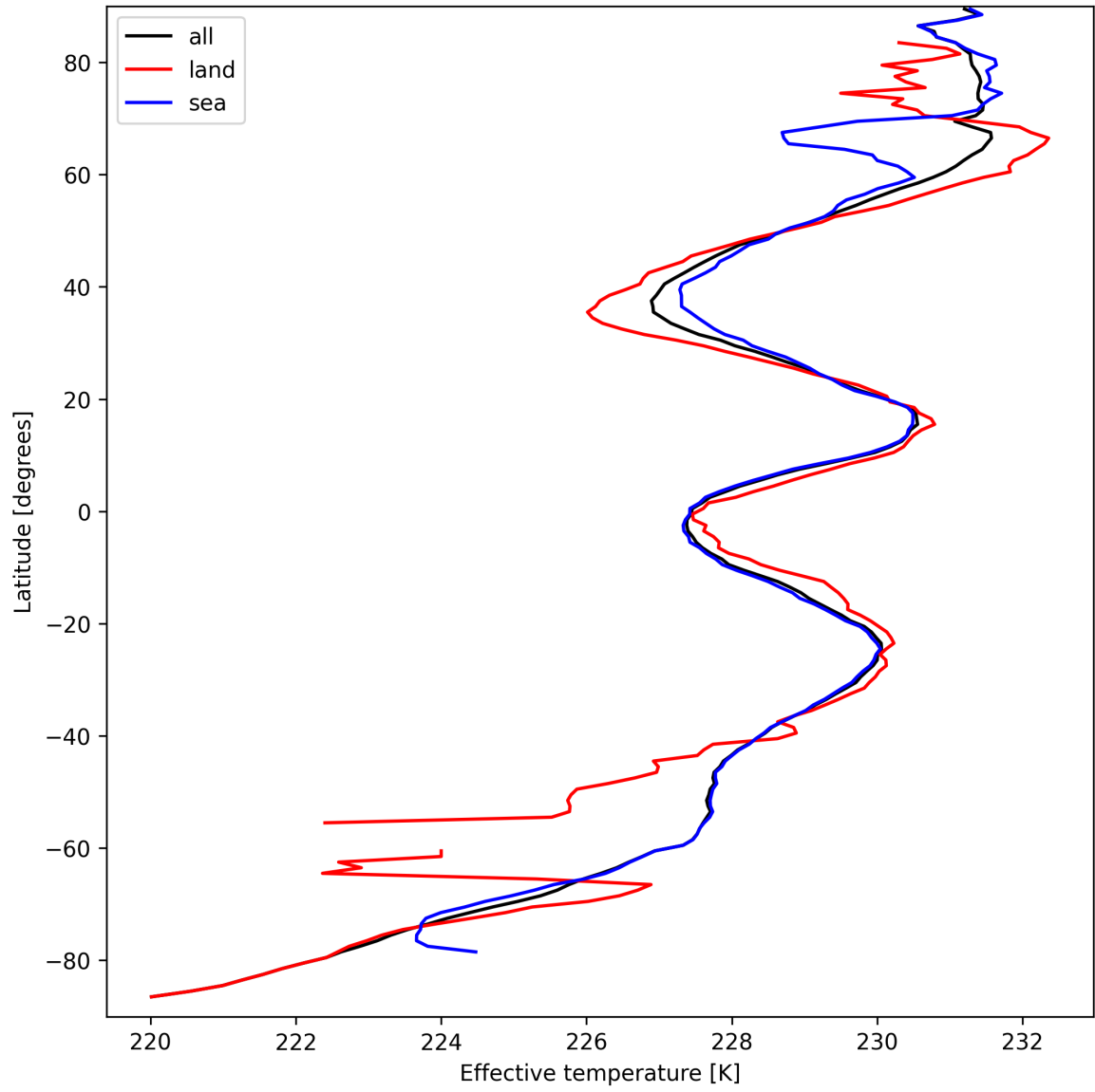
Figure 17: Zonal average of "Effective temperature" for 2025-03-25 to 2025-03-27.
