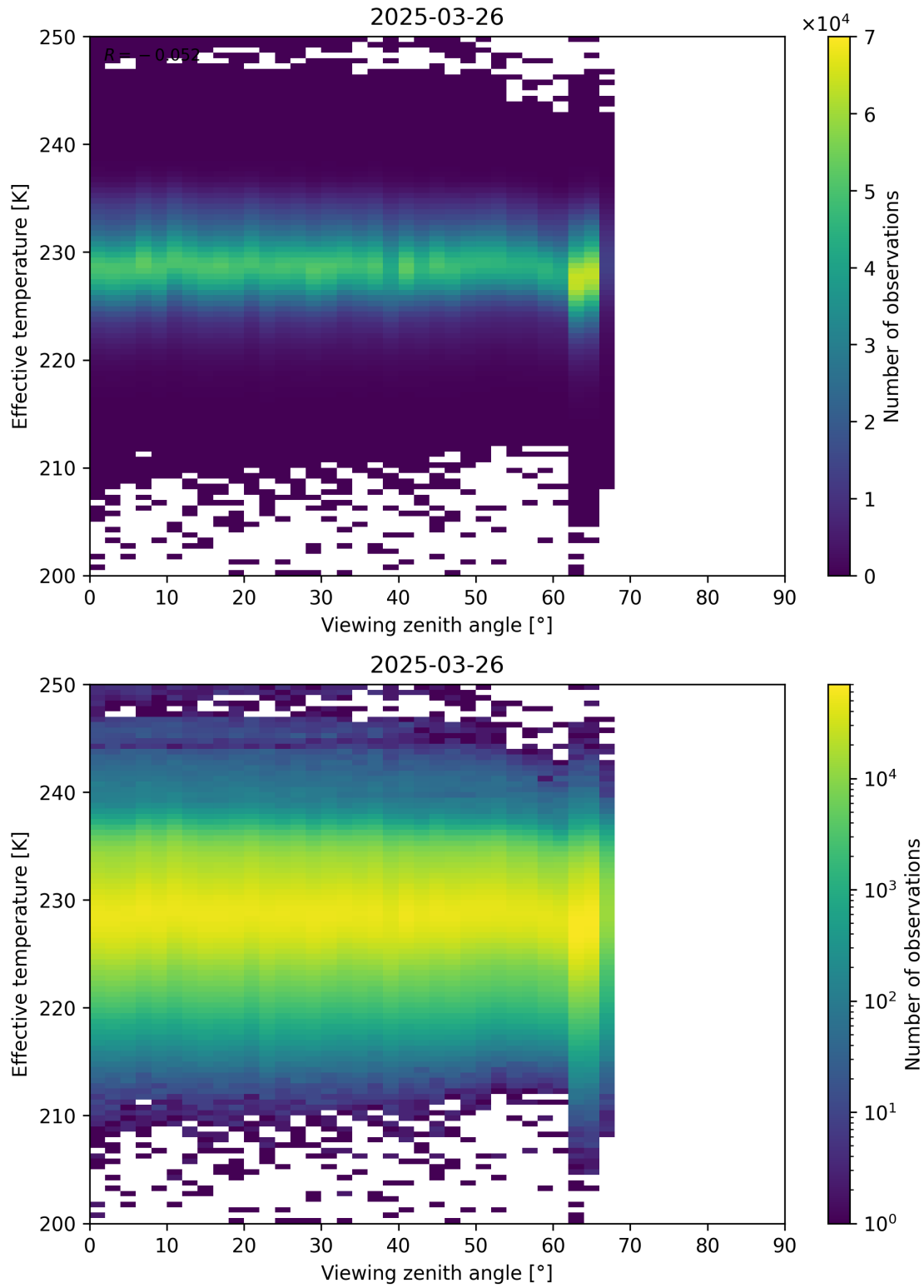
Figure 50: Scatter density plot of “Viewing zenith angle” against “Effective temperature” for 2025-03-25 to 2025-03-27.
