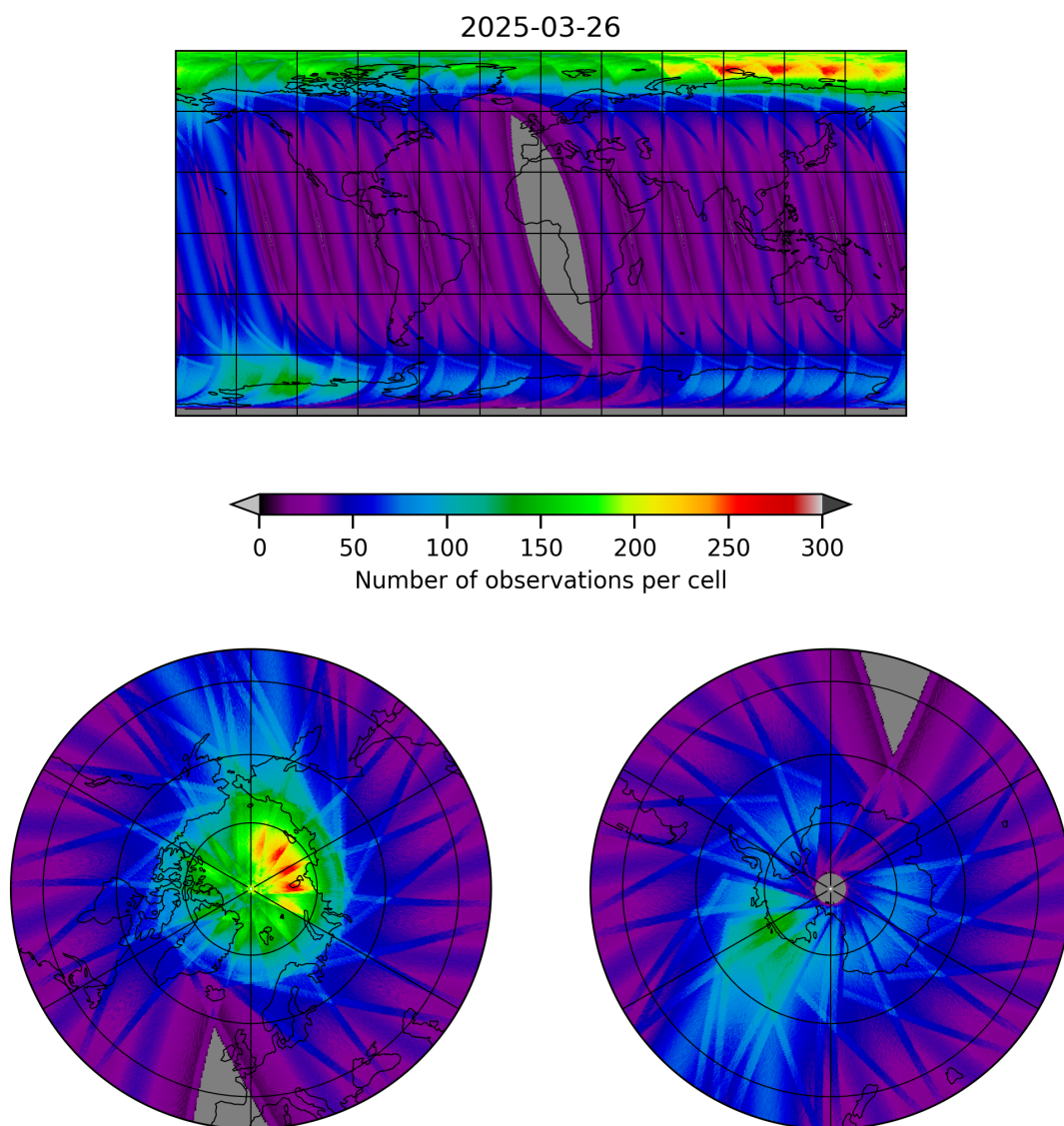
Figure 12: Map of the number of observations for 2025-03-25 to 2025-03-27
