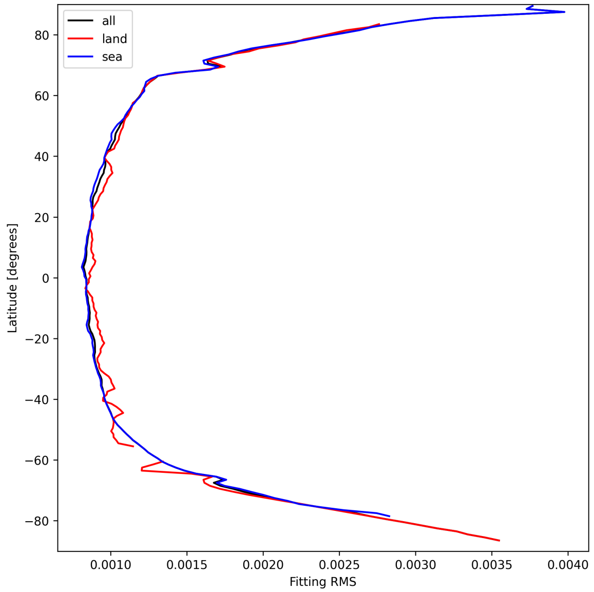
Figure 16: Zonal average of “Fitting RMS” for 2025-03-25 to 2025-03-27.
