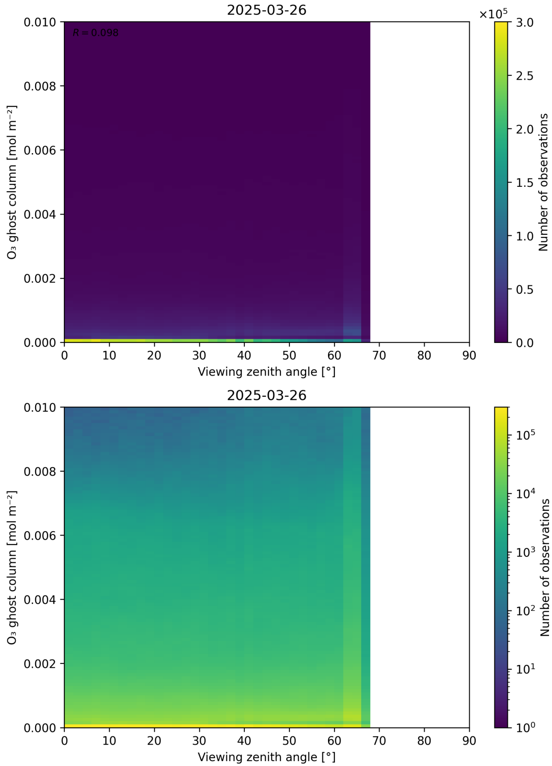
Figure 51: Scatter density plot of “Viewing zenith angle” against “O 3 ghost column” for 2025-03-25 to 2025-03-27.
