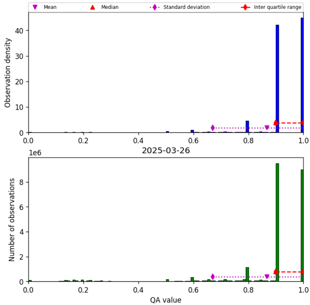
Figure 20: Histogram of “QA value” for 2025-03-25 to 2025-03-27
