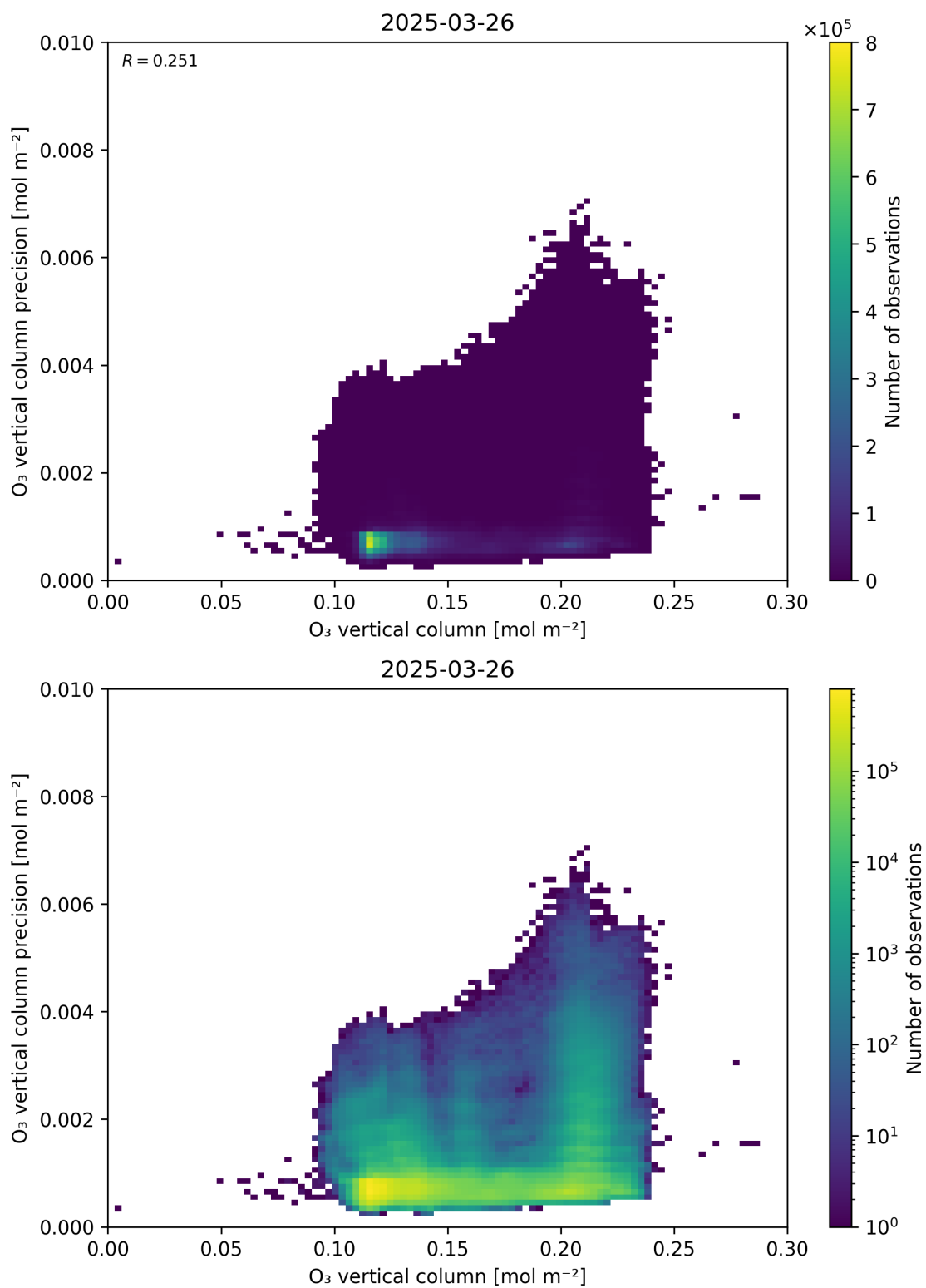
Figure 41: Scatter density plot of “O 3 vertical column” against “O 3 vertical column precision” for 2025-03-25 to 2025-03-27.
