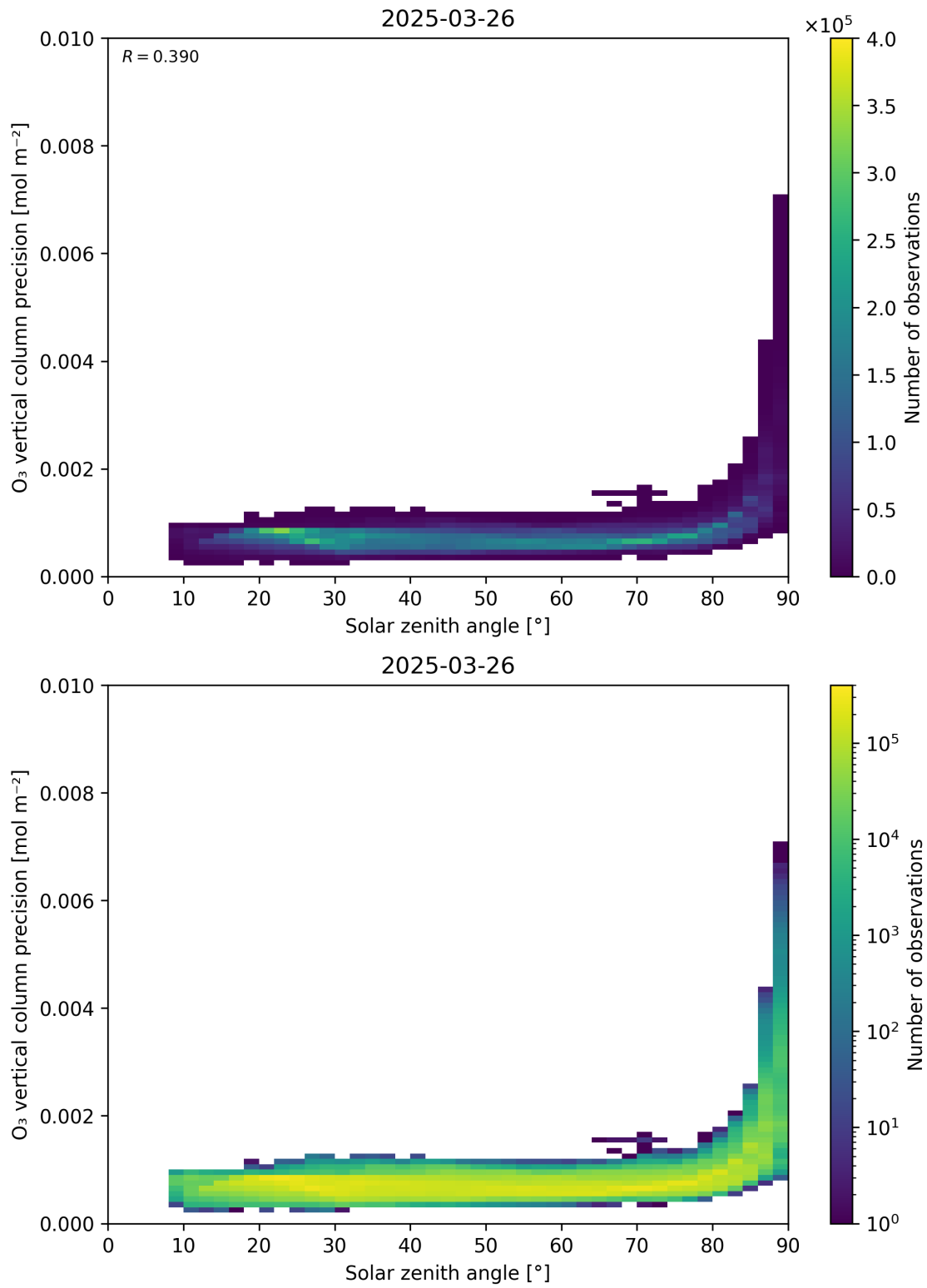
Figure 48: Scatter density plot of “Solar zenith angle” against “O 3 vertical column precision” for 2025-03-25 to 2025-03-27.
