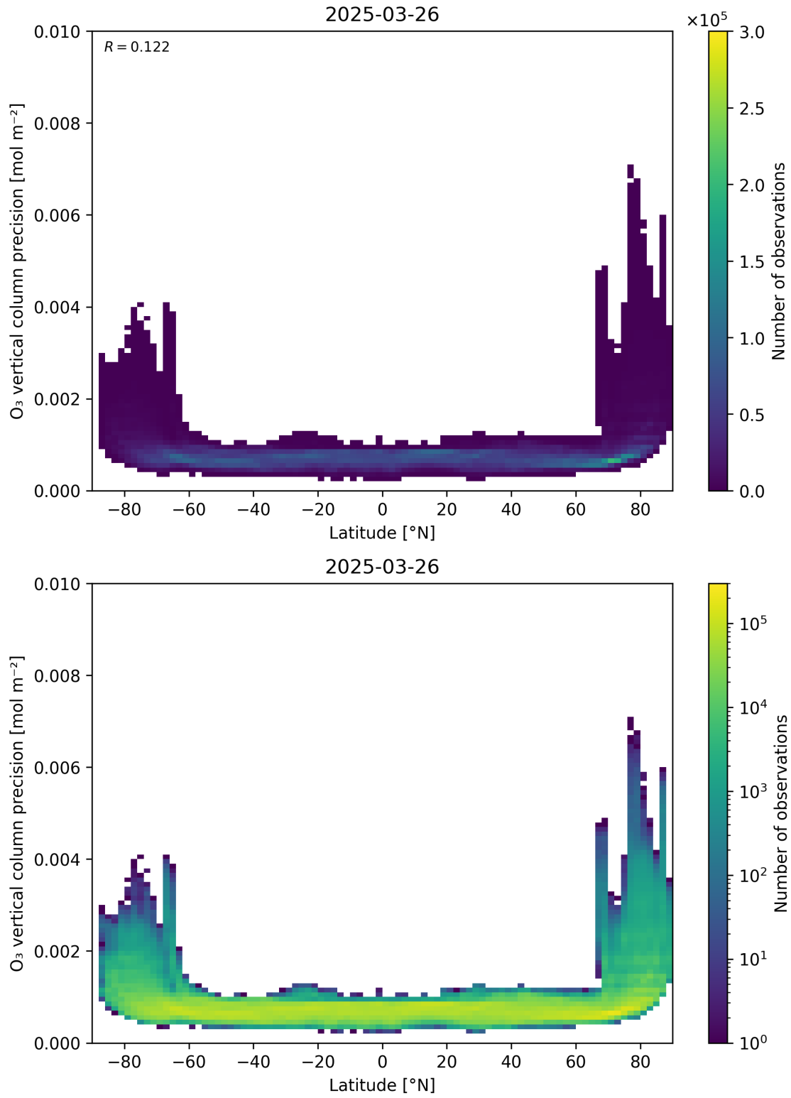
Figure 37: Scatter density plot of “Latitude” against “O 3 vertical column precision” for 2025-03-25 to 2025-03-27.
