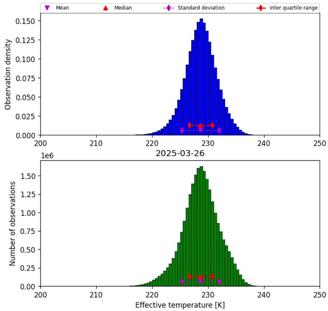
Figure 24: Histogram of “Effective temperature” for 2025-03-25 to 2025-03-27
