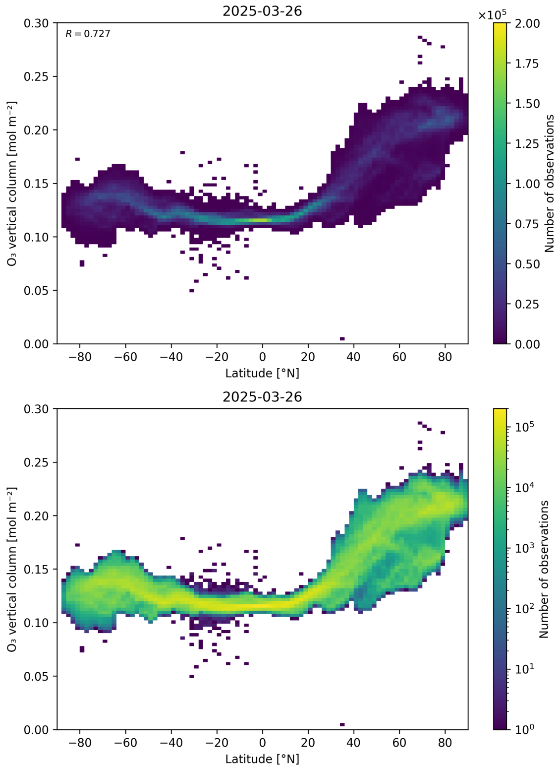
Figure 36: Scatter density plot of “Latitude” against “O 3 vertical column” for 2025-03-25 to 2025-03-27.
