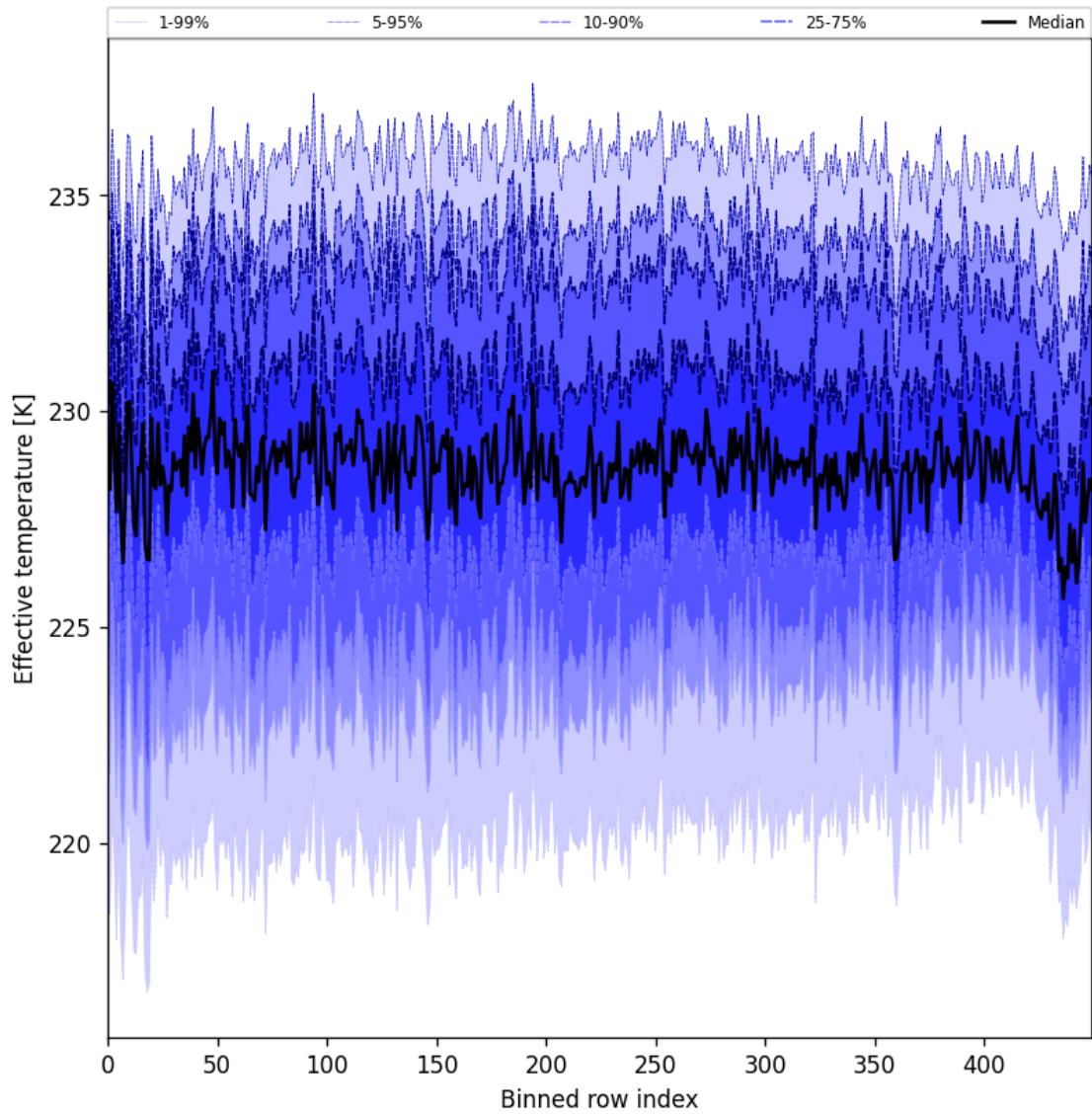
Figure 31: Along track statistics of “Effective temperature” for 2025-03-25 to 2025-03-27
