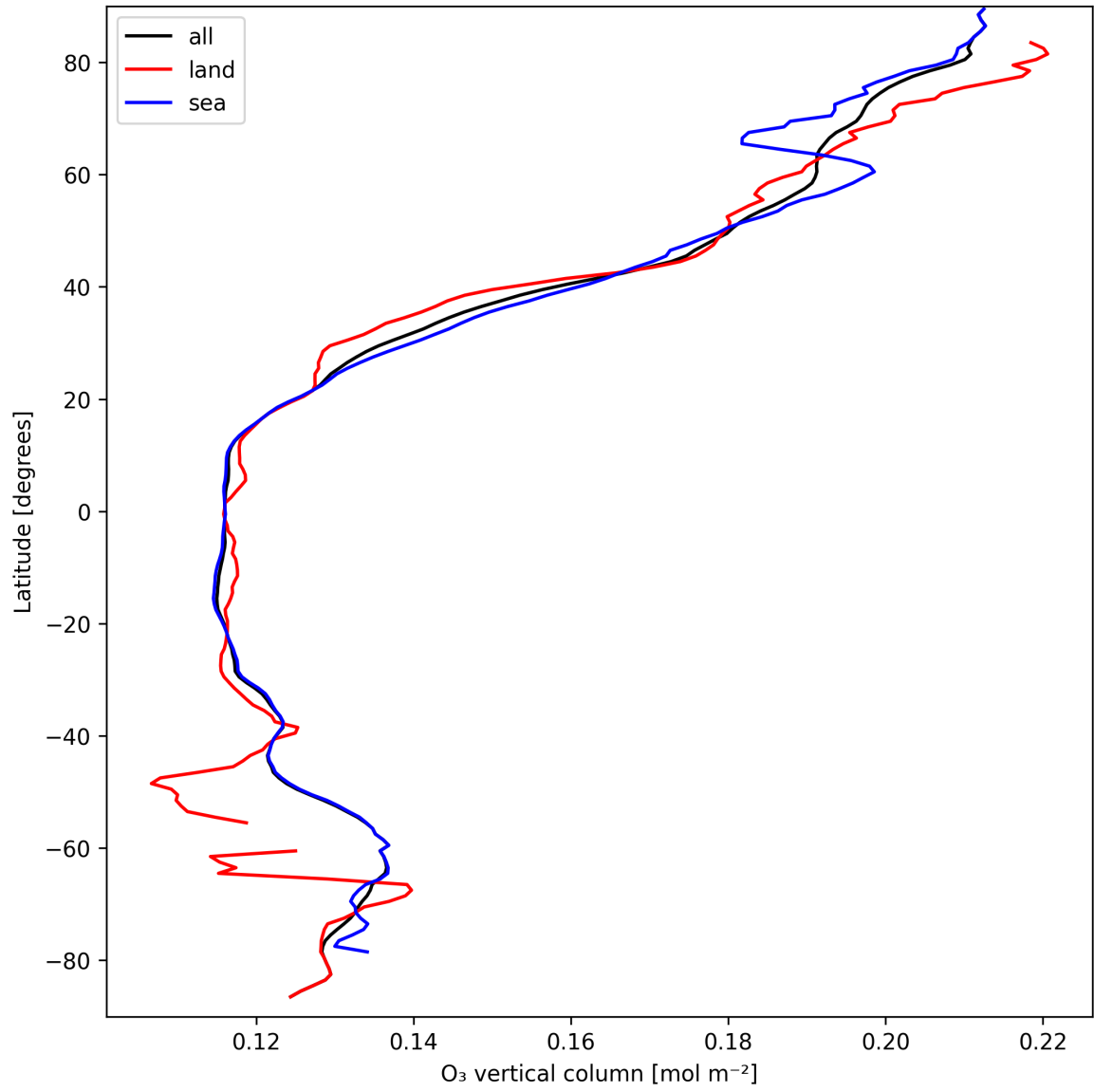
Figure 14: Zonal average of “O 3 vertical column” for 2025-03-25 to 2025-03-27.
