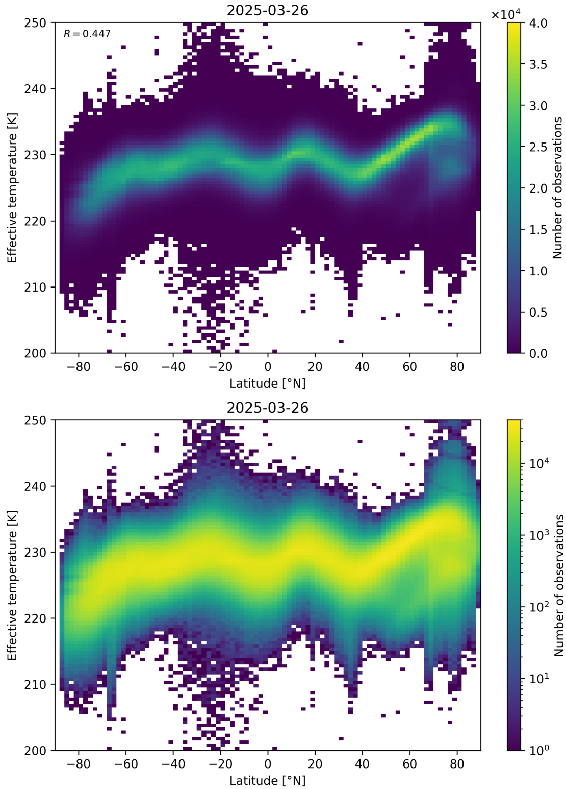
Figure 34: Scatter density plot of “Latitude” against “Effective temperature” for 2025-03-25 to 2025-03-27.
