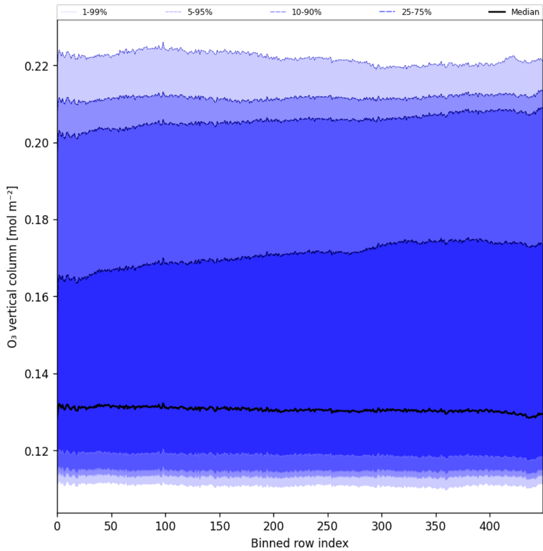
Figure 28: Along track statistics of “O 3 vertical column” for 2025-03-26 to 2025-03-28
