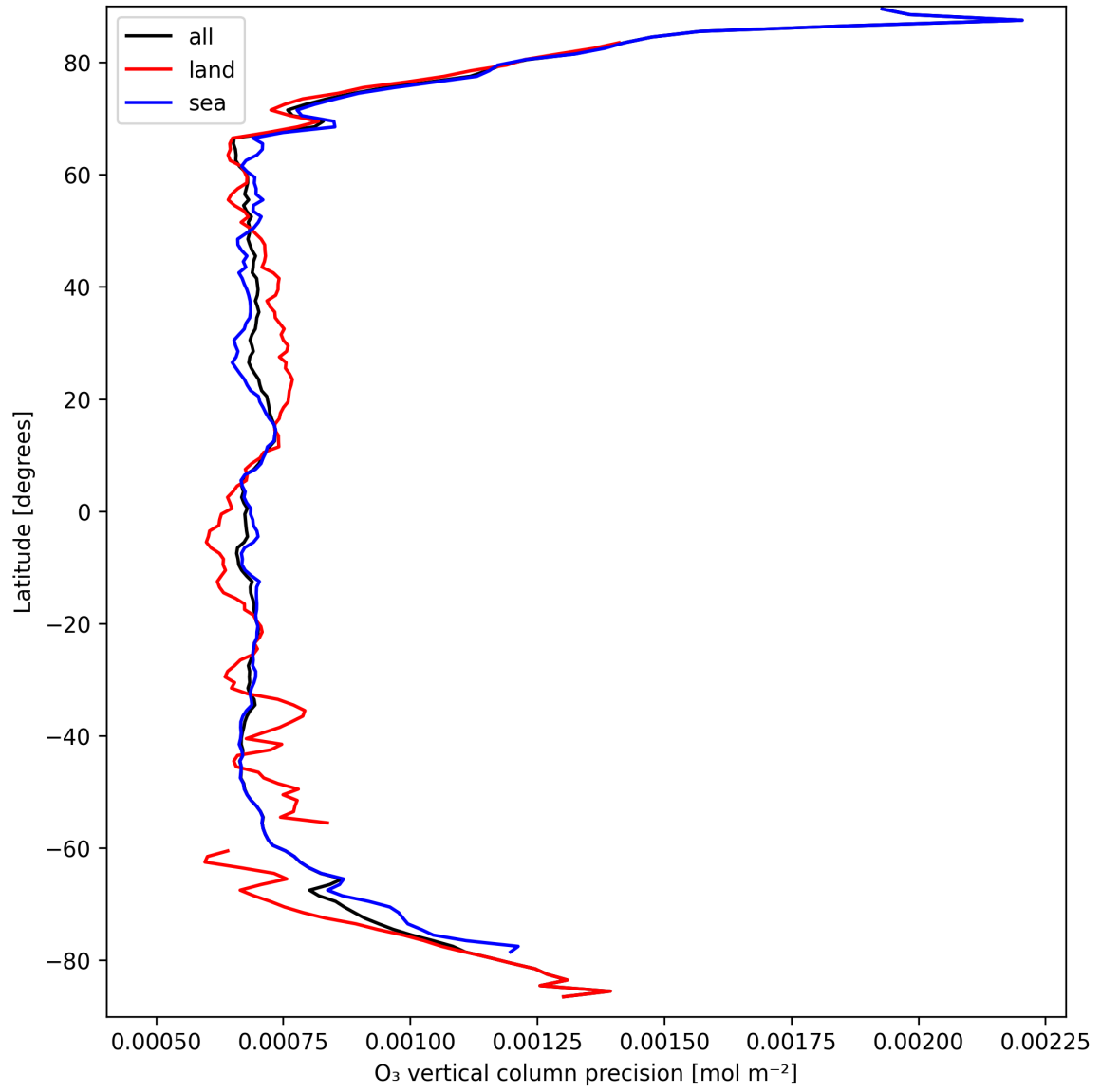
Figure 15: Zonal average of “O 3 vertical column precision” for 2025-03-26 to 2025-03-28.
