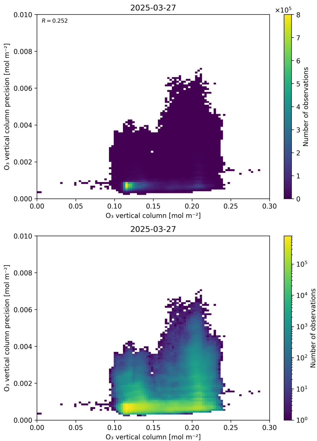
Figure 41: Scatter density plot of “O 3 vertical column” against “O 3 vertical column precision” for 2025-03-26 to 2025-03-28.
