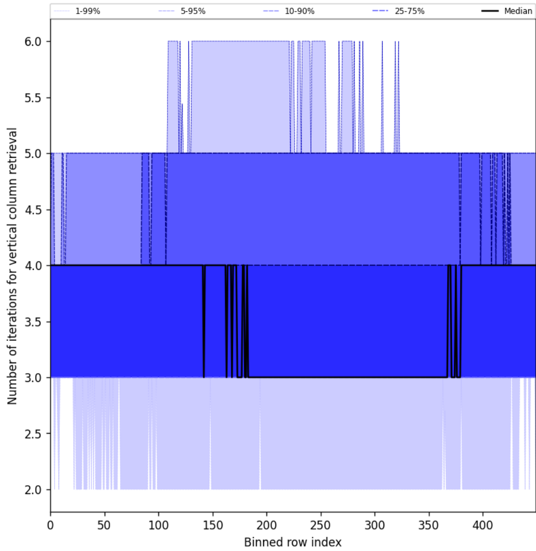
Figure 33: Along track statistics of “Number of iterations for vertical column retrieval” for 2025-03-26 to 2025-03-28
