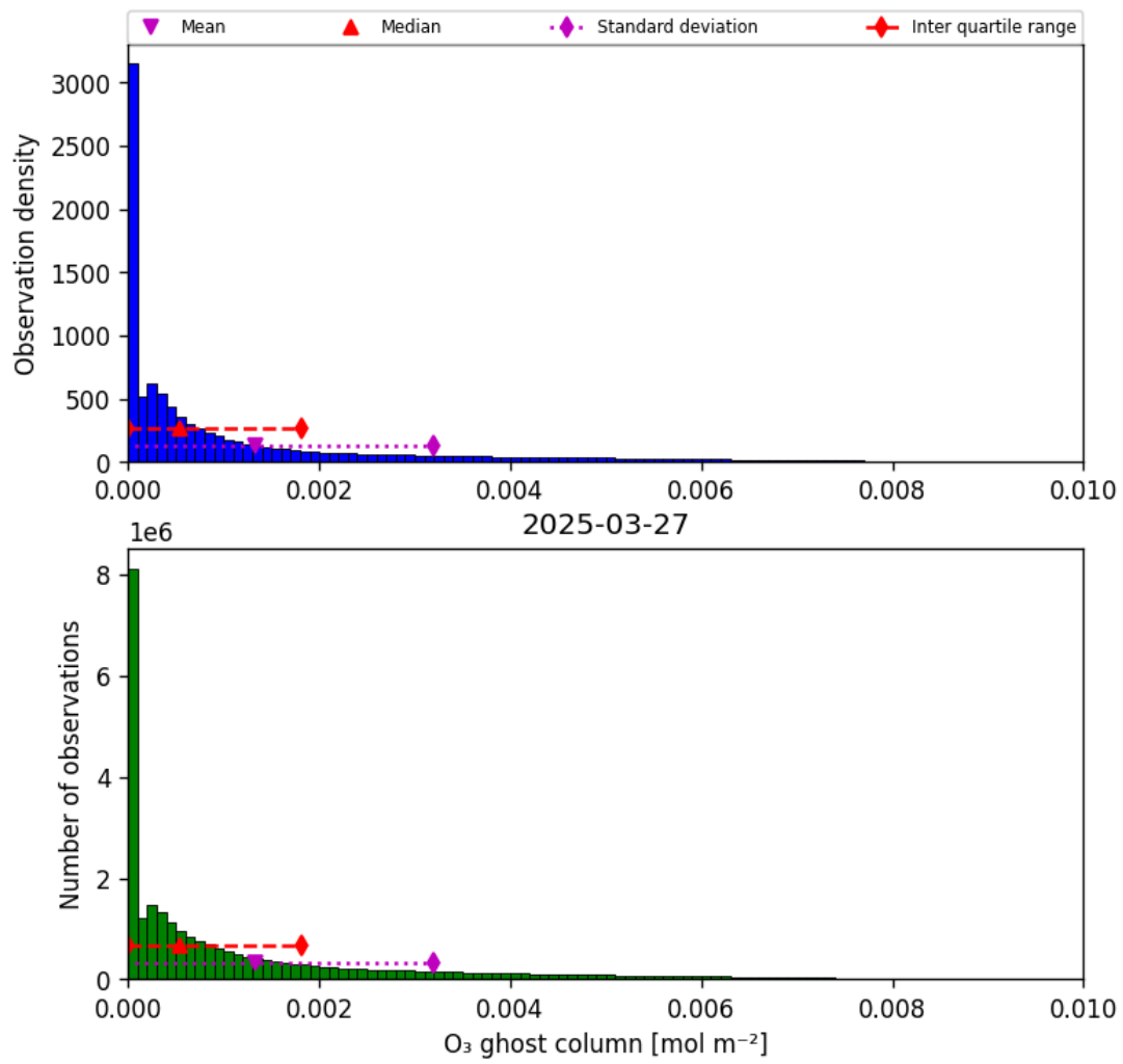
Figure 25: Histogram of “O 3 ghost column” for 2025-03-26 to 2025-03-28
