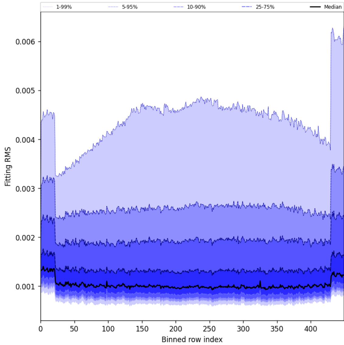
Figure 30: Along track statistics of “Fitting RMS” for 2025-03-26 to 2025-03-28
