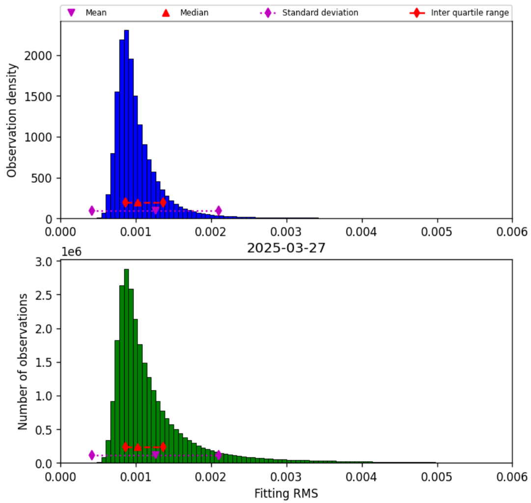
Figure 23: Histogram of “Fitting RMS” for 2025-03-26 to 2025-03-28
