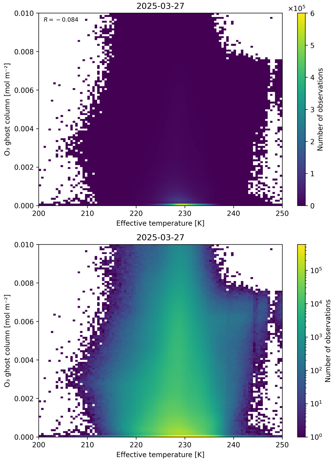
Figure 38: Scatter density plot of “Effective temperature” against “O 3 ghost column” for 2025-03-26 to 2025-03-28.
