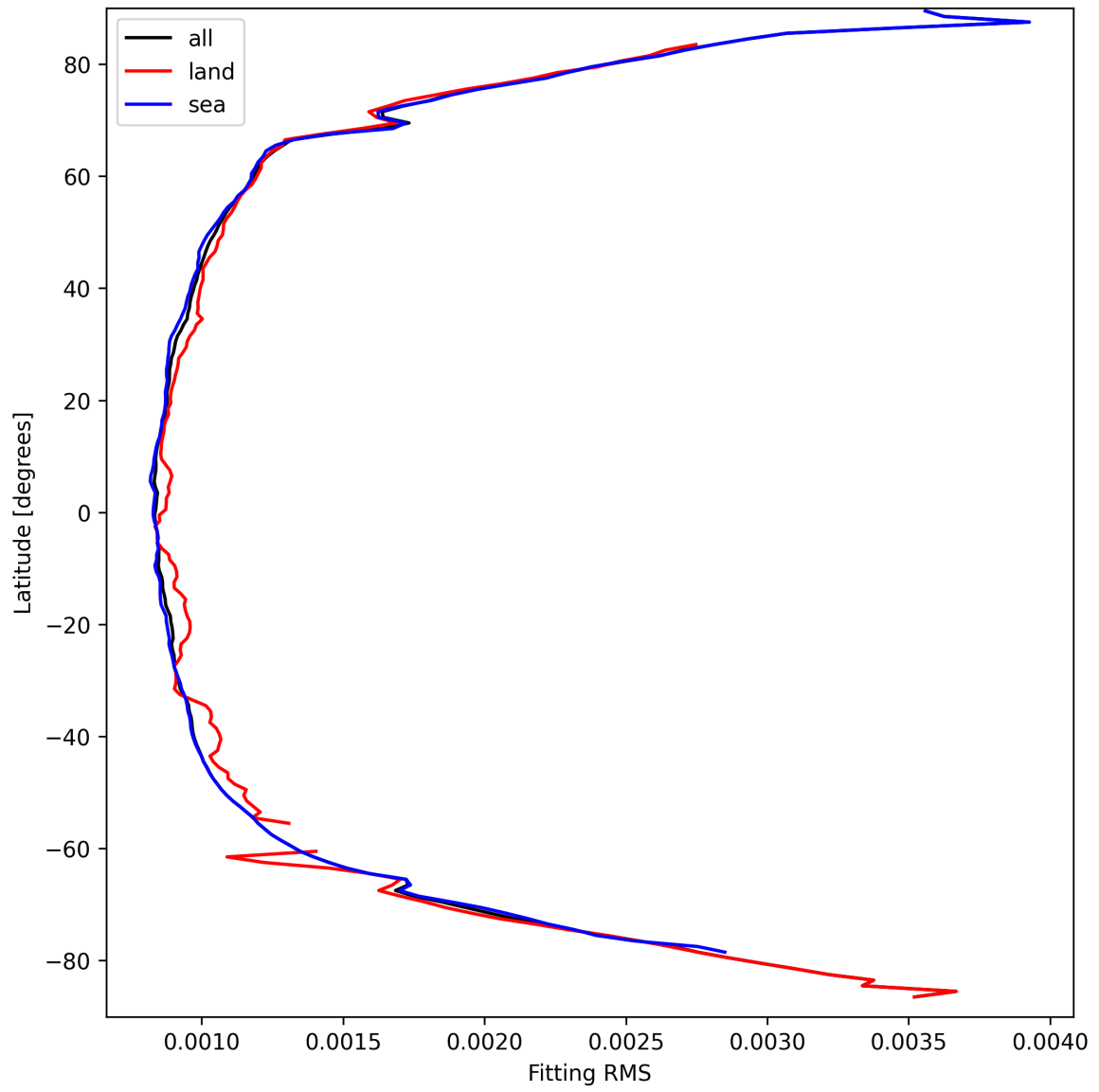
Figure 16: Zonal average of “Fitting RMS” for 2025-03-26 to 2025-03-28.
