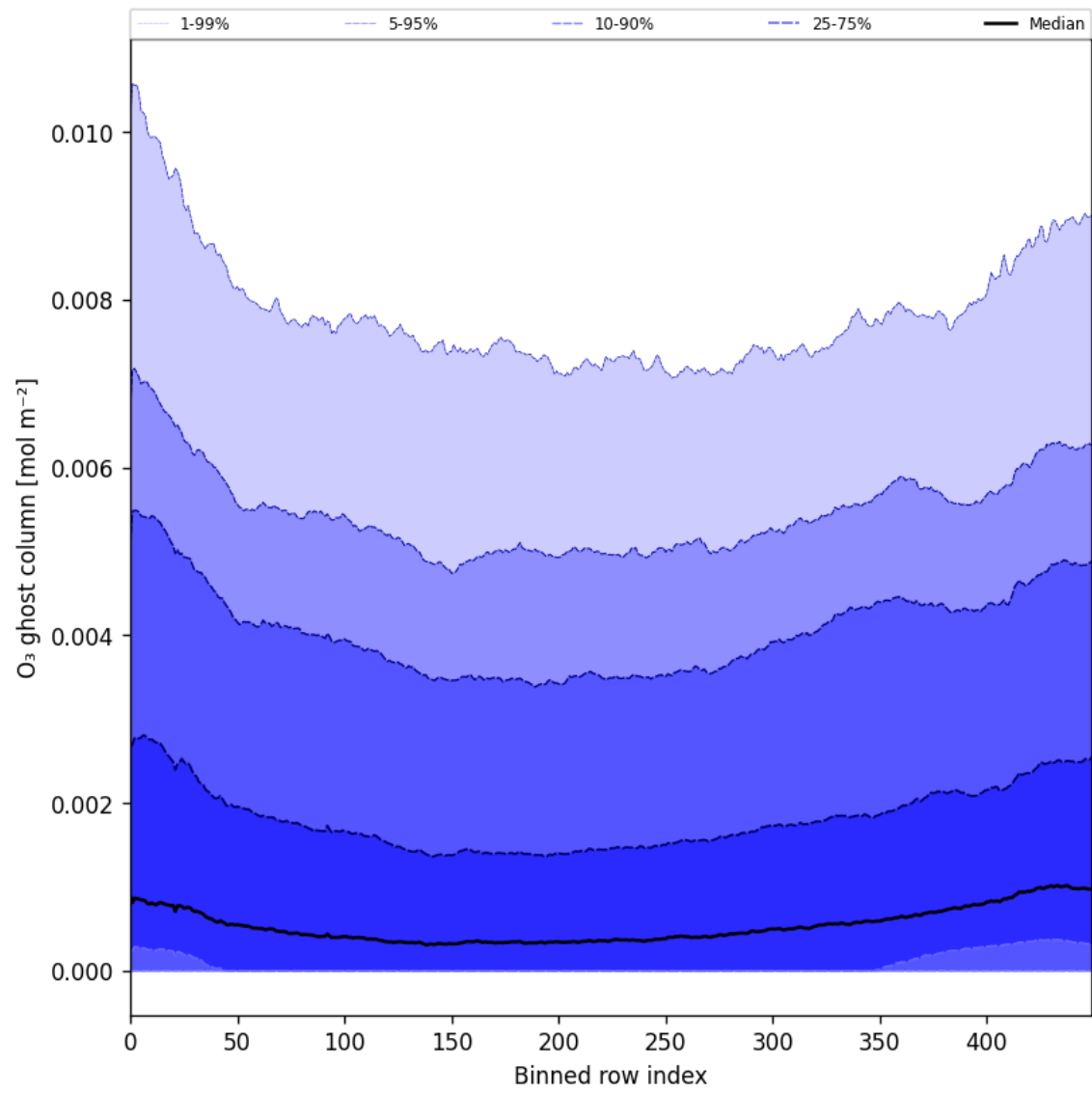
Figure 32: Along track statistics of “O 3 ghost column” for 2025-03-26 to 2025-03-28
