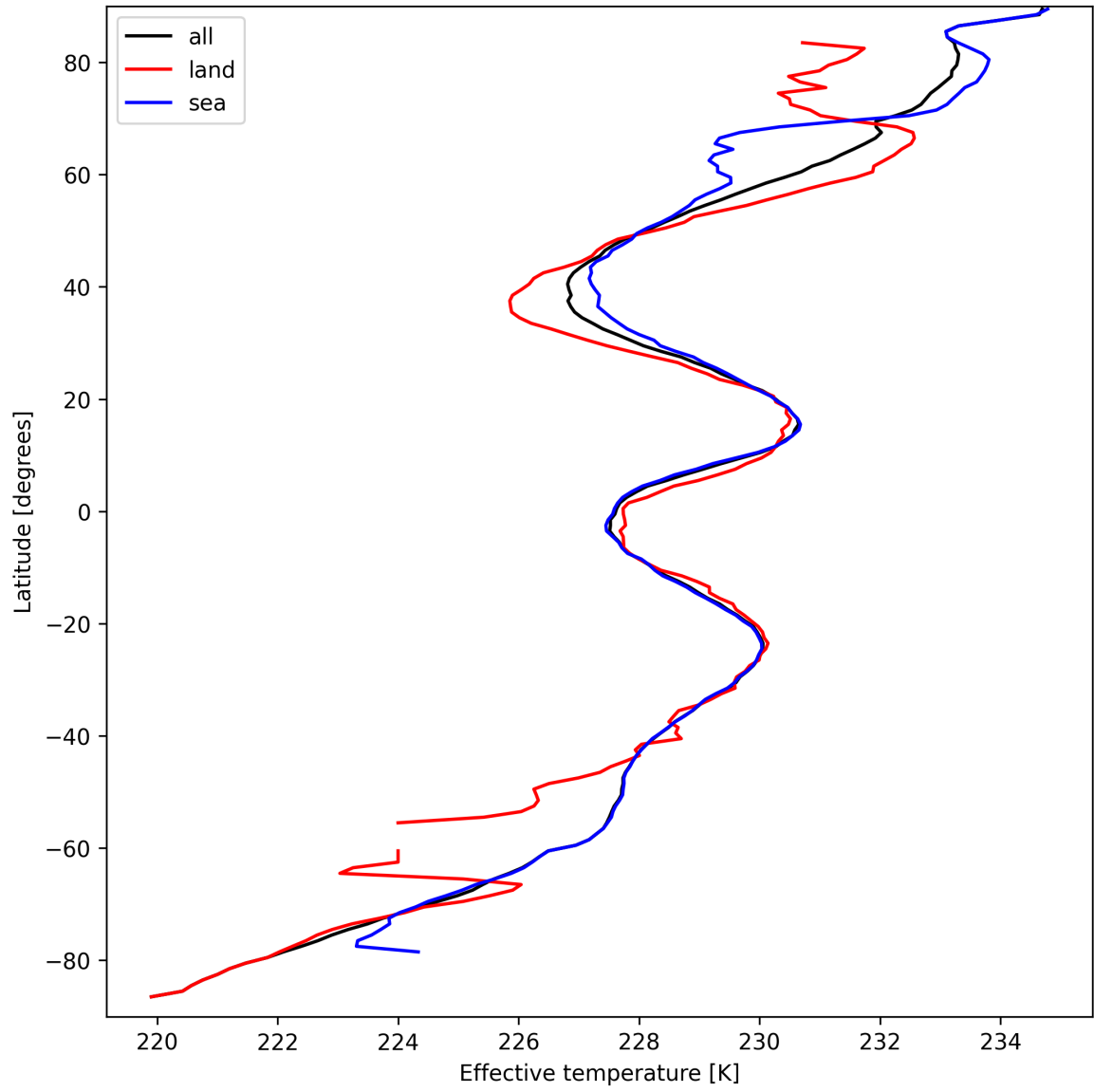
Figure 17: Zonal average of “Effective temperature” for 2025-03-26 to 2025-03-28.
