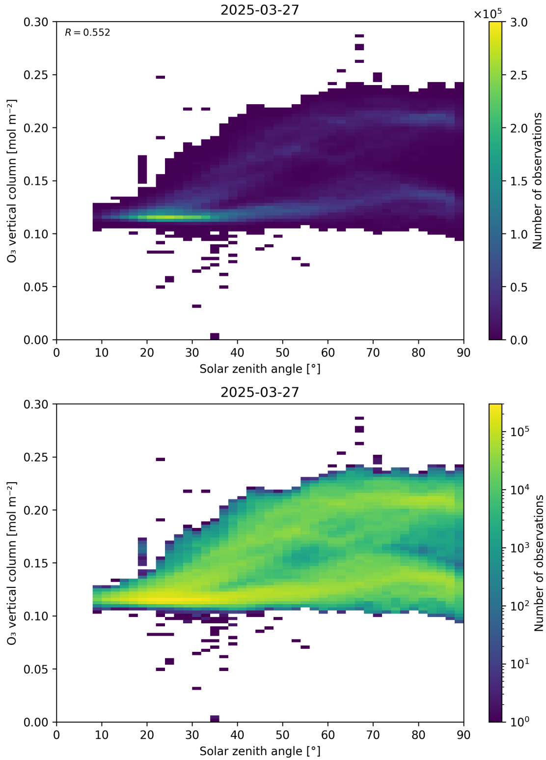
Figure 47: Scatter density plot of “Solar zenith angle” against “O 3 vertical column” for 2025-03-26 to 2025-03-28.
