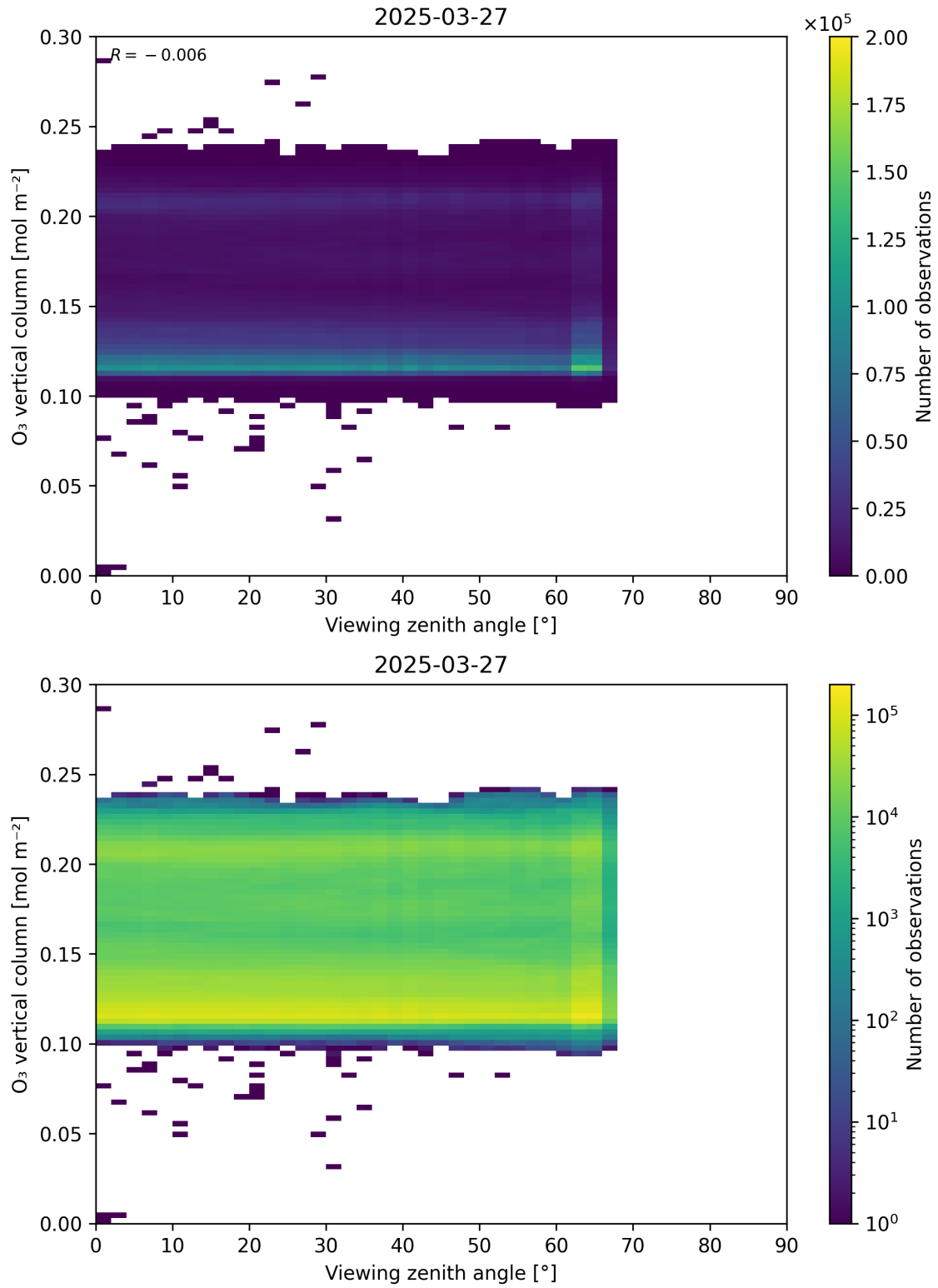
Figure 52: Scatter density plot of “Viewing zenith angle” against “O 3 vertical column” for 2025-03-26 to 2025-03-28.
