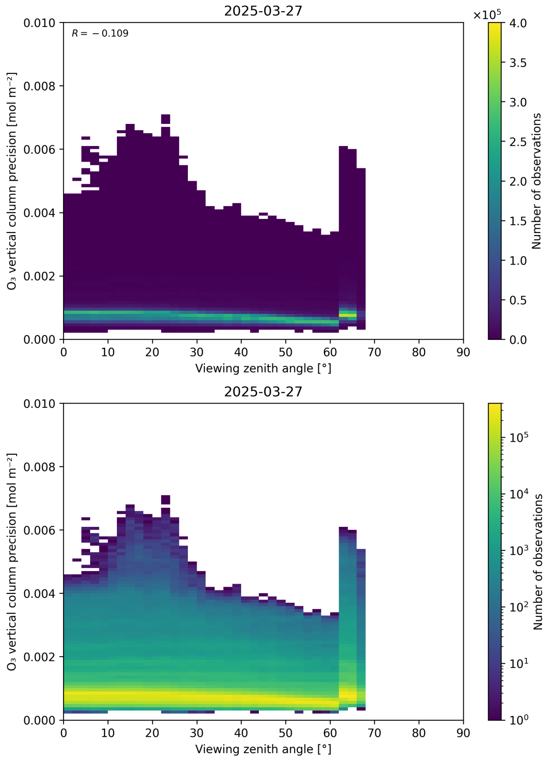
Figure 53: Scatter density plot of “Viewing zenith angle” against “O 3 vertical column precision” for 2025-03-26 to 2025-03-28.
