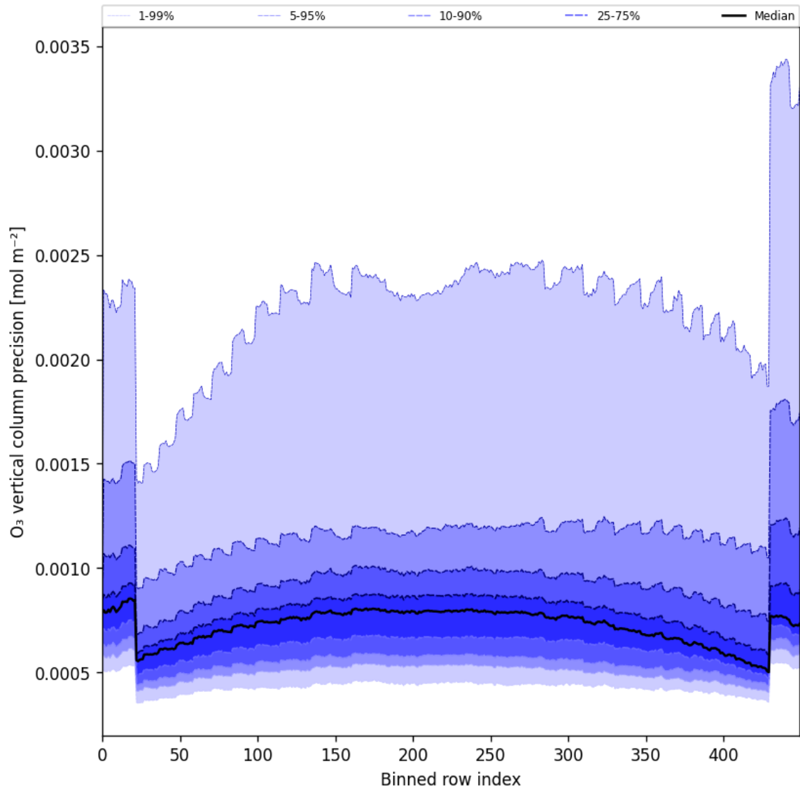
Figure 29: Along track statistics of “O 3 vertical column precision” for 2025-03-26 to 2025-03-28
