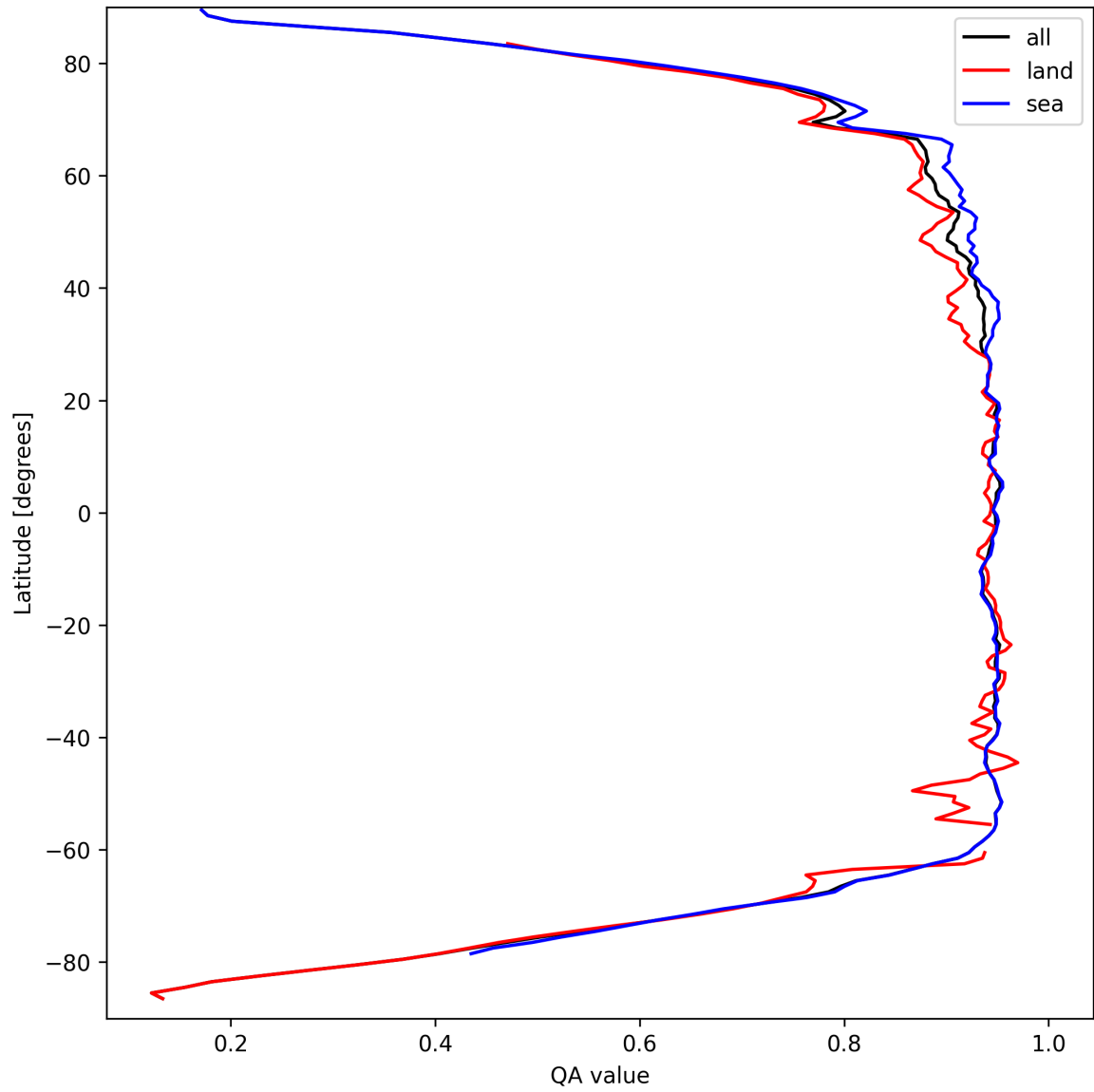
Figure 13: Zonal average of “QA value” for 2025-03-26 to 2025-03-28.
