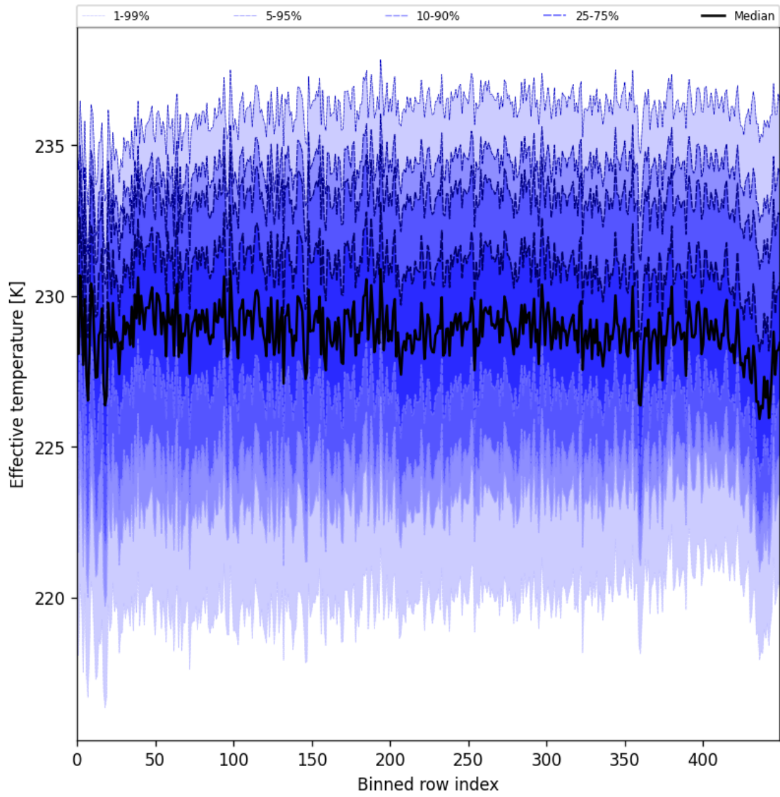
Figure 31: Along track statistics of “Effective temperature” for 2025-03-26 to 2025-03-28
