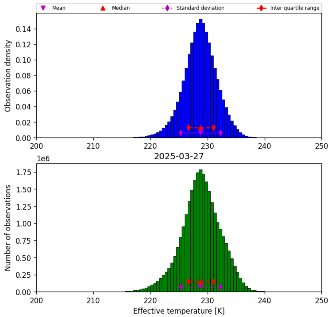
Figure 24: Histogram of “Effective temperature” for 2025-03-26 to 2025-03-28
