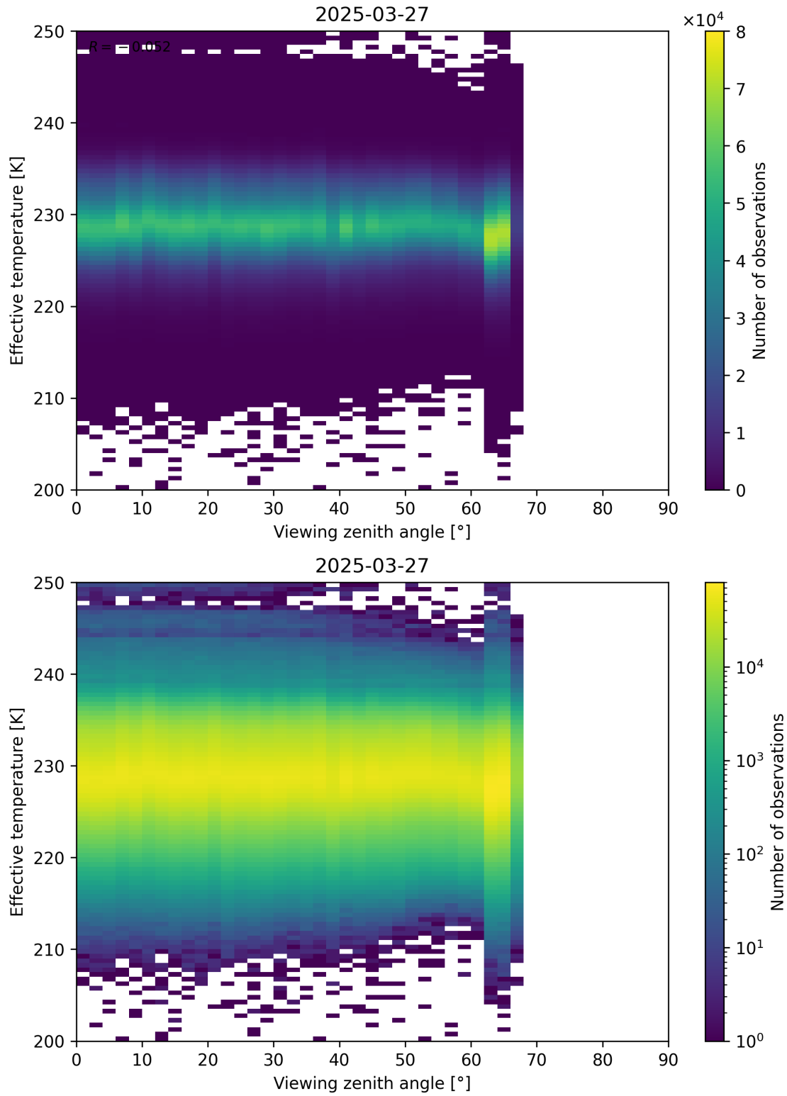
Figure 50: Scatter density plot of “Viewing zenith angle” against “Effective temperature” for 2025-03-26 to 2025-03-28.
