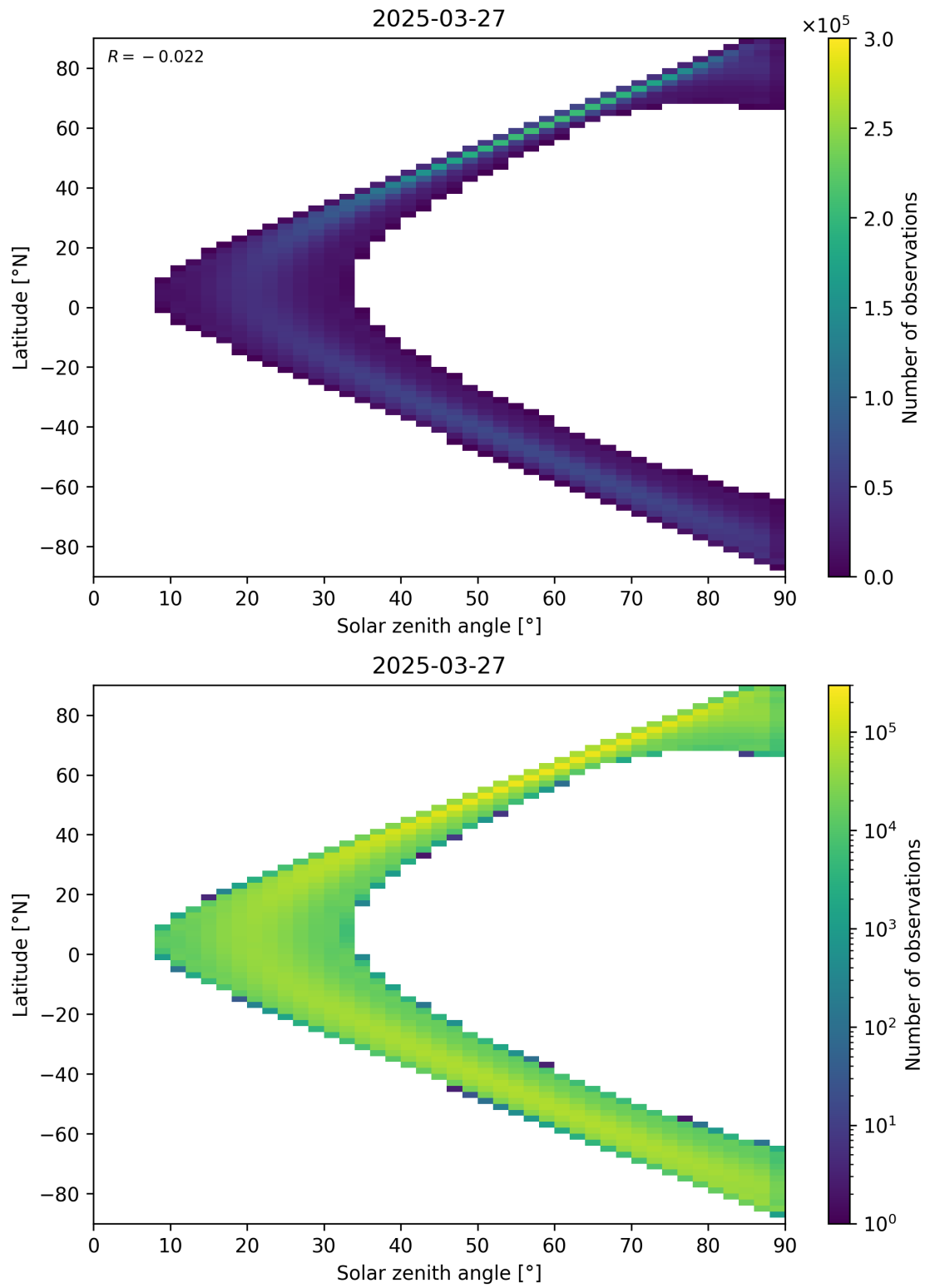
Figure 44: Scatter density plot of “Solar zenith angle” against “Latitude” for 2025-03-26 to 2025-03-28.
