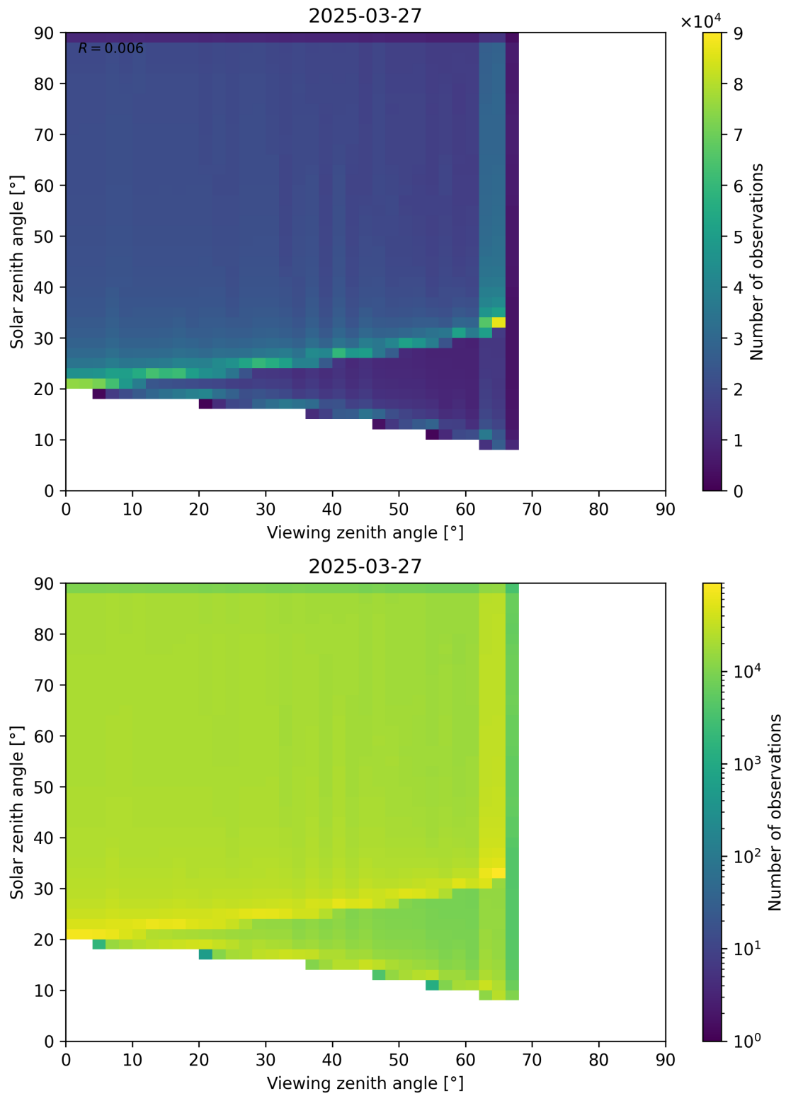
Figure 54: Scatter density plot of “Viewing zenith angle” against “Solar zenith angle” for 2025-03-26 to 2025-03-28.
