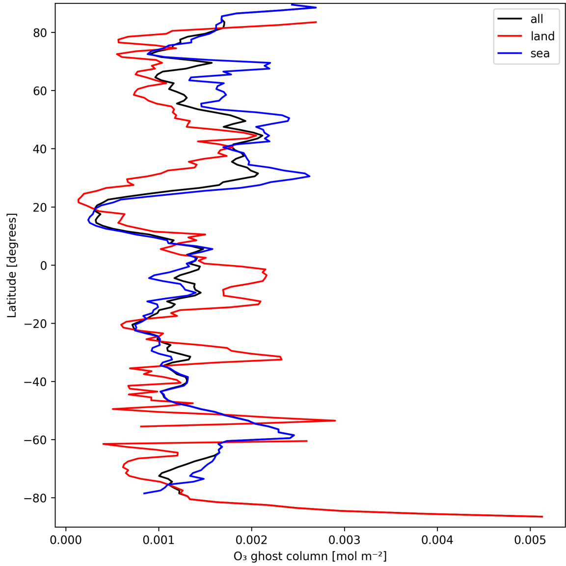
Figure 18: Zonal average of “O 3 ghost column” for 2025-03-26 to 2025-03-28.
