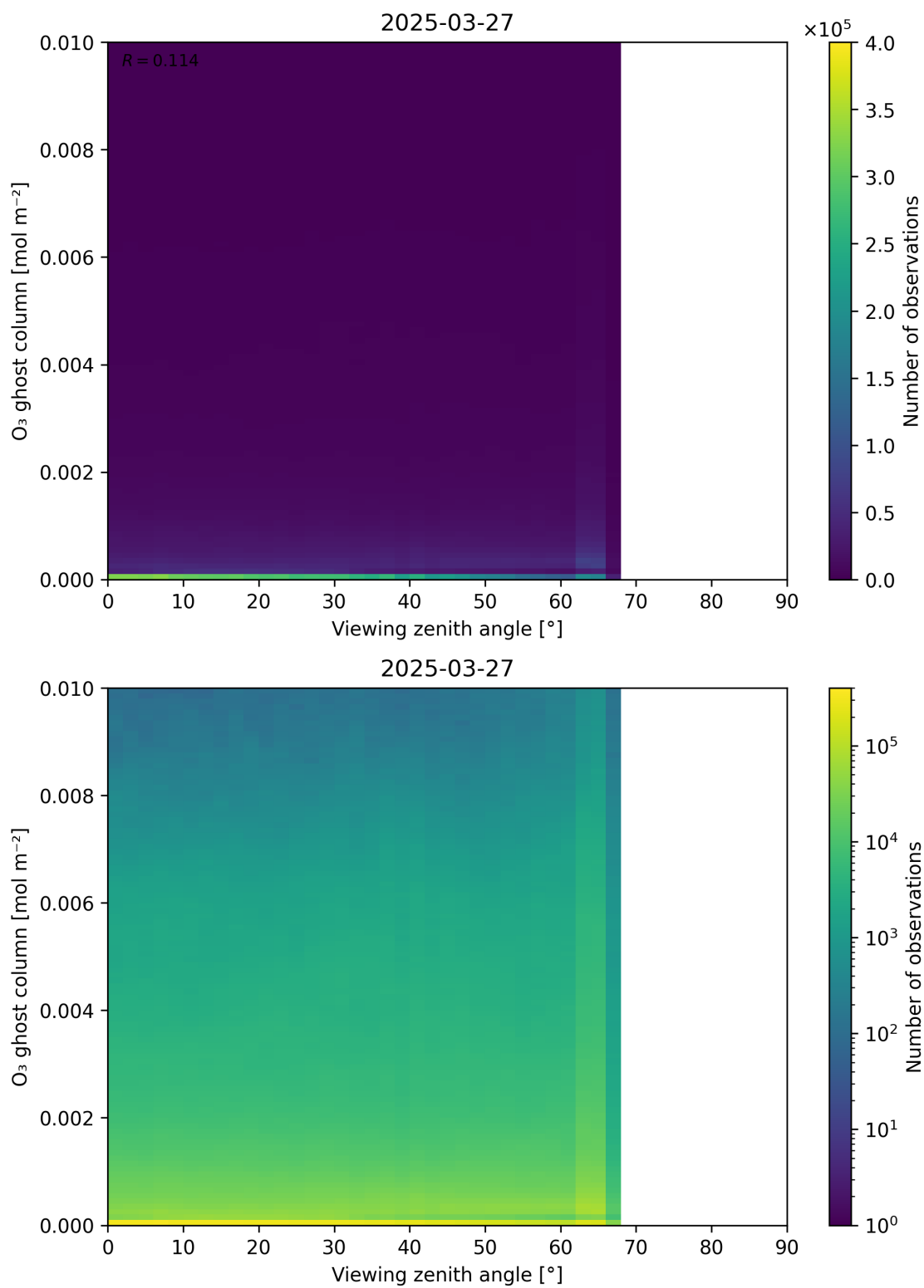
Figure 51: Scatter density plot of “Viewing zenith angle” against “O 3 ghost column” for 2025-03-26 to 2025-03-28.
