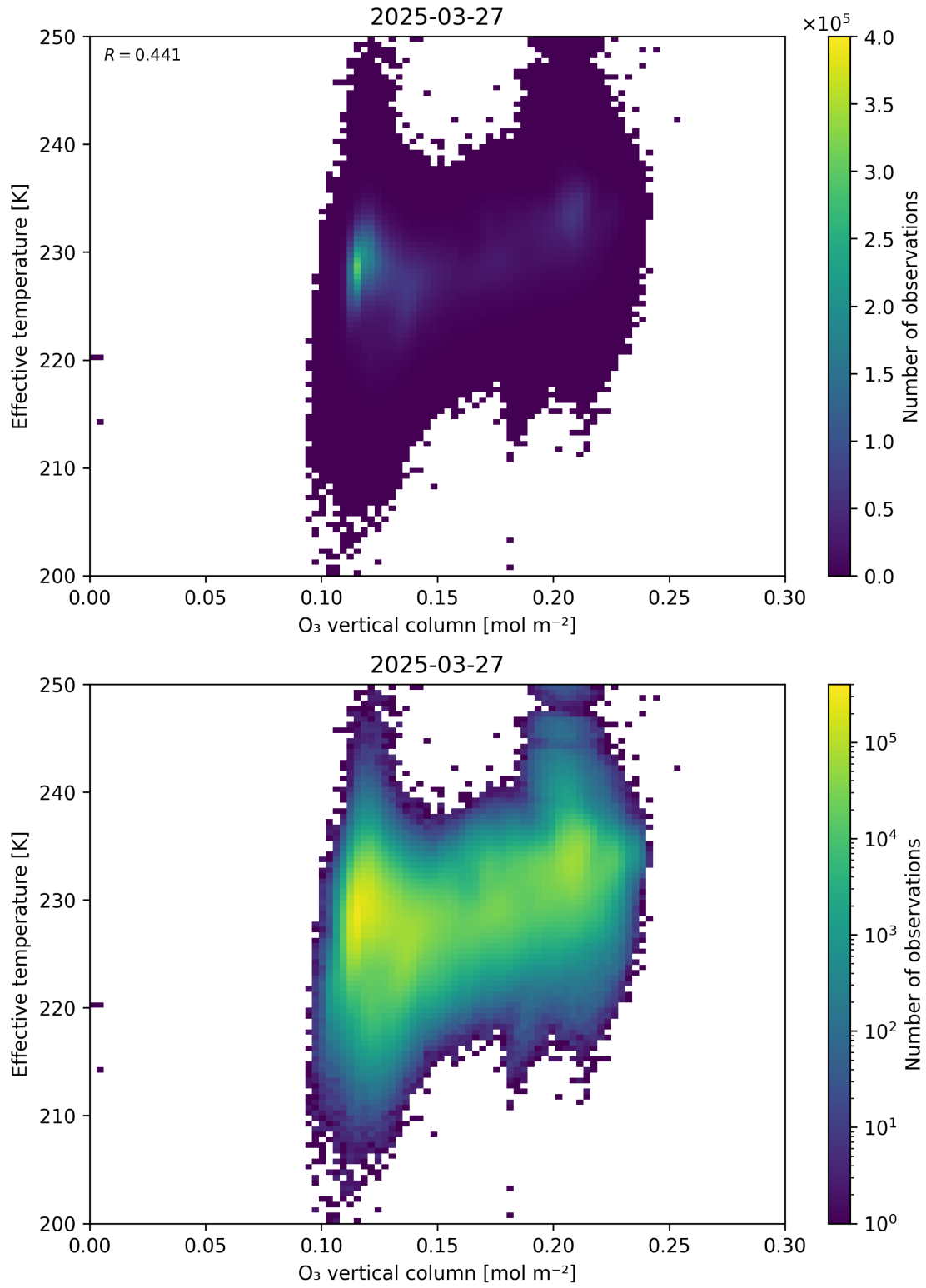
Figure 39: Scatter density plot of “O 3 vertical column” against “Effective temperature” for 2025-03-26 to 2025-03-28.
