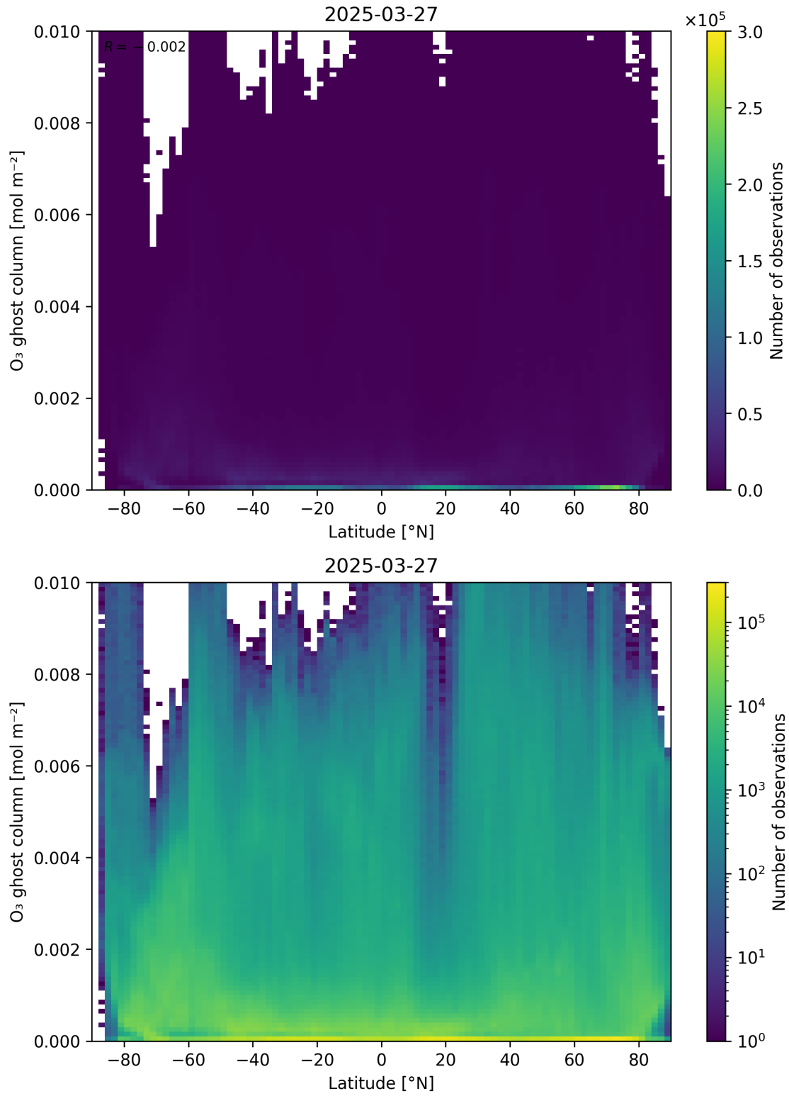
Figure 35: Scatter density plot of “Latitude” against “O 3 ghost column” for 2025-03-26 to 2025-03-28.
