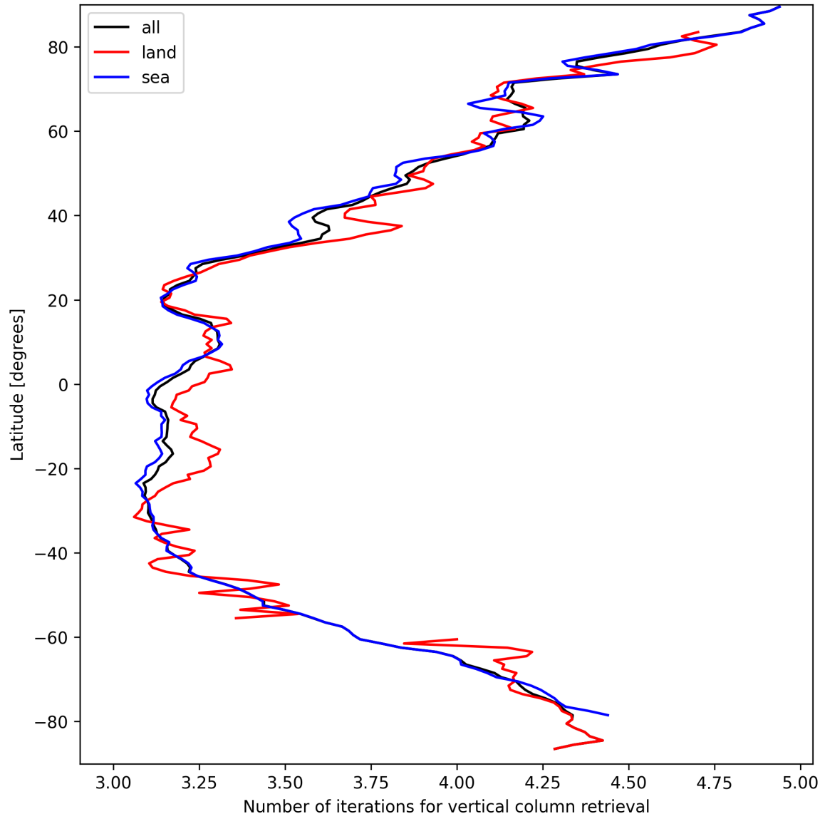
Figure 19: Zonal average of “Number of iterations for vertical column retrieval” for 2025-03-26 to 2025-03-28.
