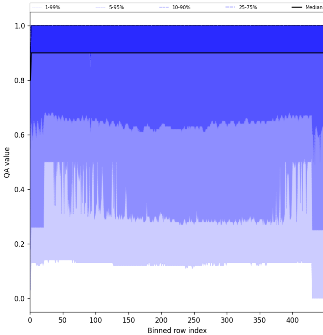
Figure 27: Along track statistics of “QA value” for 2025-03-26 to 2025-03-28
