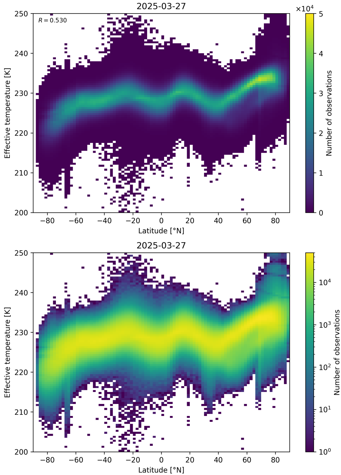
Figure 34: Scatter density plot of “Latitude” against “Effective temperature” for 2025-03-26 to 2025-03-28.
