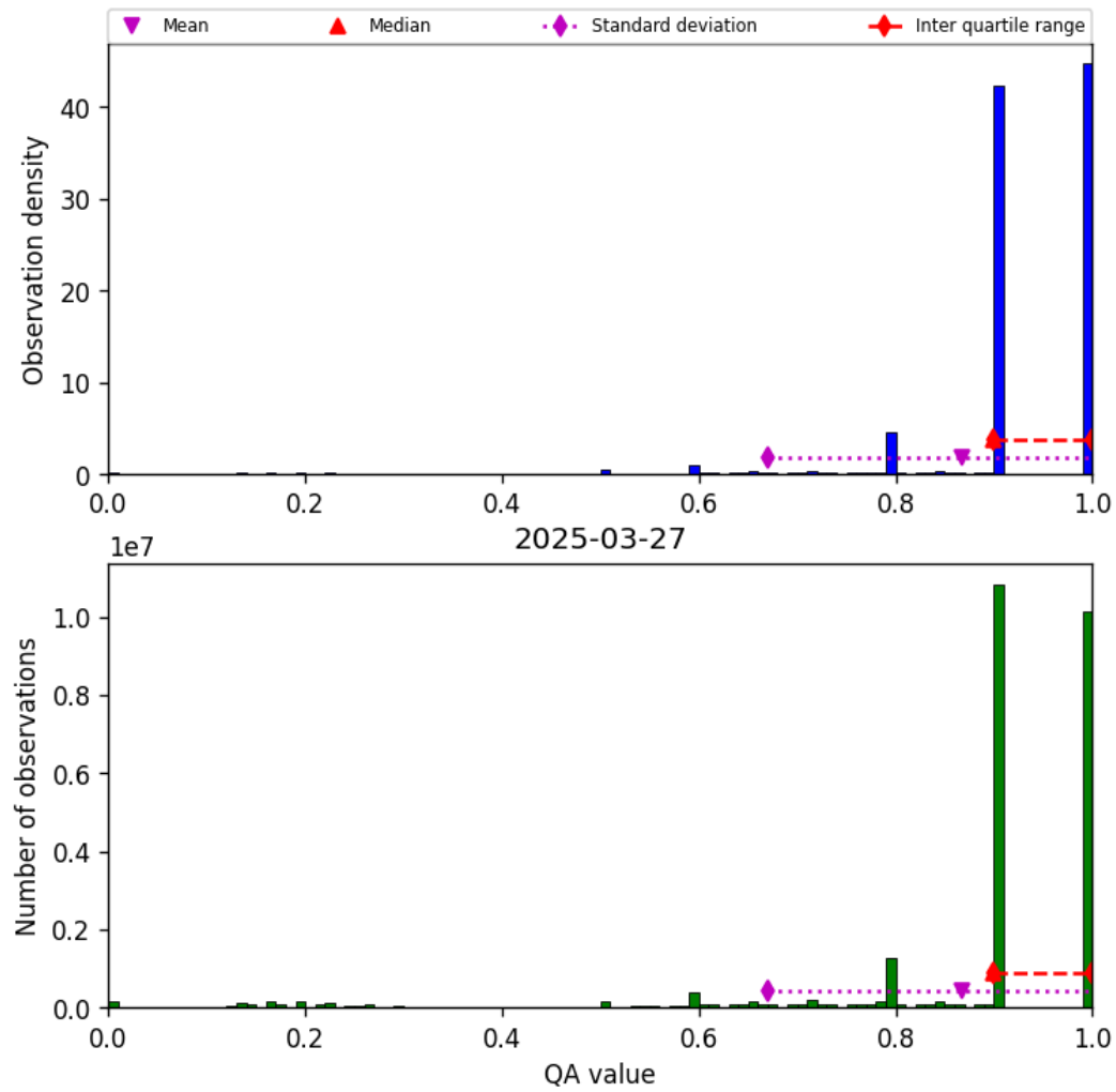
Figure 20: Histogram of “QA value” for 2025-03-26 to 2025-03-28
