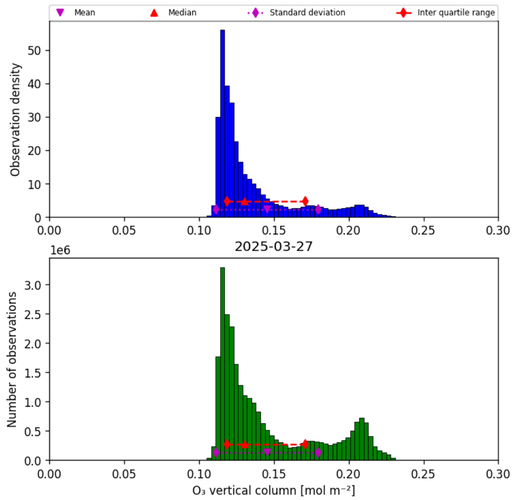
Figure 21: Histogram of “O 3 vertical column” for 2025-03-26 to 2025-03-28
