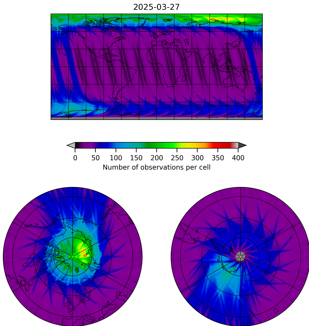
Figure 12: Map of the number of observations for 2025-03-26 to 2025-03-28
