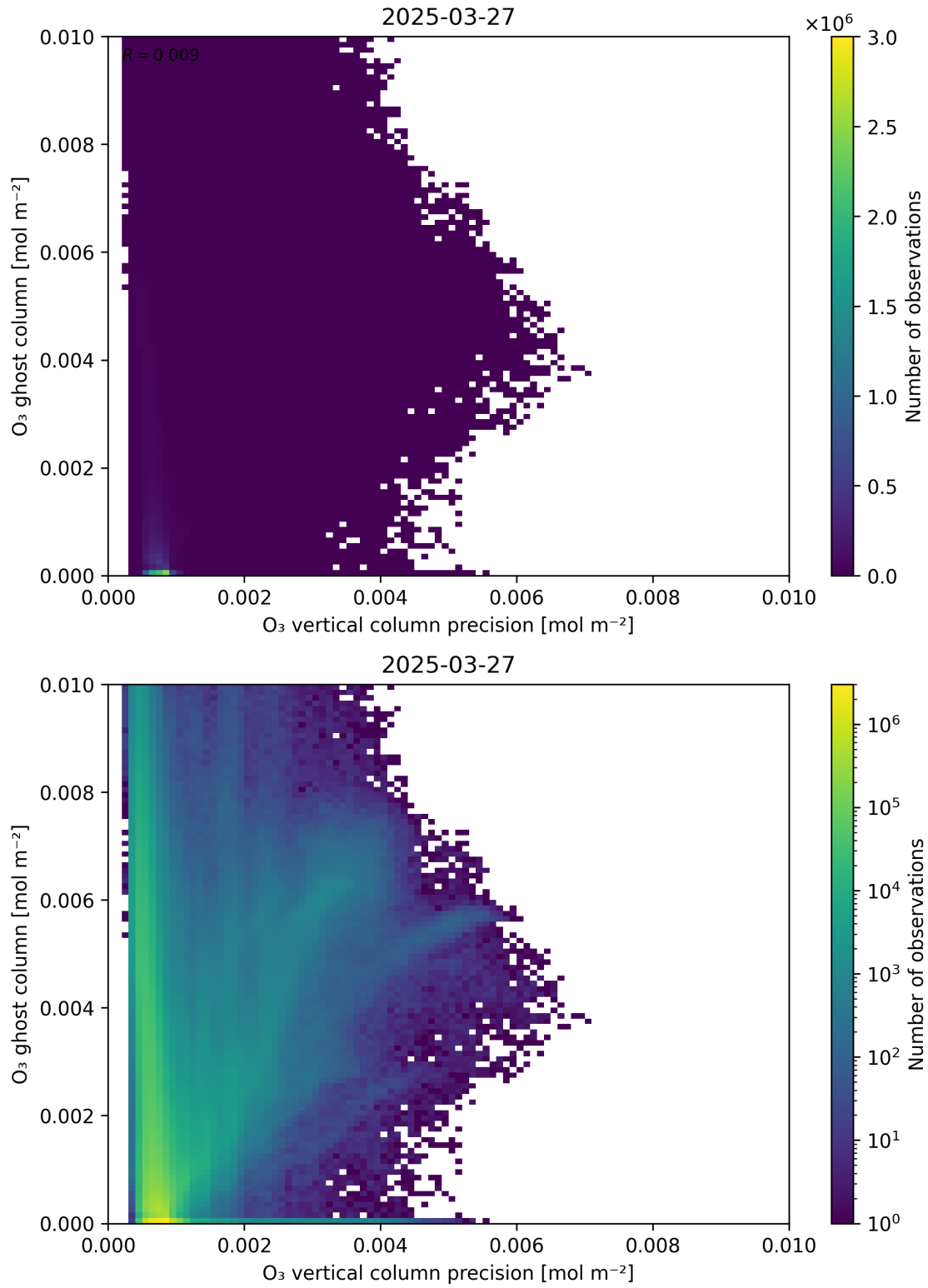
Figure 43: Scatter density plot of “ O_3 vertical column precision” against “ O_3 ghost column” for 2025-03-26 to 2025-03-28.
