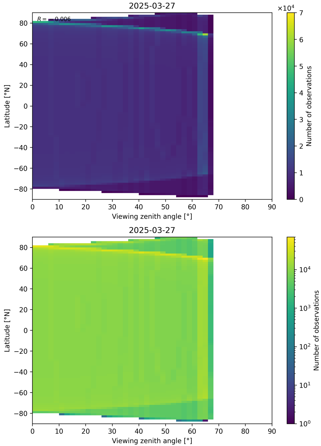
Figure 49: Scatter density plot of “Viewing zenith angle” against “Latitude” for 2025-03-26 to 2025-03-28.
