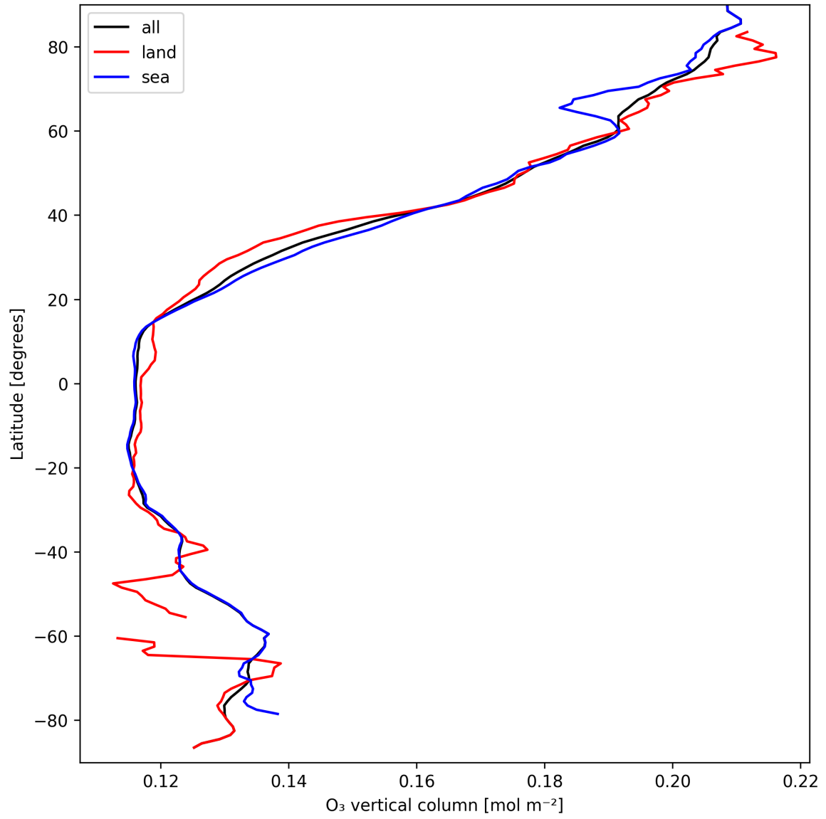
Figure 14: Zonal average of “O 3 vertical column” for 2025-03-26 to 2025-03-28.
