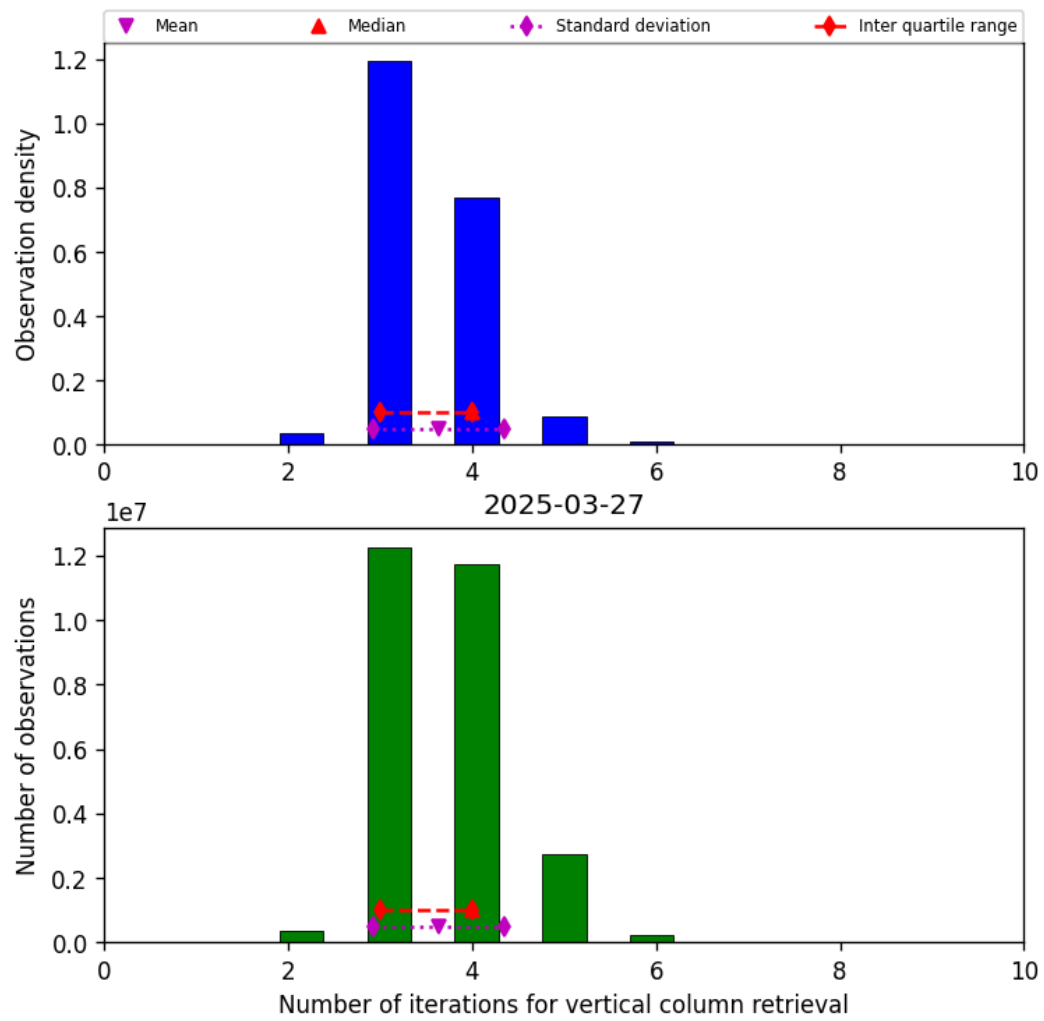
Figure 26: Histogram of “Number of iterations for vertical column retrieval” for 2025-03-26 to 2025-03-28
