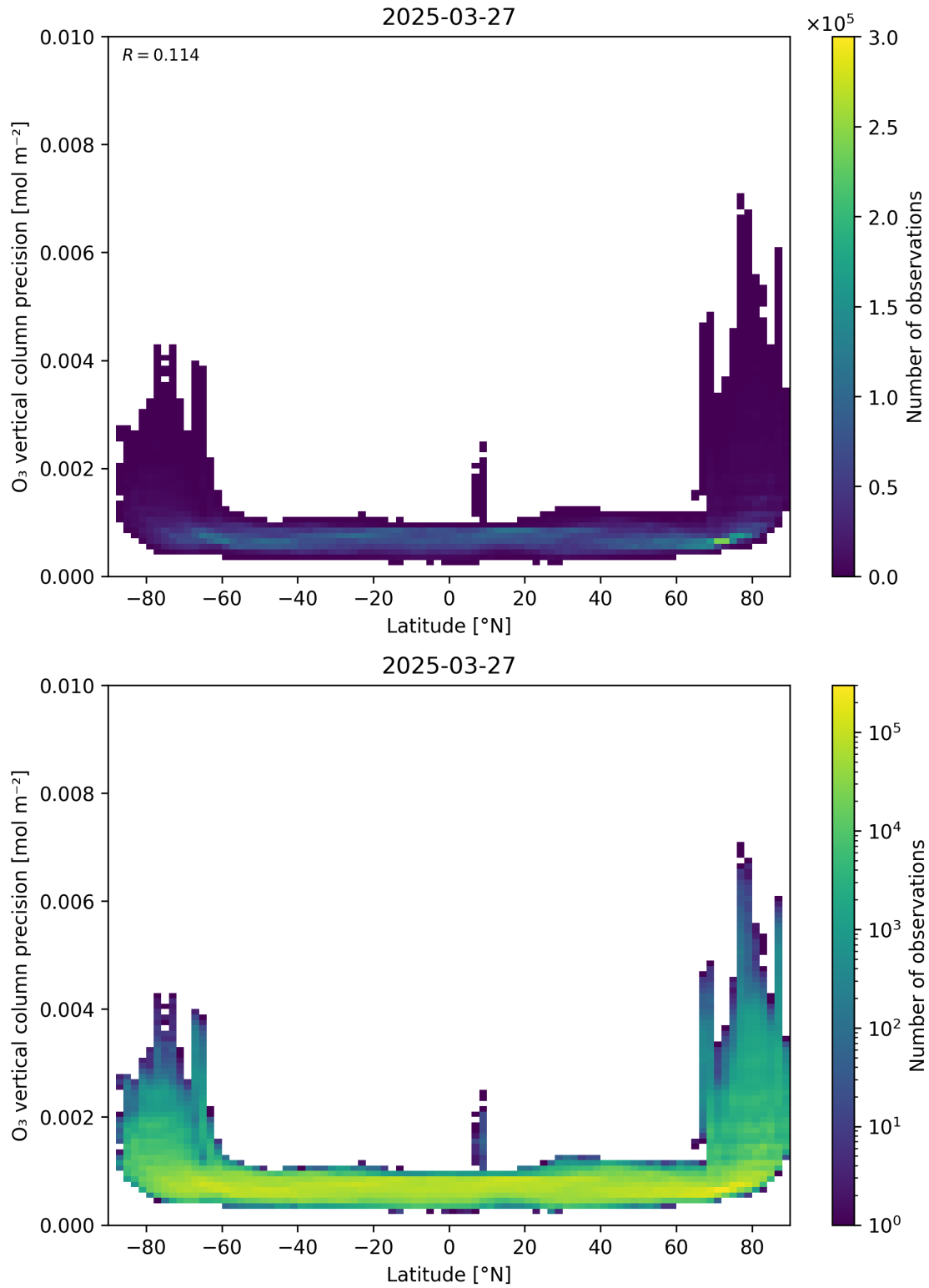
Figure 37: Scatter density plot of “Latitude” against “O 3 vertical column precision” for 2025-03-26 to 2025-03-28.
