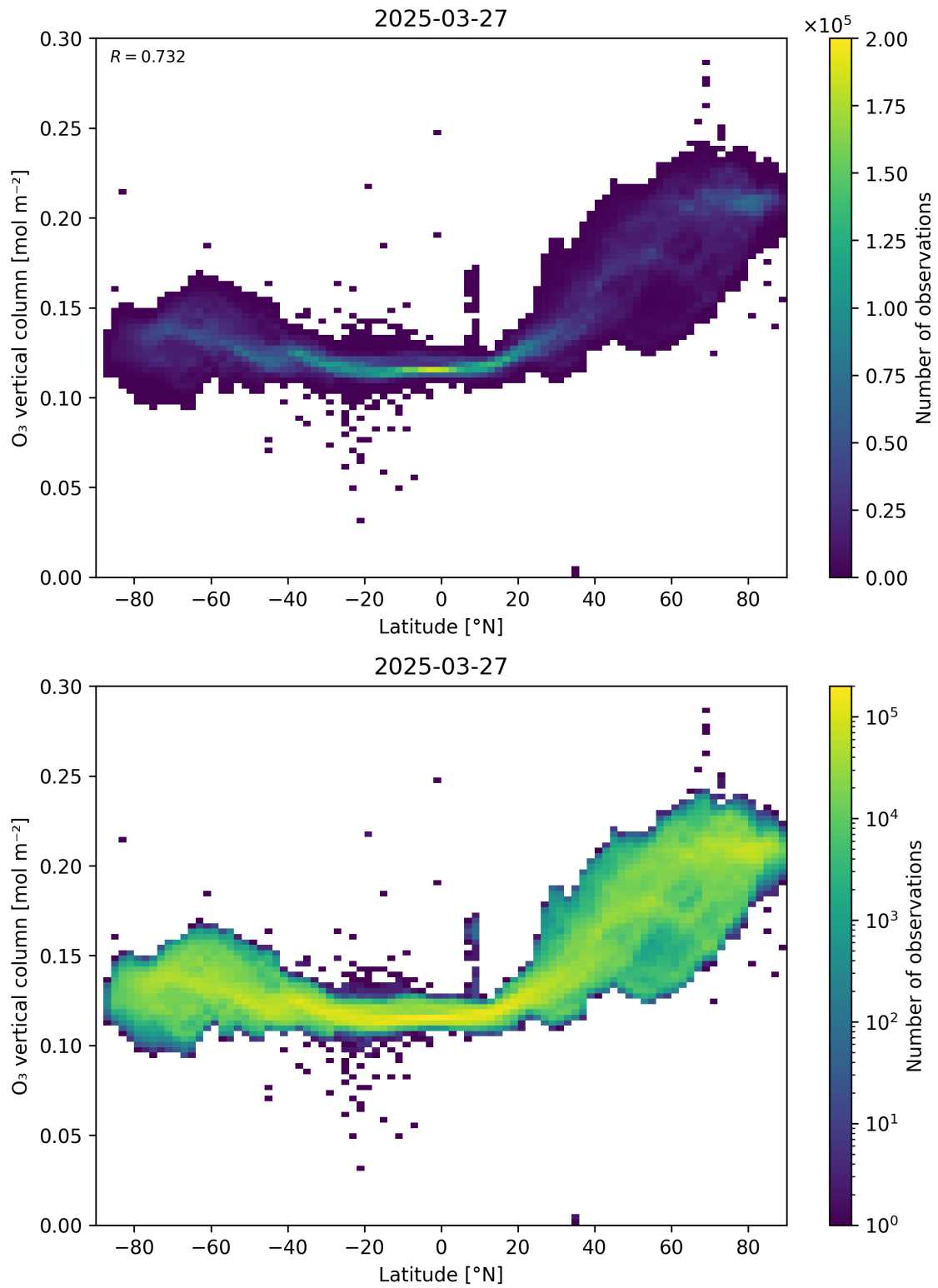
Figure 36: Scatter density plot of “Latitude” against “O 3 vertical column” for 2025-03-26 to 2025-03-28.
