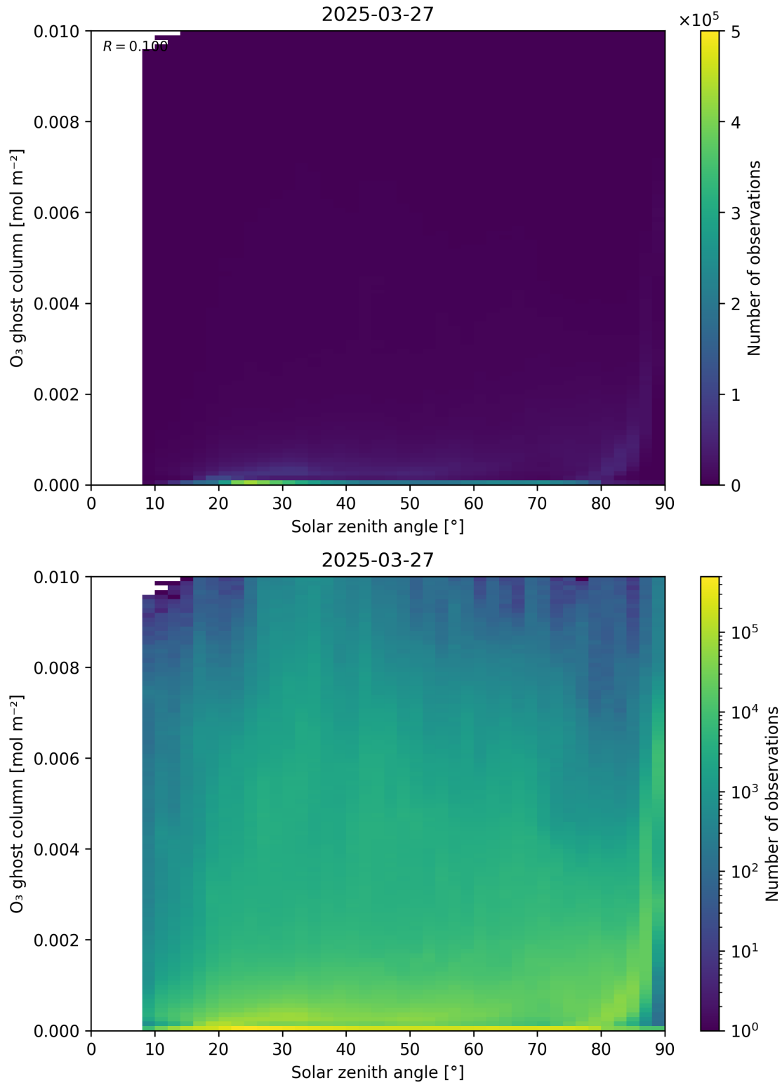
Figure 46: Scatter density plot of “Solar zenith angle” against “O 3 ghost column” for 2025-03-26 to 2025-03-28.
