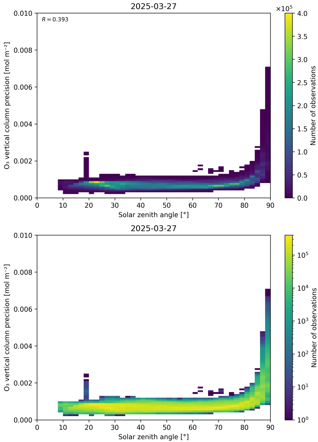
Figure 48: Scatter density plot of “Solar zenith angle” against “O 3 vertical column precision” for 2025-03-26 to 2025-03-28.
