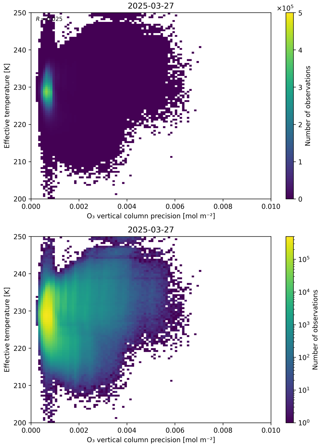
Figure 42: Scatter density plot of “O 3 vertical column precision” against “Effective temperature” for 2025-03-26 to 2025-03-28.
