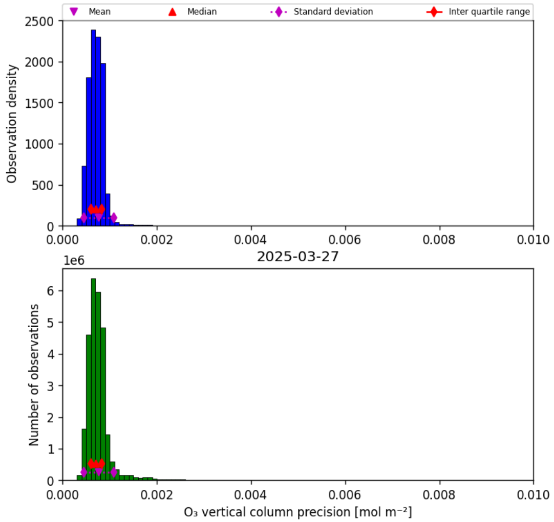
Figure 22: Histogram of “O 3 vertical column precision” for 2025-03-26 to 2025-03-28
