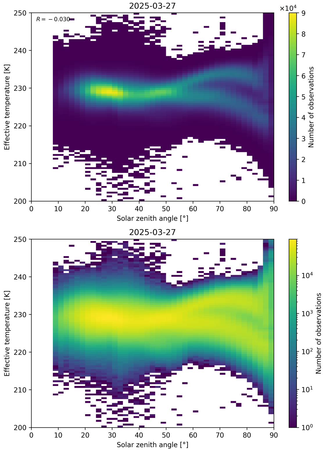
Figure 45: Scatter density plot of “Solar zenith angle” against “Effective temperature” for 2025-03-26 to 2025-03-28.
