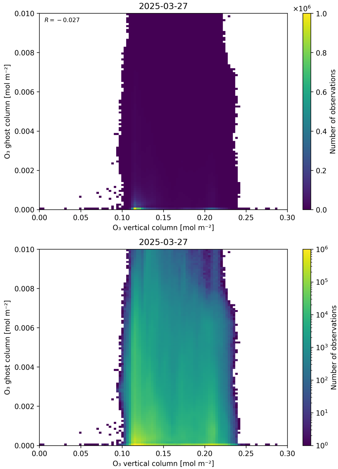
Figure 40: Scatter density plot of “O 3 vertical column” against “O 3 ghost column” for 2025-03-26 to 2025-03-28.
