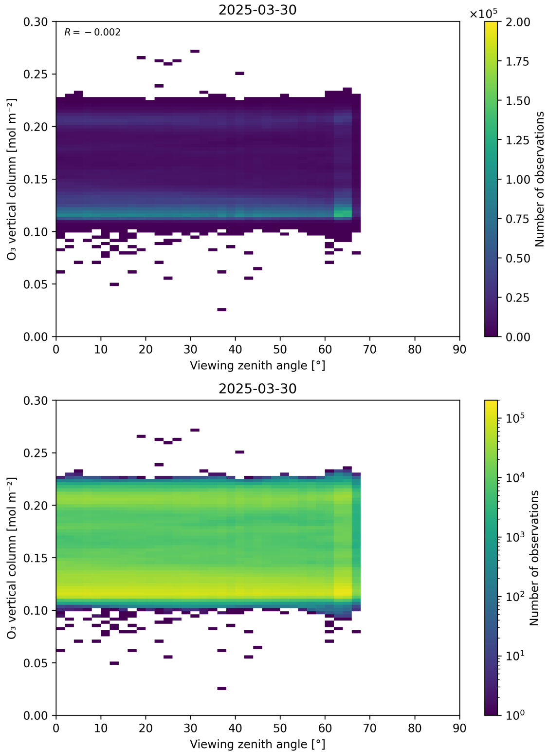
Figure 52: Scatter density plot of “Viewing zenith angle” against “O 3 vertical column” for 2025-03-29 to 2025-03-31.
