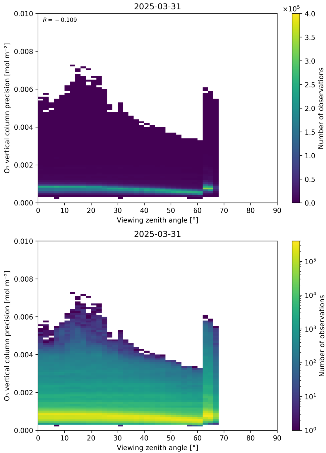
Figure 53: Scatter density plot of “Viewing zenith angle” against “O 3 vertical column precision” for 2025-03-30 to 2025-04-01.
