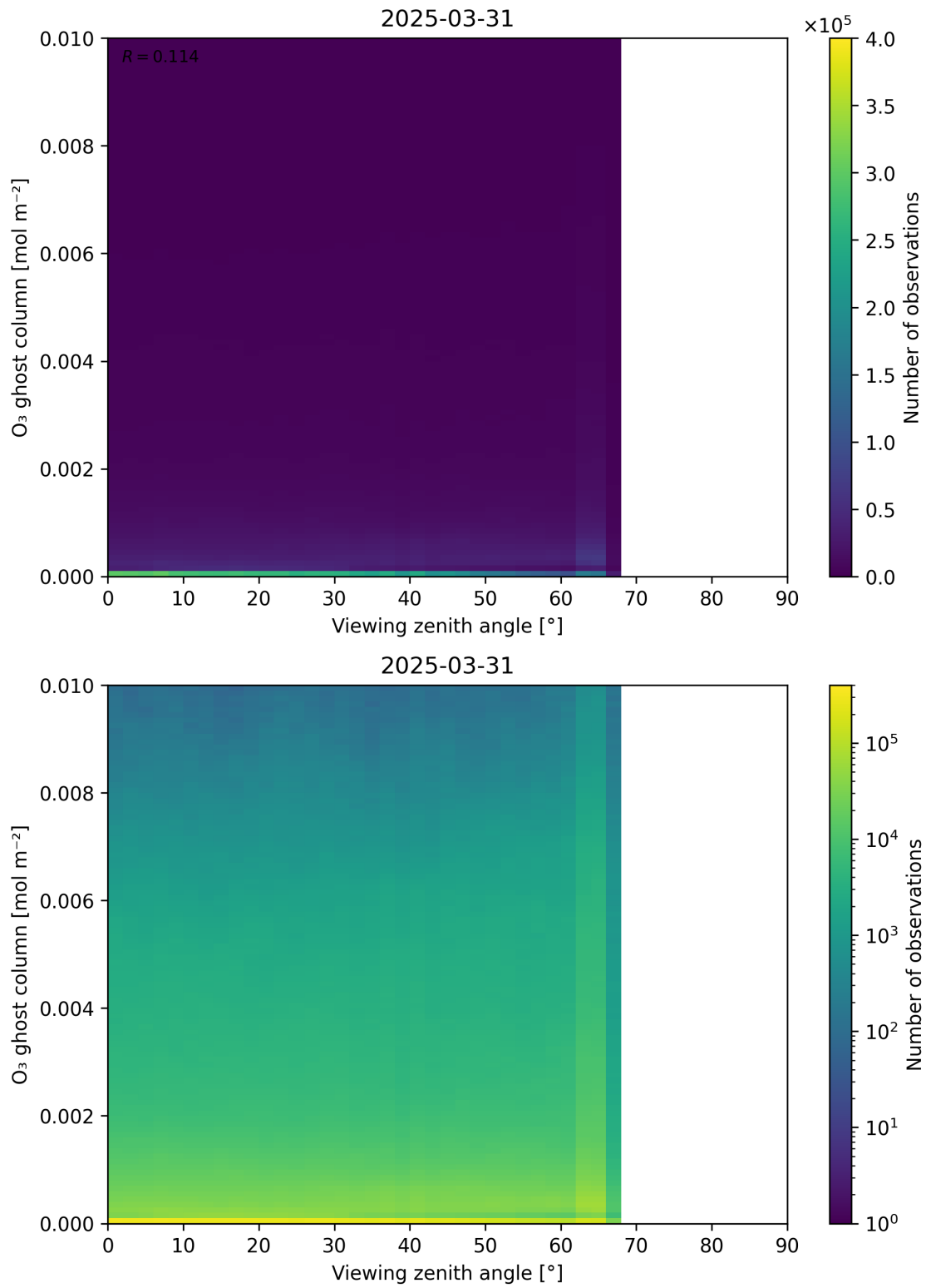
Figure 51: Scatter density plot of “Viewing zenith angle” against “O 3 ghost column” for 2025-03-30 to 2025-04-01.
