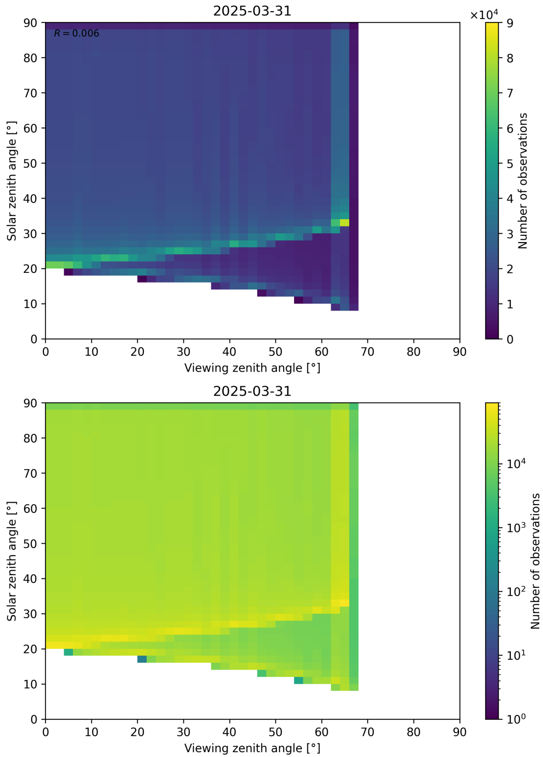
Figure 54: Scatter density plot of “Viewing zenith angle” against “Solar zenith angle” for 2025-03-30 to 2025-04-01.
