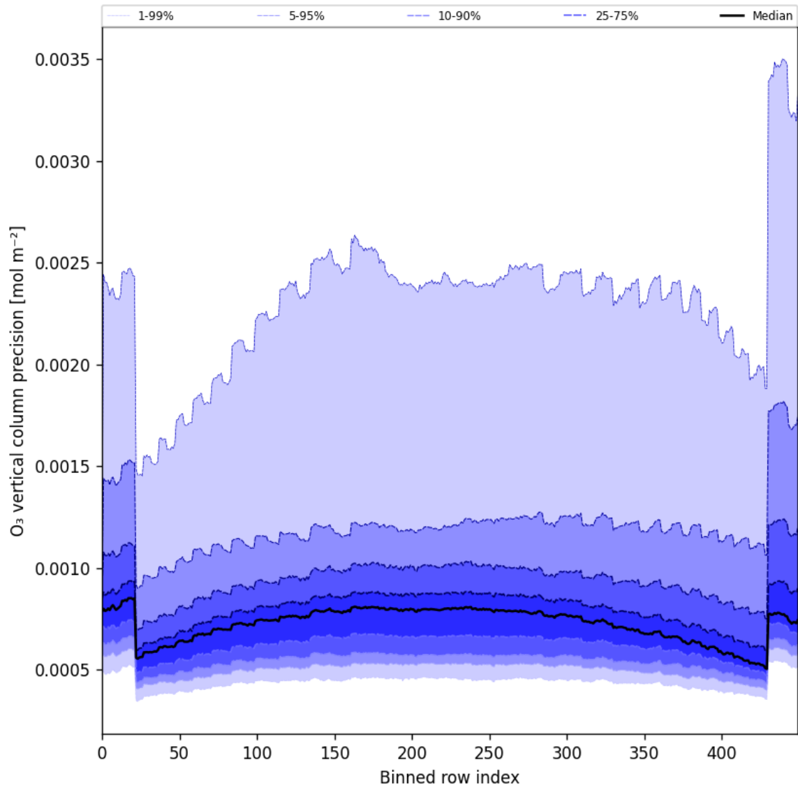
Figure 29: Along track statistics of “O 3 vertical column precision” for 2025-03-30 to 2025-04-01
