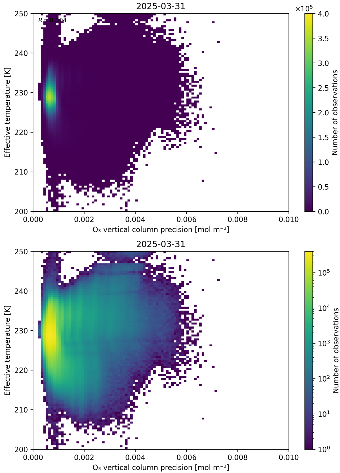
Figure 42: Scatter density plot of “O 3 vertical column precision” against “Effective temperature” for 2025-03-30 to 2025-04-01.
