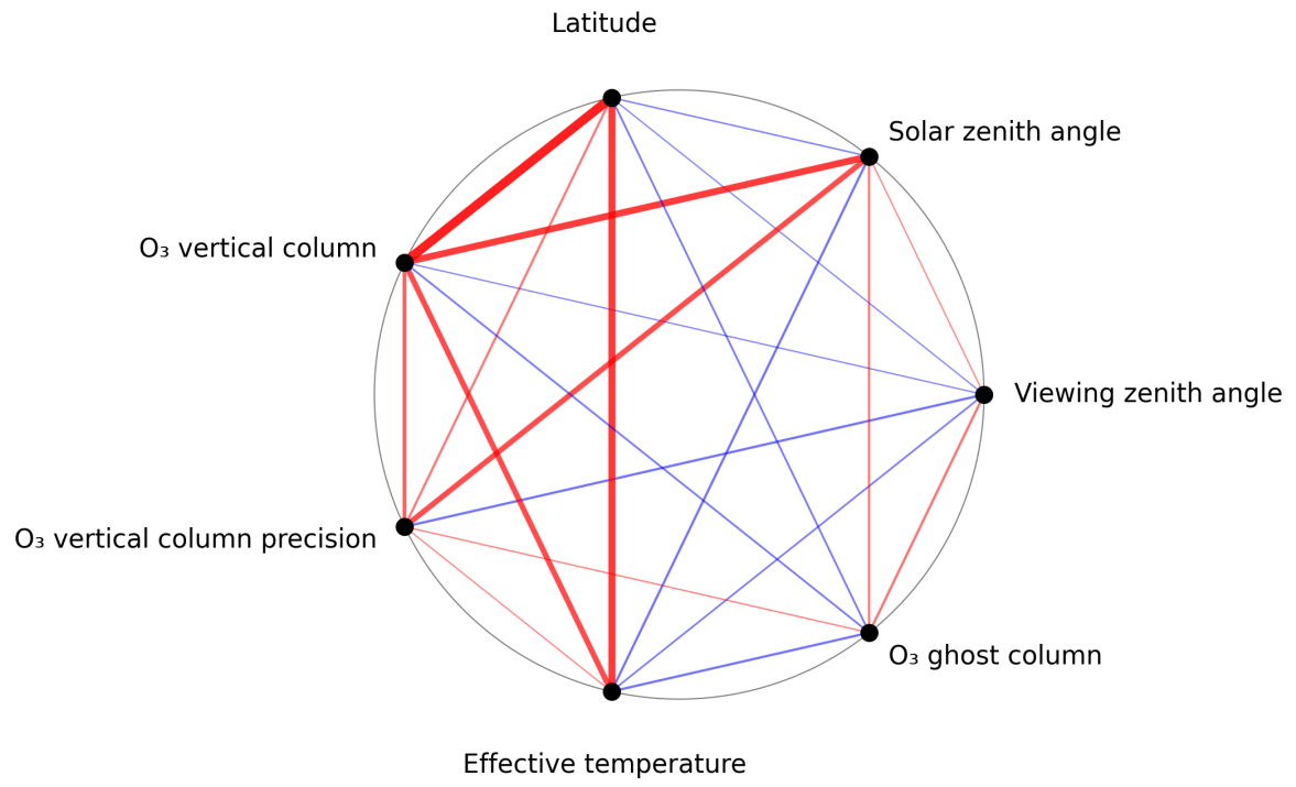
Figure 1: Map of correlation graph for 2025-03-30 to 2025-04-01.
