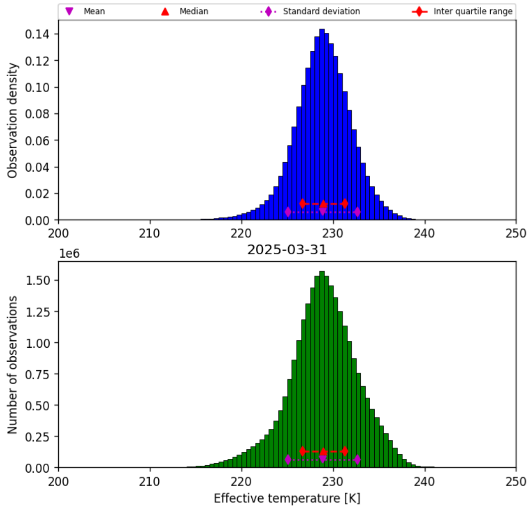
Figure 24: Histogram of “Effective temperature” for 2025-03-30 to 2025-04-01
