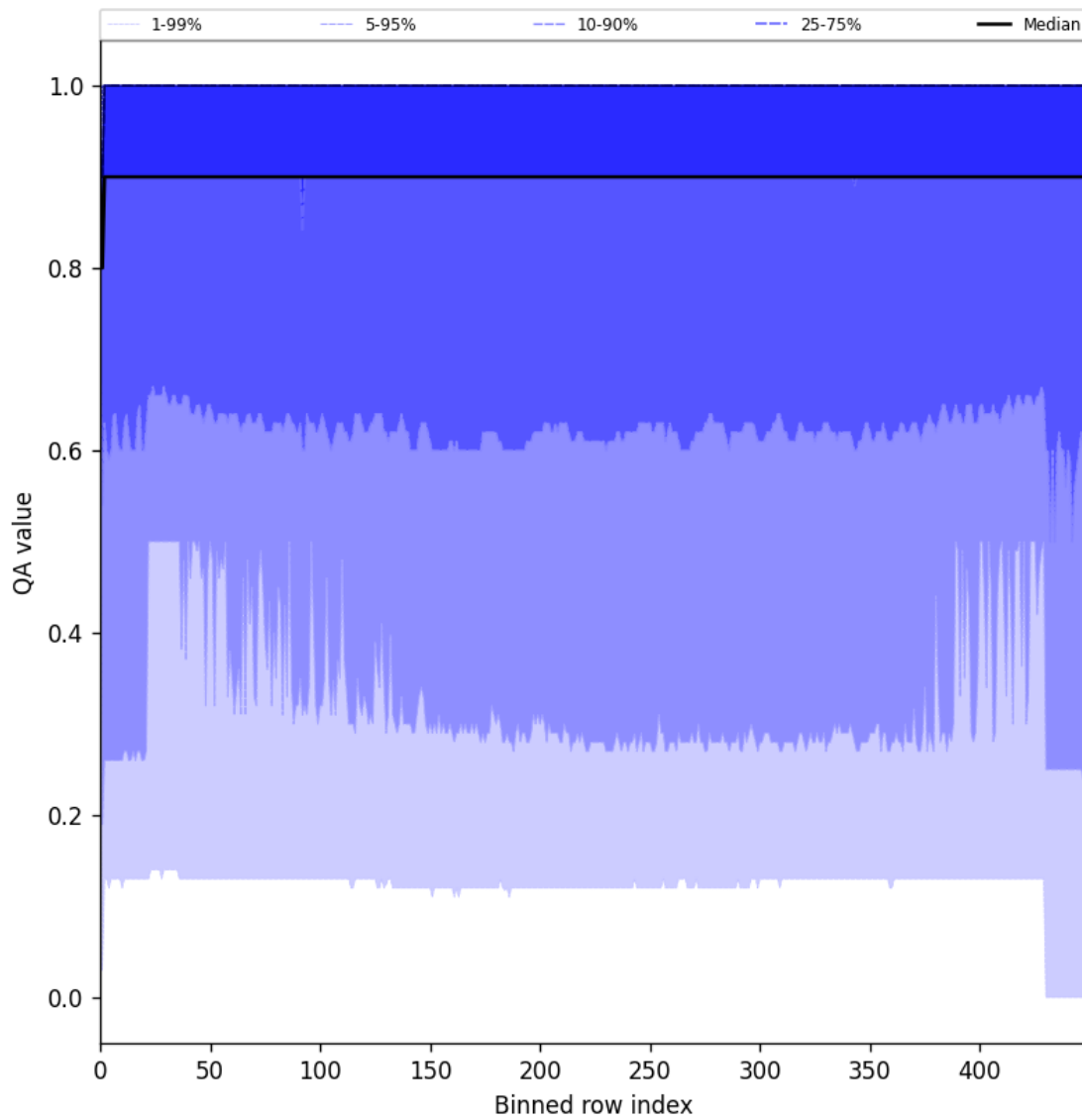
Figure 27: Along track statistics of “QA value” for 2025-03-30 to 2025-04-01
