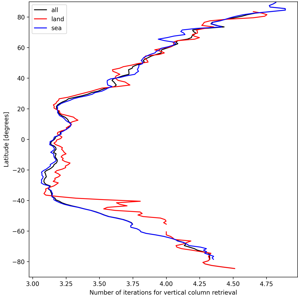
Figure 19: Zonal average of “Number of iterations for vertical column retrieval” for 2025-03-30 to 2025-04-01.
