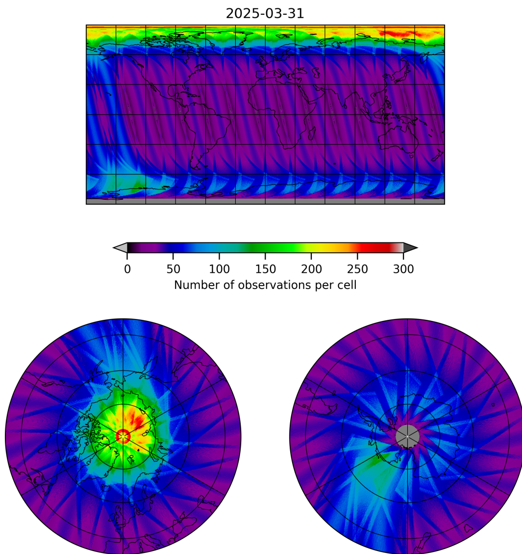
Figure 12: Map of the number of observations for 2025-03-30 to 2025-04-01
