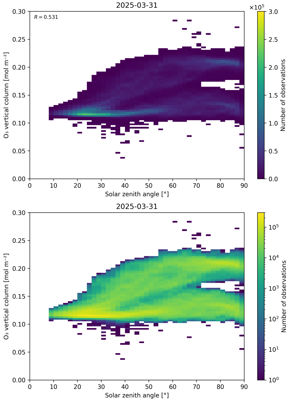
Figure 47: Scatter density plot of “Solar zenith angle” against “O 3 vertical column” for 2025-03-30 to 2025-04-01.
