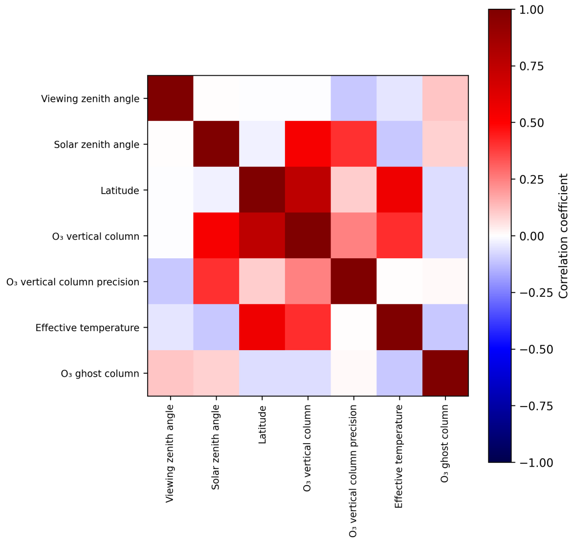
Figure 2: Map of correlation matrix for 2025-03-30 to 2025-04-01.
