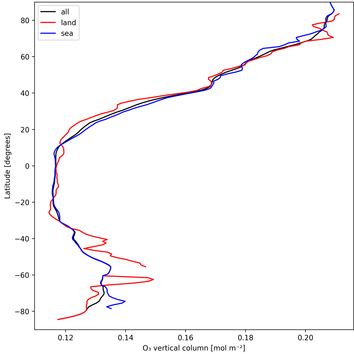
Figure 14: Zonal average of “O 3 vertical column” for 2025-03-30 to 2025-04-01.
