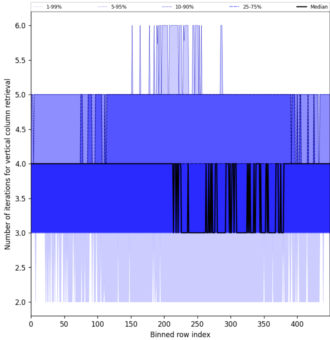
Figure 33: Along track statistics of “Number of iterations for vertical column retrieval” for 2025-03-30 to 2025-04-01
