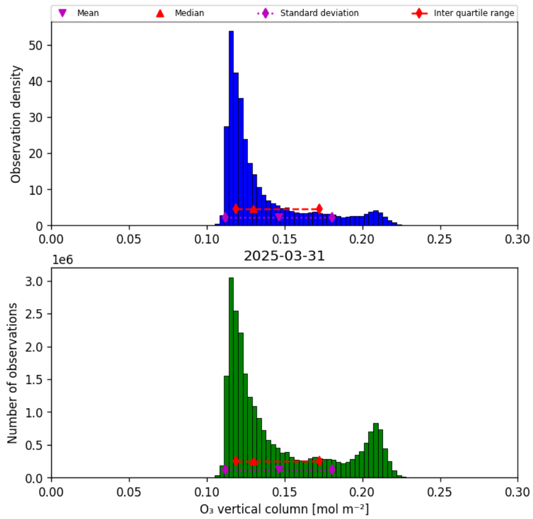
Figure 21: Histogram of “O 3 vertical column” for 2025-03-30 to 2025-04-01
