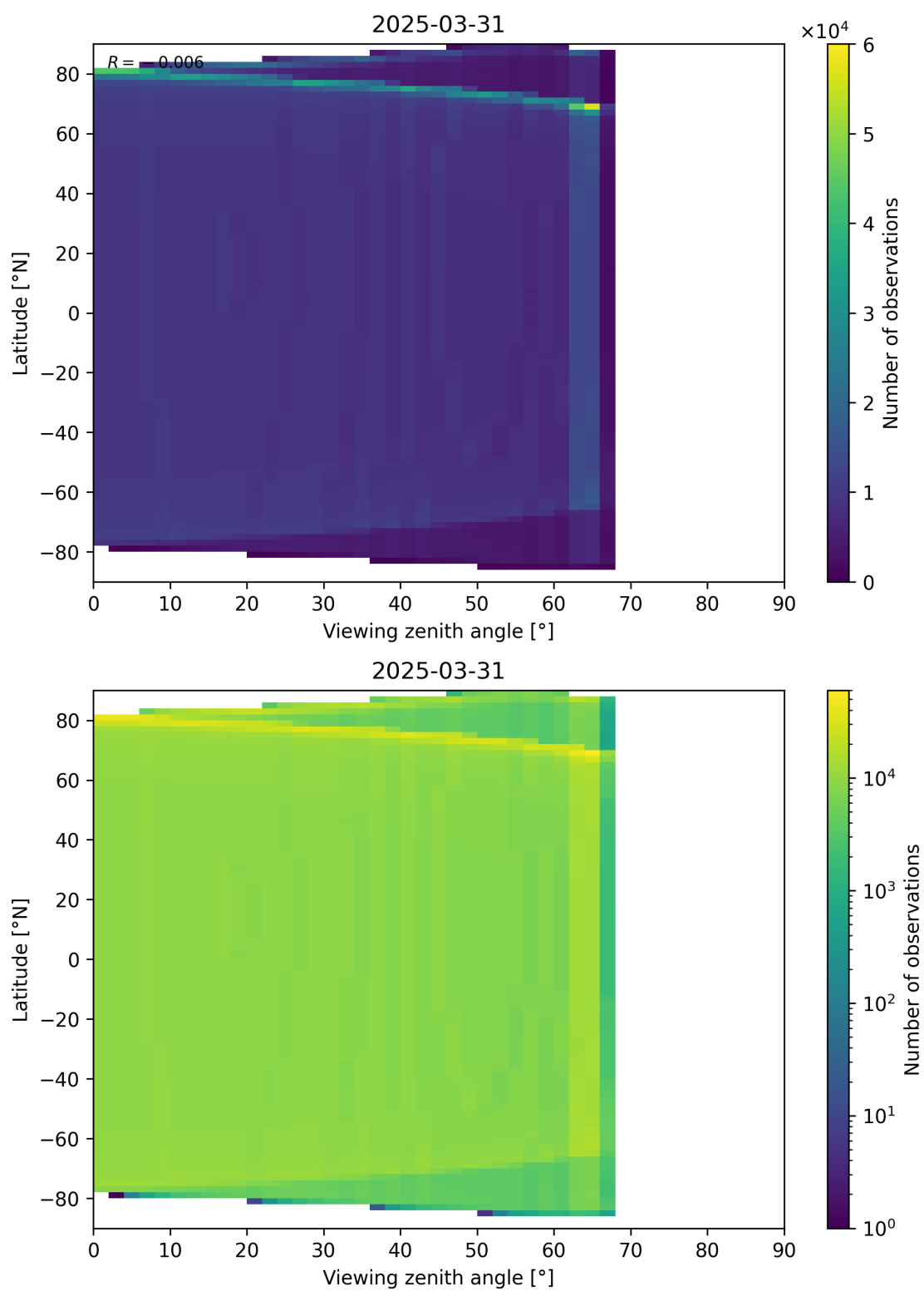
Figure 49: Scatter density plot of “Viewing zenith angle” against “Latitude” for 2025-03-30 to 2025-04-01.
