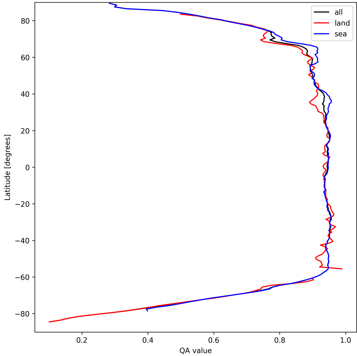
Figure 13: Zonal average of “QA value” for 2025-03-30 to 2025-04-01.
