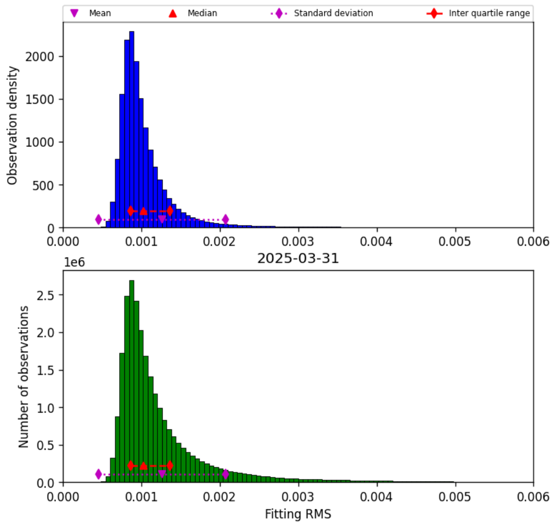
Figure 23: Histogram of “Fitting RMS” for 2025-03-30 to 2025-04-01
