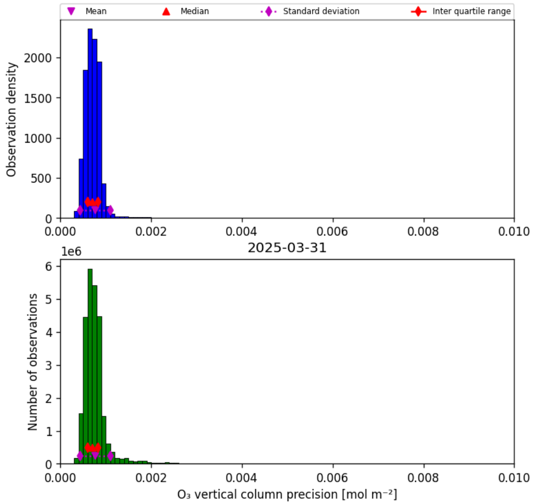
Figure 22: Histogram of “O 3 vertical column precision” for 2025-03-30 to 2025-04-01
