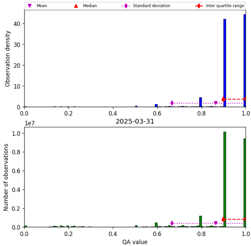
Figure 20: Histogram of “QA value” for 2025-03-30 to 2025-04-01
