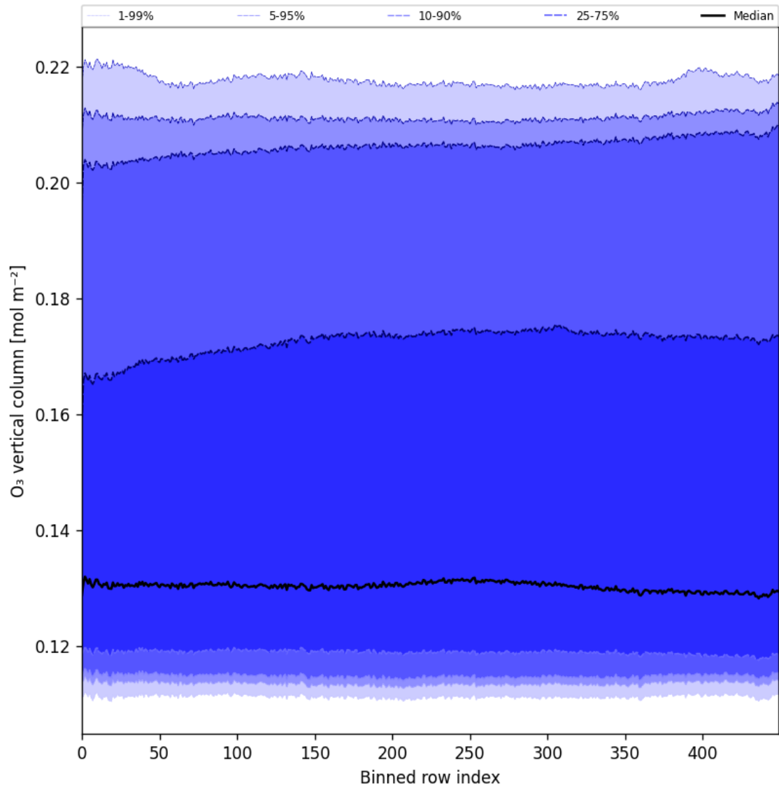
Figure 28: Along track statistics of “ O_3 vertical column” for 2025-03-30 to 2025-04-01
