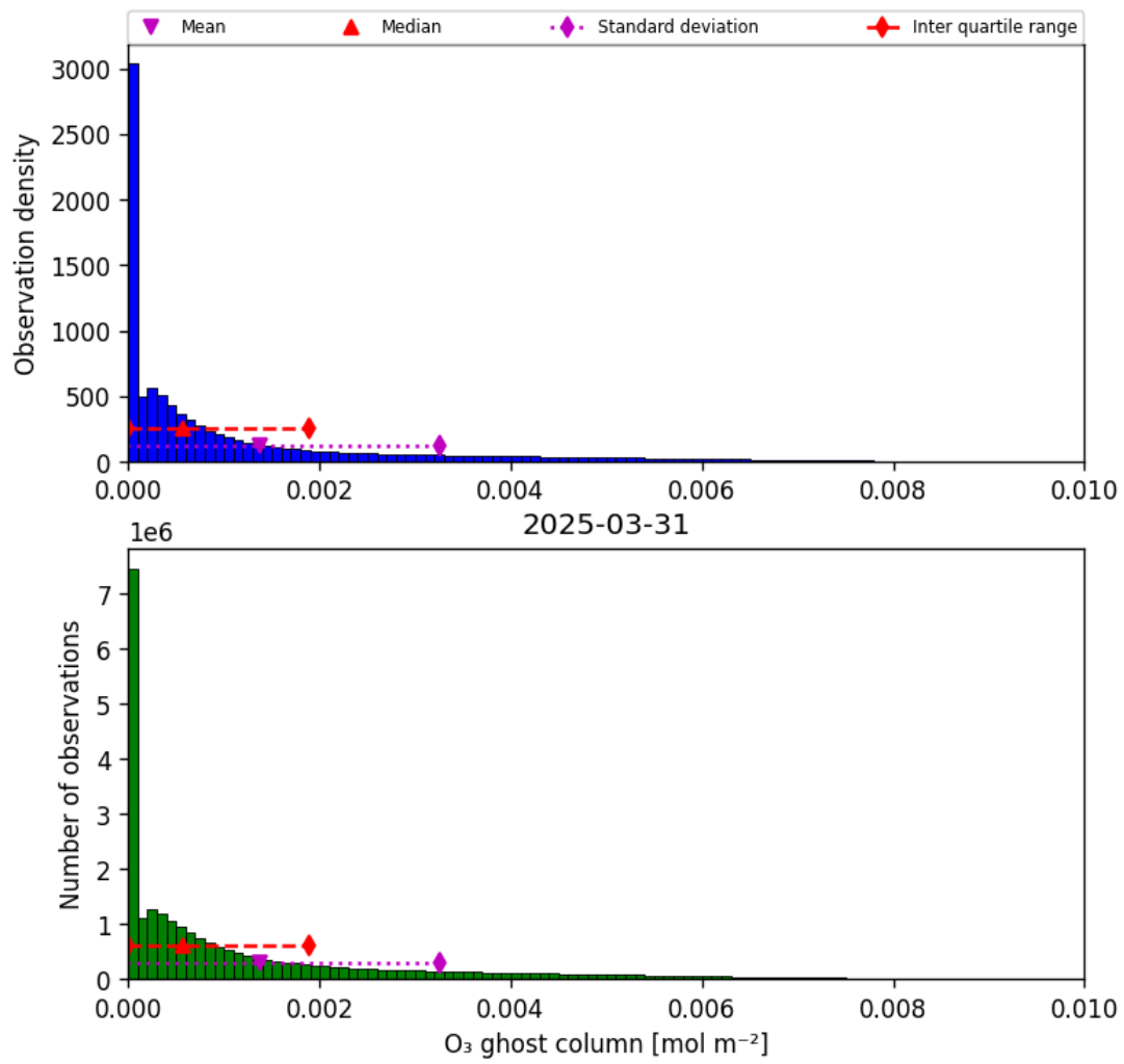
Figure 25: Histogram of “O 3 ghost column” for 2025-03-30 to 2025-04-01
