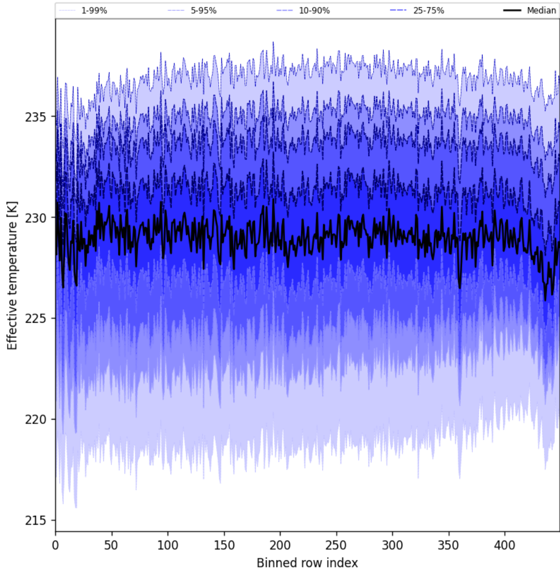
Figure 31: Along track statistics of “Effective temperature” for 2025-03-30 to 2025-04-01
