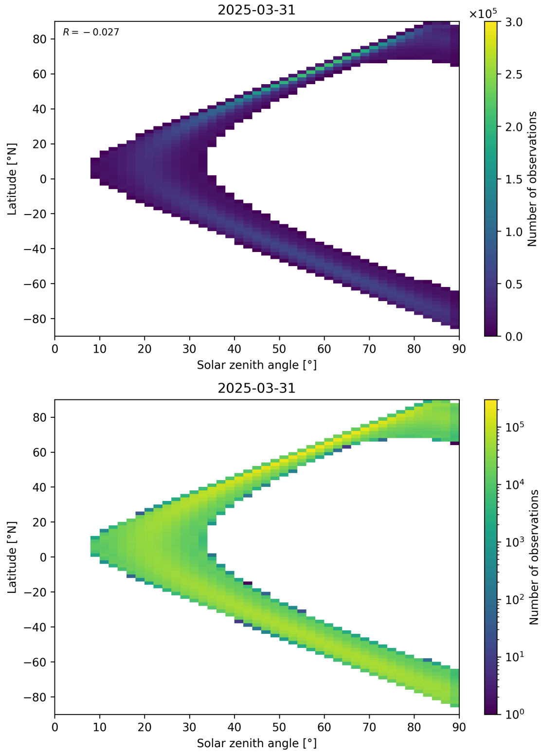
Figure 44: Scatter density plot of “Solar zenith angle” against “Latitude” for 2025-03-30 to 2025-04-01.
