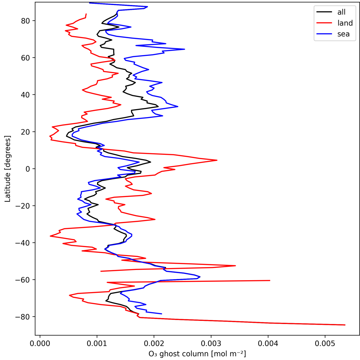
Figure 18: Zonal average of “O 3 ghost column” for 2025-03-30 to 2025-04-01.
