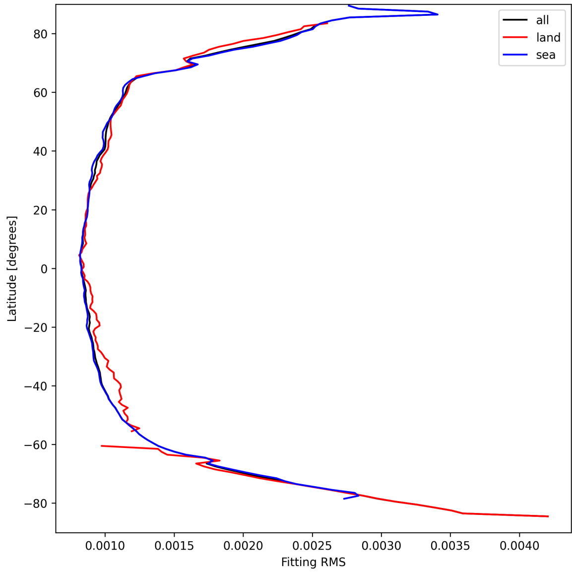
Figure 16: Zonal average of “Fitting RMS” for 2025-03-30 to 2025-04-01.
