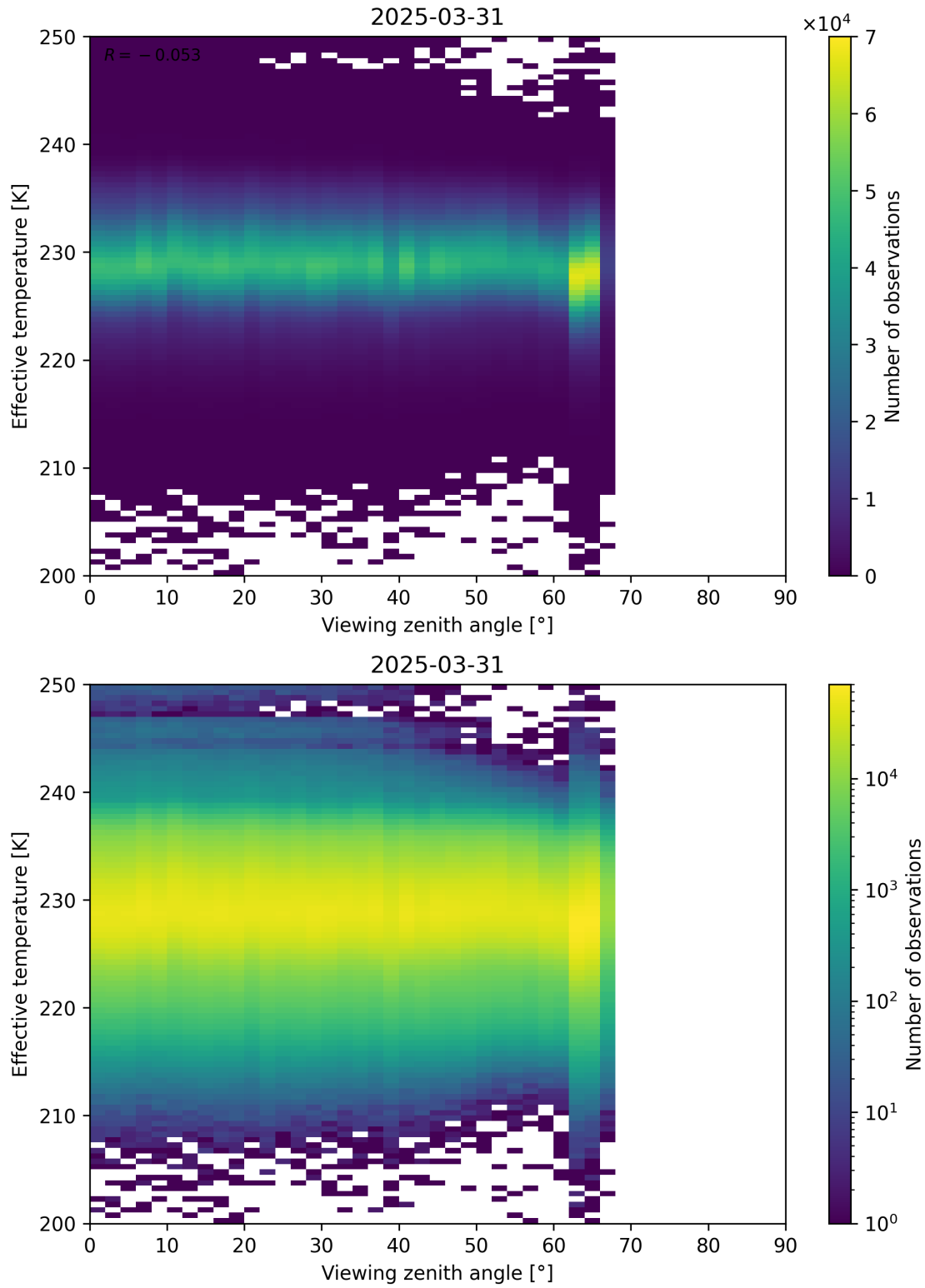
Figure 50: Scatter density plot of “Viewing zenith angle” against “Effective temperature” for 2025-03-30 to 2025-04-01.
