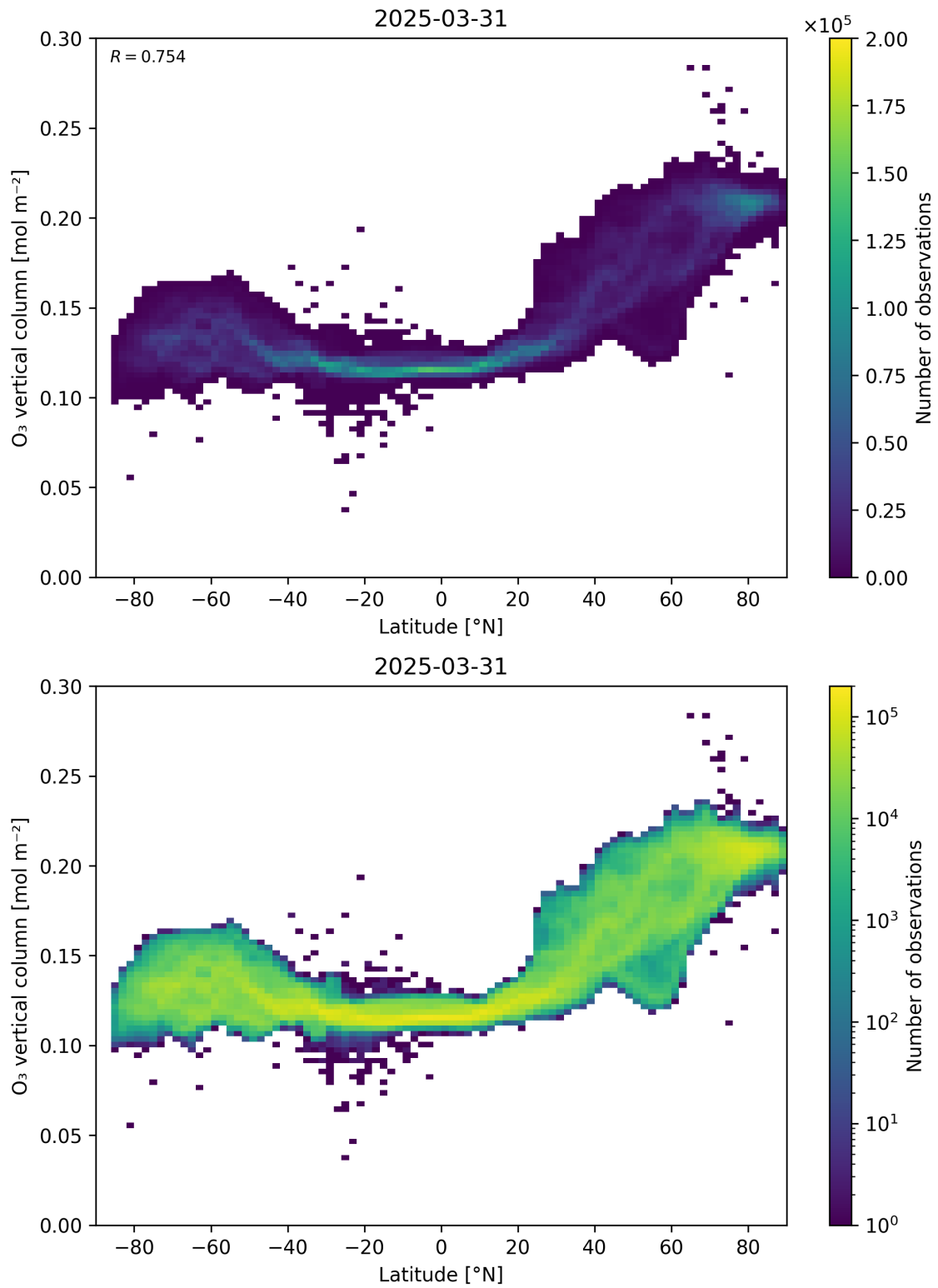
Figure 36: Scatter density plot of “Latitude” against “O 3 vertical column” for 2025-03-30 to 2025-04-01.
