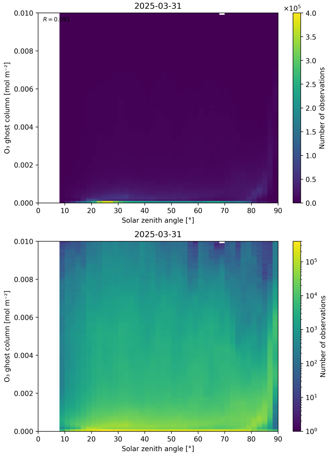
Figure 46: Scatter density plot of “Solar zenith angle” against “O 3 ghost column” for 2025-03-30 to 2025-04-01.
