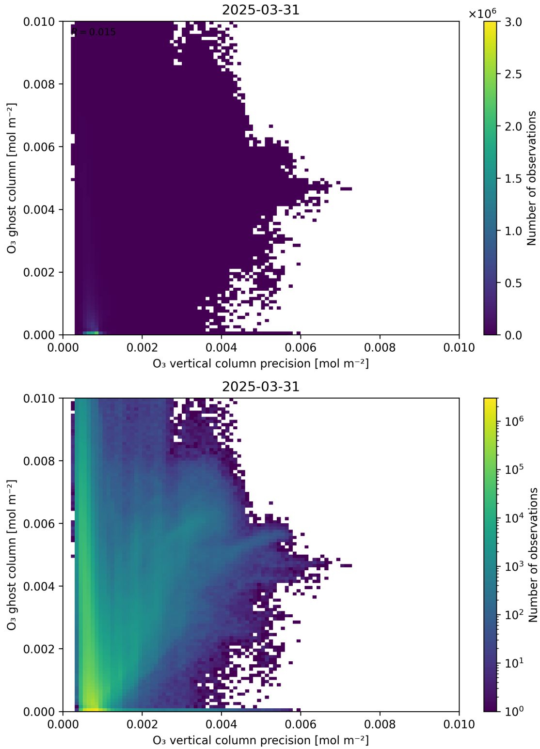
Figure 43: Scatter density plot of “O 3 vertical column precision” against “O 3 ghost column” for 2025-03-30 to 2025-04-01.
