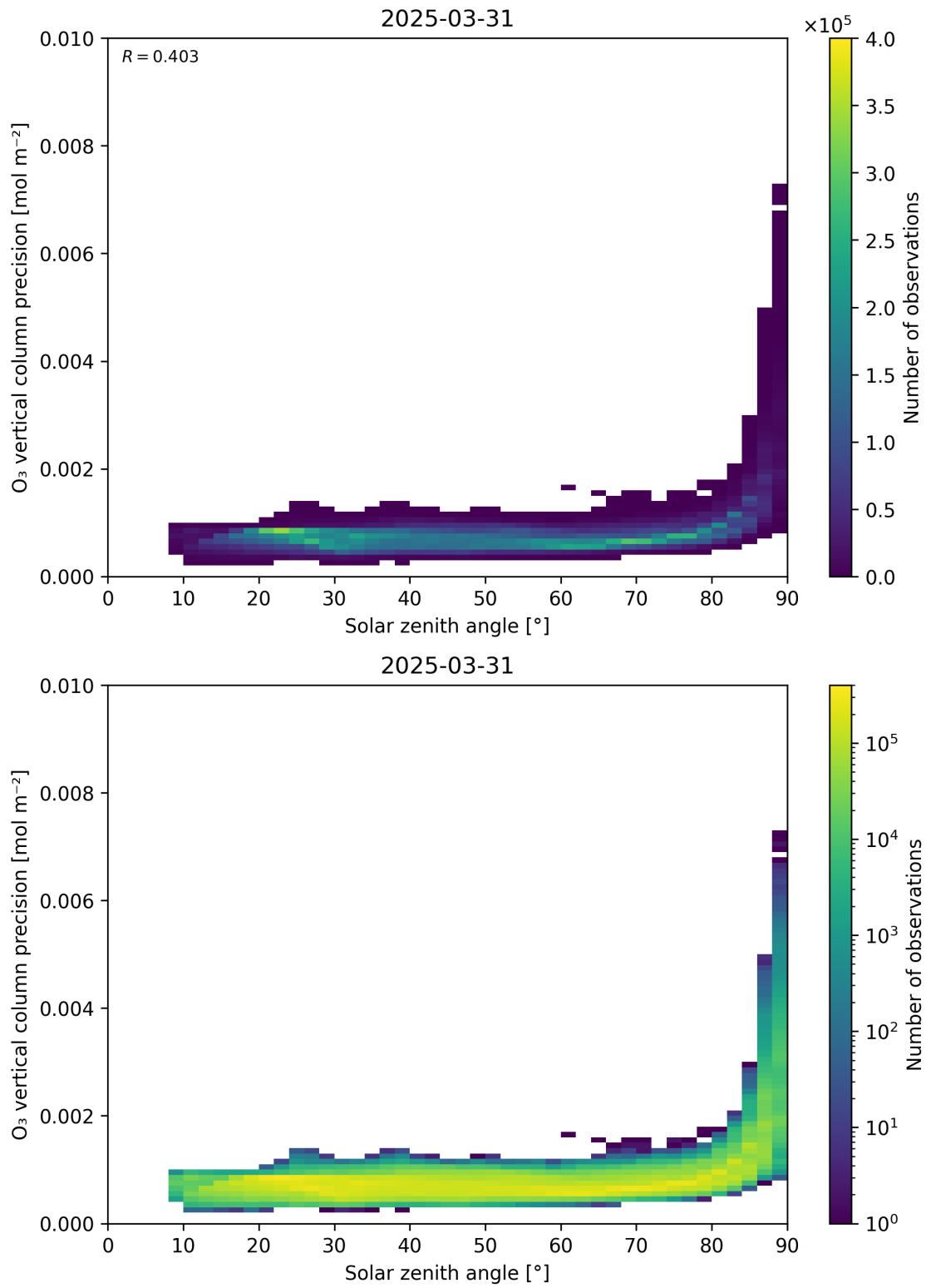
Figure 48: Scatter density plot of “Solar zenith angle” against “O 3 vertical column precision” for 2025-03-30 to 2025-04-01.
