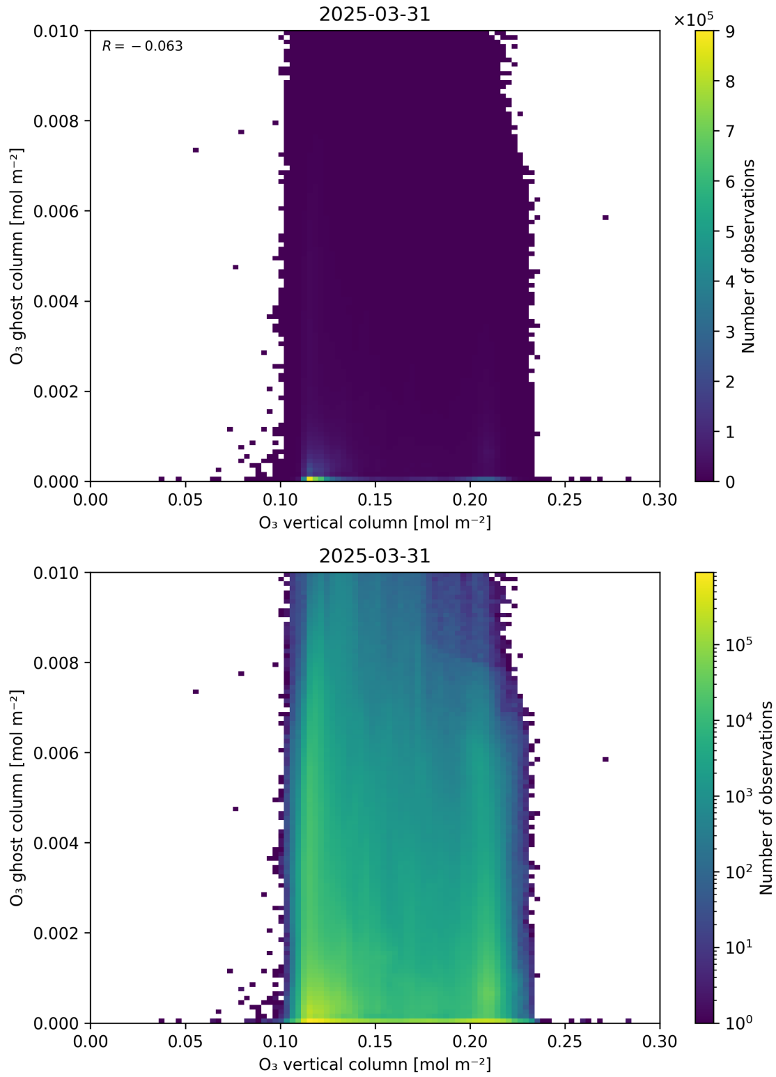
Figure 40: Scatter density plot of “O 3 vertical column” against “O 3 ghost column” for 2025-03-30 to 2025-04-01.
