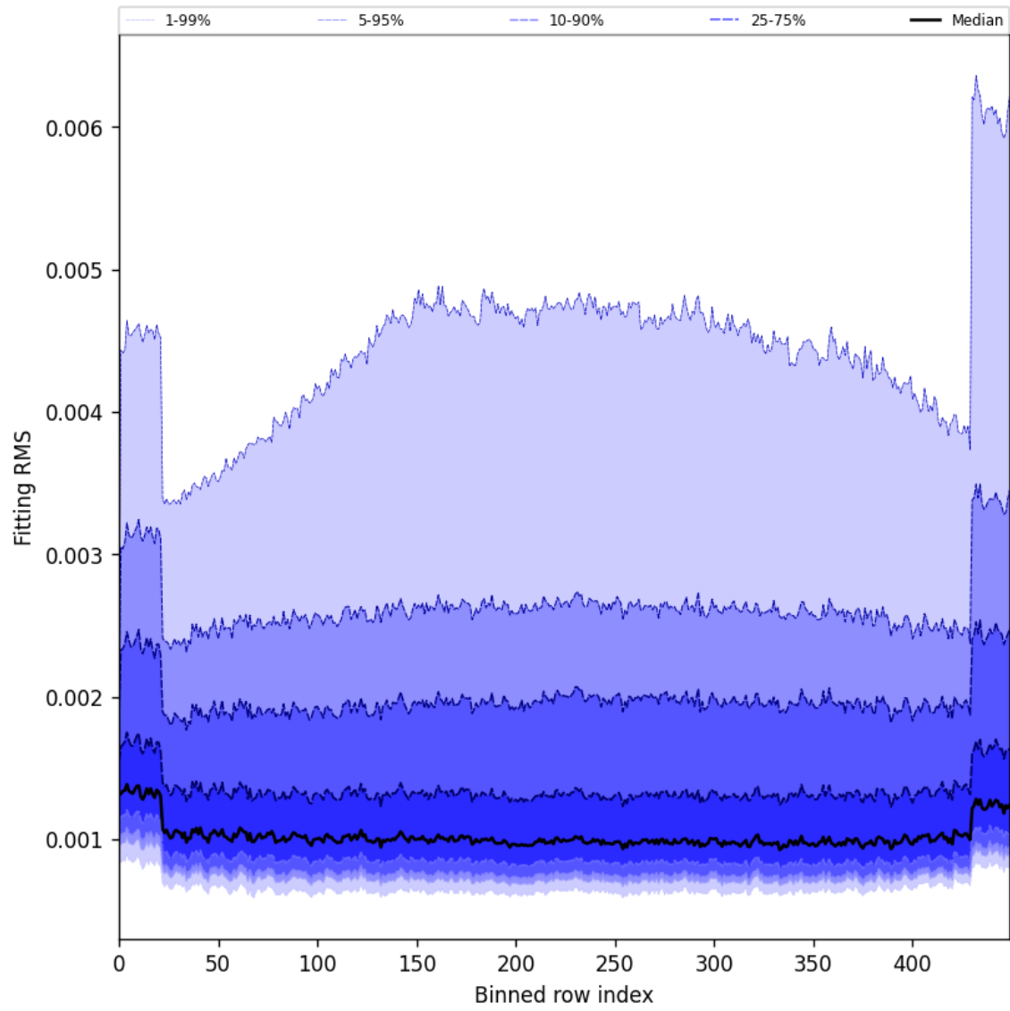
Figure 30: Along track statistics of “Fitting RMS” for 2025-03-30 to 2025-04-01
