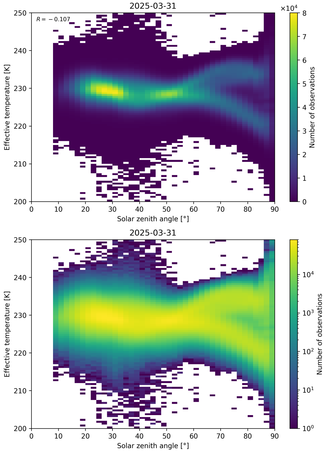
Figure 45: Scatter density plot of “Solar zenith angle” against “Effective temperature” for 2025-03-30 to 2025-04-01.
