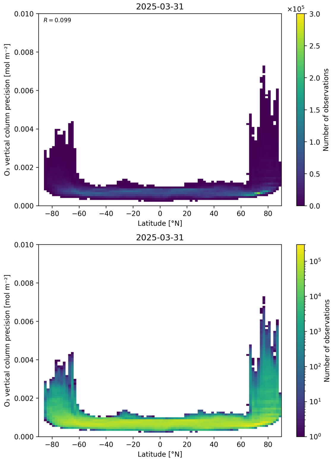
Figure 37: Scatter density plot of “Latitude” against “O 3 vertical column precision” for 2025-03-30 to 2025-04-01.
