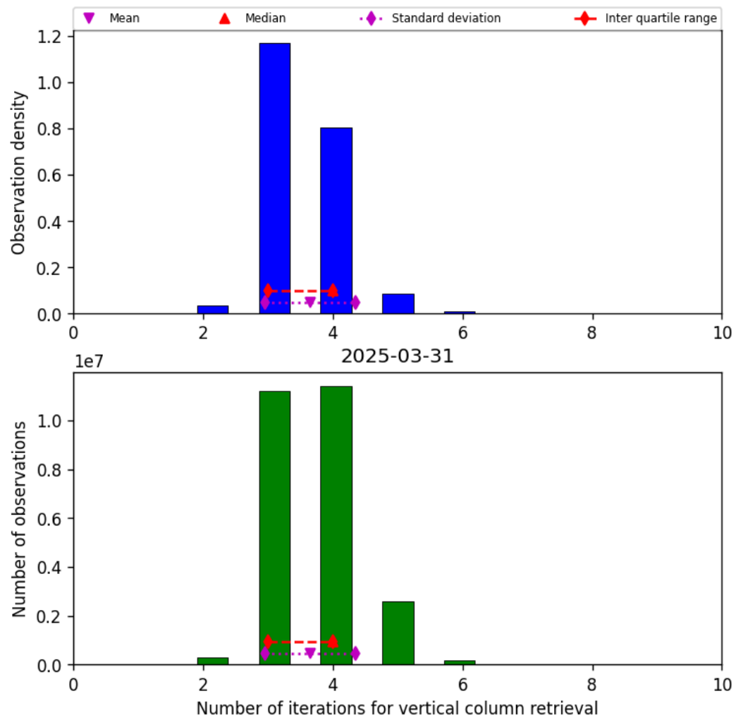
Figure 26: Histogram of “Number of iterations for vertical column retrieval” for 2025-03-30 to 2025-04-01
