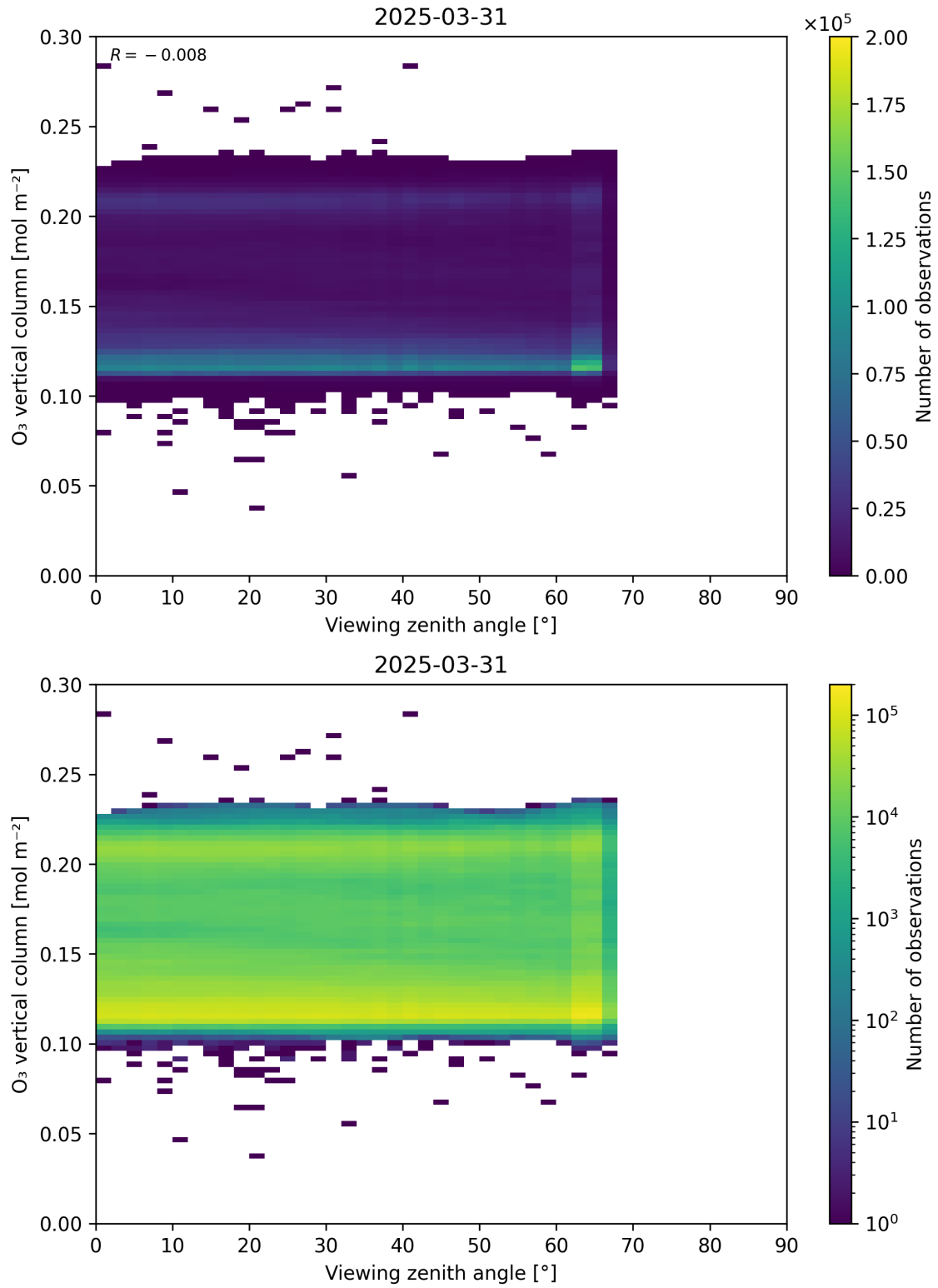
Figure 52: Scatter density plot of “Viewing zenith angle” against “O 3 vertical column” for 2025-03-30 to 2025-04-01.
