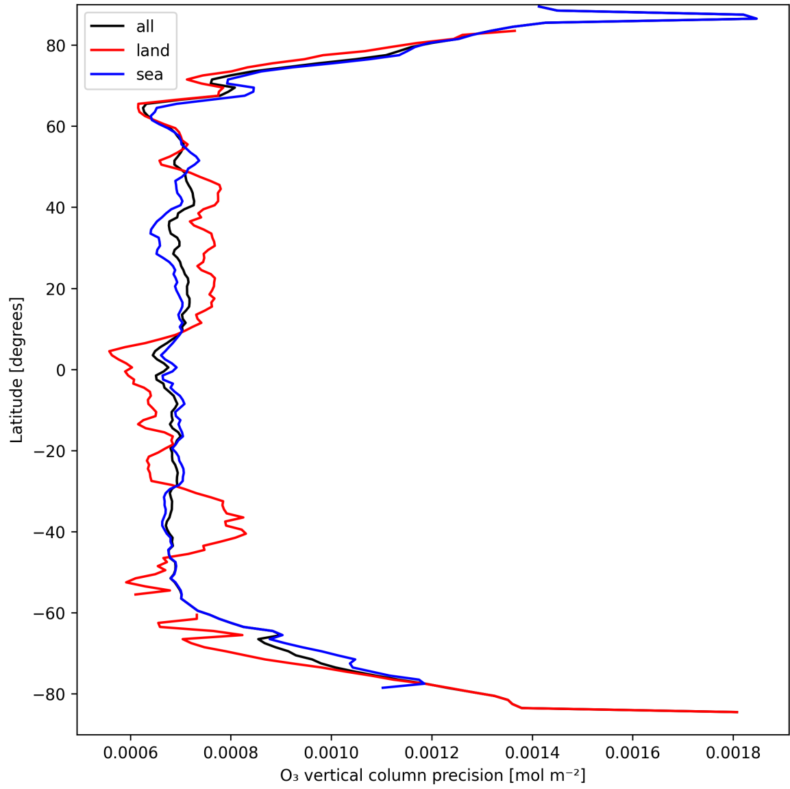
Figure 15: Zonal average of “O 3 vertical column precision” for 2025-03-30 to 2025-04-01.
