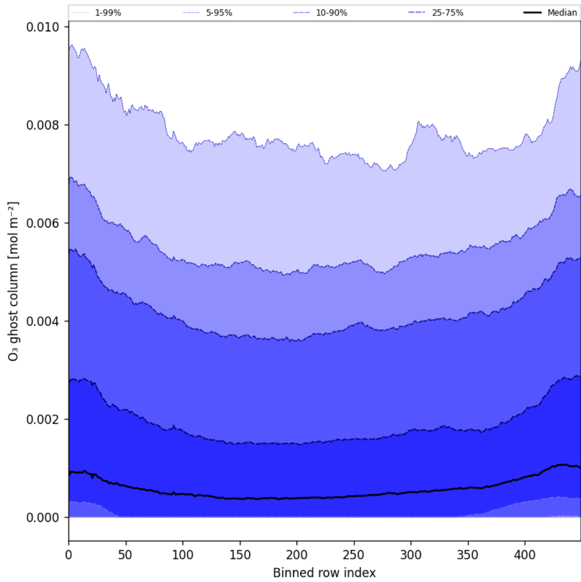
Figure 32: Along track statistics of “O 3 ghost column” for 2025-03-30 to 2025-04-01
