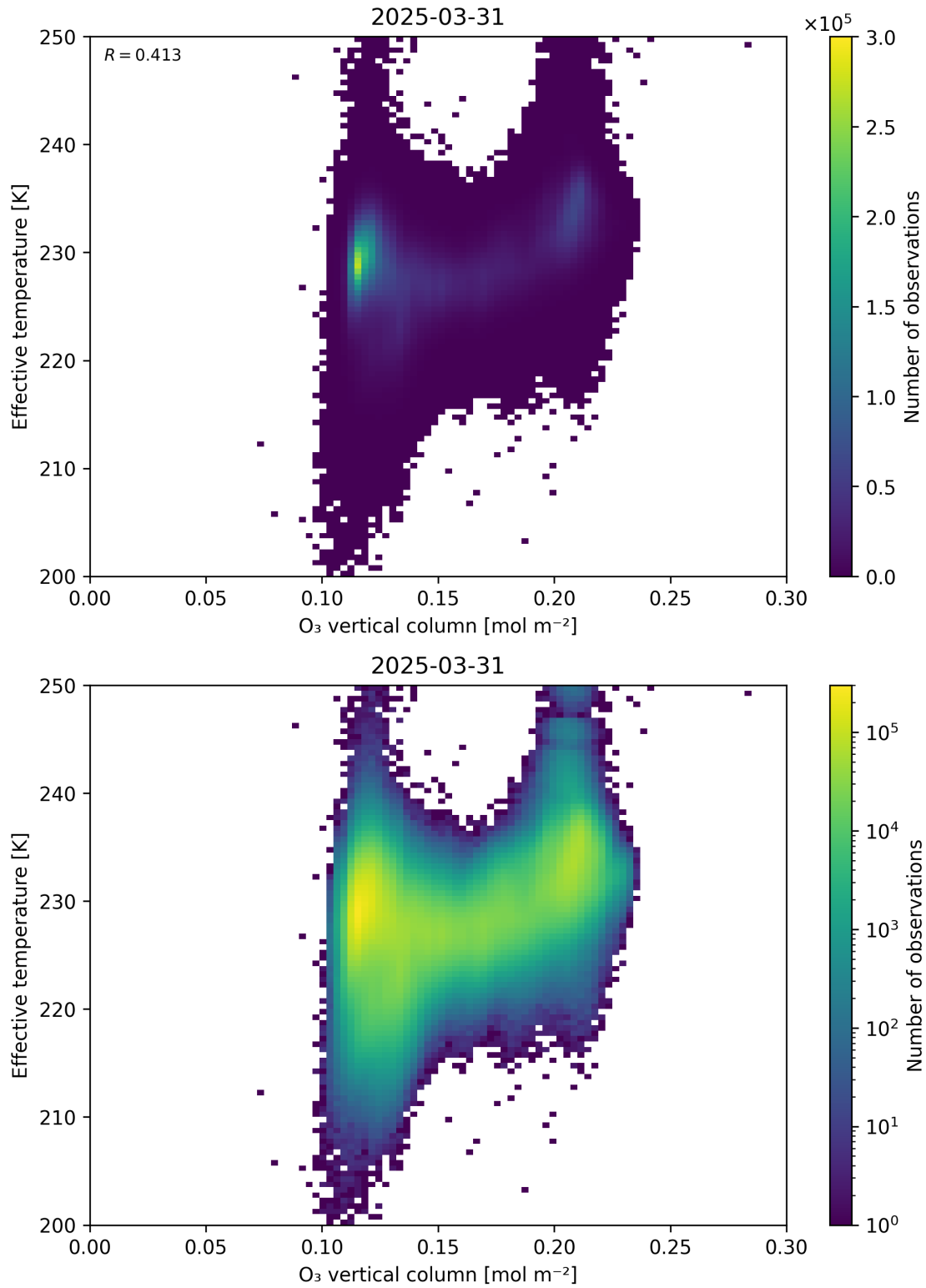
Figure 39: Scatter density plot of “O 3 vertical column” against “Effective temperature” for 2025-03-30 to 2025-04-01.
