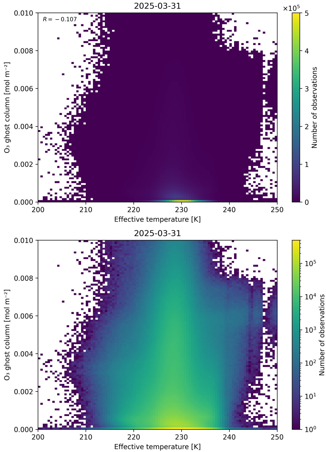
Figure 38: Scatter density plot of “Effective temperature” against “O 3 ghost column” for 2025-03-30 to 2025-04-01.
