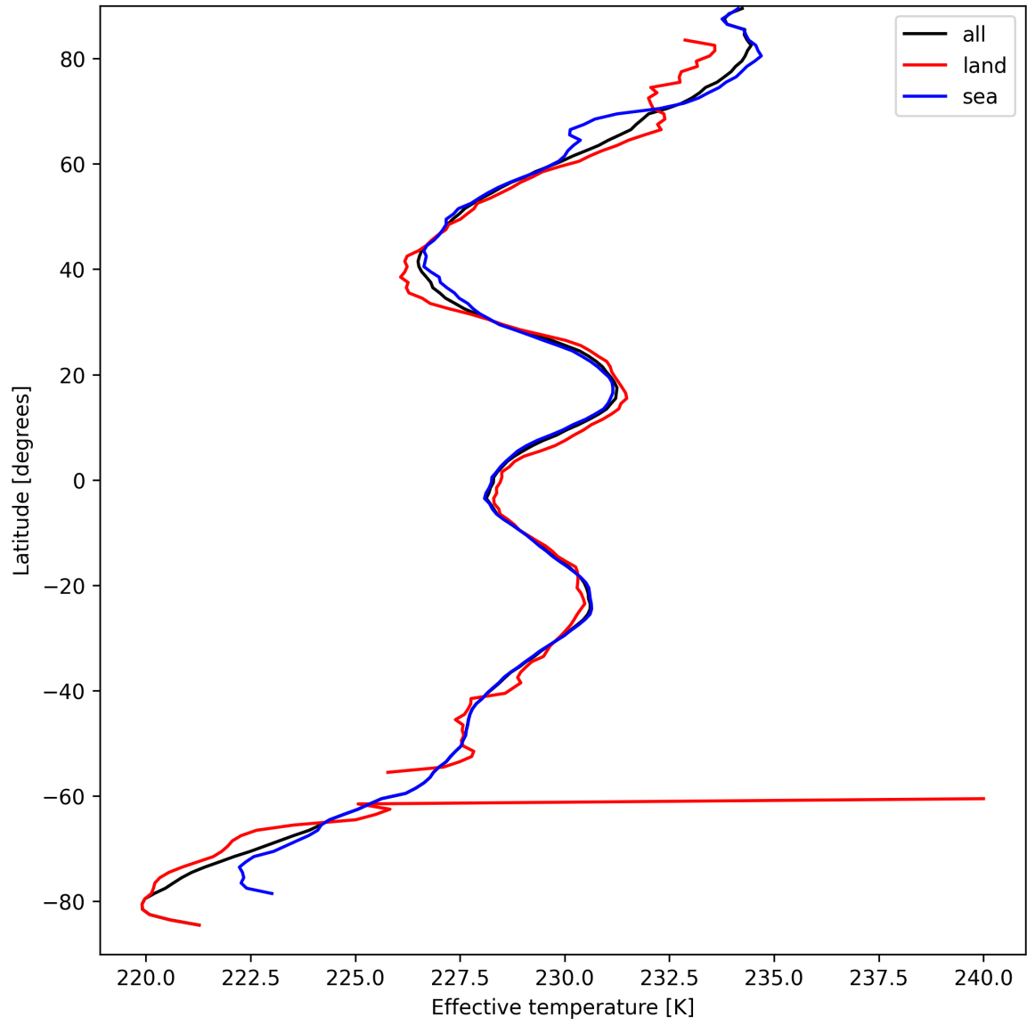
Figure 17: Zonal average of “Effective temperature” for 2025-03-30 to 2025-04-01.
