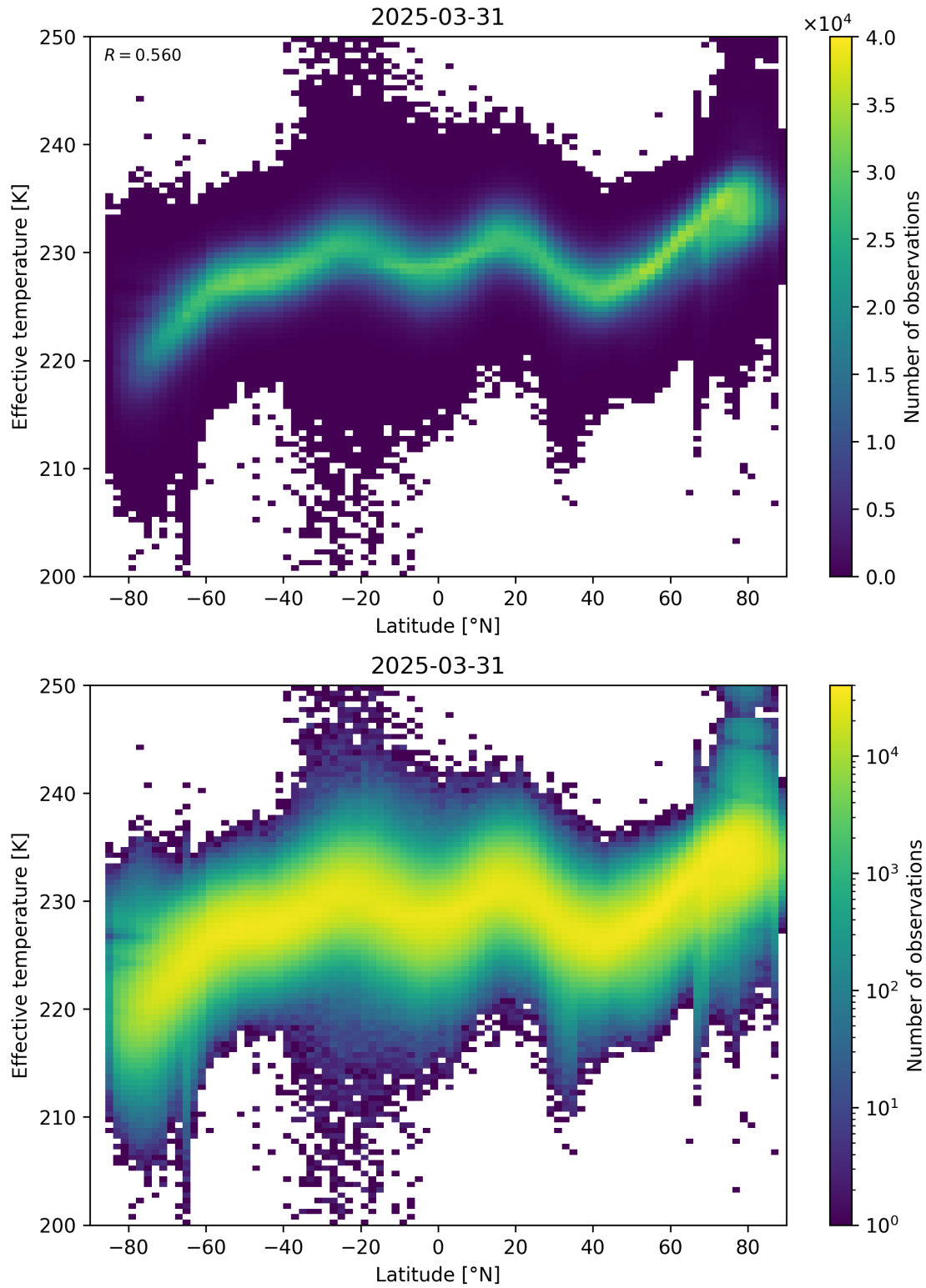
Figure 34: Scatter density plot of “Latitude” against “Effective temperature” for 2025-03-30 to 2025-04-01.
