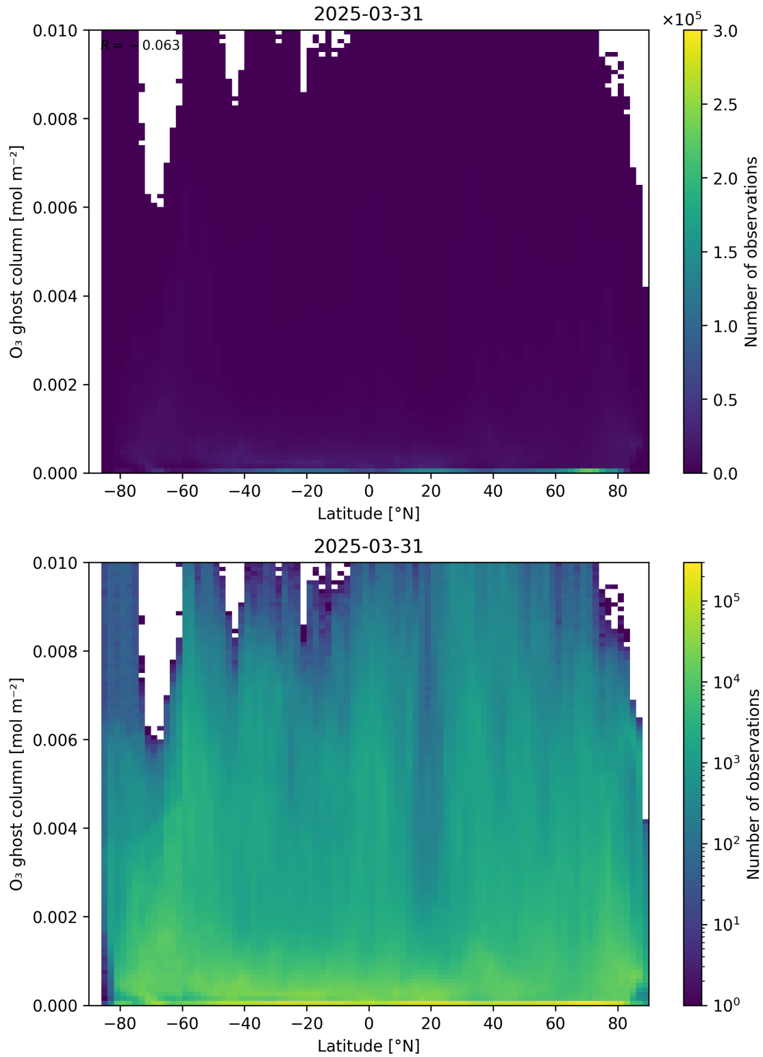
Figure 35: Scatter density plot of “Latitude” against “O 3 ghost column” for 2025-03-30 to 2025-04-01.
