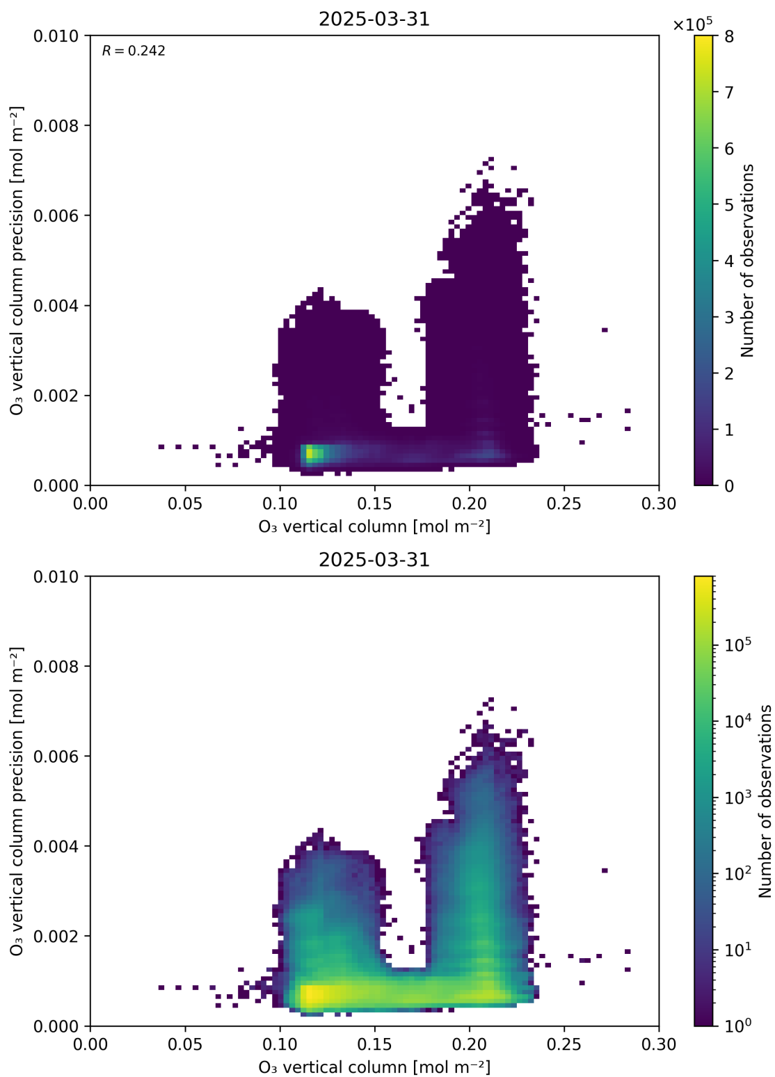
Figure 41: Scatter density plot of “O 3 vertical column” against “O 3 vertical column precision” for 2025-03-30 to 2025-04-01.
