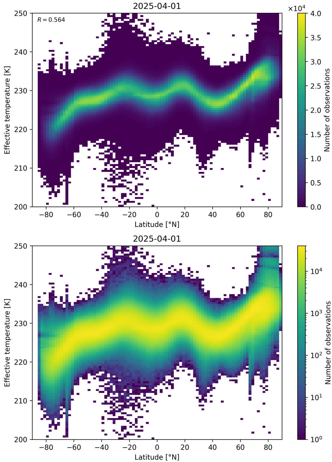
Figure 34: Scatter density plot of “Latitude” against “Effective temperature” for 2025-03-31 to 2025-04-02.
