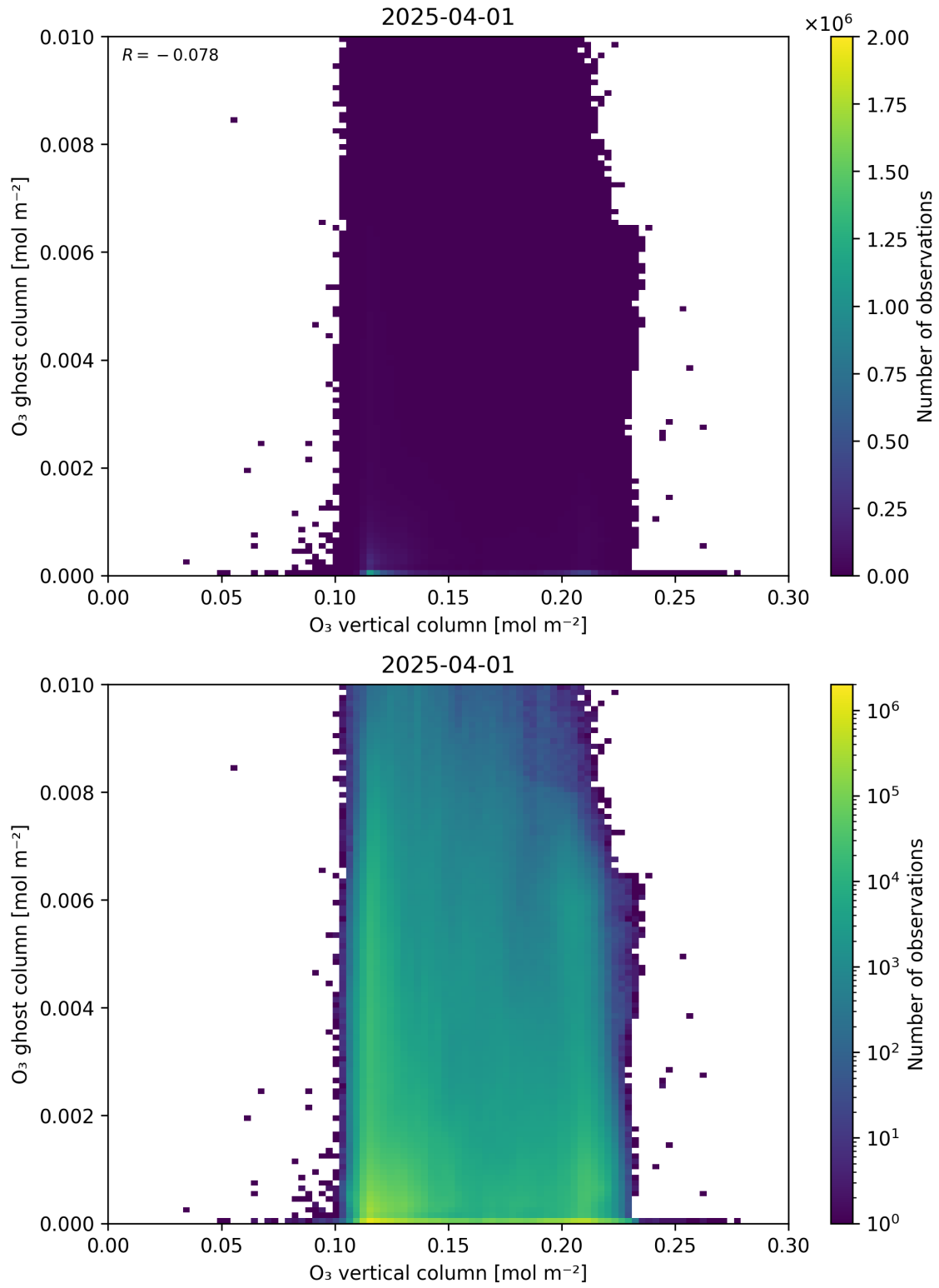
Figure 40: Scatter density plot of “O 3 vertical column” against “O 3 ghost column” for 2025-03-31 to 2025-04-02.
