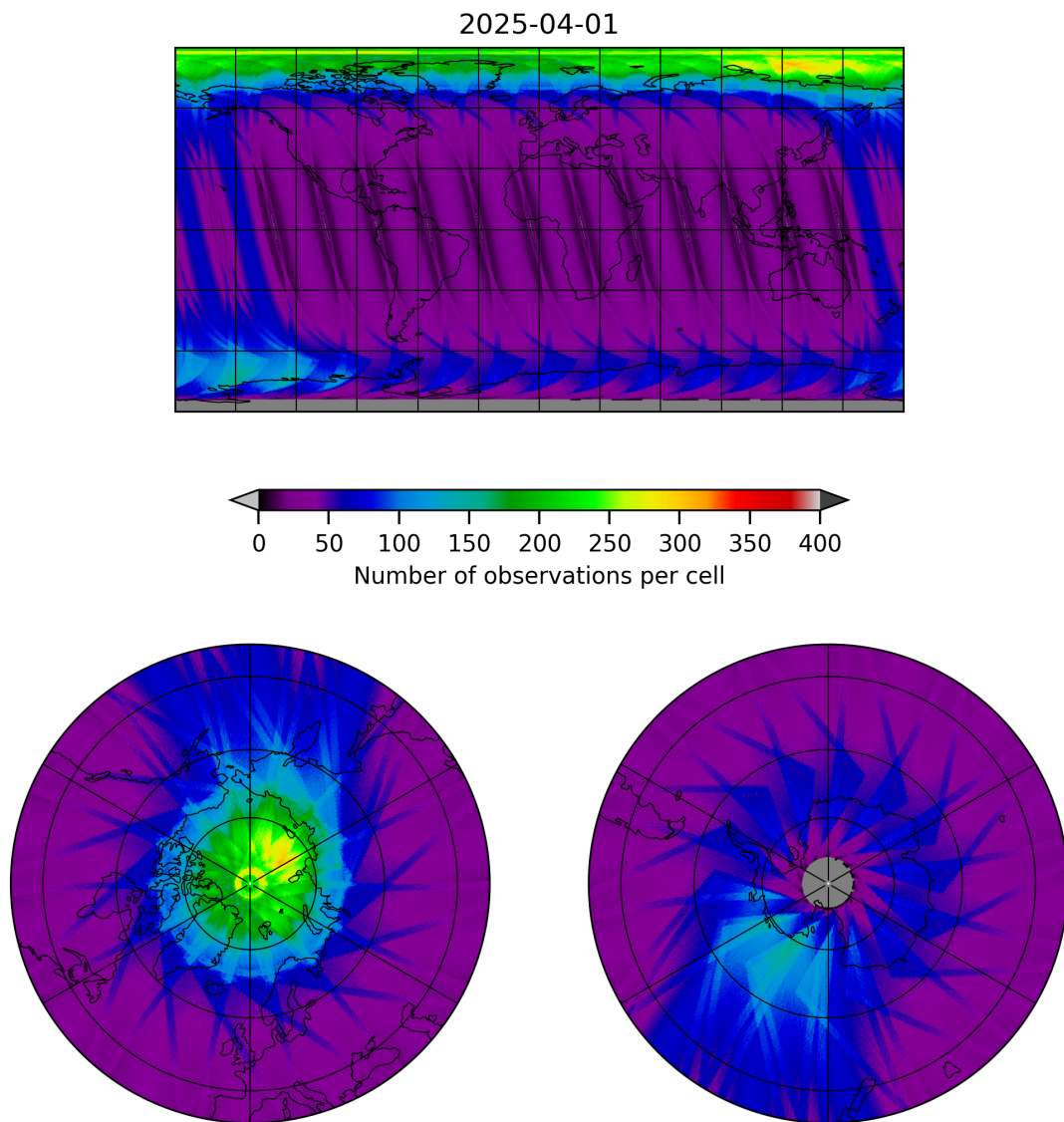
Figure 12: Map of the number of observations for 2025-03-31 to 2025-04-02
