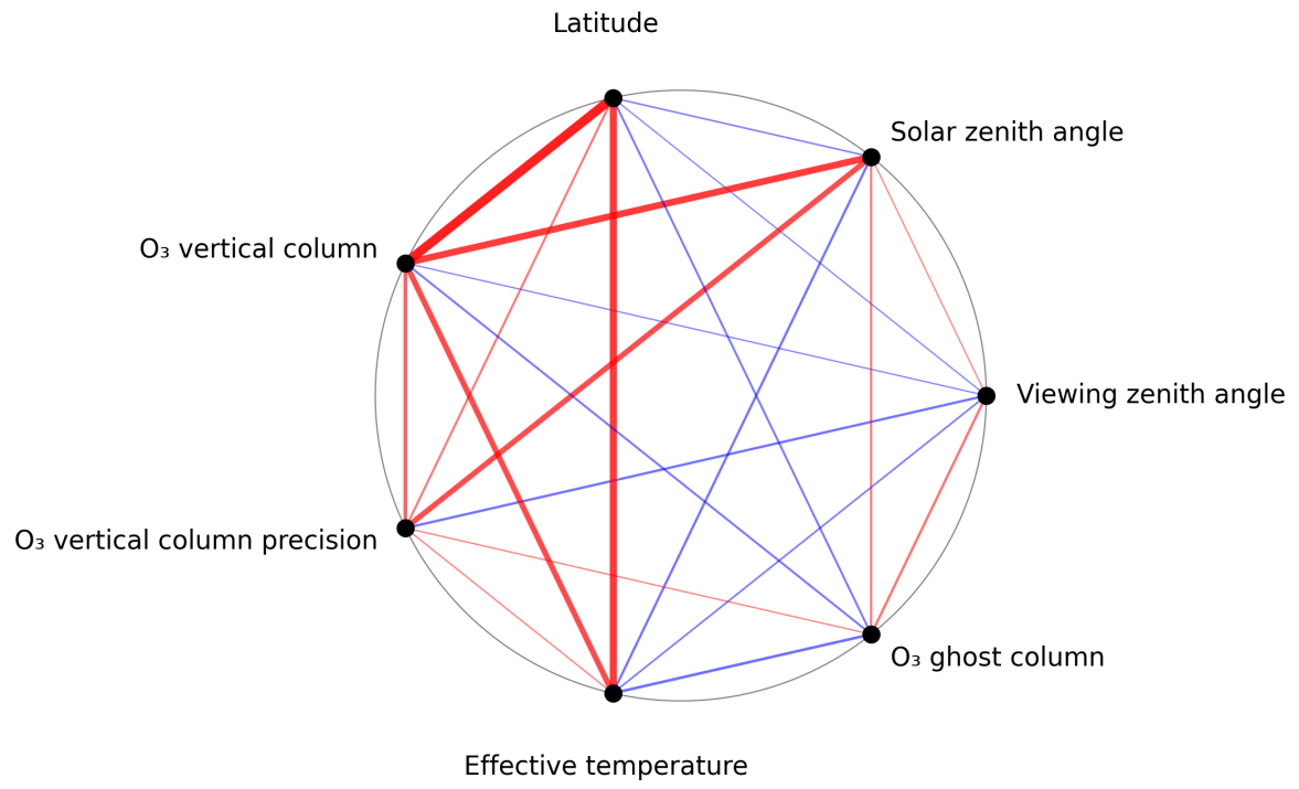
Figure 1: Map of correlation graph for 2025-03-31 to 2025-04-02.
