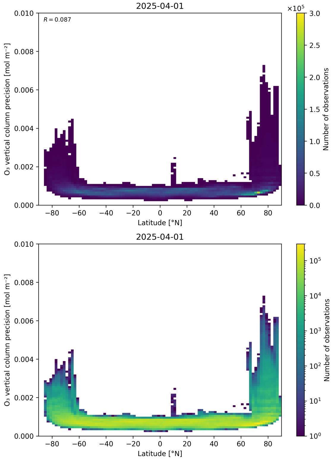
Figure 37: Scatter density plot of “Latitude” against “O 3 vertical column precision” for 2025-03-31 to 2025-04-02.
