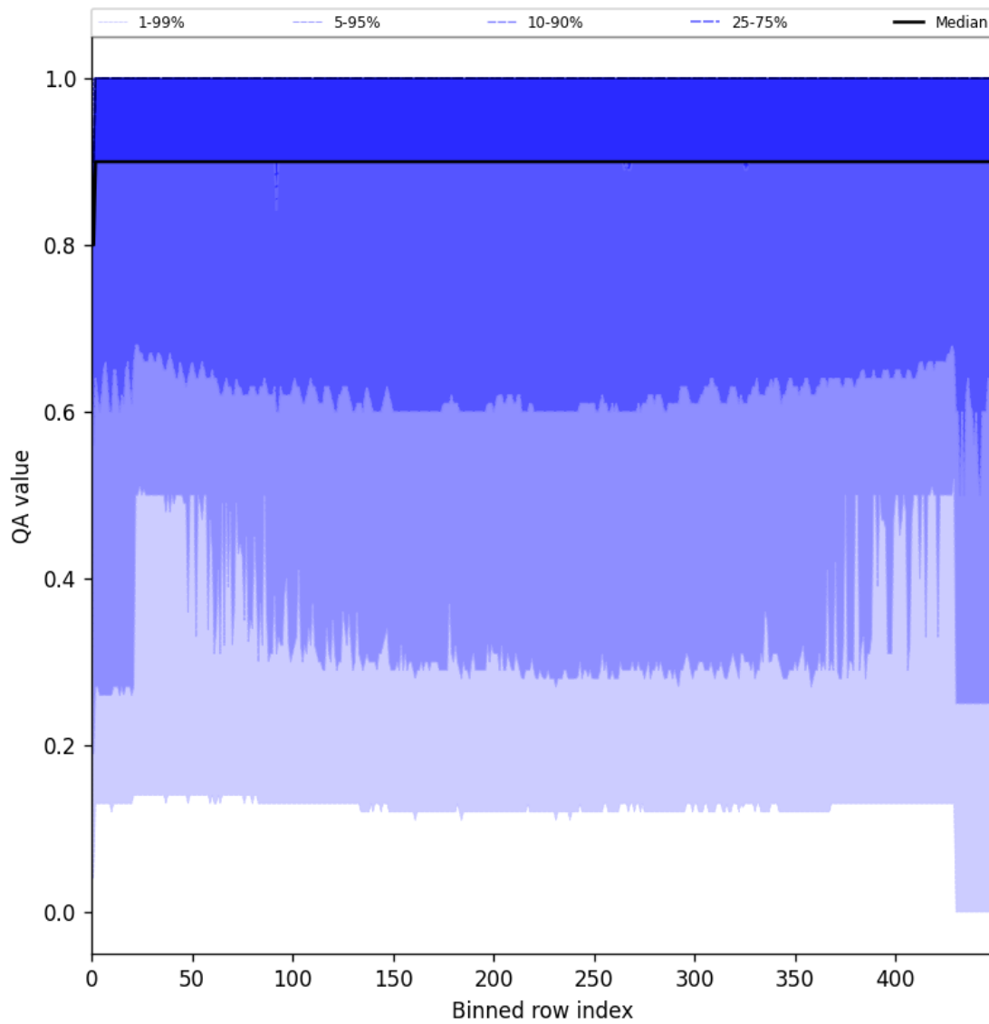
Figure 27: Along track statistics of “QA value” for 2025-03-31 to 2025-04-02
