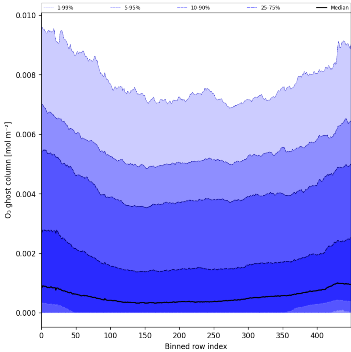
Figure 32: Along track statistics of “O 3 ghost column” for 2025-03-31 to 2025-04-02
