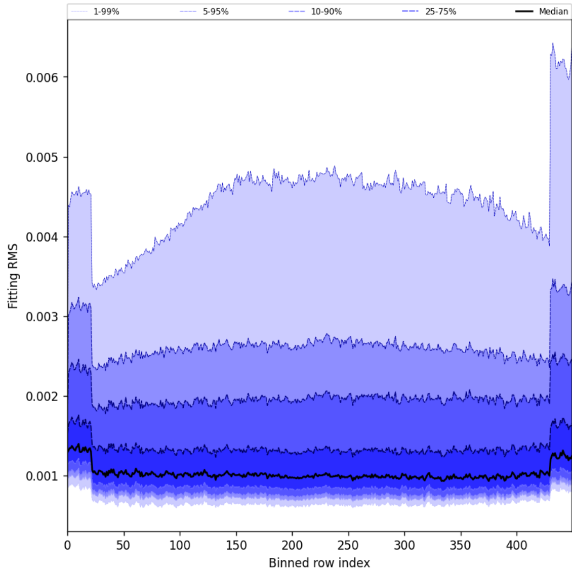
Figure 30: Along track statistics of “Fitting RMS” for 2025-03-31 to 2025-04-02
