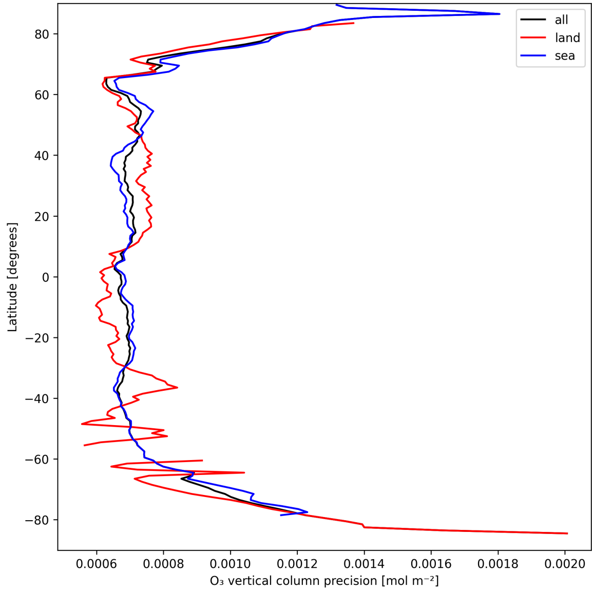
Figure 15: Zonal average of “O 3 vertical column precision” for 2025-03-31 to 2025-04-02.
