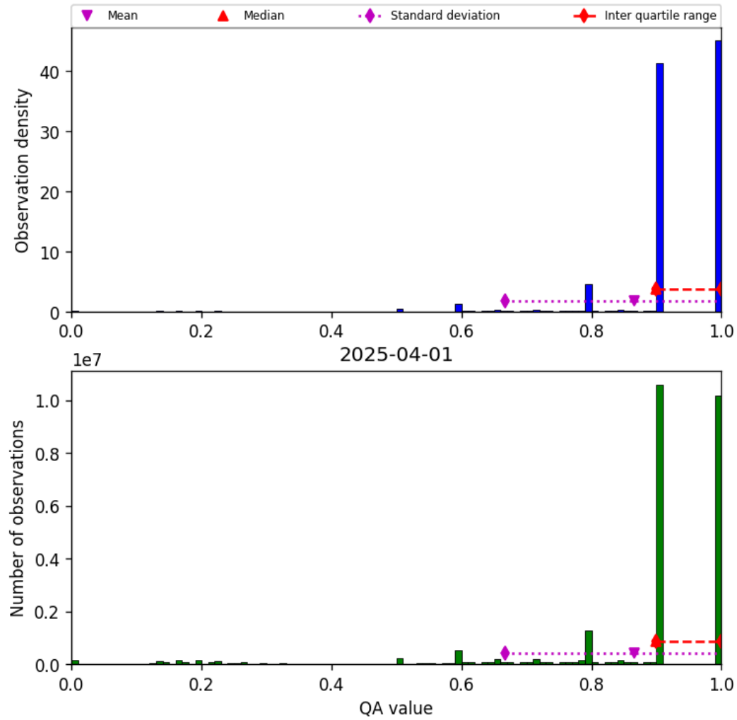
Figure 20: Histogram of “QA value” for 2025-03-31 to 2025-04-02
