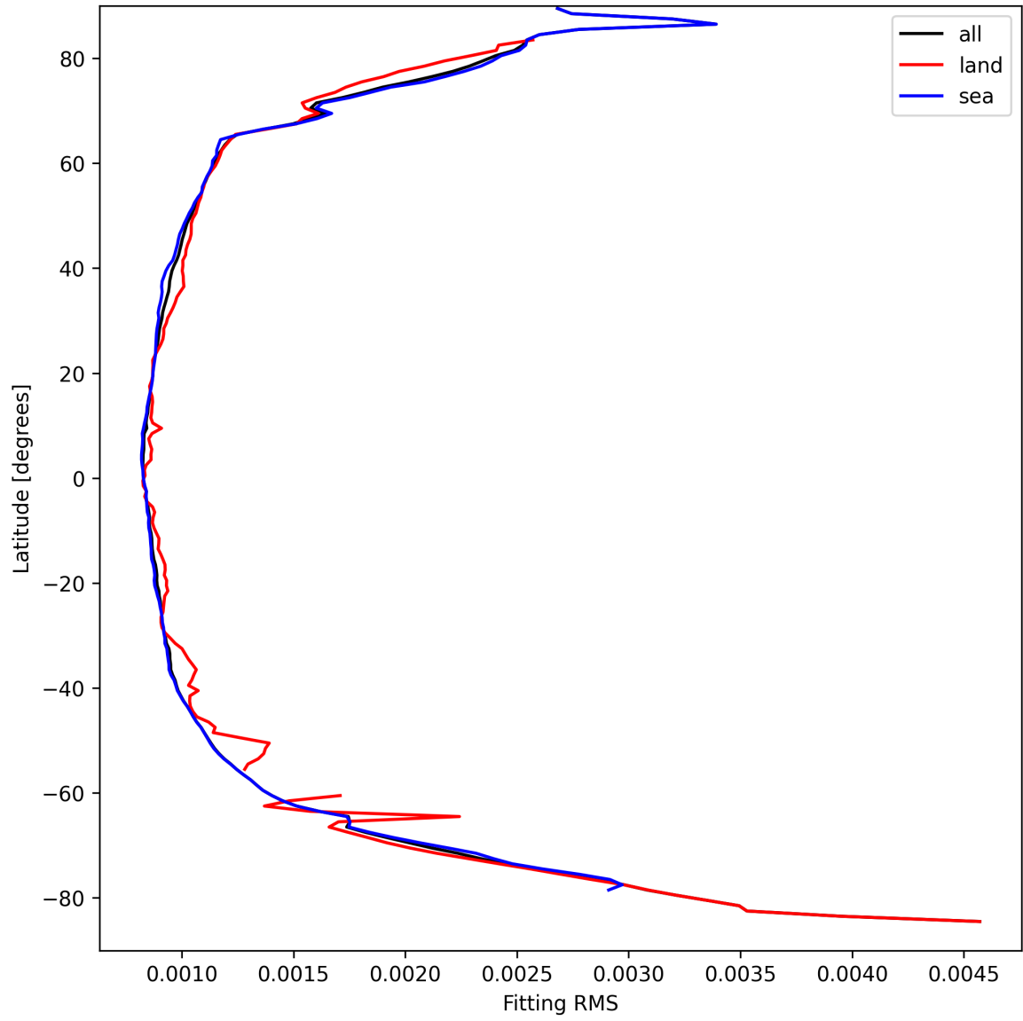
Figure 16: Zonal average of “Fitting RMS” for 2025-03-31 to 2025-04-02.
