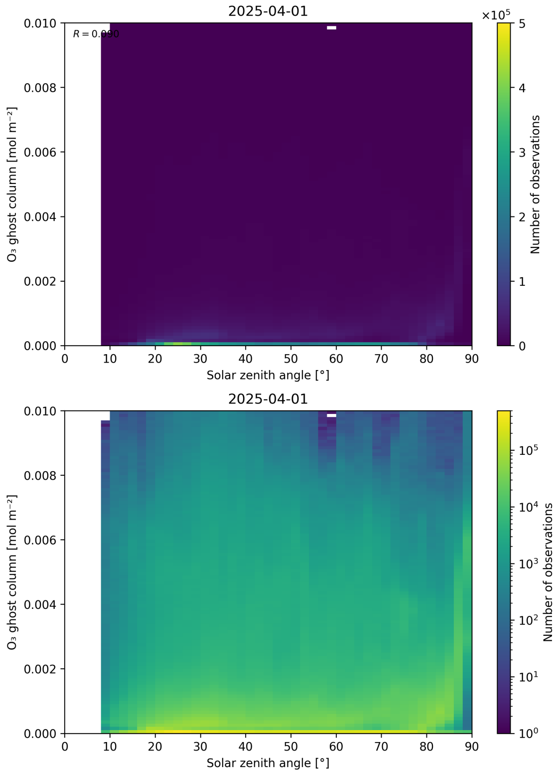
Figure 46: Scatter density plot of “Solar zenith angle” against “O 3 ghost column” for 2025-03-31 to 2025-04-02.
