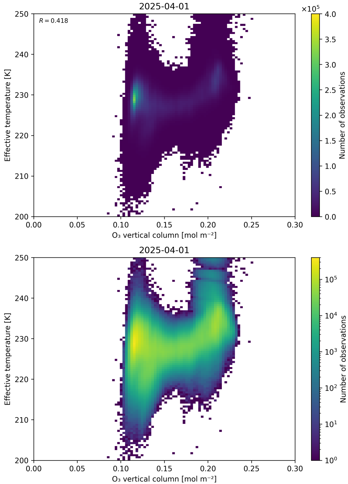
Figure 39: Scatter density plot of “O 3 vertical column” against “Effective temperature” for 2025-03-31 to 2025-04-02.
