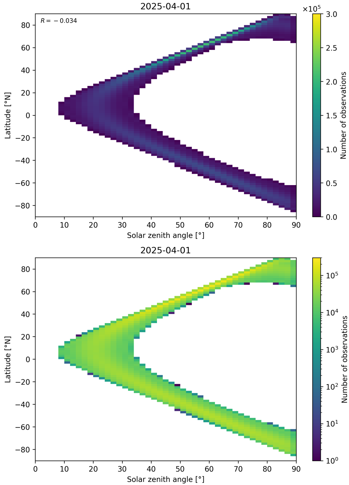
Figure 44: Scatter density plot of “Solar zenith angle” against “Latitude” for 2025-03-31 to 2025-04-02.
