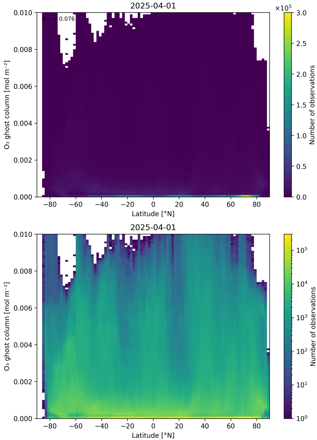
Figure 35: Scatter density plot of “Latitude” against “O 3 ghost column” for 2025-03-31 to 2025-04-02.
