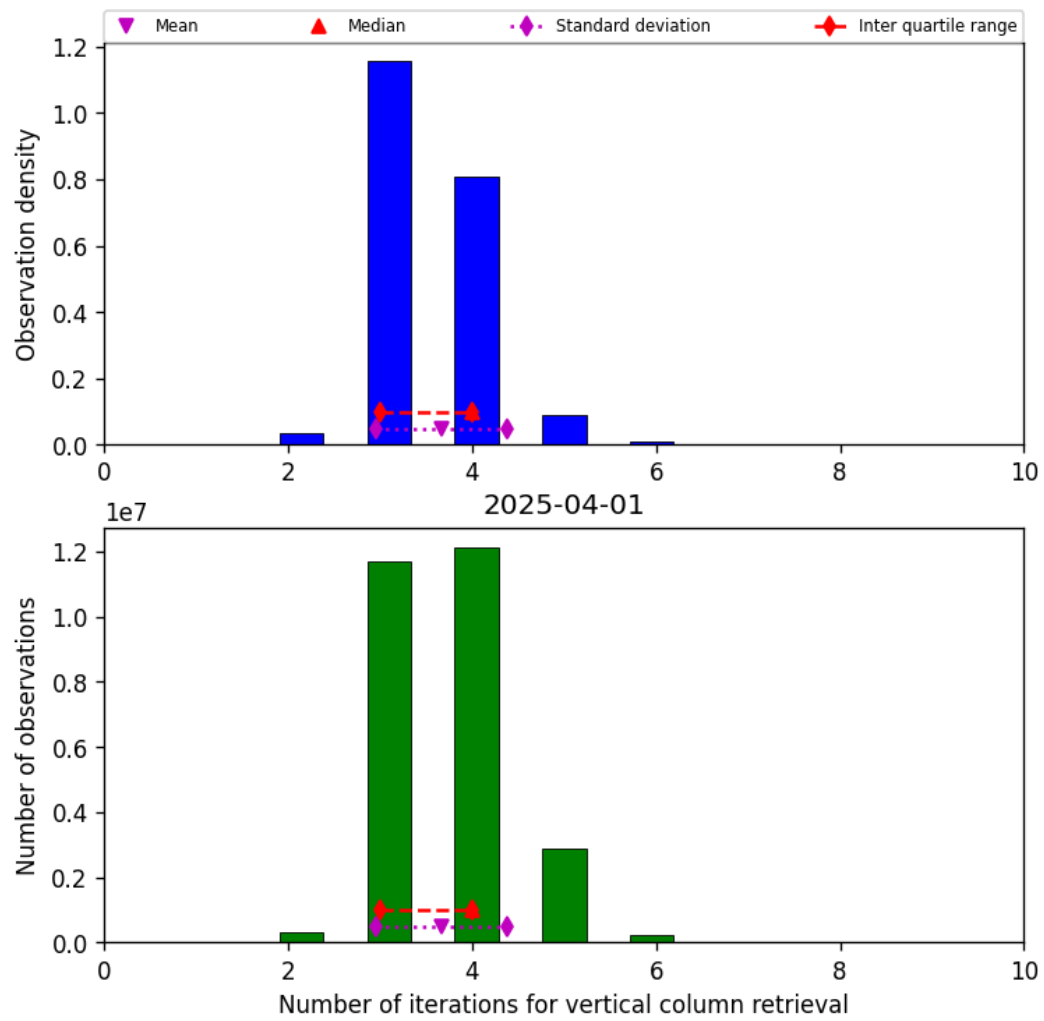
Figure 26: Histogram of “Number of iterations for vertical column retrieval” for 2025-03-31 to 2025-04-02
