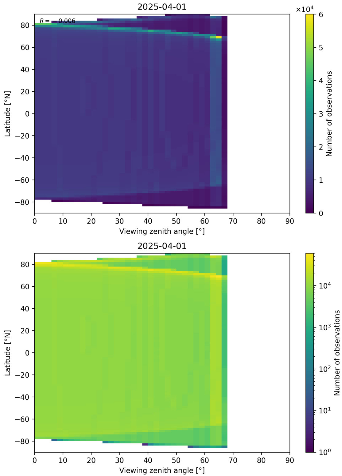
Figure 49: Scatter density plot of “Viewing zenith angle” against “Latitude” for 2025-03-31 to 2025-04-02.
