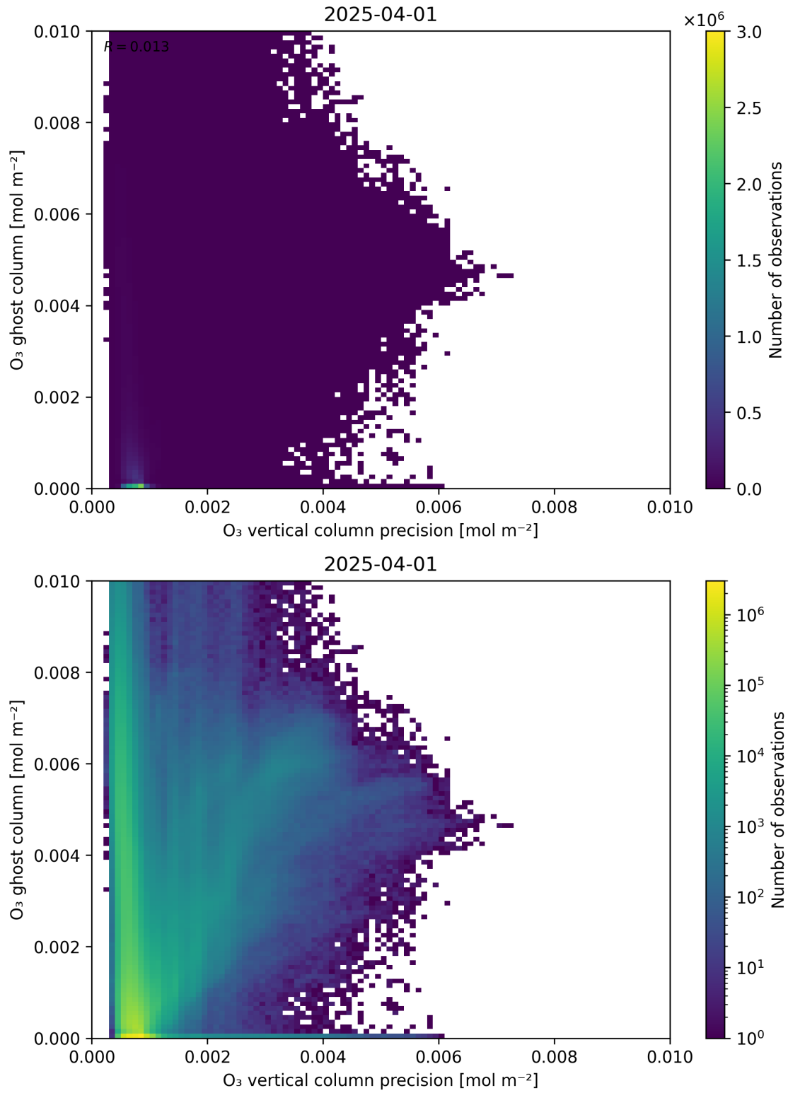
Figure 43: Scatter density plot of “O 3 vertical column precision” against “O 3 ghost column” for 2025-03-31 to 2025-04-02.
