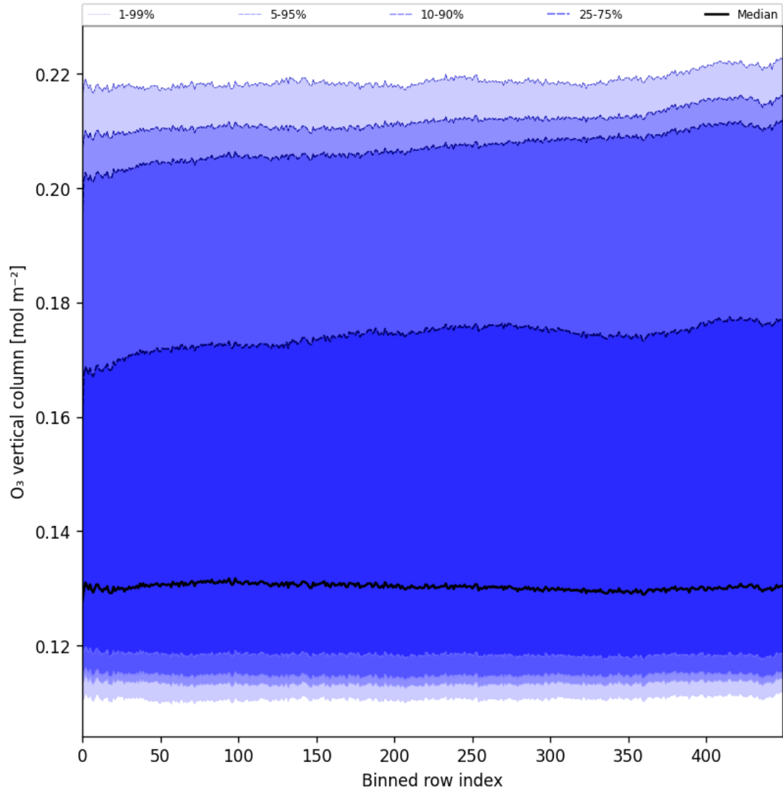
Figure 28: Along track statistics of “O 3 vertical column” for 2025-03-31 to 2025-04-02
