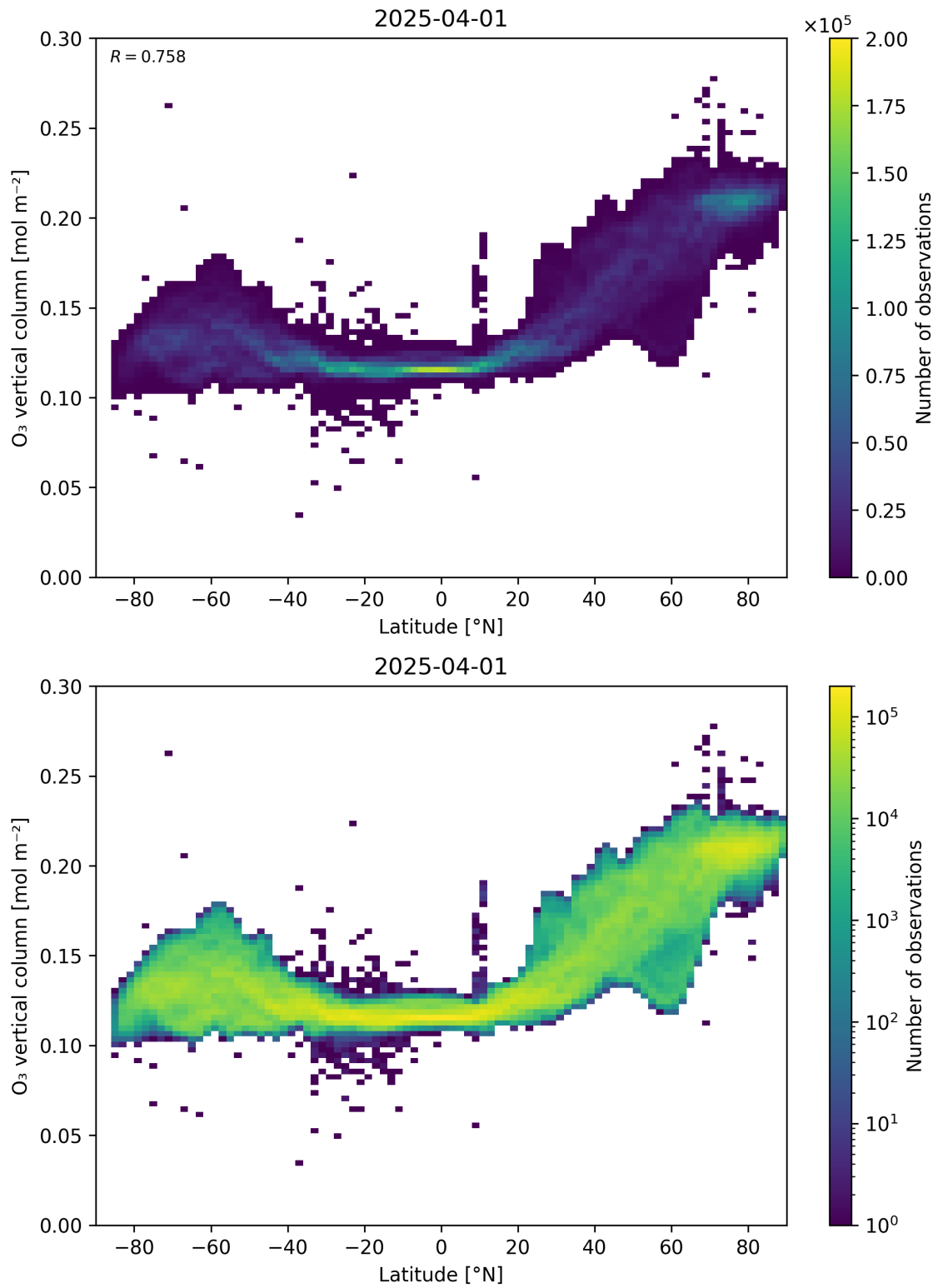
Figure 36: Scatter density plot of “Latitude” against “O 3 vertical column” for 2025-03-31 to 2025-04-02.
