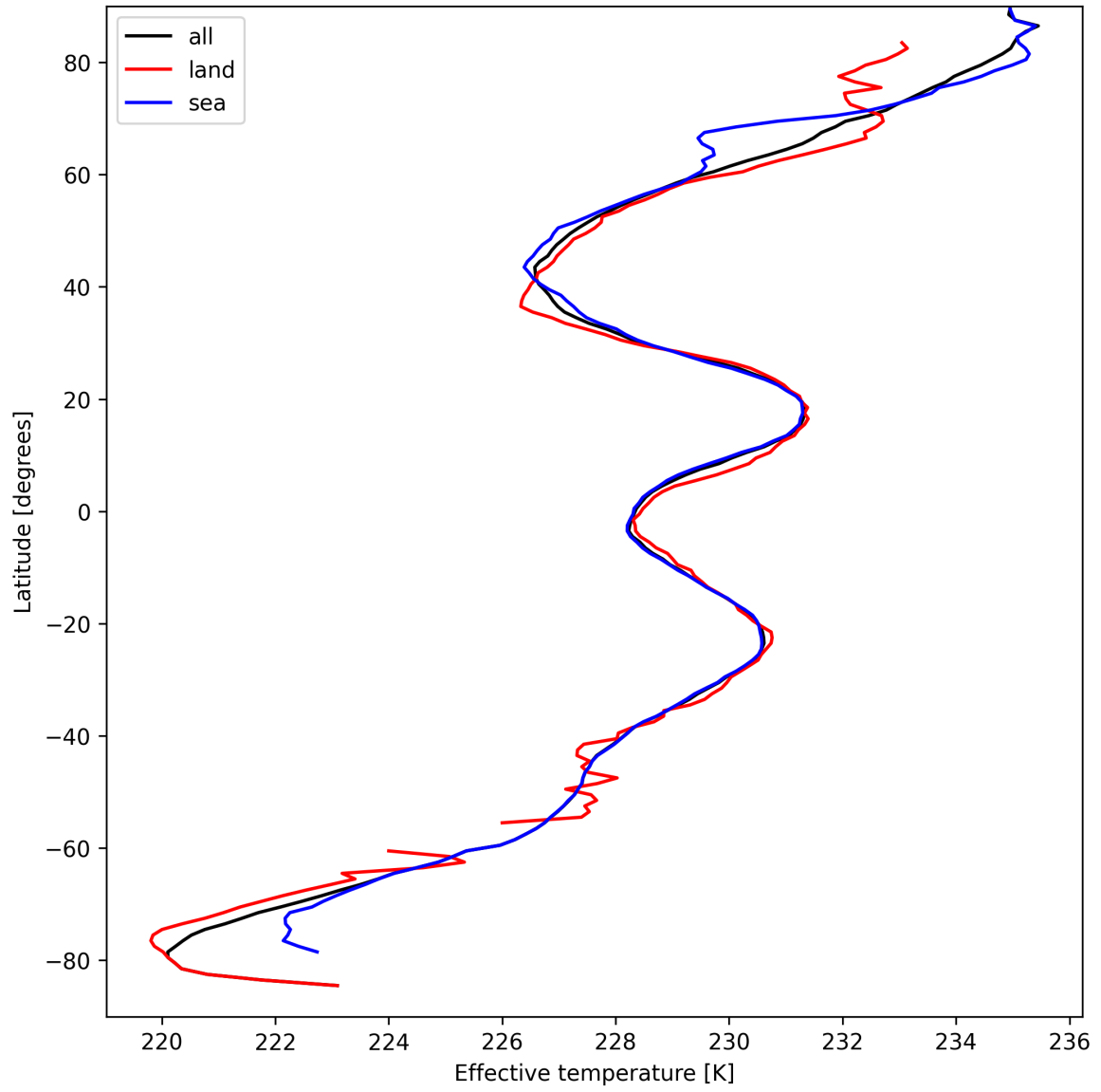
Figure 17: Zonal average of "Effective temperature" for 2025-03-31 to 2025-04-02.
