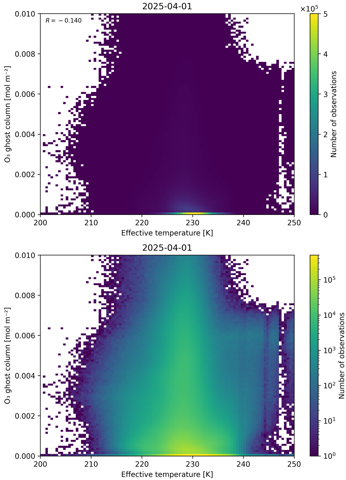
Figure 38: Scatter density plot of “Effective temperature” against “O 3 ghost column” for 2025-03-31 to 2025-04-02.
