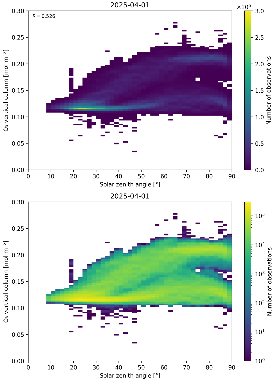
Figure 47: Scatter density plot of “Solar zenith angle” against “O 3 vertical column” for 2025-03-31 to 2025-04-02.
