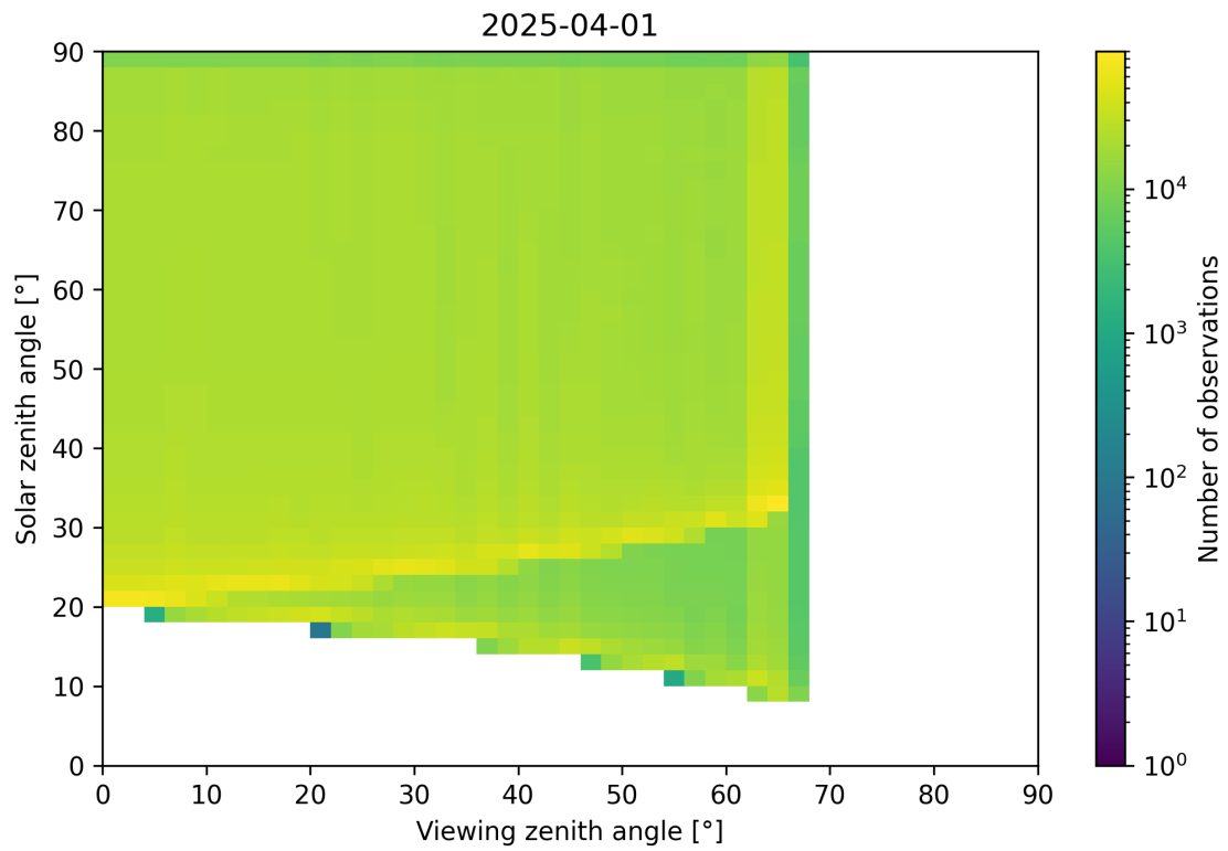
Figure 54: Scatter density plot of “Viewing zenith angle” against “Solar zenith angle” for 2025-03-31 to 2025-04-02.
