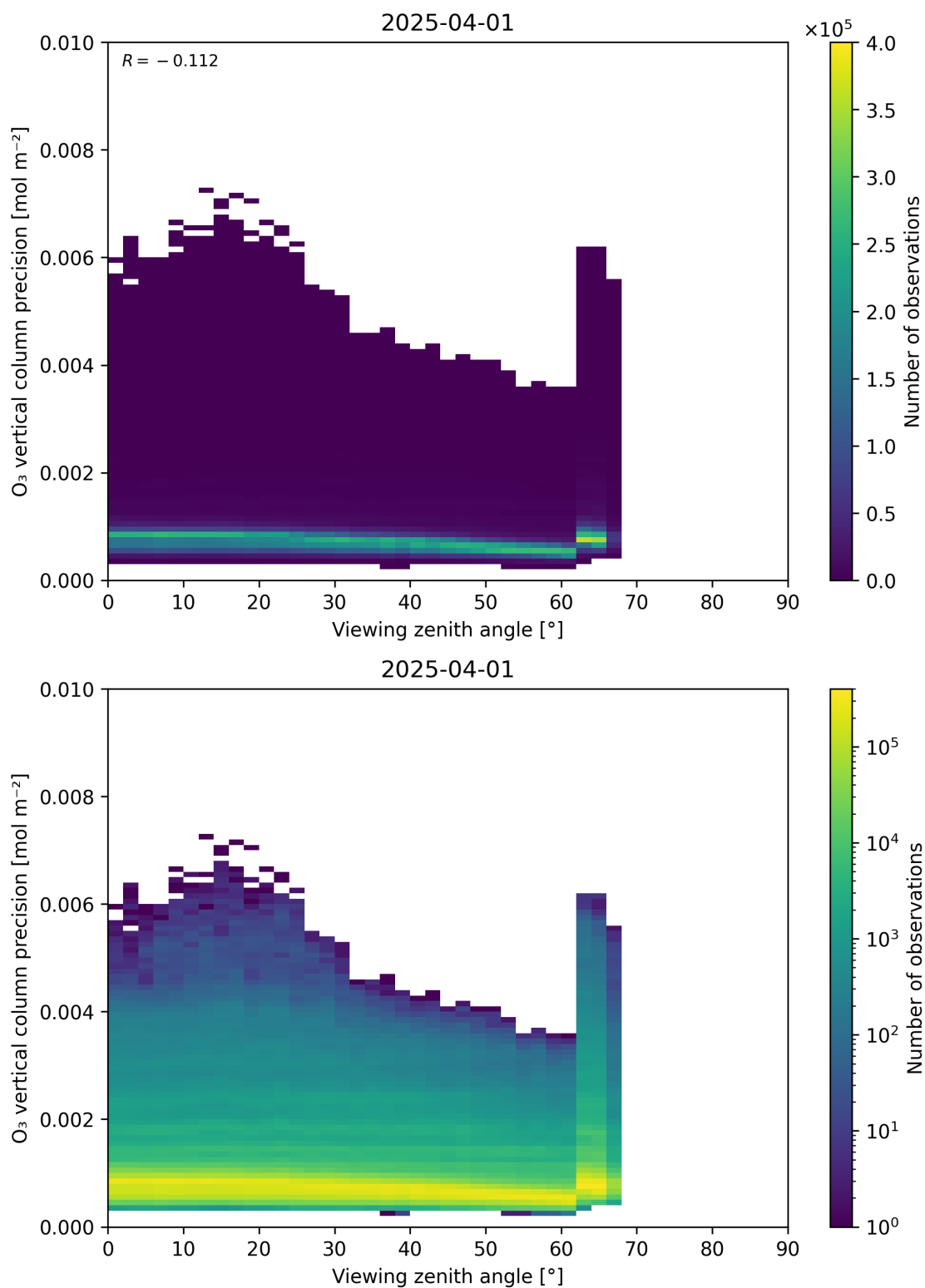
Figure 53: Scatter density plot of “Viewing zenith angle” against “O 3 vertical column precision” for 2025-03-31 to 2025-04-02.
