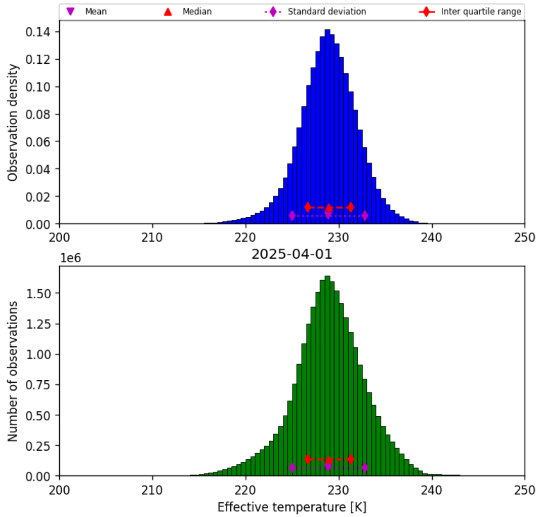
Figure 24: Histogram of “Effective temperature” for 2025-03-31 to 2025-04-02
