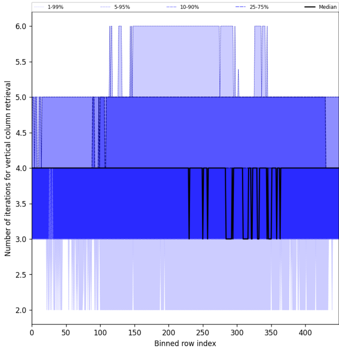
Figure 33: Along track statistics of “Number of iterations for vertical column retrieval” for 2025-03-31 to 2025-04-02
