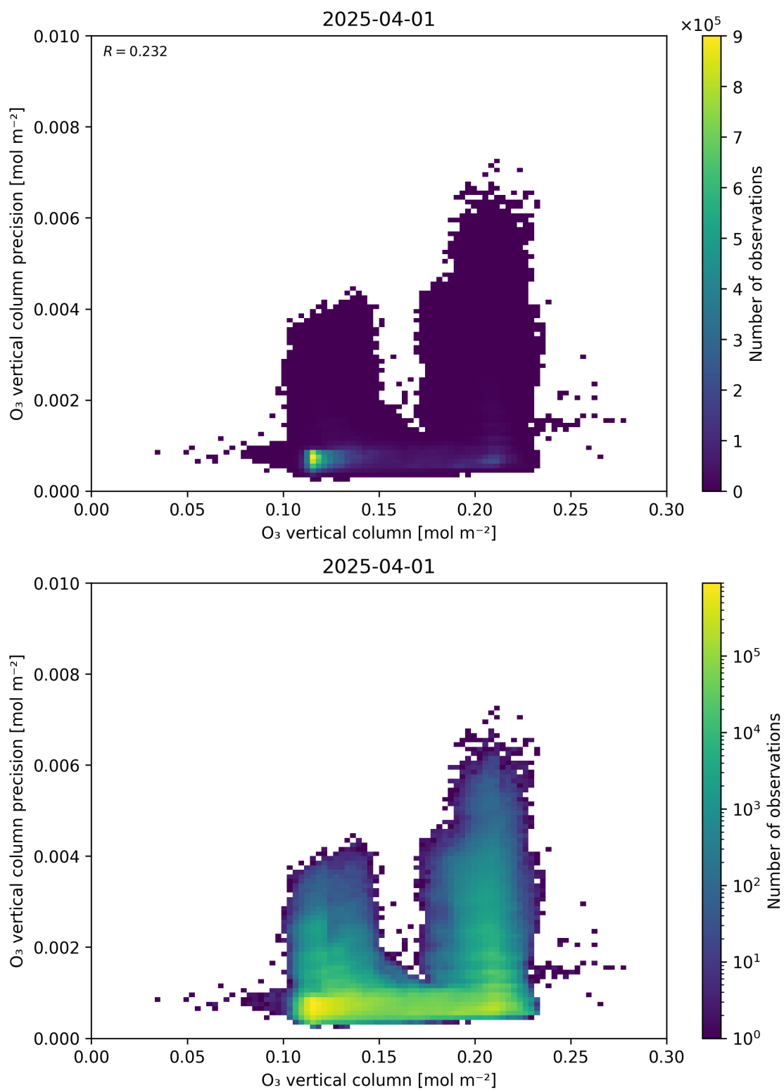
Figure 41: Scatter density plot of “O 3 vertical column” against “O 3 vertical column precision” for 2025-03-31 to 2025-04-02.
