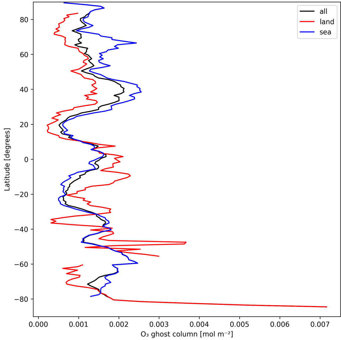
Figure 18: Zonal average of “O 3 ghost column” for 2025-03-31 to 2025-04-02.
