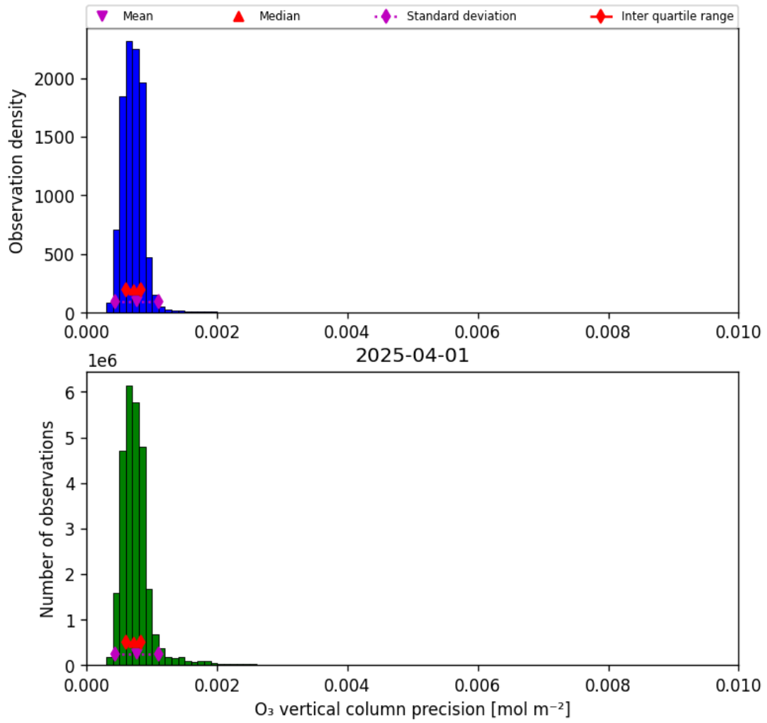
Figure 22: Histogram of “O 3 vertical column precision” for 2025-03-31 to 2025-04-02
