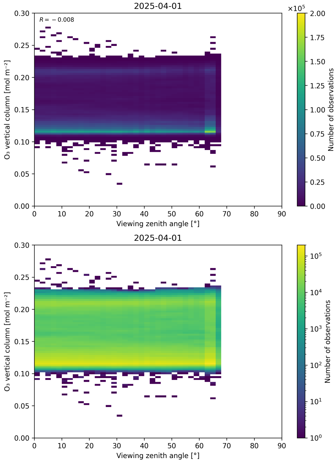
Figure 52: Scatter density plot of “Viewing zenith angle” against “O 3 vertical column” for 2025-03-31 to 2025-04-02.
