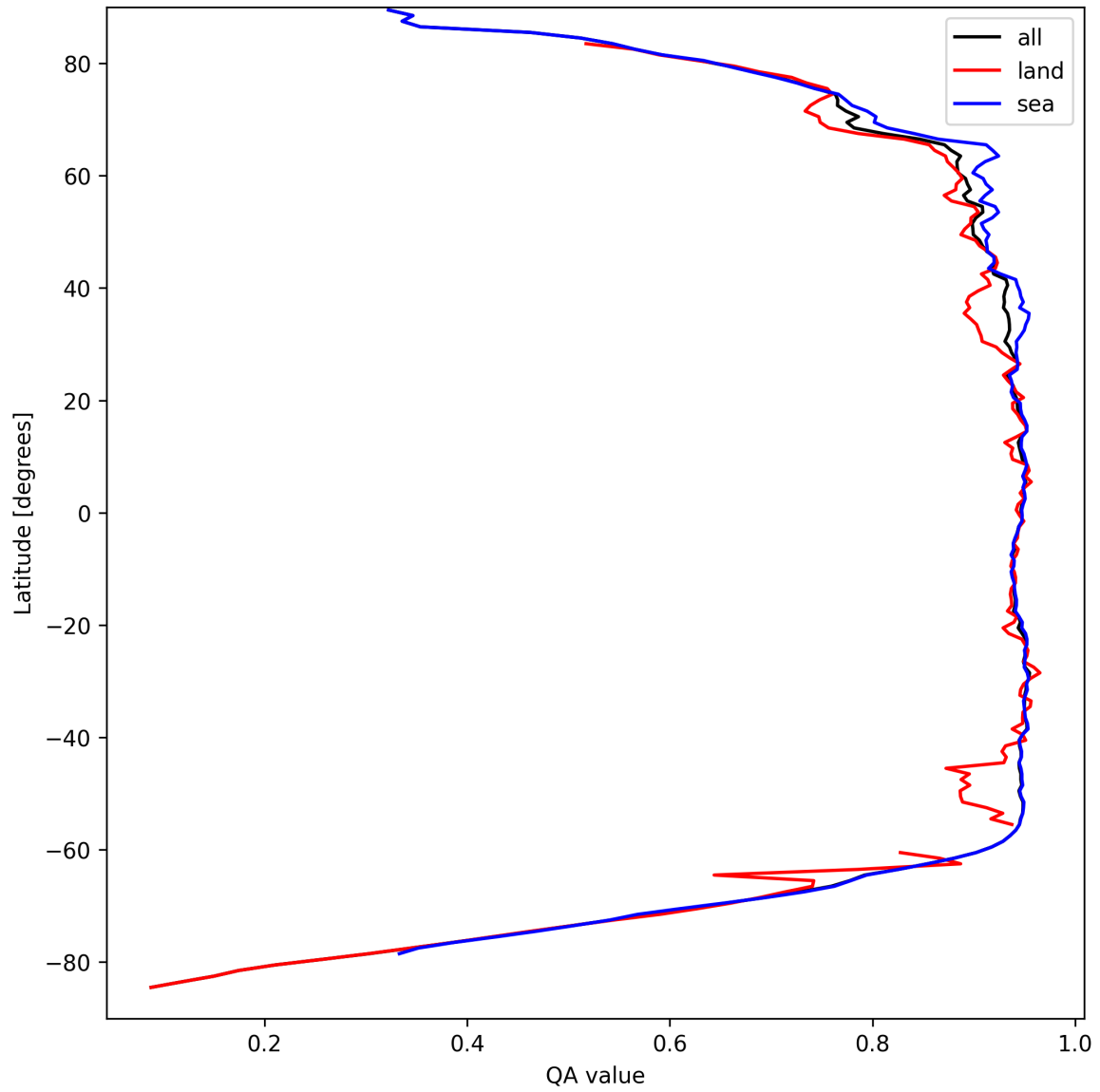
Figure 13: Zonal average of “QA value” for 2025-03-31 to 2025-04-02.
