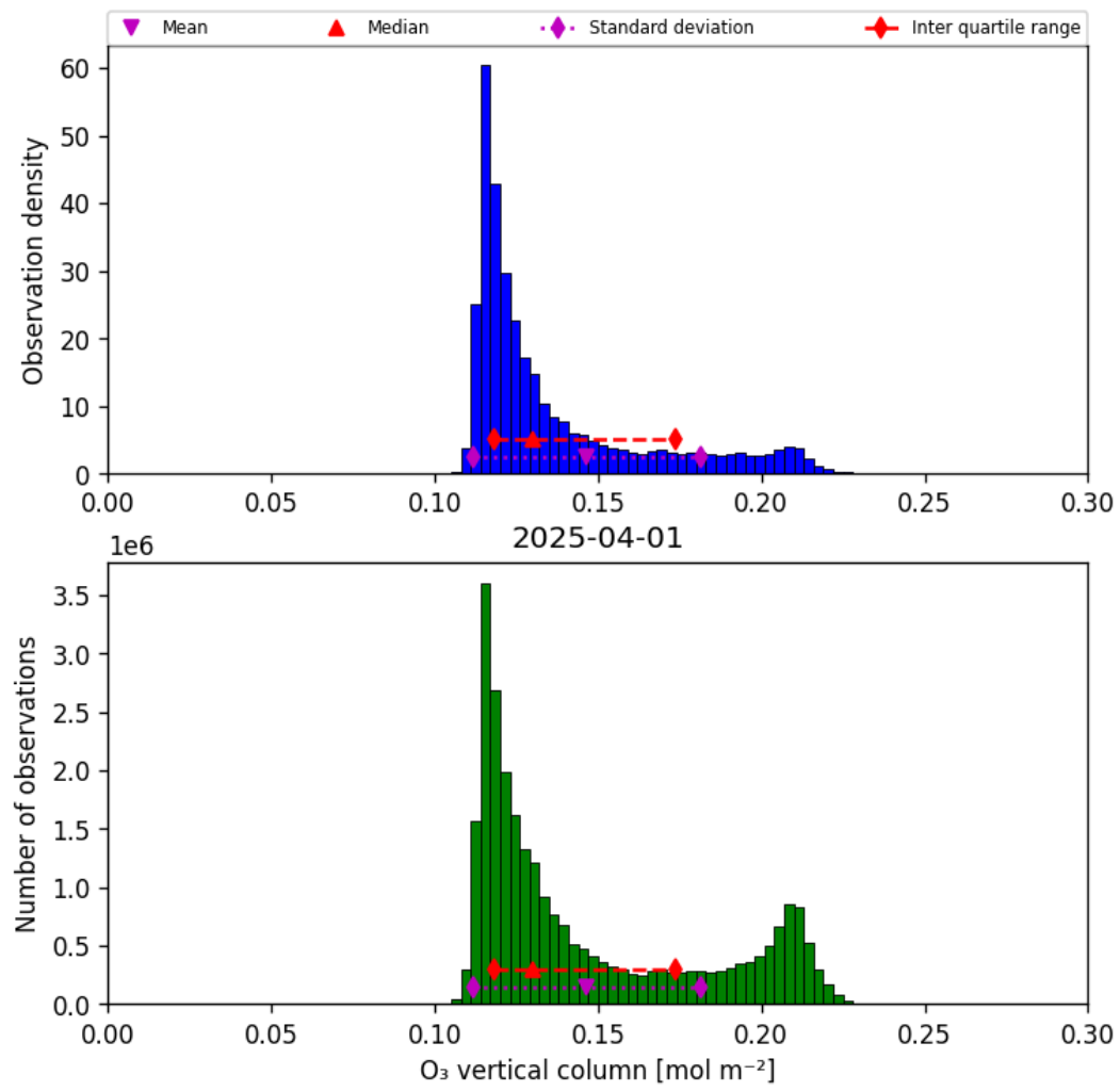
Figure 21: Histogram of “O 3 vertical column” for 2025-03-31 to 2025-04-02
