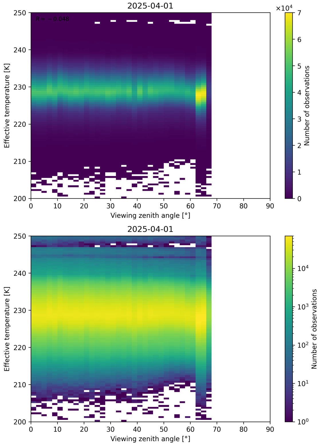
Figure 50: Scatter density plot of “Viewing zenith angle” against “Effective temperature” for 2025-03-31 to 2025-04-02.
