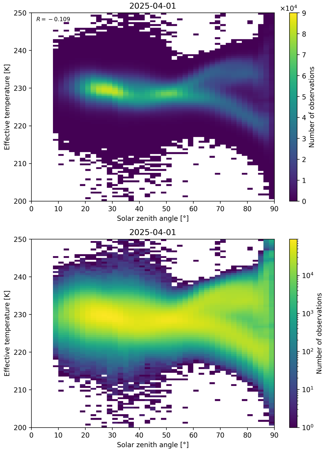
Figure 45: Scatter density plot of “Solar zenith angle” against “Effective temperature” for 2025-03-31 to 2025-04-02.
