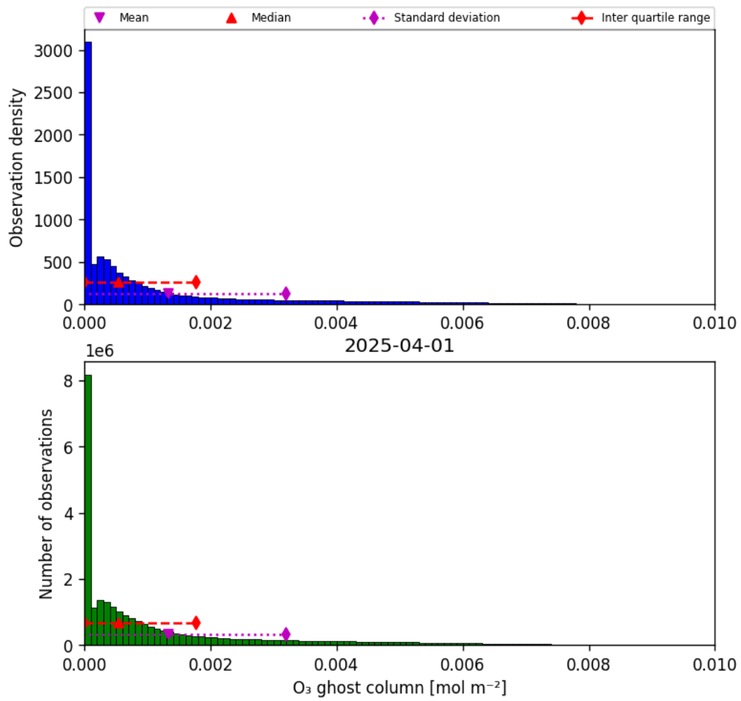
Figure 25: Histogram of “O 3 ghost column” for 2025-03-31 to 2025-04-02
