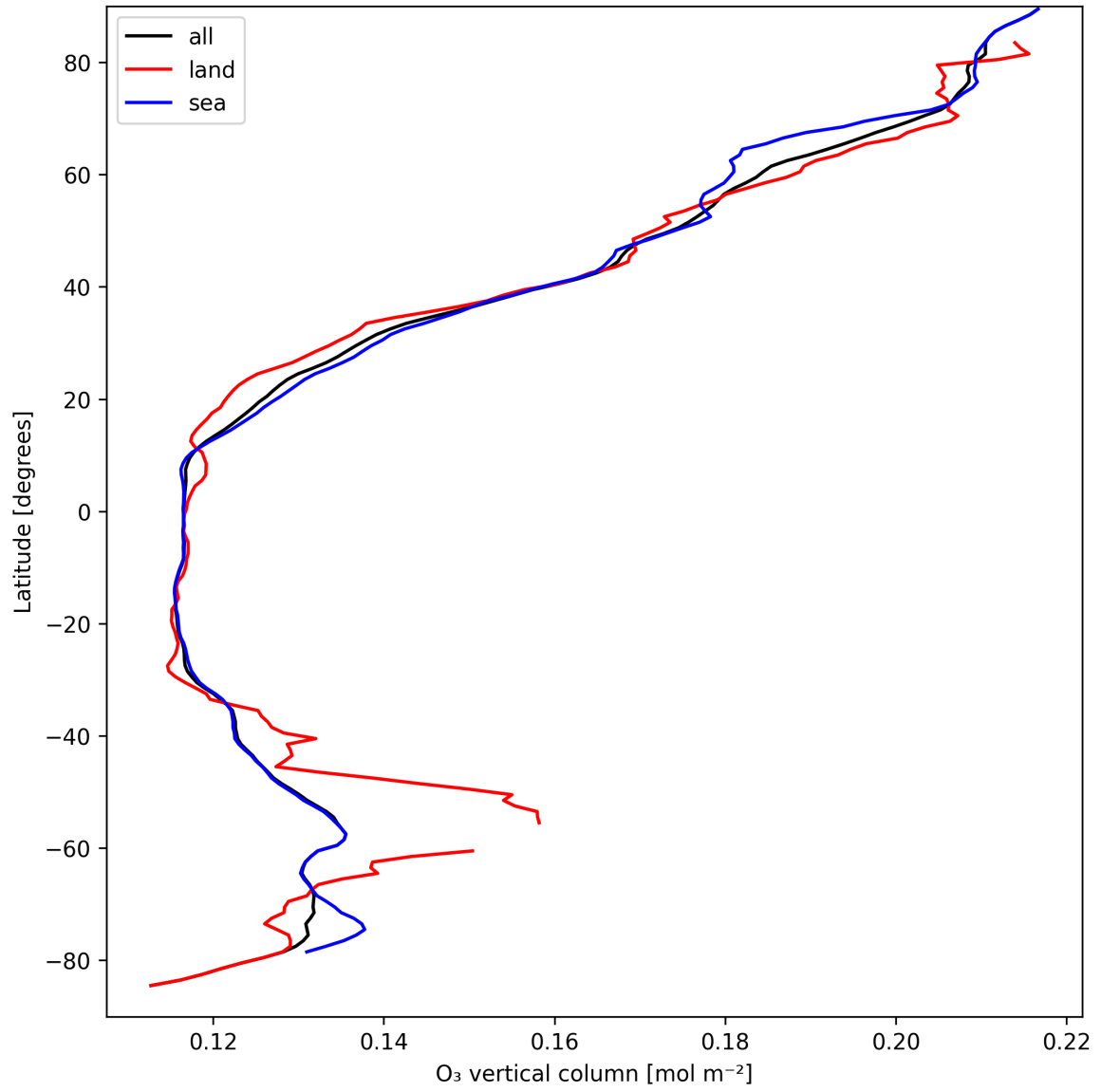
Figure 14: Zonal average of “O 3 vertical column” for 2025-03-31 to 2025-04-02.
