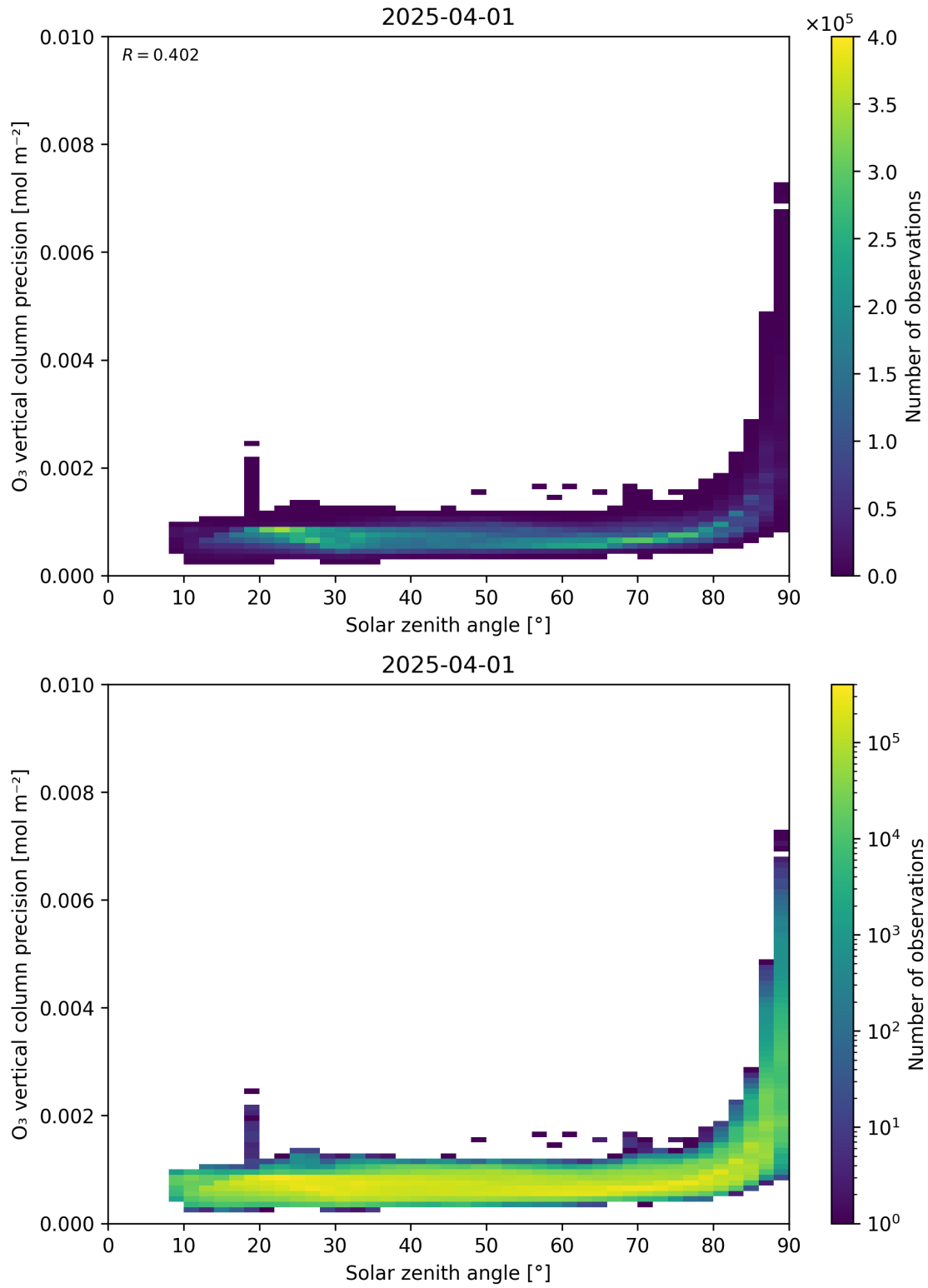
Figure 48: Scatter density plot of “Solar zenith angle” against “O 3 vertical column precision” for 2025-03-31 to 2025-04-02.
