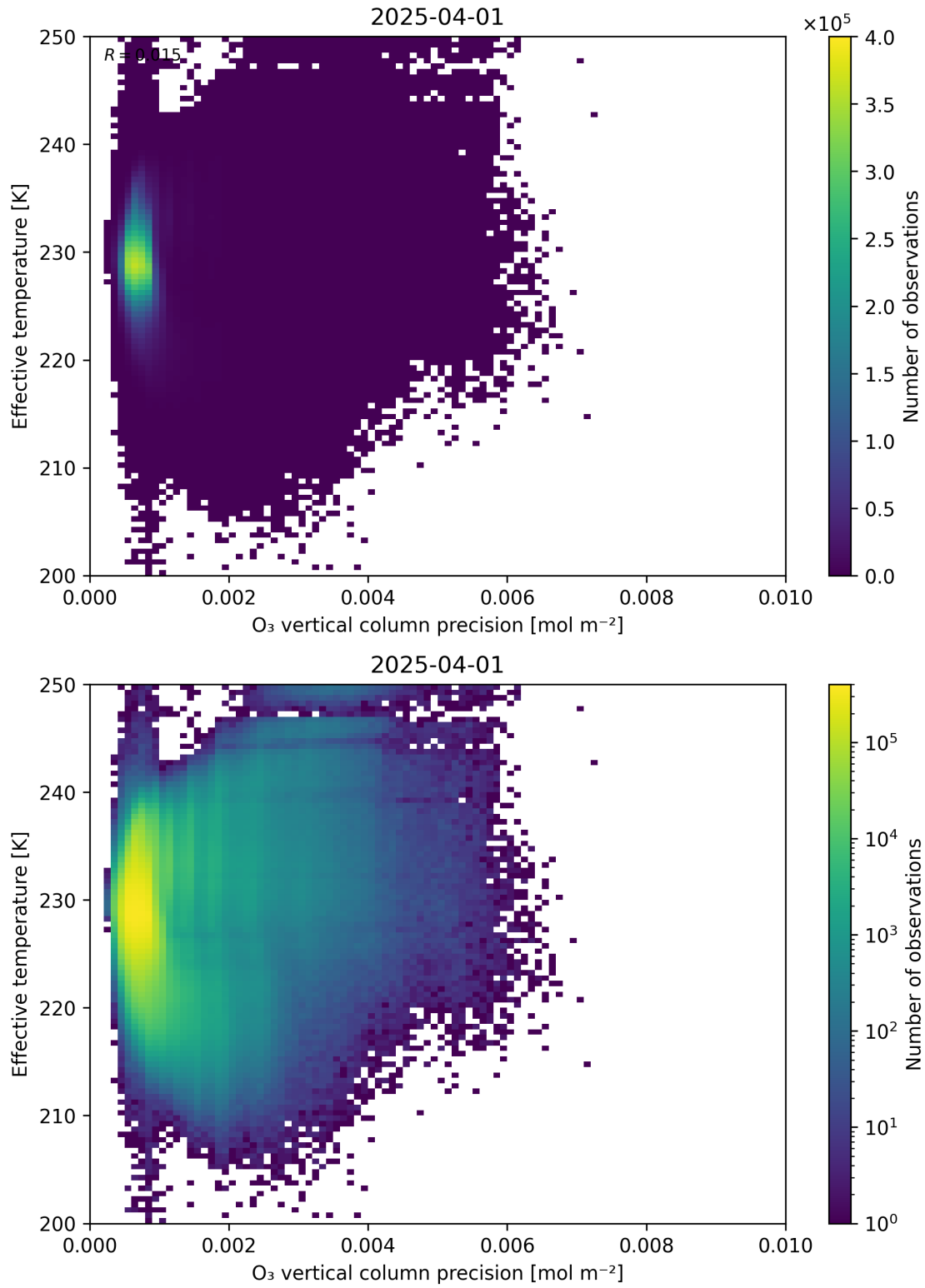
Figure 42: Scatter density plot of “O 3 vertical column precision” against “Effective temperature” for 2025-03-31 to 2025-04-02.
