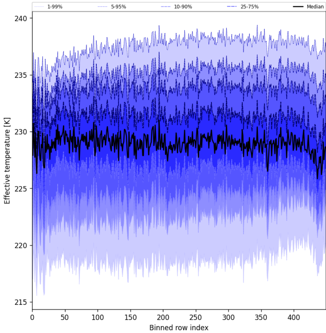
Figure 31: Along track statistics of “Effective temperature” for 2025-03-31 to 2025-04-02
