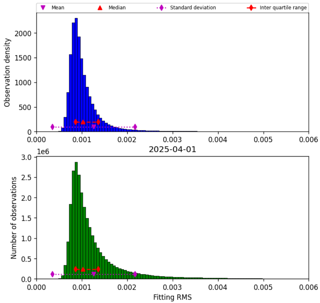
Figure 23: Histogram of “Fitting RMS” for 2025-03-31 to 2025-04-02
