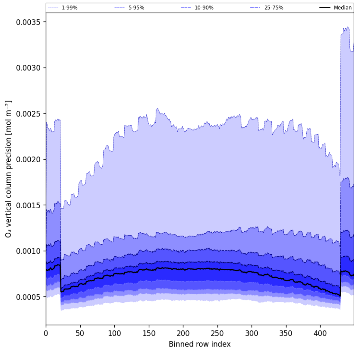
Figure 29: Along track statistics of “O 3 vertical column precision” for 2025-03-31 to 2025-04-02
