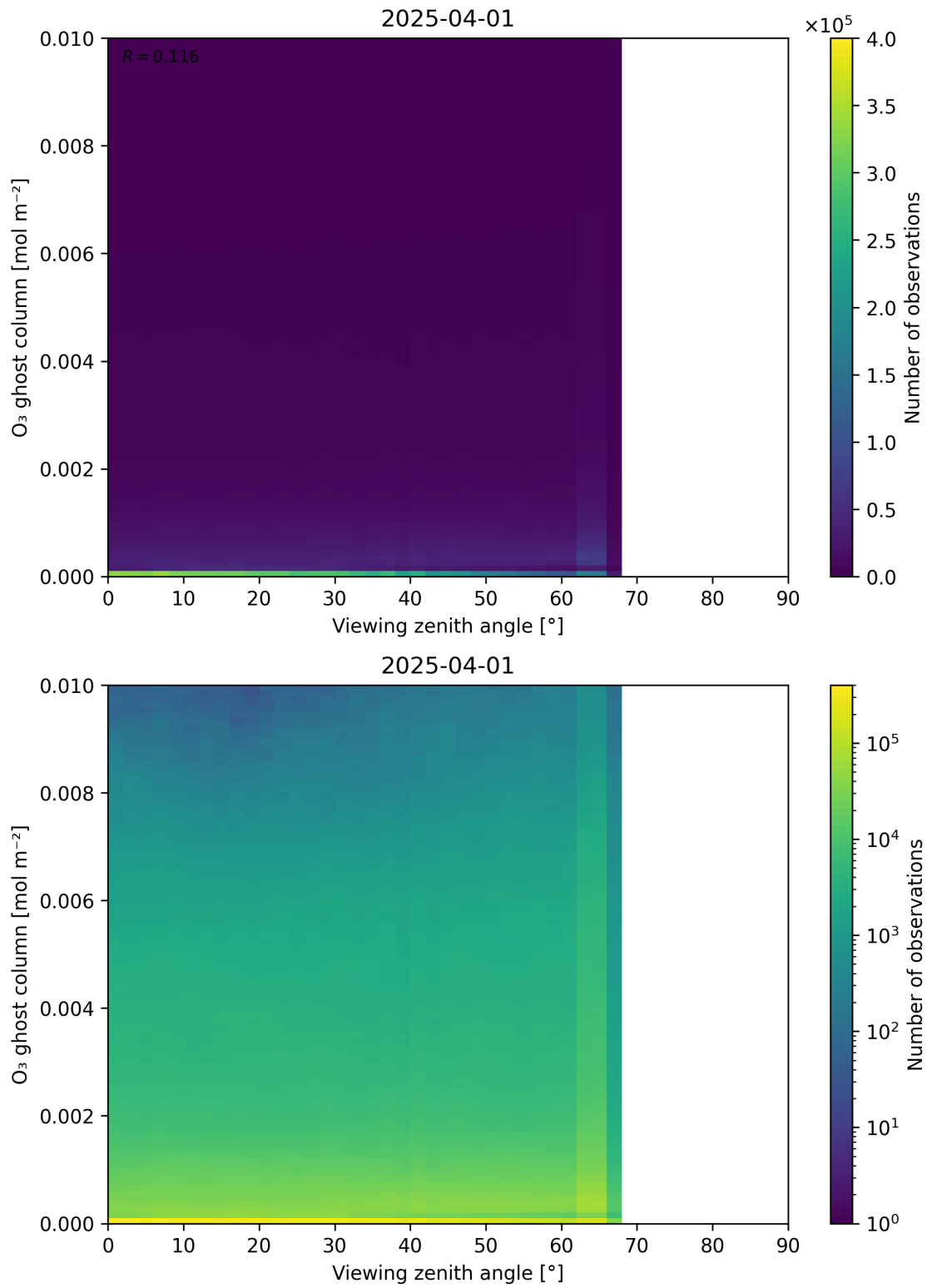
Figure 51: Scatter density plot of “Viewing zenith angle” against “O 3 ghost column” for 2025-03-31 to 2025-04-02.
