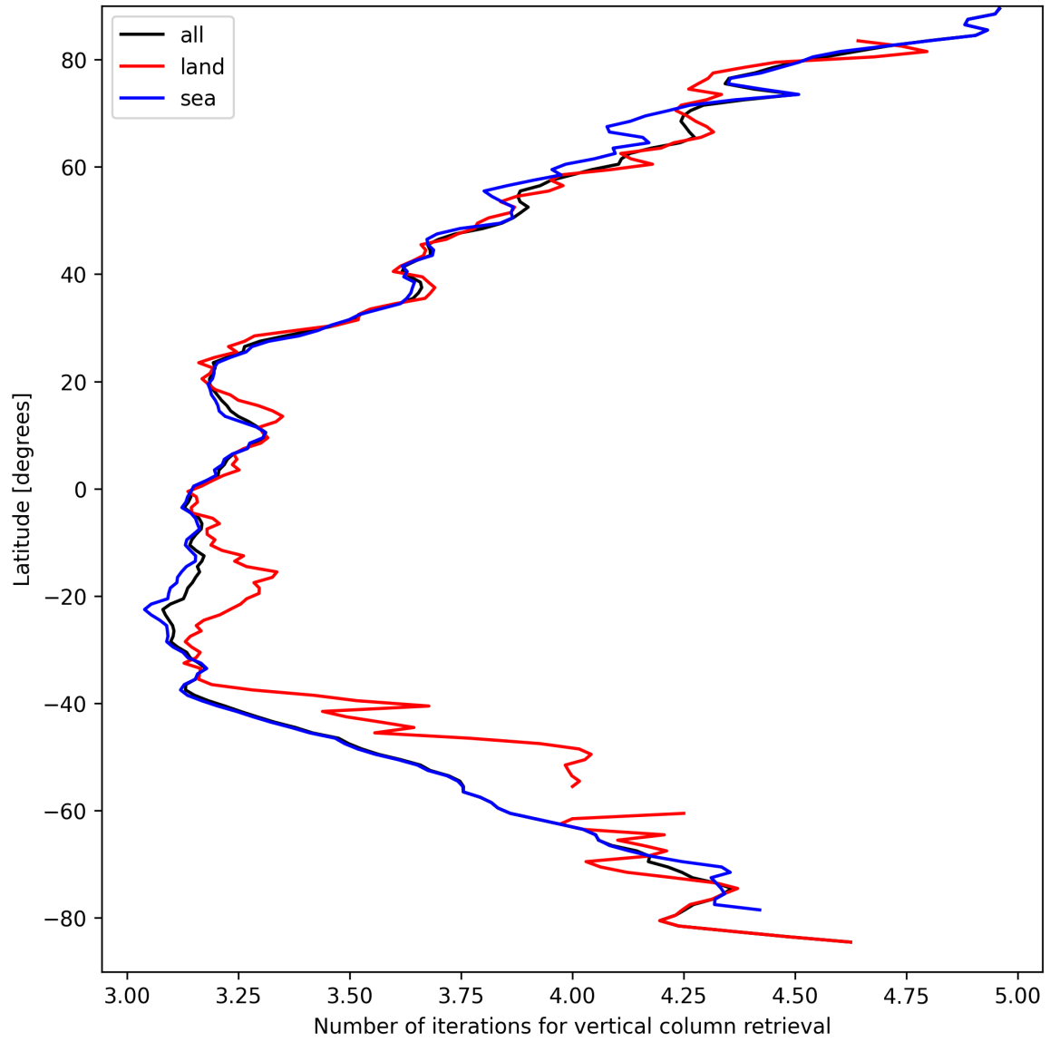
Figure 19: Zonal average of “Number of iterations for vertical column retrieval” for 2025-03-31 to 2025-04-02.
