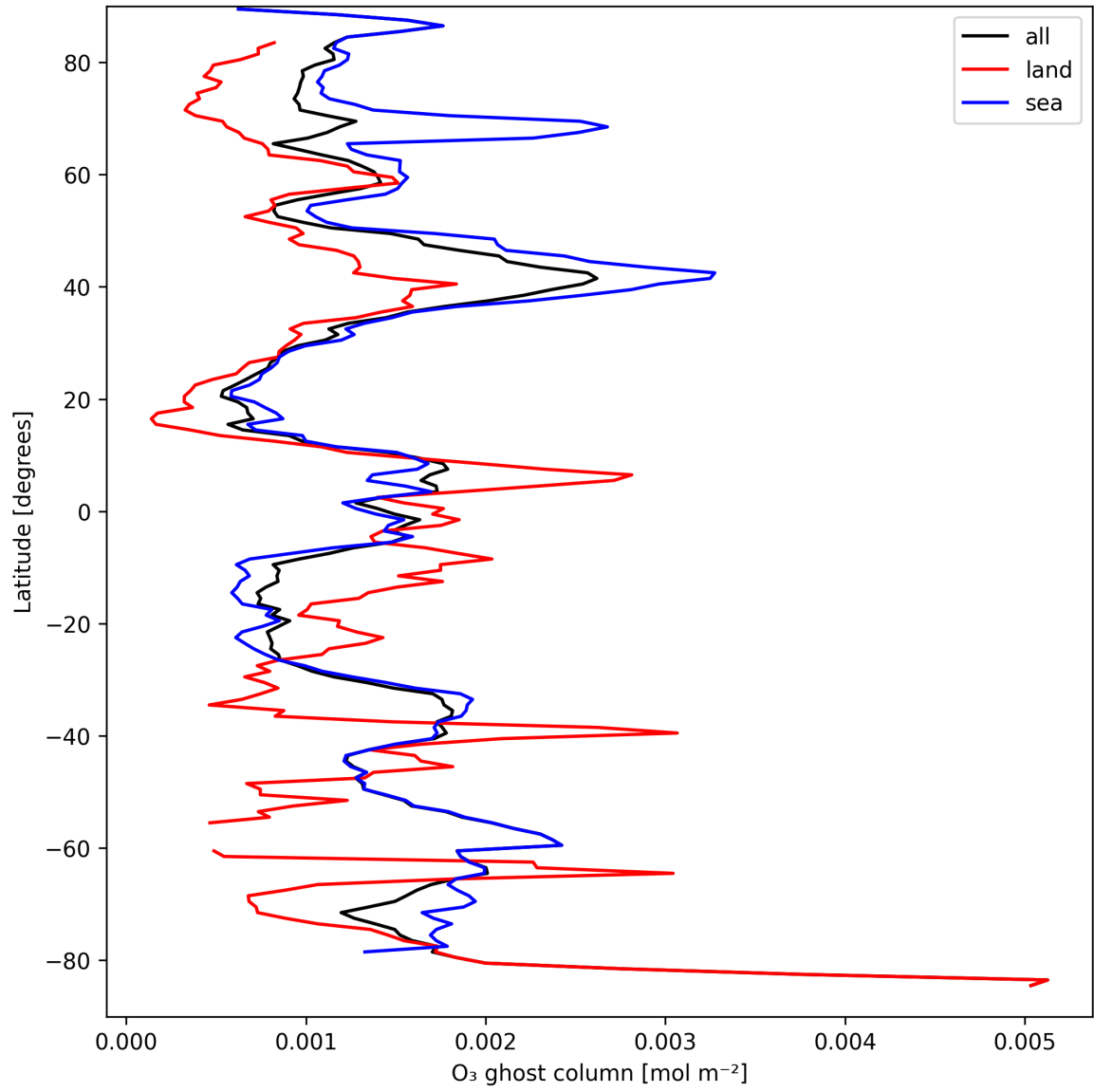
Figure 18: Zonal average of “O 3 ghost column” for 2025-04-02 to 2025-04-03.
