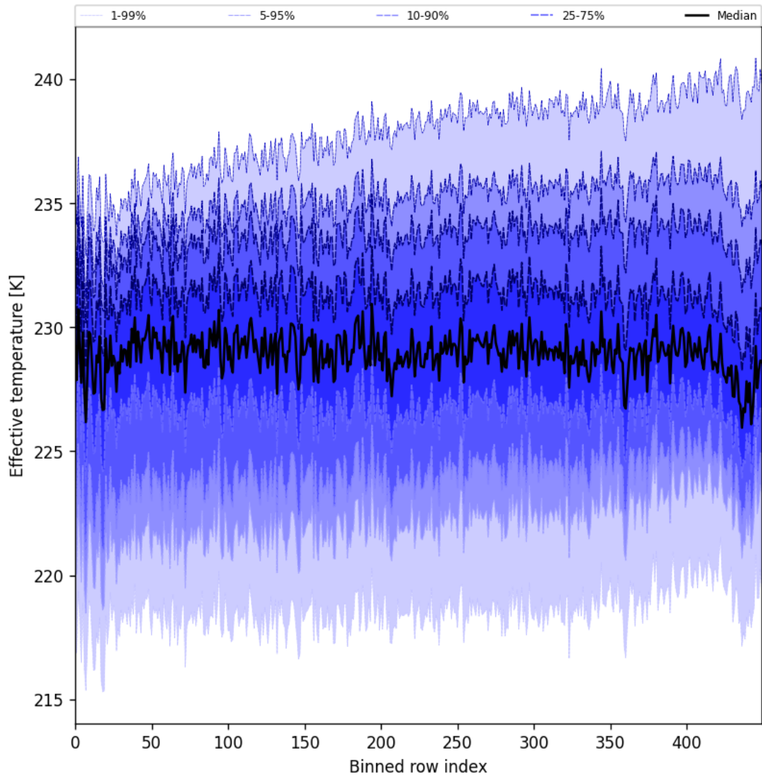
Figure 31: Along track statistics of “Effective temperature” for 2025-04-02 to 2025-04-03
