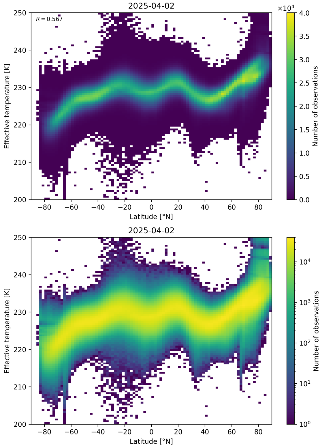
Figure 34: Scatter density plot of “Latitude” against “Effective temperature” for 2025-04-02 to 2025-04-03.
