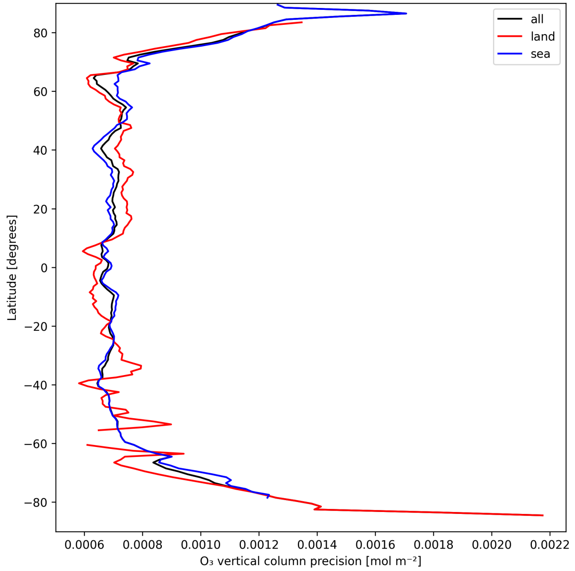
Figure 15: Zonal average of “O 3 vertical column precision” for 2025-04-02 to 2025-04-03.
