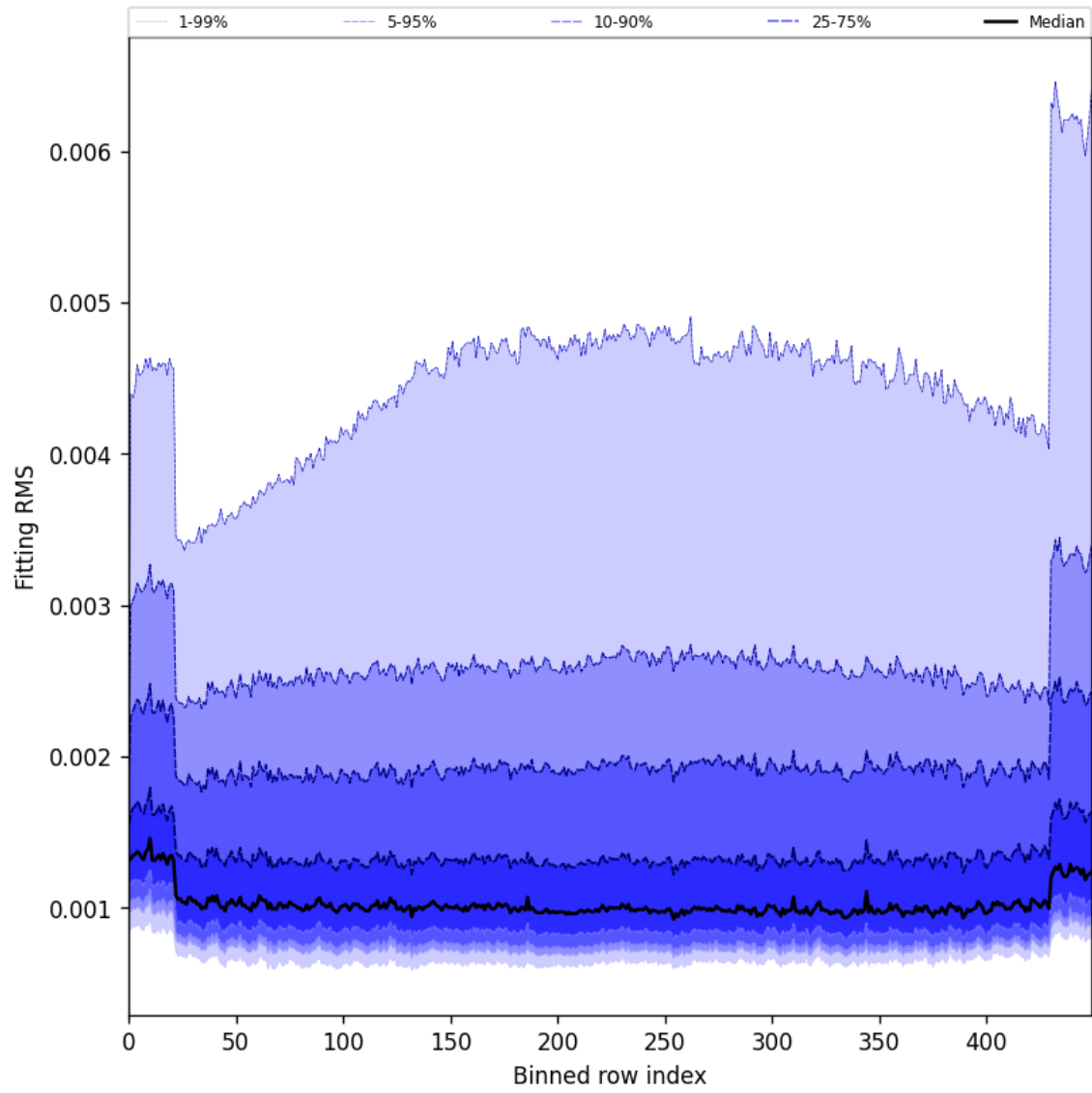
Figure 30: Along track statistics of “Fitting RMS” for 2025-04-02 to 2025-04-03
