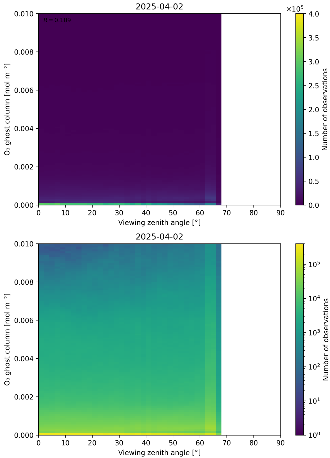
Figure 51: Scatter density plot of “Viewing zenith angle” against “O 3 ghost column” for 2025-04-02 to 2025-04-03.
