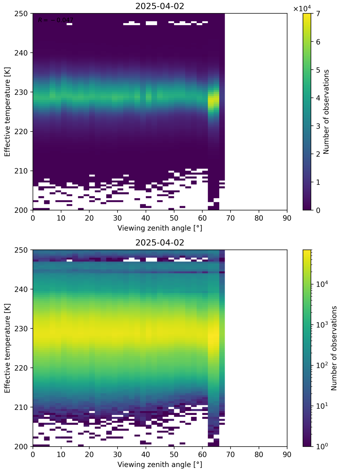
Figure 50: Scatter density plot of “Viewing zenith angle” against “Effective temperature” for 2025-04-02 to 2025-04-03.
