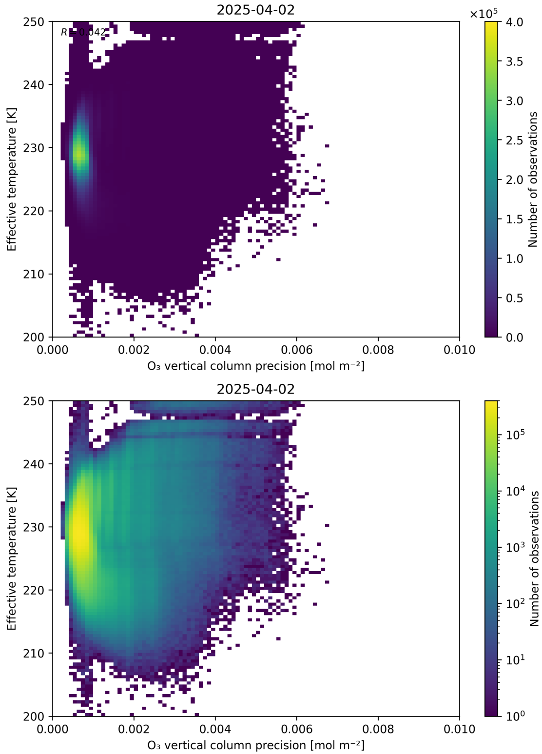
Figure 42: Scatter density plot of “ O_3 vertical column precision” against “Effective temperature” for 2025-04-02 to 2025-04-03.
