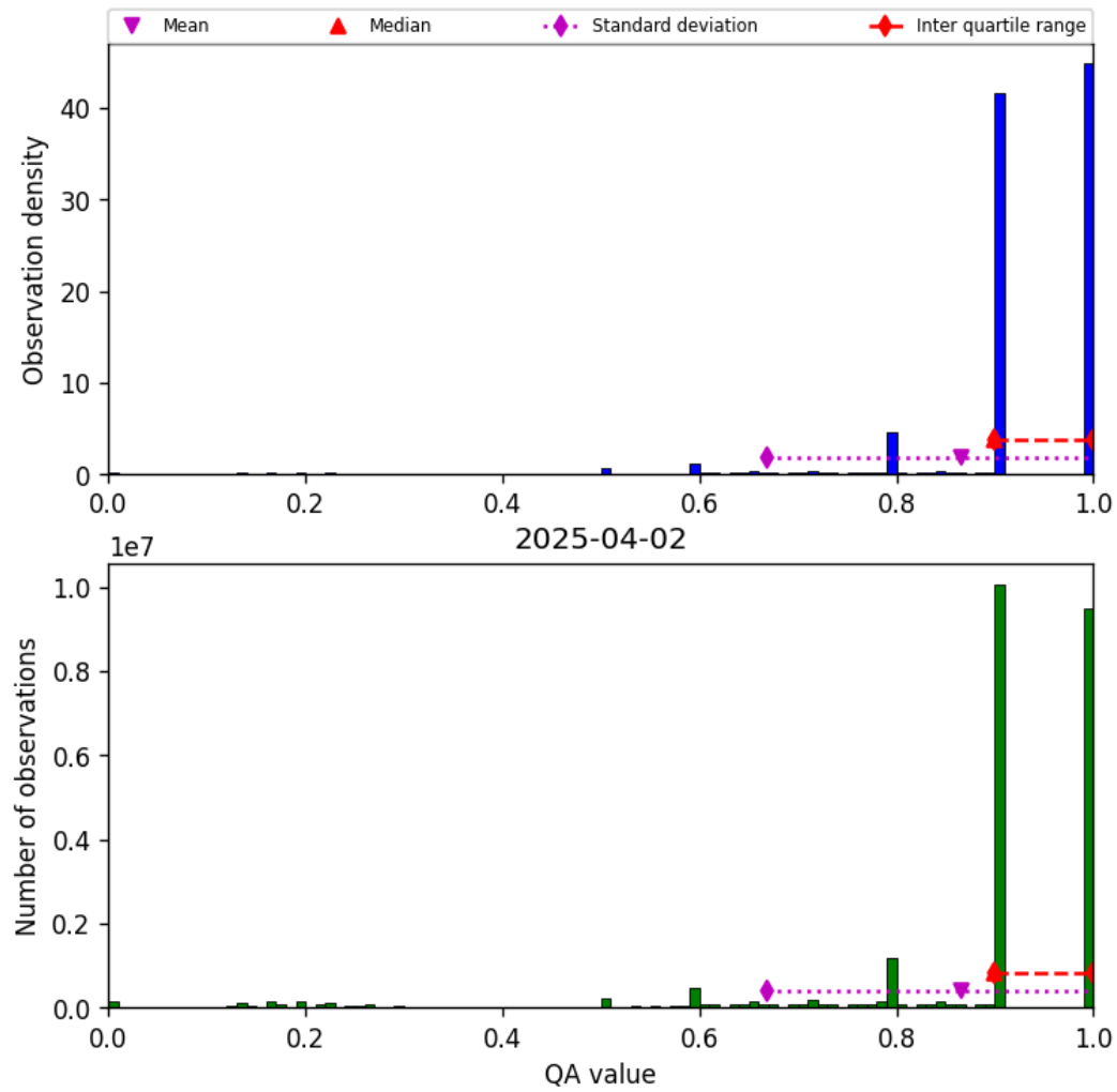
Figure 20: Histogram of “QA value” for 2025-04-02 to 2025-04-03
