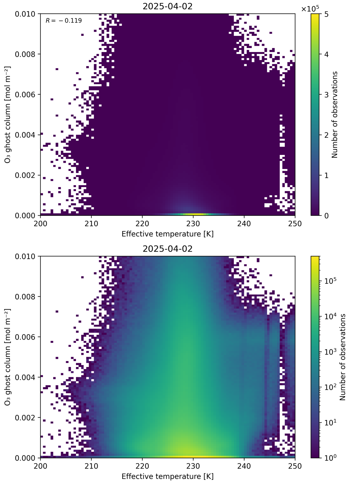
Figure 38: Scatter density plot of “Effective temperature” against “O 3 ghost column” for 2025-04-02 to 2025-04-03.
