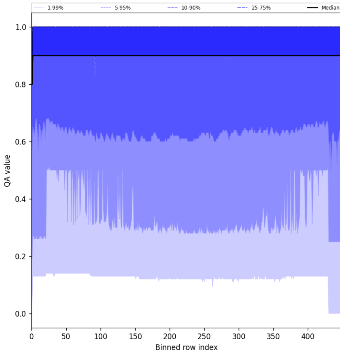
Figure 27: Along track statistics of “QA value” for 2025-04-02 to 2025-04-03
