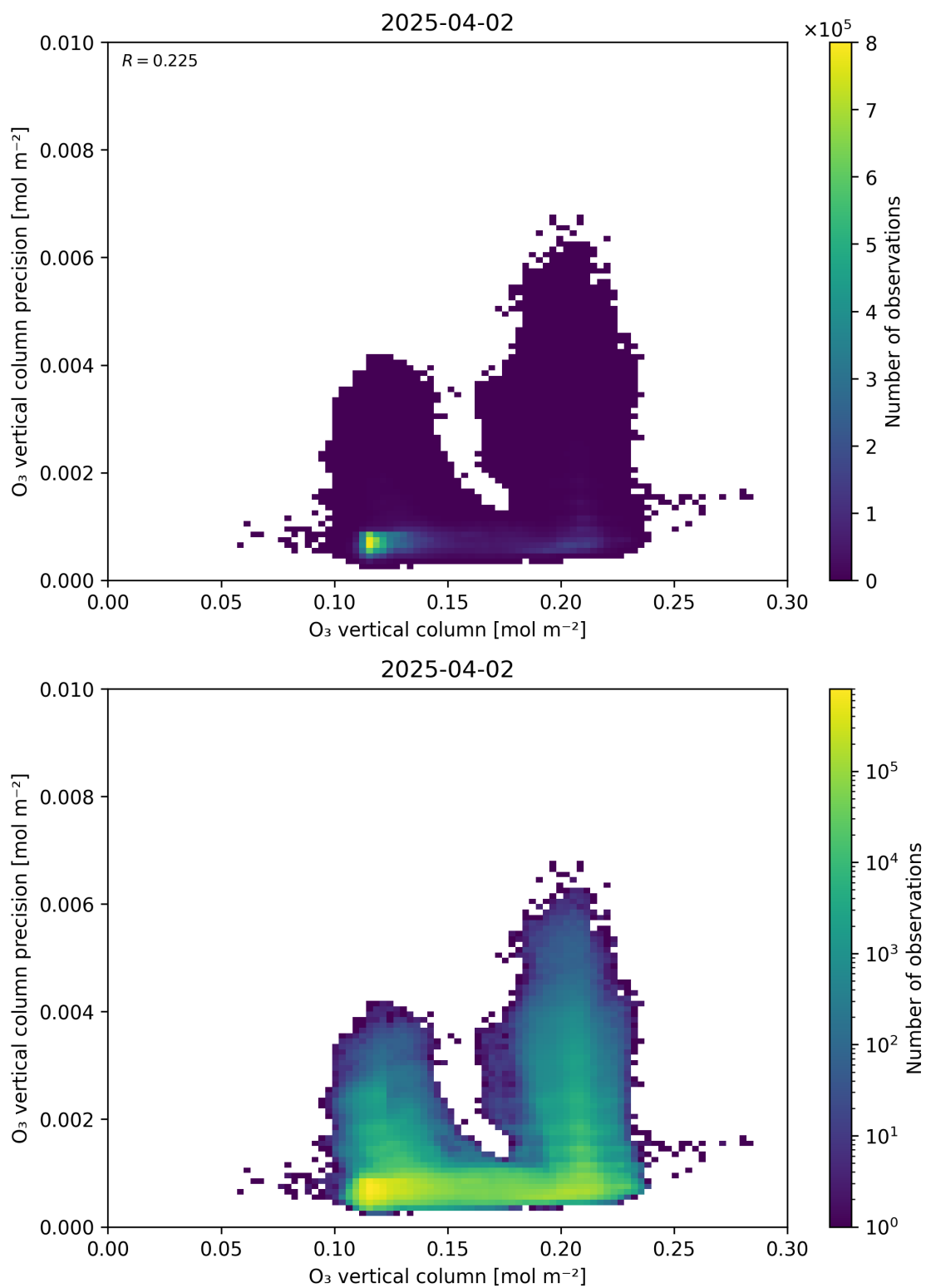
Figure 41: Scatter density plot of “O 3 vertical column” against “O 3 vertical column precision” for 2025-04-02 to 2025-04-03.
