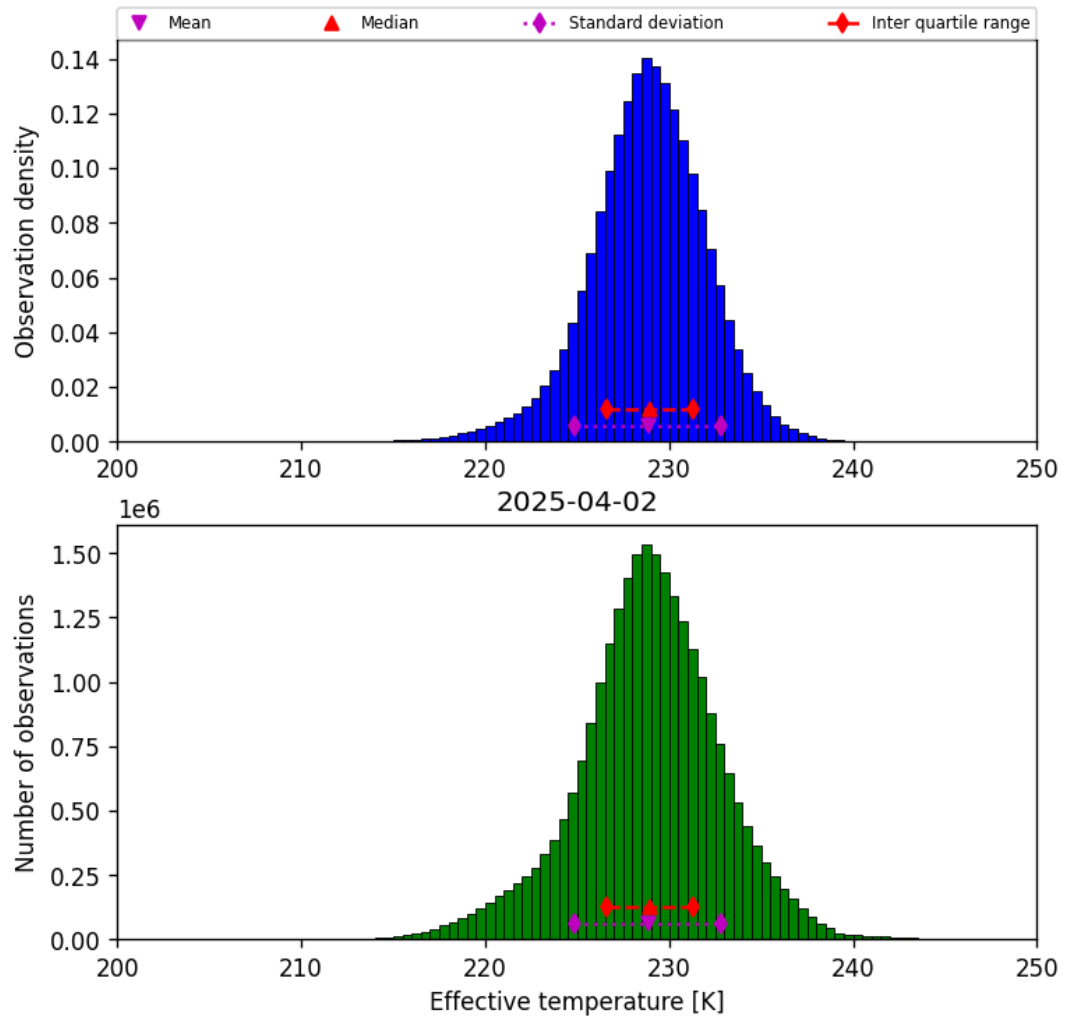
Figure 24: Histogram of “Effective temperature” for 2025-04-02 to 2025-04-03
