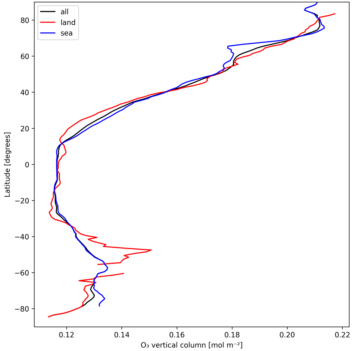
Figure 14: Zonal average of “O 3 vertical column” for 2025-04-02 to 2025-04-03.
