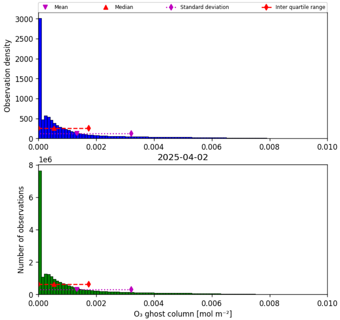
Figure 25: Histogram of “O 3 ghost column” for 2025-04-02 to 2025-04-03
