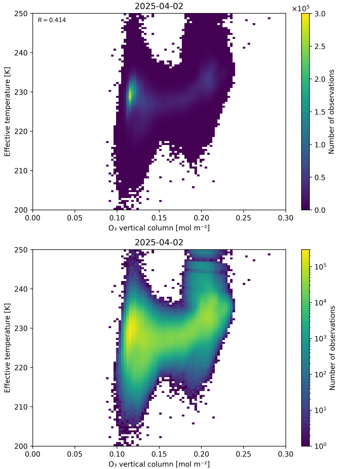
Figure 39: Scatter density plot of “O 3 vertical column” against “Effective temperature” for 2025-04-02 to 2025-04-03.
