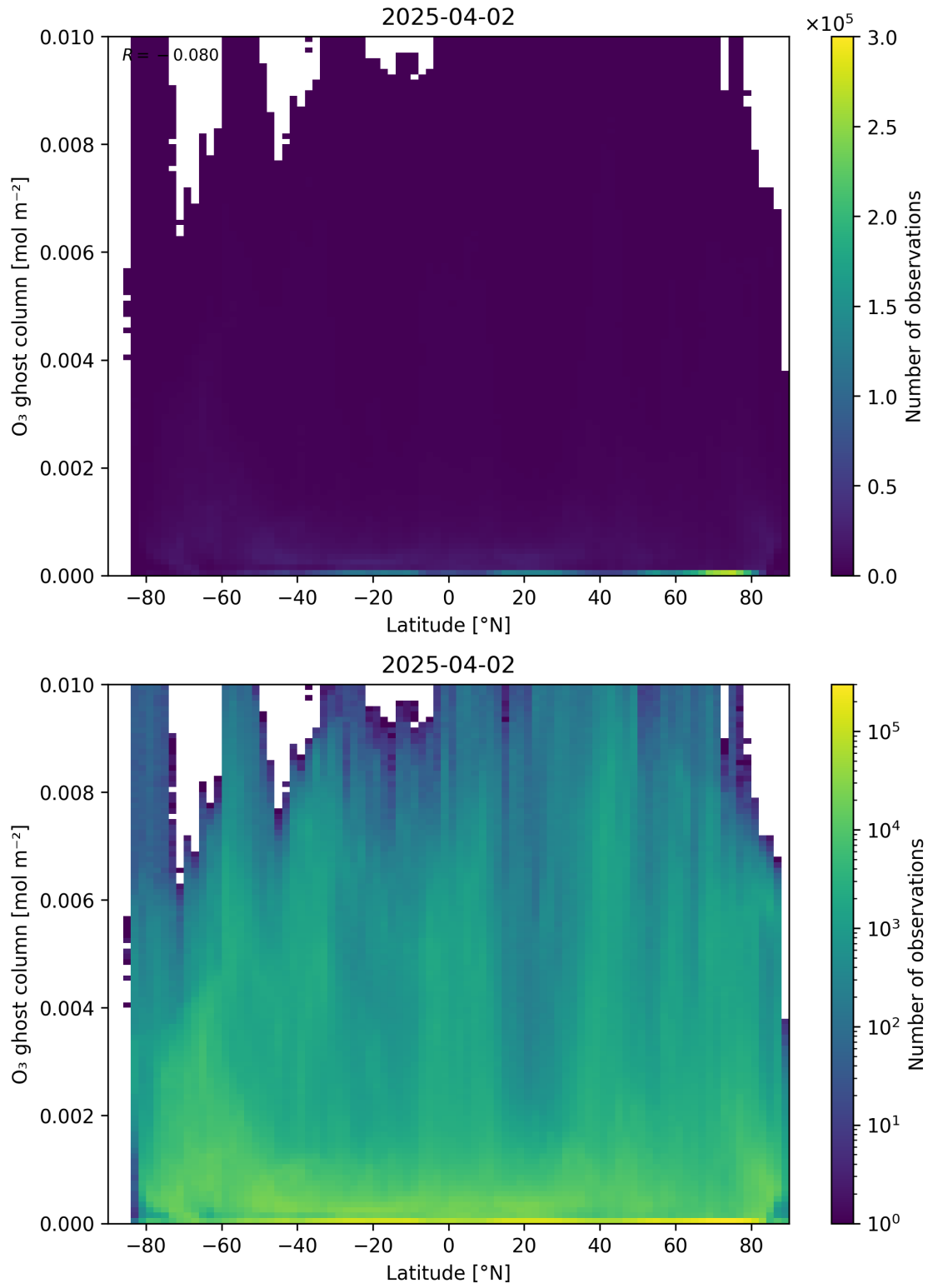
Figure 35: Scatter density plot of “Latitude” against “O 3 ghost column” for 2025-04-02 to 2025-04-03.
