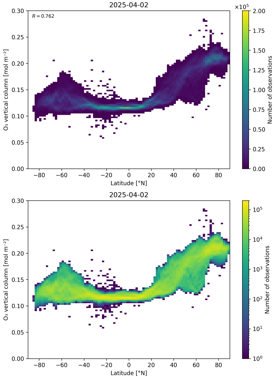
Figure 36: Scatter density plot of “Latitude” against “O 3 vertical column” for 2025-04-02 to 2025-04-03.
