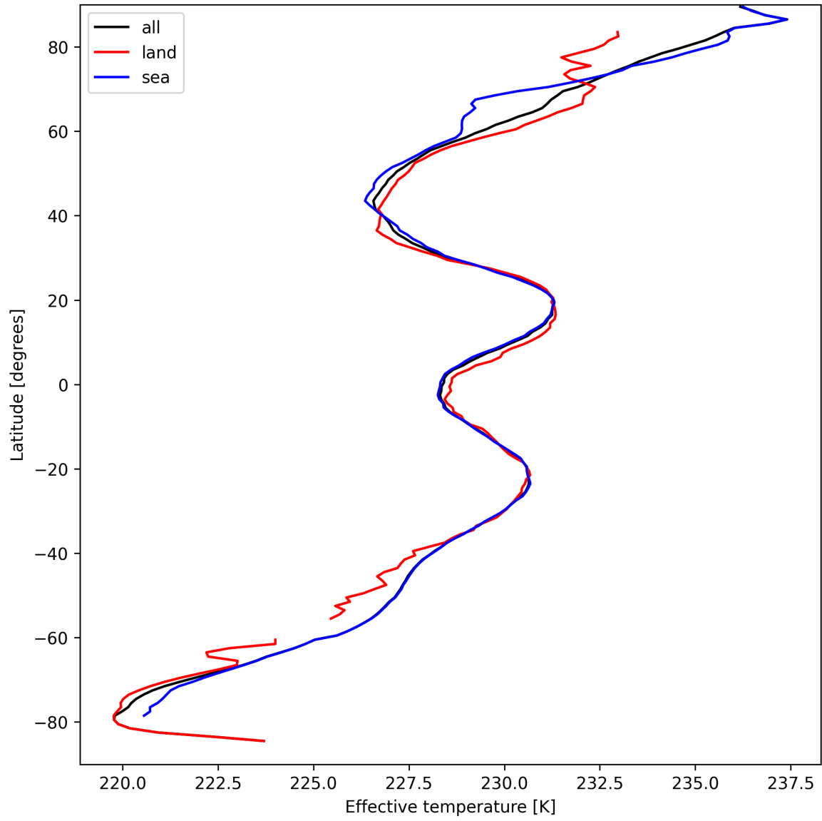
Figure 17: Zonal average of "Effective temperature" for 2025-04-02 to 2025-04-03.
