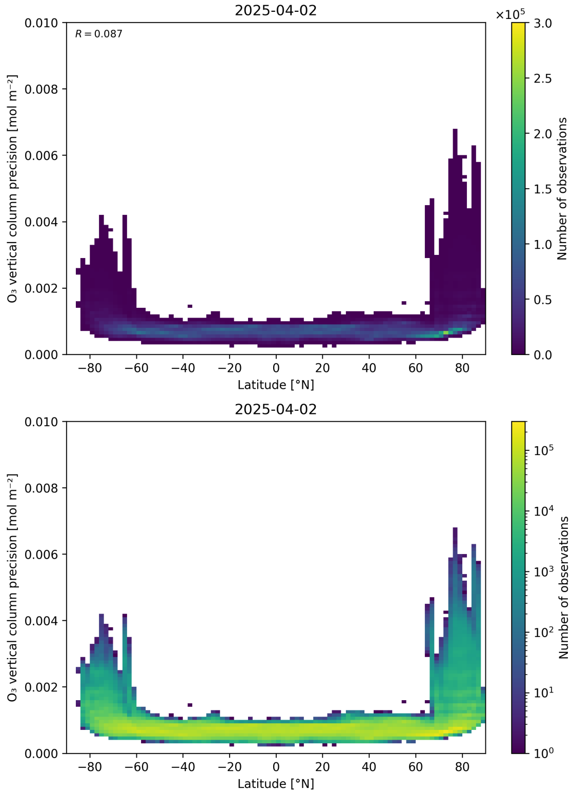
Figure 37: Scatter density plot of “Latitude” against “O 3 vertical column precision” for 2025-04-02 to 2025-04-03.
