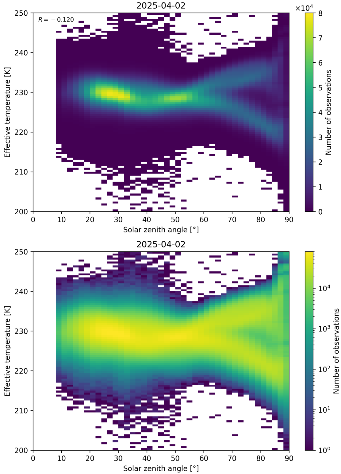
Figure 45: Scatter density plot of “Solar zenith angle” against “Effective temperature” for 2025-04-02 to 2025-04-03.
