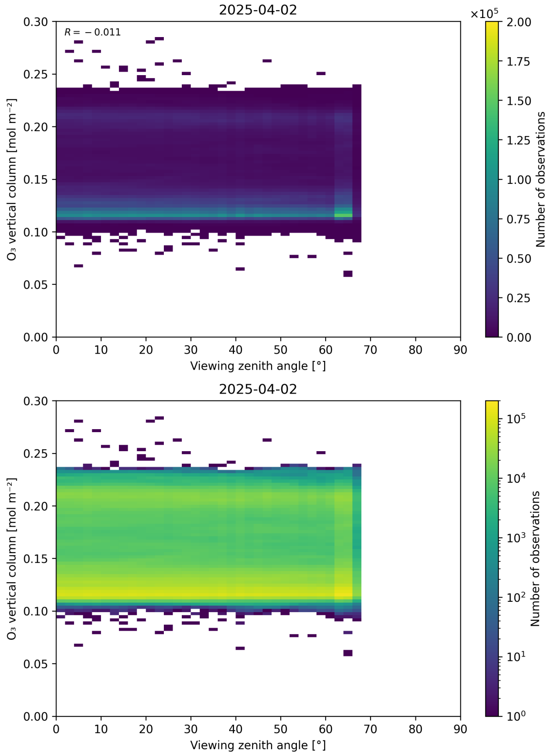
Figure 52: Scatter density plot of “Viewing zenith angle” against “O 3 vertical column” for 2025-04-02 to 2025-04-03.
