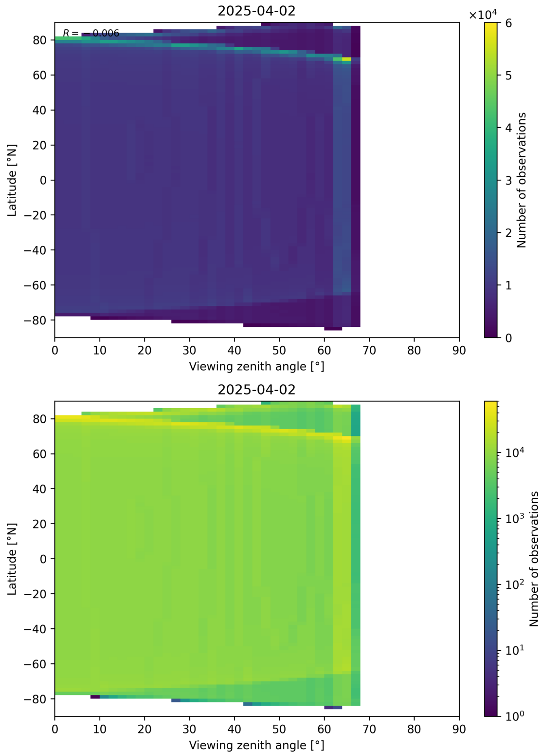
Figure 49: Scatter density plot of “Viewing zenith angle” against “Latitude” for 2025-04-02 to 2025-04-03.
