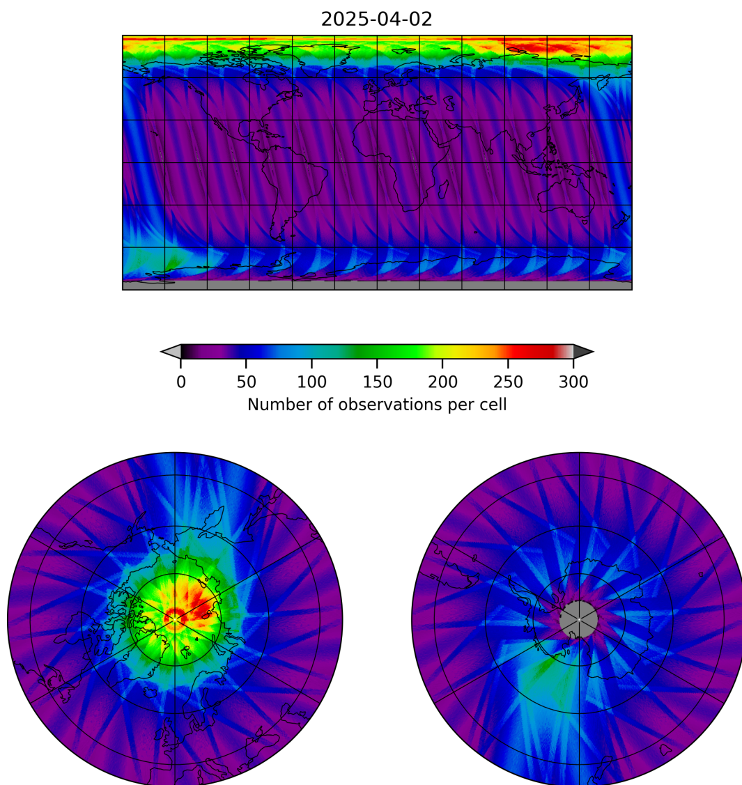
Figure 12: Map of the number of observations for 2025-04-02 to 2025-04-03
