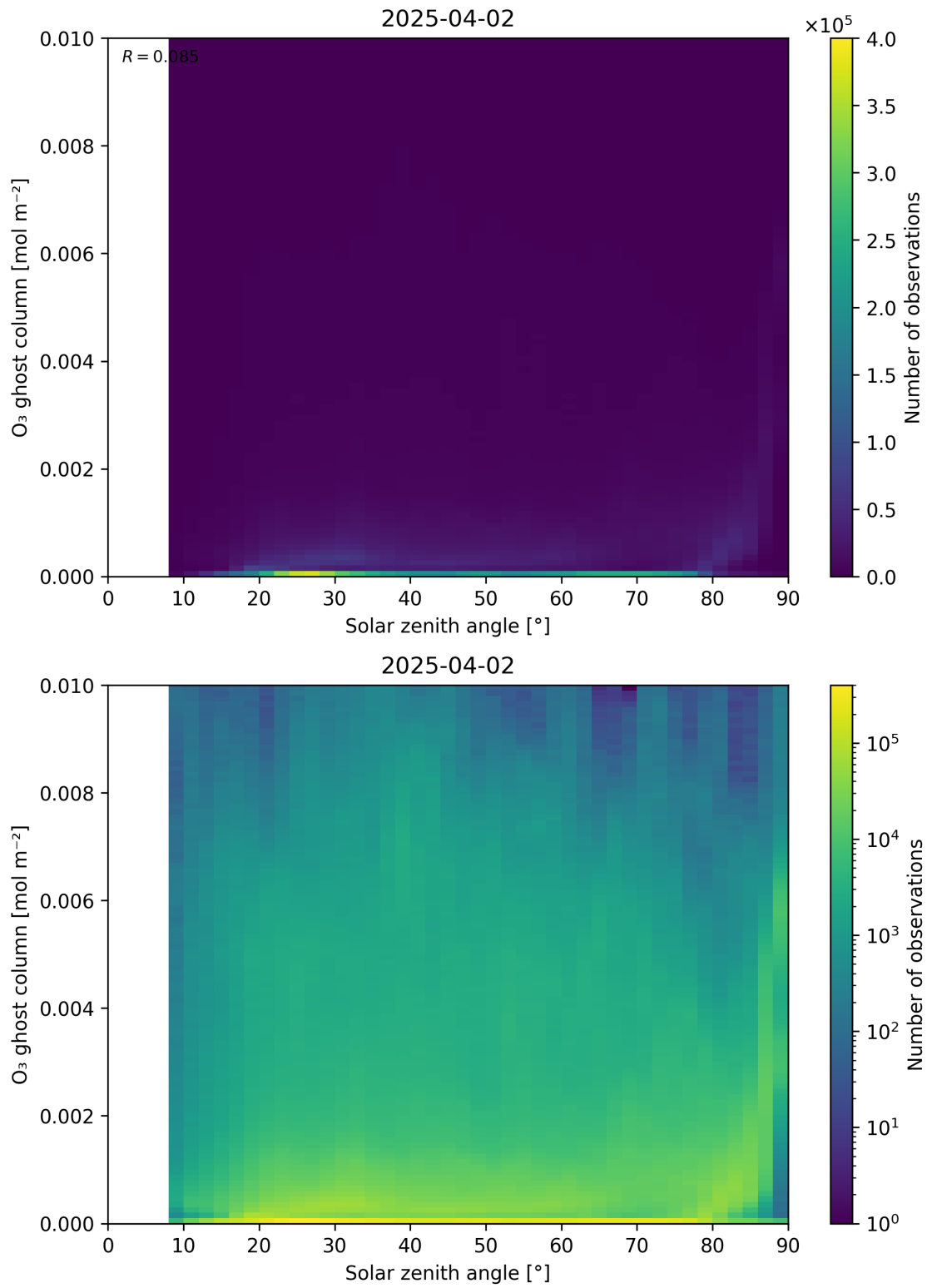
Figure 46: Scatter density plot of “Solar zenith angle” against “O 3 ghost column” for 2025-04-02 to 2025-04-03.
