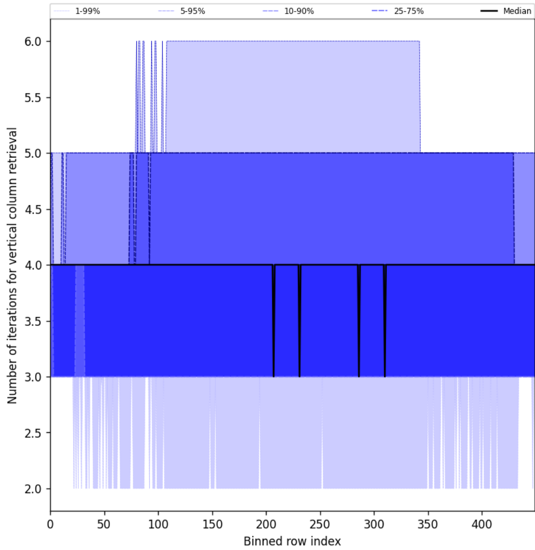
Figure 33: Along track statistics of “Number of iterations for vertical column retrieval” for 2025-04-02 to 2025-04-03
