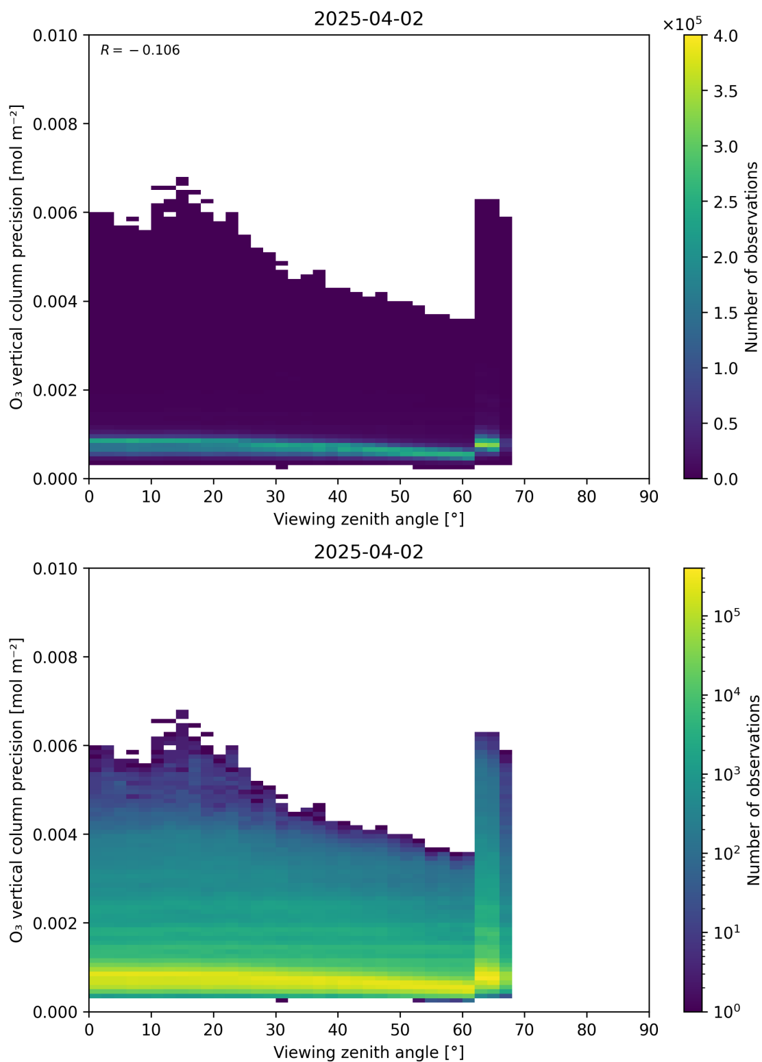
Figure 53: Scatter density plot of “Viewing zenith angle” against “O 3 vertical column precision” for 2025-04-02 to 2025-04-03.
