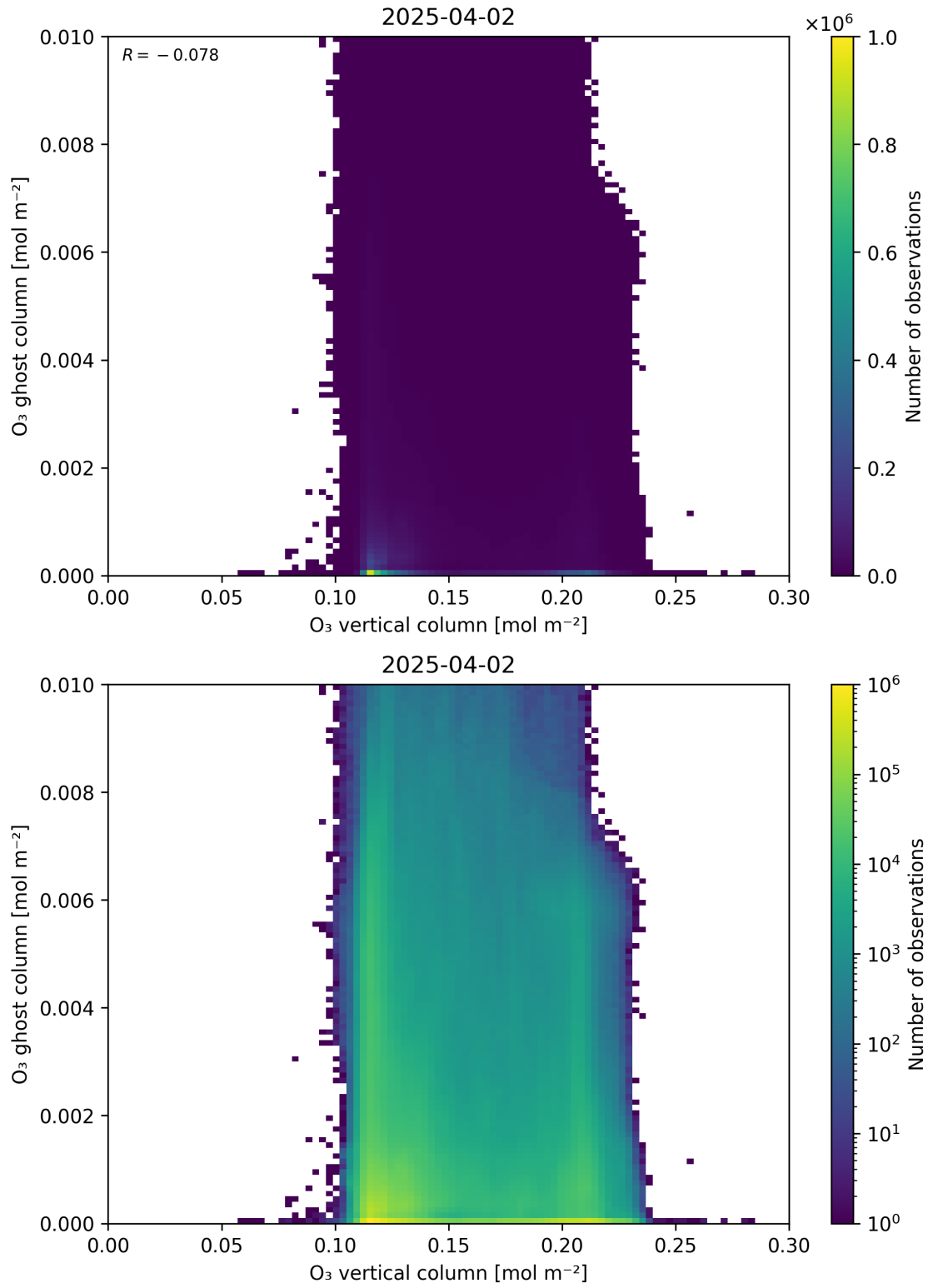
Figure 40: Scatter density plot of “O 3 vertical column” against “O 3 ghost column” for 2025-04-02 to 2025-04-03.
