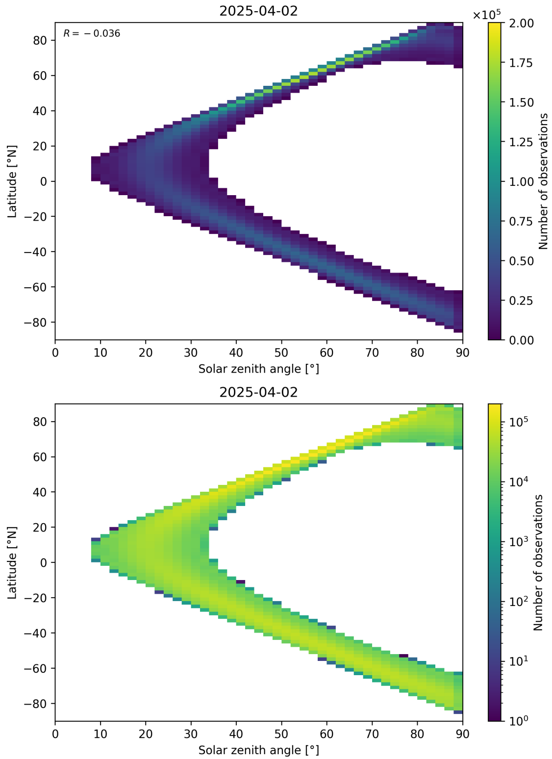
Figure 44: Scatter density plot of “Solar zenith angle” against “Latitude” for 2025-04-02 to 2025-04-03.
