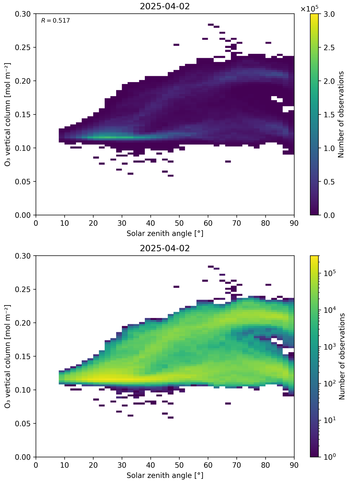
Figure 47: Scatter density plot of “Solar zenith angle” against “O 3 vertical column” for 2025-04-02 to 2025-04-03.
