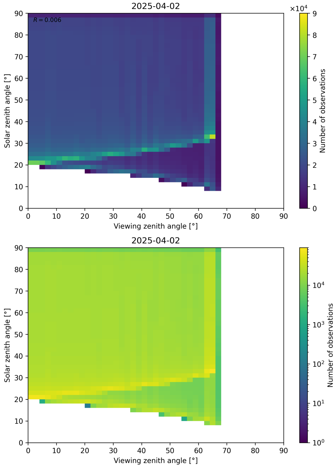
Figure 54: Scatter density plot of “Viewing zenith angle” against “Solar zenith angle” for 2025-04-02 to 2025-04-03.
