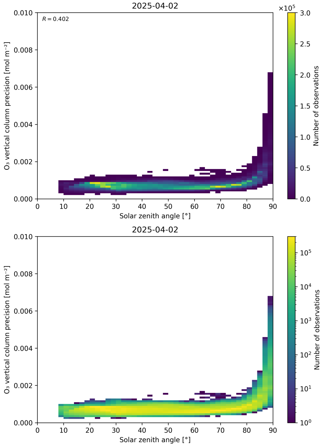
Figure 48: Scatter density plot of “Solar zenith angle” against “O 3 vertical column precision” for 2025-04-02 to 2025-04-03.
