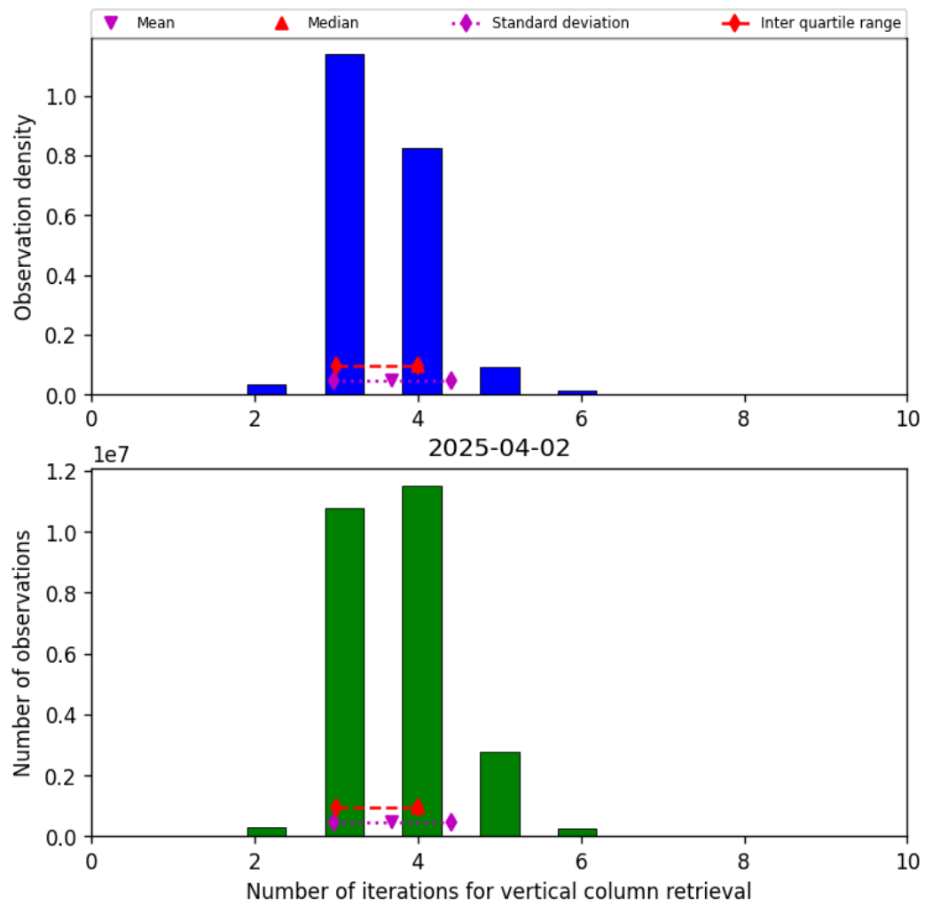
Figure 26: Histogram of “Number of iterations for vertical column retrieval” for 2025-04-02 to 2025-04-03
