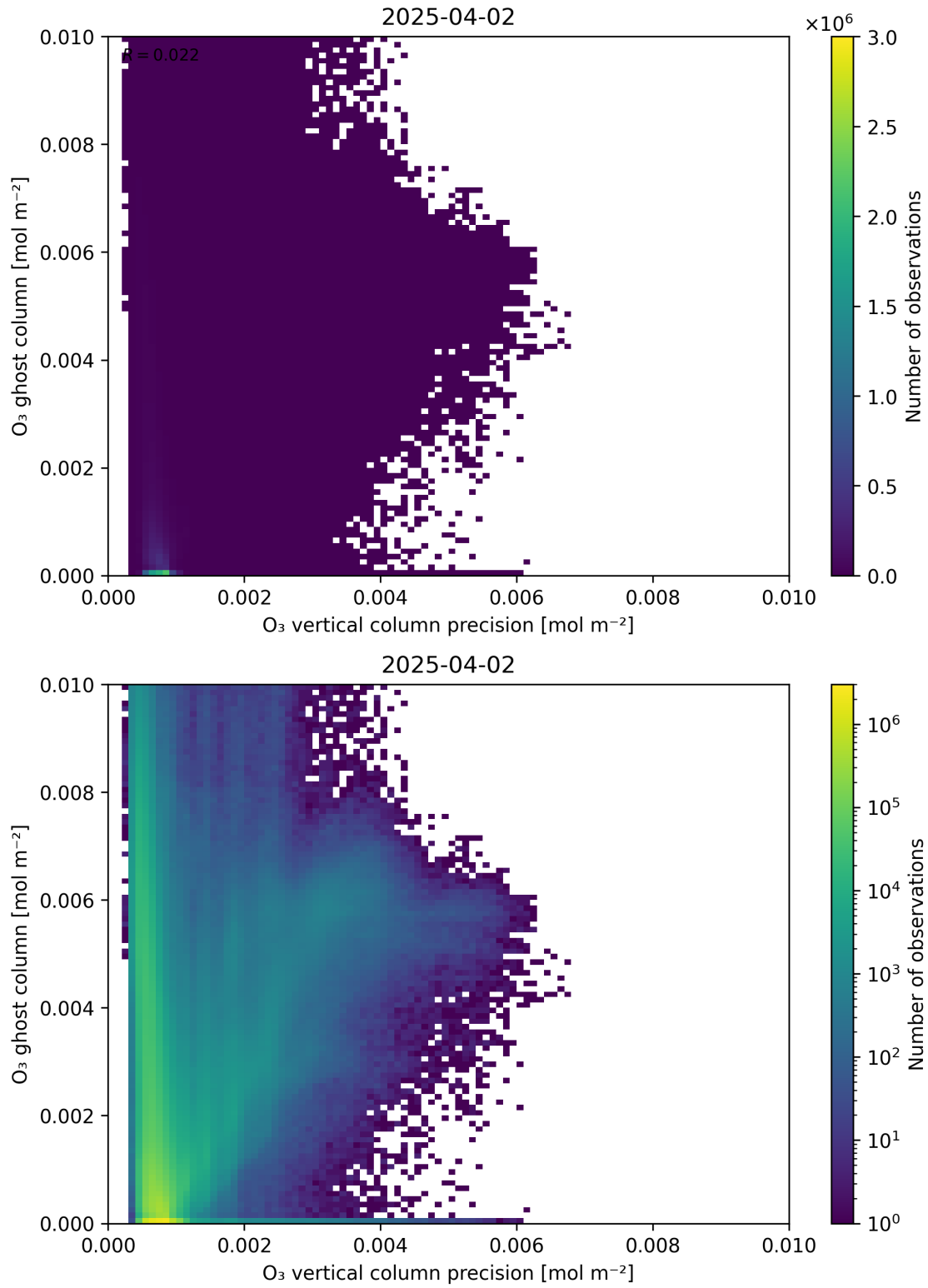
Figure 43: Scatter density plot of “O 3 vertical column precision” against “O 3 ghost column” for 2025-04-02 to 2025-04-03.
