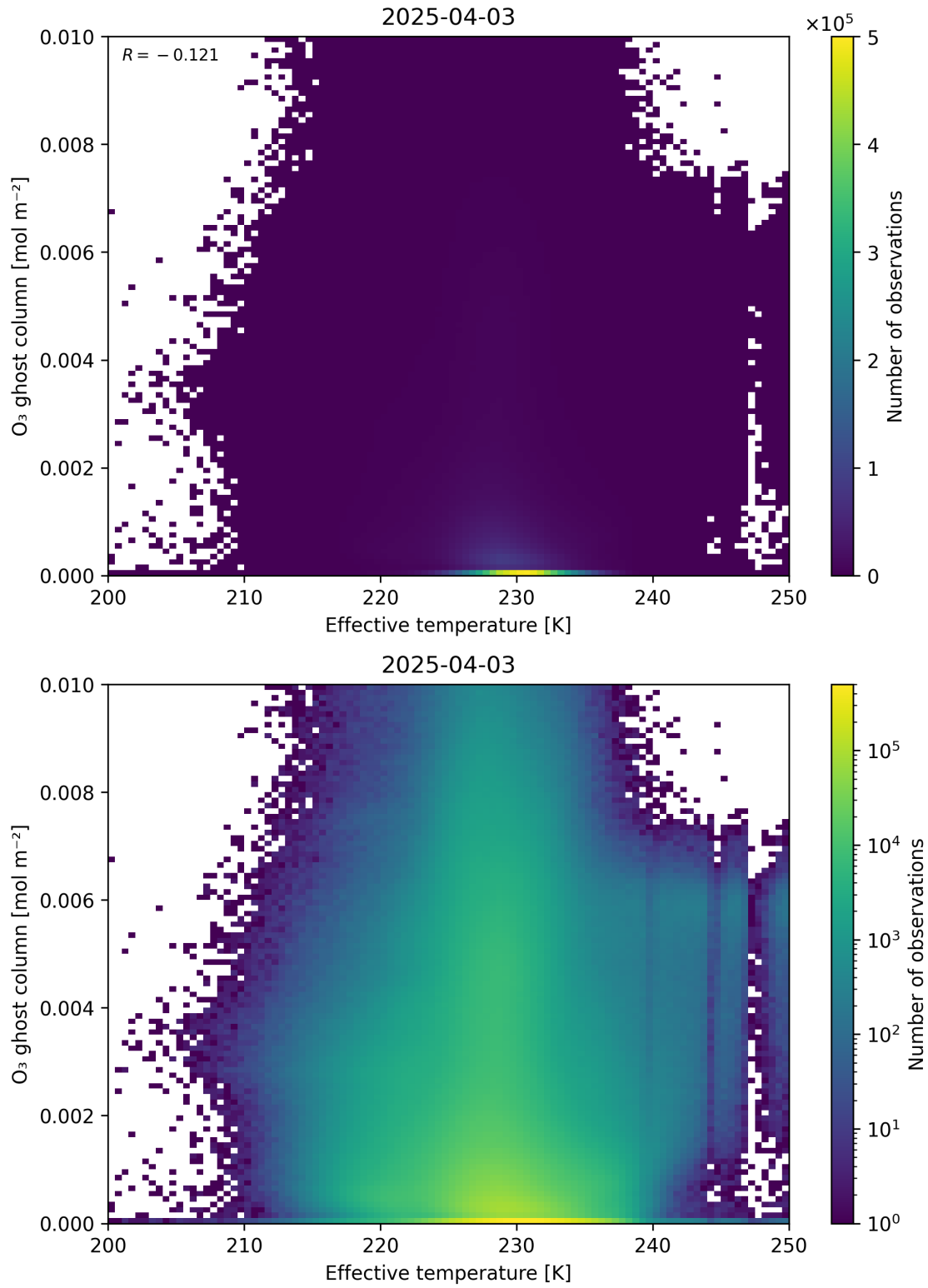
Figure 38: Scatter density plot of “Effective temperature” against “O 3 ghost column” for 2025-04-03 to 2025-04-04.
