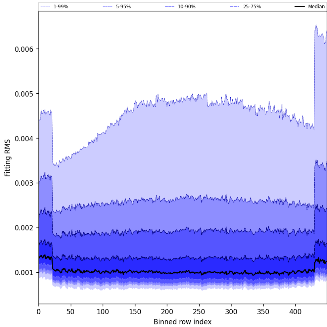
Figure 30: Along track statistics of “Fitting RMS” for 2025-04-03 to 2025-04-04
