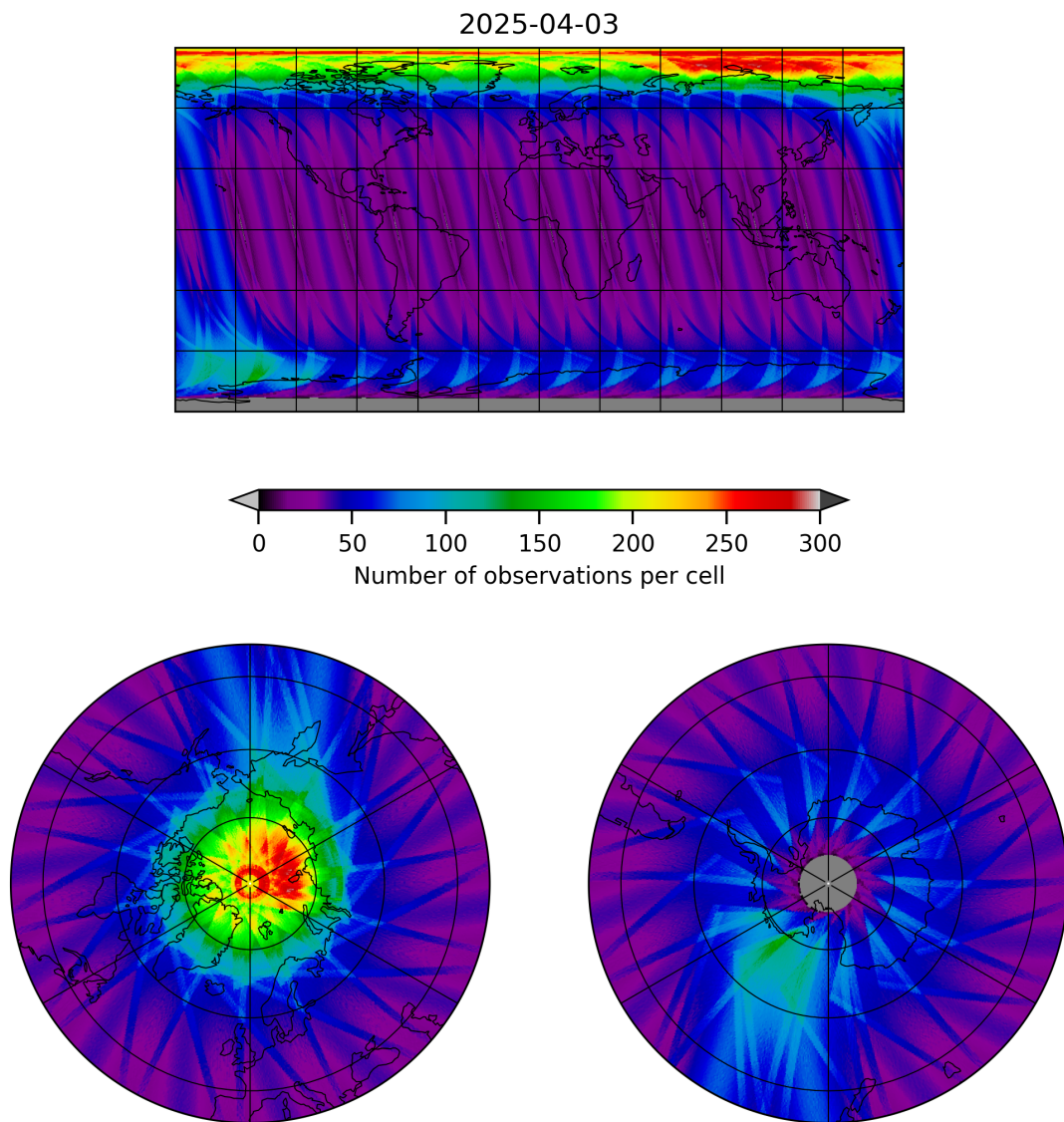
Figure 12: Map of the number of observations for 2025-04-03 to 2025-04-04
