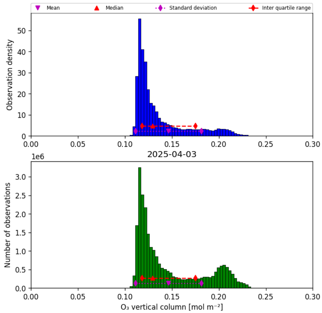
Figure 21: Histogram of “O 3 vertical column” for 2025-04-03 to 2025-04-04
