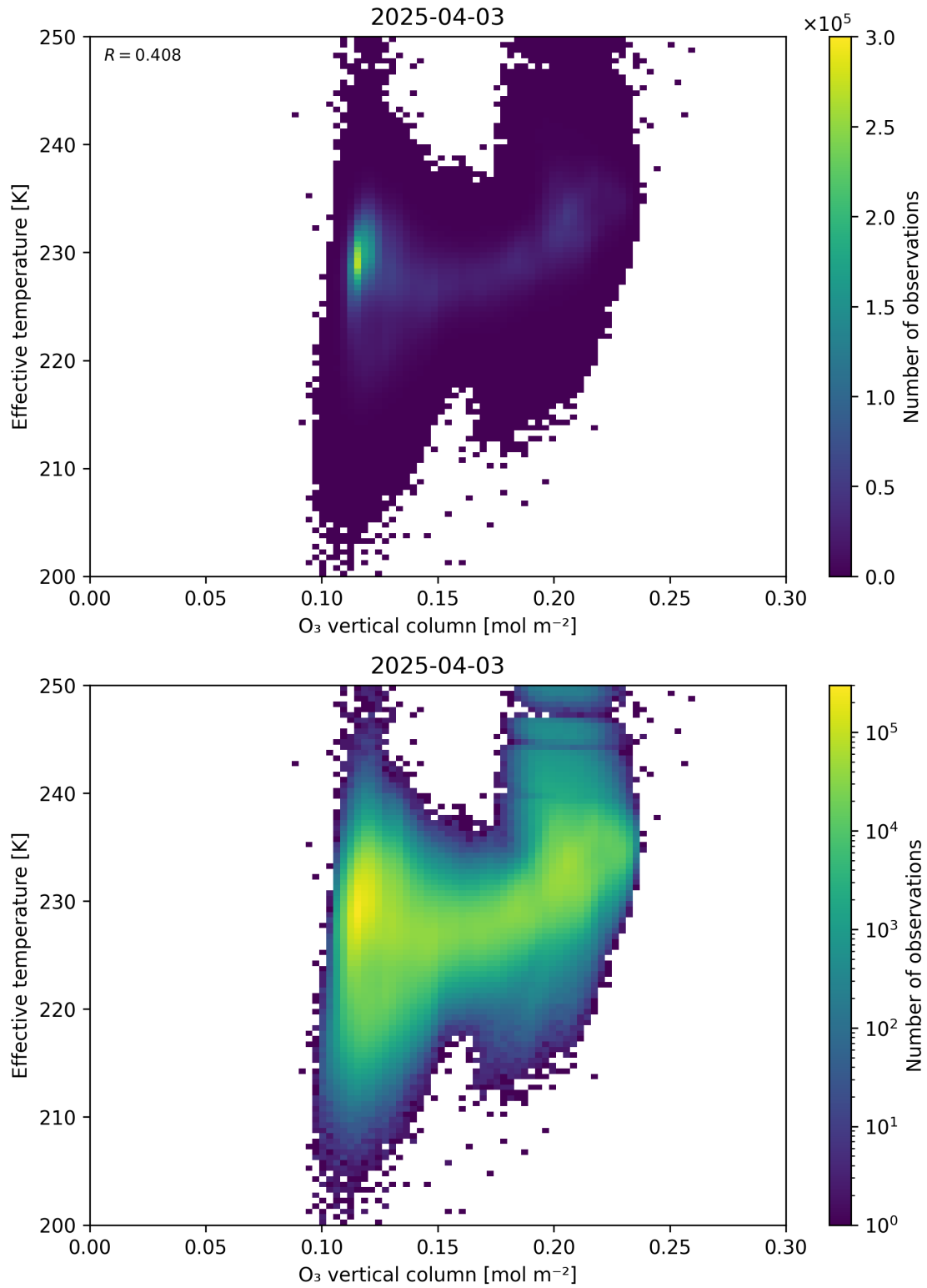
Figure 39: Scatter density plot of “O 3 vertical column” against “Effective temperature” for 2025-04-03 to 2025-04-04.
