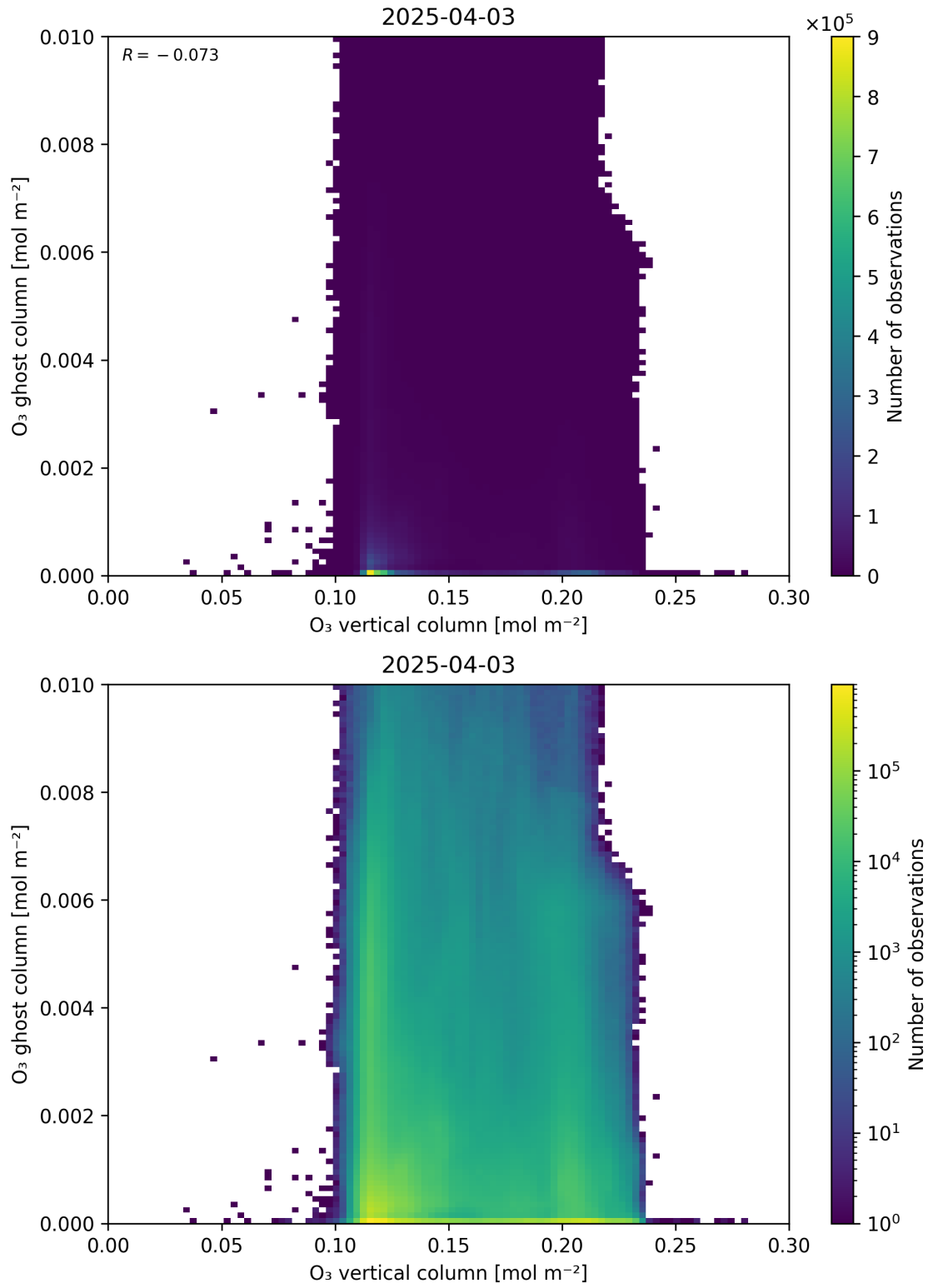
Figure 40: Scatter density plot of “O 3 vertical column” against “O 3 ghost column” for 2025-04-03 to 2025-04-04.
