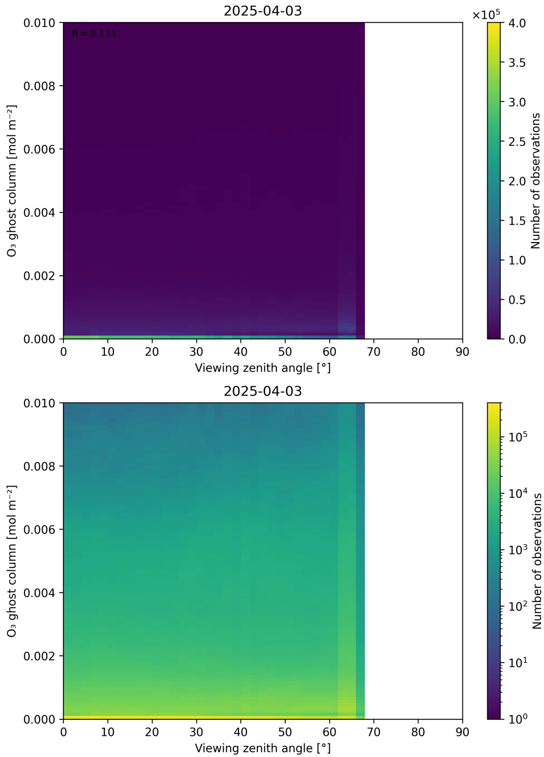
Figure 51: Scatter density plot of “Viewing zenith angle” against “O 3 ghost column” for 2025-04-03 to 2025-04-04.
