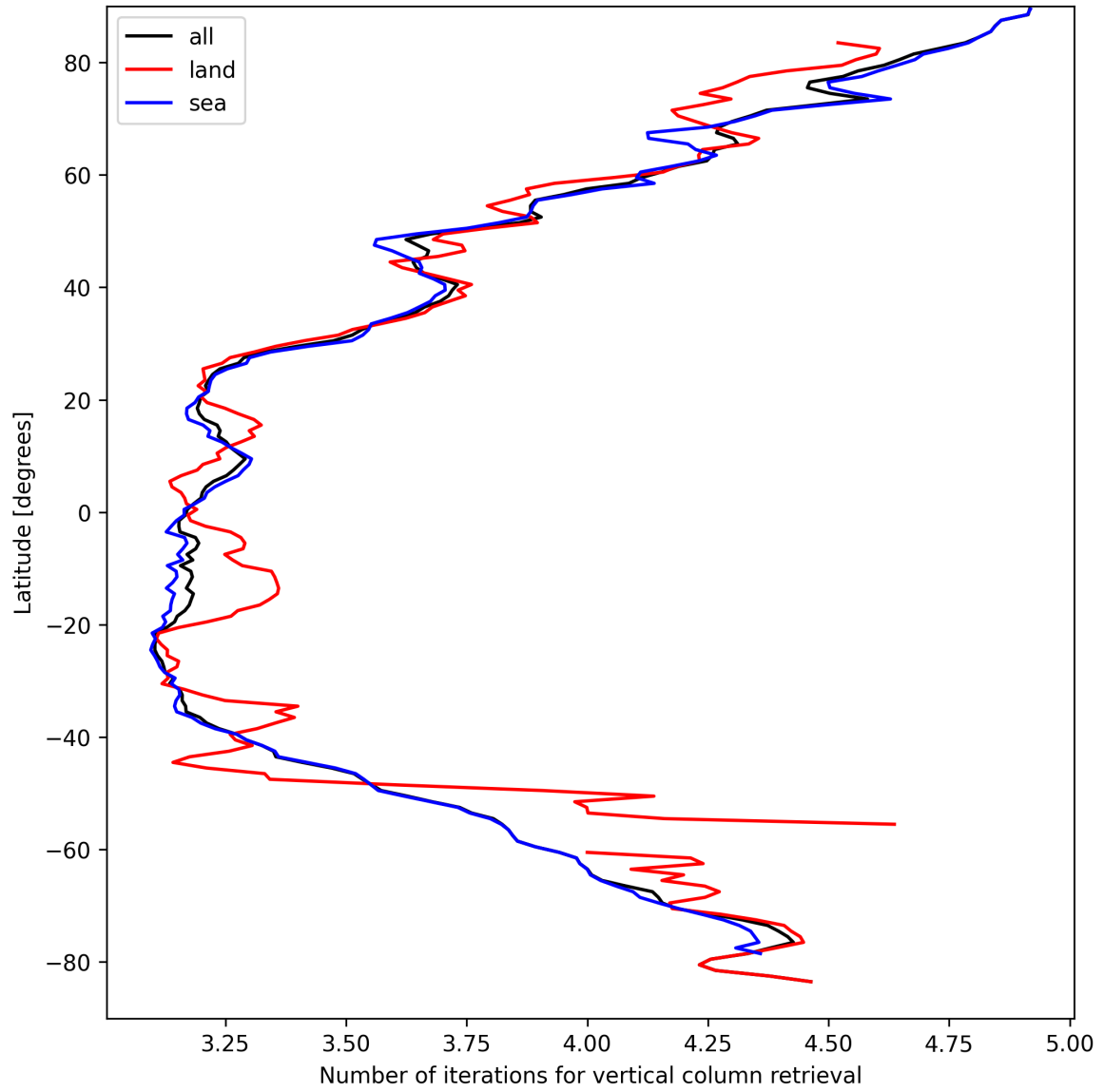
Figure 19: Zonal average of “Number of iterations for vertical column retrieval” for 2025-04-03 to 2025-04-04.
