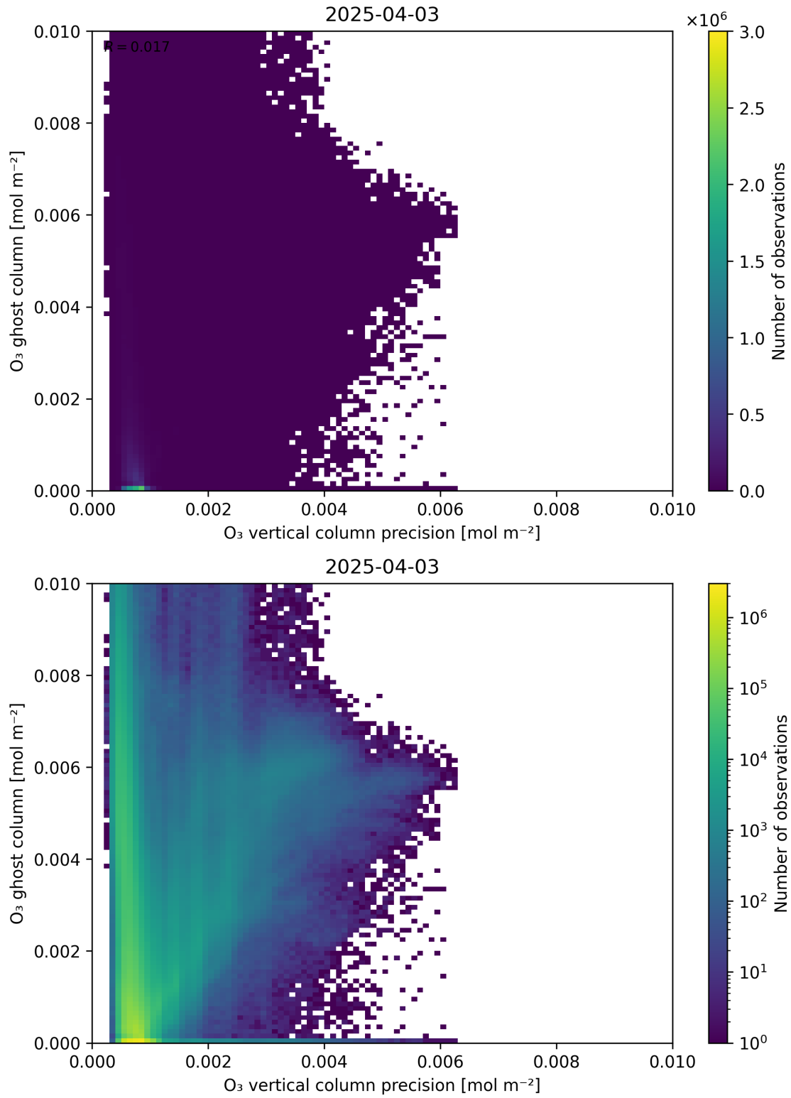
Figure 43: Scatter density plot of “O 3 vertical column precision” against “O 3 ghost column” for 2025-04-03 to 2025-04-04.
