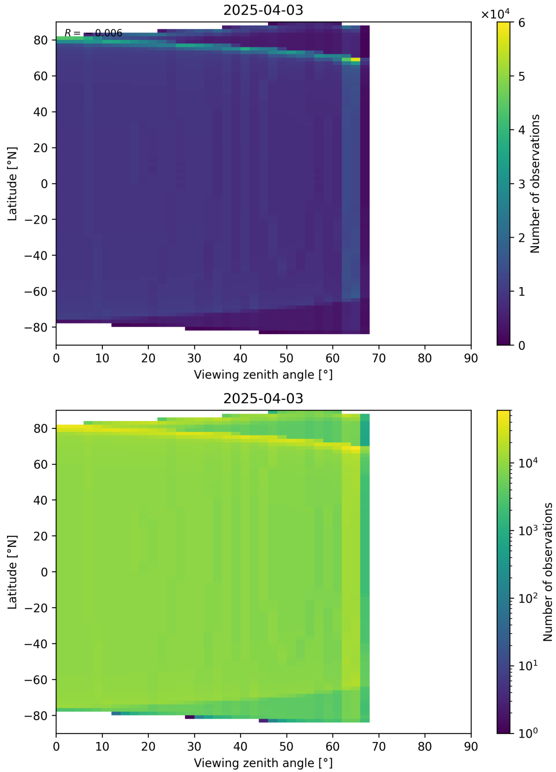
Figure 49: Scatter density plot of “Viewing zenith angle” against “Latitude” for 2025-04-03 to 2025-04-04.
