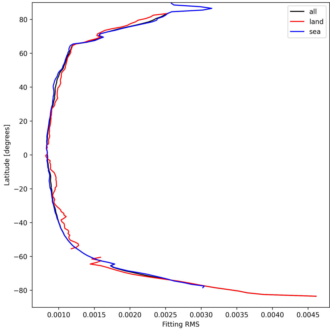
Figure 16: Zonal average of “Fitting RMS” for 2025-04-03 to 2025-04-04.
