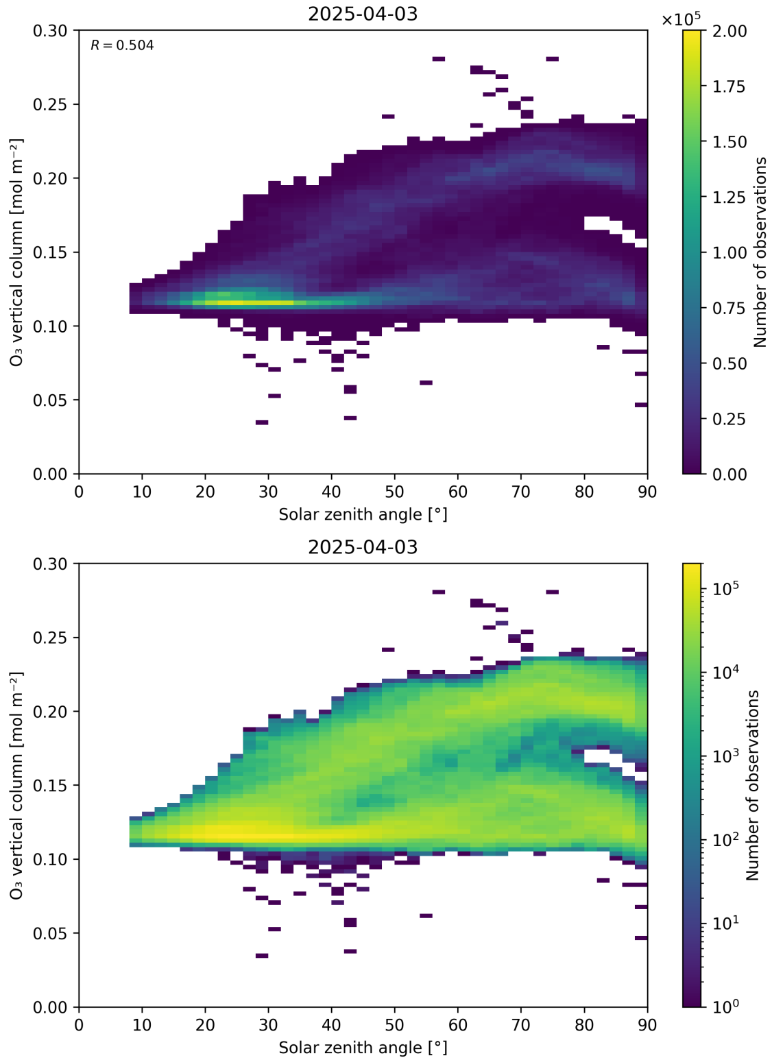
Figure 47: Scatter density plot of “Solar zenith angle” against “O 3 vertical column” for 2025-04-03 to 2025-04-04.
