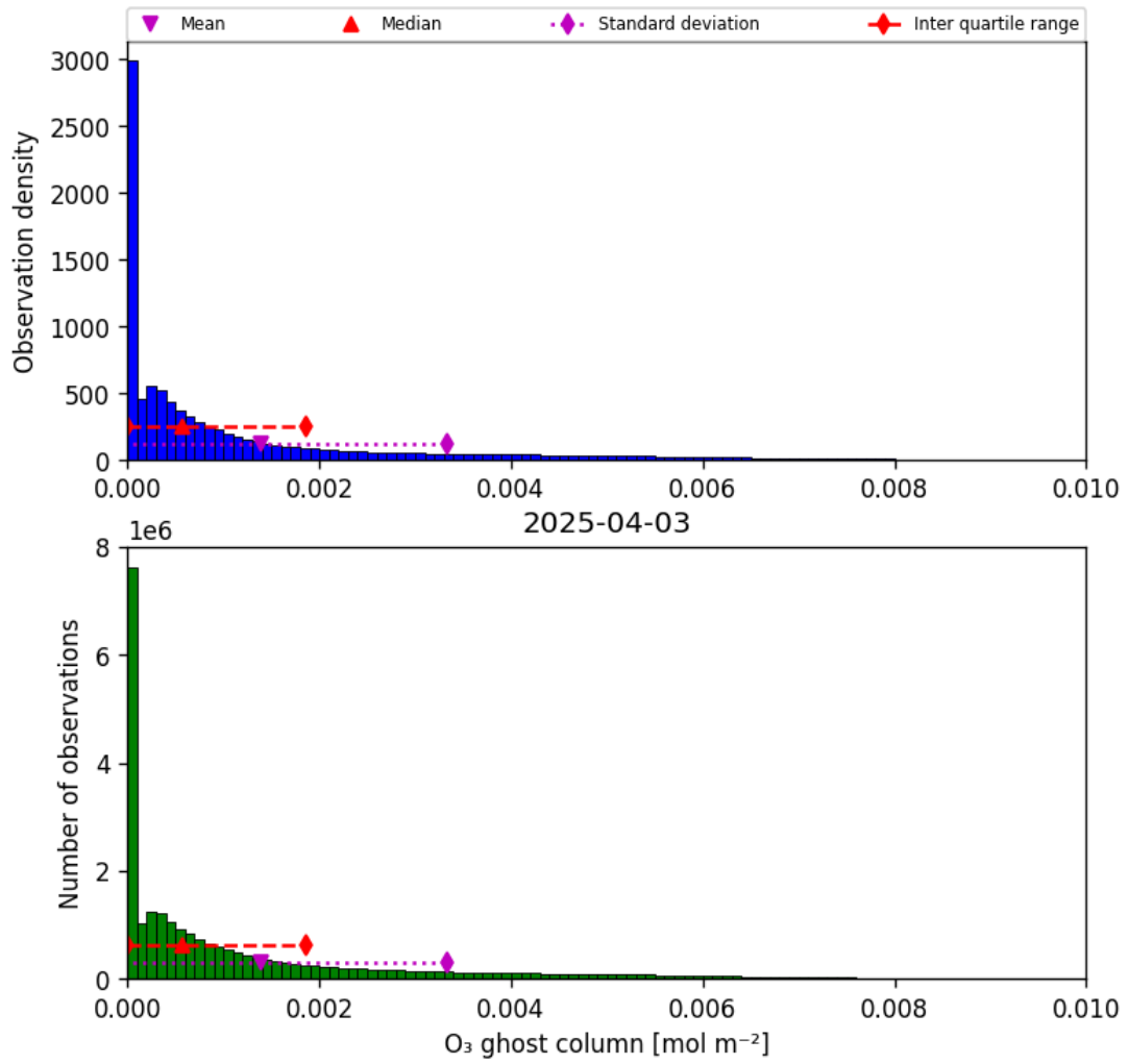
Figure 25: Histogram of “O 3 ghost column” for 2025-04-03 to 2025-04-04
