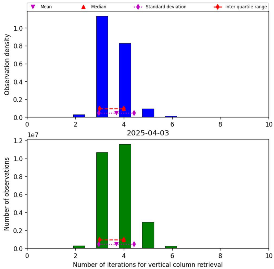
Figure 26: Histogram of “Number of iterations for vertical column retrieval” for 2025-04-03 to 2025-04-04
