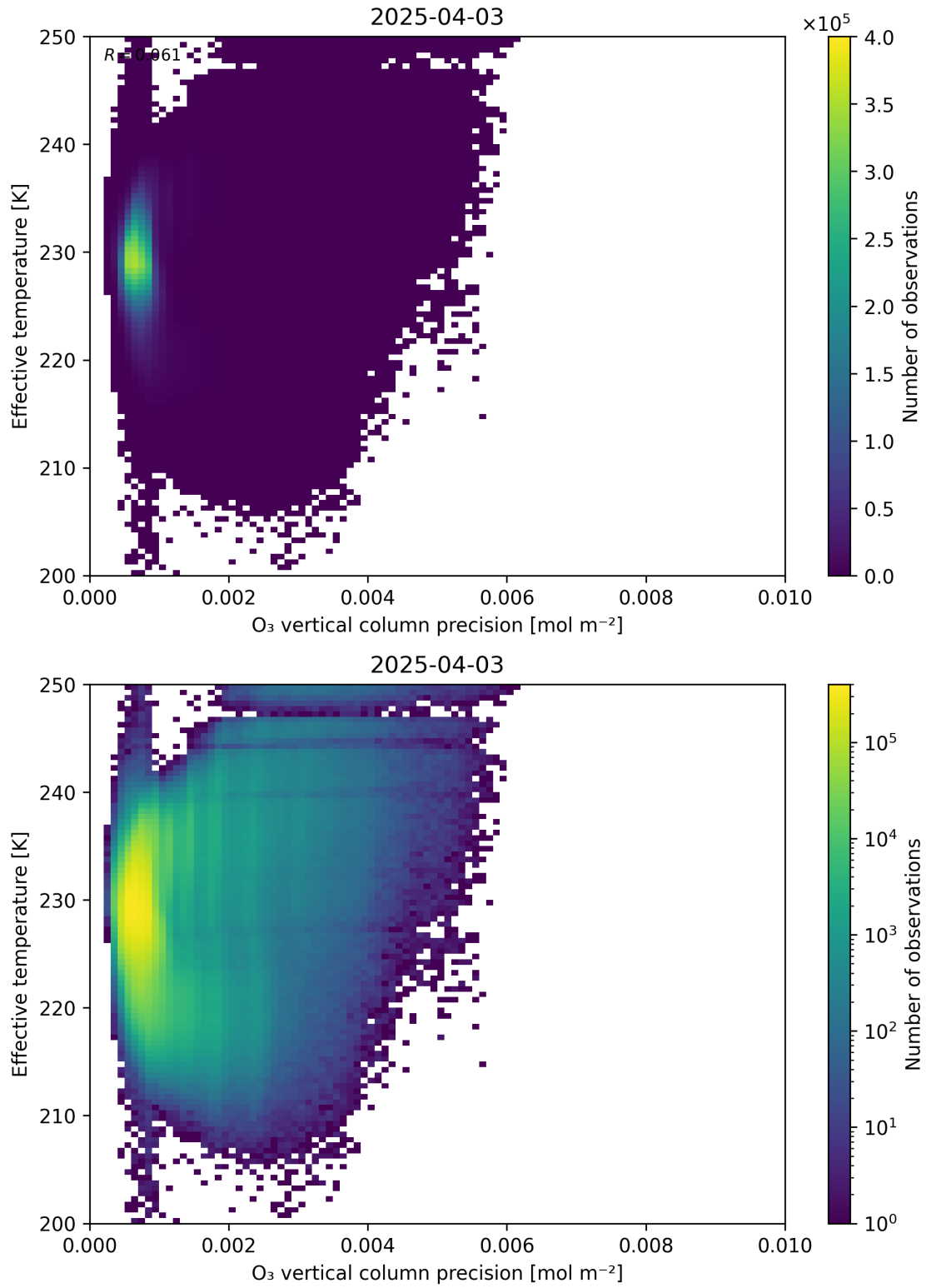
Figure 42: Scatter density plot of “O 3 vertical column precision” against “Effective temperature” for 2025-04-03 to 2025-04-04.
