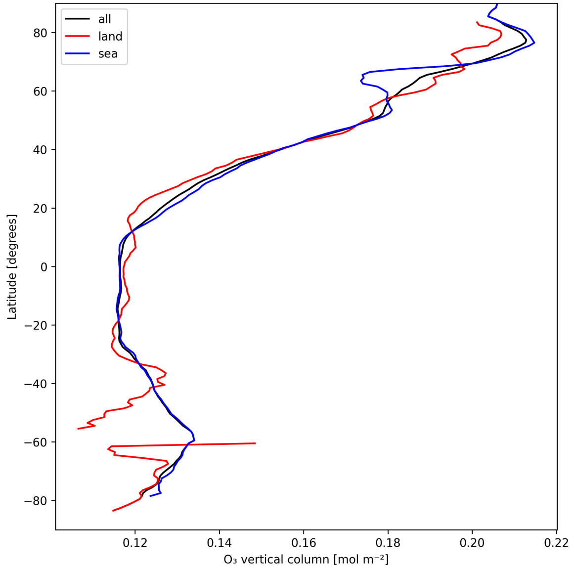
Figure 14: Zonal average of “O 3 vertical column” for 2025-04-03 to 2025-04-04.
