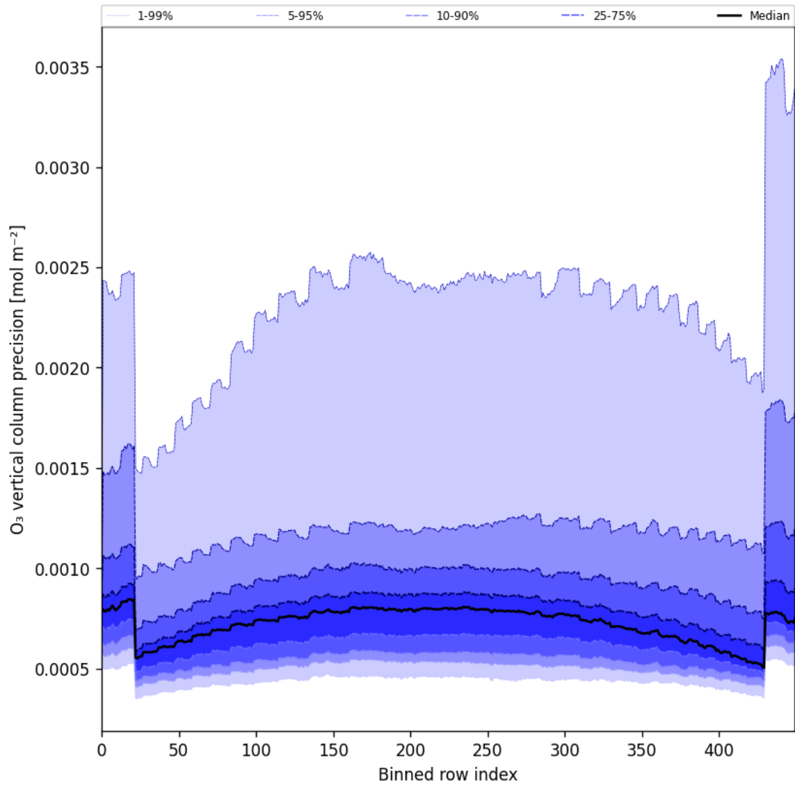
Figure 29: Along track statistics of “O 3 vertical column precision” for 2025-04-03 to 2025-04-04
