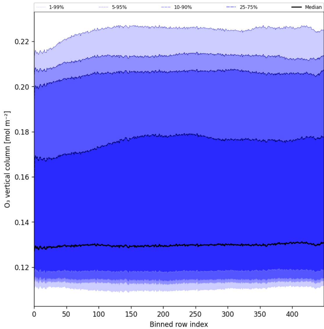
Figure 28: Along track statistics of “O 3 vertical column” for 2025-04-03 to 2025-04-04
