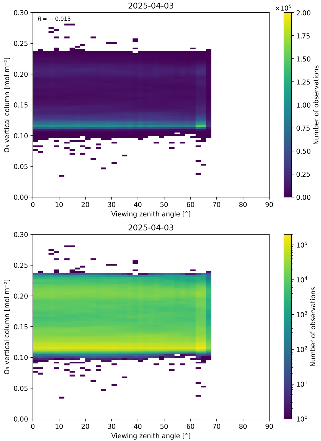
Figure 52: Scatter density plot of “Viewing zenith angle” against “O 3 vertical column” for 2025-04-03 to 2025-04-04.
