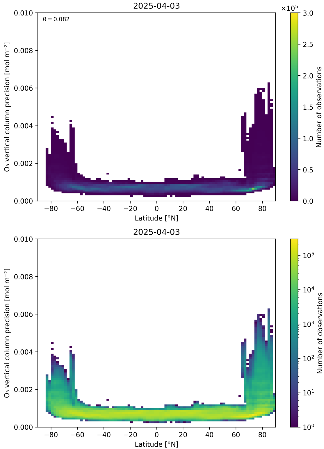
Figure 37: Scatter density plot of “Latitude” against “O 3 vertical column precision” for 2025-04-03 to 2025-04-04.
