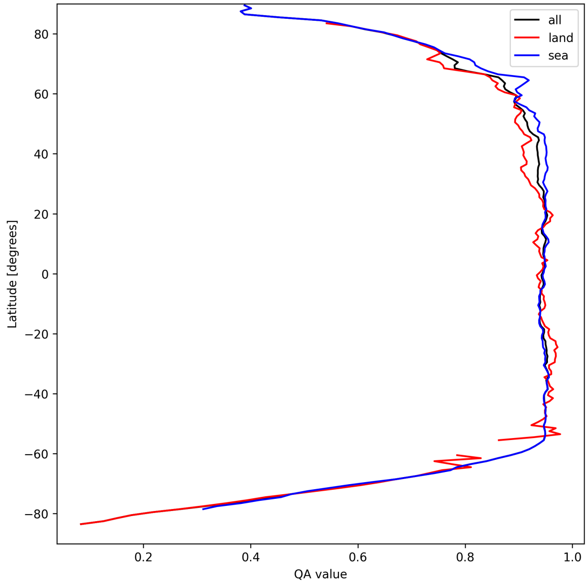
Figure 13: Zonal average of “QA value” for 2025-04-03 to 2025-04-04.
