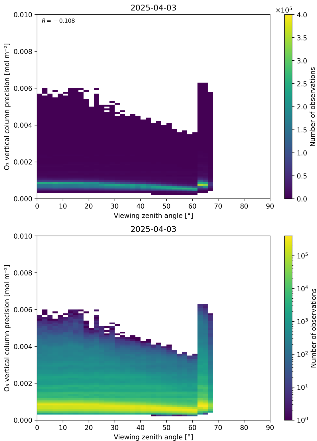
Figure 53: Scatter density plot of “Viewing zenith angle” against “O 3 vertical column precision” for 2025-04-03 to 2025-04-04.
