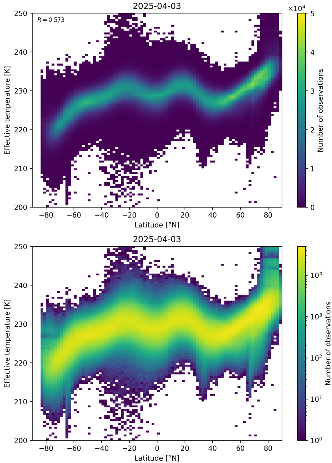
Figure 34: Scatter density plot of “Latitude” against “Effective temperature” for 2025-04-03 to 2025-04-04.
