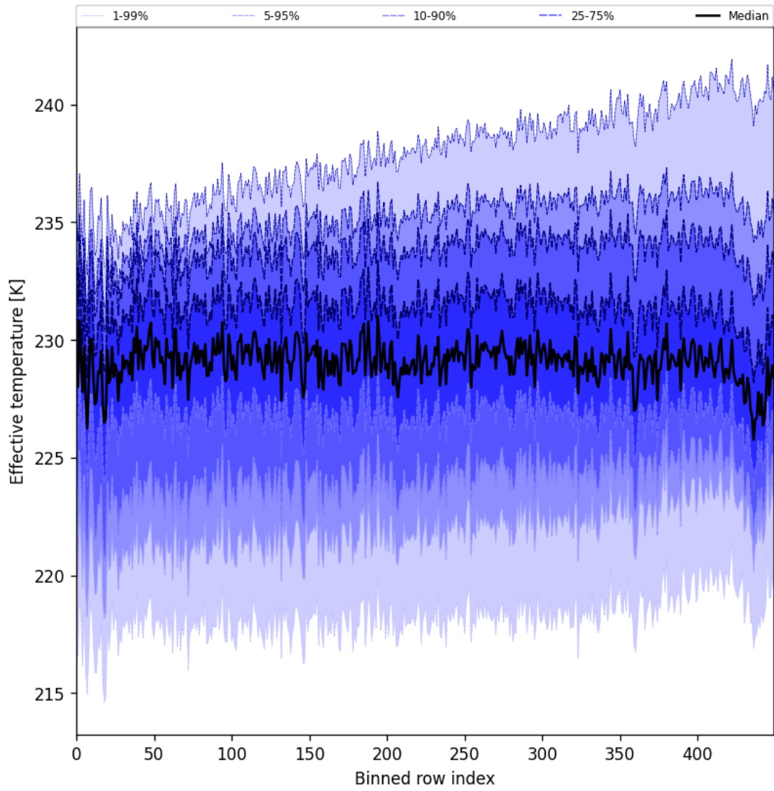
Figure 31: Along track statistics of “Effective temperature” for 2025-04-03 to 2025-04-04
