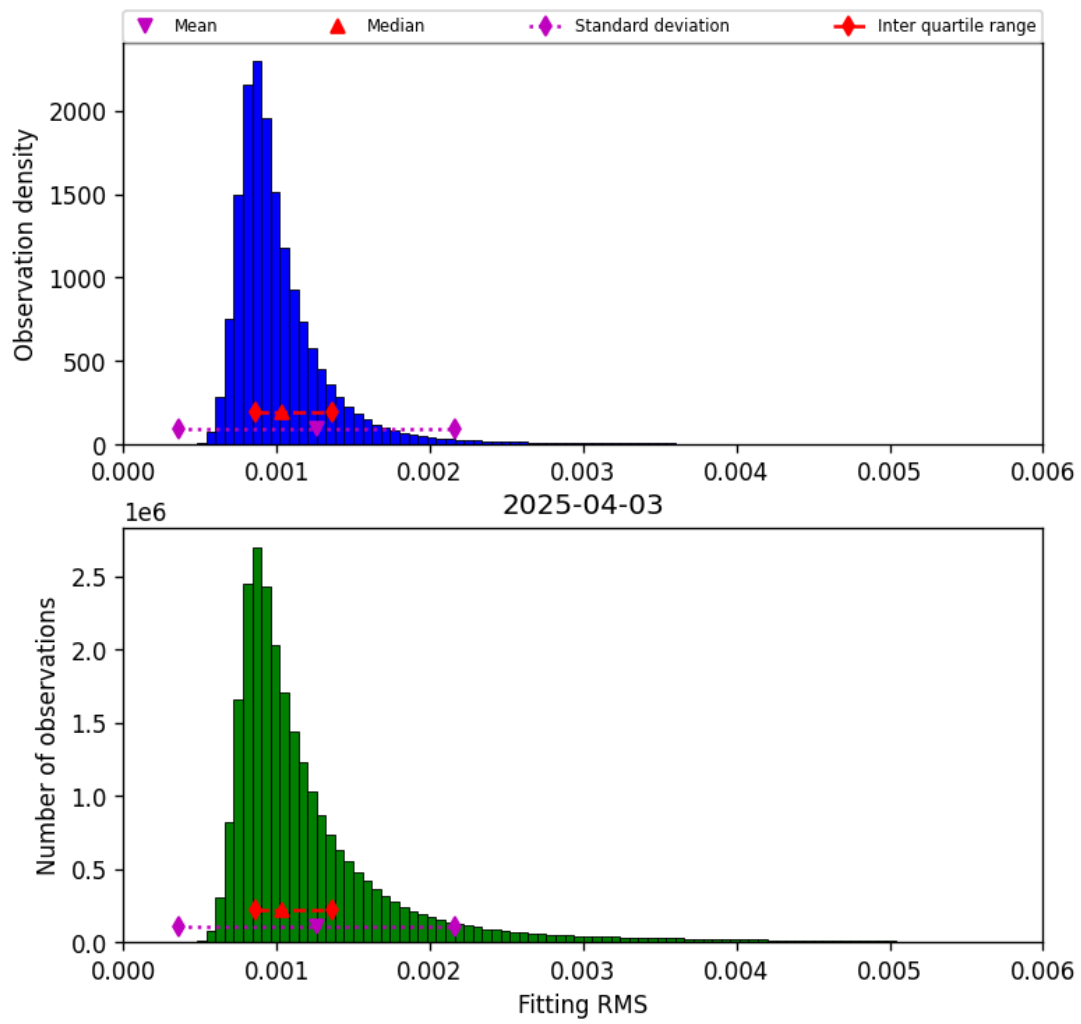
Figure 23: Histogram of “Fitting RMS” for 2025-04-03 to 2025-04-04
