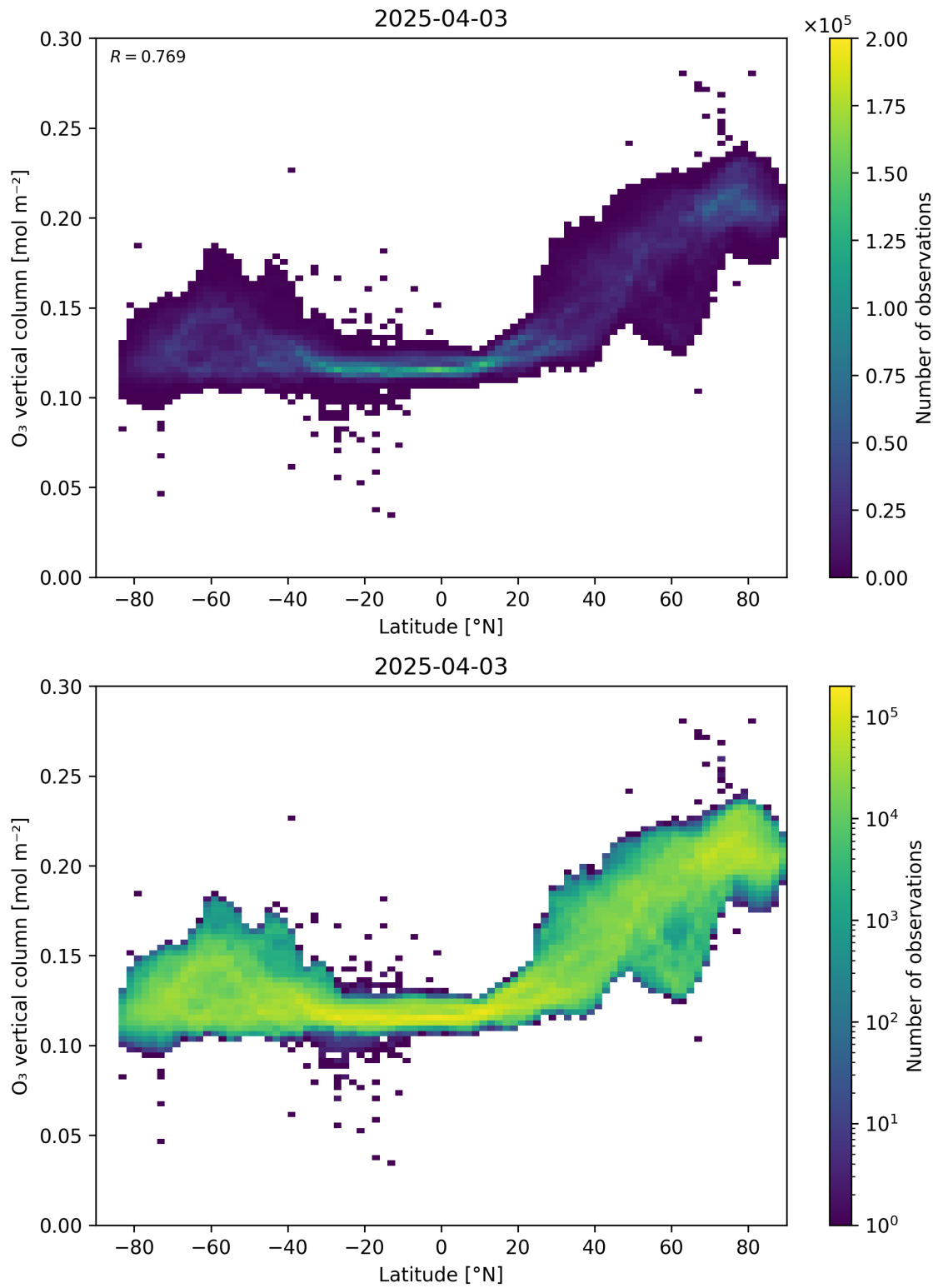
Figure 36: Scatter density plot of “Latitude” against “O 3 vertical column” for 2025-04-03 to 2025-04-04.
