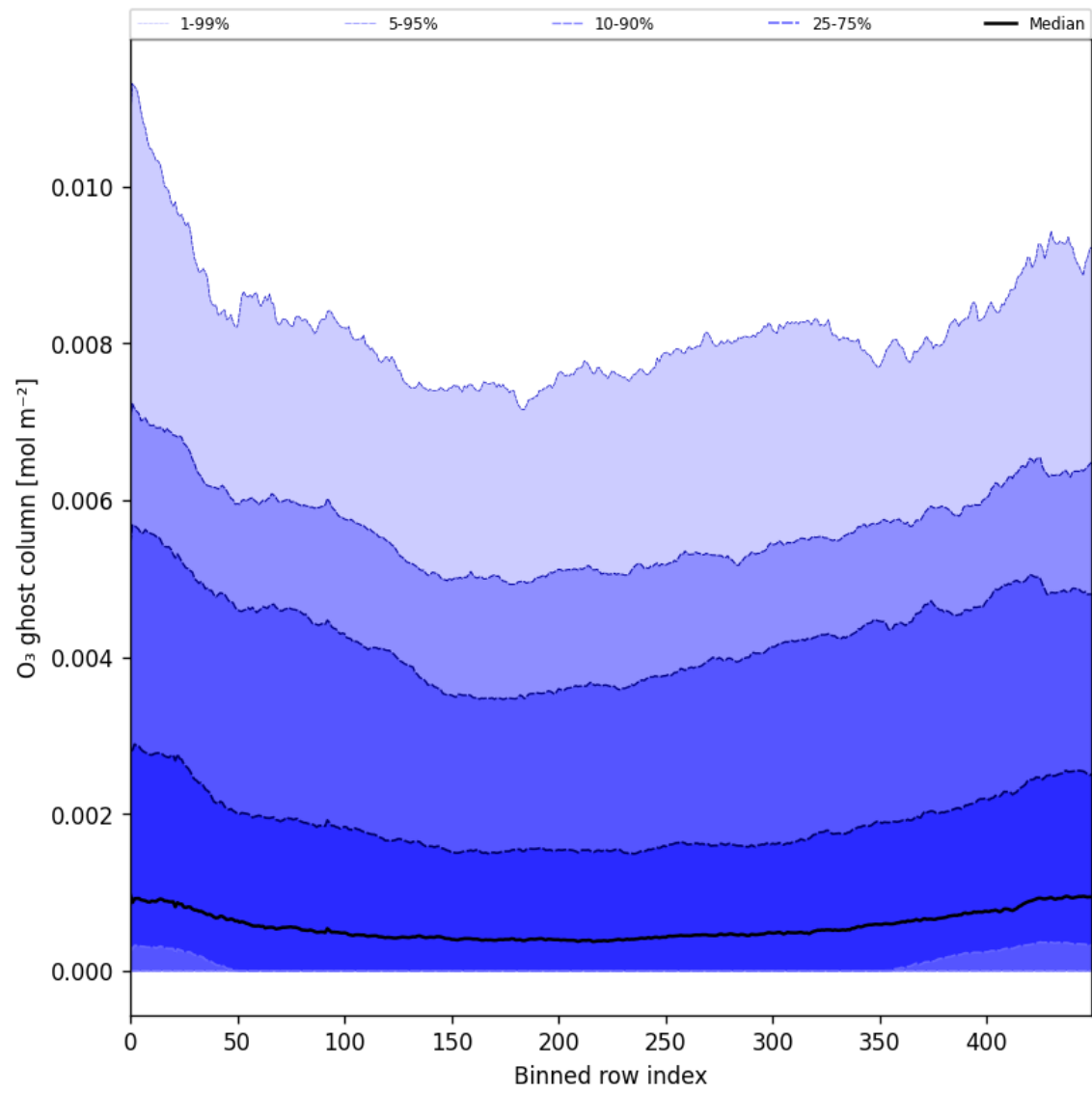
Figure 32: Along track statistics of “O 3 ghost column” for 2025-04-03 to 2025-04-04
