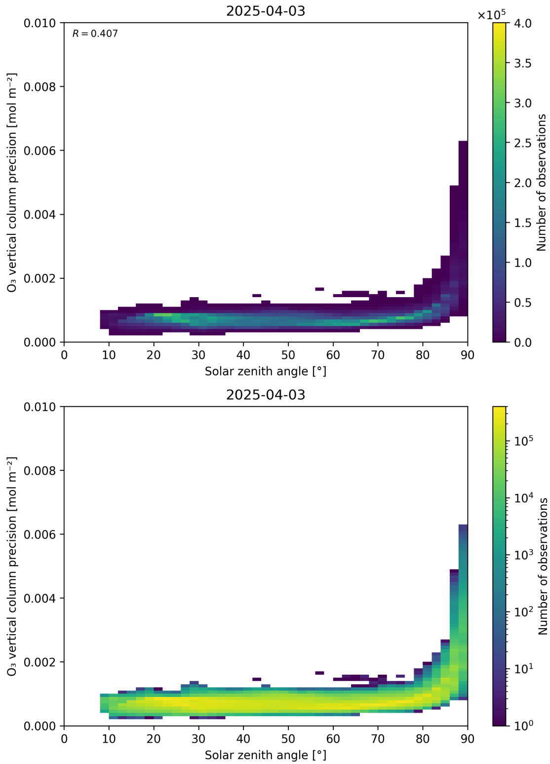
Figure 48: Scatter density plot of “Solar zenith angle” against “O 3 vertical column precision” for 2025-04-03 to 2025-04-04.
