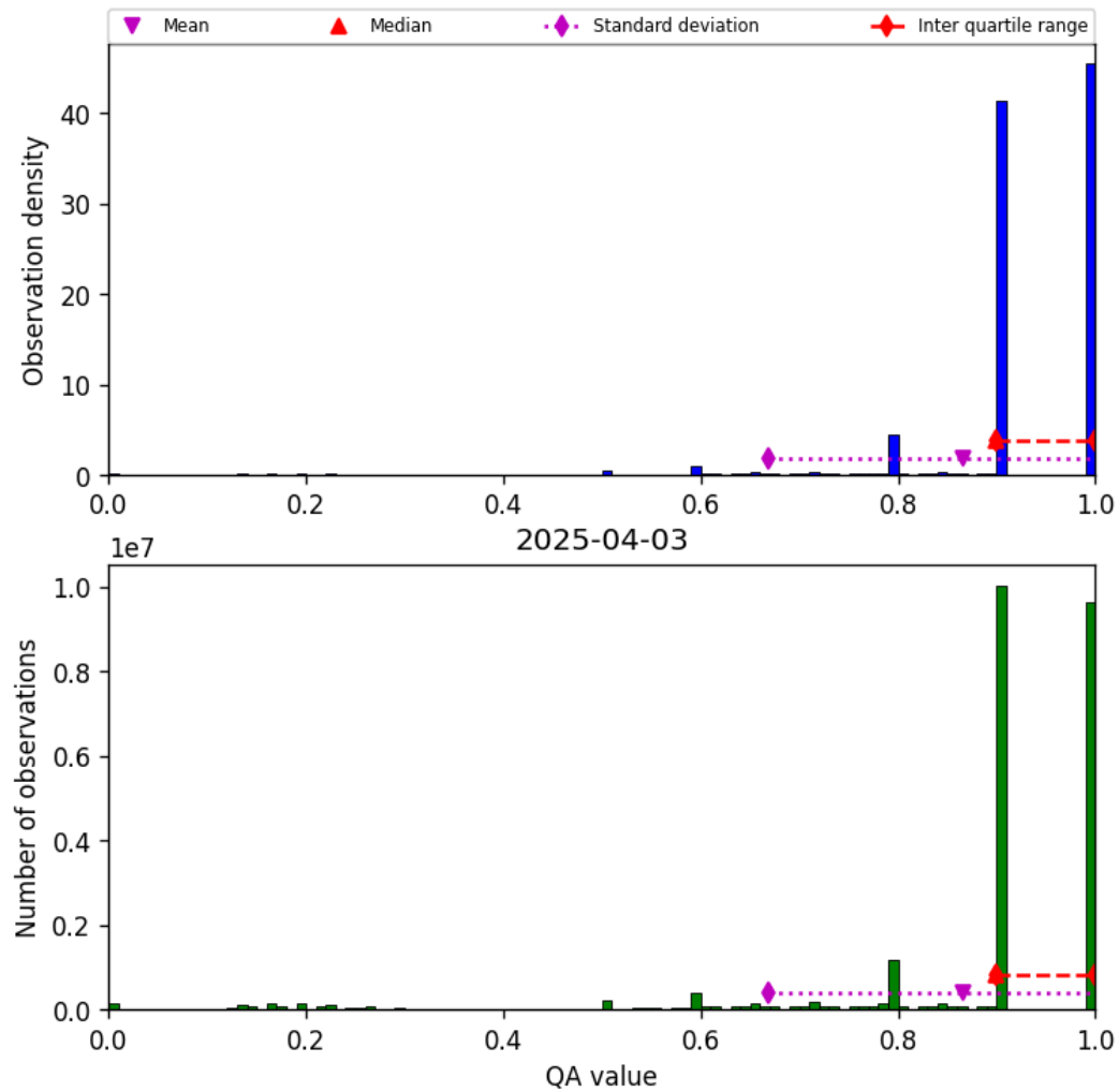
Figure 20: Histogram of “QA value” for 2025-04-03 to 2025-04-04
