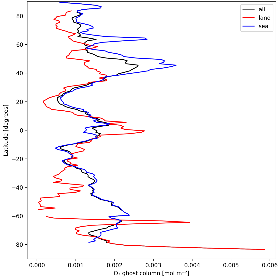
Figure 18: Zonal average of "O 3 ghost column" for 2025-04-03 to 2025-04-04.
