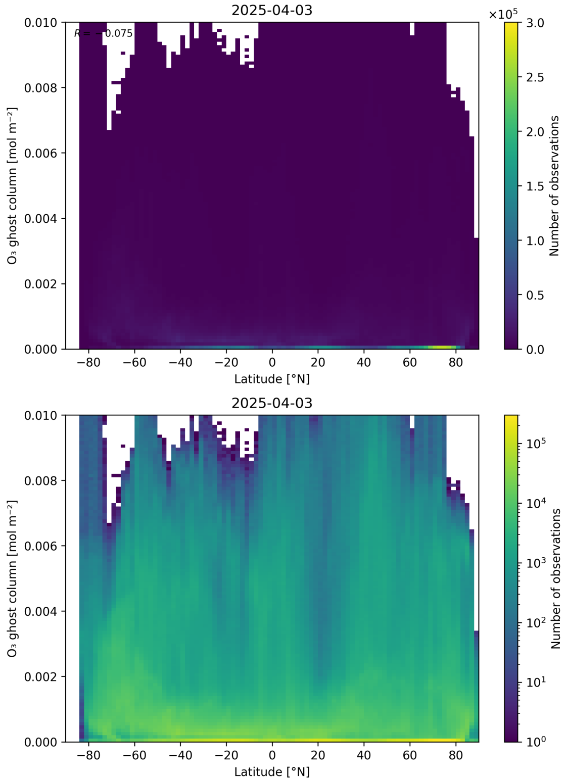
Figure 35: Scatter density plot of “Latitude” against “O 3 ghost column” for 2025-04-03 to 2025-04-04.
