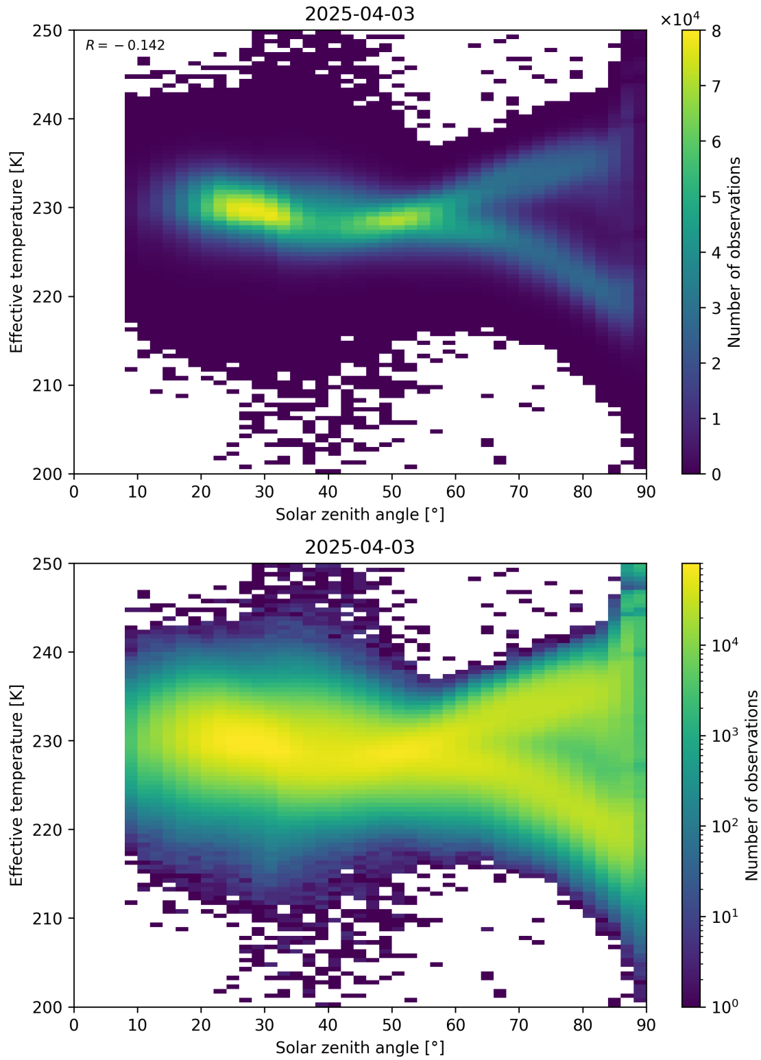
Figure 45: Scatter density plot of “Solar zenith angle” against “Effective temperature” for 2025-04-03 to 2025-04-04.
