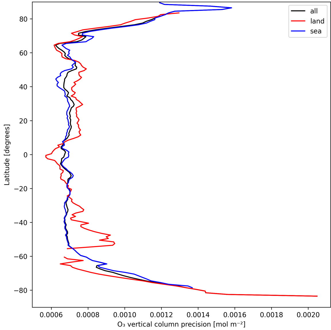
Figure 15: Zonal average of “O 3 vertical column precision” for 2025-04-03 to 2025-04-04.
