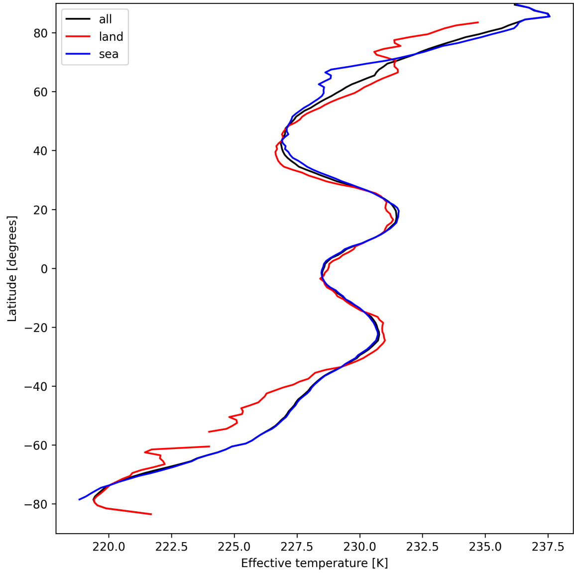
Figure 17: Zonal average of "Effective temperature" for 2025-04-03 to 2025-04-04.
