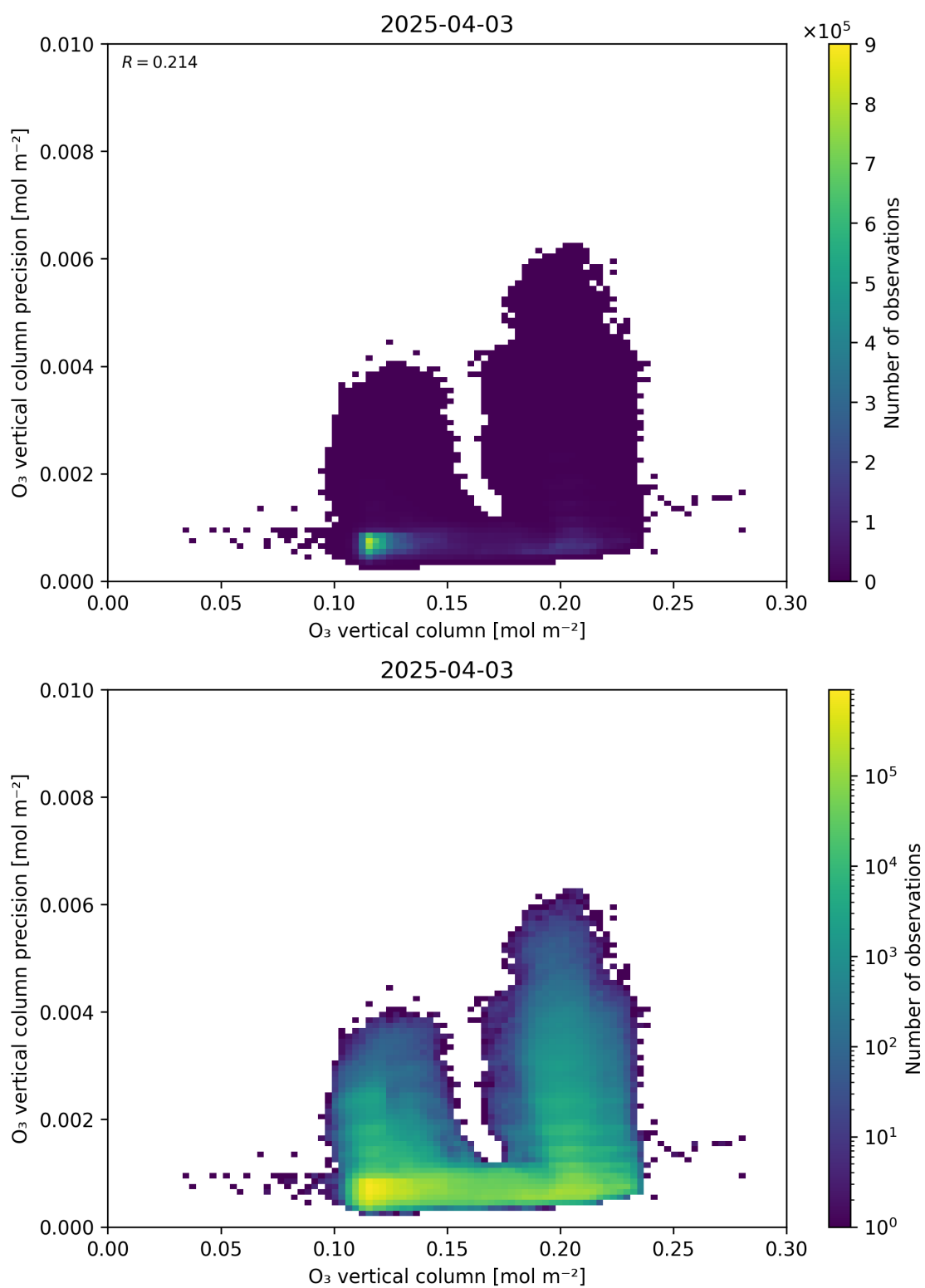
Figure 41: Scatter density plot of “O 3 vertical column” against “O 3 vertical column precision” for 2025-04-03 to 2025-04-04.
