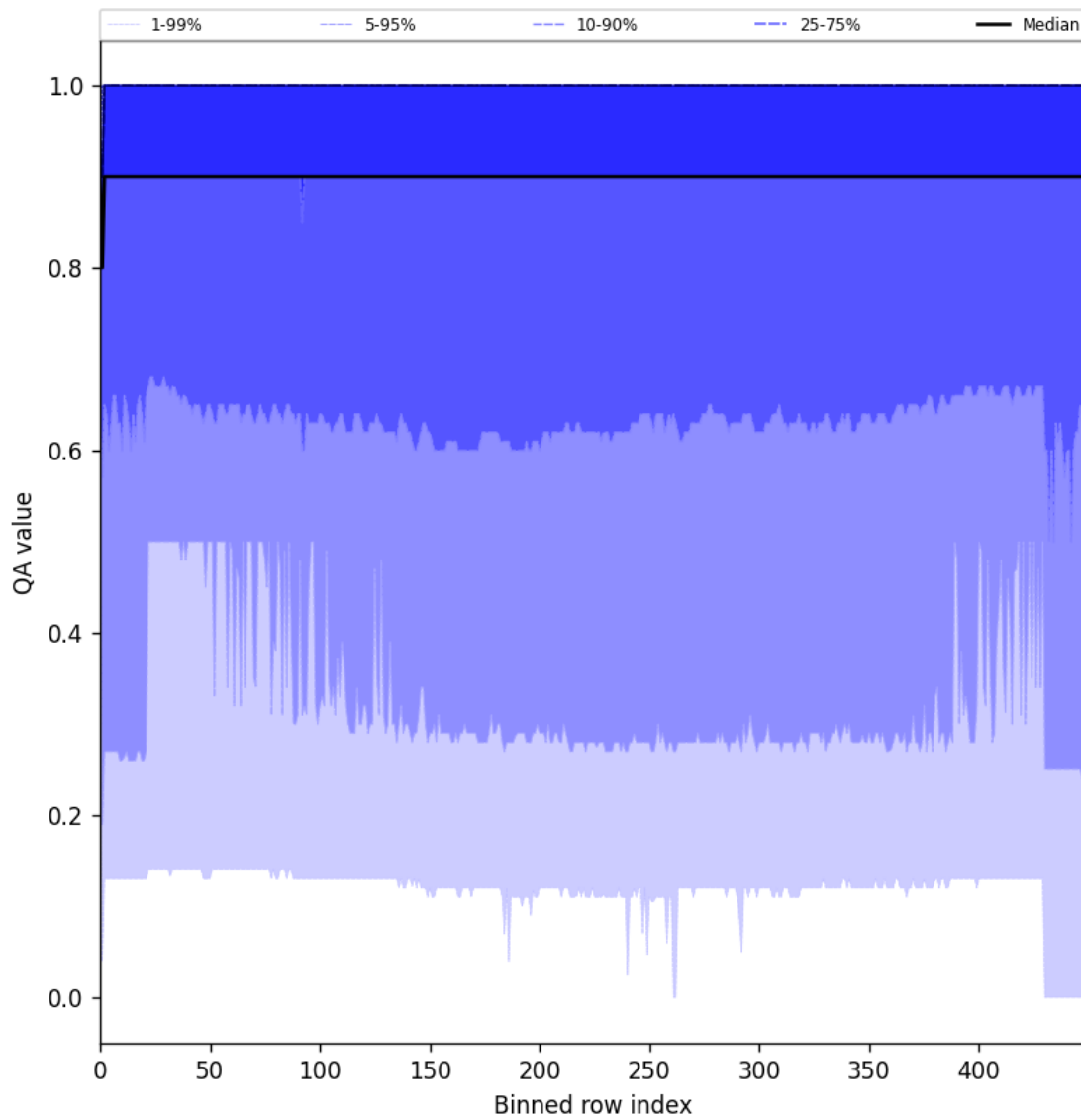
Figure 27: Along track statistics of “QA value” for 2025-04-03 to 2025-04-04
