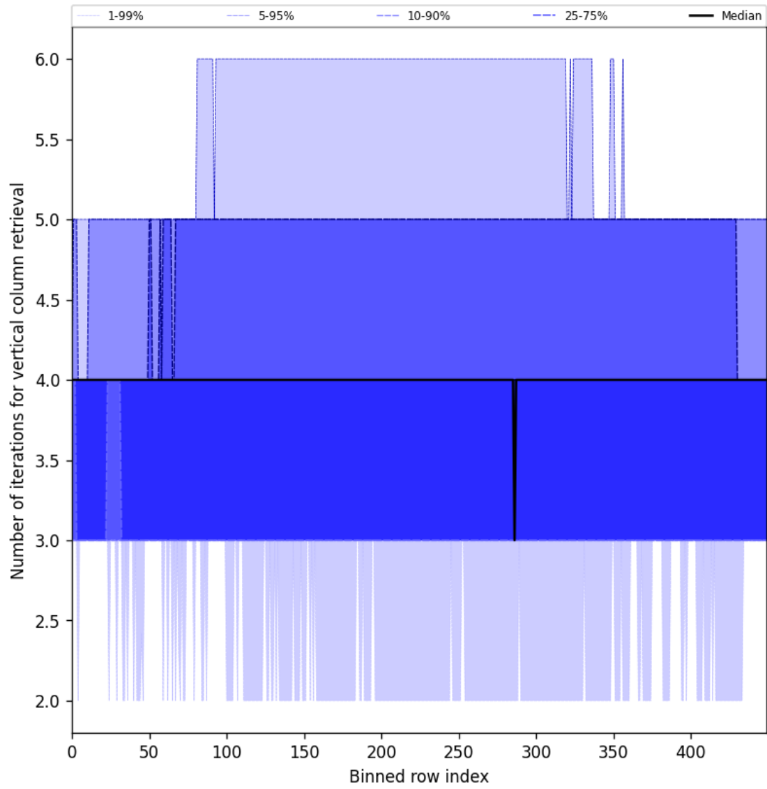
Figure 33: Along track statistics of “Number of iterations for vertical column retrieval” for 2025-04-03 to 2025-04-04
