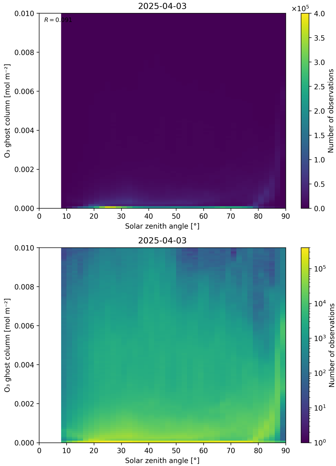
Figure 46: Scatter density plot of “Solar zenith angle” against “O 3 ghost column” for 2025-04-03 to 2025-04-04.
