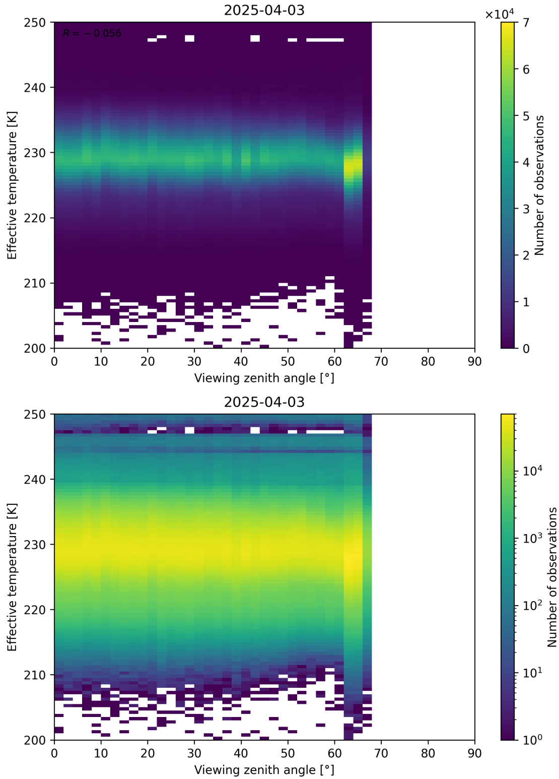
Figure 50: Scatter density plot of “Viewing zenith angle” against “Effective temperature” for 2025-04-03 to 2025-04-04.
