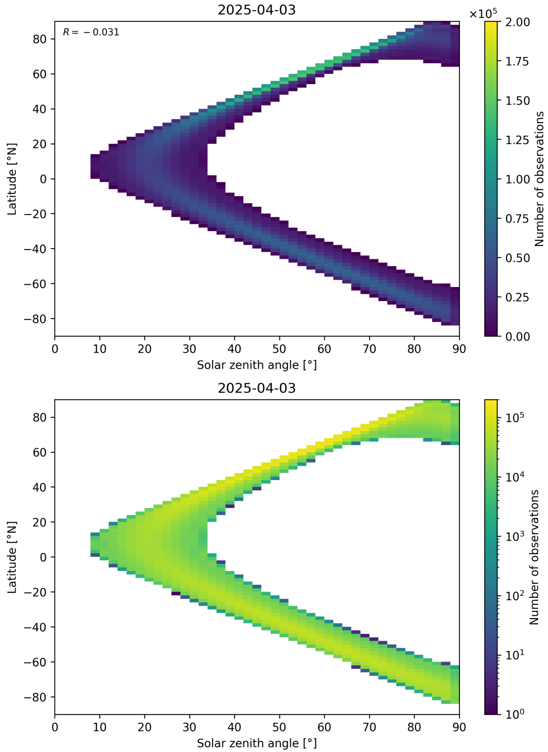
Figure 44: Scatter density plot of “Solar zenith angle” against “Latitude” for 2025-04-03 to 2025-04-04.
