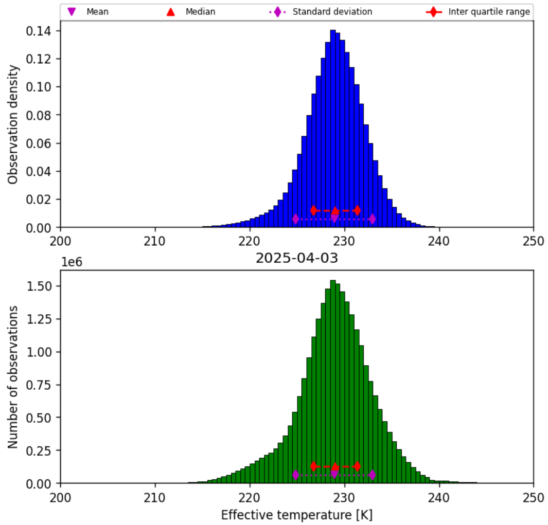
Figure 24: Histogram of “Effective temperature” for 2025-04-03 to 2025-04-04
