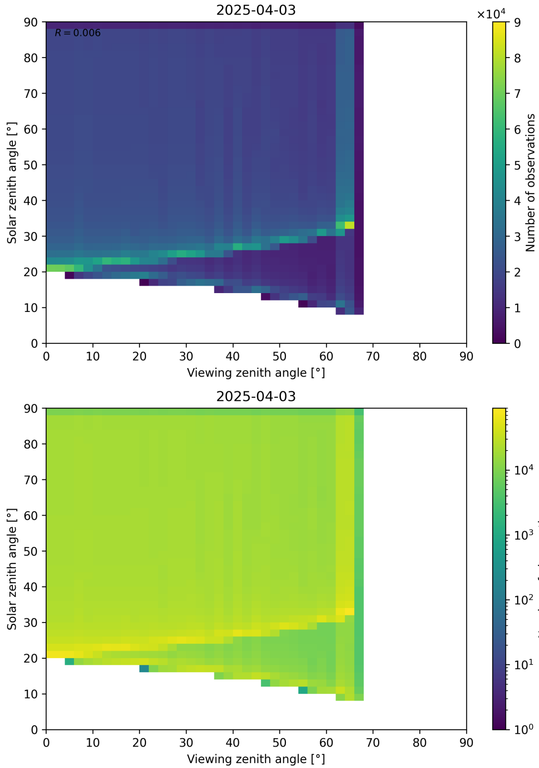
Figure 54: Scatter density plot of “Viewing zenith angle” against “Solar zenith angle” for 2025-04-03 to 2025-04-04.
