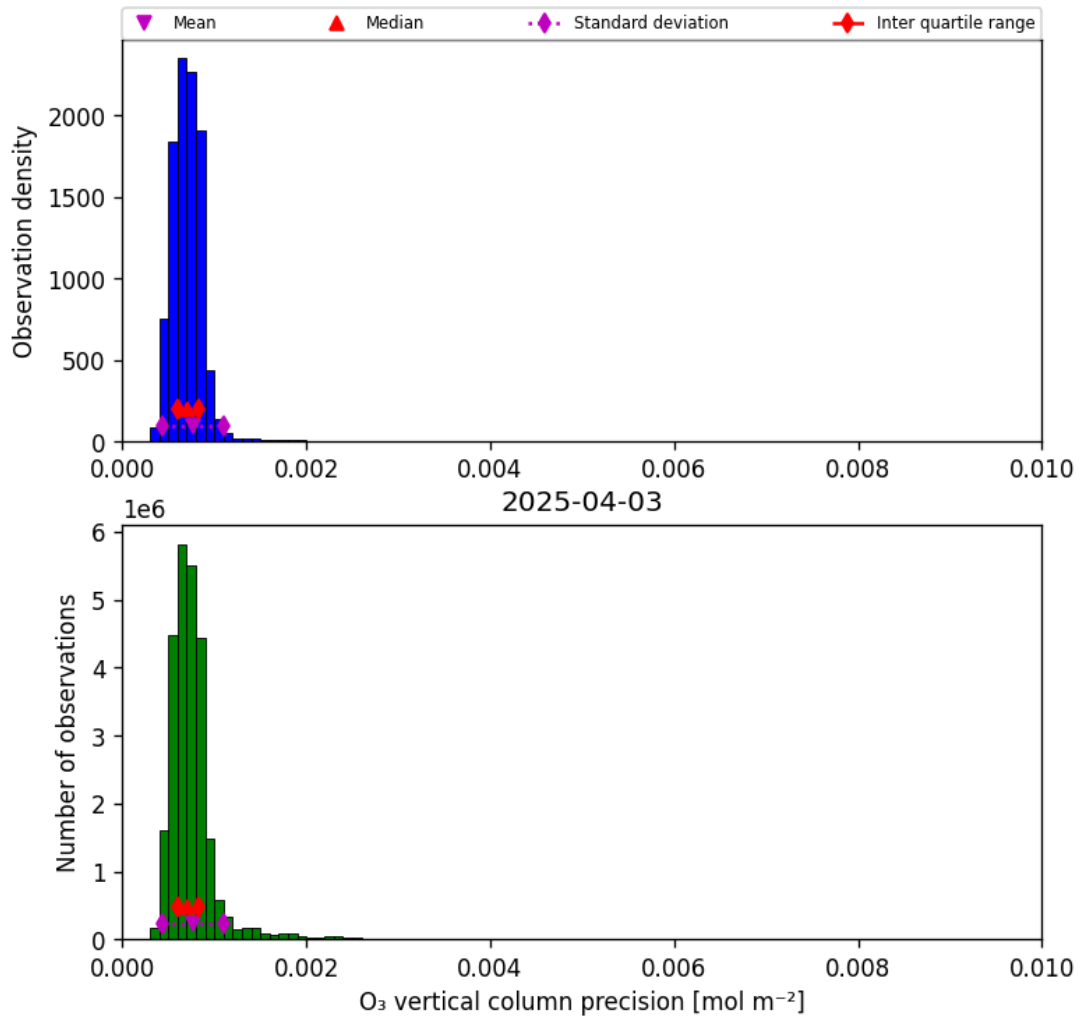
Figure 22: Histogram of “O 3 vertical column precision” for 2025-04-03 to 2025-04-04
